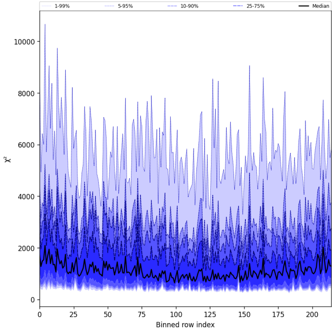
Figure 24: Along track statistics of “ \chi^2 ” for 2025-11-02 to 2025-11-03
