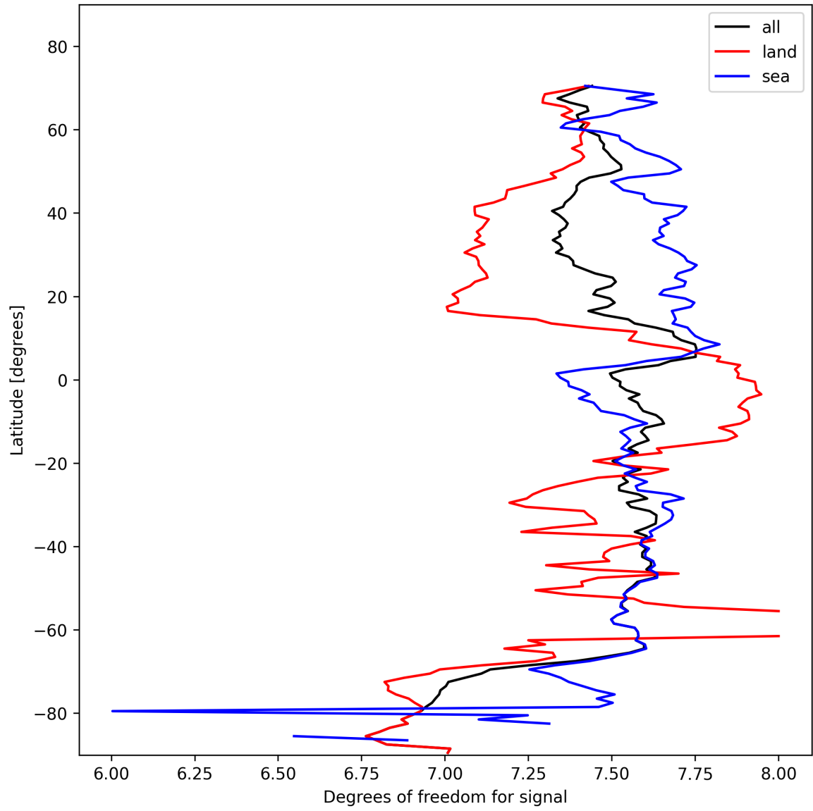
Figure 11: Zonal average of “Degrees of freedom for signal” for 2025-11-02 to 2025-11-03.
