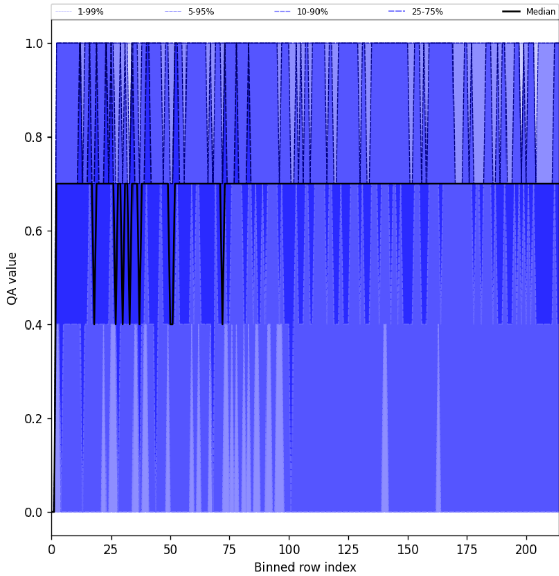
Figure 20: Along track statistics of “QA value” for 2025-11-02 to 2025-11-03
