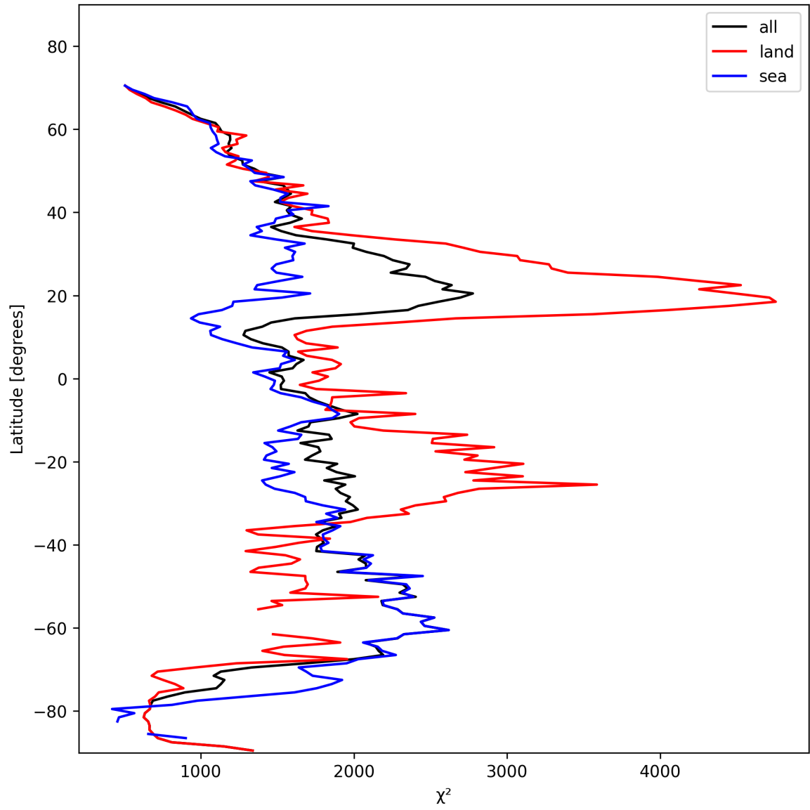
Figure 10: Zonal average of “ \chi^2 ” for 2025-11-02 to 2025-11-03.
