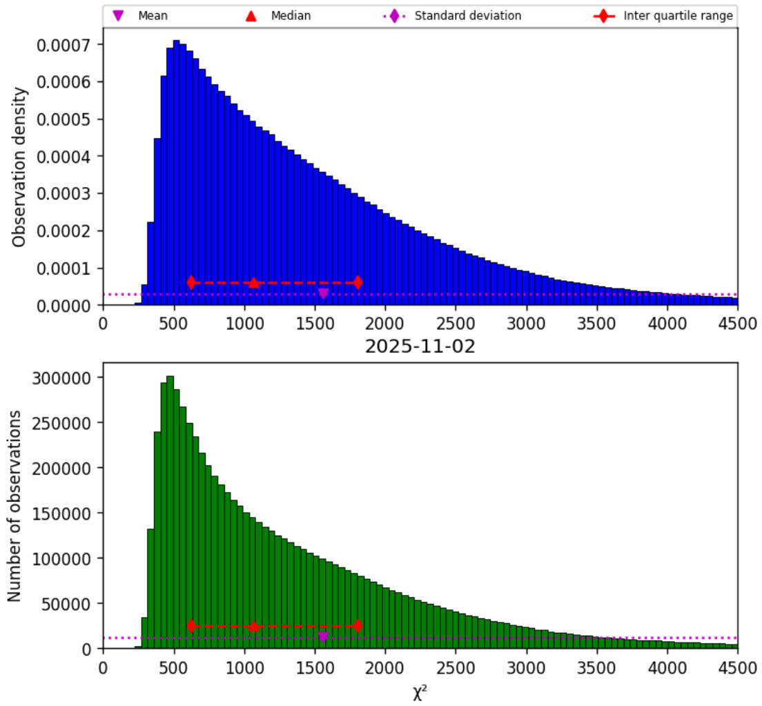
Figure 17: Histogram of “ \chi^2 ” for 2025-11-02 to 2025-11-03
