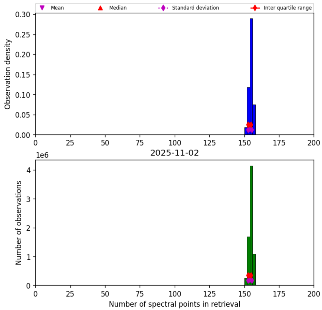
Figure 16: Histogram of “Number of spectral points in retrieval” for 2025-11-02 to 2025-11-03
