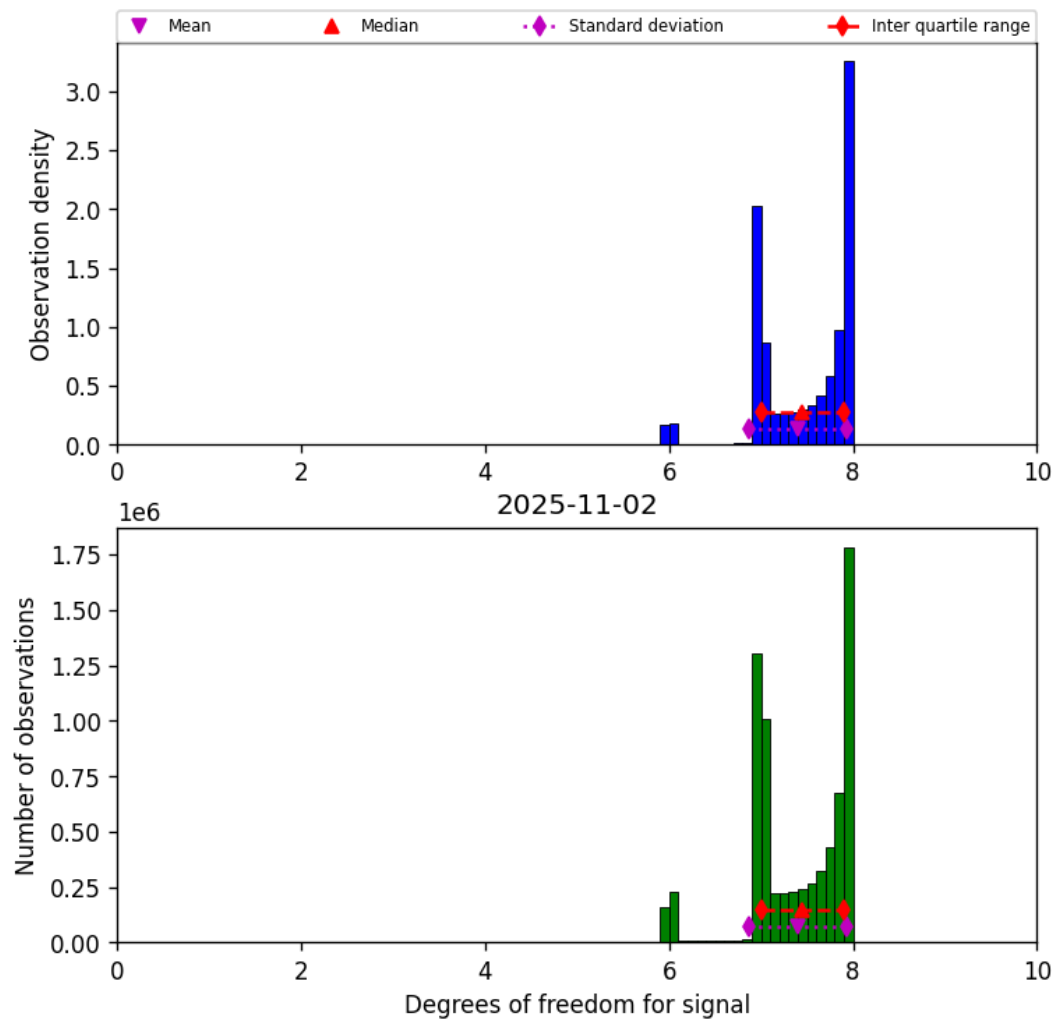
Figure 18: Histogram of “Degrees of freedom for signal” for 2025-11-02 to 2025-11-03
