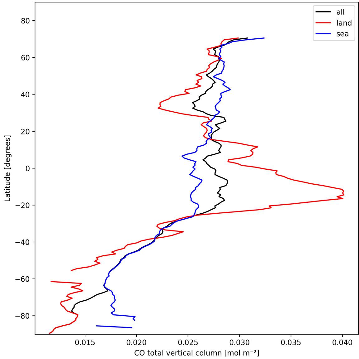
Figure 7: Zonal average of “CO total vertical column” for 2025-11-02 to 2025-11-03.
