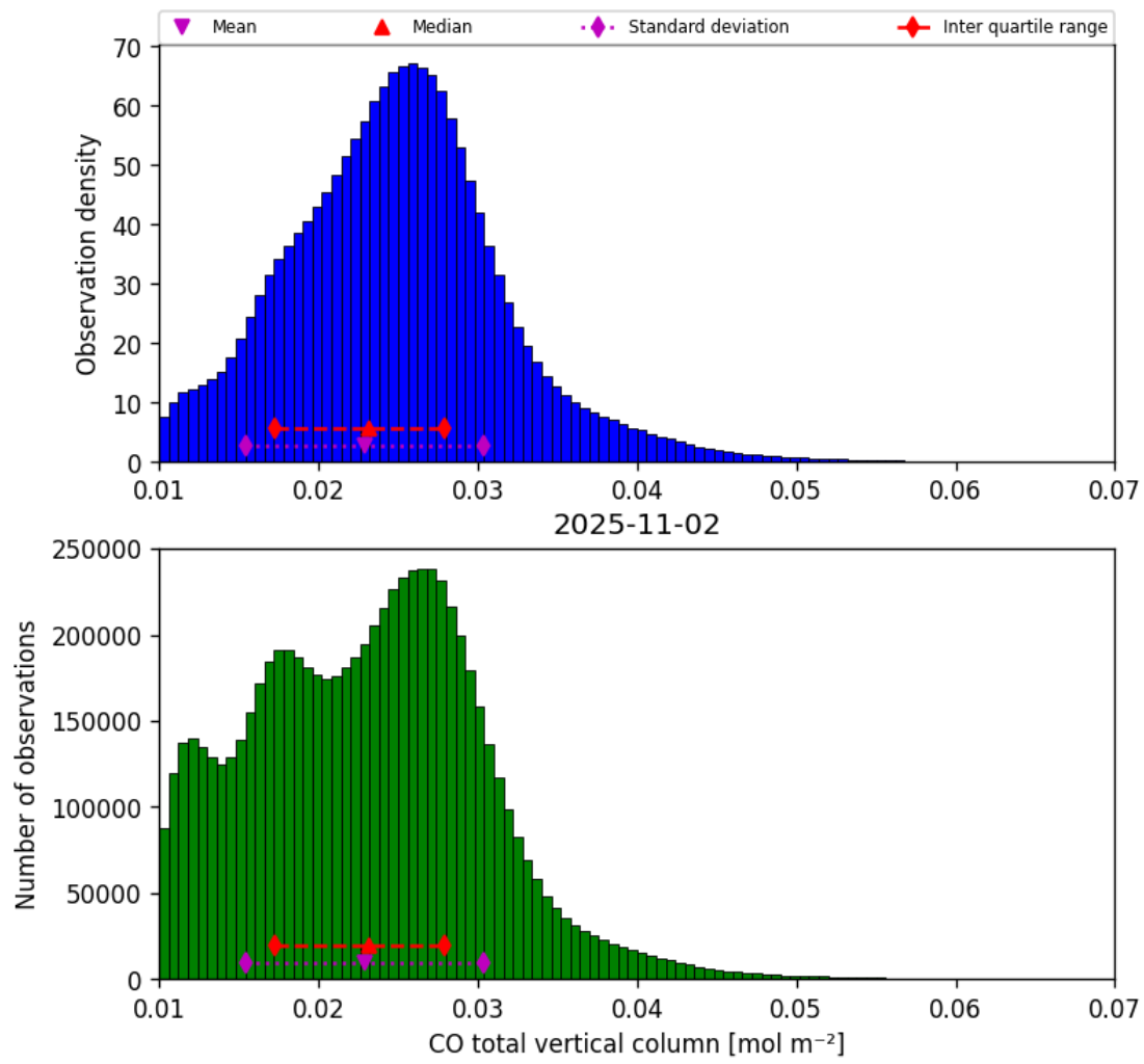
Figure 14: Histogram of “CO total vertical column” for 2025-11-02 to 2025-11-03
