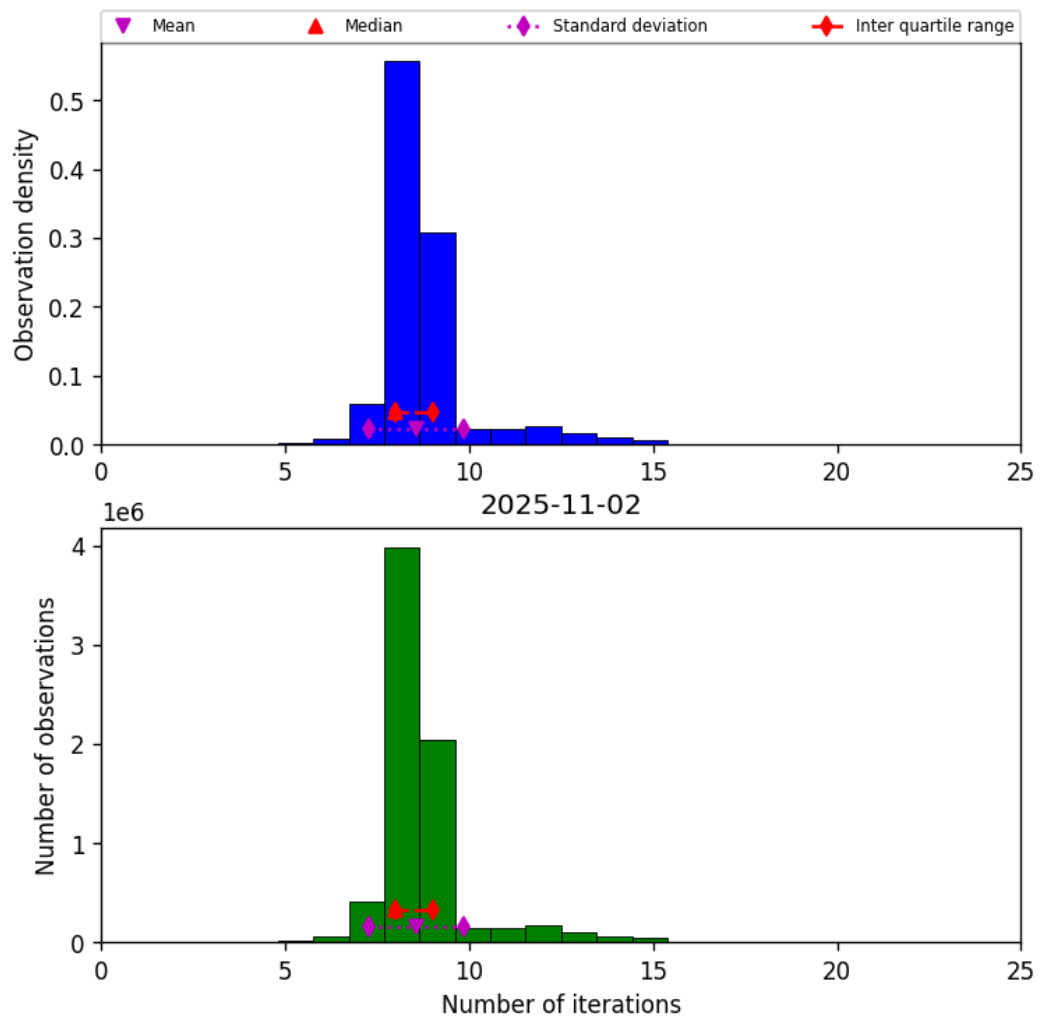
Figure 19: Histogram of “Number of iterations” for 2025-11-02 to 2025-11-03
