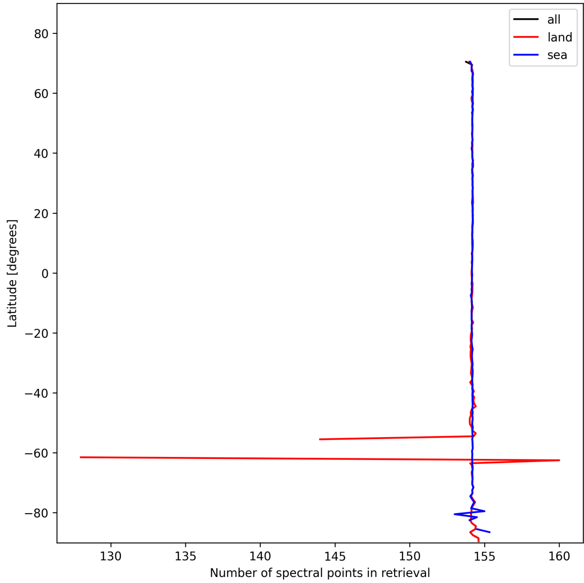
Figure 9: Zonal average of “Number of spectral points in retrieval” for 2025-11-02 to 2025-11-03.
