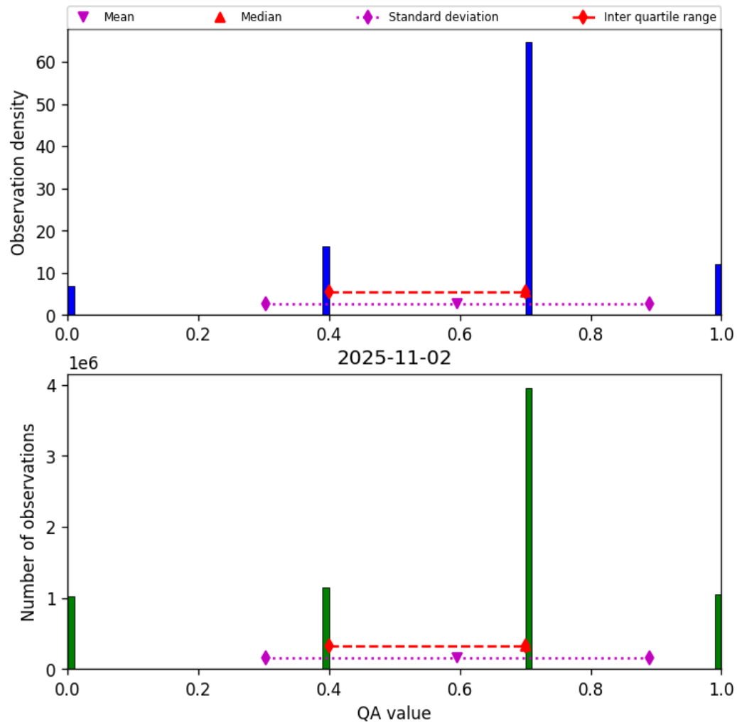
Figure 13: Histogram of “QA value” for 2025-11-02 to 2025-11-03
