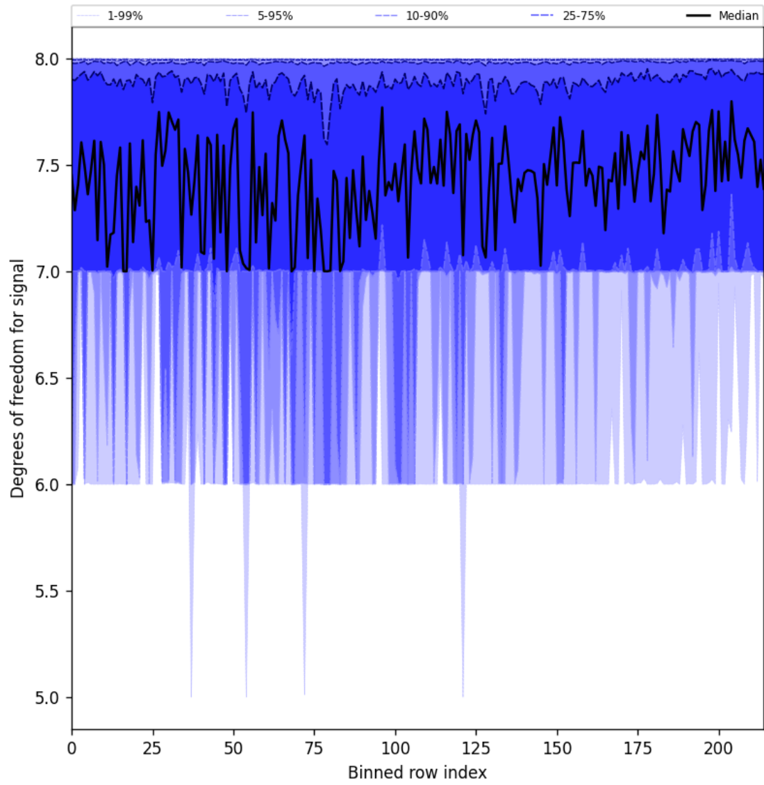
Figure 25: Along track statistics of “Degrees of freedom for signal” for 2025-11-02 to 2025-11-03
