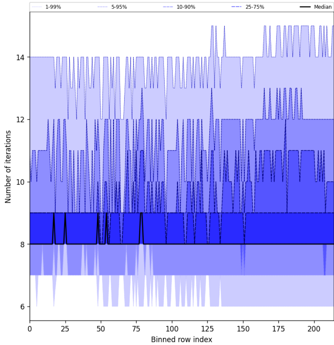
Figure 26: Along track statistics of “Number of iterations” for 2025-11-02 to 2025-11-03
