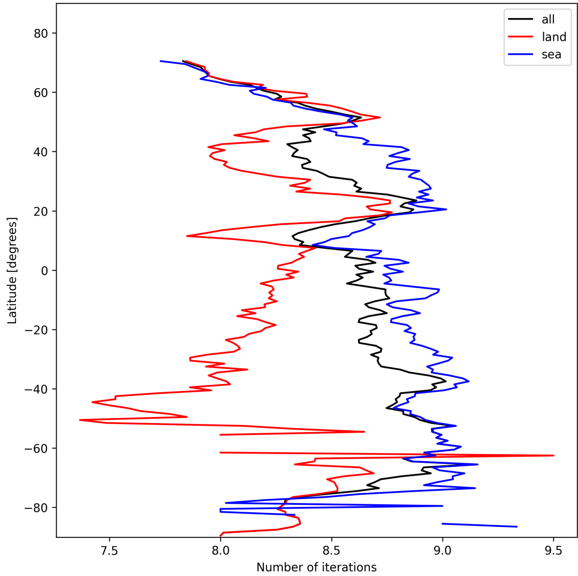
Figure 12: Zonal average of “Number of iterations” for 2025-11-02 to 2025-11-03.
