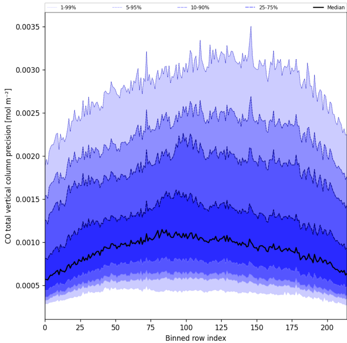
Figure 22: Along track statistics of “CO total vertical column precision” for 2025-11-02 to 2025-11-03
