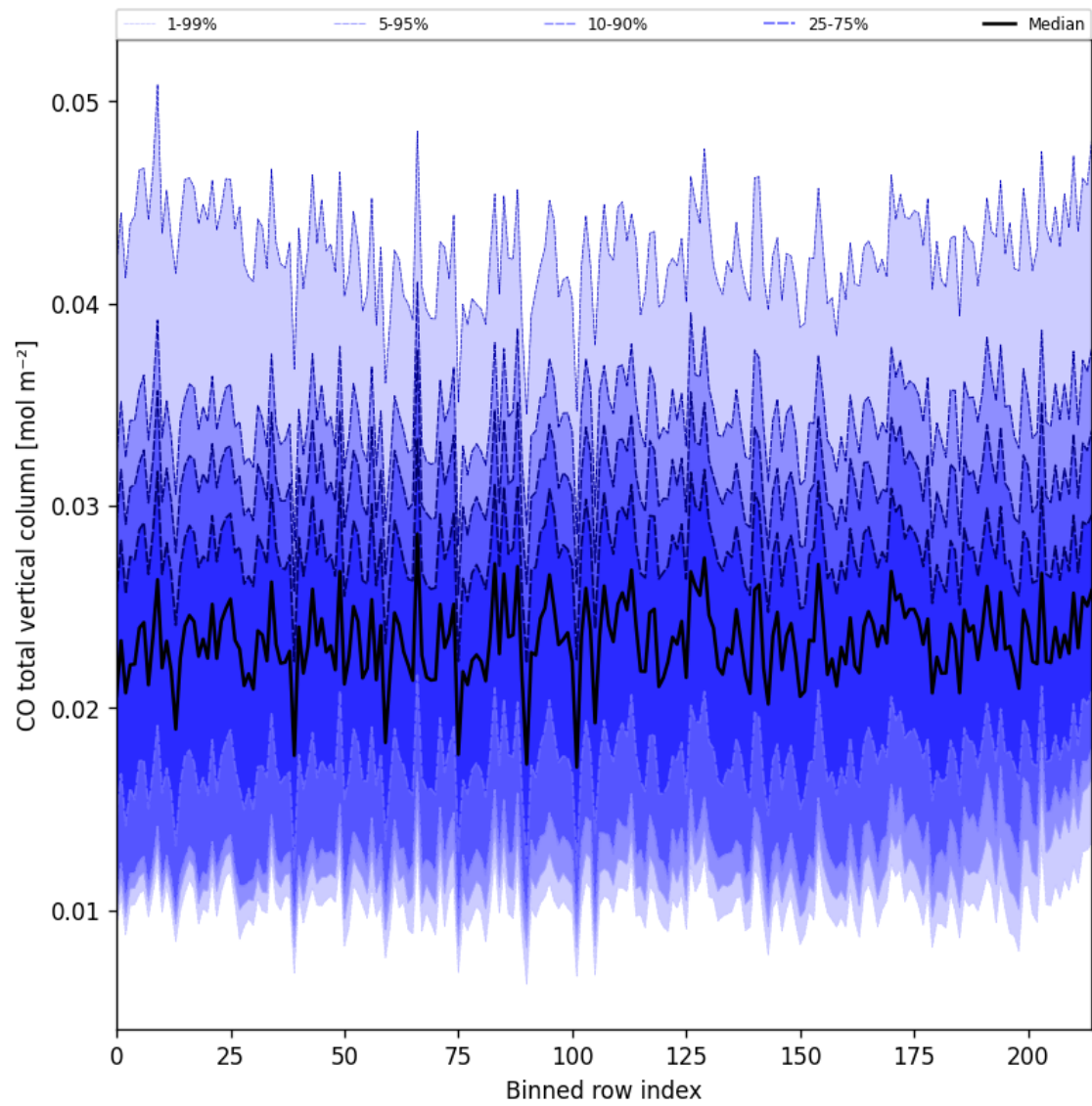
Figure 21: Along track statistics of “CO total vertical column” for 2025-11-02 to 2025-11-03
