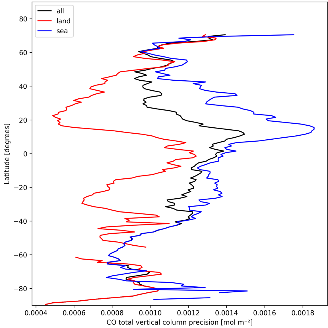
Figure 8: Zonal average of “CO total vertical column precision” for 2025-11-02 to 2025-11-03.
