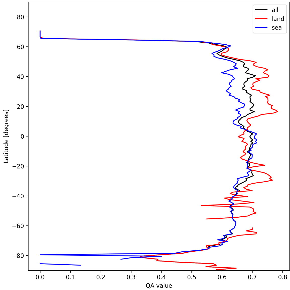
Figure 6: Zonal average of “QA value” for 2025-11-02 to 2025-11-03.
