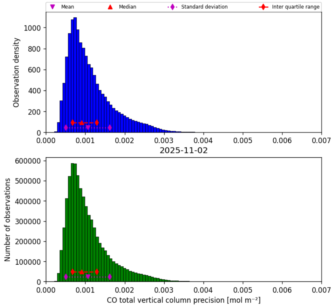
Figure 15: Histogram of “CO total vertical column precision” for 2025-11-02 to 2025-11-03
