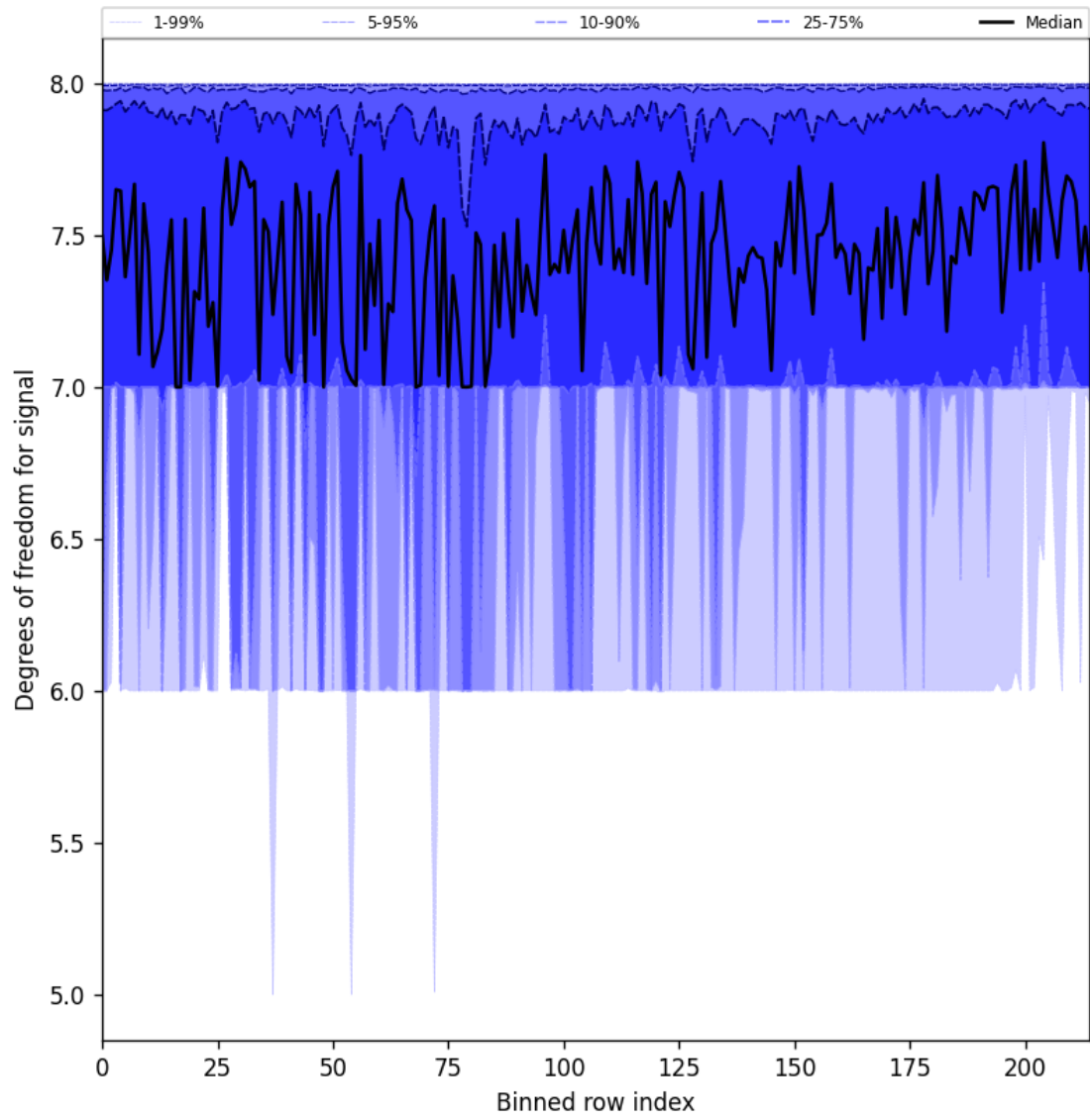
Figure 25: Along track statistics of “Degrees of freedom for signal” for 2025-11-03 to 2025-11-04
