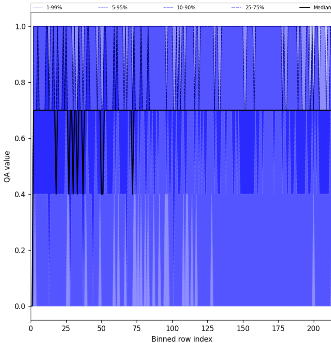
Figure 20: Along track statistics of “QA value” for 2025-11-03 to 2025-11-04
