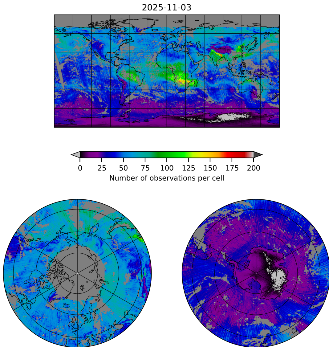
Figure 5: Map of the number of observations for 2025-11-03 to 2025-11-04
