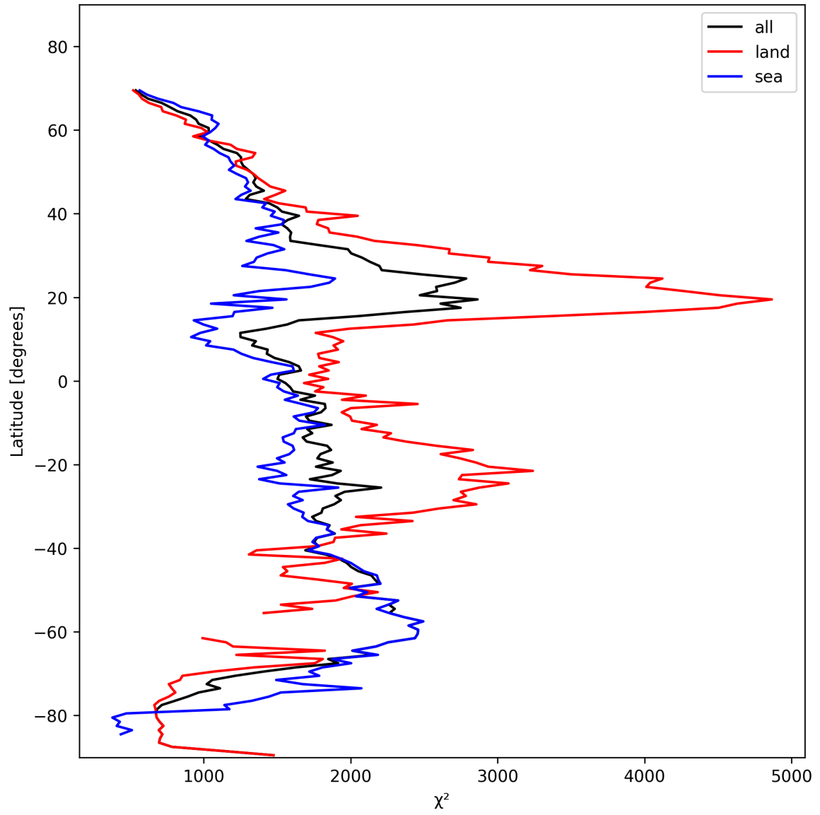
Figure 10: Zonal average of “ \chi^2 ” for 2025-11-03 to 2025-11-04.
