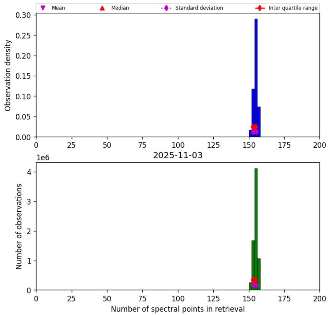
Figure 16: Histogram of “Number of spectral points in retrieval” for 2025-11-03 to 2025-11-04
