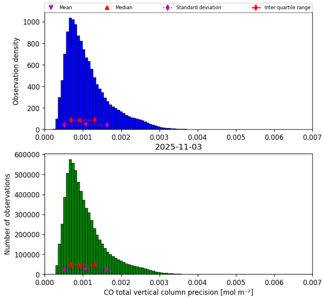
Figure 15: Histogram of “CO total vertical column precision” for 2025-11-03 to 2025-11-04
