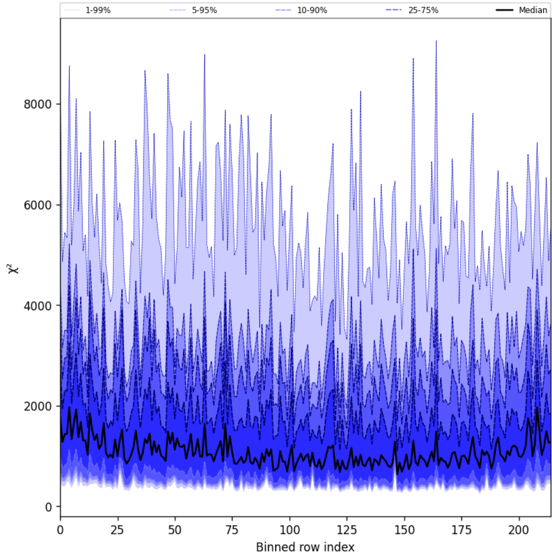
Figure 24: Along track statistics of “ \chi^2 ” for 2025-11-03 to 2025-11-04
