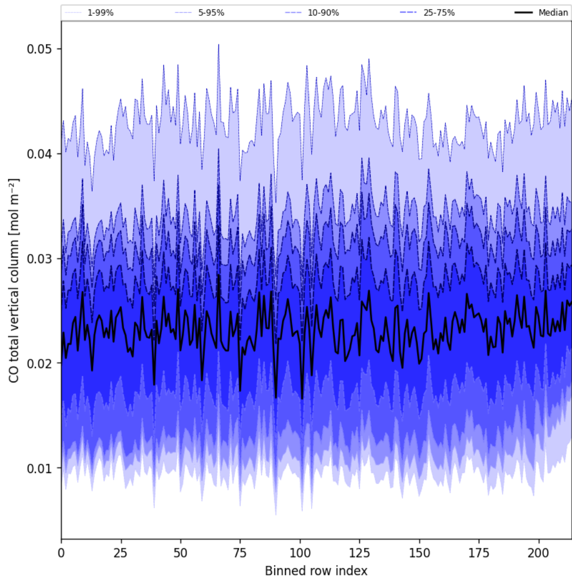
Figure 21: Along track statistics of “CO total vertical column” for 2025-11-03 to 2025-11-04
