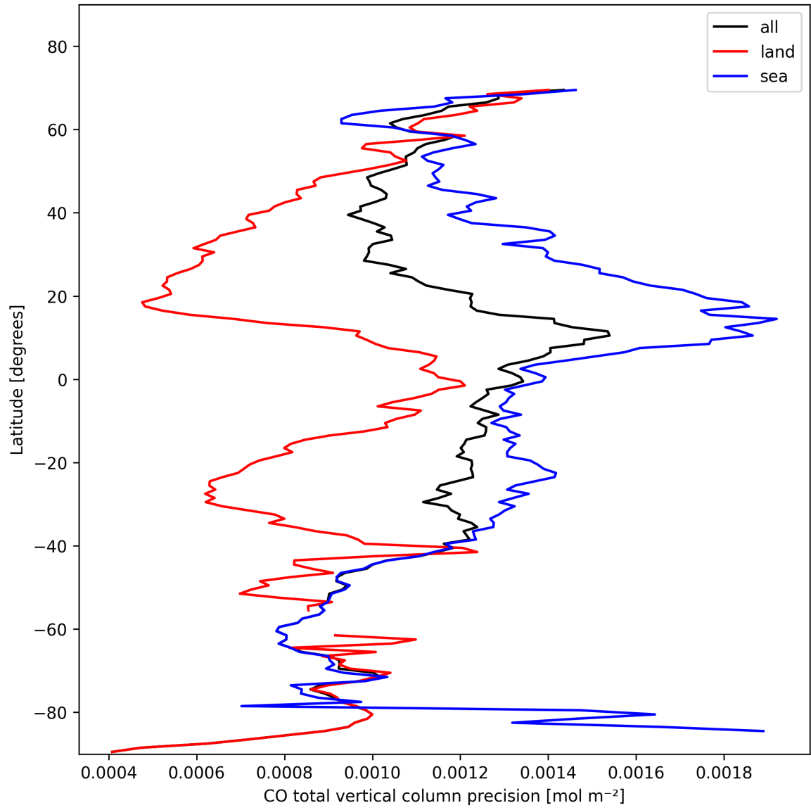
Figure 8: Zonal average of "CO total vertical column precision" for 2025-11-03 to 2025-11-04.
