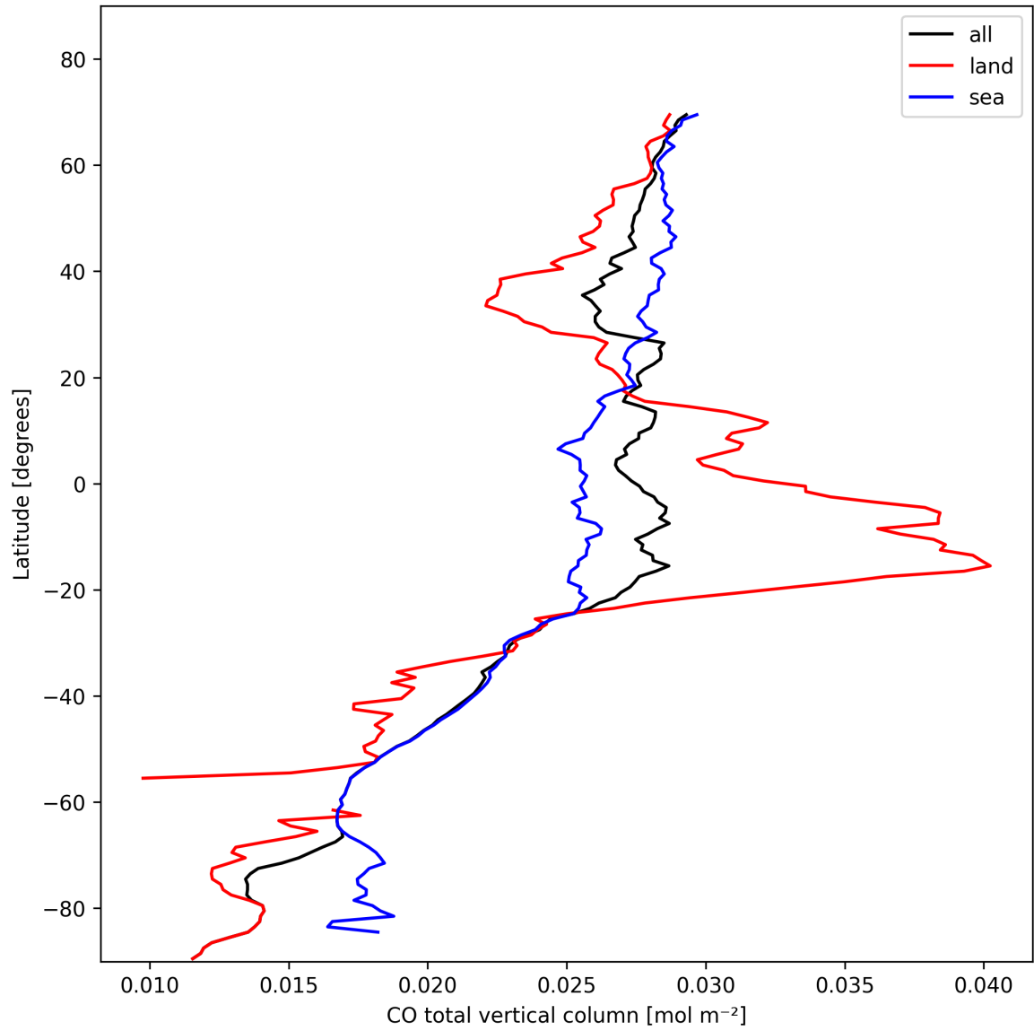
Figure 7: Zonal average of “CO total vertical column” for 2025-11-03 to 2025-11-04.
