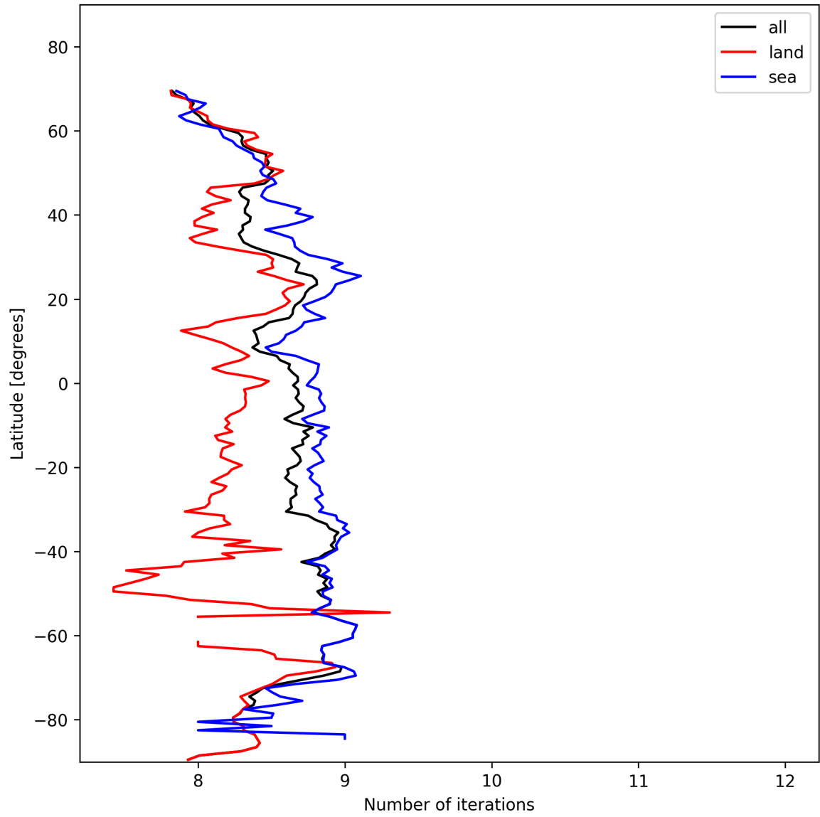
Figure 12: Zonal average of “Number of iterations” for 2025-11-03 to 2025-11-04.
