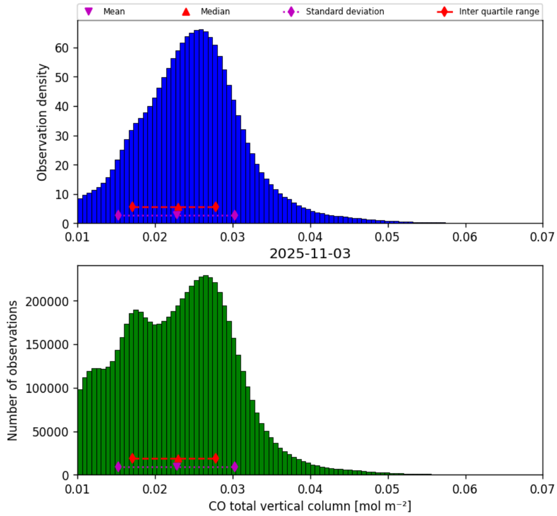
Figure 14: Histogram of “CO total vertical column” for 2025-11-03 to 2025-11-04
