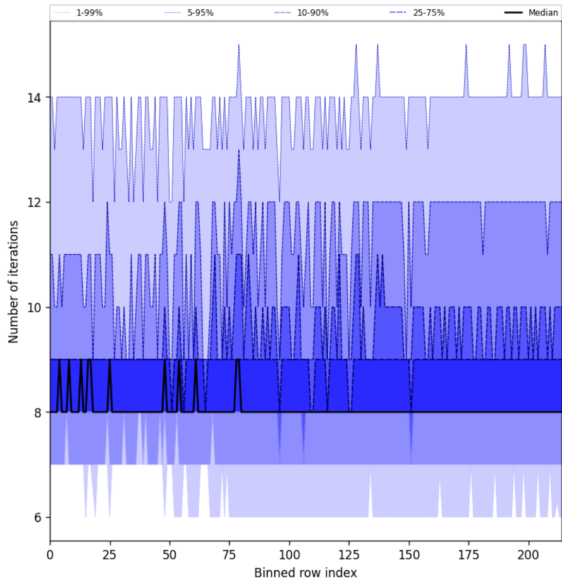
Figure 26: Along track statistics of “Number of iterations” for 2025-11-03 to 2025-11-04
