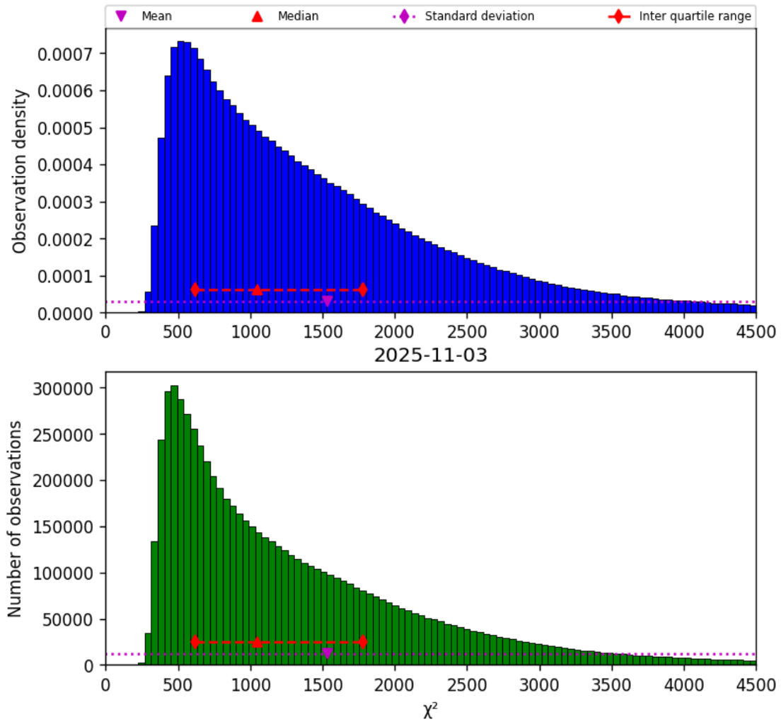
Figure 17: Histogram of “ \chi^2 ” for 2025-11-03 to 2025-11-04
