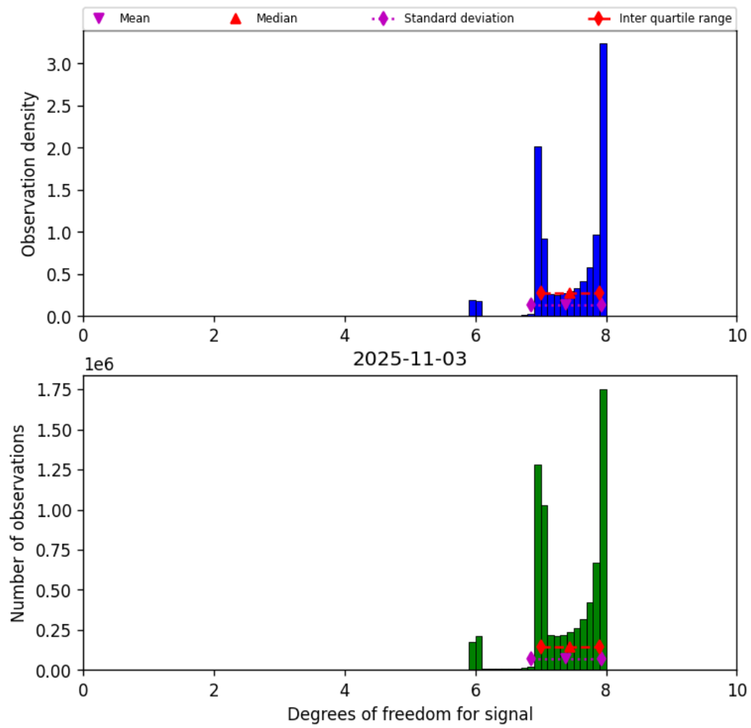
Figure 18: Histogram of “Degrees of freedom for signal” for 2025-11-03 to 2025-11-04
