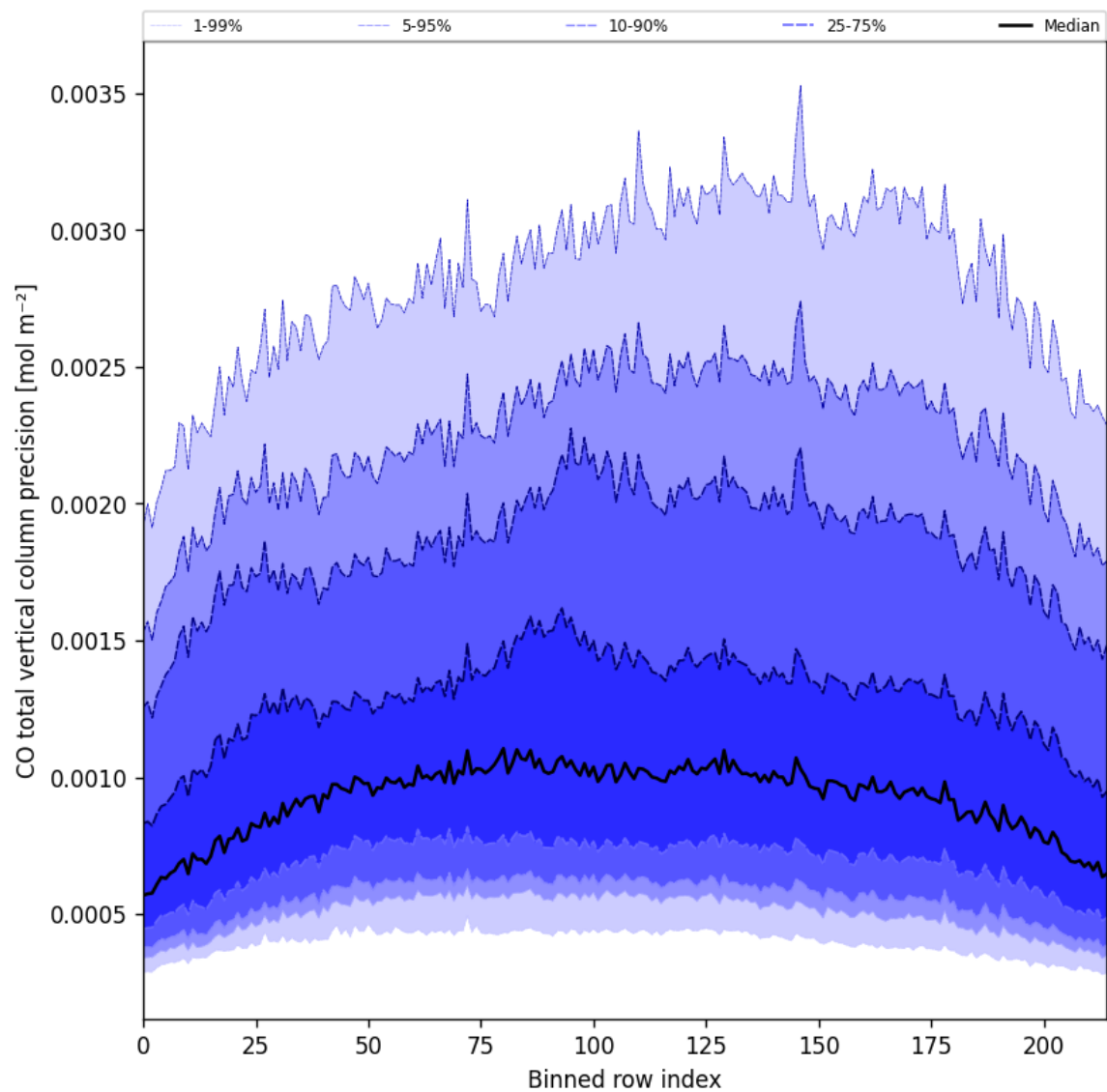
Figure 22: Along track statistics of “CO total vertical column precision” for 2025-11-03 to 2025-11-04
