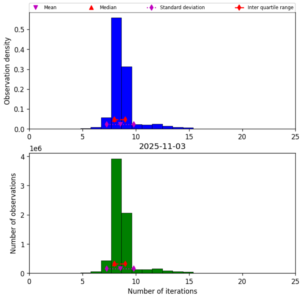
Figure 19: Histogram of “Number of iterations” for 2025-11-03 to 2025-11-04
