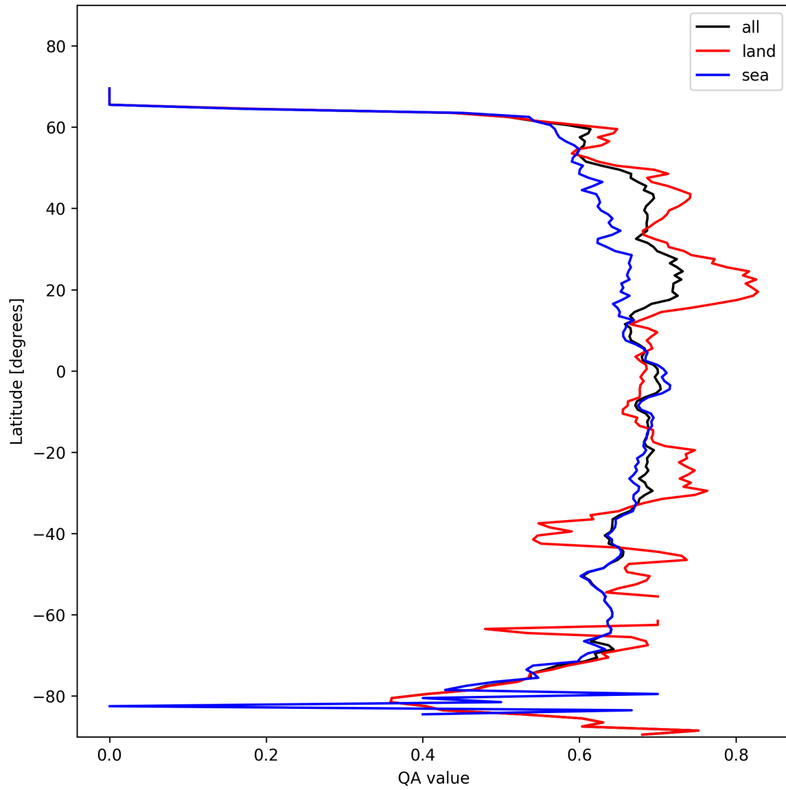
Figure 6: Zonal average of “QA value” for 2025-11-03 to 2025-11-04.
