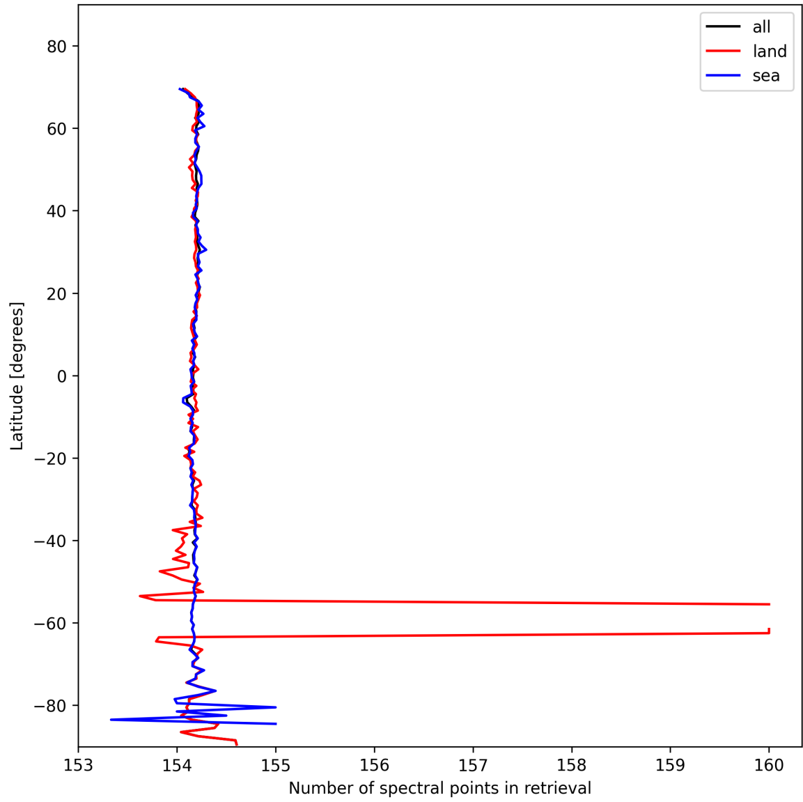
Figure 9: Zonal average of “Number of spectral points in retrieval” for 2025-11-03 to 2025-11-04.
