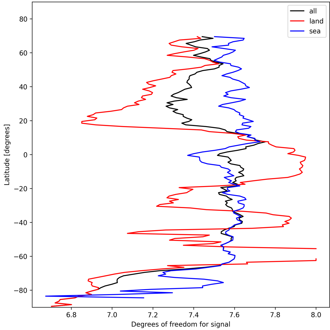
Figure 11: Zonal average of “Degrees of freedom for signal” for 2025-11-03 to 2025-11-04.
