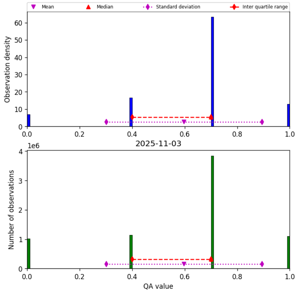
Figure 13: Histogram of “QA value” for 2025-11-03 to 2025-11-04
