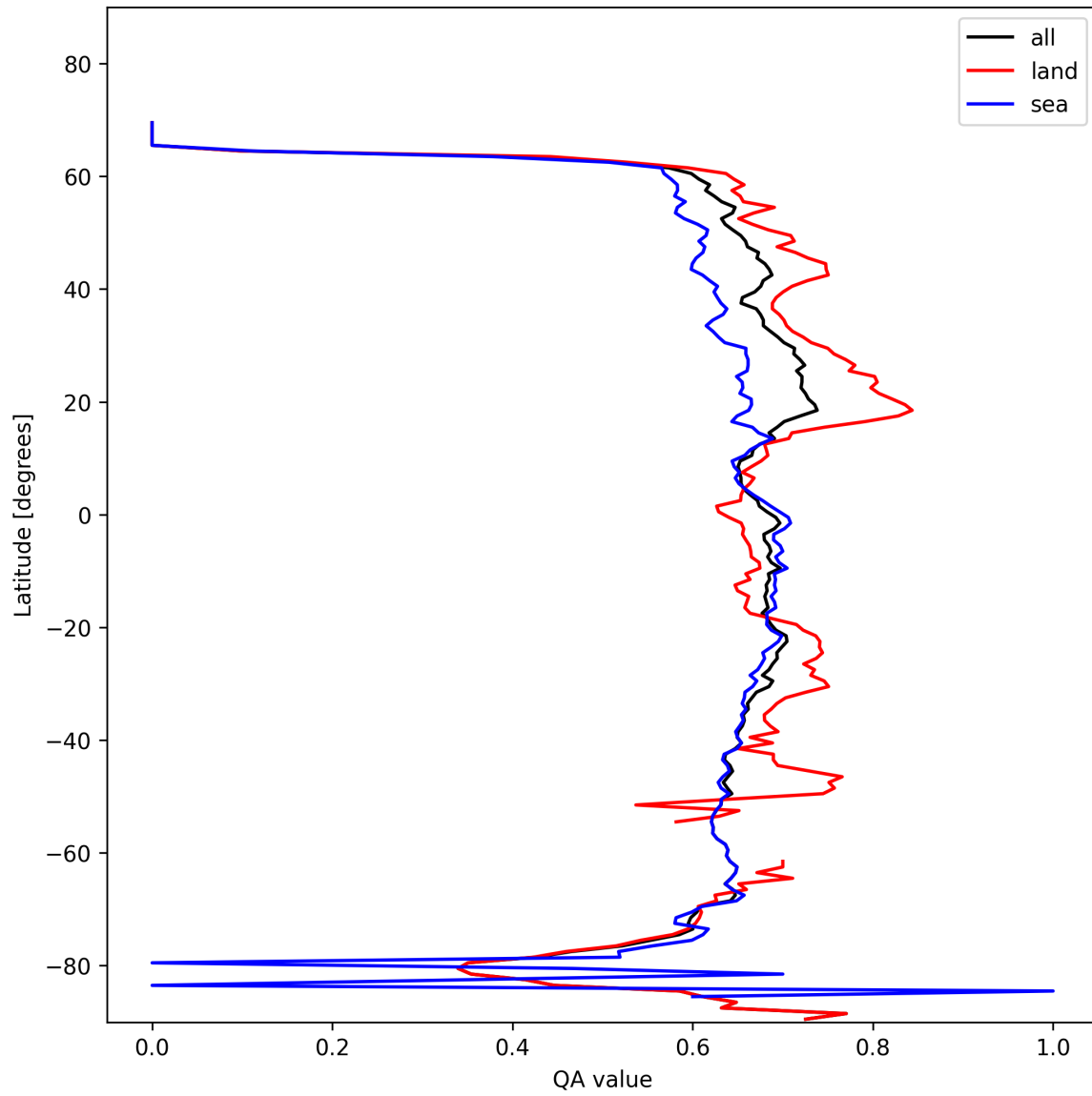
Figure 6: Zonal average of “QA value” for 2025-11-04 to 2025-11-05.
