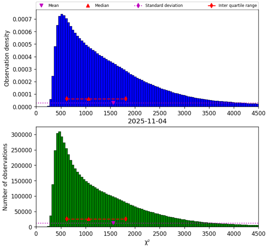
Figure 17: Histogram of " \chi^2 " for 2025-11-04 to 2025-11-05
