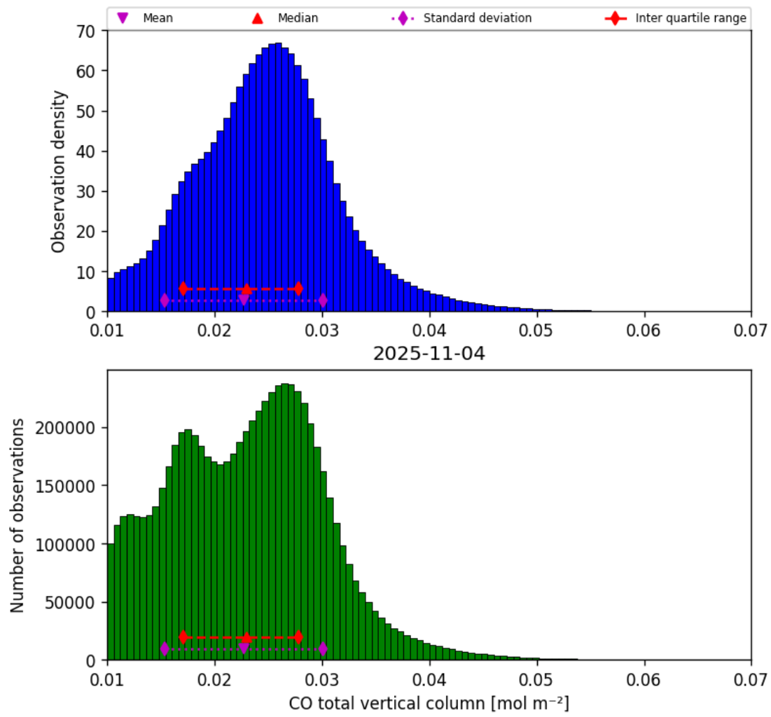
Figure 14: Histogram of “CO total vertical column” for 2025-11-04 to 2025-11-05
