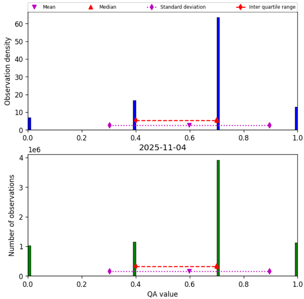
Figure 13: Histogram of “QA value” for 2025-11-04 to 2025-11-05
