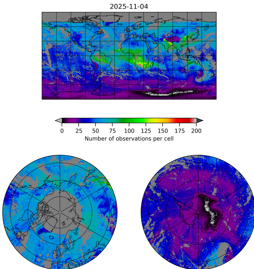
Figure 5: Map of the number of observations for 2025-11-04 to 2025-11-05
