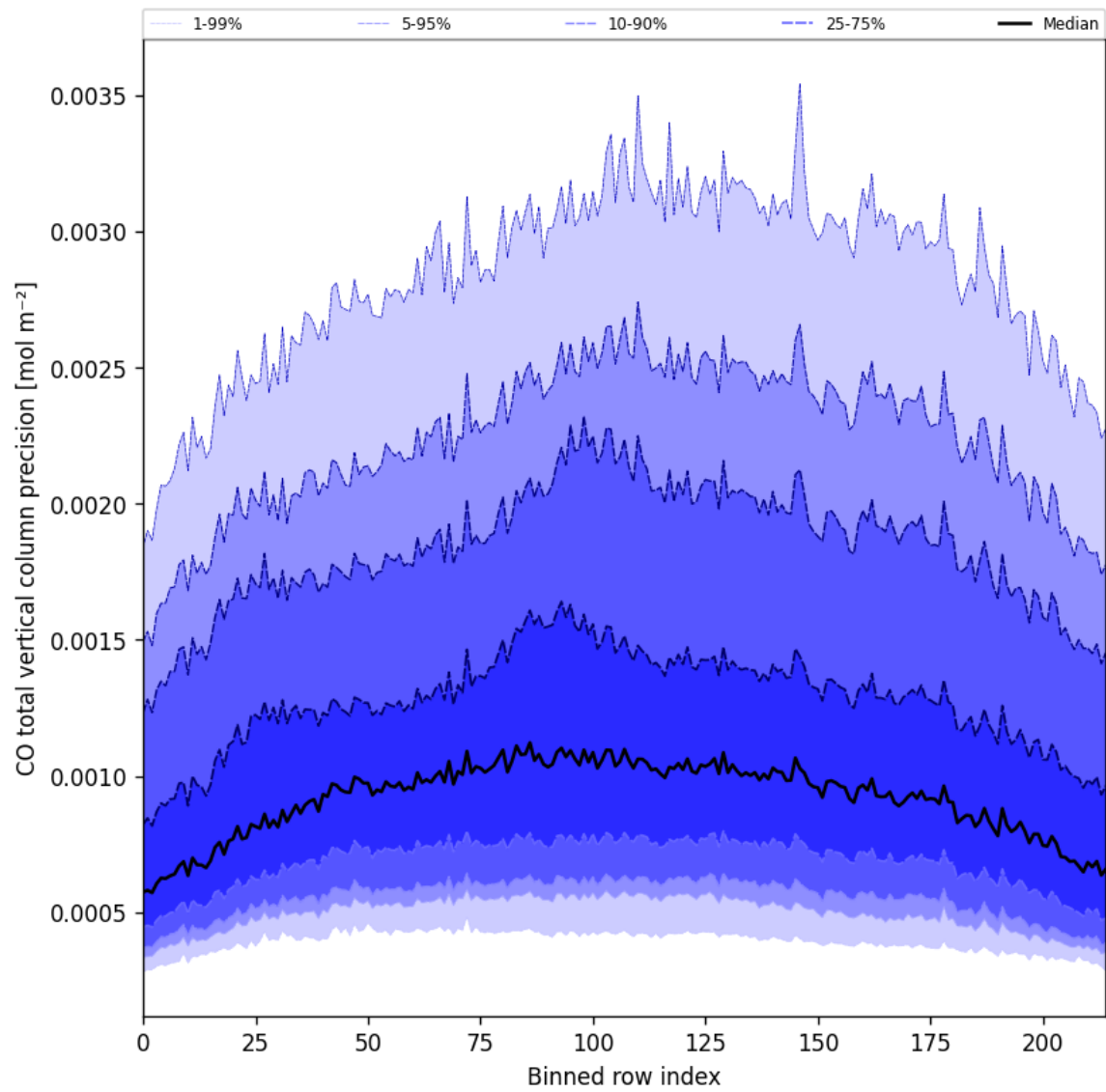
Figure 22: Along track statistics of “CO total vertical column precision” for 2025-11-04 to 2025-11-05
