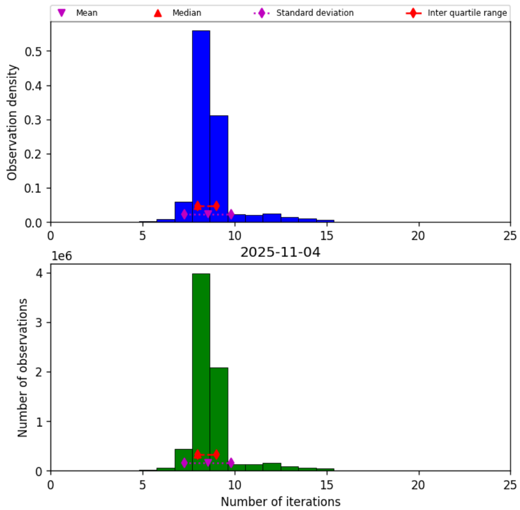
Figure 19: Histogram of “Number of iterations” for 2025-11-04 to 2025-11-05
