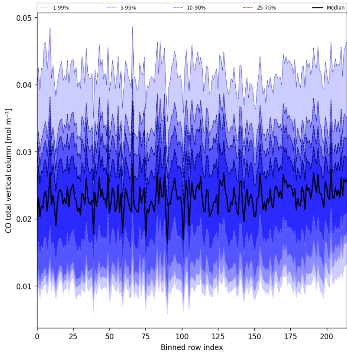
Figure 21: Along track statistics of “CO total vertical column” for 2025-11-04 to 2025-11-05
