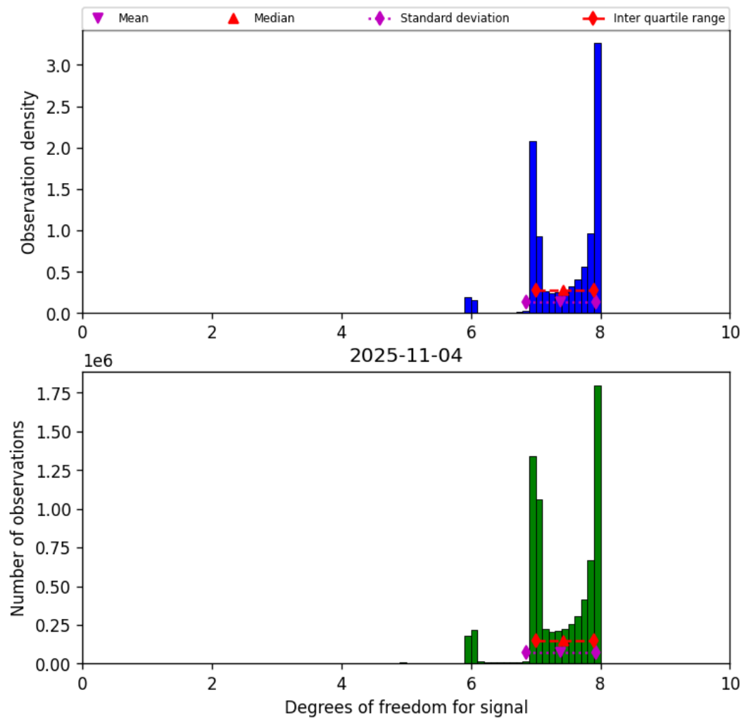
Figure 18: Histogram of “Degrees of freedom for signal” for 2025-11-04 to 2025-11-05
