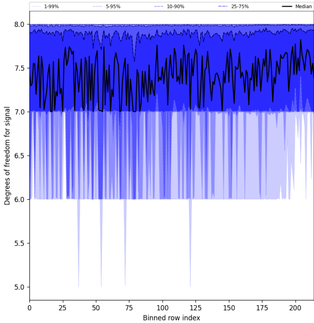
Figure 25: Along track statistics of “Degrees of freedom for signal” for 2025-11-04 to 2025-11-05
