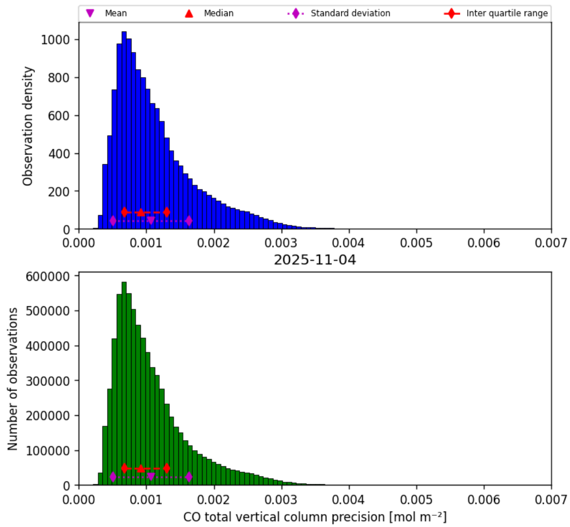
Figure 15: Histogram of “CO total vertical column precision” for 2025-11-04 to 2025-11-05
