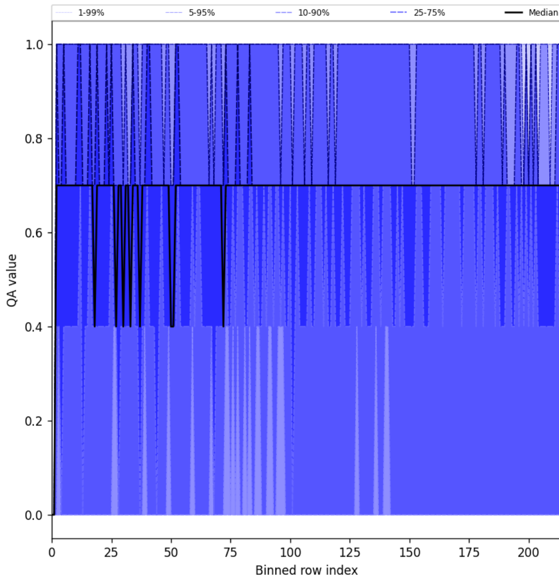
Figure 20: Along track statistics of “QA value” for 2025-11-04 to 2025-11-05
