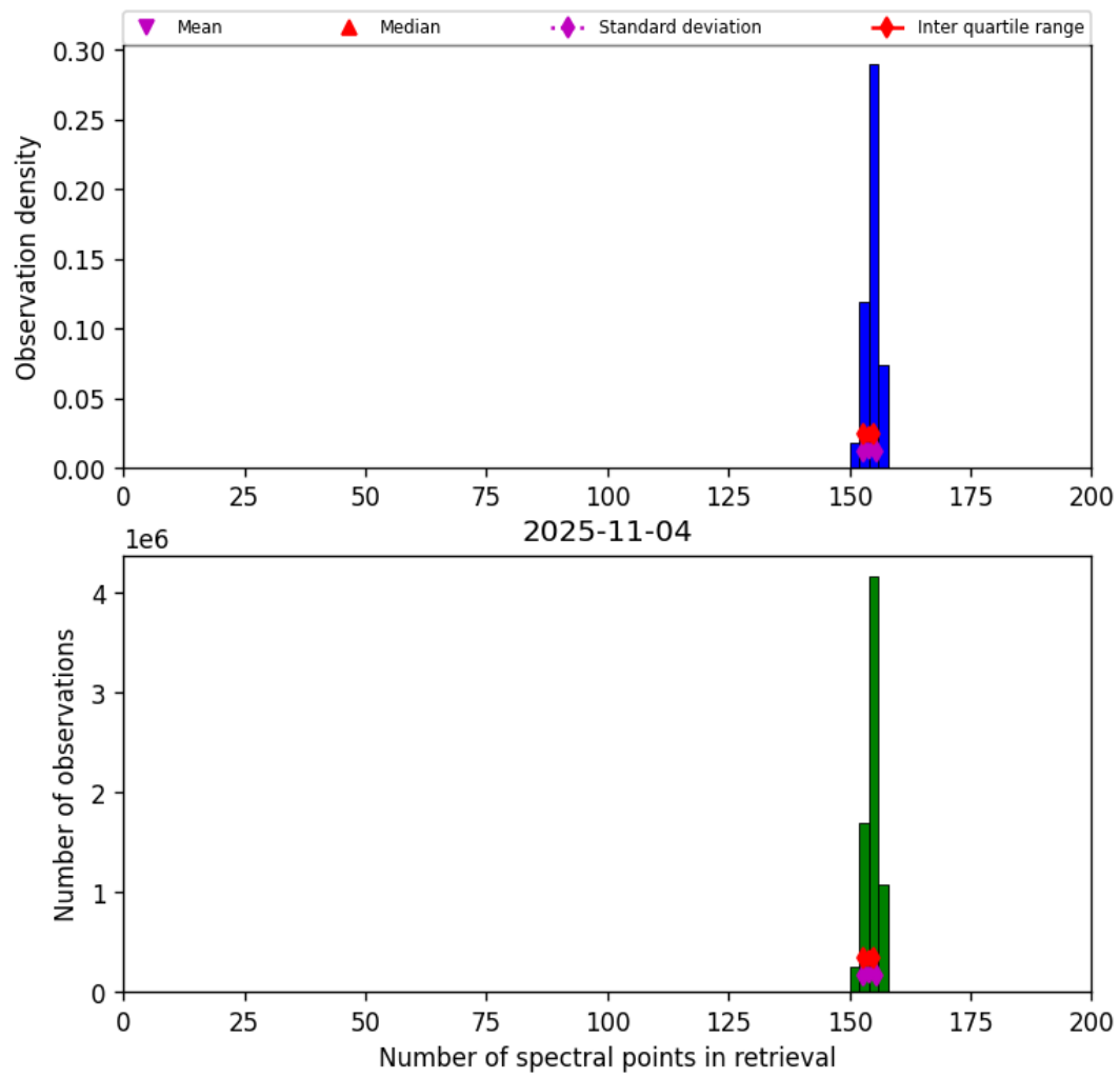
Figure 16: Histogram of “Number of spectral points in retrieval” for 2025-11-04 to 2025-11-05
