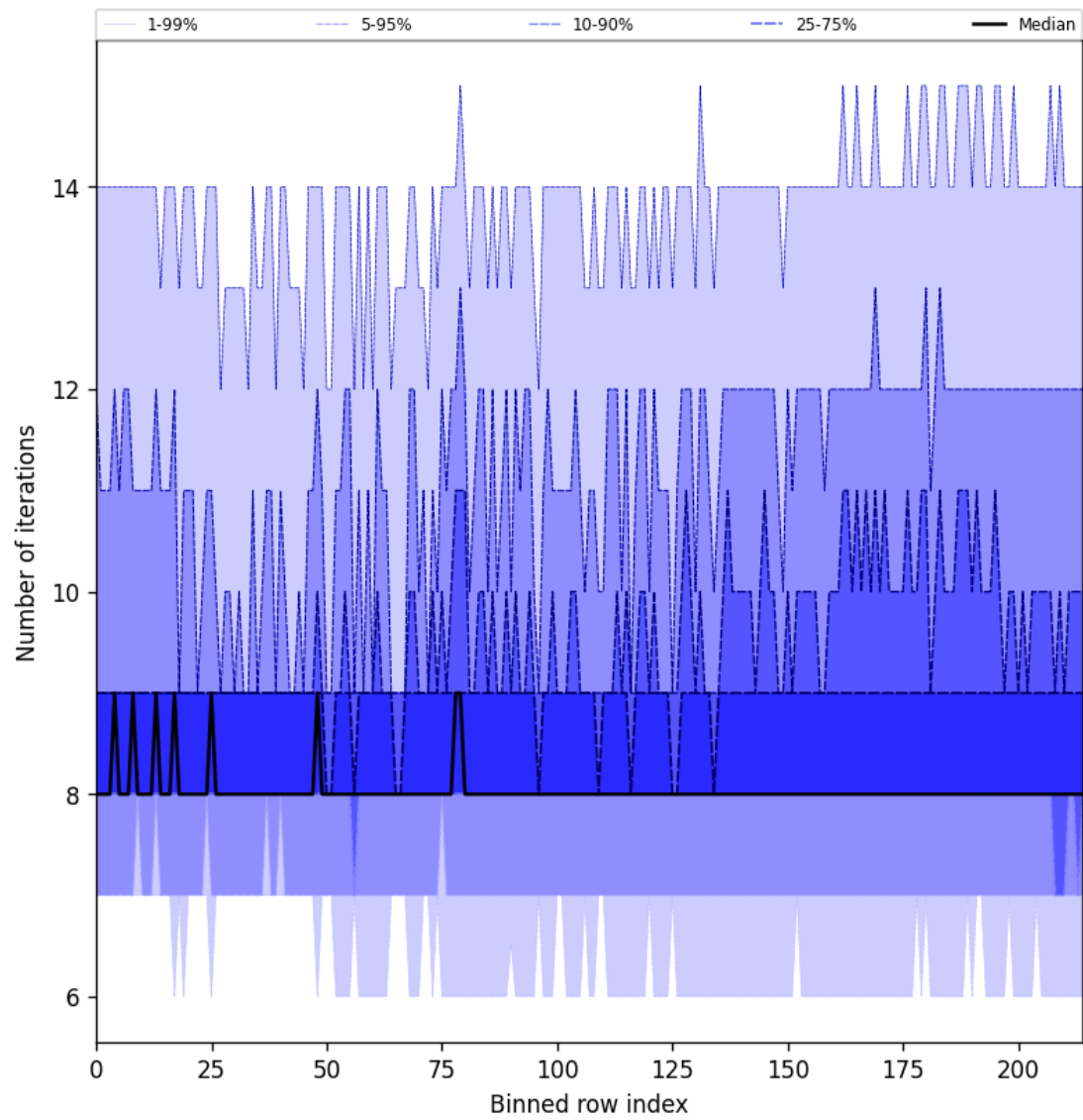
Figure 26: Along track statistics of “Number of iterations” for 2025-11-04 to 2025-11-05
