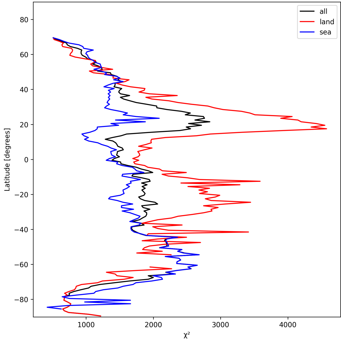
Figure 10: Zonal average of “ \chi^2 ” for 2025-11-04 to 2025-11-05.
