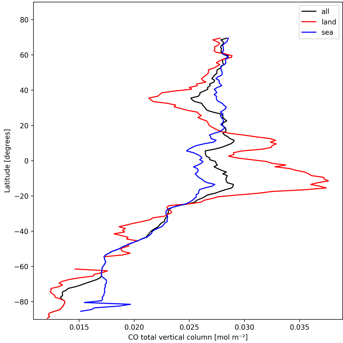
Figure 7: Zonal average of “CO total vertical column” for 2025-11-04 to 2025-11-05.
