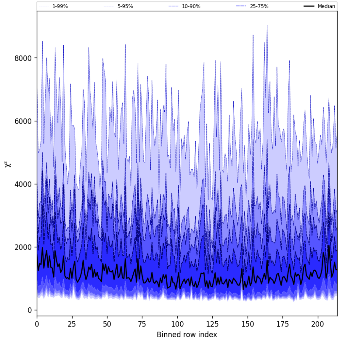
Figure 24: Along track statistics of “ \chi^2 ” for 2025-11-04 to 2025-11-05
