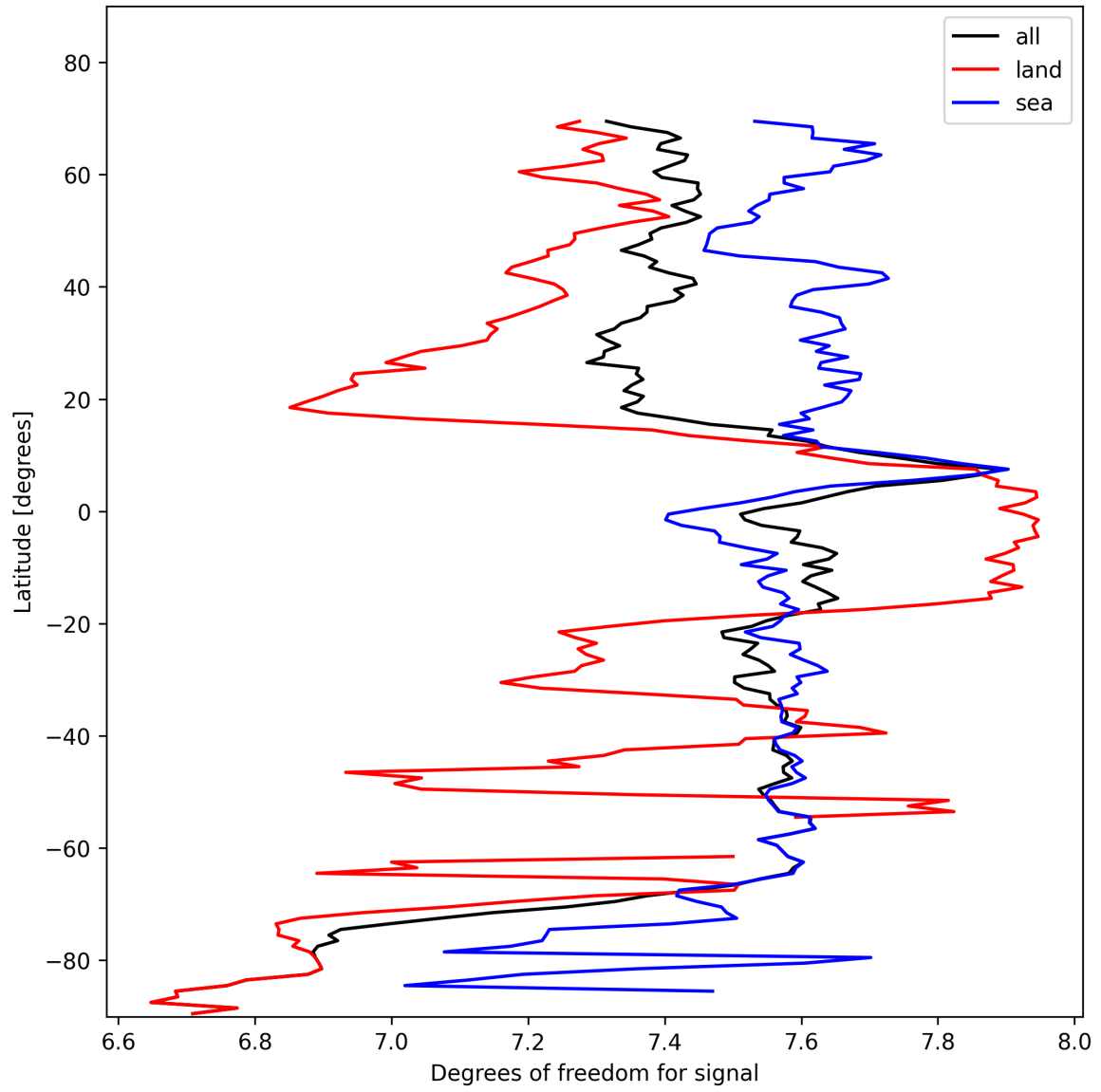
Figure 11: Zonal average of “Degrees of freedom for signal” for 2025-11-04 to 2025-11-05.
