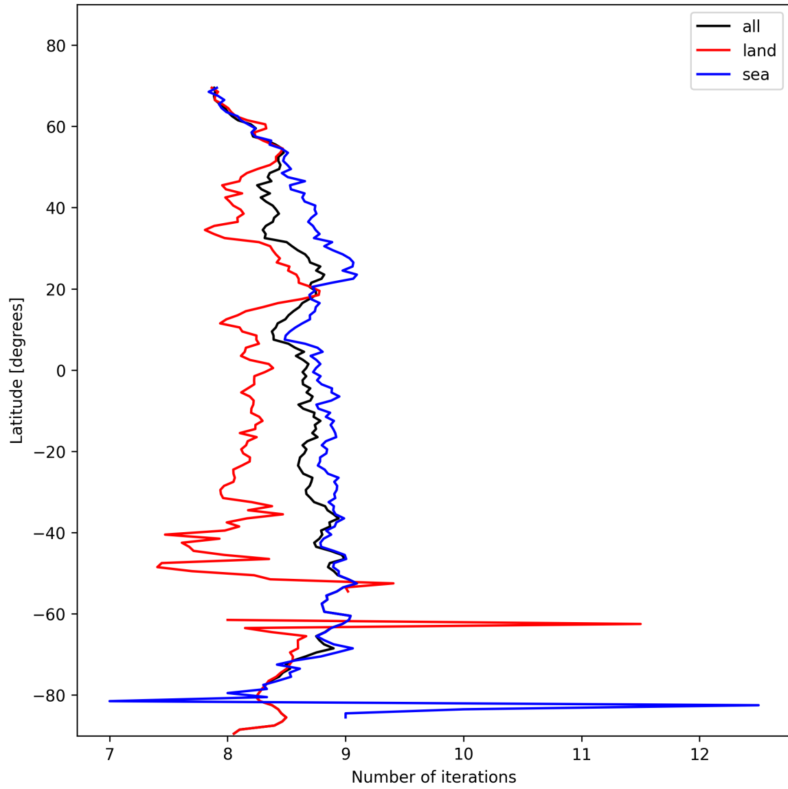
Figure 12: Zonal average of “Number of iterations” for 2025-11-04 to 2025-11-05.
