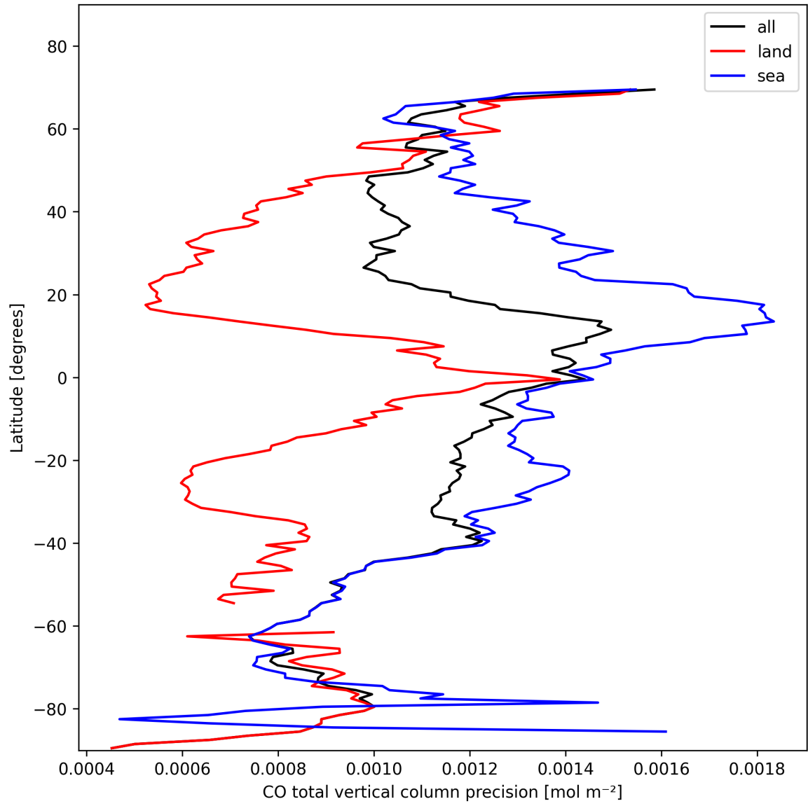
Figure 8: Zonal average of “CO total vertical column precision” for 2025-11-04 to 2025-11-05.
