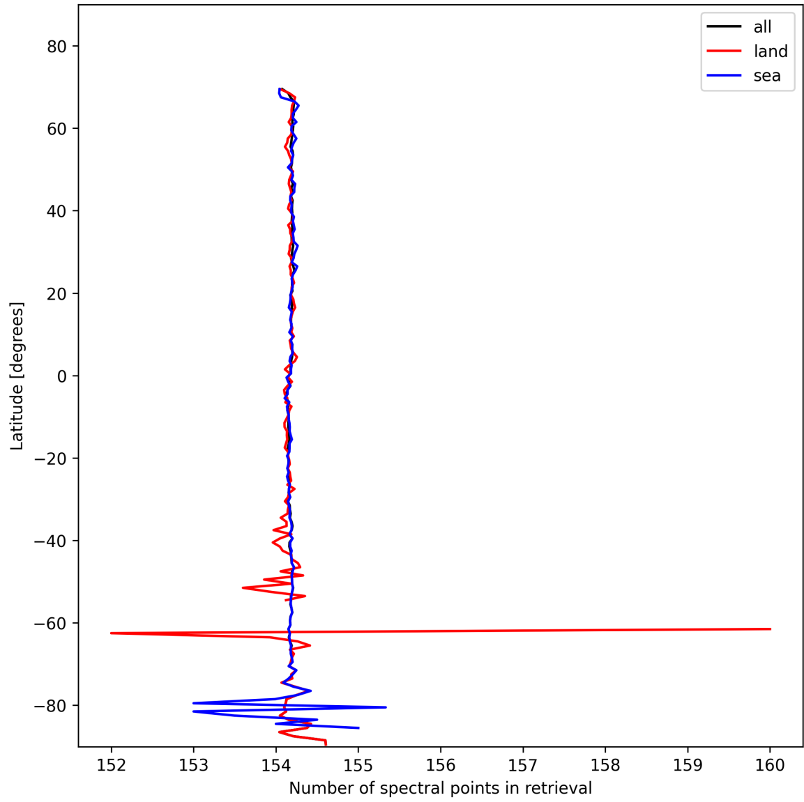
Figure 9: Zonal average of “Number of spectral points in retrieval” for 2025-11-04 to 2025-11-05.
