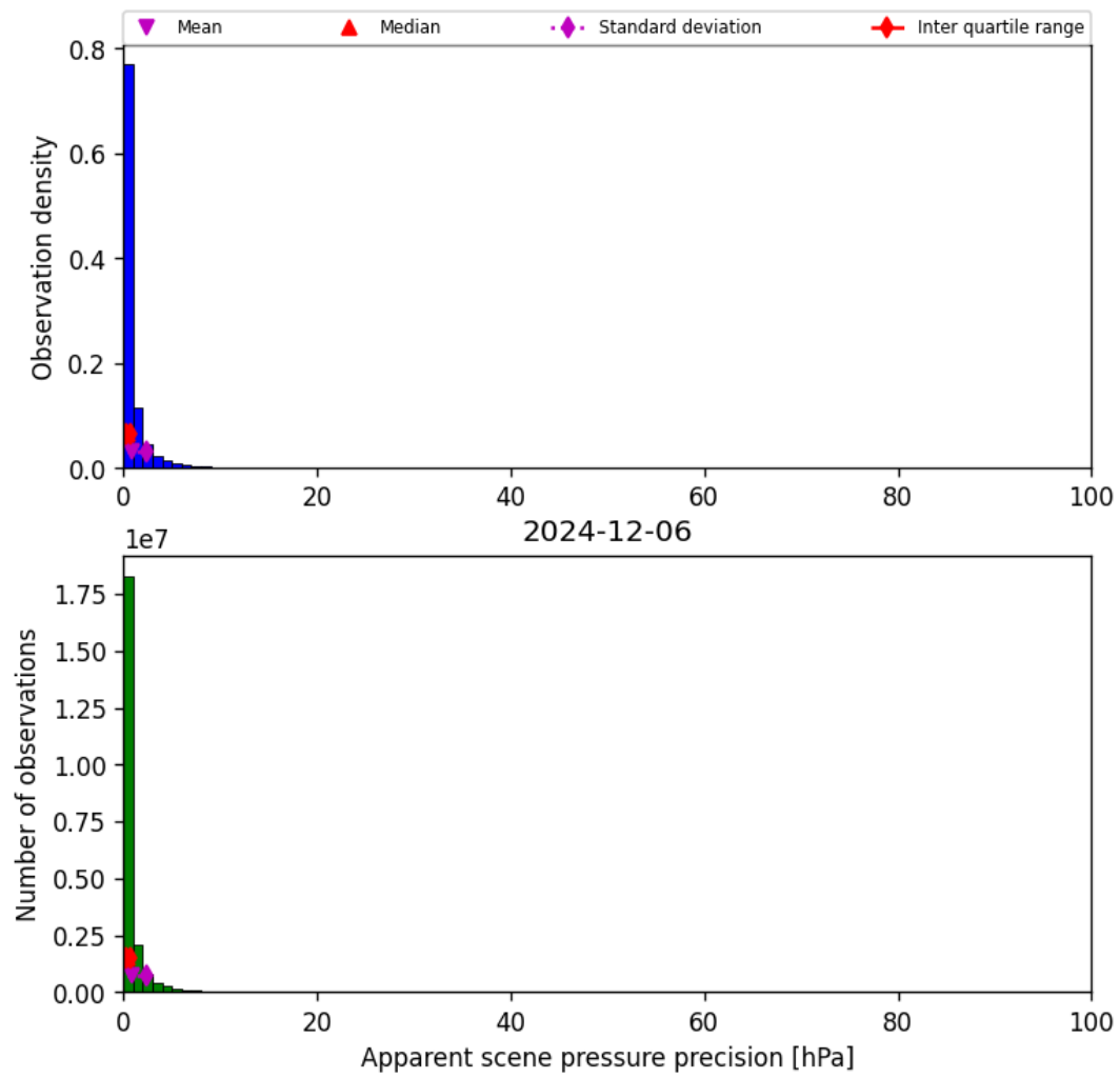
Figure 35: Histogram of “Apparent scene pressure precision” for 2024-12-06 to 2024-12-07
