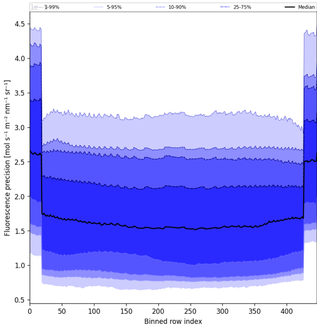
Figure 56: Along track statistics of “Fluorescence precision” for 2024-12-06 to 2024-12-07
