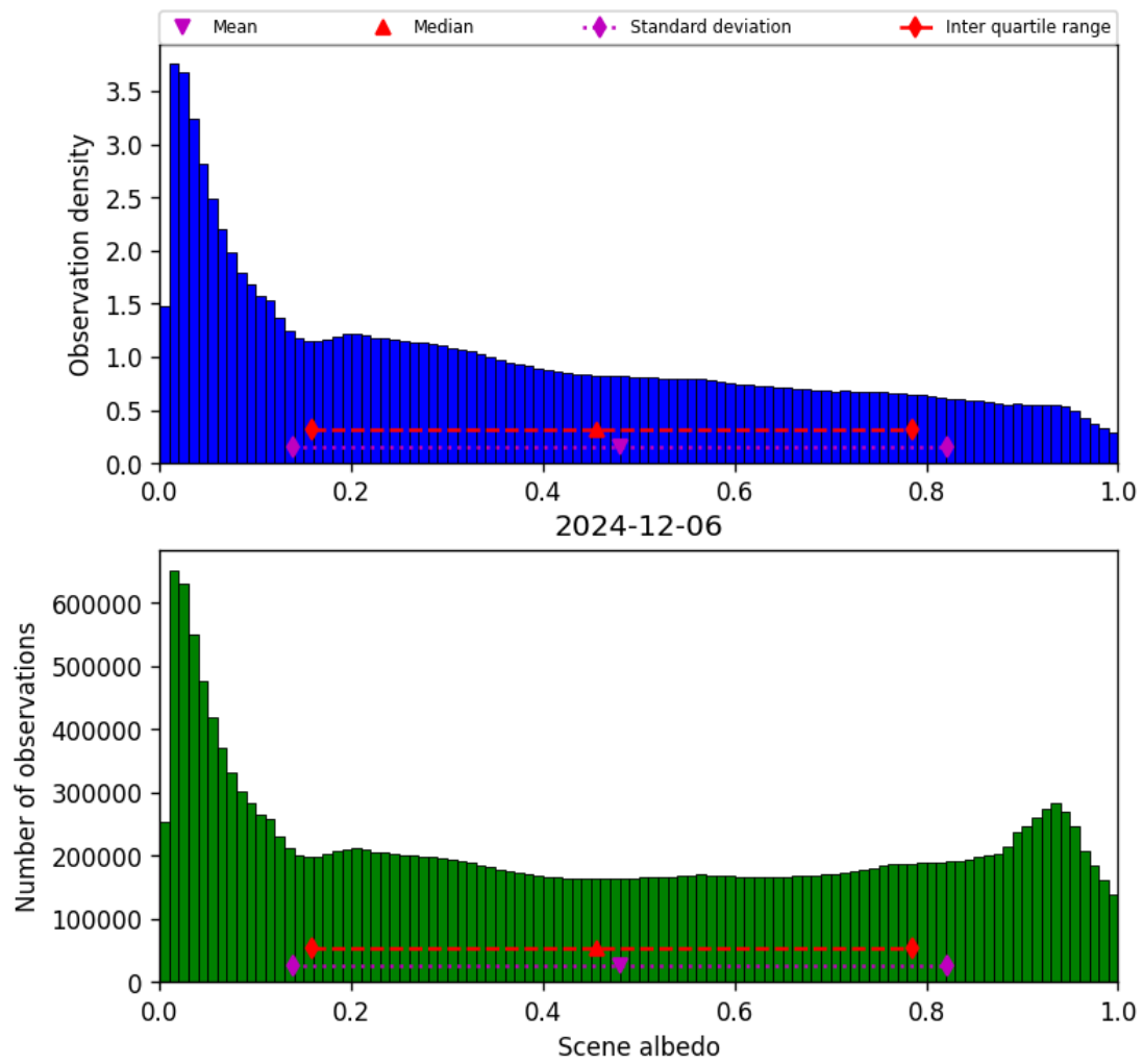
Figure 32: Histogram of “Scene albedo” for 2024-12-06 to 2024-12-07
