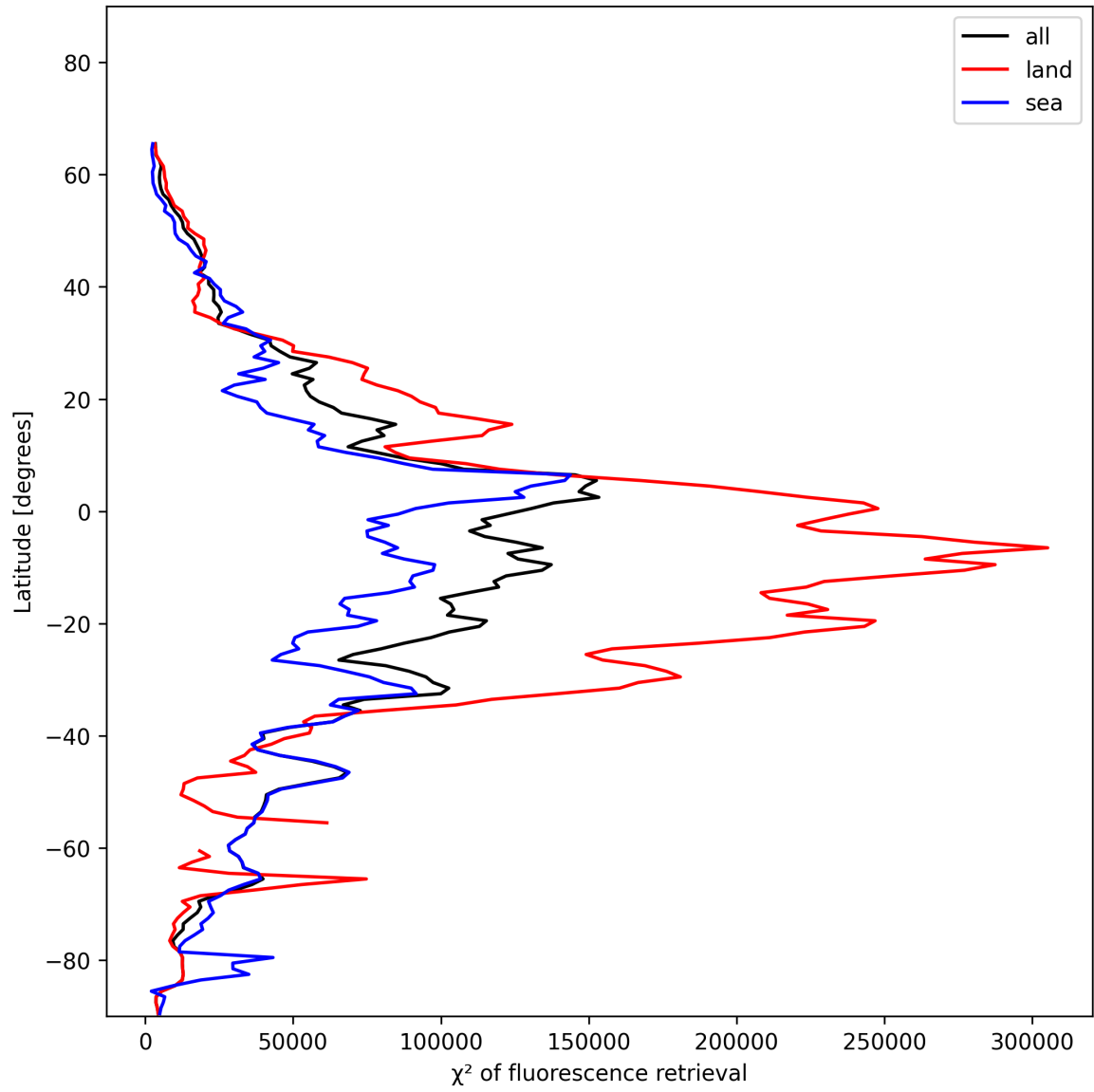
Figure 23: Zonal average of “ \chi^2 of fluorescence retrieval” for 2024-12-06 to 2024-12-07.
