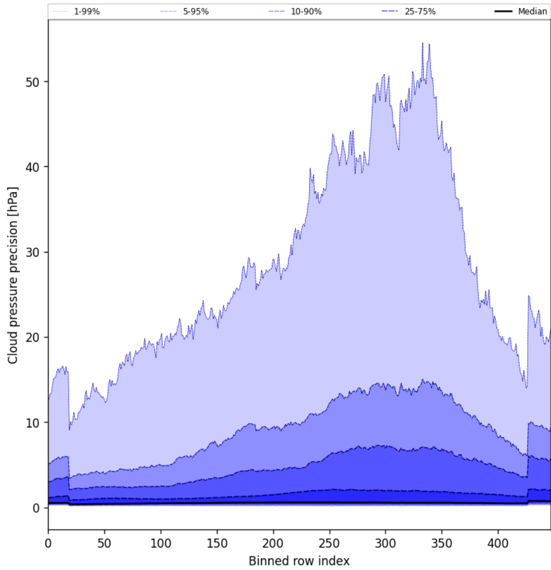
Figure 46: Along track statistics of “Cloud pressure precision” for 2024-12-06 to 2024-12-07
