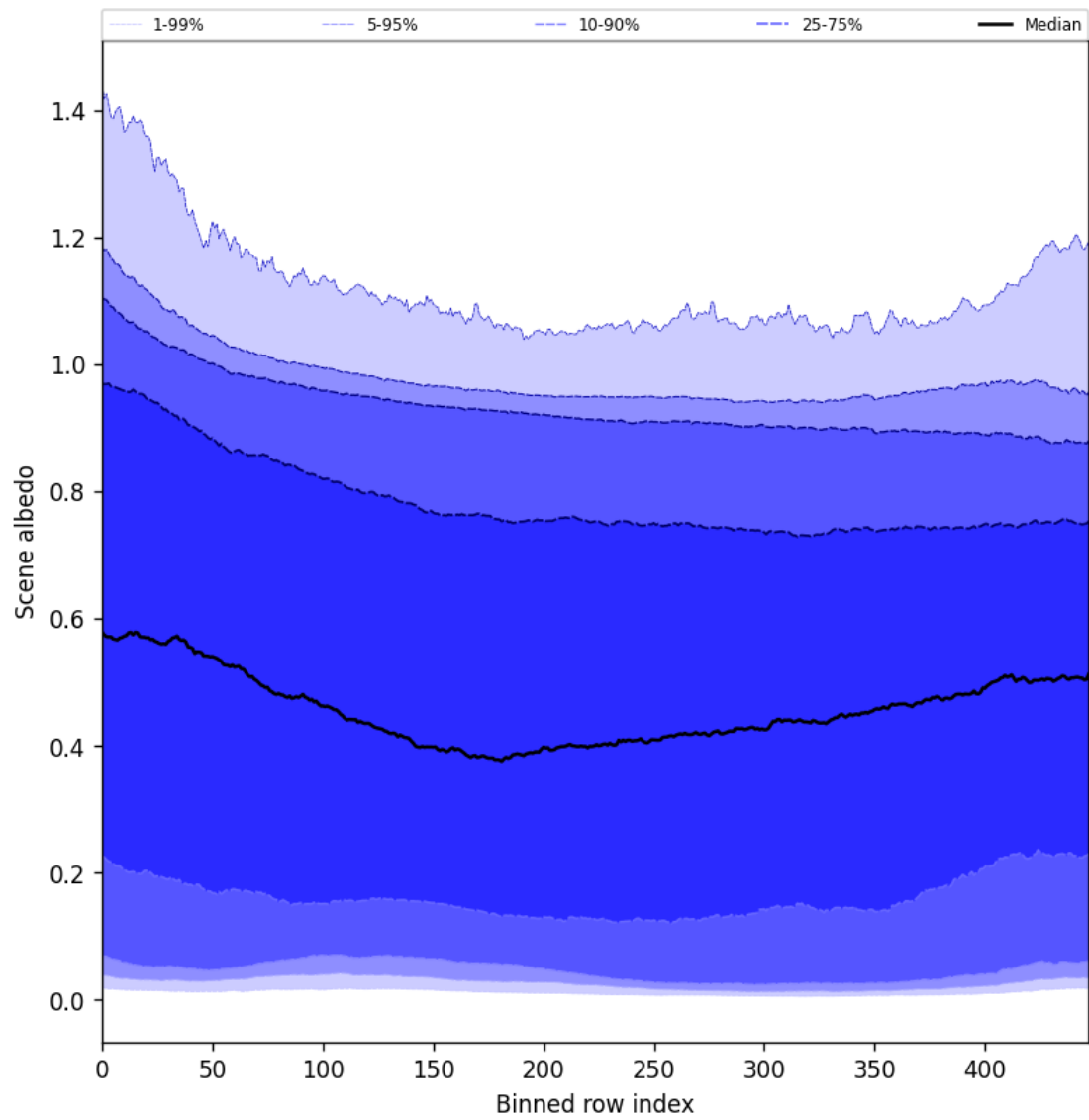
Figure 49: Along track statistics of “Scene albedo” for 2024-12-06 to 2024-12-07
