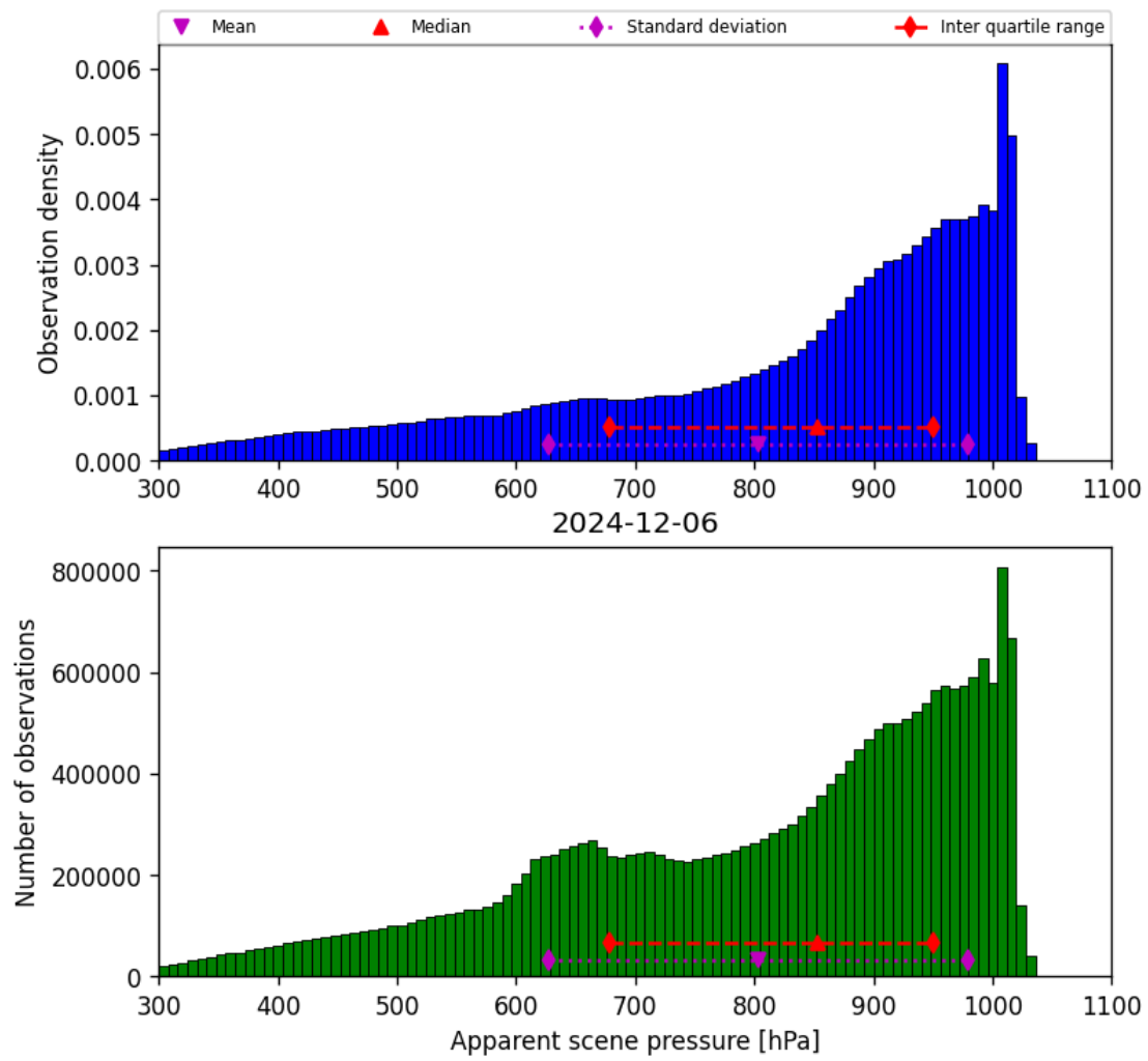
Figure 34: Histogram of “Apparent scene pressure” for 2024-12-06 to 2024-12-07
