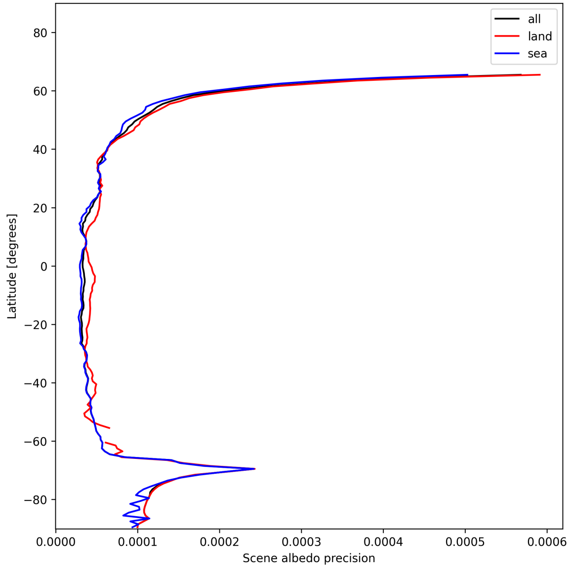
Figure 16: Zonal average of “Scene albedo precision” for 2024-12-06 to 2024-12-07.
