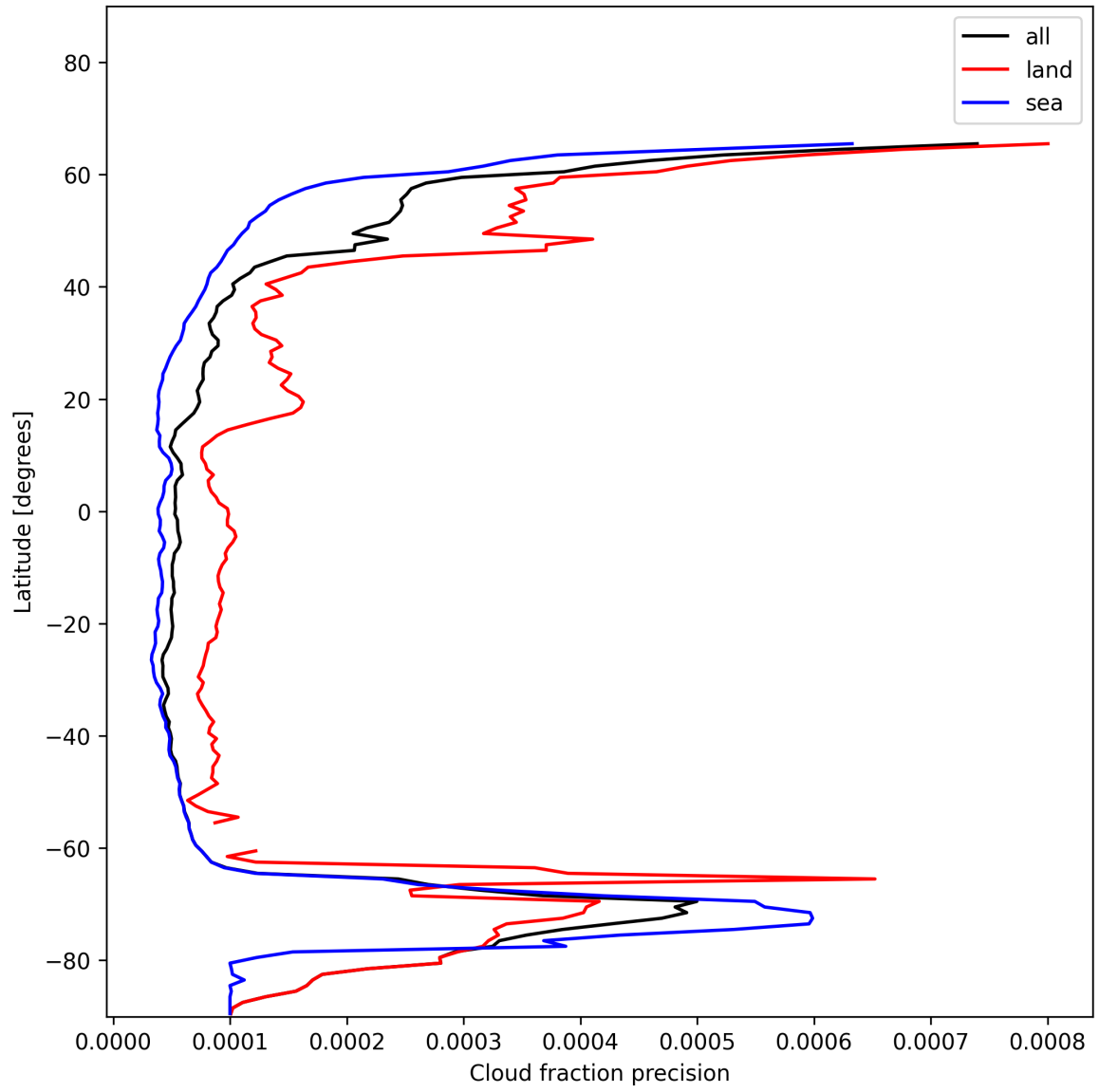
Figure 14: Zonal average of “Cloud fraction precision” for 2024-12-06 to 2024-12-07.
