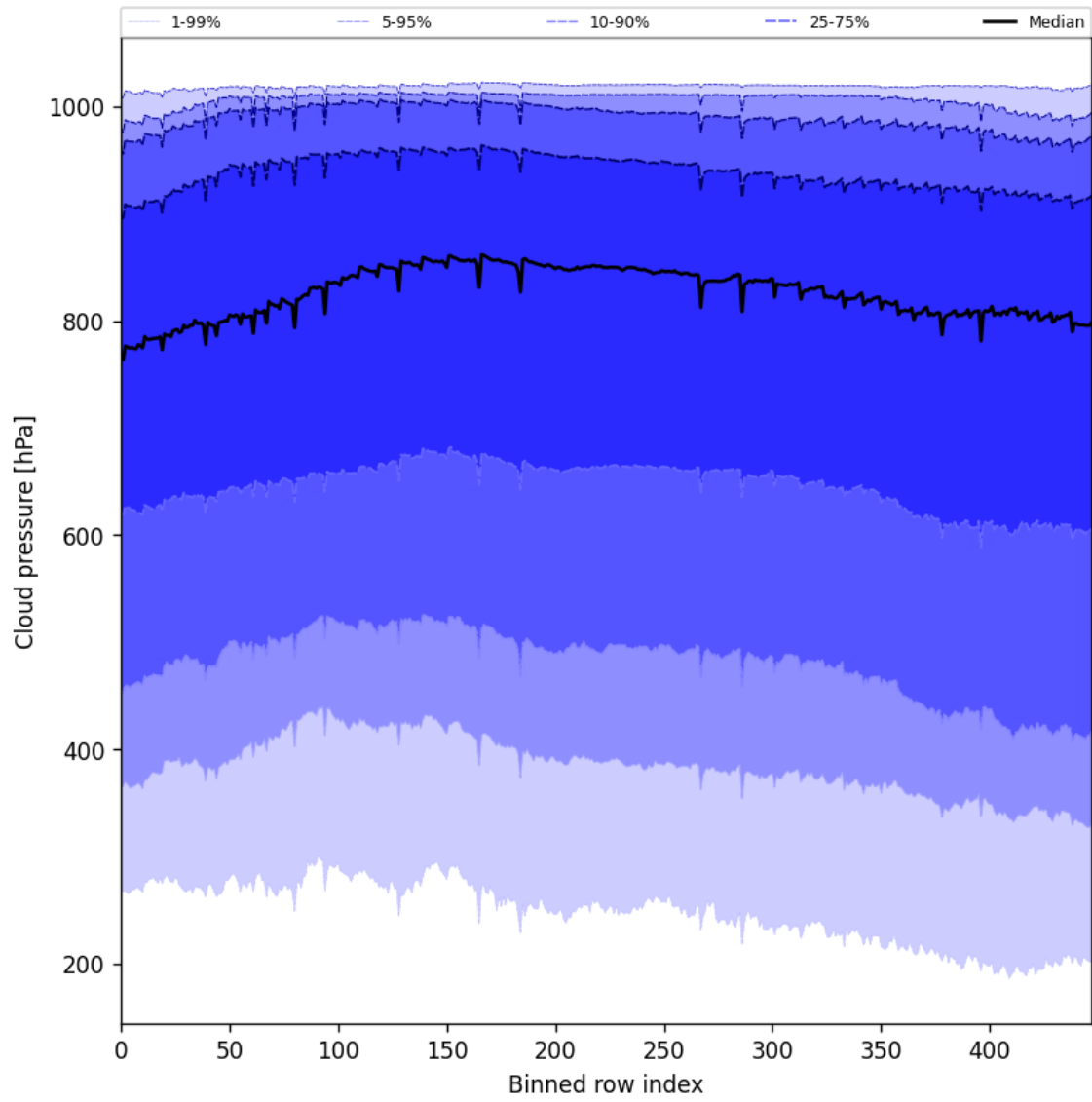
Figure 45: Along track statistics of “Cloud pressure” for 2024-12-06 to 2024-12-07
