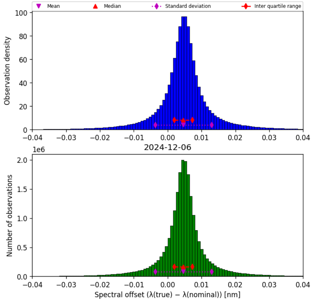
Figure 43: Histogram of “Spectral offset ( \lambda_{\text{true}} - \lambda_{\text{nominal}} )” for 2024-12-06 to 2024-12-07
