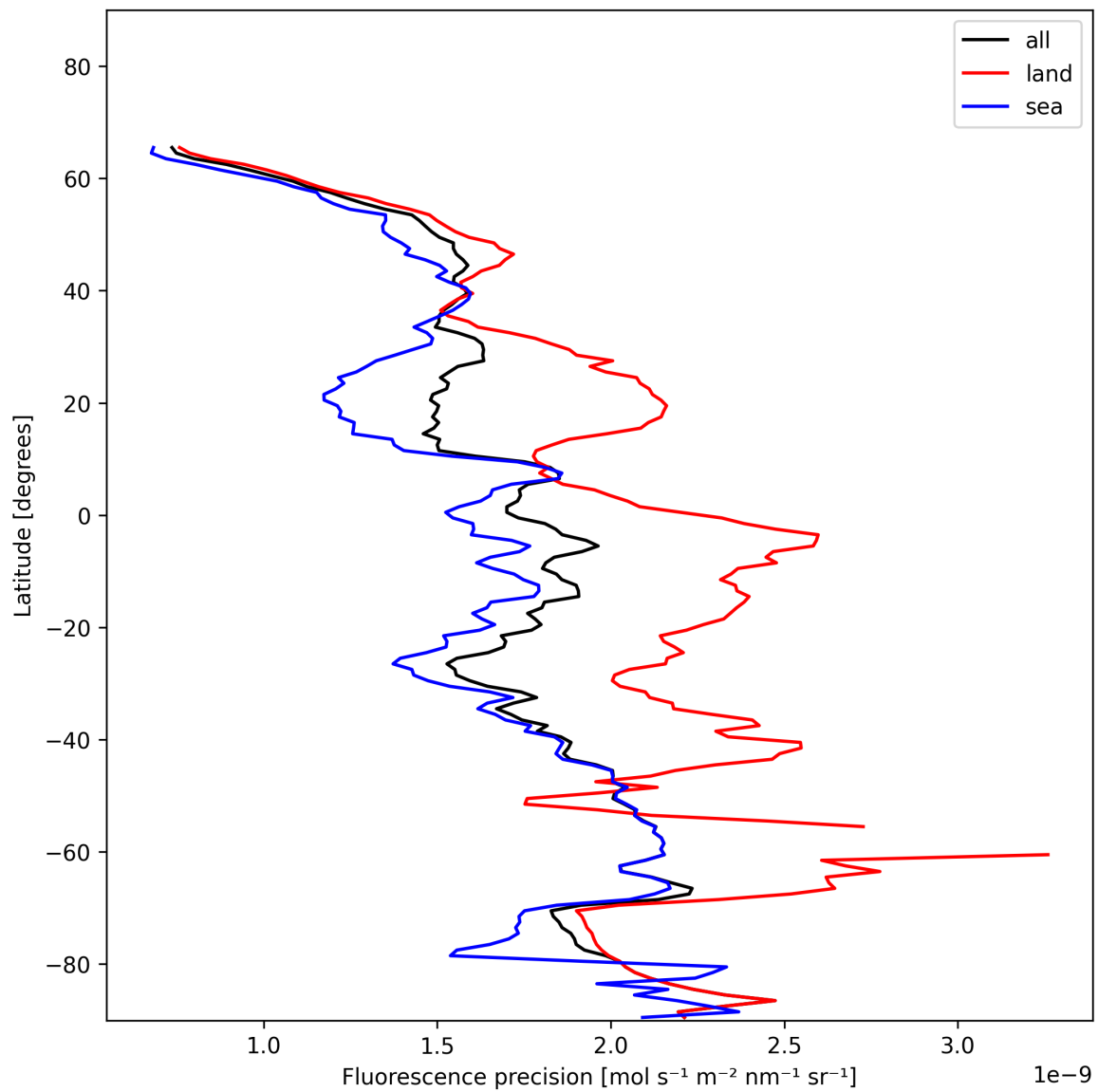
Figure 22: Zonal average of “Fluorescence precision” for 2024-12-06 to 2024-12-07.
