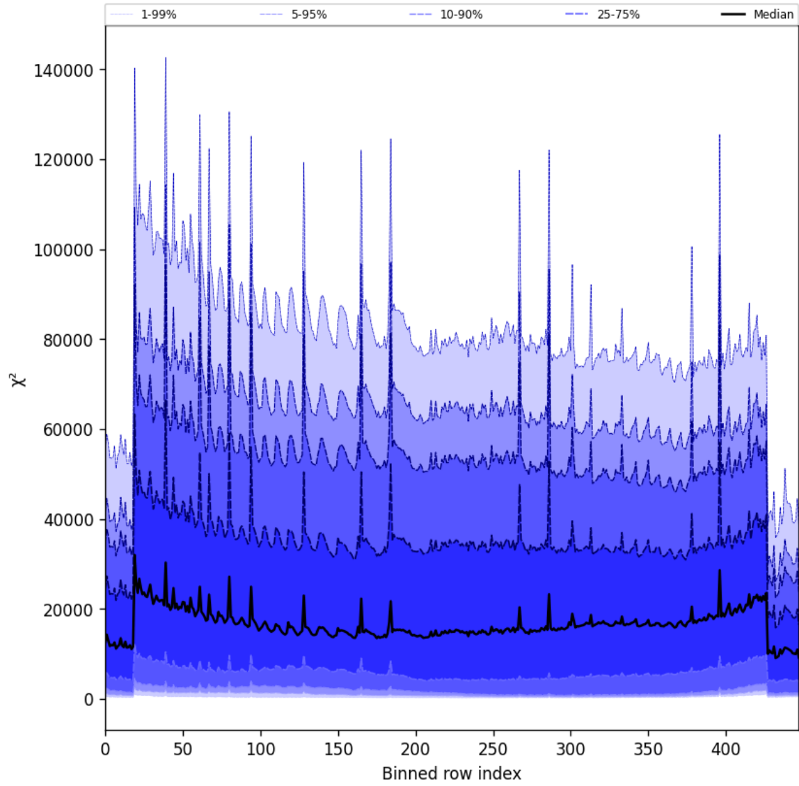
Figure 53: Along track statistics of “ \chi^2 ” for 2024-12-06 to 2024-12-07
