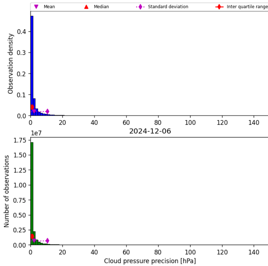
Figure 29: Histogram of “Cloud pressure precision” for 2024-12-06 to 2024-12-07
