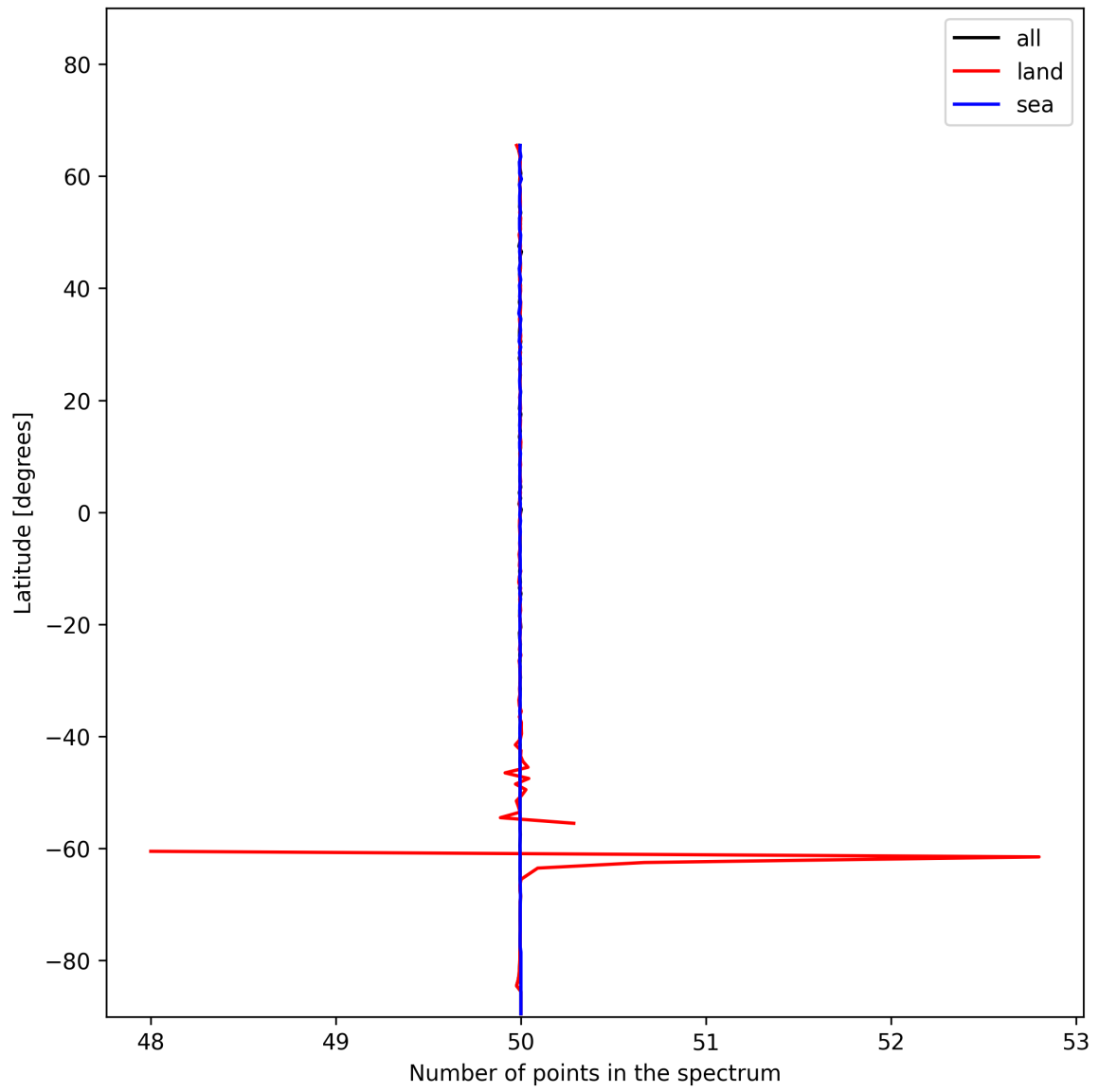
Figure 25: Zonal average of “Number of points in the spectrum” for 2024-12-06 to 2024-12-07.
