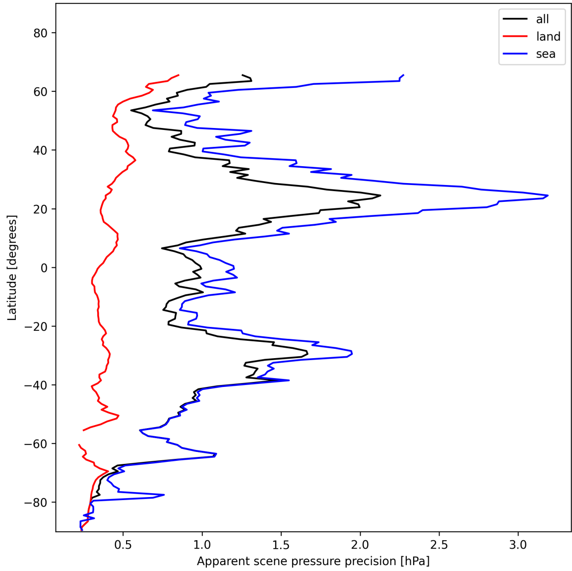
Figure 18: Zonal average of “Apparent scene pressure precision” for 2024-12-06 to 2024-12-07.
