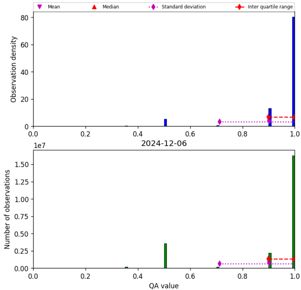
Figure 27: Histogram of “QA value” for 2024-12-06 to 2024-12-07
