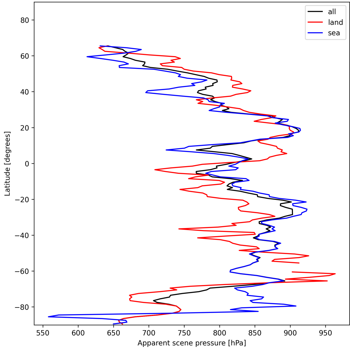
Figure 17: Zonal average of “Apparent scene pressure” for 2024-12-06 to 2024-12-07.
