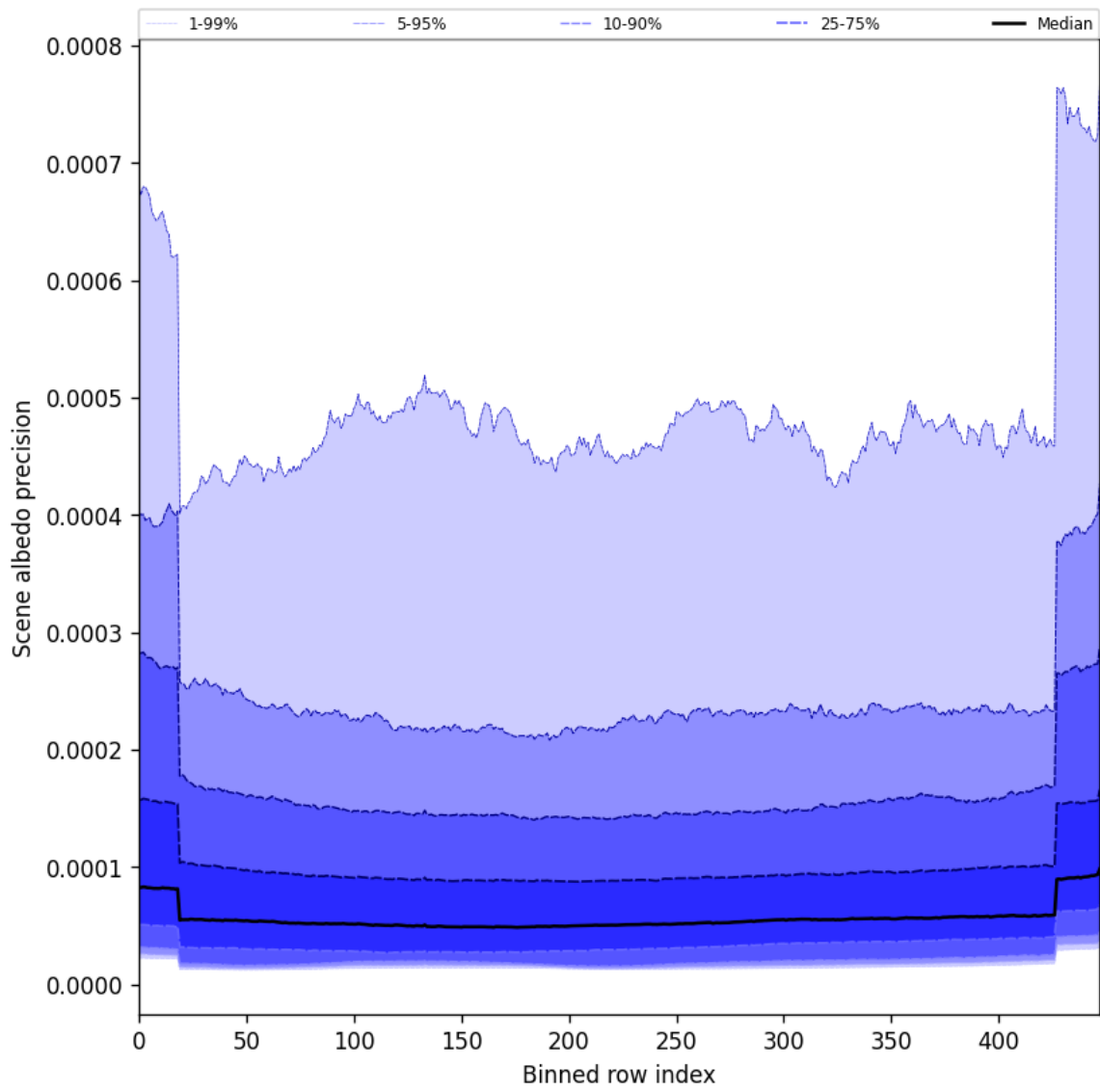
Figure 50: Along track statistics of “Scene albedo precision” for 2024-12-06 to 2024-12-07
