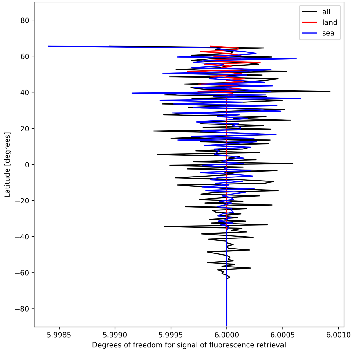
Figure 24: Zonal average of “Degrees of freedom for signal of fluorescence retrieval” for 2024-12-06 to 2024-12-07.
