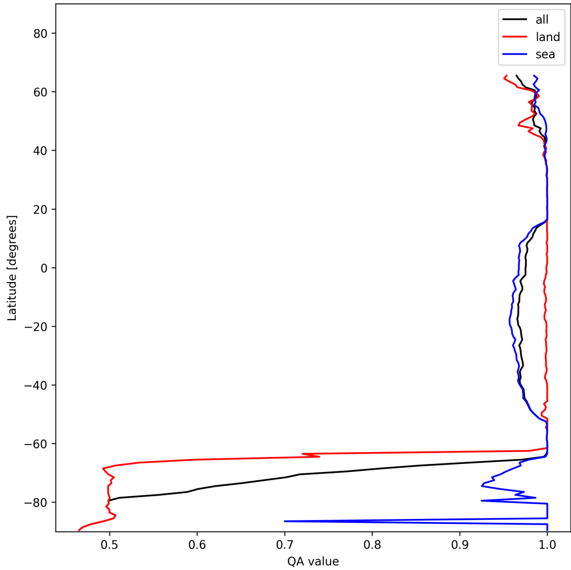
Figure 10: Zonal average of “QA value” for 2024-12-06 to 2024-12-07.
