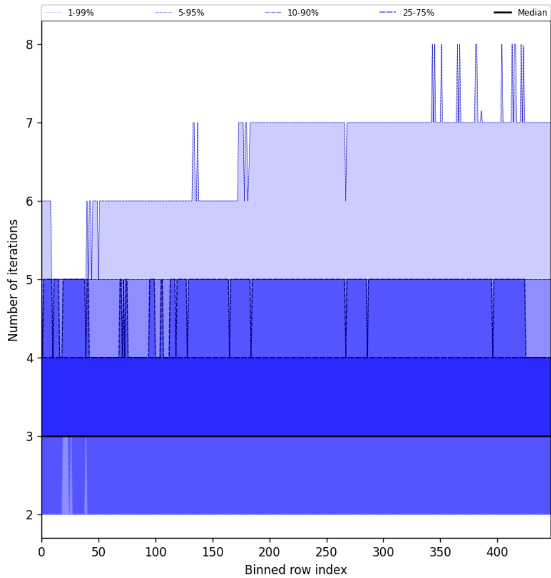
Figure 54: Along track statistics of “Number of iterations” for 2024-12-06 to 2024-12-07
