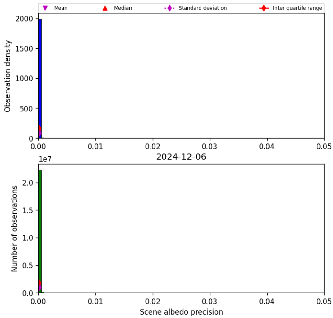
Figure 33: Histogram of “Scene albedo precision” for 2024-12-06 to 2024-12-07
