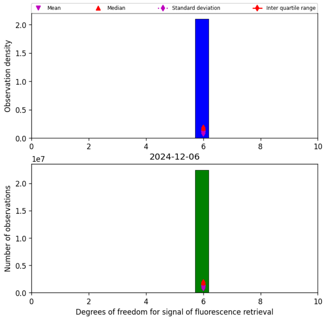
Figure 41: Histogram of “Degrees of freedom for signal of fluorescence retrieval” for 2024-12-06 to 2024-12-07
