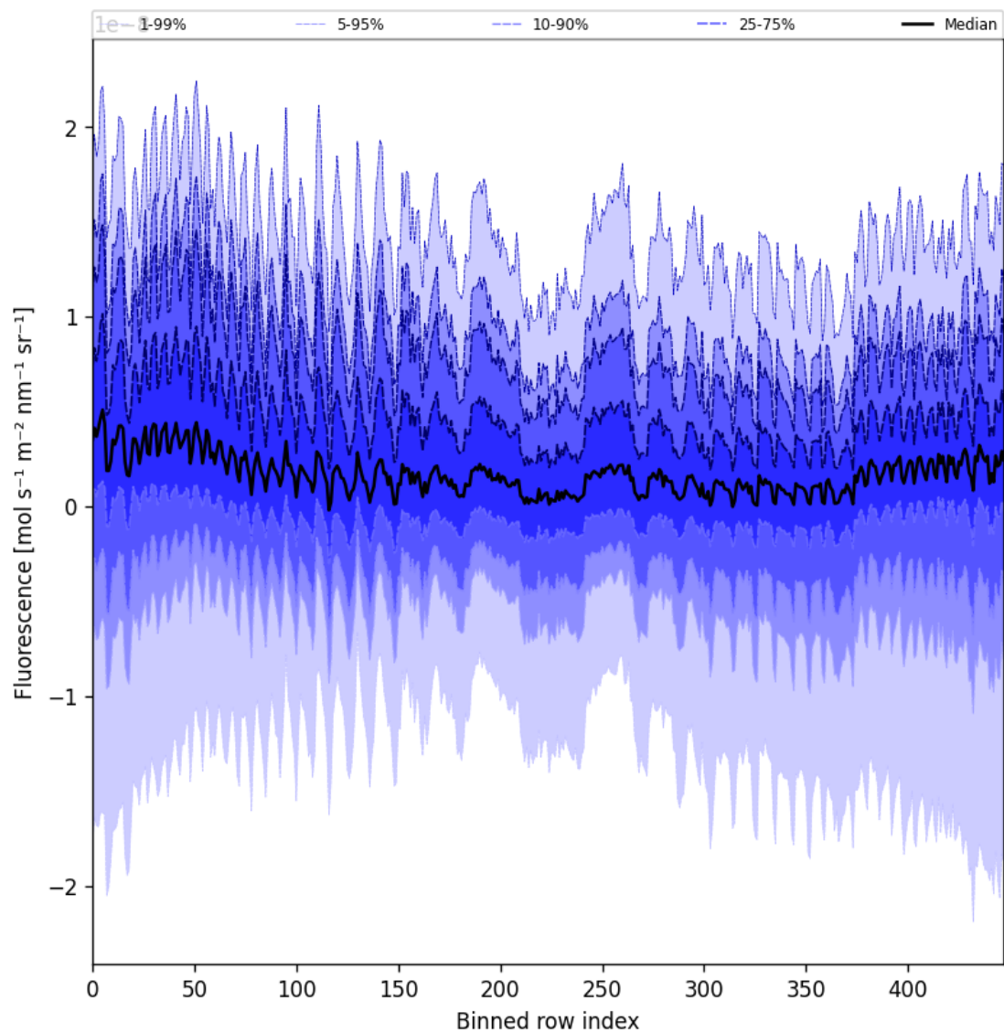
Figure 55: Along track statistics of “Fluorescence” for 2024-12-06 to 2024-12-07
