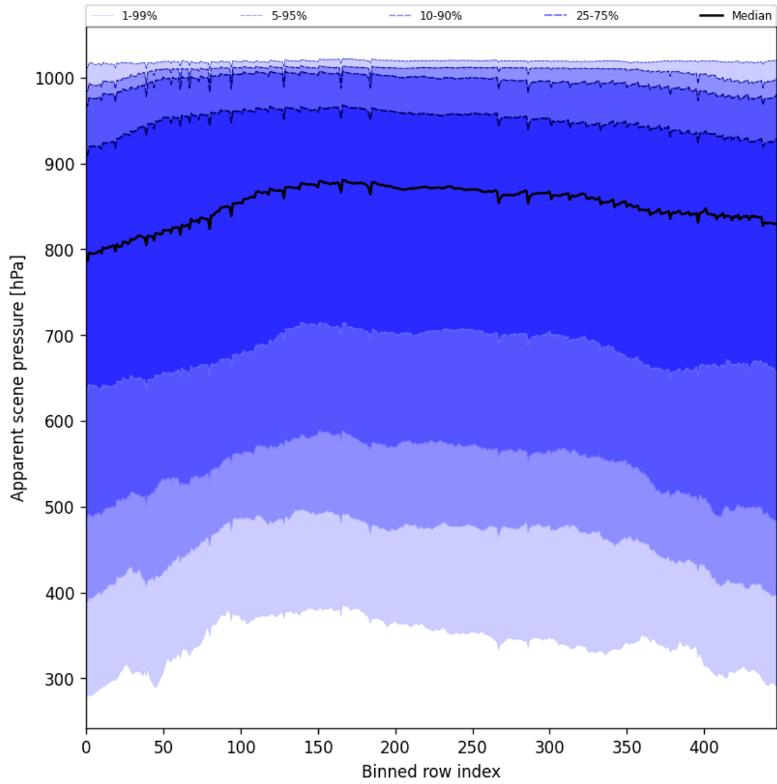
Figure 51: Along track statistics of “Apparent scene pressure” for 2024-12-06 to 2024-12-07
