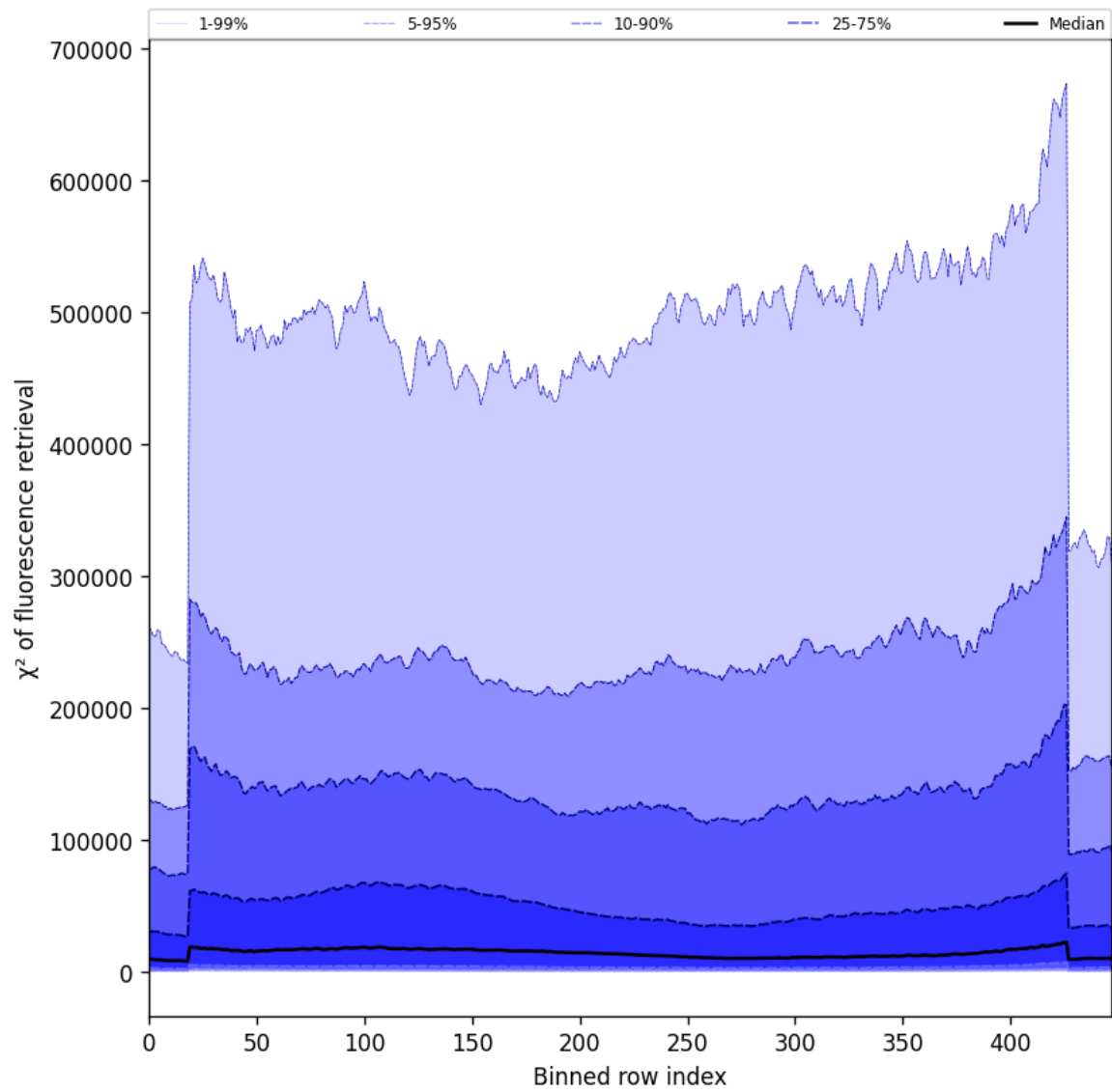
Figure 57: Along track statistics of “ \chi^2 of fluorescence retrieval” for 2024-12-06 to 2024-12-07
