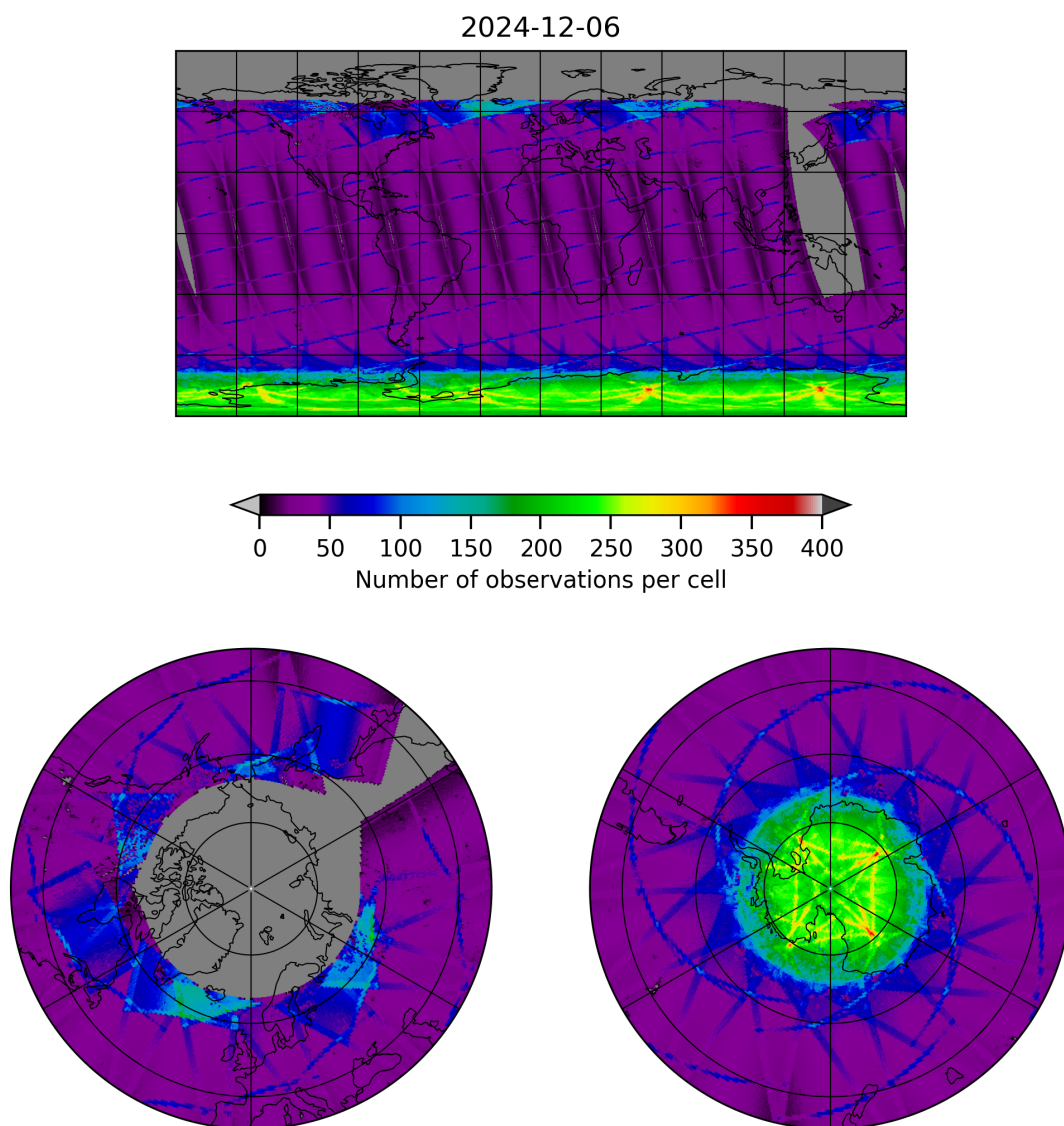
Figure 9: Map of the number of observations for 2024-12-06 to 2024-12-07
