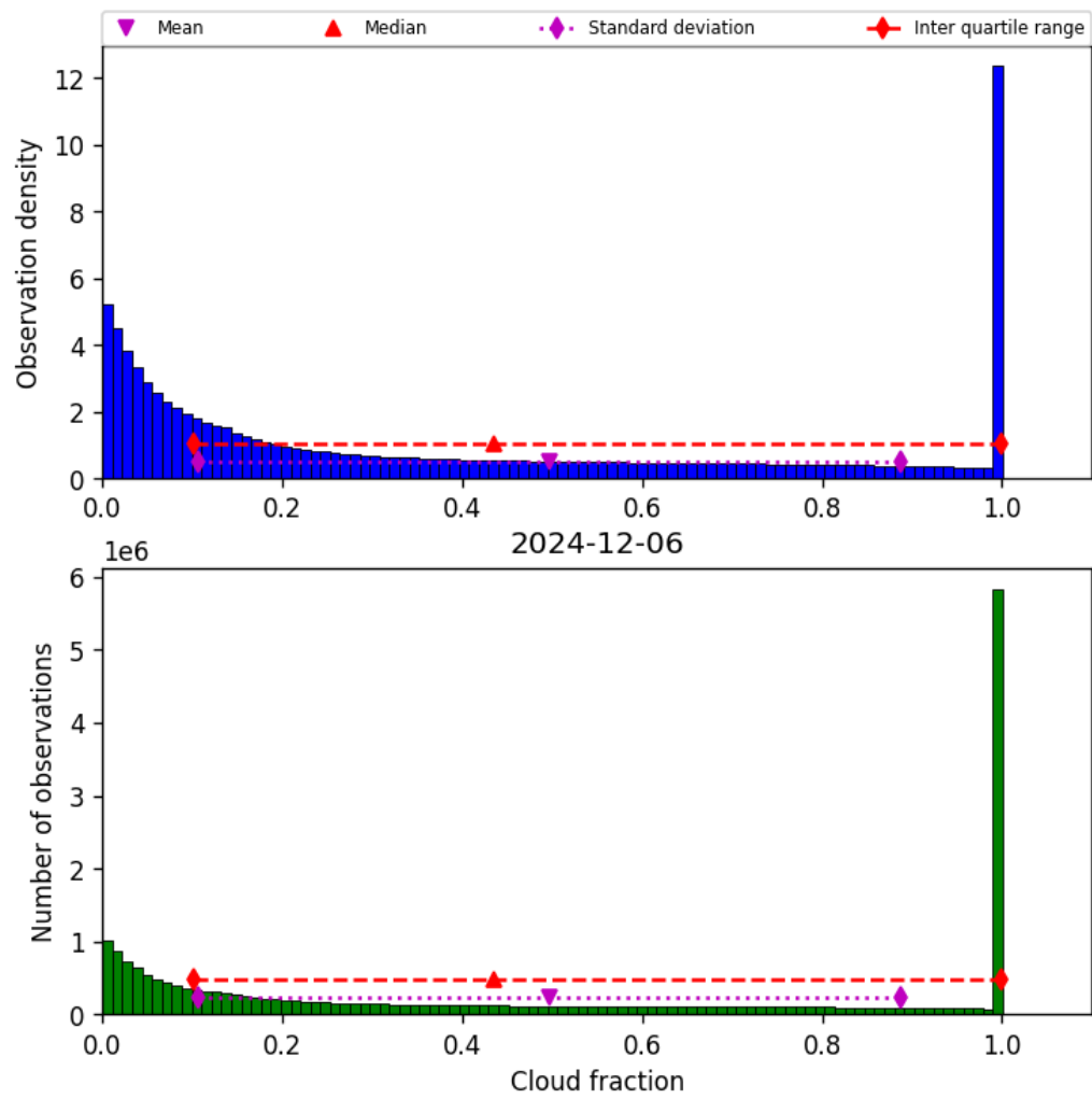
Figure 30: Histogram of “Cloud fraction” for 2024-12-06 to 2024-12-07
