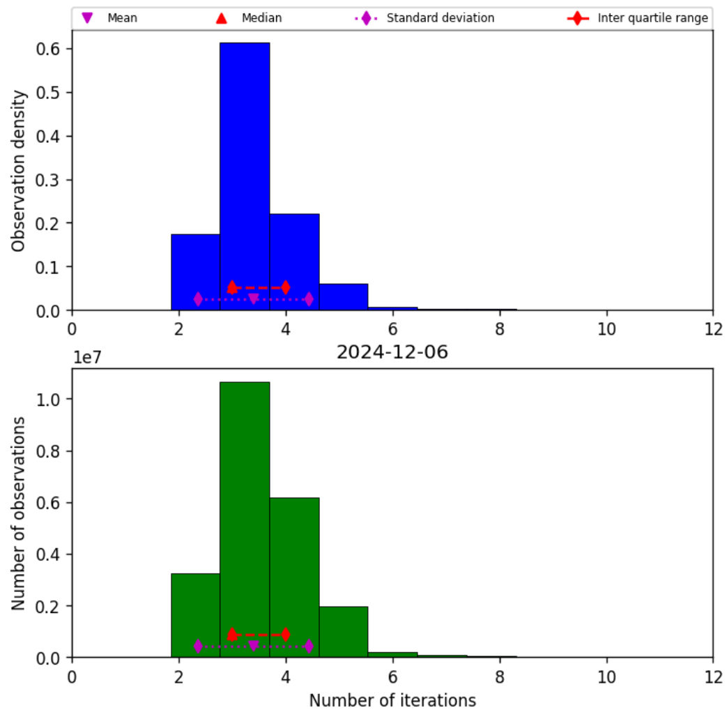
Figure 37: Histogram of “Number of iterations” for 2024-12-06 to 2024-12-07
