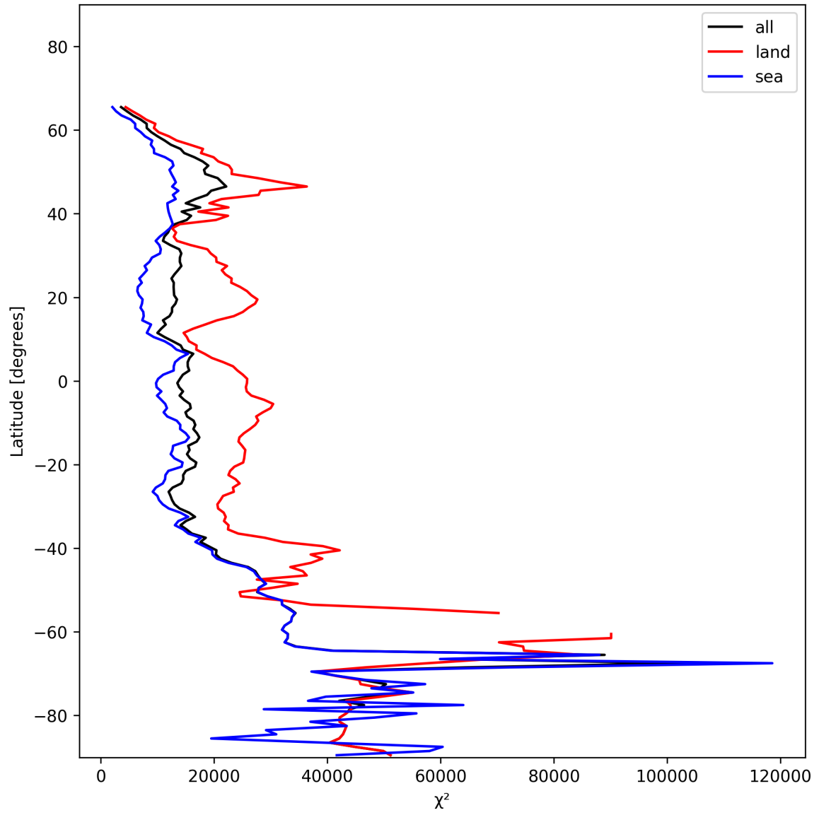
Figure 19: Zonal average of “ \chi^2 ” for 2024-12-06 to 2024-12-07.
