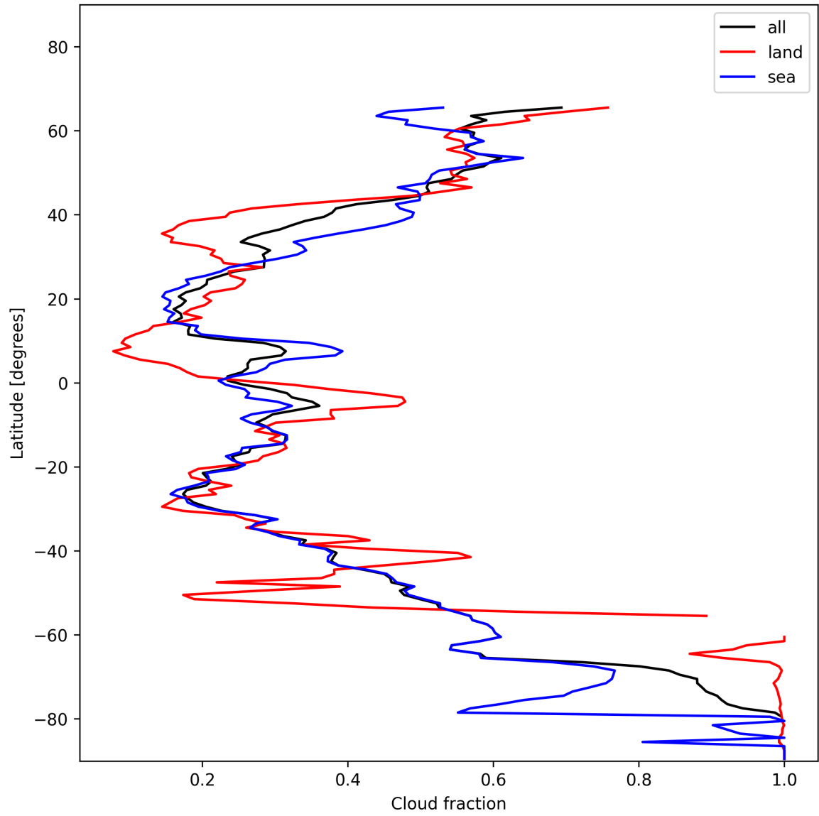
Figure 13: Zonal average of “Cloud fraction” for 2024-12-06 to 2024-12-07.
