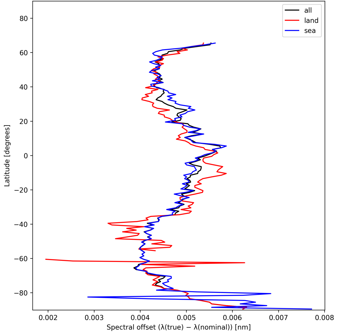
Figure 26: Zonal average of “Spectral offset ( \lambda_{\text{true}} - \lambda_{\text{nominal}} )” for 2024-12-06 to 2024-12-07.
