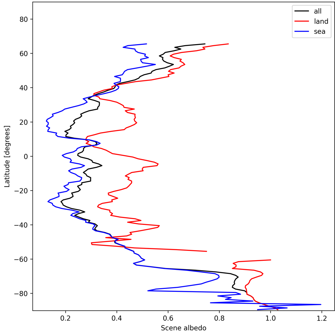
Figure 15: Zonal average of “Scene albedo” for 2024-12-06 to 2024-12-07.
