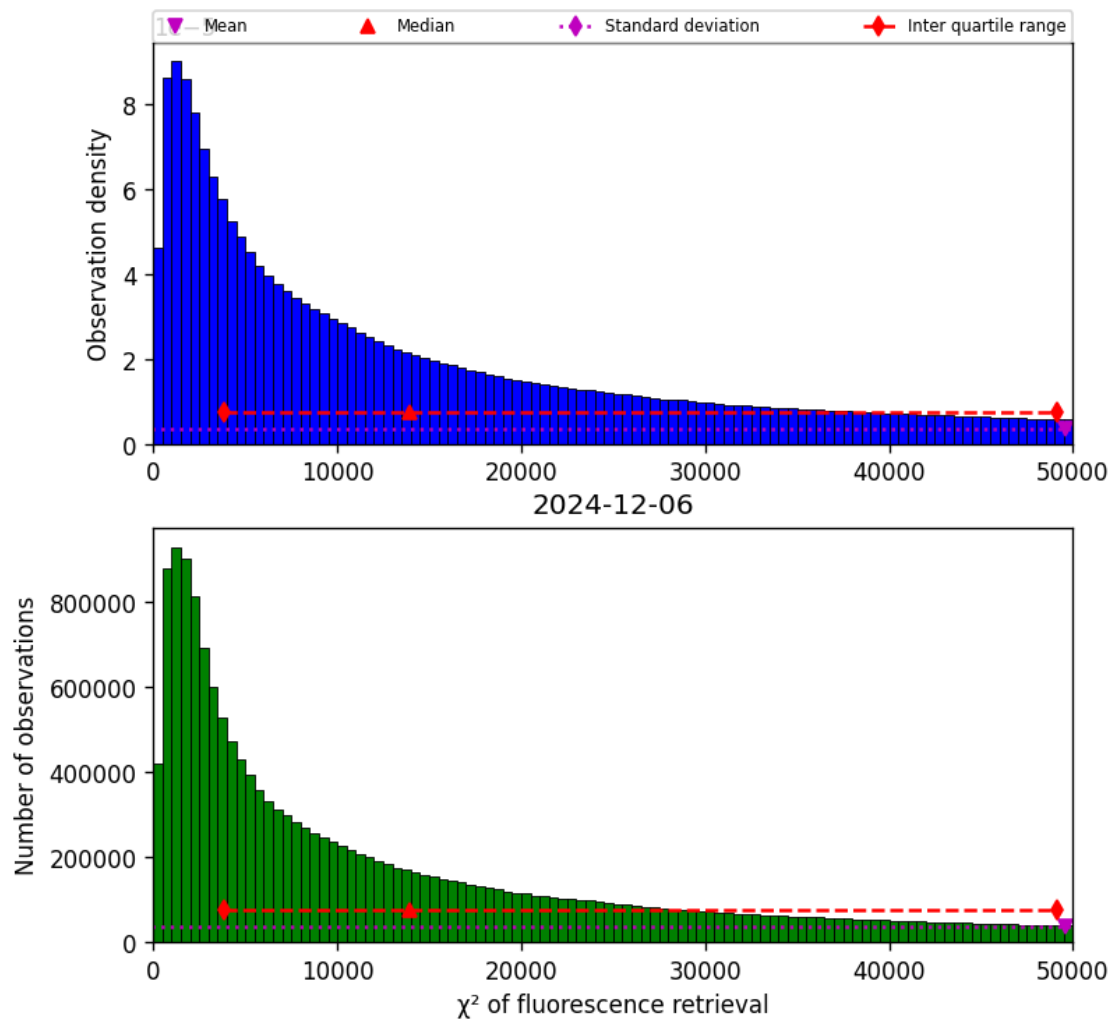
Figure 40: Histogram of “ \chi^2 of fluorescence retrieval” for 2024-12-06 to 2024-12-07
