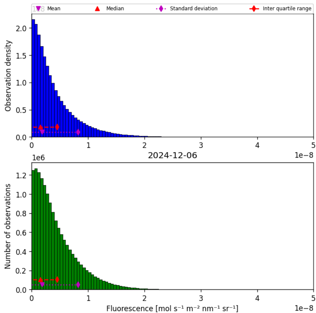
Figure 38: Histogram of “Fluorescence” for 2024-12-06 to 2024-12-07
