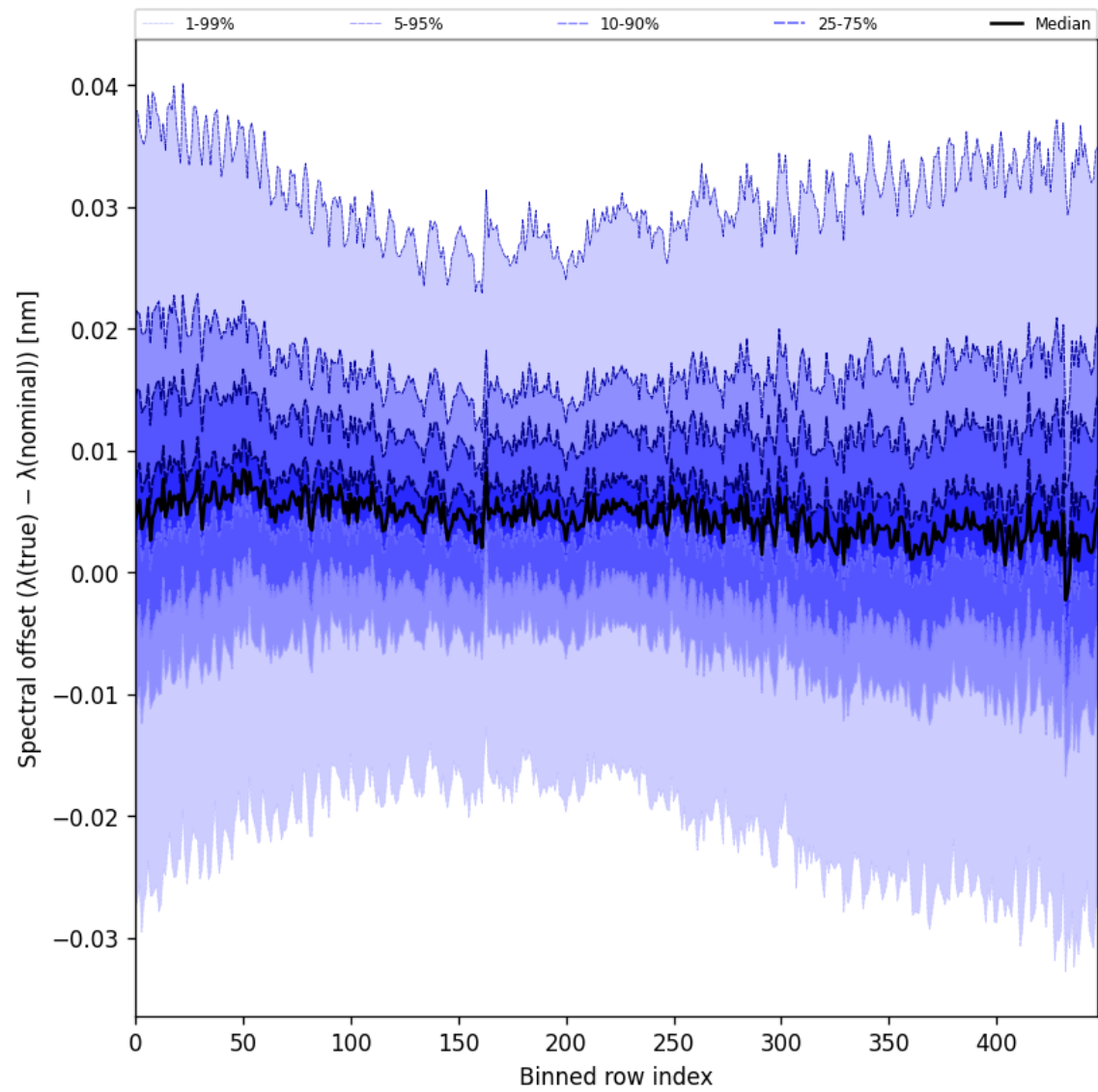
Figure 60: Along track statistics of “Spectral offset ( \lambda_{\text{true}} - \lambda_{\text{nominal}} )” for 2024-12-06 to 2024-12-07
