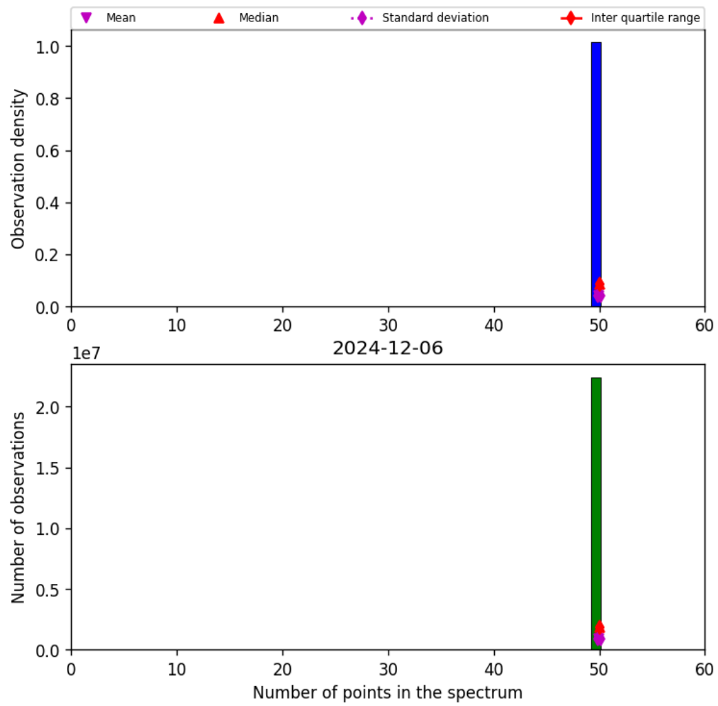
Figure 42: Histogram of “Number of points in the spectrum” for 2024-12-06 to 2024-12-07
