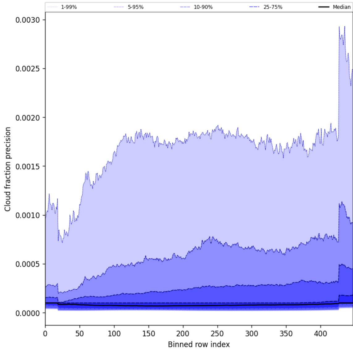
Figure 48: Along track statistics of “Cloud fraction precision” for 2024-12-06 to 2024-12-07
