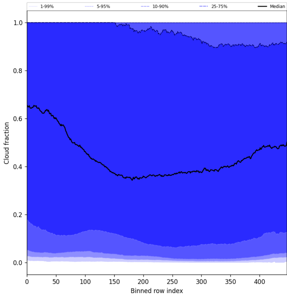
Figure 47: Along track statistics of “Cloud fraction” for 2024-12-06 to 2024-12-07
