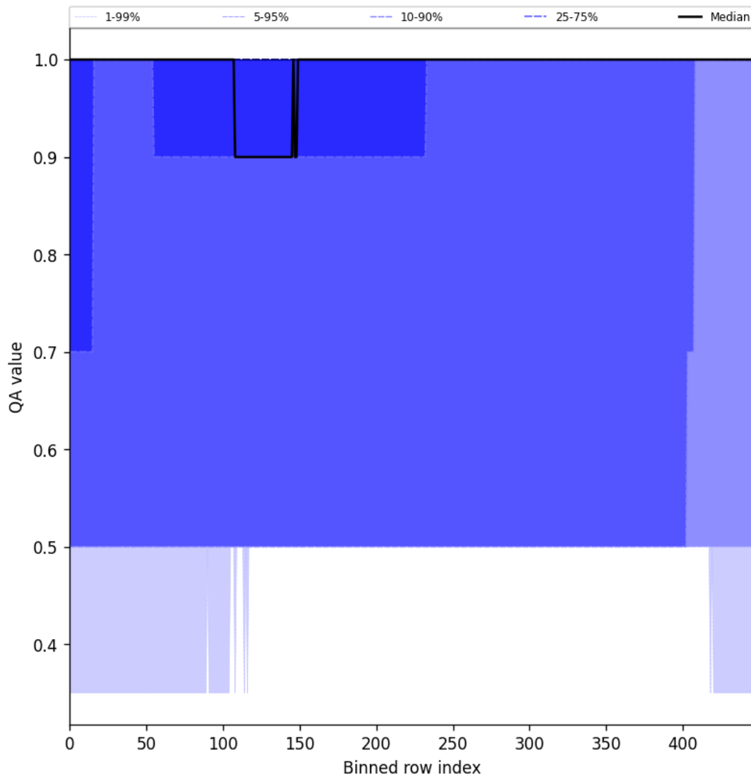
Figure 44: Along track statistics of “QA value” for 2024-12-06 to 2024-12-07
