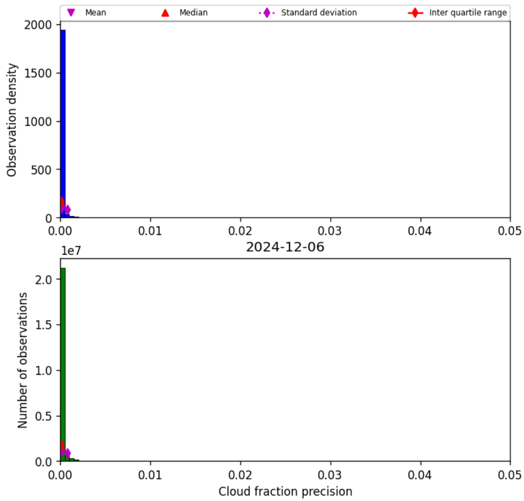
Figure 31: Histogram of “Cloud fraction precision” for 2024-12-06 to 2024-12-07
