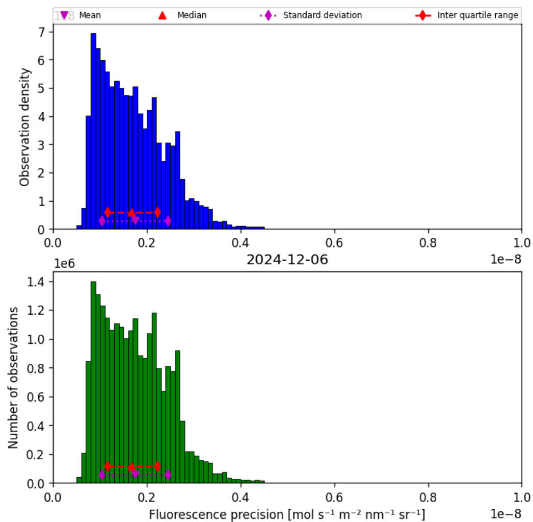
Figure 39: Histogram of “Fluorescence precision” for 2024-12-06 to 2024-12-07
