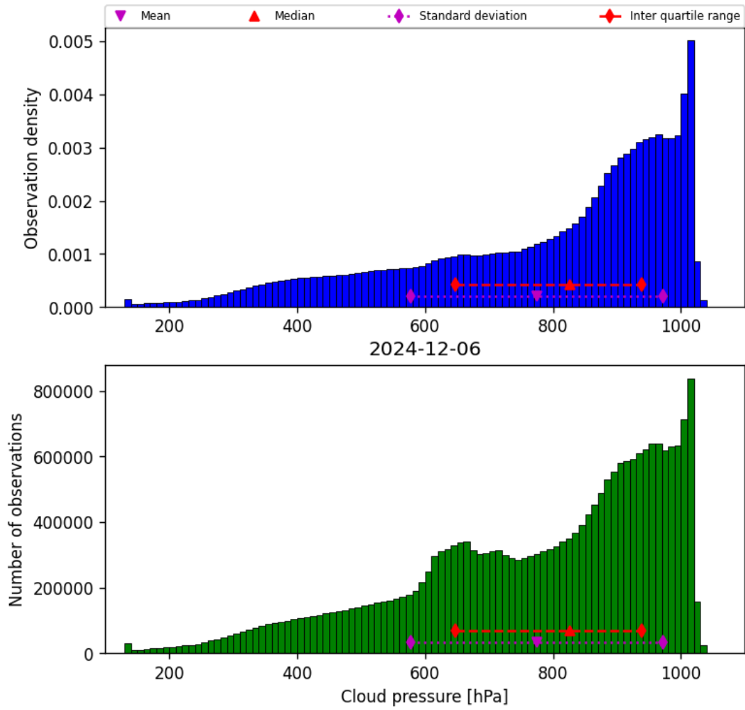
Figure 28: Histogram of “Cloud pressure” for 2024-12-06 to 2024-12-07
