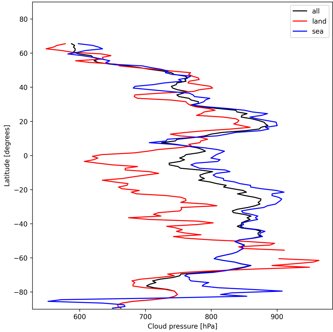
Figure 11: Zonal average of “Cloud pressure” for 2024-12-06 to 2024-12-07.
