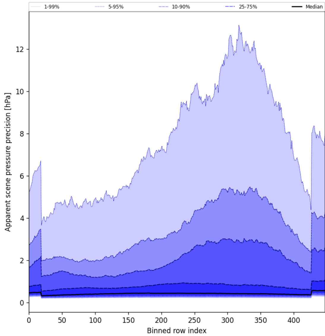
Figure 52: Along track statistics of “Apparent scene pressure precision” for 2024-12-06 to 2024-12-07
