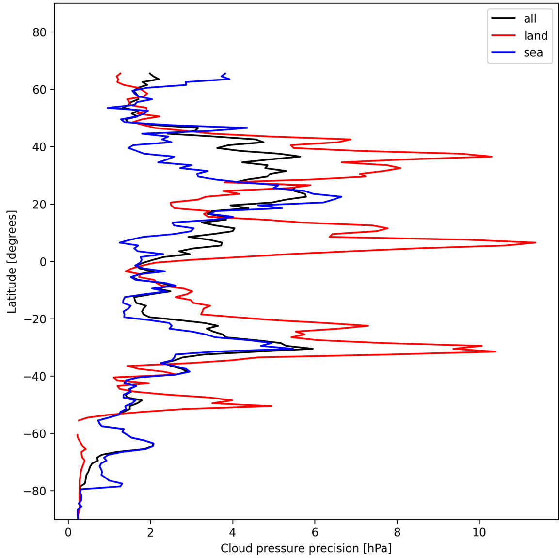
Figure 12: Zonal average of “Cloud pressure precision” for 2024-12-06 to 2024-12-07.
