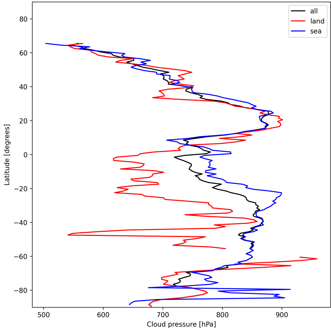
Figure 11: Zonal average of “Cloud pressure” for 2024-12-07 to 2024-12-08.
