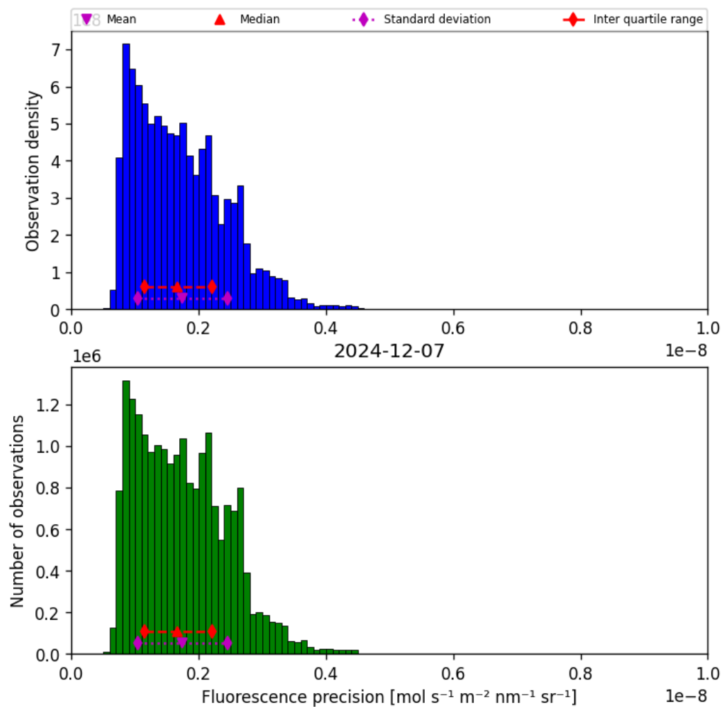
Figure 39: Histogram of “Fluorescence precision” for 2024-12-07 to 2024-12-08
