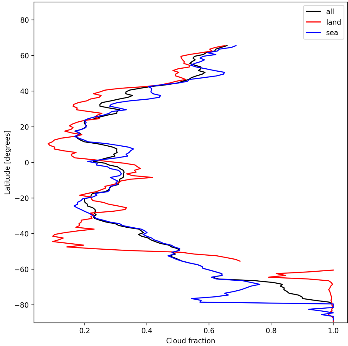
Figure 13: Zonal average of “Cloud fraction” for 2024-12-07 to 2024-12-08.
