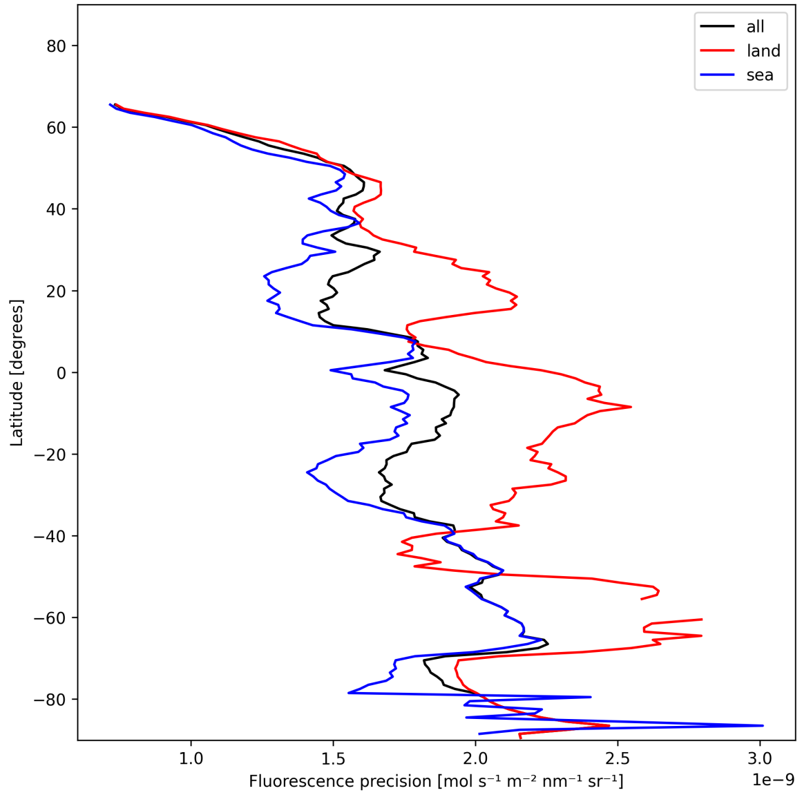
Figure 22: Zonal average of “Fluorescence precision” for 2024-12-07 to 2024-12-08.
