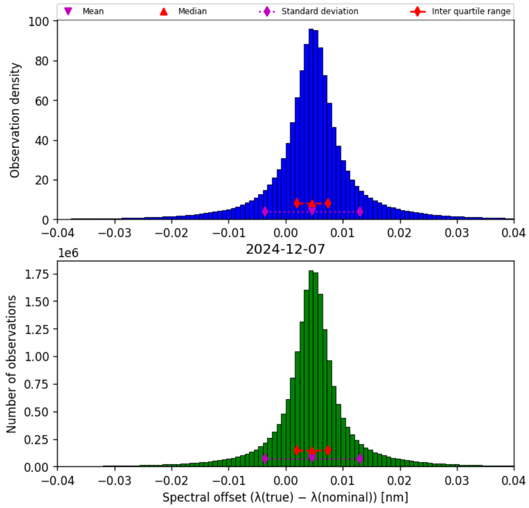
Figure 43: Histogram of “Spectral offset ( \lambda_{\text{true}} - \lambda_{\text{nominal}} )” for 2024-12-07 to 2024-12-08
