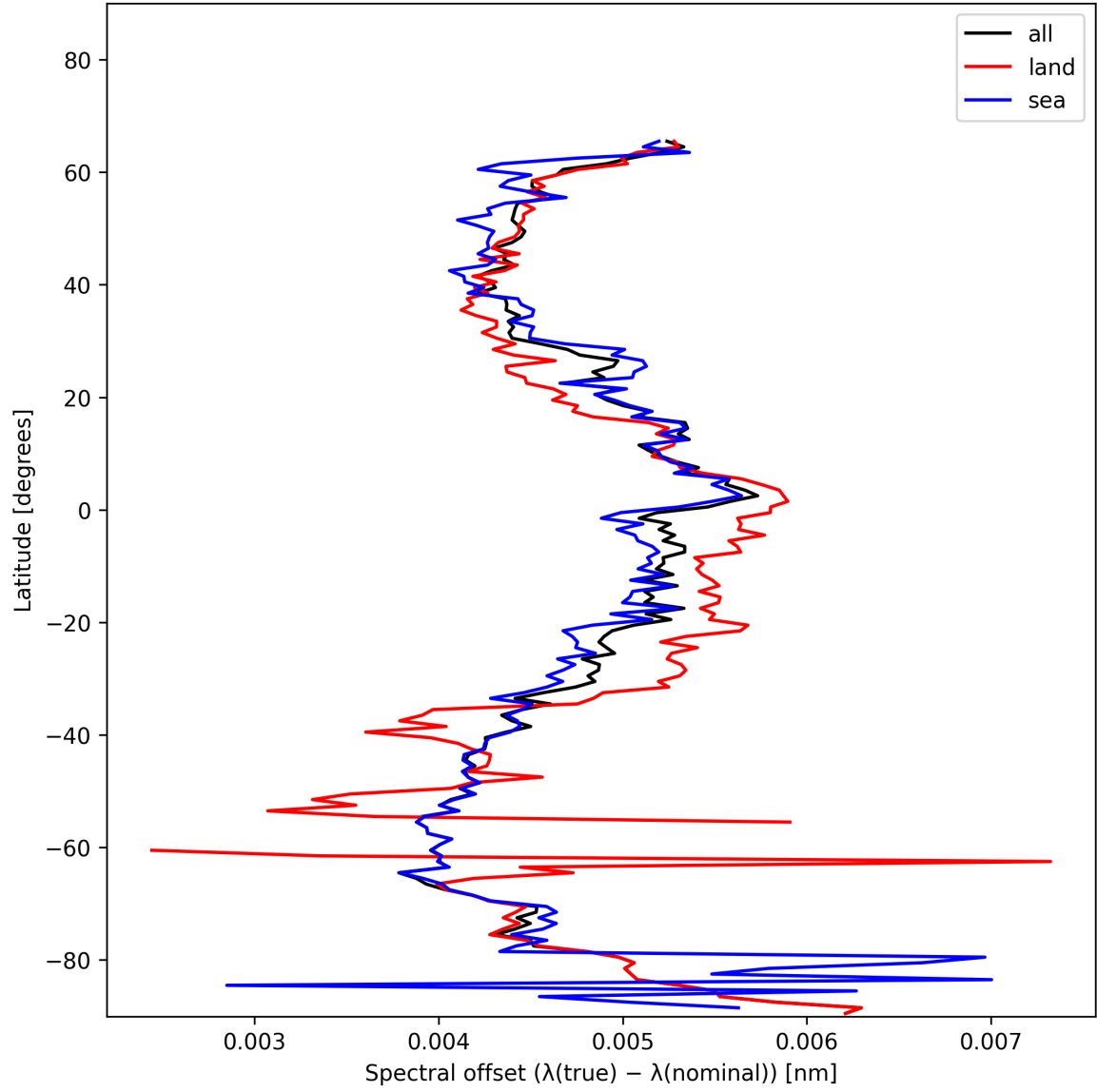
Figure 26: Zonal average of “Spectral offset ( \lambda_{\text{true}} - \lambda_{\text{nominal}} )” for 2024-12-07 to 2024-12-08.
