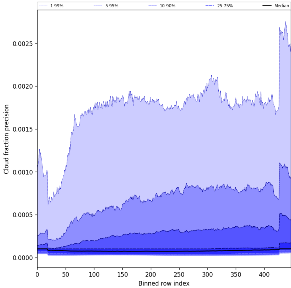
Figure 48: Along track statistics of “Cloud fraction precision” for 2024-12-07 to 2024-12-08
