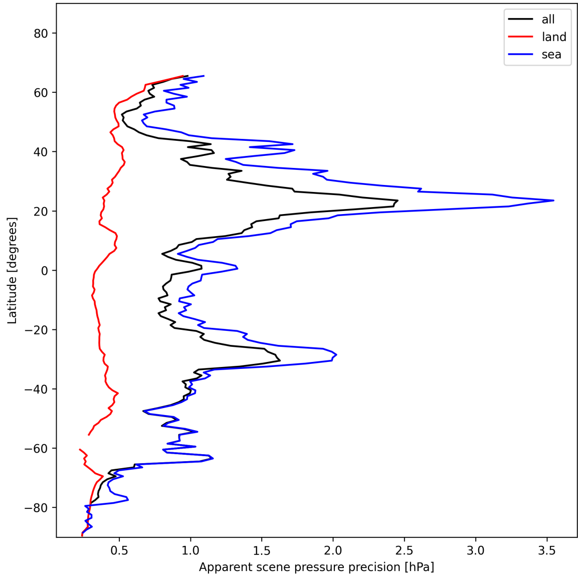
Figure 18: Zonal average of “Apparent scene pressure precision” for 2024-12-07 to 2024-12-08.
