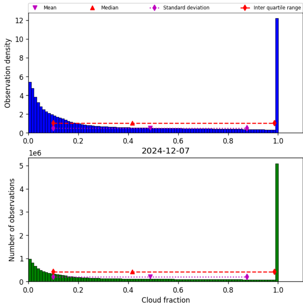
Figure 30: Histogram of “Cloud fraction” for 2024-12-07 to 2024-12-08
