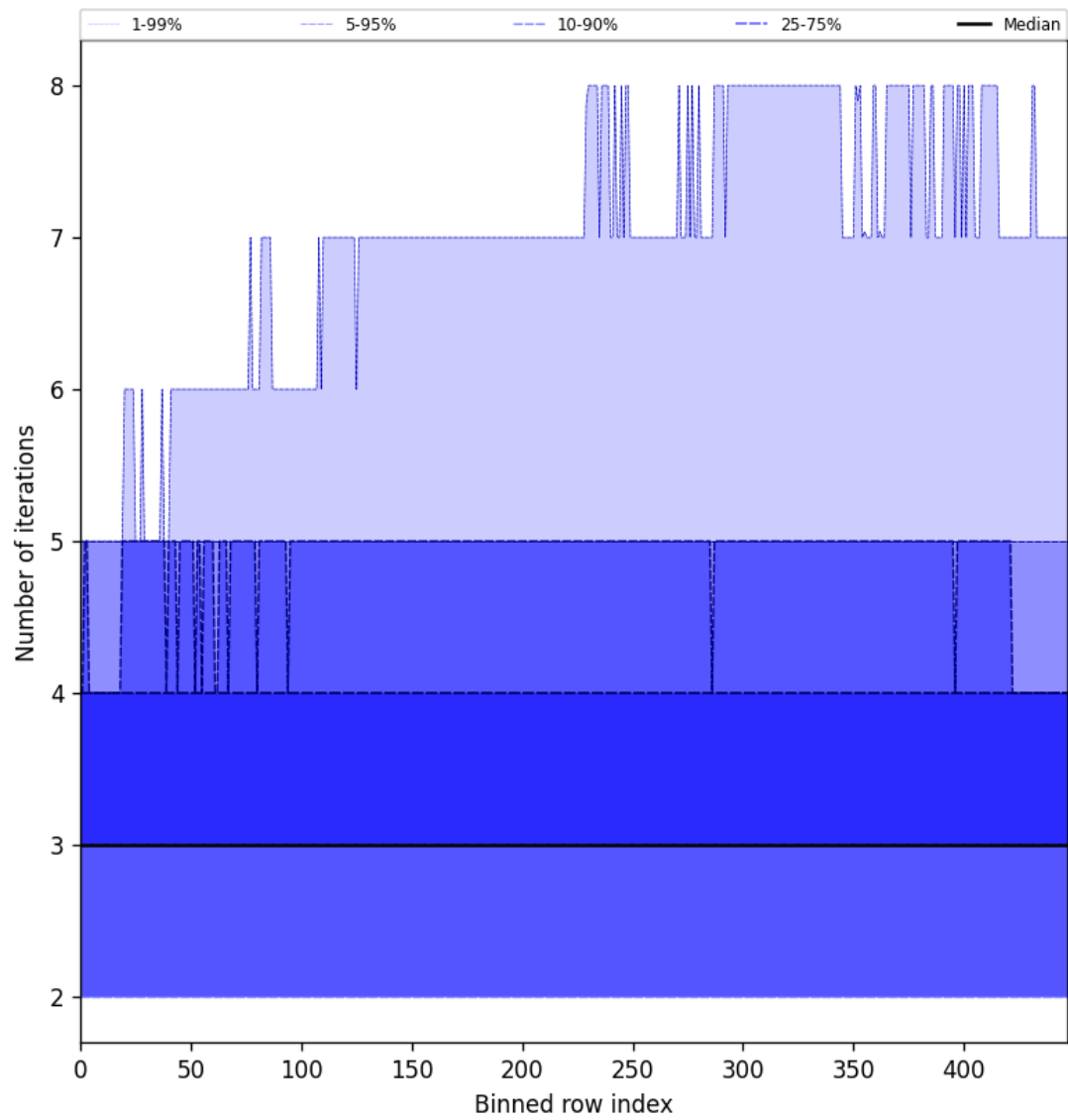
Figure 54: Along track statistics of “Number of iterations” for 2024-12-07 to 2024-12-08
