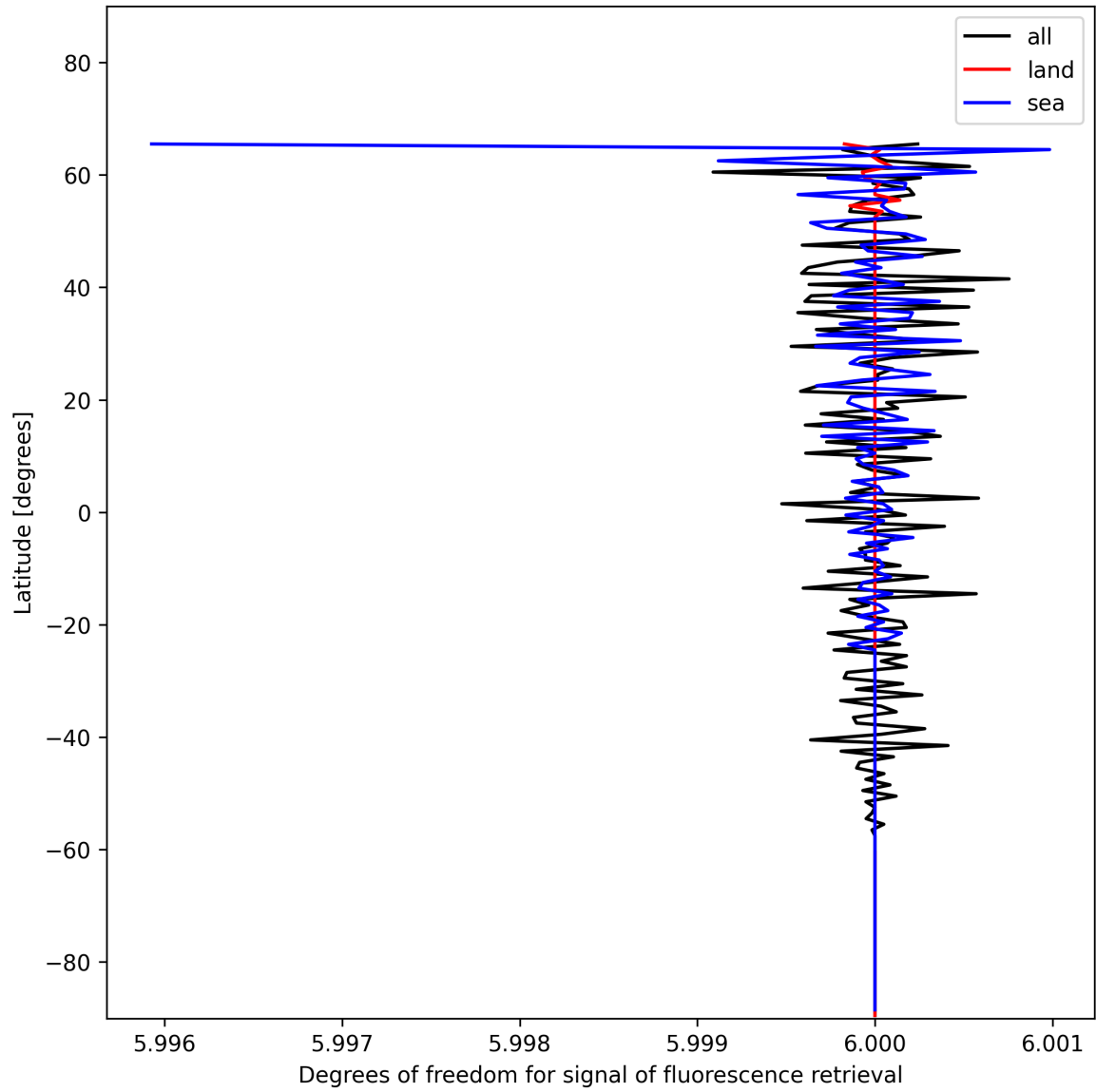
Figure 24: Zonal average of “Degrees of freedom for signal of fluorescence retrieval” for 2024-12-07 to 2024-12-08.
