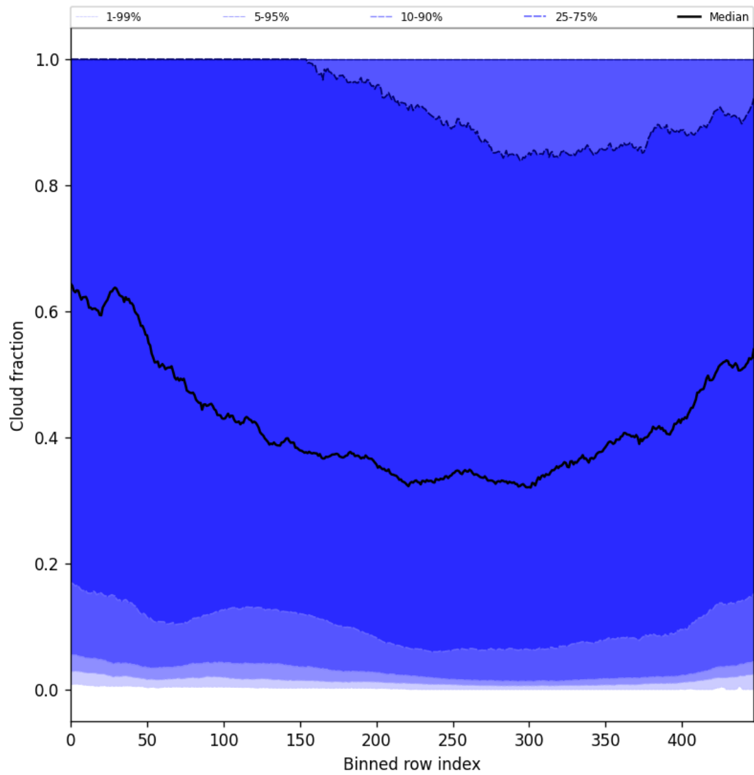
Figure 47: Along track statistics of “Cloud fraction” for 2024-12-07 to 2024-12-08
