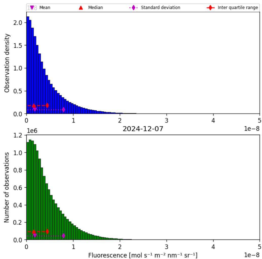
Figure 38: Histogram of “Fluorescence” for 2024-12-07 to 2024-12-08
