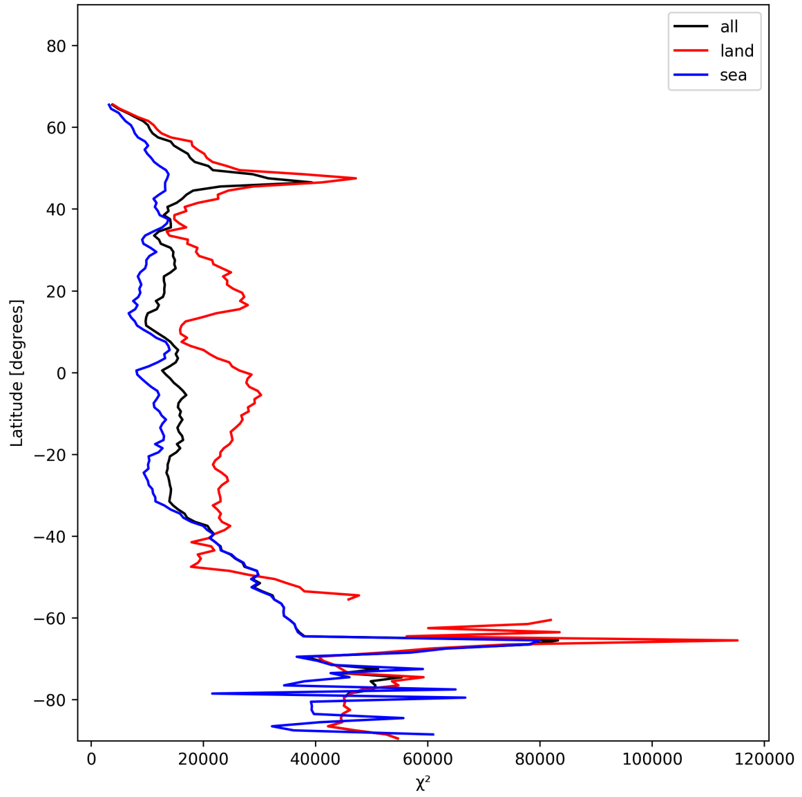
Figure 19: Zonal average of “ \chi^2 ” for 2024-12-07 to 2024-12-08.
