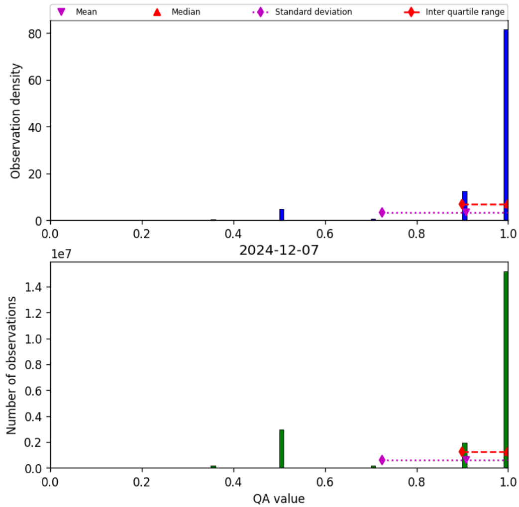
Figure 27: Histogram of “QA value” for 2024-12-07 to 2024-12-08
