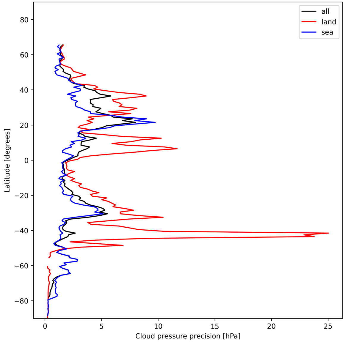
Figure 12: Zonal average of “Cloud pressure precision” for 2024-12-07 to 2024-12-08.
