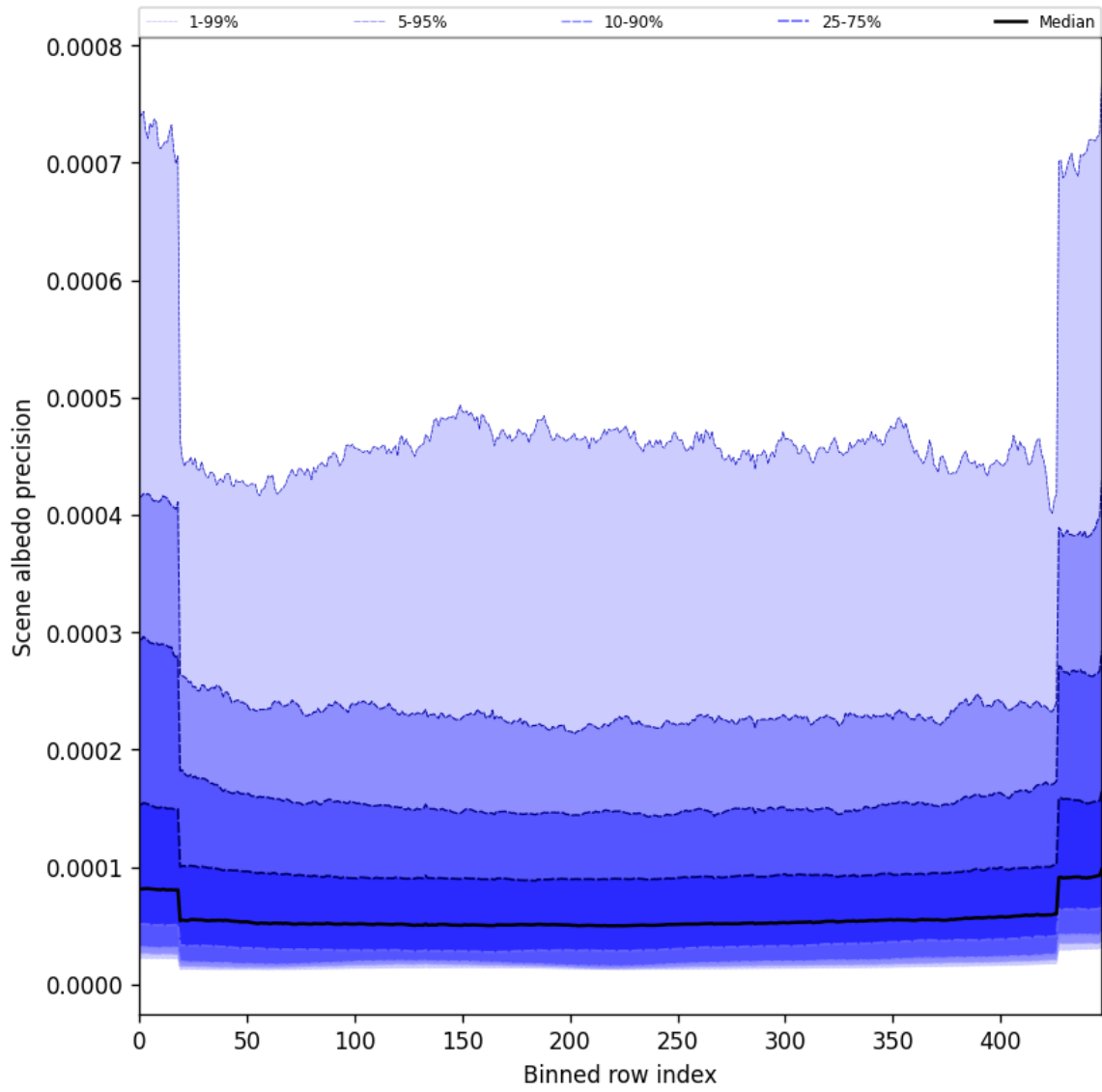
Figure 50: Along track statistics of “Scene albedo precision” for 2024-12-07 to 2024-12-08
