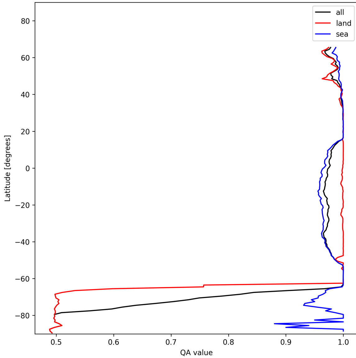
Figure 10: Zonal average of “QA value” for 2024-12-07 to 2024-12-08.
