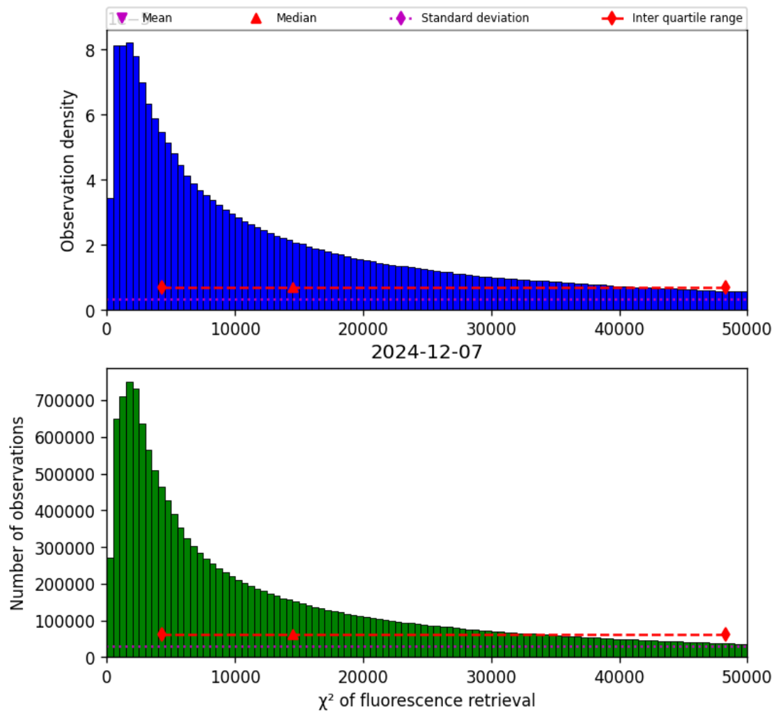
Figure 40: Histogram of “ \chi^2 of fluorescence retrieval” for 2024-12-07 to 2024-12-08
