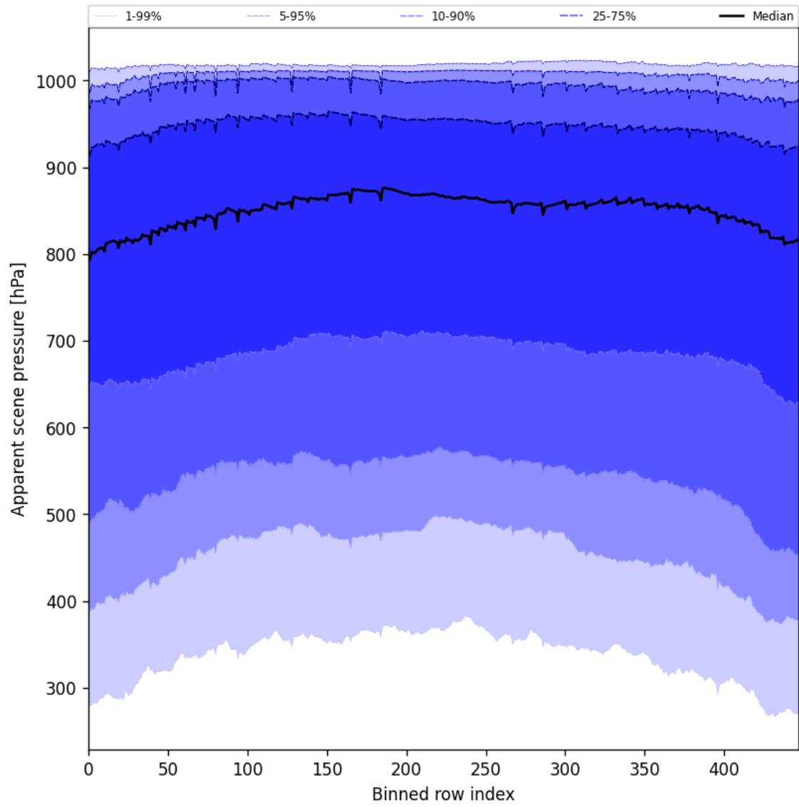
Figure 51: Along track statistics of “Apparent scene pressure” for 2024-12-07 to 2024-12-08
