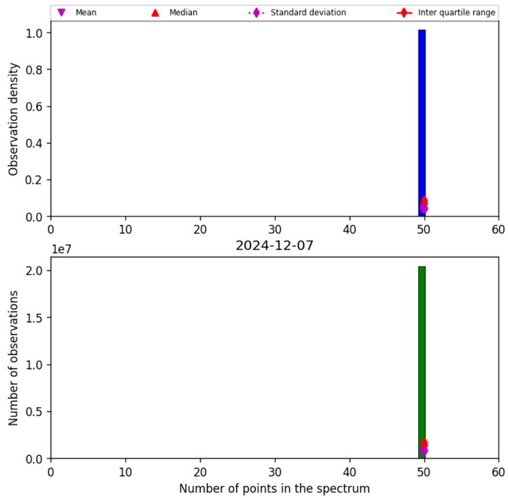
Figure 42: Histogram of “Number of points in the spectrum” for 2024-12-07 to 2024-12-08
