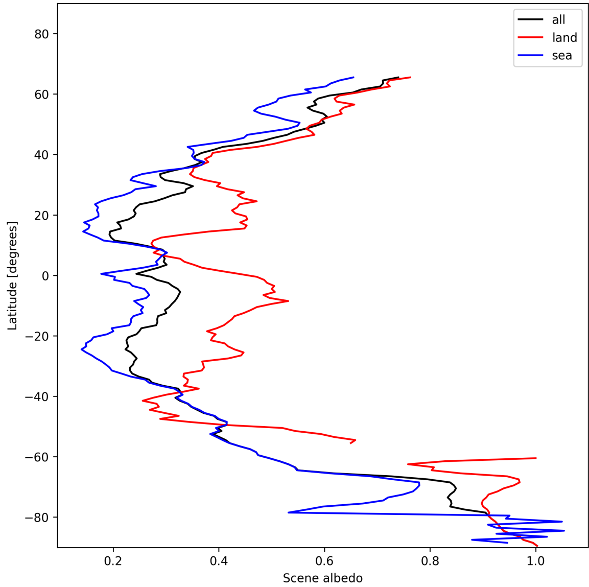
Figure 15: Zonal average of “Scene albedo” for 2024-12-07 to 2024-12-08.
