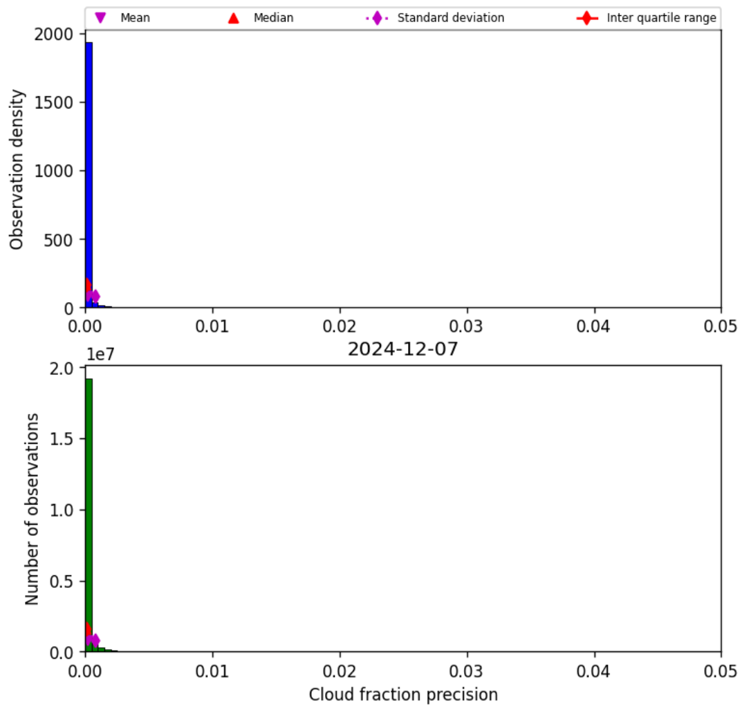
Figure 31: Histogram of “Cloud fraction precision” for 2024-12-07 to 2024-12-08
