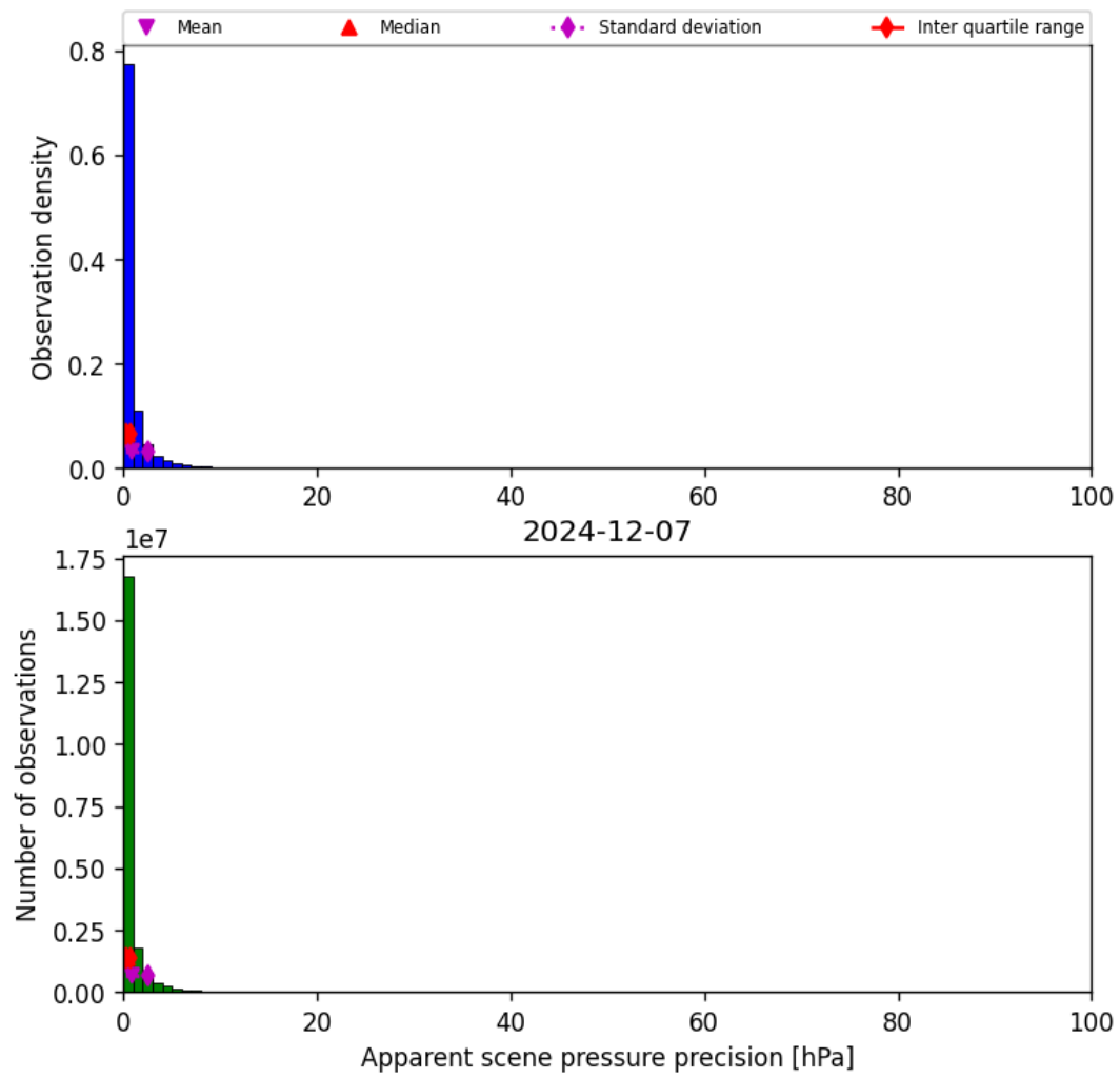
Figure 35: Histogram of “Apparent scene pressure precision” for 2024-12-07 to 2024-12-08
