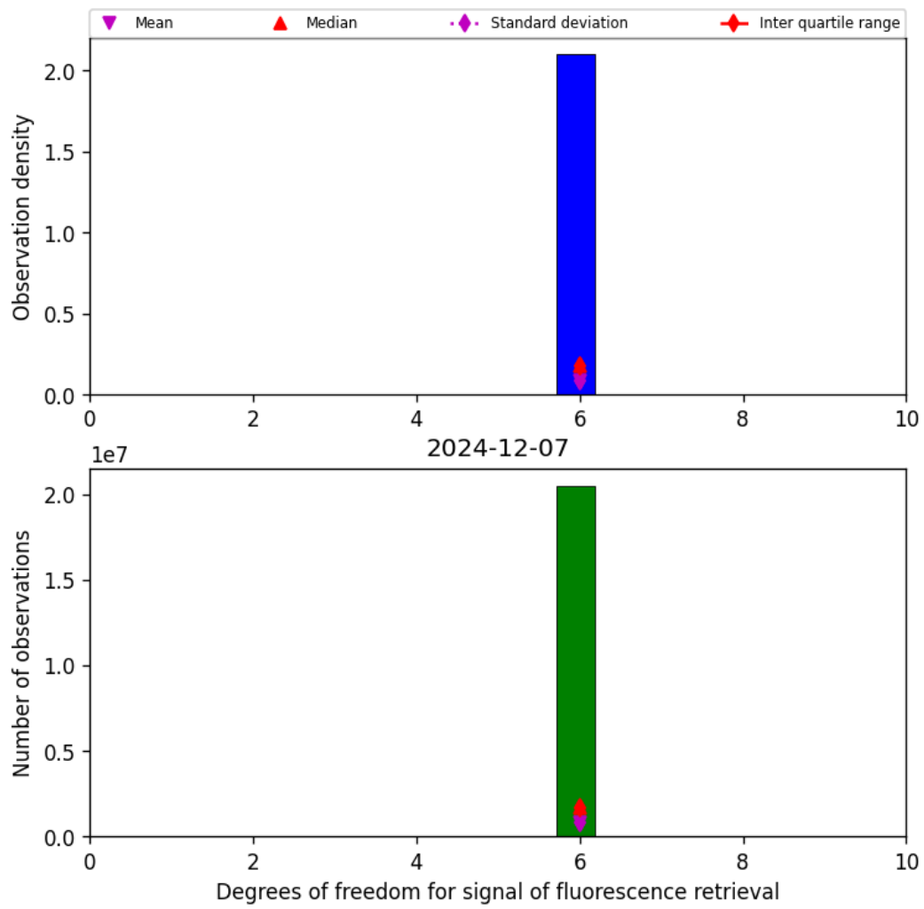
Figure 41: Histogram of “Degrees of freedom for signal of fluorescence retrieval” for 2024-12-07 to 2024-12-08
