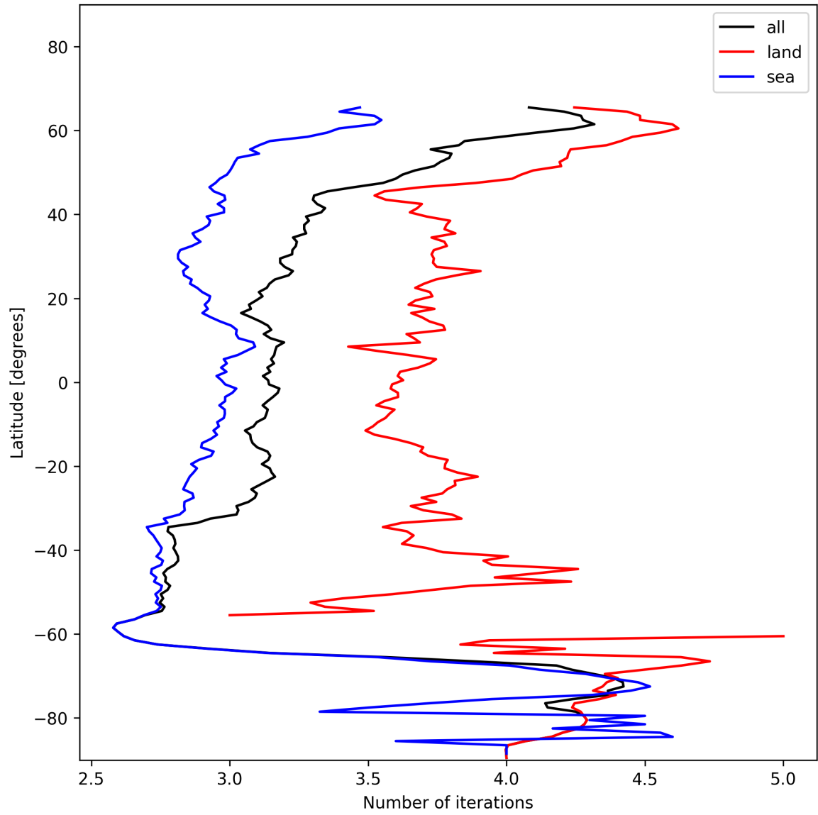
Figure 20: Zonal average of “Number of iterations” for 2024-12-07 to 2024-12-08.
