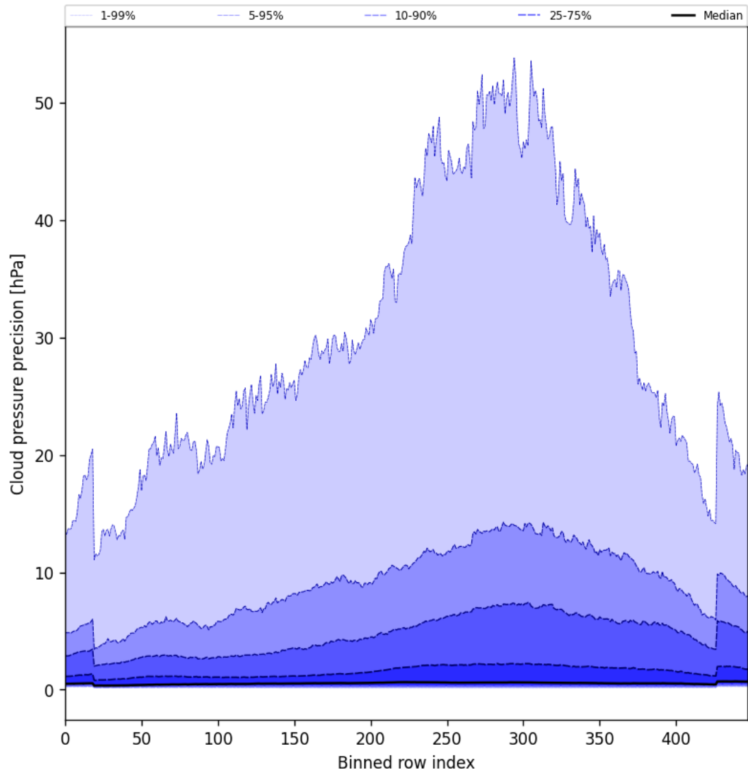
Figure 46: Along track statistics of “Cloud pressure precision” for 2024-12-07 to 2024-12-08
