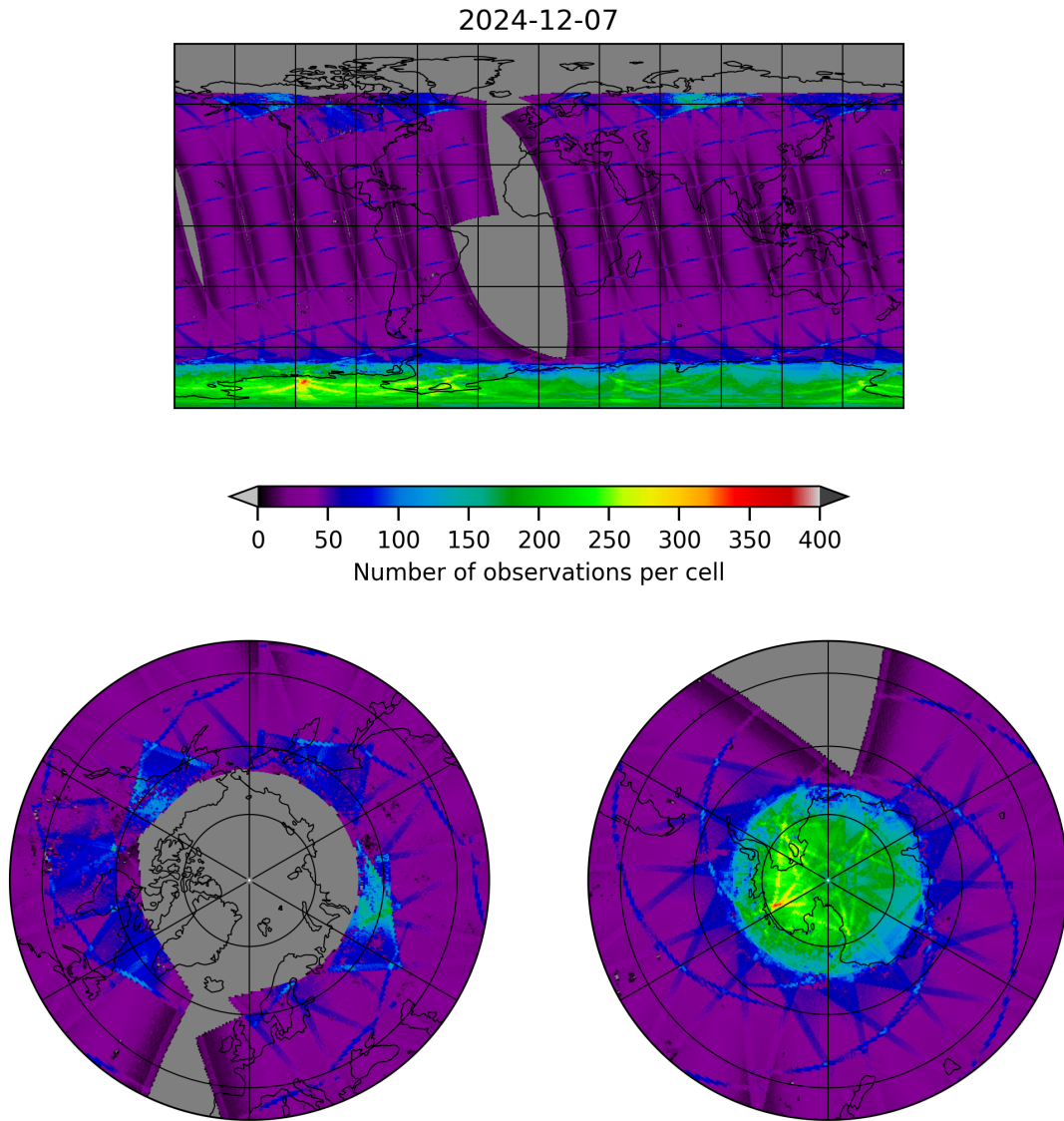
Figure 9: Map of the number of observations for 2024-12-07 to 2024-12-08
