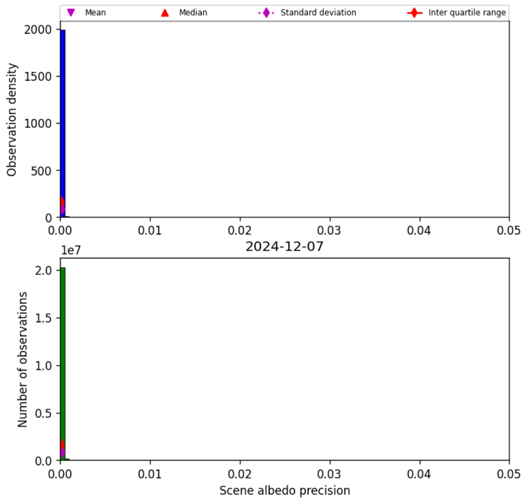
Figure 33: Histogram of “Scene albedo precision” for 2024-12-07 to 2024-12-08
