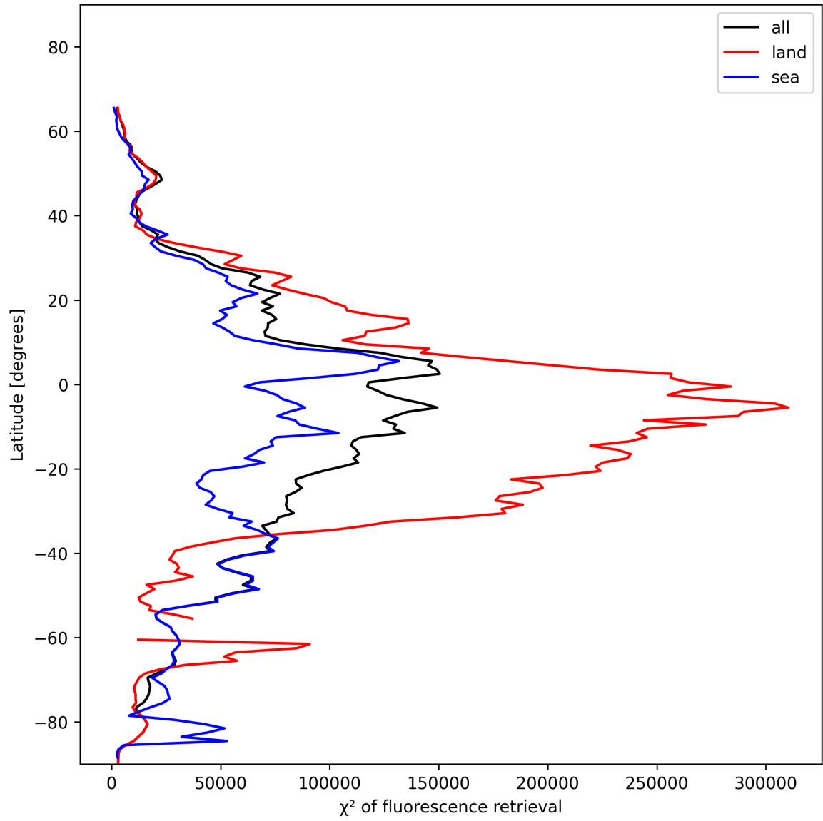
Figure 23: Zonal average of “ \chi^2 of fluorescence retrieval” for 2024-12-07 to 2024-12-08.
