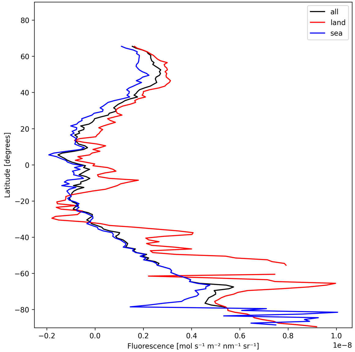
Figure 21: Zonal average of “Fluorescence” for 2024-12-07 to 2024-12-08.
