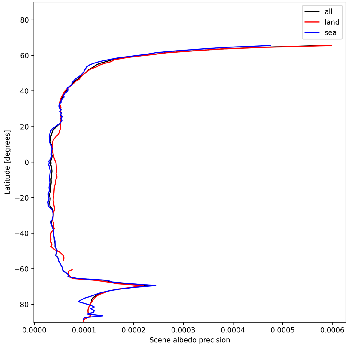
Figure 16: Zonal average of “Scene albedo precision” for 2024-12-07 to 2024-12-08.
