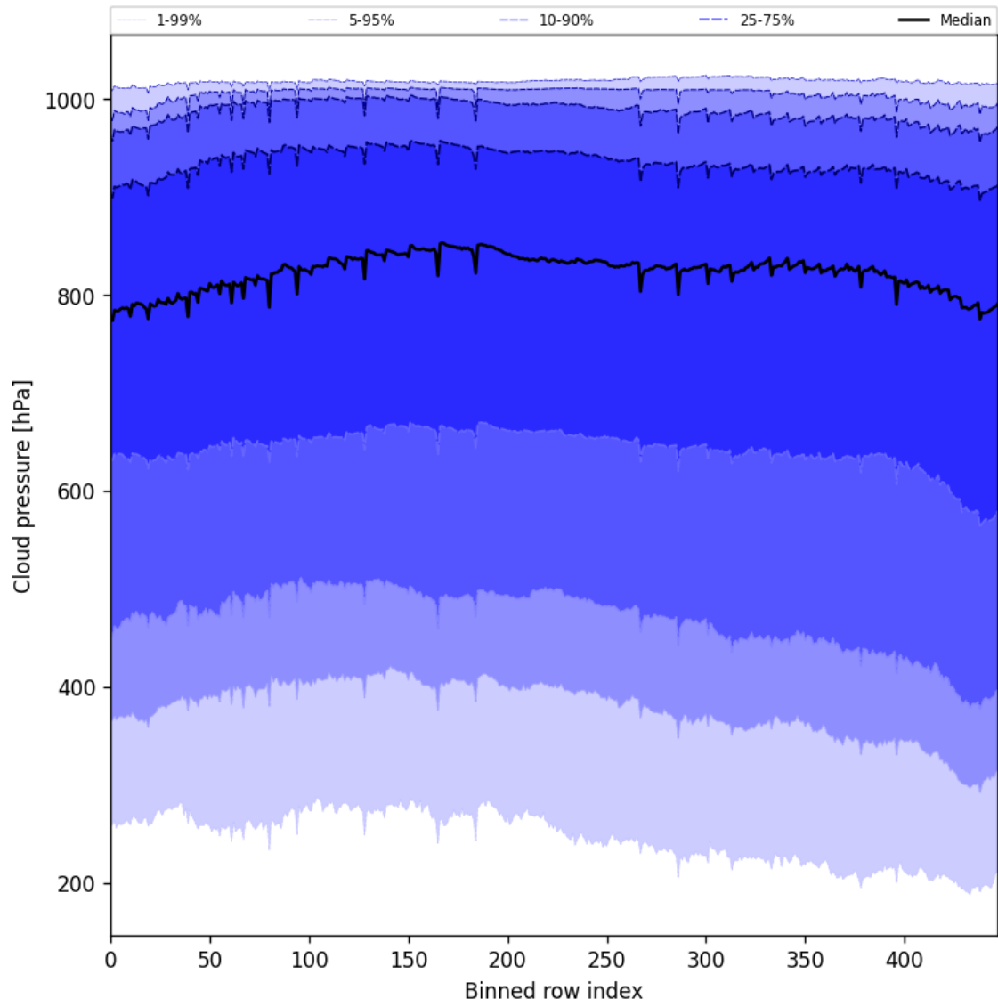
Figure 45: Along track statistics of “Cloud pressure” for 2024-12-07 to 2024-12-08
