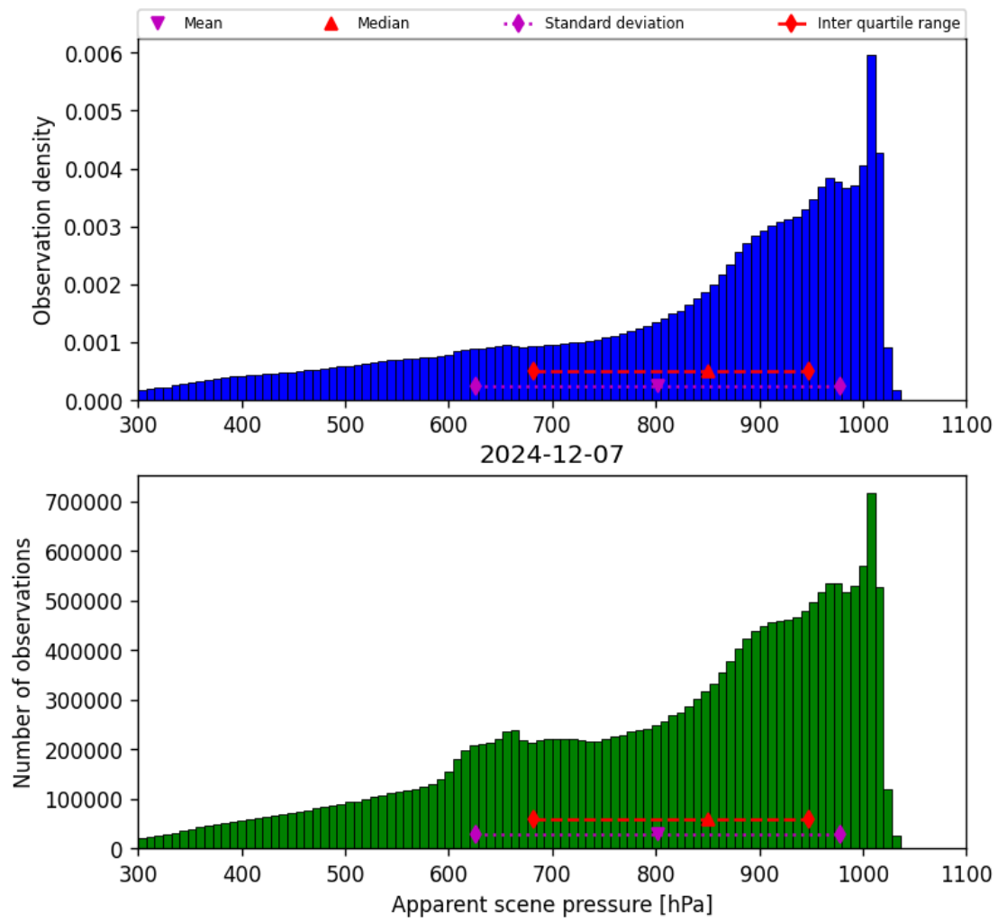
Figure 34: Histogram of “Apparent scene pressure” for 2024-12-07 to 2024-12-08
