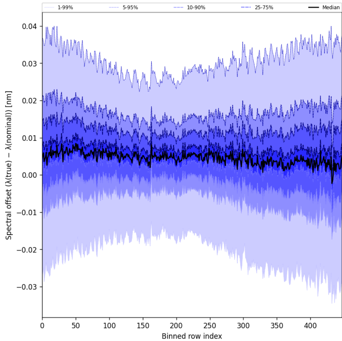
Figure 60: Along track statistics of “Spectral offset ( \lambda_{\text{true}} - \lambda_{\text{nominal}} )” for 2024-12-07 to 2024-12-08
