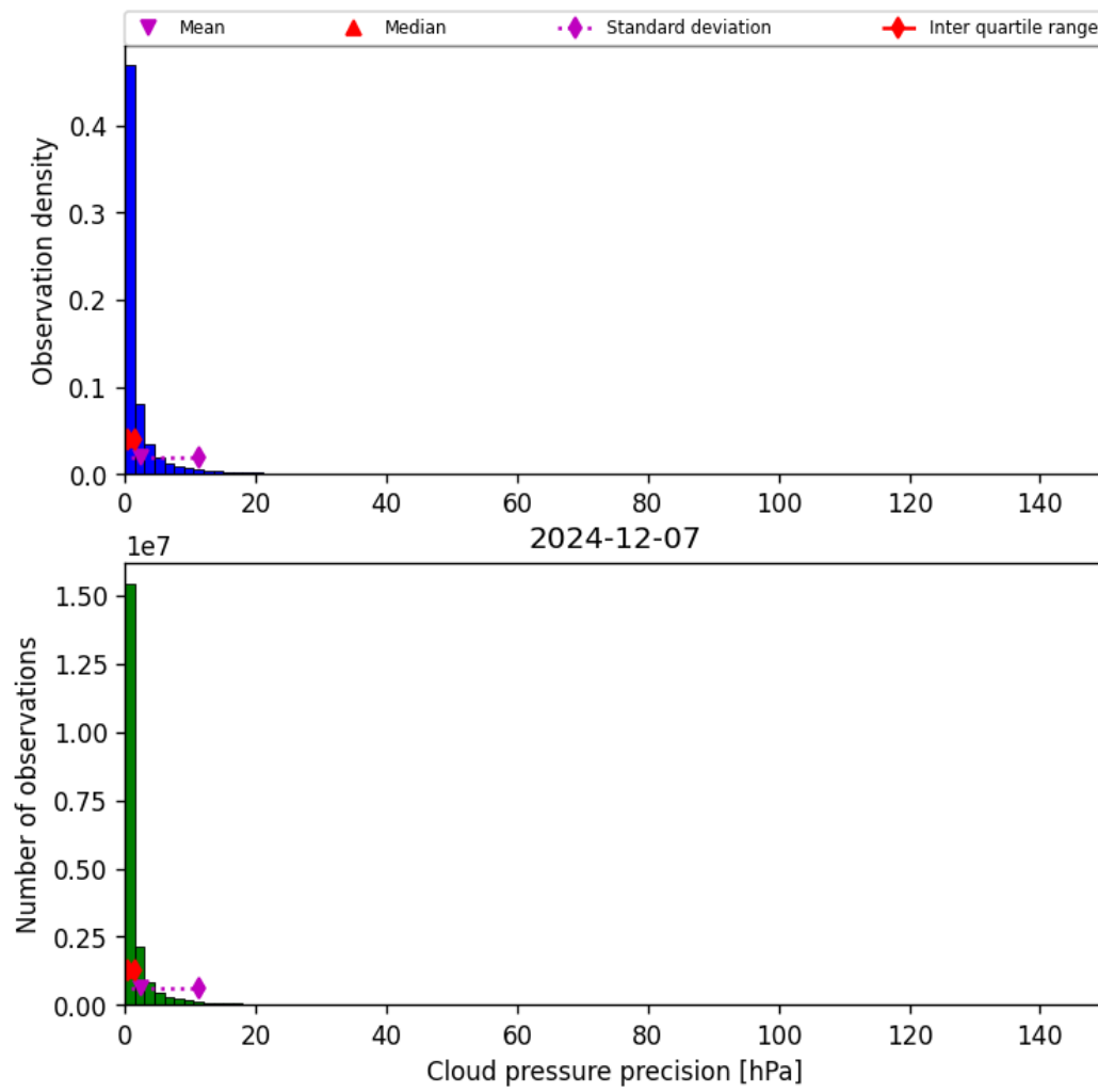
Figure 29: Histogram of “Cloud pressure precision” for 2024-12-07 to 2024-12-08
