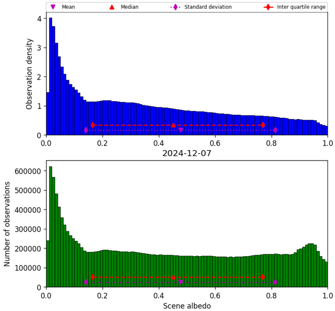
Figure 32: Histogram of “Scene albedo” for 2024-12-07 to 2024-12-08
