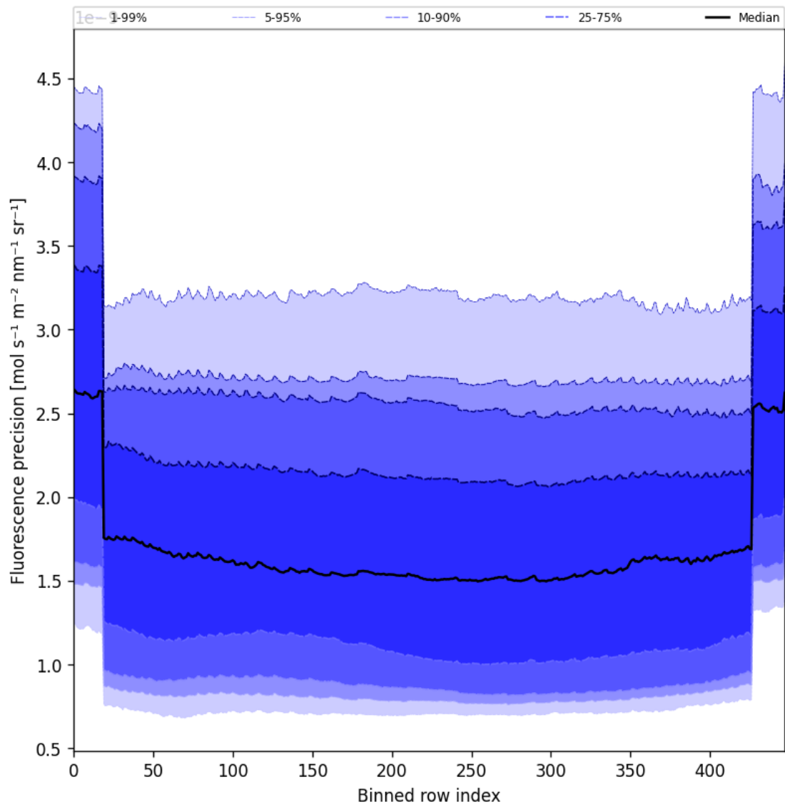
Figure 56: Along track statistics of “Fluorescence precision” for 2024-12-07 to 2024-12-08
