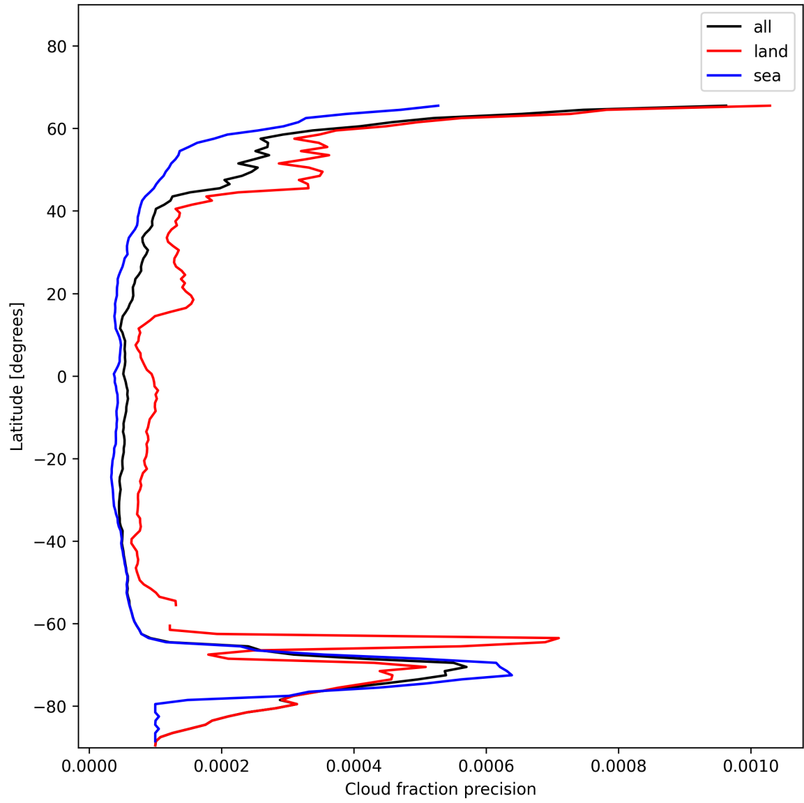
Figure 14: Zonal average of “Cloud fraction precision” for 2024-12-07 to 2024-12-08.
