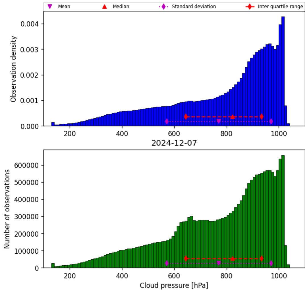
Figure 28: Histogram of “Cloud pressure” for 2024-12-07 to 2024-12-08
