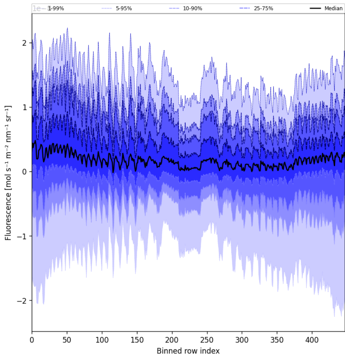
Figure 55: Along track statistics of “Fluorescence” for 2024-12-07 to 2024-12-08
