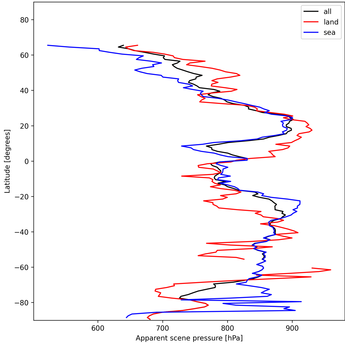
Figure 17: Zonal average of “Apparent scene pressure” for 2024-12-07 to 2024-12-08.
