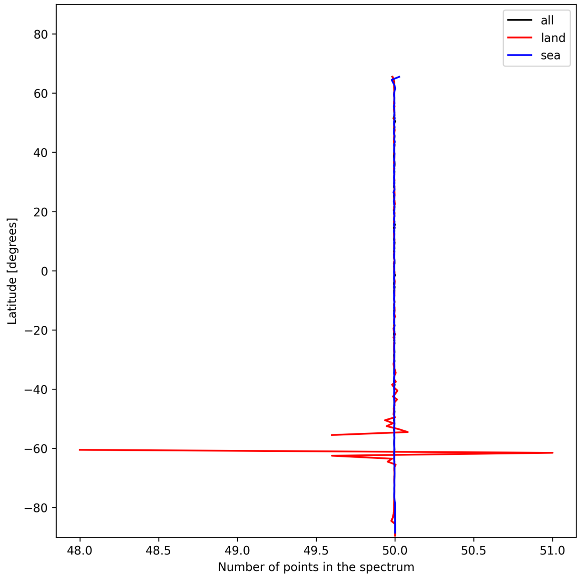
Figure 25: Zonal average of “Number of points in the spectrum” for 2024-12-07 to 2024-12-08.
