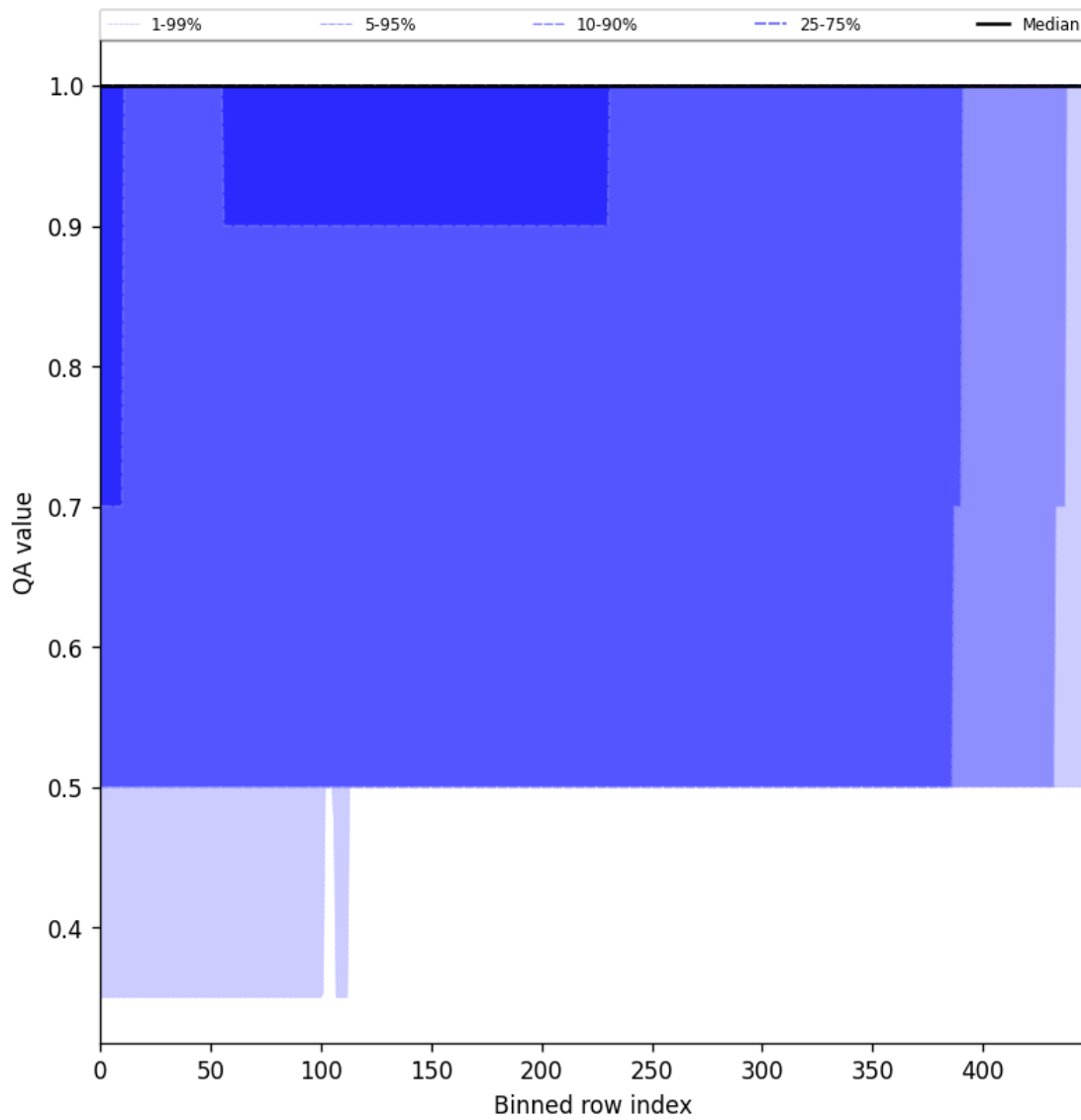
Figure 44: Along track statistics of “QA value” for 2024-12-07 to 2024-12-08
