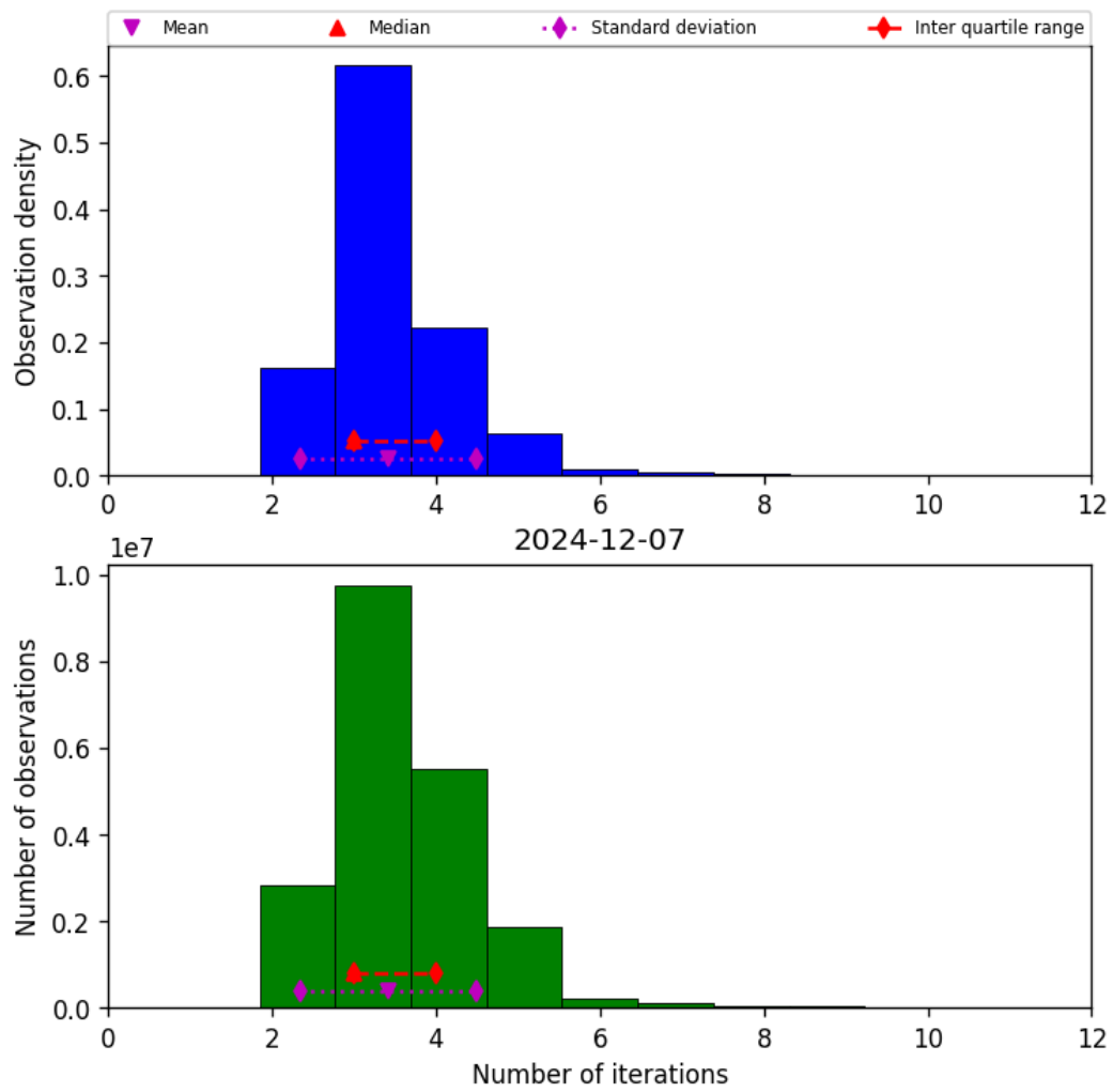
Figure 37: Histogram of “Number of iterations” for 2024-12-07 to 2024-12-08
