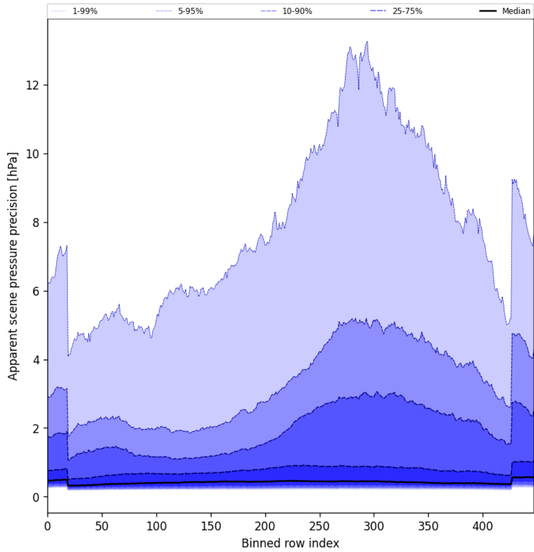
Figure 52: Along track statistics of “Apparent scene pressure precision” for 2024-12-07 to 2024-12-08
