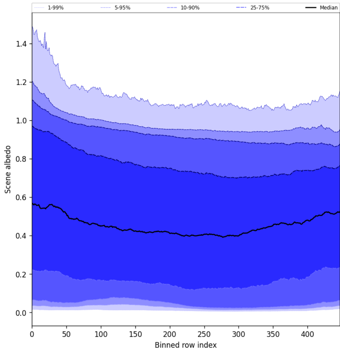
Figure 49: Along track statistics of “Scene albedo” for 2024-12-07 to 2024-12-08
