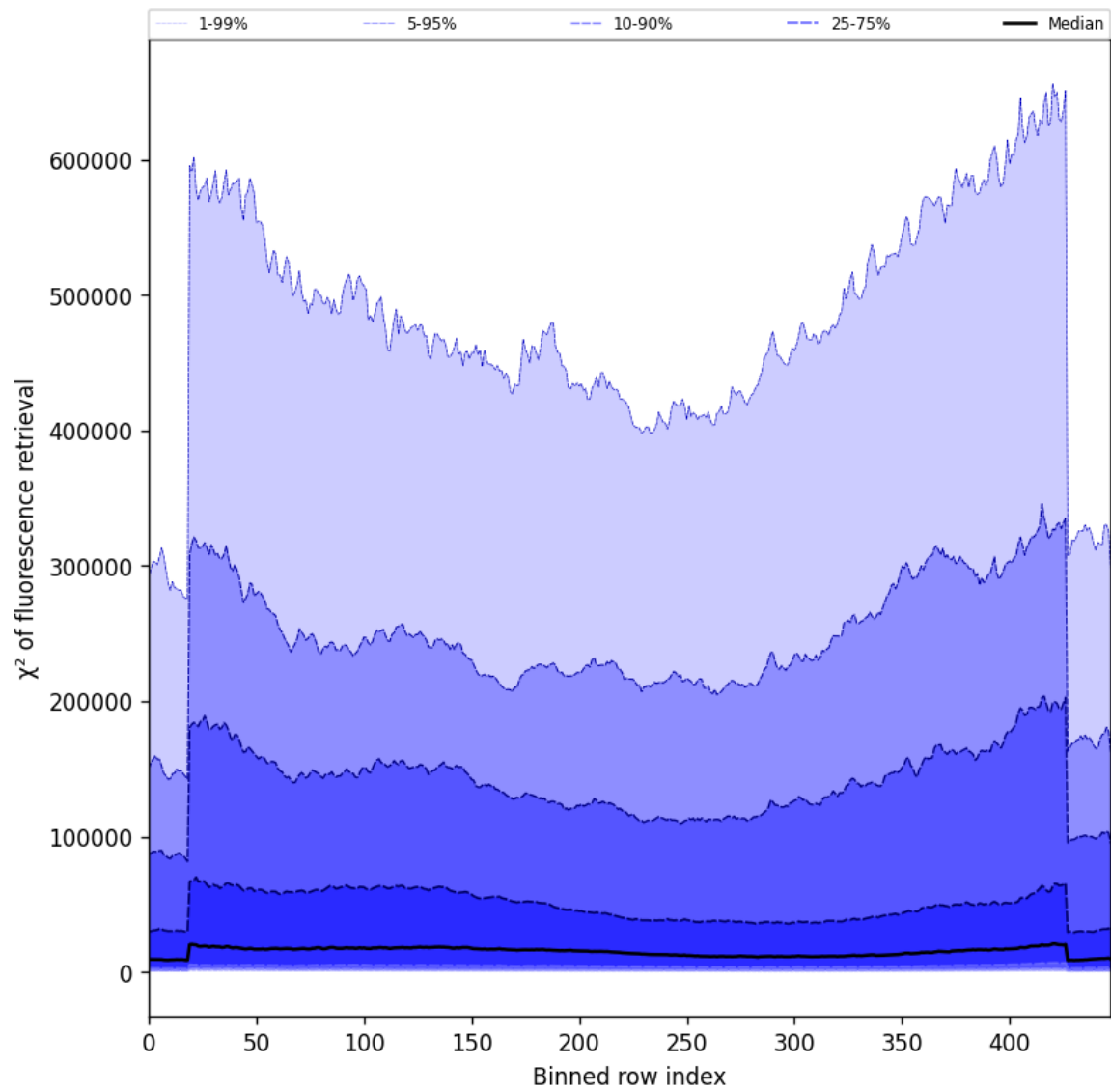
Figure 57: Along track statistics of “ \chi^2 of fluorescence retrieval” for 2024-12-07 to 2024-12-08
