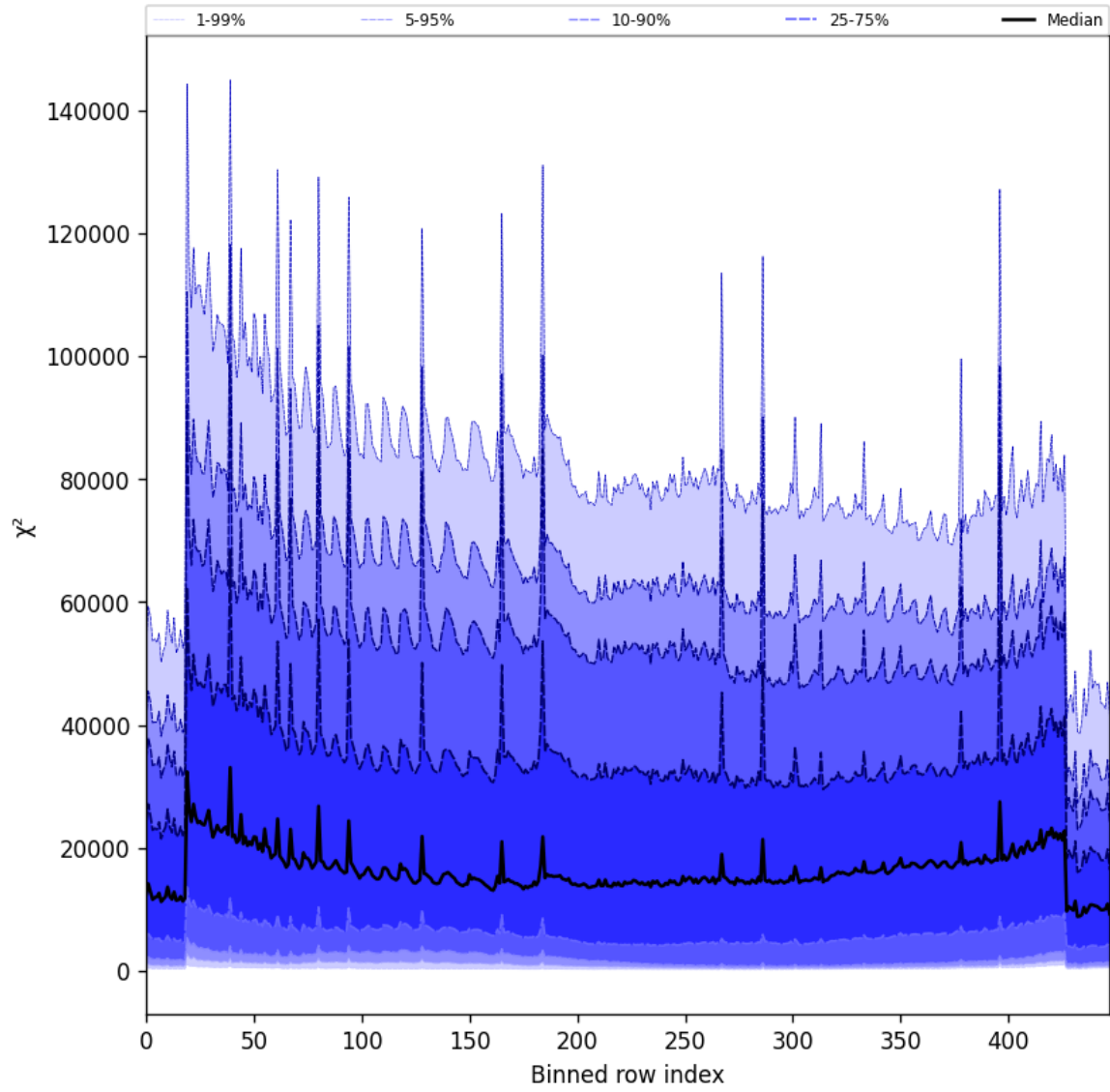
Figure 53: Along track statistics of “ \chi^2 ” for 2024-12-07 to 2024-12-08
