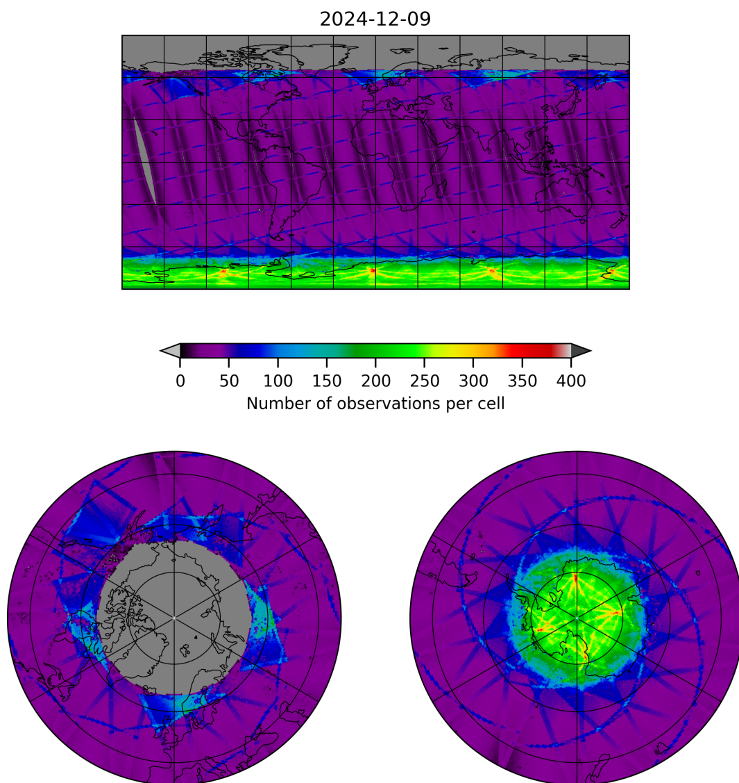
Figure 9: Map of the number of observations for 2024-12-09 to 2024-12-09
