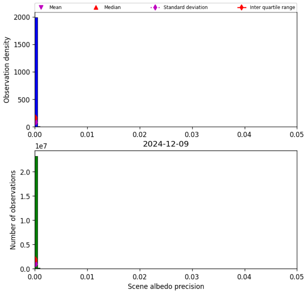
Figure 33: Histogram of “Scene albedo precision” for 2024-12-09 to 2024-12-09
