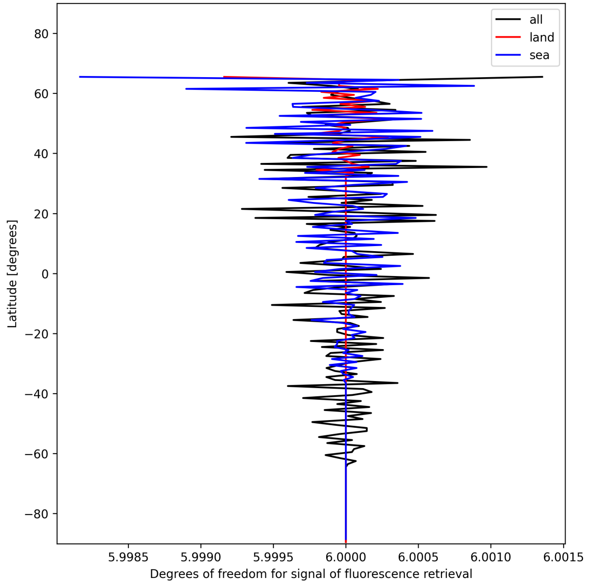
Figure 24: Zonal average of “Degrees of freedom for signal of fluorescence retrieval” for 2024-12-09 to 2024-12-09.
