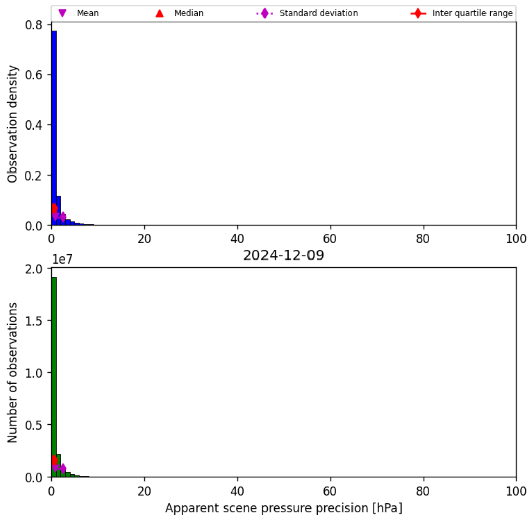
Figure 35: Histogram of “Apparent scene pressure precision” for 2024-12-09 to 2024-12-09
