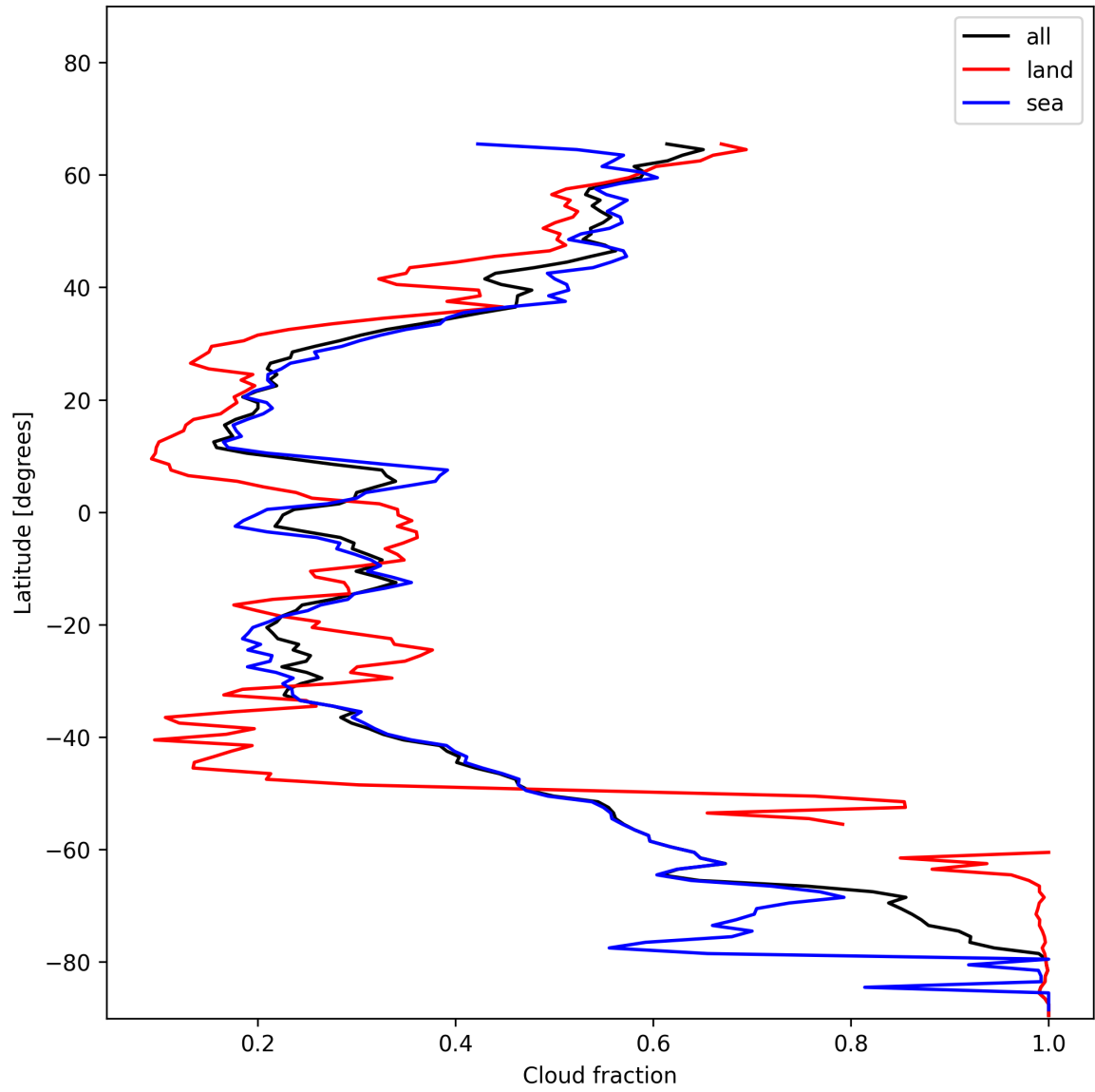
Figure 13: Zonal average of “Cloud fraction” for 2024-12-09 to 2024-12-09.
