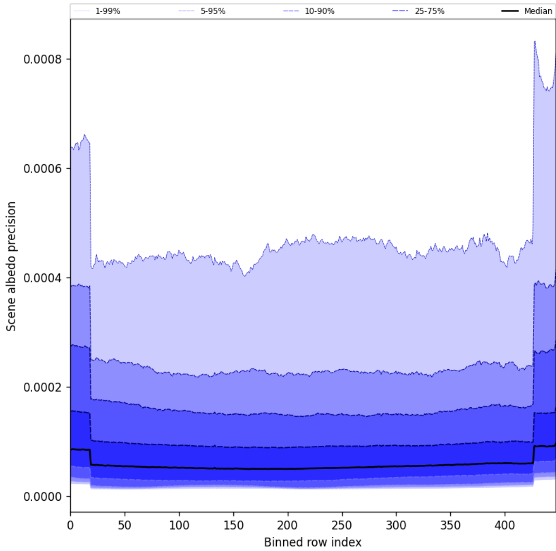
Figure 50: Along track statistics of “Scene albedo precision” for 2024-12-09 to 2024-12-09
