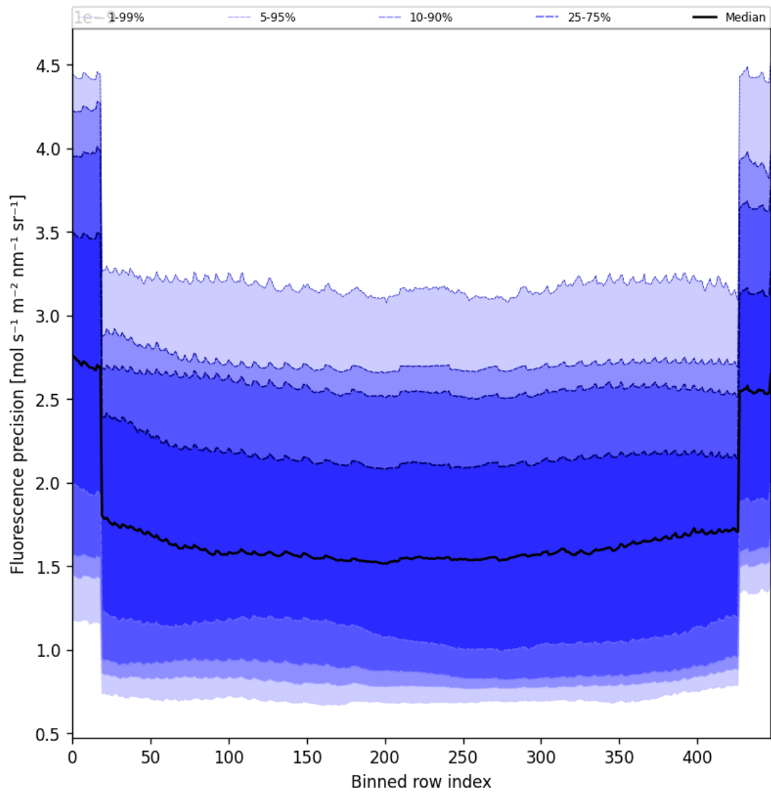
Figure 56: Along track statistics of “Fluorescence precision” for 2024-12-09 to 2024-12-09
