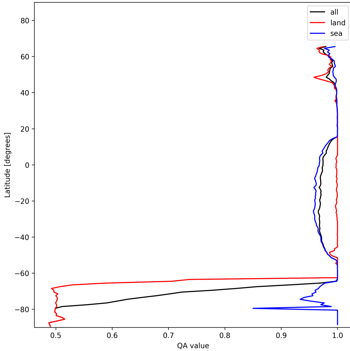
Figure 10: Zonal average of “QA value” for 2024-12-09 to 2024-12-09.
