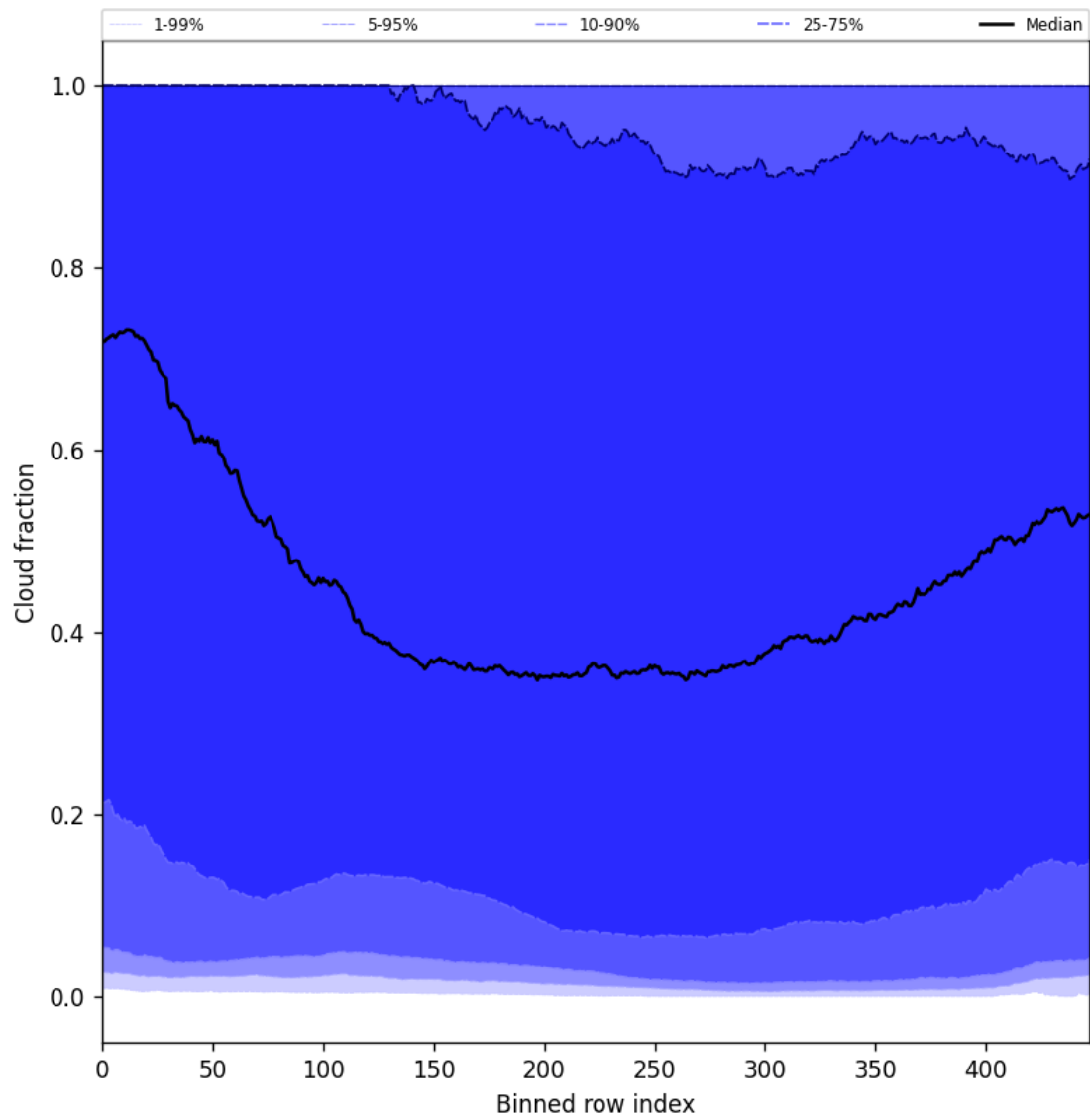
Figure 47: Along track statistics of “Cloud fraction” for 2024-12-09 to 2024-12-09
