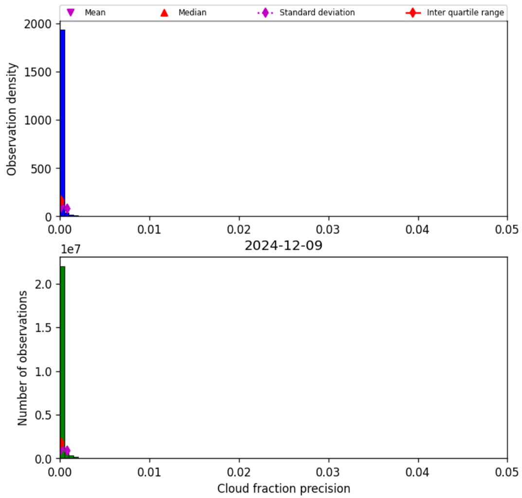
Figure 31: Histogram of “Cloud fraction precision” for 2024-12-09 to 2024-12-09
