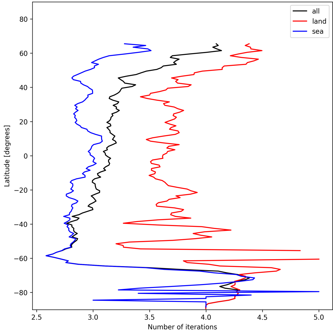
Figure 20: Zonal average of “Number of iterations” for 2024-12-09 to 2024-12-09.
