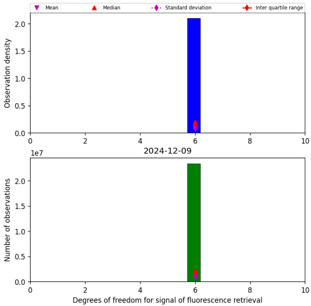
Figure 41: Histogram of “Degrees of freedom for signal of fluorescence retrieval” for 2024-12-09 to 2024-12-09
