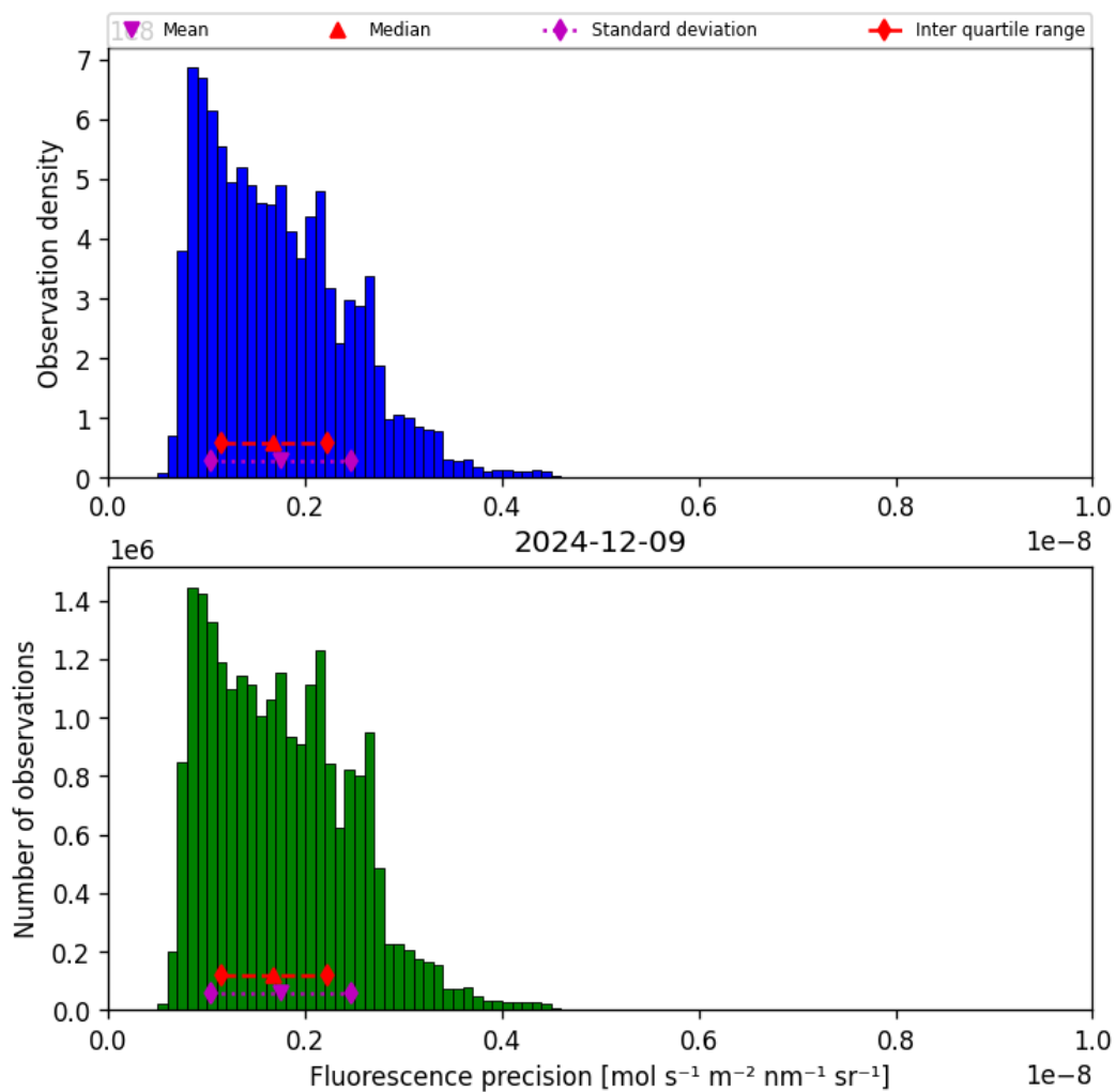
Figure 39: Histogram of “Fluorescence precision” for 2024-12-09 to 2024-12-09
