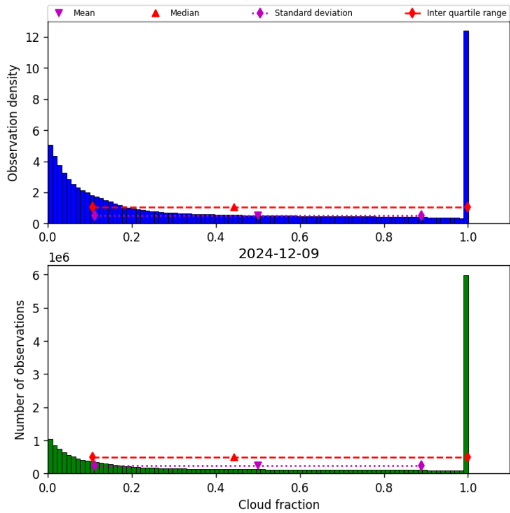
Figure 30: Histogram of “Cloud fraction” for 2024-12-09 to 2024-12-09
