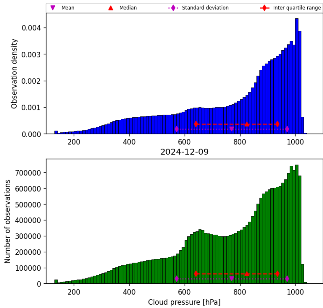
Figure 28: Histogram of “Cloud pressure” for 2024-12-09 to 2024-12-09
