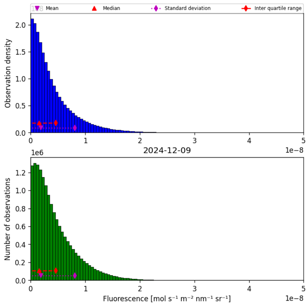
Figure 38: Histogram of “Fluorescence” for 2024-12-09 to 2024-12-09
