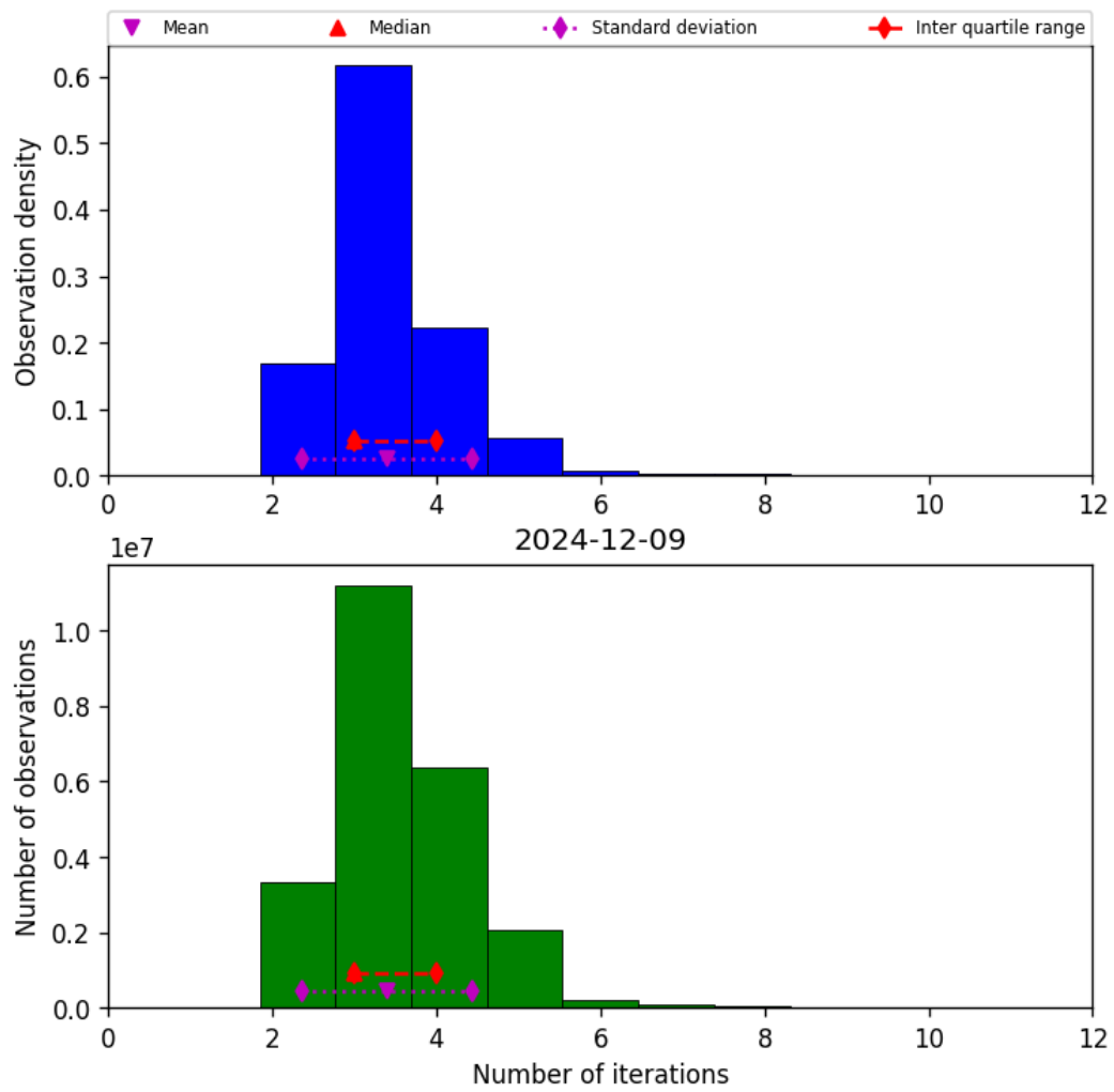
Figure 37: Histogram of “Number of iterations” for 2024-12-09 to 2024-12-09
