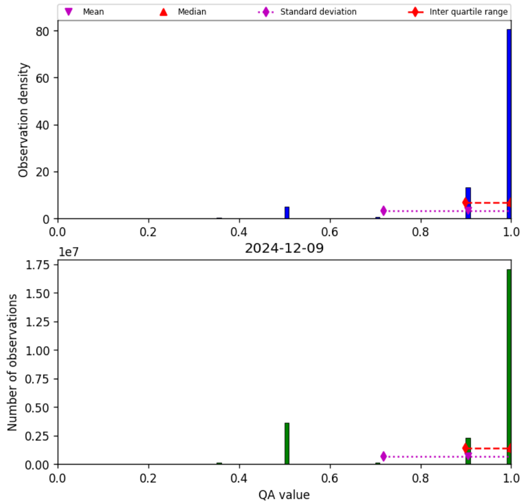
Figure 27: Histogram of “QA value” for 2024-12-09 to 2024-12-09
