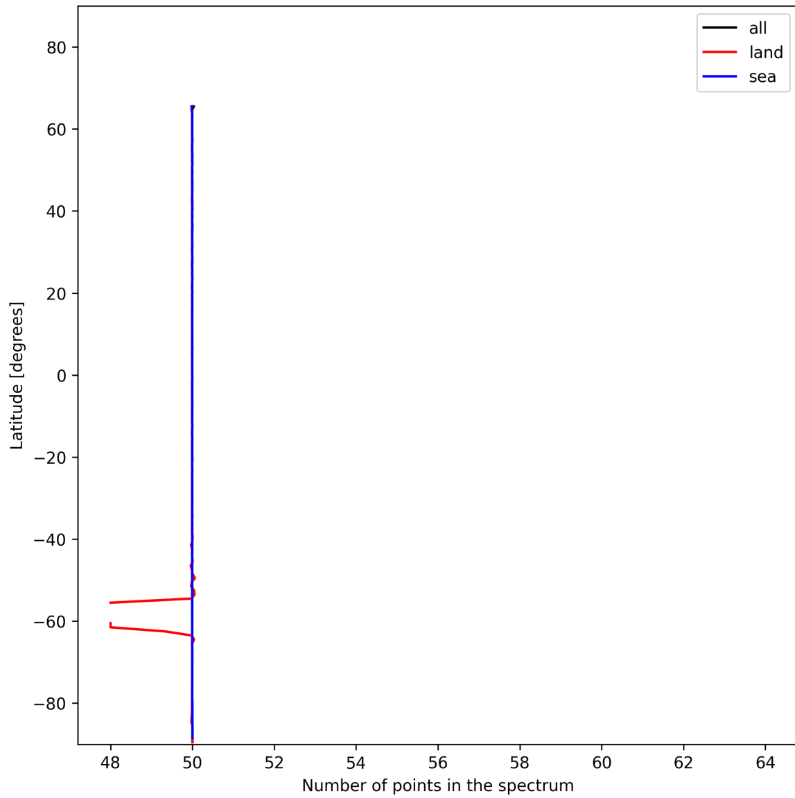
Figure 25: Zonal average of “Number of points in the spectrum” for 2024-12-09 to 2024-12-09.
