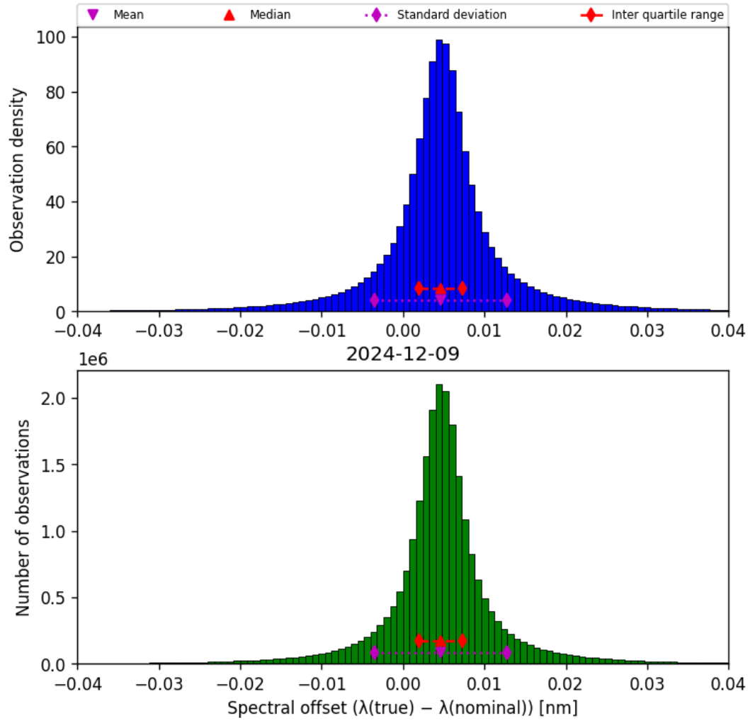
Figure 43: Histogram of “Spectral offset ( \lambda_{\text{true}} - \lambda_{\text{nominal}} )” for 2024-12-09 to 2024-12-09
