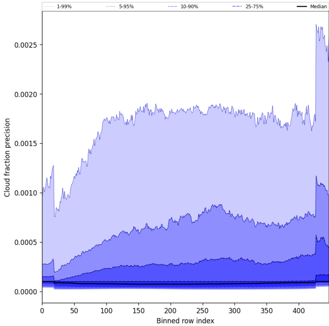
Figure 48: Along track statistics of “Cloud fraction precision” for 2024-12-09 to 2024-12-09
