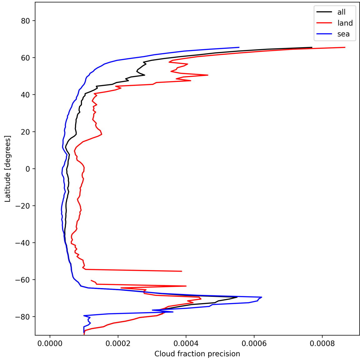
Figure 14: Zonal average of “Cloud fraction precision” for 2024-12-09 to 2024-12-09.
