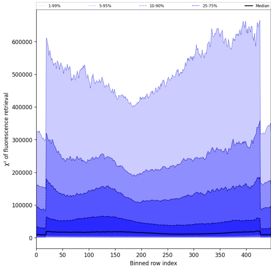
Figure 57: Along track statistics of “ \chi^2 of fluorescence retrieval” for 2024-12-09 to 2024-12-09
