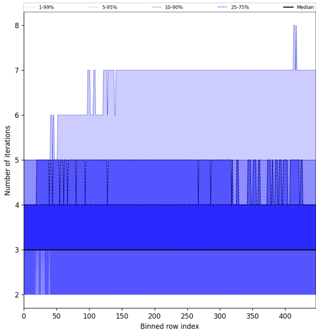
Figure 54: Along track statistics of “Number of iterations” for 2024-12-09 to 2024-12-09
