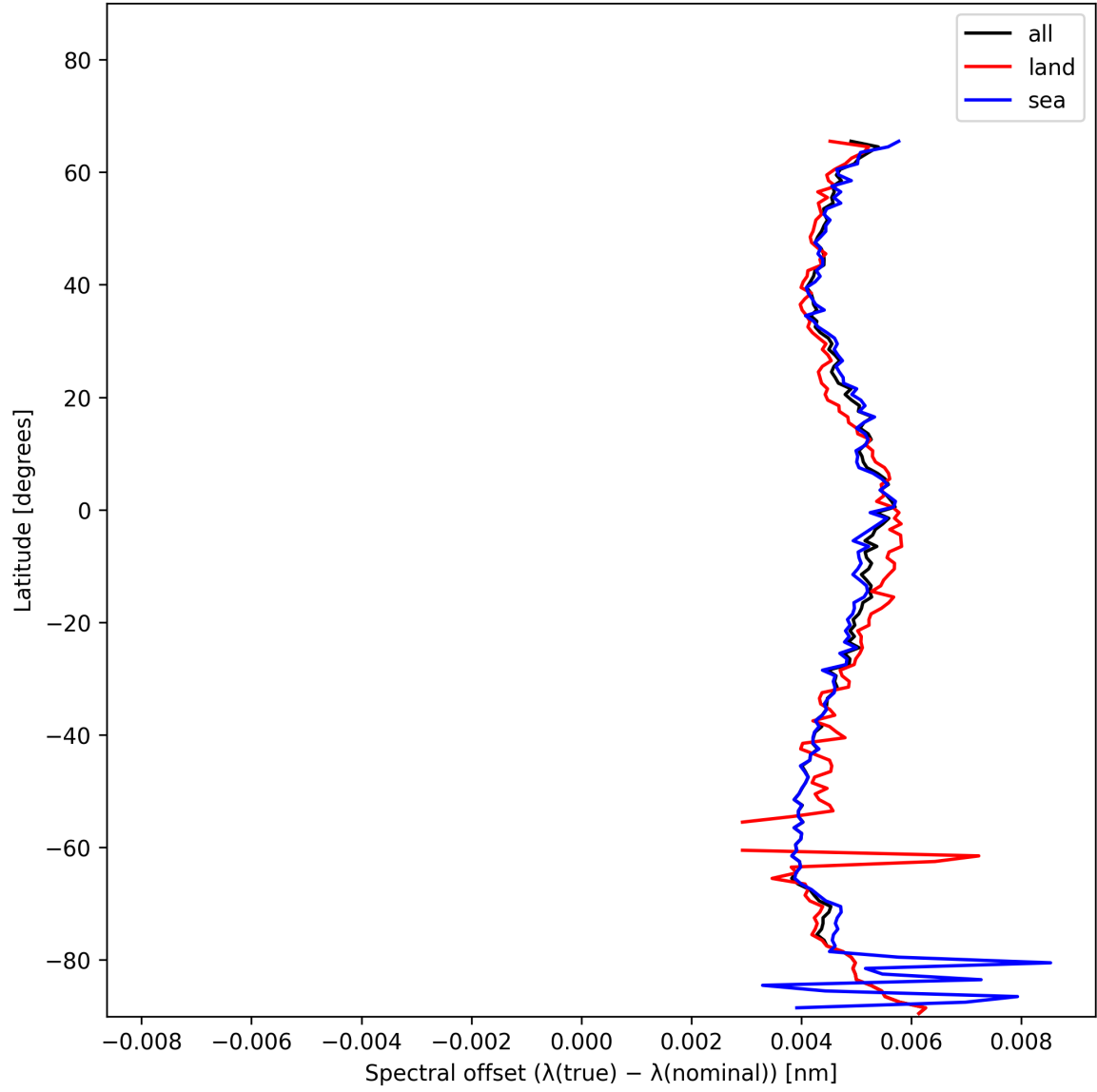
Figure 26: Zonal average of “Spectral offset ( \lambda_{\text{true}} - \lambda_{\text{nominal}} )” for 2024-12-09 to 2024-12-09.
