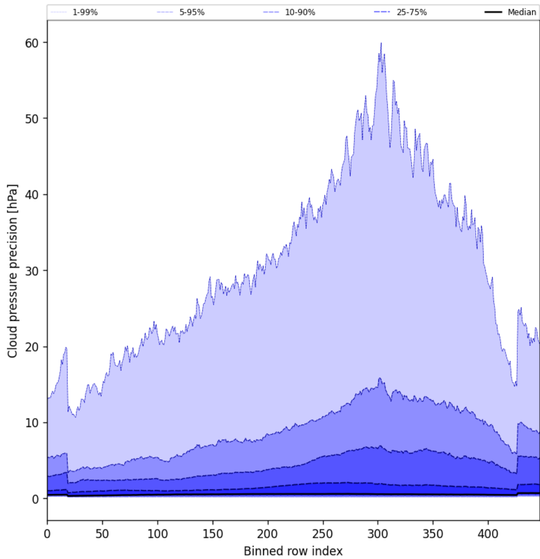
Figure 46: Along track statistics of “Cloud pressure precision” for 2024-12-09 to 2024-12-09
