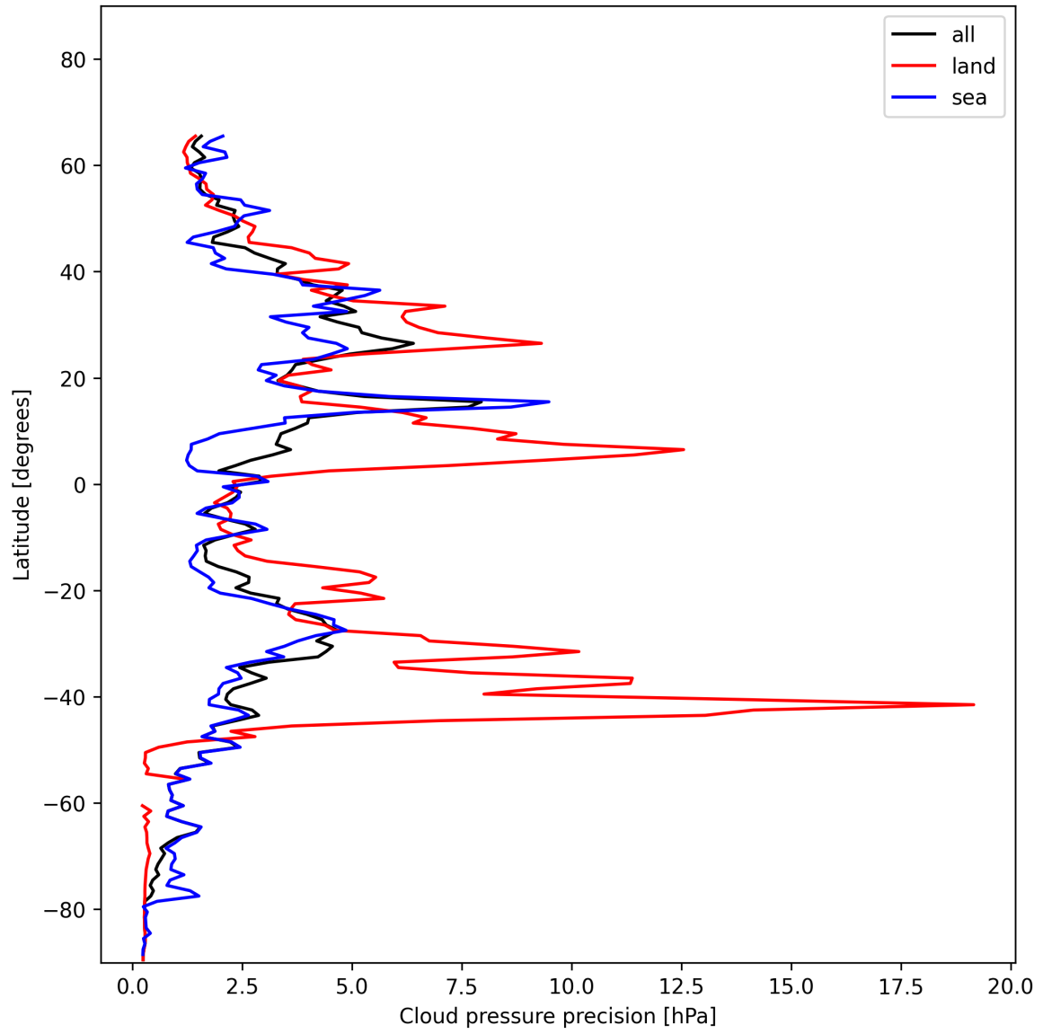
Figure 12: Zonal average of “Cloud pressure precision” for 2024-12-09 to 2024-12-09.
