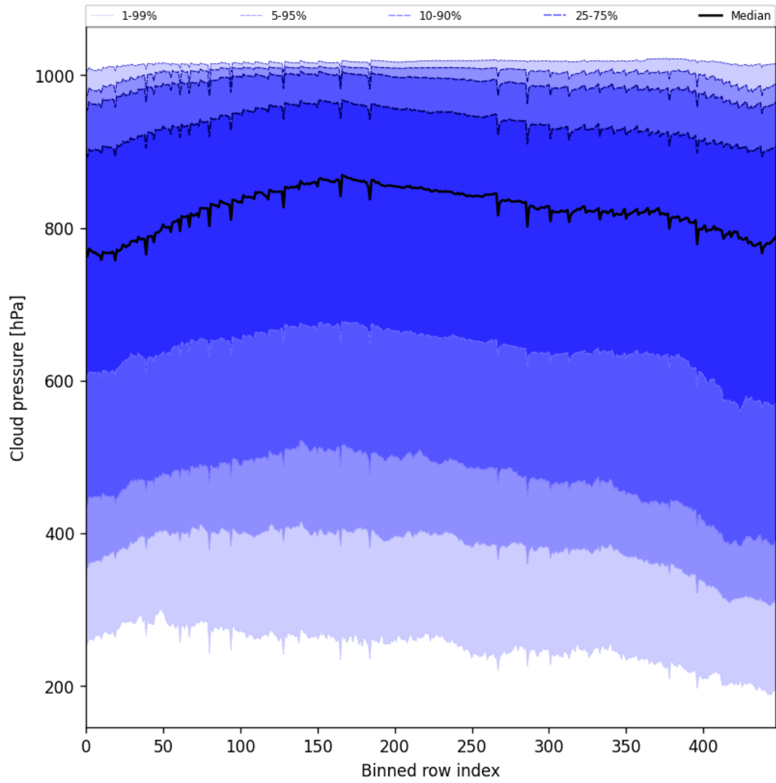
Figure 45: Along track statistics of “Cloud pressure” for 2024-12-09 to 2024-12-09
