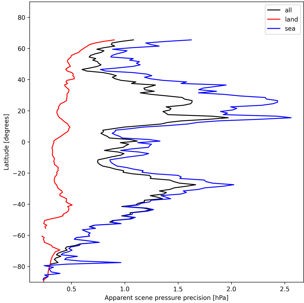
Figure 18: Zonal average of “Apparent scene pressure precision” for 2024-12-09 to 2024-12-09.
