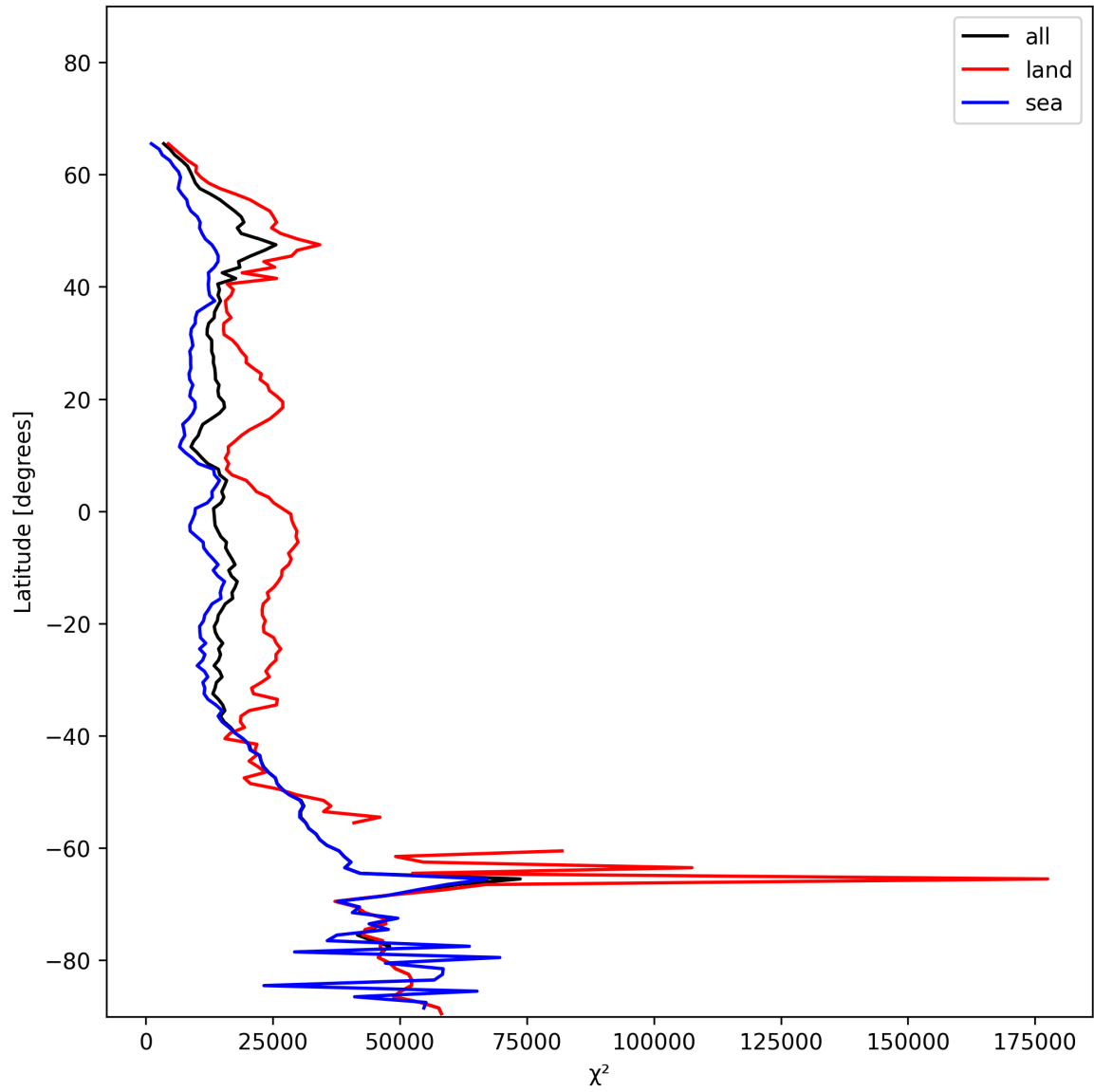
Figure 19: Zonal average of “ \chi^2 ” for 2024-12-09 to 2024-12-09.
