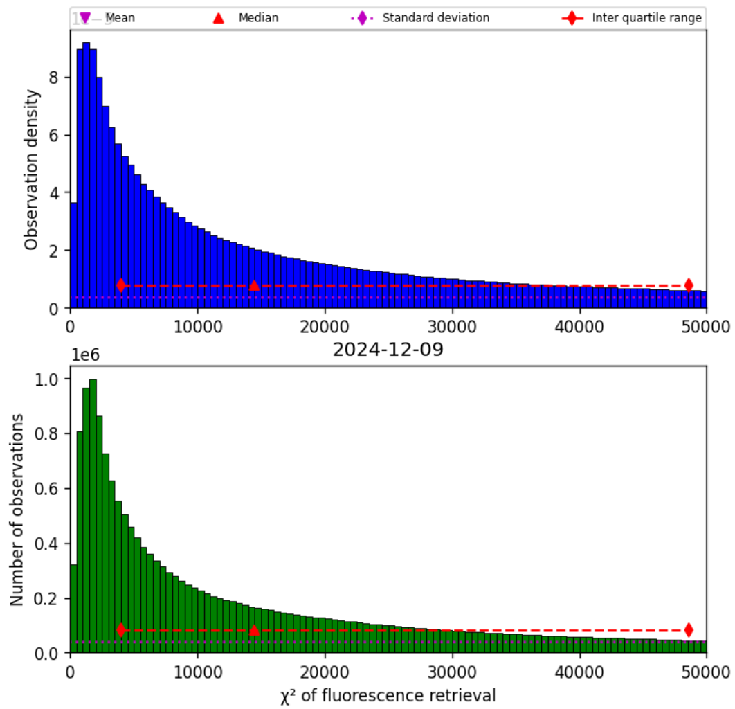
Figure 40: Histogram of “ \chi^2 of fluorescence retrieval” for 2024-12-09 to 2024-12-09
