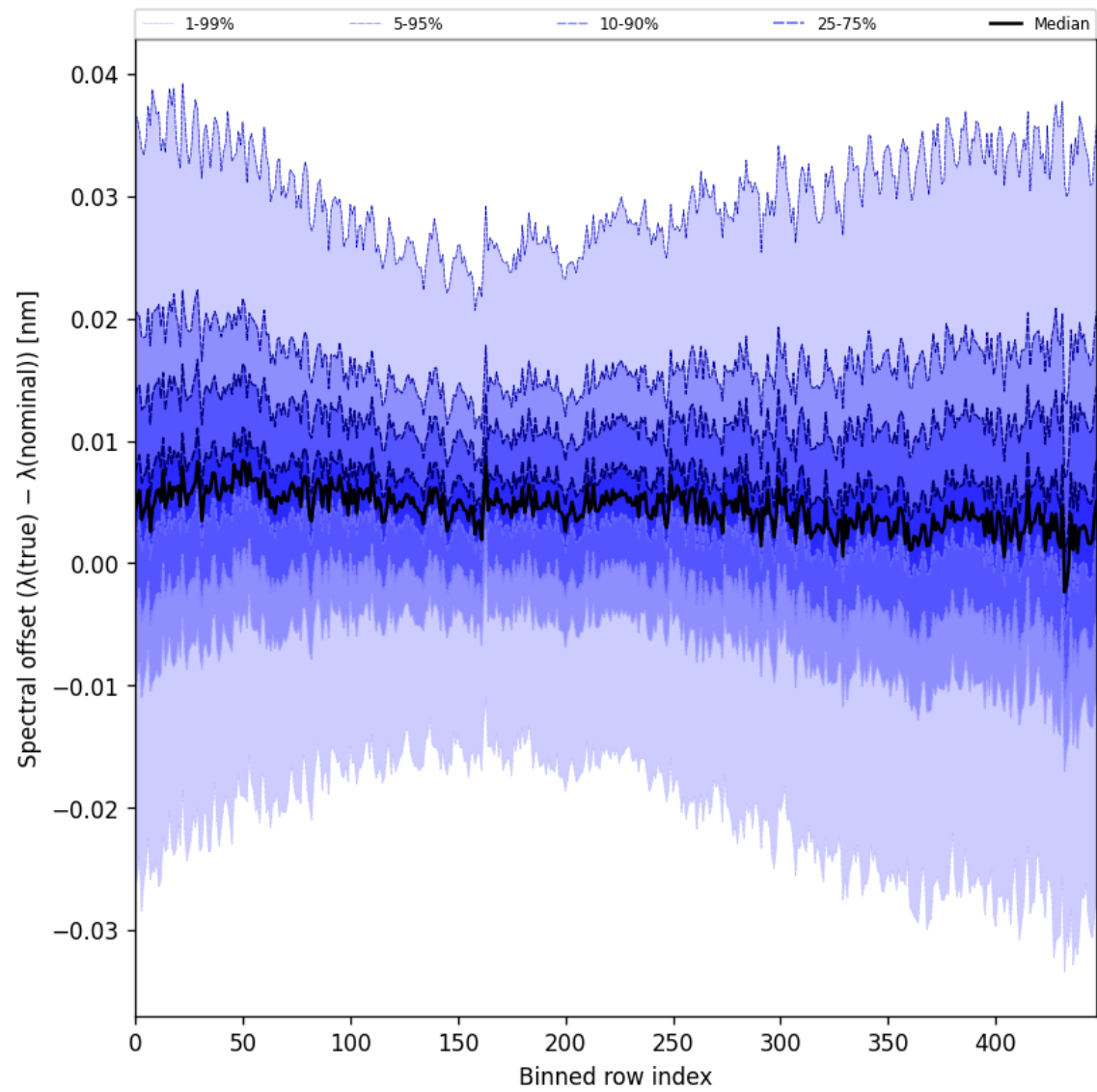
Figure 60: Along track statistics of “Spectral offset ( \lambda_{\text{true}} - \lambda_{\text{nominal}} )” for 2024-12-09 to 2024-12-09
