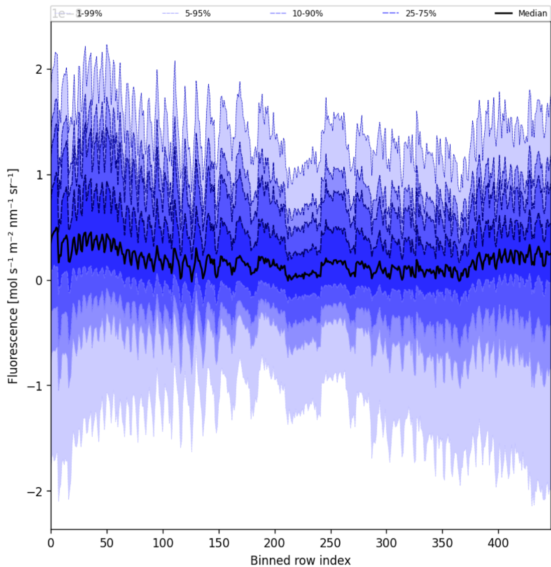
Figure 55: Along track statistics of “Fluorescence” for 2024-12-09 to 2024-12-09
