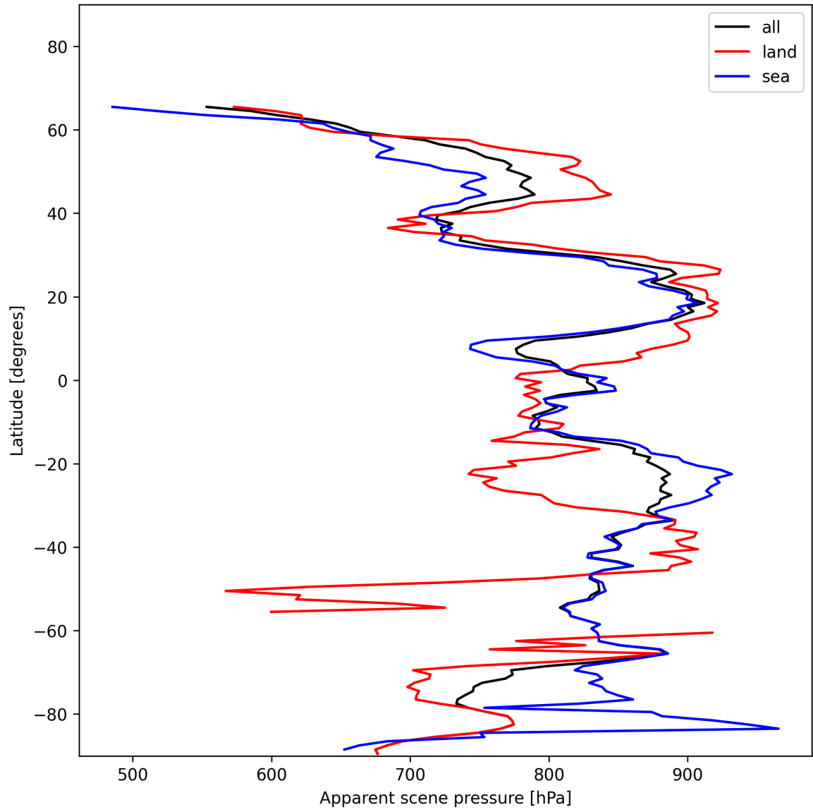
Figure 17: Zonal average of “Apparent scene pressure” for 2024-12-09 to 2024-12-09.
