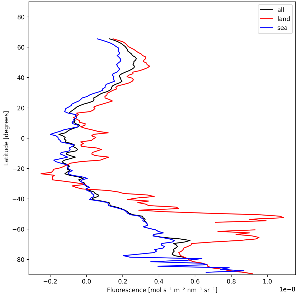
Figure 21: Zonal average of “Fluorescence” for 2024-12-09 to 2024-12-09.
