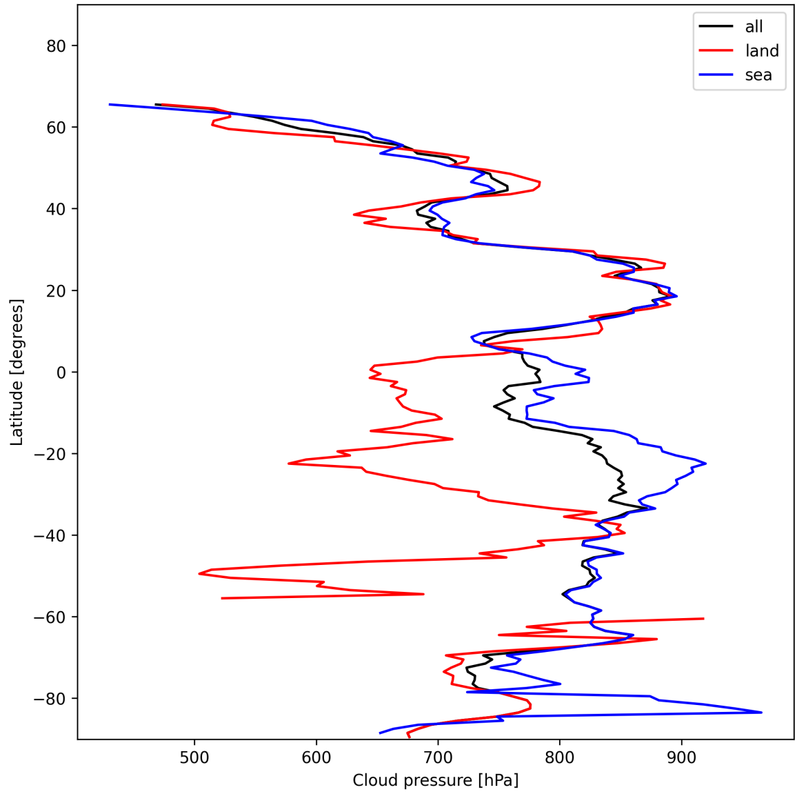
Figure 11: Zonal average of “Cloud pressure” for 2024-12-09 to 2024-12-09.
