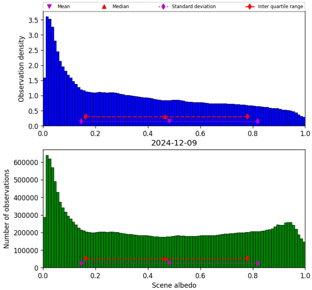
Figure 32: Histogram of “Scene albedo” for 2024-12-09 to 2024-12-09
