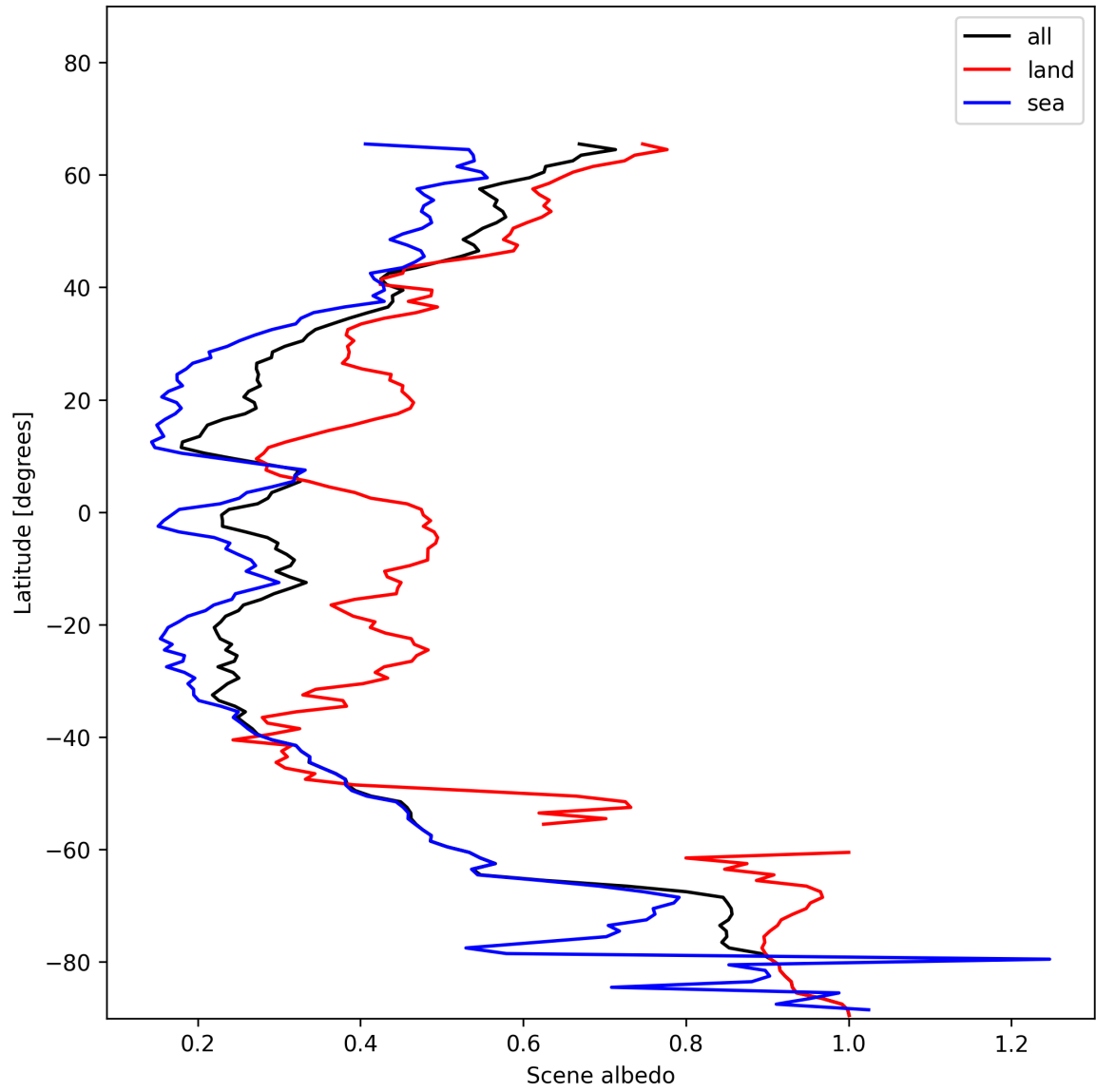
Figure 15: Zonal average of “Scene albedo” for 2024-12-09 to 2024-12-09.
