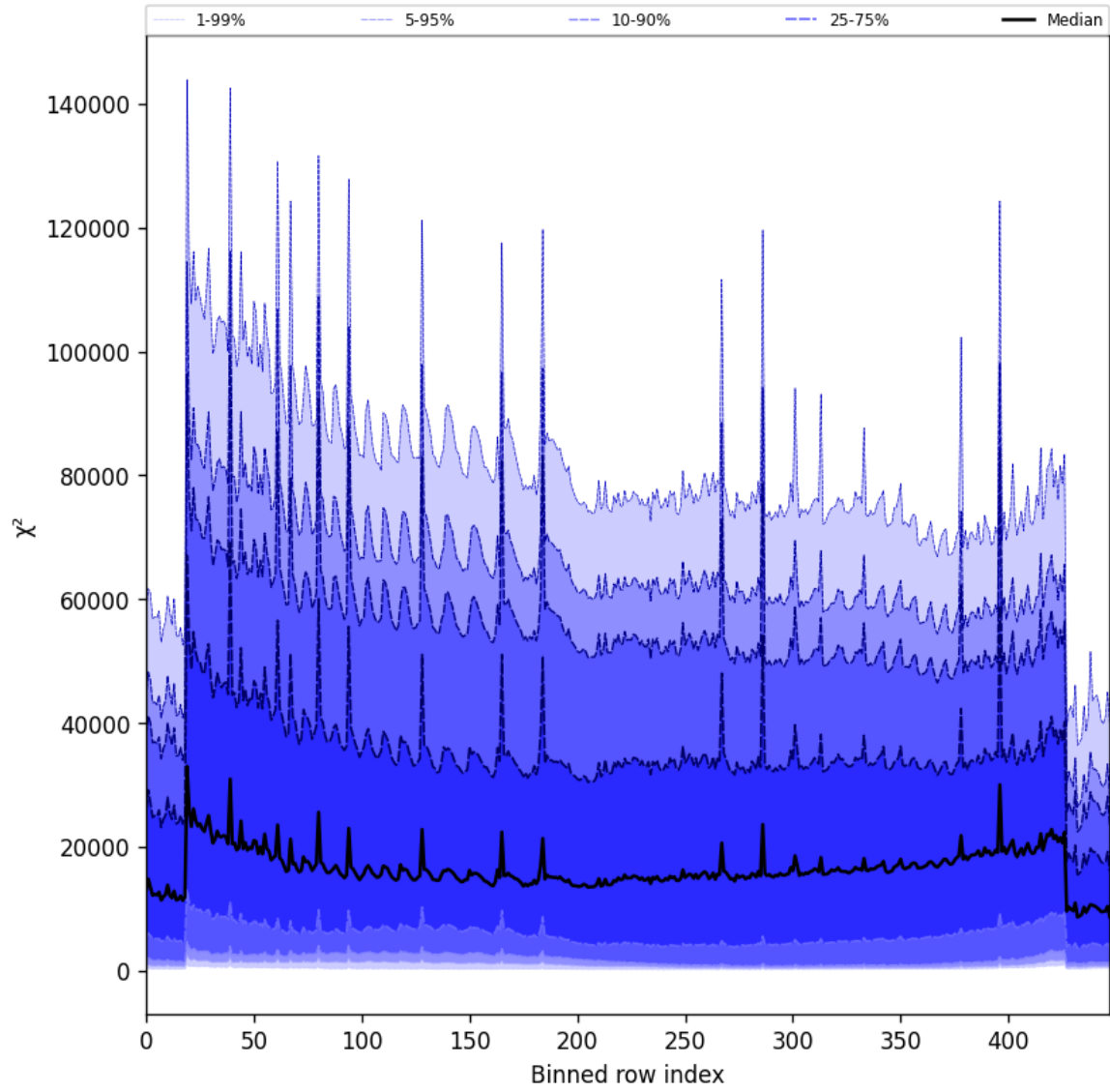
Figure 53: Along track statistics of “ \chi^2 ” for 2024-12-09 to 2024-12-09
