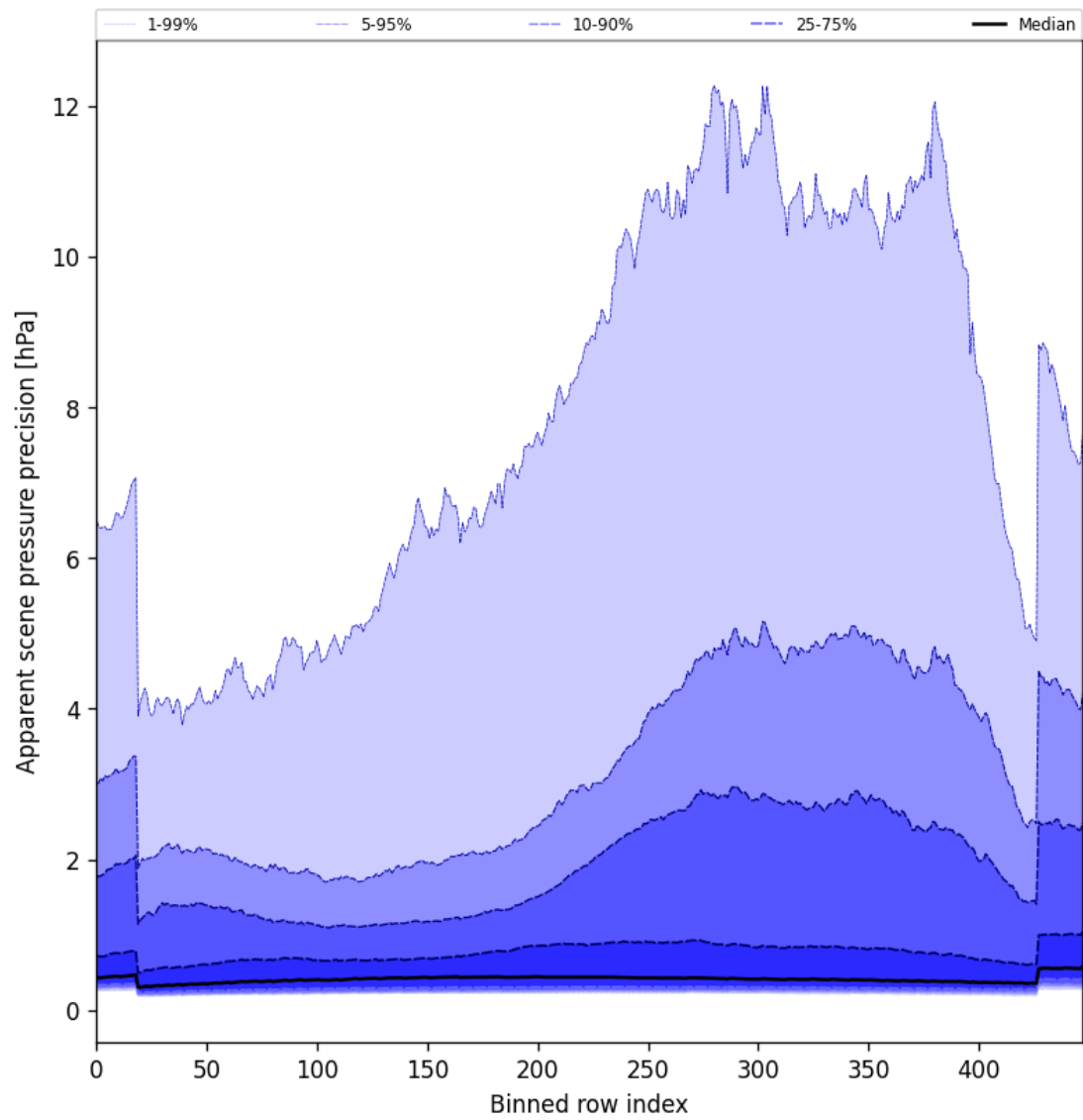
Figure 52: Along track statistics of “Apparent scene pressure precision” for 2024-12-09 to 2024-12-09
