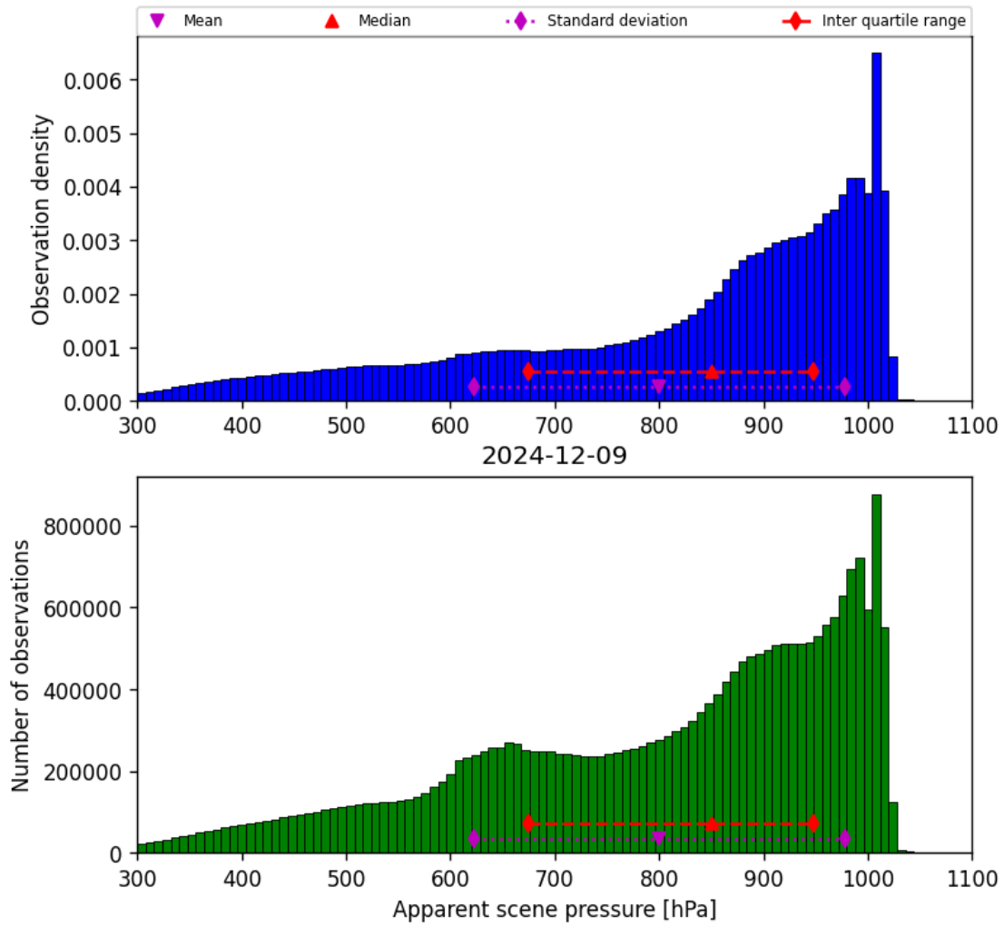
Figure 34: Histogram of “Apparent scene pressure” for 2024-12-09 to 2024-12-09
