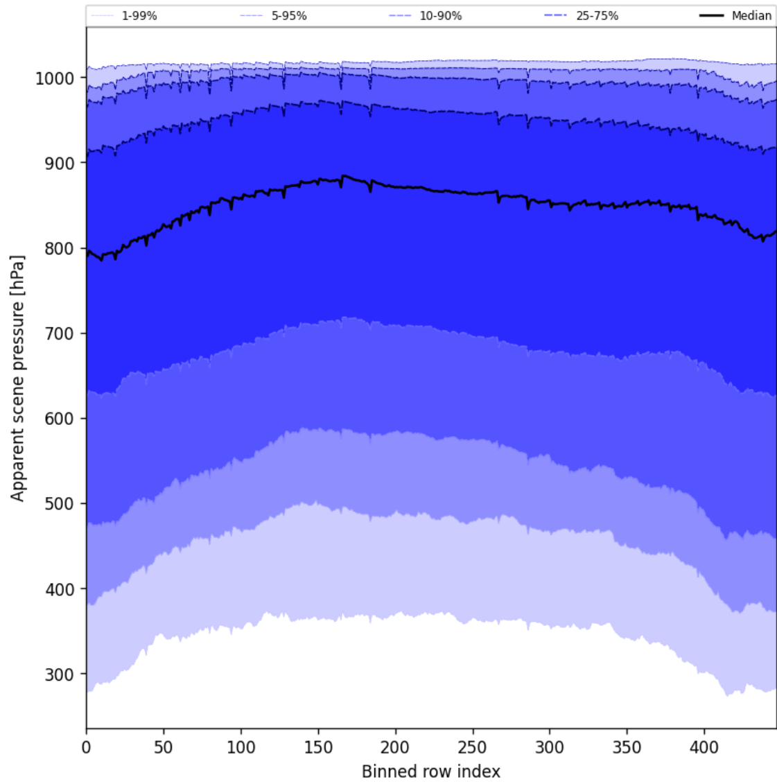
Figure 51: Along track statistics of “Apparent scene pressure” for 2024-12-09 to 2024-12-09
