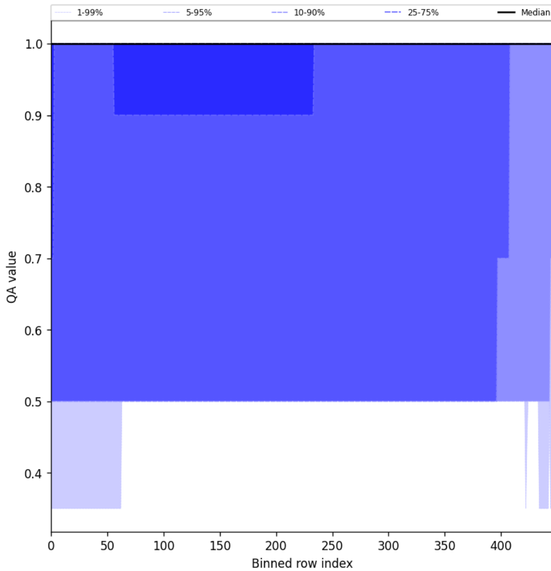
Figure 44: Along track statistics of “QA value” for 2024-12-09 to 2024-12-09
