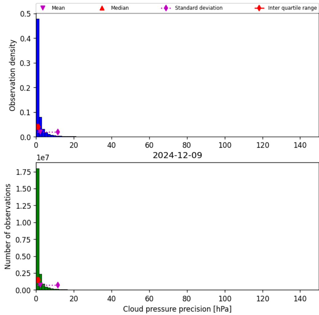
Figure 29: Histogram of “Cloud pressure precision” for 2024-12-09 to 2024-12-09
