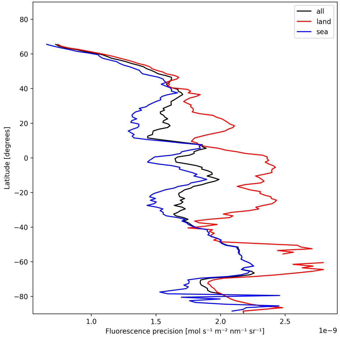
Figure 22: Zonal average of “Fluorescence precision” for 2024-12-09 to 2024-12-09.
