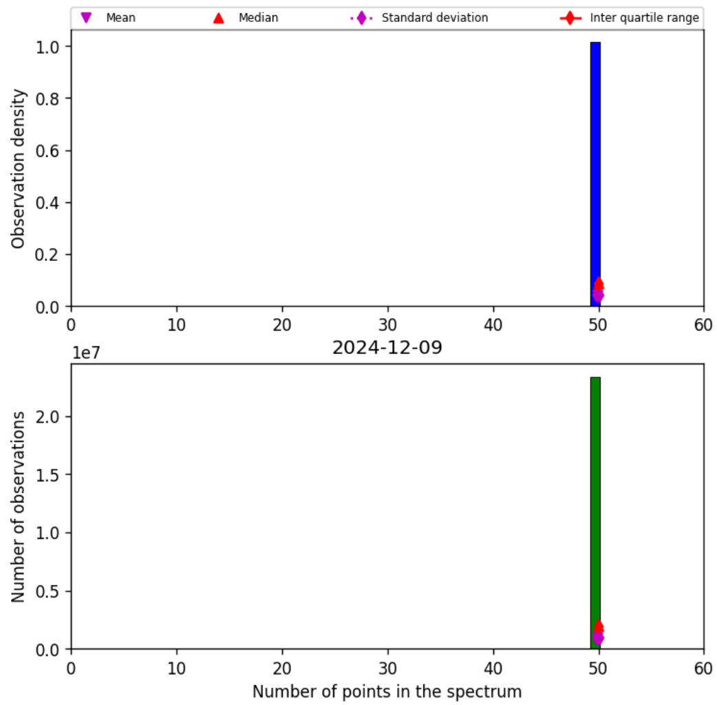
Figure 42: Histogram of "Number of points in the spectrum" for 2024-12-09 to 2024-12-09
