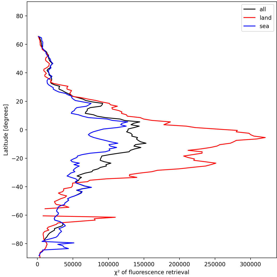
Figure 23: Zonal average of “ \chi^2 of fluorescence retrieval” for 2024-12-09 to 2024-12-09.
