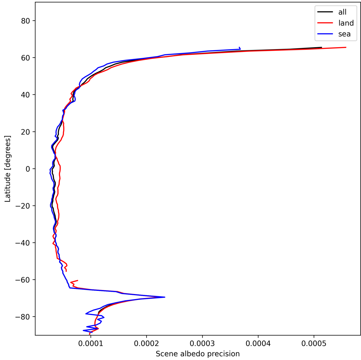
Figure 16: Zonal average of “Scene albedo precision” for 2024-12-09 to 2024-12-09.
