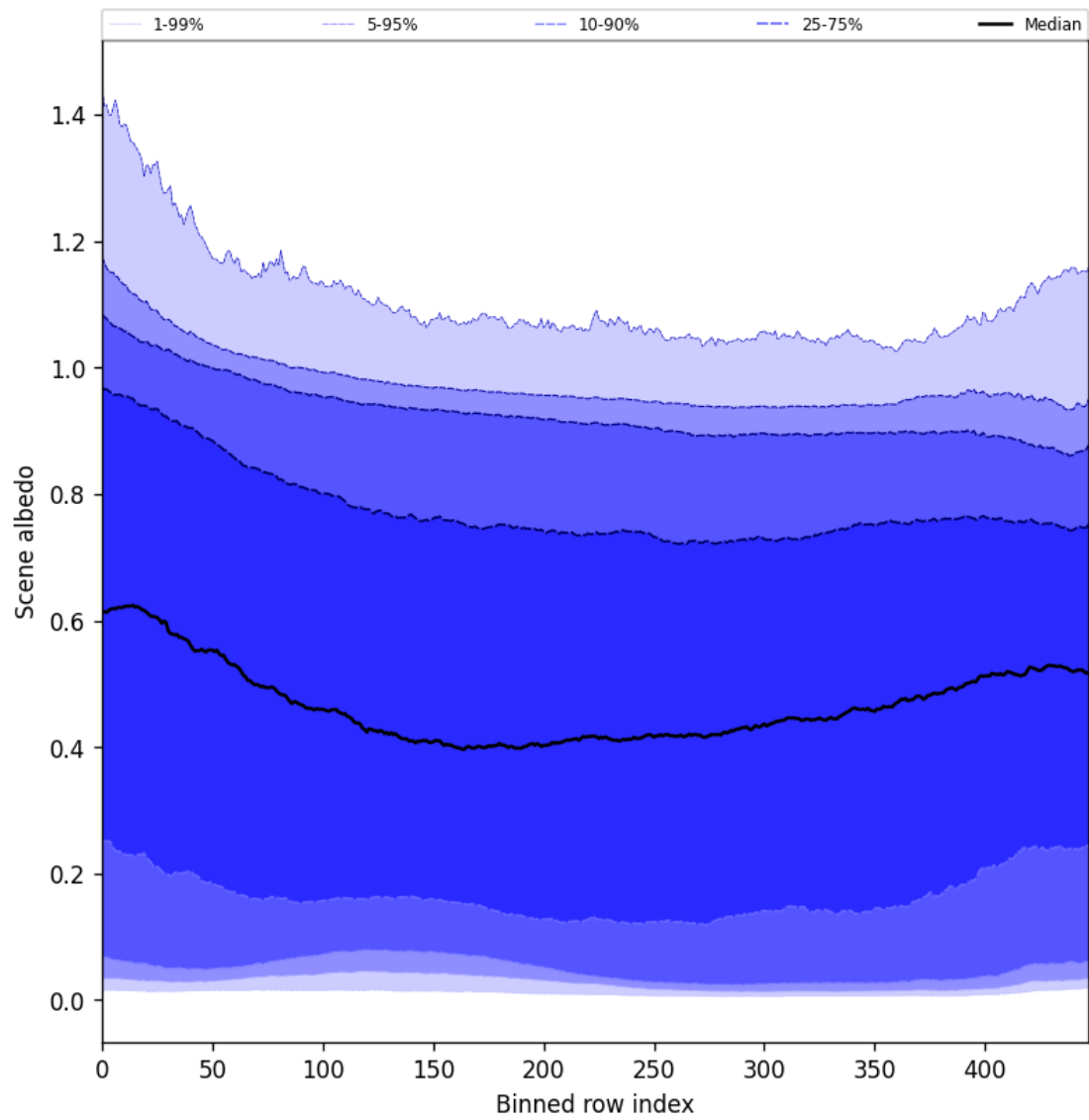
Figure 49: Along track statistics of “Scene albedo” for 2024-12-09 to 2024-12-09
