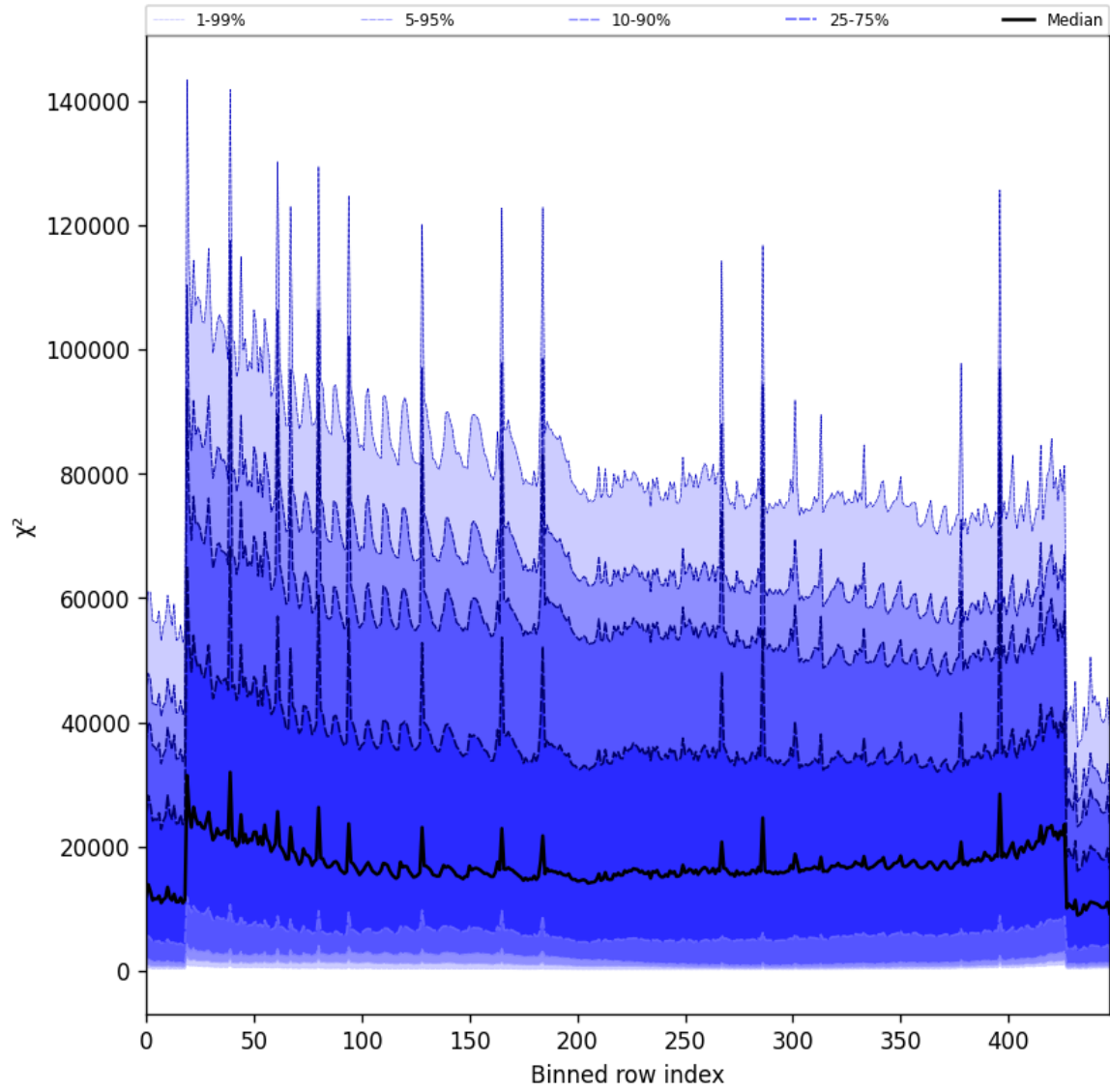
Figure 53: Along track statistics of “ \chi^2 ” for 2024-12-13 to 2024-12-14
