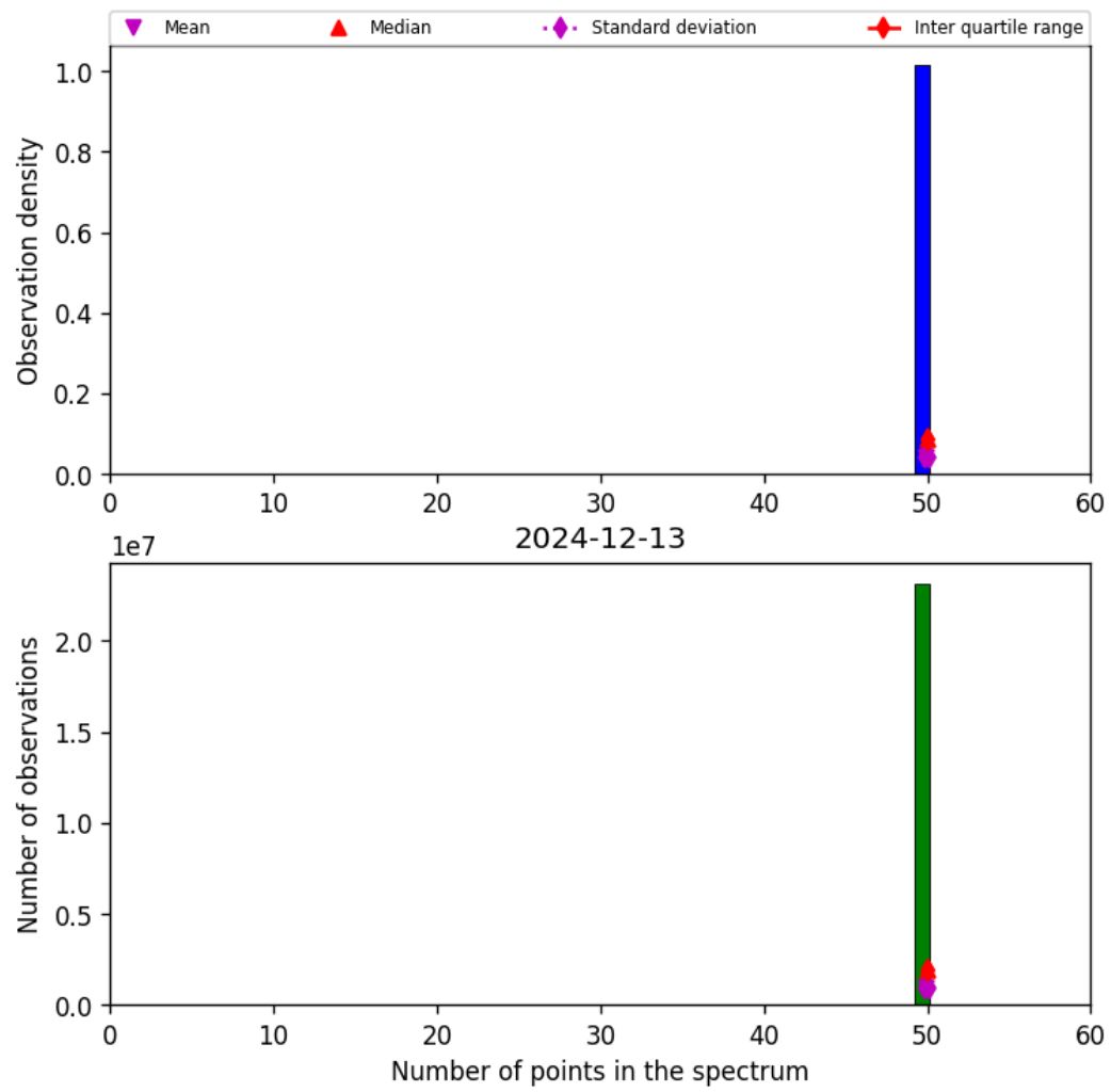
Figure 42: Histogram of “Number of points in the spectrum” for 2024-12-13 to 2024-12-14
