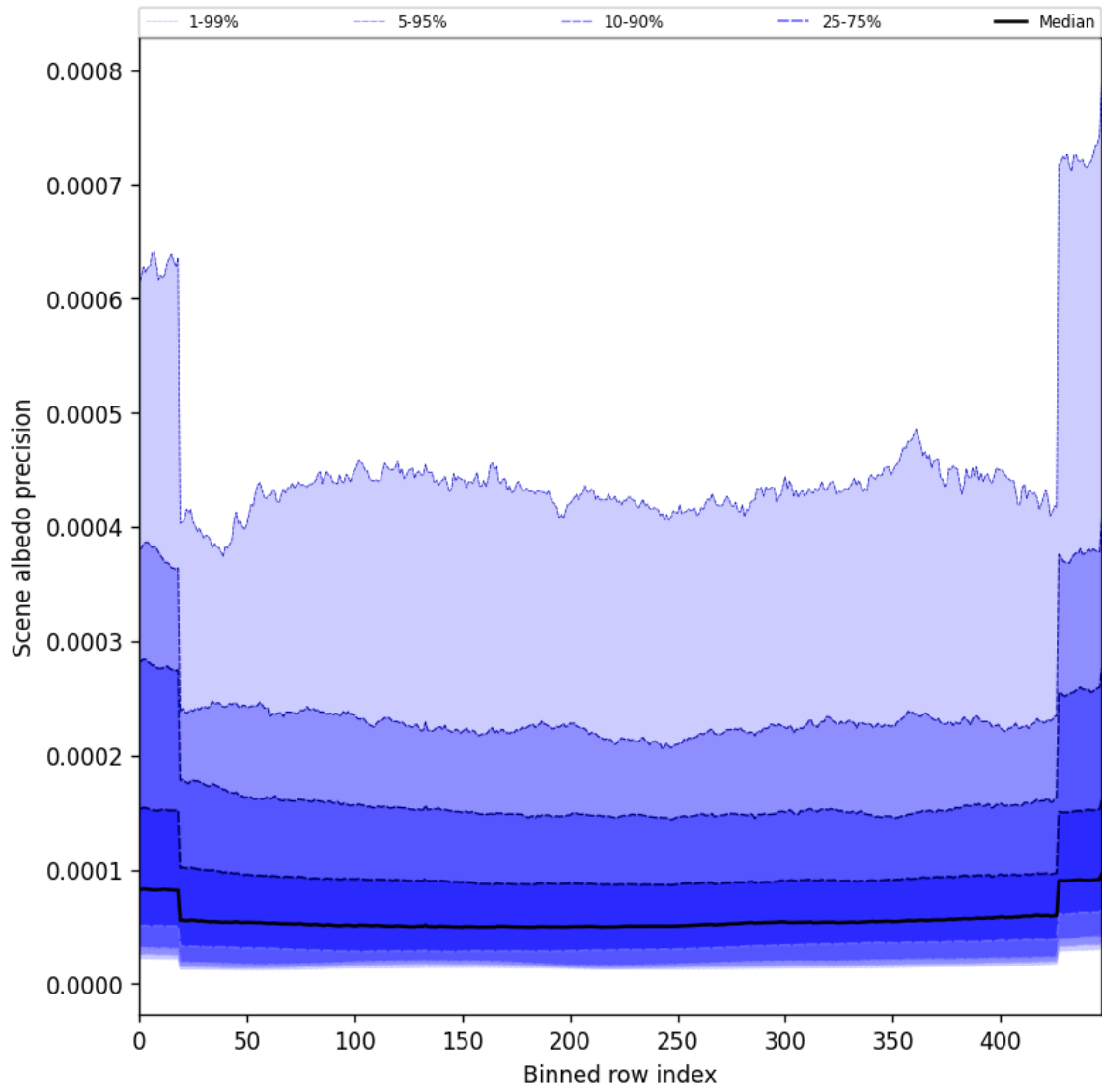
Figure 50: Along track statistics of “Scene albedo precision” for 2024-12-13 to 2024-12-14
