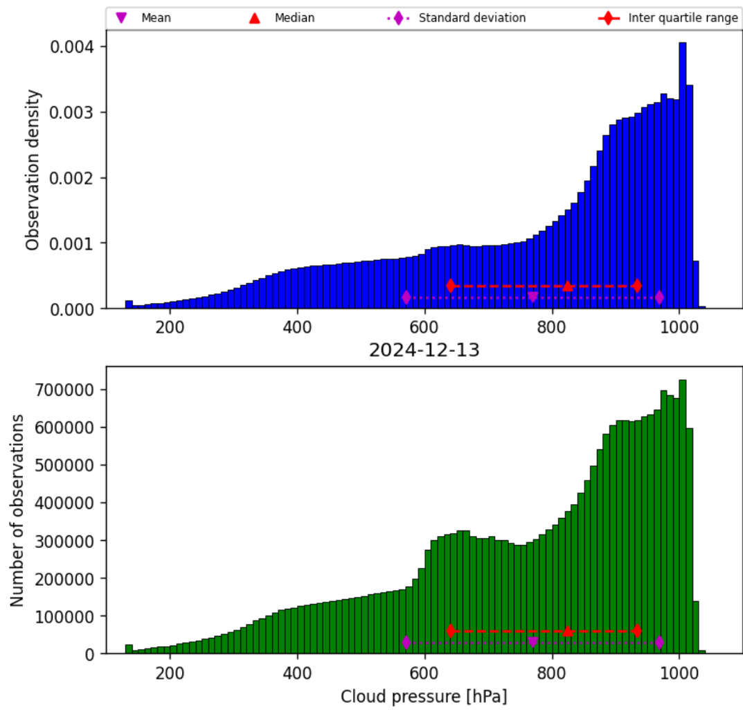
Figure 28: Histogram of “Cloud pressure” for 2024-12-13 to 2024-12-14
