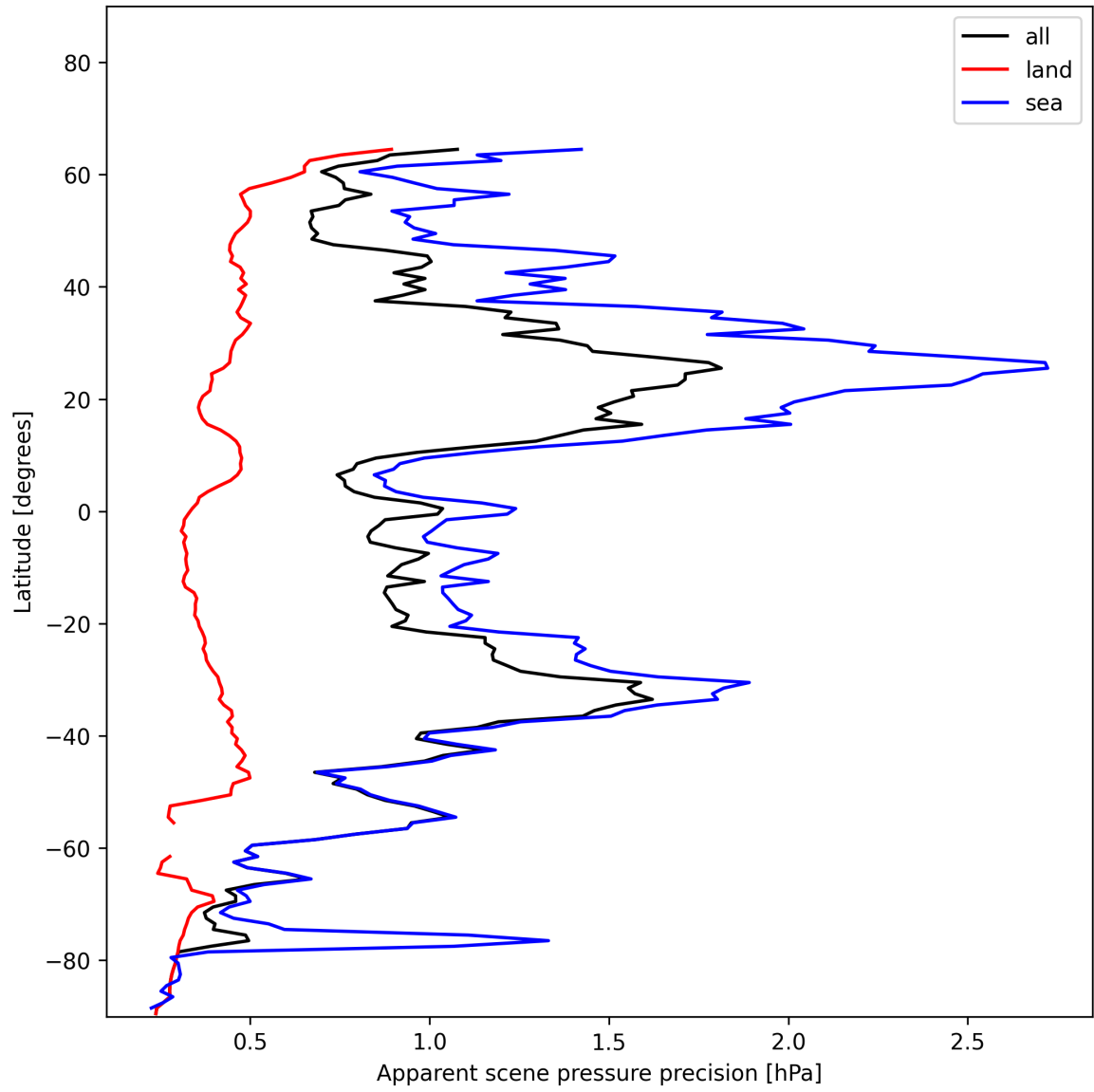
Figure 18: Zonal average of “Apparent scene pressure precision” for 2024-12-13 to 2024-12-14.
