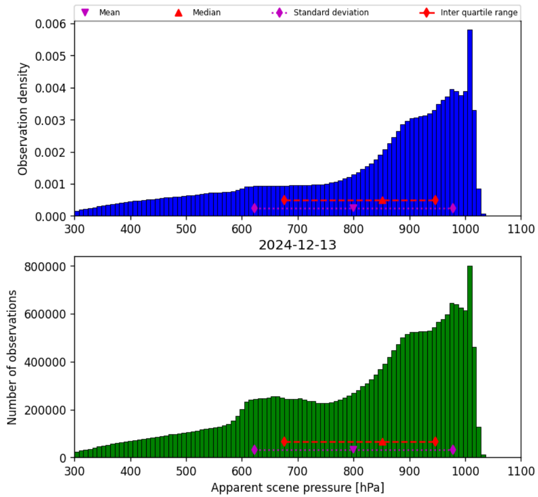
Figure 34: Histogram of “Apparent scene pressure” for 2024-12-13 to 2024-12-14
