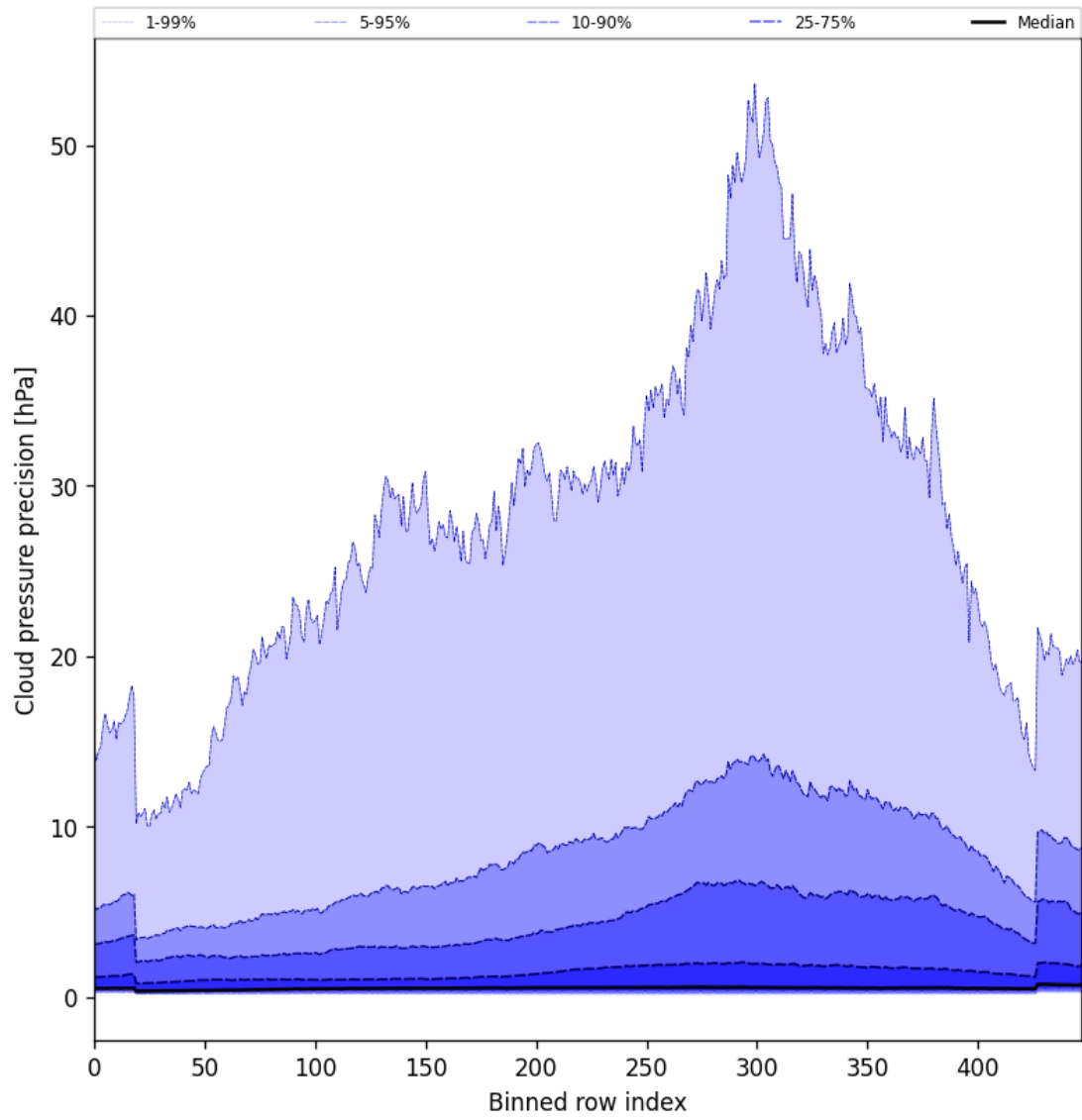
Figure 46: Along track statistics of “Cloud pressure precision” for 2024-12-13 to 2024-12-14
