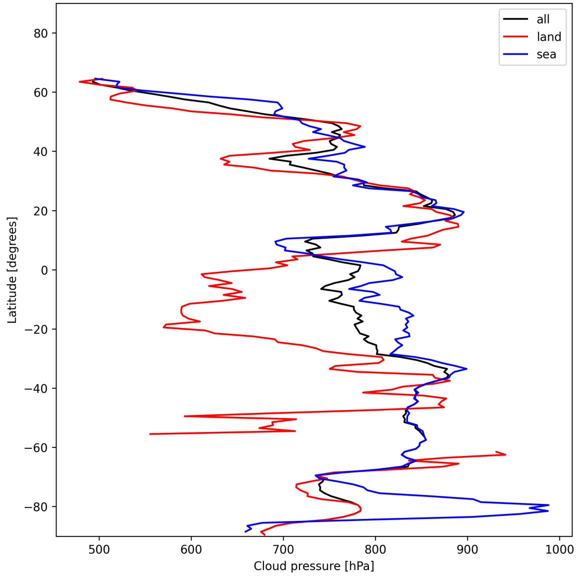
Figure 11: Zonal average of “Cloud pressure” for 2024-12-13 to 2024-12-14.
