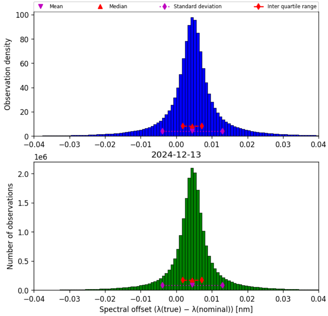
Figure 43: Histogram of “Spectral offset ( \lambda_{\text{true}} - \lambda_{\text{nominal}} )” for 2024-12-13 to 2024-12-14
