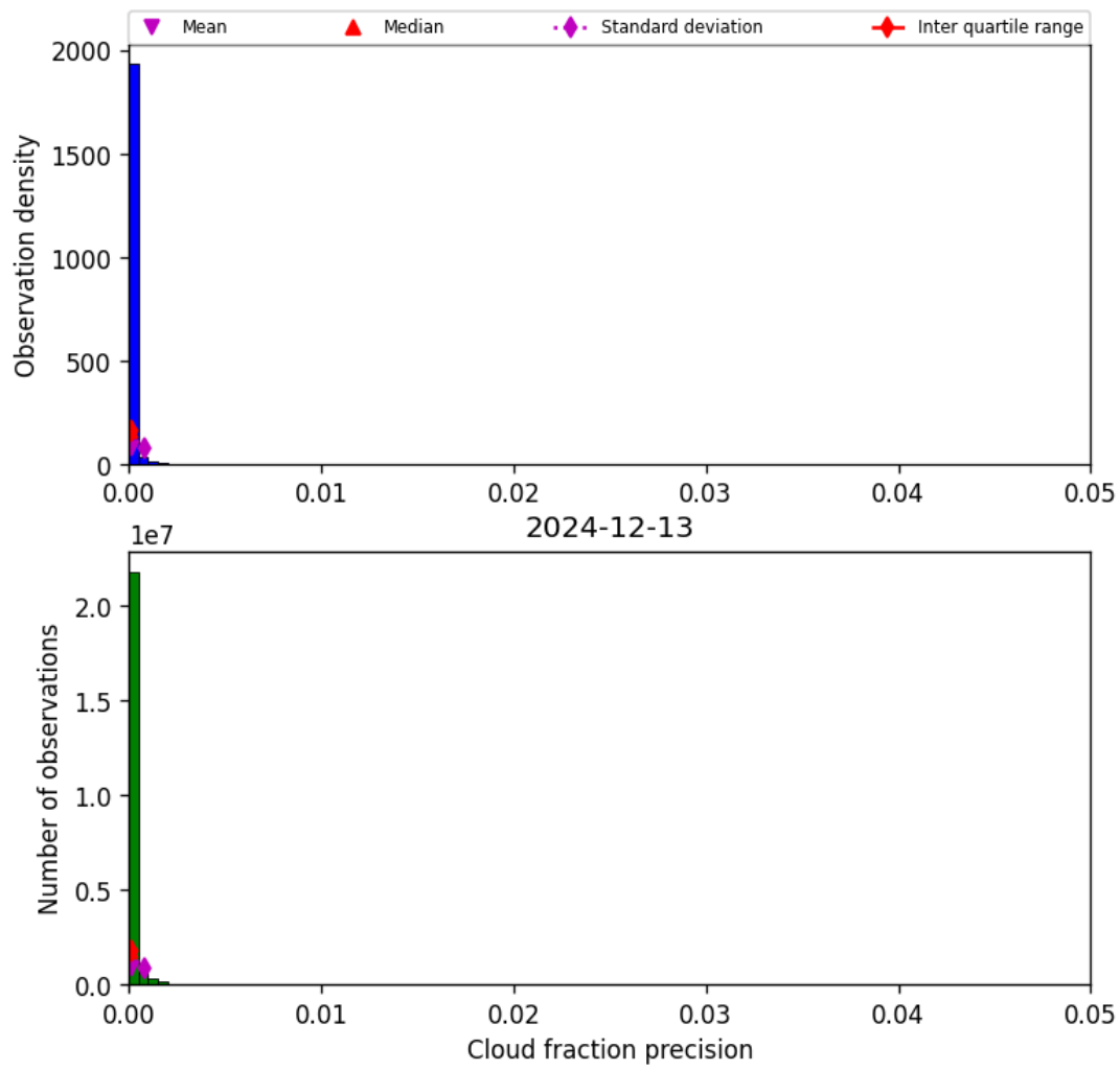
Figure 31: Histogram of “Cloud fraction precision” for 2024-12-13 to 2024-12-14
