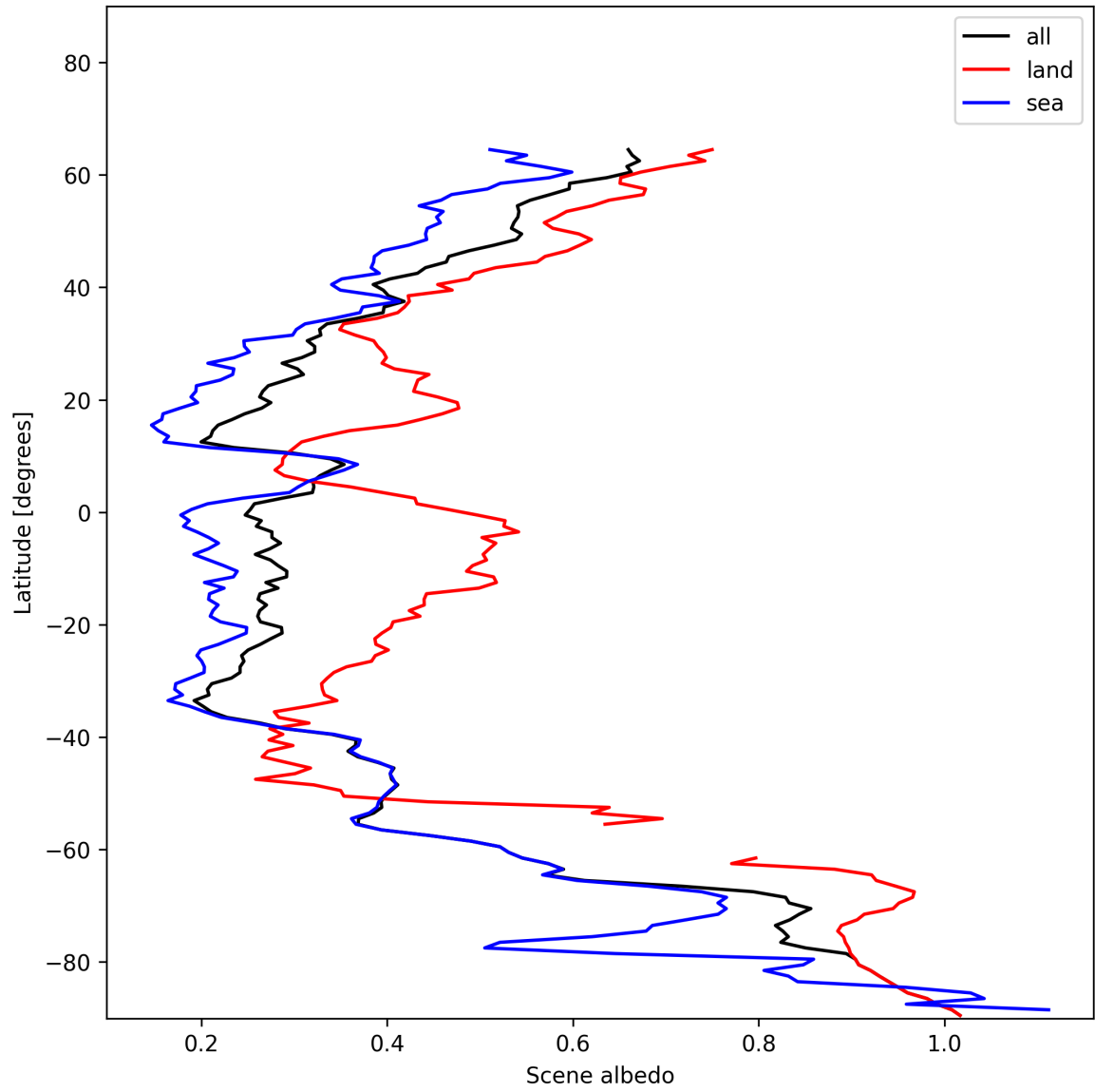
Figure 15: Zonal average of “Scene albedo” for 2024-12-13 to 2024-12-14.
