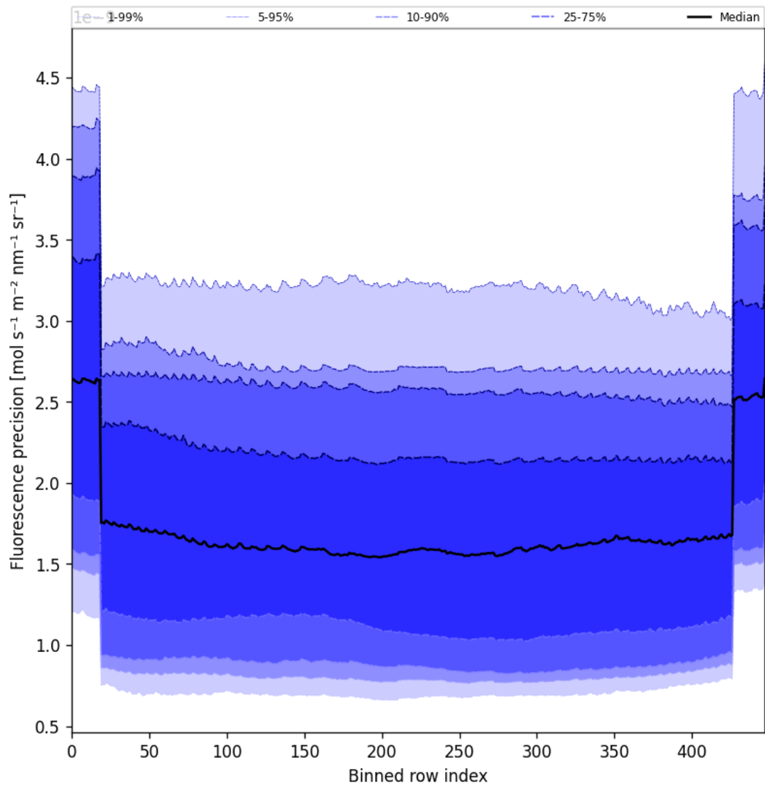
Figure 56: Along track statistics of “Fluorescence precision” for 2024-12-13 to 2024-12-14
