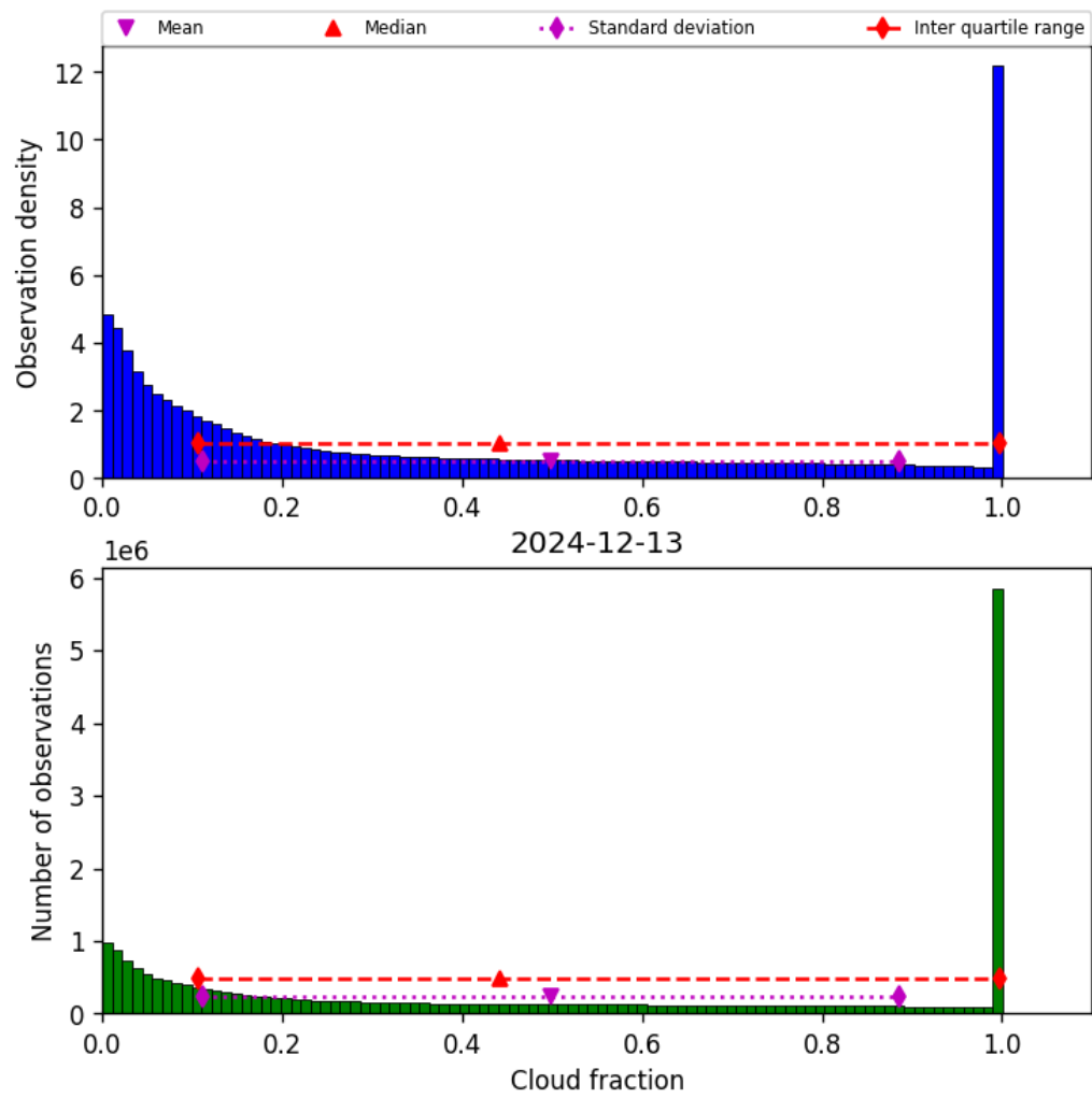
Figure 30: Histogram of “Cloud fraction” for 2024-12-13 to 2024-12-14
