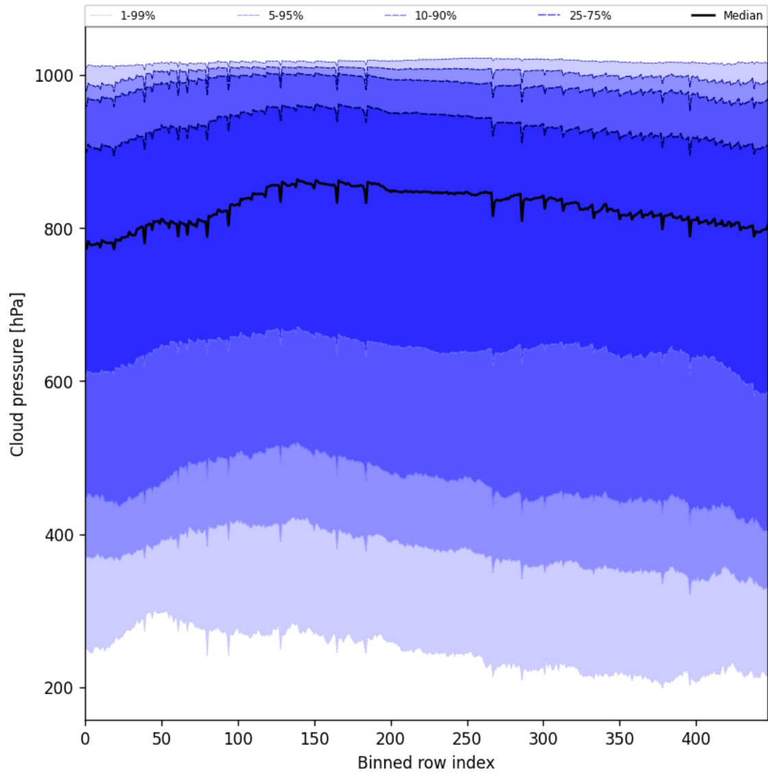
Figure 45: Along track statistics of “Cloud pressure” for 2024-12-13 to 2024-12-14
