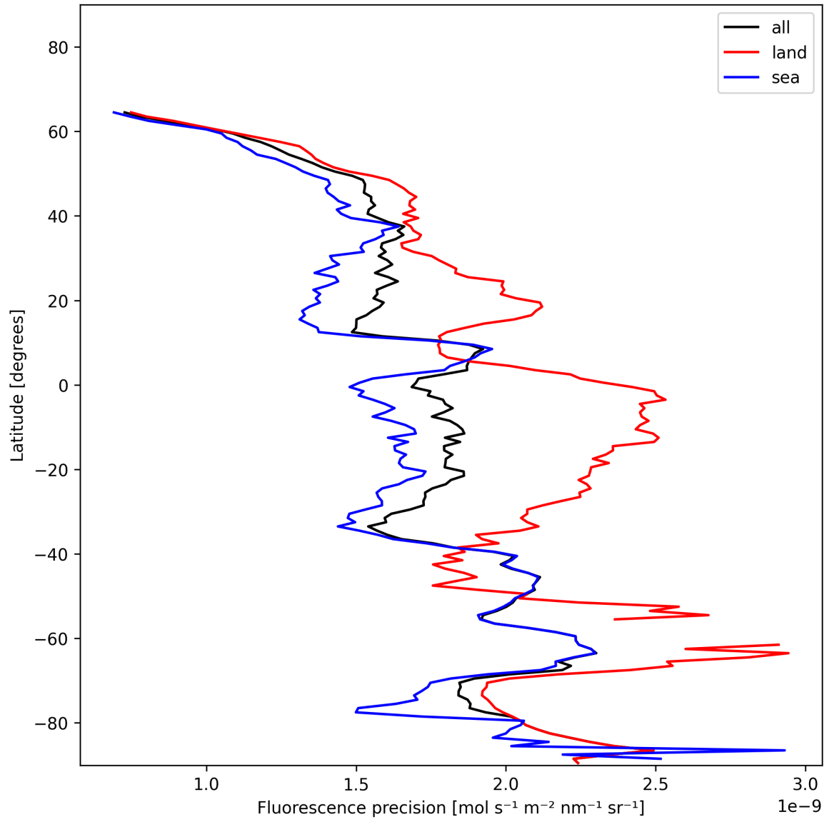
Figure 22: Zonal average of “Fluorescence precision” for 2024-12-13 to 2024-12-14.
