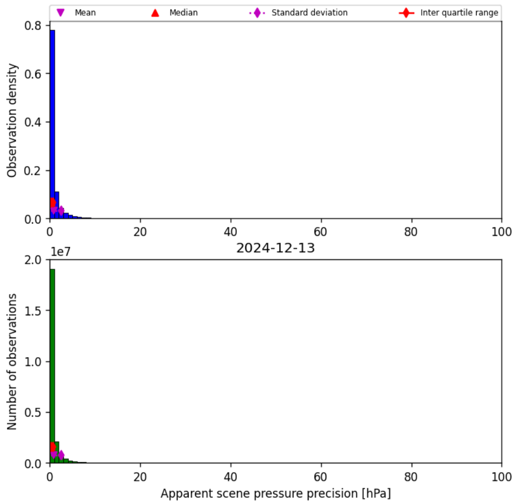
Figure 35: Histogram of “Apparent scene pressure precision” for 2024-12-13 to 2024-12-14
