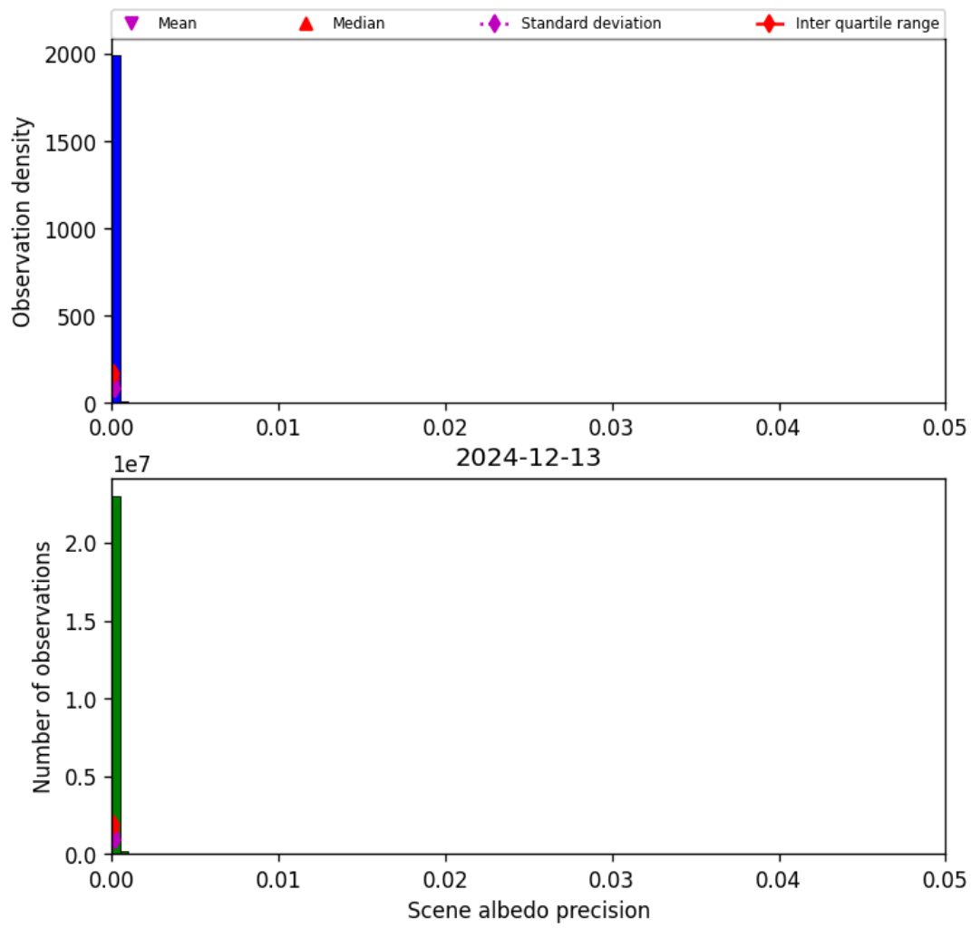
Figure 33: Histogram of “Scene albedo precision” for 2024-12-13 to 2024-12-14
