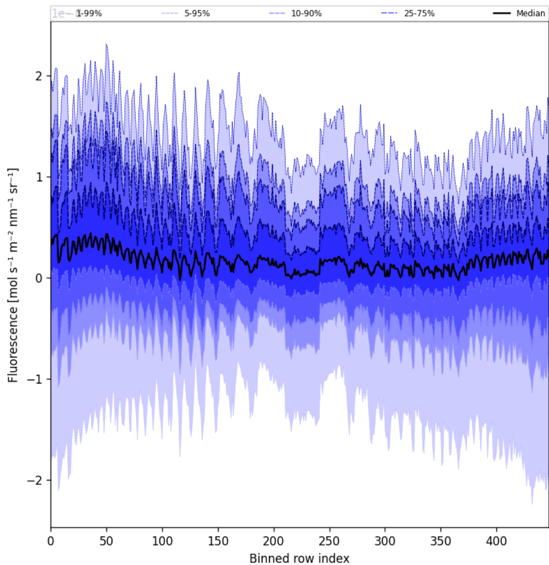
Figure 55: Along track statistics of “Fluorescence” for 2024-12-13 to 2024-12-14
