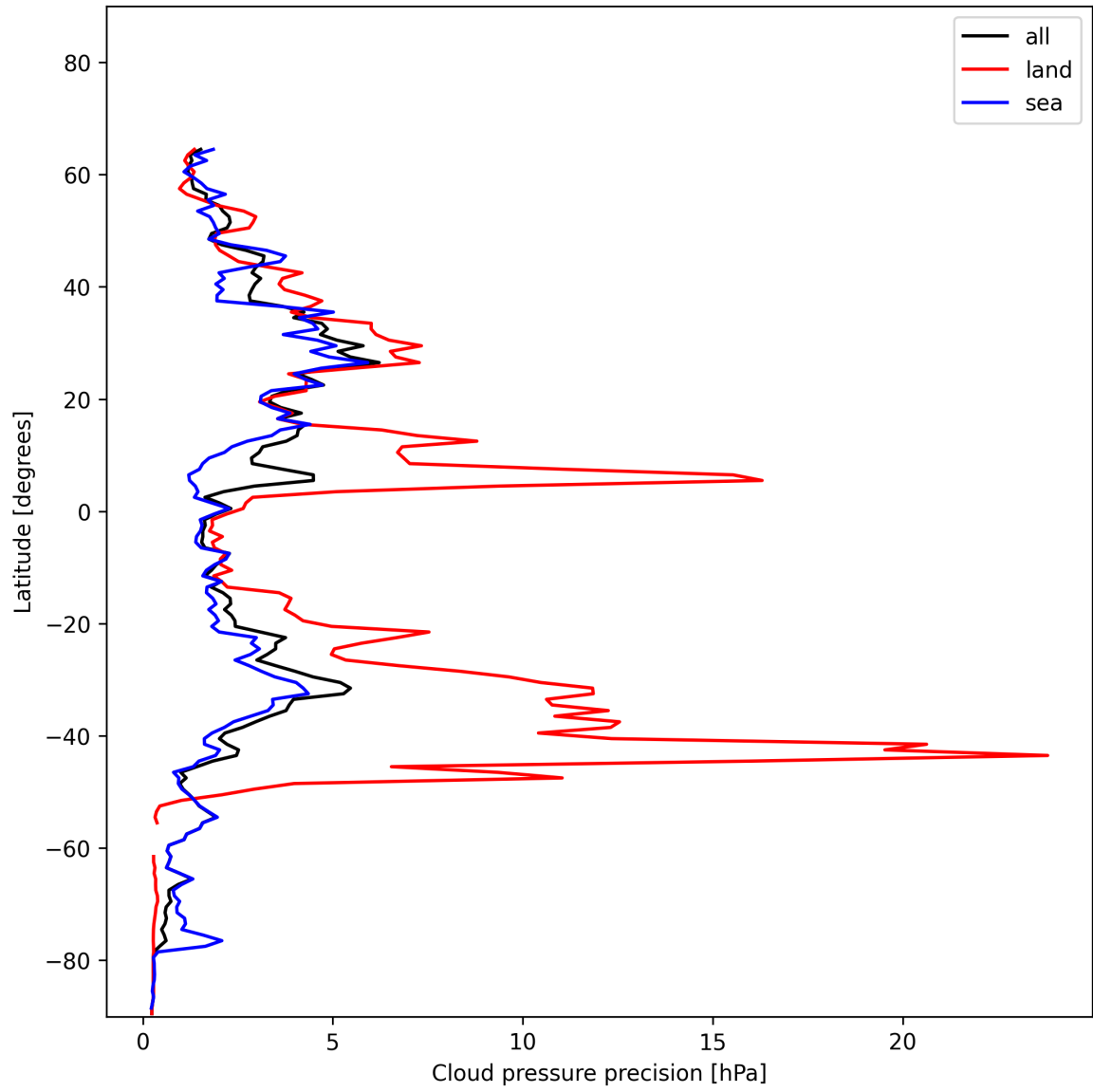
Figure 12: Zonal average of “Cloud pressure precision” for 2024-12-13 to 2024-12-14.
