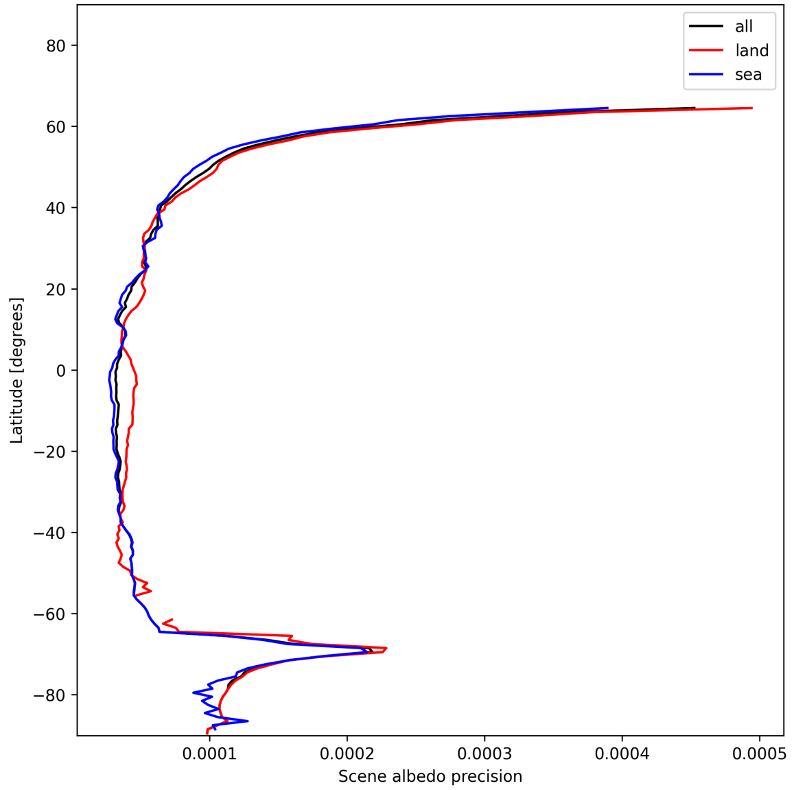
Figure 16: Zonal average of “Scene albedo precision” for 2024-12-13 to 2024-12-14.
