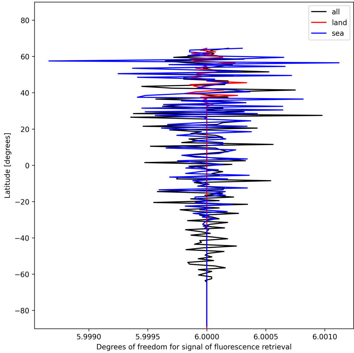
Figure 24: Zonal average of “Degrees of freedom for signal of fluorescence retrieval” for 2024-12-13 to 2024-12-14.
