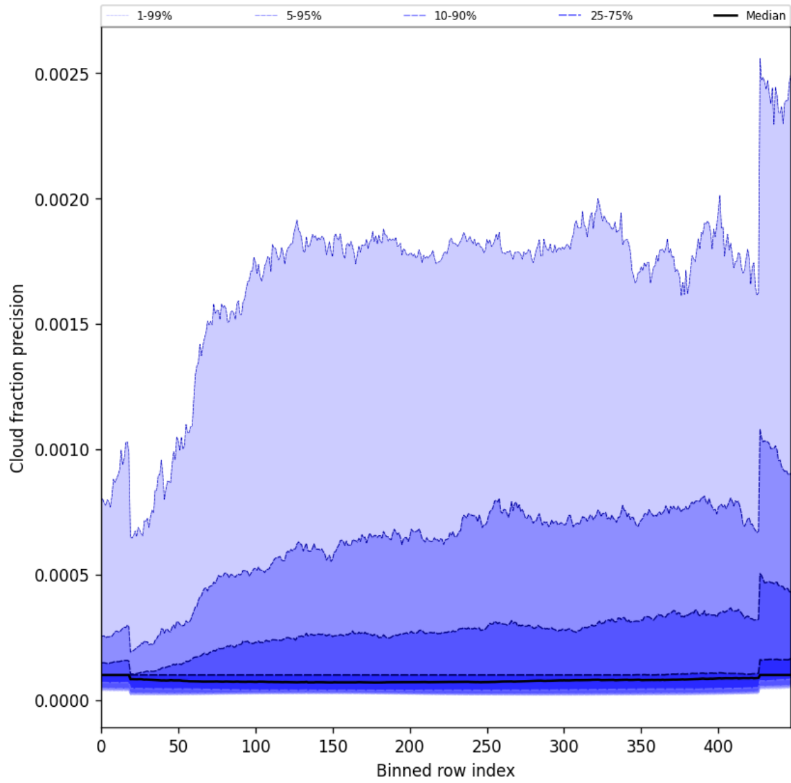
Figure 48: Along track statistics of “Cloud fraction precision” for 2024-12-13 to 2024-12-14
