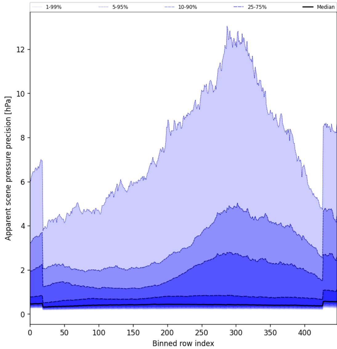
Figure 52: Along track statistics of “Apparent scene pressure precision” for 2024-12-13 to 2024-12-14
