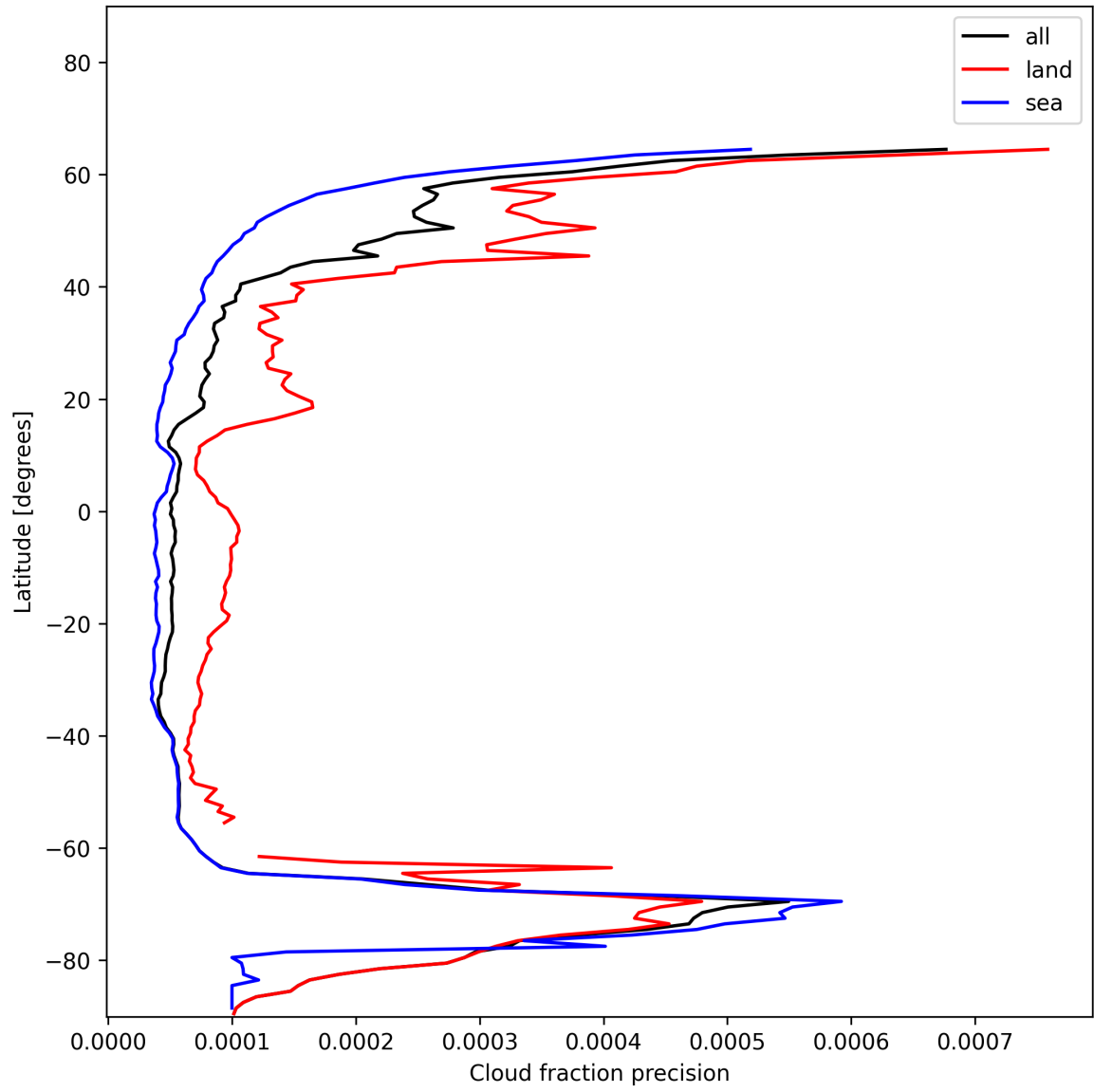
Figure 14: Zonal average of “Cloud fraction precision” for 2024-12-13 to 2024-12-14.
