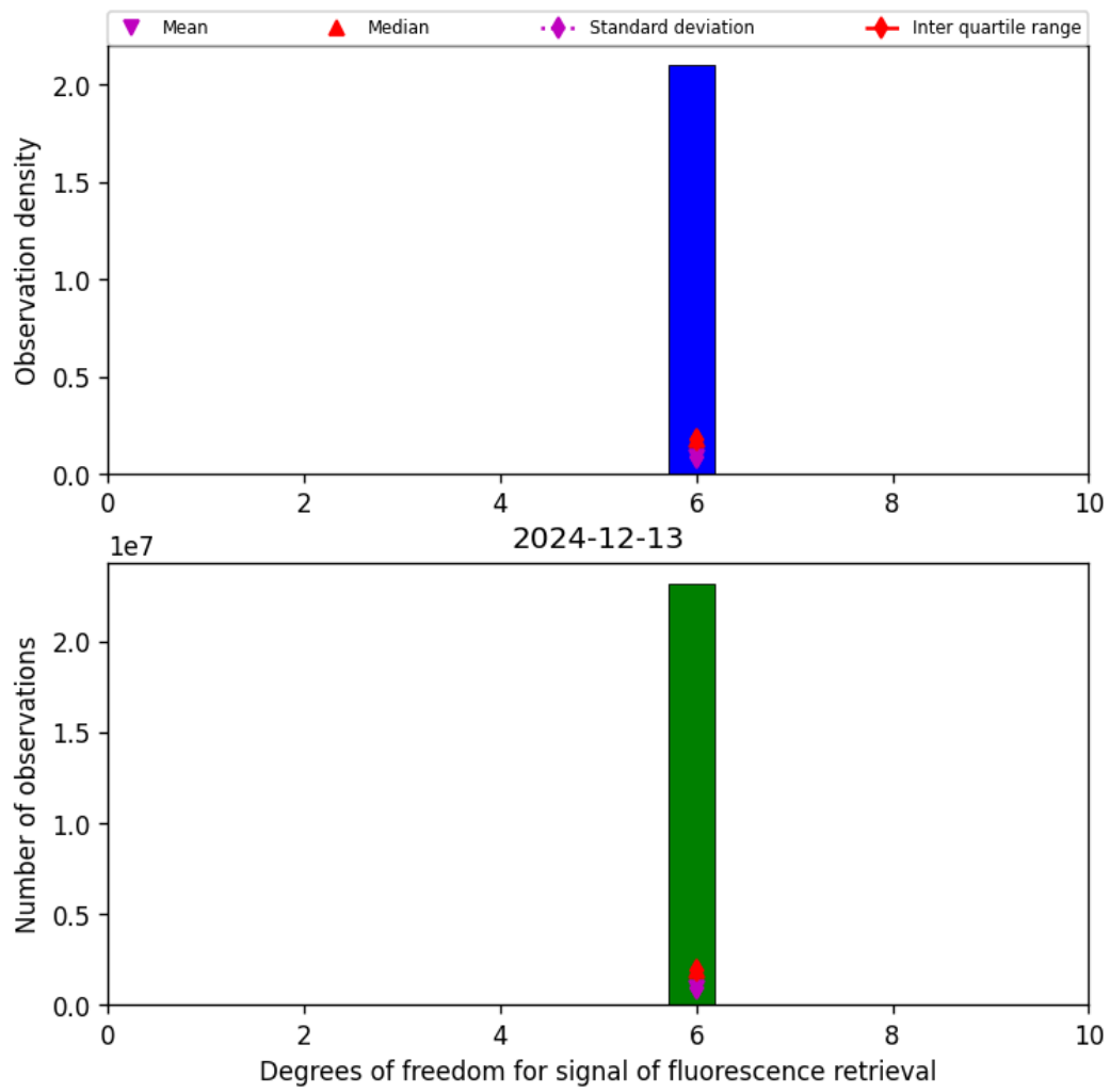
Figure 41: Histogram of “Degrees of freedom for signal of fluorescence retrieval” for 2024-12-13 to 2024-12-14
