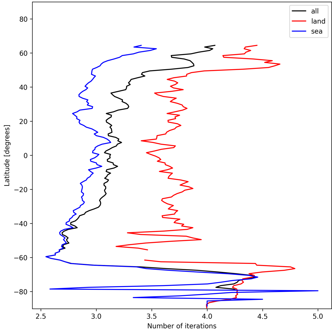
Figure 20: Zonal average of “Number of iterations” for 2024-12-13 to 2024-12-14.
