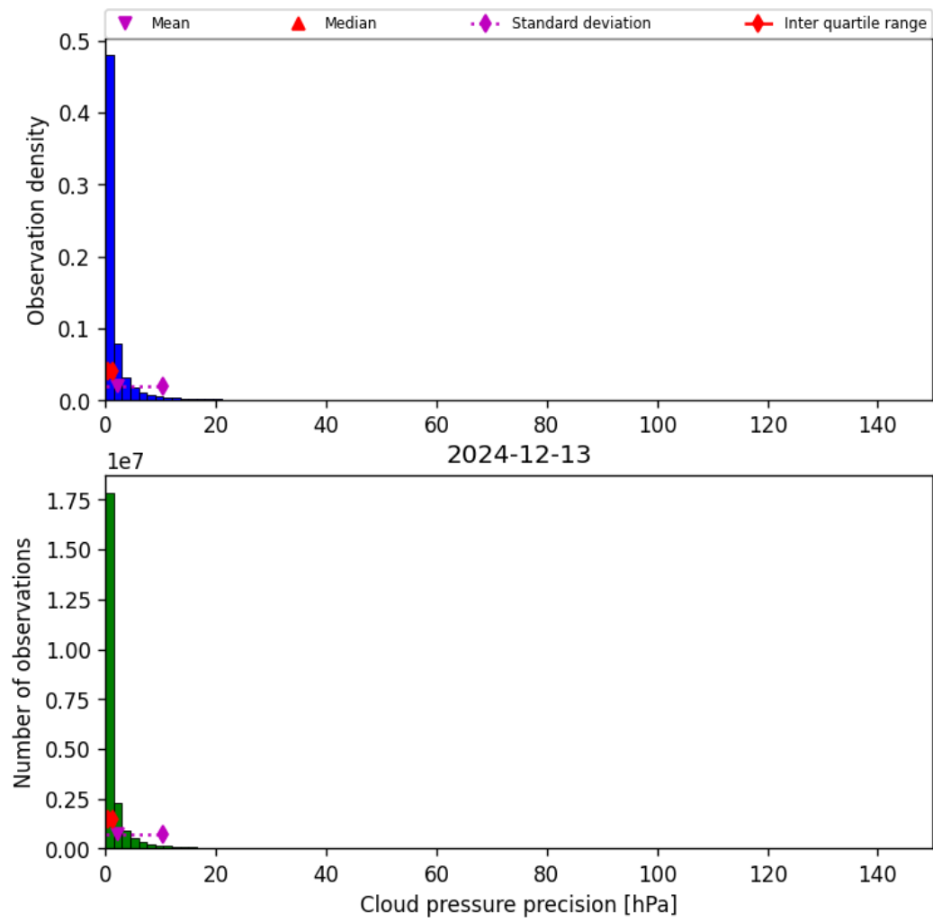
Figure 29: Histogram of “Cloud pressure precision” for 2024-12-13 to 2024-12-14
