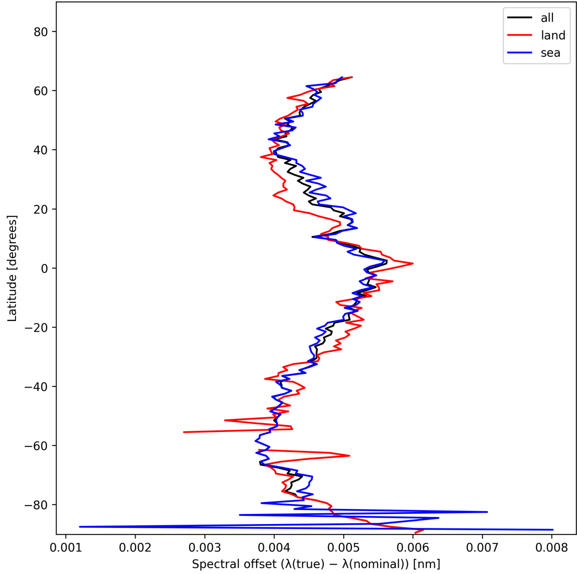
Figure 26: Zonal average of “Spectral offset ( \lambda_{\text{true}} - \lambda_{\text{nominal}} )” for 2024-12-13 to 2024-12-14.
