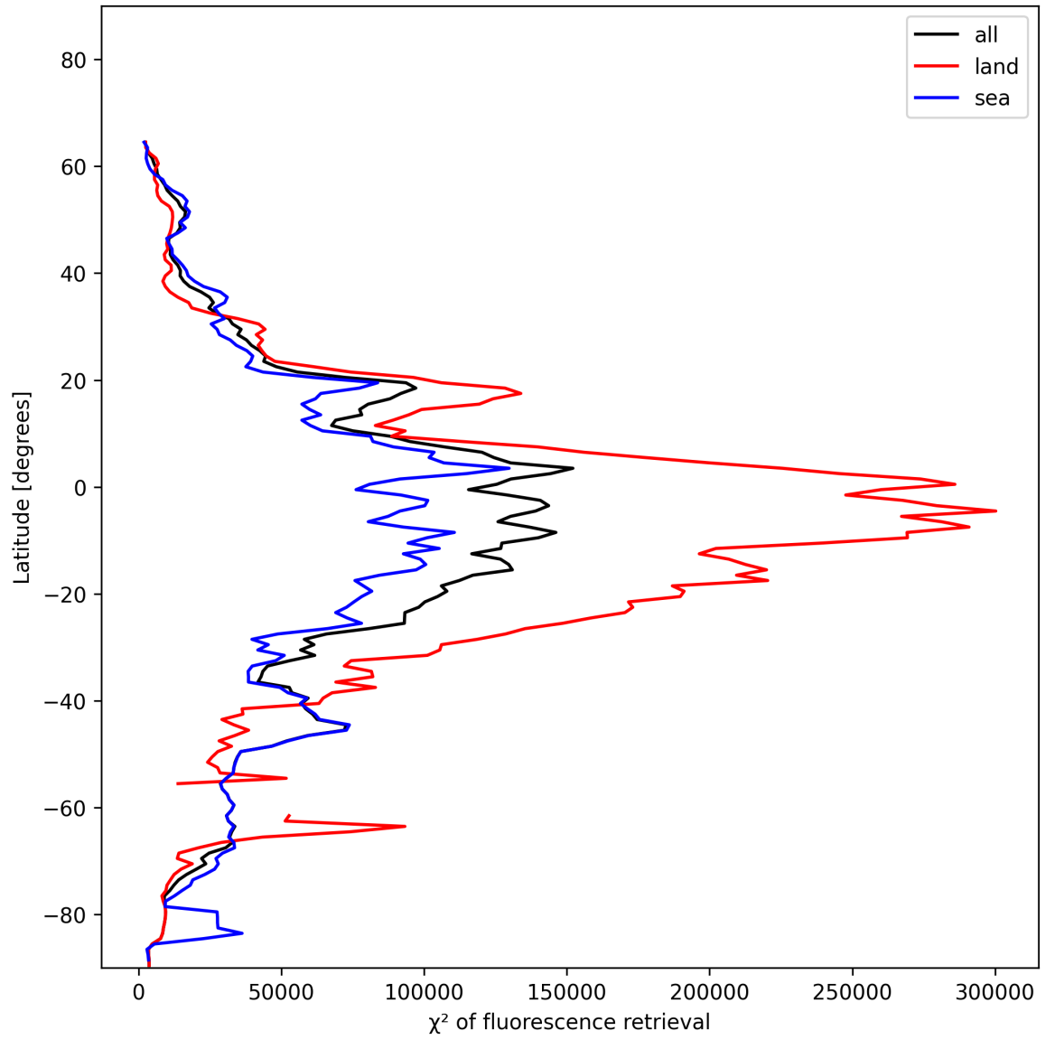
Figure 23: Zonal average of “ \chi^2 of fluorescence retrieval” for 2024-12-13 to 2024-12-14.
