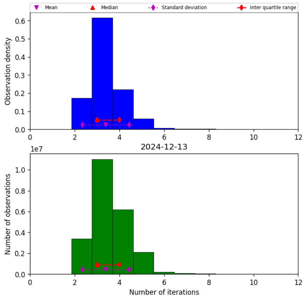
Figure 37: Histogram of “Number of iterations” for 2024-12-13 to 2024-12-14
