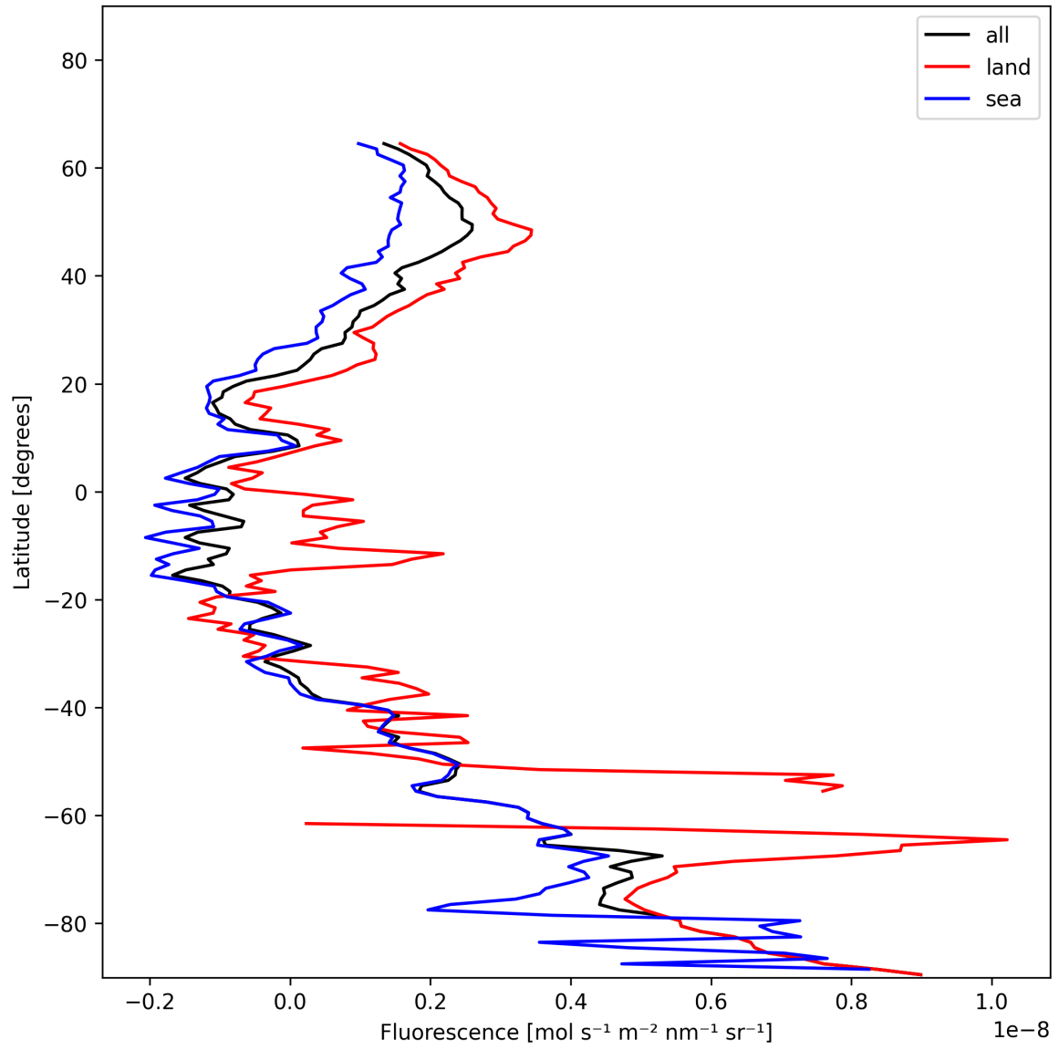
Figure 21: Zonal average of “Fluorescence” for 2024-12-13 to 2024-12-14.
