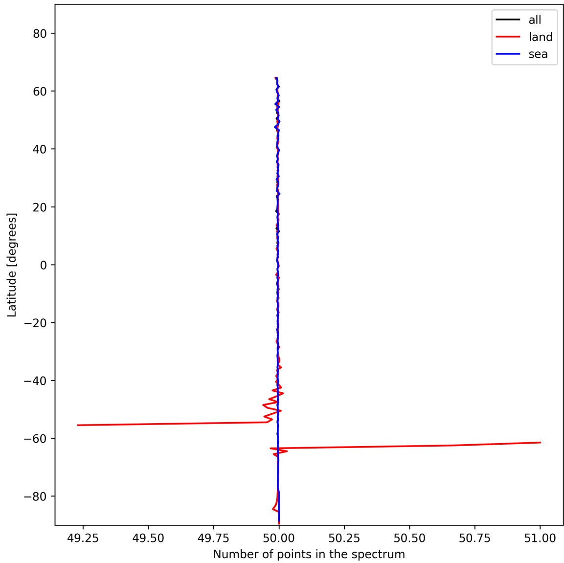
Figure 25: Zonal average of “Number of points in the spectrum” for 2024-12-13 to 2024-12-14.
