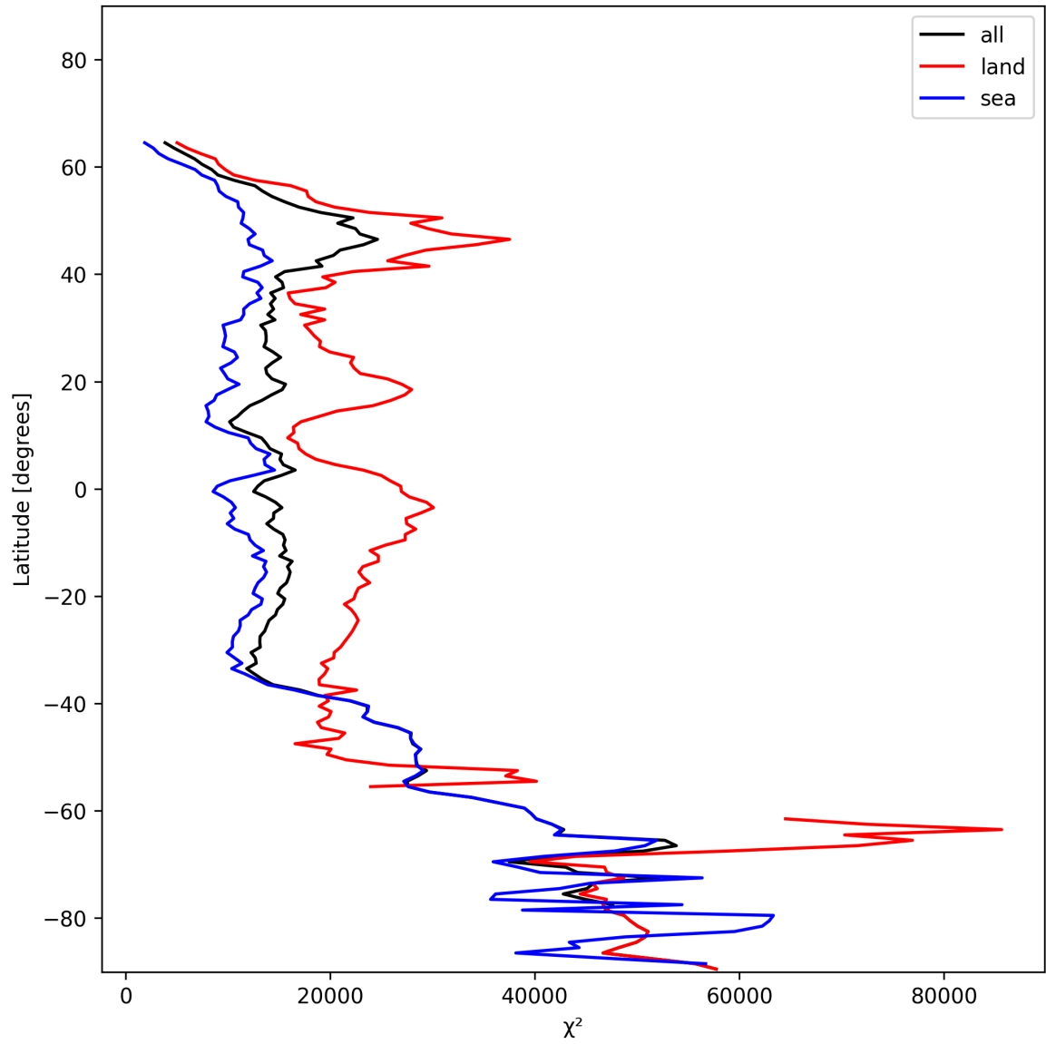
Figure 19: Zonal average of “ \chi^2 ” for 2024-12-13 to 2024-12-14.
