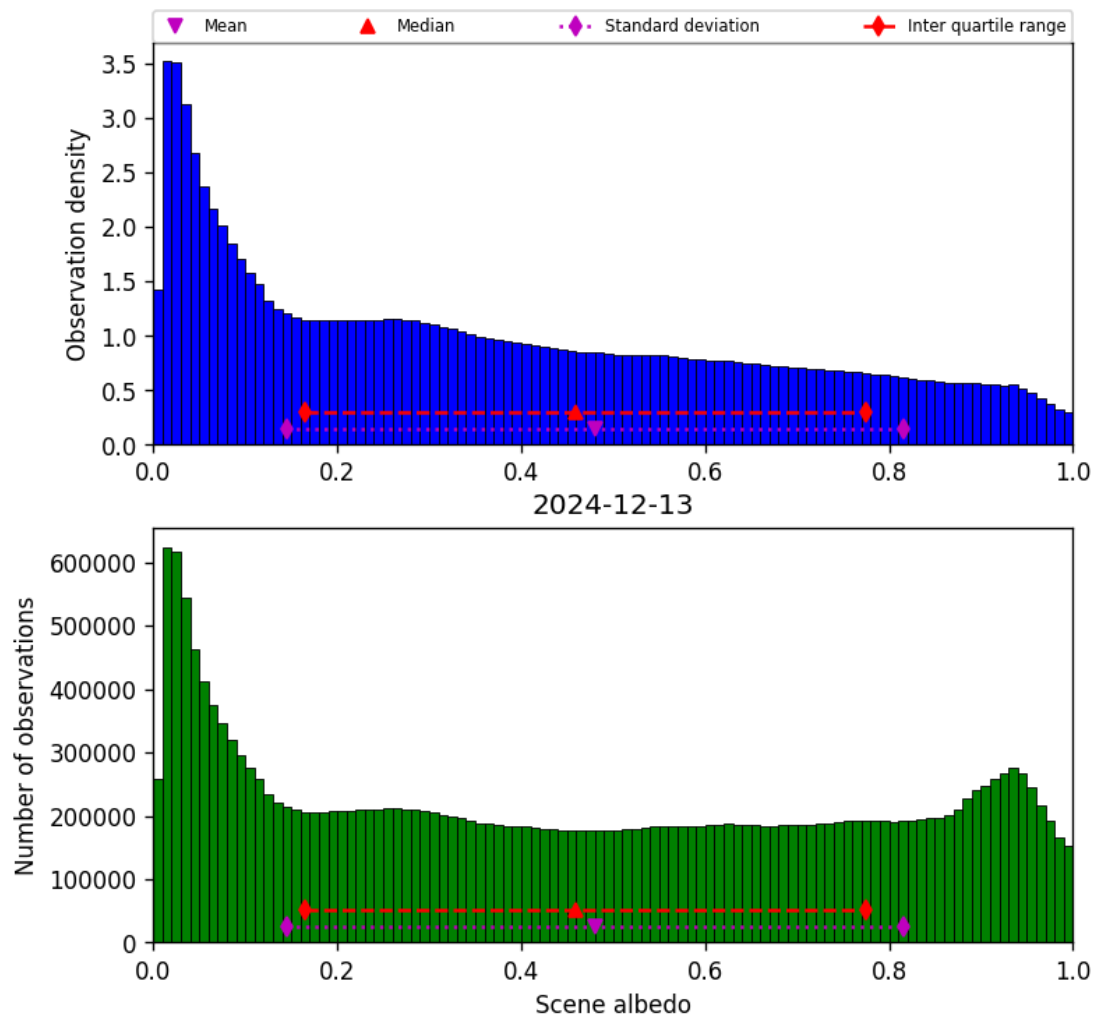
Figure 32: Histogram of “Scene albedo” for 2024-12-13 to 2024-12-14
