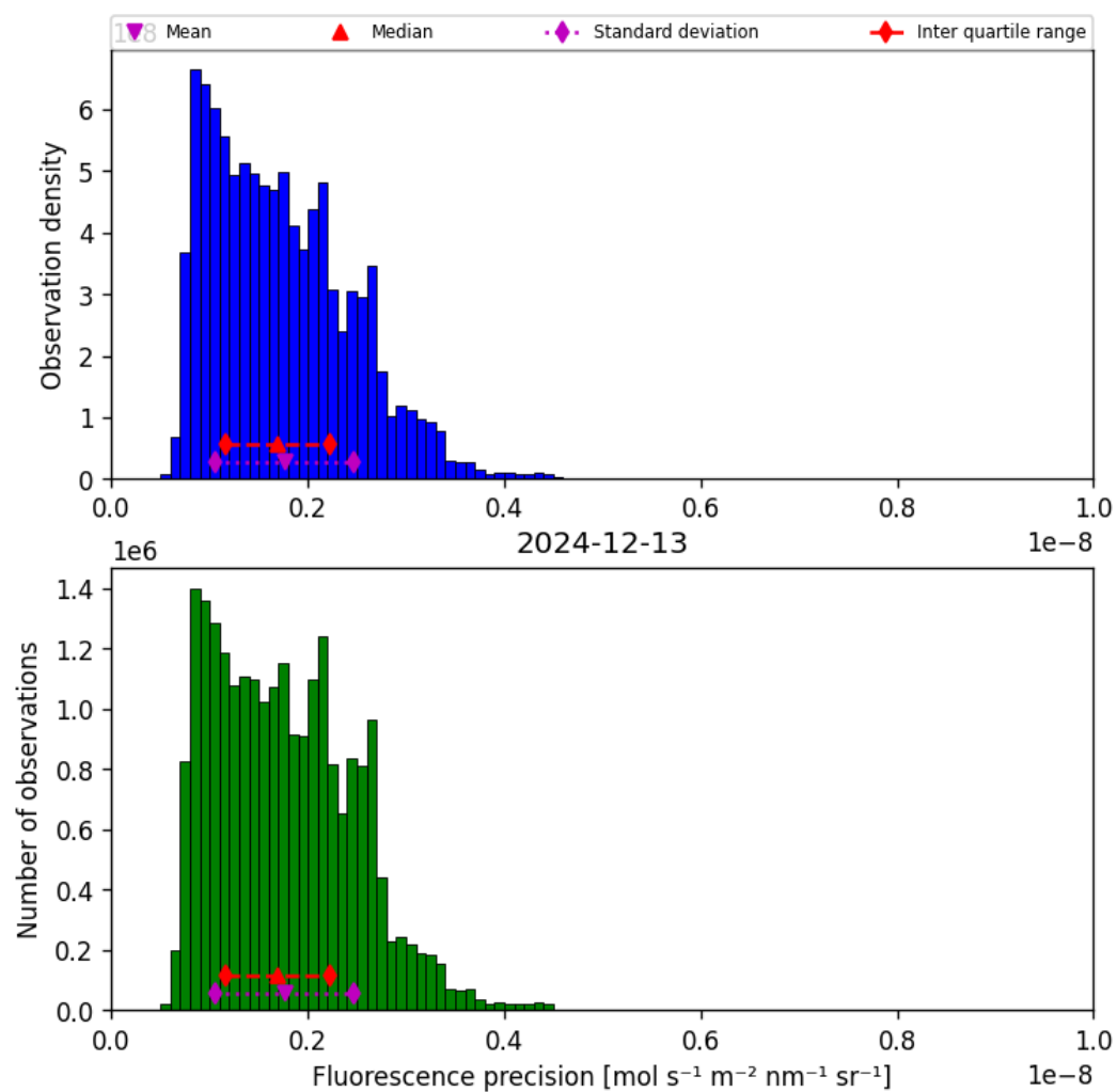
Figure 39: Histogram of “Fluorescence precision” for 2024-12-13 to 2024-12-14
