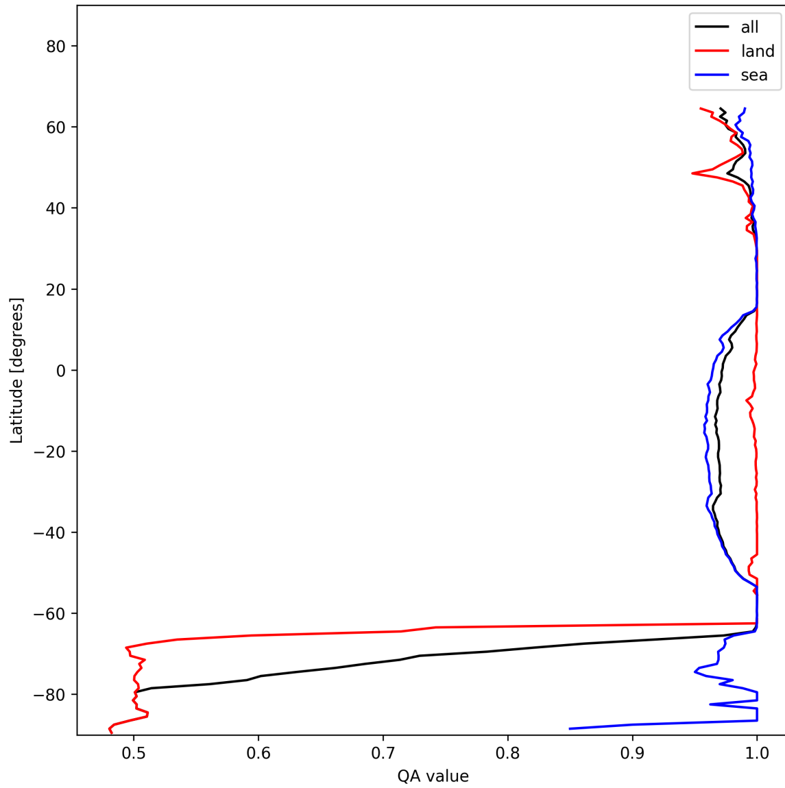
Figure 10: Zonal average of “QA value” for 2024-12-13 to 2024-12-14.
