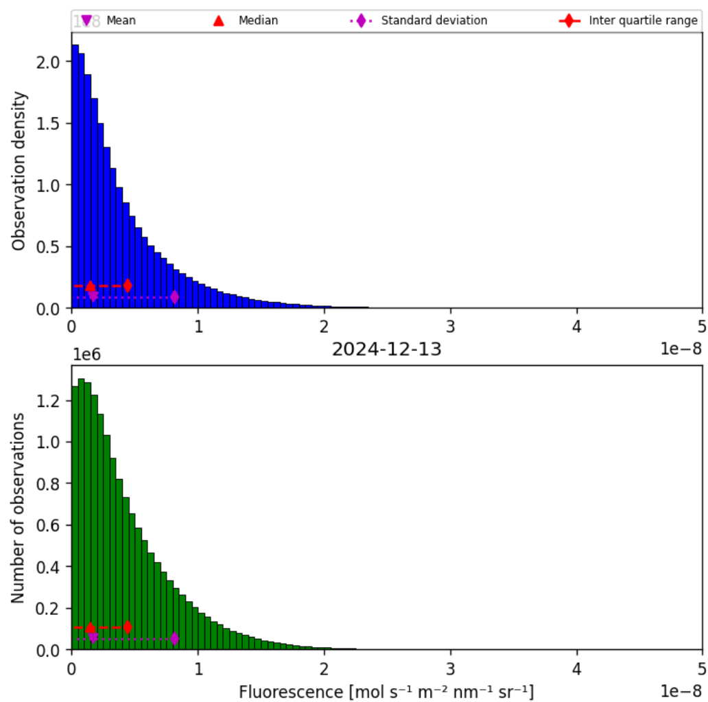
Figure 38: Histogram of “Fluorescence” for 2024-12-13 to 2024-12-14
