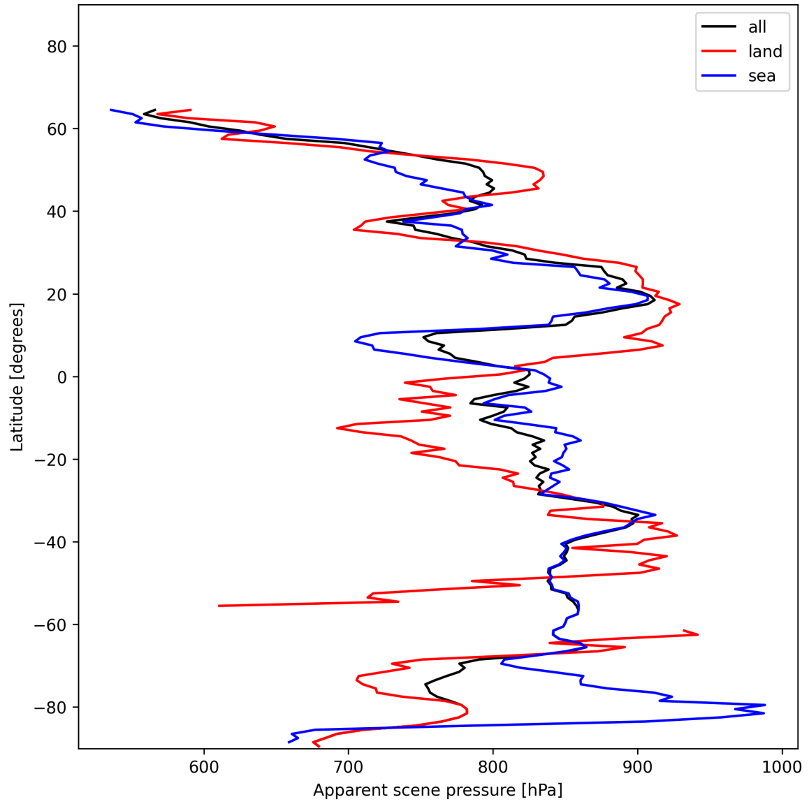
Figure 17: Zonal average of “Apparent scene pressure” for 2024-12-13 to 2024-12-14.
