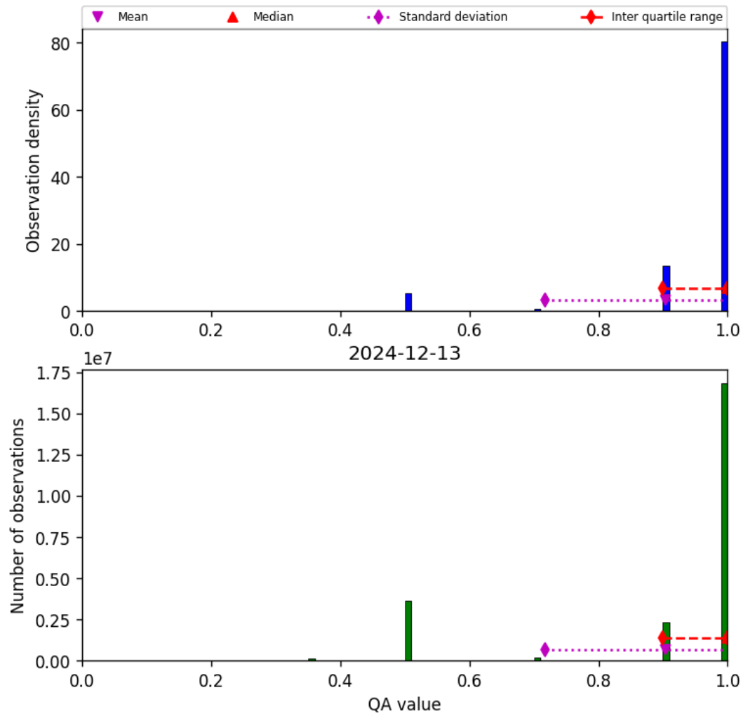
Figure 27: Histogram of “QA value” for 2024-12-13 to 2024-12-14
