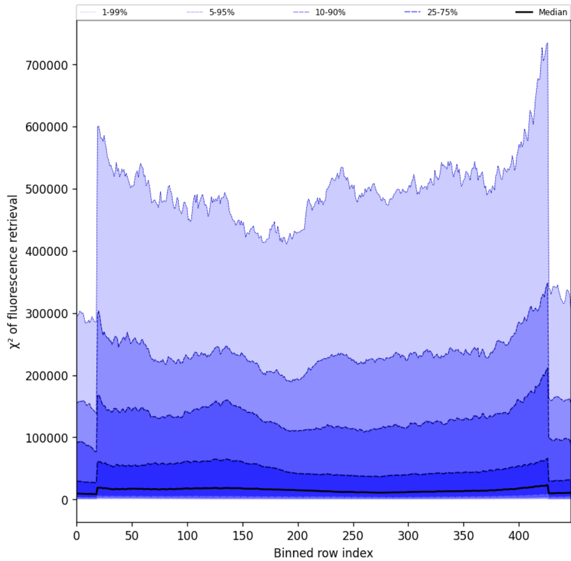
Figure 57: Along track statistics of “ \chi^2 of fluorescence retrieval” for 2024-12-13 to 2024-12-14
