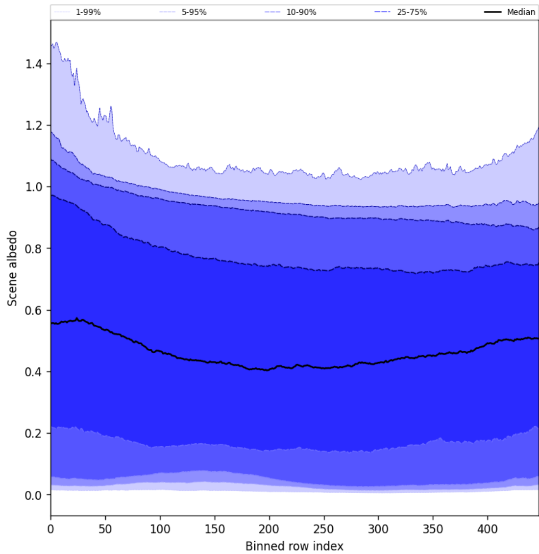
Figure 49: Along track statistics of “Scene albedo” for 2024-12-13 to 2024-12-14
