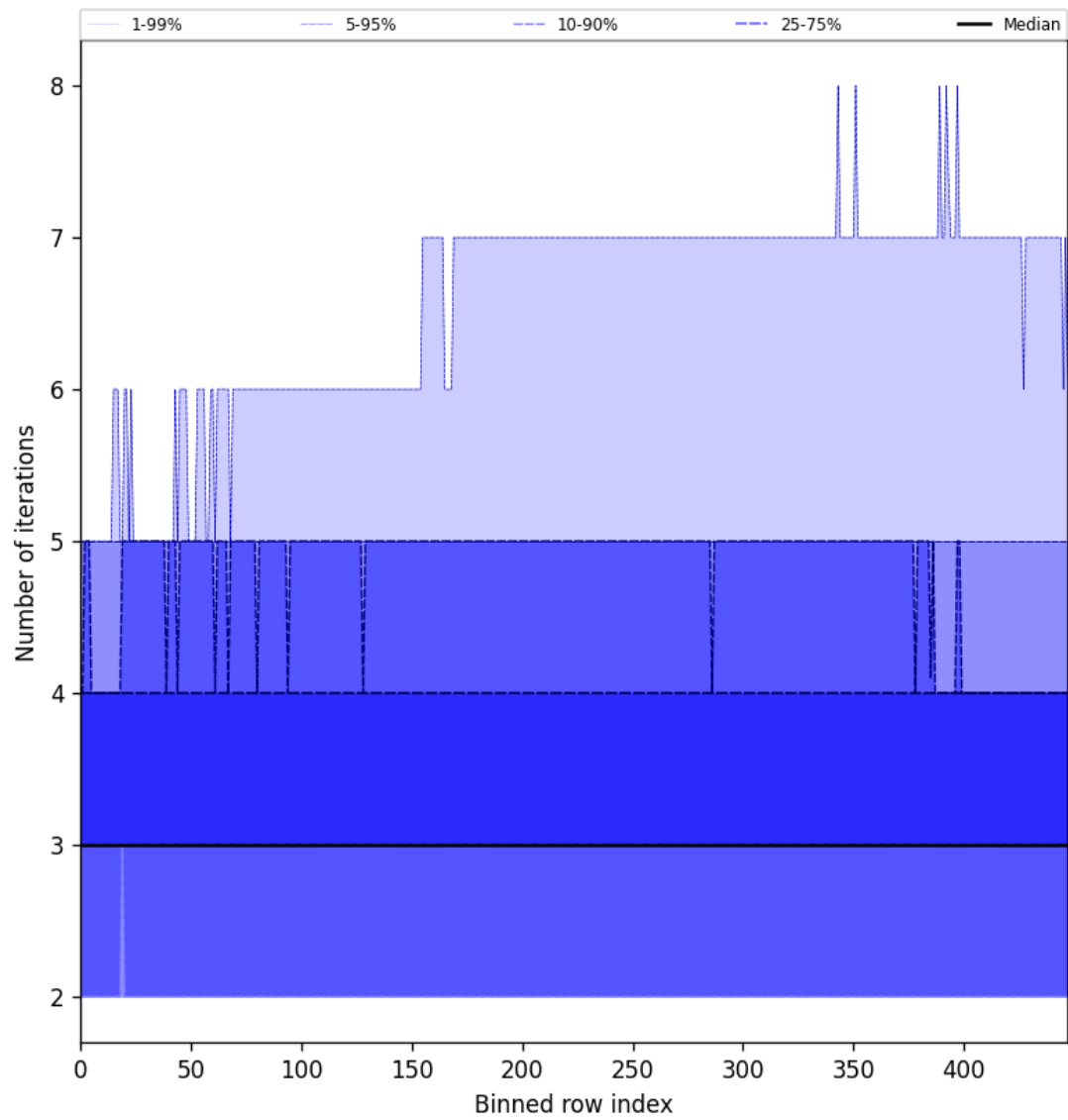
Figure 54: Along track statistics of “Number of iterations” for 2024-12-13 to 2024-12-14
