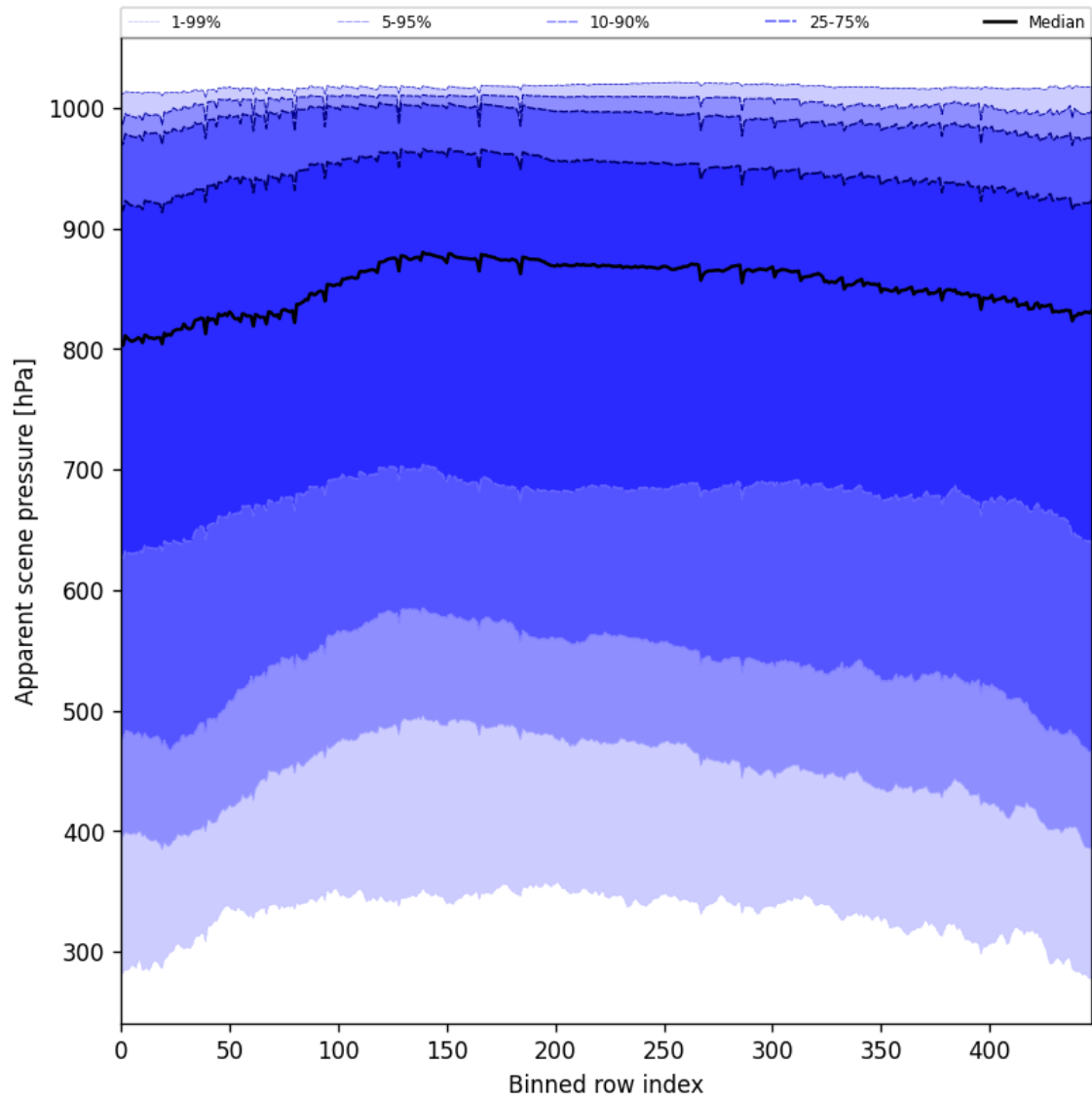
Figure 51: Along track statistics of “Apparent scene pressure” for 2024-12-13 to 2024-12-14
