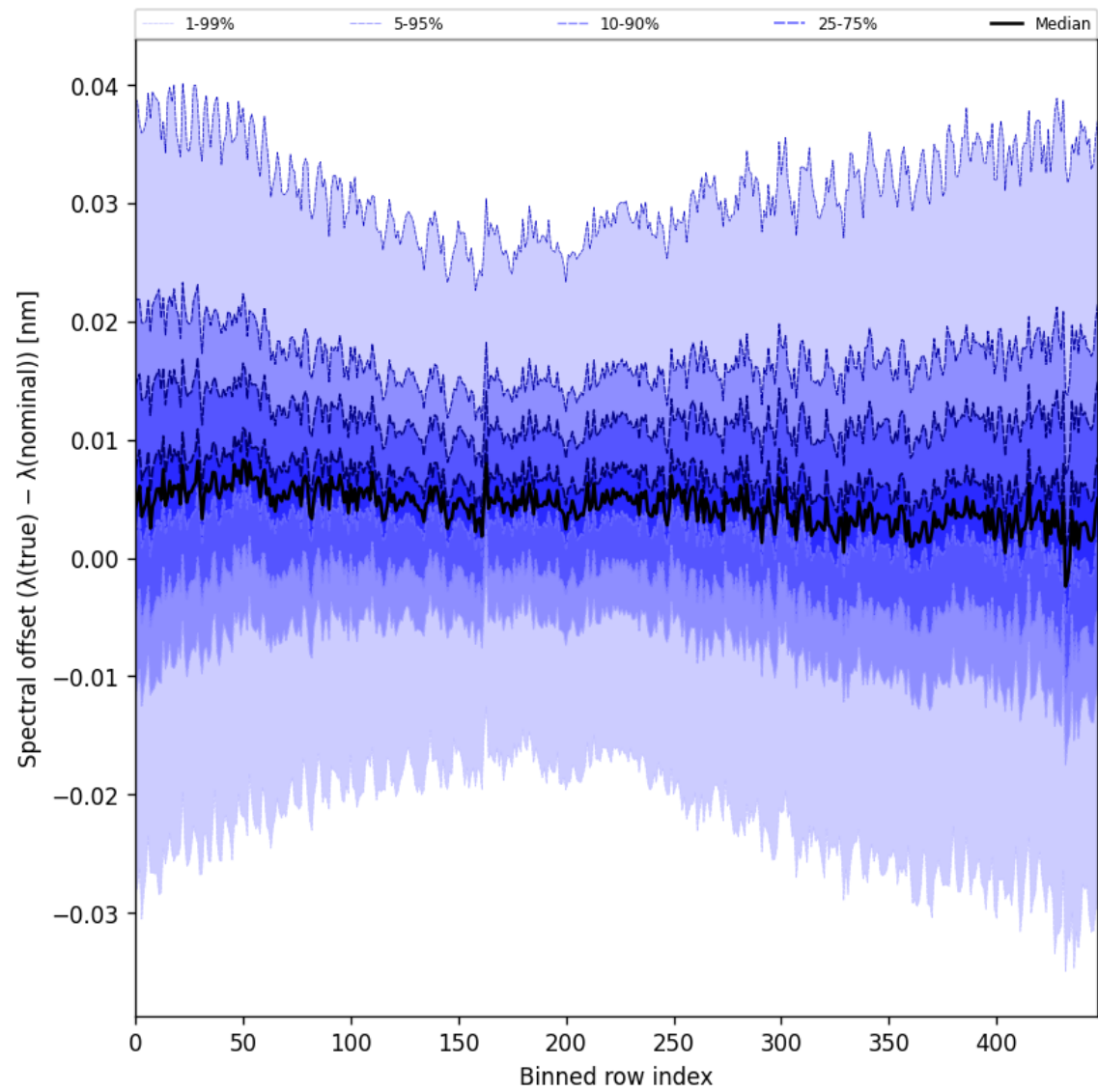
Figure 60: Along track statistics of “Spectral offset ( \lambda_{\text{true}} - \lambda_{\text{nominal}} )” for 2024-12-13 to 2024-12-14
