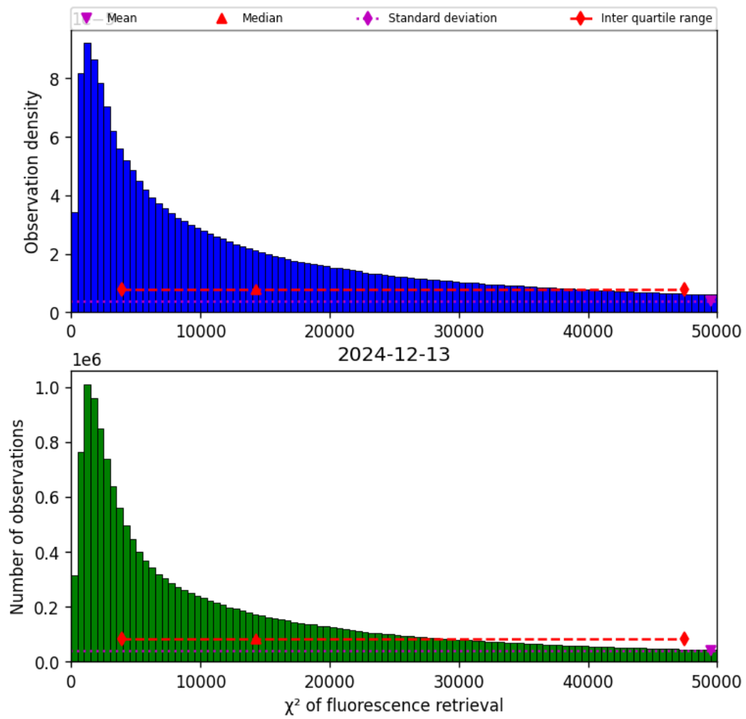
Figure 40: Histogram of “ \chi^2 of fluorescence retrieval” for 2024-12-13 to 2024-12-14
