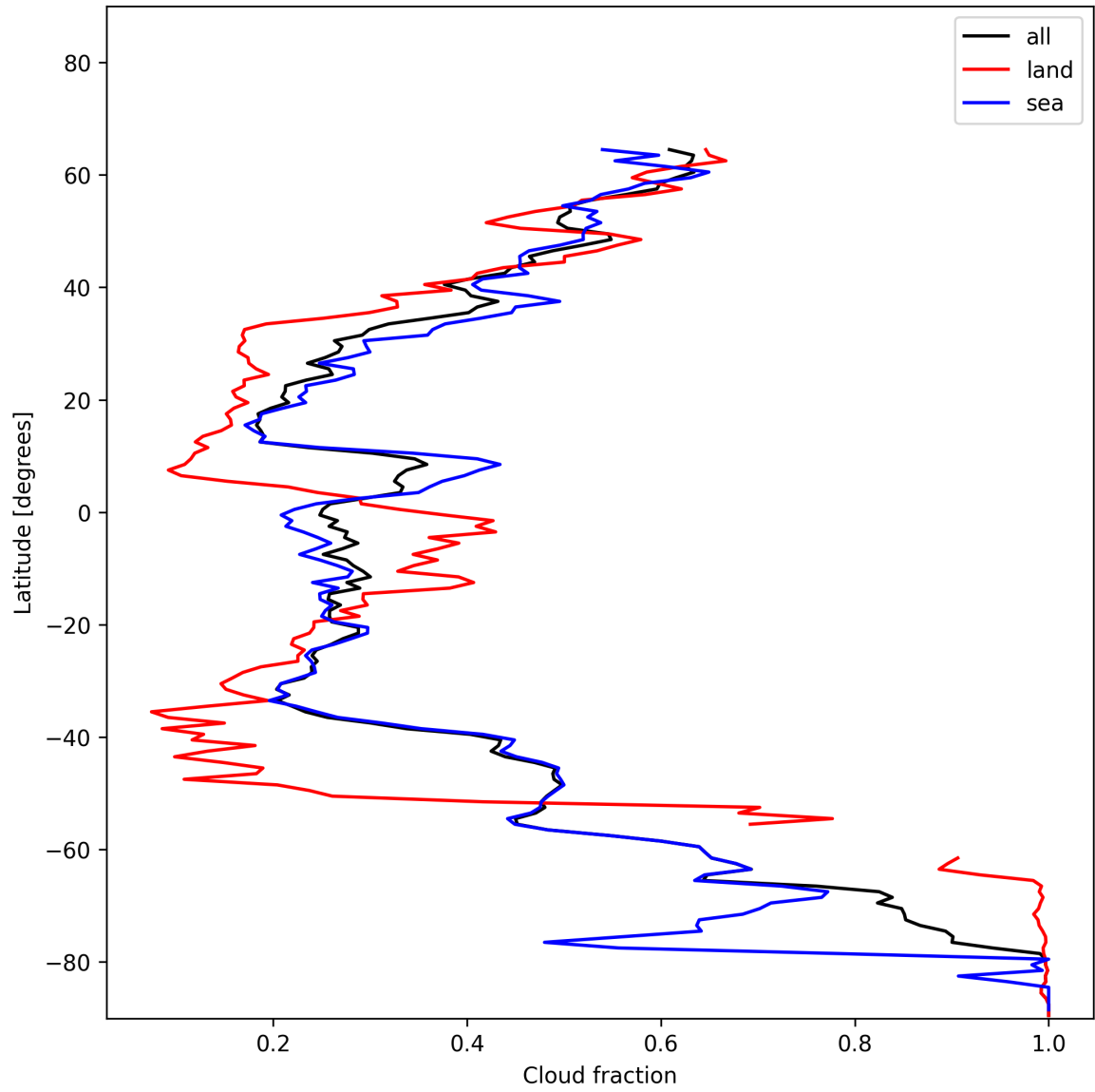
Figure 13: Zonal average of “Cloud fraction” for 2024-12-13 to 2024-12-14.
