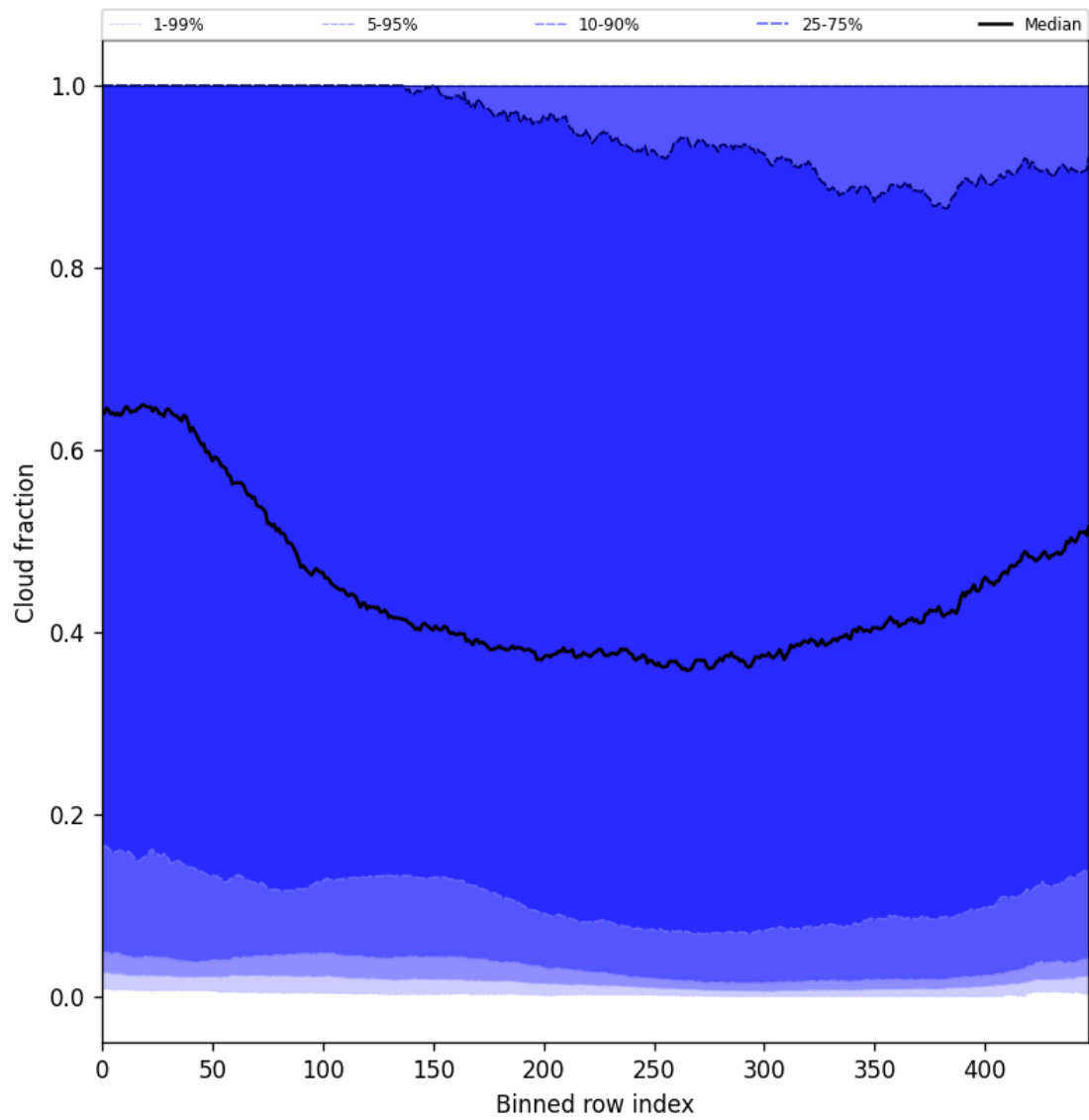
Figure 47: Along track statistics of “Cloud fraction” for 2024-12-13 to 2024-12-14
