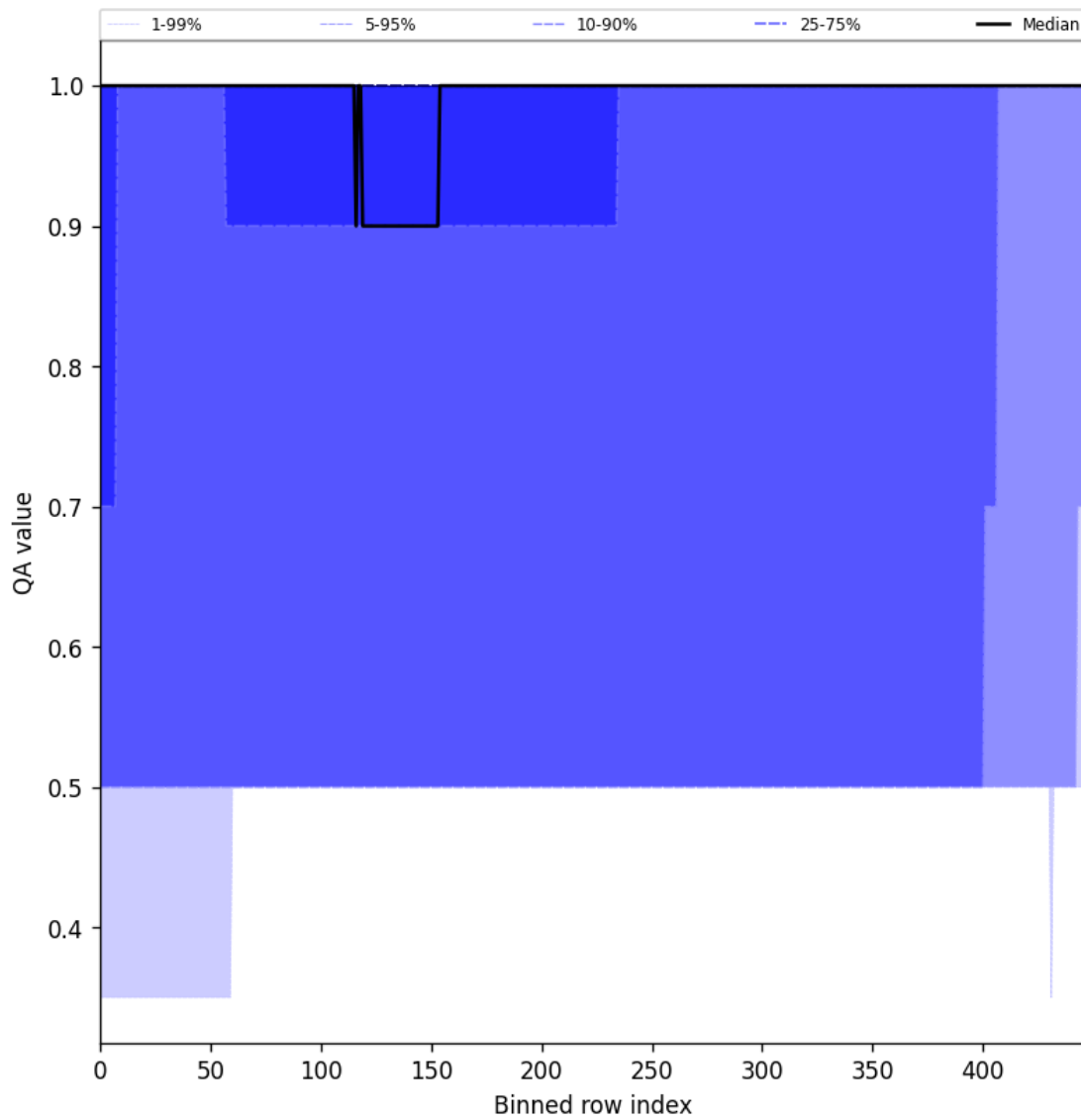
Figure 44: Along track statistics of “QA value” for 2024-12-13 to 2024-12-14
