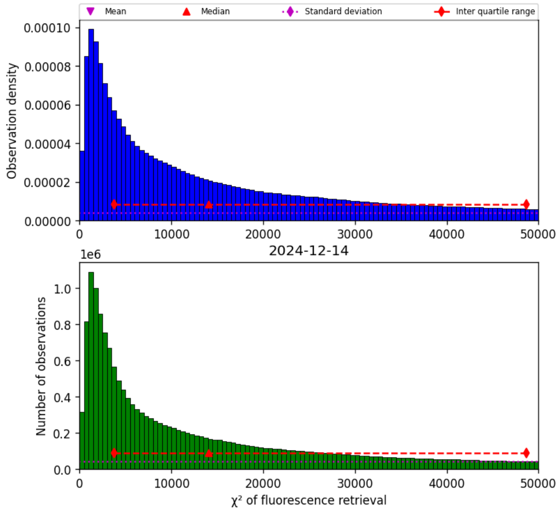
Figure 40: Histogram of “ \chi^2 of fluorescence retrieval” for 2024-12-14 to 2024-12-14
