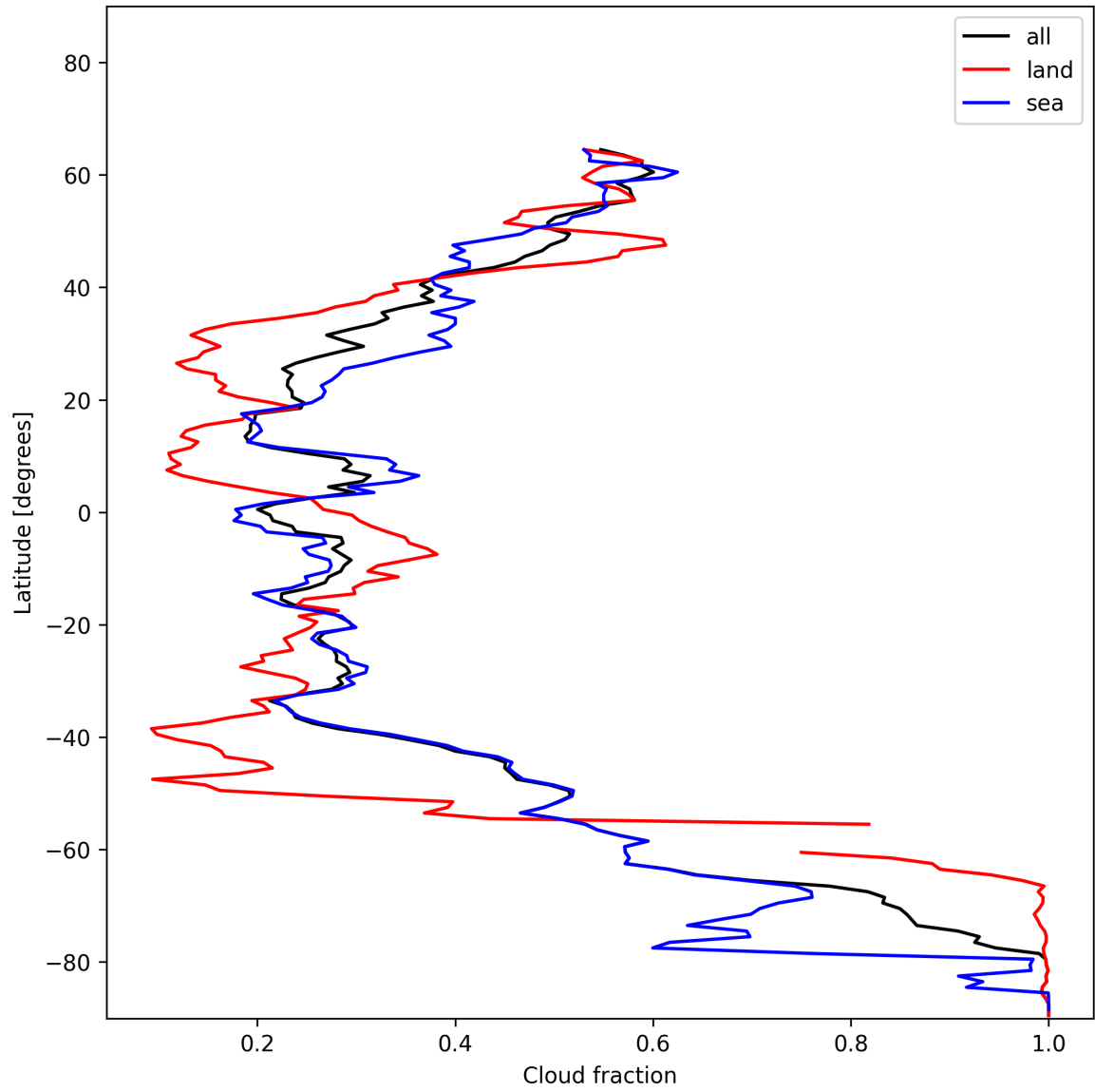
Figure 13: Zonal average of “Cloud fraction” for 2024-12-14 to 2024-12-14.
