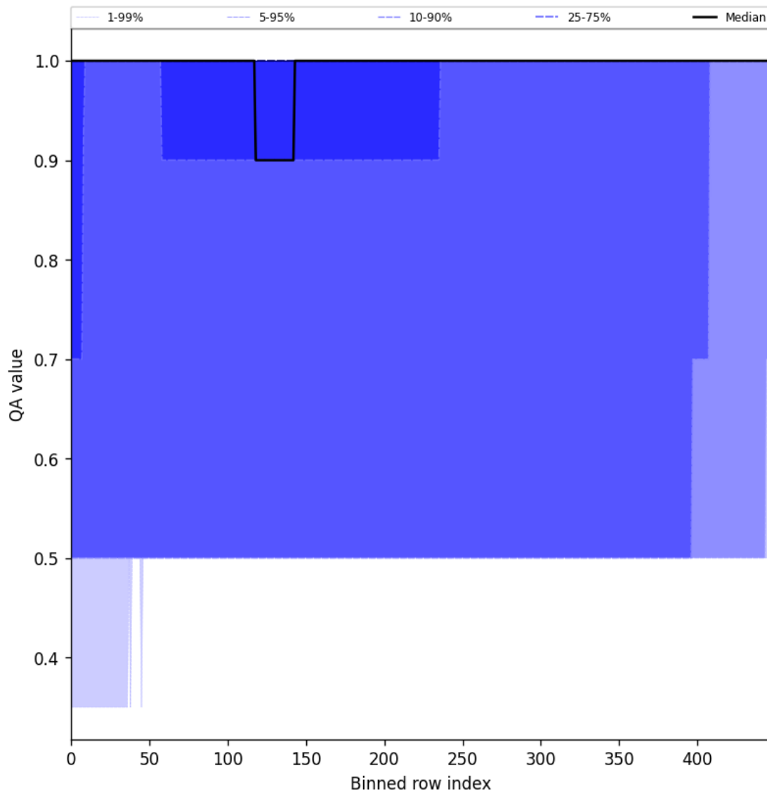
Figure 44: Along track statistics of “QA value” for 2024-12-14 to 2024-12-14
