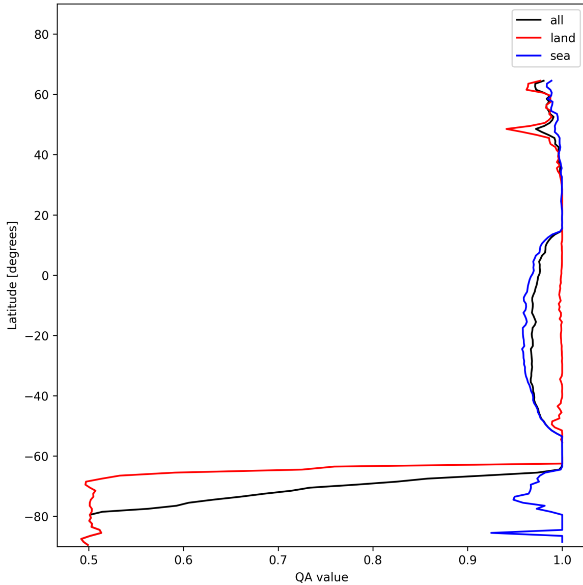
Figure 10: Zonal average of “QA value” for 2024-12-14 to 2024-12-14.
