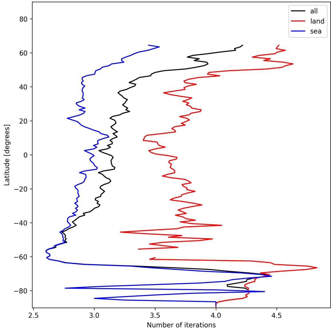
Figure 20: Zonal average of “Number of iterations” for 2024-12-14 to 2024-12-14.
