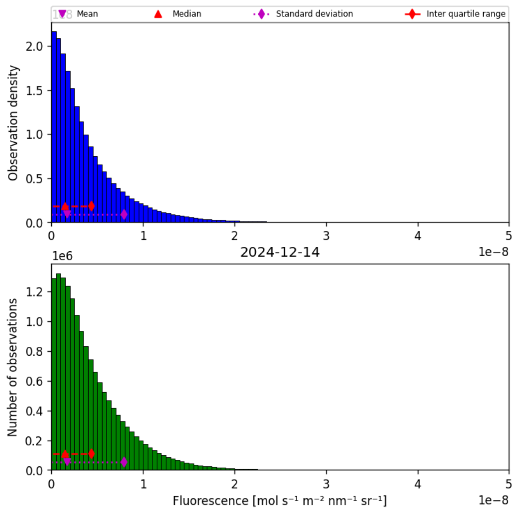
Figure 38: Histogram of “Fluorescence” for 2024-12-14 to 2024-12-14
