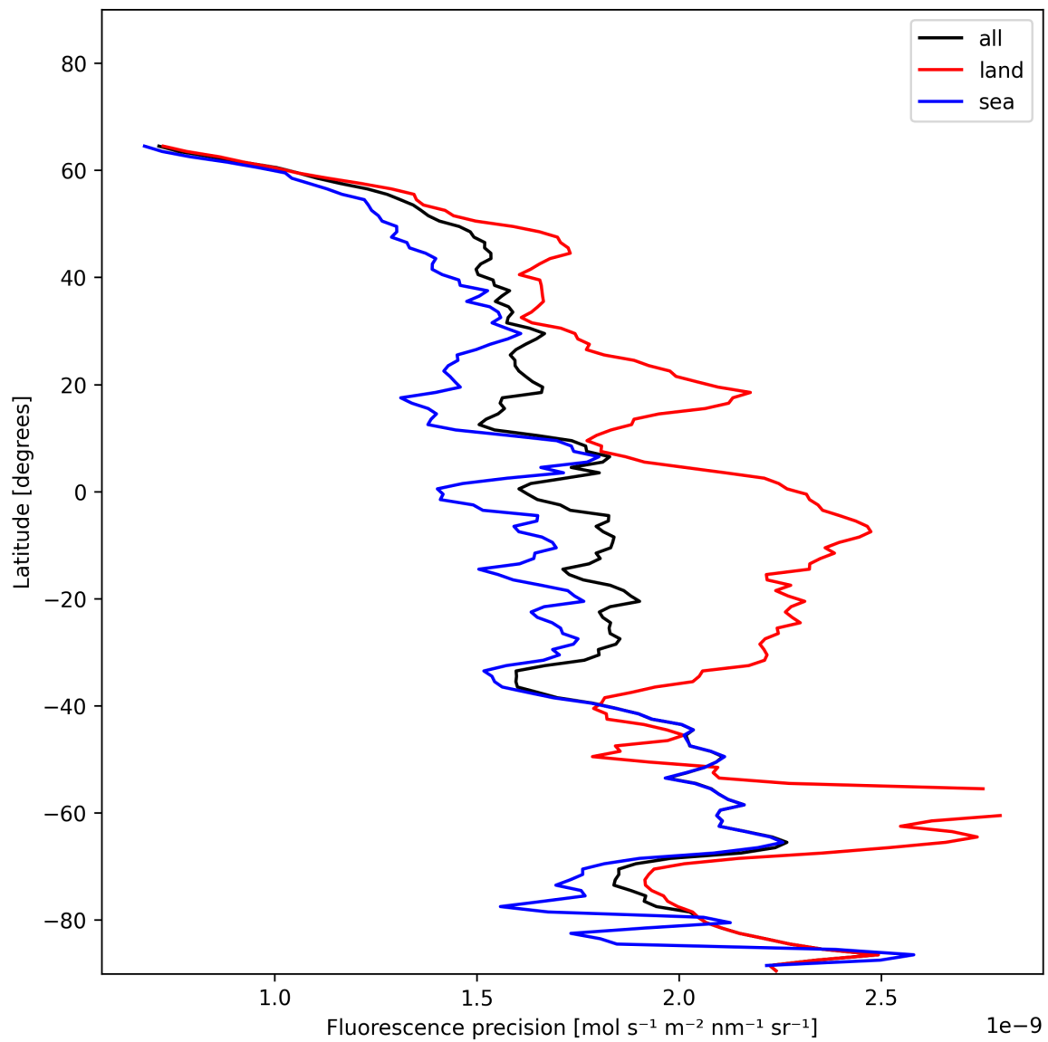
Figure 22: Zonal average of “Fluorescence precision” for 2024-12-14 to 2024-12-14.
