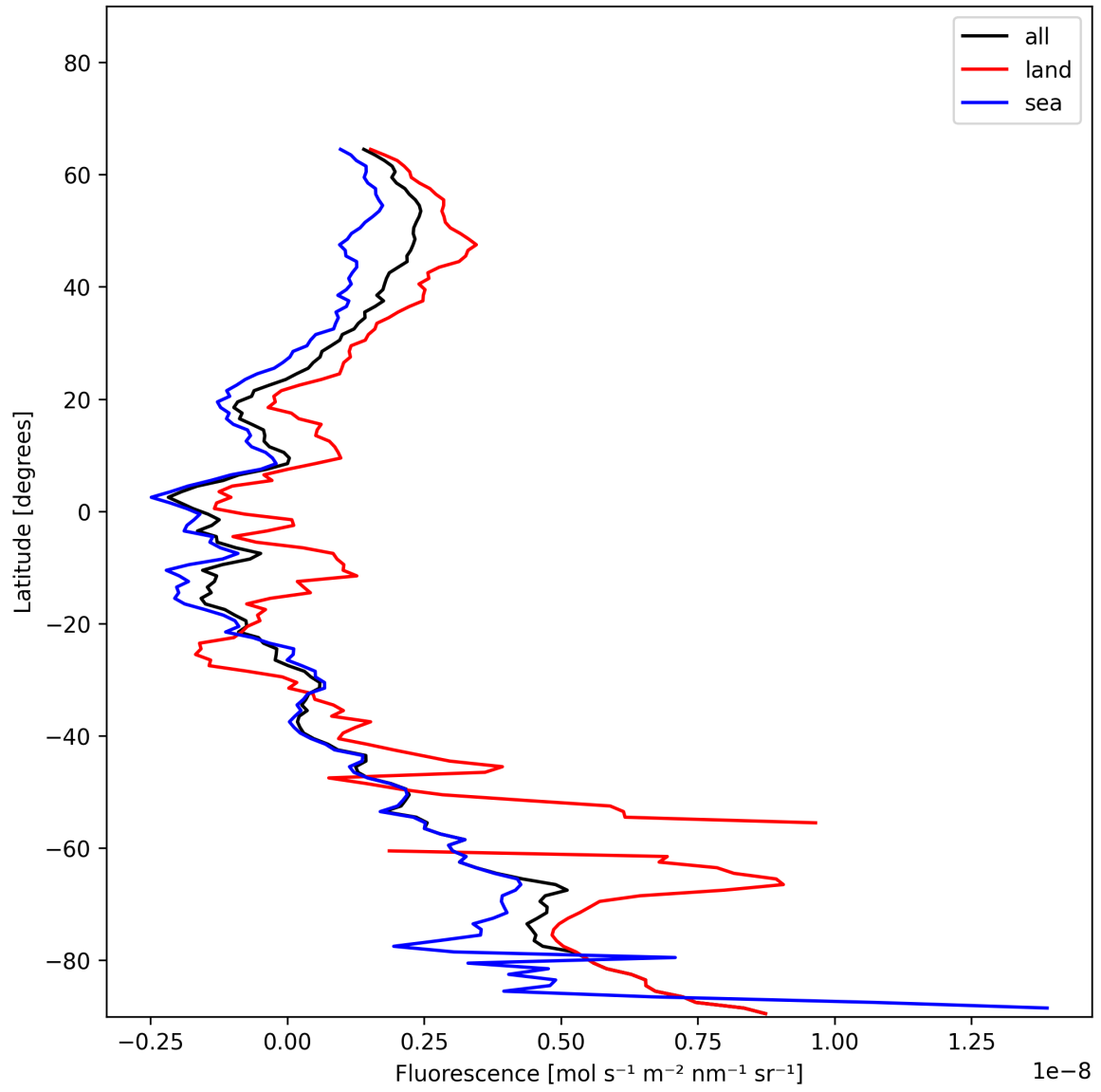
Figure 21: Zonal average of “Fluorescence” for 2024-12-14 to 2024-12-14.
