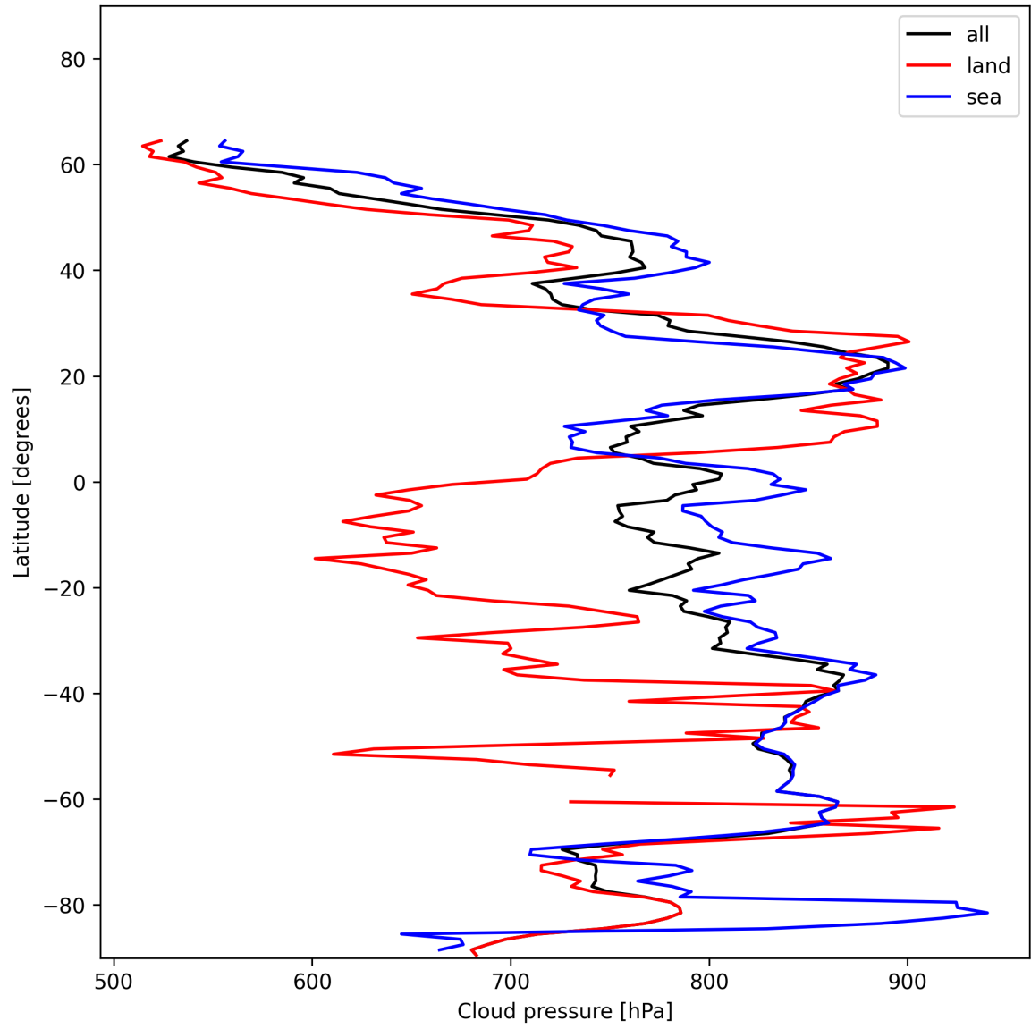
Figure 11: Zonal average of “Cloud pressure” for 2024-12-14 to 2024-12-14.
