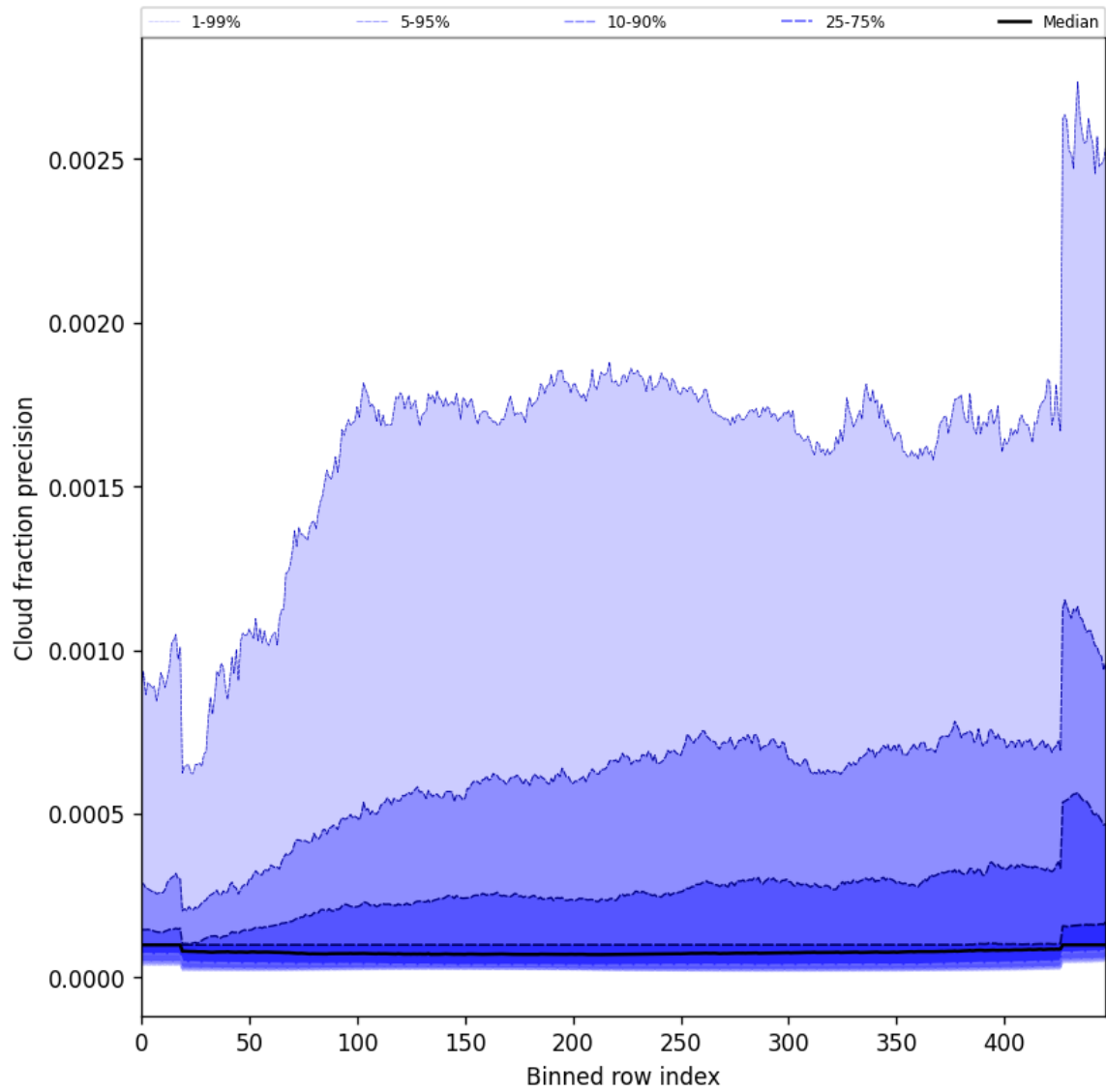
Figure 48: Along track statistics of “Cloud fraction precision” for 2024-12-14 to 2024-12-14
