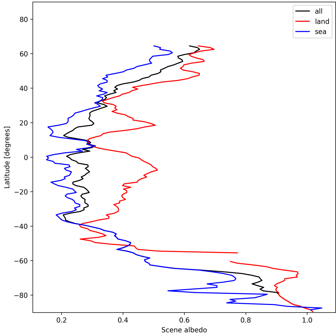
Figure 15: Zonal average of “Scene albedo” for 2024-12-14 to 2024-12-14.
