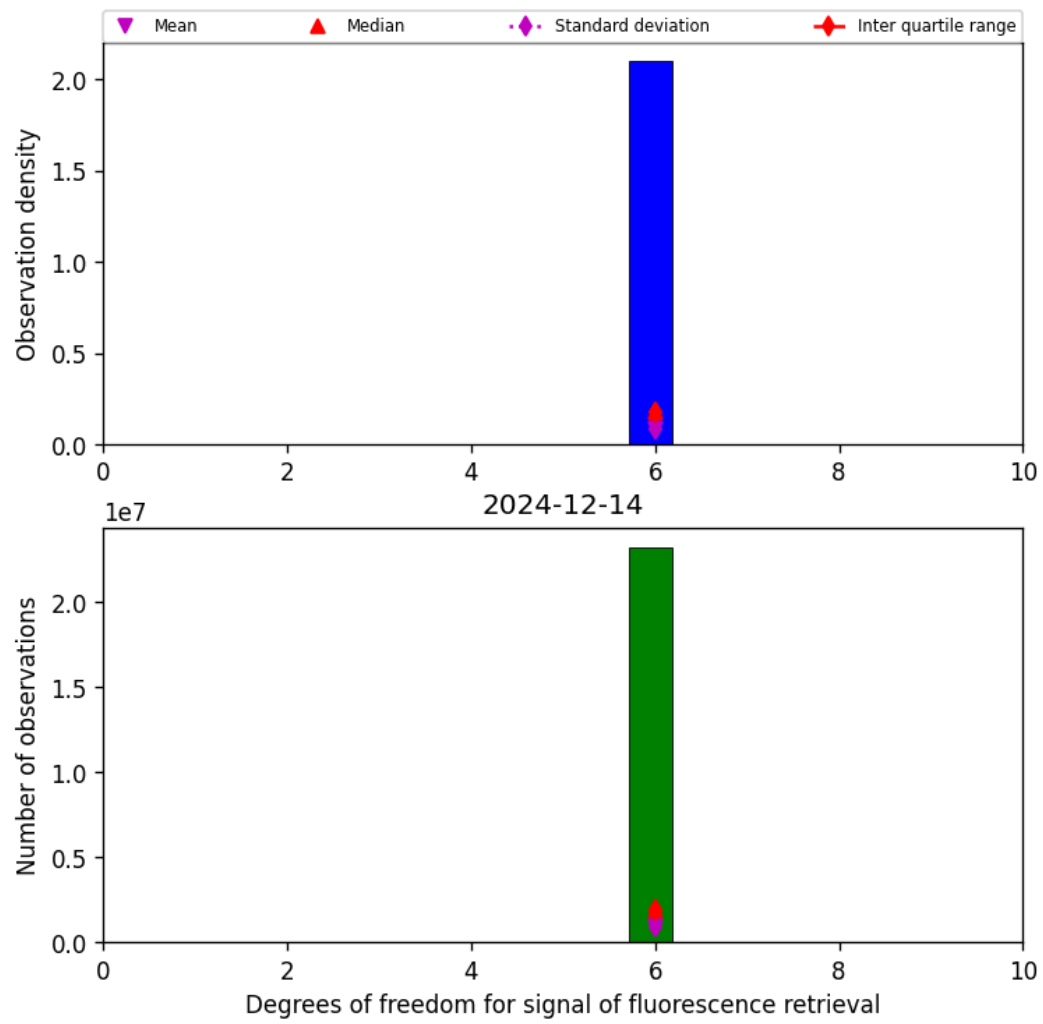
Figure 41: Histogram of “Degrees of freedom for signal of fluorescence retrieval” for 2024-12-14 to 2024-12-14
