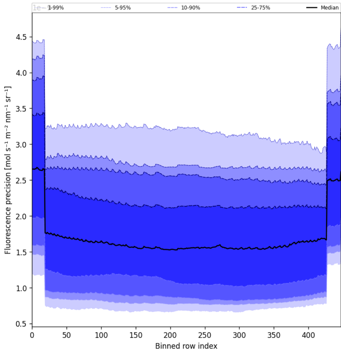
Figure 56: Along track statistics of “Fluorescence precision” for 2024-12-14 to 2024-12-14
