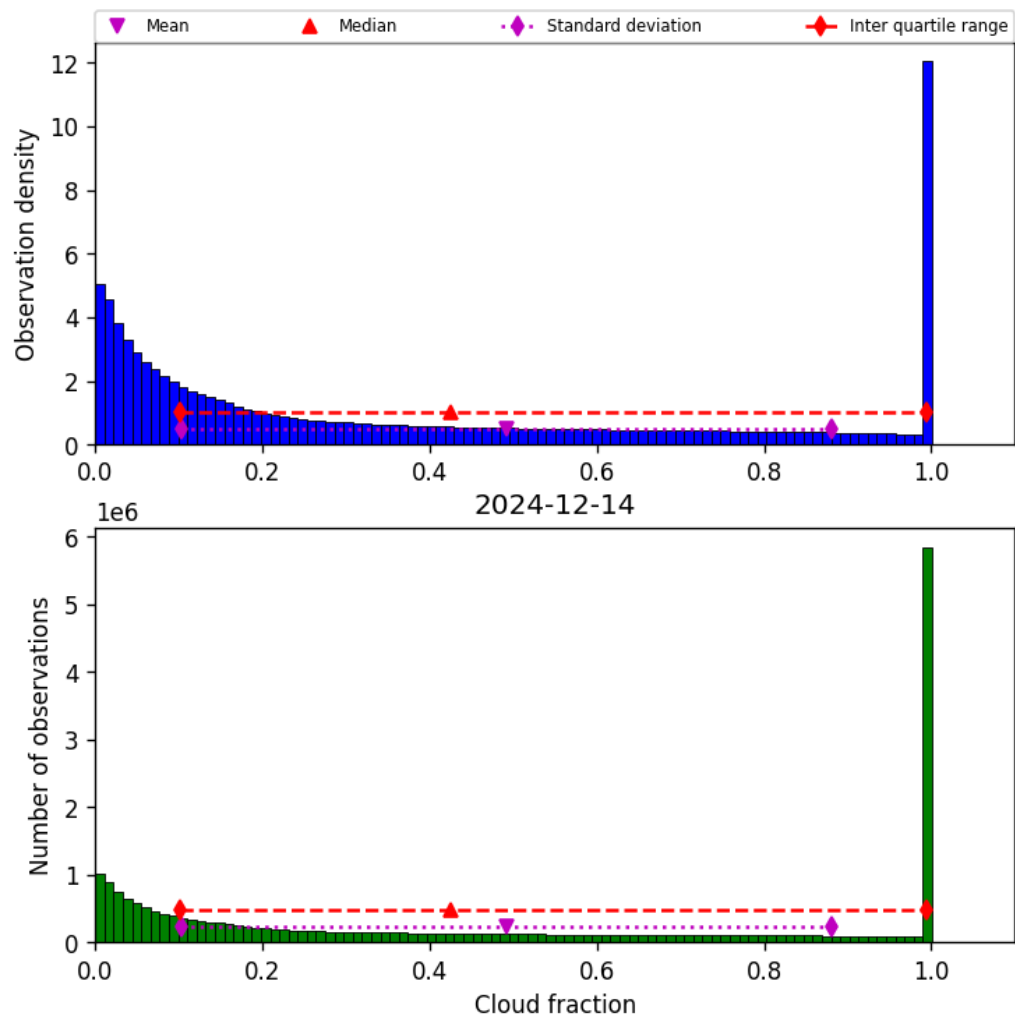
Figure 30: Histogram of “Cloud fraction” for 2024-12-14 to 2024-12-14
