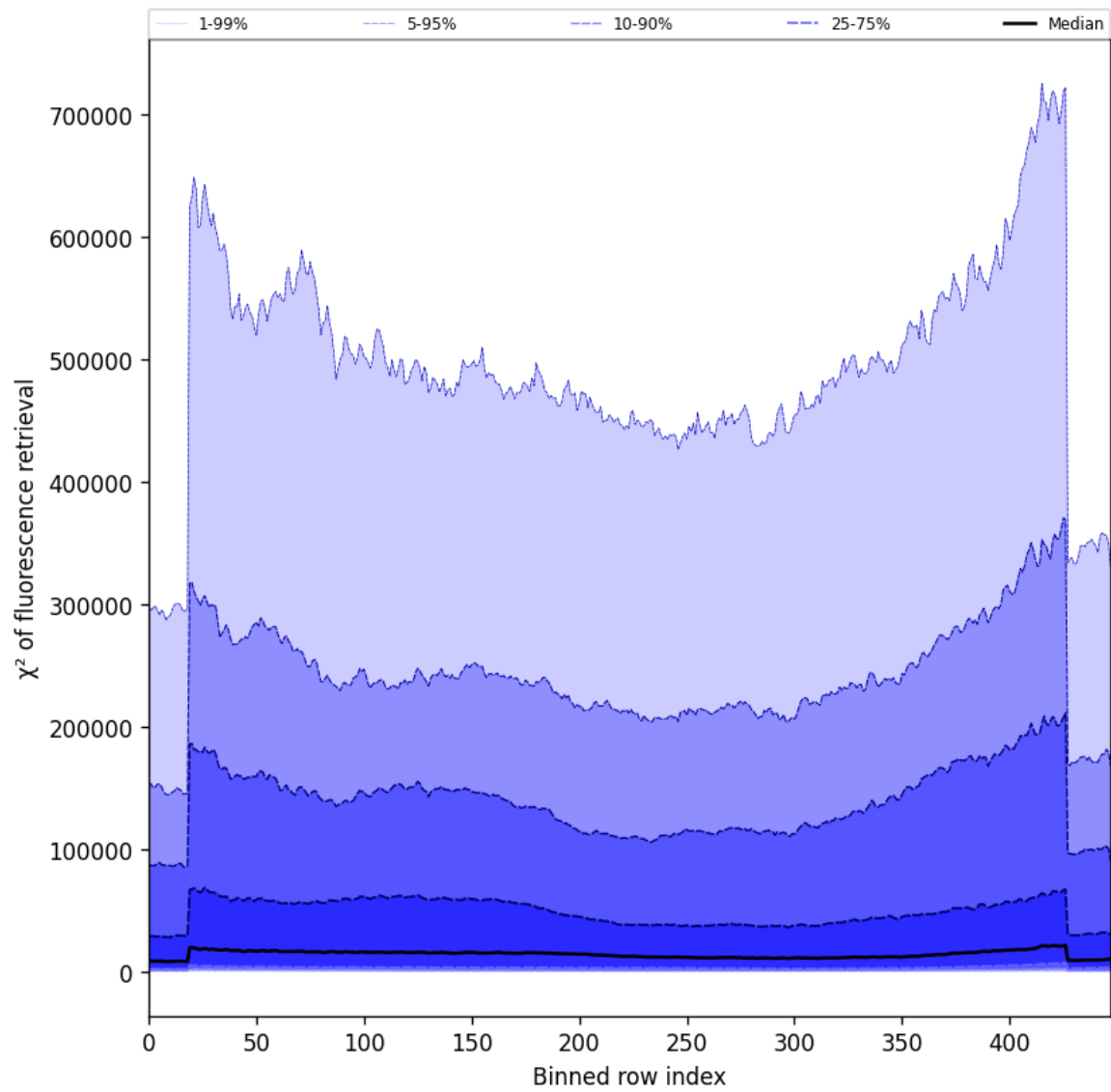
Figure 57: Along track statistics of “ \chi^2 of fluorescence retrieval” for 2024-12-14 to 2024-12-14
