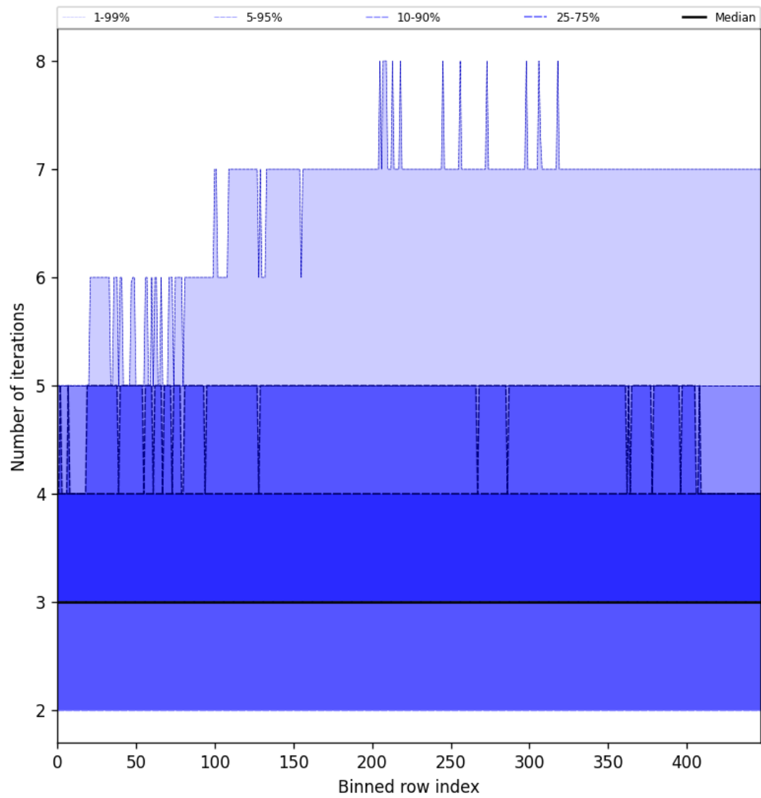
Figure 54: Along track statistics of “Number of iterations” for 2024-12-14 to 2024-12-14
