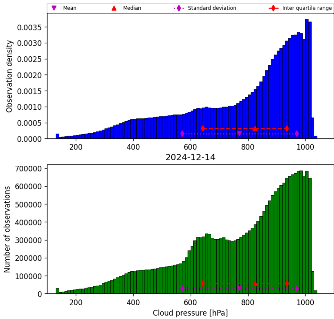
Figure 28: Histogram of “Cloud pressure” for 2024-12-14 to 2024-12-14
