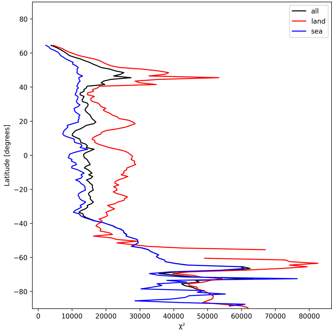
Figure 19: Zonal average of “ \chi^2 ” for 2024-12-14 to 2024-12-14.
