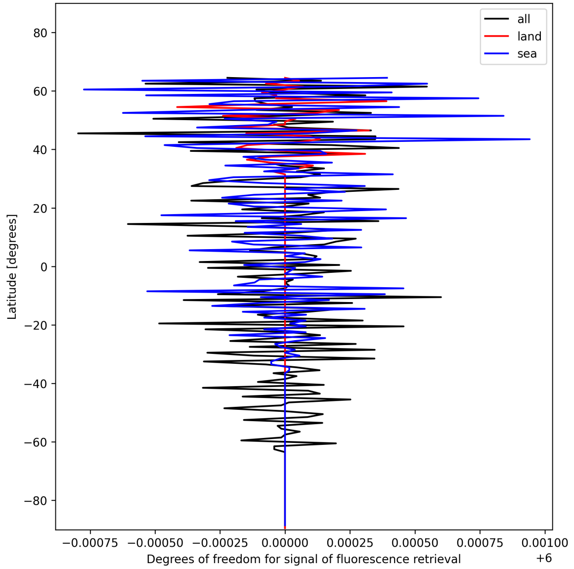
Figure 24: Zonal average of “Degrees of freedom for signal of fluorescence retrieval” for 2024-12-14 to 2024-12-14.
