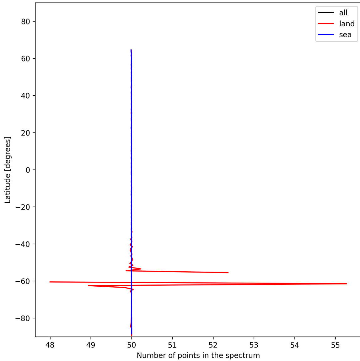
Figure 25: Zonal average of “Number of points in the spectrum” for 2024-12-14 to 2024-12-14.
