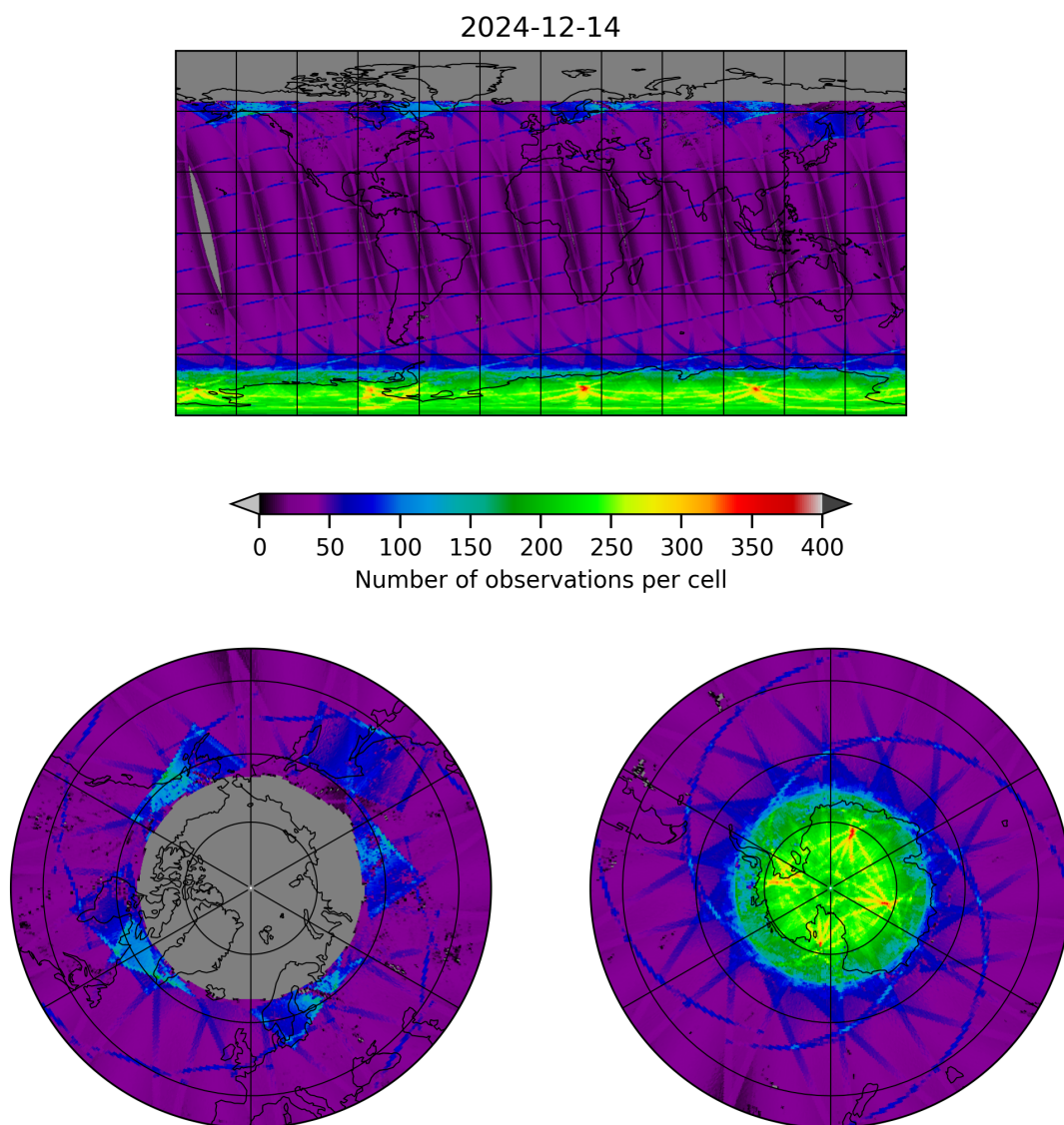
Figure 9: Map of the number of observations for 2024-12-14 to 2024-12-14
