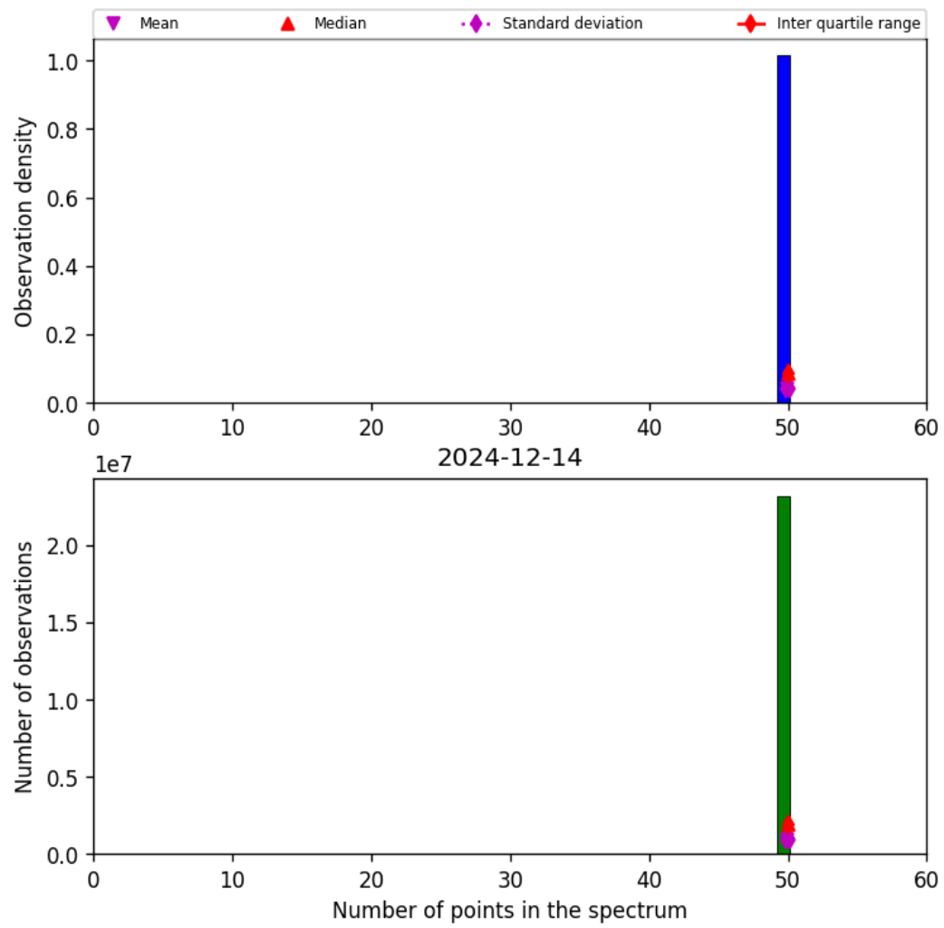
Figure 42: Histogram of “Number of points in the spectrum” for 2024-12-14 to 2024-12-14
