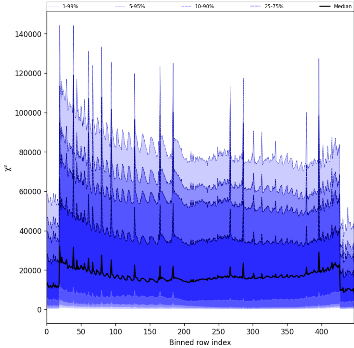
Figure 53: Along track statistics of “ \chi^2 ” for 2024-12-14 to 2024-12-14
