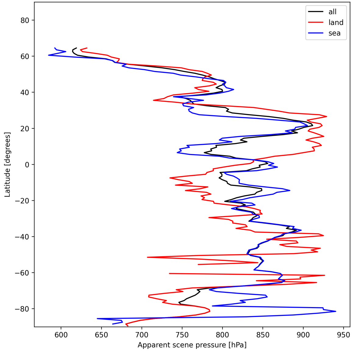
Figure 17: Zonal average of “Apparent scene pressure” for 2024-12-14 to 2024-12-14.
