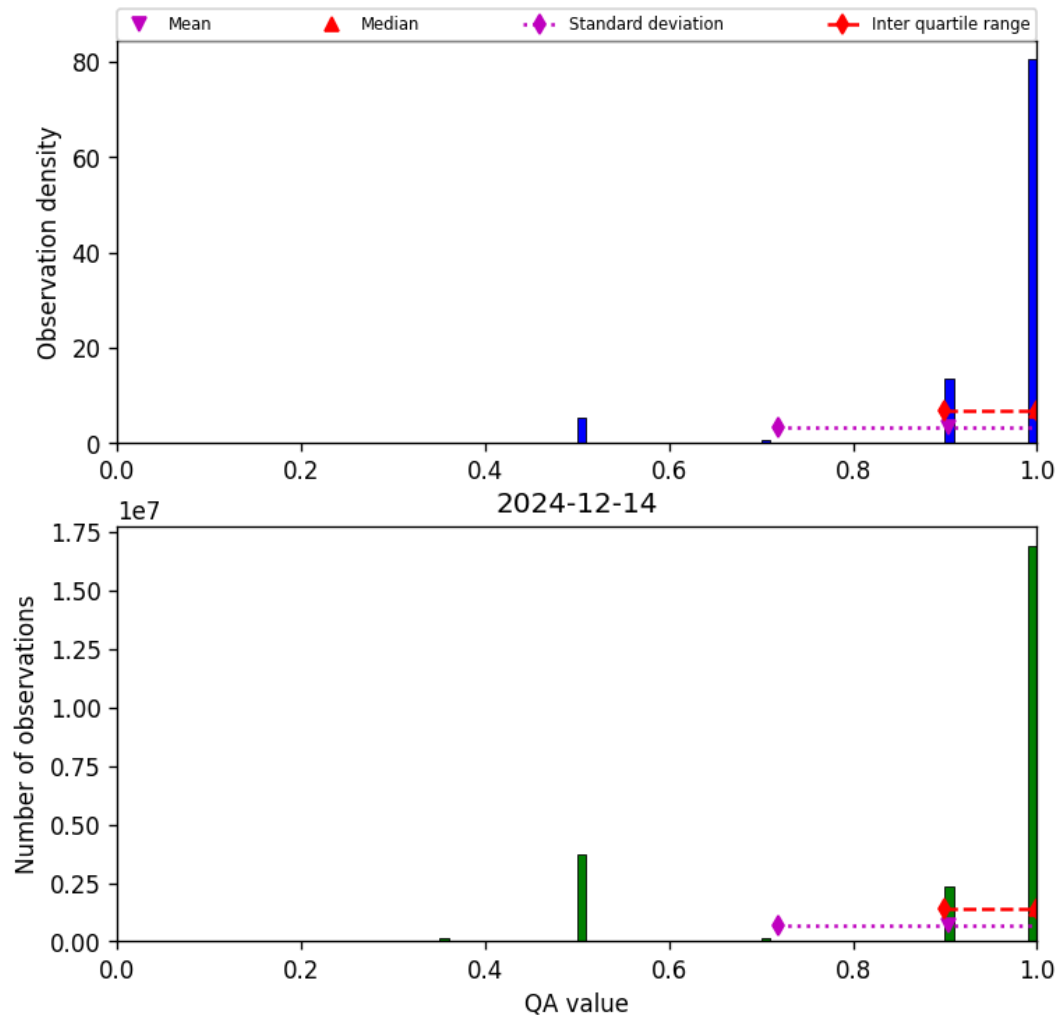
Figure 27: Histogram of “QA value” for 2024-12-14 to 2024-12-14
