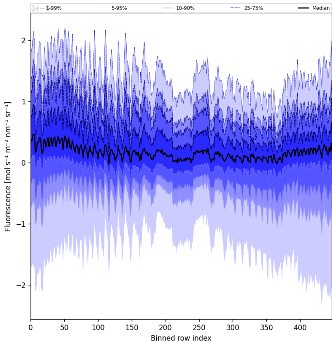
Figure 55: Along track statistics of “Fluorescence” for 2024-12-14 to 2024-12-14
