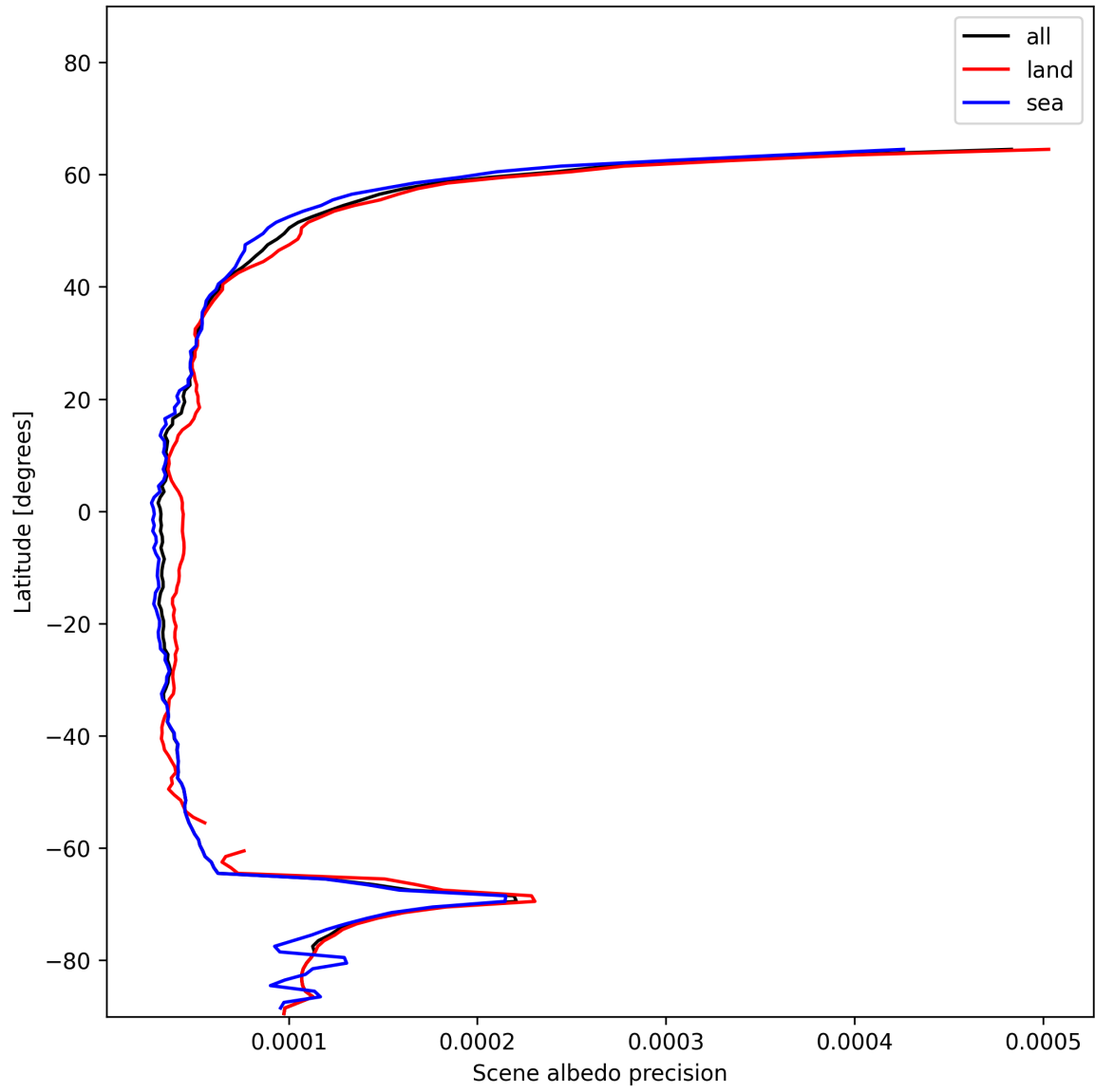
Figure 16: Zonal average of “Scene albedo precision” for 2024-12-14 to 2024-12-14.
