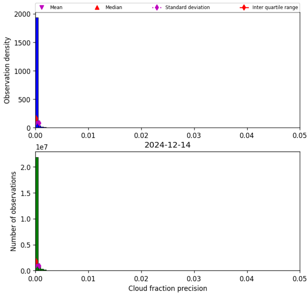
Figure 31: Histogram of “Cloud fraction precision” for 2024-12-14 to 2024-12-14
