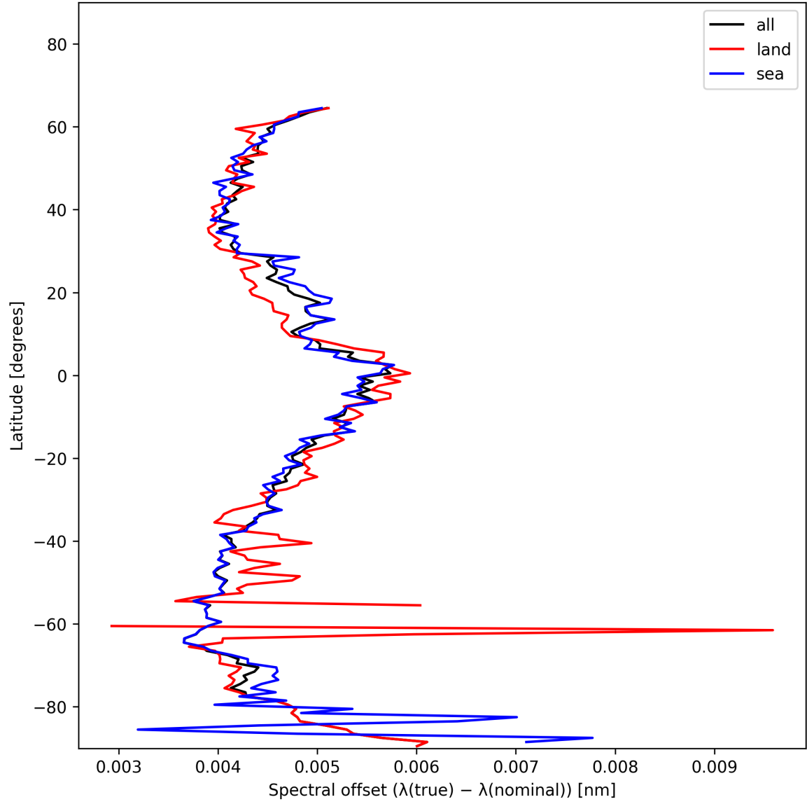
Figure 26: Zonal average of “Spectral offset ( \lambda_{\text{true}} - \lambda_{\text{nominal}} )” for 2024-12-14 to 2024-12-14.
