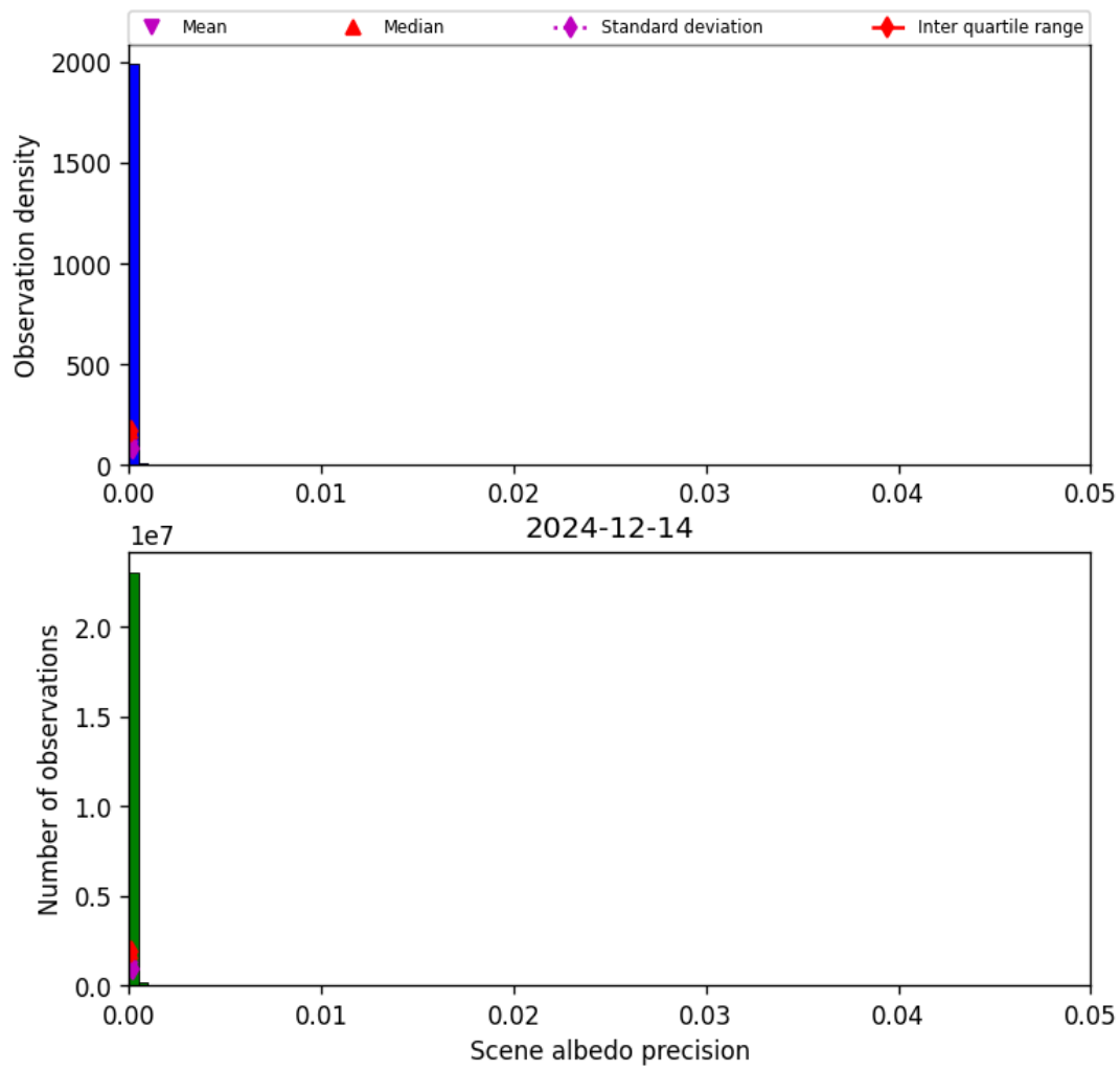
Figure 33: Histogram of “Scene albedo precision” for 2024-12-14 to 2024-12-14
