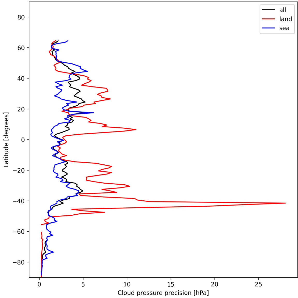
Figure 12: Zonal average of “Cloud pressure precision” for 2024-12-14 to 2024-12-14.
