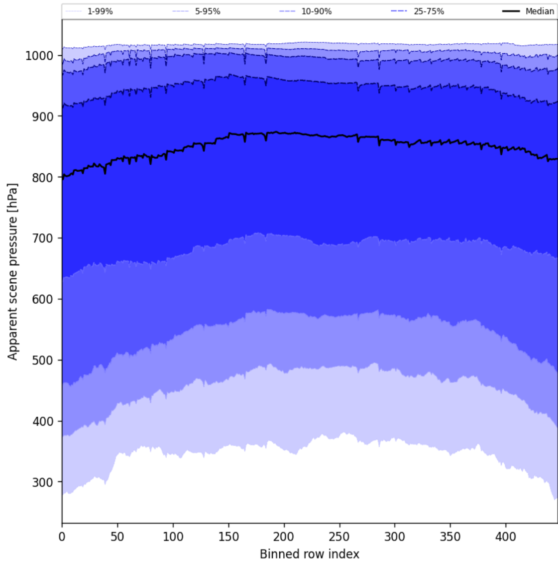
Figure 51: Along track statistics of “Apparent scene pressure” for 2024-12-14 to 2024-12-14
