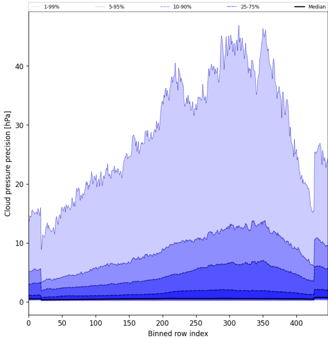
Figure 46: Along track statistics of “Cloud pressure precision” for 2024-12-14 to 2024-12-14
