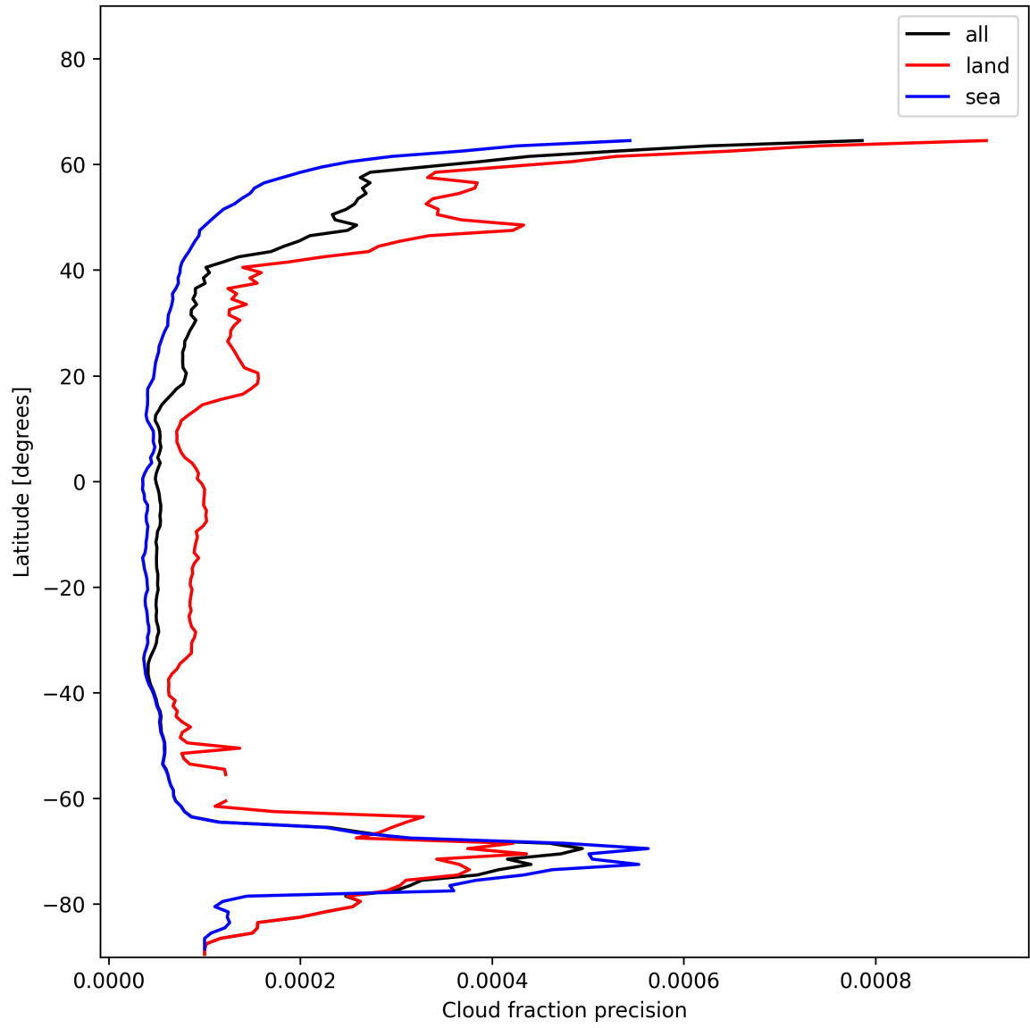
Figure 14: Zonal average of “Cloud fraction precision” for 2024-12-14 to 2024-12-14.
