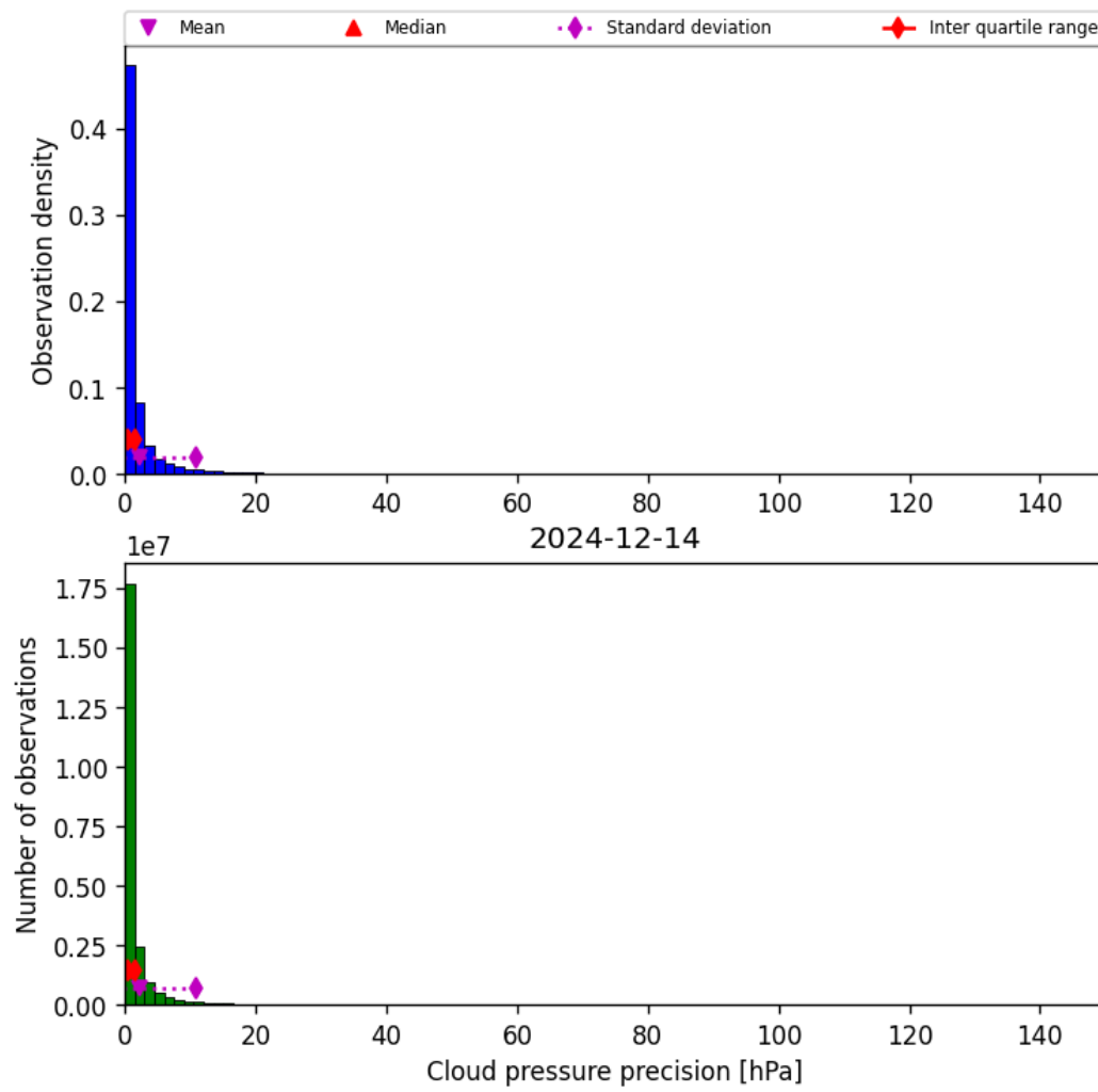
Figure 29: Histogram of “Cloud pressure precision” for 2024-12-14 to 2024-12-14
