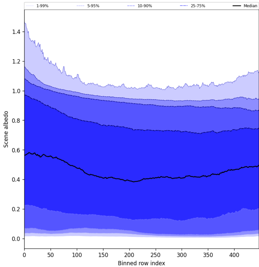
Figure 49: Along track statistics of “Scene albedo” for 2024-12-14 to 2024-12-14
