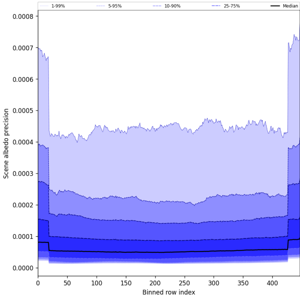
Figure 50: Along track statistics of “Scene albedo precision” for 2024-12-14 to 2024-12-14
