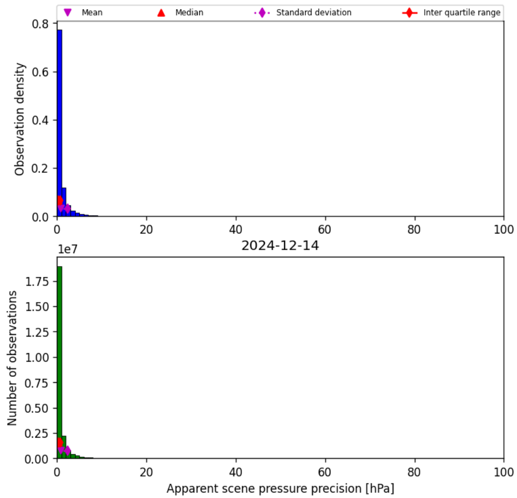
Figure 35: Histogram of “Apparent scene pressure precision” for 2024-12-14 to 2024-12-14
