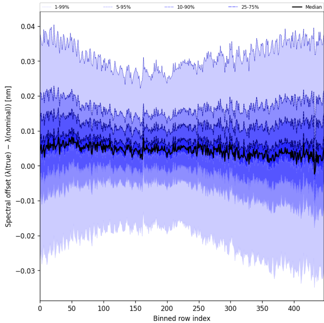
Figure 60: Along track statistics of “Spectral offset ( \lambda_{\text{true}} - \lambda_{\text{nominal}} )” for 2024-12-14 to 2024-12-14
