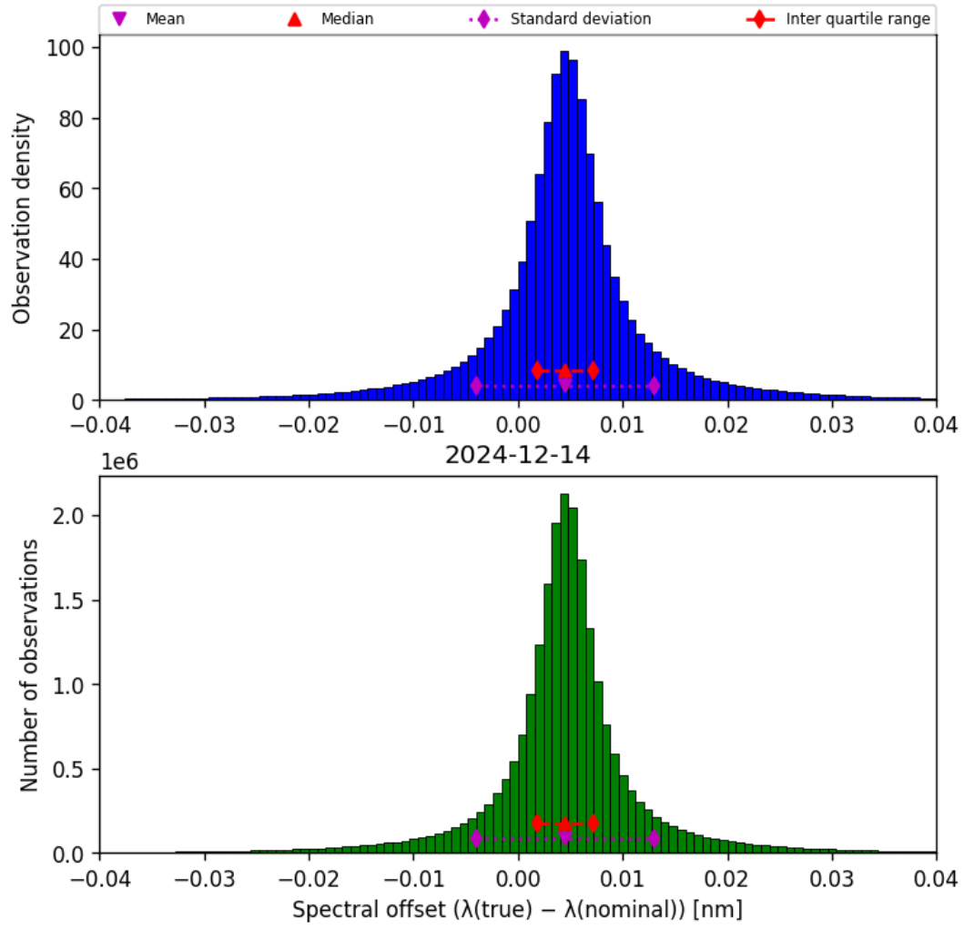
Figure 43: Histogram of “Spectral offset ( \lambda_{\text{true}} - \lambda_{\text{nominal}} )” for 2024-12-14 to 2024-12-14
