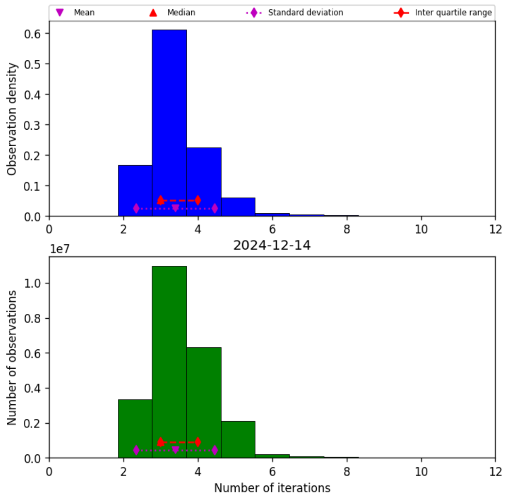
Figure 37: Histogram of “Number of iterations” for 2024-12-14 to 2024-12-14
