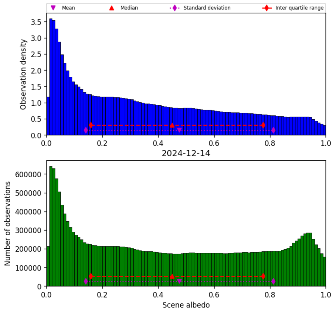
Figure 32: Histogram of “Scene albedo” for 2024-12-14 to 2024-12-14
