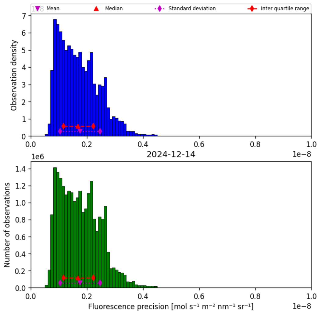
Figure 39: Histogram of “Fluorescence precision” for 2024-12-14 to 2024-12-14
