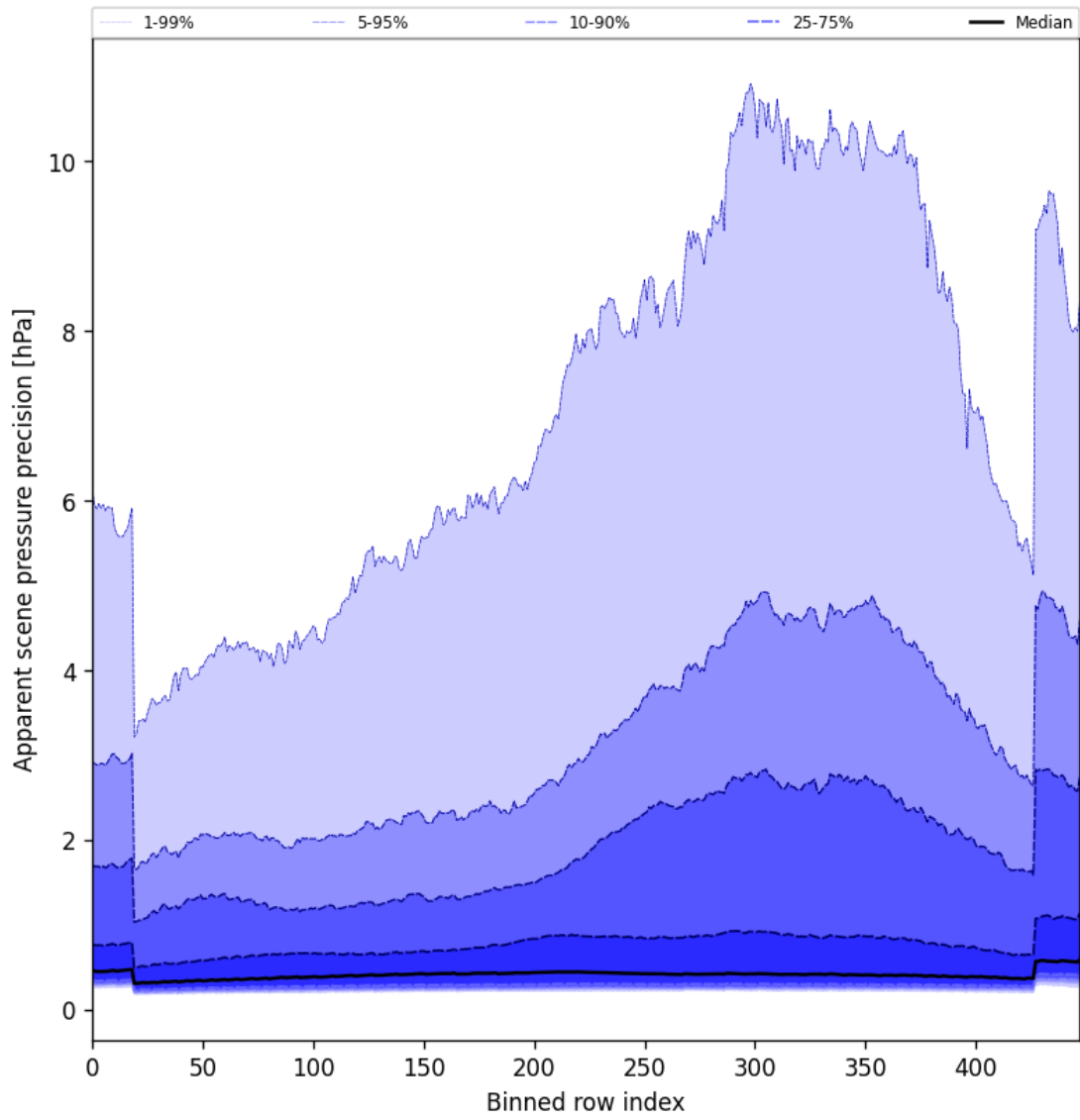
Figure 52: Along track statistics of “Apparent scene pressure precision” for 2024-12-14 to 2024-12-14
