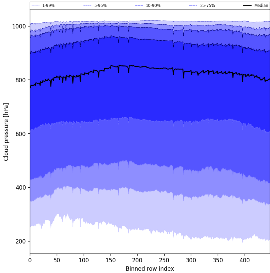
Figure 45: Along track statistics of “Cloud pressure” for 2024-12-14 to 2024-12-14
