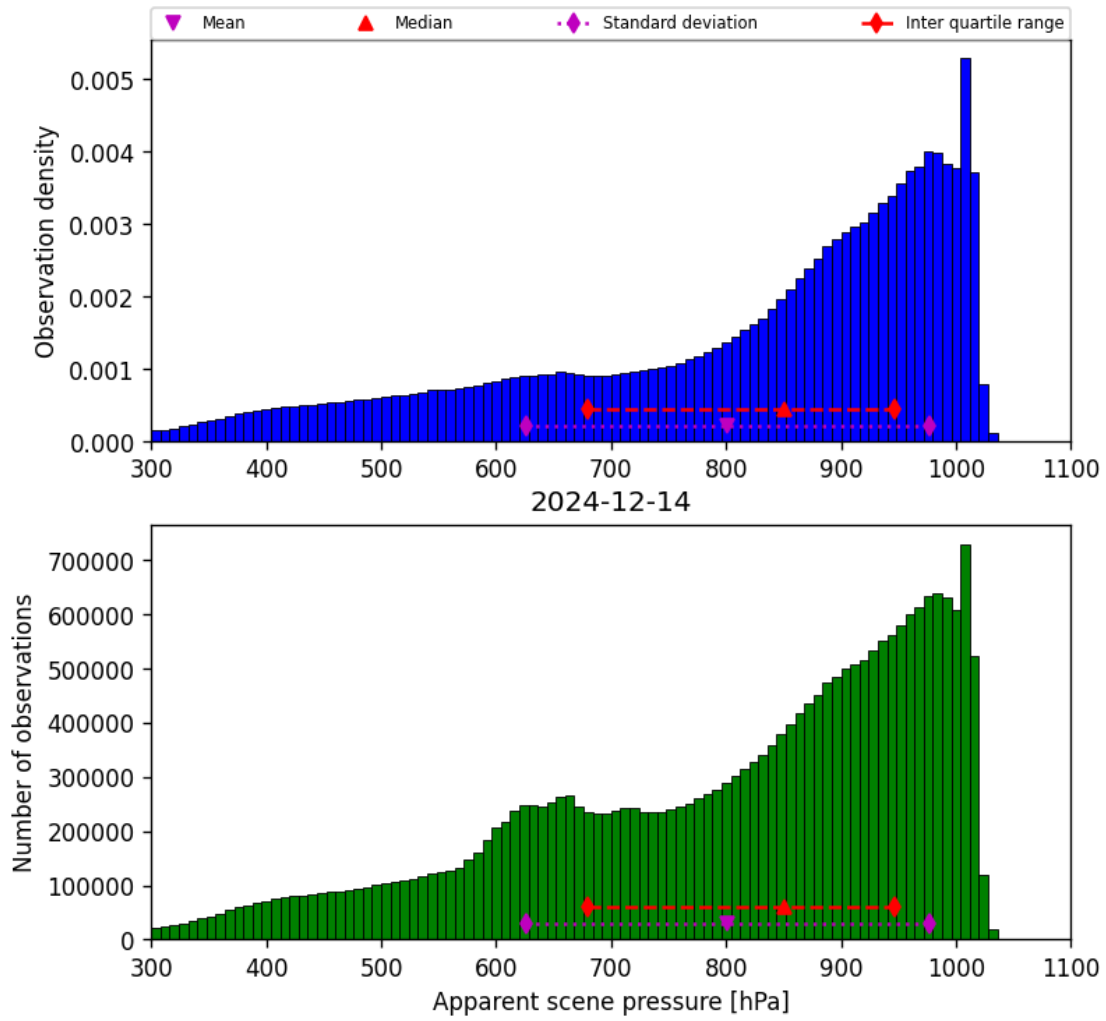
Figure 34: Histogram of “Apparent scene pressure” for 2024-12-14 to 2024-12-14
