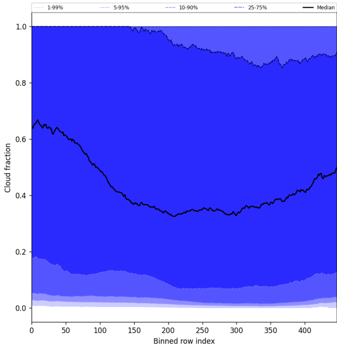
Figure 47: Along track statistics of “Cloud fraction” for 2024-12-14 to 2024-12-14
