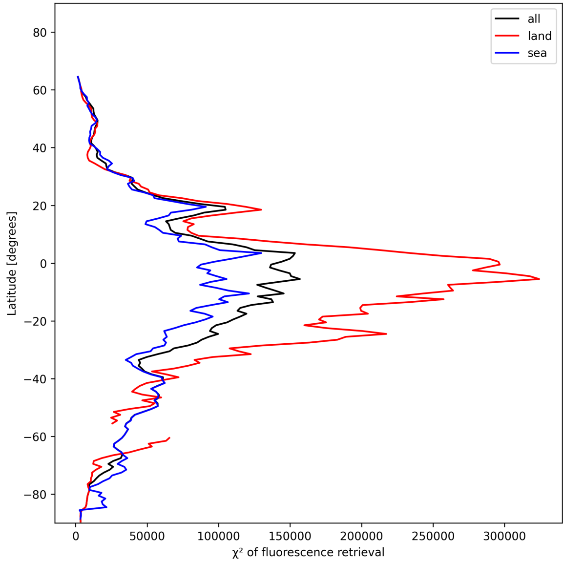
Figure 23: Zonal average of “ \chi^2 of fluorescence retrieval” for 2024-12-14 to 2024-12-14.
