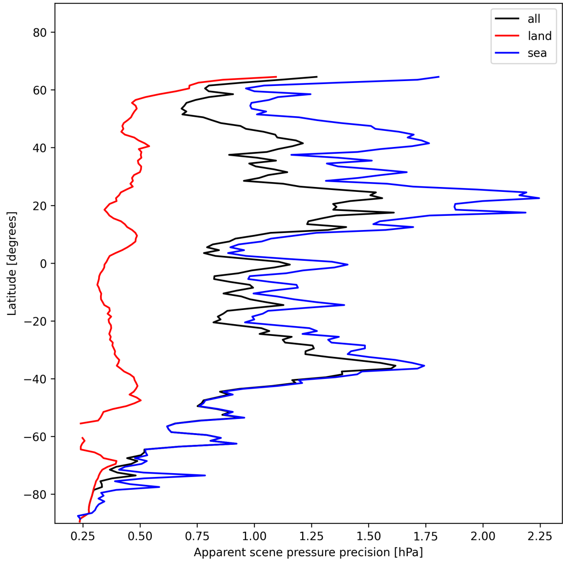
Figure 18: Zonal average of “Apparent scene pressure precision” for 2024-12-14 to 2024-12-14.
