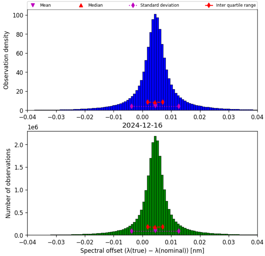
Figure 43: Histogram of “Spectral offset ( \lambda_{\text{true}} - \lambda_{\text{nominal}} )” for 2024-12-16 to 2024-12-17
