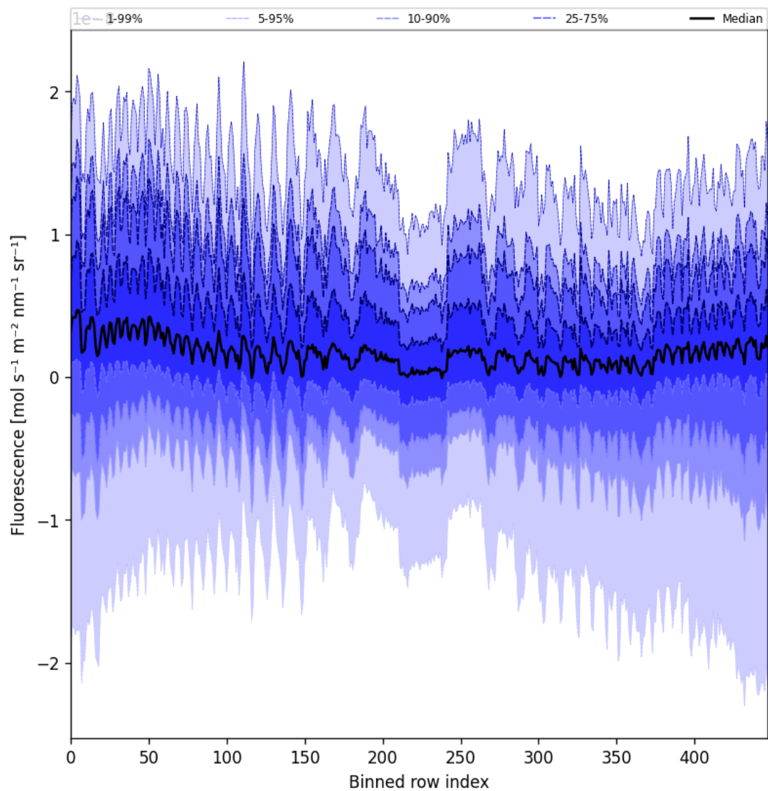
Figure 55: Along track statistics of “Fluorescence” for 2024-12-16 to 2024-12-17
