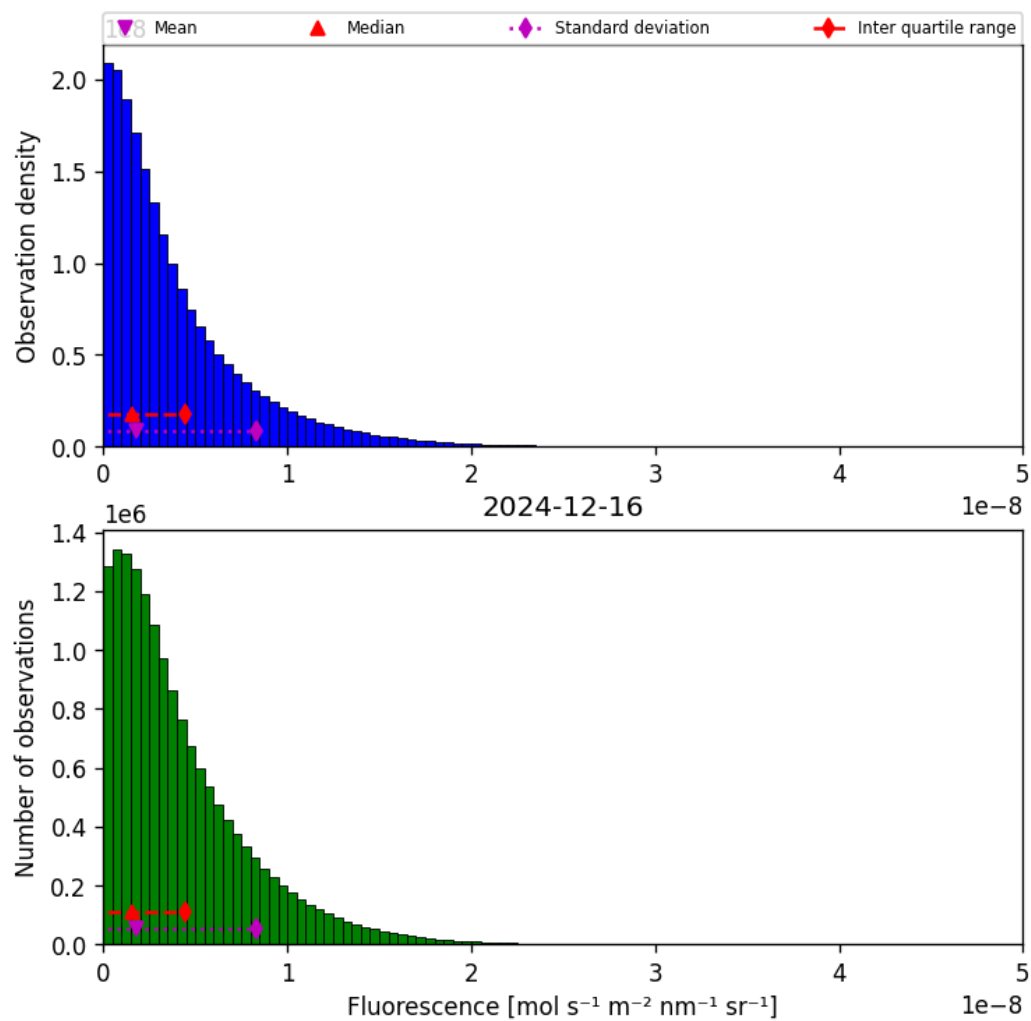
Figure 38: Histogram of “Fluorescence” for 2024-12-16 to 2024-12-17
