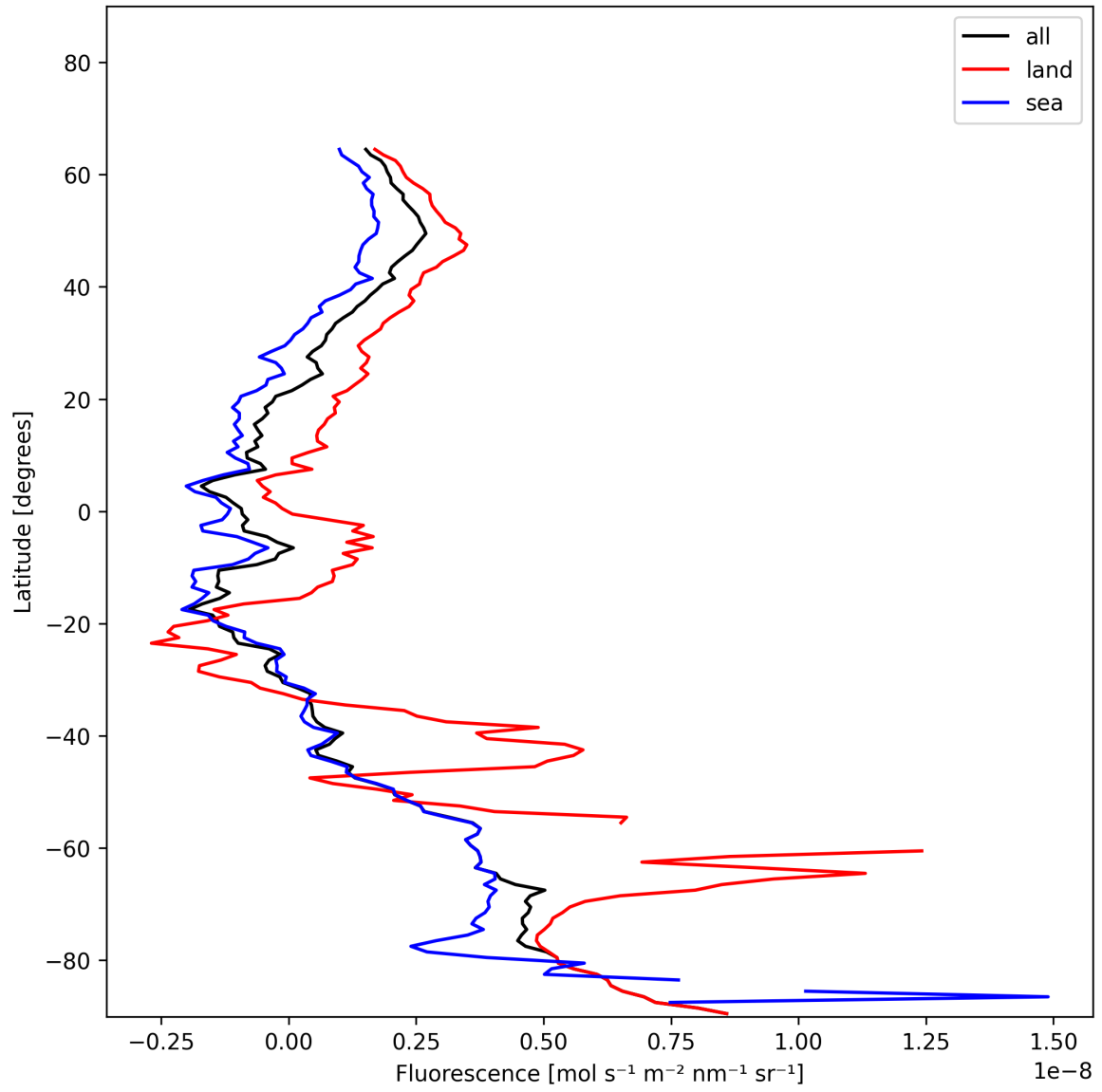
Figure 21: Zonal average of “Fluorescence” for 2024-12-16 to 2024-12-17.
