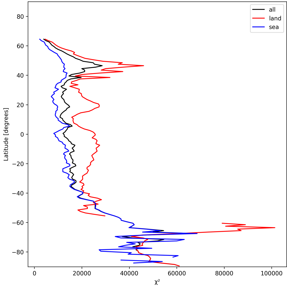
Figure 19: Zonal average of “ \chi^2 ” for 2024-12-16 to 2024-12-17.
