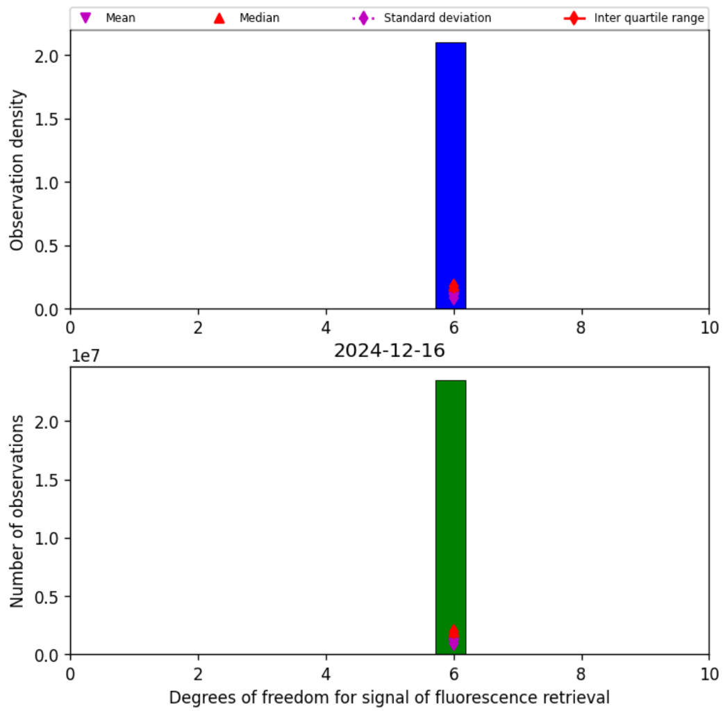
Figure 41: Histogram of “Degrees of freedom for signal of fluorescence retrieval” for 2024-12-16 to 2024-12-17
