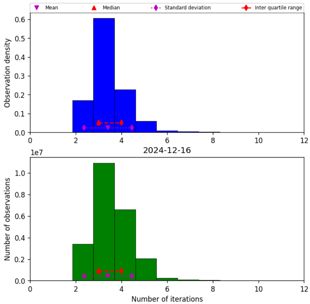
Figure 37: Histogram of “Number of iterations” for 2024-12-16 to 2024-12-17
