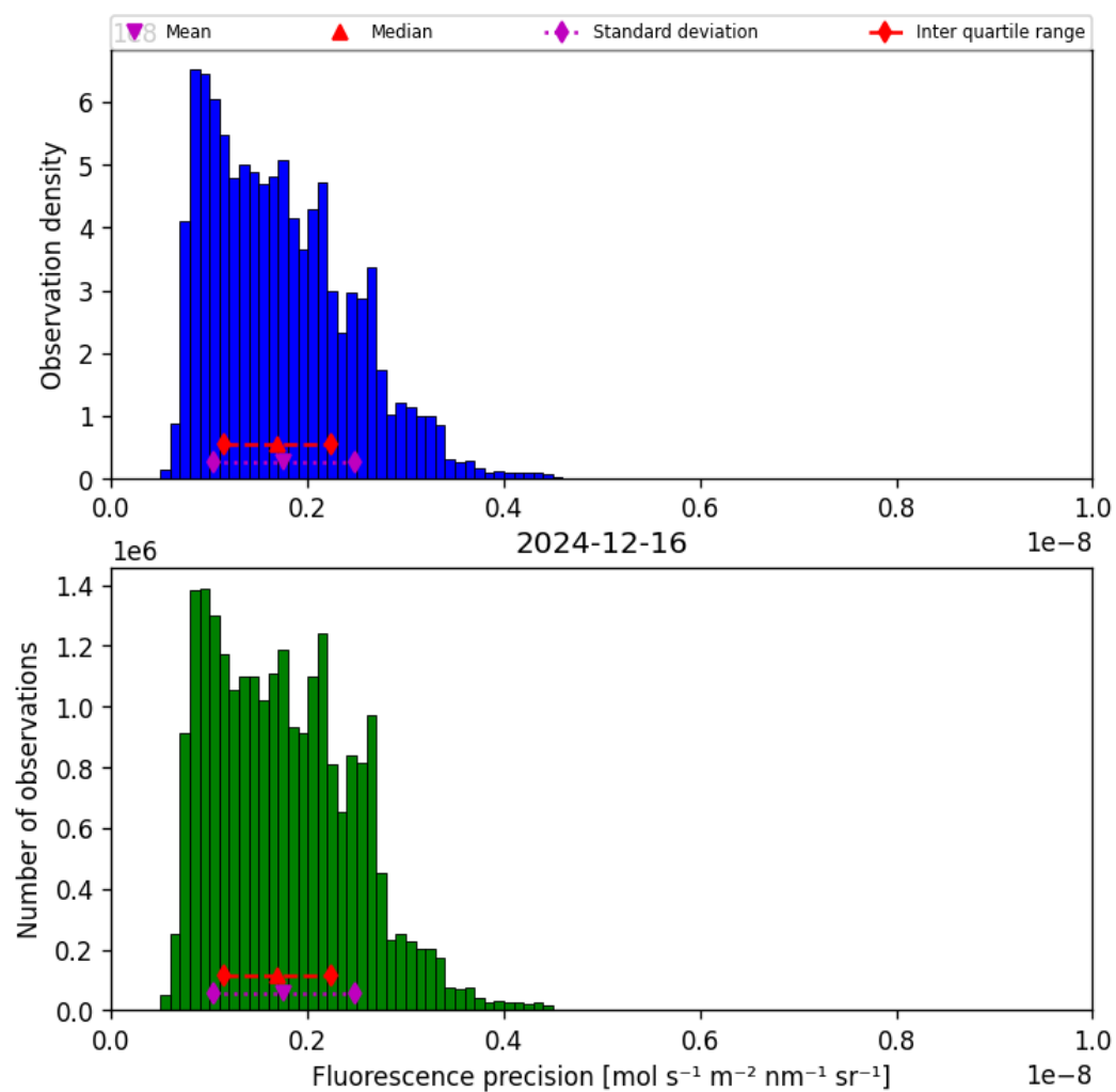
Figure 39: Histogram of “Fluorescence precision” for 2024-12-16 to 2024-12-17
