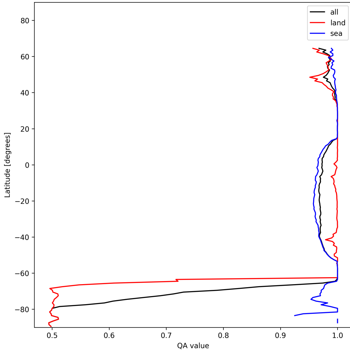
Figure 10: Zonal average of “QA value” for 2024-12-16 to 2024-12-17.
