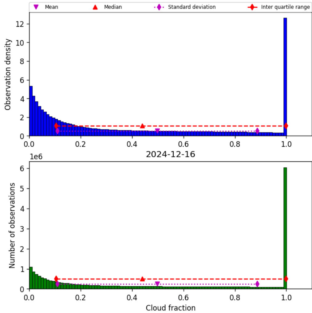
Figure 30: Histogram of “Cloud fraction” for 2024-12-16 to 2024-12-17
