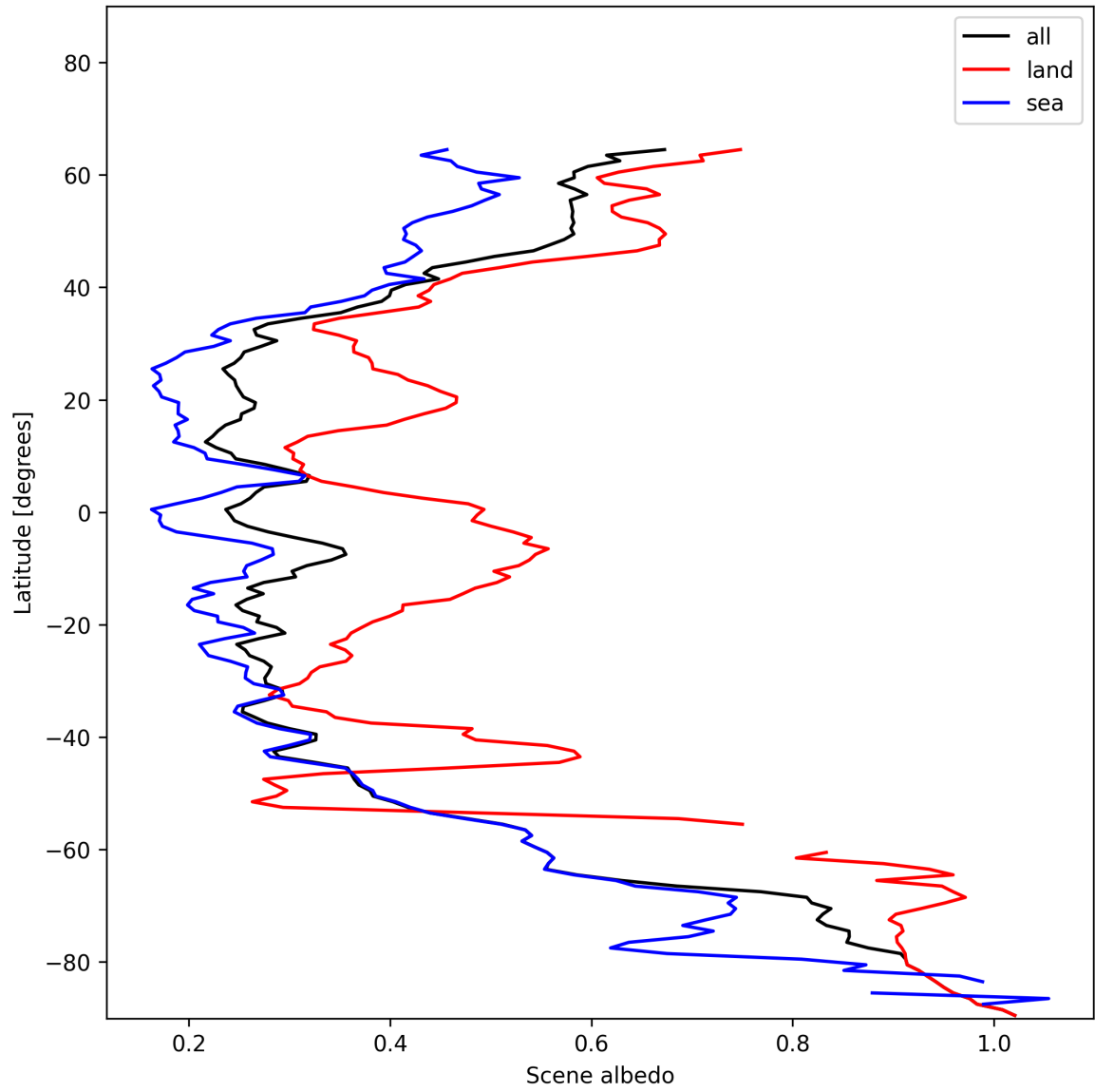
Figure 15: Zonal average of “Scene albedo” for 2024-12-16 to 2024-12-17.
