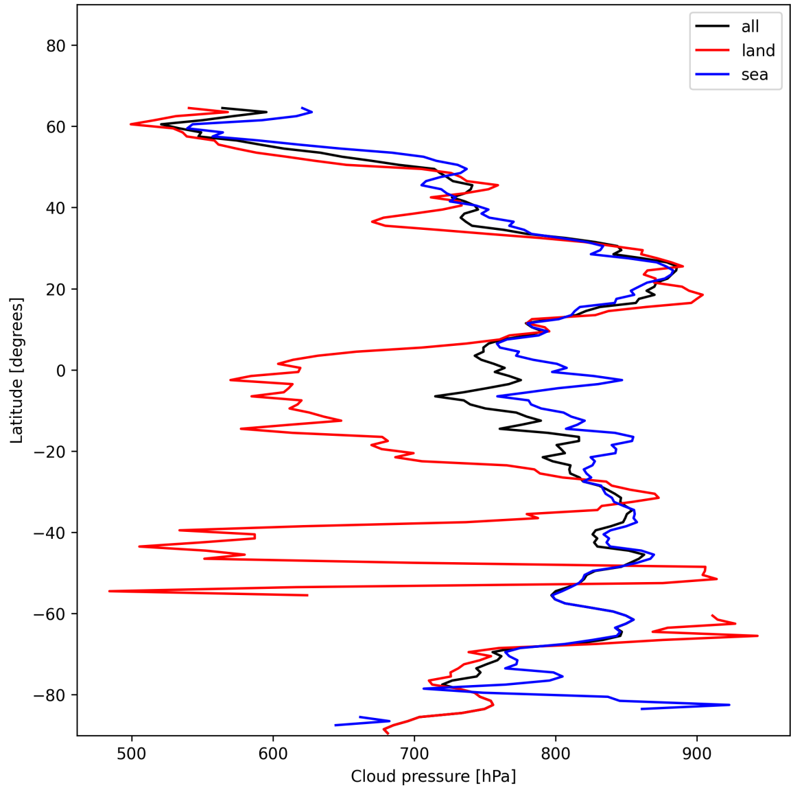
Figure 11: Zonal average of “Cloud pressure” for 2024-12-16 to 2024-12-17.
