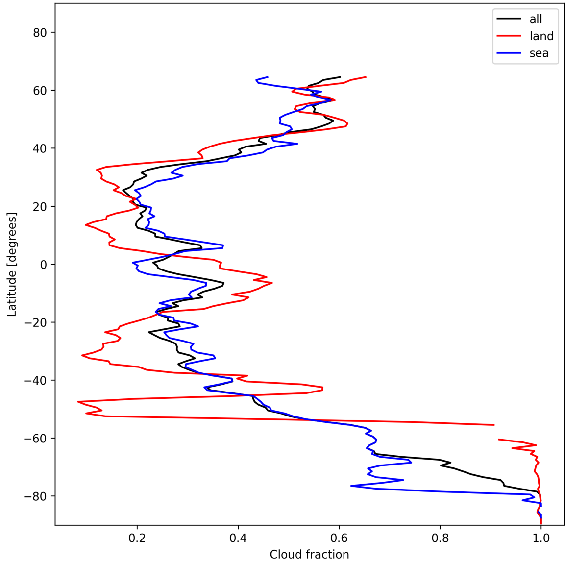
Figure 13: Zonal average of “Cloud fraction” for 2024-12-16 to 2024-12-17.
