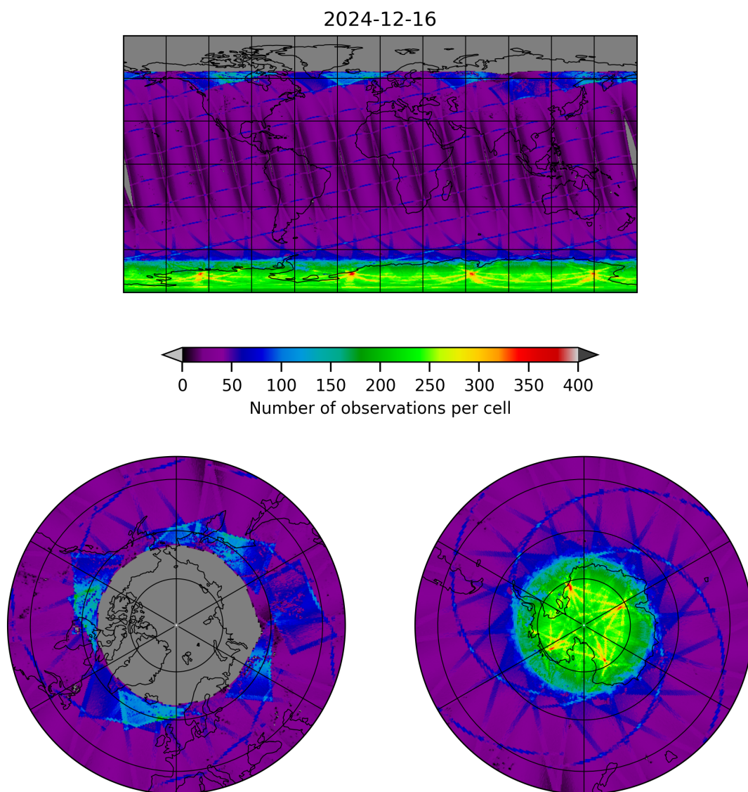
Figure 9: Map of the number of observations for 2024-12-16 to 2024-12-17
