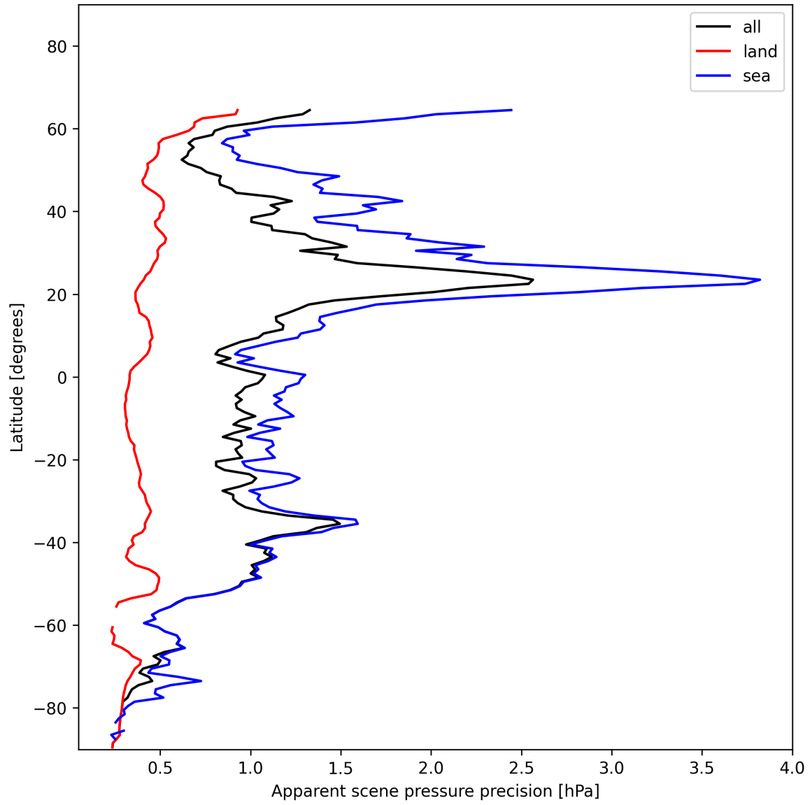
Figure 18: Zonal average of “Apparent scene pressure precision” for 2024-12-16 to 2024-12-17.
