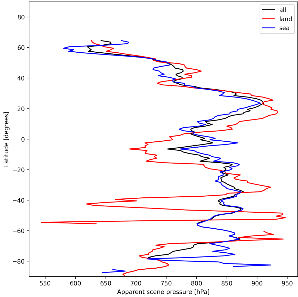
Figure 17: Zonal average of “Apparent scene pressure” for 2024-12-16 to 2024-12-17.
