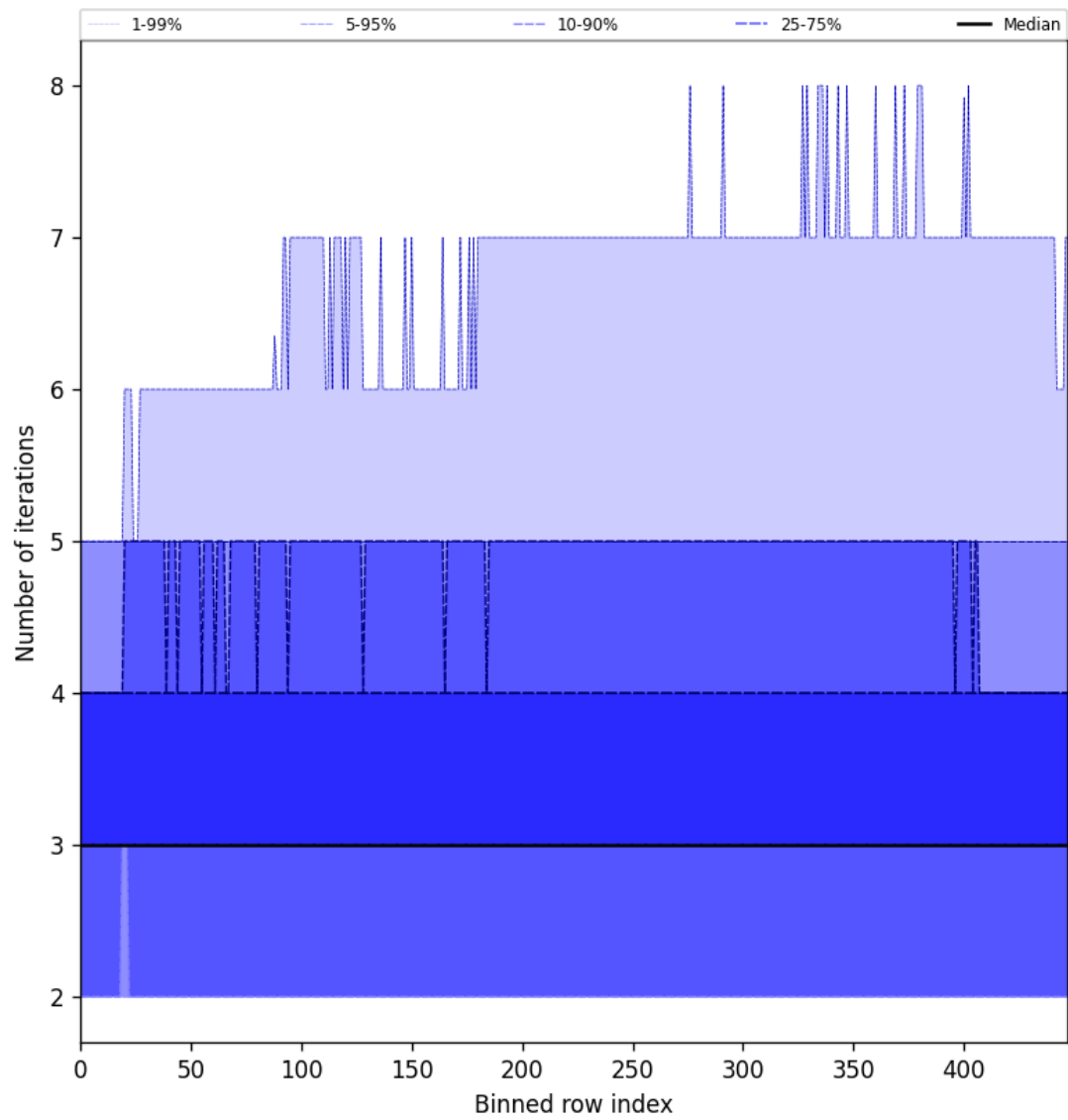
Figure 54: Along track statistics of “Number of iterations” for 2024-12-16 to 2024-12-17
