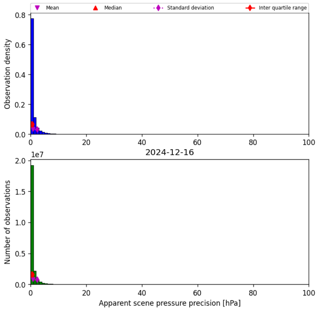
Figure 35: Histogram of “Apparent scene pressure precision” for 2024-12-16 to 2024-12-17
