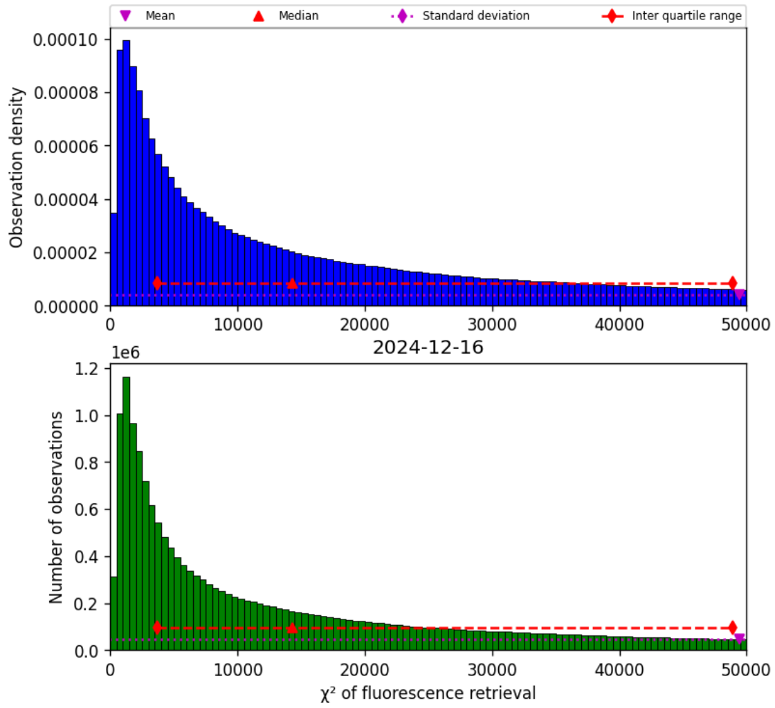
Figure 40: Histogram of “ \chi^2 of fluorescence retrieval” for 2024-12-16 to 2024-12-17
