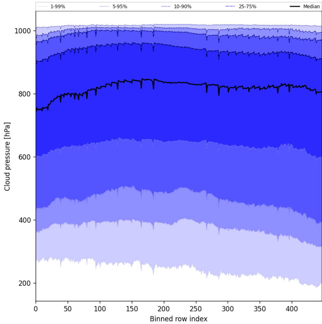
Figure 45: Along track statistics of “Cloud pressure” for 2024-12-16 to 2024-12-17
