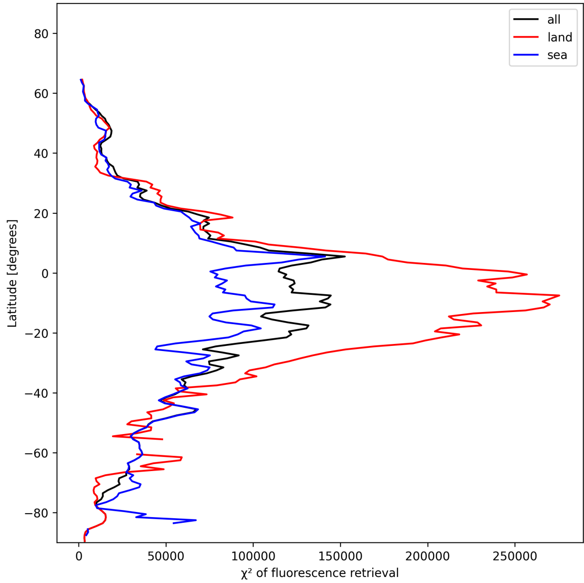
Figure 23: Zonal average of “ \chi^2 of fluorescence retrieval” for 2024-12-16 to 2024-12-17.
