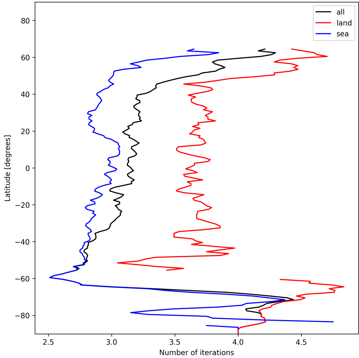
Figure 20: Zonal average of “Number of iterations” for 2024-12-16 to 2024-12-17.
