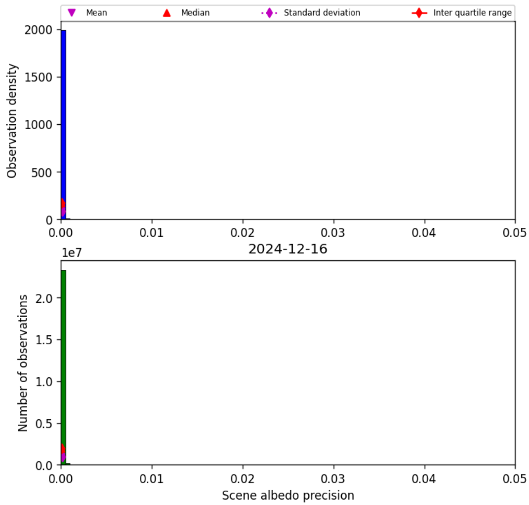
Figure 33: Histogram of “Scene albedo precision” for 2024-12-16 to 2024-12-17
