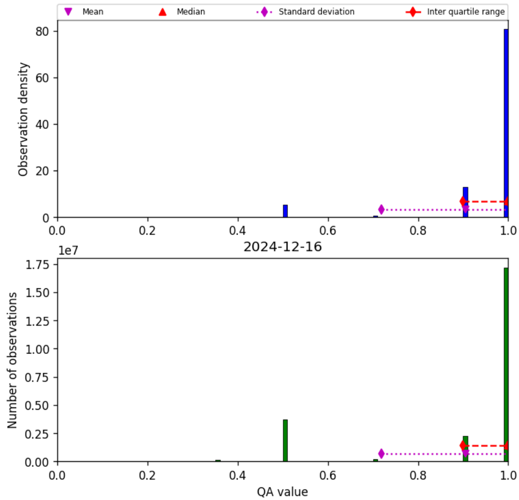
Figure 27: Histogram of “QA value” for 2024-12-16 to 2024-12-17
