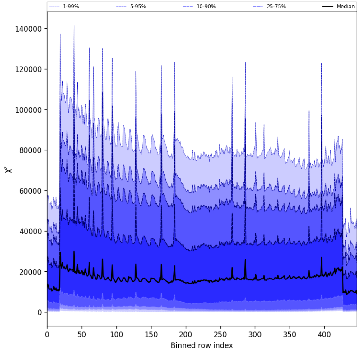
Figure 53: Along track statistics of “ \chi^2 ” for 2024-12-16 to 2024-12-17
