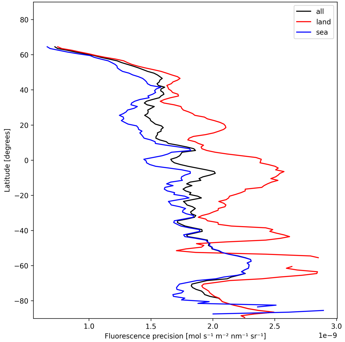
Figure 22: Zonal average of “Fluorescence precision” for 2024-12-16 to 2024-12-17.
