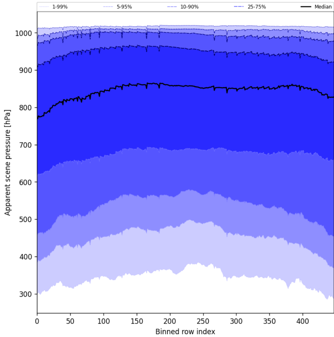
Figure 51: Along track statistics of “Apparent scene pressure” for 2024-12-16 to 2024-12-17
