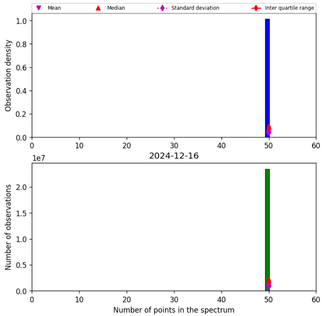
Figure 42: Histogram of “Number of points in the spectrum” for 2024-12-16 to 2024-12-17
