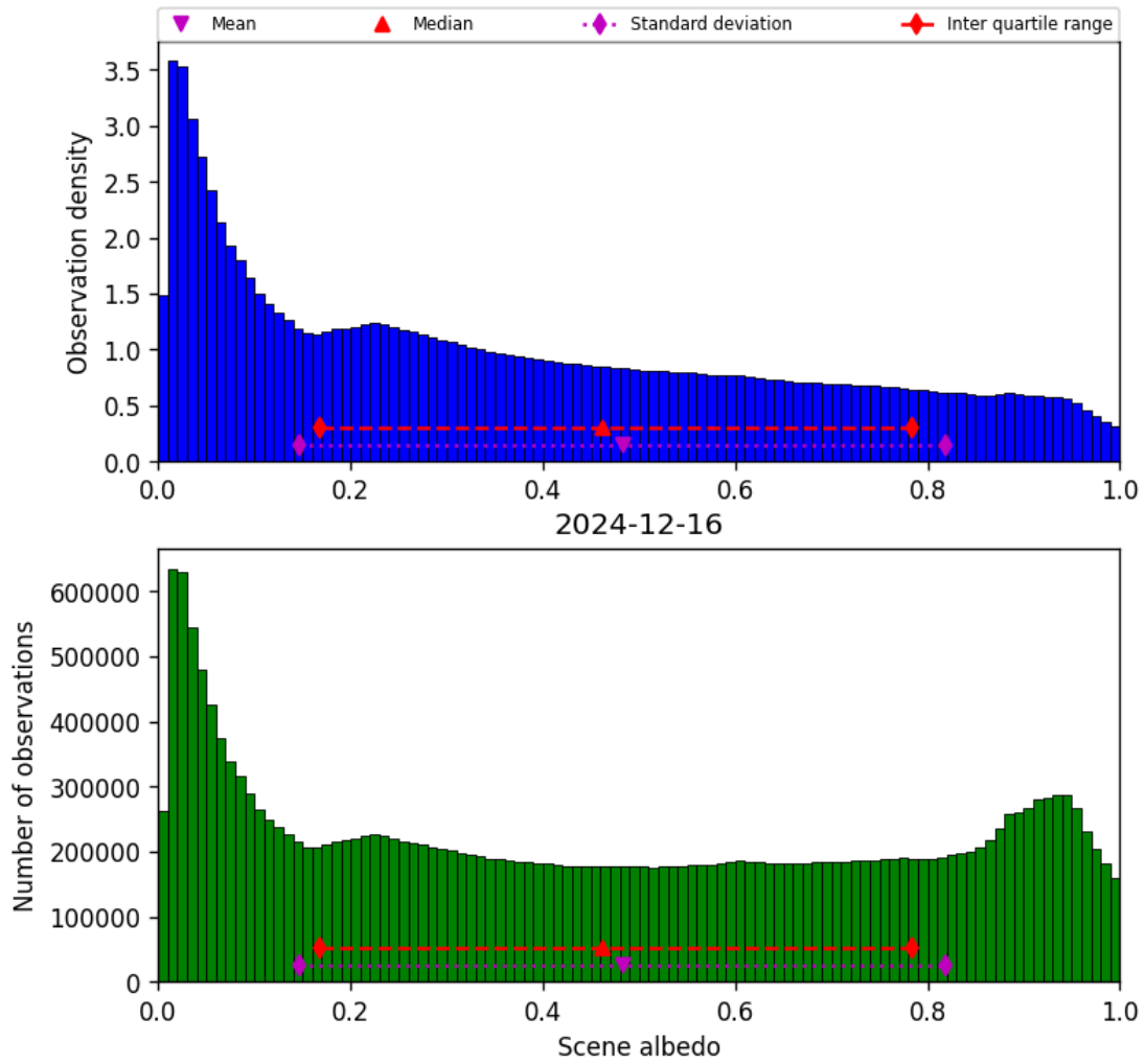
Figure 32: Histogram of “Scene albedo” for 2024-12-16 to 2024-12-17
