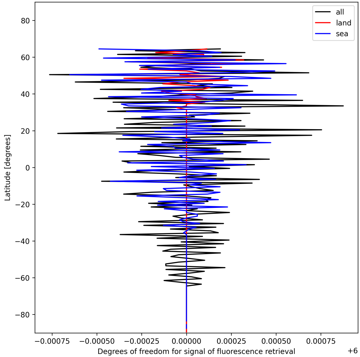
Figure 24: Zonal average of “Degrees of freedom for signal of fluorescence retrieval” for 2024-12-16 to 2024-12-17.
