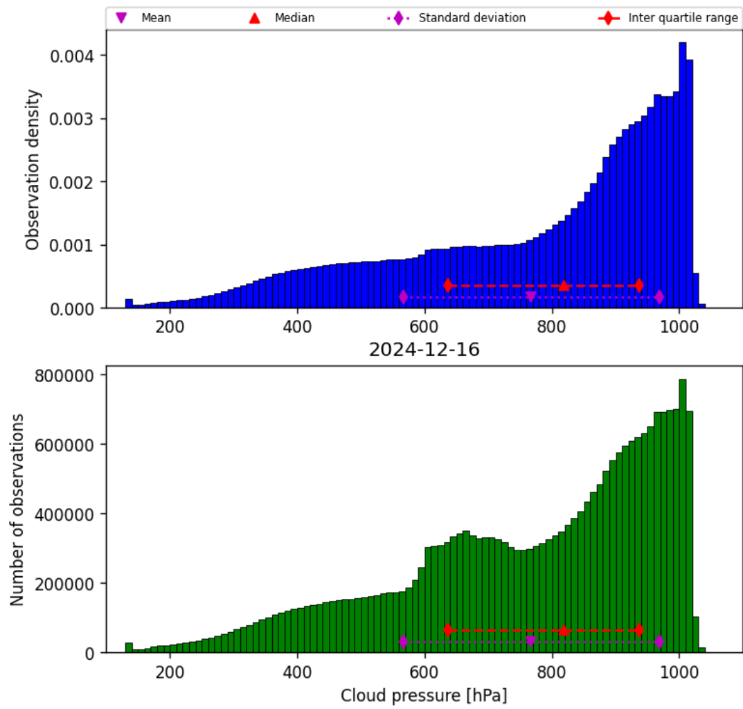
Figure 28: Histogram of “Cloud pressure” for 2024-12-16 to 2024-12-17
