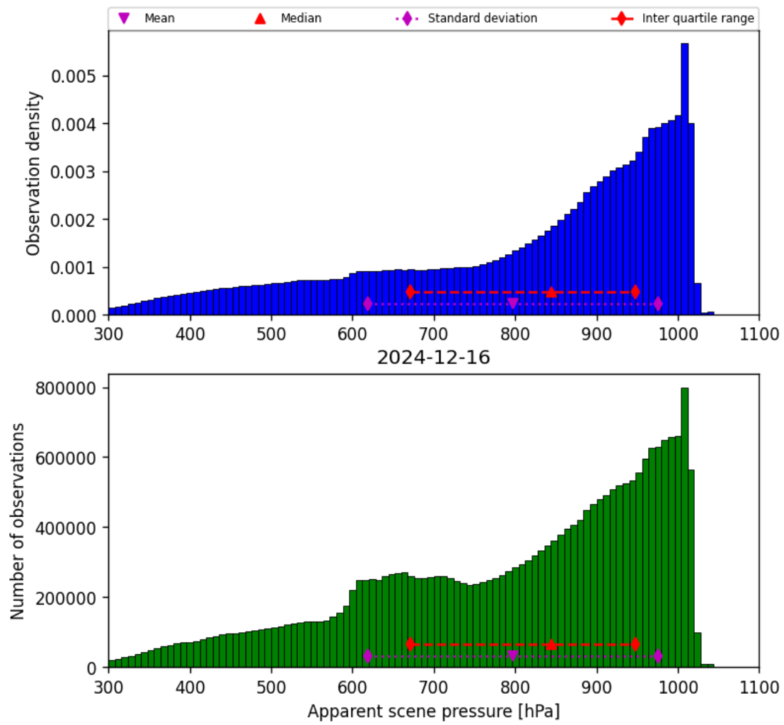
Figure 34: Histogram of “Apparent scene pressure” for 2024-12-16 to 2024-12-17
