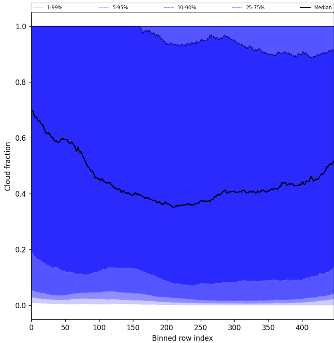
Figure 47: Along track statistics of “Cloud fraction” for 2024-12-16 to 2024-12-17
