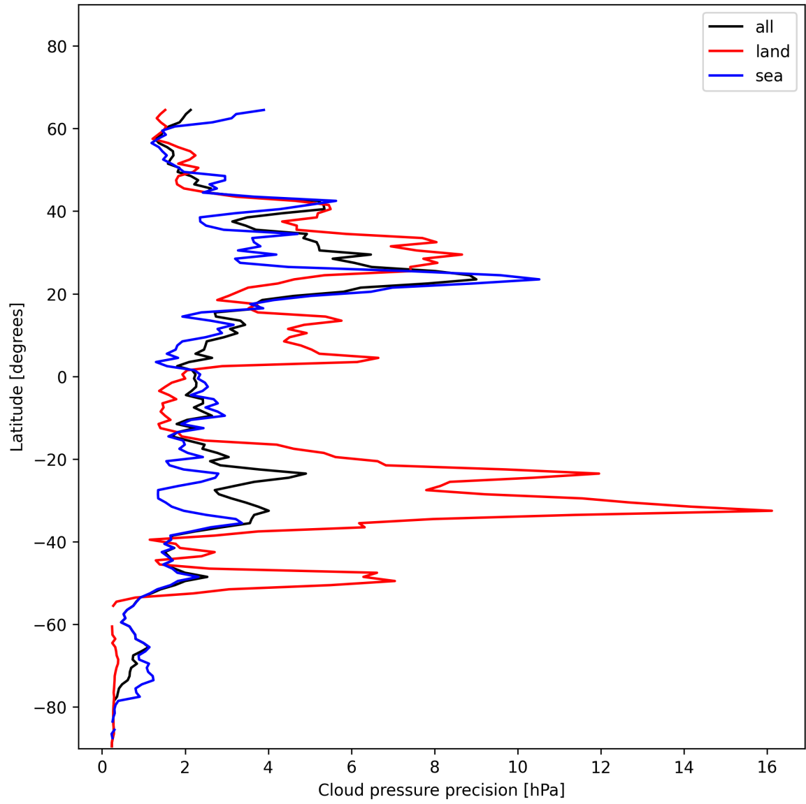
Figure 12: Zonal average of “Cloud pressure precision” for 2024-12-16 to 2024-12-17.
