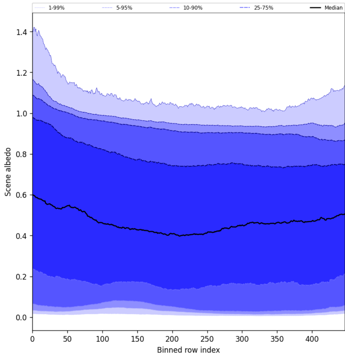
Figure 49: Along track statistics of “Scene albedo” for 2024-12-16 to 2024-12-17
