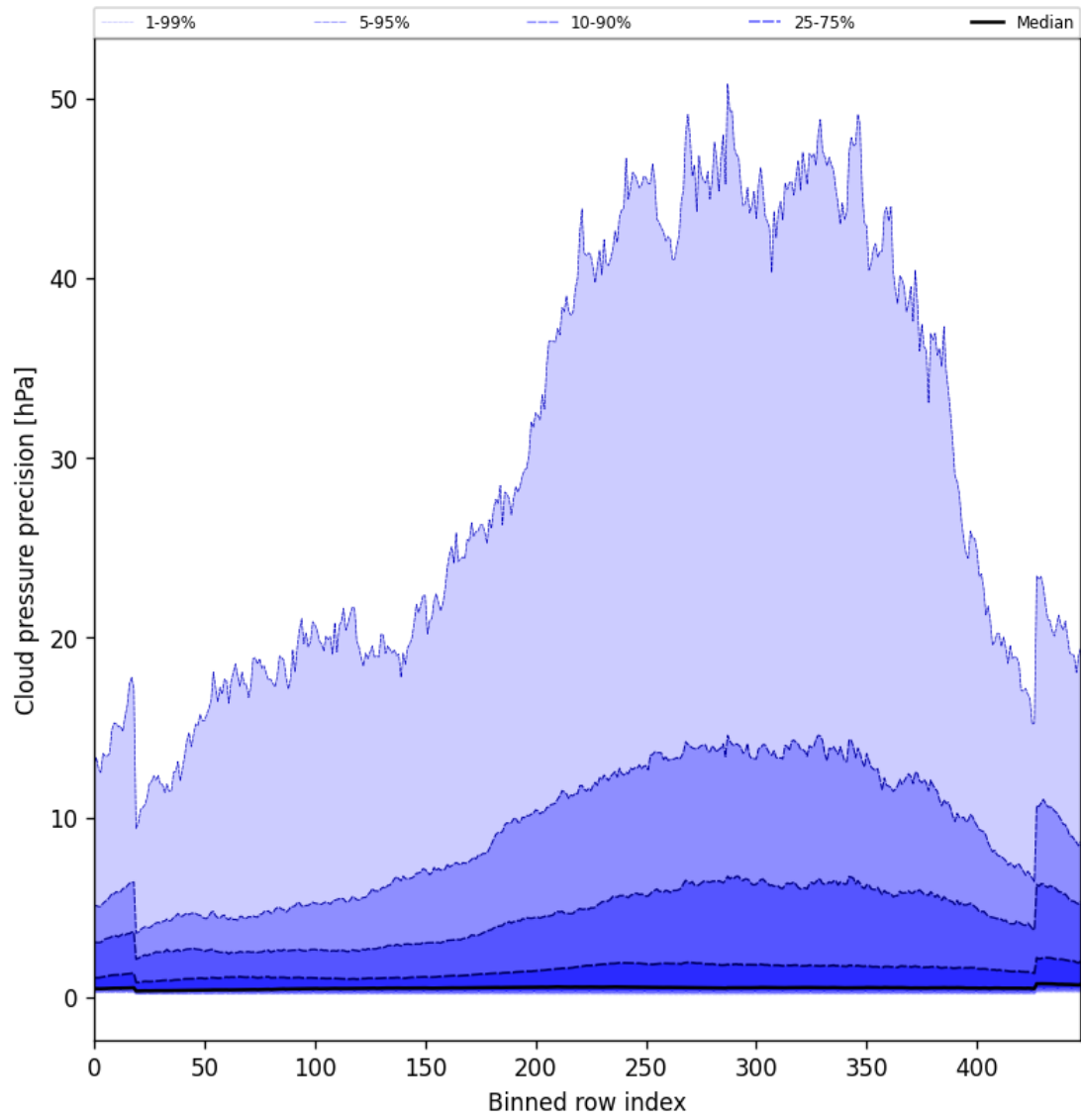
Figure 46: Along track statistics of “Cloud pressure precision” for 2024-12-16 to 2024-12-17
