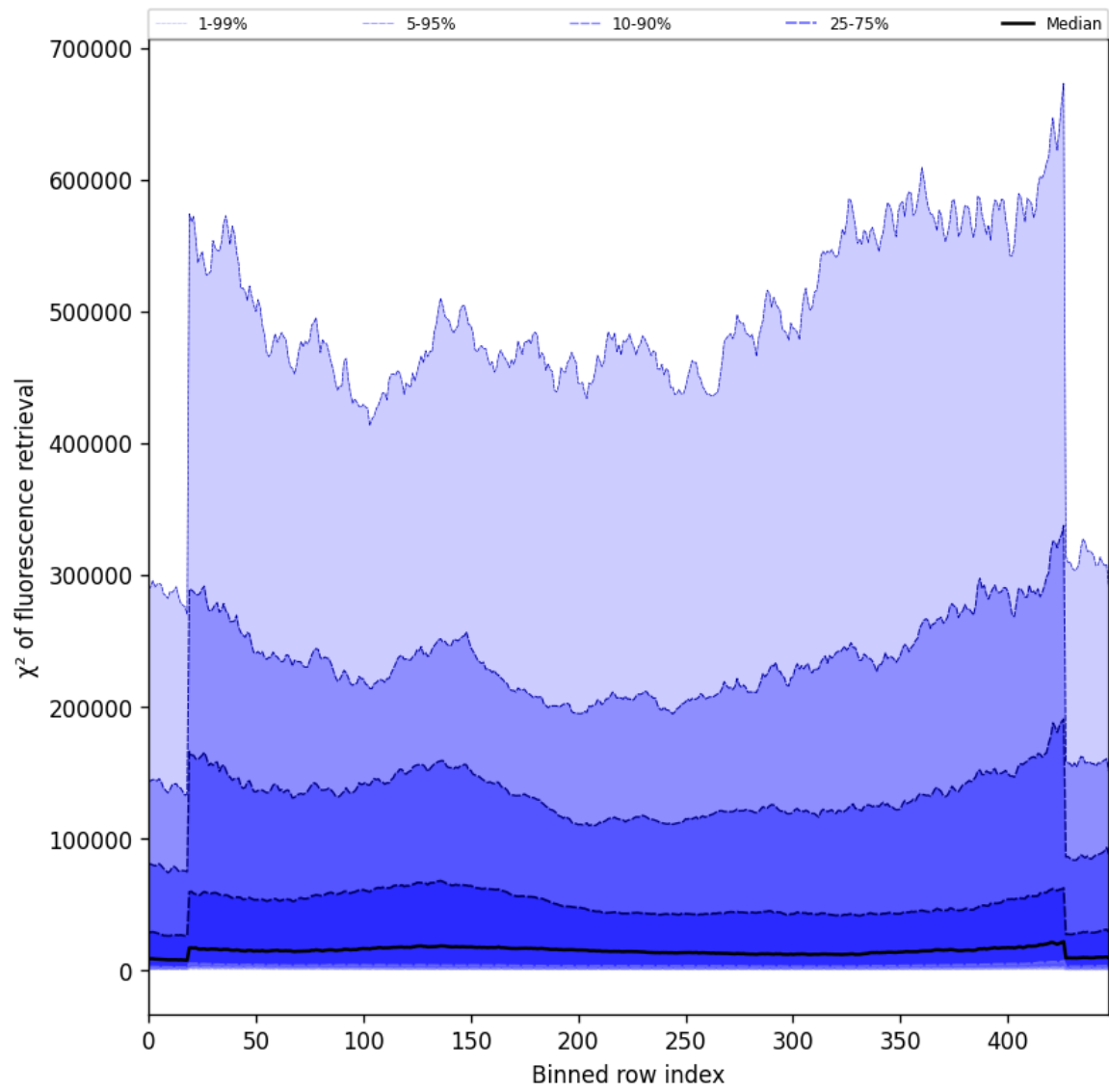
Figure 57: Along track statistics of “ \chi^2 of fluorescence retrieval” for 2024-12-16 to 2024-12-17
