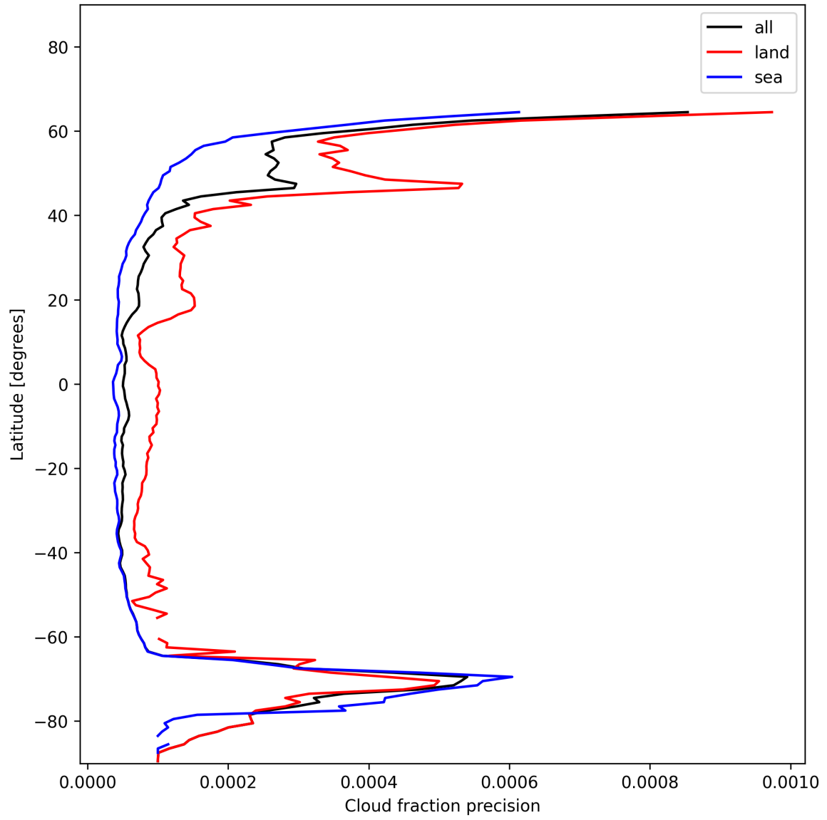
Figure 14: Zonal average of “Cloud fraction precision” for 2024-12-16 to 2024-12-17.
