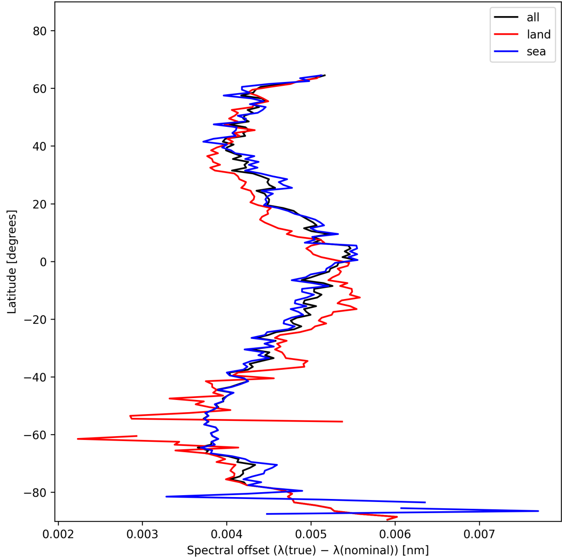
Figure 26: Zonal average of “Spectral offset ( \lambda_{\text{true}} - \lambda_{\text{nominal}} )” for 2024-12-16 to 2024-12-17.
