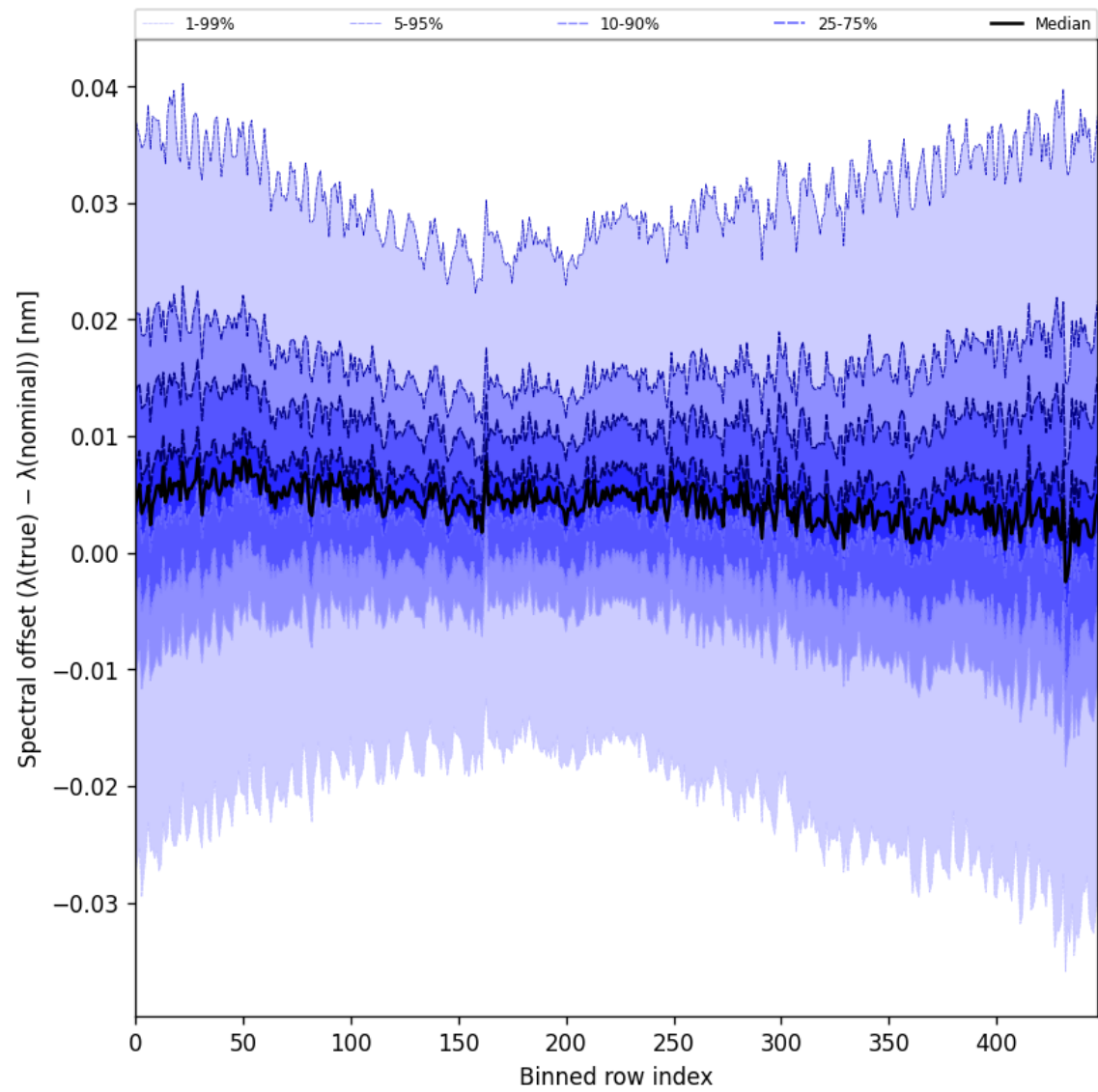
Figure 60: Along track statistics of “Spectral offset ( \lambda_{\text{true}} - \lambda_{\text{nominal}} )” for 2024-12-16 to 2024-12-17
