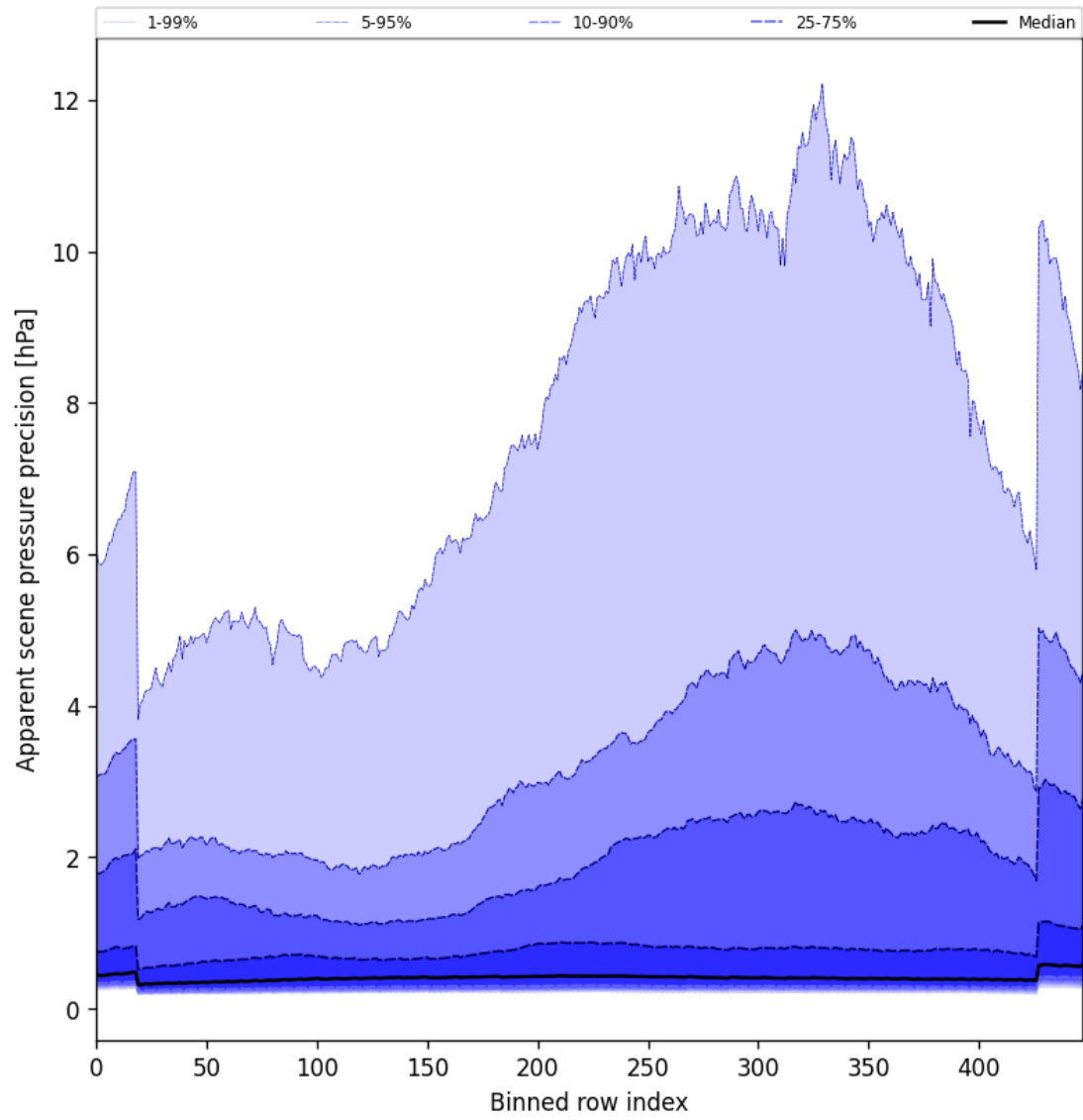
Figure 52: Along track statistics of “Apparent scene pressure precision” for 2024-12-16 to 2024-12-17
