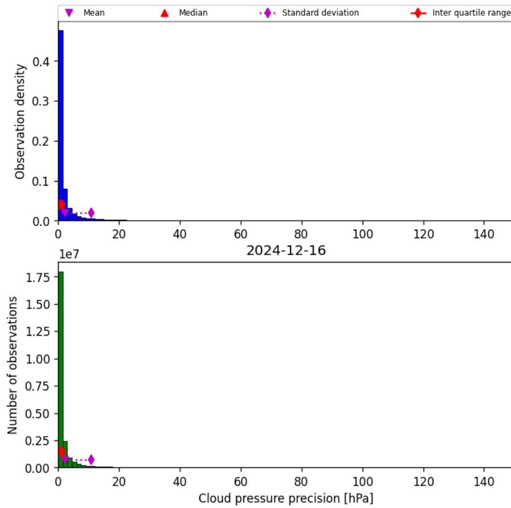
Figure 29: Histogram of “Cloud pressure precision” for 2024-12-16 to 2024-12-17
