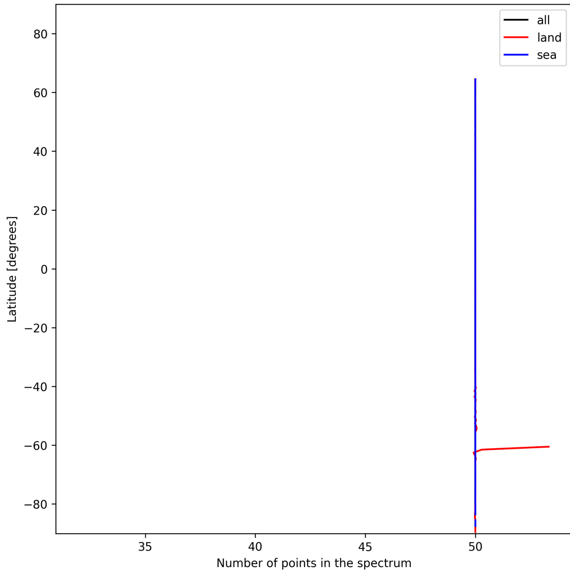
Figure 25: Zonal average of “Number of points in the spectrum” for 2024-12-16 to 2024-12-17.
