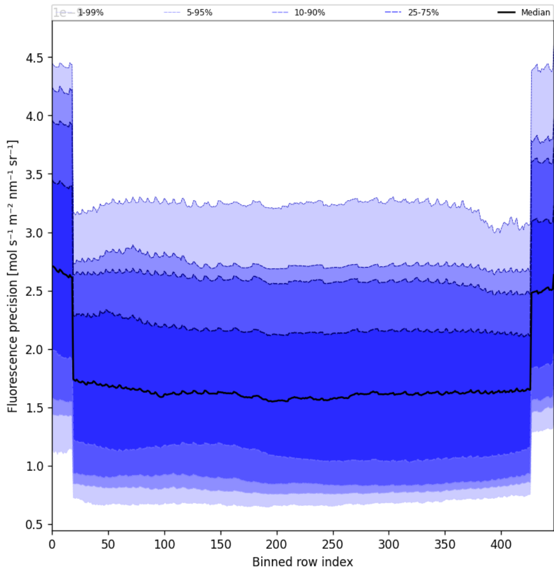
Figure 56: Along track statistics of “Fluorescence precision” for 2024-12-16 to 2024-12-17
