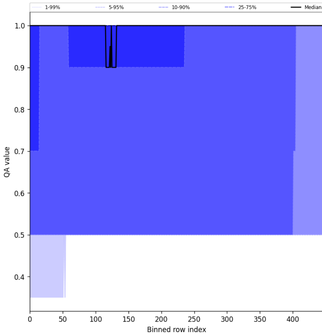
Figure 44: Along track statistics of “QA value” for 2024-12-16 to 2024-12-17
