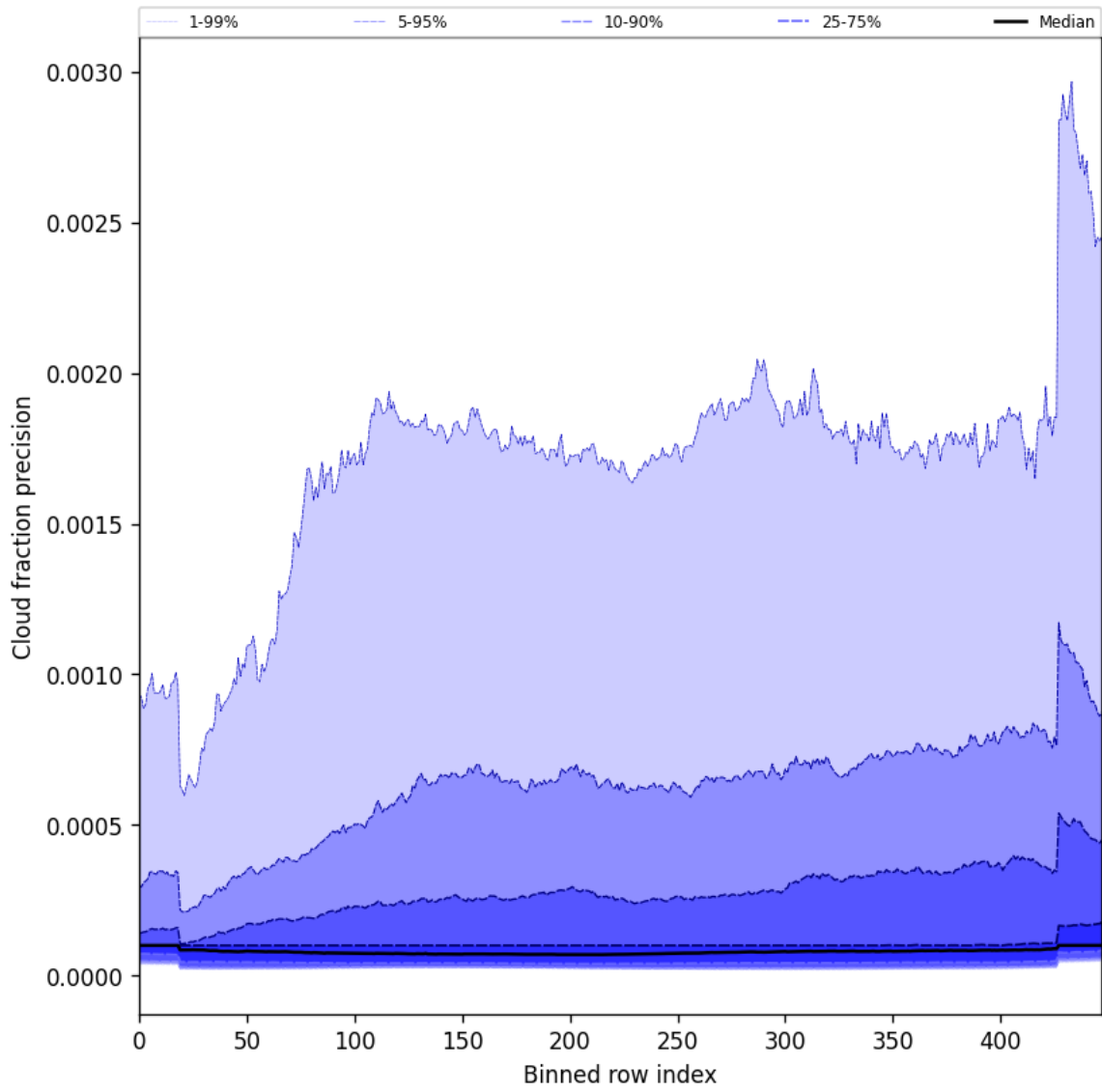
Figure 48: Along track statistics of “Cloud fraction precision” for 2024-12-16 to 2024-12-17
