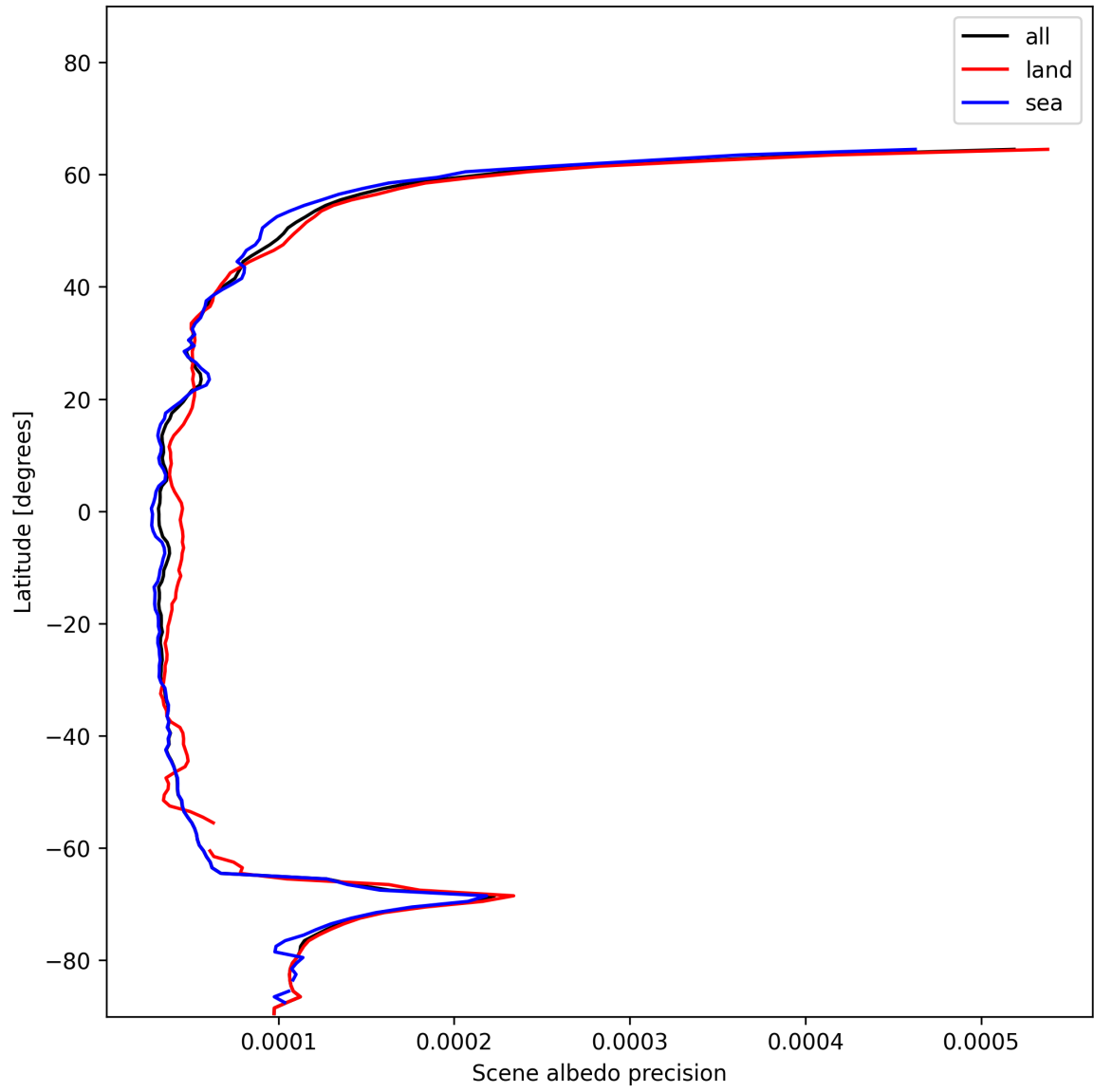
Figure 16: Zonal average of “Scene albedo precision” for 2024-12-16 to 2024-12-17.
