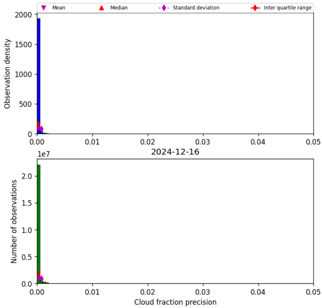
Figure 31: Histogram of “Cloud fraction precision” for 2024-12-16 to 2024-12-17
