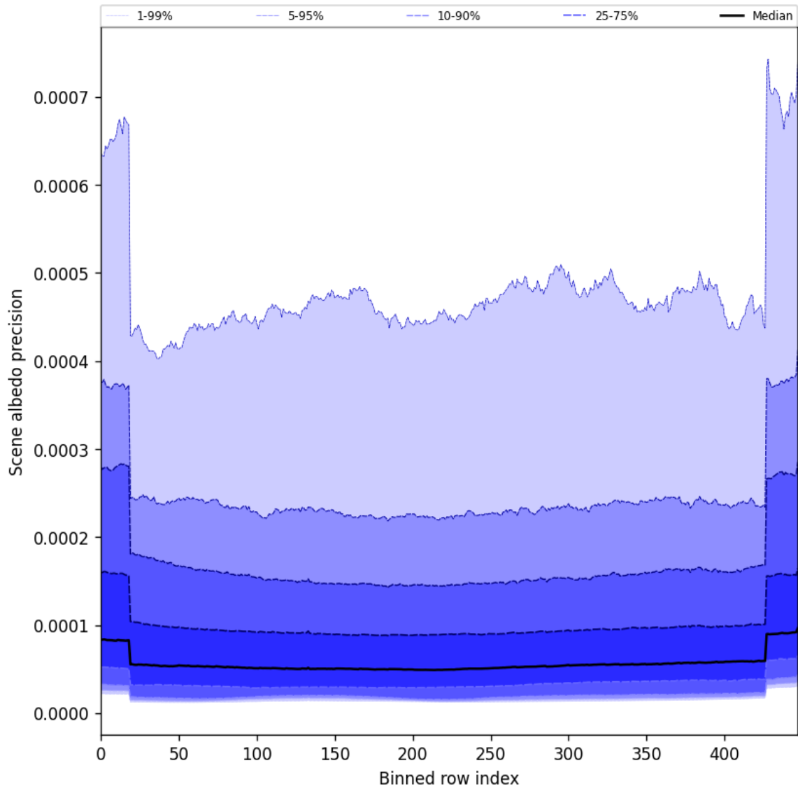
Figure 50: Along track statistics of “Scene albedo precision” for 2024-12-16 to 2024-12-17
