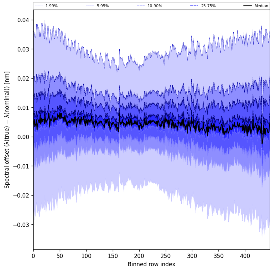
Figure 60: Along track statistics of “Spectral offset ( \lambda_{\text{true}} - \lambda_{\text{nominal}} )” for 2024-12-18 to 2024-12-19
