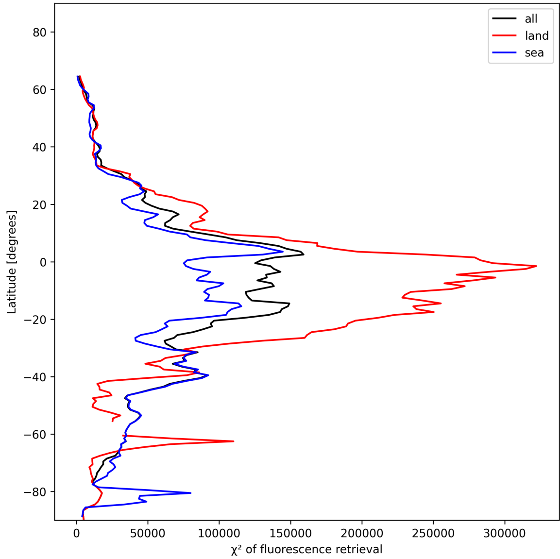
Figure 23: Zonal average of “ \chi^2 of fluorescence retrieval” for 2024-12-18 to 2024-12-19.
