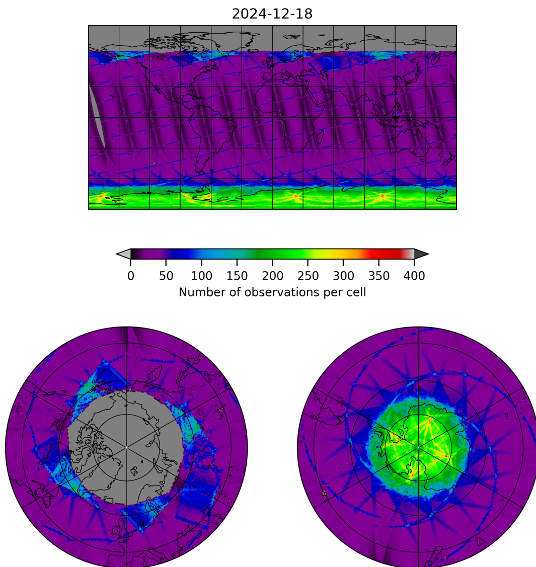
Figure 9: Map of the number of observations for 2024-12-18 to 2024-12-19
