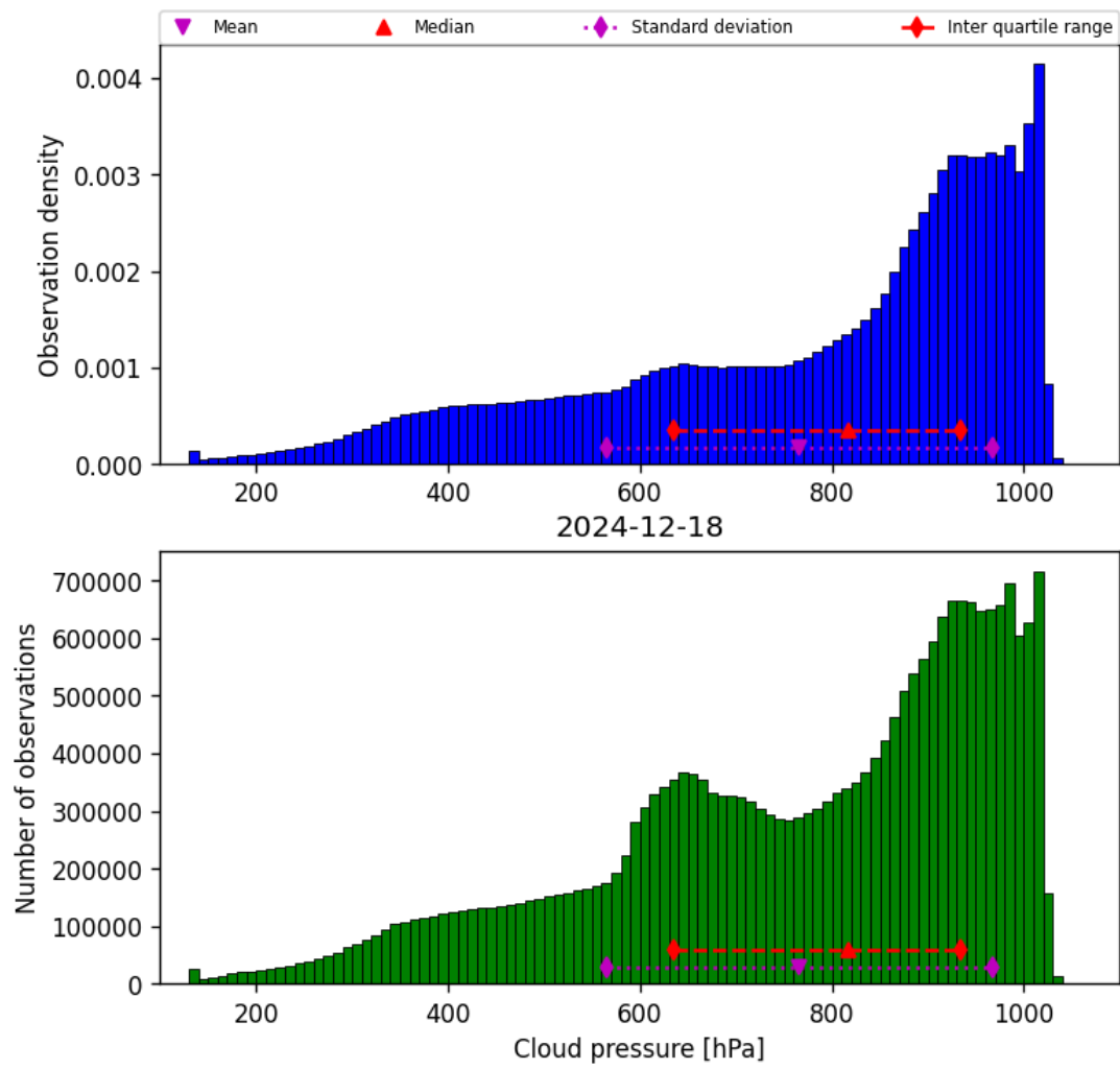
Figure 28: Histogram of “Cloud pressure” for 2024-12-18 to 2024-12-19
