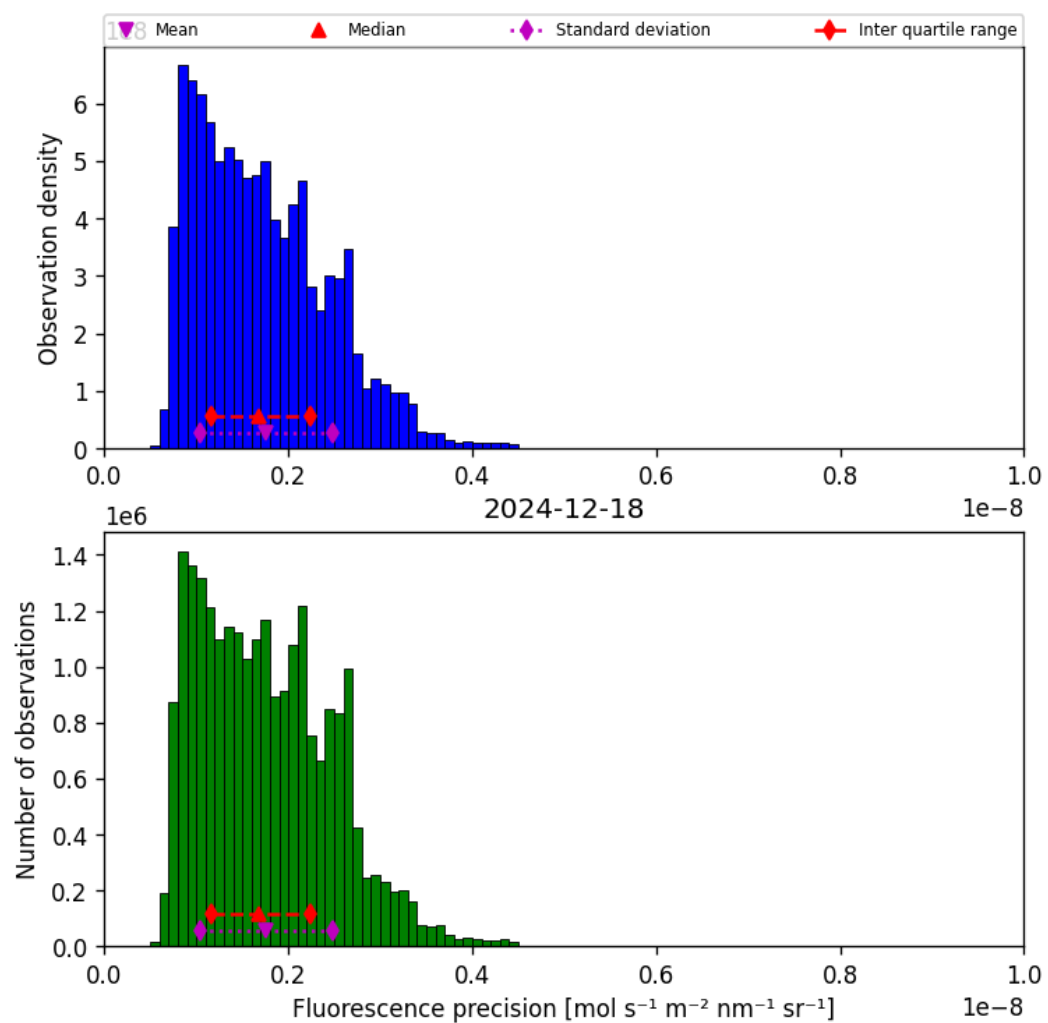
Figure 39: Histogram of “Fluorescence precision” for 2024-12-18 to 2024-12-19
