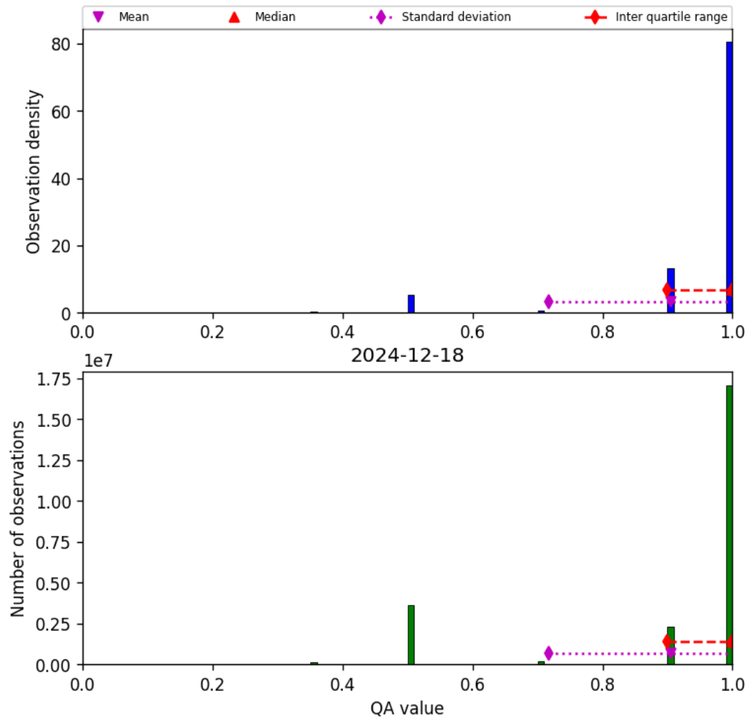
Figure 27: Histogram of “QA value” for 2024-12-18 to 2024-12-19
