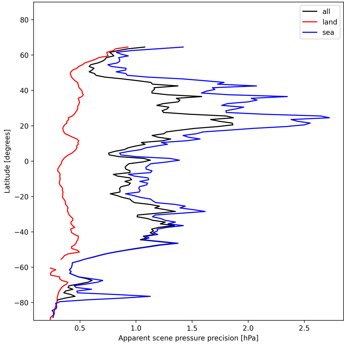
Figure 18: Zonal average of “Apparent scene pressure precision” for 2024-12-18 to 2024-12-19.
