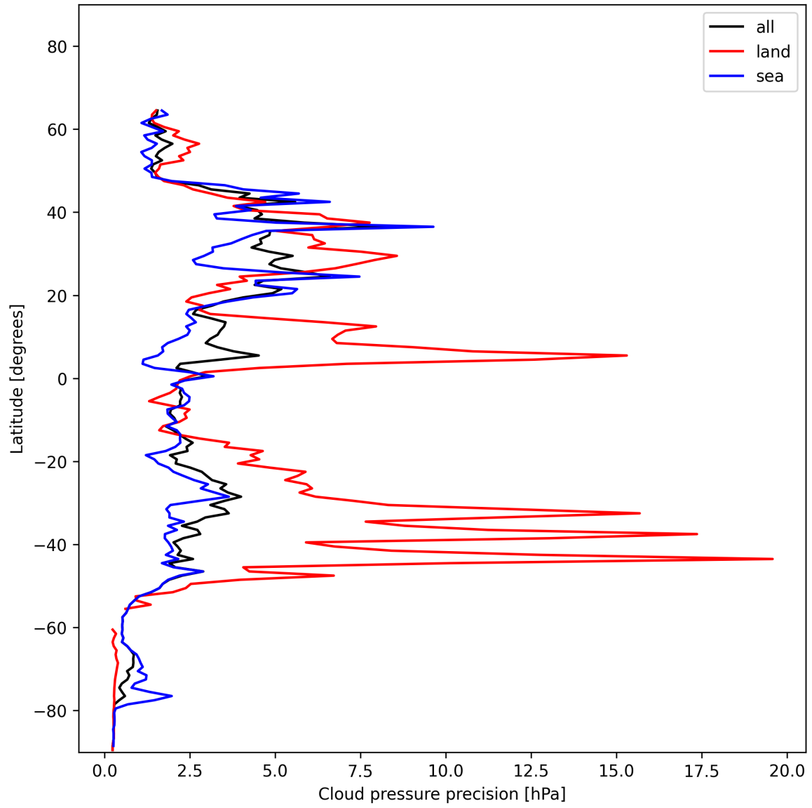
Figure 12: Zonal average of “Cloud pressure precision” for 2024-12-18 to 2024-12-19.
