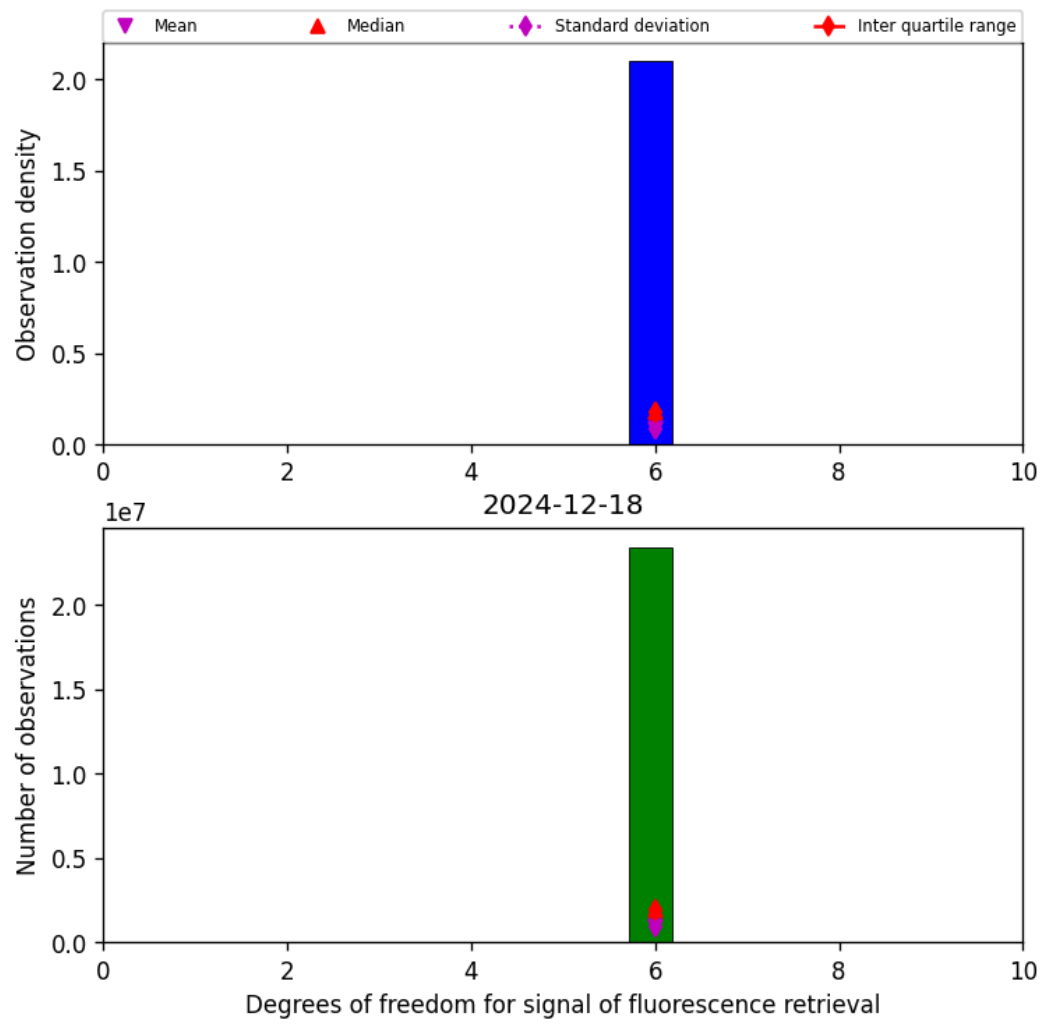
Figure 41: Histogram of “Degrees of freedom for signal of fluorescence retrieval” for 2024-12-18 to 2024-12-19
