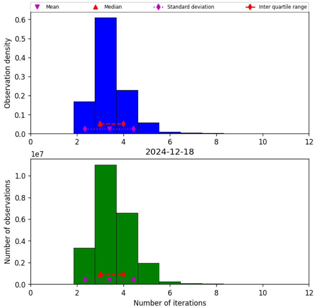
Figure 37: Histogram of “Number of iterations” for 2024-12-18 to 2024-12-19
