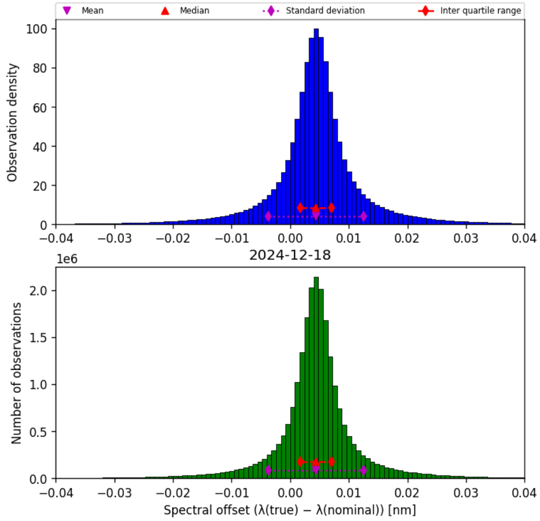
Figure 43: Histogram of “Spectral offset ( \lambda_{\text{true}} - \lambda_{\text{nominal}} )” for 2024-12-18 to 2024-12-19
