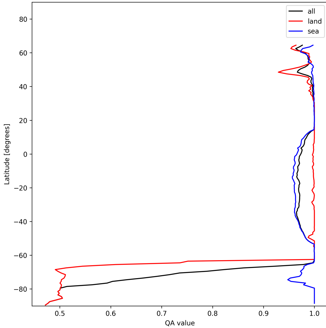
Figure 10: Zonal average of “QA value” for 2024-12-18 to 2024-12-19.
