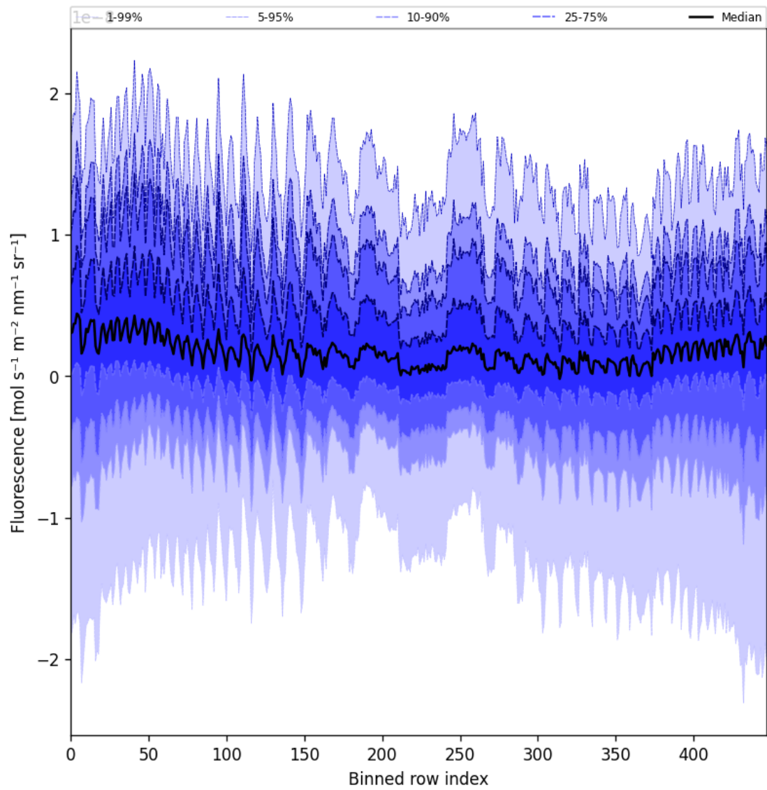
Figure 55: Along track statistics of “Fluorescence” for 2024-12-18 to 2024-12-19
