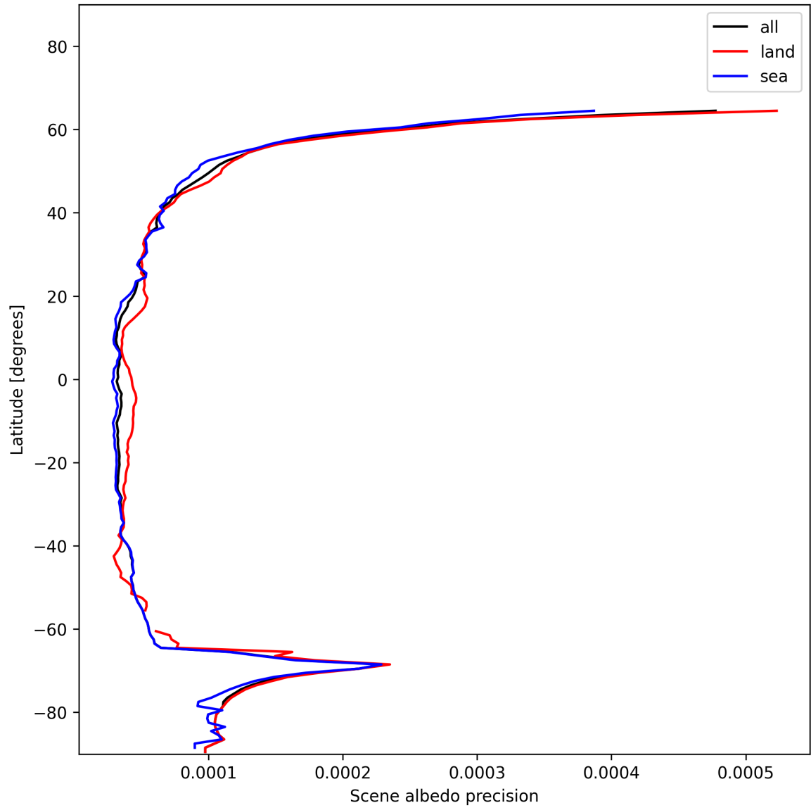
Figure 16: Zonal average of “Scene albedo precision” for 2024-12-18 to 2024-12-19.
