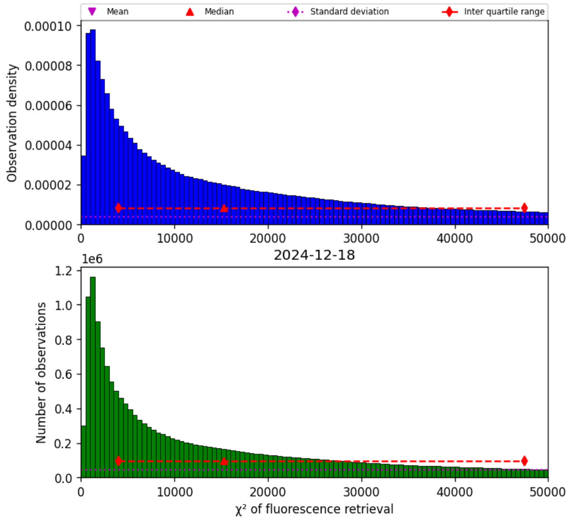
Figure 40: Histogram of “ \chi^2 of fluorescence retrieval” for 2024-12-18 to 2024-12-19
