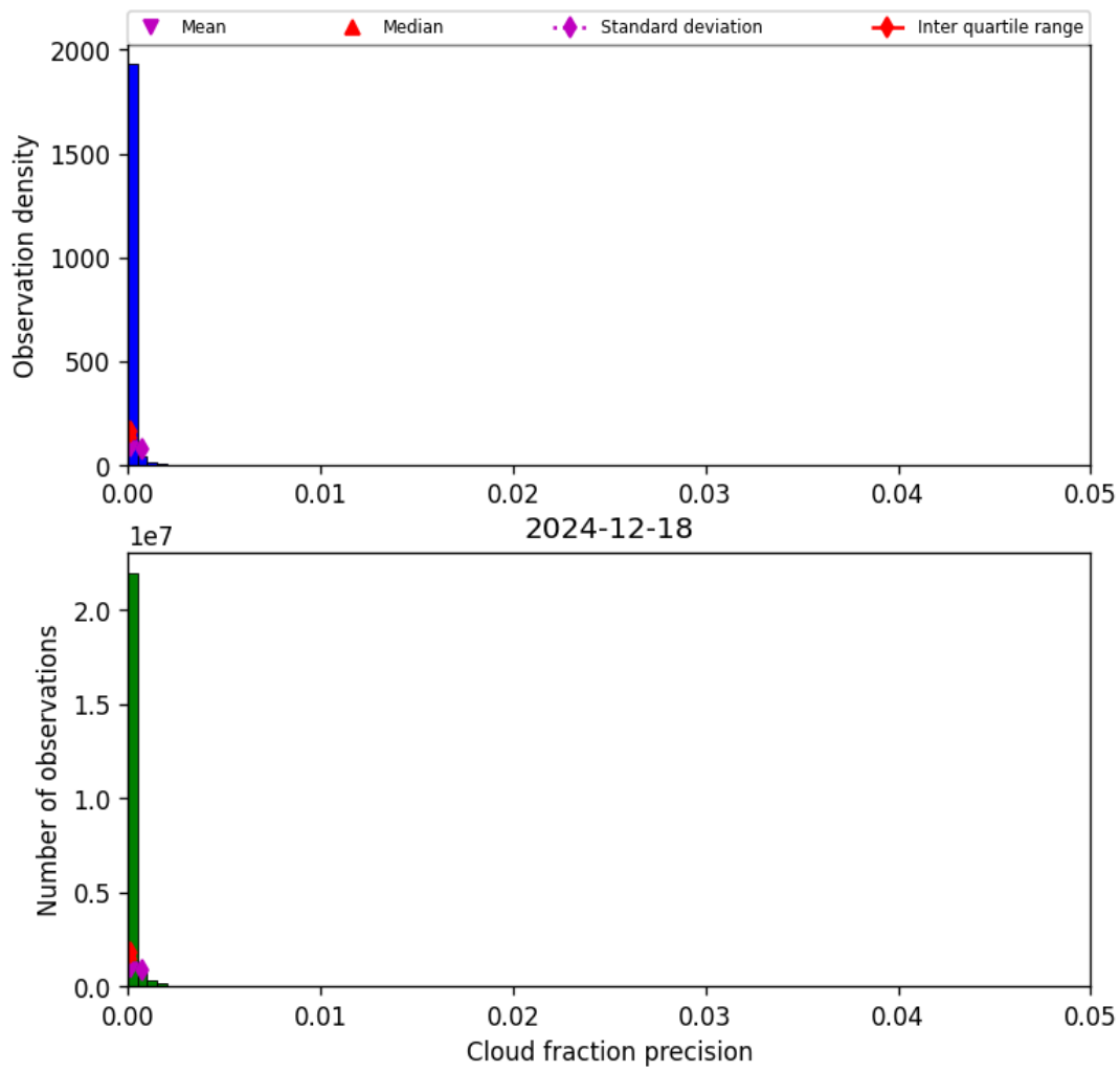
Figure 31: Histogram of “Cloud fraction precision” for 2024-12-18 to 2024-12-19
