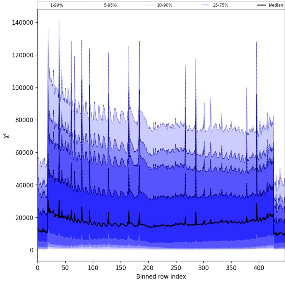
Figure 53: Along track statistics of “ \chi^2 ” for 2024-12-18 to 2024-12-19
