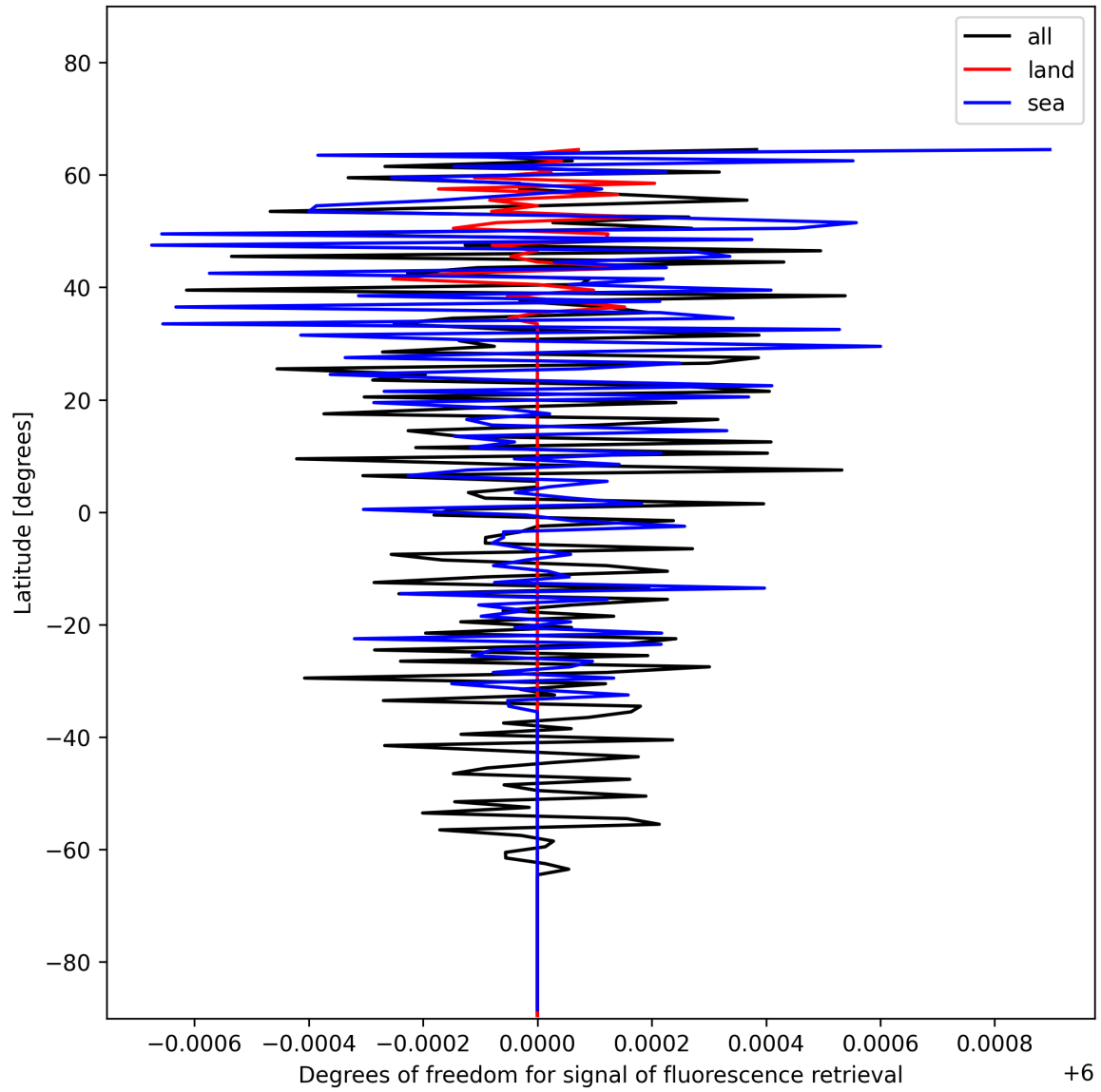
Figure 24: Zonal average of “Degrees of freedom for signal of fluorescence retrieval” for 2024-12-18 to 2024-12-19.
