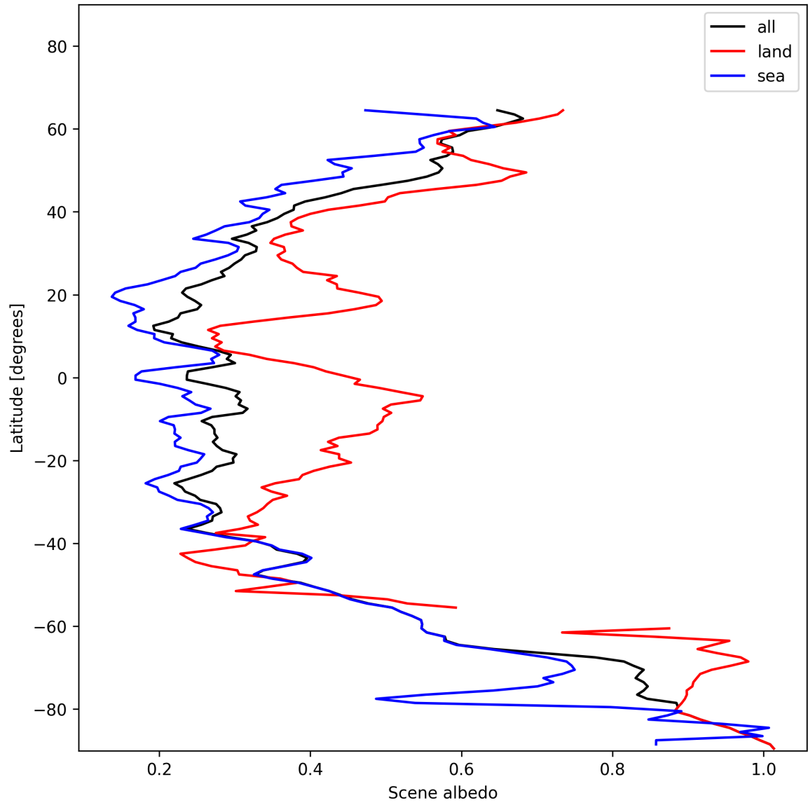
Figure 15: Zonal average of “Scene albedo” for 2024-12-18 to 2024-12-19.
