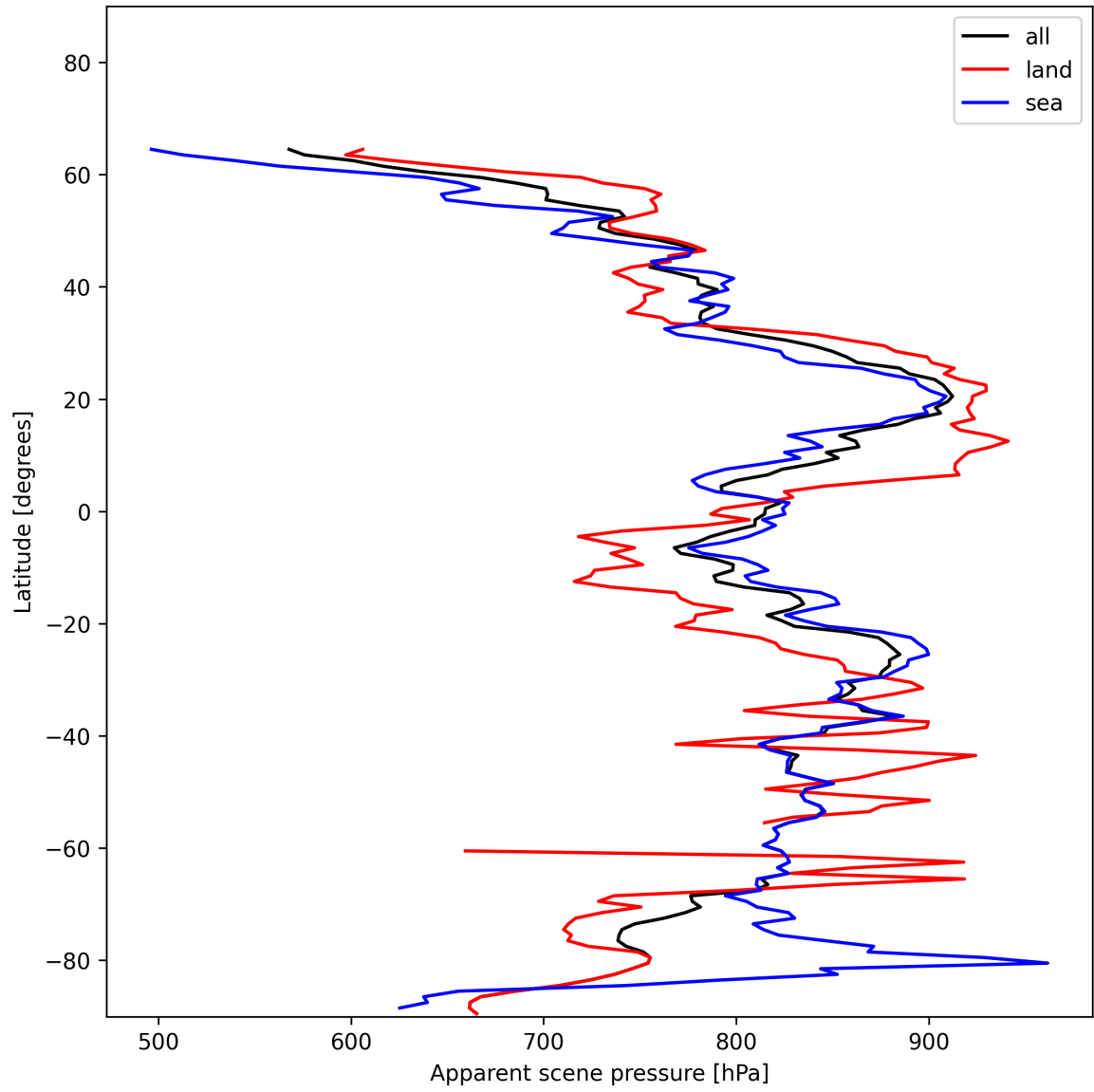
Figure 17: Zonal average of “Apparent scene pressure” for 2024-12-18 to 2024-12-19.
