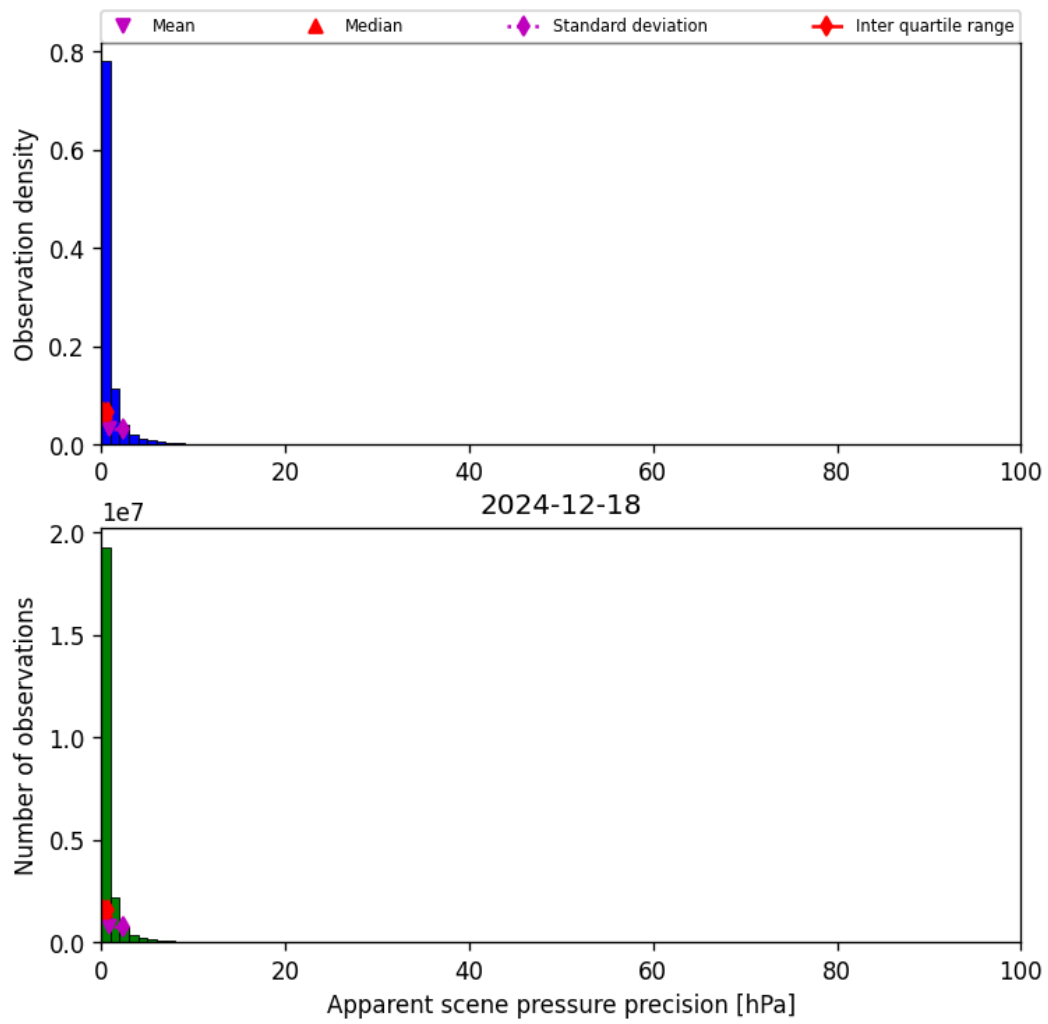
Figure 35: Histogram of “Apparent scene pressure precision” for 2024-12-18 to 2024-12-19
