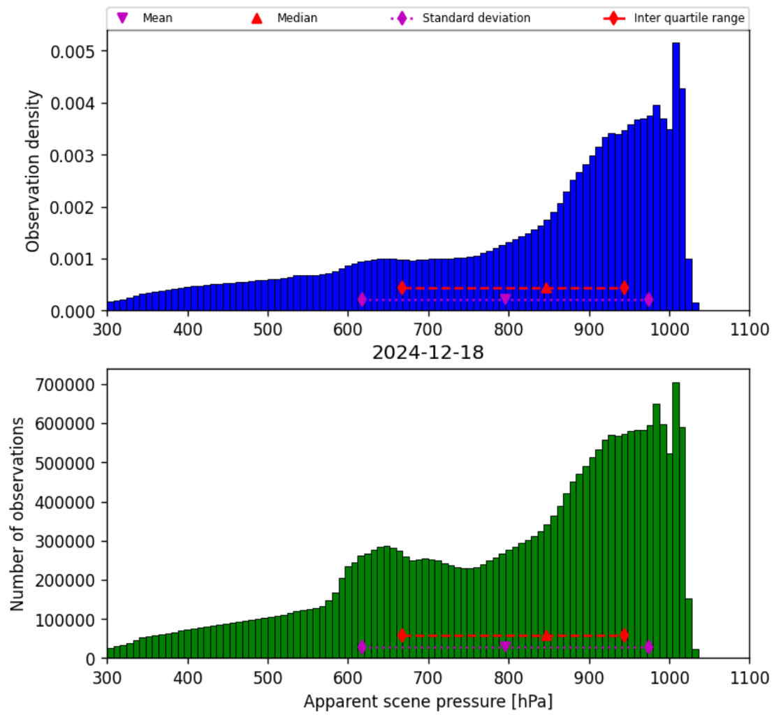
Figure 34: Histogram of “Apparent scene pressure” for 2024-12-18 to 2024-12-19
