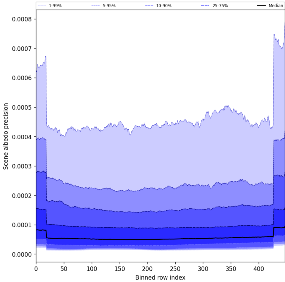
Figure 50: Along track statistics of “Scene albedo precision” for 2024-12-18 to 2024-12-19
