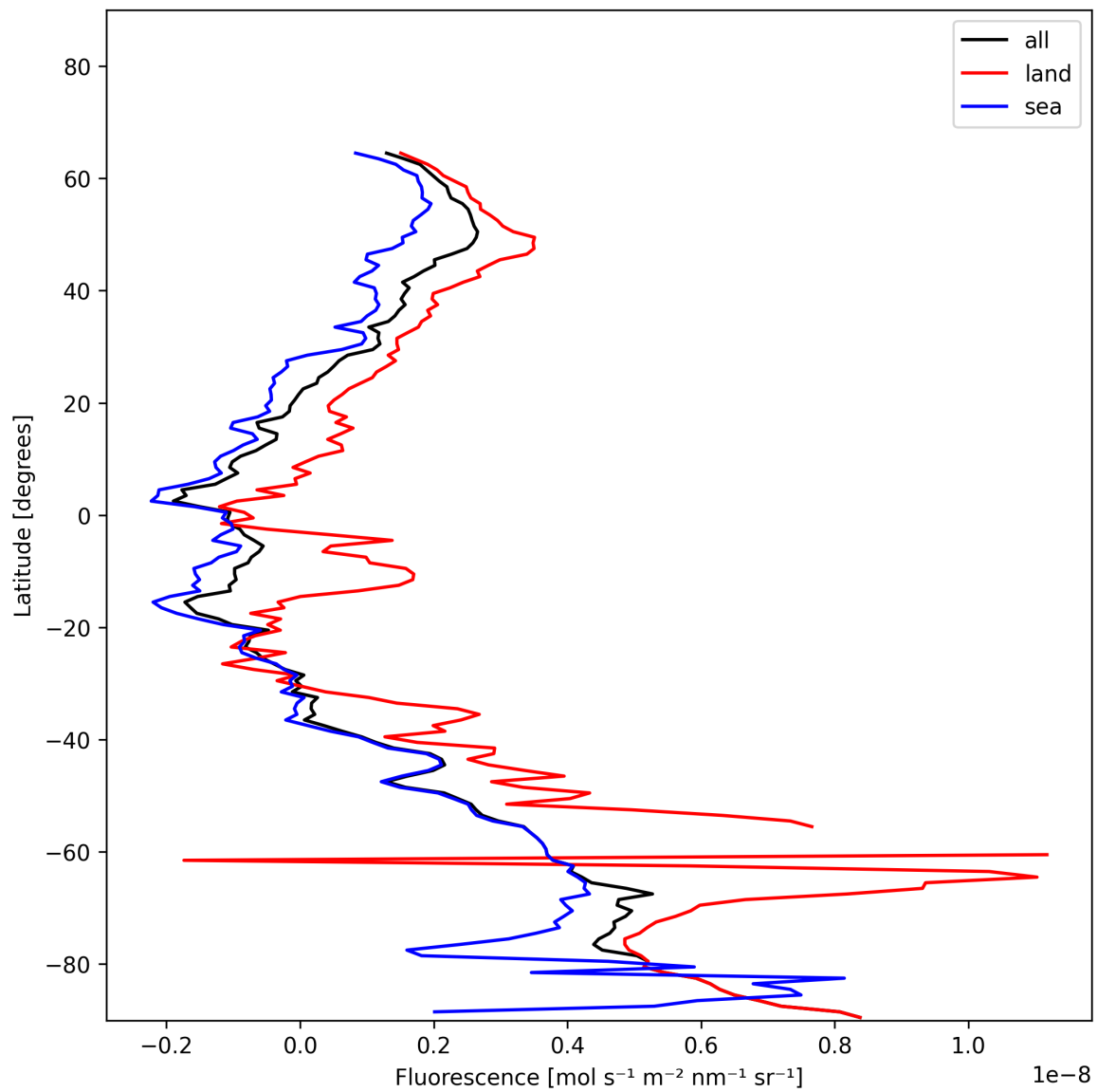
Figure 21: Zonal average of “Fluorescence” for 2024-12-18 to 2024-12-19.
