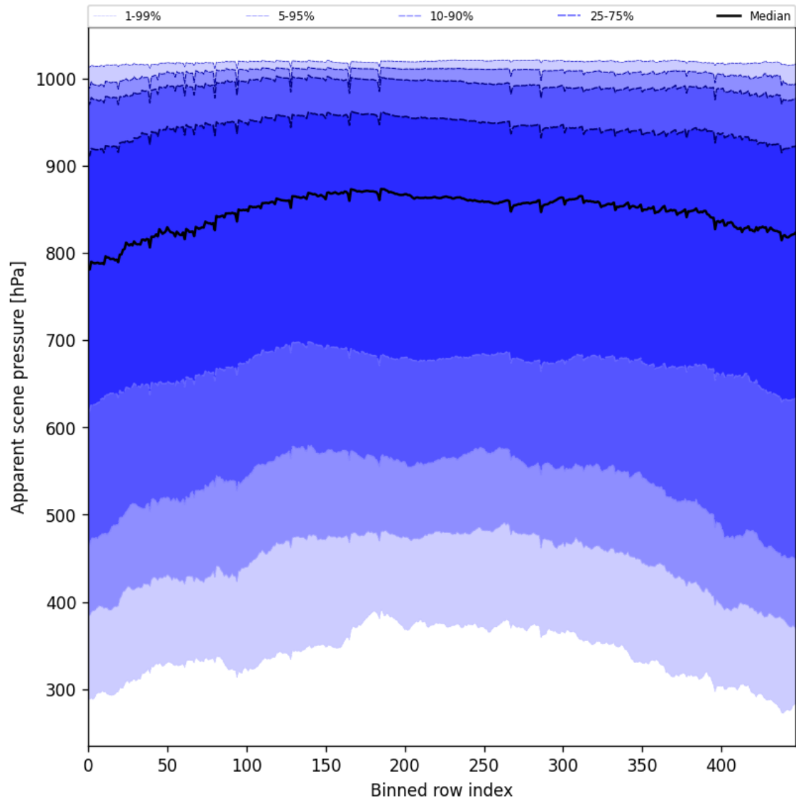
Figure 51: Along track statistics of “Apparent scene pressure” for 2024-12-18 to 2024-12-19
