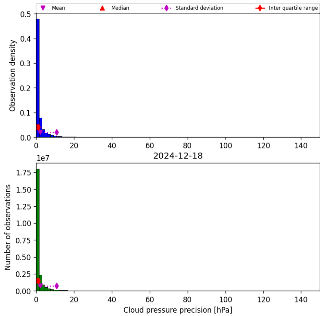
Figure 29: Histogram of “Cloud pressure precision” for 2024-12-18 to 2024-12-19
