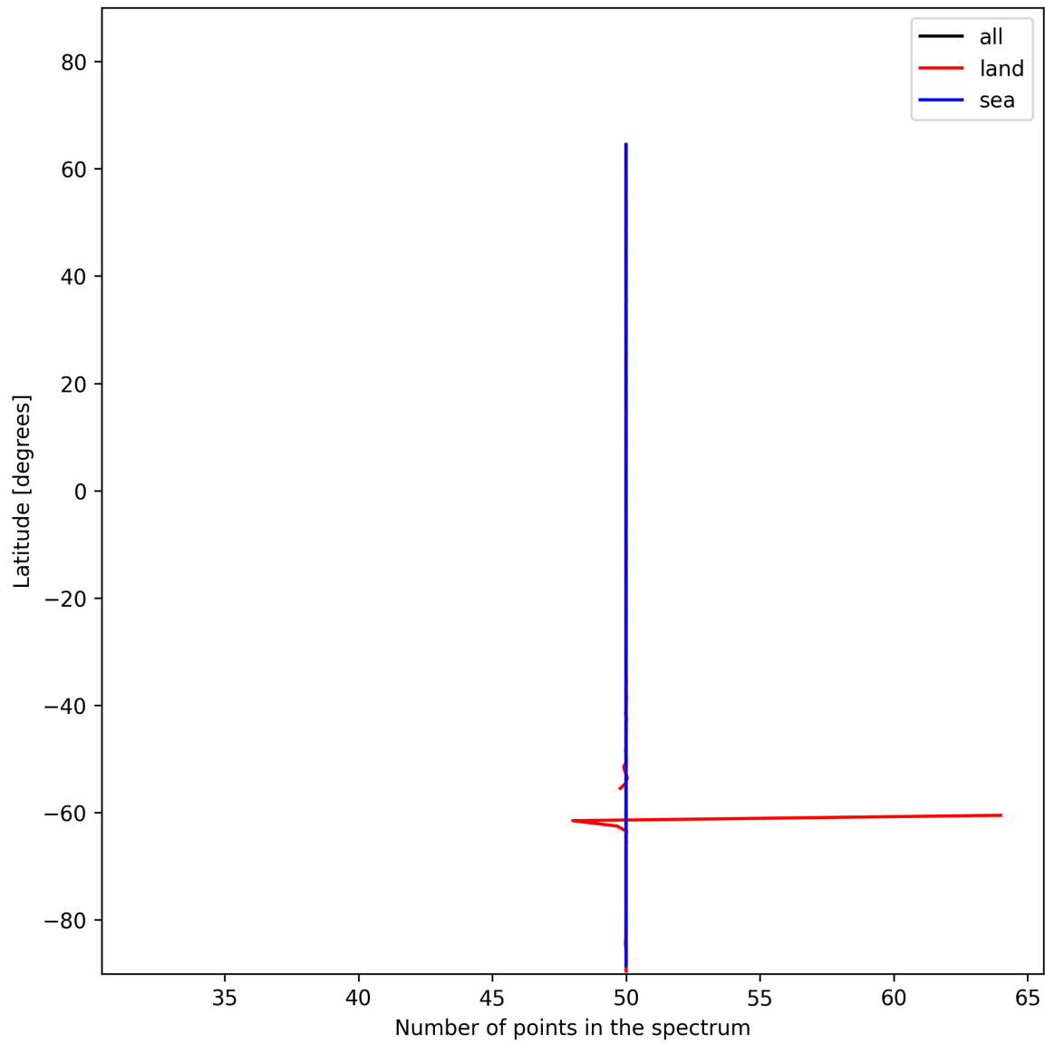
Figure 25: Zonal average of “Number of points in the spectrum” for 2024-12-18 to 2024-12-19.
