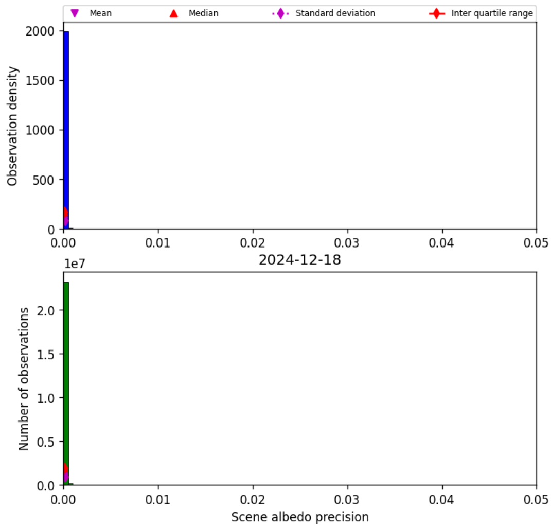
Figure 33: Histogram of “Scene albedo precision” for 2024-12-18 to 2024-12-19
