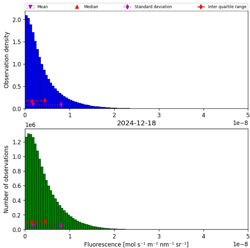
Figure 38: Histogram of “Fluorescence” for 2024-12-18 to 2024-12-19
