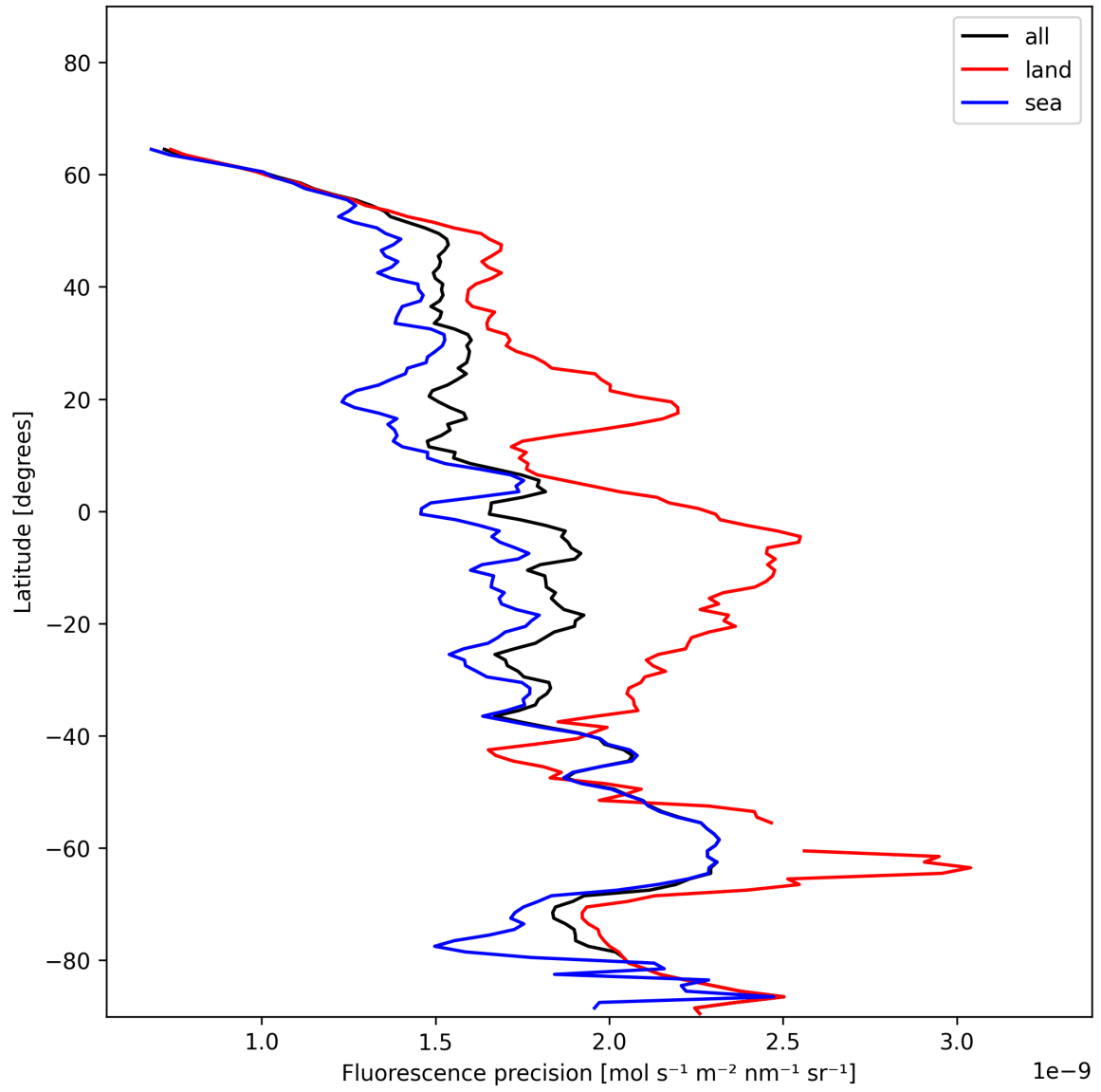
Figure 22: Zonal average of “Fluorescence precision” for 2024-12-18 to 2024-12-19.
