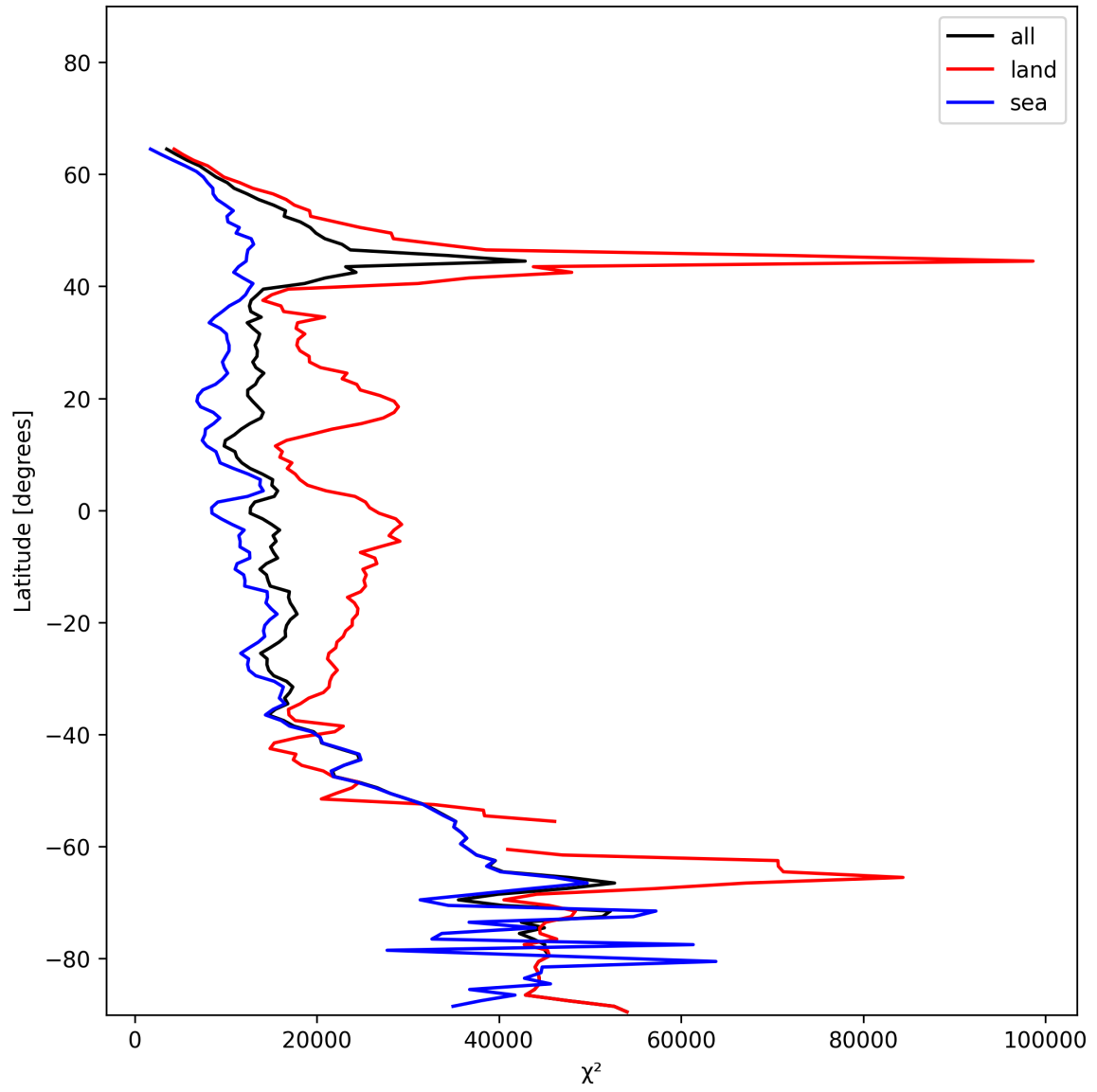
Figure 19: Zonal average of “ \chi^2 ” for 2024-12-18 to 2024-12-19.
