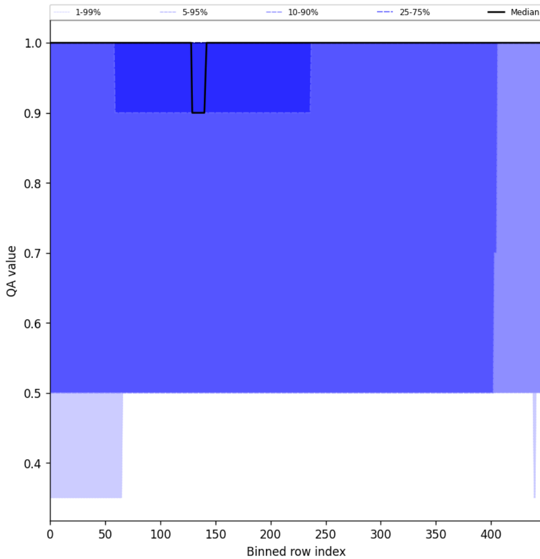
Figure 44: Along track statistics of “QA value” for 2024-12-18 to 2024-12-19
