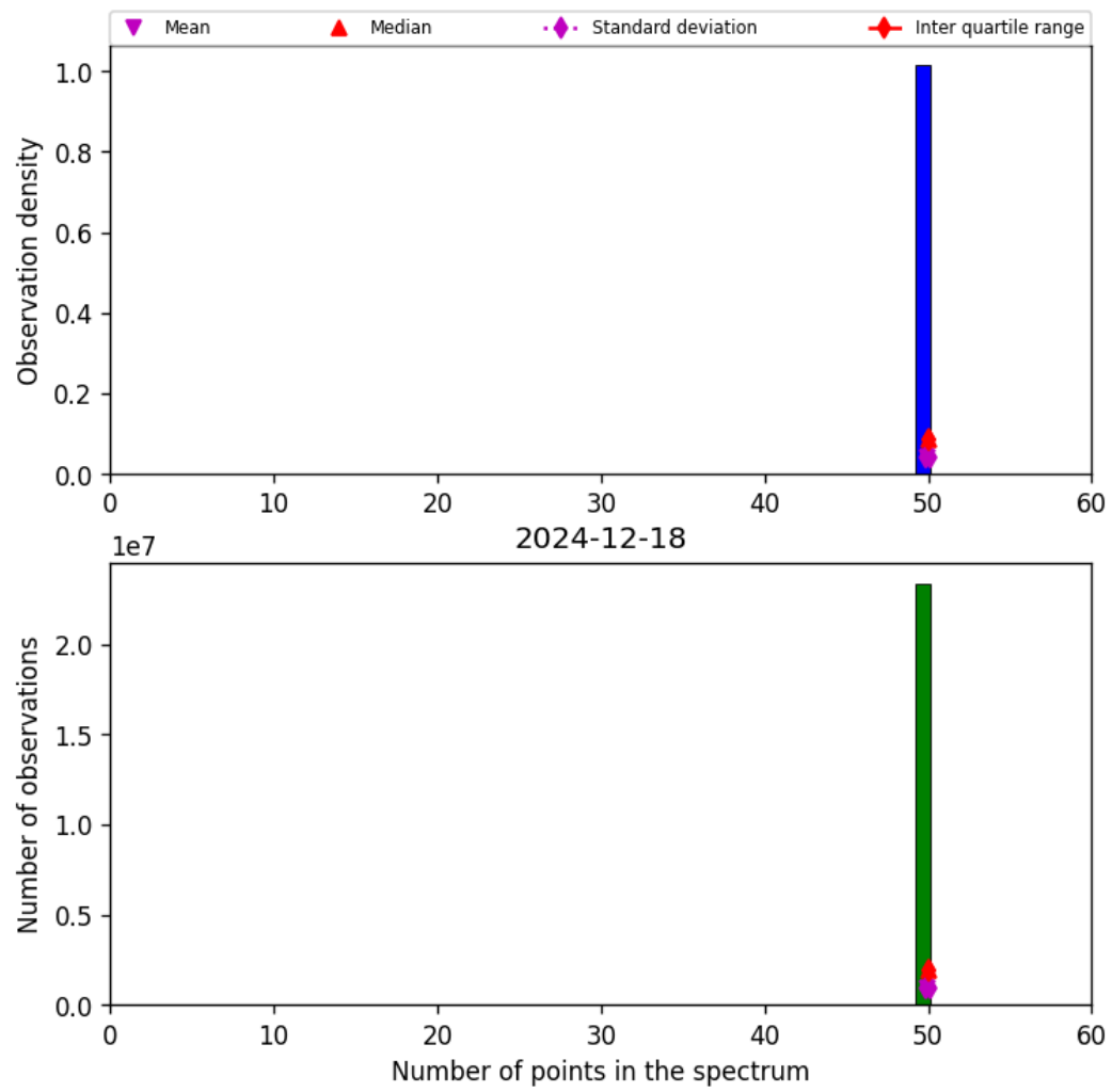
Figure 42: Histogram of “Number of points in the spectrum” for 2024-12-18 to 2024-12-19
