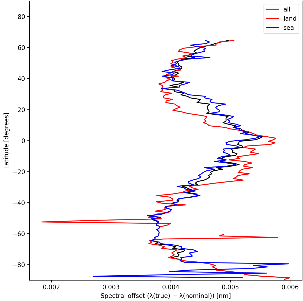
Figure 26: Zonal average of “Spectral offset ( \lambda_{\text{true}} - \lambda_{\text{nominal}} )” for 2024-12-18 to 2024-12-19.
