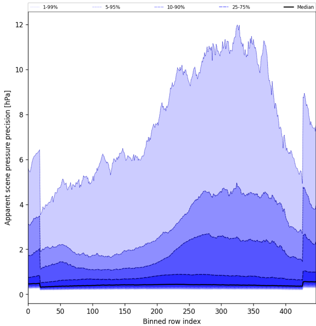
Figure 52: Along track statistics of “Apparent scene pressure precision” for 2024-12-18 to 2024-12-19
