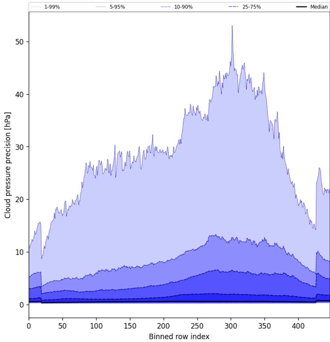
Figure 46: Along track statistics of “Cloud pressure precision” for 2024-12-18 to 2024-12-19
