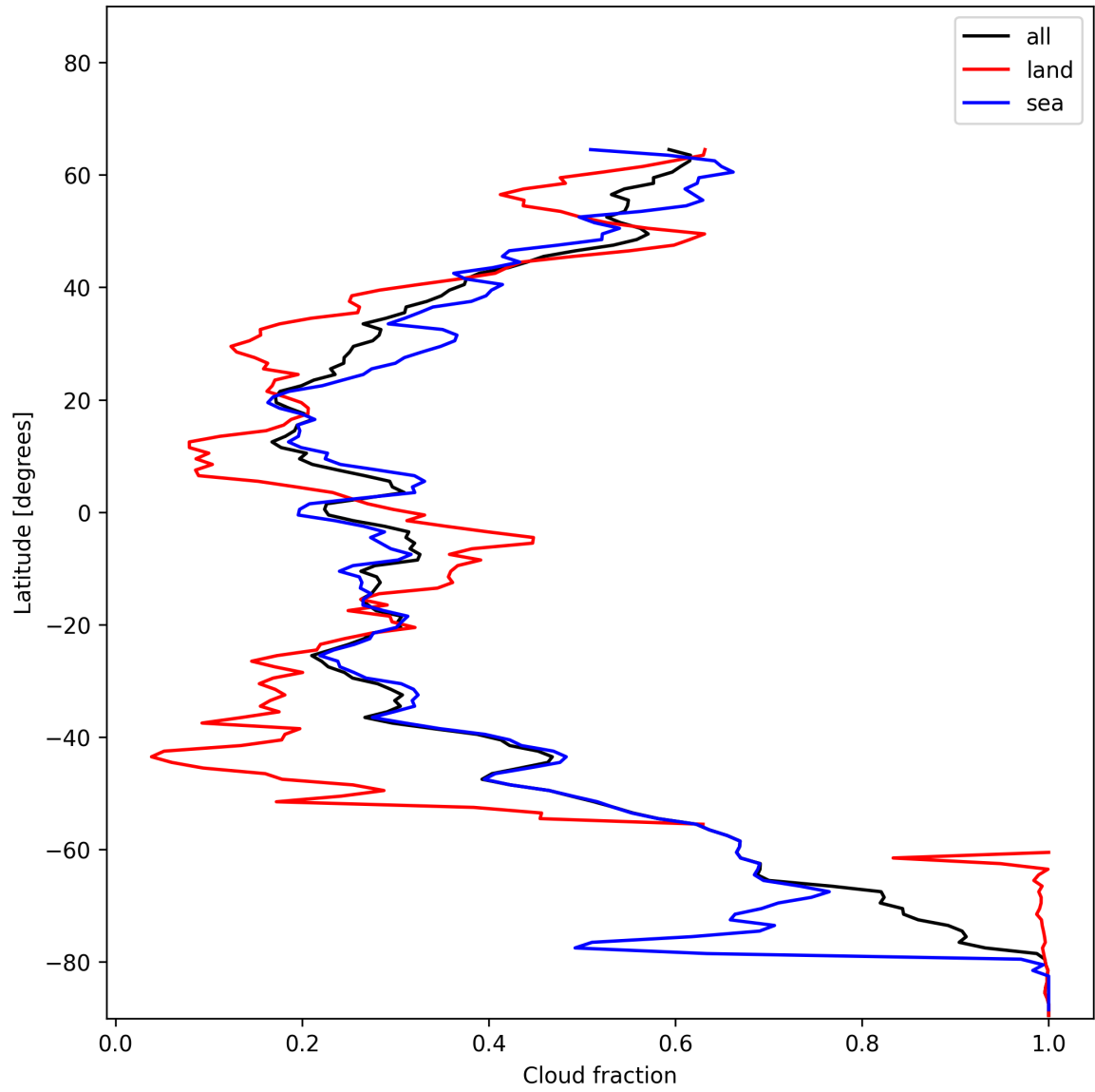
Figure 13: Zonal average of “Cloud fraction” for 2024-12-18 to 2024-12-19.
