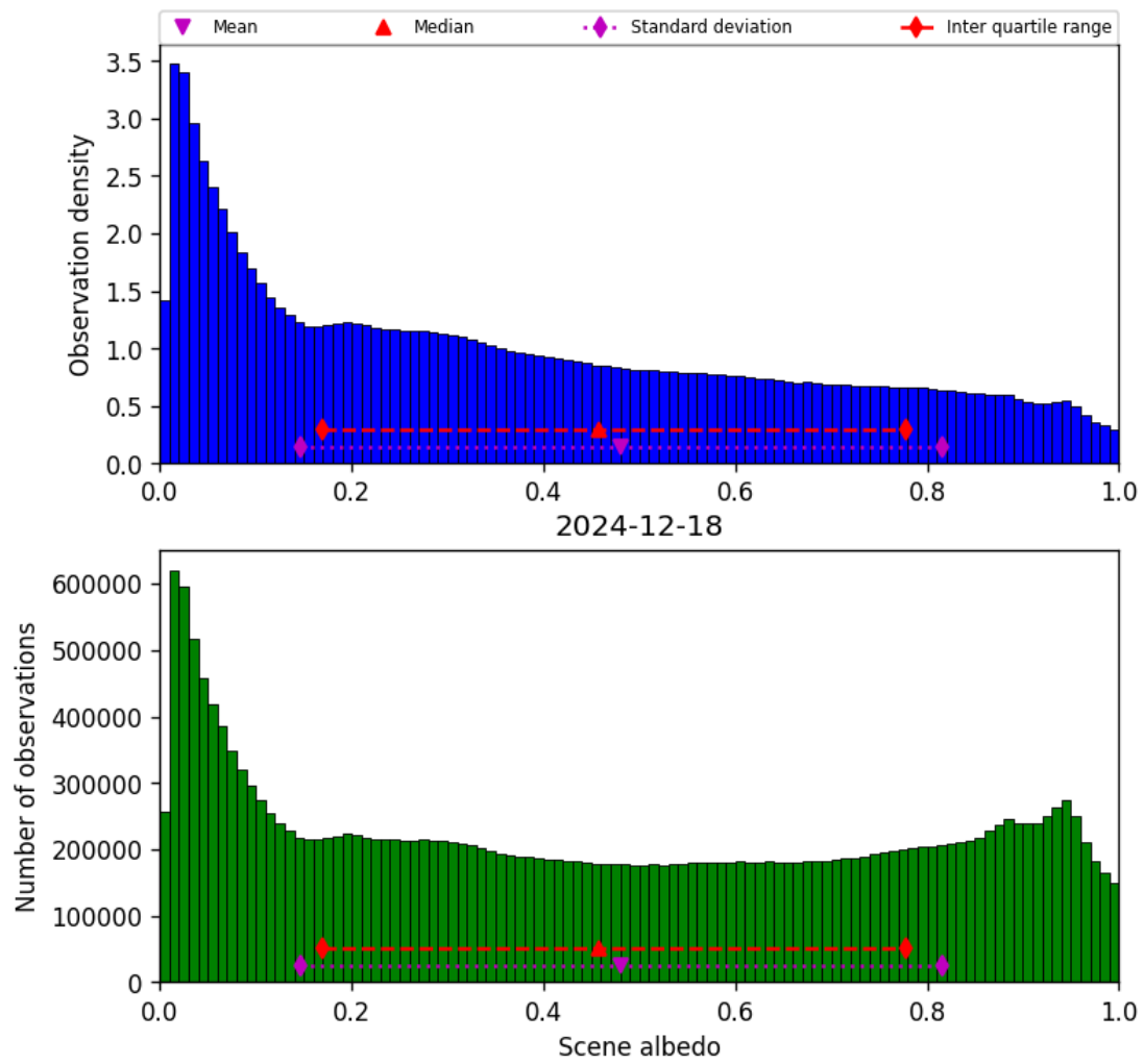
Figure 32: Histogram of “Scene albedo” for 2024-12-18 to 2024-12-19
