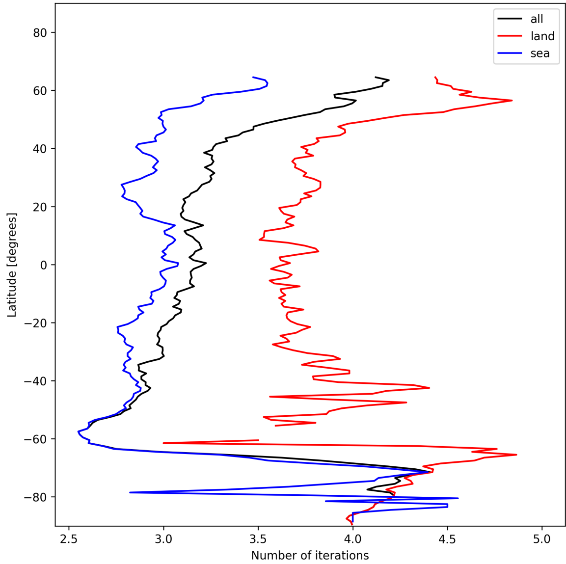
Figure 20: Zonal average of “Number of iterations” for 2024-12-18 to 2024-12-19.
