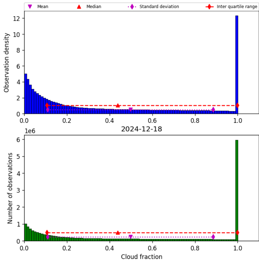
Figure 30: Histogram of “Cloud fraction” for 2024-12-18 to 2024-12-19
