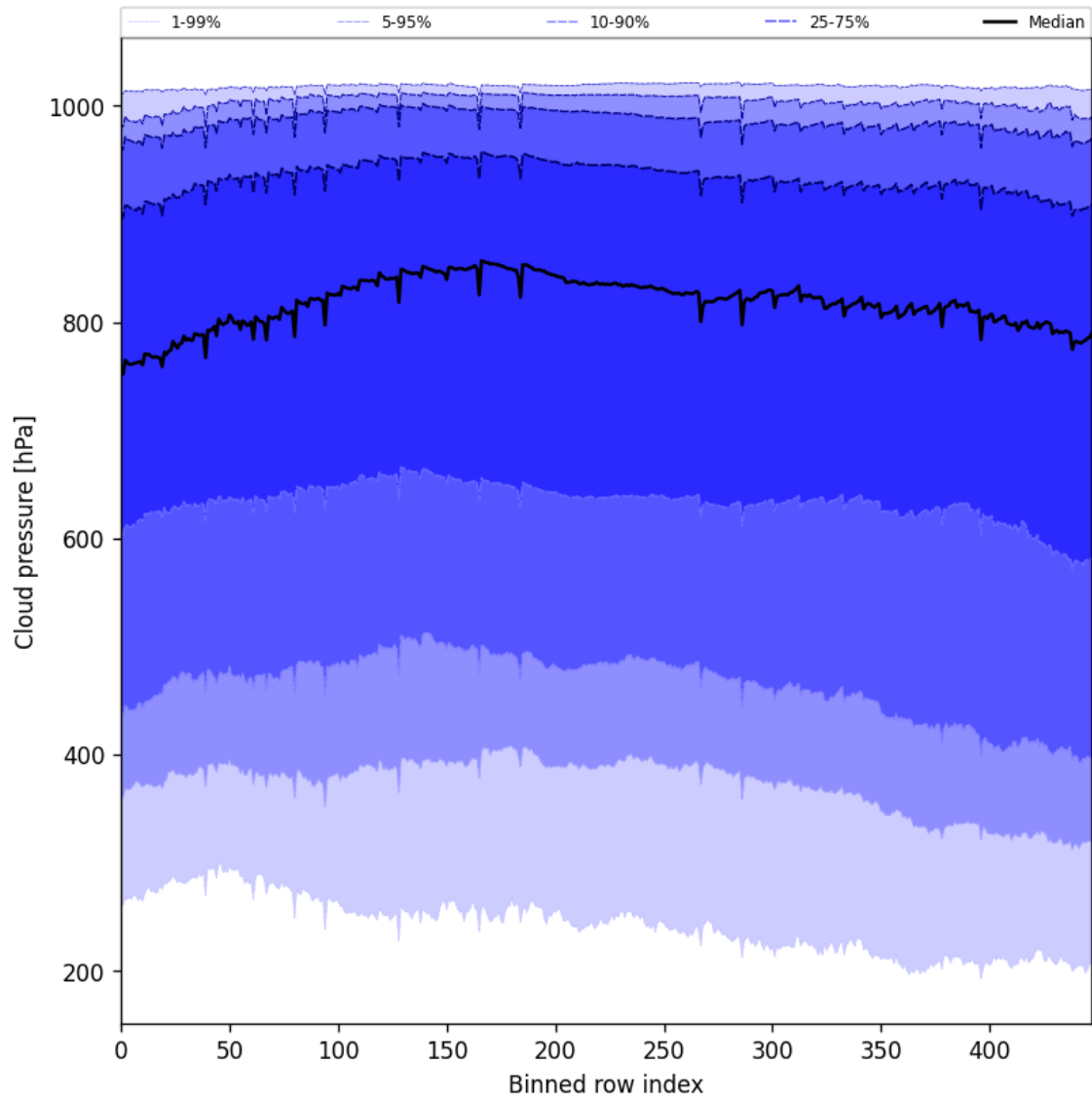
Figure 45: Along track statistics of “Cloud pressure” for 2024-12-18 to 2024-12-19
