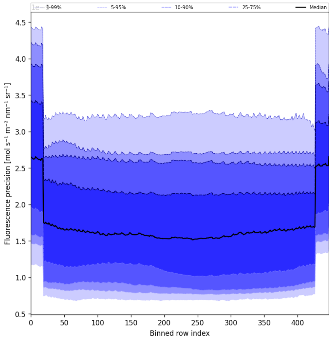
Figure 56: Along track statistics of “Fluorescence precision” for 2024-12-18 to 2024-12-19
