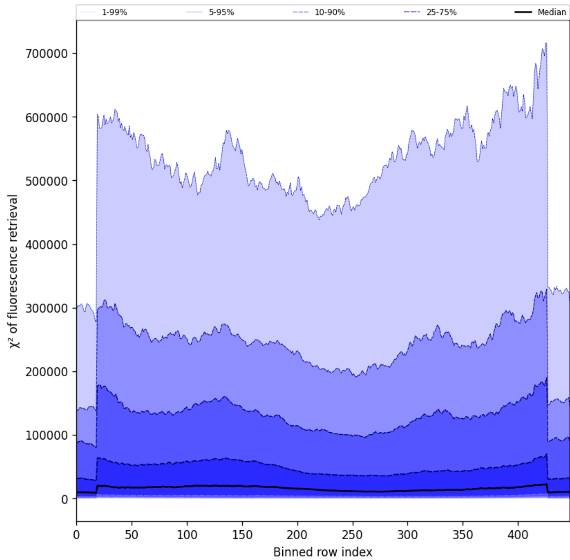
Figure 57: Along track statistics of “ \chi^2 of fluorescence retrieval” for 2024-12-18 to 2024-12-19
