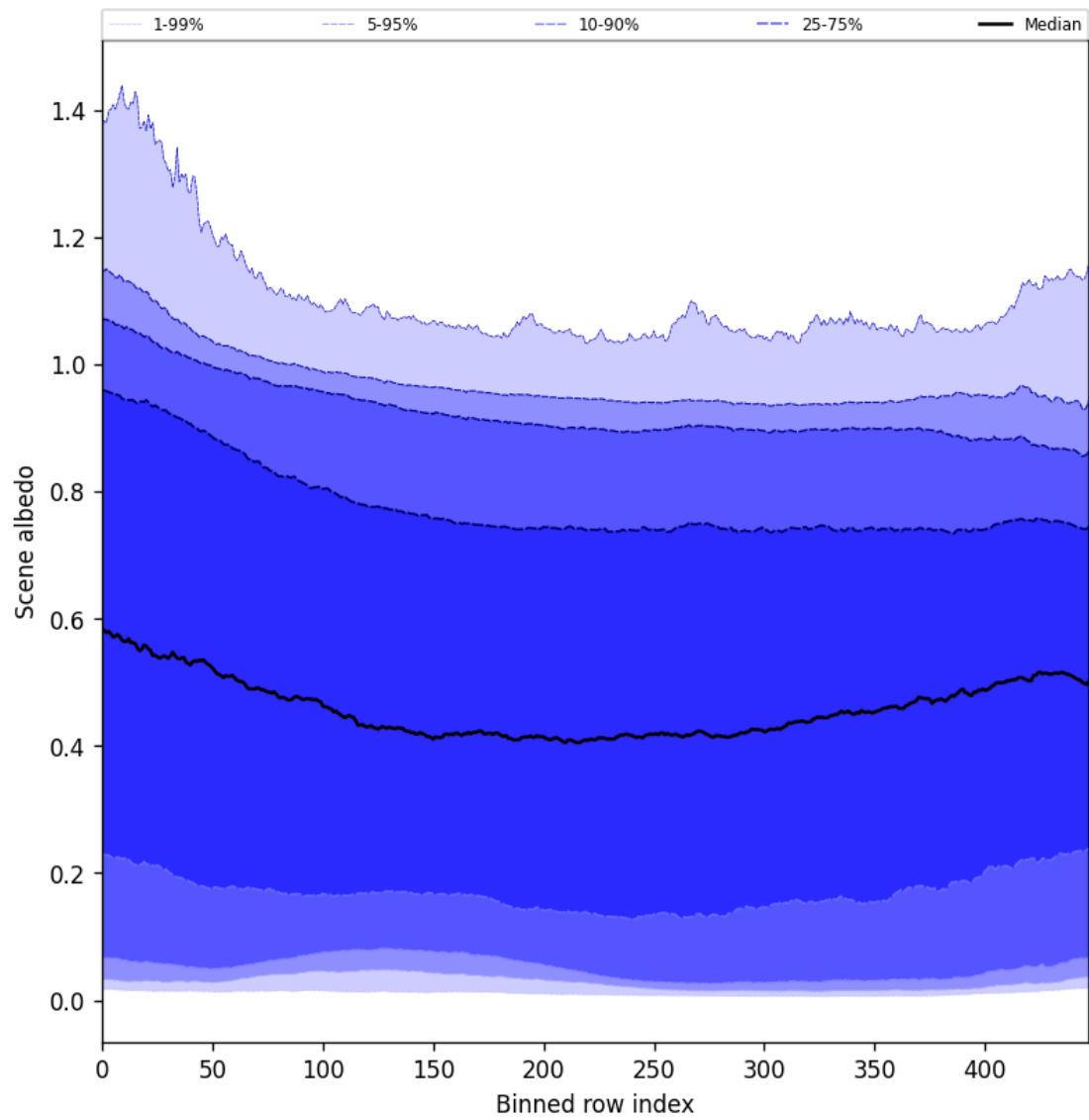
Figure 49: Along track statistics of “Scene albedo” for 2024-12-18 to 2024-12-19
