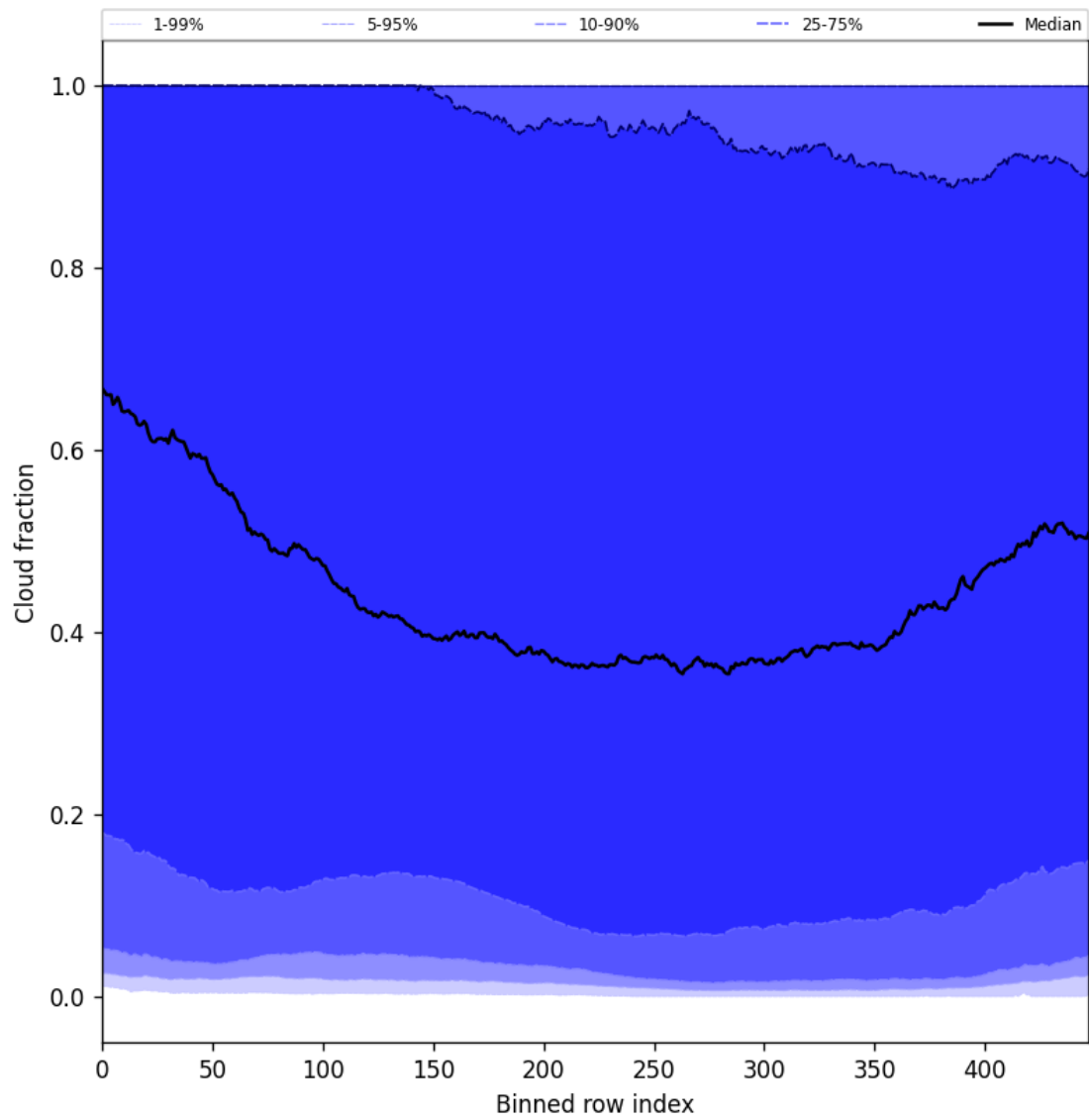
Figure 47: Along track statistics of “Cloud fraction” for 2024-12-18 to 2024-12-19
