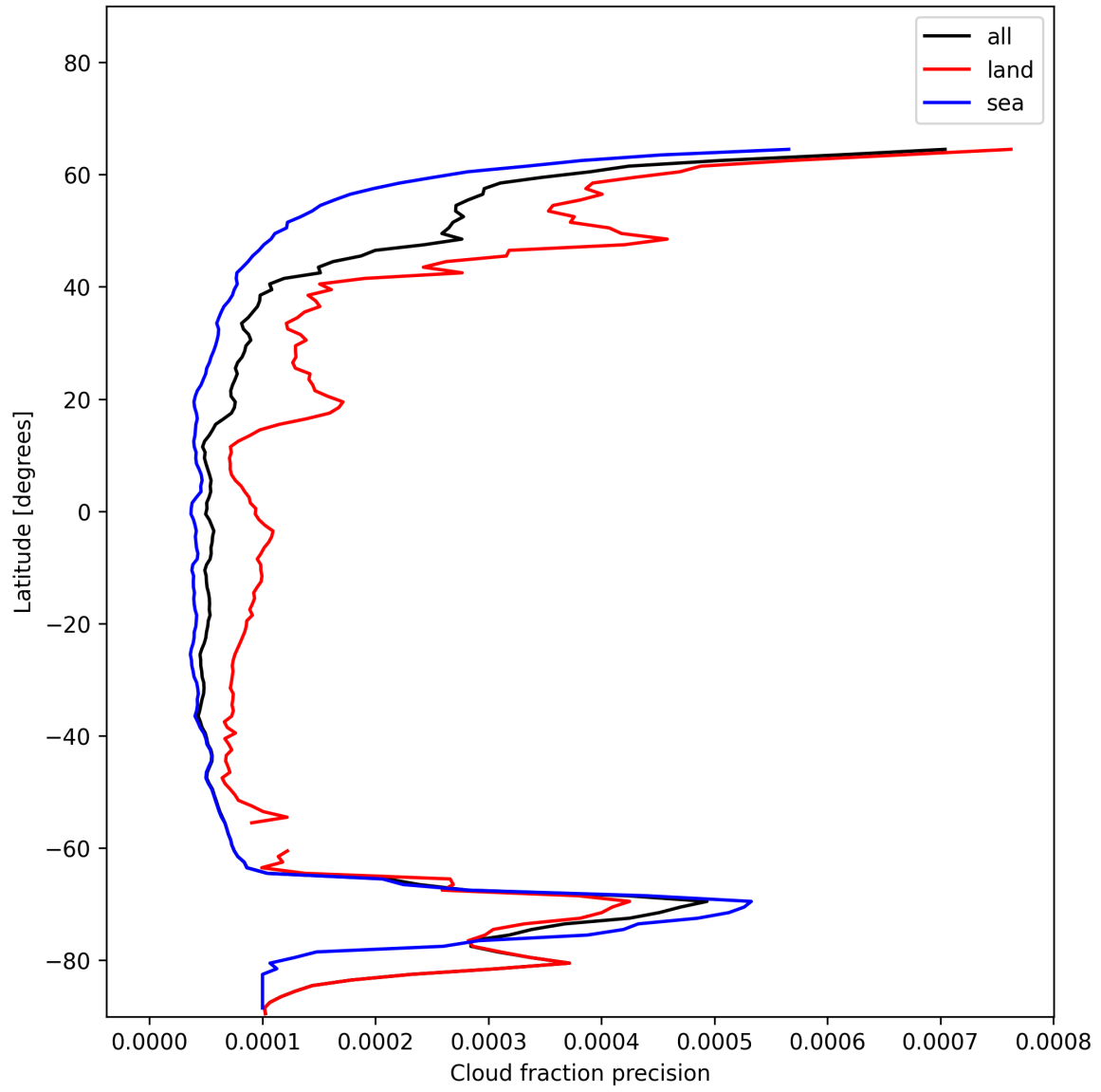
Figure 14: Zonal average of “Cloud fraction precision” for 2024-12-18 to 2024-12-19.
