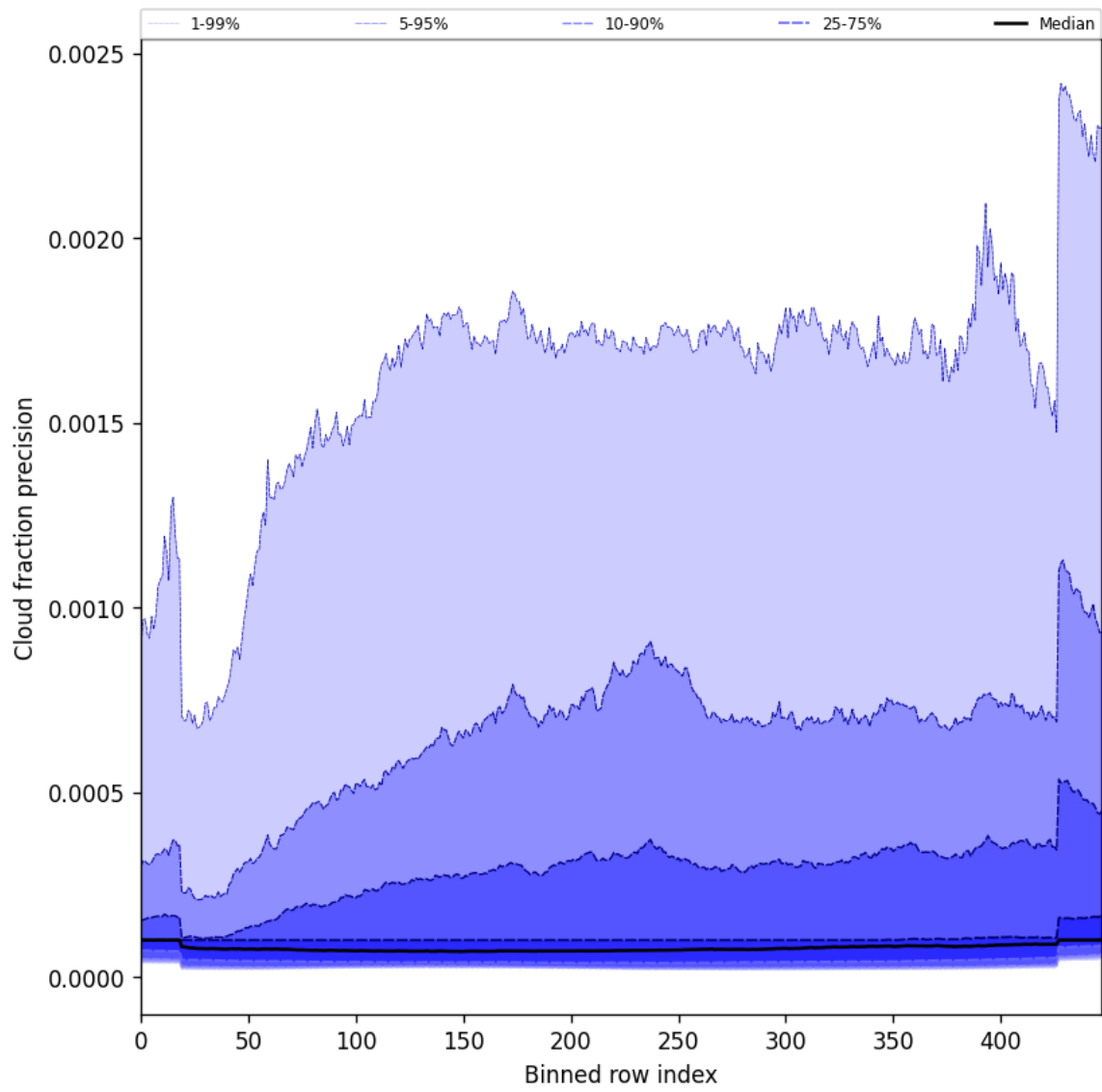
Figure 48: Along track statistics of “Cloud fraction precision” for 2024-12-18 to 2024-12-19
