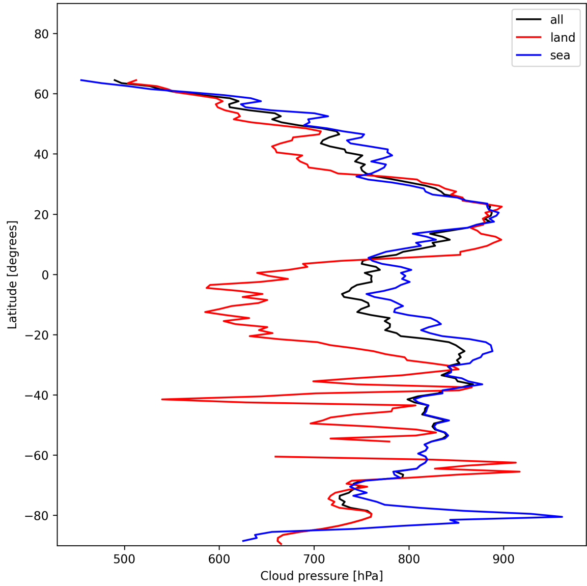
Figure 11: Zonal average of “Cloud pressure” for 2024-12-18 to 2024-12-19.
