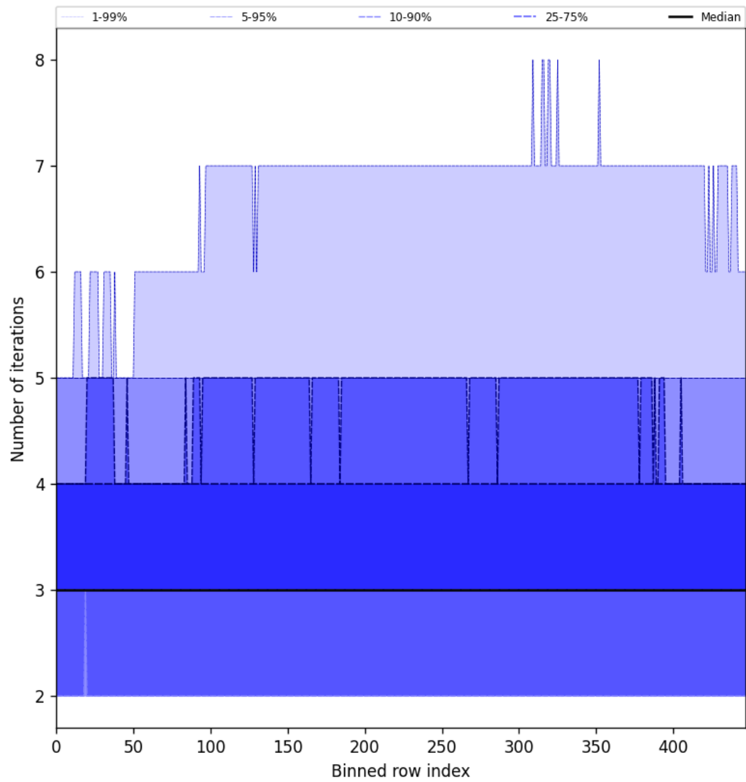
Figure 54: Along track statistics of “Number of iterations” for 2024-12-18 to 2024-12-19
