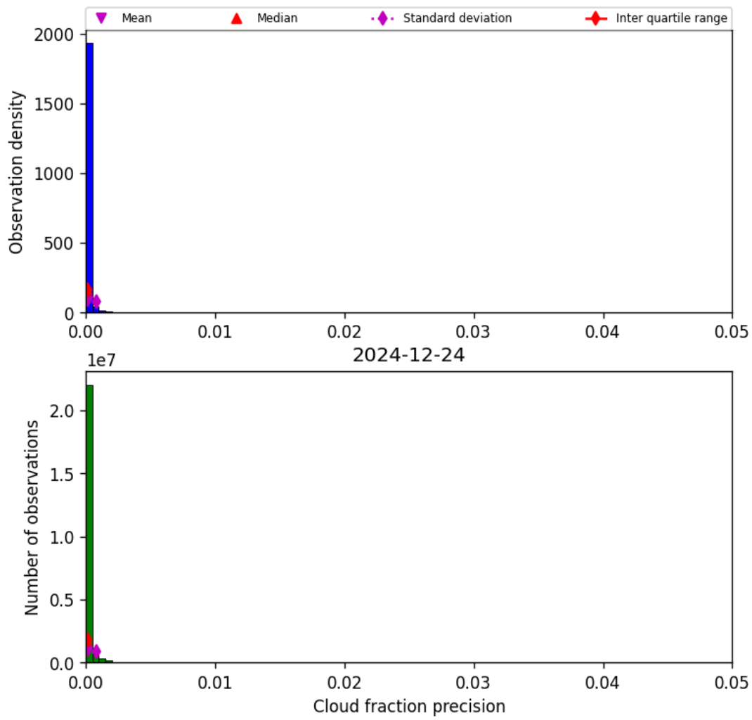
Figure 31: Histogram of “Cloud fraction precision” for 2024-12-24 to 2024-12-25
