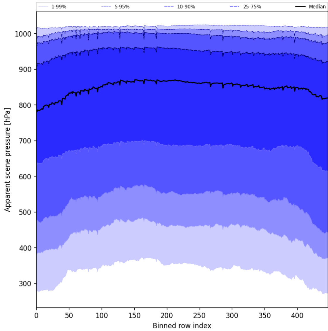
Figure 51: Along track statistics of “Apparent scene pressure” for 2024-12-24 to 2024-12-25
