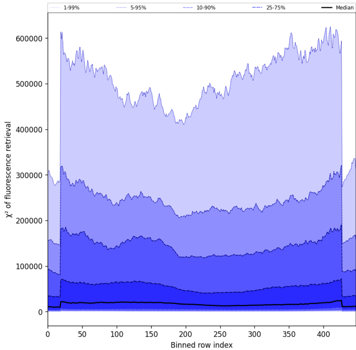
Figure 57: Along track statistics of “ \chi^2 of fluorescence retrieval” for 2024-12-24 to 2024-12-25
