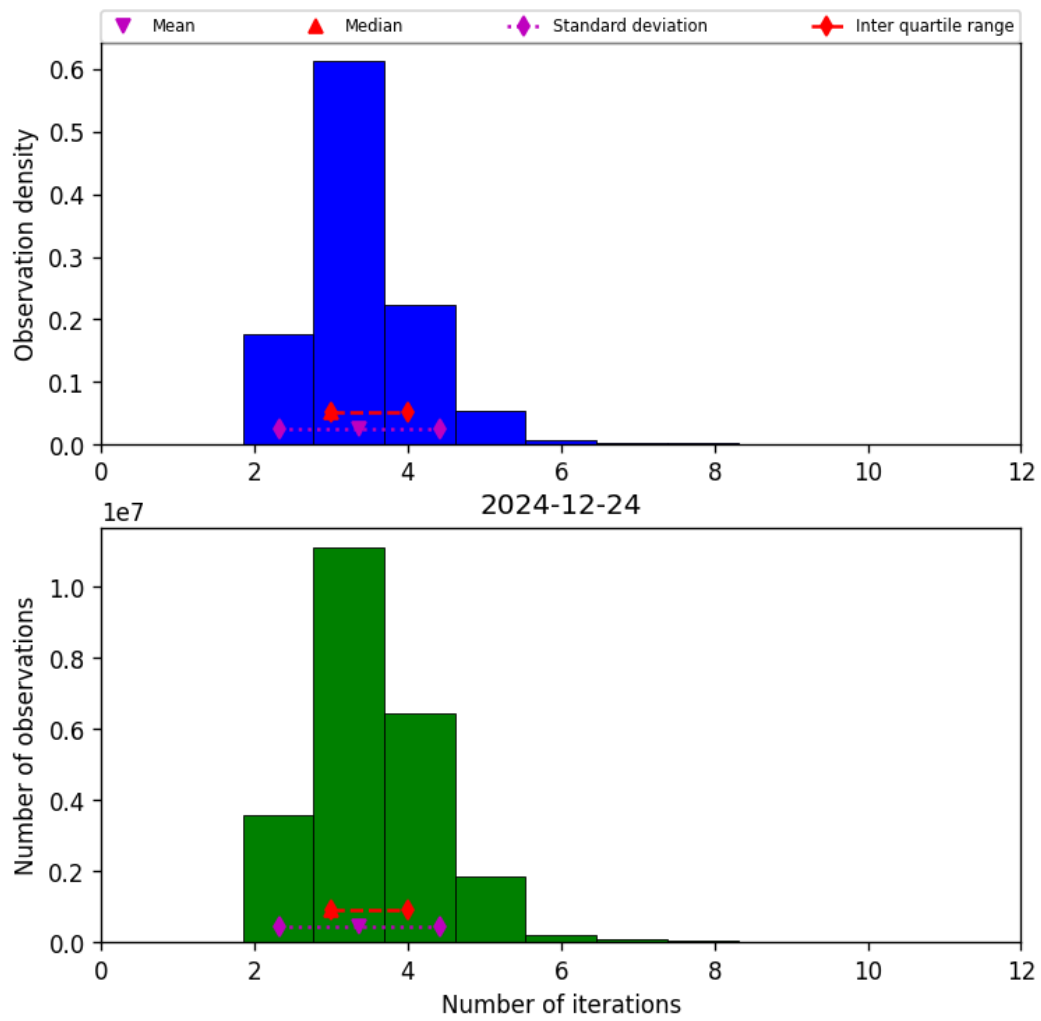
Figure 37: Histogram of “Number of iterations” for 2024-12-24 to 2024-12-25
