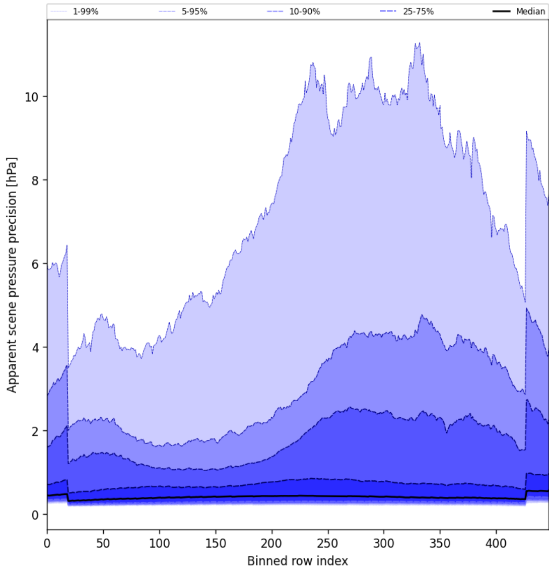
Figure 52: Along track statistics of “Apparent scene pressure precision” for 2024-12-24 to 2024-12-25
