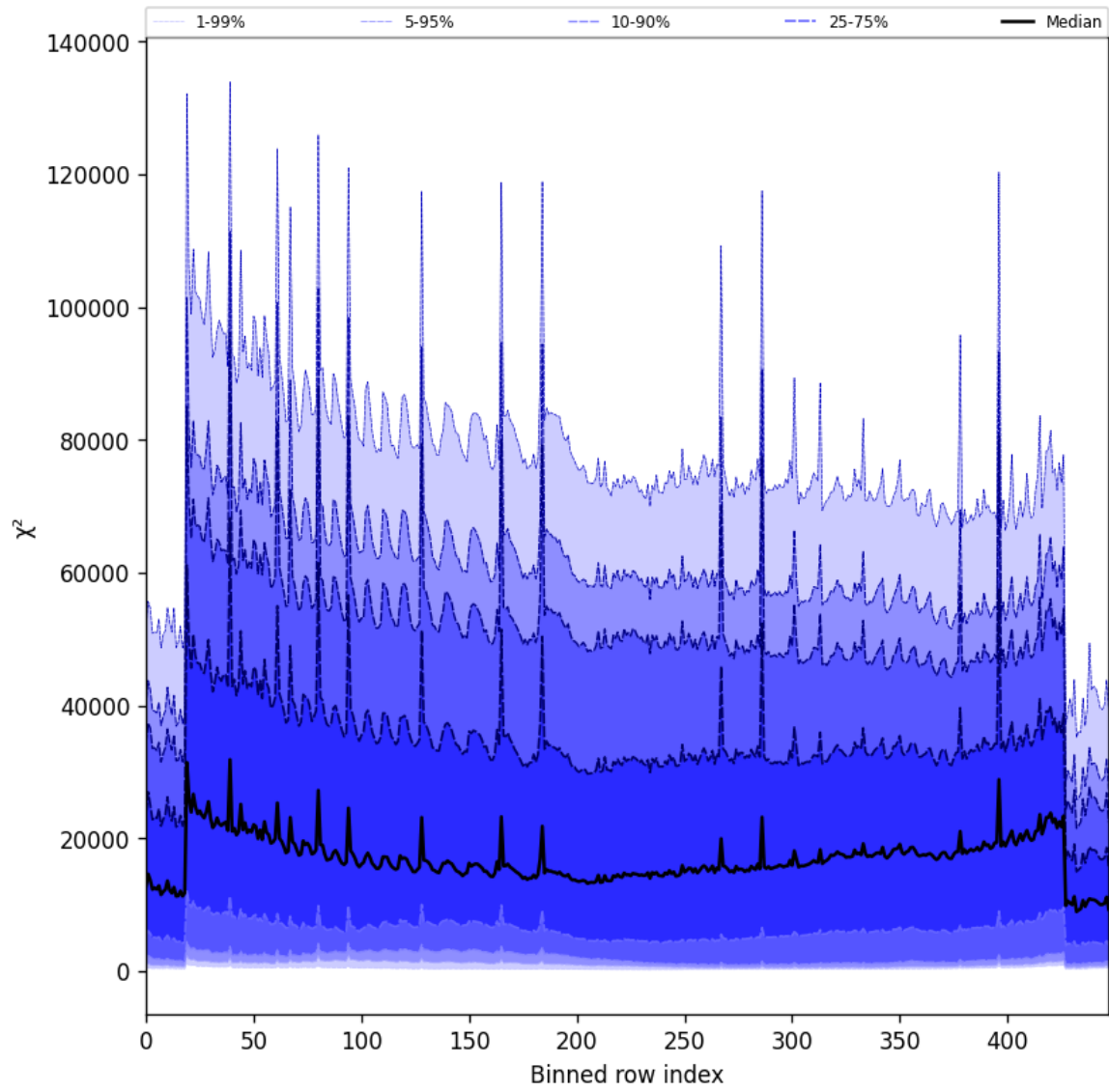
Figure 53: Along track statistics of “ \chi^2 ” for 2024-12-24 to 2024-12-25
