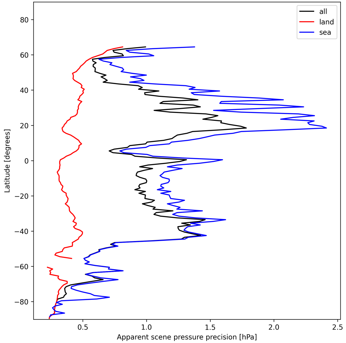
Figure 18: Zonal average of “Apparent scene pressure precision” for 2024-12-24 to 2024-12-25.
