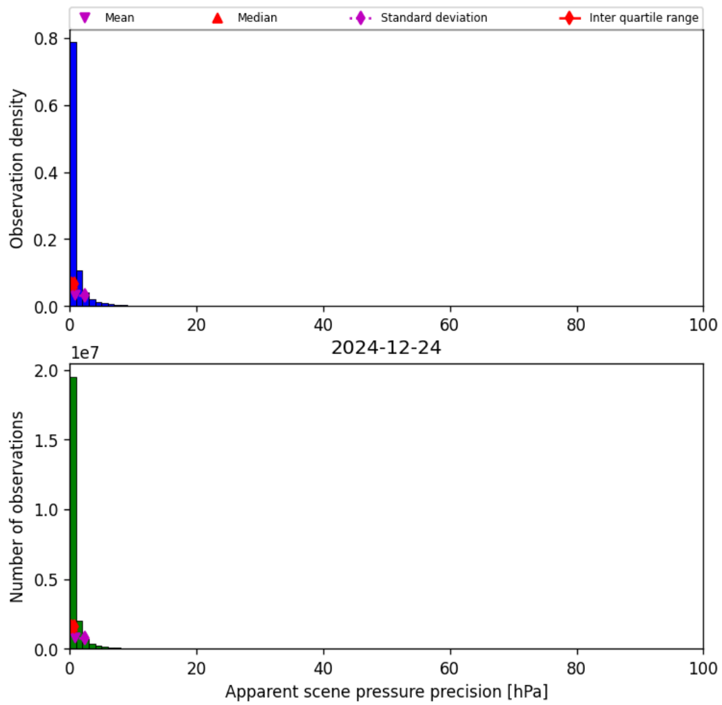
Figure 35: Histogram of “Apparent scene pressure precision” for 2024-12-24 to 2024-12-25
