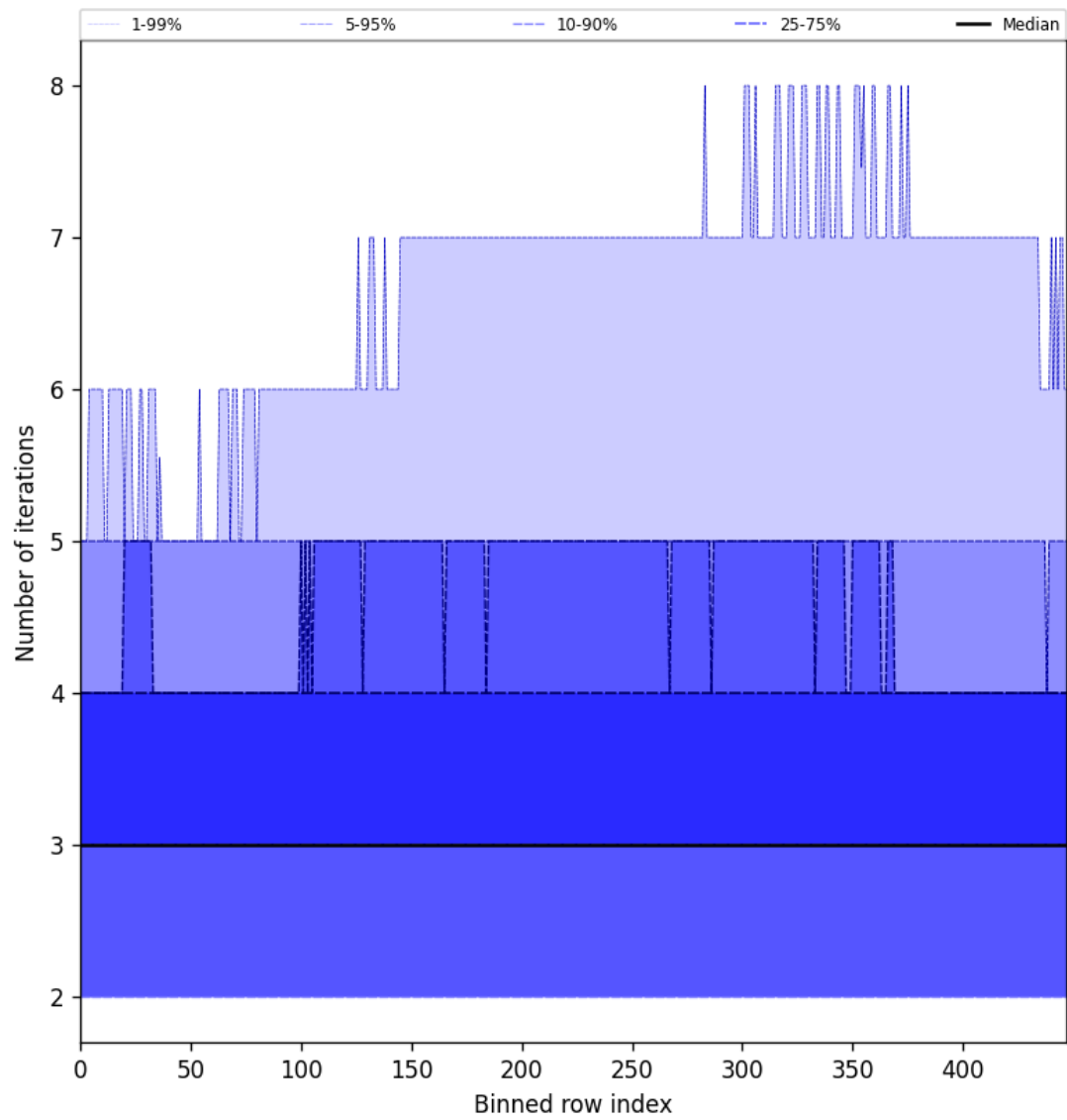
Figure 54: Along track statistics of “Number of iterations” for 2024-12-24 to 2024-12-25
