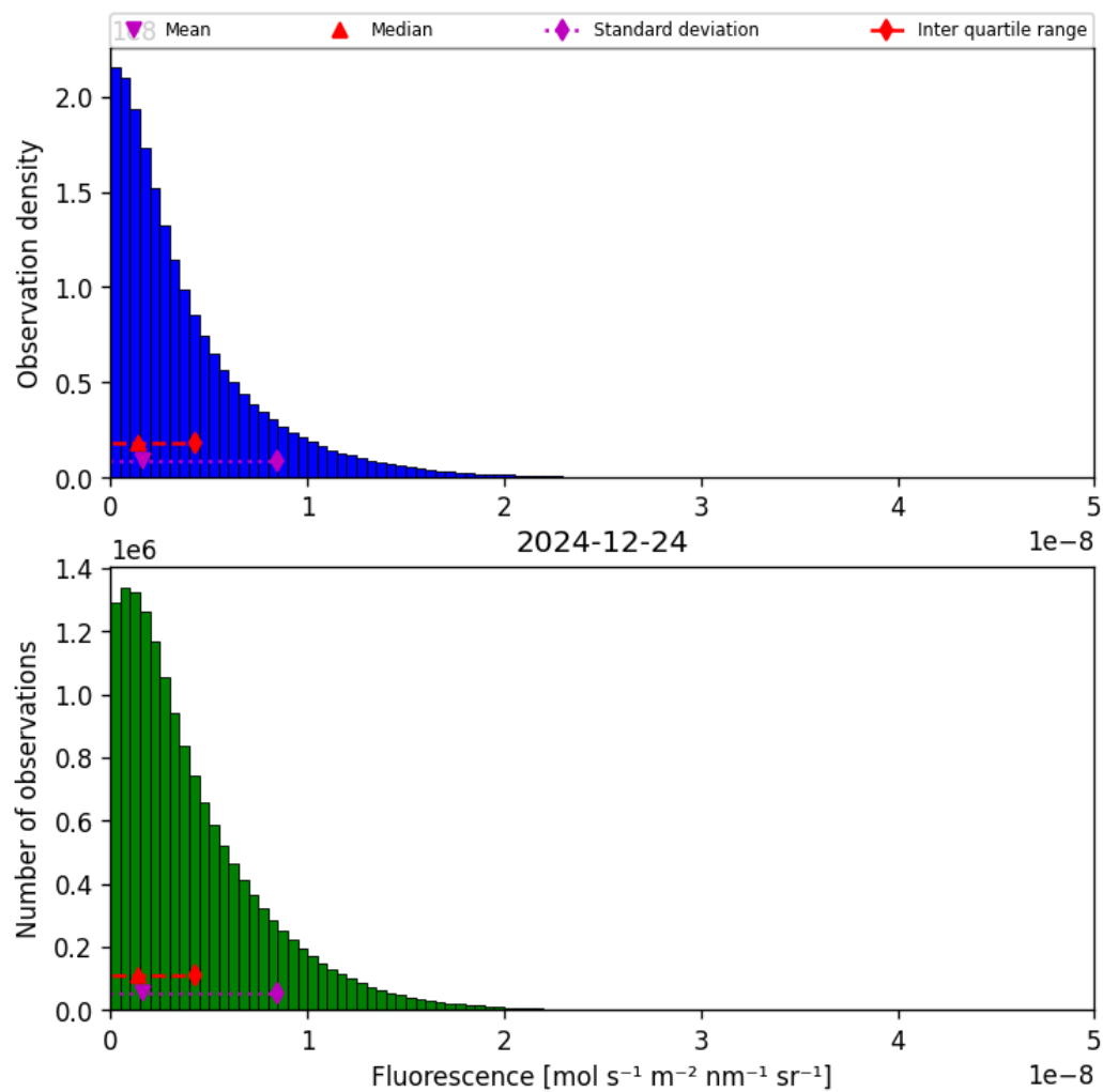
Figure 38: Histogram of “Fluorescence” for 2024-12-24 to 2024-12-25
