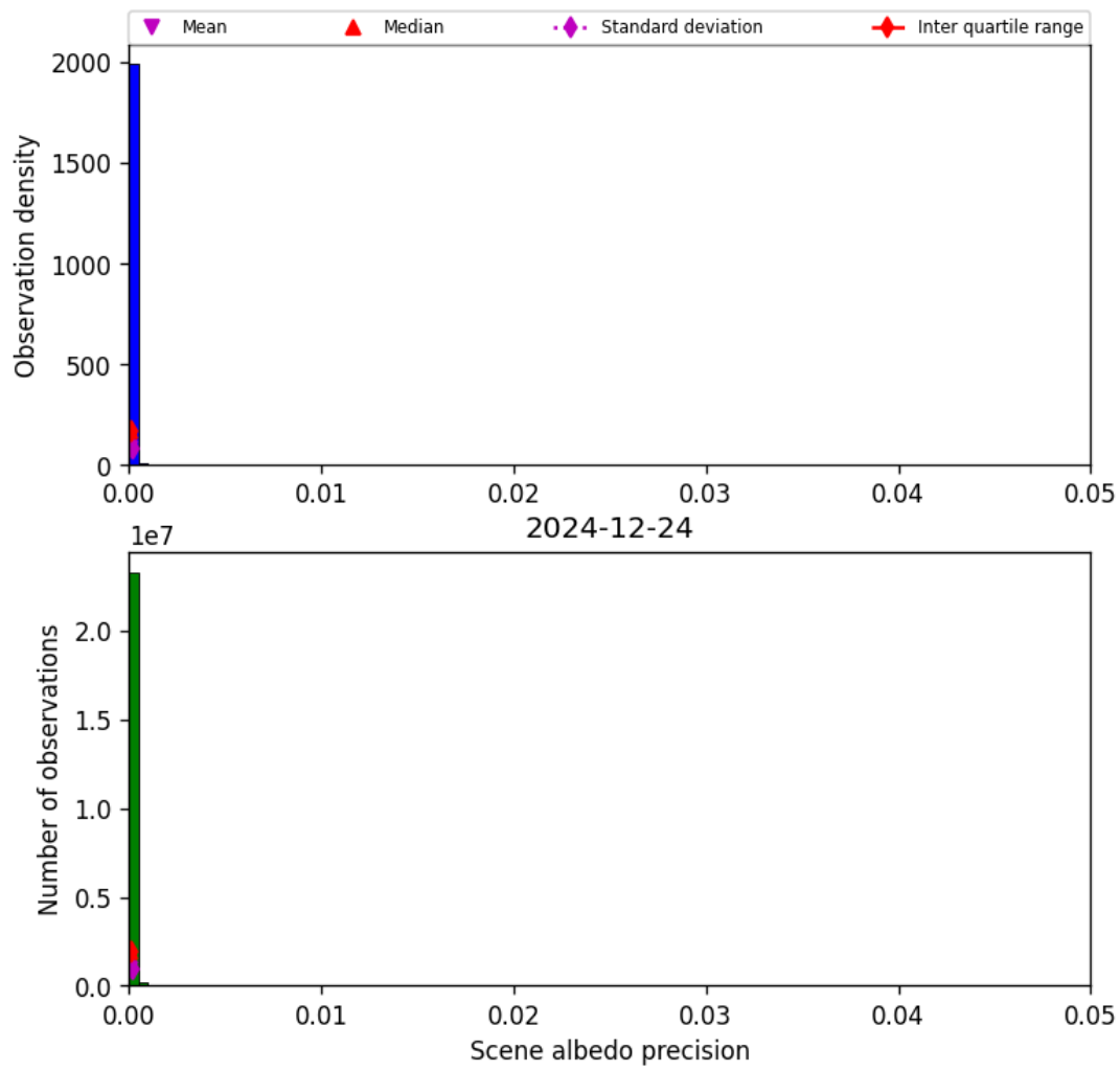
Figure 33: Histogram of “Scene albedo precision” for 2024-12-24 to 2024-12-25
