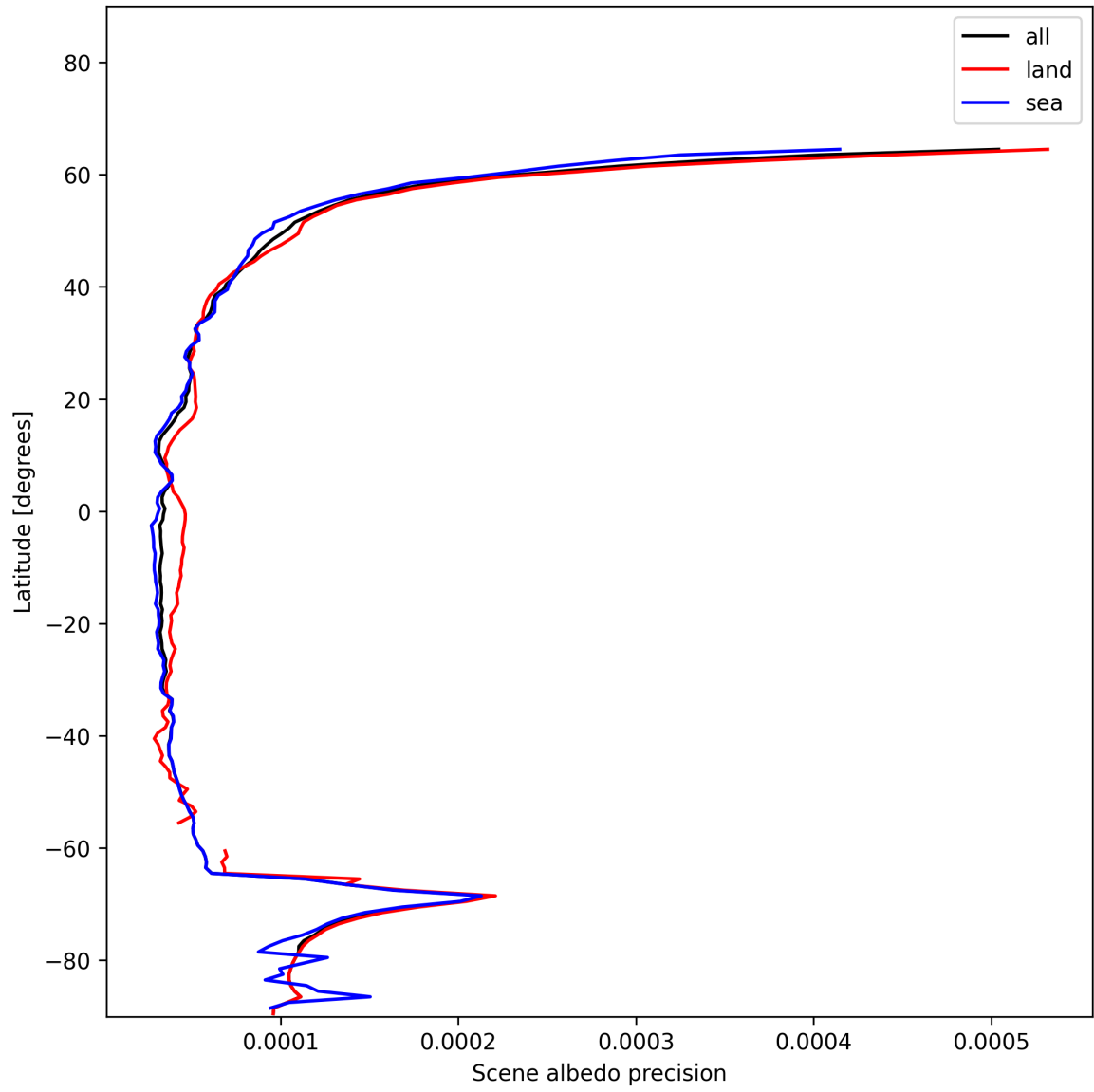
Figure 16: Zonal average of “Scene albedo precision” for 2024-12-24 to 2024-12-25.
