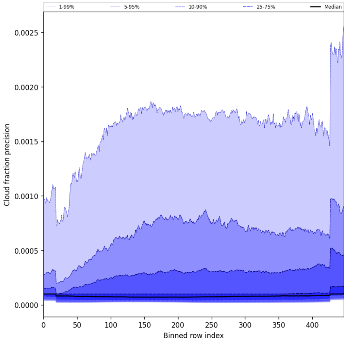
Figure 48: Along track statistics of “Cloud fraction precision” for 2024-12-24 to 2024-12-25
