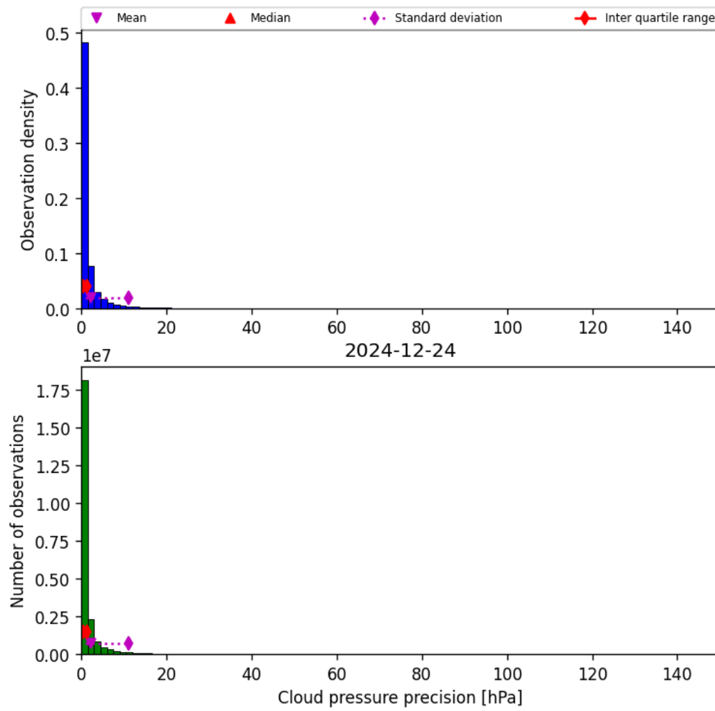
Figure 29: Histogram of “Cloud pressure precision” for 2024-12-24 to 2024-12-25
