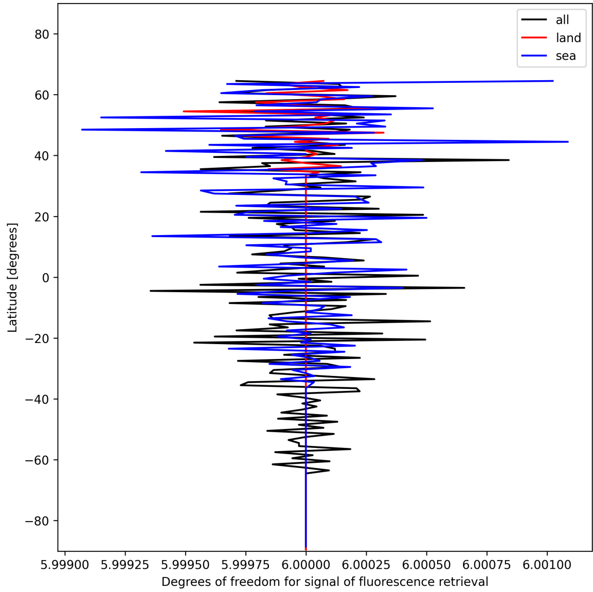
Figure 24: Zonal average of “Degrees of freedom for signal of fluorescence retrieval” for 2024-12-24 to 2024-12-25.
