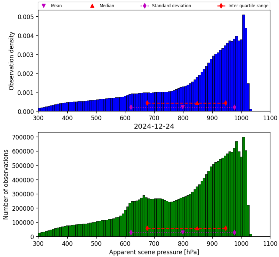
Figure 34: Histogram of “Apparent scene pressure” for 2024-12-24 to 2024-12-25
