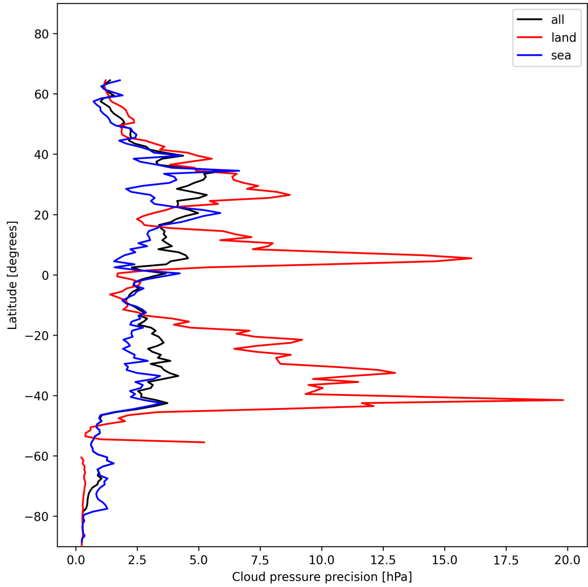
Figure 12: Zonal average of “Cloud pressure precision” for 2024-12-24 to 2024-12-25.
