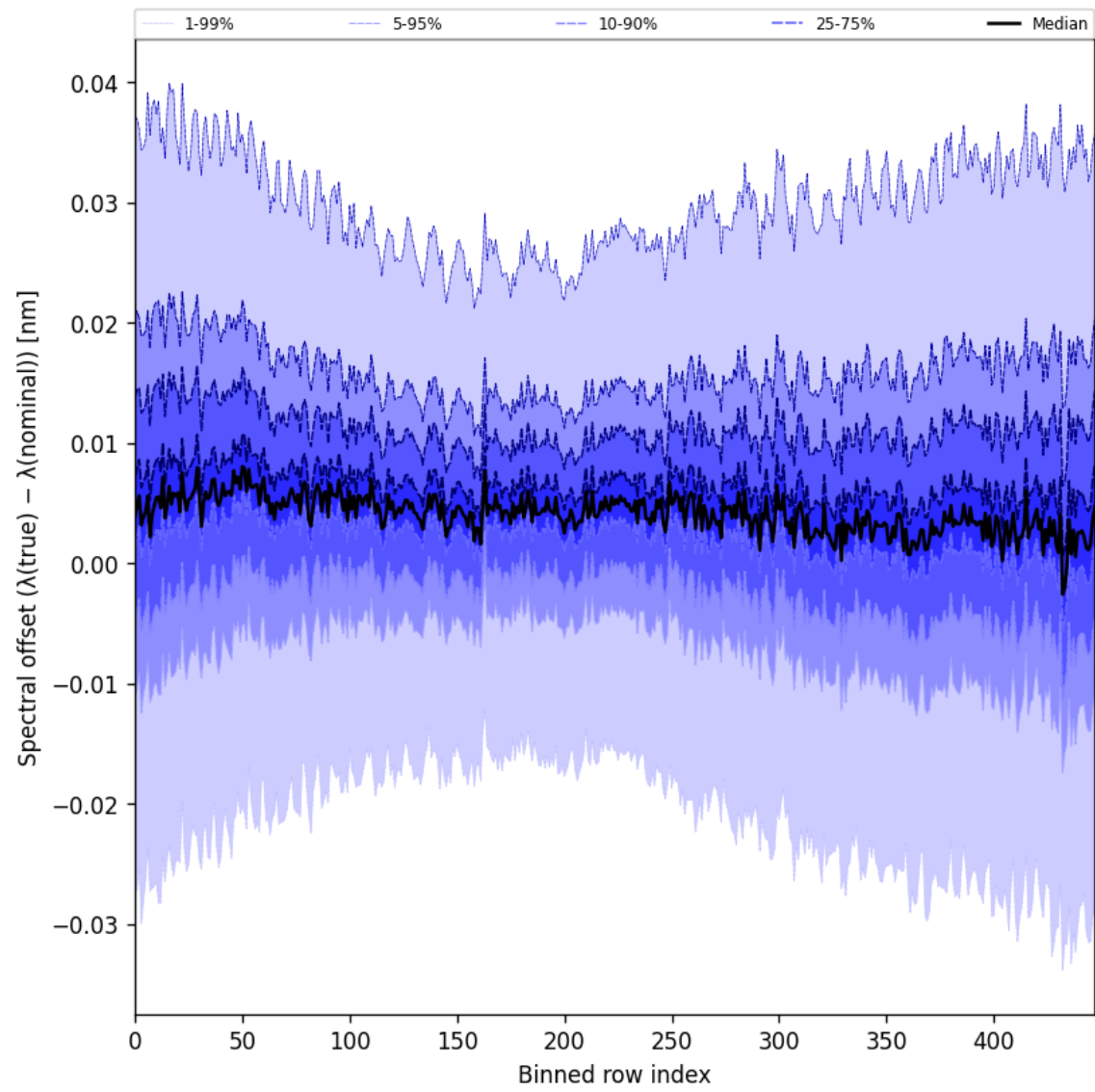
Figure 60: Along track statistics of “Spectral offset ( \lambda_{\text{true}} - \lambda_{\text{nominal}} )” for 2024-12-24 to 2024-12-25
