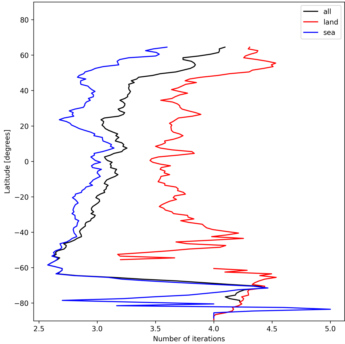
Figure 20: Zonal average of “Number of iterations” for 2024-12-24 to 2024-12-25.
