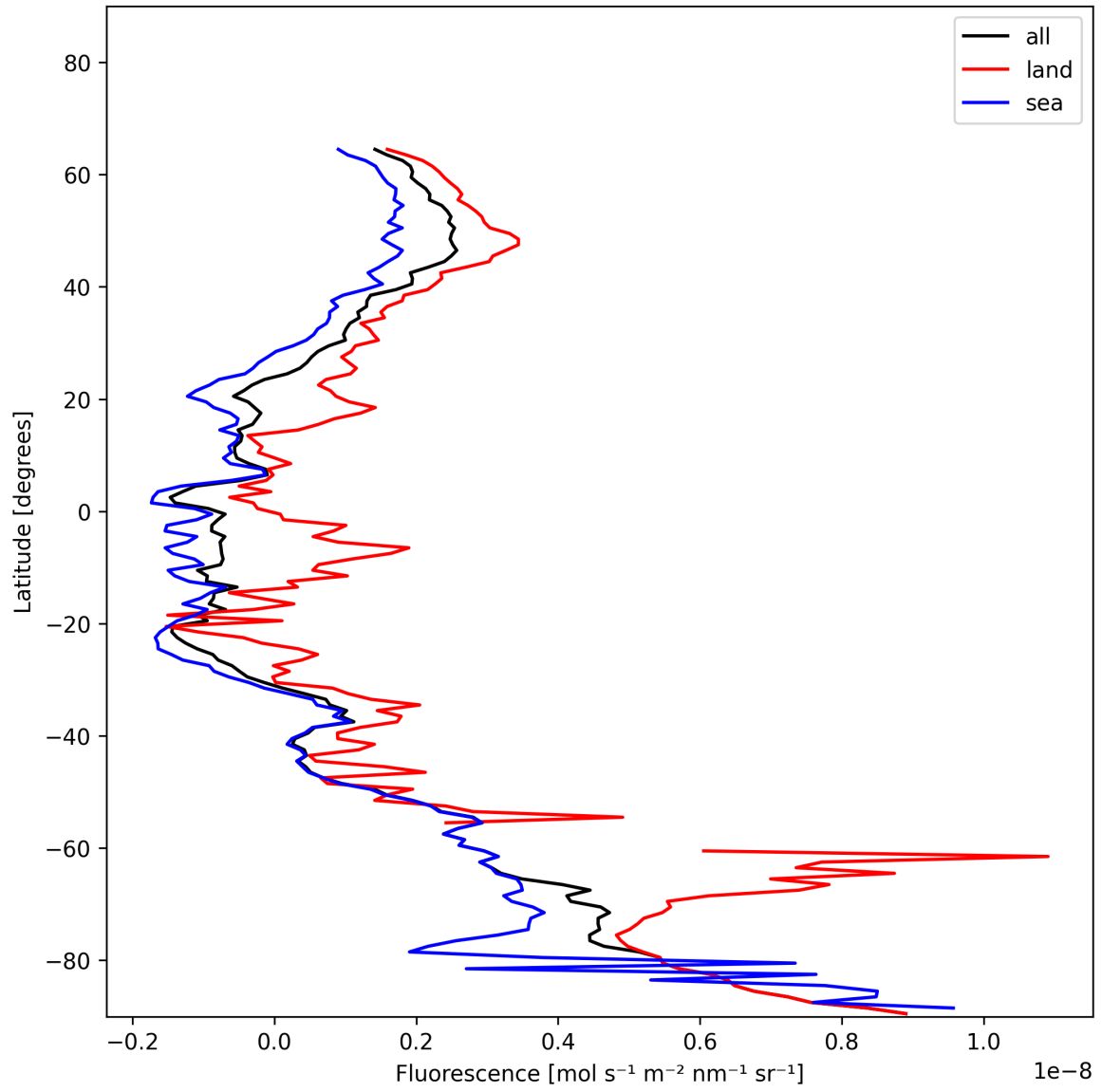
Figure 21: Zonal average of “Fluorescence” for 2024-12-24 to 2024-12-25.
