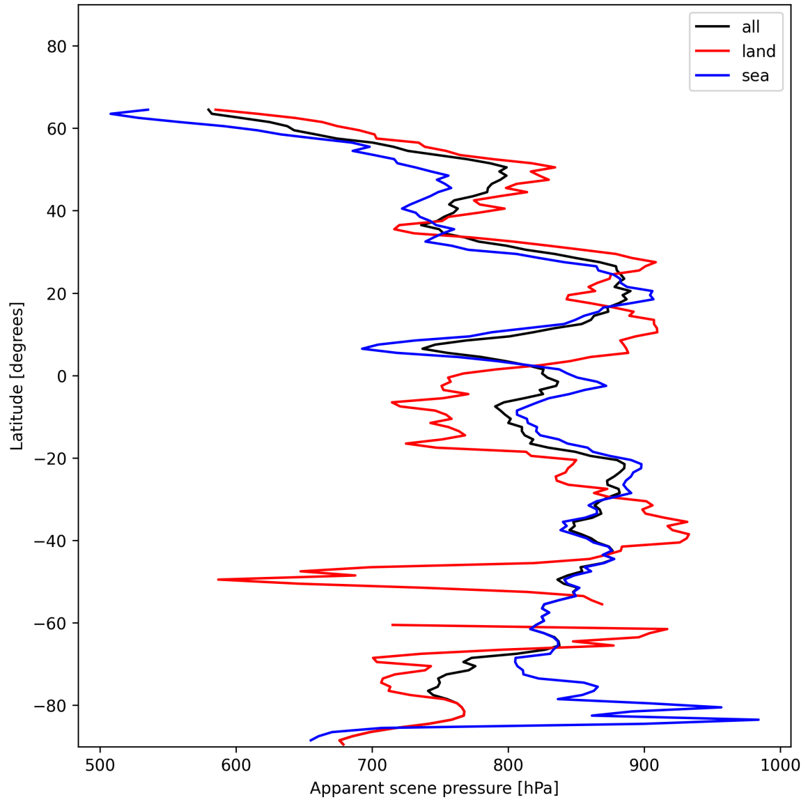
Figure 17: Zonal average of “Apparent scene pressure” for 2024-12-24 to 2024-12-25.
