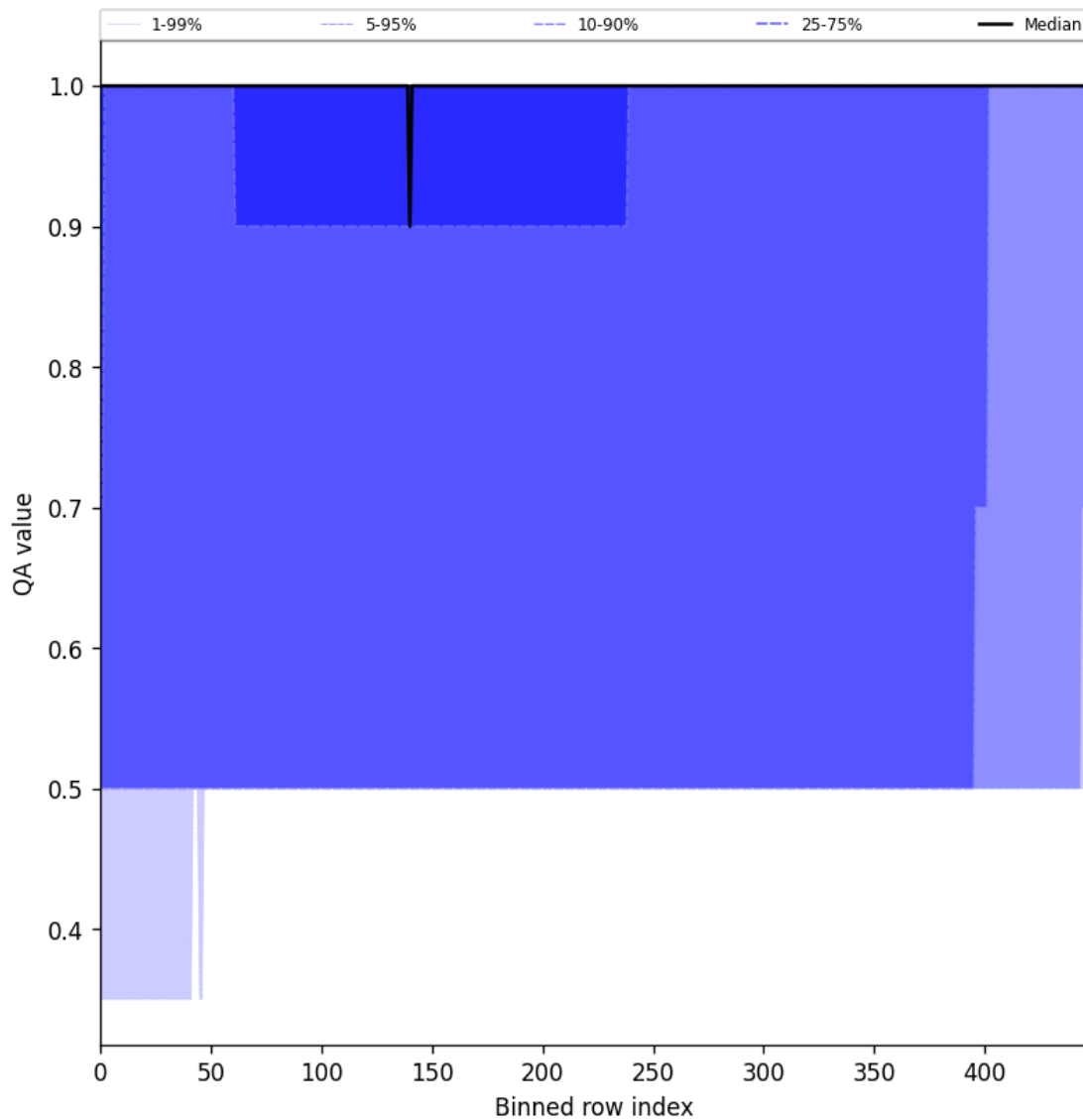
Figure 44: Along track statistics of “QA value” for 2024-12-24 to 2024-12-25
