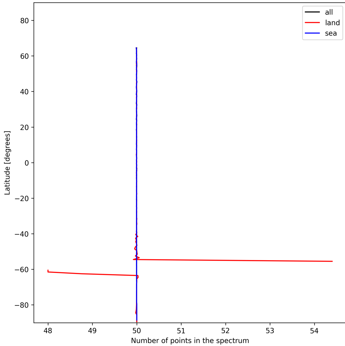
Figure 25: Zonal average of “Number of points in the spectrum” for 2024-12-24 to 2024-12-25.
