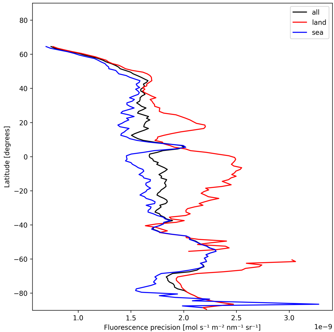
Figure 22: Zonal average of “Fluorescence precision” for 2024-12-24 to 2024-12-25.
