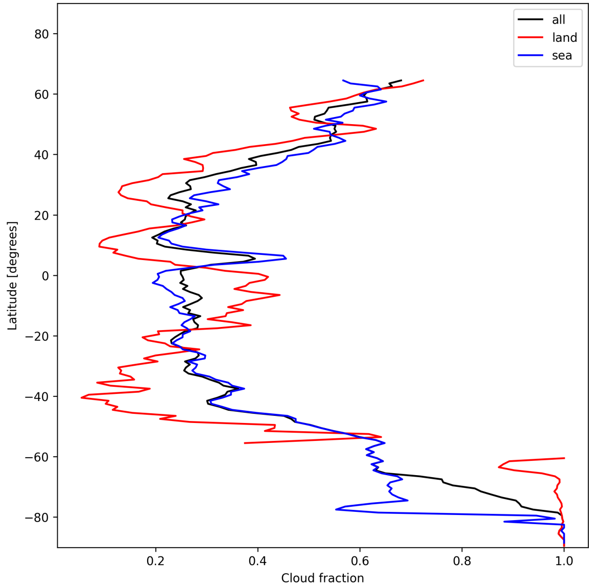
Figure 13: Zonal average of “Cloud fraction” for 2024-12-24 to 2024-12-25.
