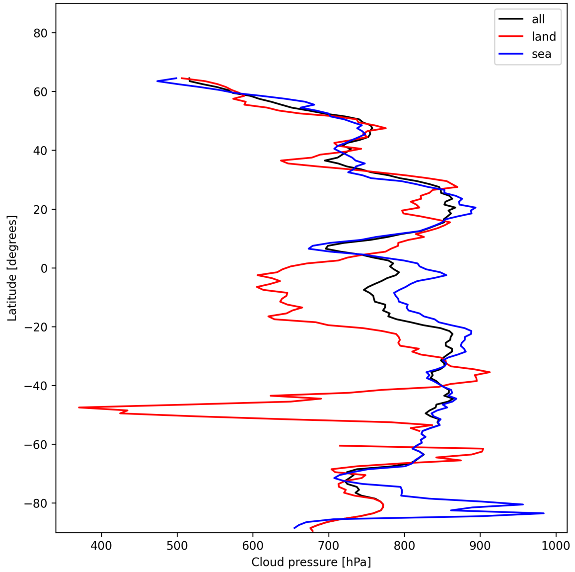
Figure 11: Zonal average of “Cloud pressure” for 2024-12-24 to 2024-12-25.
