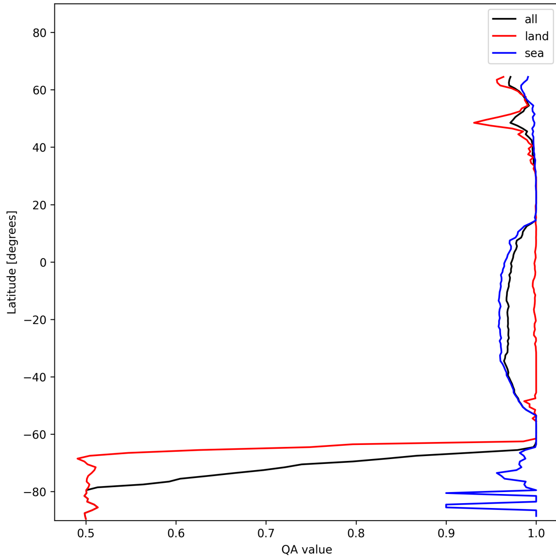
Figure 10: Zonal average of “QA value” for 2024-12-24 to 2024-12-25.
