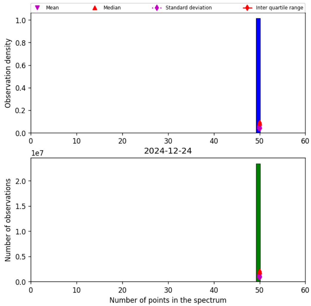
Figure 42: Histogram of “Number of points in the spectrum” for 2024-12-24 to 2024-12-25
