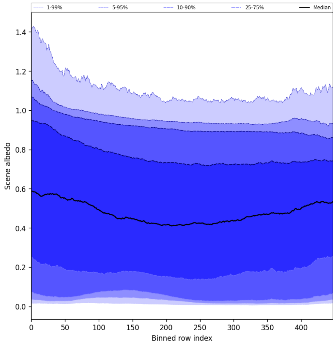
Figure 49: Along track statistics of “Scene albedo” for 2024-12-24 to 2024-12-25
