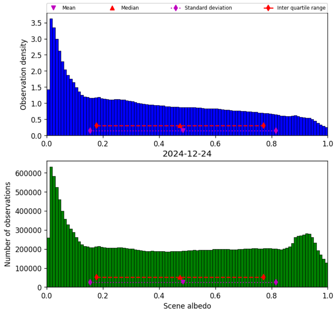
Figure 32: Histogram of “Scene albedo” for 2024-12-24 to 2024-12-25
