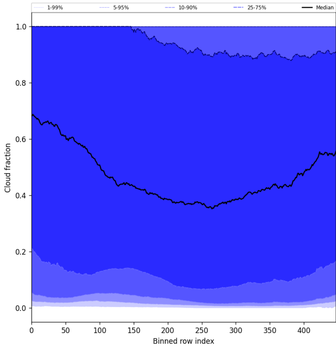
Figure 47: Along track statistics of “Cloud fraction” for 2024-12-24 to 2024-12-25
