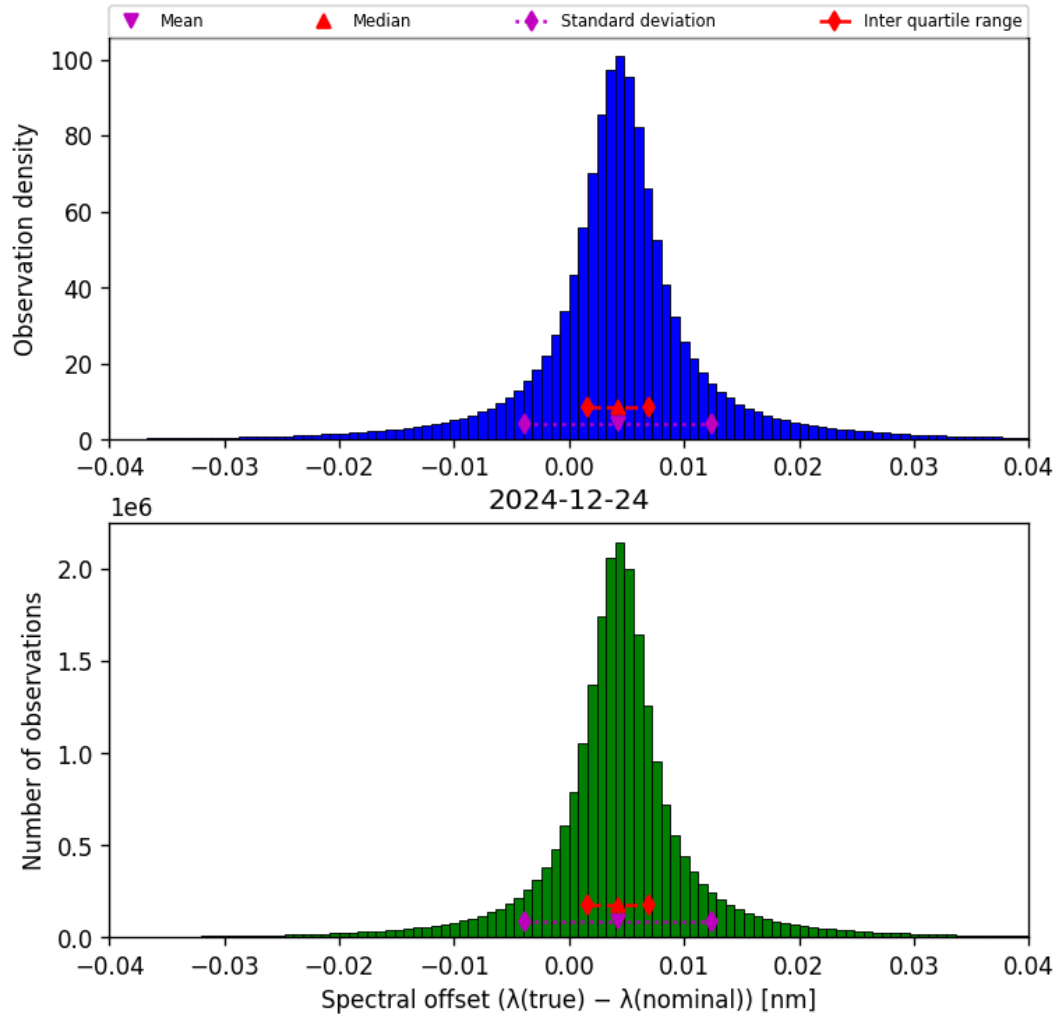
Figure 43: Histogram of “Spectral offset ( \lambda_{\text{true}} - \lambda_{\text{nominal}} )” for 2024-12-24 to 2024-12-25
