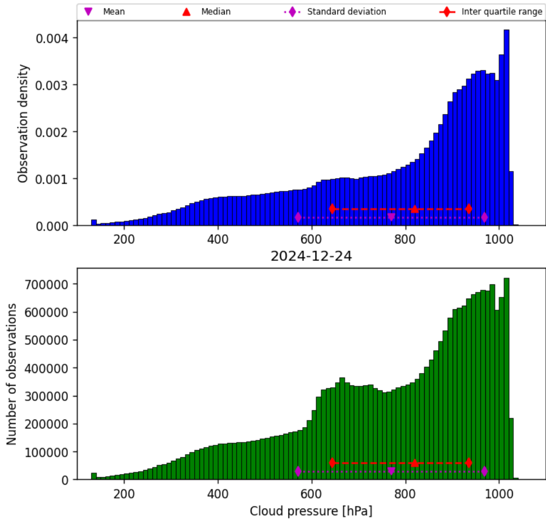
Figure 28: Histogram of “Cloud pressure” for 2024-12-24 to 2024-12-25
