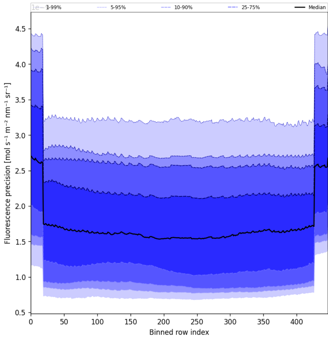
Figure 56: Along track statistics of “Fluorescence precision” for 2024-12-24 to 2024-12-25
