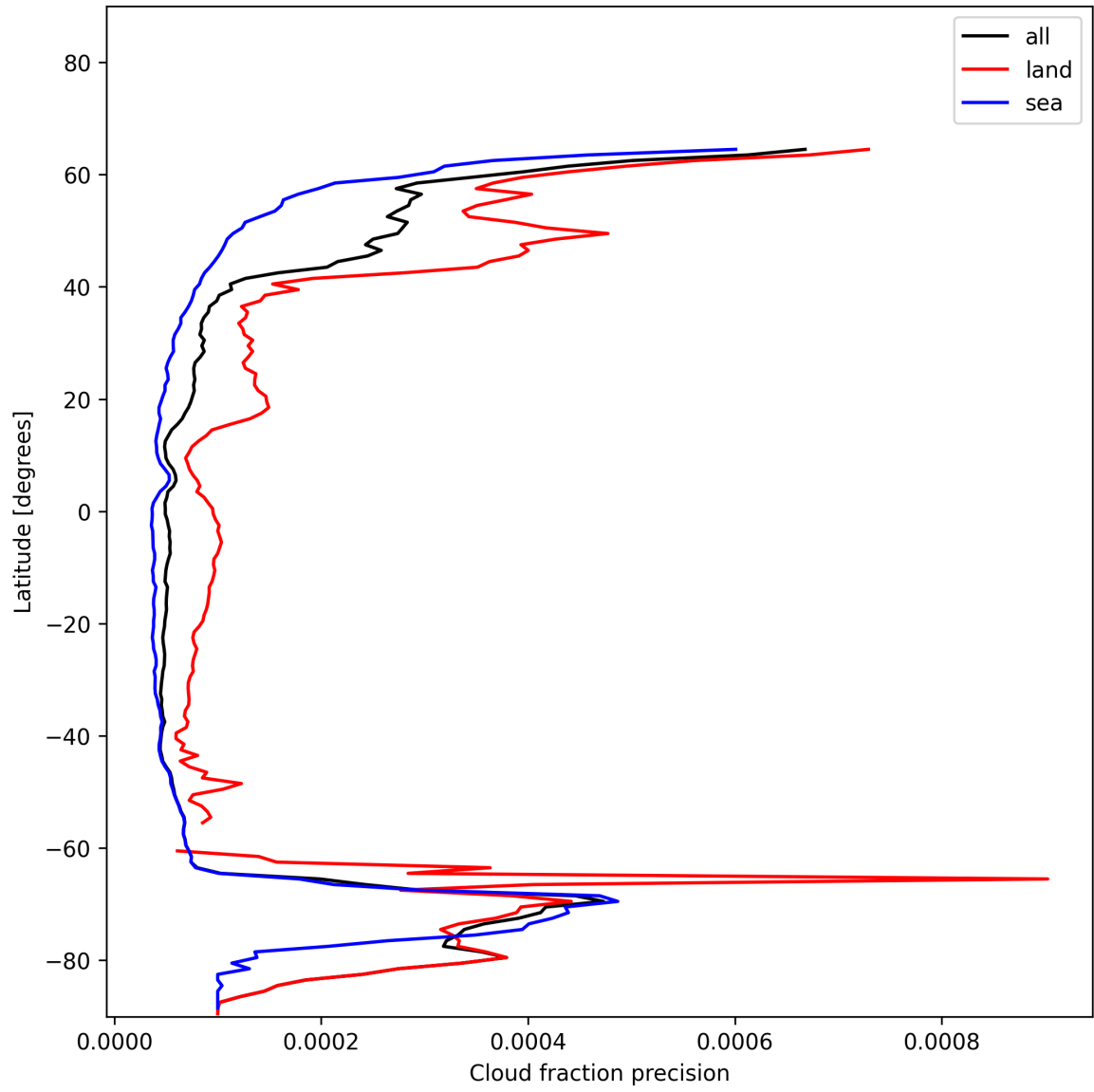
Figure 14: Zonal average of “Cloud fraction precision” for 2024-12-24 to 2024-12-25.
