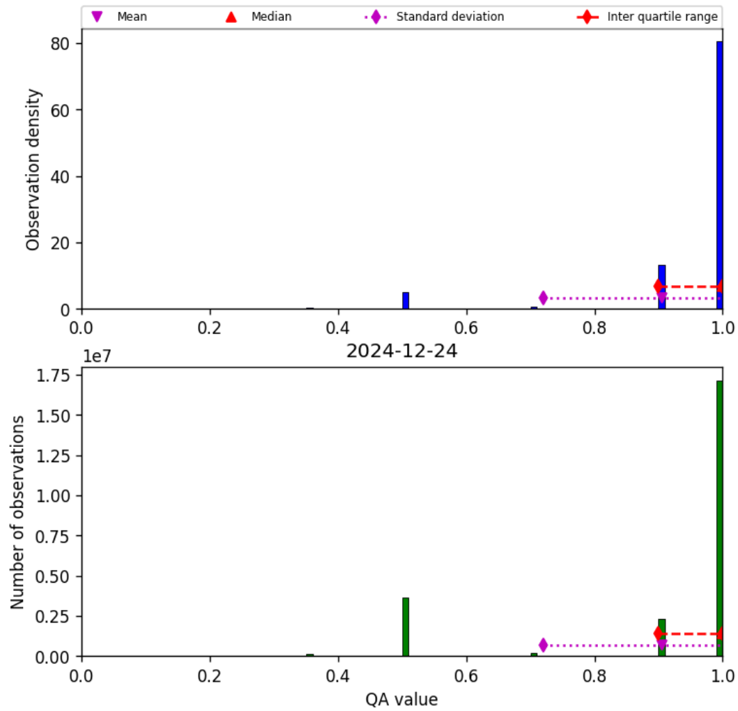
Figure 27: Histogram of “QA value” for 2024-12-24 to 2024-12-25
