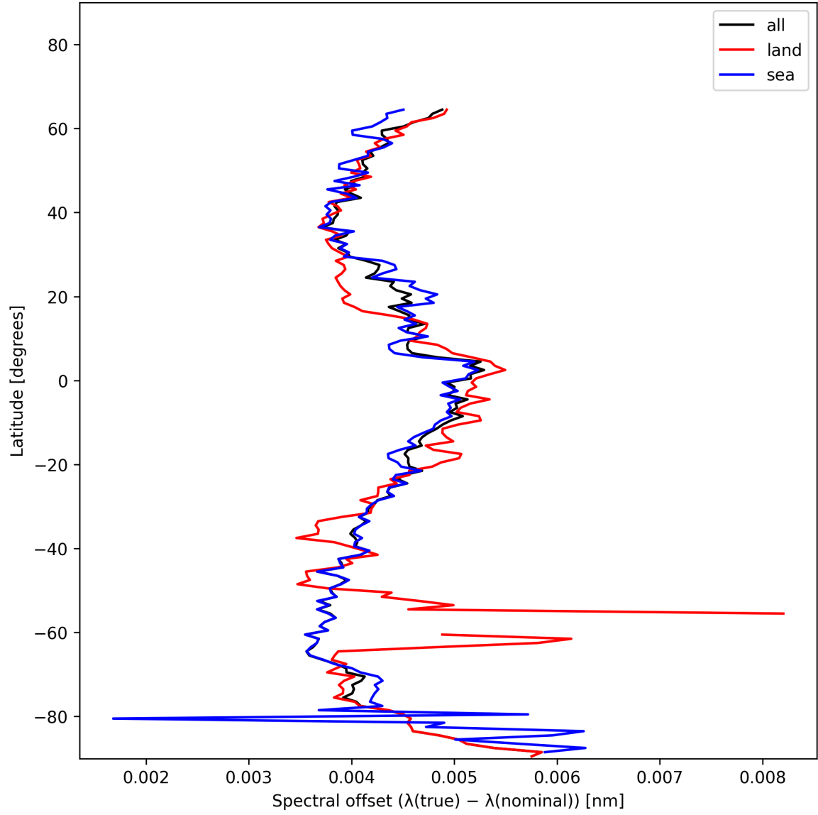
Figure 26: Zonal average of “Spectral offset ( \lambda_{\text{true}} - \lambda_{\text{nominal}} )” for 2024-12-24 to 2024-12-25.
