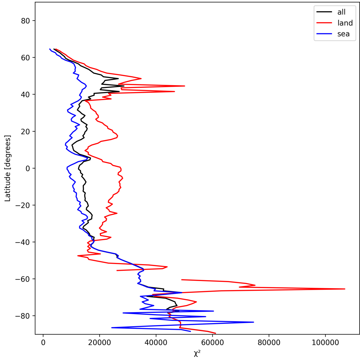
Figure 19: Zonal average of “ \chi^2 ” for 2024-12-24 to 2024-12-25.
