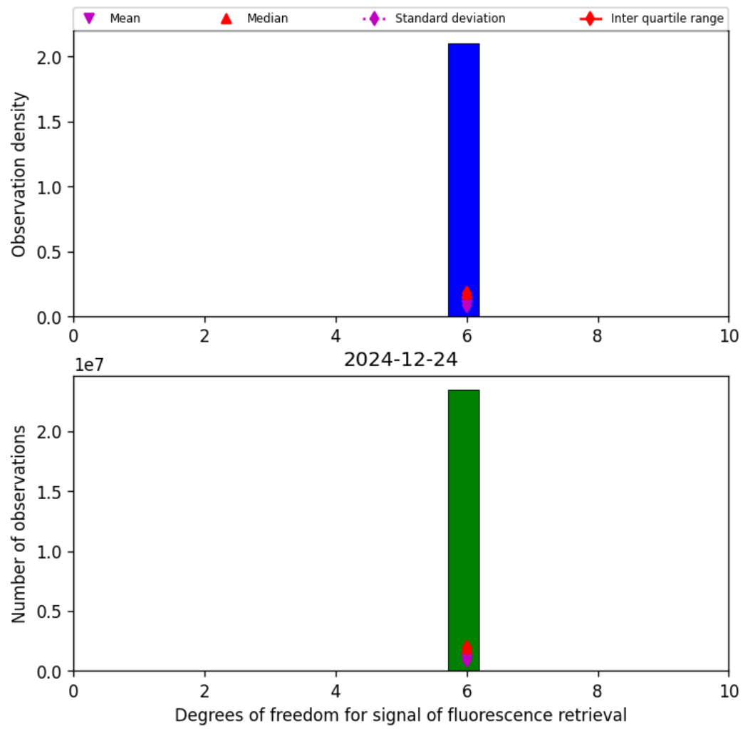
Figure 41: Histogram of “Degrees of freedom for signal of fluorescence retrieval” for 2024-12-24 to 2024-12-25
