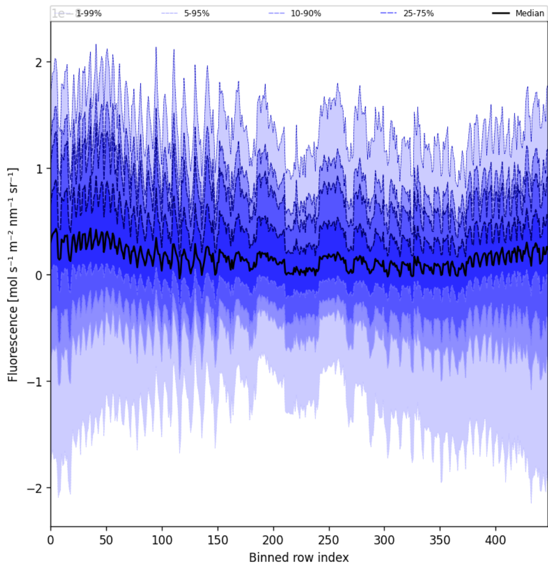
Figure 55: Along track statistics of “Fluorescence” for 2024-12-24 to 2024-12-25
