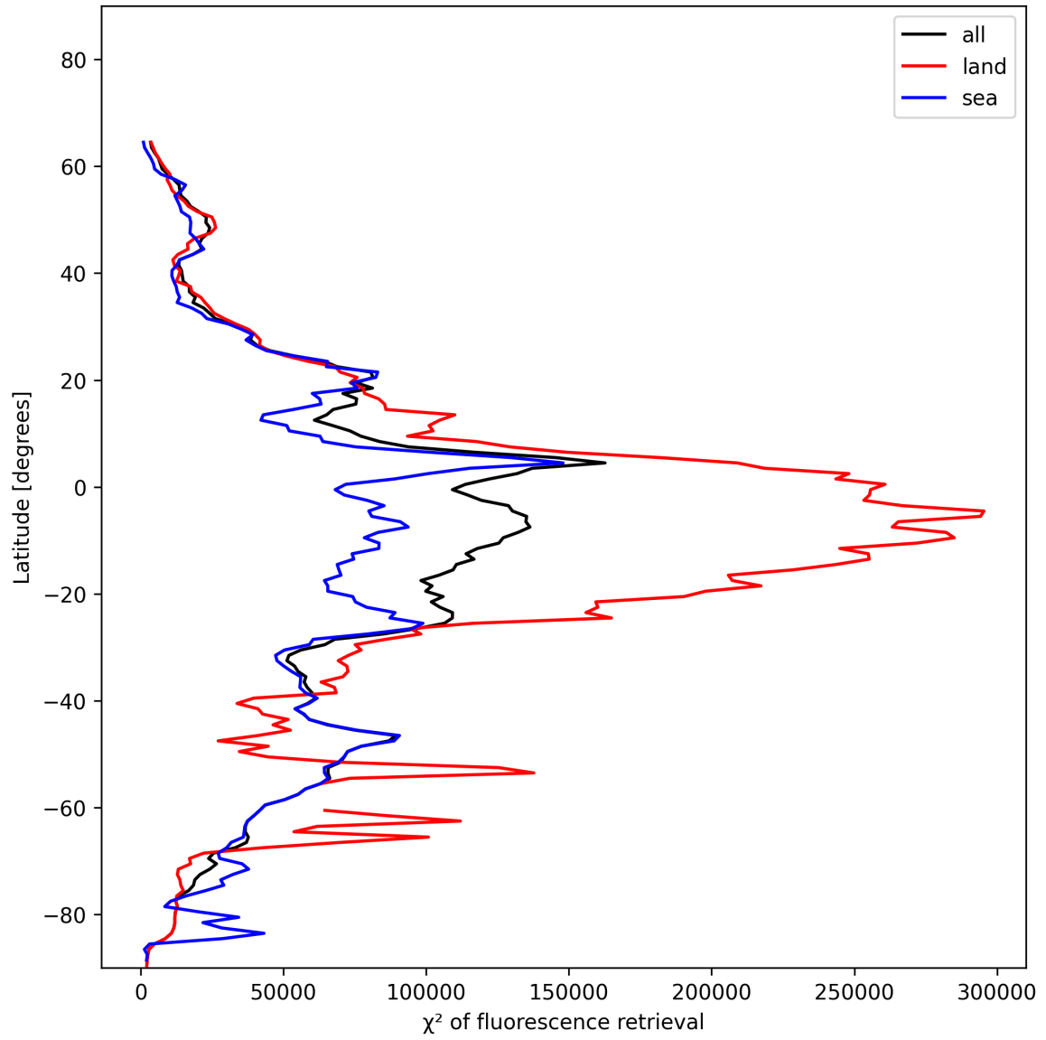
Figure 23: Zonal average of “ \chi^2 of fluorescence retrieval” for 2024-12-24 to 2024-12-25.
