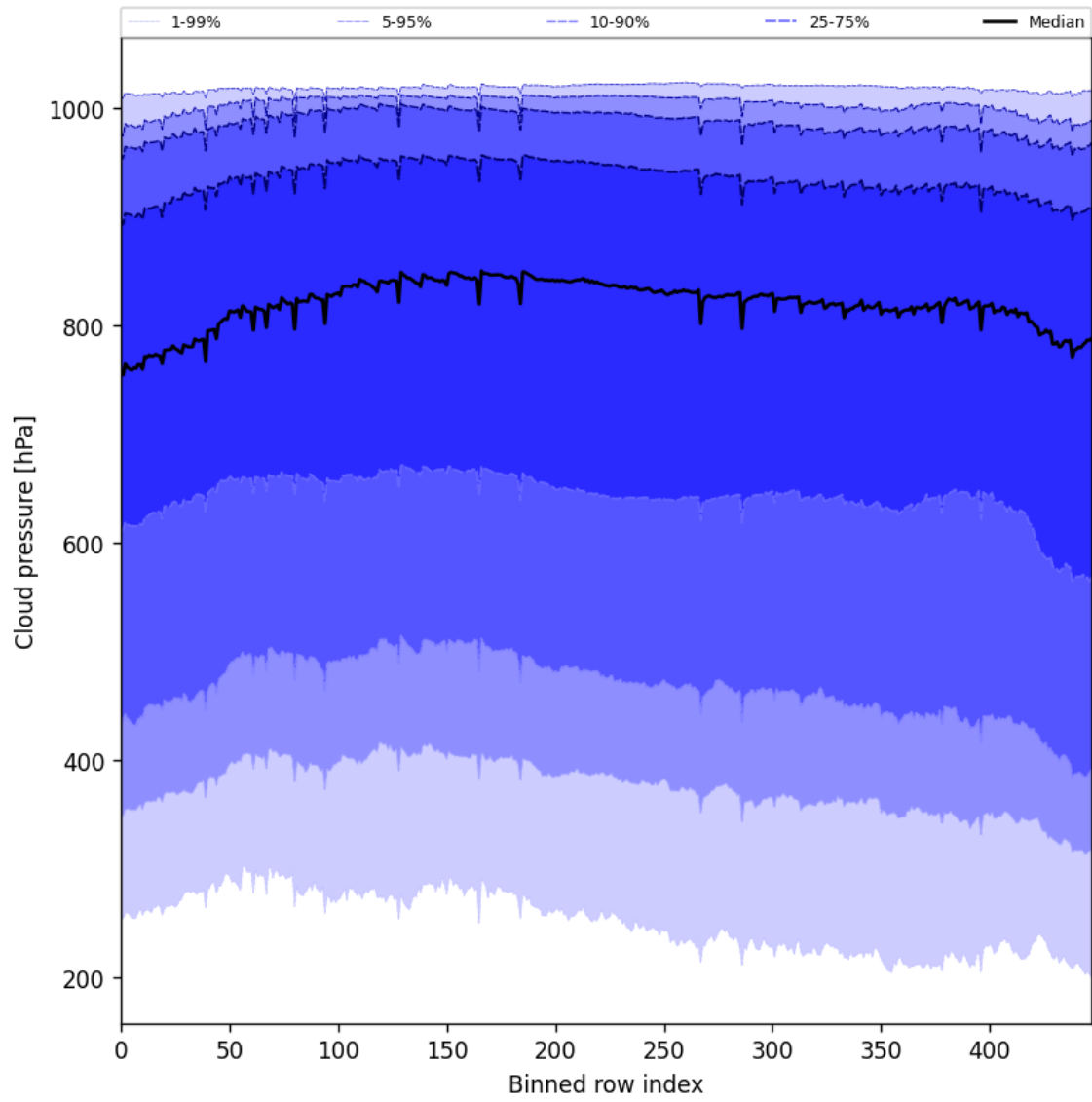
Figure 45: Along track statistics of “Cloud pressure” for 2024-12-24 to 2024-12-25
