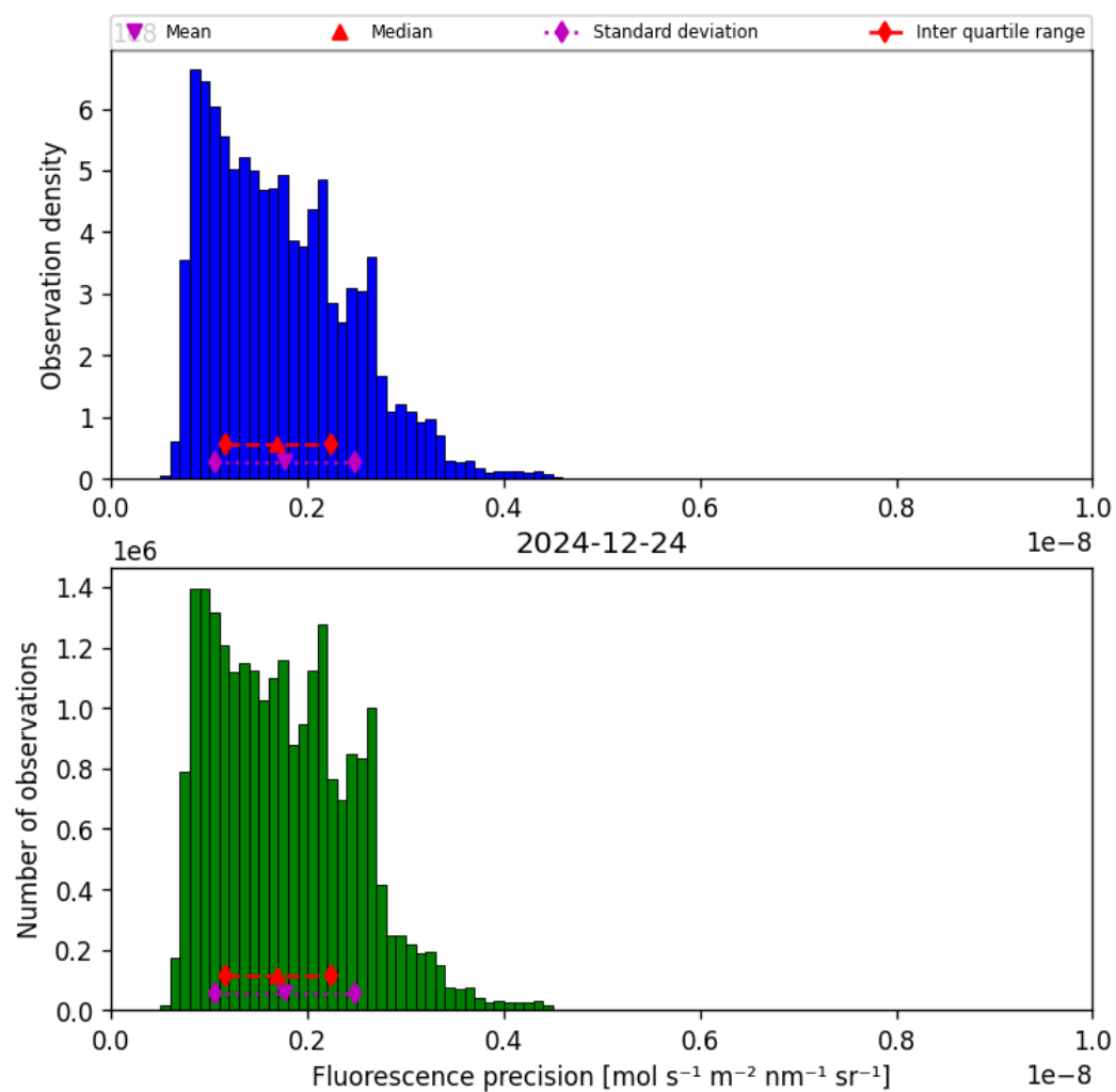
Figure 39: Histogram of “Fluorescence precision” for 2024-12-24 to 2024-12-25
