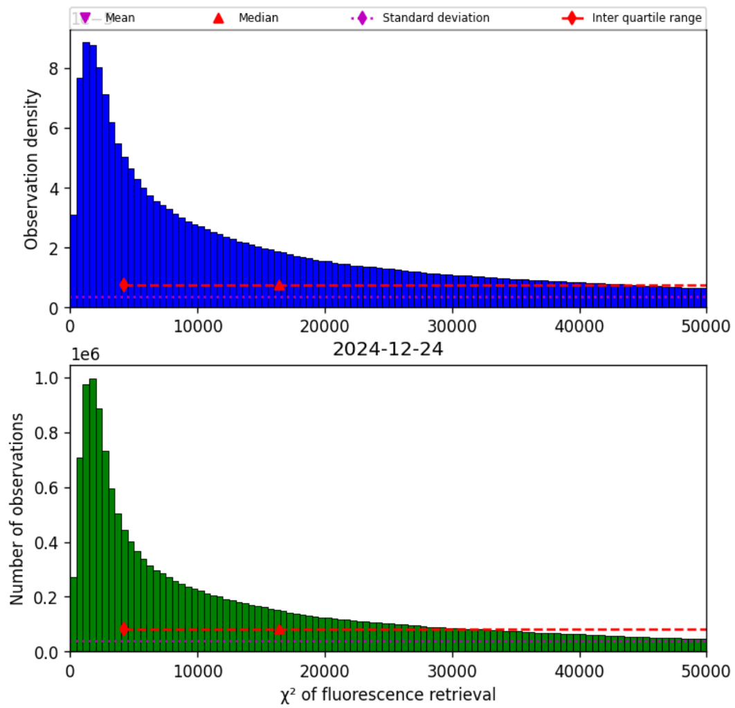
Figure 40: Histogram of “ \chi^2 of fluorescence retrieval” for 2024-12-24 to 2024-12-25
