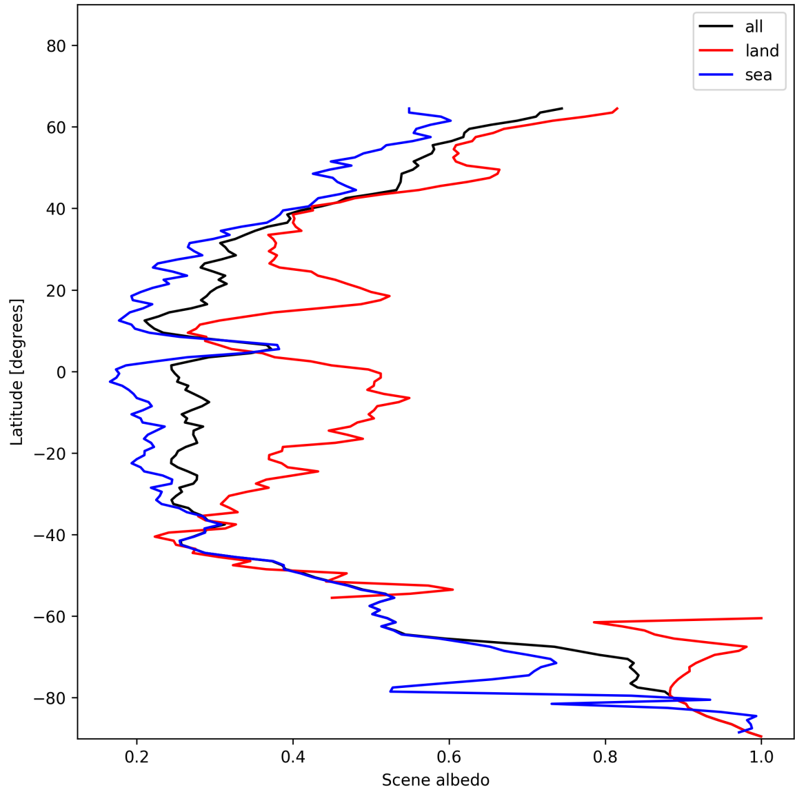
Figure 15: Zonal average of “Scene albedo” for 2024-12-24 to 2024-12-25.
