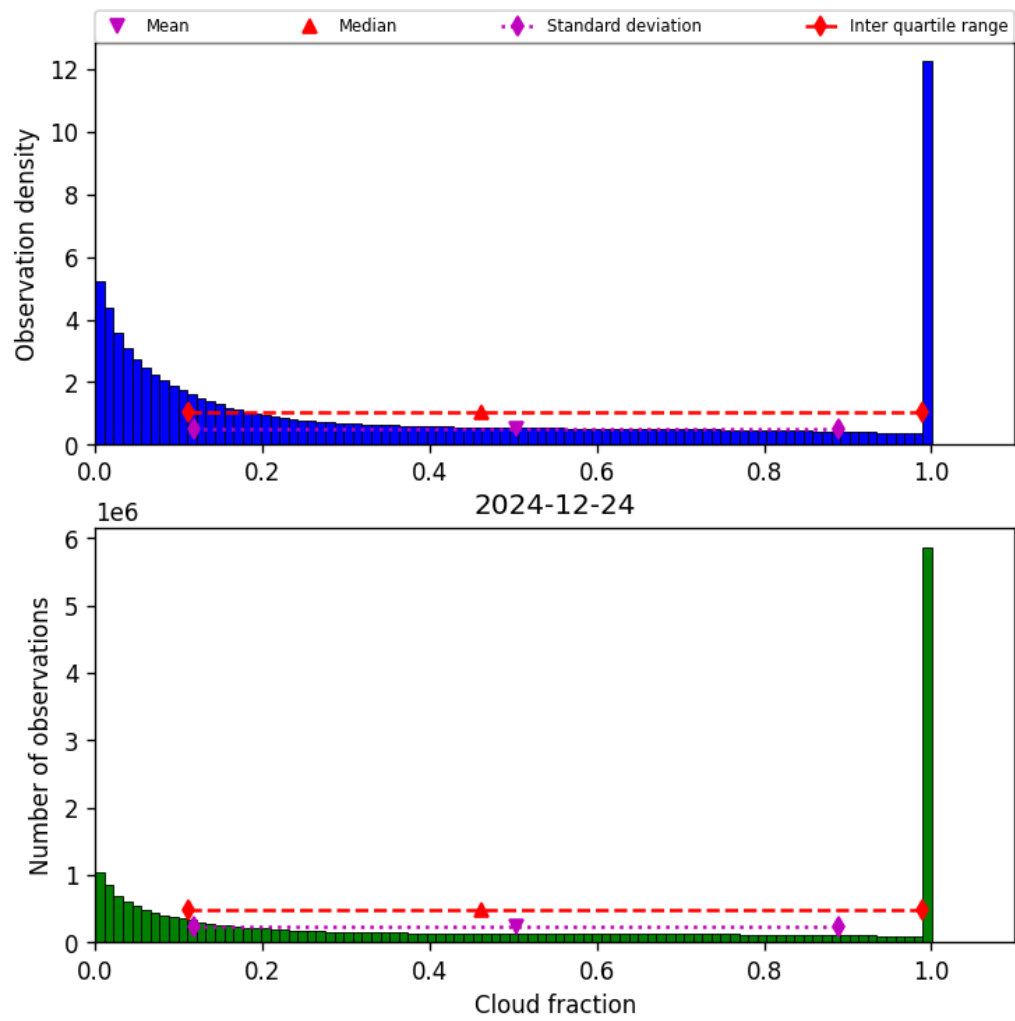
Figure 30: Histogram of “Cloud fraction” for 2024-12-24 to 2024-12-25
