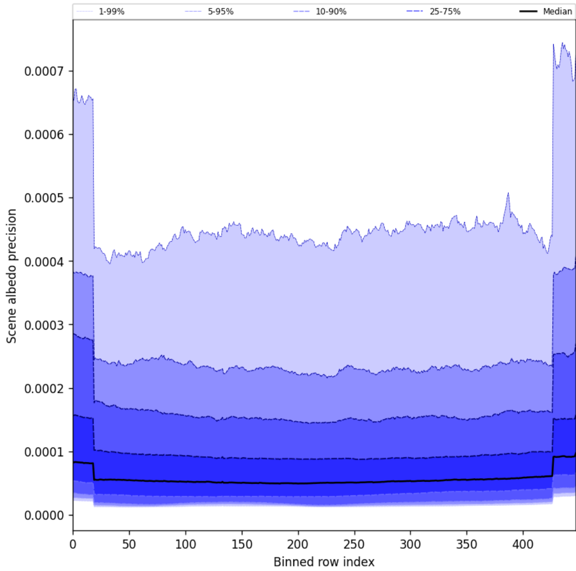
Figure 50: Along track statistics of “Scene albedo precision” for 2024-12-24 to 2024-12-25
