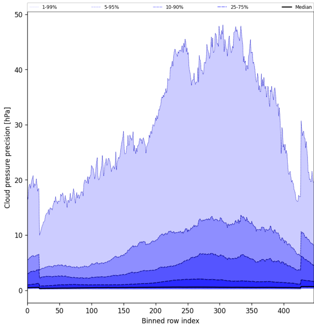
Figure 46: Along track statistics of “Cloud pressure precision” for 2024-12-24 to 2024-12-25
