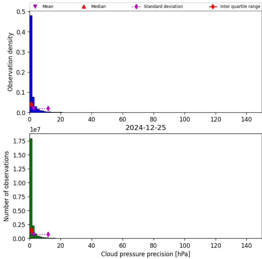
Figure 29: Histogram of “Cloud pressure precision” for 2024-12-25 to 2024-12-25
