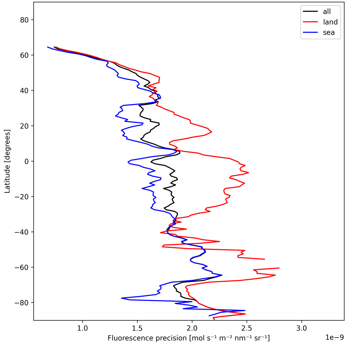
Figure 22: Zonal average of “Fluorescence precision” for 2024-12-25 to 2024-12-25.
