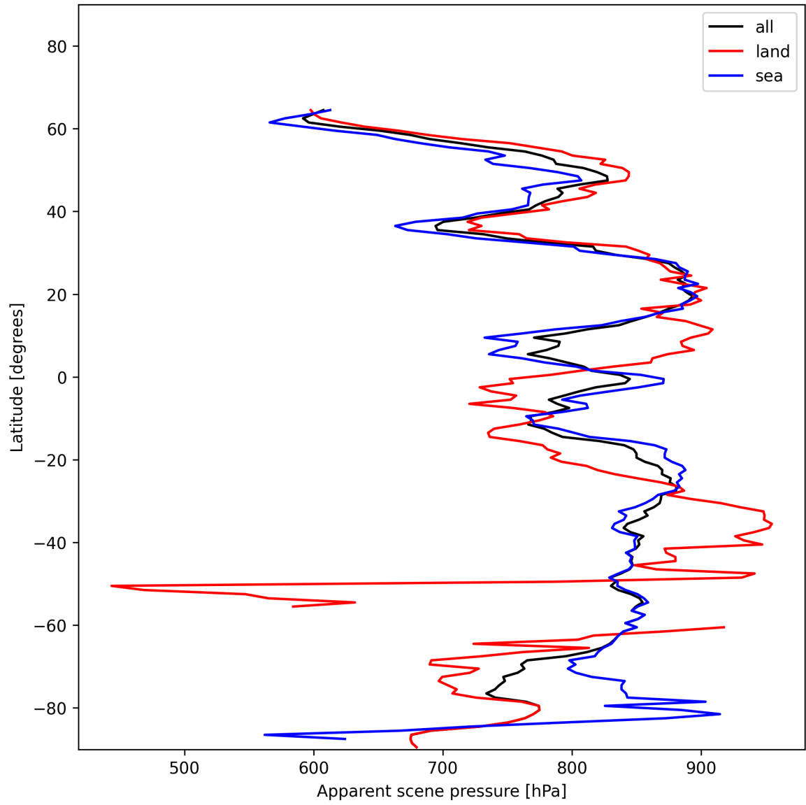
Figure 17: Zonal average of “Apparent scene pressure” for 2024-12-25 to 2024-12-25.
