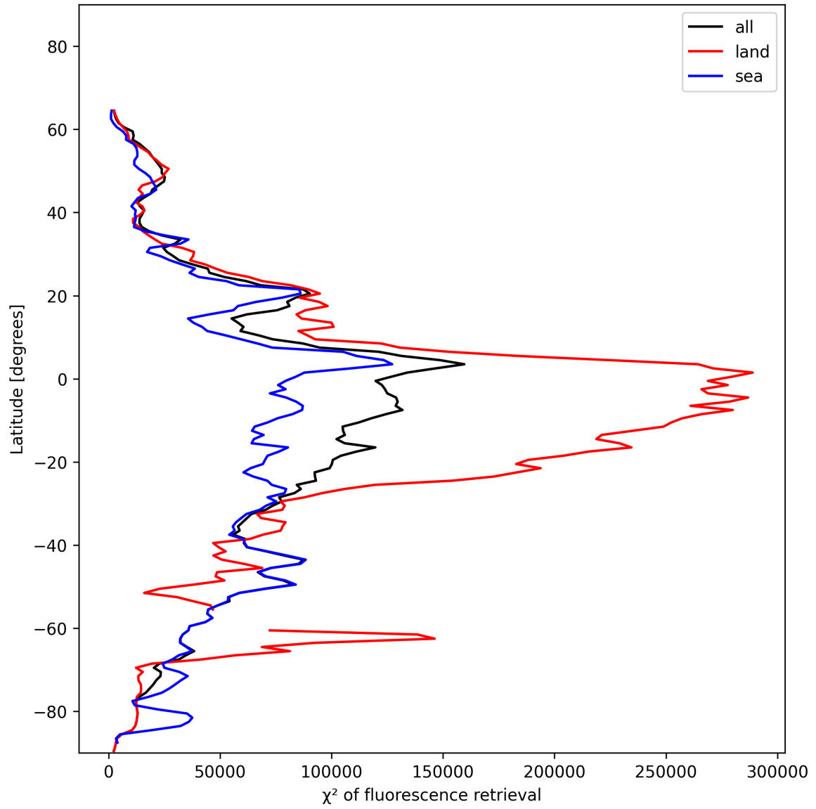
Figure 23: Zonal average of “ \chi^2 of fluorescence retrieval” for 2024-12-25 to 2024-12-25.
