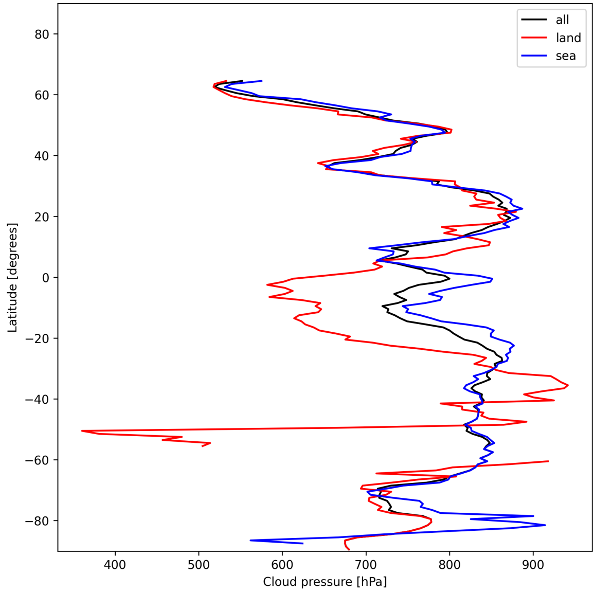
Figure 11: Zonal average of “Cloud pressure” for 2024-12-25 to 2024-12-25.
