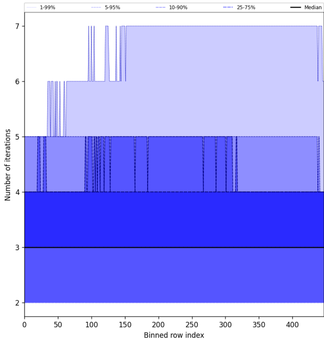
Figure 54: Along track statistics of “Number of iterations” for 2024-12-25 to 2024-12-25
