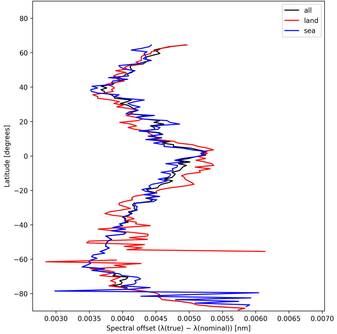
Figure 26: Zonal average of “Spectral offset ( \lambda_{\text{true}} - \lambda_{\text{nominal}} )” for 2024-12-25 to 2024-12-25.
