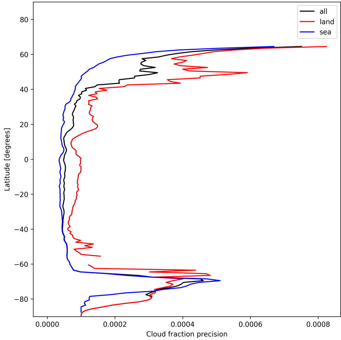
Figure 14: Zonal average of “Cloud fraction precision” for 2024-12-25 to 2024-12-25.
