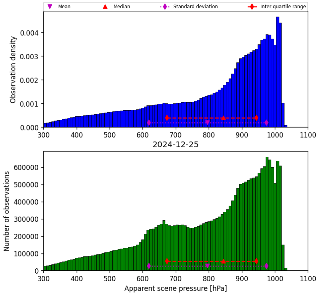
Figure 34: Histogram of “Apparent scene pressure” for 2024-12-25 to 2024-12-25
