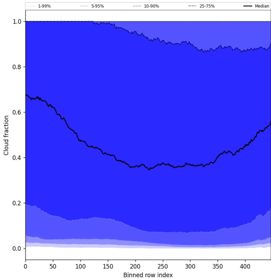
Figure 47: Along track statistics of “Cloud fraction” for 2024-12-25 to 2024-12-25
