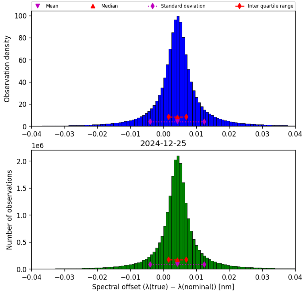
Figure 43: Histogram of “Spectral offset ( \lambda_{\text{true}} - \lambda_{\text{nominal}} )” for 2024-12-25 to 2024-12-25
