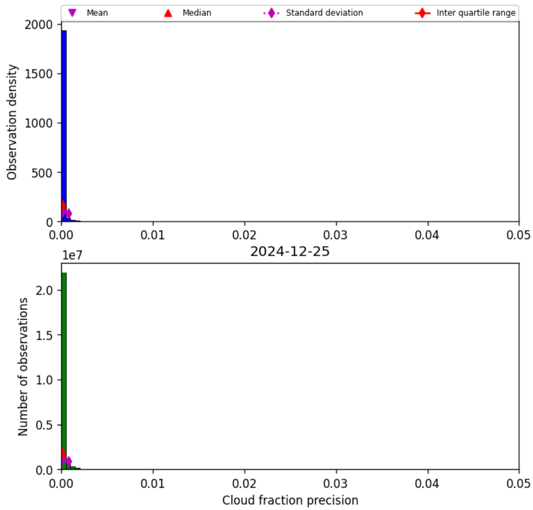
Figure 31: Histogram of “Cloud fraction precision” for 2024-12-25 to 2024-12-25
