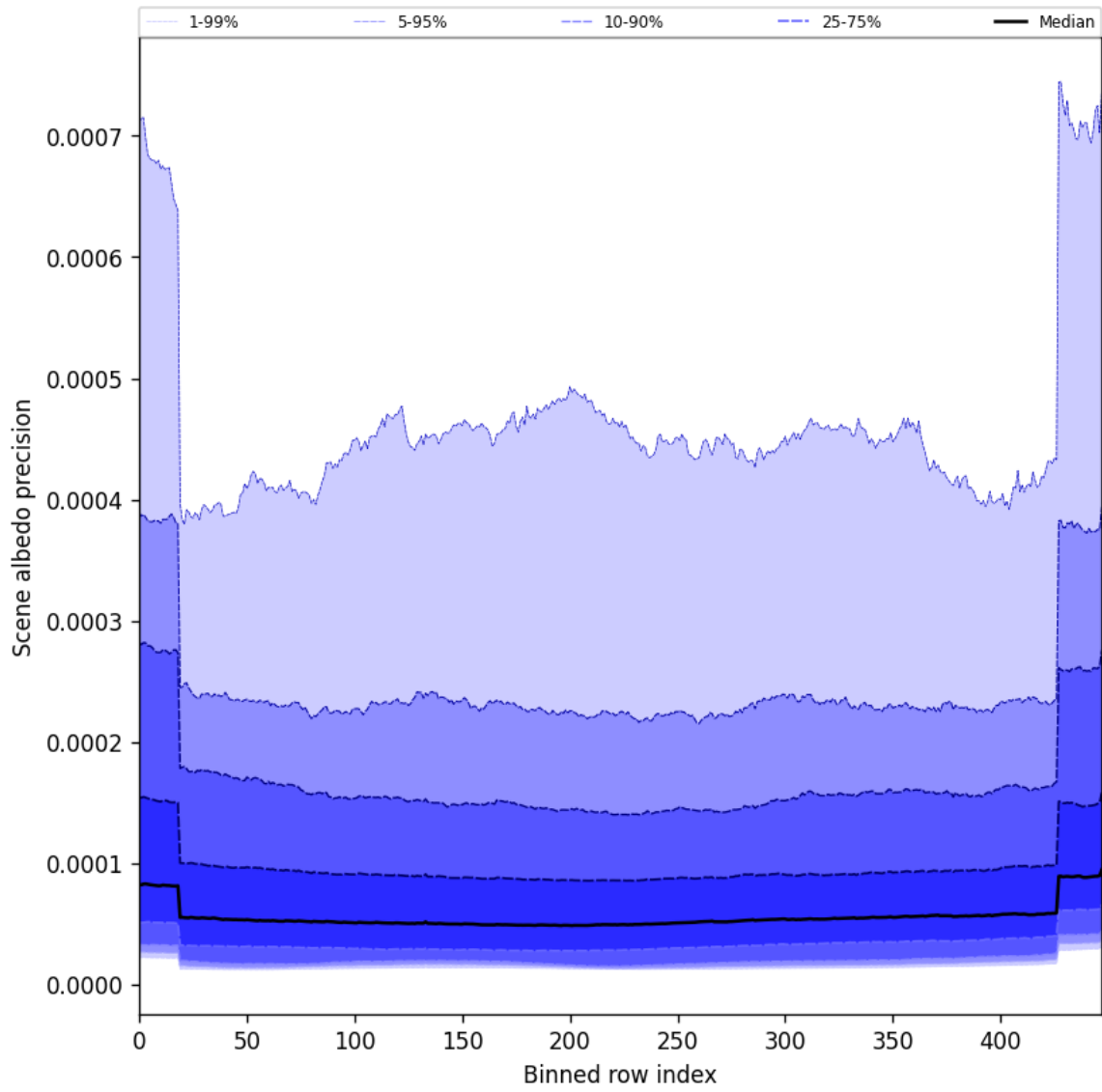
Figure 50: Along track statistics of “Scene albedo precision” for 2024-12-25 to 2024-12-25
