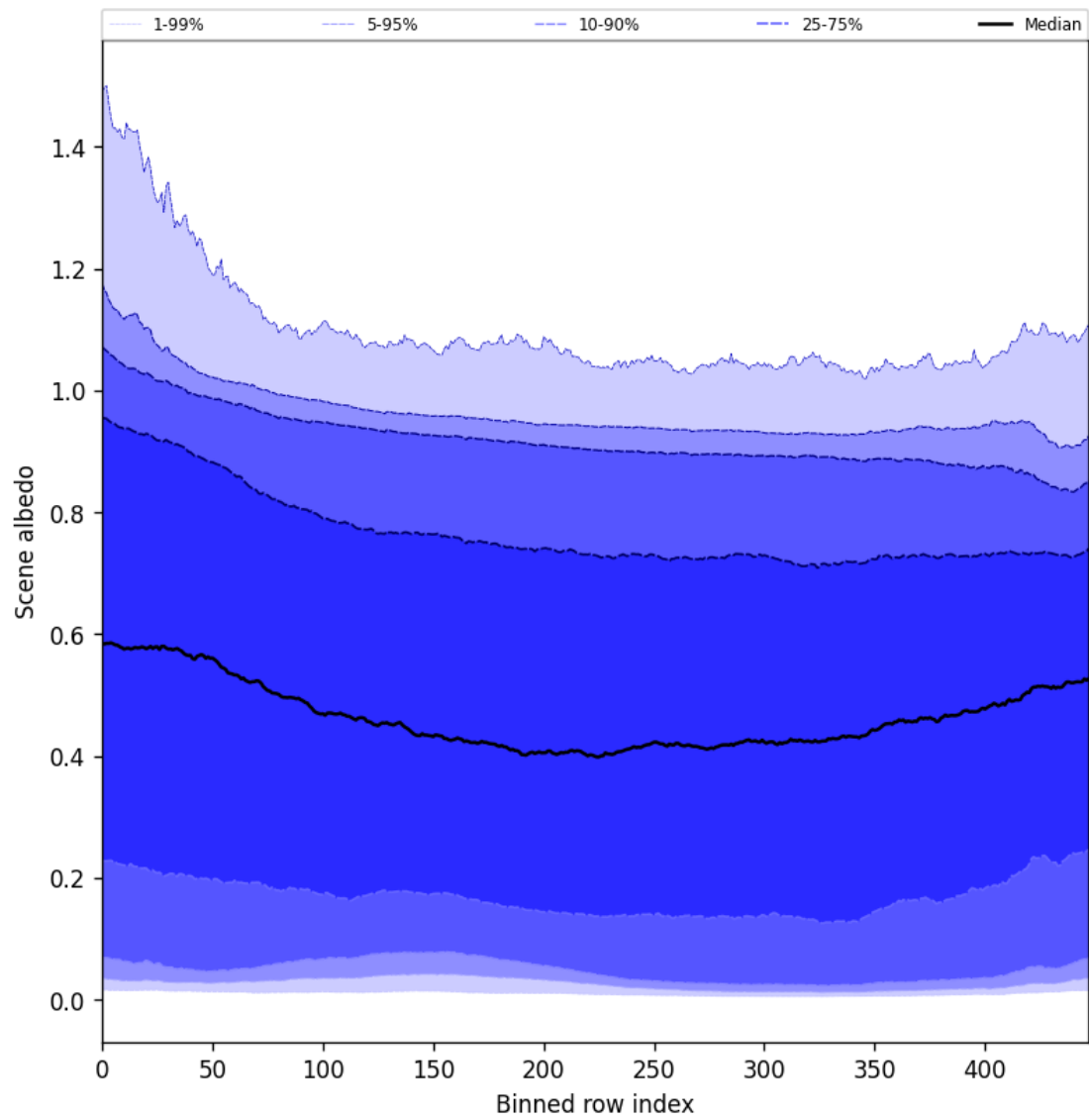
Figure 49: Along track statistics of “Scene albedo” for 2024-12-25 to 2024-12-25
