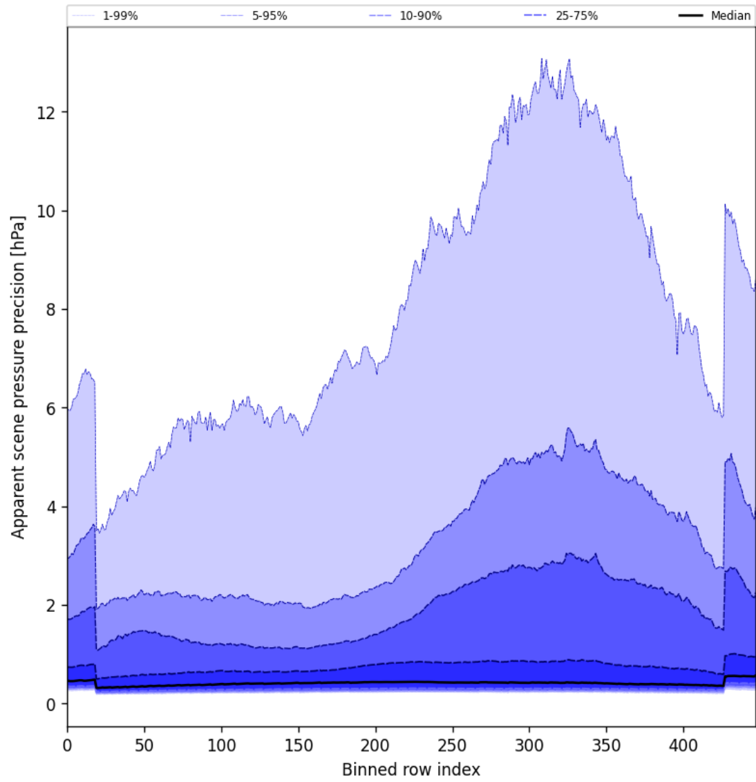
Figure 52: Along track statistics of “Apparent scene pressure precision” for 2024-12-25 to 2024-12-25
