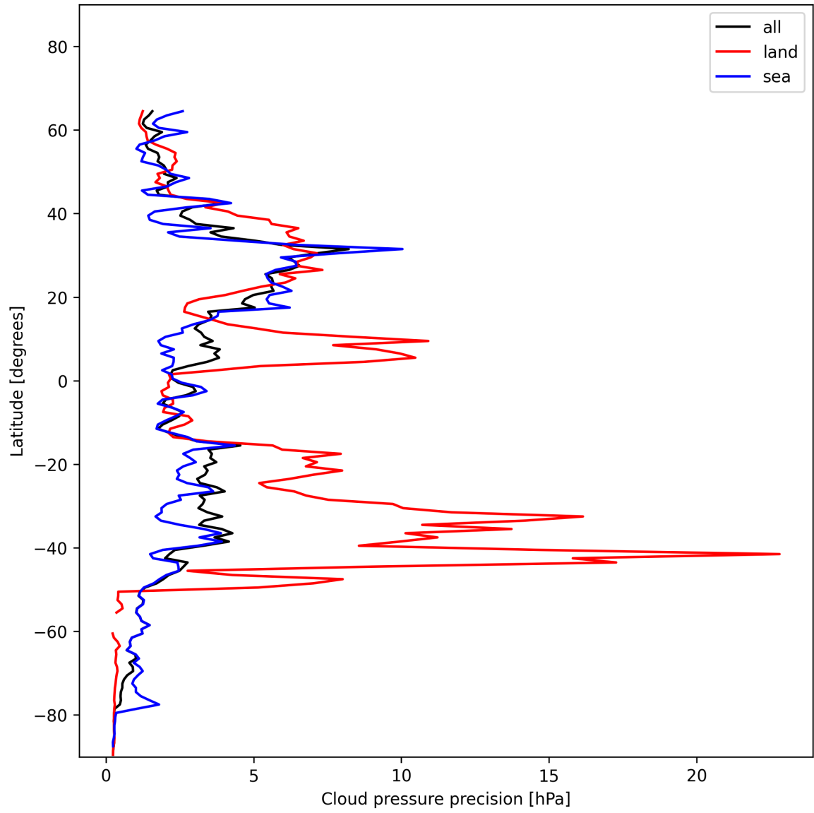
Figure 12: Zonal average of “Cloud pressure precision” for 2024-12-25 to 2024-12-25.
