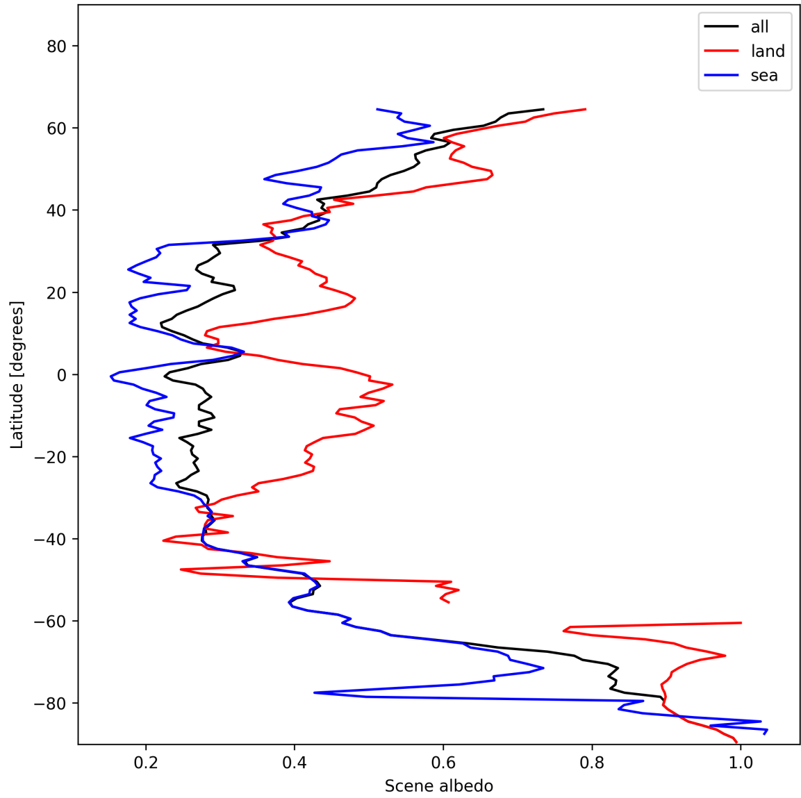
Figure 15: Zonal average of “Scene albedo” for 2024-12-25 to 2024-12-25.
