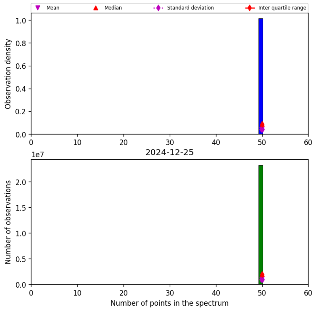
Figure 42: Histogram of "Number of points in the spectrum" for 2024-12-25 to 2024-12-25
