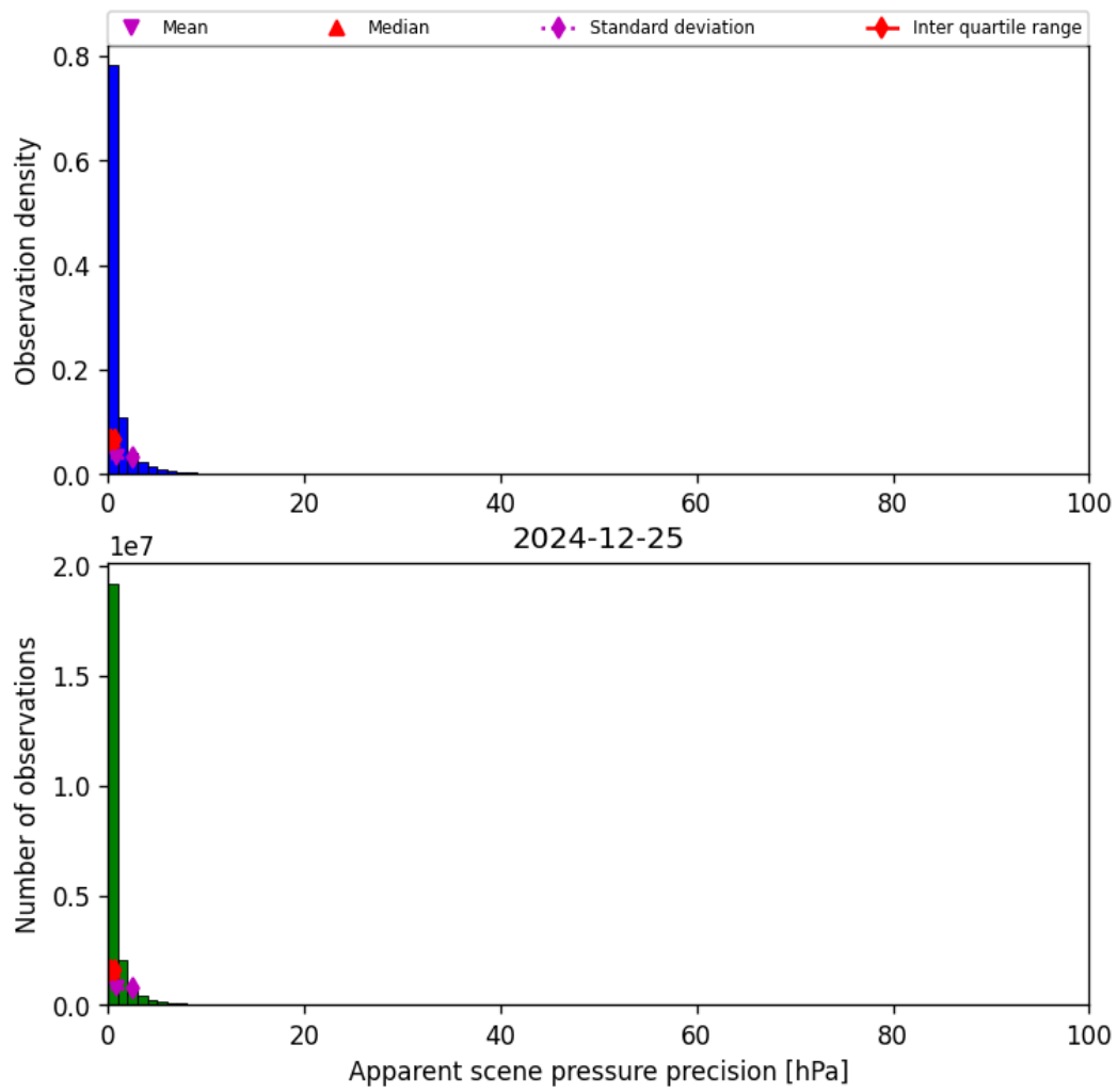
Figure 35: Histogram of “Apparent scene pressure precision” for 2024-12-25 to 2024-12-25
