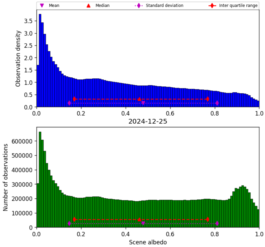
Figure 32: Histogram of “Scene albedo” for 2024-12-25 to 2024-12-25
