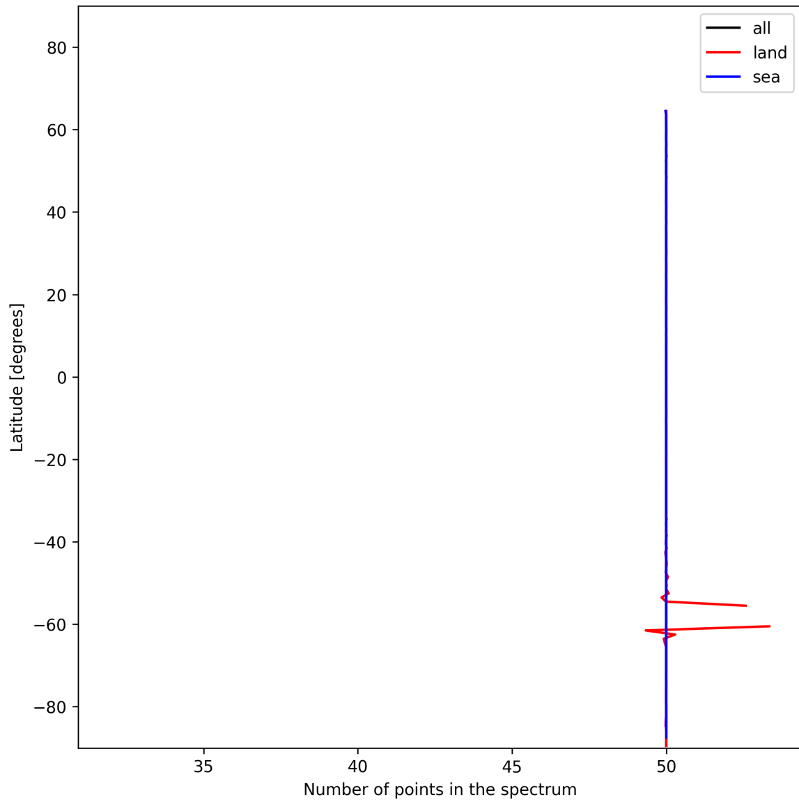
Figure 25: Zonal average of “Number of points in the spectrum” for 2024-12-25 to 2024-12-25.
