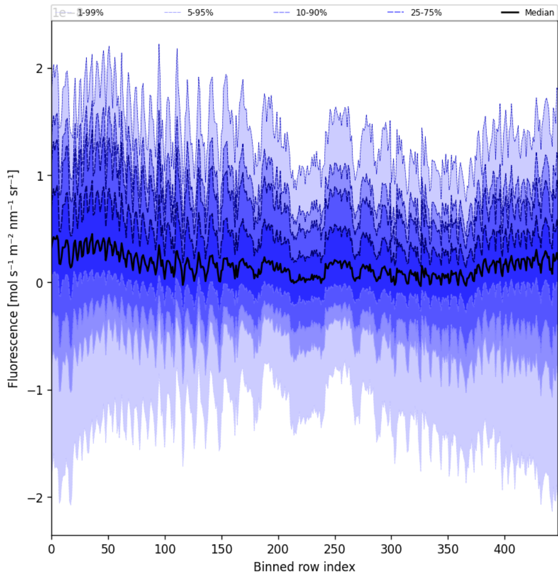
Figure 55: Along track statistics of “Fluorescence” for 2024-12-25 to 2024-12-25
