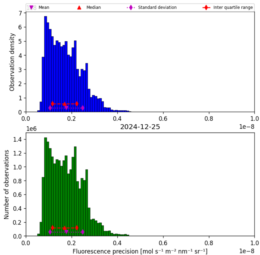
Figure 39: Histogram of “Fluorescence precision” for 2024-12-25 to 2024-12-25
