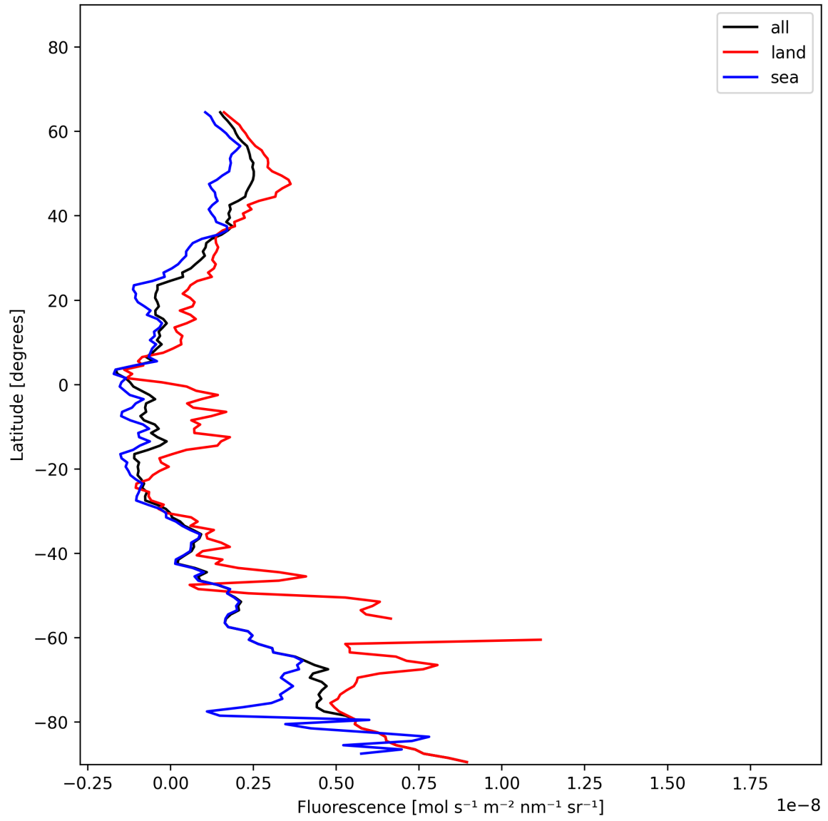
Figure 21: Zonal average of “Fluorescence” for 2024-12-25 to 2024-12-25.
