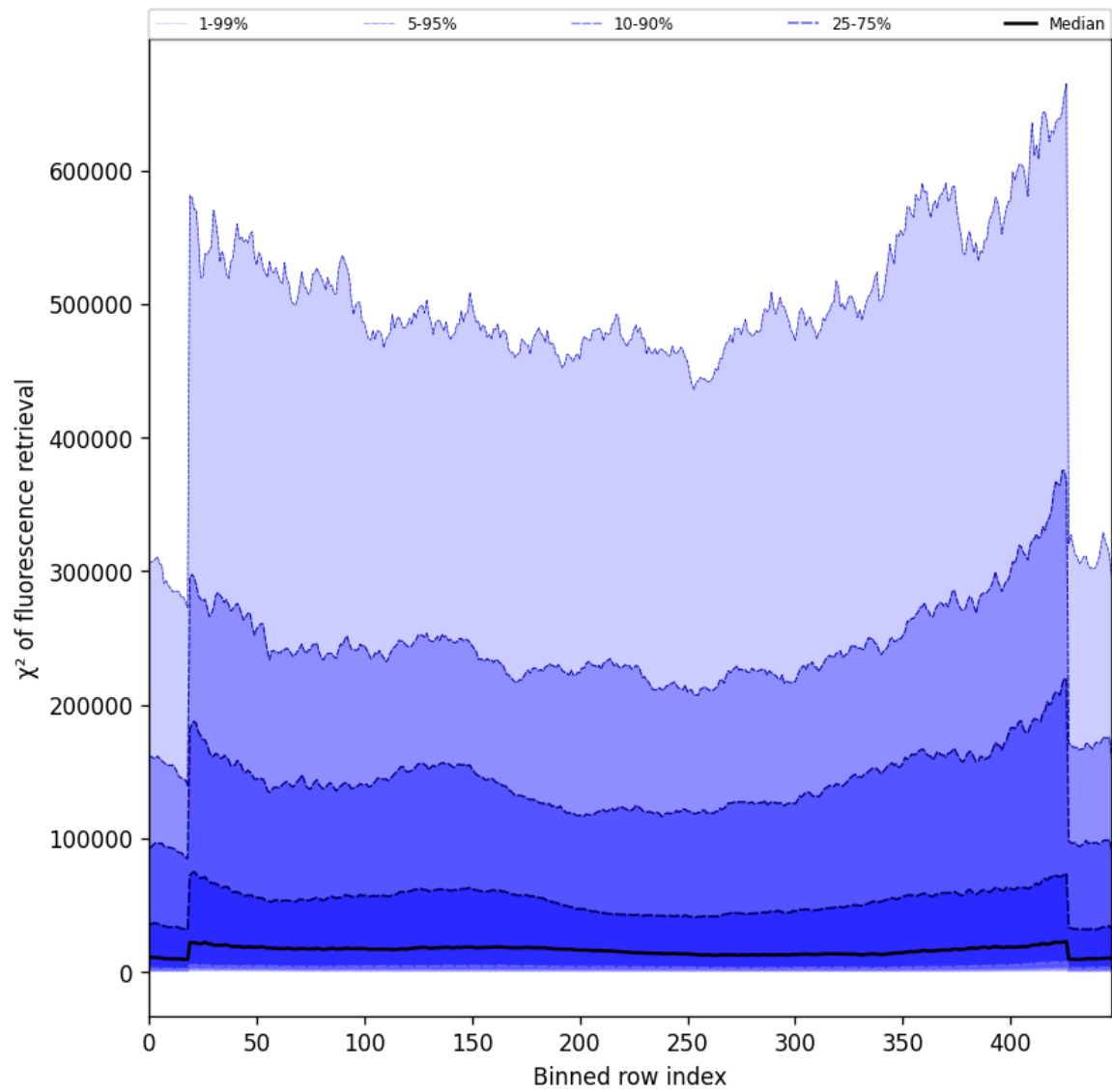
Figure 57: Along track statistics of “ \chi^2 of fluorescence retrieval” for 2024-12-25 to 2024-12-25
