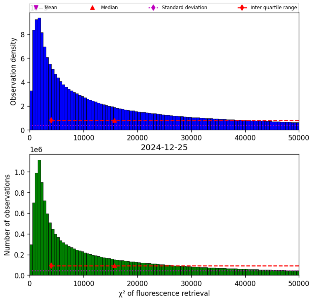
Figure 40: Histogram of “ \chi^2 of fluorescence retrieval” for 2024-12-25 to 2024-12-25
