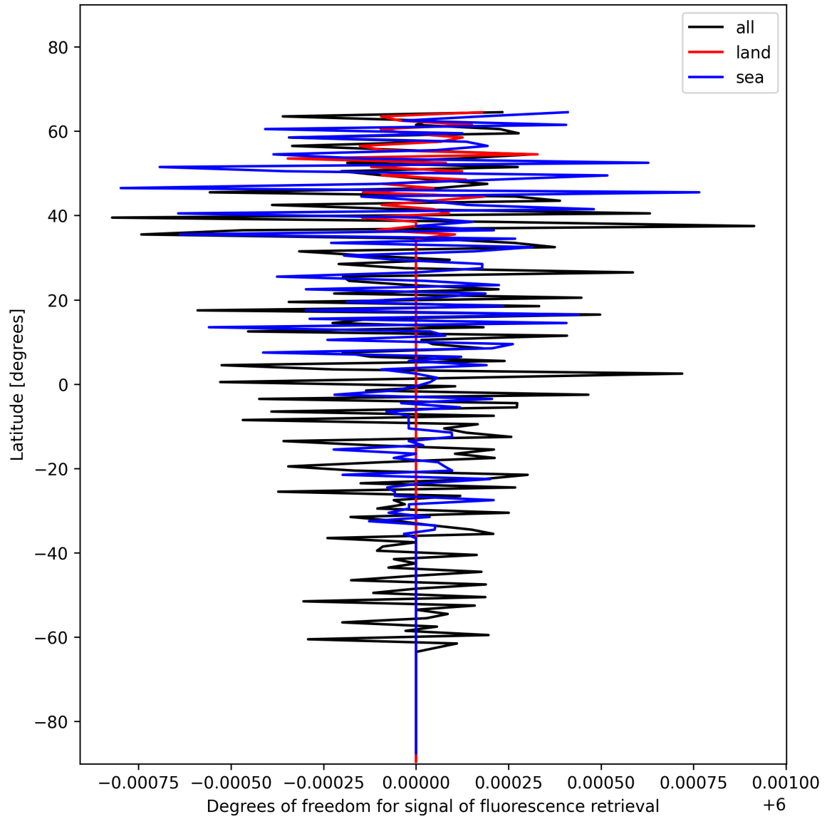
Figure 24: Zonal average of “Degrees of freedom for signal of fluorescence retrieval” for 2024-12-25 to 2024-12-25.
