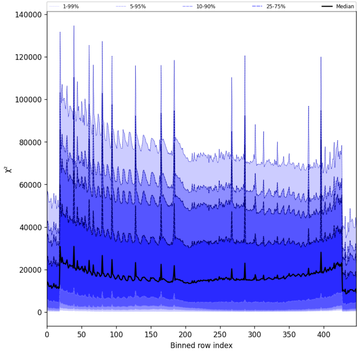
Figure 53: Along track statistics of “ \chi^2 ” for 2024-12-25 to 2024-12-25
