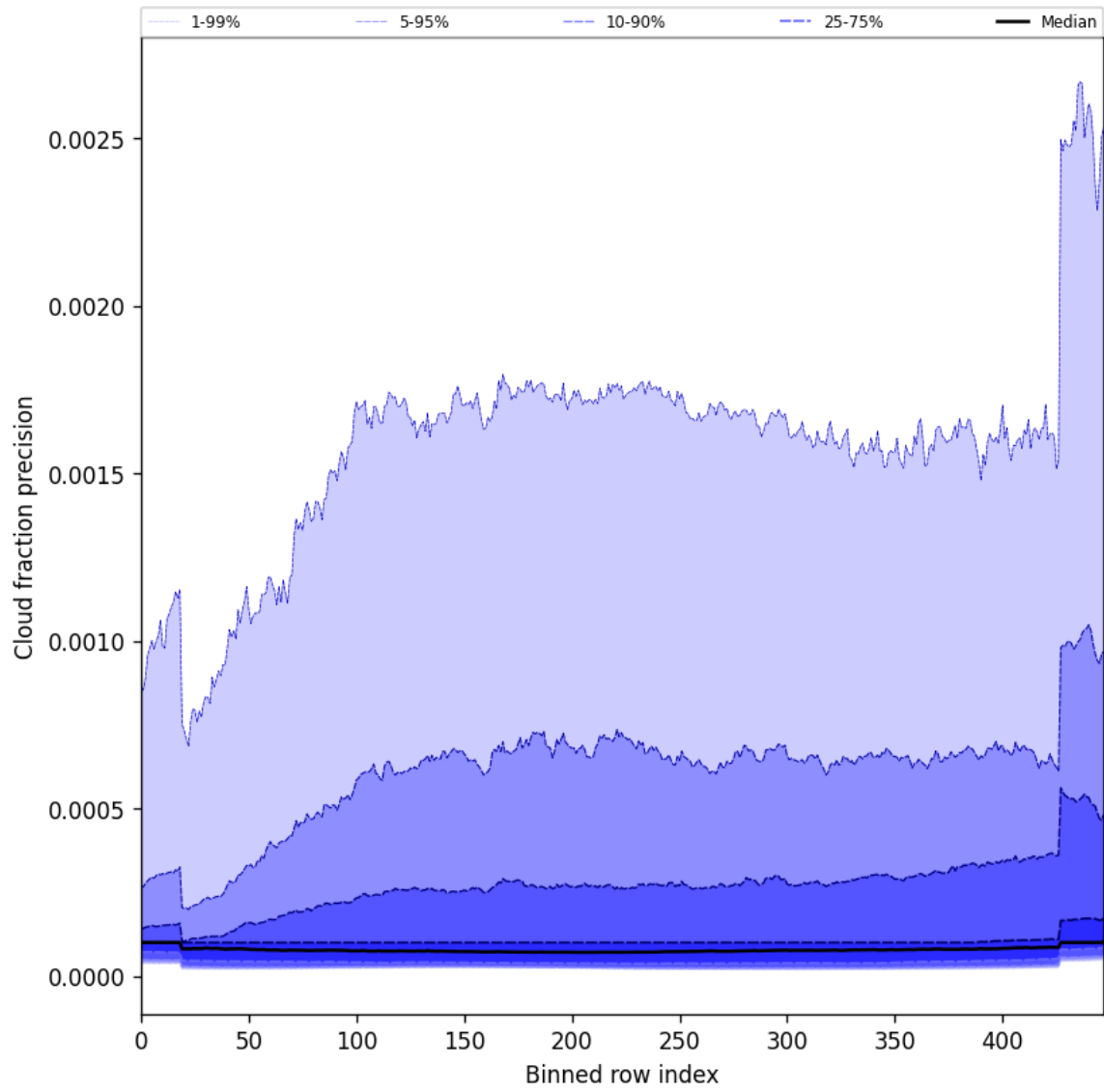
Figure 48: Along track statistics of “Cloud fraction precision” for 2024-12-25 to 2024-12-25
