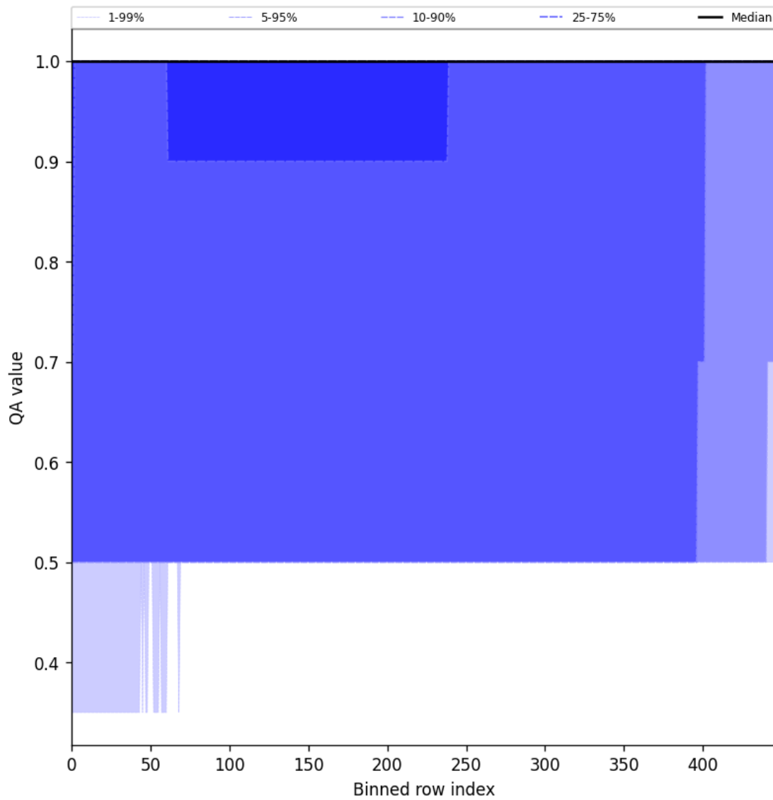
Figure 44: Along track statistics of “QA value” for 2024-12-25 to 2024-12-25
