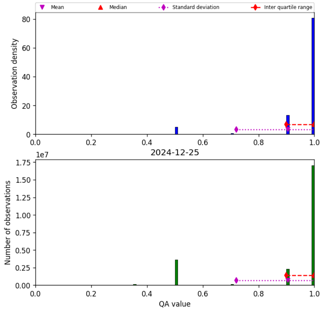
Figure 27: Histogram of “QA value” for 2024-12-25 to 2024-12-25
