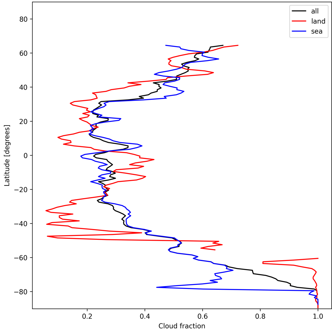
Figure 13: Zonal average of “Cloud fraction” for 2024-12-25 to 2024-12-25.
