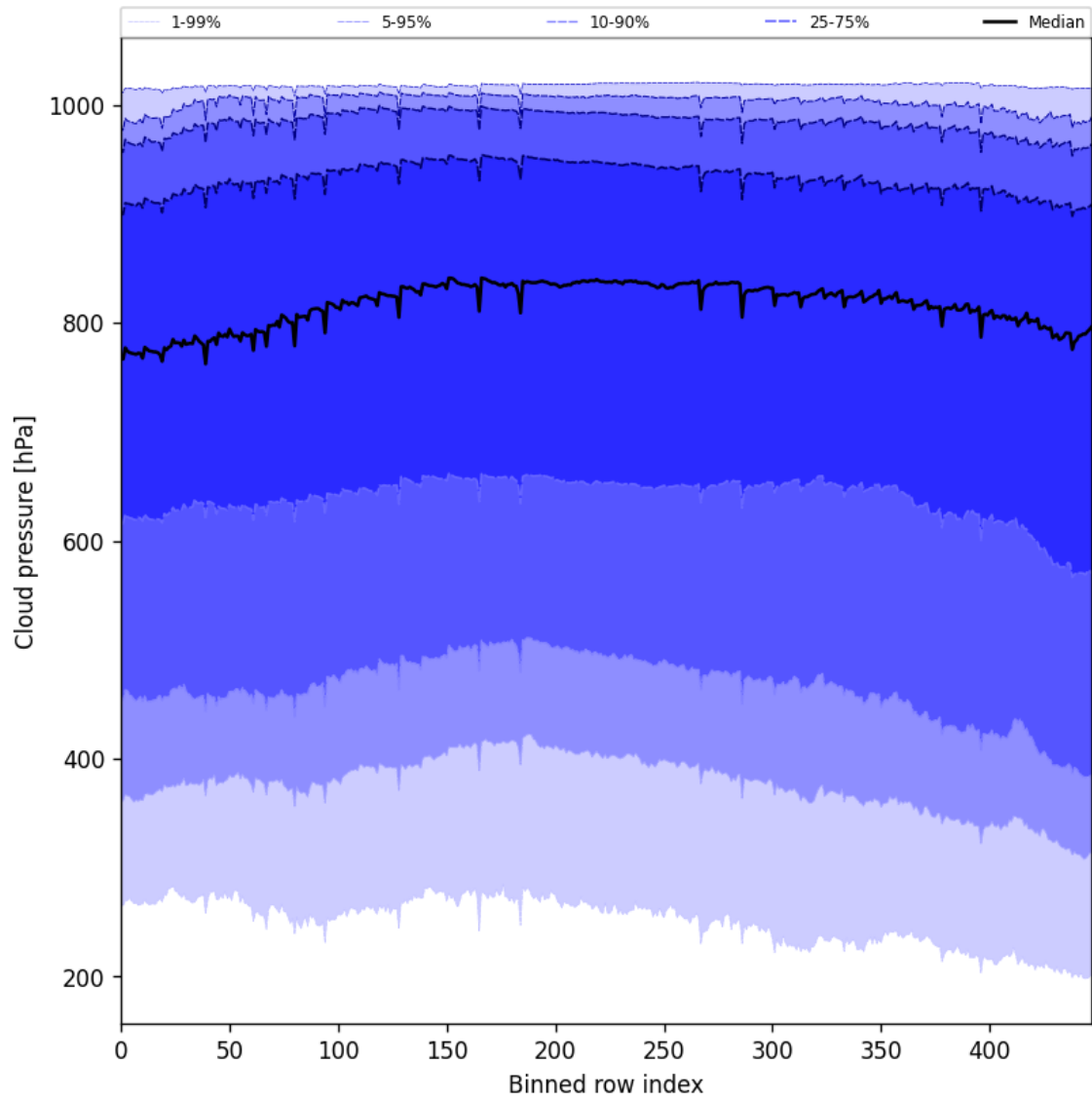
Figure 45: Along track statistics of “Cloud pressure” for 2024-12-25 to 2024-12-25
