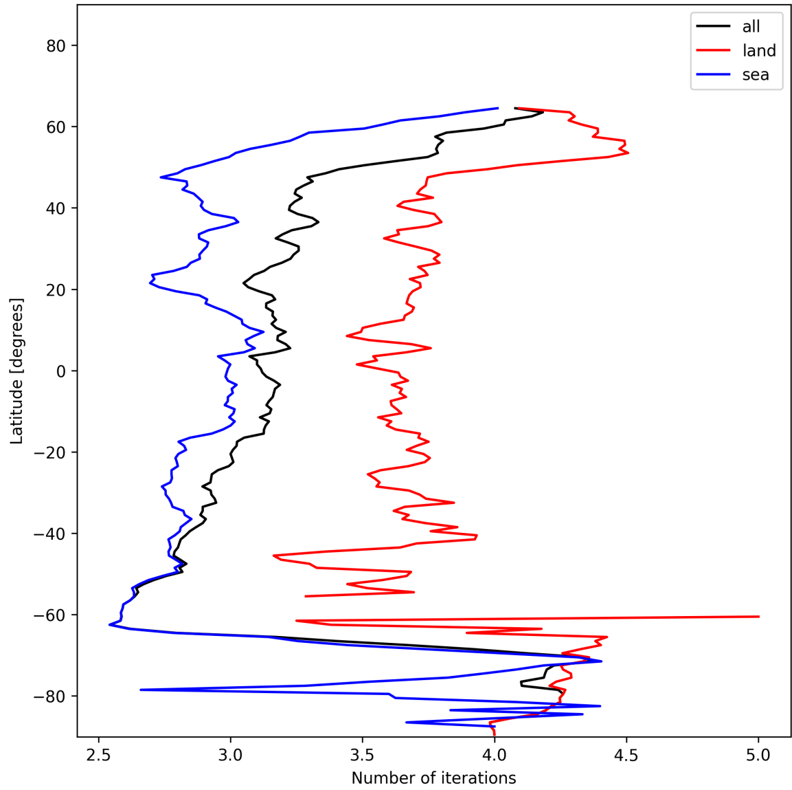
Figure 20: Zonal average of “Number of iterations” for 2024-12-25 to 2024-12-25.
