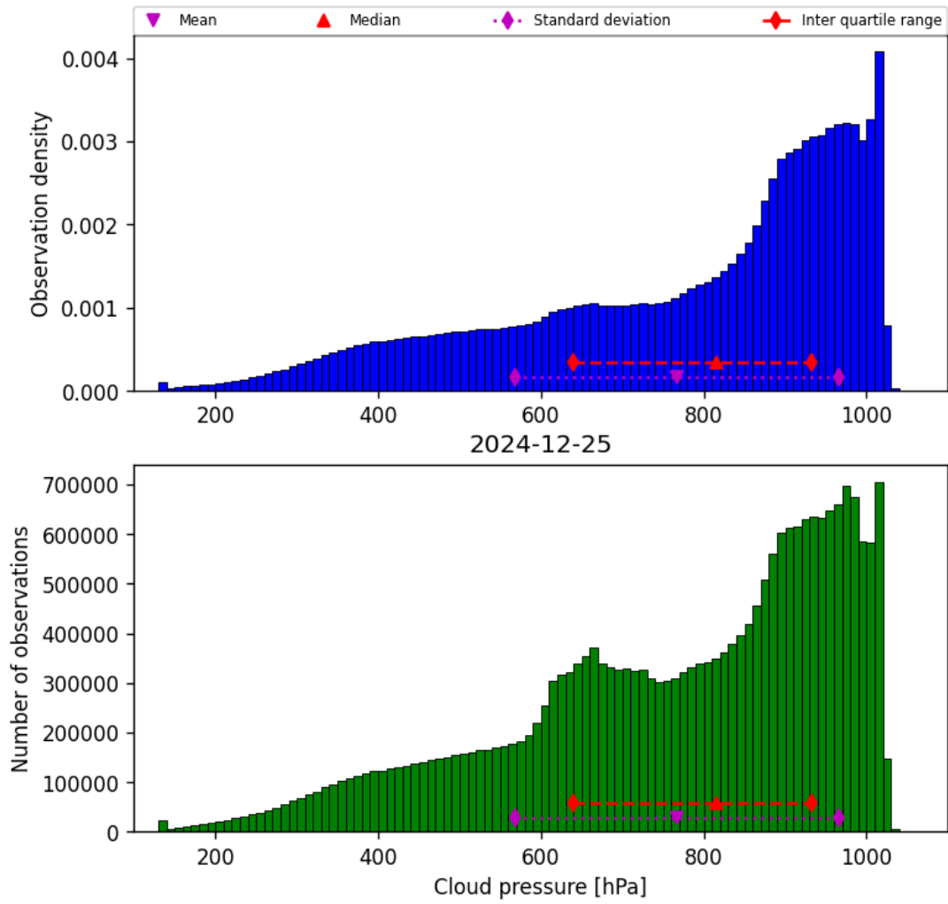
Figure 28: Histogram of “Cloud pressure” for 2024-12-25 to 2024-12-25
