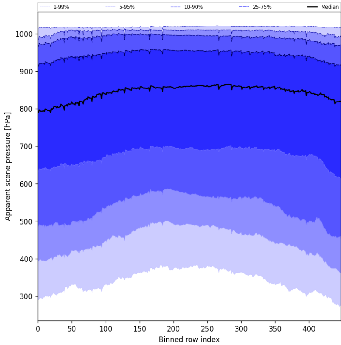
Figure 51: Along track statistics of “Apparent scene pressure” for 2024-12-25 to 2024-12-25
