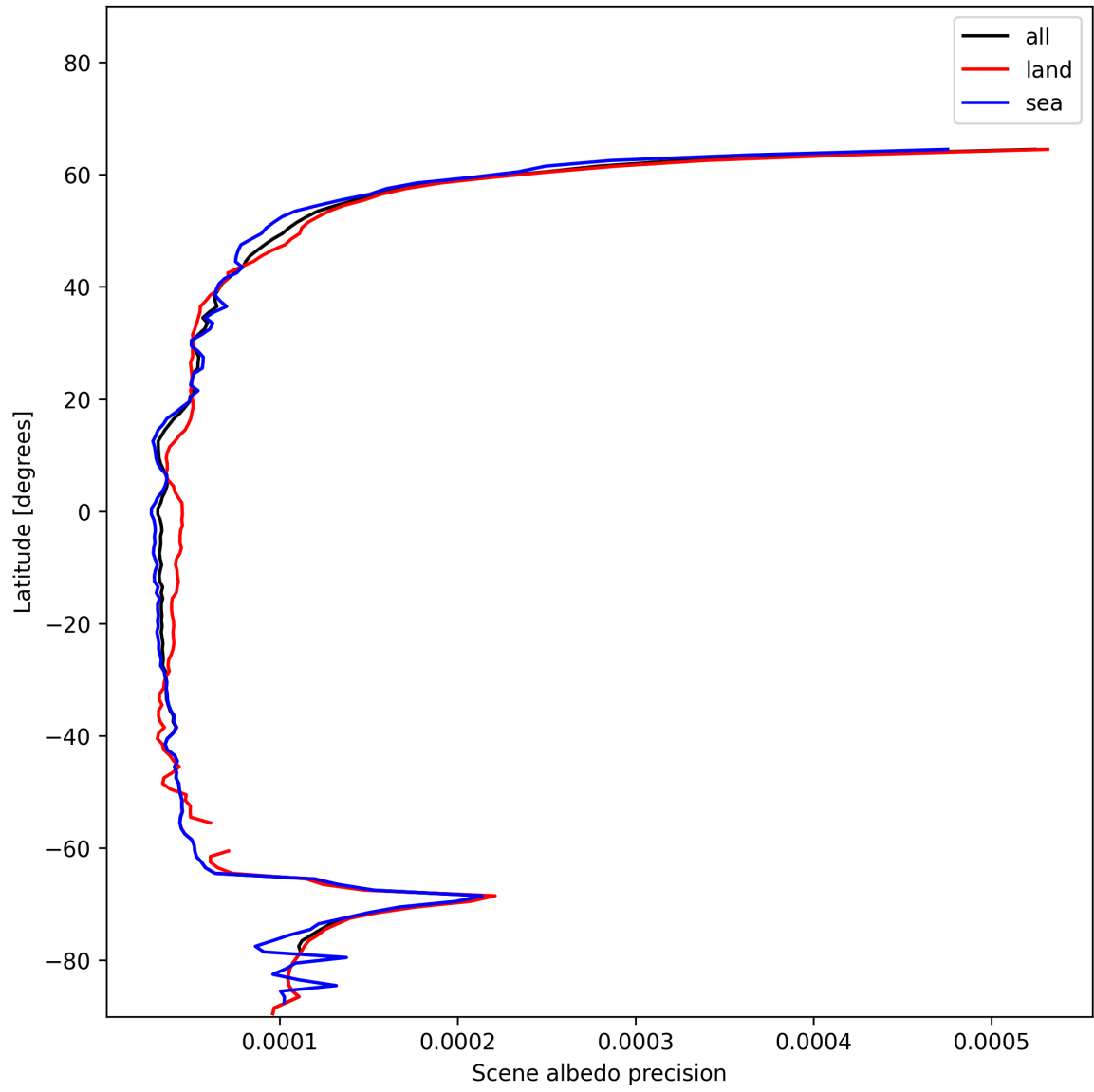
Figure 16: Zonal average of “Scene albedo precision” for 2024-12-25 to 2024-12-25.
