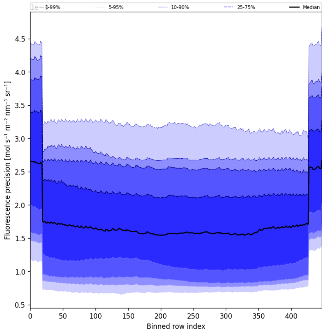
Figure 56: Along track statistics of “Fluorescence precision” for 2024-12-25 to 2024-12-25
