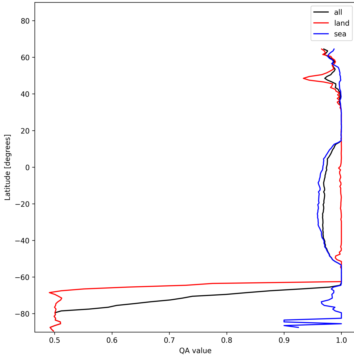
Figure 10: Zonal average of “QA value” for 2024-12-25 to 2024-12-25.
