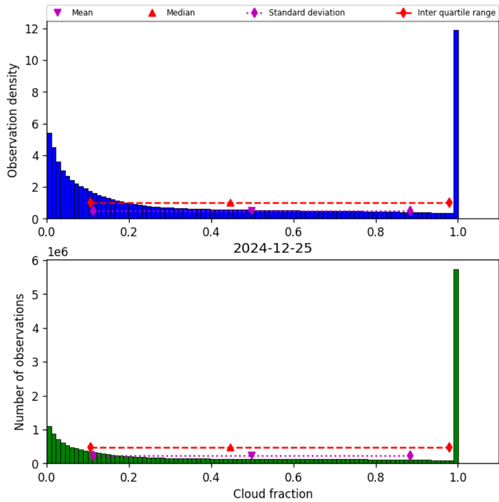
Figure 30: Histogram of “Cloud fraction” for 2024-12-25 to 2024-12-25
