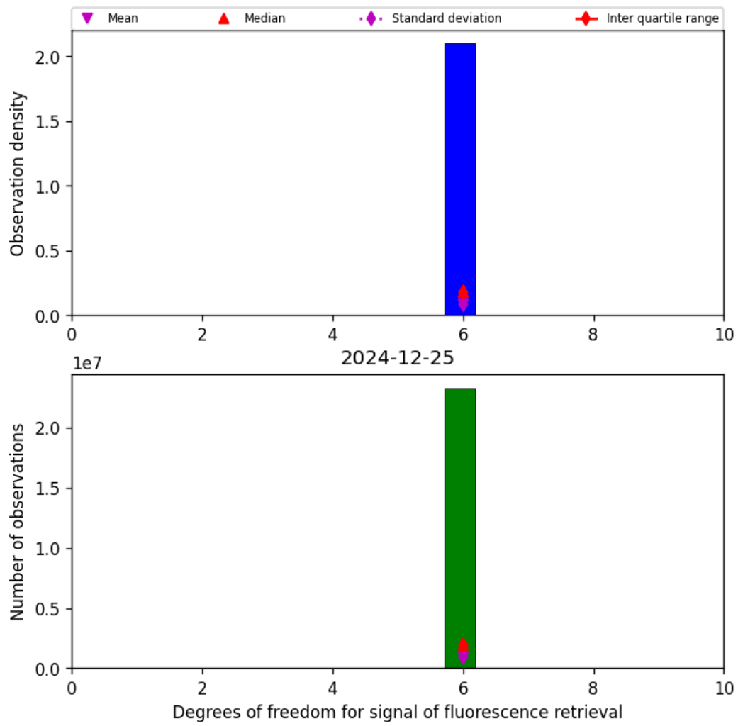
Figure 41: Histogram of “Degrees of freedom for signal of fluorescence retrieval” for 2024-12-25 to 2024-12-25
