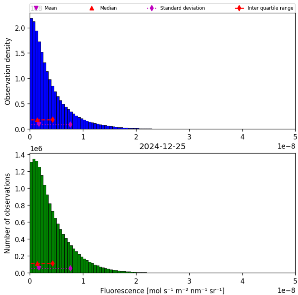
Figure 38: Histogram of “Fluorescence” for 2024-12-25 to 2024-12-25
