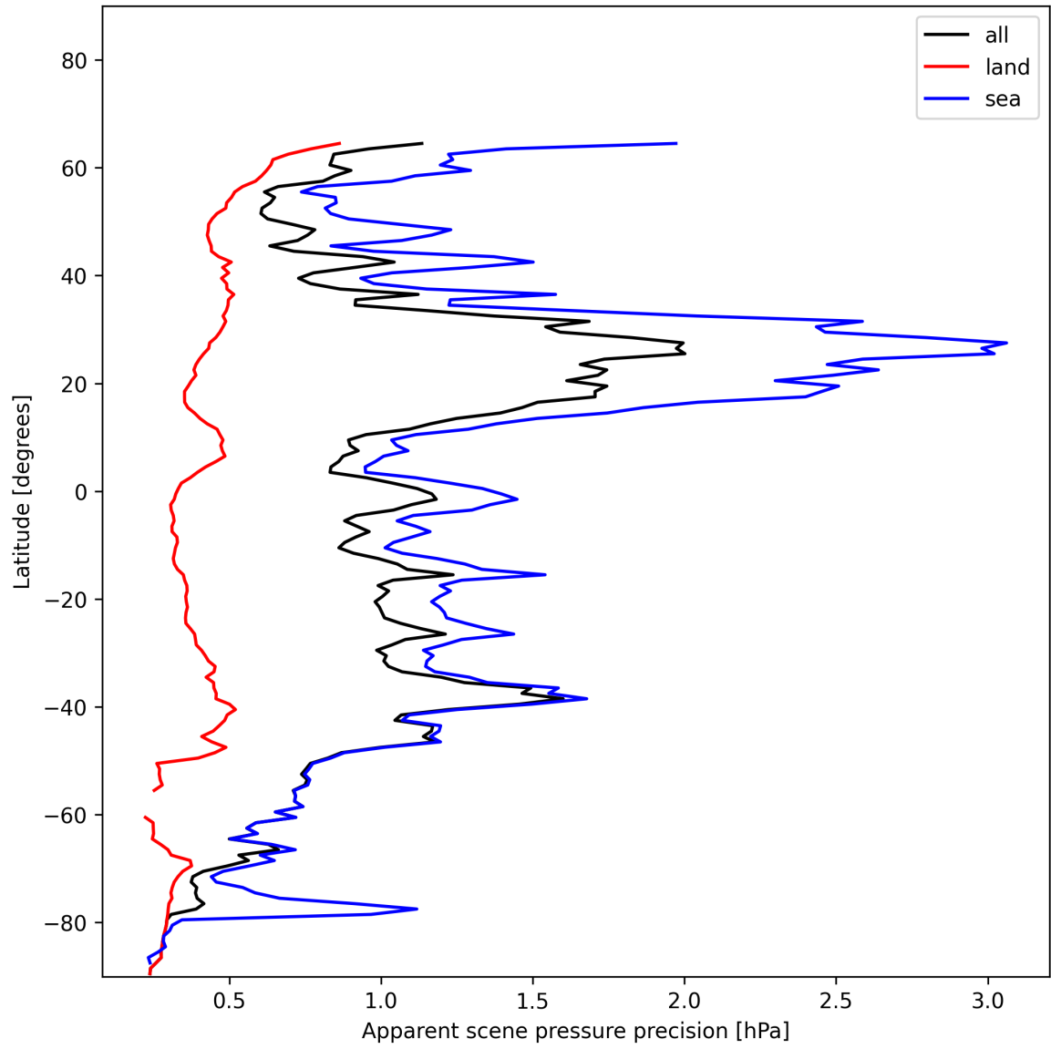
Figure 18: Zonal average of “Apparent scene pressure precision” for 2024-12-25 to 2024-12-25.
