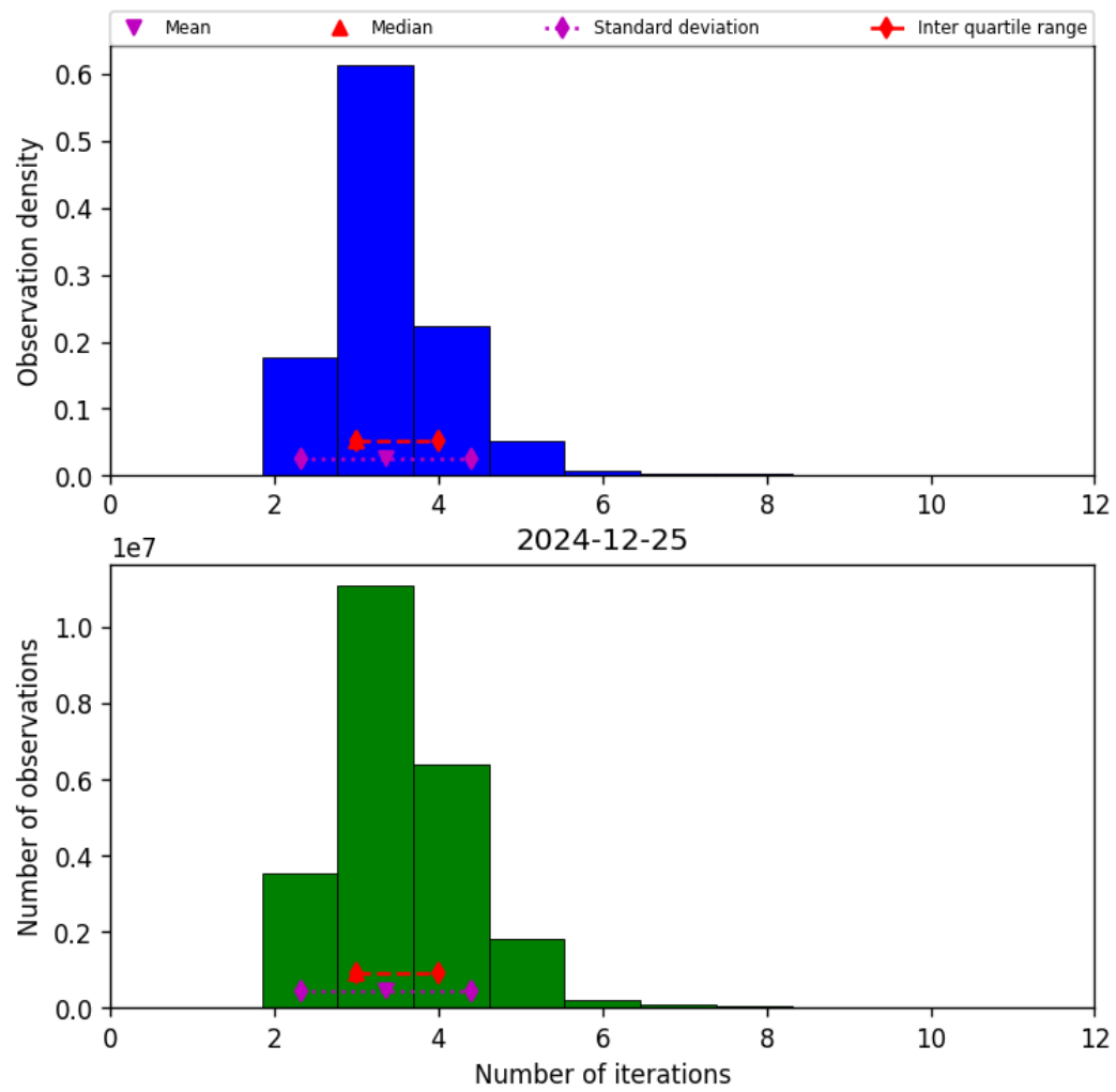
Figure 37: Histogram of “Number of iterations” for 2024-12-25 to 2024-12-25
