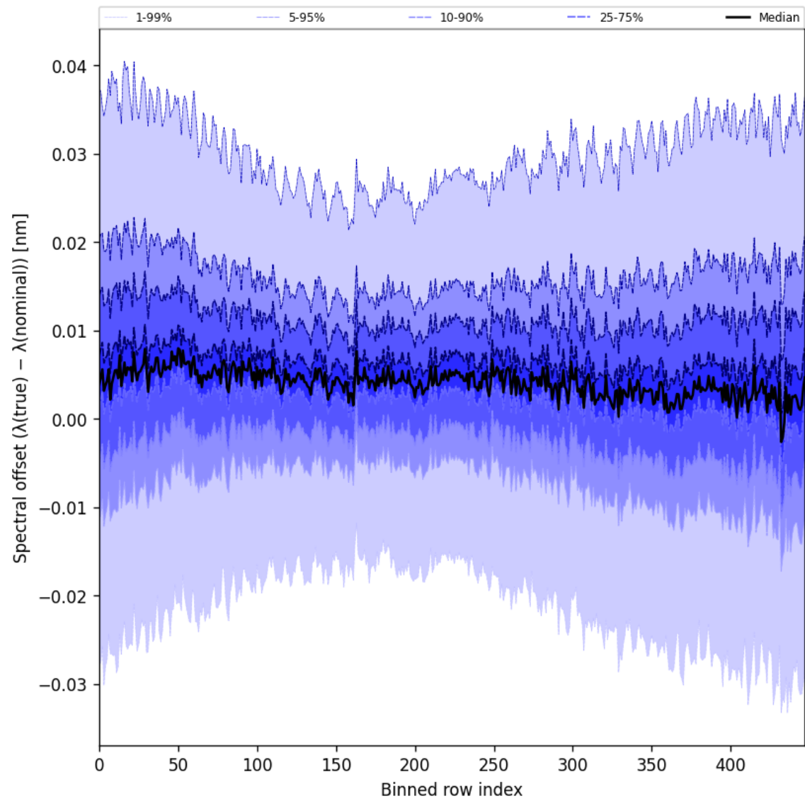
Figure 60: Along track statistics of “Spectral offset ( \lambda_{\text{true}} - \lambda_{\text{nominal}} )” for 2024-12-25 to 2024-12-25
