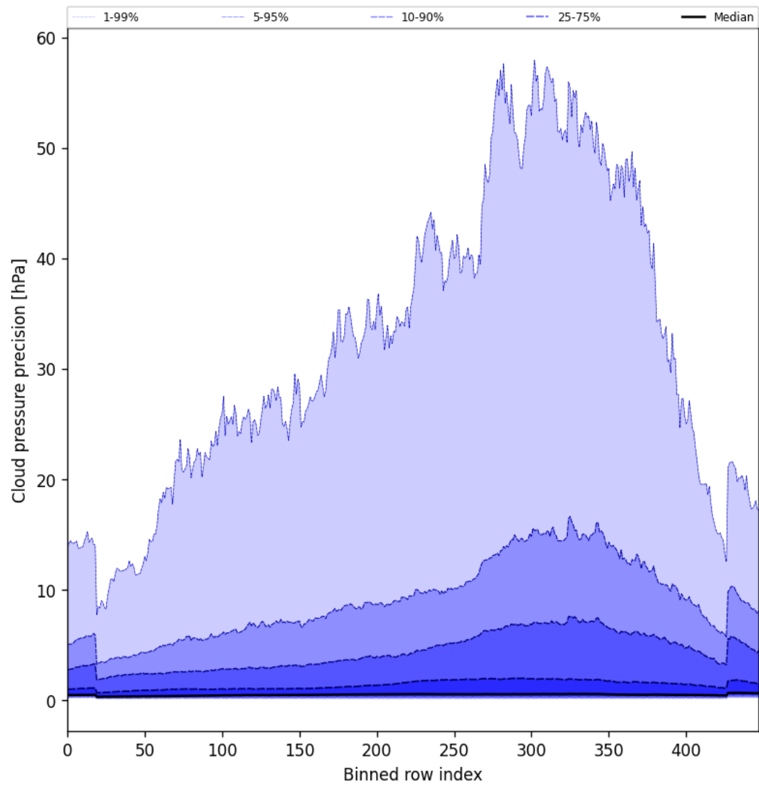
Figure 46: Along track statistics of “Cloud pressure precision” for 2024-12-25 to 2024-12-25
