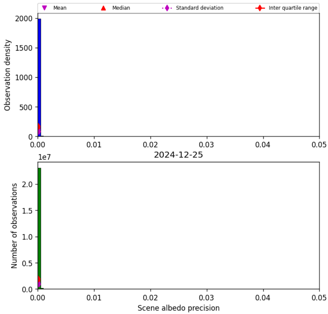
Figure 33: Histogram of “Scene albedo precision” for 2024-12-25 to 2024-12-25
