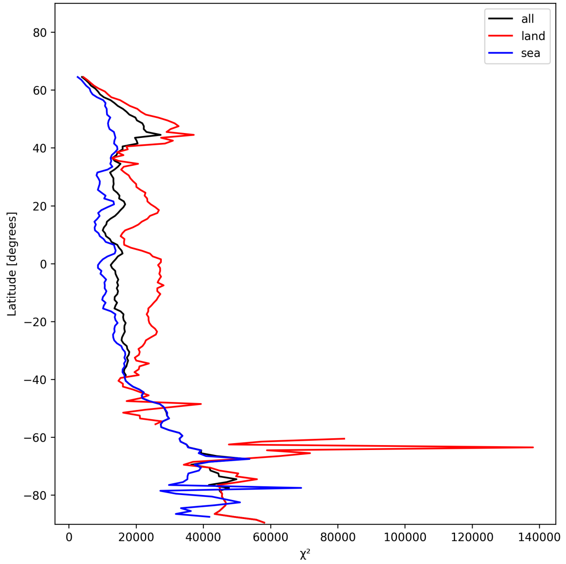
Figure 19: Zonal average of “ \chi^2 ” for 2024-12-25 to 2024-12-25.
