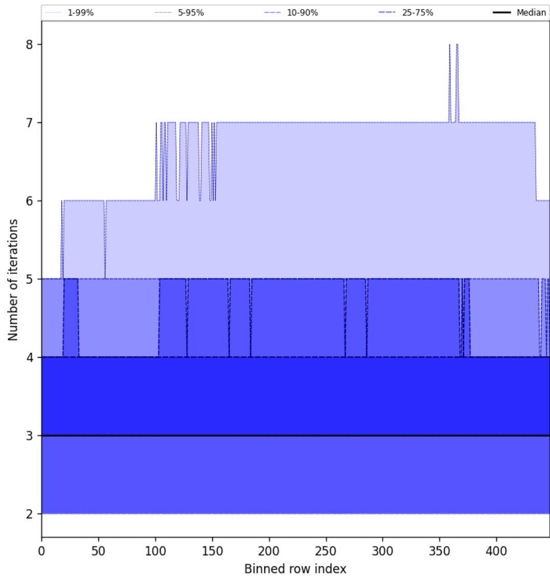
Figure 54: Along track statistics of “Number of iterations” for 2024-12-28 to 2024-12-29
