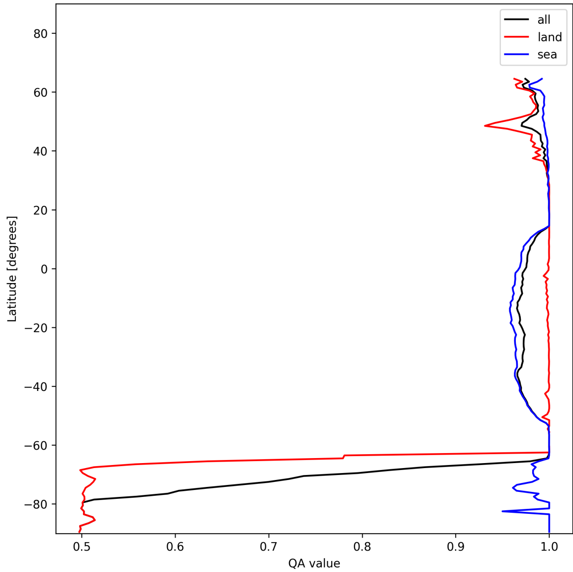
Figure 10: Zonal average of “QA value” for 2024-12-28 to 2024-12-29.
