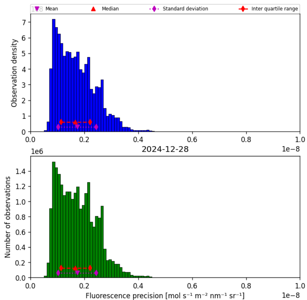
Figure 39: Histogram of “Fluorescence precision” for 2024-12-28 to 2024-12-29
