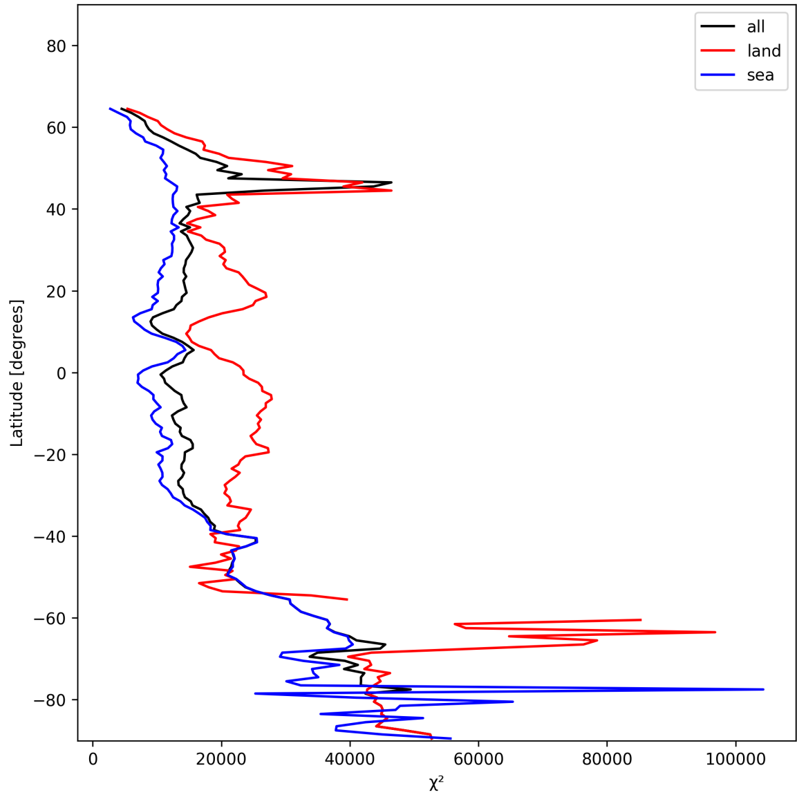
Figure 19: Zonal average of “ \chi^2 ” for 2024-12-28 to 2024-12-29.
