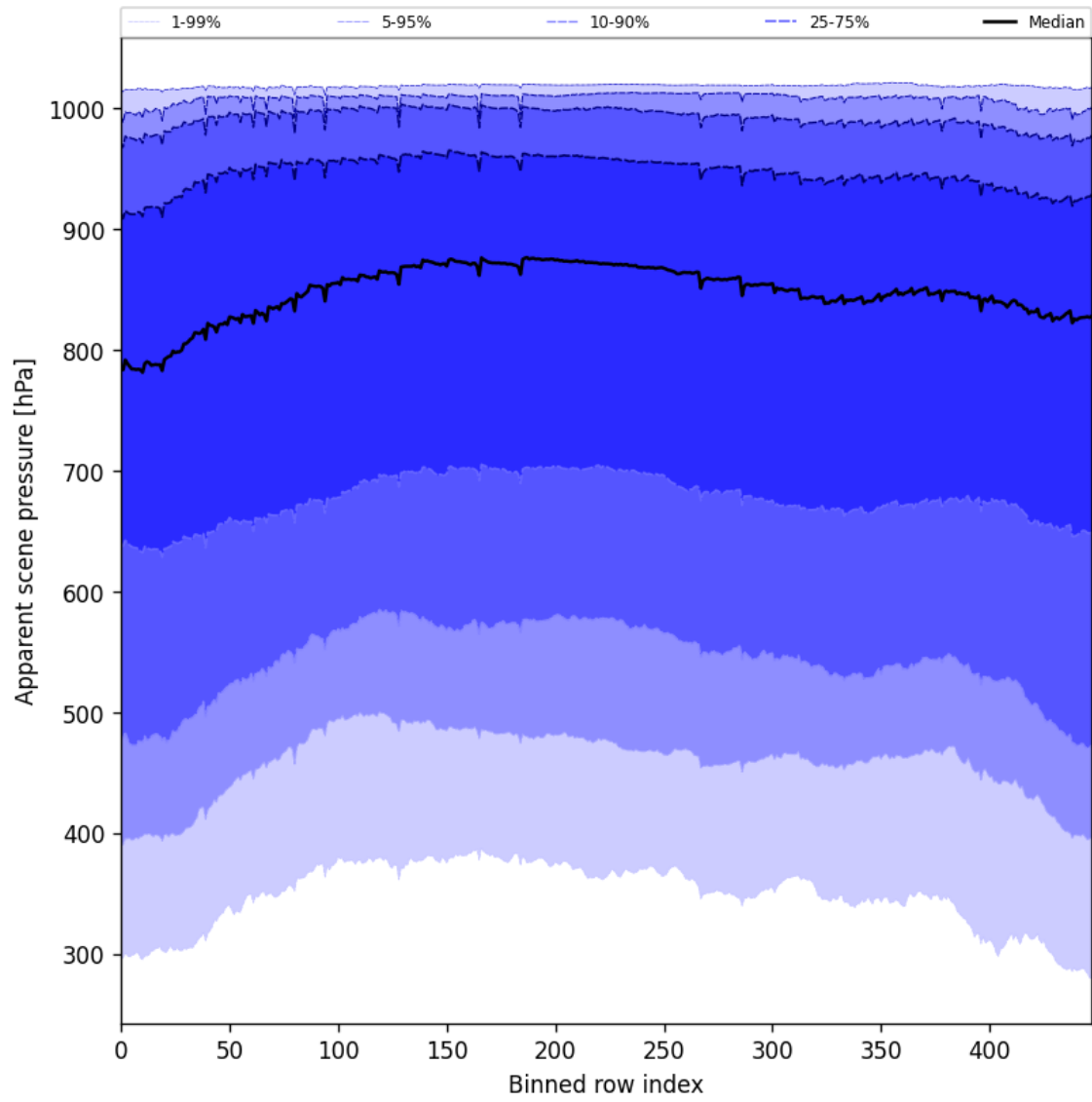
Figure 51: Along track statistics of “Apparent scene pressure” for 2024-12-28 to 2024-12-29
