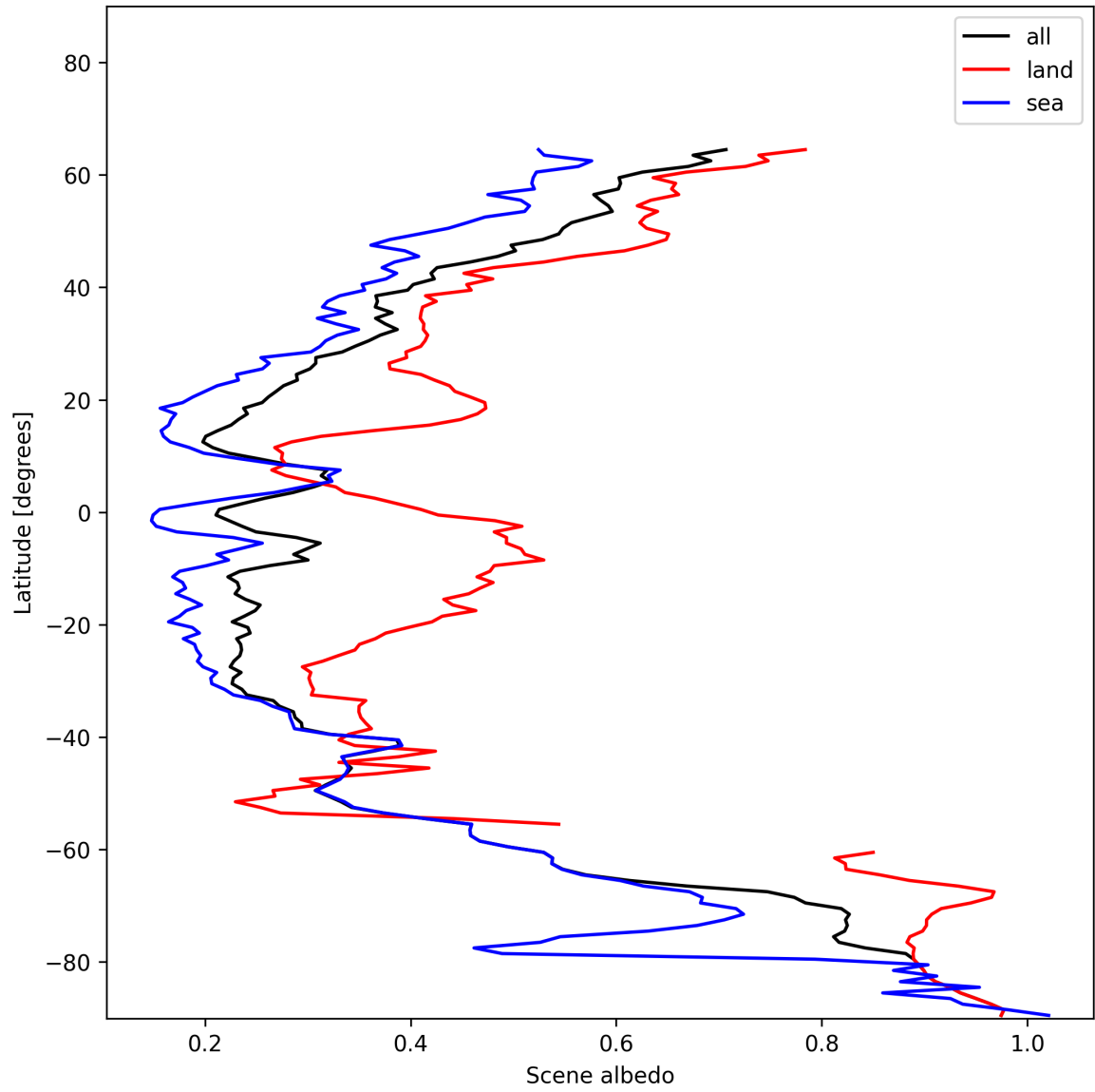
Figure 15: Zonal average of “Scene albedo” for 2024-12-28 to 2024-12-29.
