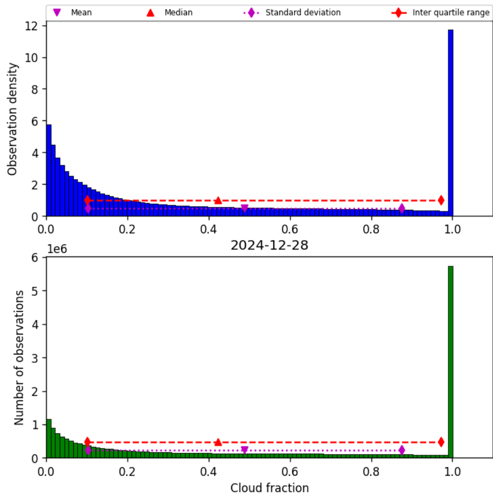
Figure 30: Histogram of “Cloud fraction” for 2024-12-28 to 2024-12-29
