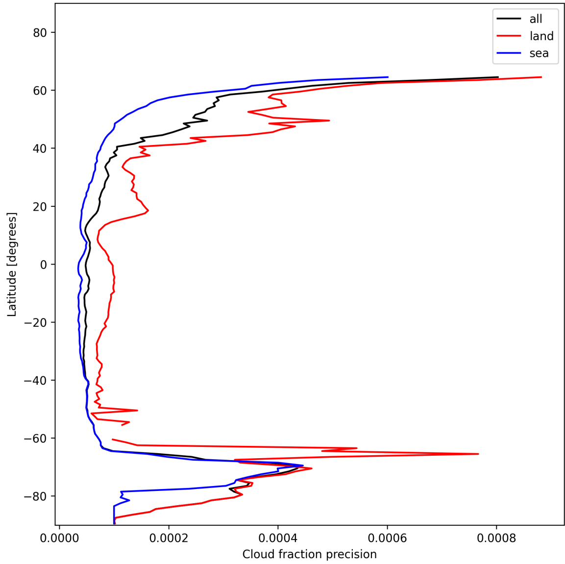
Figure 14: Zonal average of “Cloud fraction precision” for 2024-12-28 to 2024-12-29.
