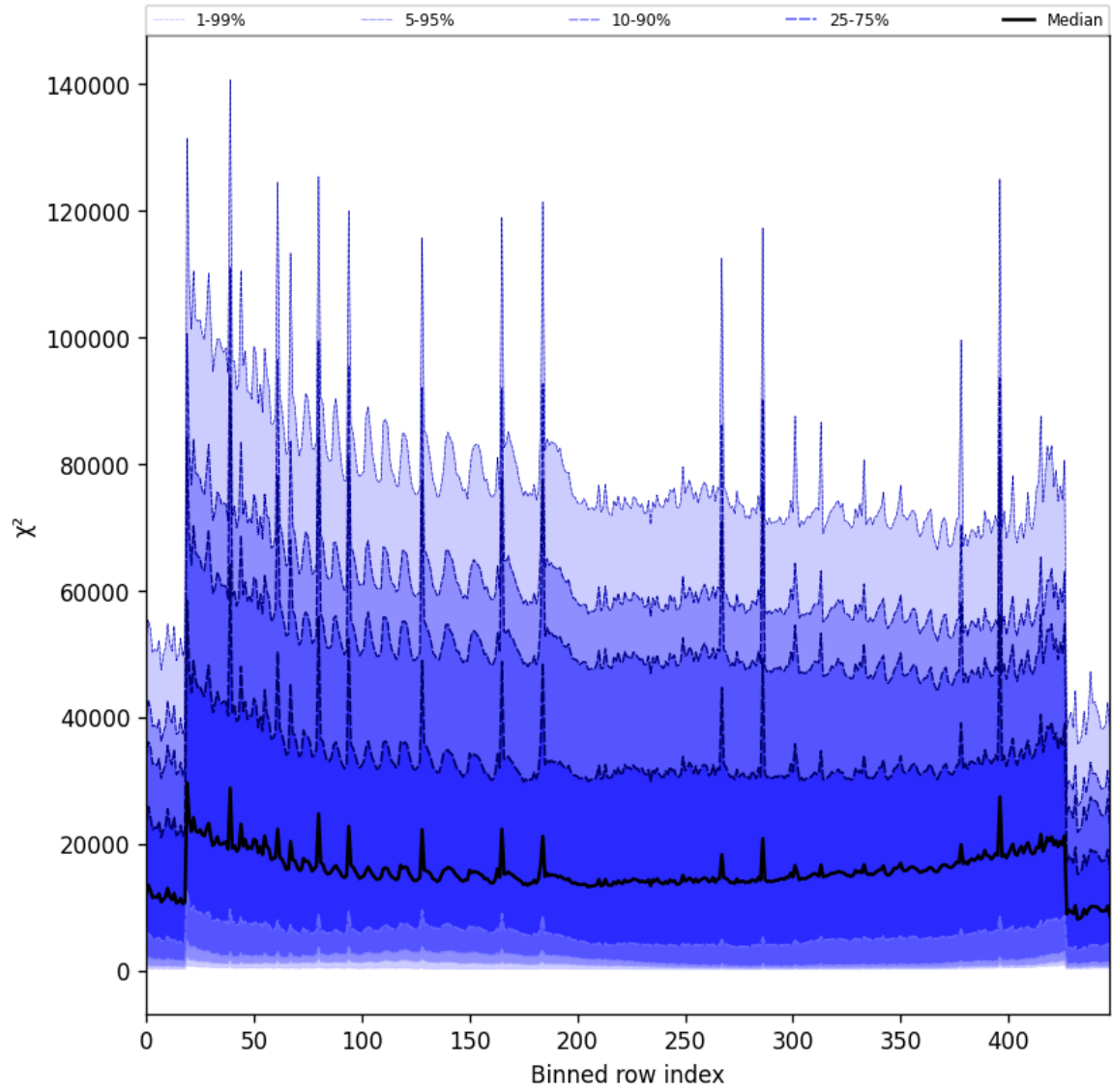
Figure 53: Along track statistics of “ \chi^2 ” for 2024-12-28 to 2024-12-29
