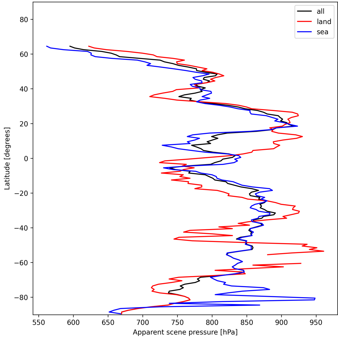
Figure 17: Zonal average of “Apparent scene pressure” for 2024-12-28 to 2024-12-29.
