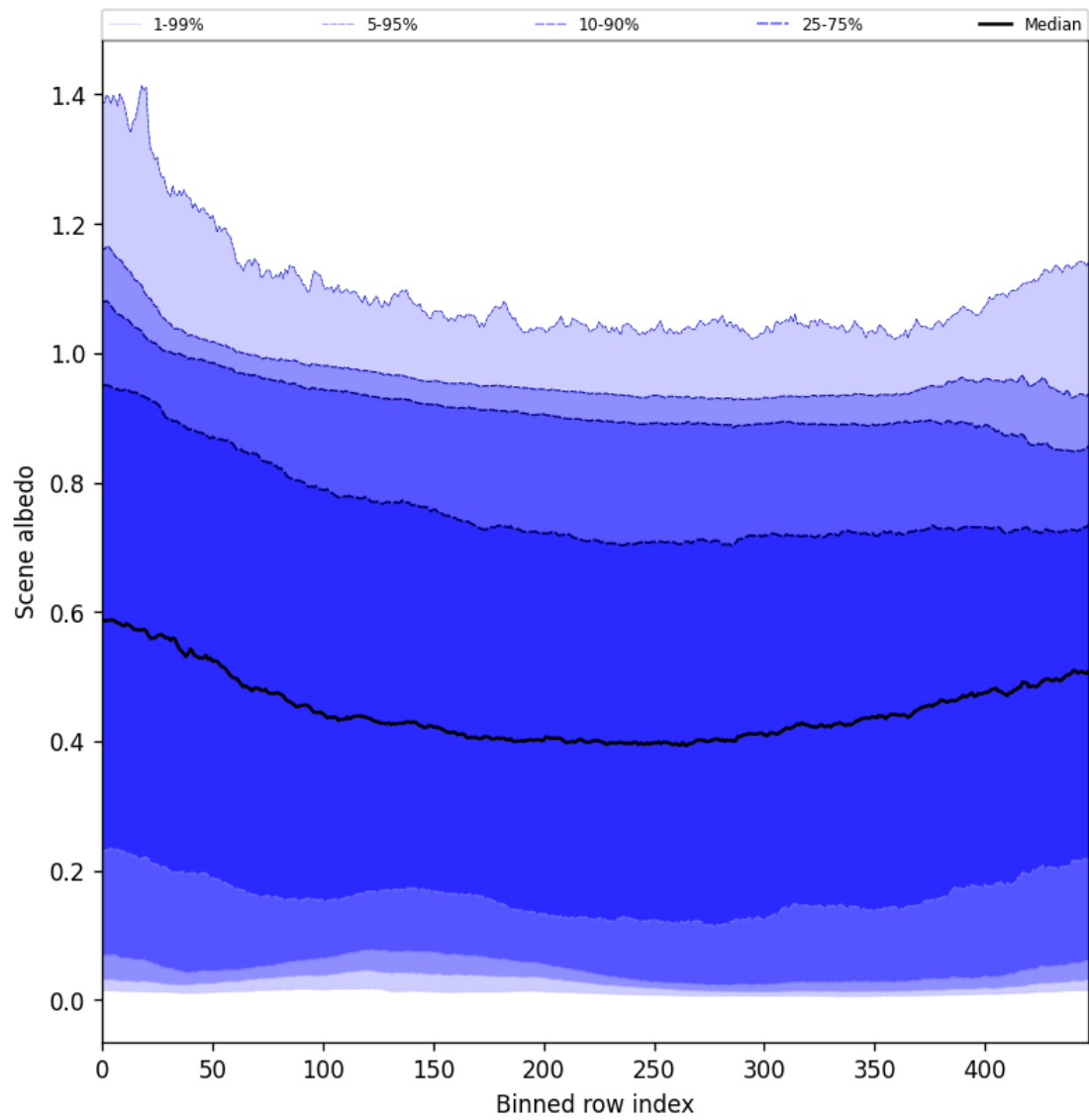
Figure 49: Along track statistics of “Scene albedo” for 2024-12-28 to 2024-12-29
