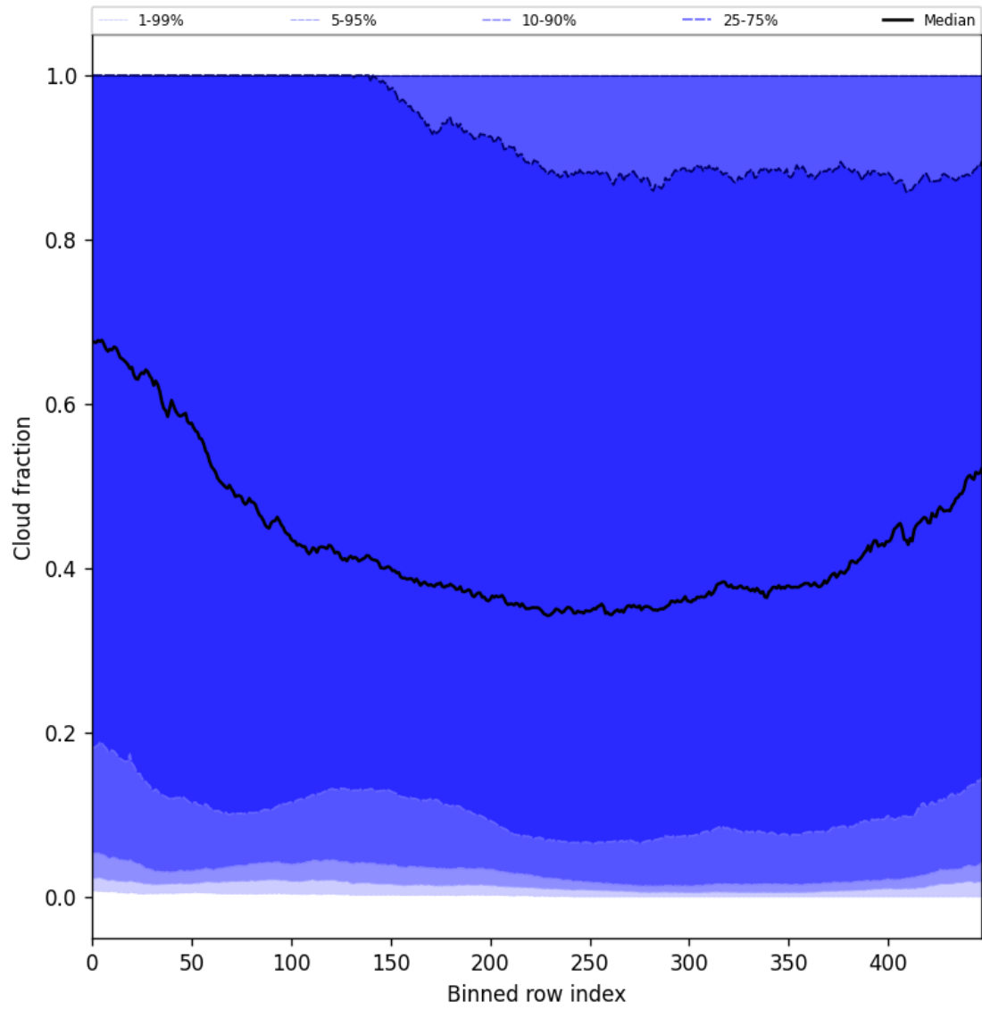
Figure 47: Along track statistics of “Cloud fraction” for 2024-12-28 to 2024-12-29
