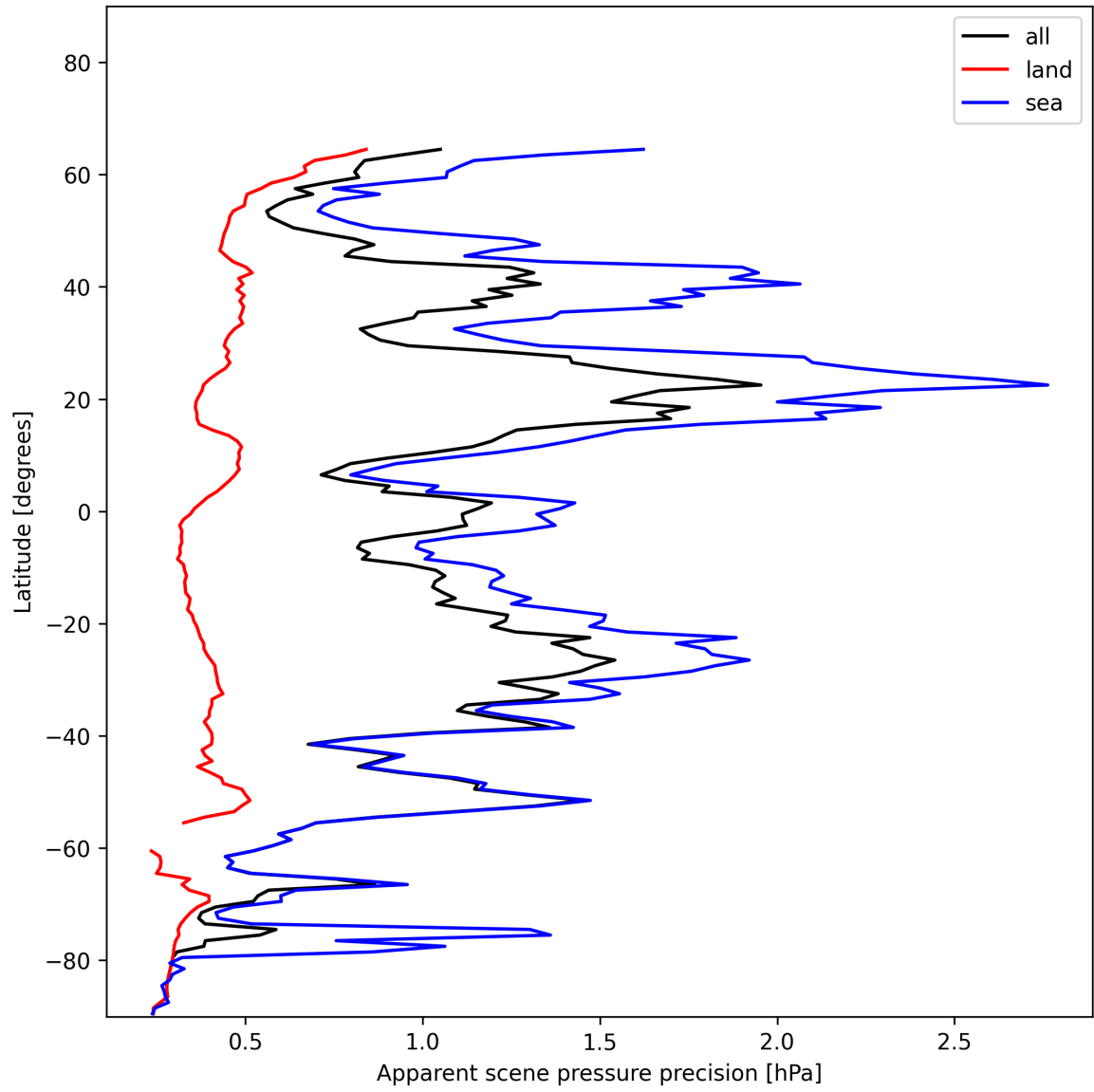
Figure 18: Zonal average of “Apparent scene pressure precision” for 2024-12-28 to 2024-12-29.
