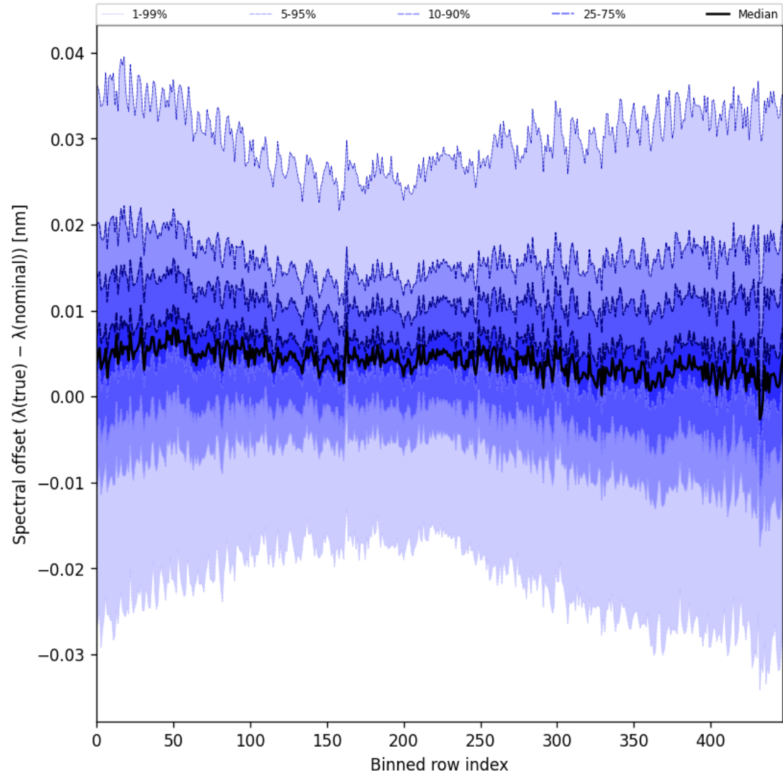
Figure 60: Along track statistics of “Spectral offset ( \lambda_{\text{true}} - \lambda_{\text{nominal}} )” for 2024-12-28 to 2024-12-29
