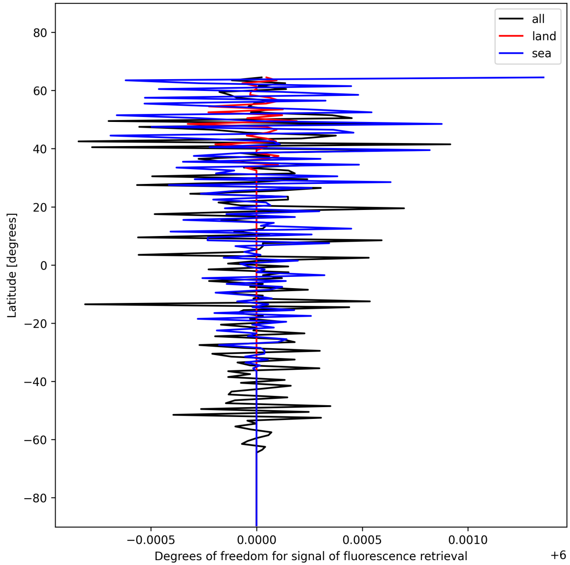
Figure 24: Zonal average of “Degrees of freedom for signal of fluorescence retrieval” for 2024-12-28 to 2024-12-29.
