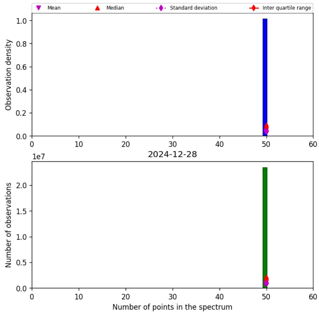
Figure 42: Histogram of “Number of points in the spectrum” for 2024-12-28 to 2024-12-29
