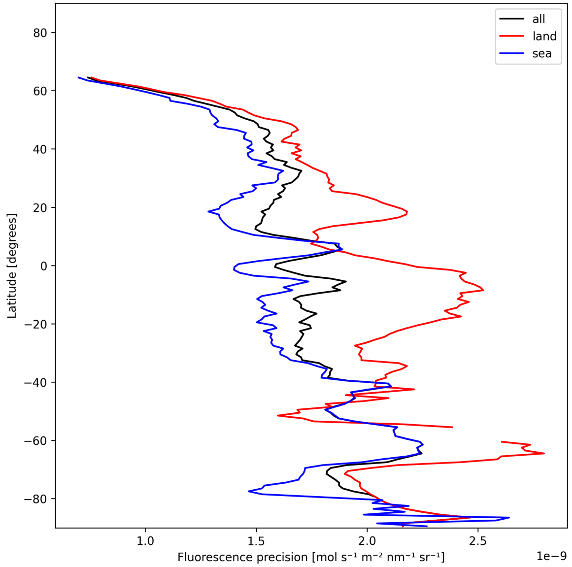
Figure 22: Zonal average of “Fluorescence precision” for 2024-12-28 to 2024-12-29.
