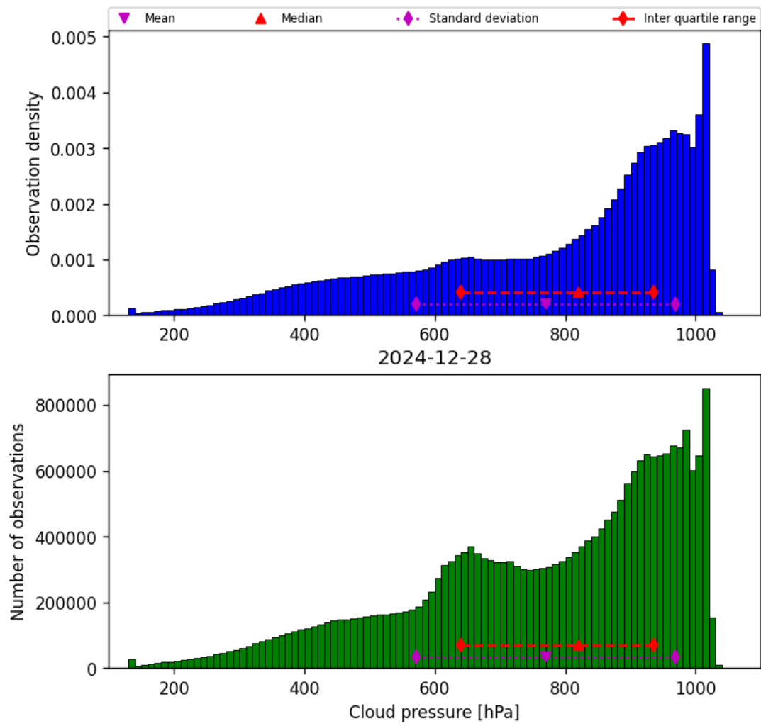
Figure 28: Histogram of “Cloud pressure” for 2024-12-28 to 2024-12-29
