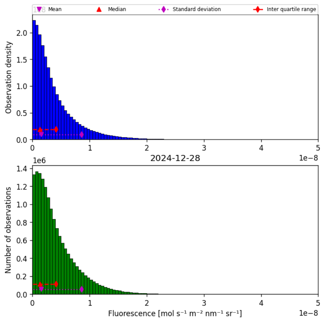
Figure 38: Histogram of “Fluorescence” for 2024-12-28 to 2024-12-29
