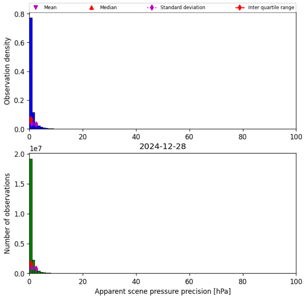
Figure 35: Histogram of “Apparent scene pressure precision” for 2024-12-28 to 2024-12-29
