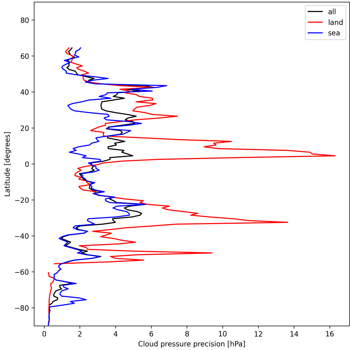
Figure 12: Zonal average of “Cloud pressure precision” for 2024-12-28 to 2024-12-29.
