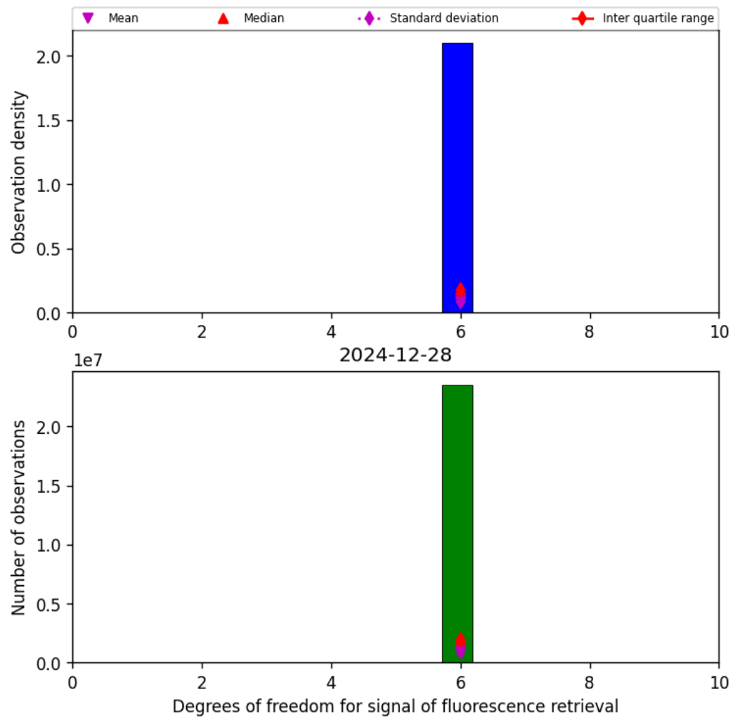
Figure 41: Histogram of “Degrees of freedom for signal of fluorescence retrieval” for 2024-12-28 to 2024-12-29
