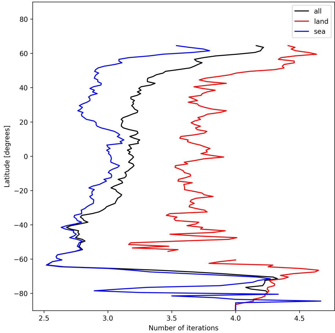
Figure 20: Zonal average of “Number of iterations” for 2024-12-28 to 2024-12-29.
