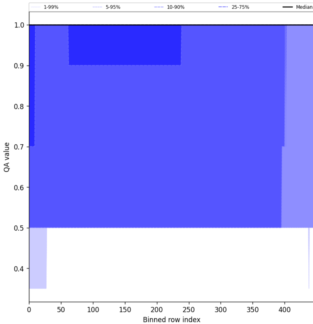
Figure 44: Along track statistics of “QA value” for 2024-12-28 to 2024-12-29
