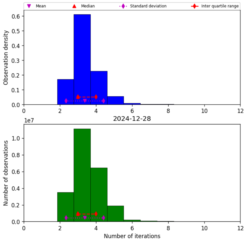
Figure 37: Histogram of “Number of iterations” for 2024-12-28 to 2024-12-29
