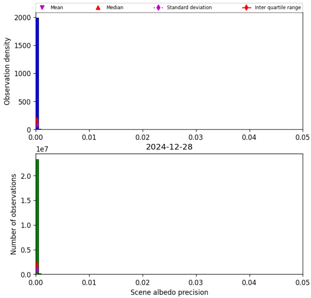
Figure 33: Histogram of “Scene albedo precision” for 2024-12-28 to 2024-12-29
