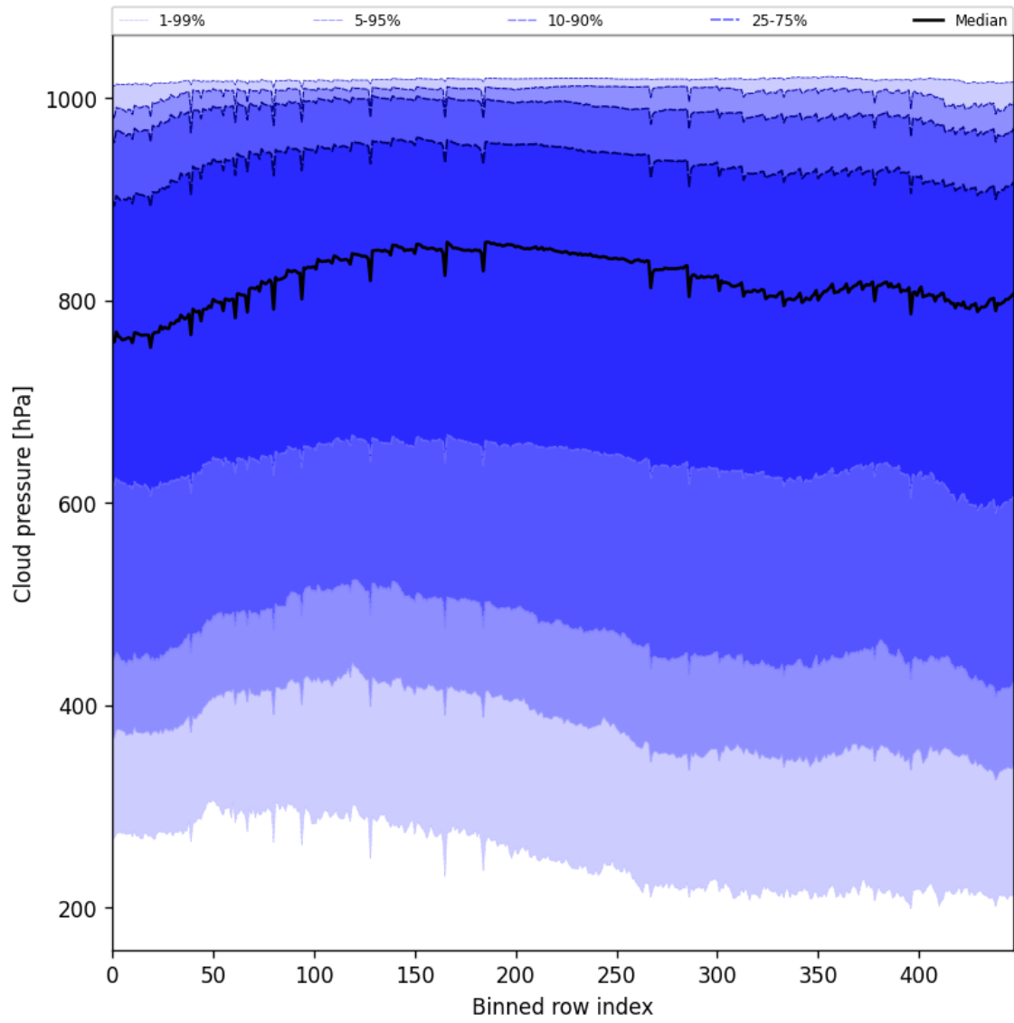
Figure 45: Along track statistics of “Cloud pressure” for 2024-12-28 to 2024-12-29
