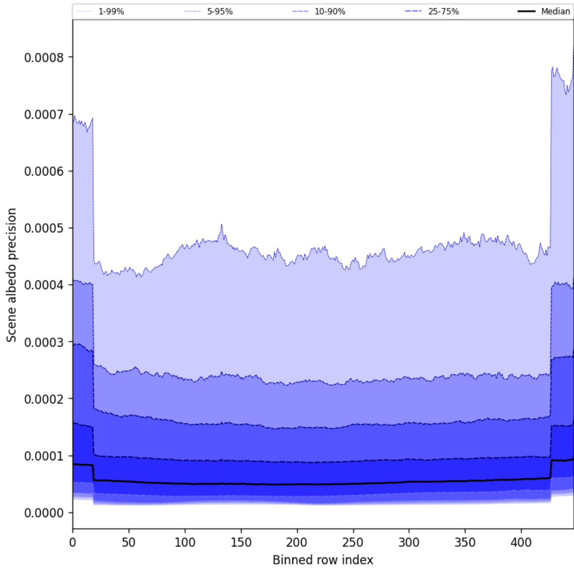
Figure 50: Along track statistics of “Scene albedo precision” for 2024-12-28 to 2024-12-29
