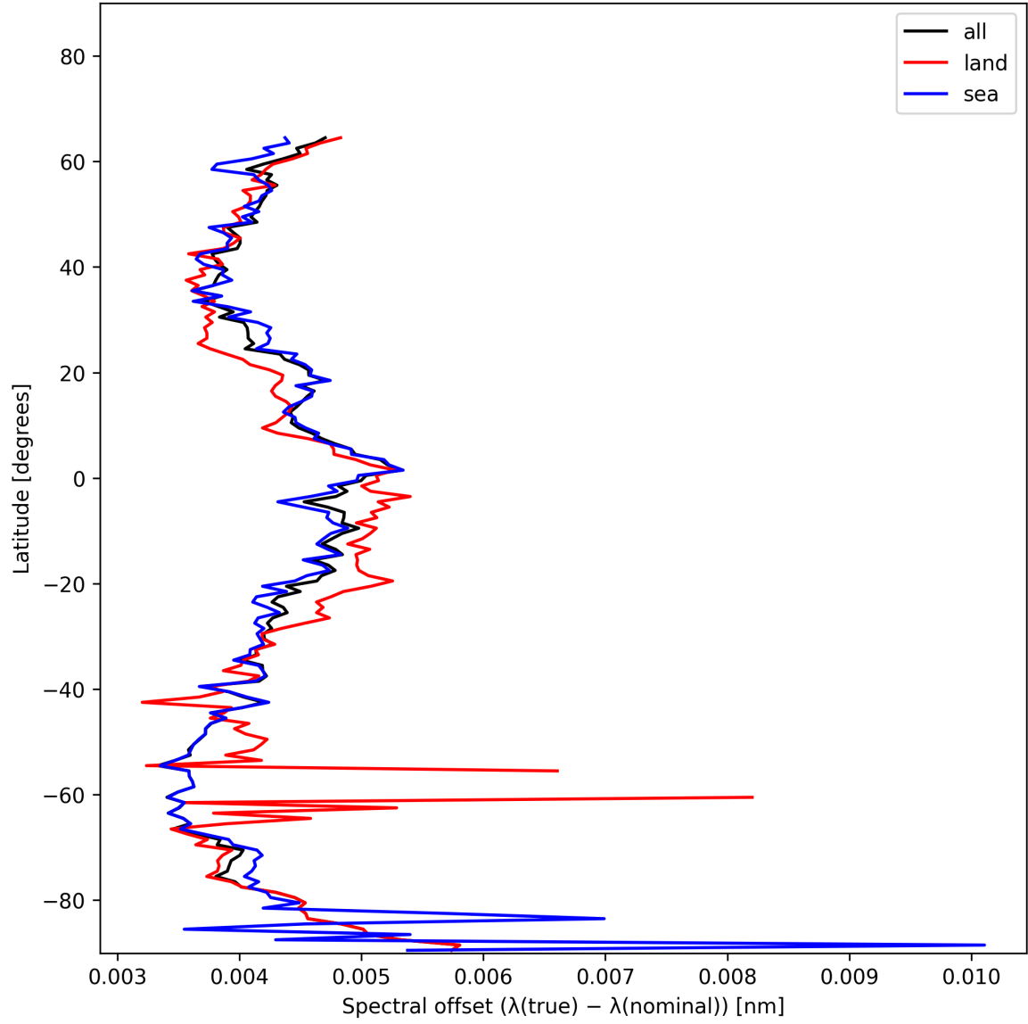
Figure 26: Zonal average of “Spectral offset ( \lambda_{\text{true}} - \lambda_{\text{nominal}} )” for 2024-12-28 to 2024-12-29.
