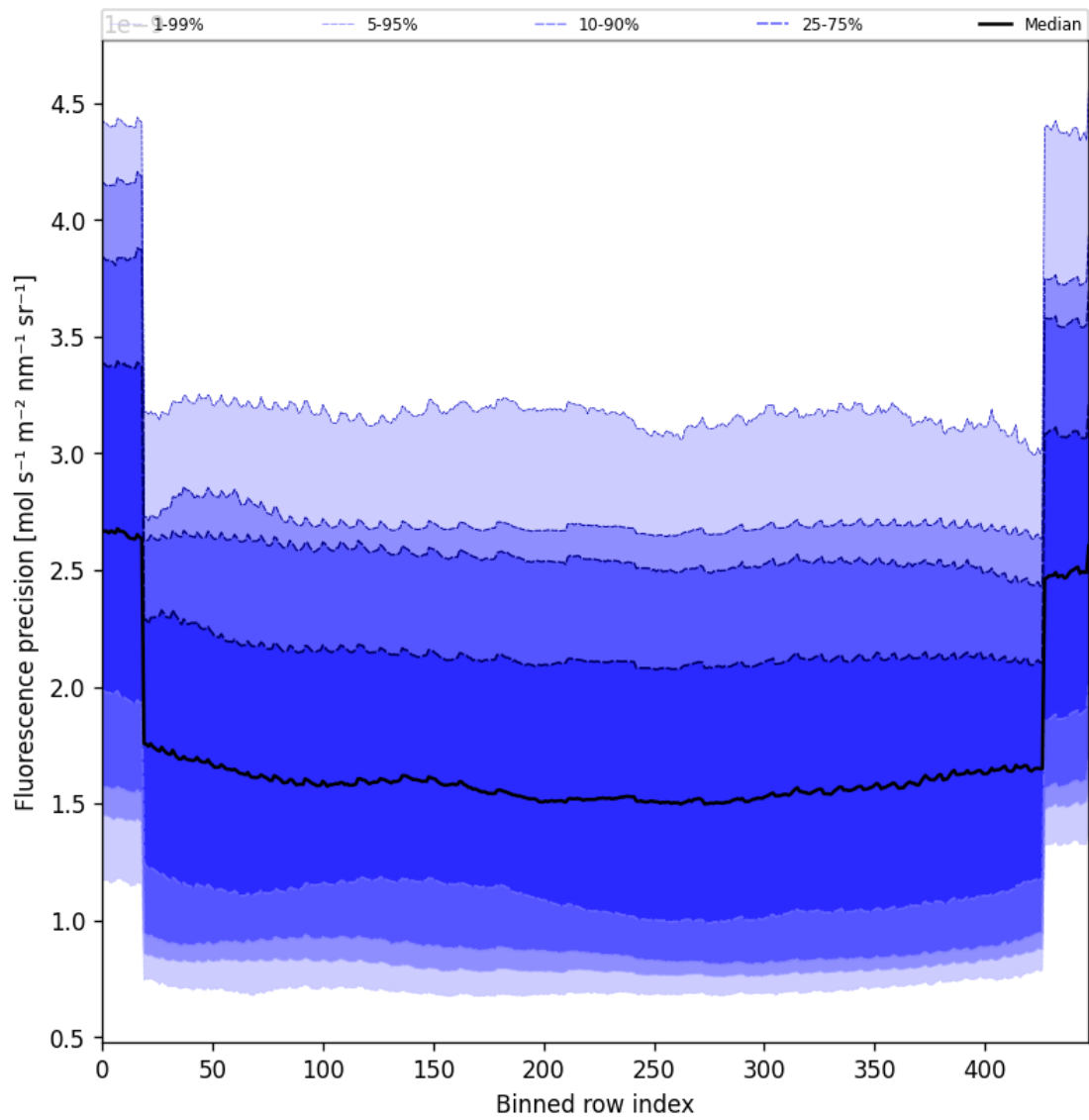
Figure 56: Along track statistics of “Fluorescence precision” for 2024-12-28 to 2024-12-29
