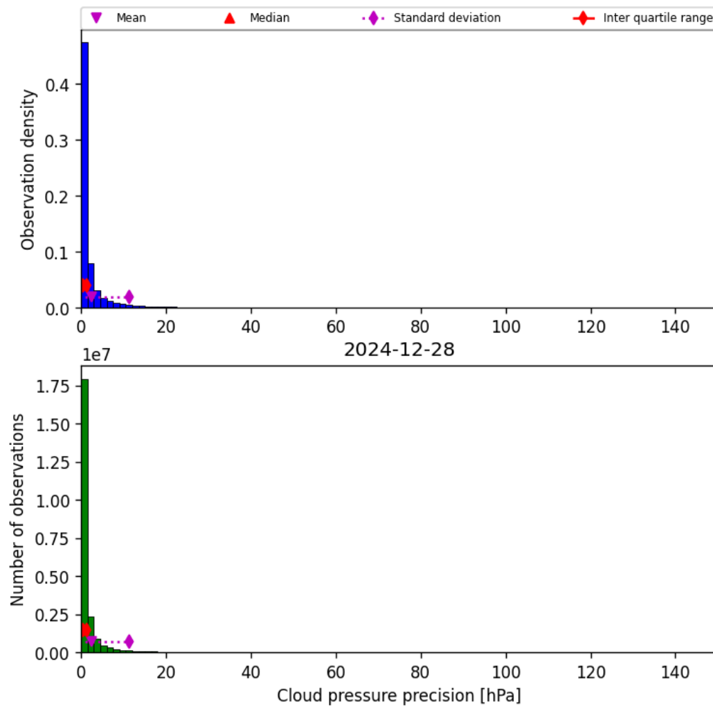
Figure 29: Histogram of “Cloud pressure precision” for 2024-12-28 to 2024-12-29
