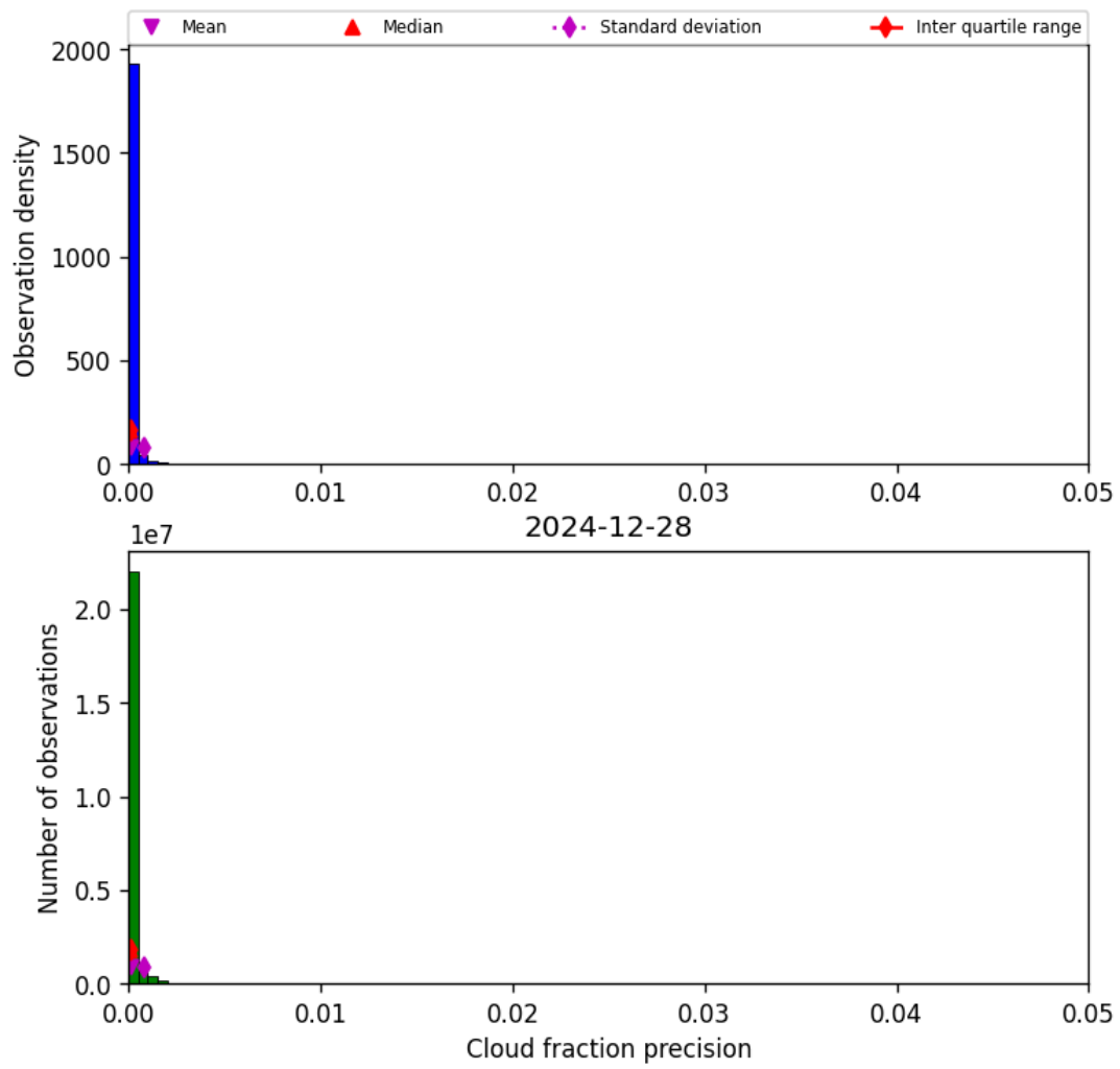
Figure 31: Histogram of “Cloud fraction precision” for 2024-12-28 to 2024-12-29
