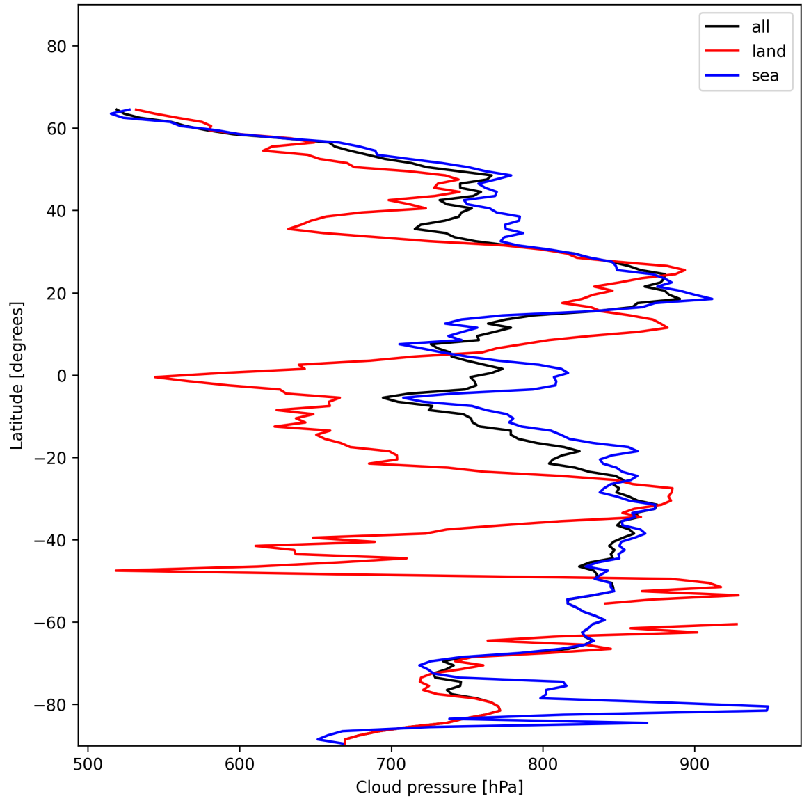
Figure 11: Zonal average of “Cloud pressure” for 2024-12-28 to 2024-12-29.
