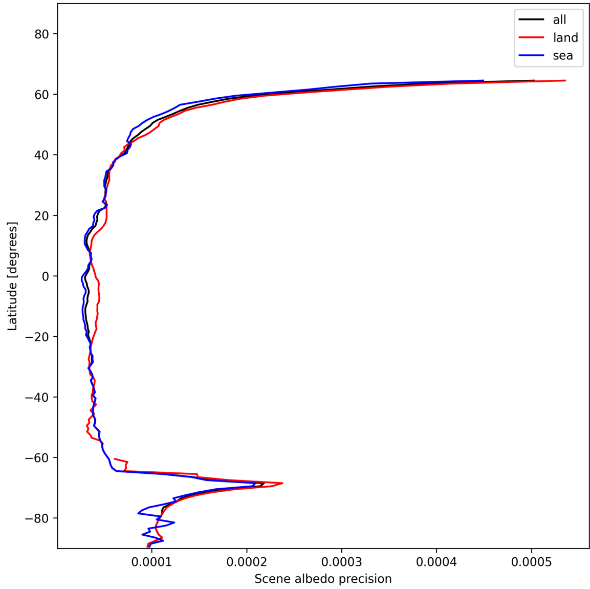
Figure 16: Zonal average of “Scene albedo precision” for 2024-12-28 to 2024-12-29.
