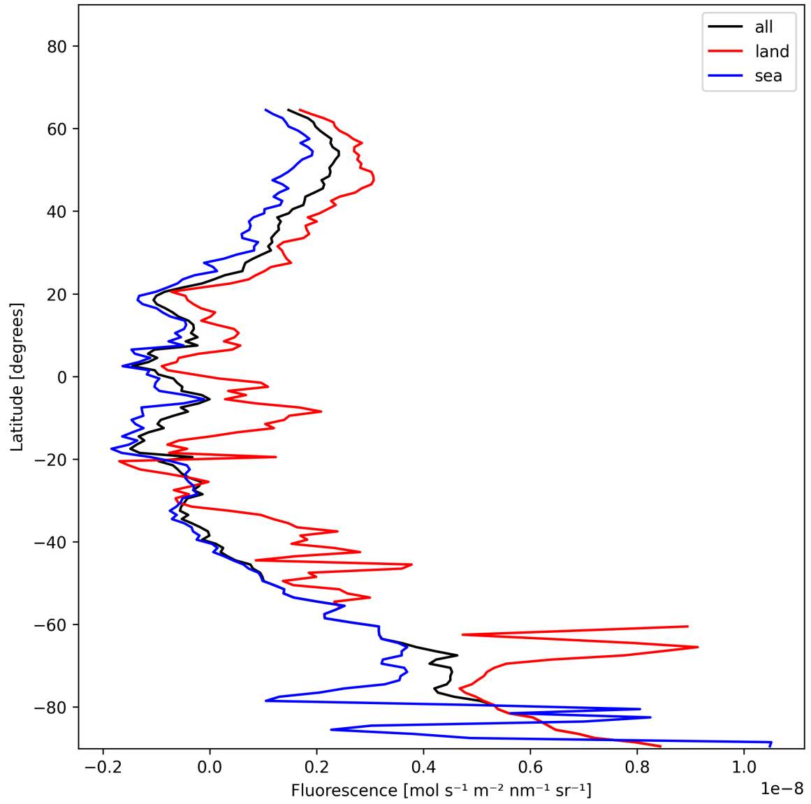
Figure 21: Zonal average of “Fluorescence” for 2024-12-28 to 2024-12-29.
