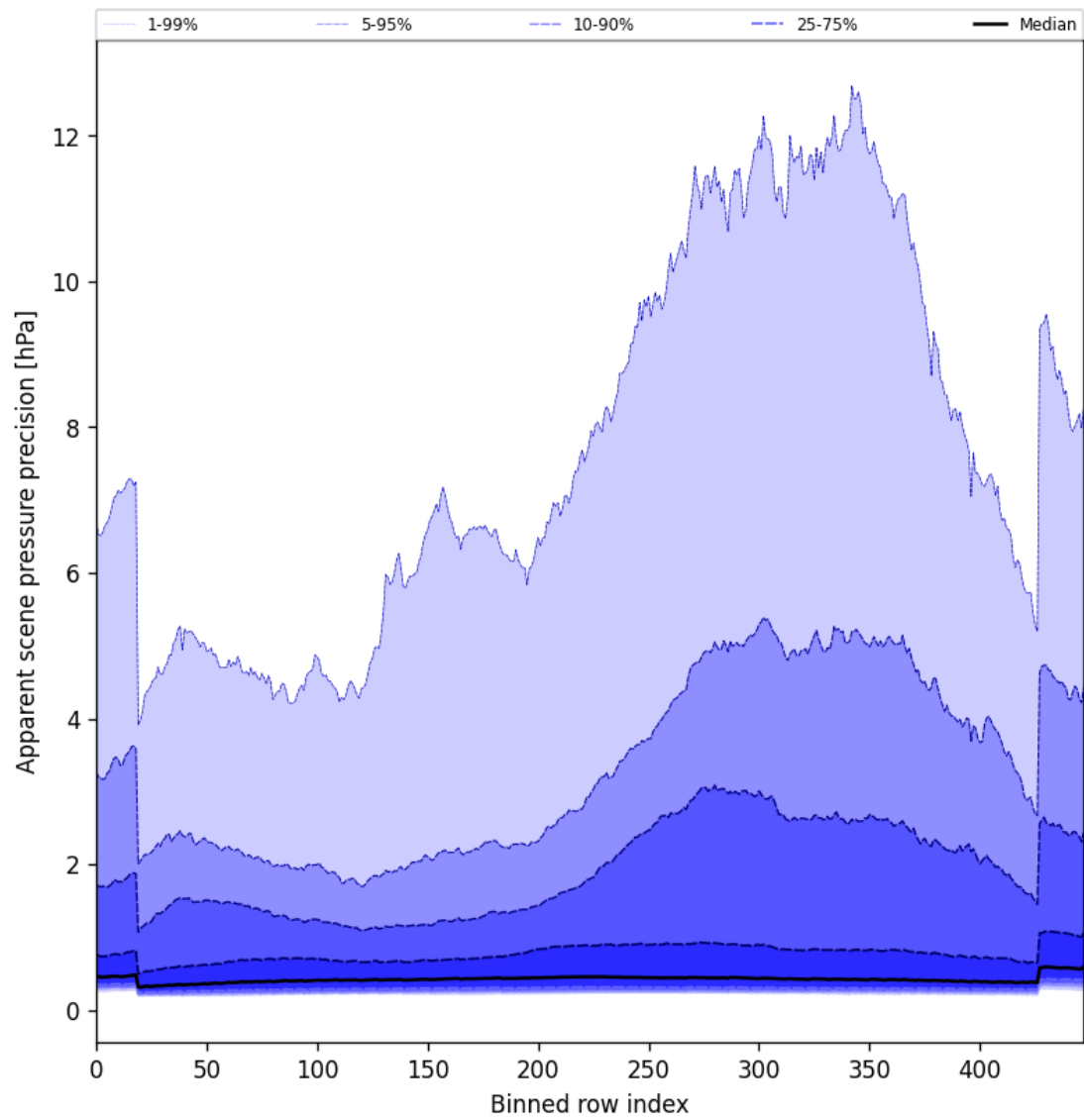
Figure 52: Along track statistics of “Apparent scene pressure precision” for 2024-12-28 to 2024-12-29
