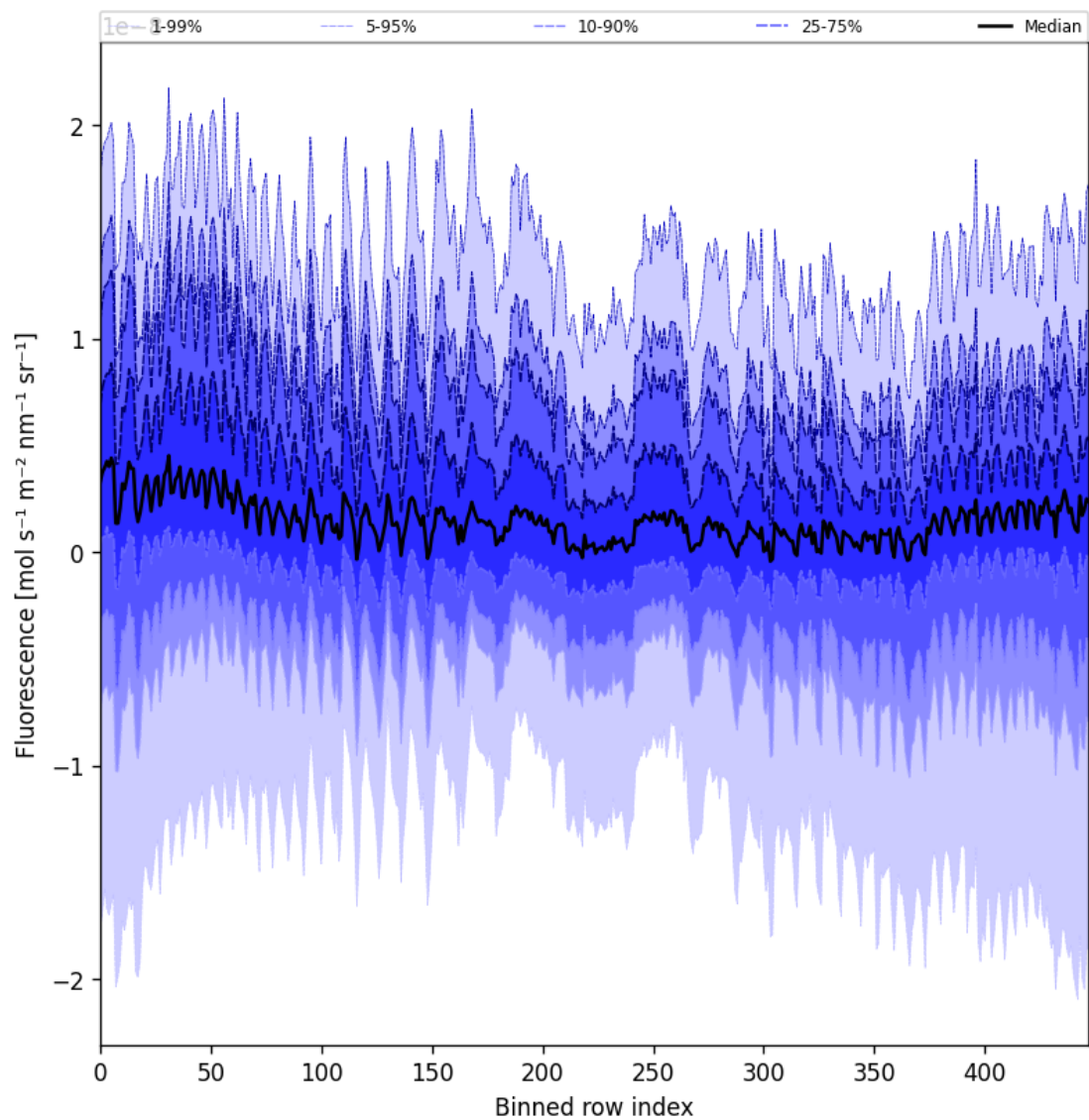
Figure 55: Along track statistics of “Fluorescence” for 2024-12-28 to 2024-12-29
