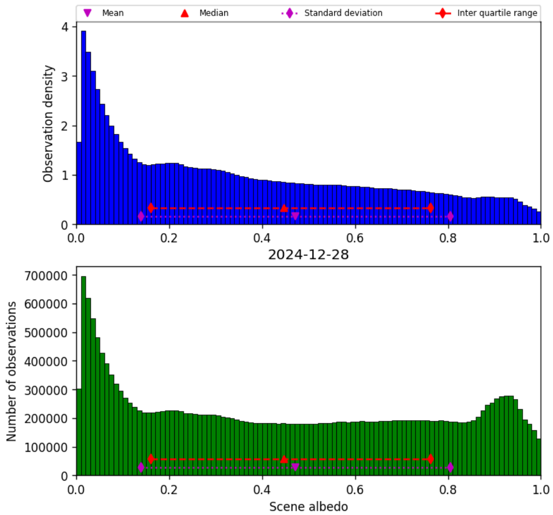
Figure 32: Histogram of “Scene albedo” for 2024-12-28 to 2024-12-29
