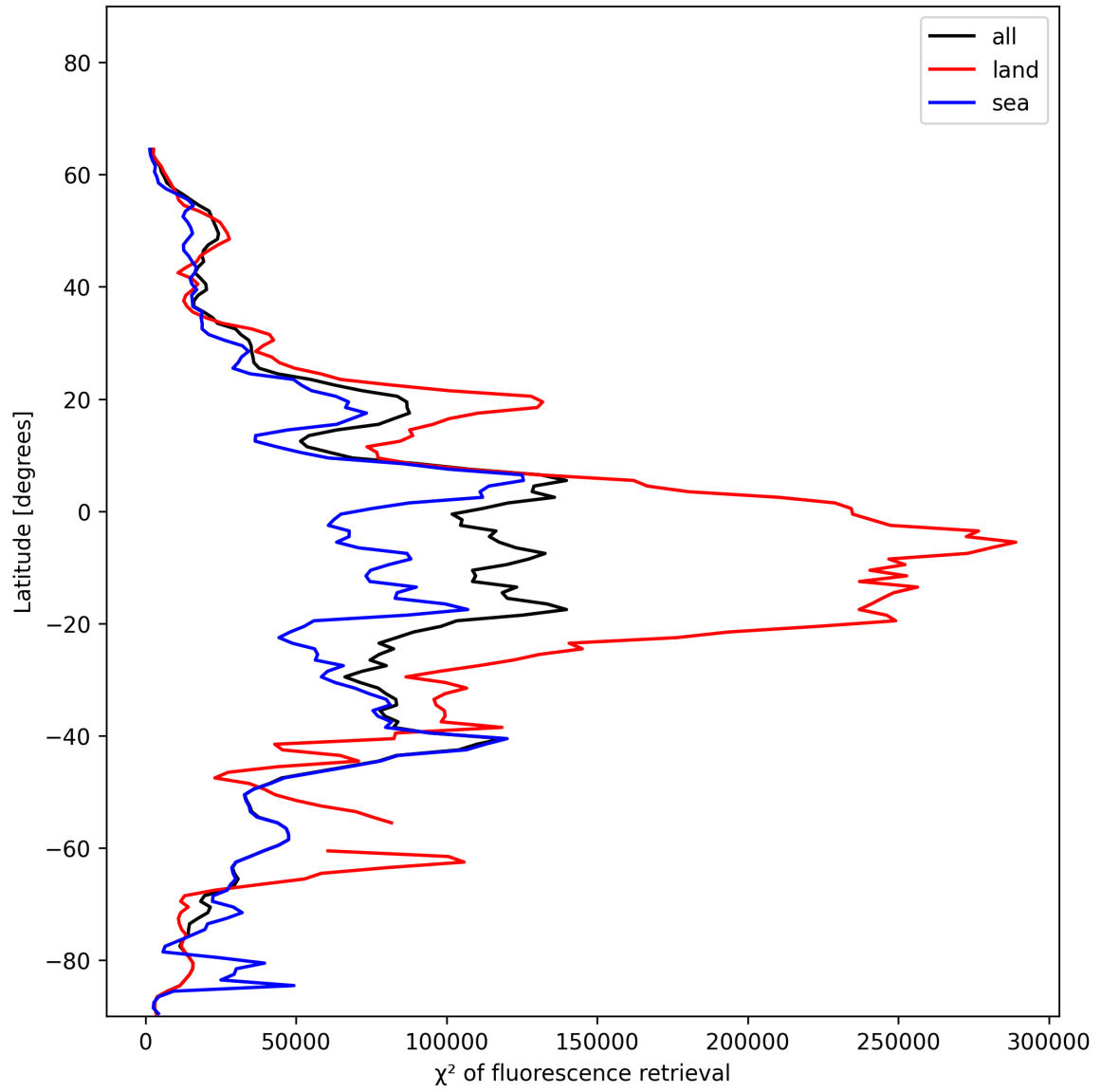
Figure 23: Zonal average of “ \chi^2 of fluorescence retrieval” for 2024-12-28 to 2024-12-29.
