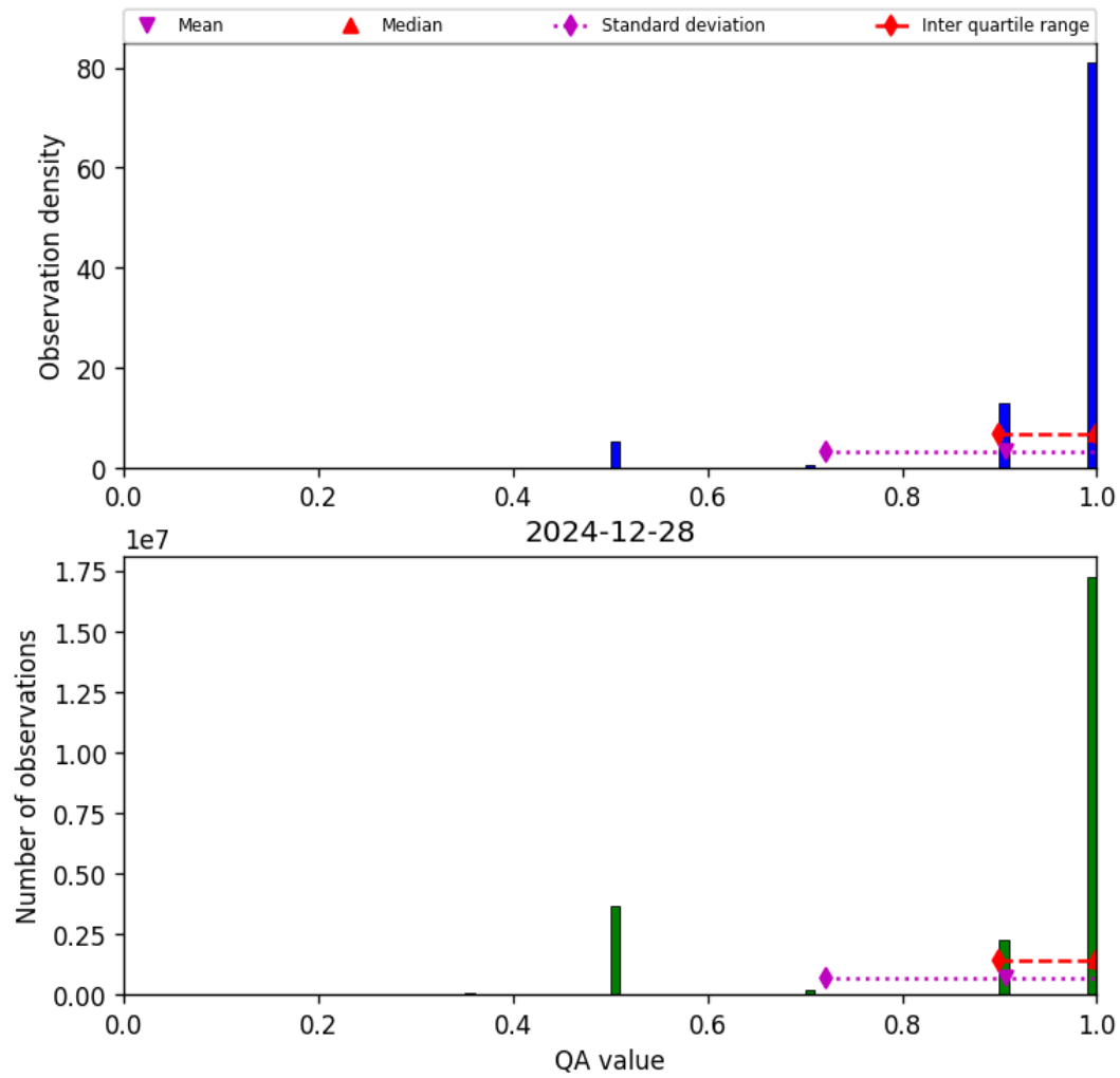
Figure 27: Histogram of “QA value” for 2024-12-28 to 2024-12-29
