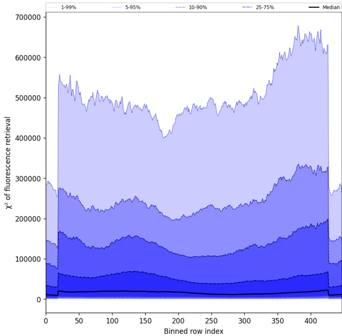
Figure 57: Along track statistics of “ \chi^2 of fluorescence retrieval” for 2024-12-28 to 2024-12-29
