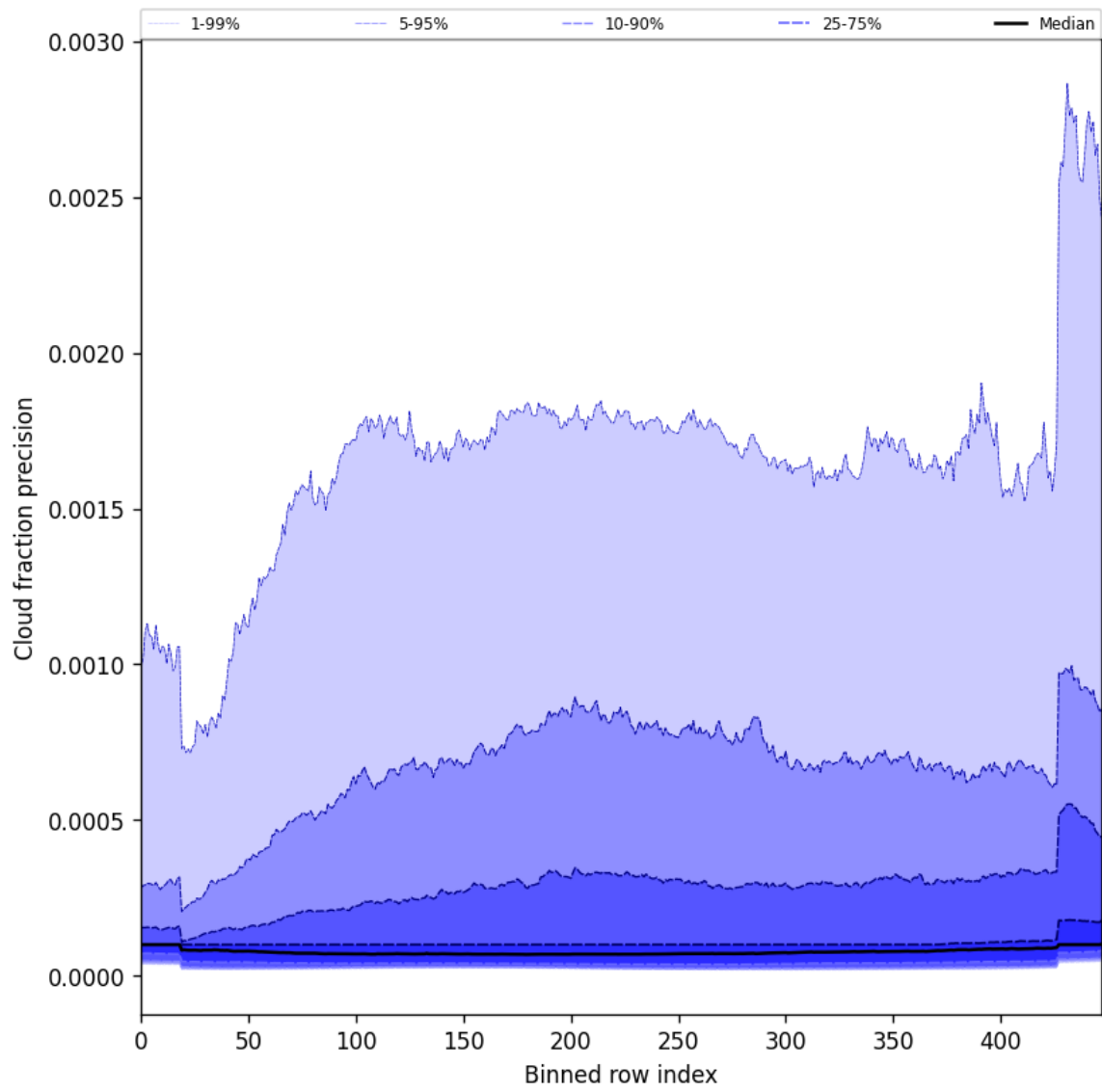
Figure 48: Along track statistics of “Cloud fraction precision” for 2024-12-28 to 2024-12-29
