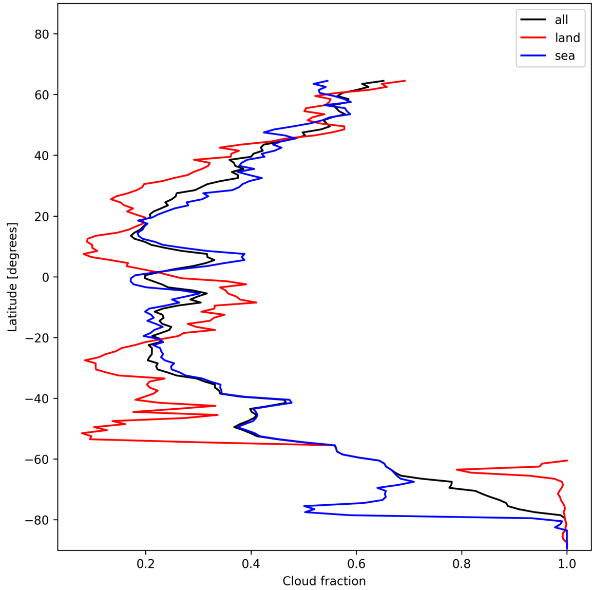
Figure 13: Zonal average of “Cloud fraction” for 2024-12-28 to 2024-12-29.
