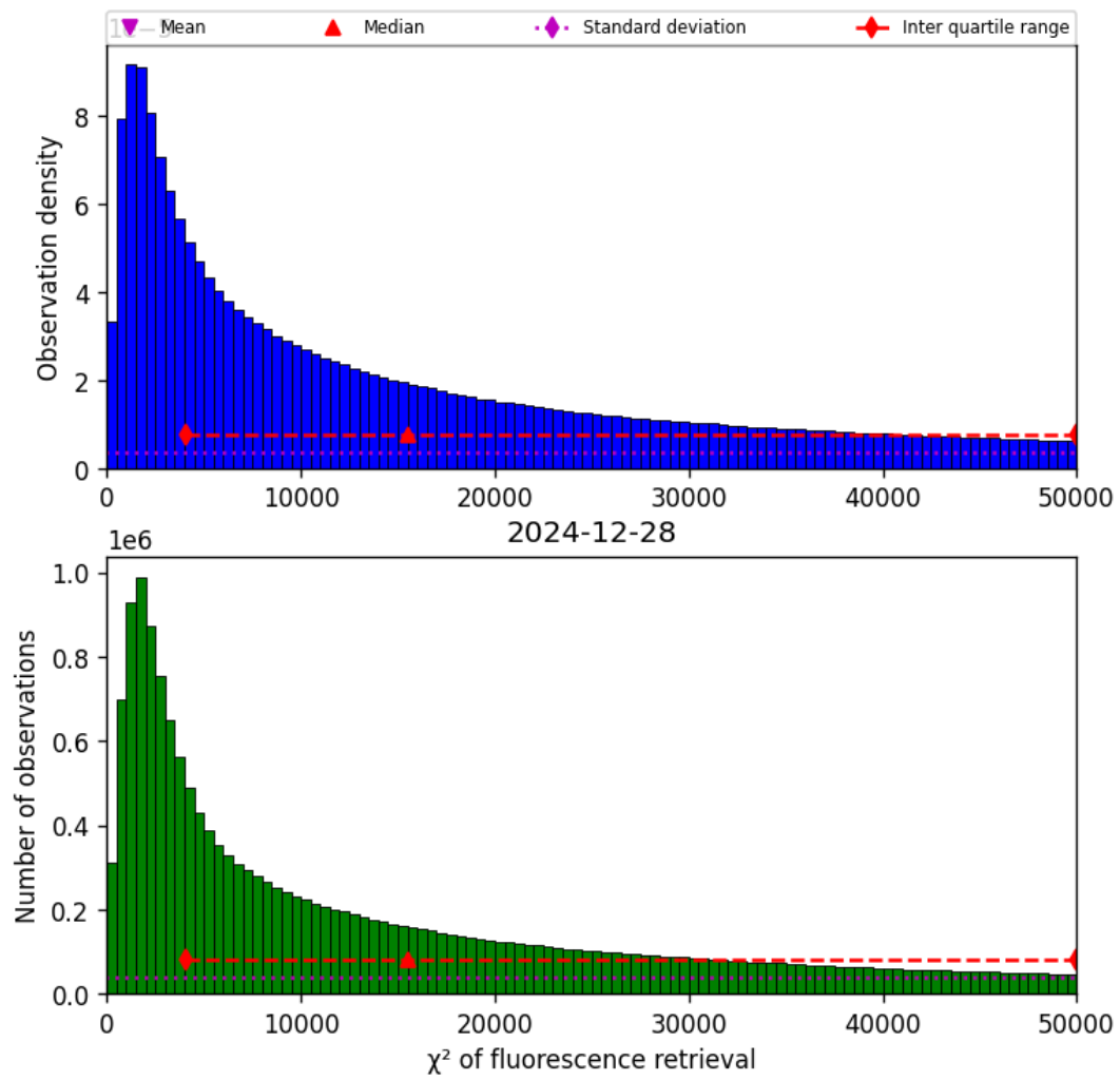
Figure 40: Histogram of “ \chi^2 of fluorescence retrieval” for 2024-12-28 to 2024-12-29
