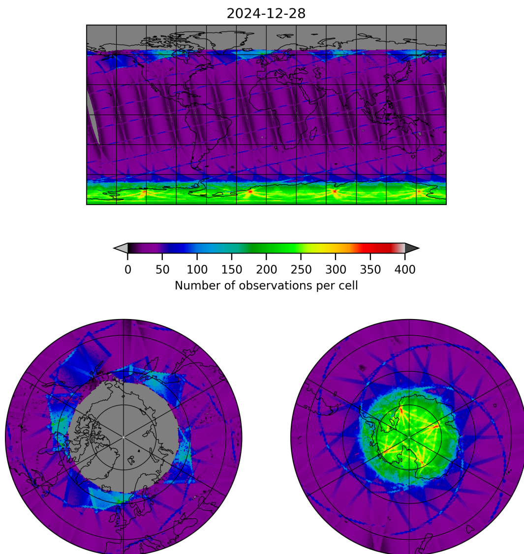
Figure 9: Map of the number of observations for 2024-12-28 to 2024-12-29
