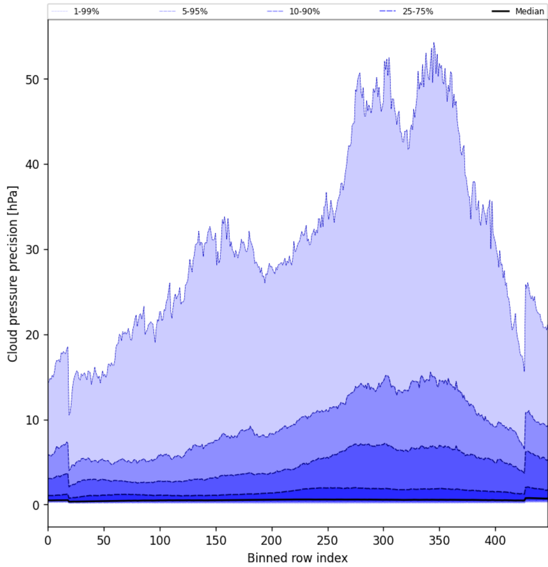
Figure 46: Along track statistics of “Cloud pressure precision” for 2024-12-28 to 2024-12-29
