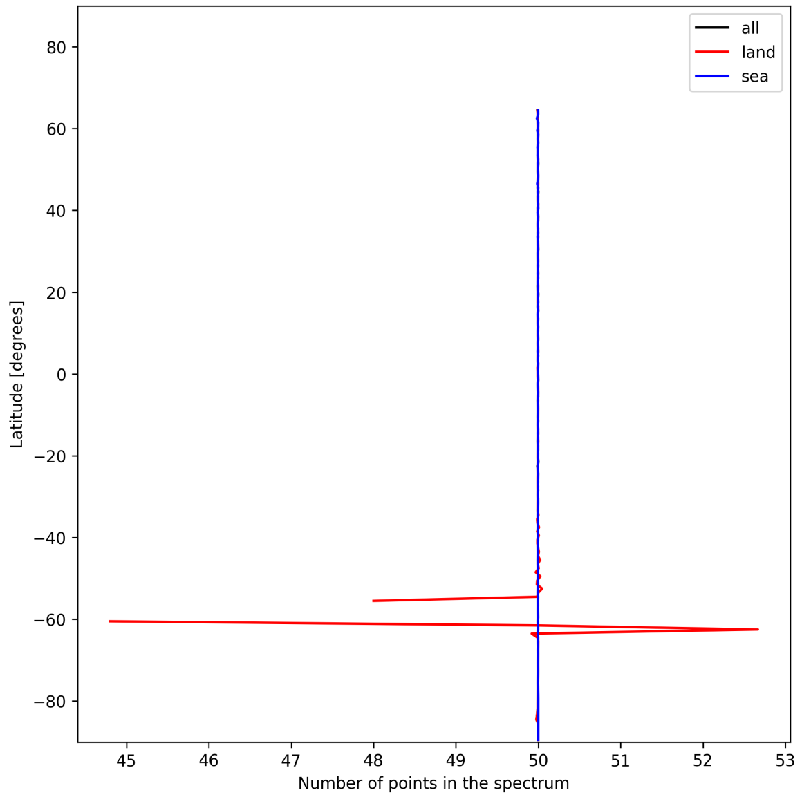
Figure 25: Zonal average of “Number of points in the spectrum” for 2024-12-28 to 2024-12-29.
