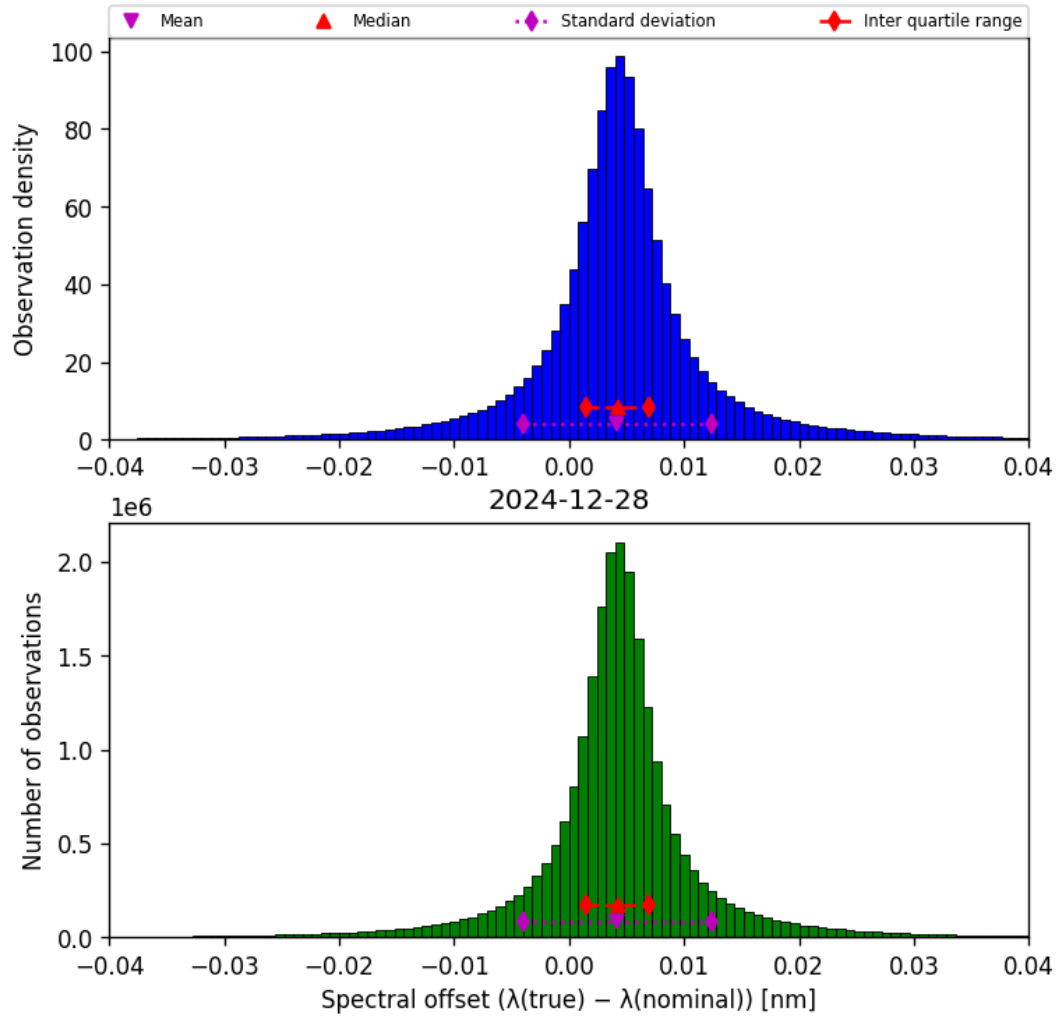
Figure 43: Histogram of “Spectral offset ( \lambda_{\text{true}} - \lambda_{\text{nominal}} )” for 2024-12-28 to 2024-12-29
