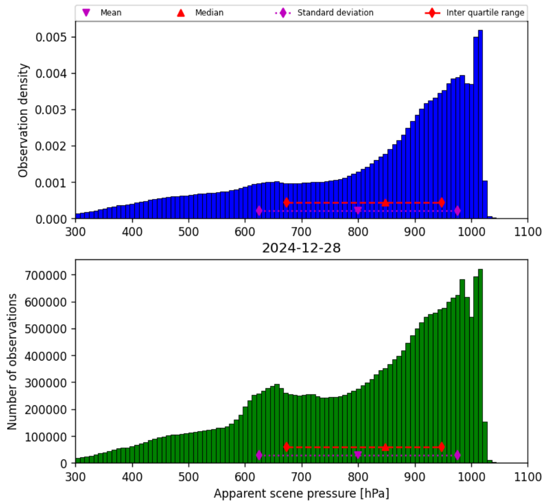
Figure 34: Histogram of “Apparent scene pressure” for 2024-12-28 to 2024-12-29
