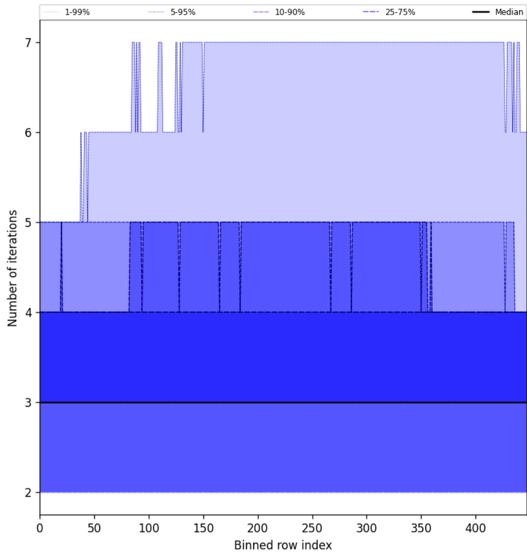
Figure 54: Along track statistics of “Number of iterations” for 2024-12-29 to 2024-12-30
