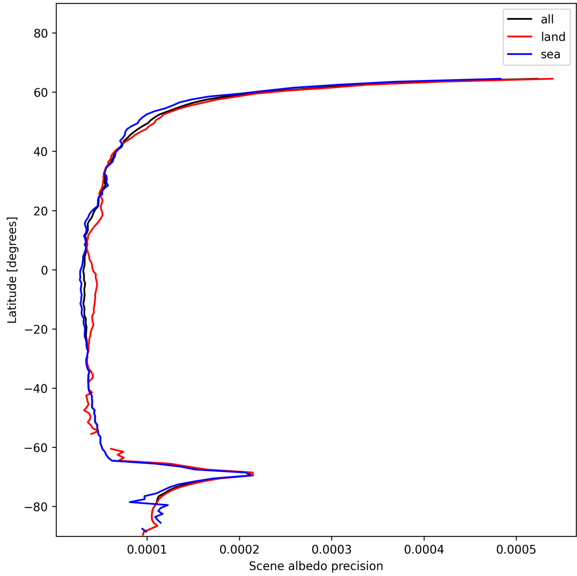
Figure 16: Zonal average of “Scene albedo precision” for 2024-12-29 to 2024-12-30.
