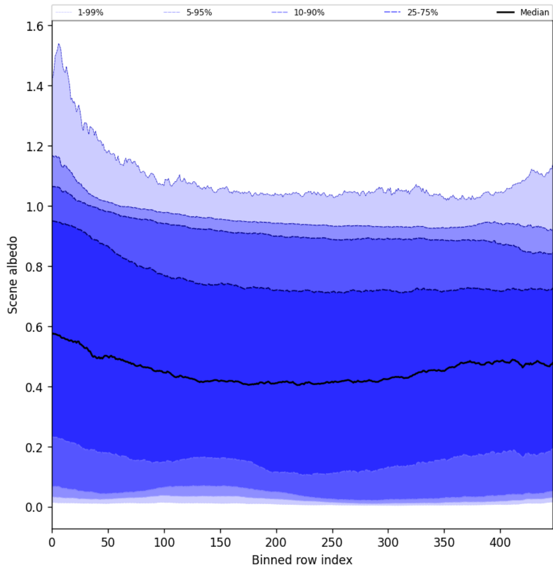
Figure 49: Along track statistics of “Scene albedo” for 2024-12-29 to 2024-12-30
