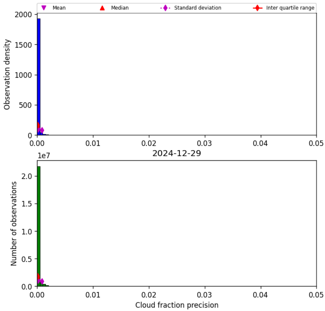
Figure 31: Histogram of “Cloud fraction precision” for 2024-12-29 to 2024-12-30
