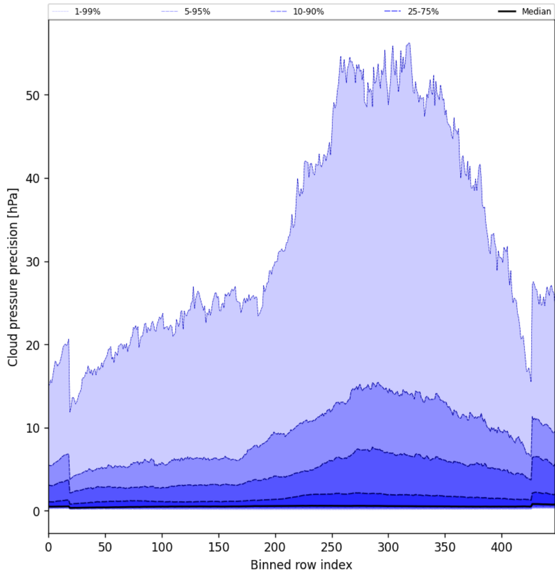
Figure 46: Along track statistics of “Cloud pressure precision” for 2024-12-29 to 2024-12-30
