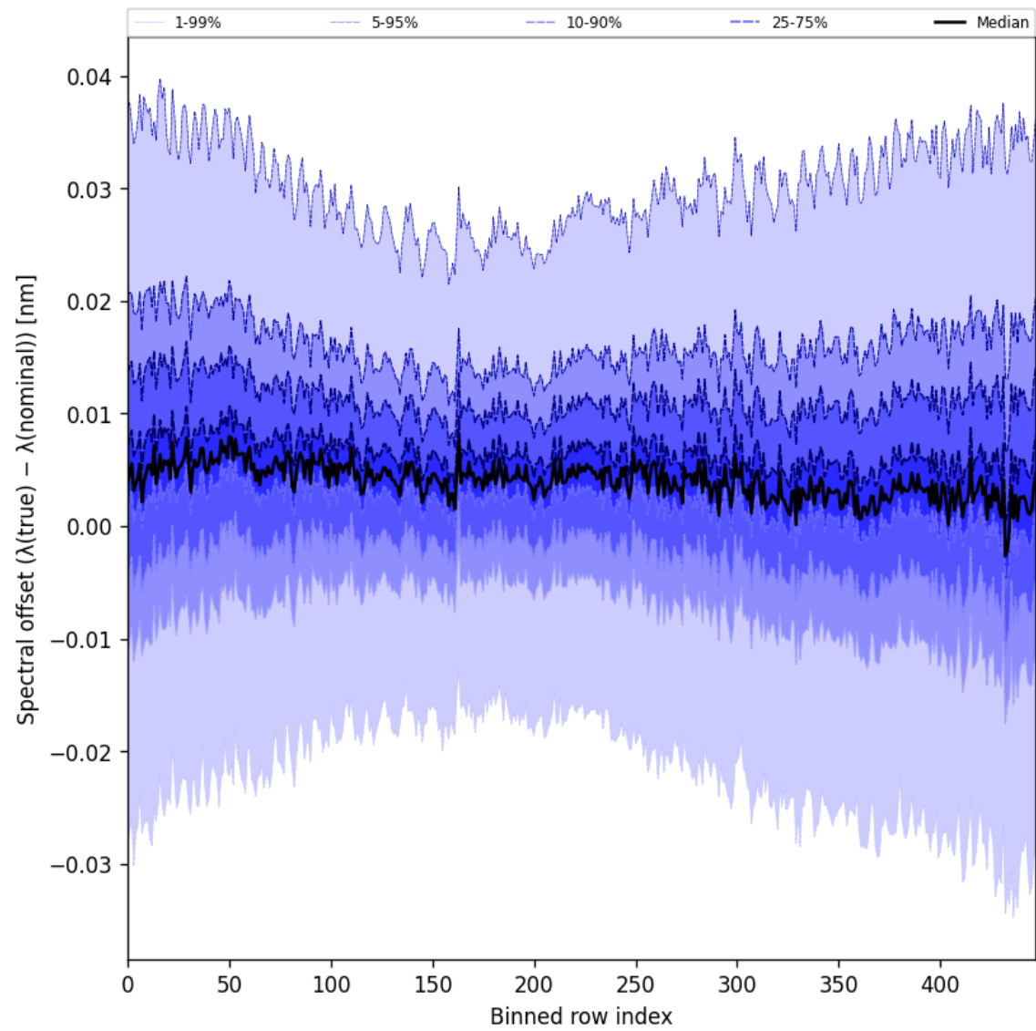
Figure 60: Along track statistics of “Spectral offset ( \lambda_{\text{true}} - \lambda_{\text{nominal}} )” for 2024-12-29 to 2024-12-30
