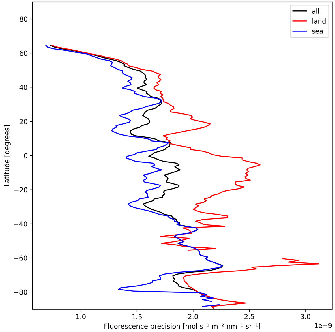
Figure 22: Zonal average of “Fluorescence precision” for 2024-12-29 to 2024-12-30.
