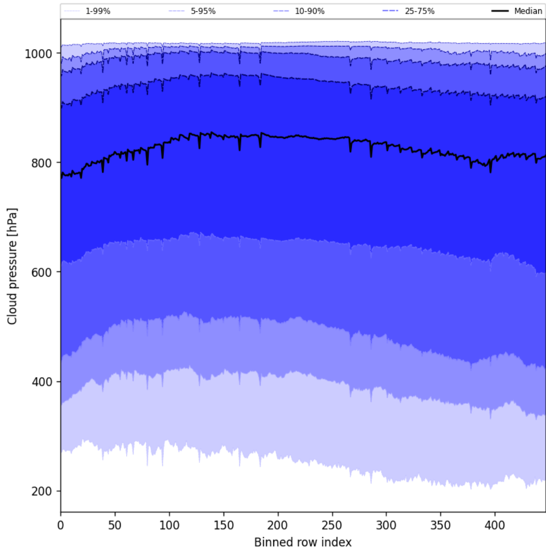
Figure 45: Along track statistics of “Cloud pressure” for 2024-12-29 to 2024-12-30
