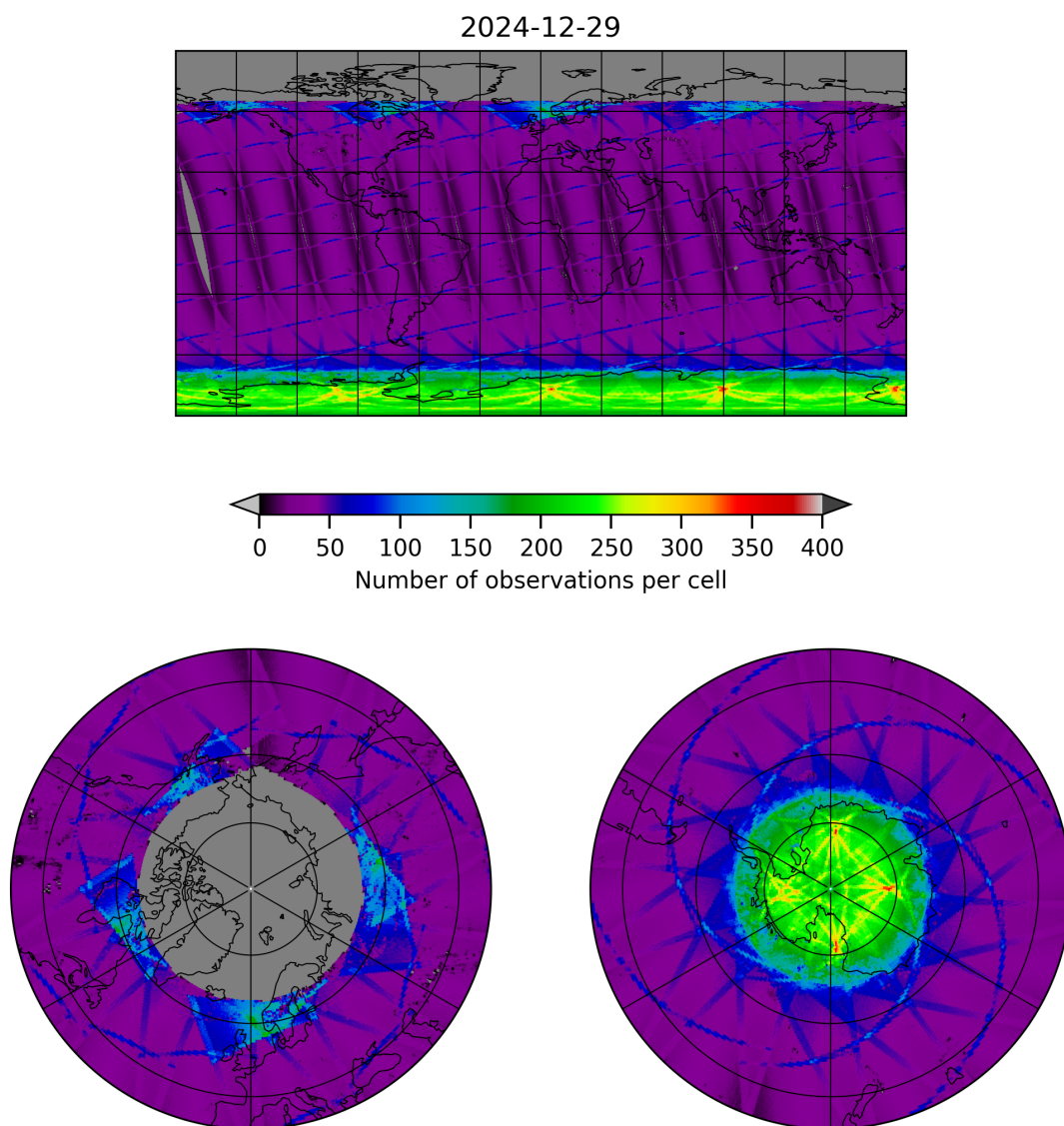
Figure 9: Map of the number of observations for 2024-12-29 to 2024-12-30
