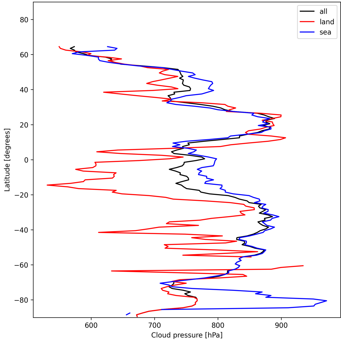
Figure 11: Zonal average of “Cloud pressure” for 2024-12-29 to 2024-12-30.
