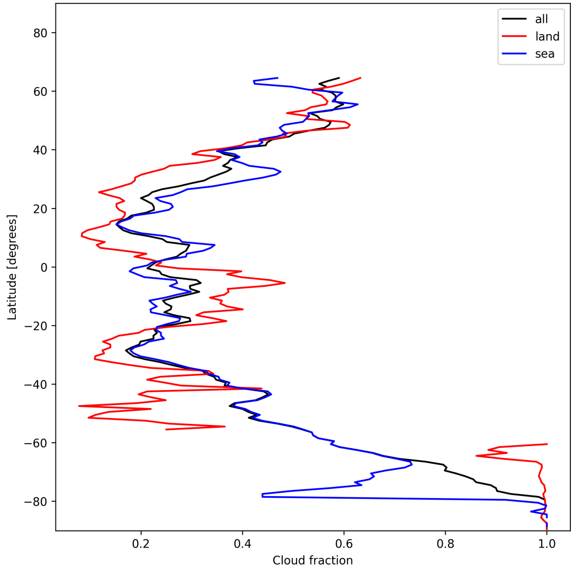
Figure 13: Zonal average of “Cloud fraction” for 2024-12-29 to 2024-12-30.
