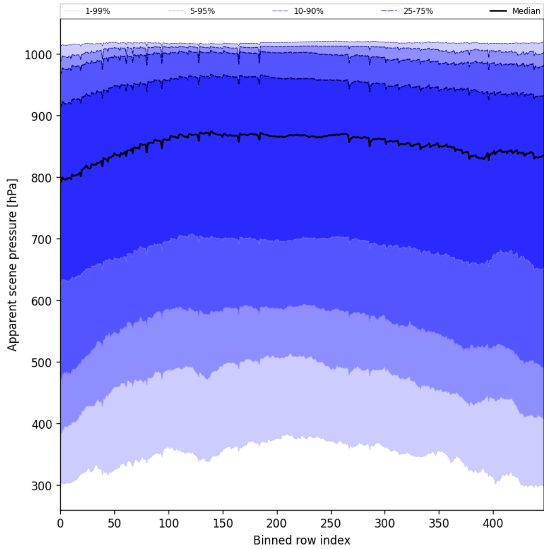
Figure 51: Along track statistics of “Apparent scene pressure” for 2024-12-29 to 2024-12-30
