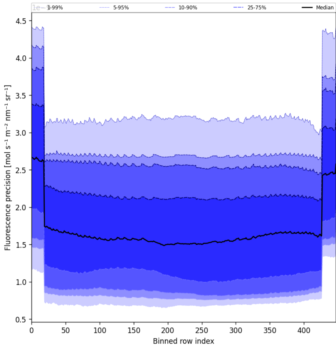
Figure 56: Along track statistics of “Fluorescence precision” for 2024-12-29 to 2024-12-30
