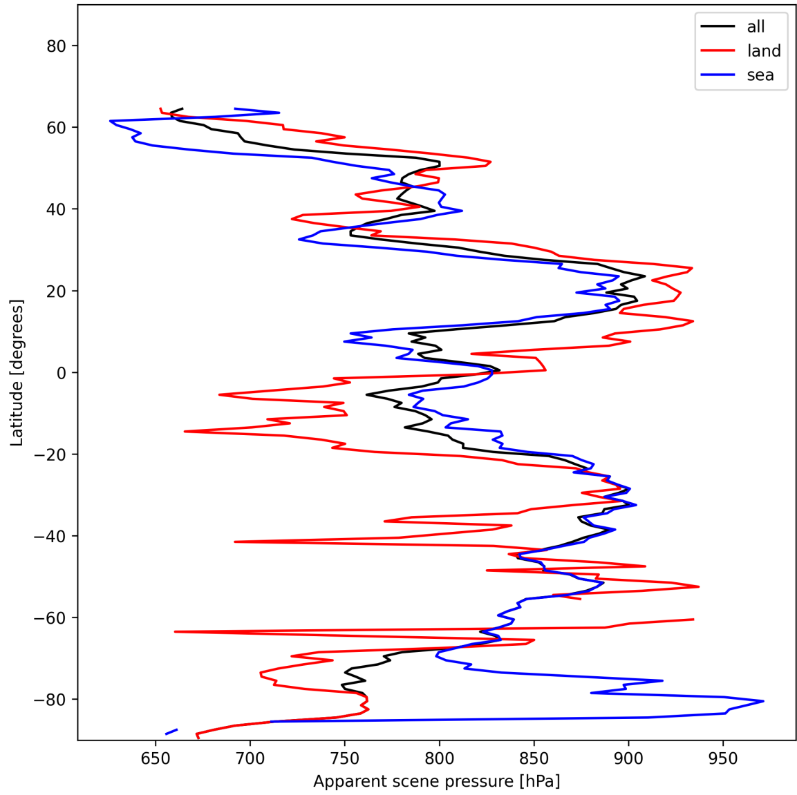
Figure 17: Zonal average of “Apparent scene pressure” for 2024-12-29 to 2024-12-30.
