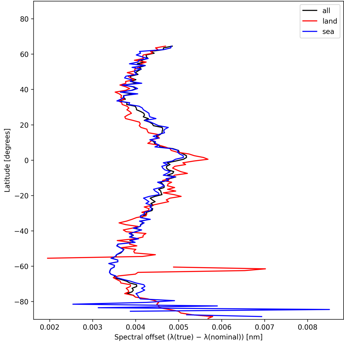
Figure 26: Zonal average of “Spectral offset ( \lambda_{\text{true}} - \lambda_{\text{nominal}} )” for 2024-12-29 to 2024-12-30.
