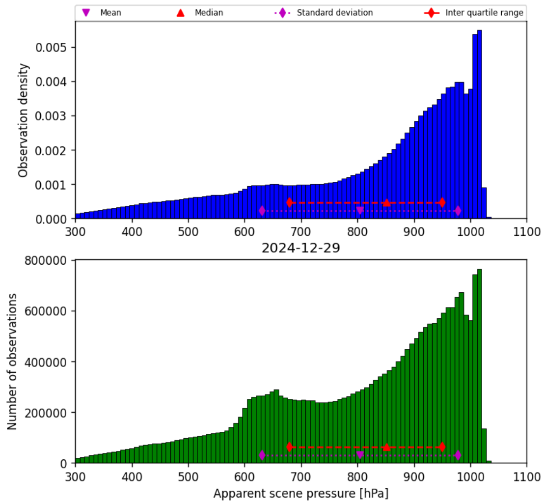
Figure 34: Histogram of “Apparent scene pressure” for 2024-12-29 to 2024-12-30
