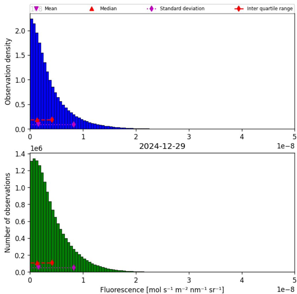
Figure 38: Histogram of “Fluorescence” for 2024-12-29 to 2024-12-30
