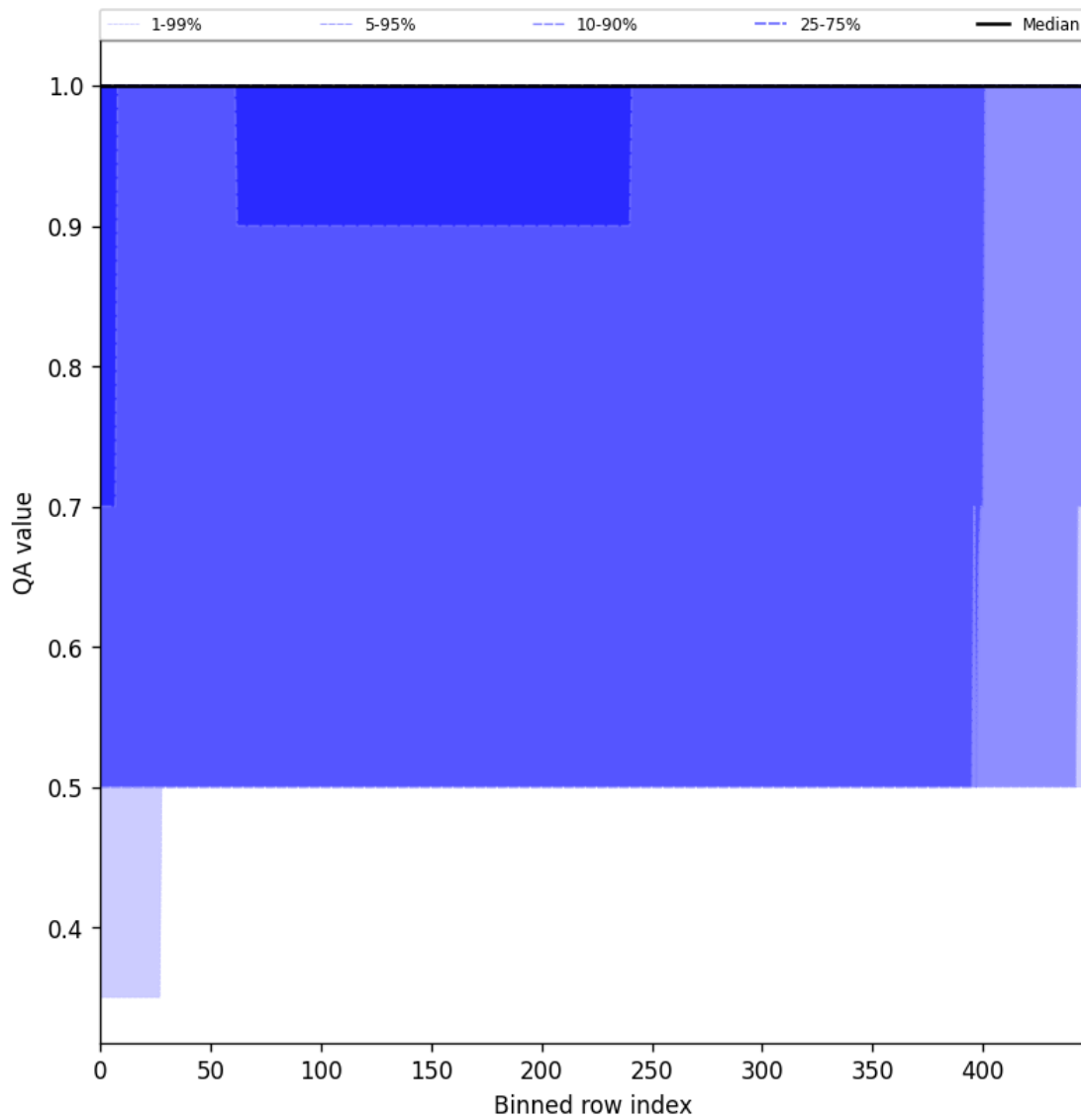
Figure 44: Along track statistics of “QA value” for 2024-12-29 to 2024-12-30
