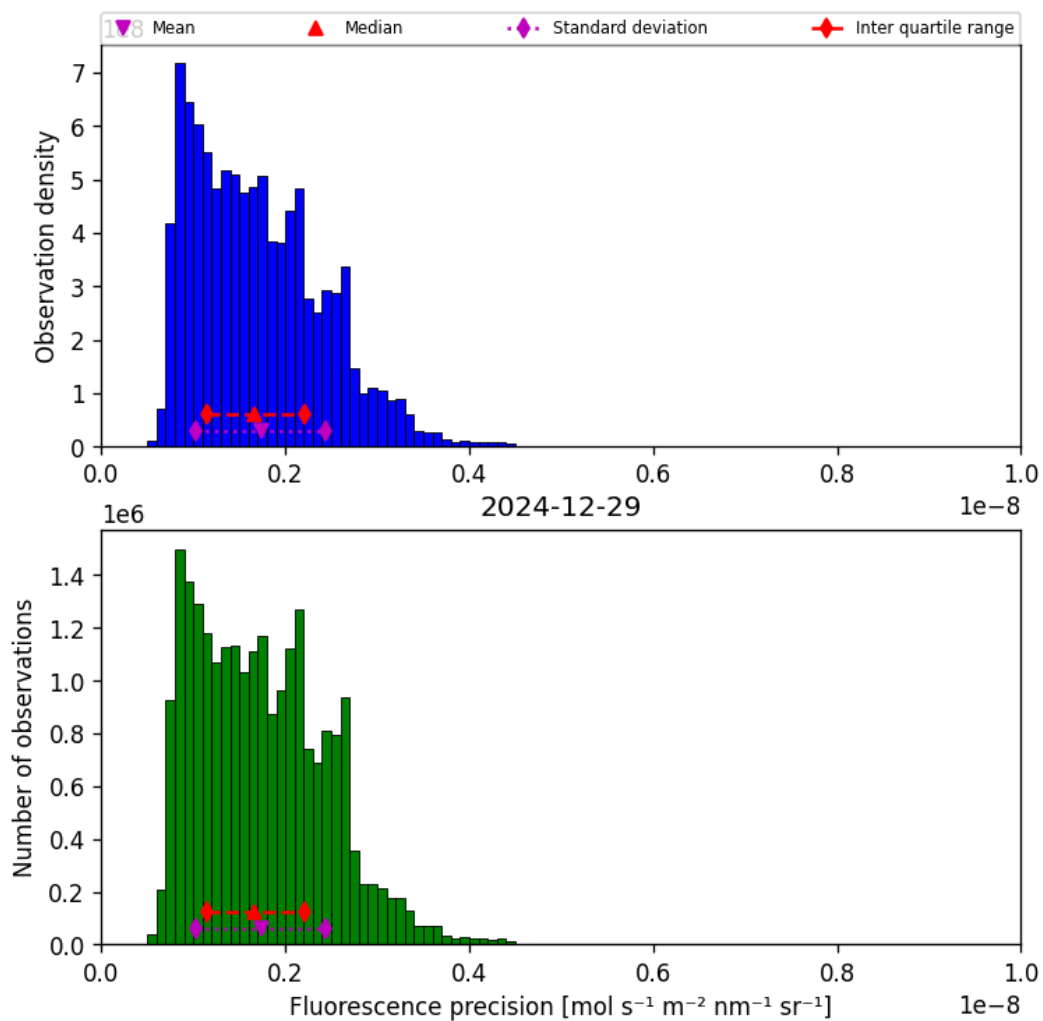
Figure 39: Histogram of “Fluorescence precision” for 2024-12-29 to 2024-12-30
