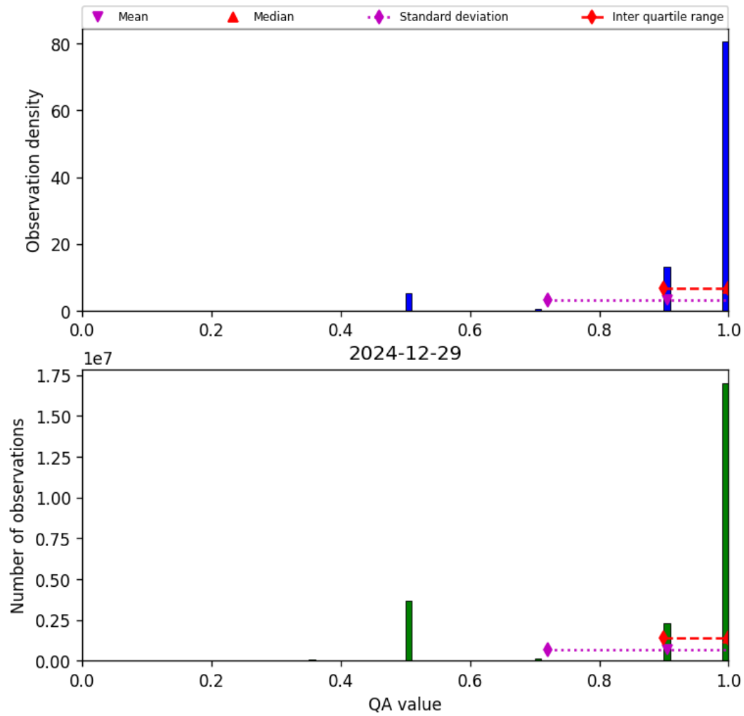
Figure 27: Histogram of “QA value” for 2024-12-29 to 2024-12-30
