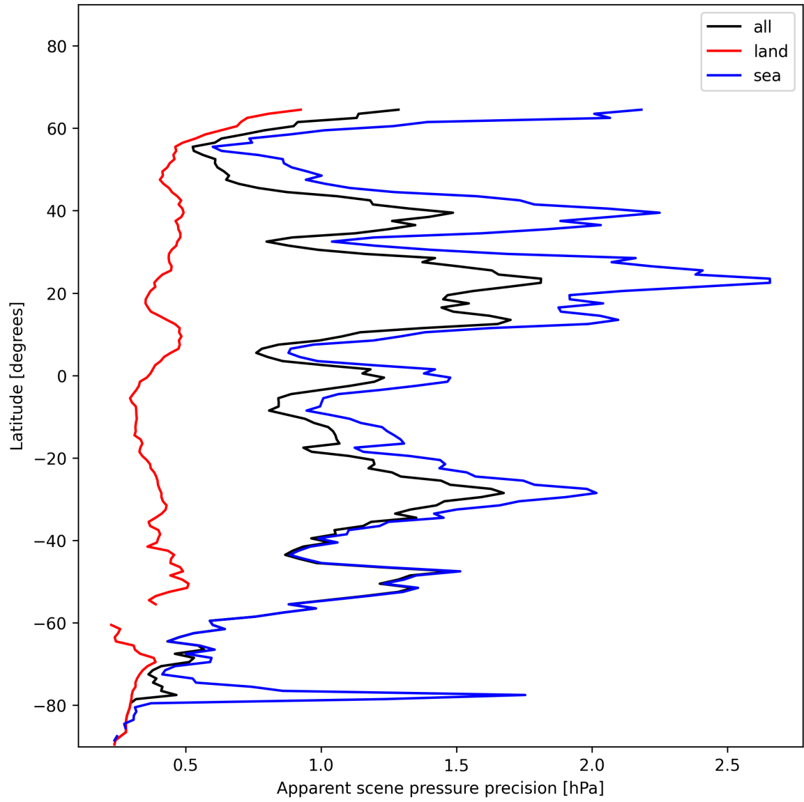
Figure 18: Zonal average of “Apparent scene pressure precision” for 2024-12-29 to 2024-12-30.
