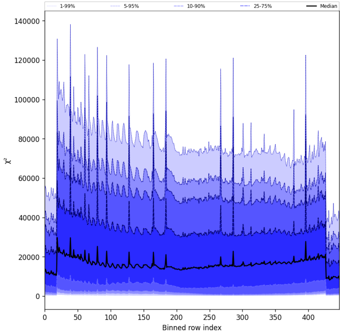
Figure 53: Along track statistics of “ \chi^2 ” for 2024-12-29 to 2024-12-30
