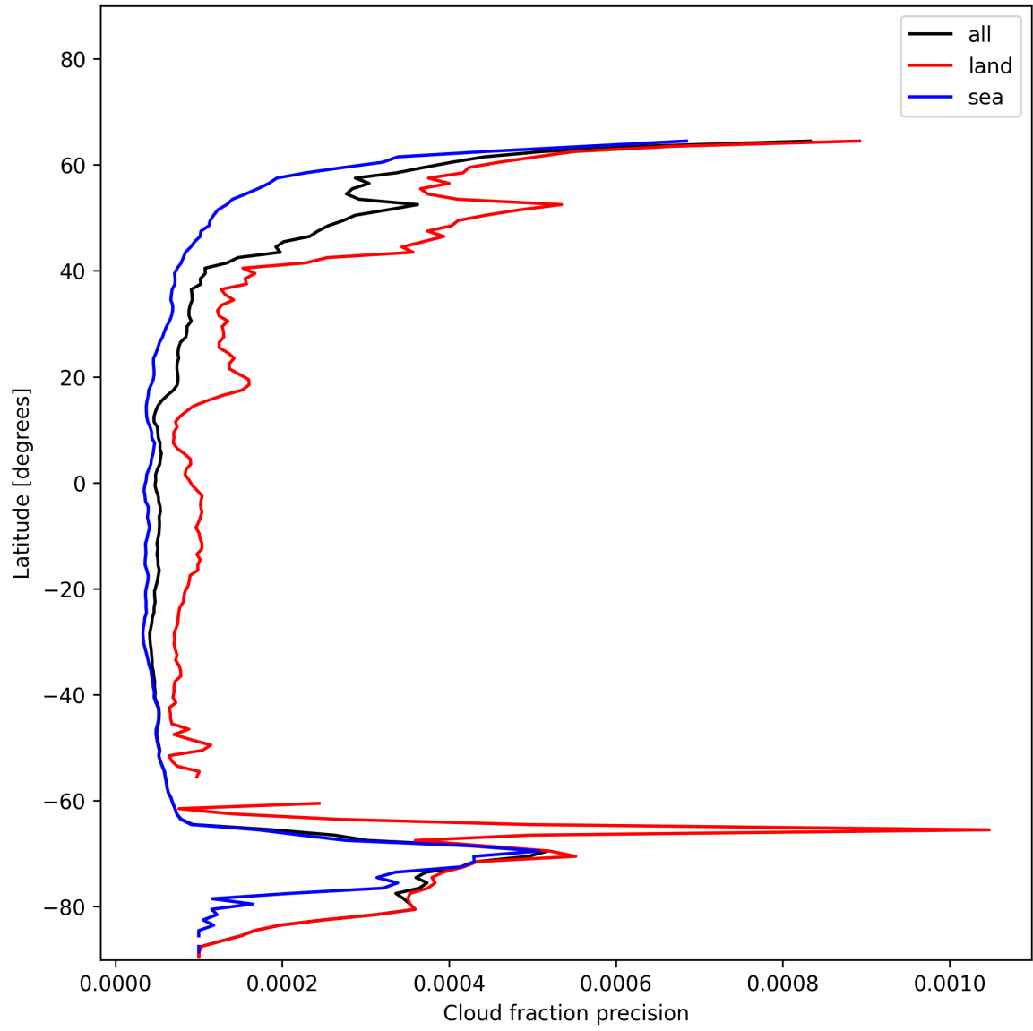
Figure 14: Zonal average of “Cloud fraction precision” for 2024-12-29 to 2024-12-30.
