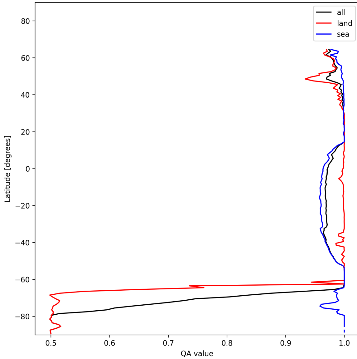
Figure 10: Zonal average of “QA value” for 2024-12-29 to 2024-12-30.
