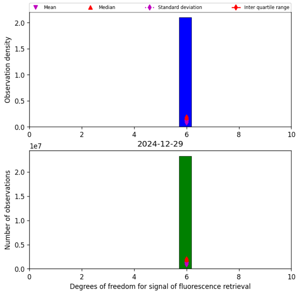
Figure 41: Histogram of “Degrees of freedom for signal of fluorescence retrieval” for 2024-12-29 to 2024-12-30
