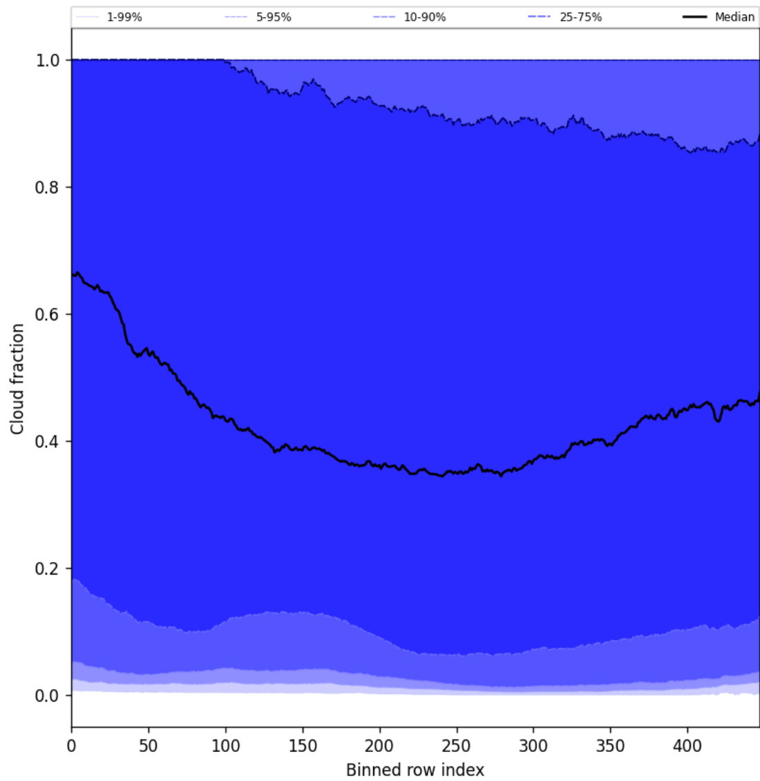
Figure 47: Along track statistics of “Cloud fraction” for 2024-12-29 to 2024-12-30
