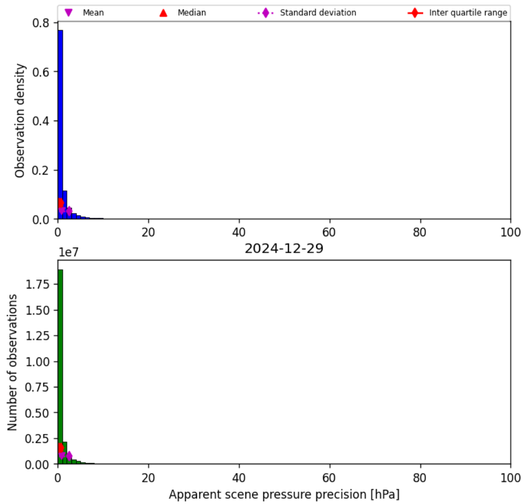
Figure 35: Histogram of “Apparent scene pressure precision” for 2024-12-29 to 2024-12-30
