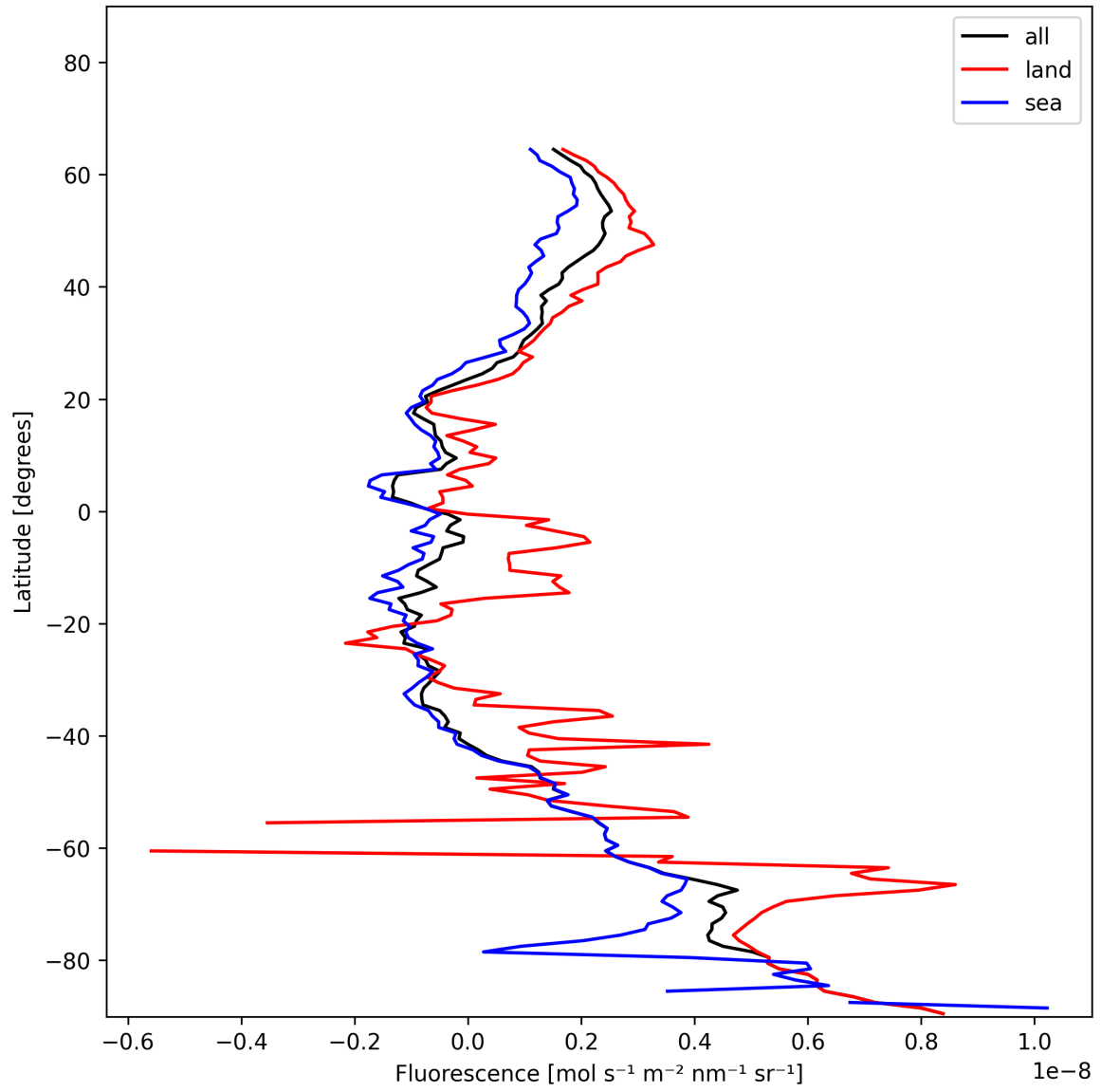
Figure 21: Zonal average of “Fluorescence” for 2024-12-29 to 2024-12-30.
