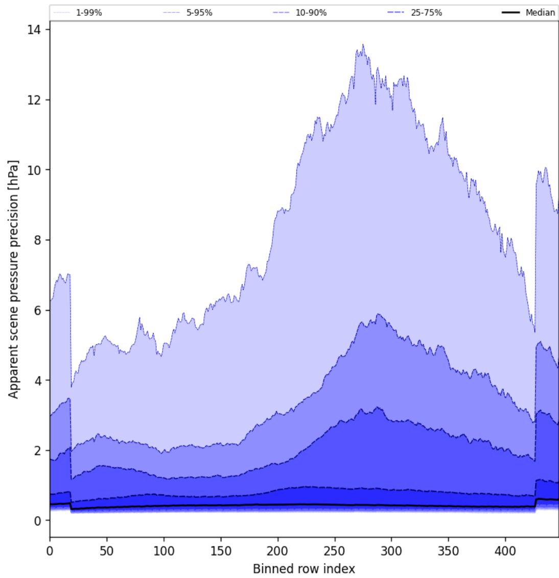
Figure 52: Along track statistics of “Apparent scene pressure precision” for 2024-12-29 to 2024-12-30
