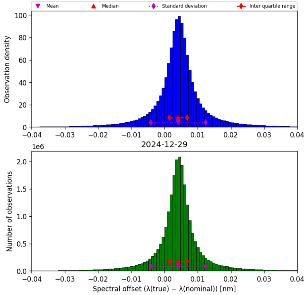
Figure 43: Histogram of “Spectral offset ( \lambda_{\text{true}} - \lambda_{\text{nominal}} )” for 2024-12-29 to 2024-12-30
