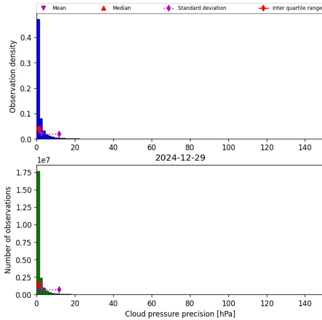
Figure 29: Histogram of “Cloud pressure precision” for 2024-12-29 to 2024-12-30
