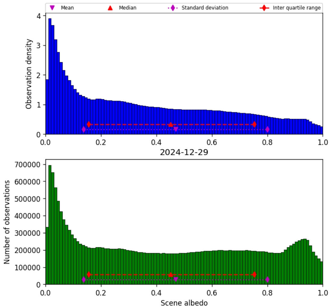
Figure 32: Histogram of “Scene albedo” for 2024-12-29 to 2024-12-30
