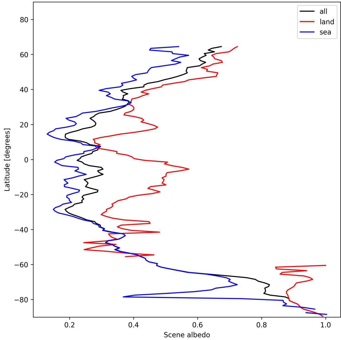
Figure 15: Zonal average of “Scene albedo” for 2024-12-29 to 2024-12-30.
