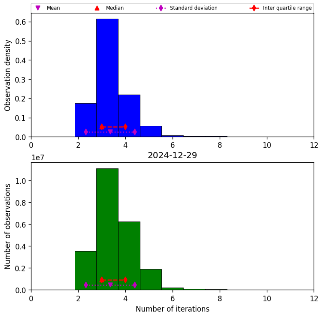
Figure 37: Histogram of “Number of iterations” for 2024-12-29 to 2024-12-30
