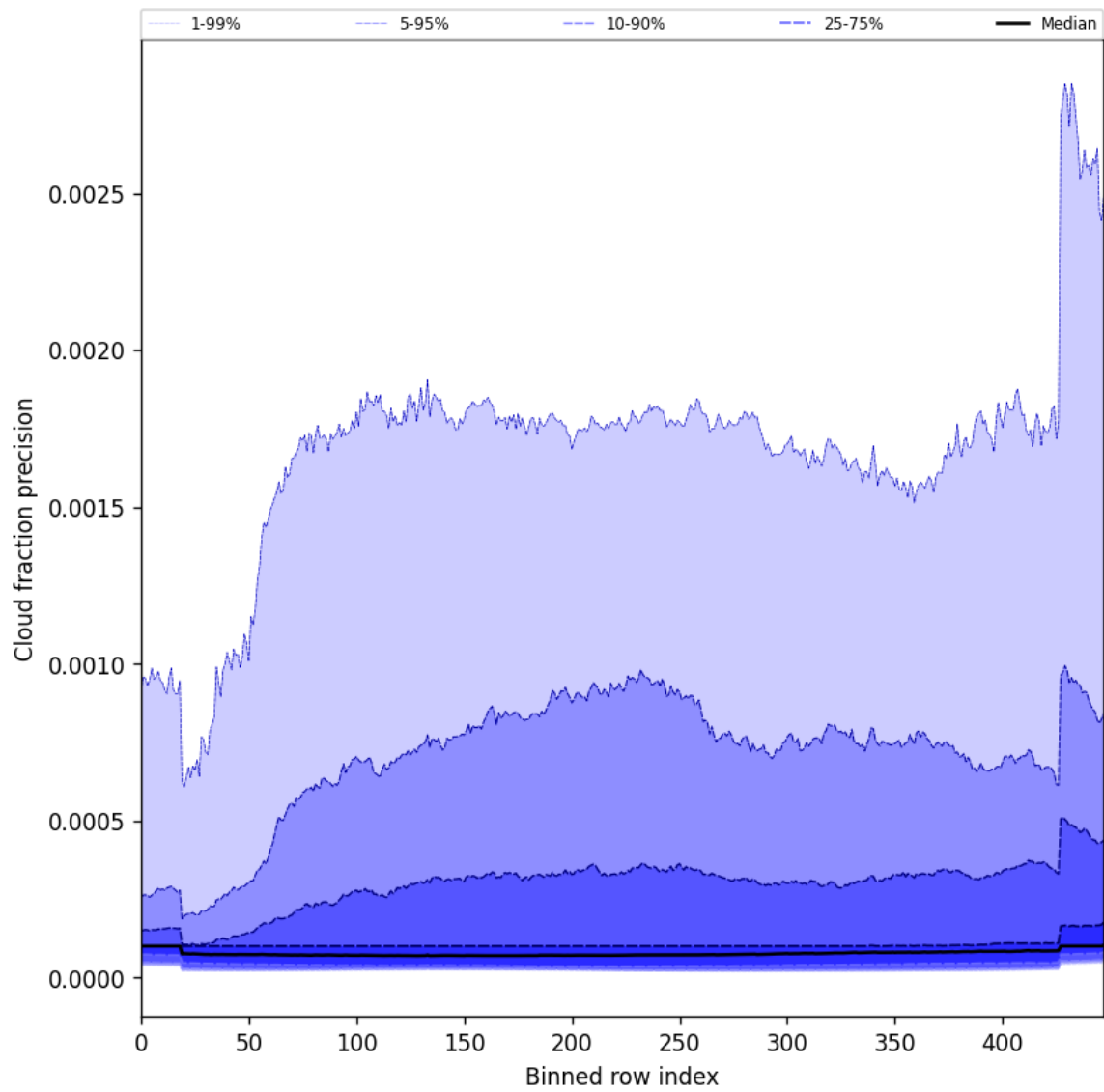
Figure 48: Along track statistics of “Cloud fraction precision” for 2024-12-29 to 2024-12-30
