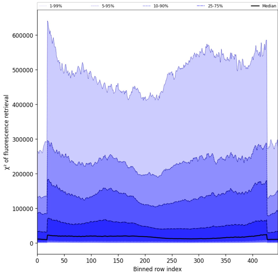
Figure 57: Along track statistics of “ \chi^2 of fluorescence retrieval” for 2024-12-29 to 2024-12-30
