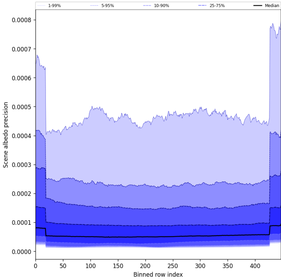
Figure 50: Along track statistics of “Scene albedo precision” for 2024-12-29 to 2024-12-30
