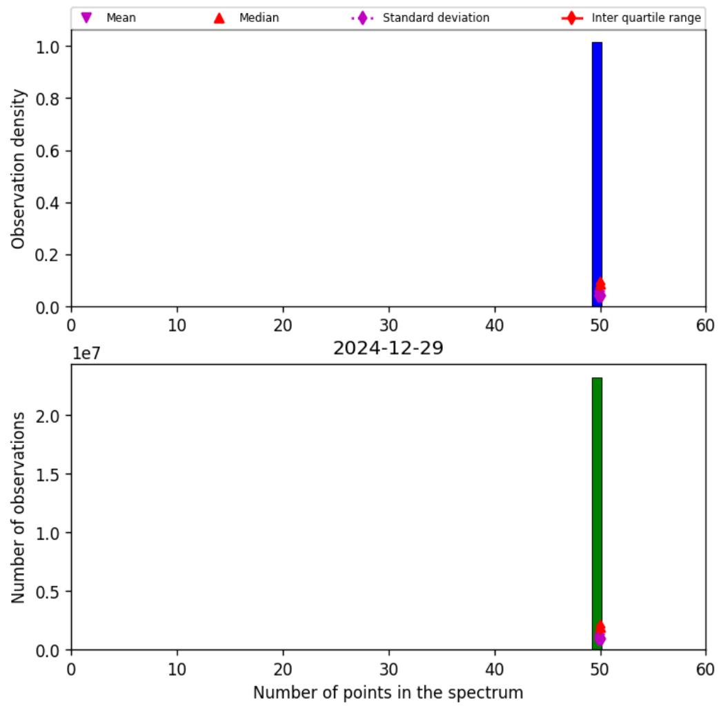
Figure 42: Histogram of “Number of points in the spectrum” for 2024-12-29 to 2024-12-30
