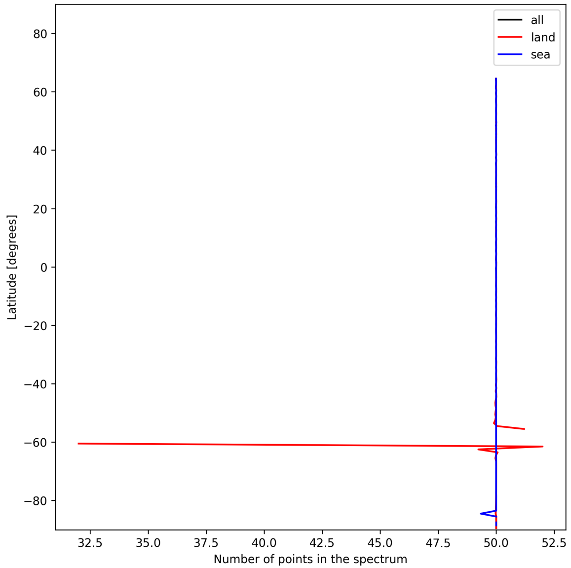
Figure 25: Zonal average of “Number of points in the spectrum” for 2024-12-29 to 2024-12-30.
