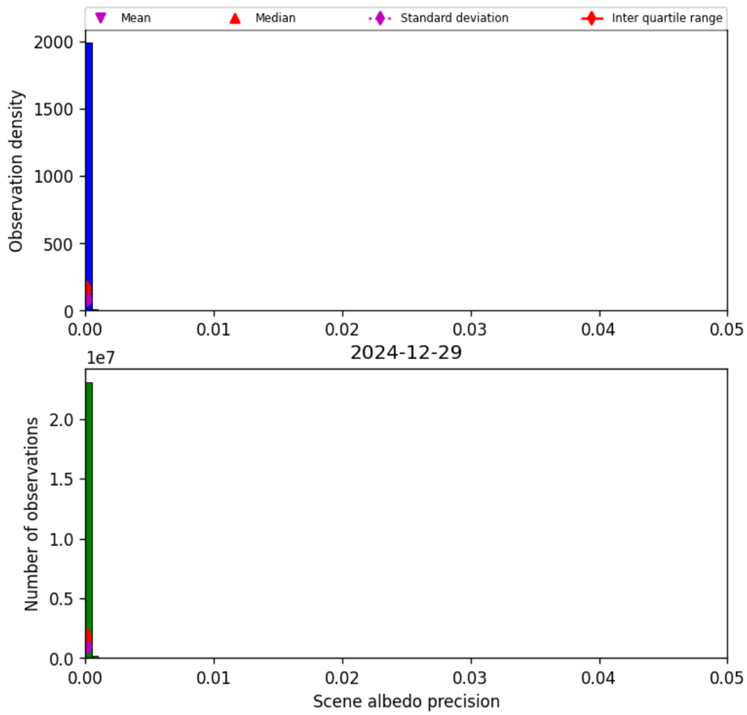
Figure 33: Histogram of “Scene albedo precision” for 2024-12-29 to 2024-12-30
