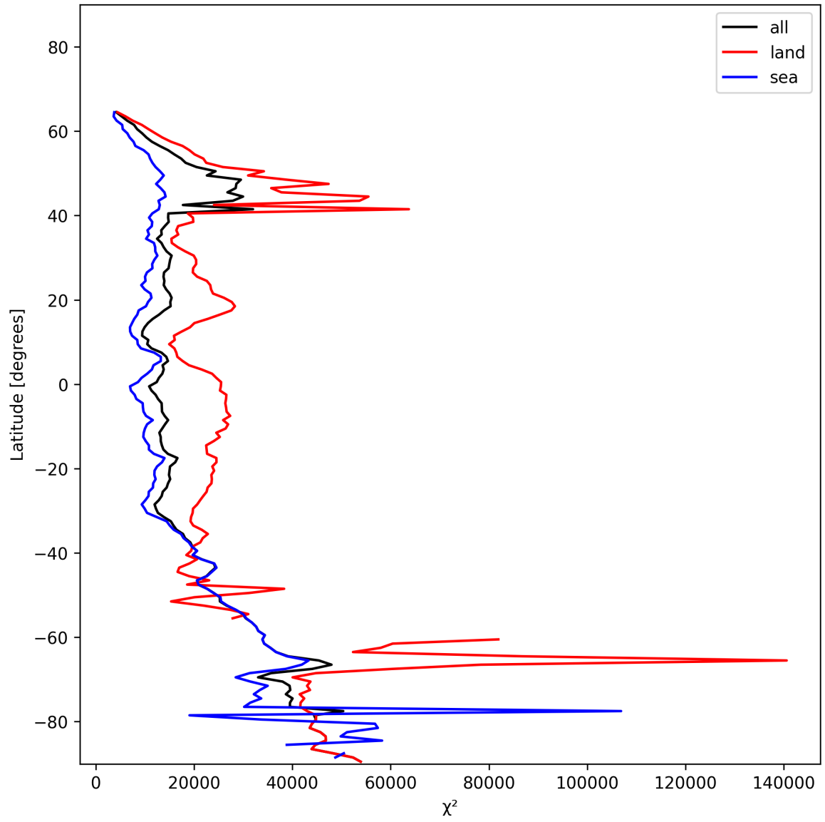
Figure 19: Zonal average of “ \chi^2 ” for 2024-12-29 to 2024-12-30.
