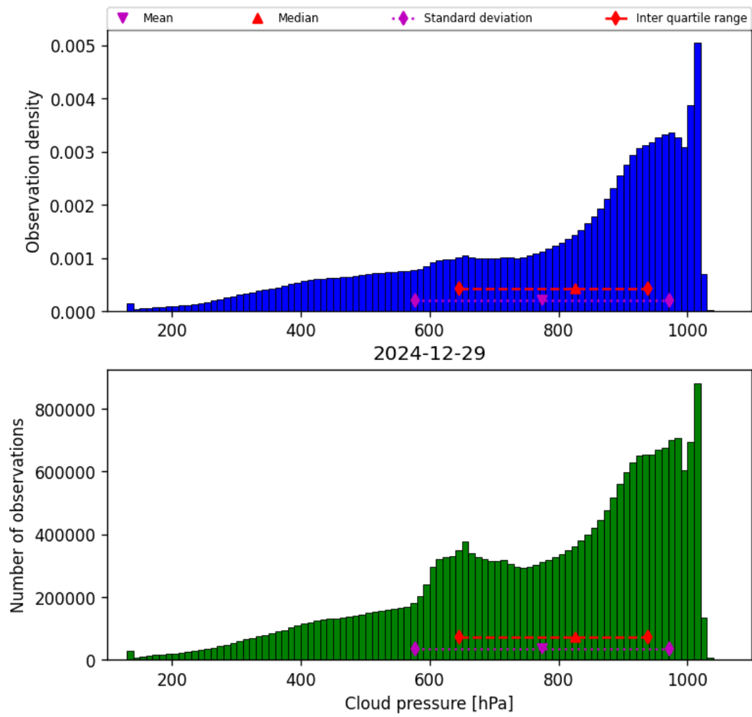
Figure 28: Histogram of “Cloud pressure” for 2024-12-29 to 2024-12-30
