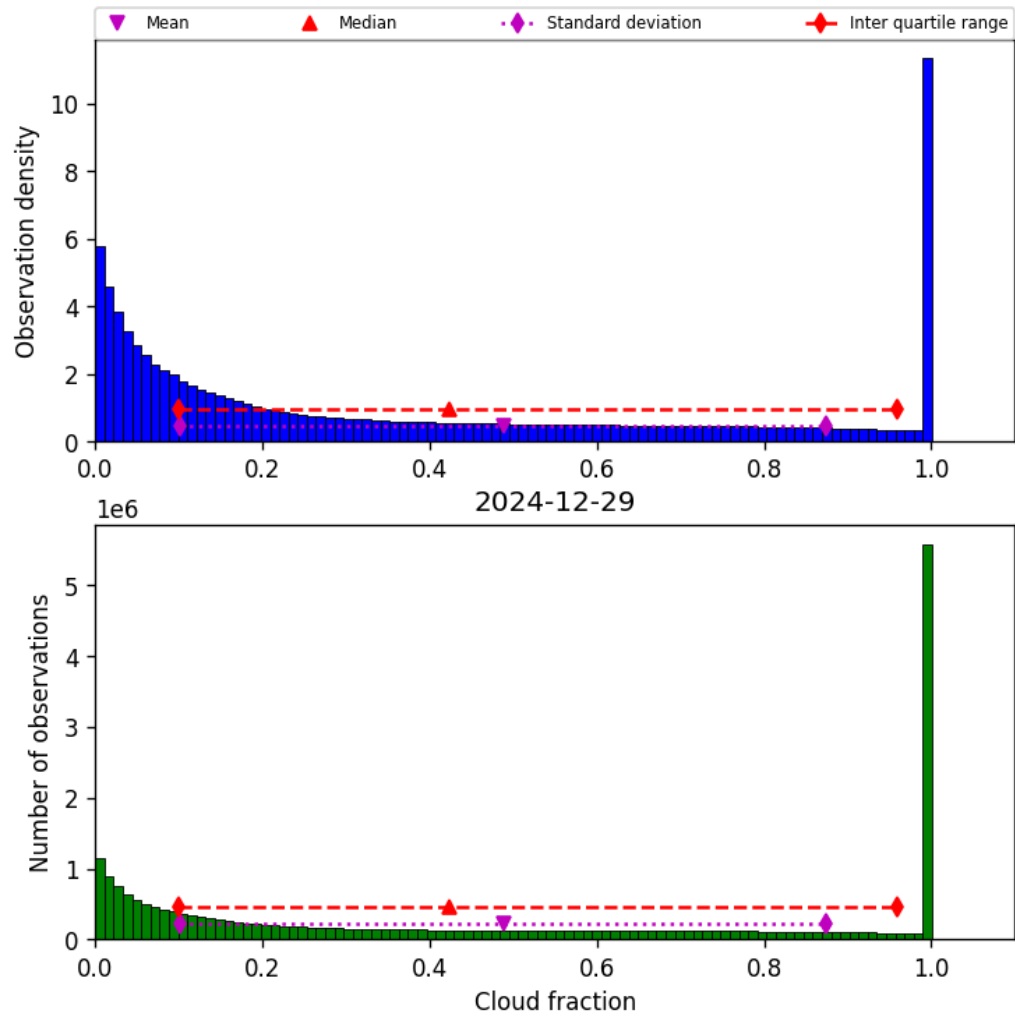
Figure 30: Histogram of “Cloud fraction” for 2024-12-29 to 2024-12-30
