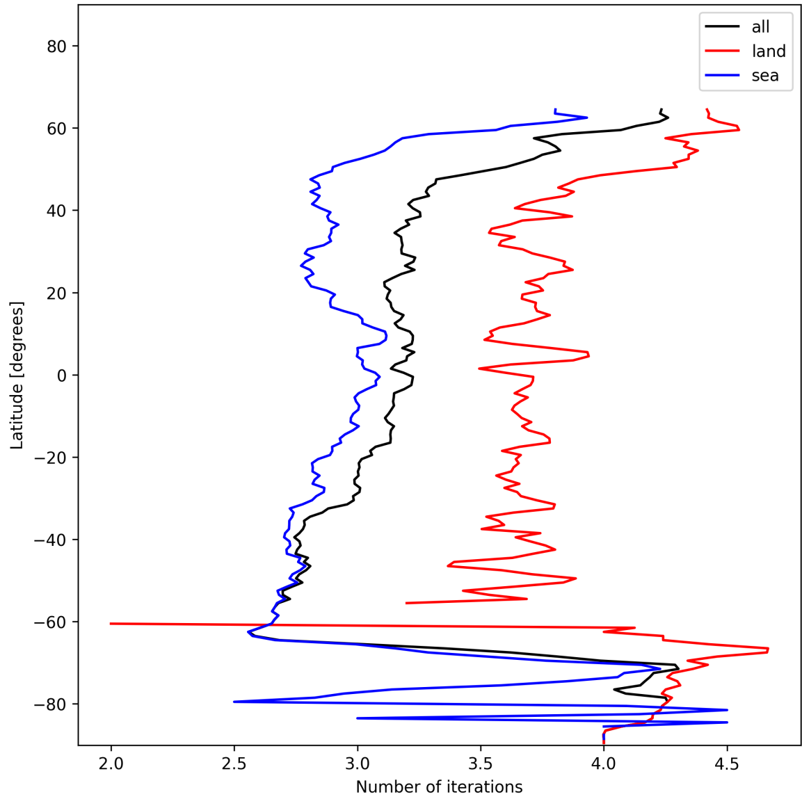
Figure 20: Zonal average of “Number of iterations” for 2024-12-29 to 2024-12-30.
