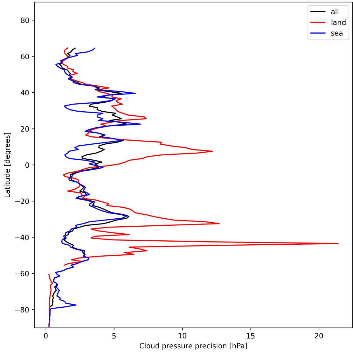
Figure 12: Zonal average of “Cloud pressure precision” for 2024-12-29 to 2024-12-30.
