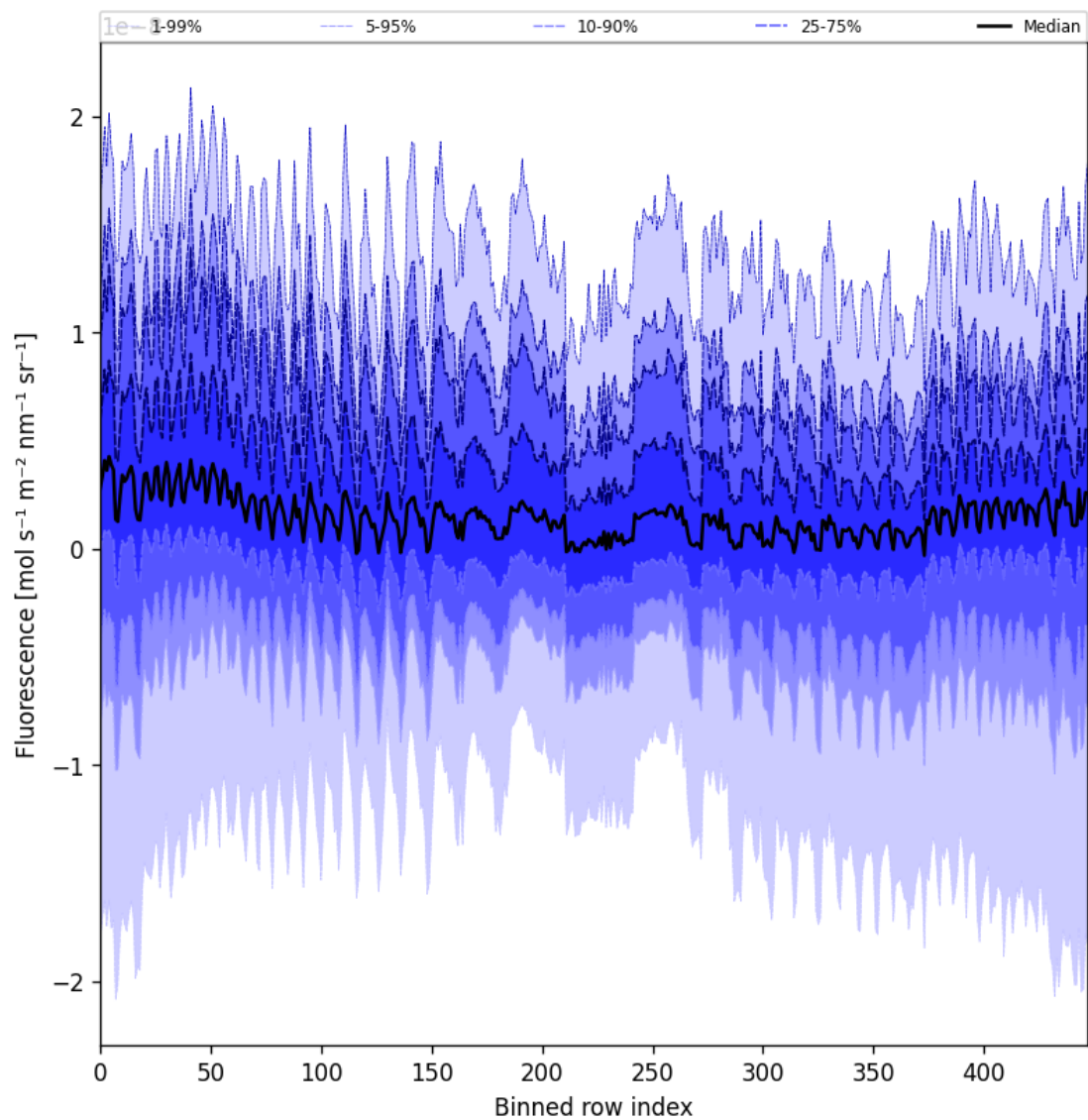
Figure 55: Along track statistics of "Fluorescence" for 2024-12-29 to 2024-12-30
