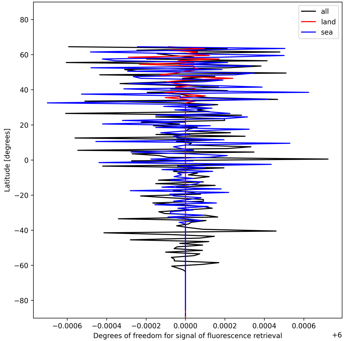
Figure 24: Zonal average of “Degrees of freedom for signal of fluorescence retrieval” for 2024-12-29 to 2024-12-30.
