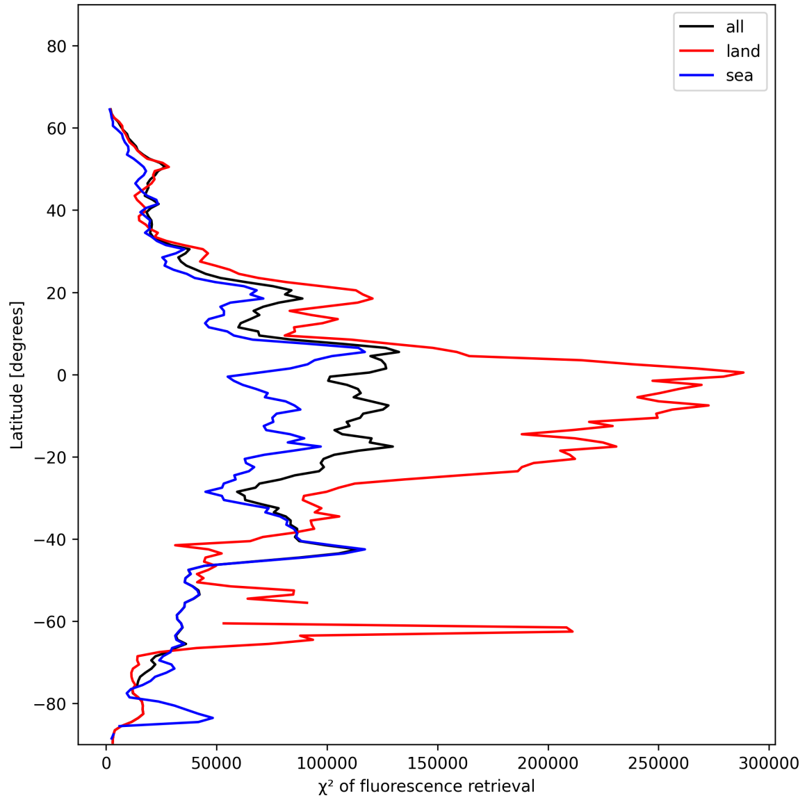
Figure 23: Zonal average of “ \chi^2 of fluorescence retrieval” for 2024-12-29 to 2024-12-30.
