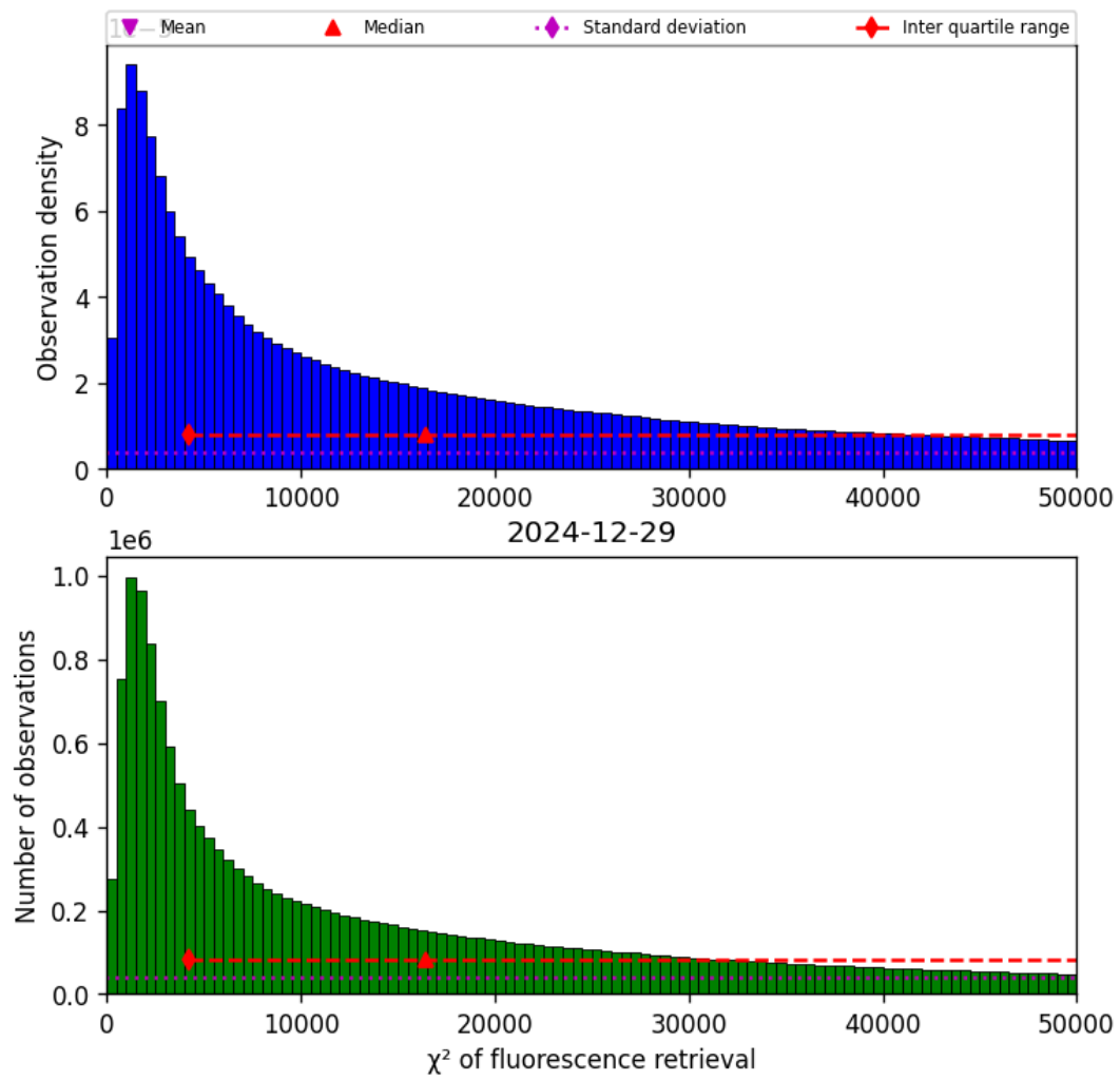
Figure 40: Histogram of “ \chi^2 of fluorescence retrieval” for 2024-12-29 to 2024-12-30
