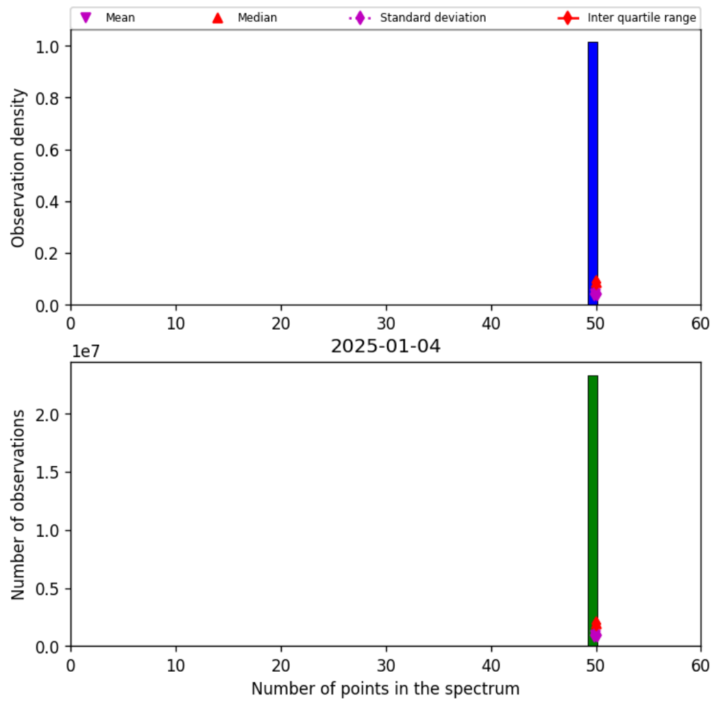
Figure 42: Histogram of "Number of points in the spectrum" for 2025-01-04 to 2025-01-04
