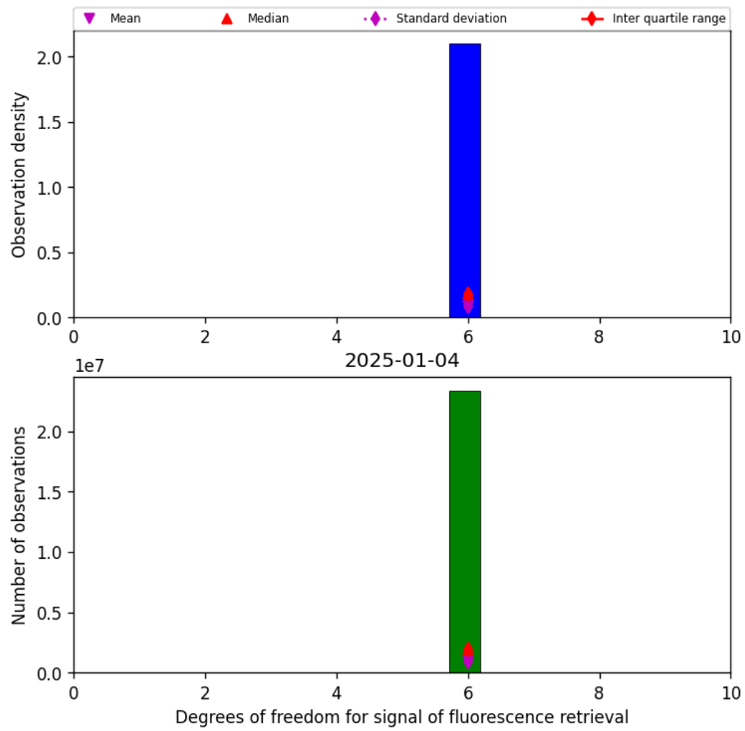
Figure 41: Histogram of “Degrees of freedom for signal of fluorescence retrieval” for 2025-01-04 to 2025-01-04
