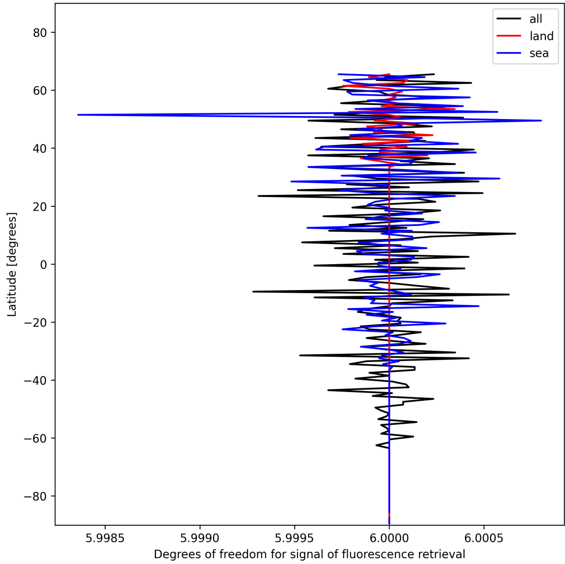
Figure 24: Zonal average of “Degrees of freedom for signal of fluorescence retrieval” for 2025-01-04 to 2025-01-04.
