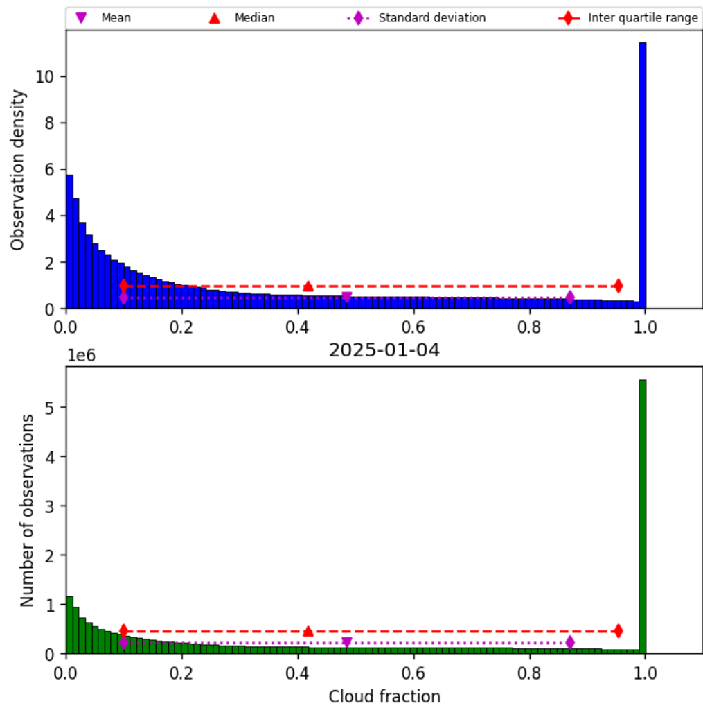
Figure 30: Histogram of “Cloud fraction” for 2025-01-04 to 2025-01-04
