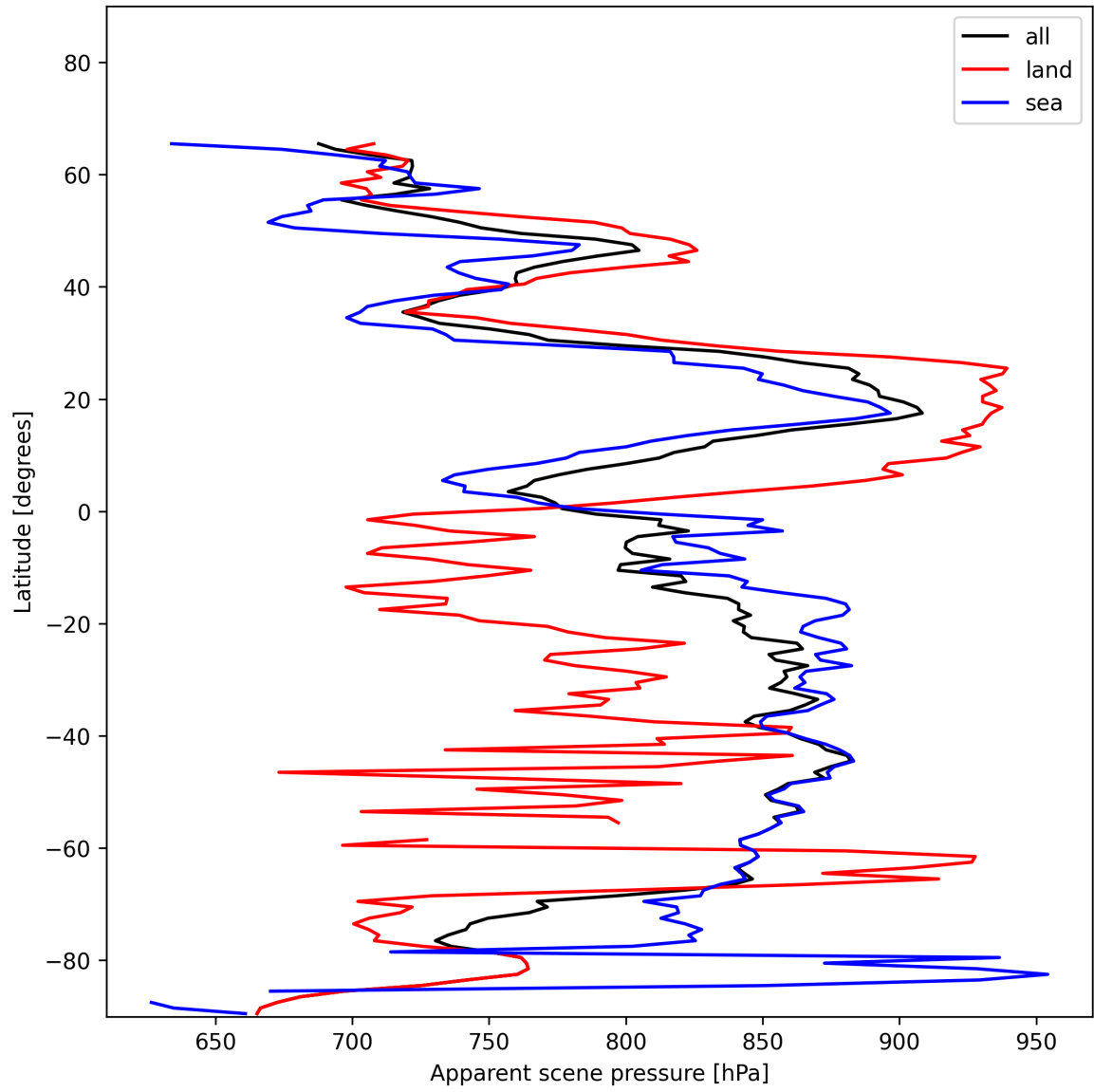
Figure 17: Zonal average of “Apparent scene pressure” for 2025-01-04 to 2025-01-04.
