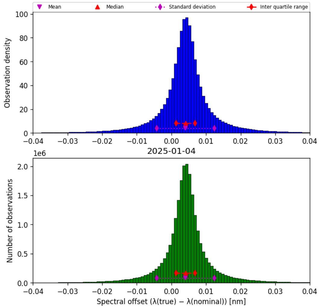
Figure 43: Histogram of “Spectral offset ( \lambda_{\text{true}} - \lambda_{\text{nominal}} )” for 2025-01-04 to 2025-01-04
