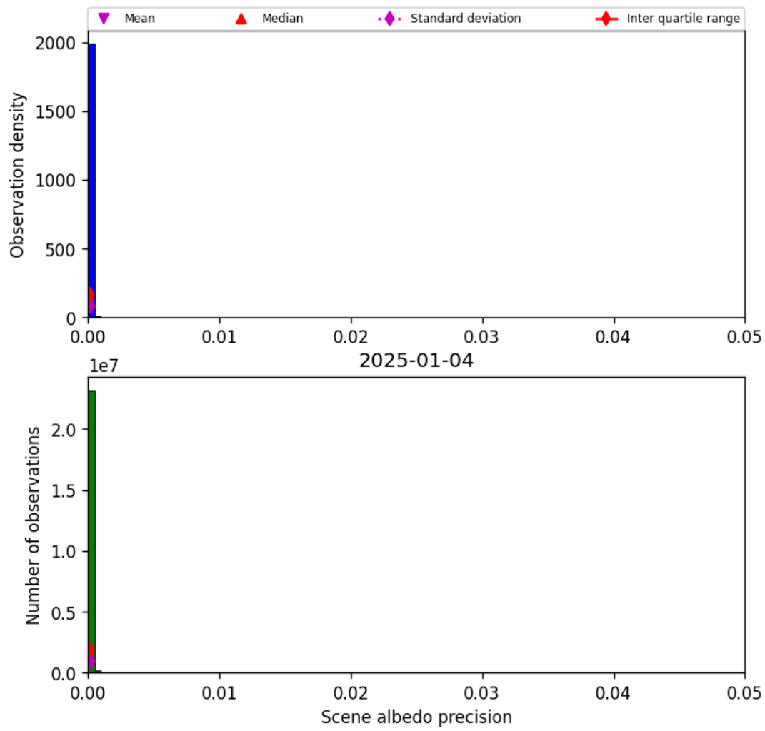
Figure 33: Histogram of “Scene albedo precision” for 2025-01-04 to 2025-01-04
