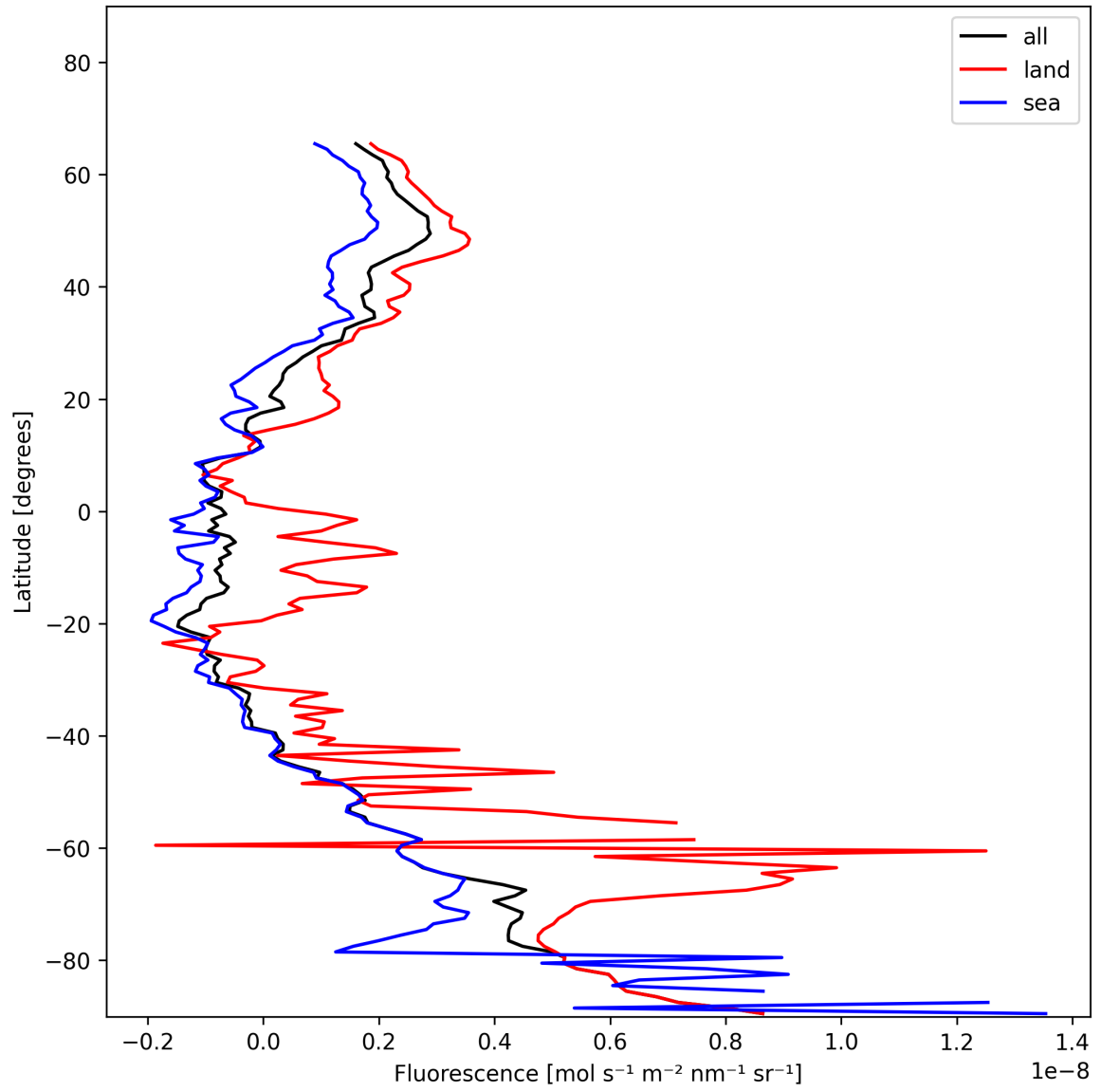
Figure 21: Zonal average of "Fluorescence" for 2025-01-04 to 2025-01-04.
