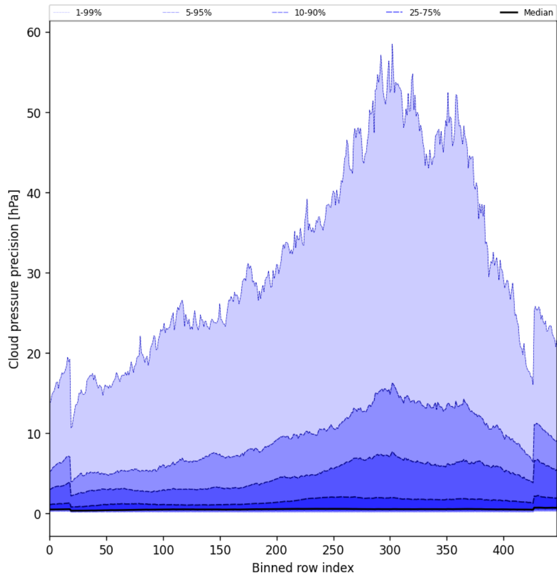
Figure 46: Along track statistics of “Cloud pressure precision” for 2025-01-04 to 2025-01-04
