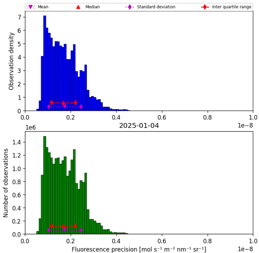
Figure 39: Histogram of “Fluorescence precision” for 2025-01-04 to 2025-01-04
