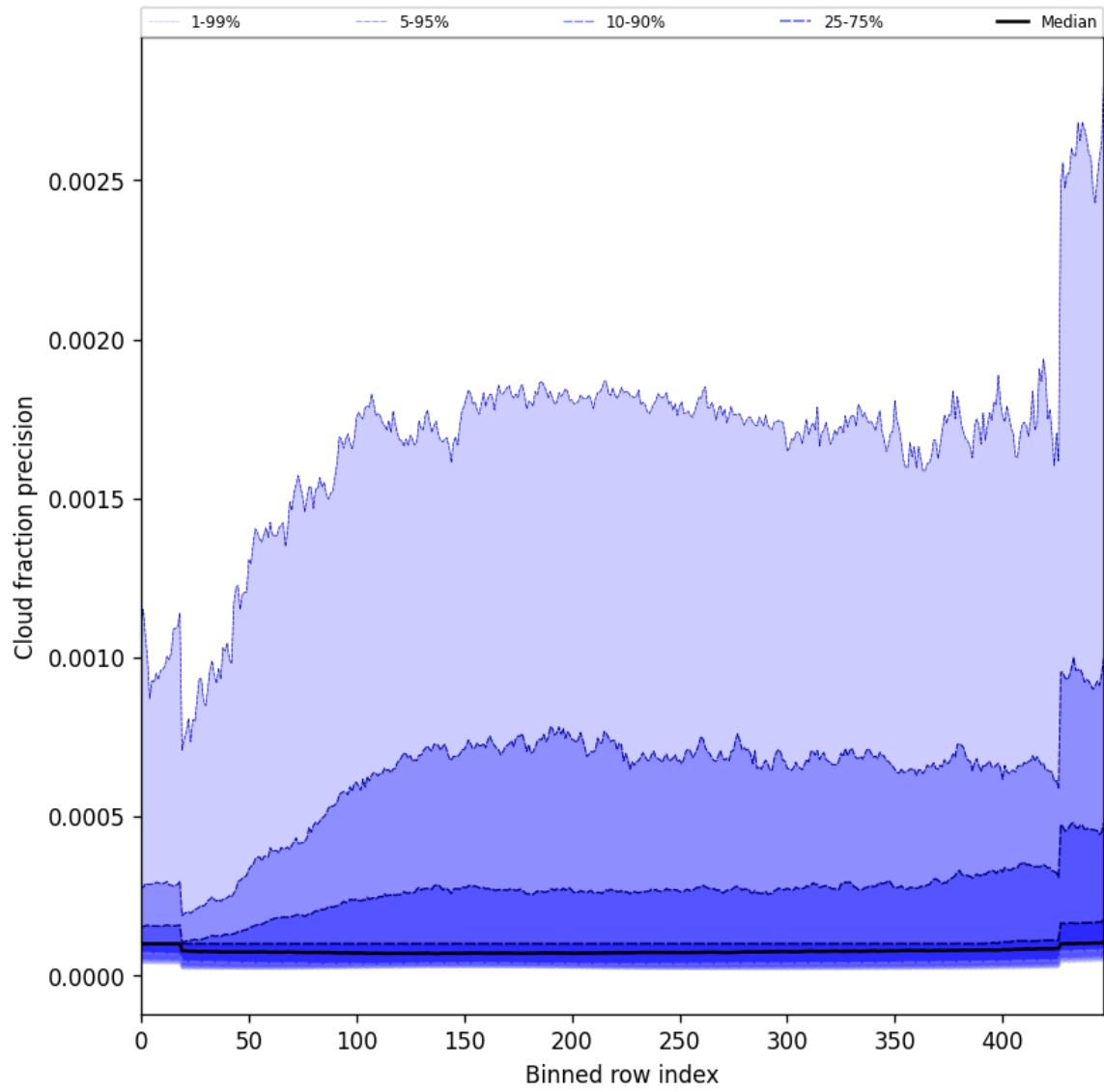
Figure 48: Along track statistics of “Cloud fraction precision” for 2025-01-04 to 2025-01-04
