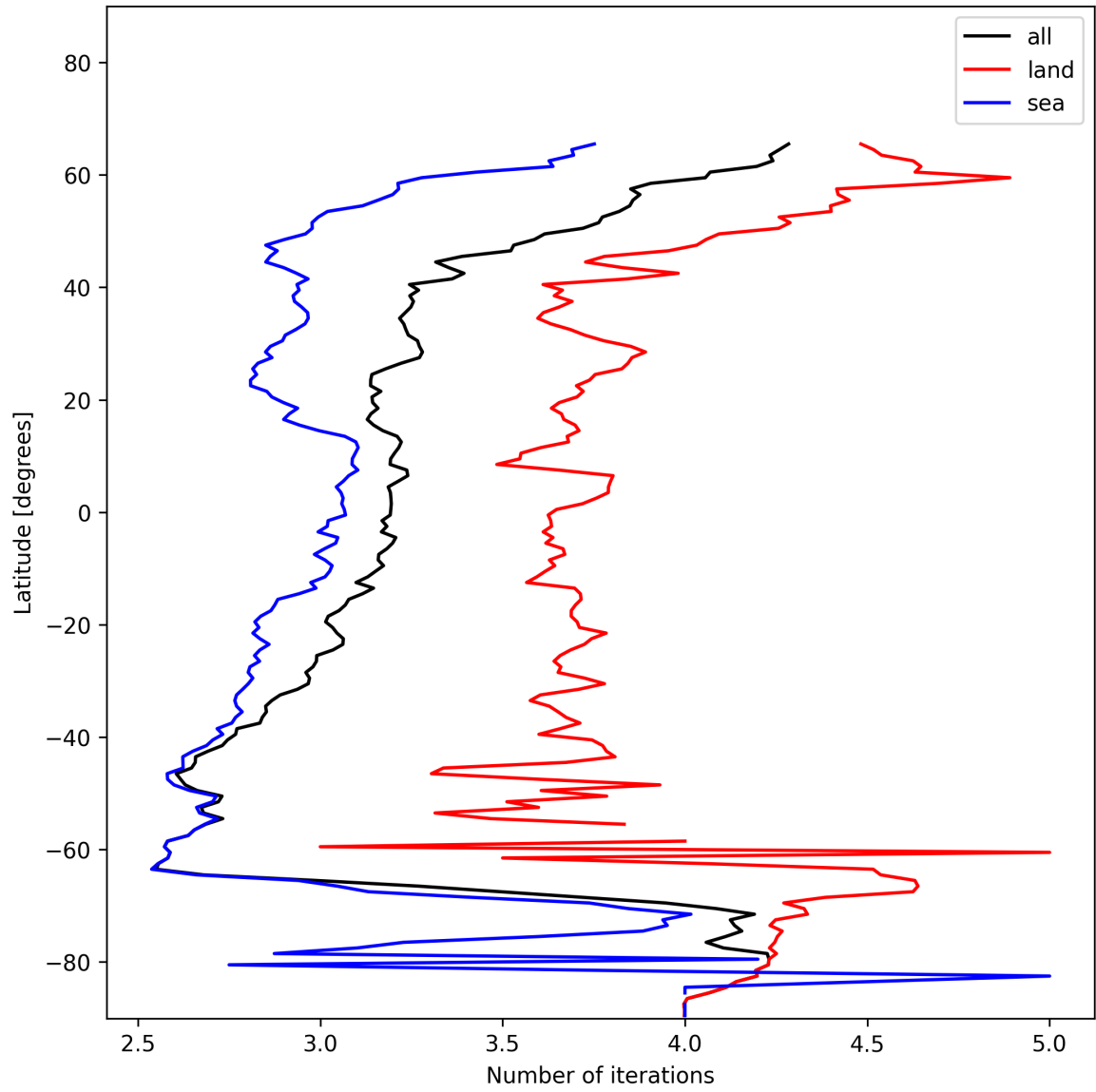
Figure 20: Zonal average of “Number of iterations” for 2025-01-04 to 2025-01-04.
