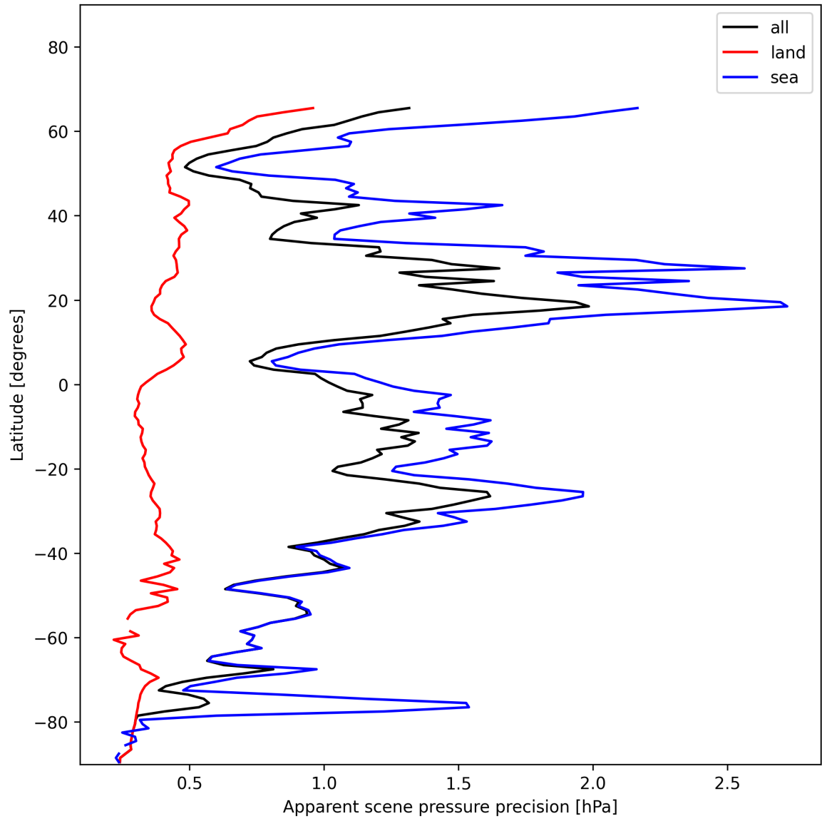
Figure 18: Zonal average of “Apparent scene pressure precision” for 2025-01-04 to 2025-01-04.
