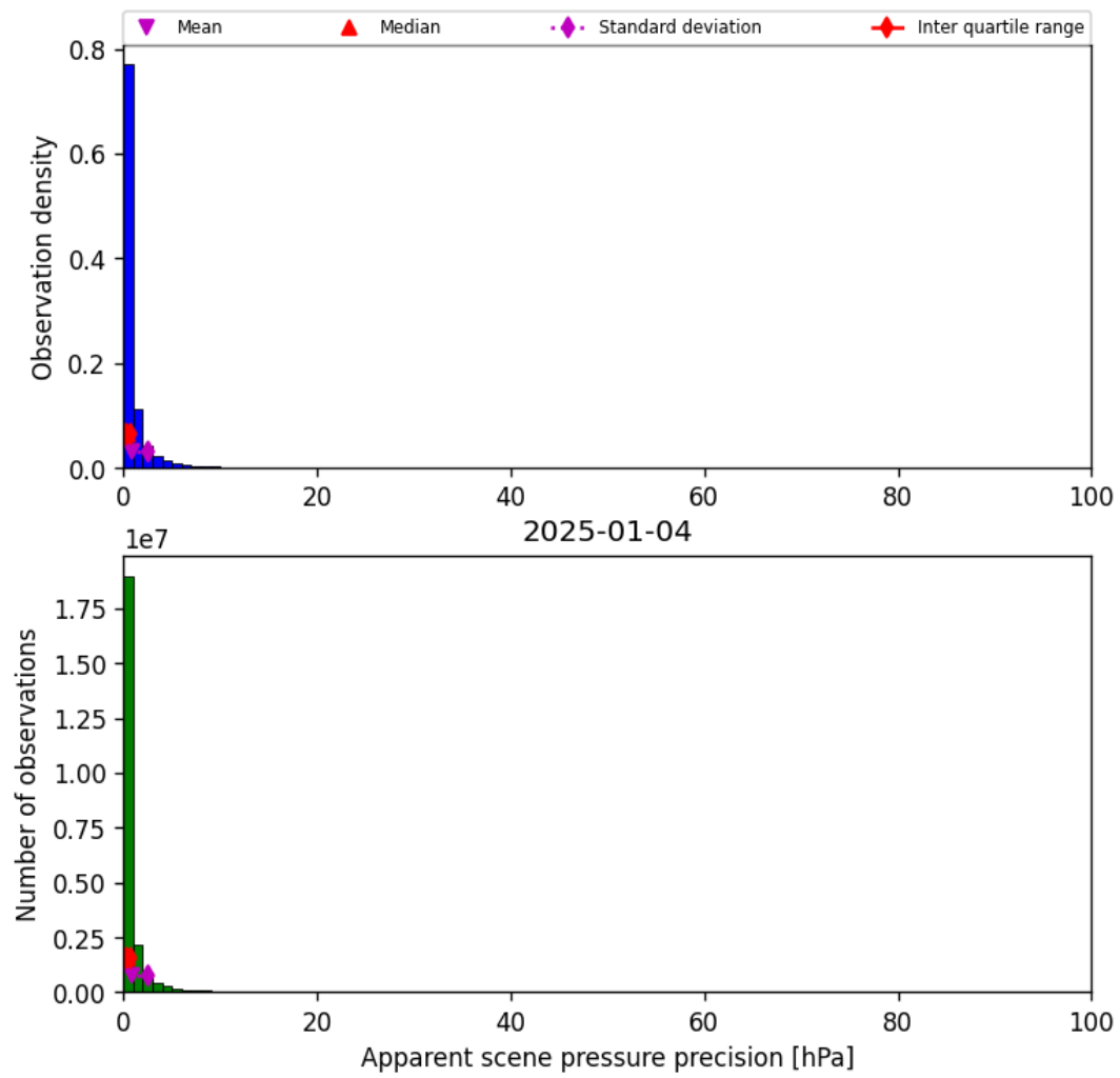
Figure 35: Histogram of “Apparent scene pressure precision” for 2025-01-04 to 2025-01-04
