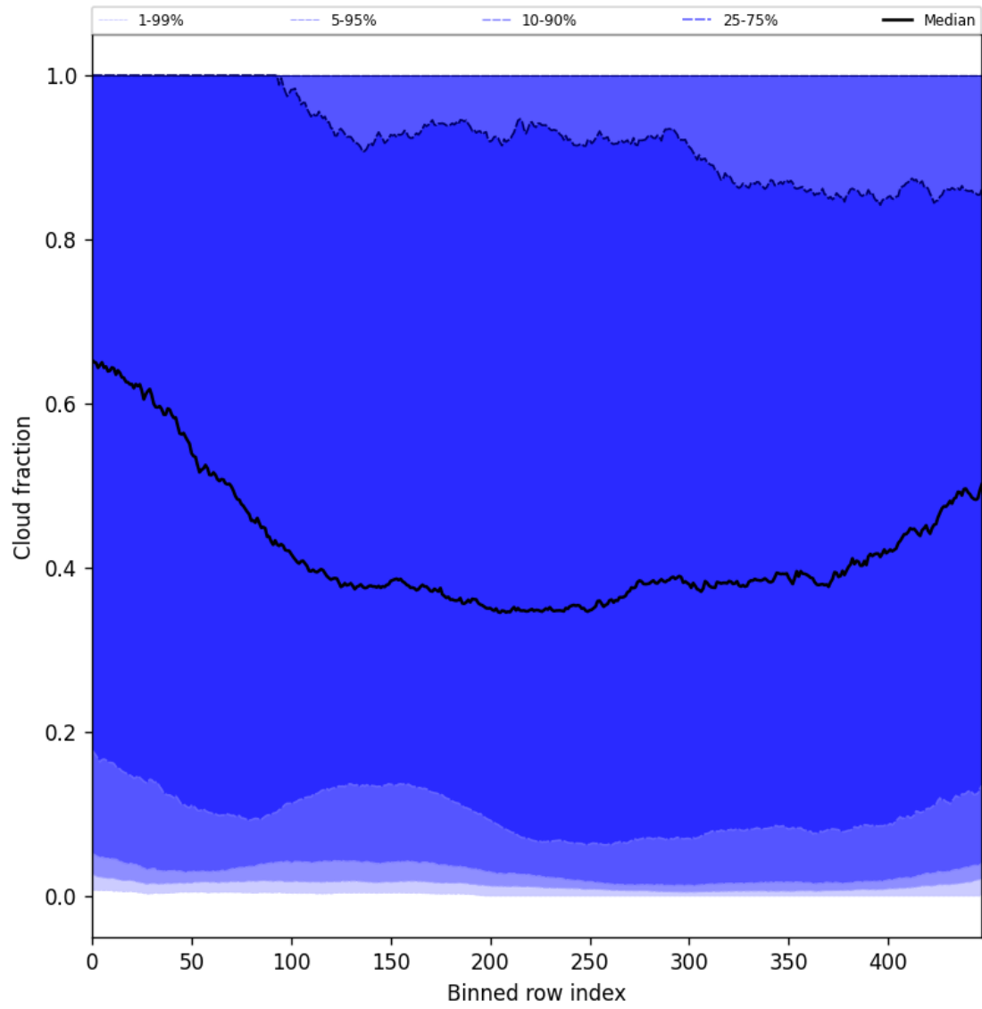
Figure 47: Along track statistics of “Cloud fraction” for 2025-01-04 to 2025-01-04
