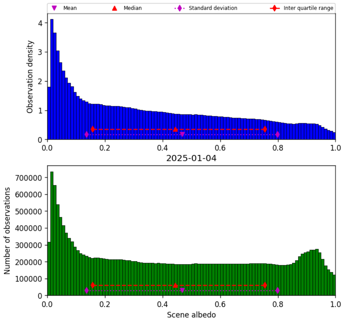
Figure 32: Histogram of “Scene albedo” for 2025-01-04 to 2025-01-04
