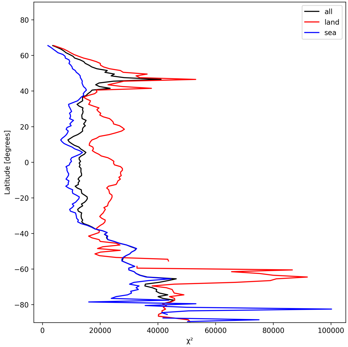
Figure 19: Zonal average of “ \chi^2 ” for 2025-01-04 to 2025-01-04.
