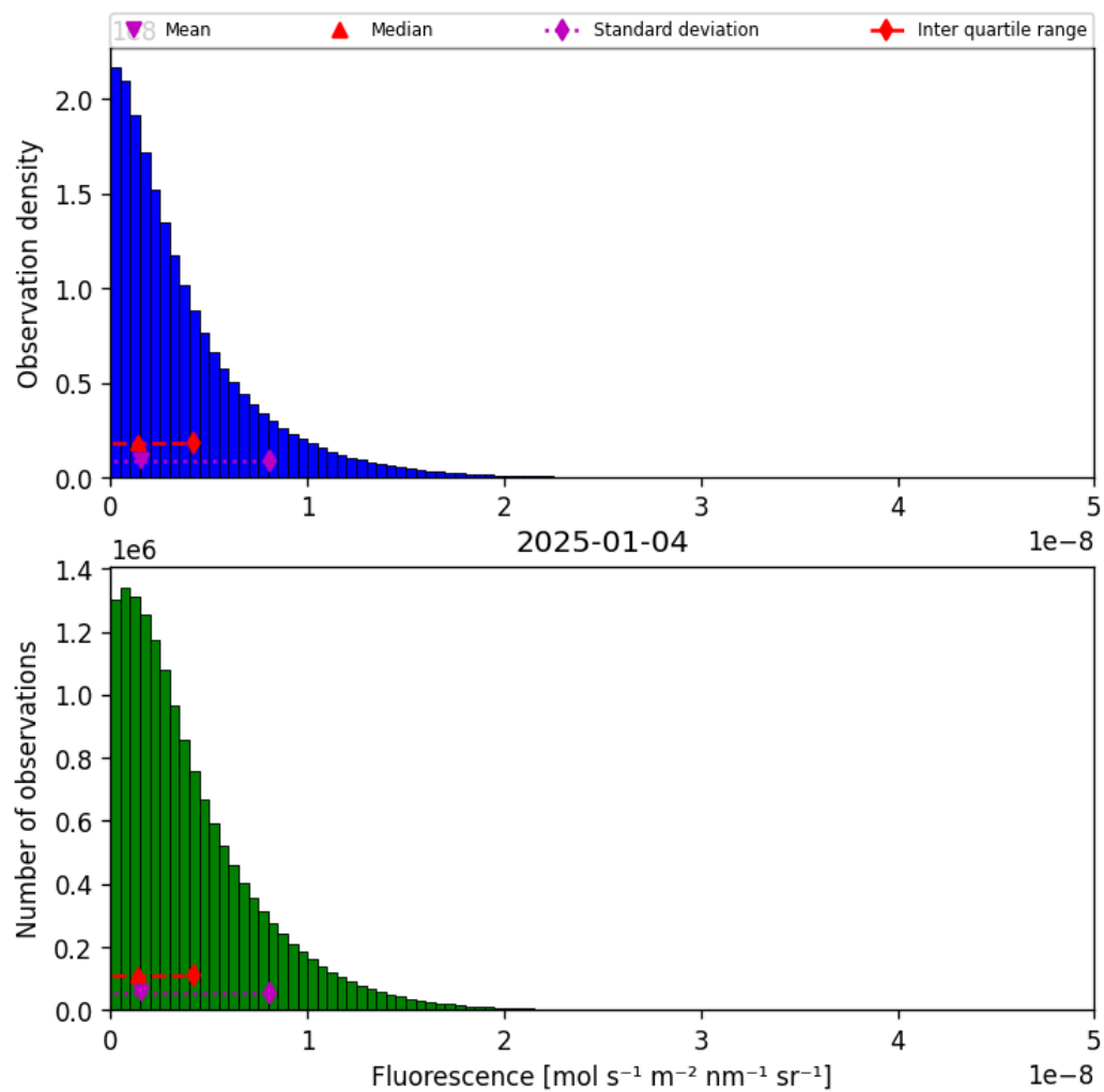
Figure 38: Histogram of “Fluorescence” for 2025-01-04 to 2025-01-04
