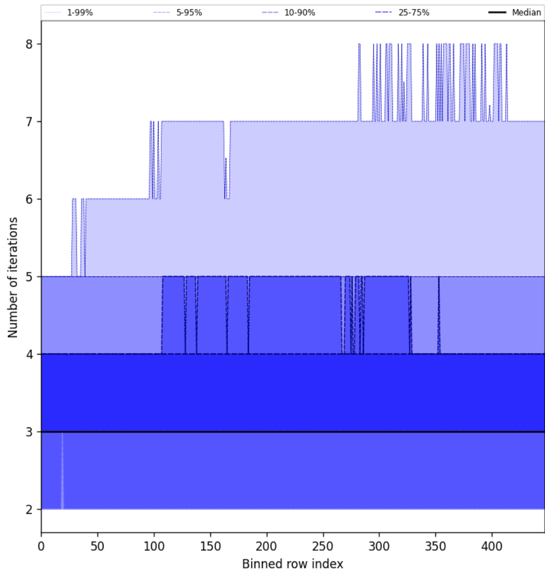
Figure 54: Along track statistics of “Number of iterations” for 2025-01-04 to 2025-01-04
