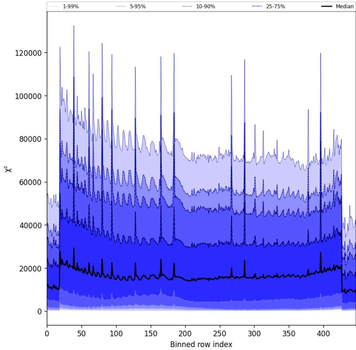
Figure 53: Along track statistics of “ \chi^2 ” for 2025-01-04 to 2025-01-04
