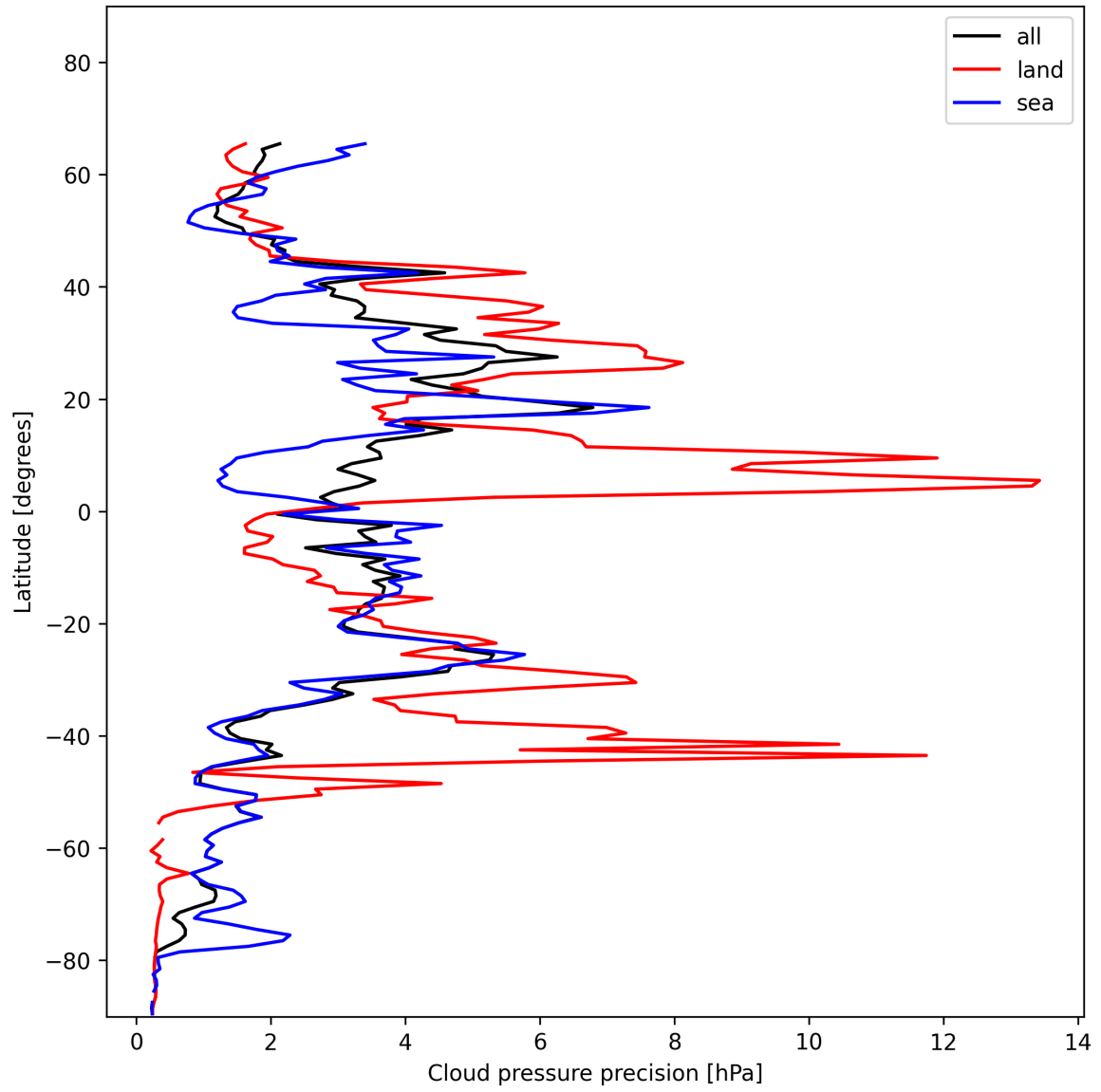
Figure 12: Zonal average of "Cloud pressure precision" for 2025-01-04 to 2025-01-04.
