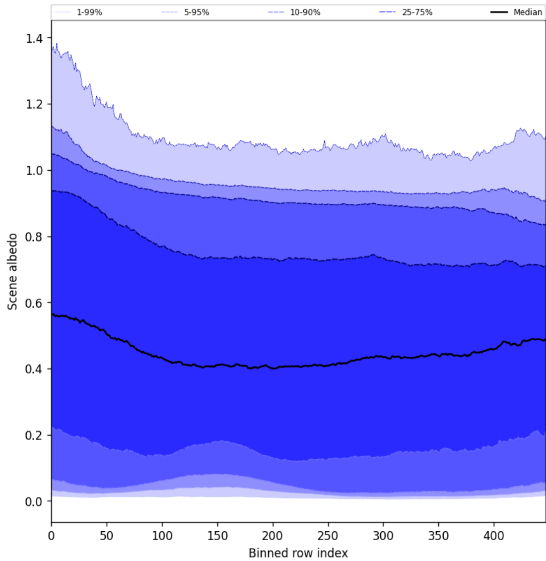
Figure 49: Along track statistics of “Scene albedo” for 2025-01-04 to 2025-01-04
