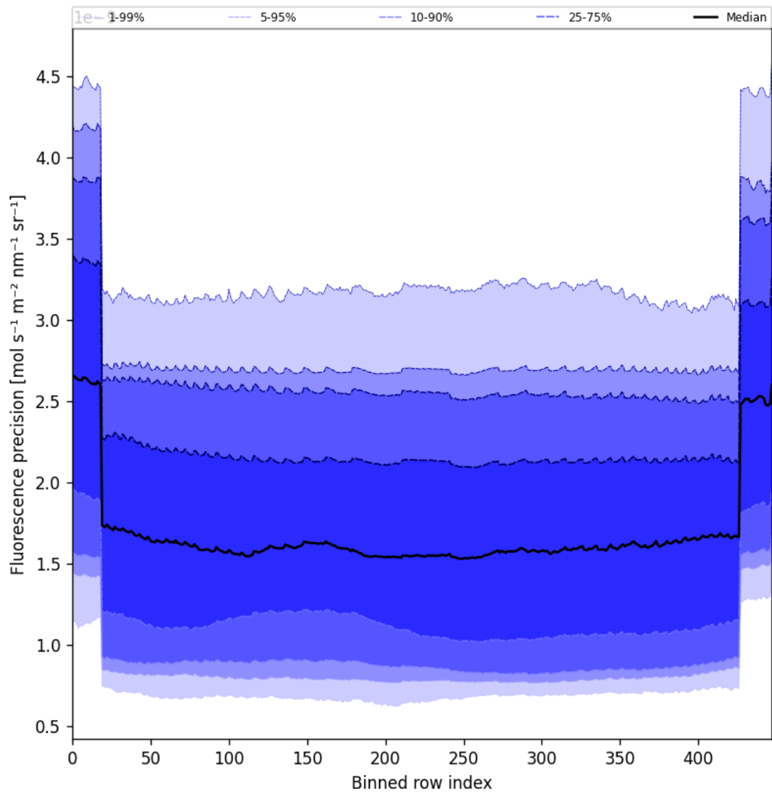
Figure 56: Along track statistics of “Fluorescence precision” for 2025-01-04 to 2025-01-04
