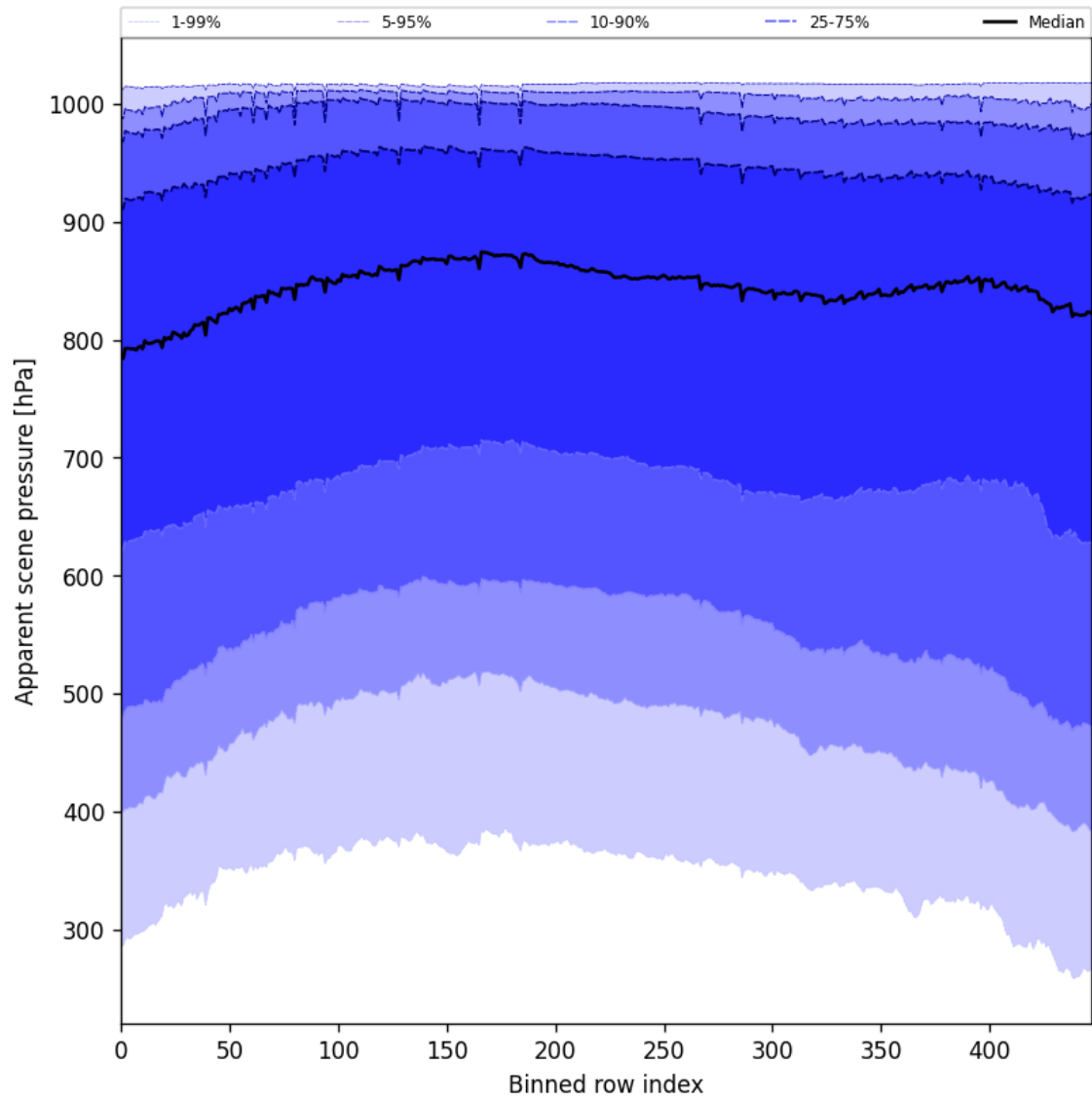
Figure 51: Along track statistics of “Apparent scene pressure” for 2025-01-04 to 2025-01-04
