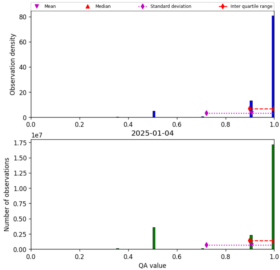
Figure 27: Histogram of “QA value” for 2025-01-04 to 2025-01-04
