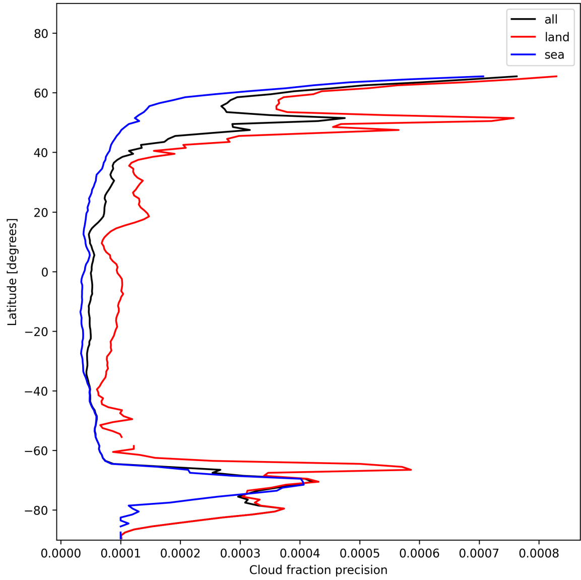
Figure 14: Zonal average of “Cloud fraction precision” for 2025-01-04 to 2025-01-04.
