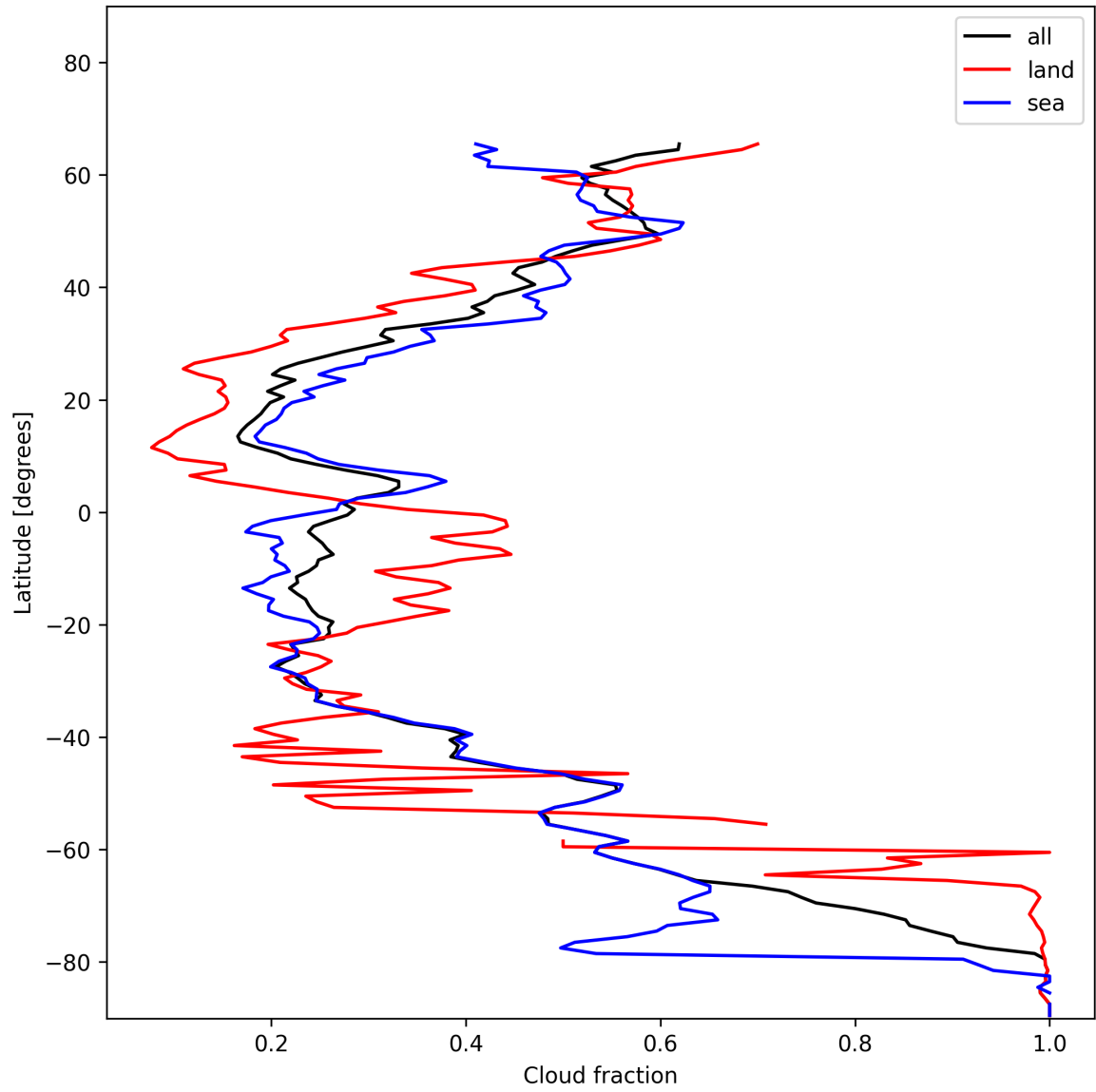
Figure 13: Zonal average of “Cloud fraction” for 2025-01-04 to 2025-01-04.
