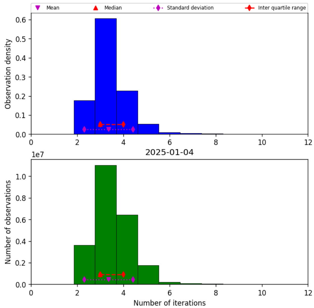
Figure 37: Histogram of “Number of iterations” for 2025-01-04 to 2025-01-04
