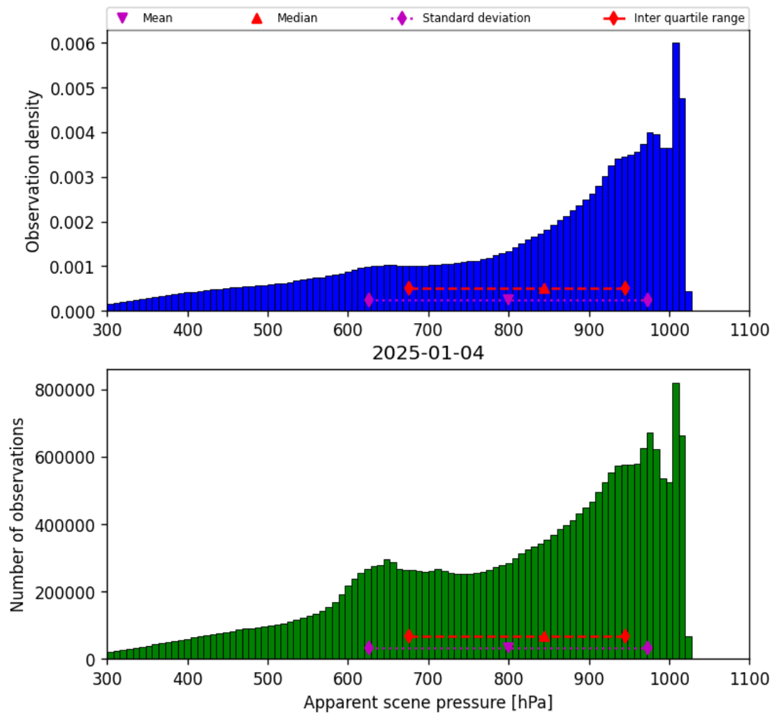
Figure 34: Histogram of “Apparent scene pressure” for 2025-01-04 to 2025-01-04
