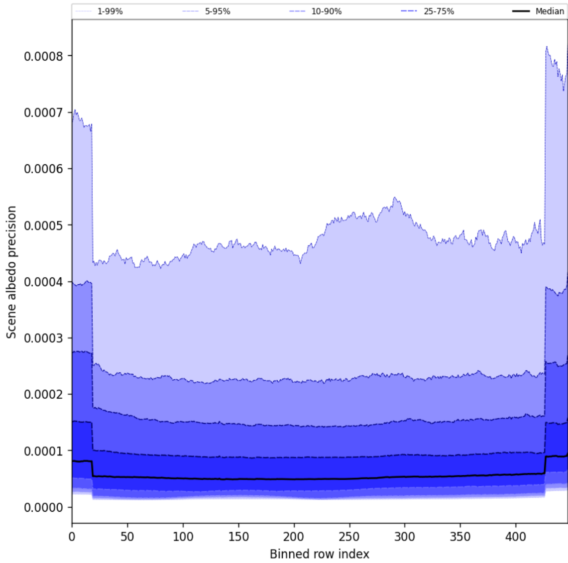
Figure 50: Along track statistics of “Scene albedo precision” for 2025-01-04 to 2025-01-04
