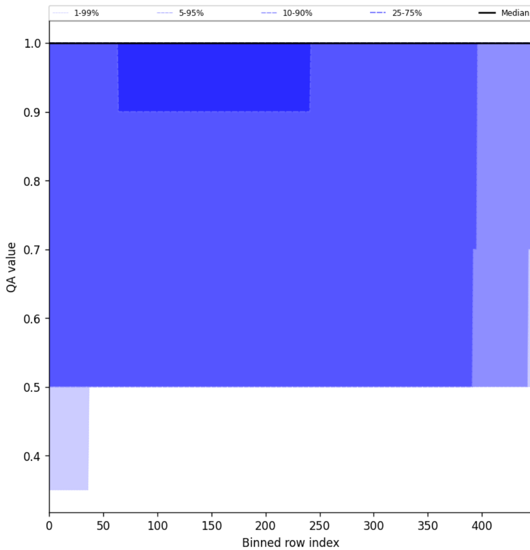
Figure 44: Along track statistics of “QA value” for 2025-01-04 to 2025-01-04
