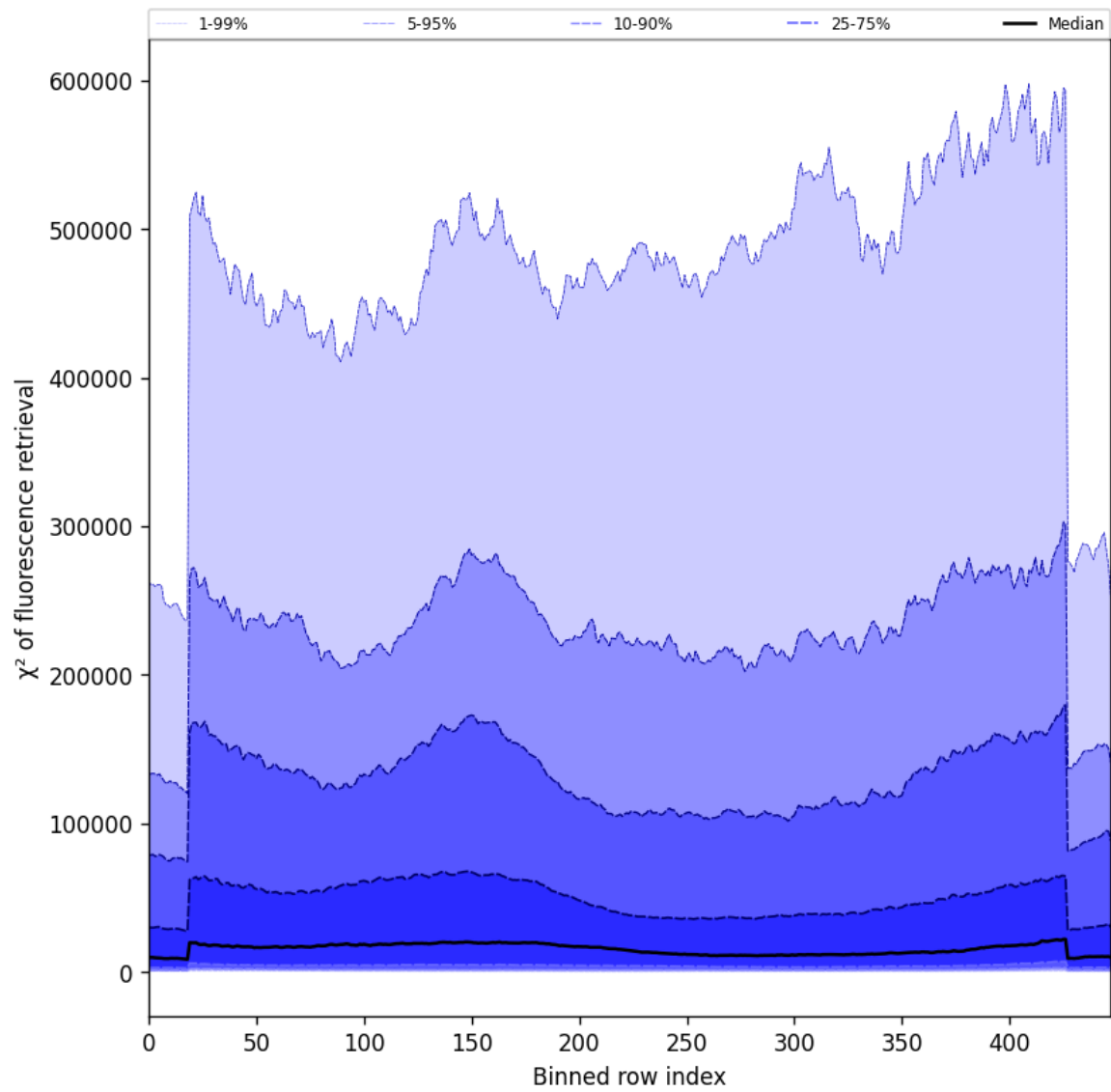
Figure 57: Along track statistics of “ \chi^2 of fluorescence retrieval” for 2025-01-04 to 2025-01-04
