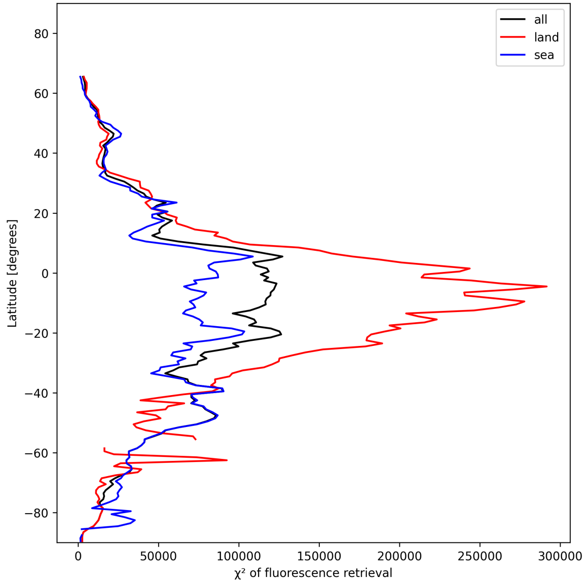
Figure 23: Zonal average of “ \chi^2 of fluorescence retrieval” for 2025-01-04 to 2025-01-04.
