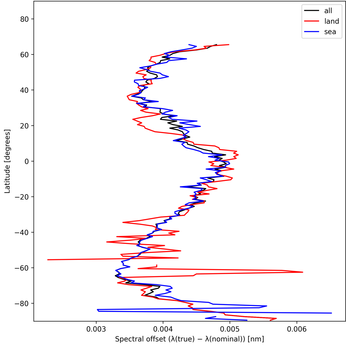
Figure 26: Zonal average of “Spectral offset ( \lambda_{\text{true}} - \lambda_{\text{nominal}} )” for 2025-01-04 to 2025-01-04.
