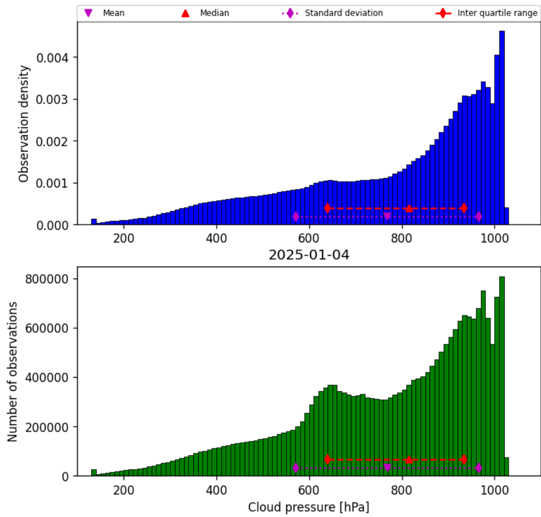
Figure 28: Histogram of “Cloud pressure” for 2025-01-04 to 2025-01-04
