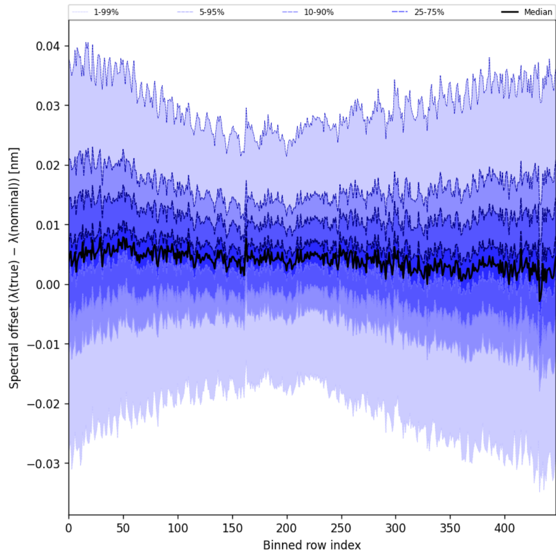
Figure 60: Along track statistics of “Spectral offset ( \lambda_{\text{true}} - \lambda_{\text{nominal}} )” for 2025-01-04 to 2025-01-04
