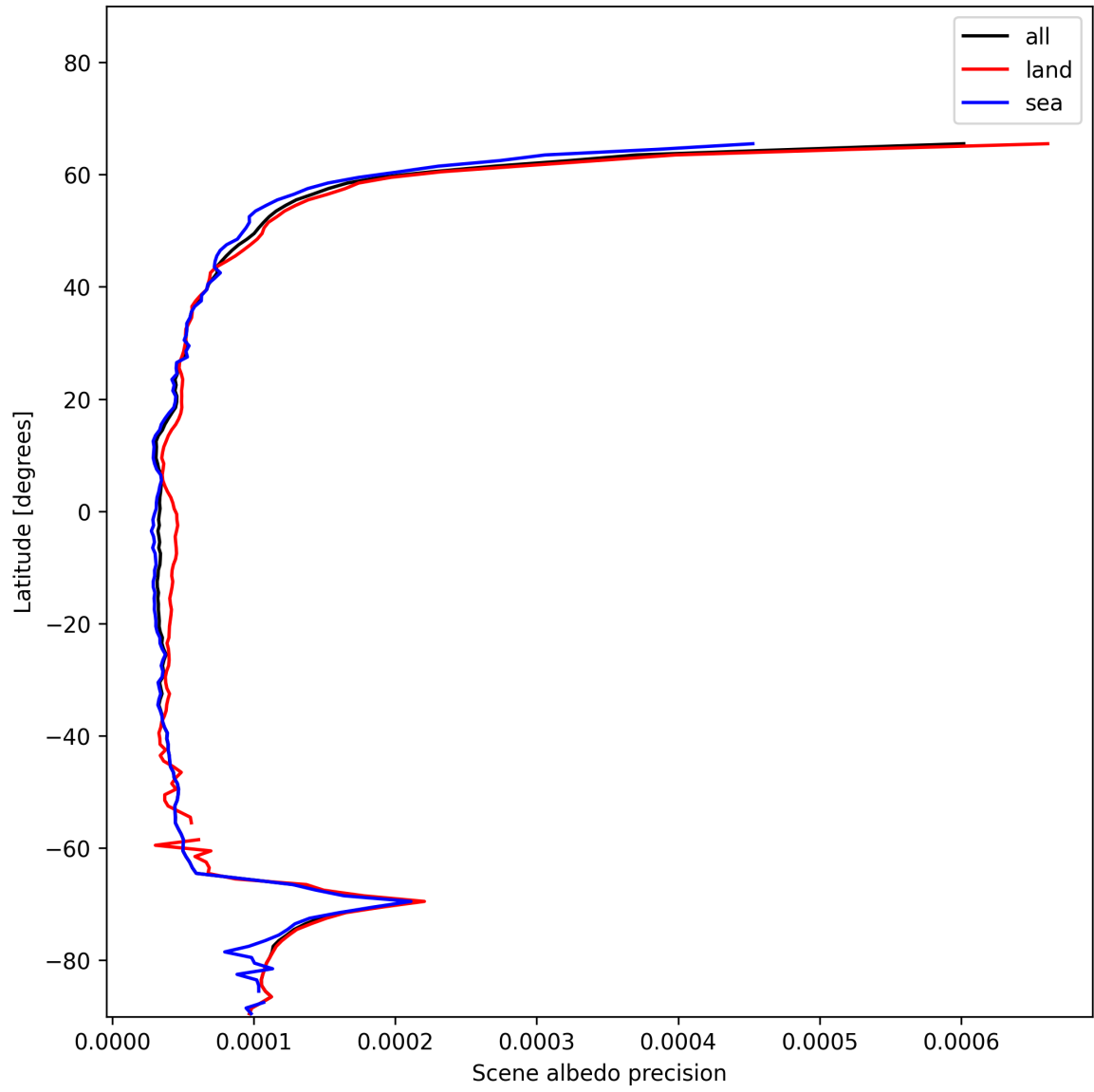
Figure 16: Zonal average of “Scene albedo precision” for 2025-01-04 to 2025-01-04.
