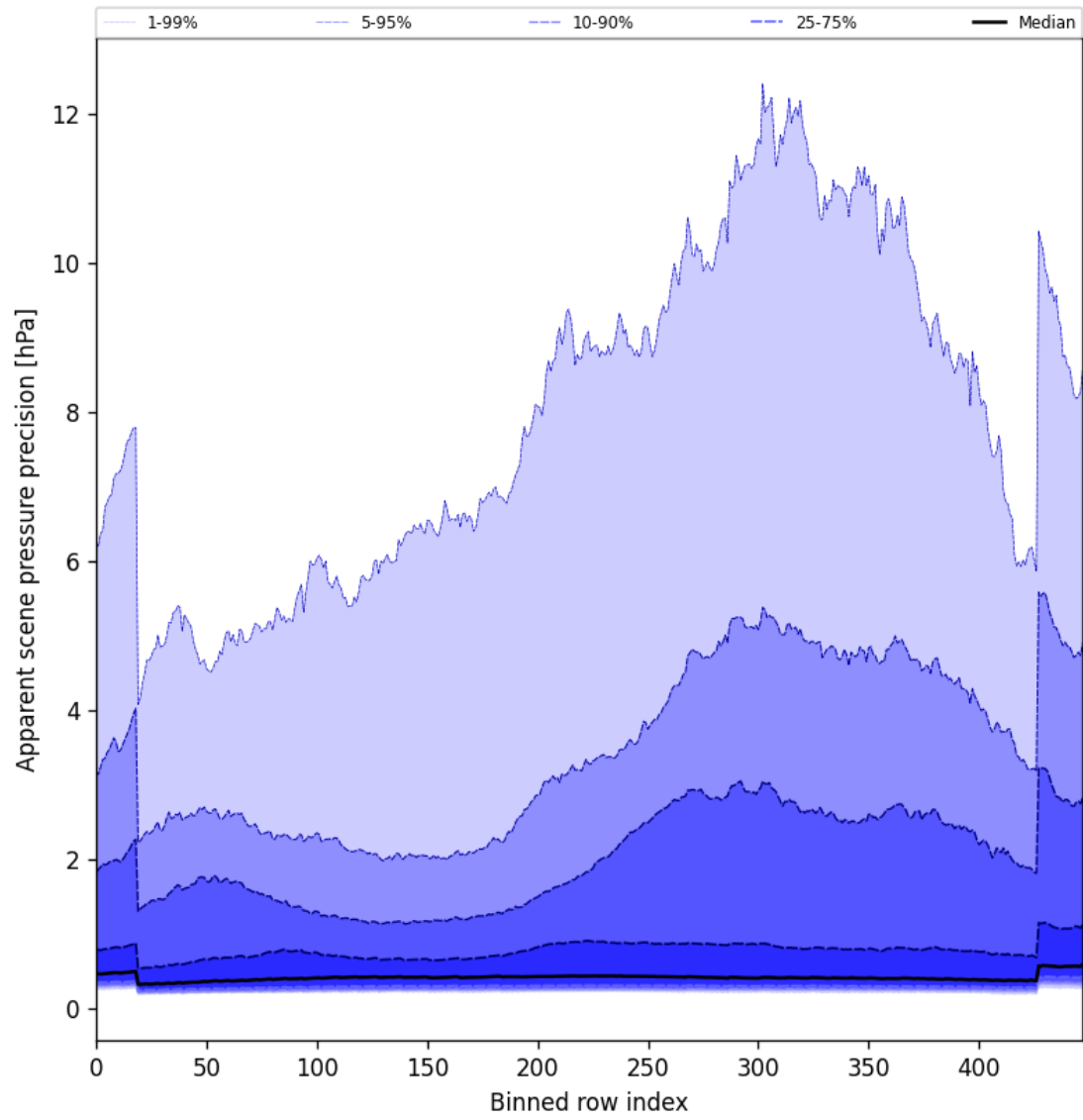
Figure 52: Along track statistics of “Apparent scene pressure precision” for 2025-01-04 to 2025-01-04
