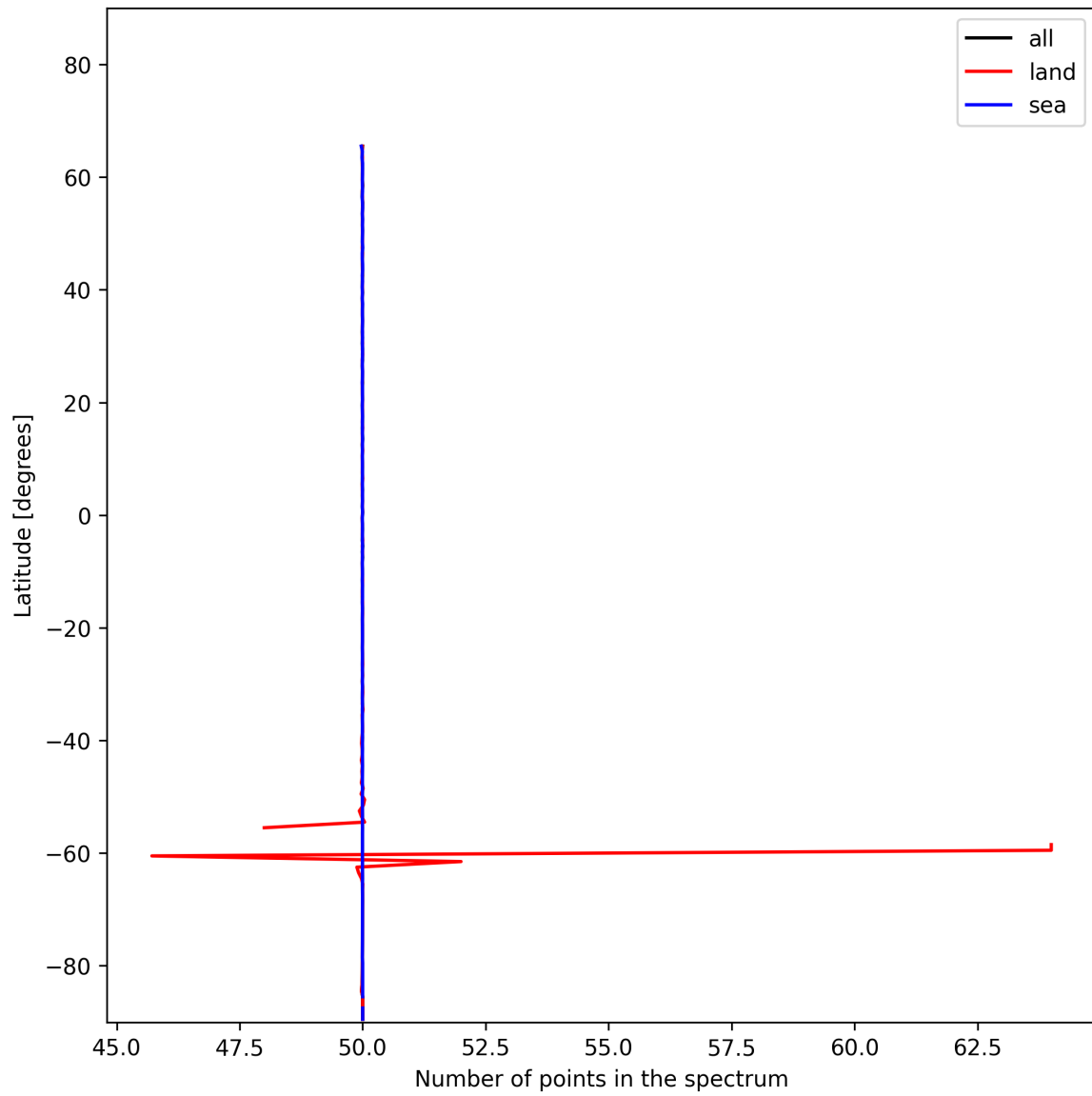
Figure 25: Zonal average of “Number of points in the spectrum” for 2025-01-04 to 2025-01-04.
