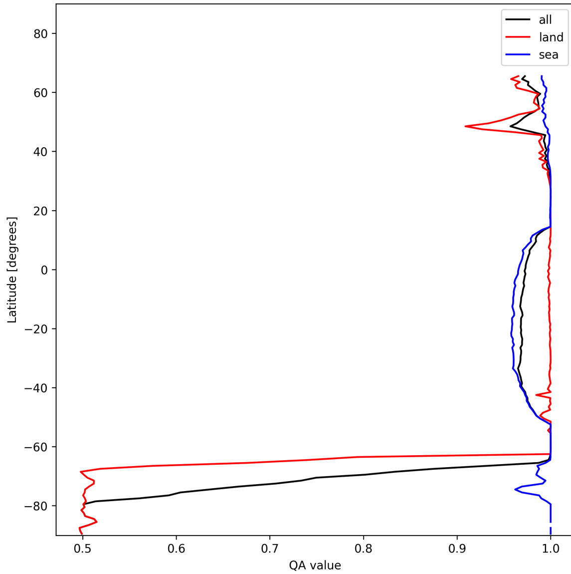
Figure 10: Zonal average of “QA value” for 2025-01-04 to 2025-01-04.
