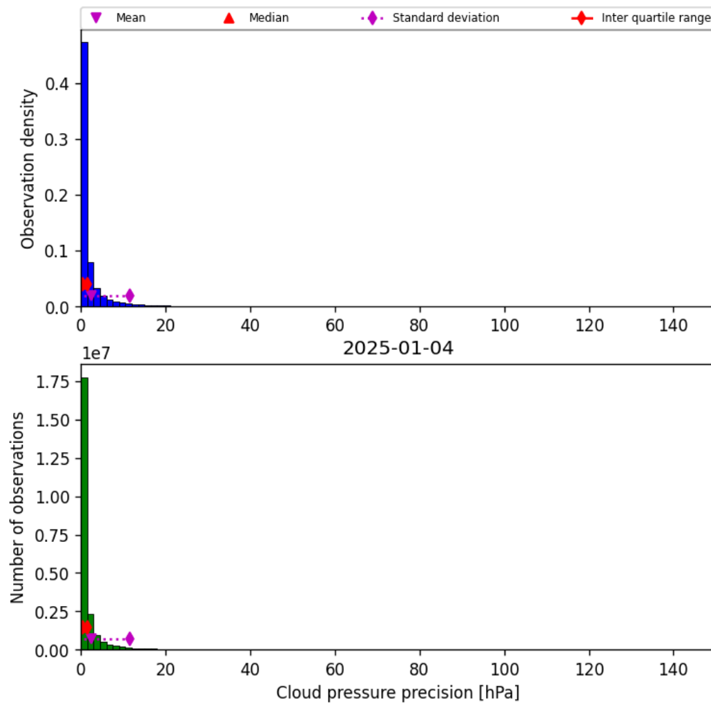
Figure 29: Histogram of “Cloud pressure precision” for 2025-01-04 to 2025-01-04
