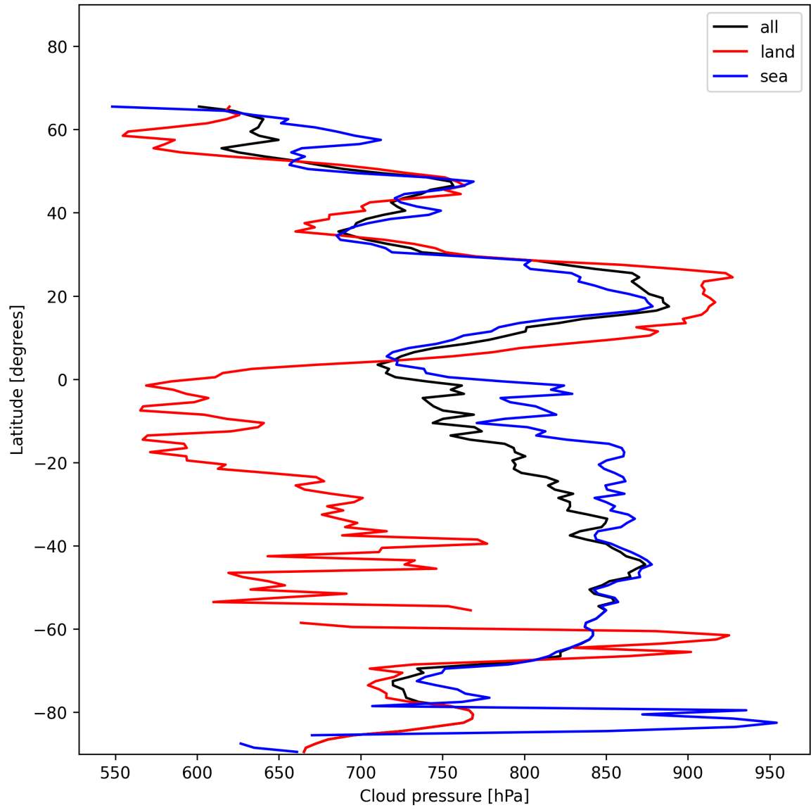
Figure 11: Zonal average of “Cloud pressure” for 2025-01-04 to 2025-01-04.
