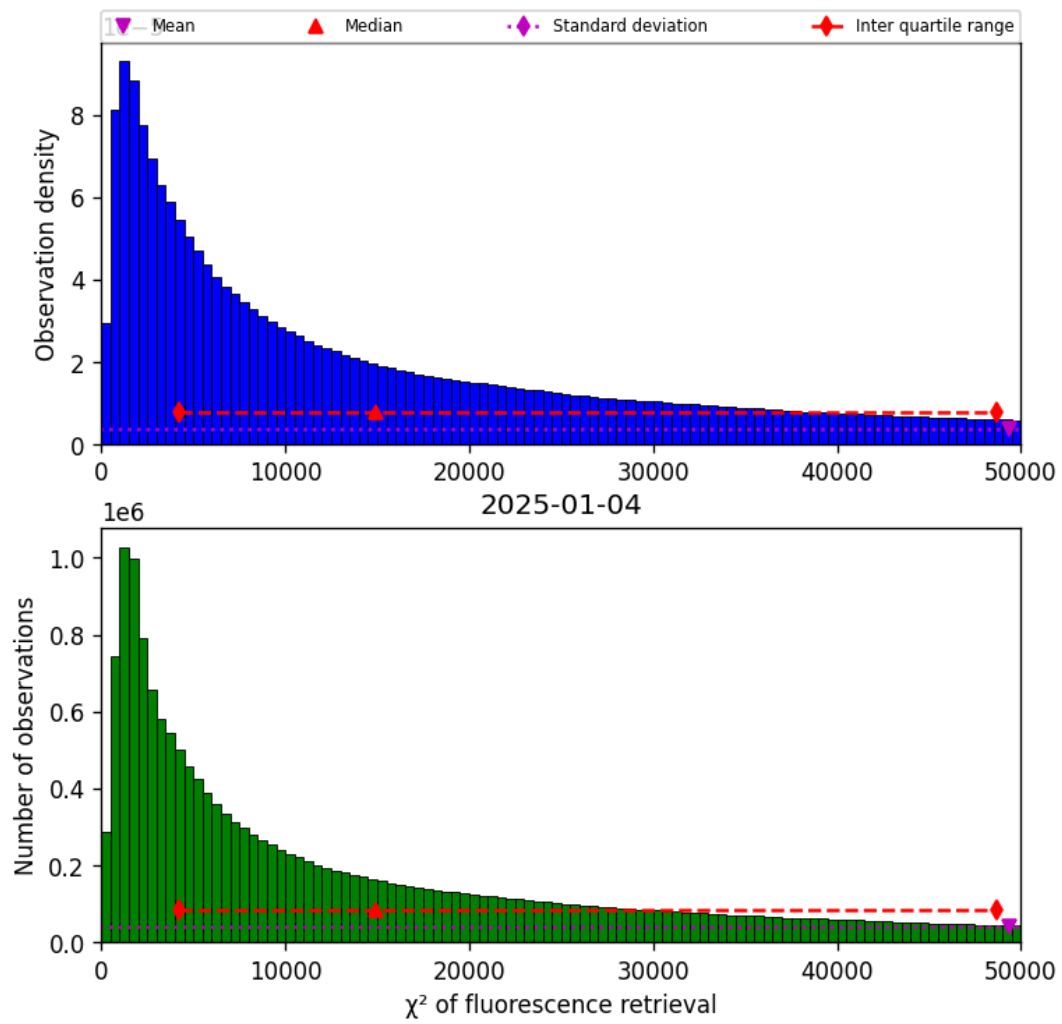
Figure 40: Histogram of “ \chi^2 of fluorescence retrieval” for 2025-01-04 to 2025-01-04
