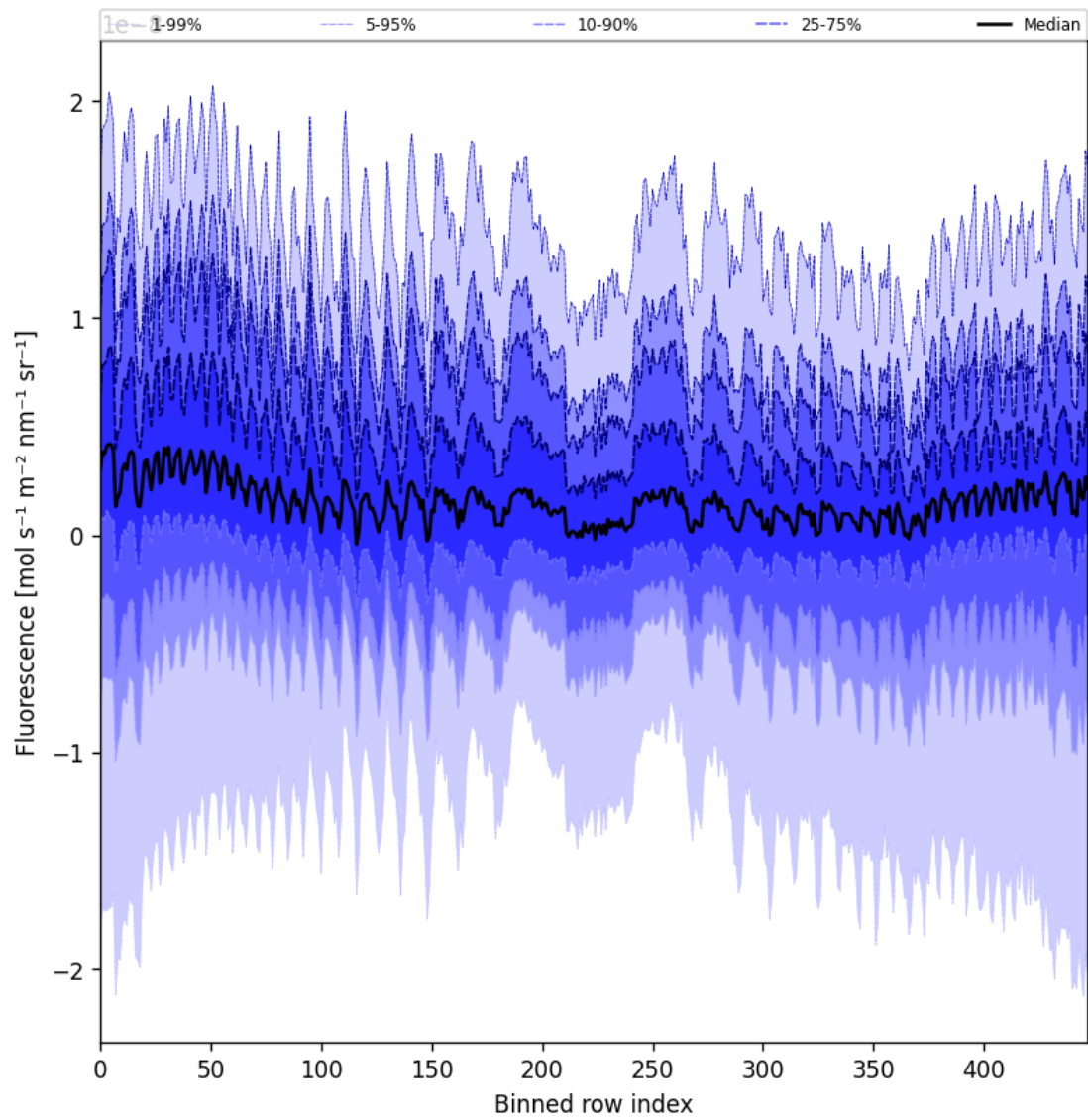
Figure 55: Along track statistics of “Fluorescence” for 2025-01-04 to 2025-01-04
