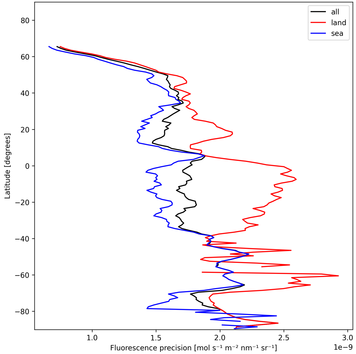
Figure 22: Zonal average of “Fluorescence precision” for 2025-01-04 to 2025-01-04.
