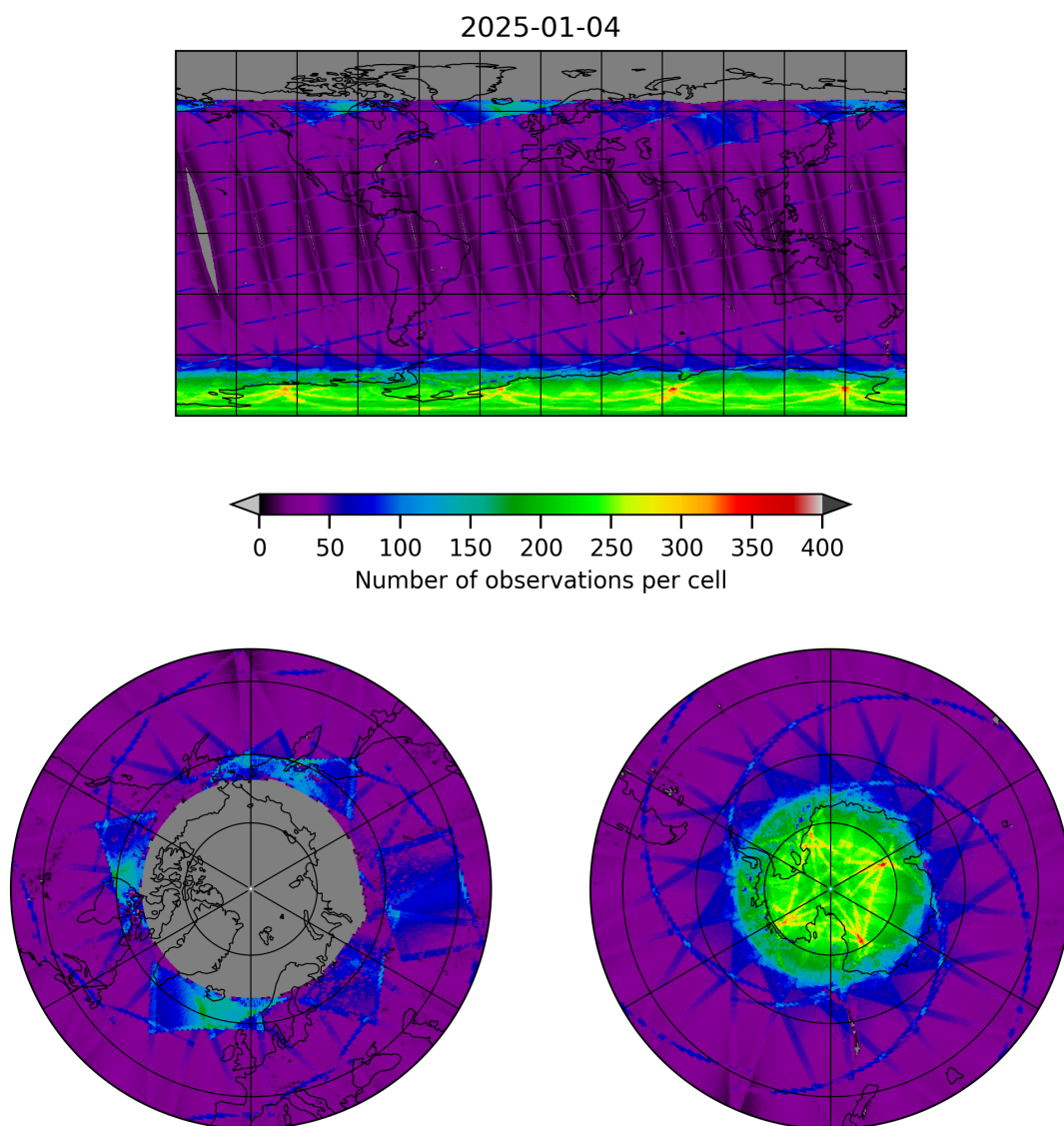
Figure 9: Map of the number of observations for 2025-01-04 to 2025-01-04
