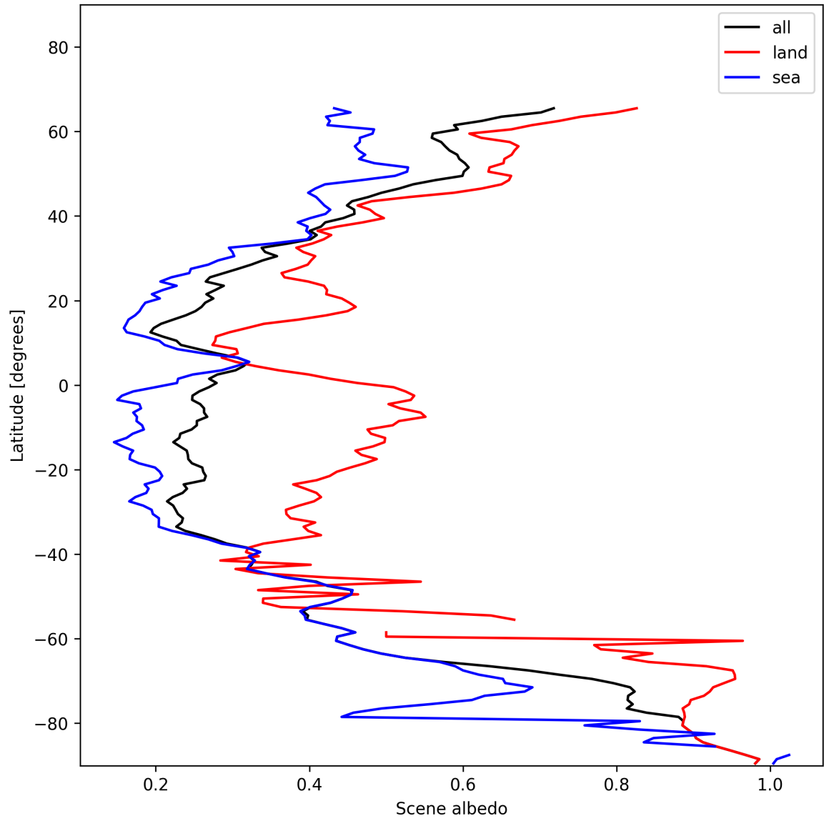
Figure 15: Zonal average of “Scene albedo” for 2025-01-04 to 2025-01-04.
