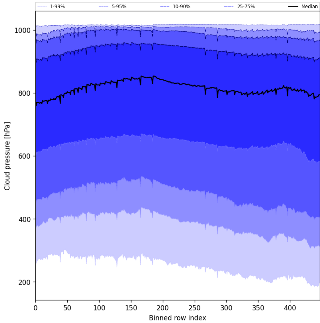
Figure 45: Along track statistics of “Cloud pressure” for 2025-01-04 to 2025-01-04
