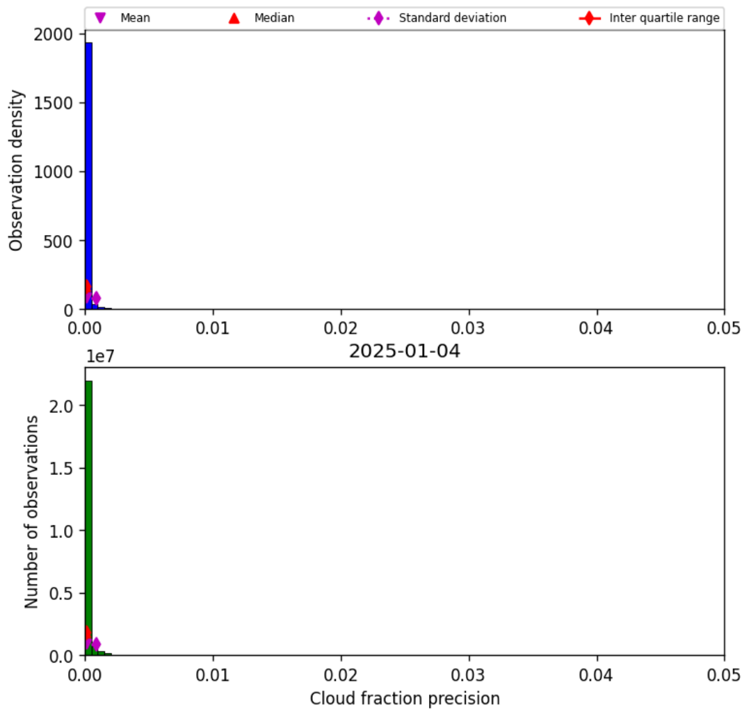
Figure 31: Histogram of “Cloud fraction precision” for 2025-01-04 to 2025-01-04
