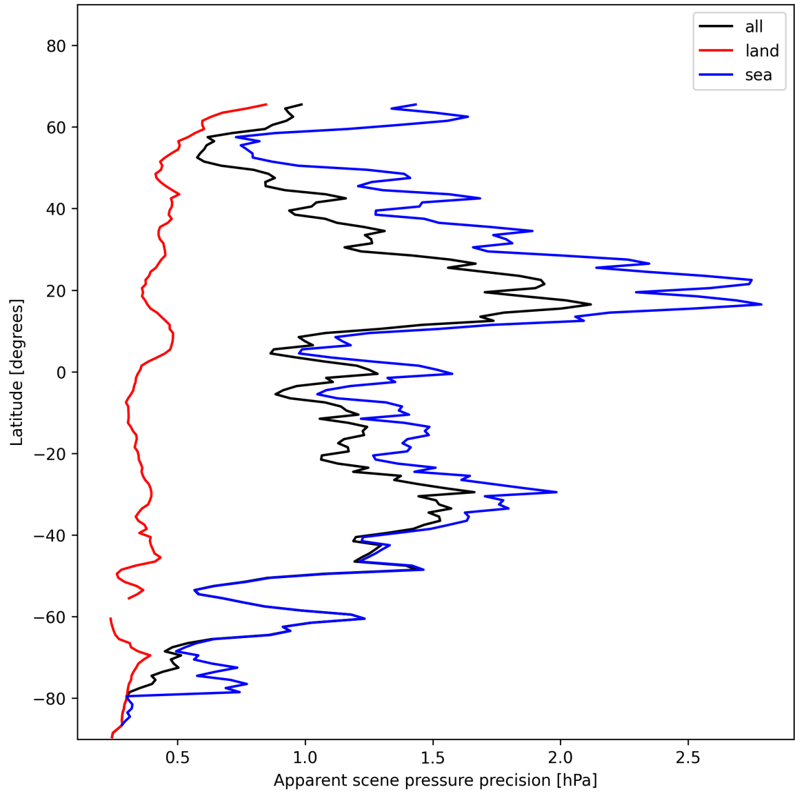
Figure 18: Zonal average of “Apparent scene pressure precision” for 2025-01-06 to 2025-01-07.
