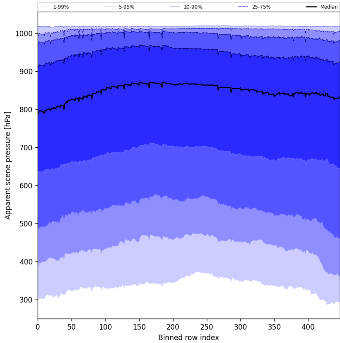
Figure 51: Along track statistics of “Apparent scene pressure” for 2025-01-06 to 2025-01-07
