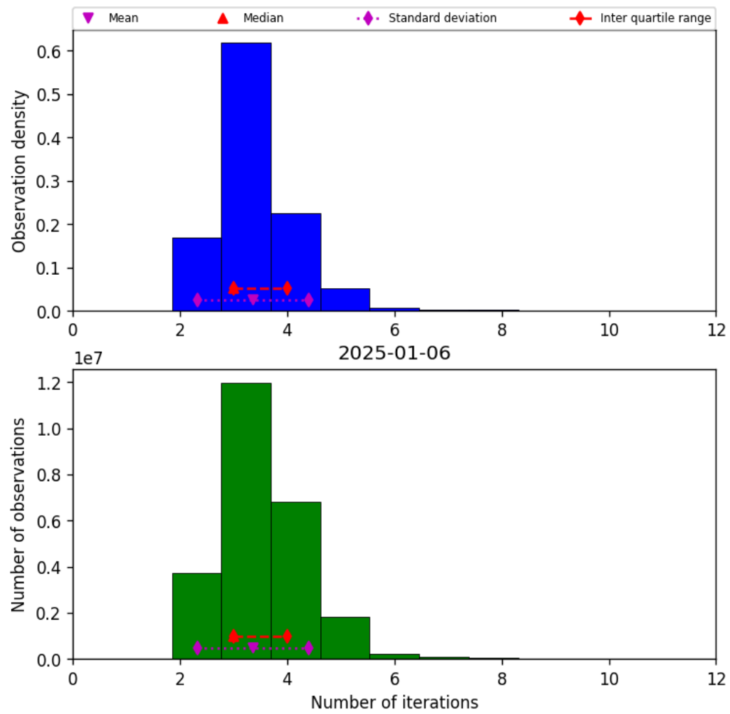
Figure 37: Histogram of “Number of iterations” for 2025-01-06 to 2025-01-07
