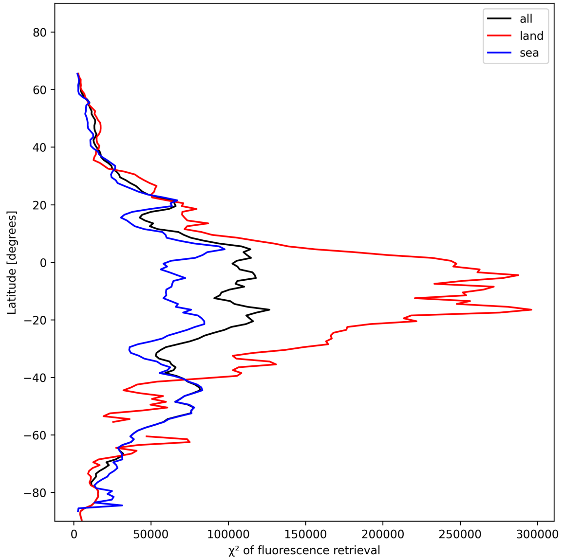
Figure 23: Zonal average of “ \chi^2 of fluorescence retrieval” for 2025-01-06 to 2025-01-07.
