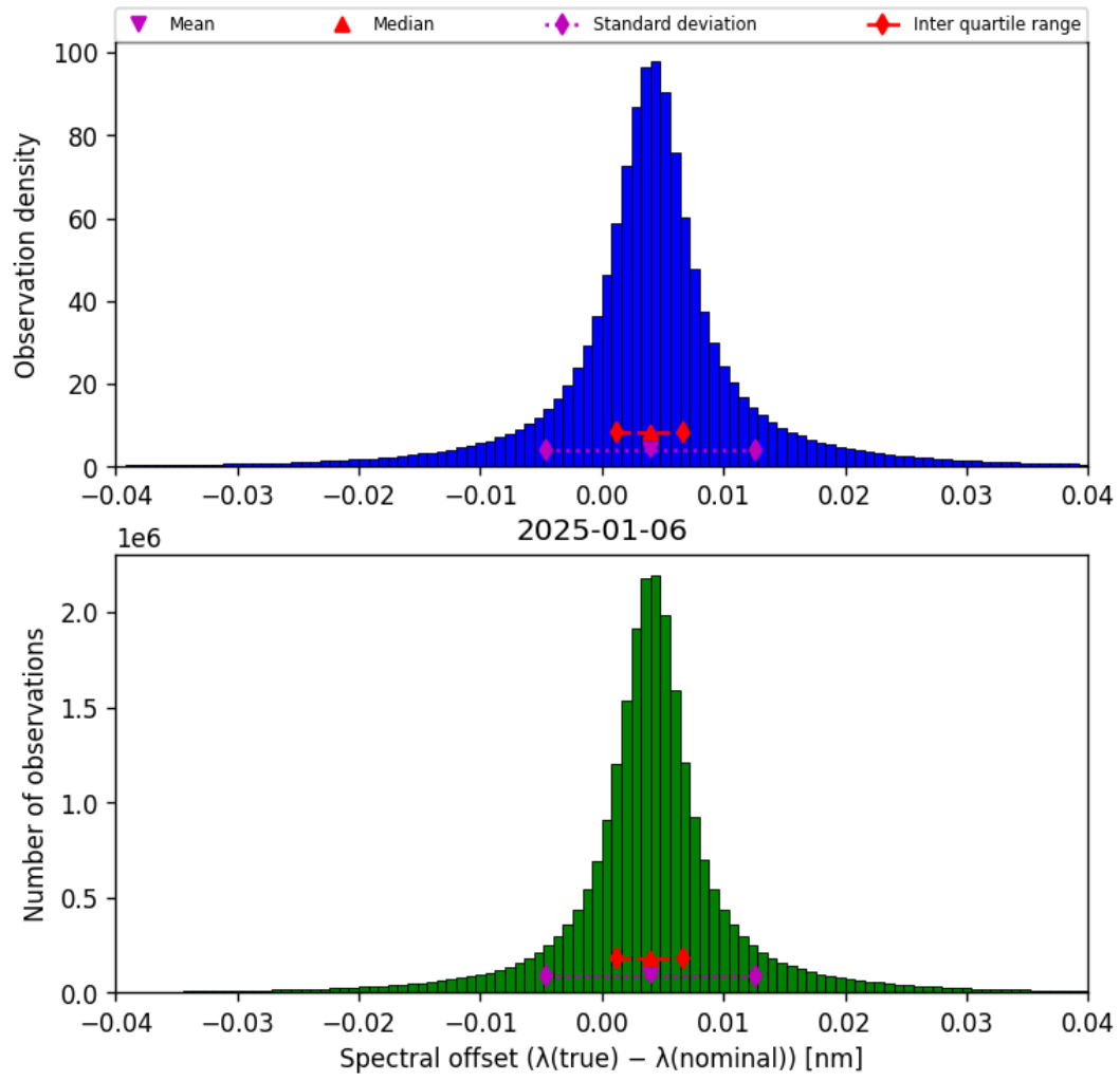
Figure 43: Histogram of “Spectral offset ( \lambda_{\text{true}} - \lambda_{\text{nominal}} )” for 2025-01-06 to 2025-01-07
