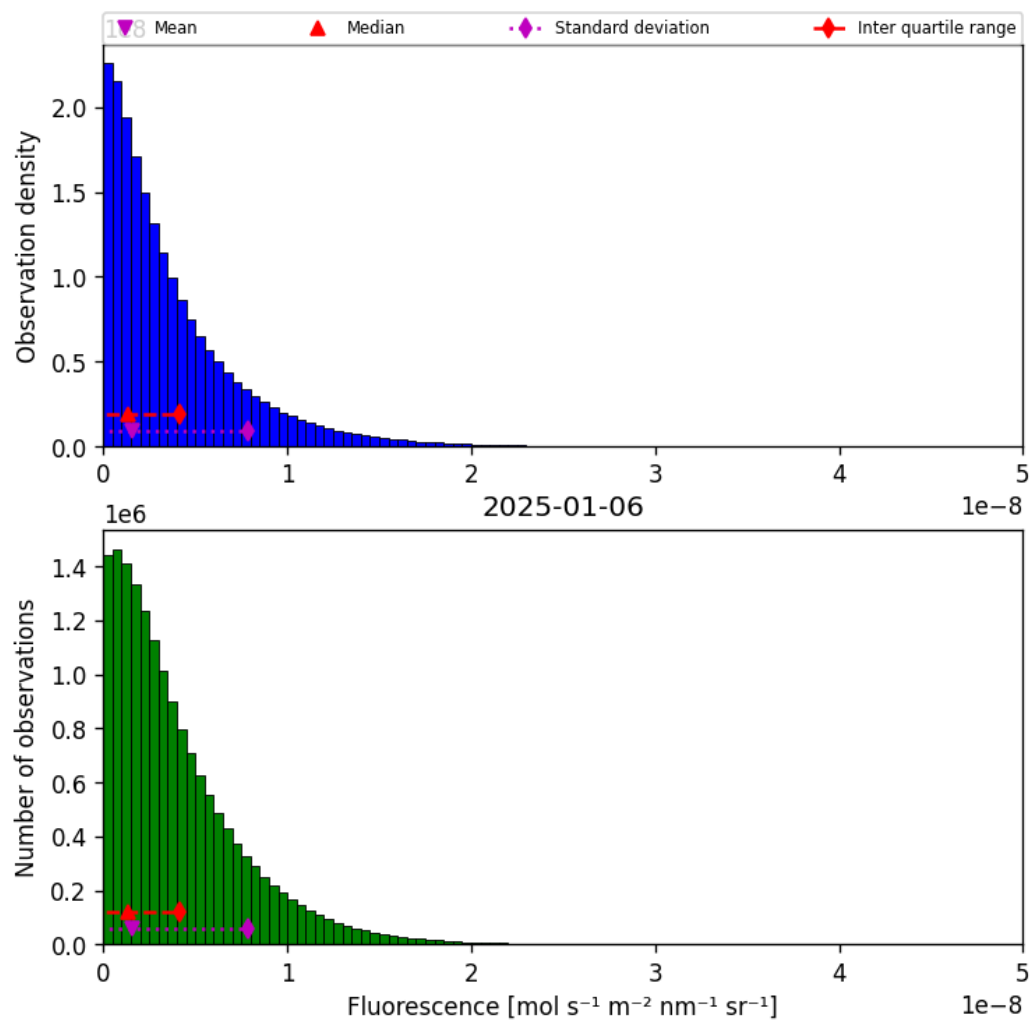
Figure 38: Histogram of “Fluorescence” for 2025-01-06 to 2025-01-07
