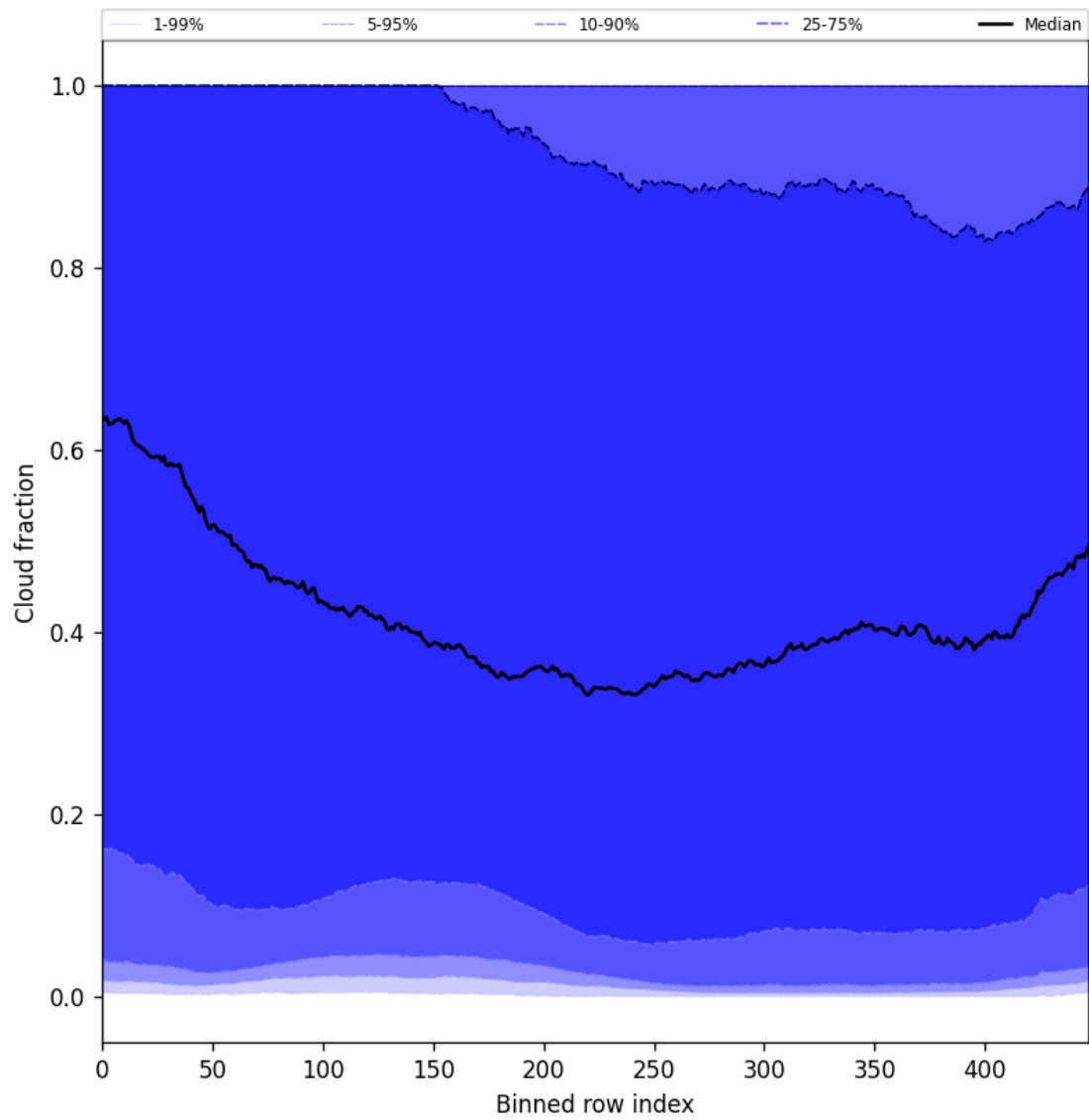
Figure 47: Along track statistics of “Cloud fraction” for 2025-01-06 to 2025-01-07
