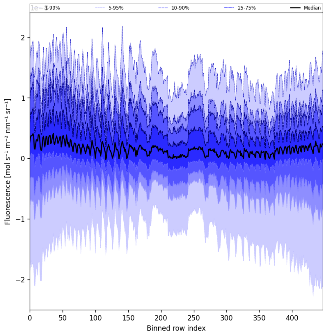
Figure 55: Along track statistics of “Fluorescence” for 2025-01-06 to 2025-01-07
