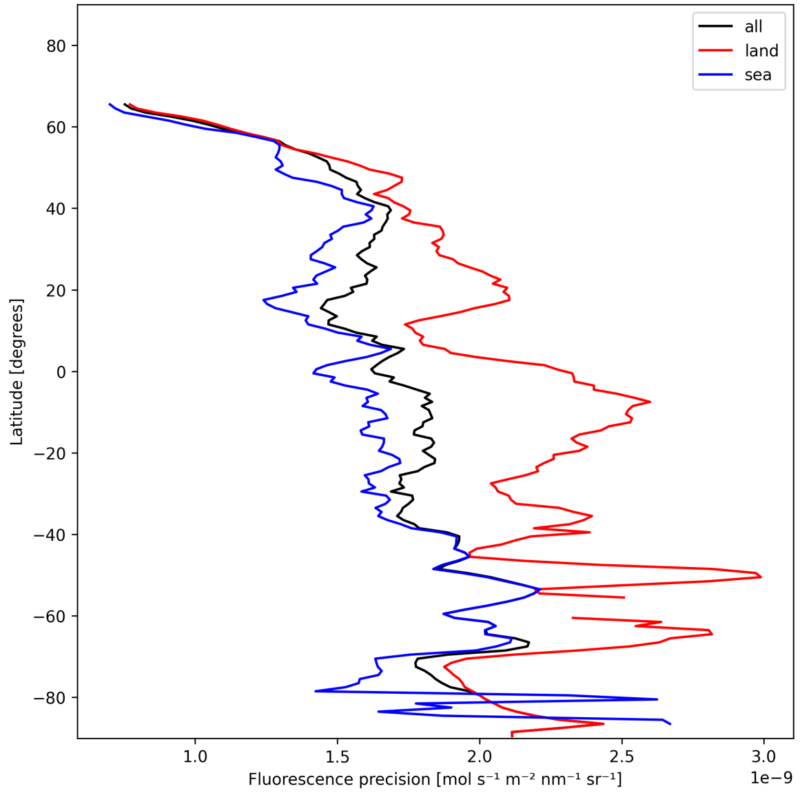
Figure 22: Zonal average of “Fluorescence precision” for 2025-01-06 to 2025-01-07.
