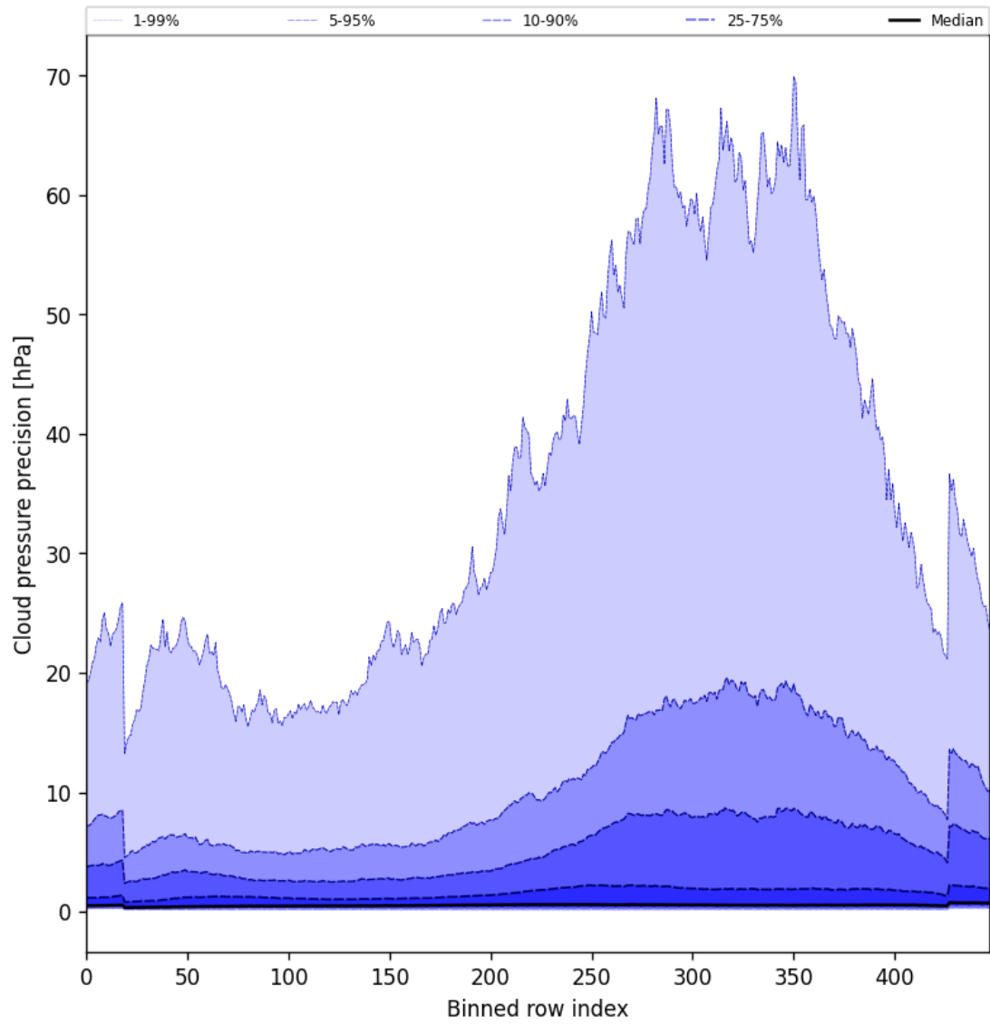
Figure 46: Along track statistics of “Cloud pressure precision” for 2025-01-06 to 2025-01-07
