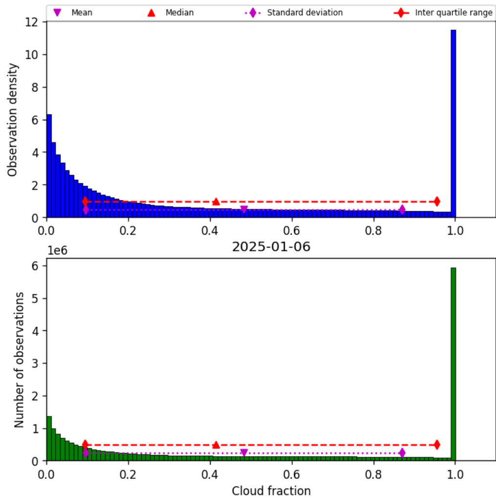
Figure 30: Histogram of “Cloud fraction” for 2025-01-06 to 2025-01-07
