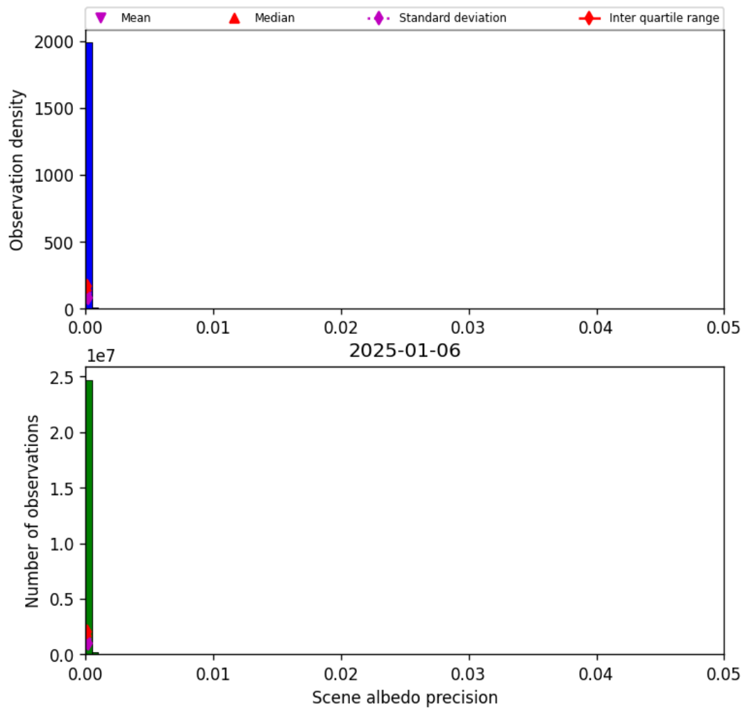
Figure 33: Histogram of “Scene albedo precision” for 2025-01-06 to 2025-01-07
