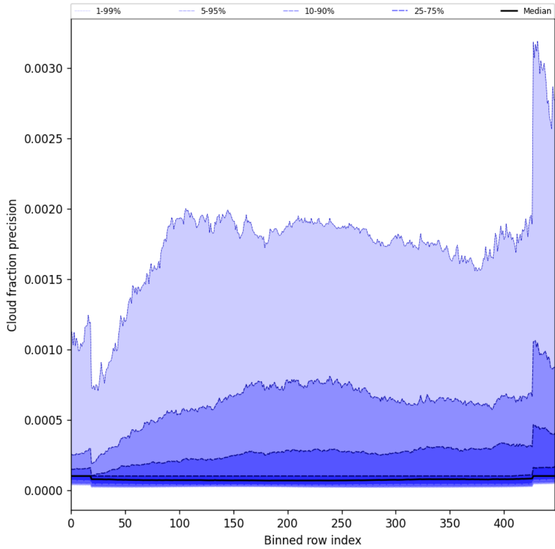
Figure 48: Along track statistics of “Cloud fraction precision” for 2025-01-06 to 2025-01-07
