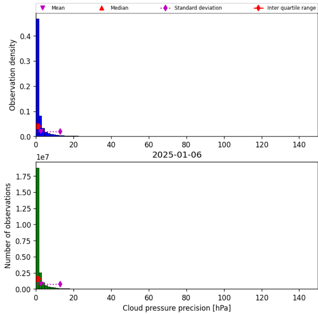
Figure 29: Histogram of “Cloud pressure precision” for 2025-01-06 to 2025-01-07
