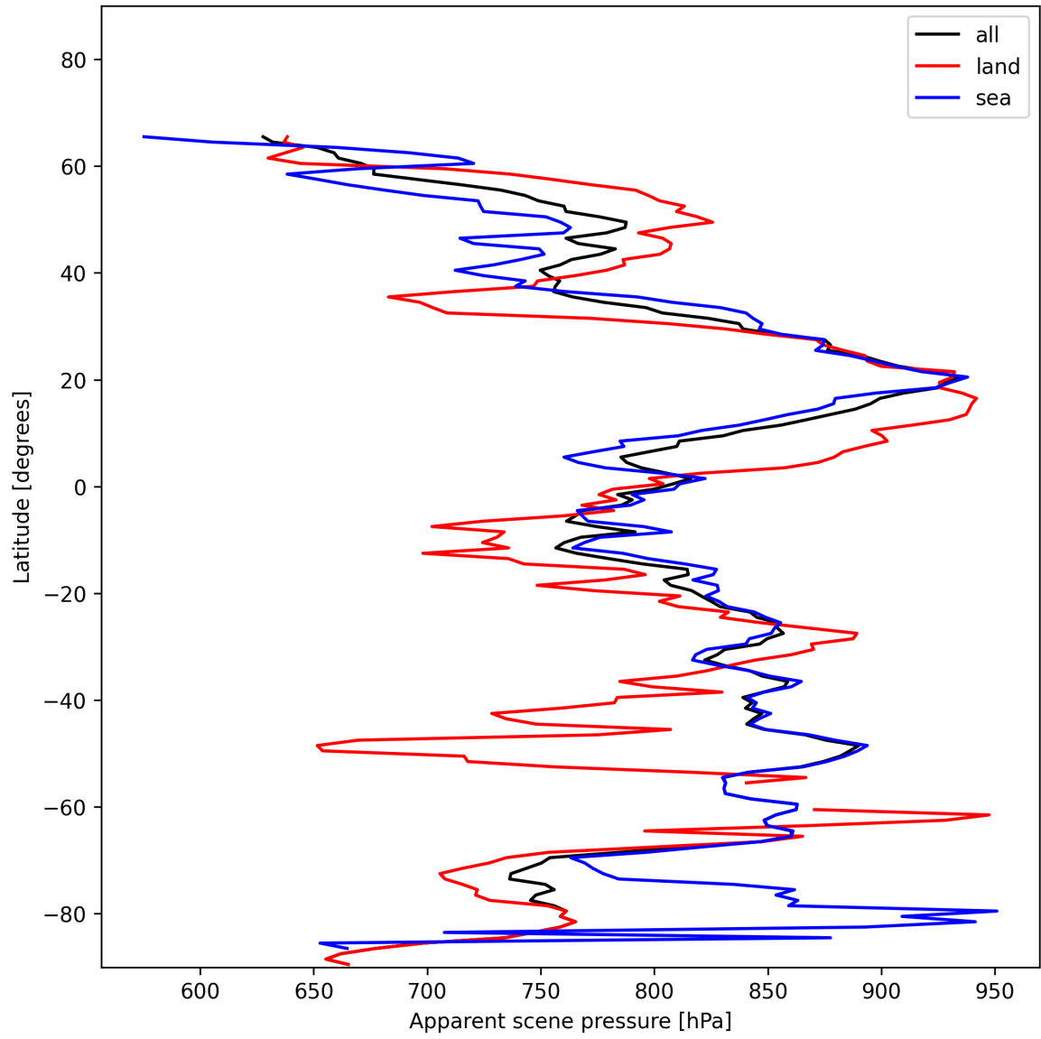
Figure 17: Zonal average of “Apparent scene pressure” for 2025-01-06 to 2025-01-07.
