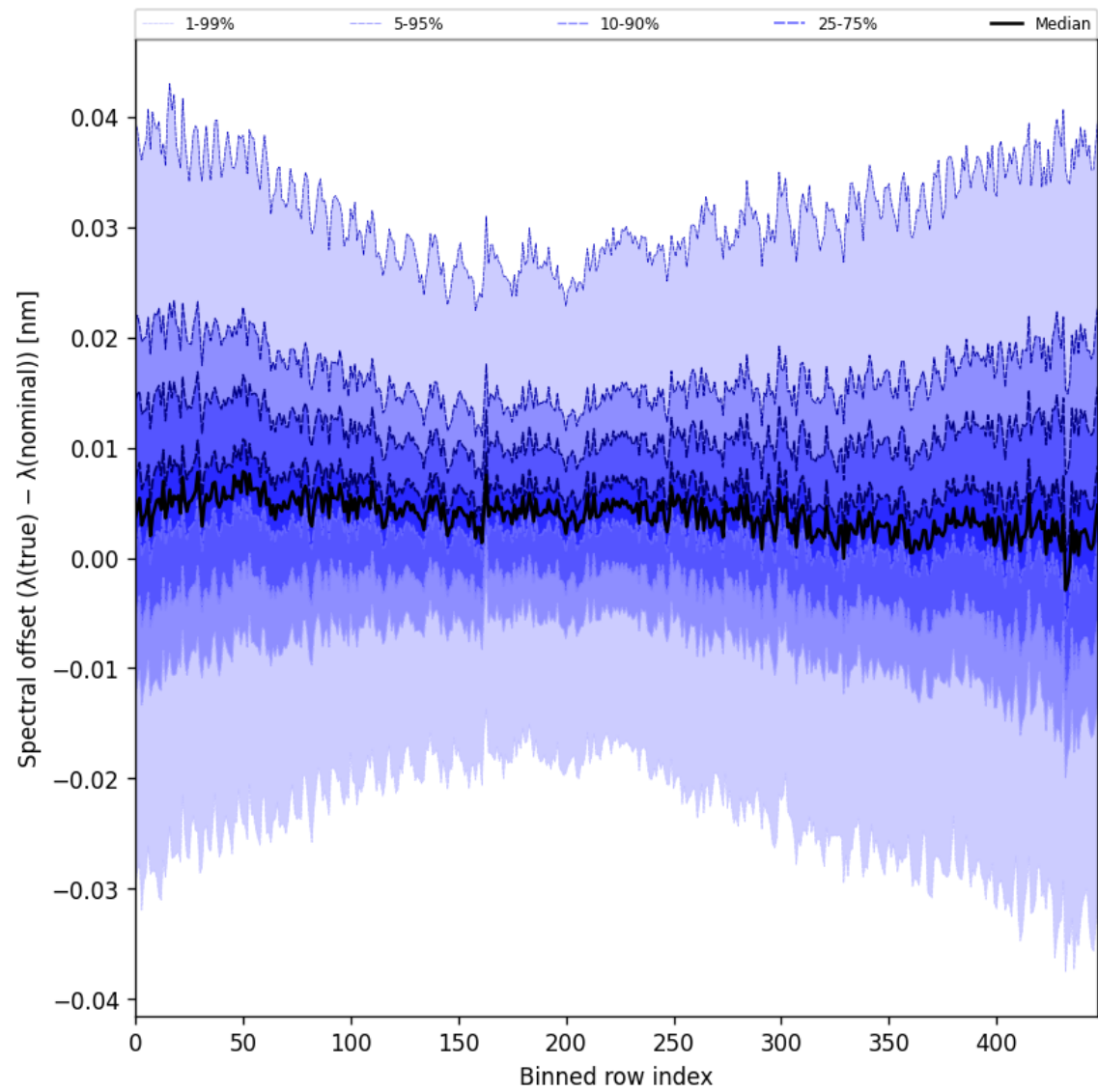
Figure 60: Along track statistics of “Spectral offset ( \lambda_{\text{true}} - \lambda_{\text{nominal}} )” for 2025-01-06 to 2025-01-07
