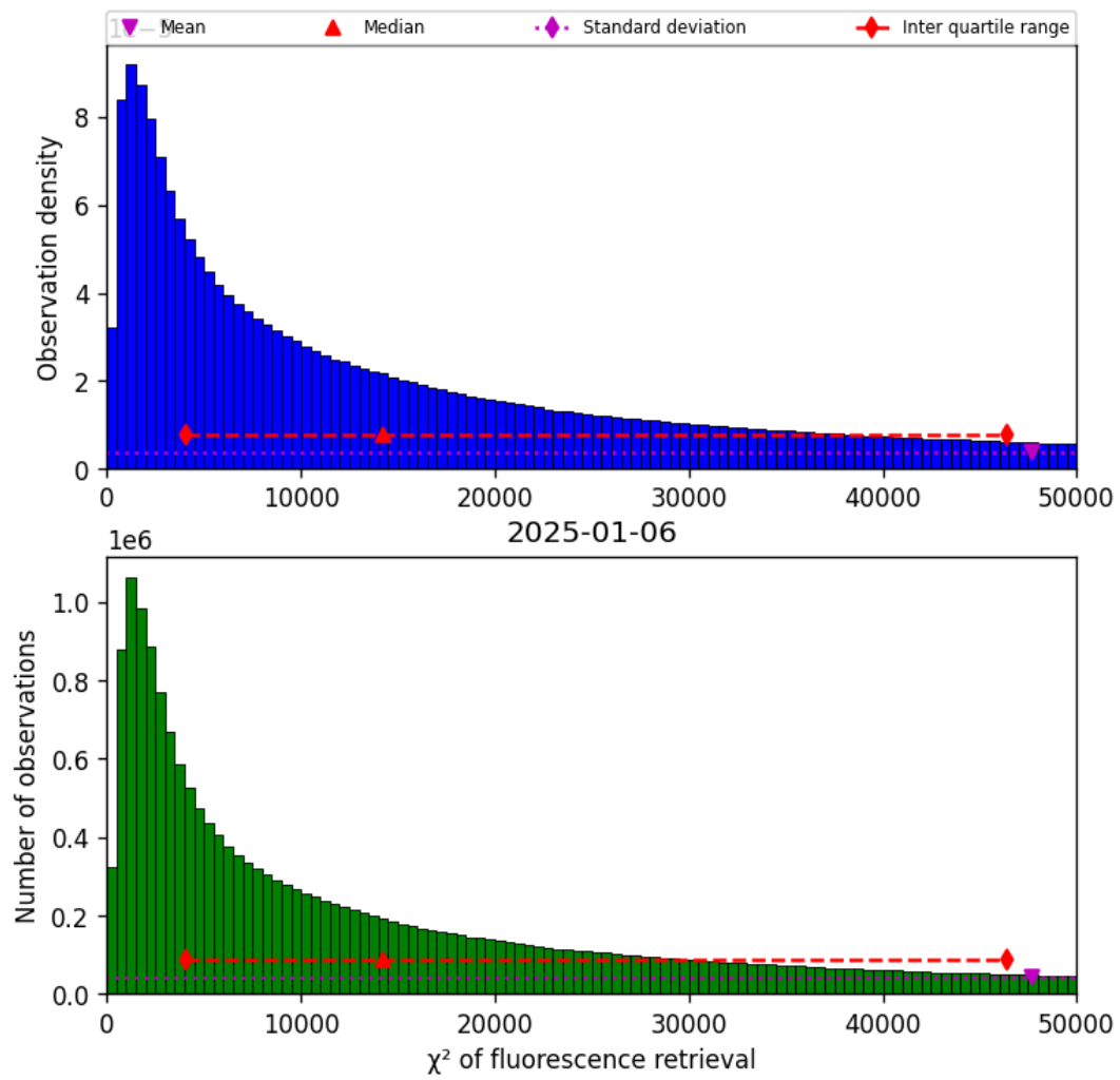
Figure 40: Histogram of “ \chi^2 of fluorescence retrieval” for 2025-01-06 to 2025-01-07
