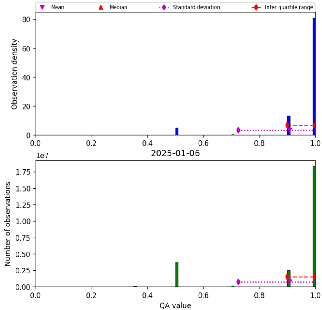
Figure 27: Histogram of “QA value” for 2025-01-06 to 2025-01-07
