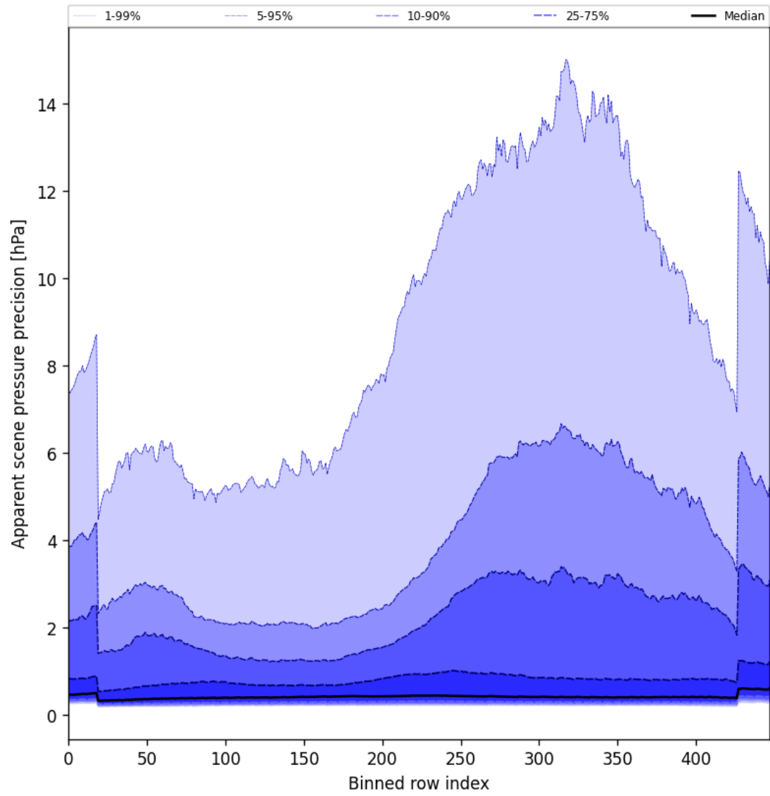
Figure 52: Along track statistics of “Apparent scene pressure precision” for 2025-01-06 to 2025-01-07
