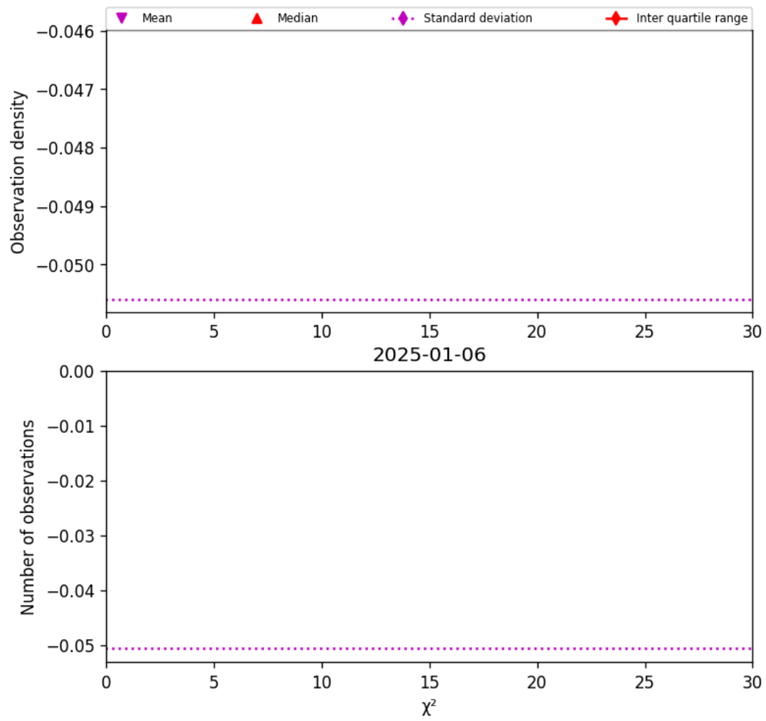
Figure 36: Histogram of " \chi^2 " for 2025-01-06 to 2025-01-07
