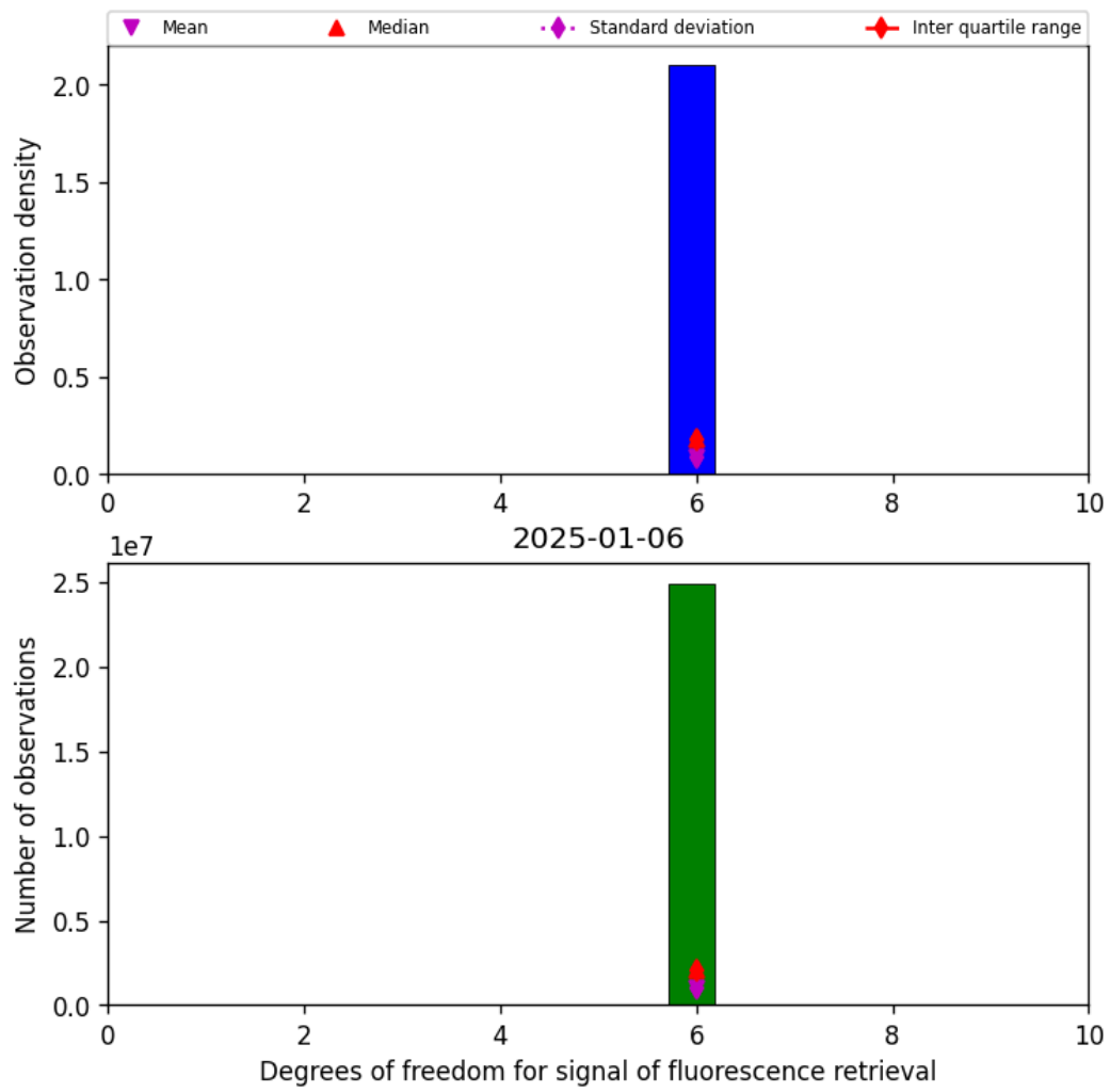
Figure 41: Histogram of “Degrees of freedom for signal of fluorescence retrieval” for 2025-01-06 to 2025-01-07
