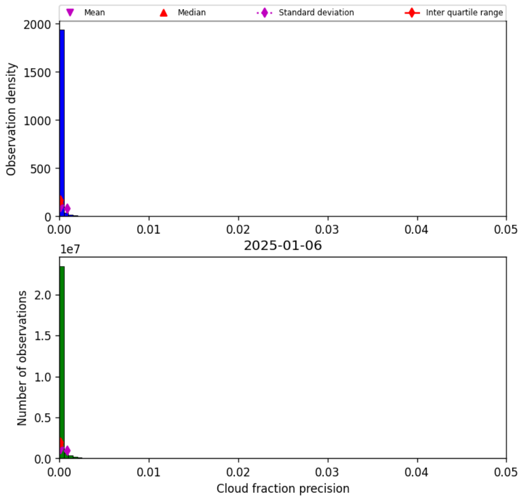
Figure 31: Histogram of “Cloud fraction precision” for 2025-01-06 to 2025-01-07
