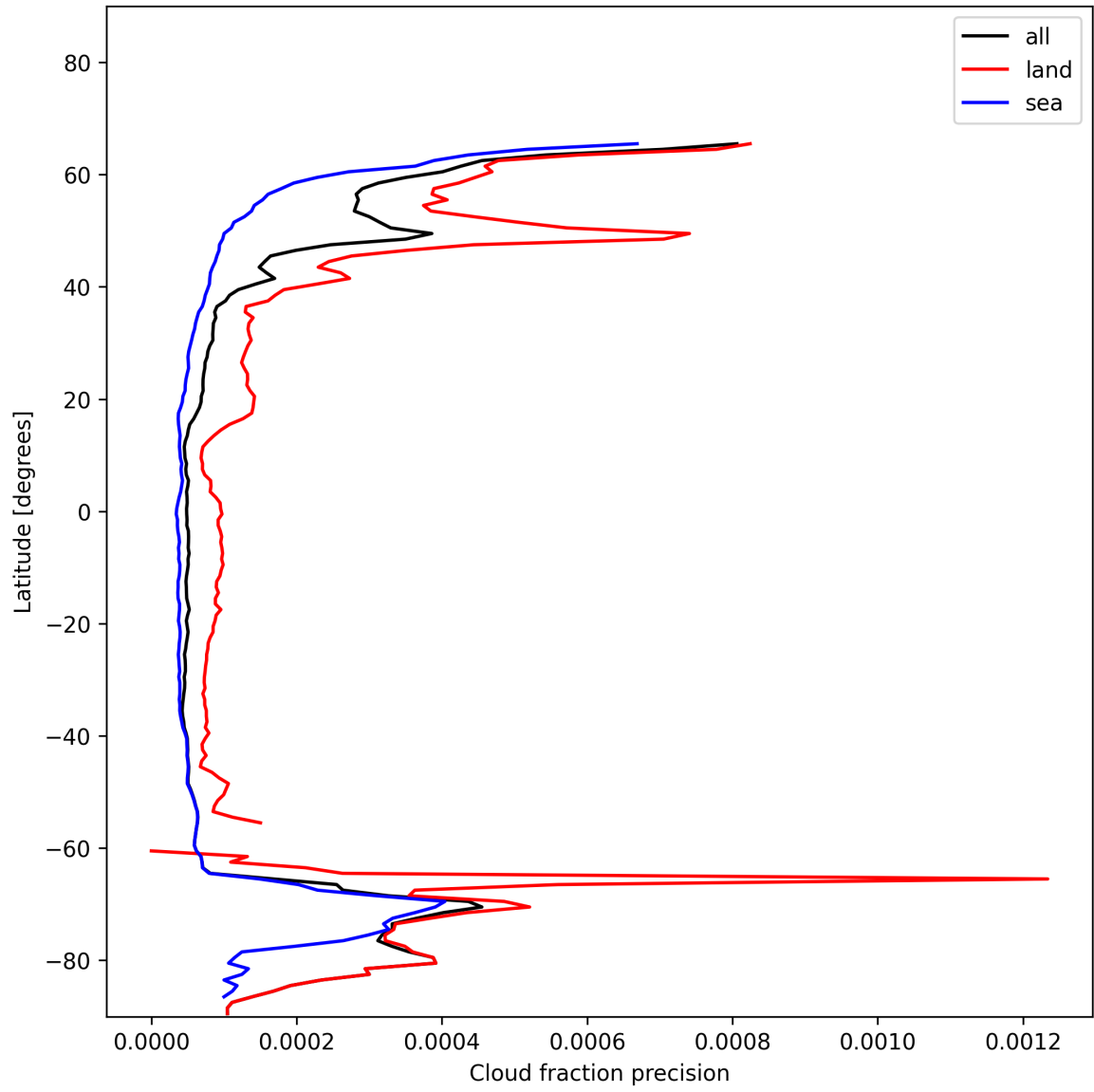
Figure 14: Zonal average of “Cloud fraction precision” for 2025-01-06 to 2025-01-07.
