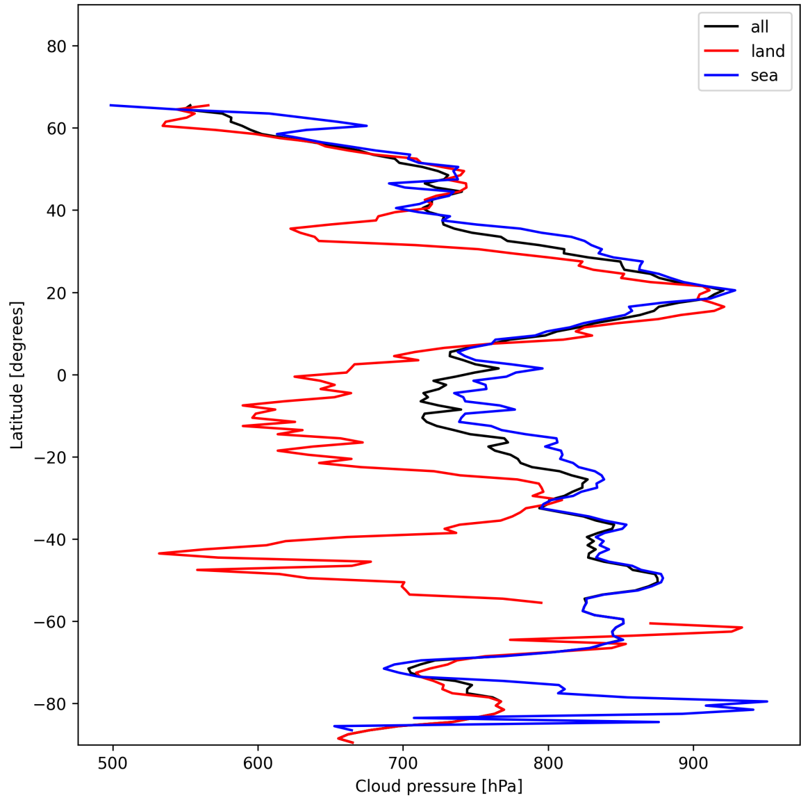
Figure 11: Zonal average of “Cloud pressure” for 2025-01-06 to 2025-01-07.
