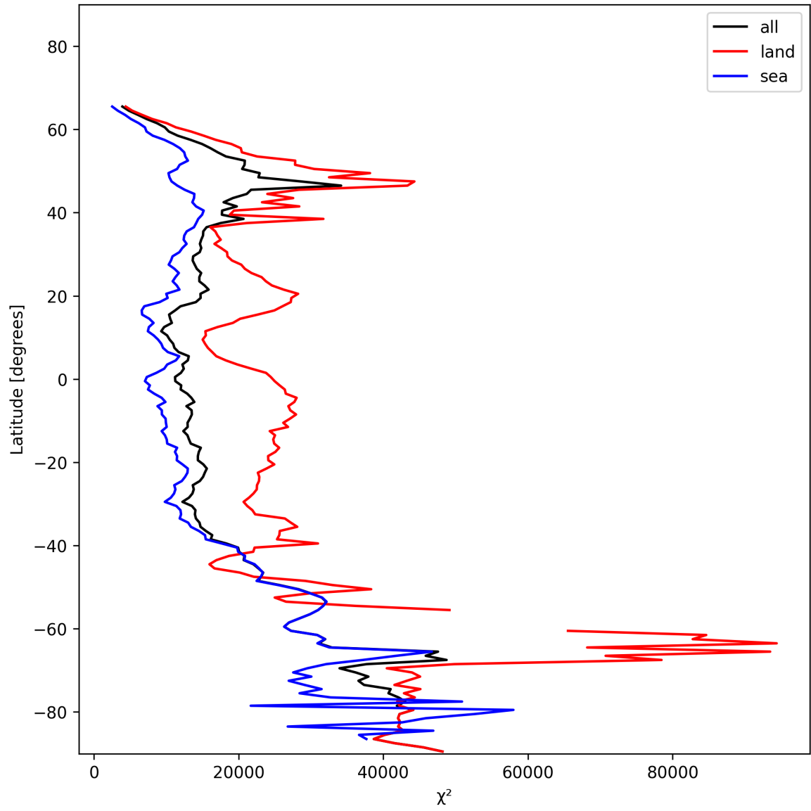
Figure 19: Zonal average of “ \chi^2 ” for 2025-01-06 to 2025-01-07.
