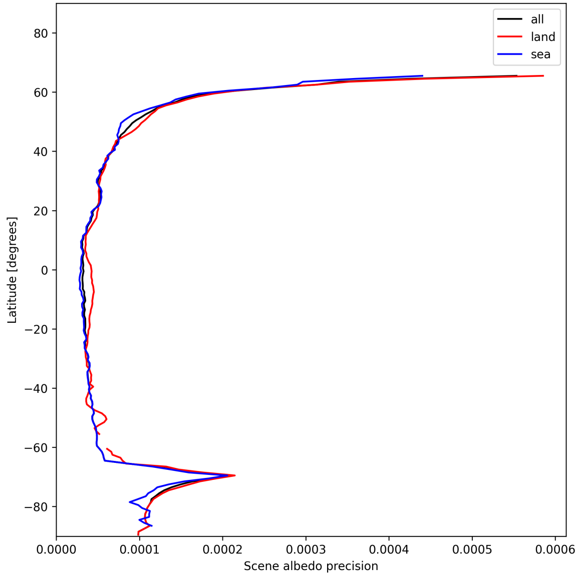
Figure 16: Zonal average of “Scene albedo precision” for 2025-01-06 to 2025-01-07.
