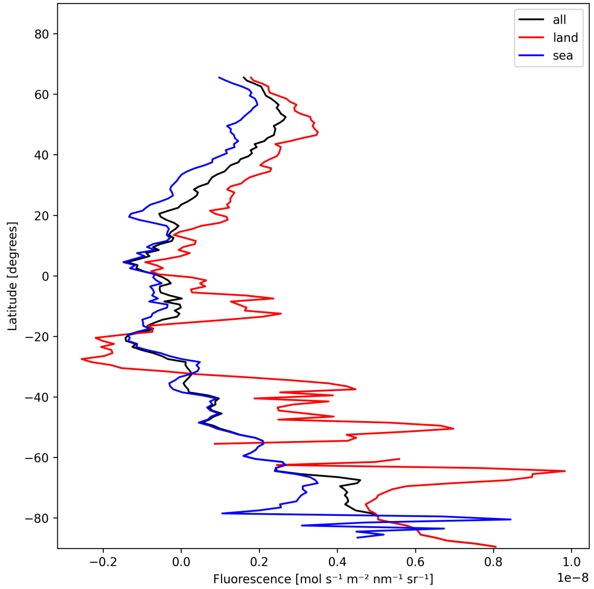
Figure 21: Zonal average of “Fluorescence” for 2025-01-06 to 2025-01-07.
