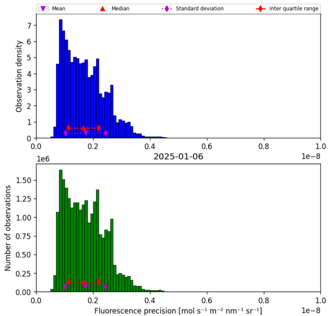
Figure 39: Histogram of “Fluorescence precision” for 2025-01-06 to 2025-01-07
