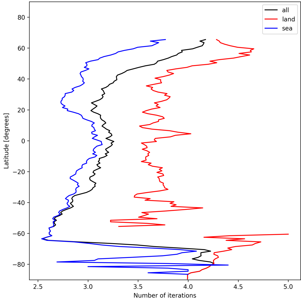
Figure 20: Zonal average of “Number of iterations” for 2025-01-06 to 2025-01-07.
