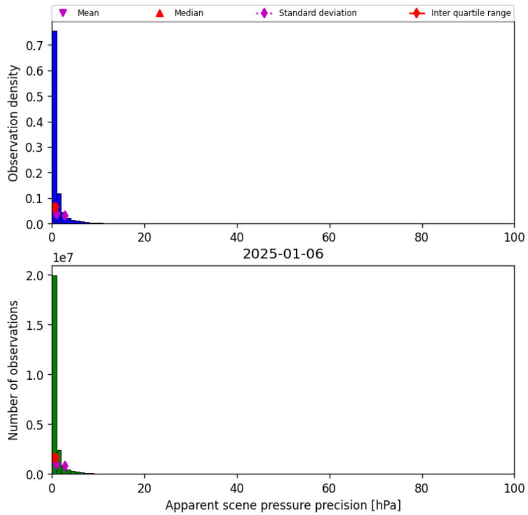
Figure 35: Histogram of “Apparent scene pressure precision” for 2025-01-06 to 2025-01-07
