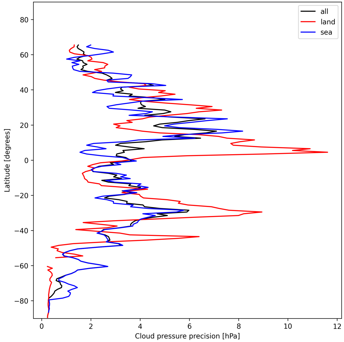
Figure 12: Zonal average of “Cloud pressure precision” for 2025-01-06 to 2025-01-07.
