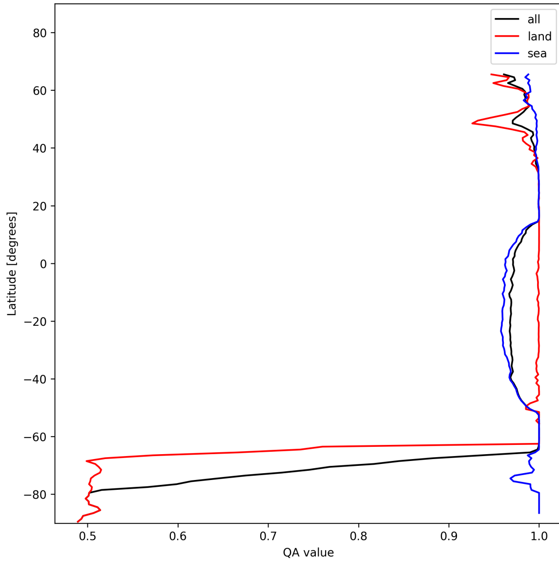
Figure 10: Zonal average of “QA value” for 2025-01-06 to 2025-01-07.
