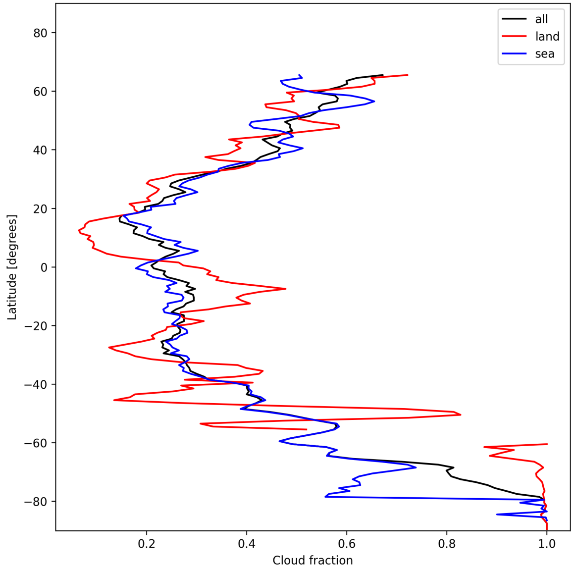
Figure 13: Zonal average of “Cloud fraction” for 2025-01-06 to 2025-01-07.
