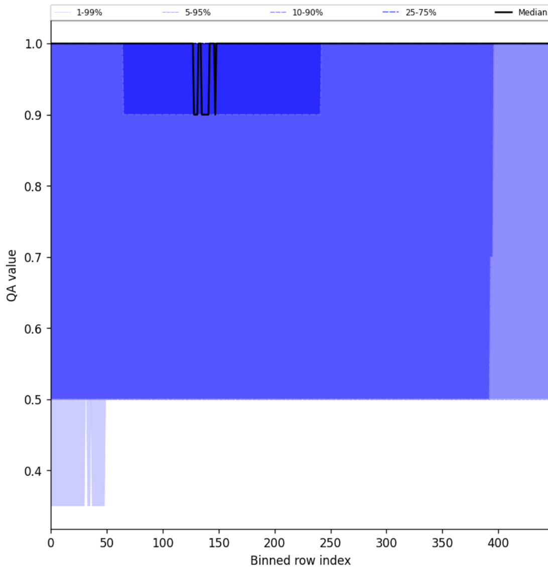
Figure 44: Along track statistics of “QA value” for 2025-01-06 to 2025-01-07
