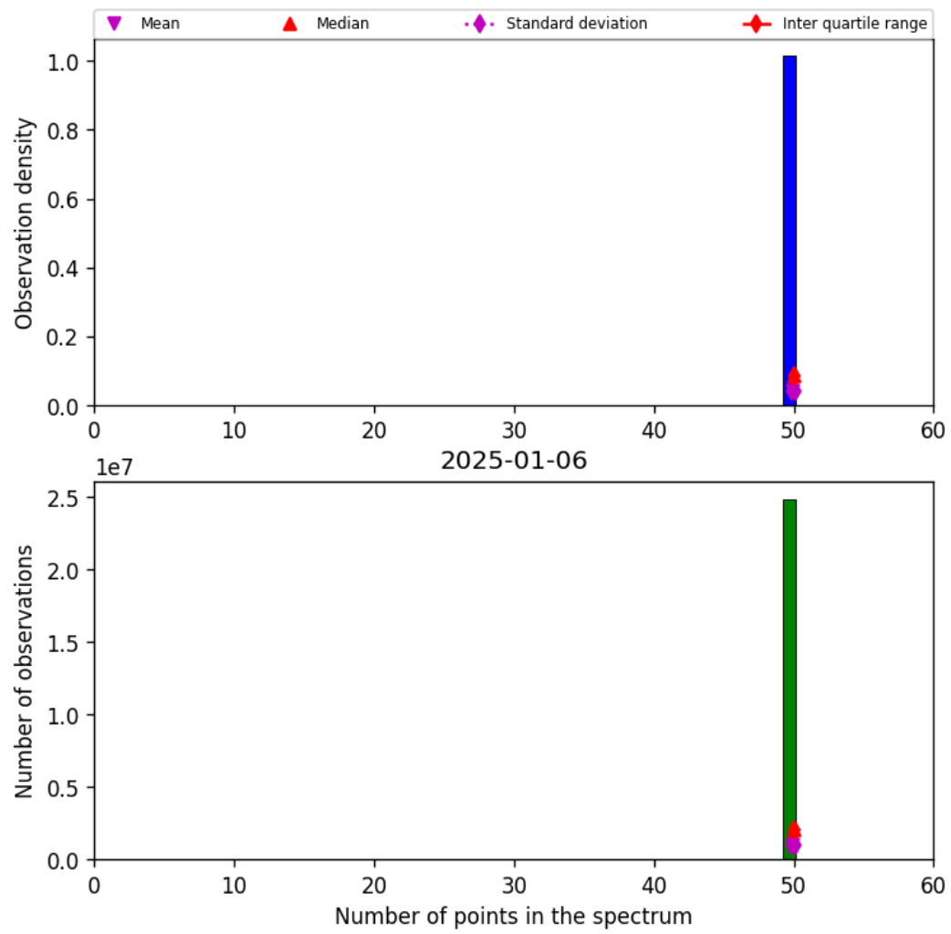
Figure 42: Histogram of “Number of points in the spectrum” for 2025-01-06 to 2025-01-07
