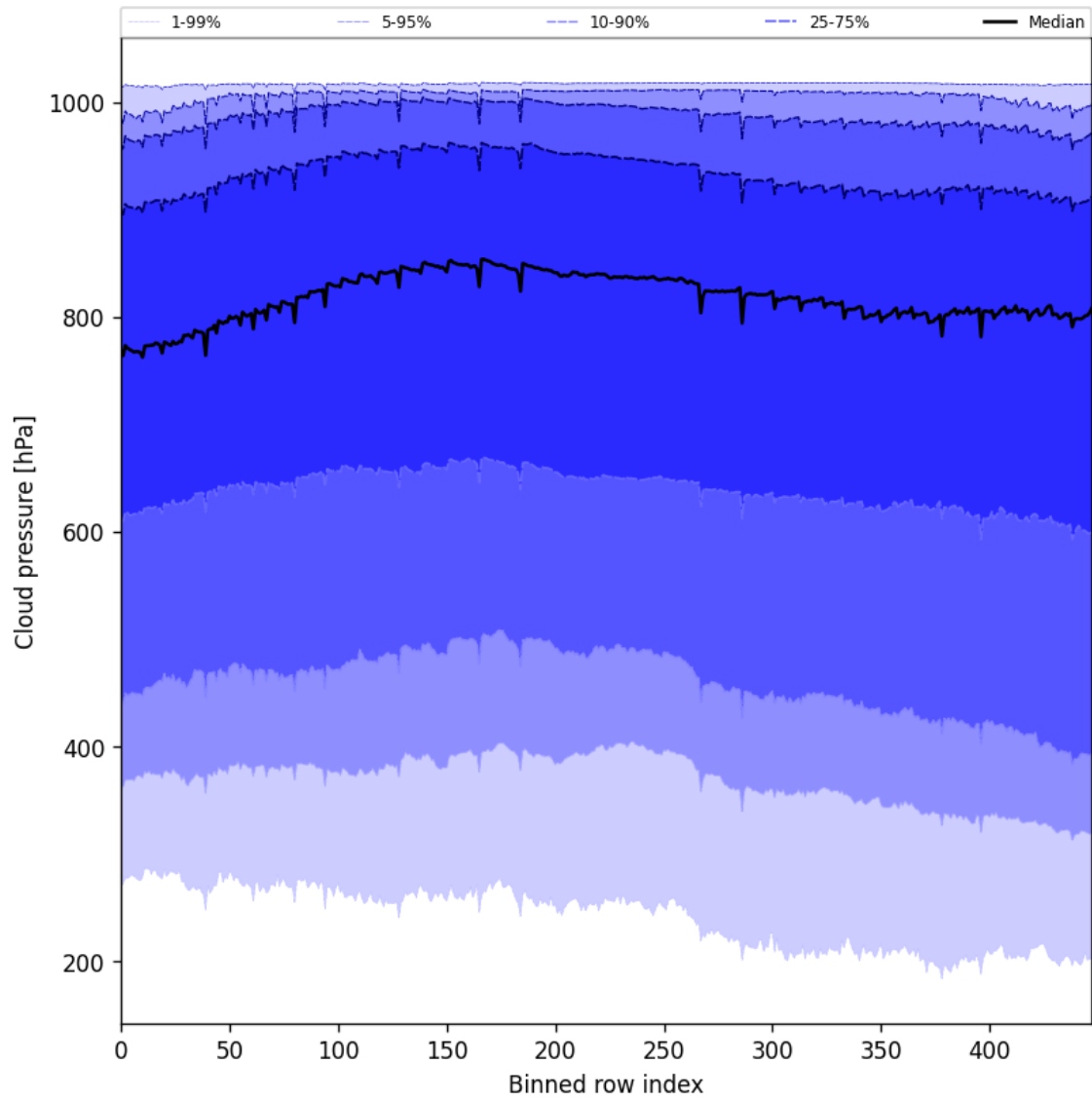
Figure 45: Along track statistics of “Cloud pressure” for 2025-01-06 to 2025-01-07
