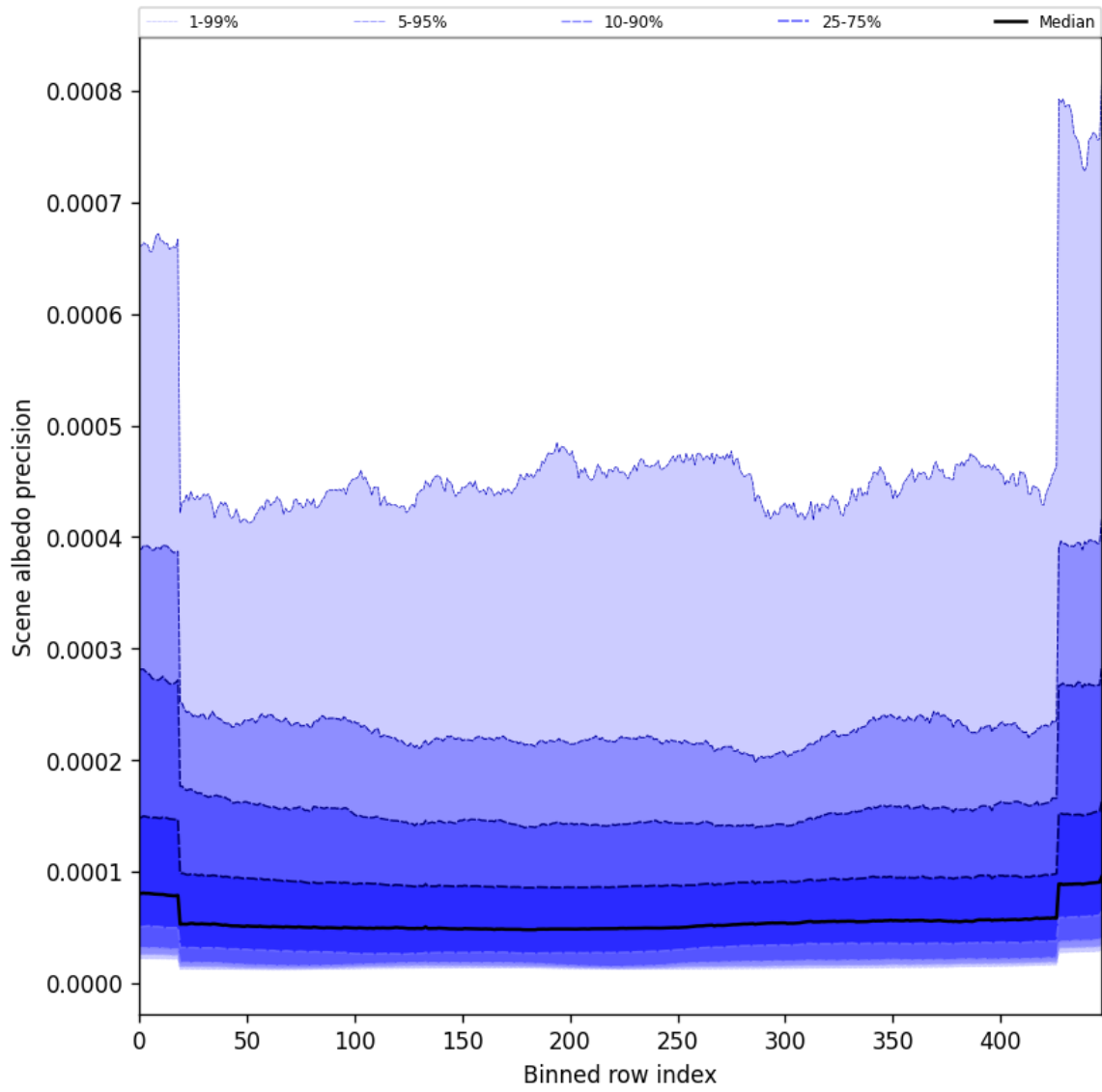
Figure 50: Along track statistics of “Scene albedo precision” for 2025-01-06 to 2025-01-07
