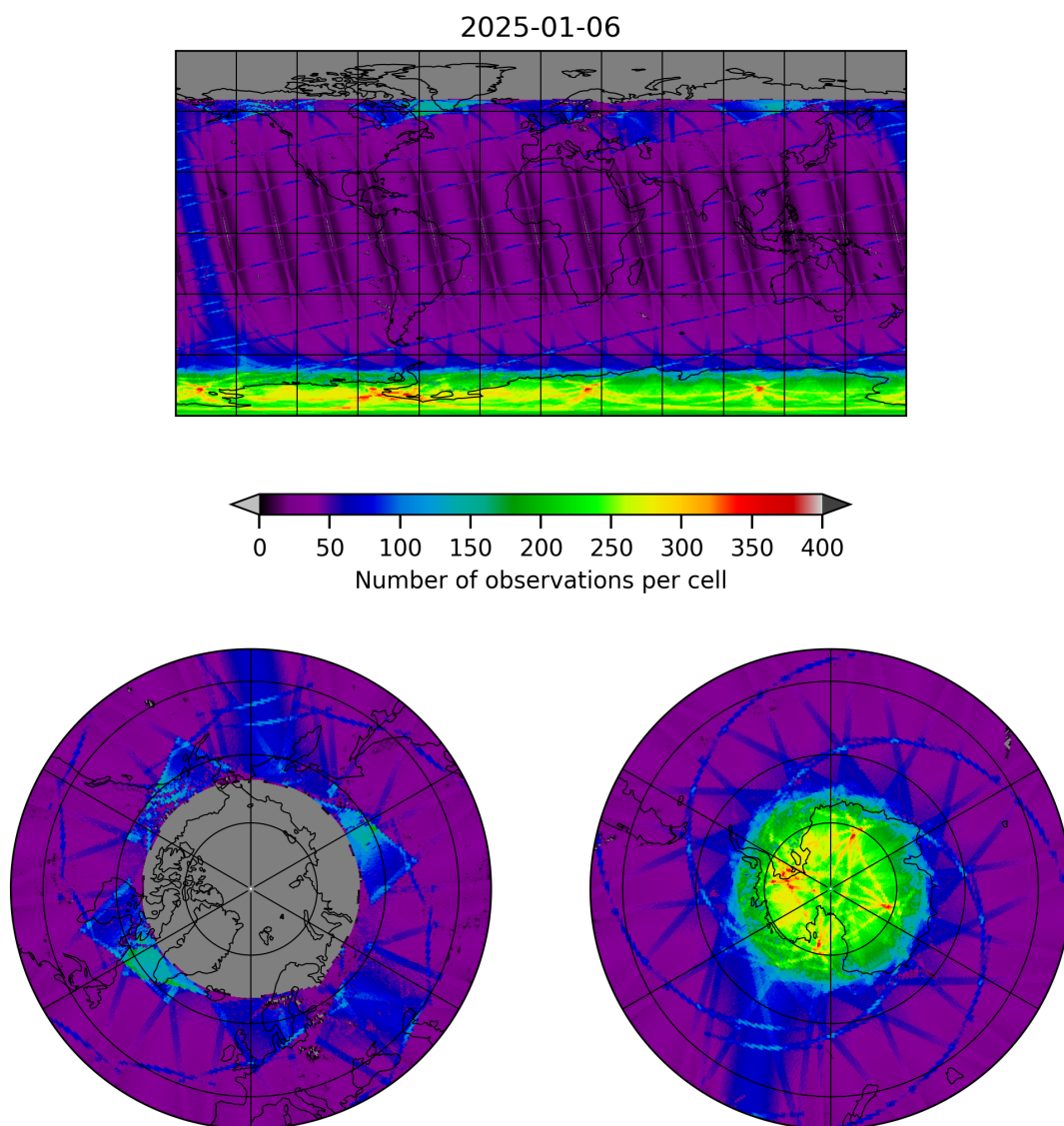
Figure 9: Map of the number of observations for 2025-01-06 to 2025-01-07
