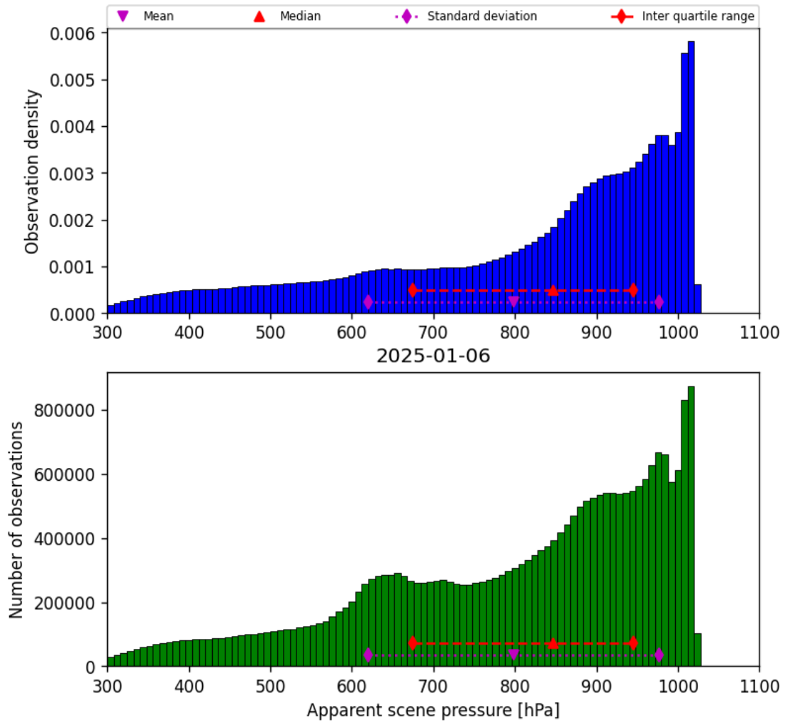
Figure 34: Histogram of “Apparent scene pressure” for 2025-01-06 to 2025-01-07
