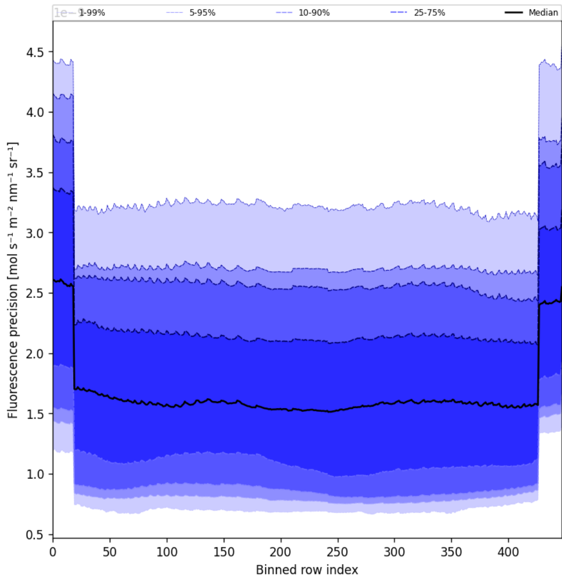
Figure 56: Along track statistics of “Fluorescence precision” for 2025-01-06 to 2025-01-07
