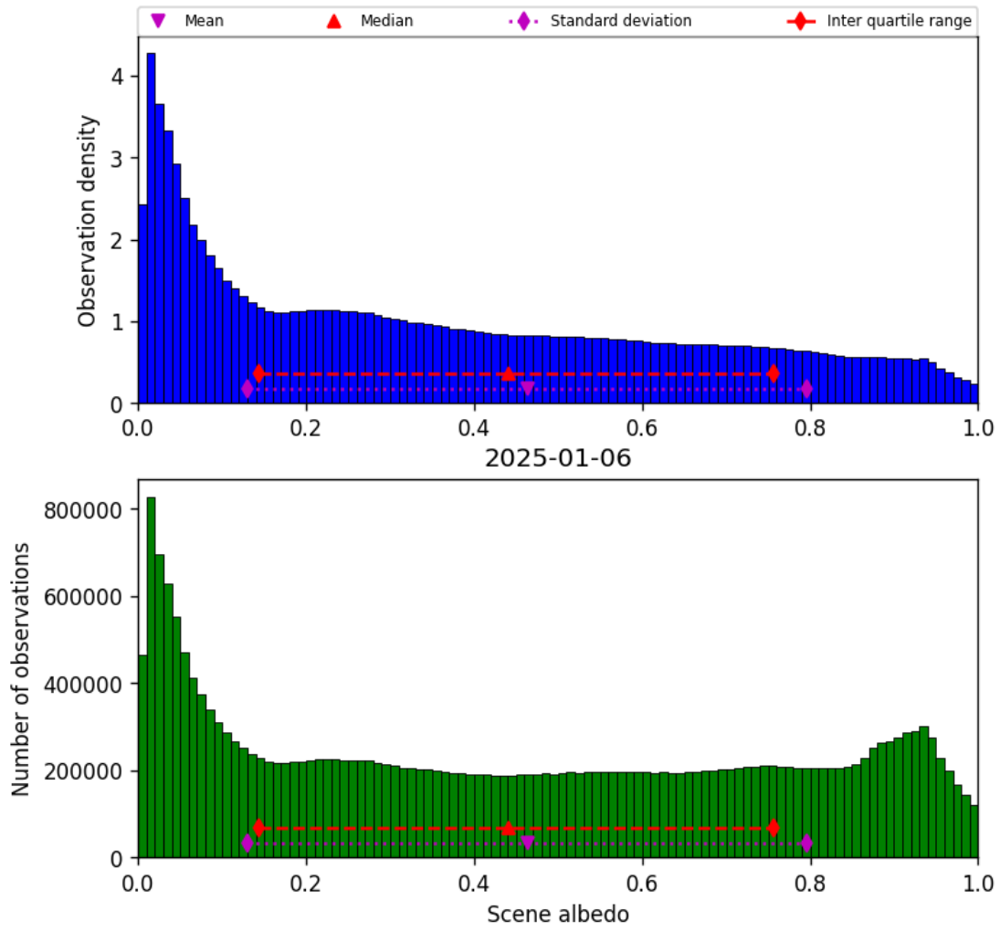
Figure 32: Histogram of “Scene albedo” for 2025-01-06 to 2025-01-07
