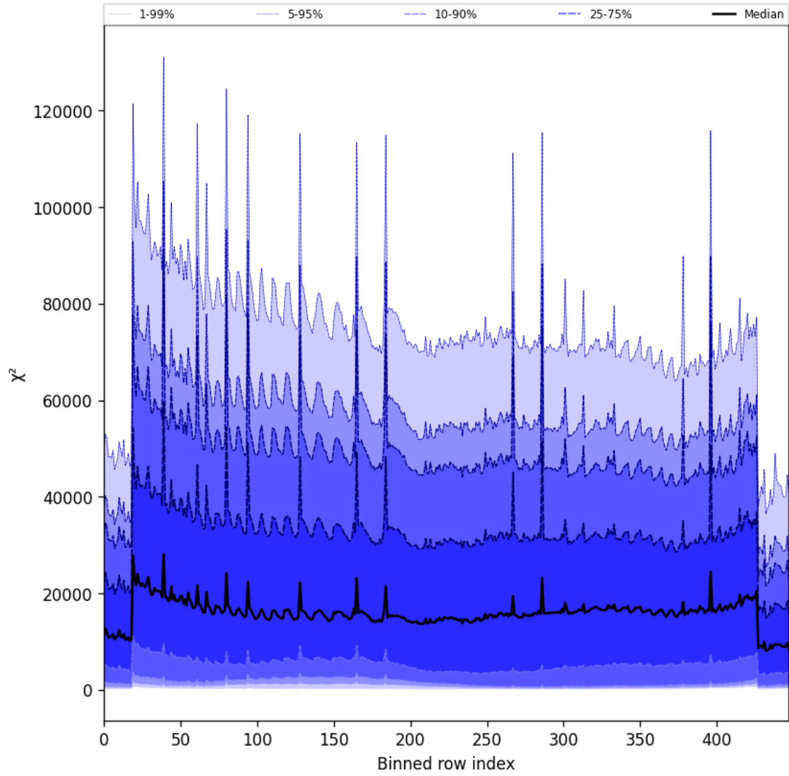
Figure 53: Along track statistics of “ \chi^2 ” for 2025-01-06 to 2025-01-07
