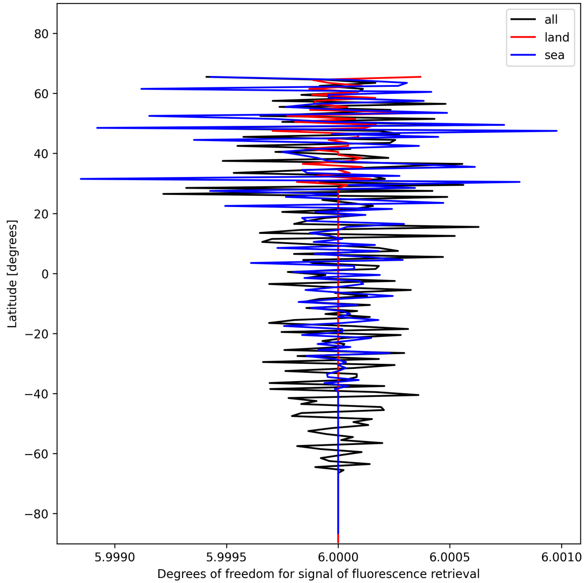
Figure 24: Zonal average of “Degrees of freedom for signal of fluorescence retrieval” for 2025-01-06 to 2025-01-07.
