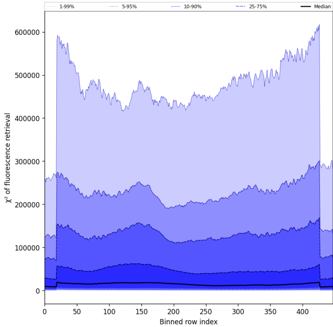
Figure 57: Along track statistics of “ \chi^2 of fluorescence retrieval” for 2025-01-06 to 2025-01-07
