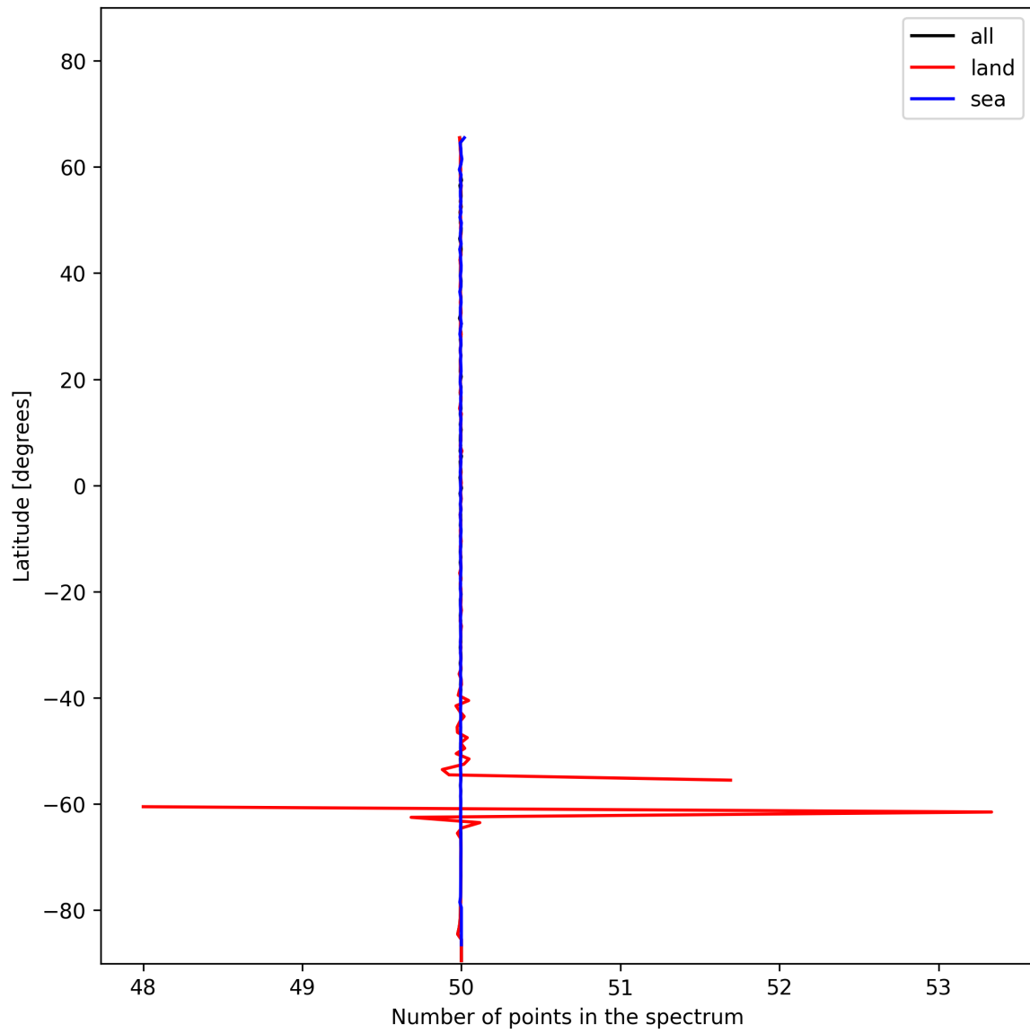
Figure 25: Zonal average of “Number of points in the spectrum” for 2025-01-06 to 2025-01-07.
