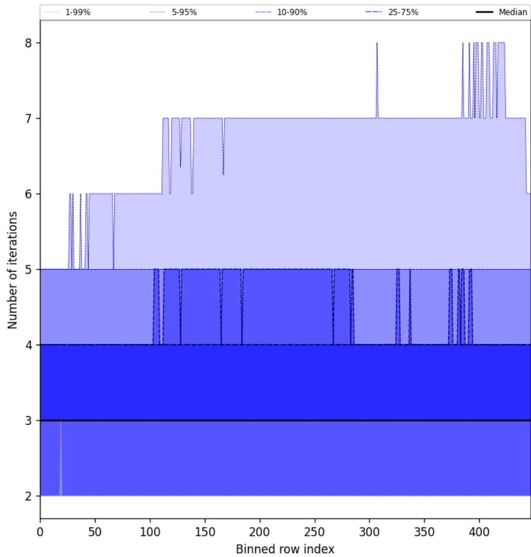
Figure 54: Along track statistics of “Number of iterations” for 2025-01-06 to 2025-01-07
