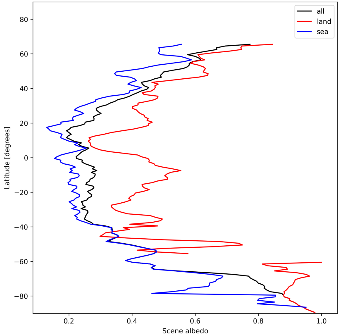
Figure 15: Zonal average of “Scene albedo” for 2025-01-06 to 2025-01-07.
