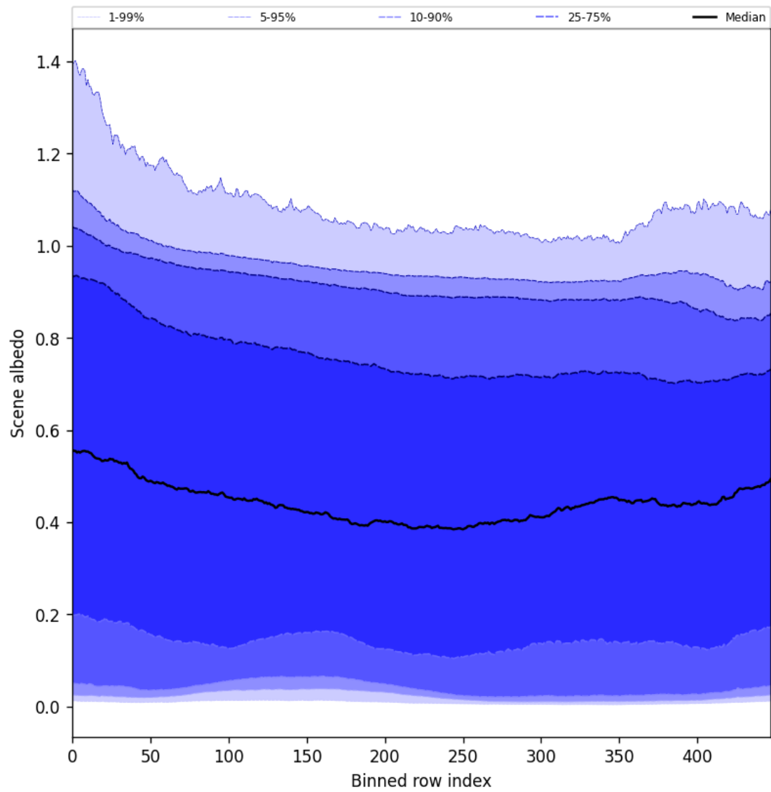
Figure 49: Along track statistics of “Scene albedo” for 2025-01-06 to 2025-01-07
