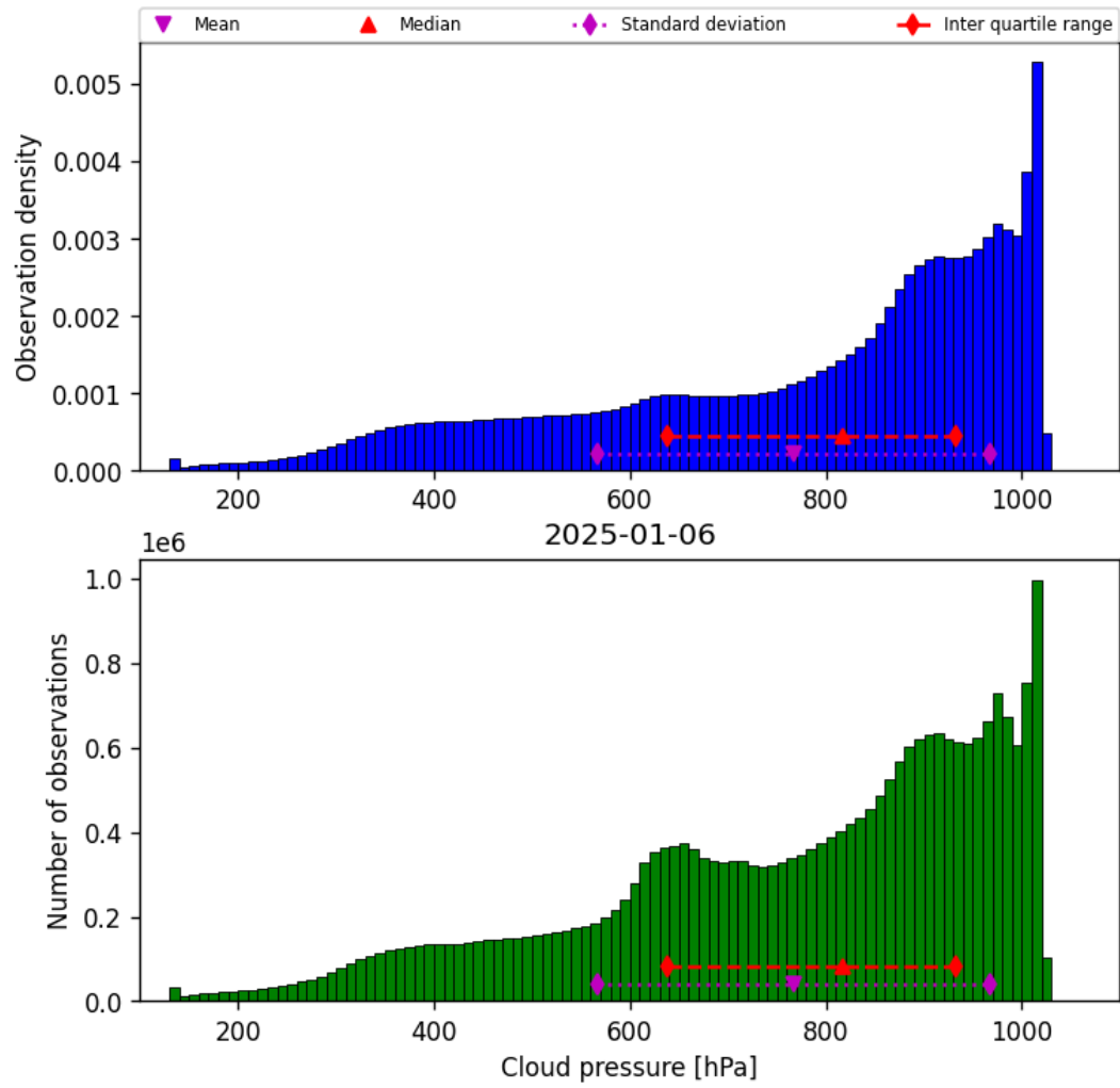
Figure 28: Histogram of “Cloud pressure” for 2025-01-06 to 2025-01-07
