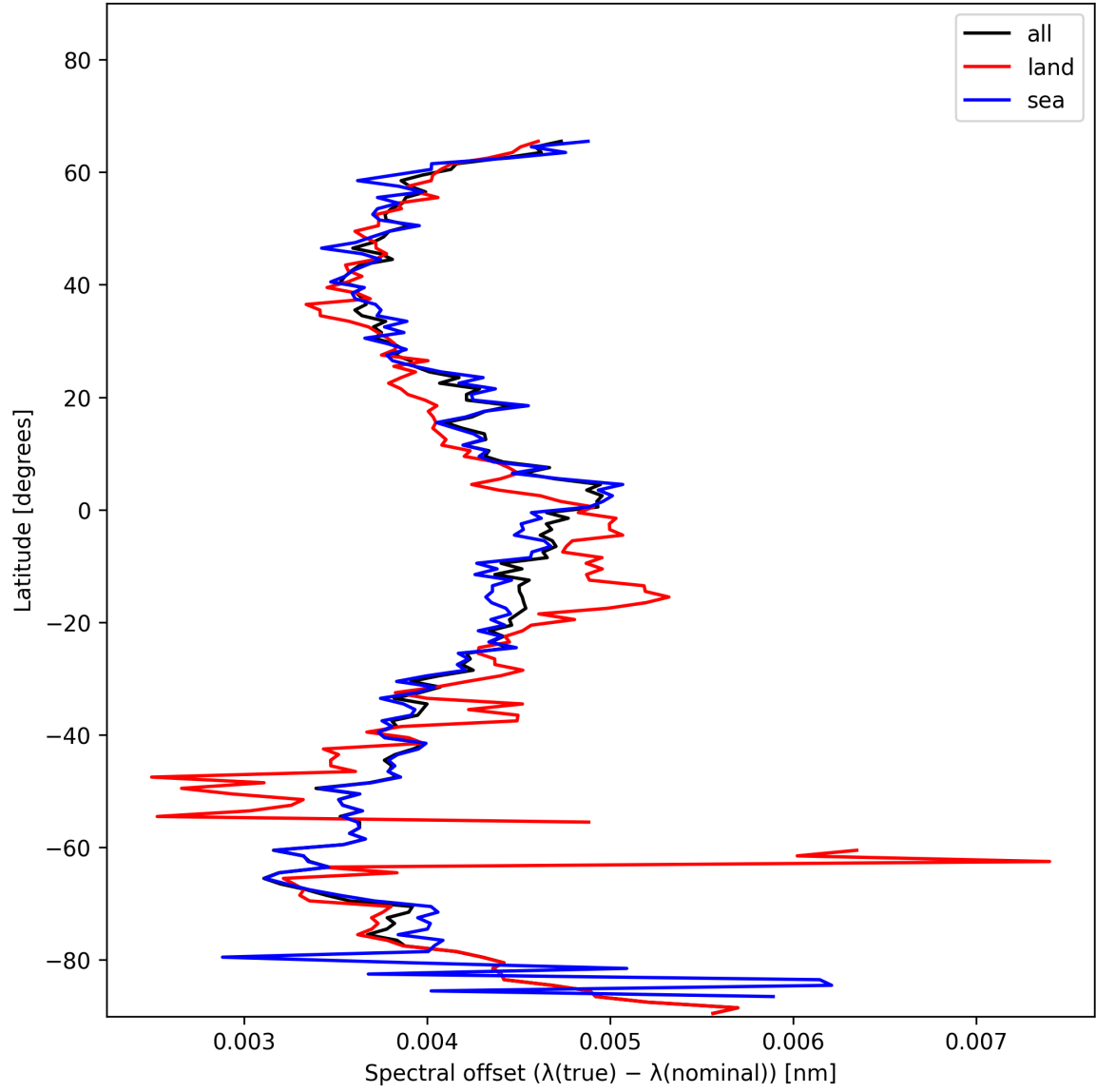
Figure 26: Zonal average of “Spectral offset ( \lambda_{\text{true}} - \lambda_{\text{nominal}} )” for 2025-01-06 to 2025-01-07.
