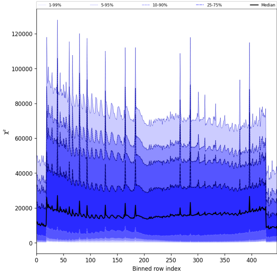
Figure 53: Along track statistics of “ \chi^2 ” for 2025-01-10 to 2025-01-10
