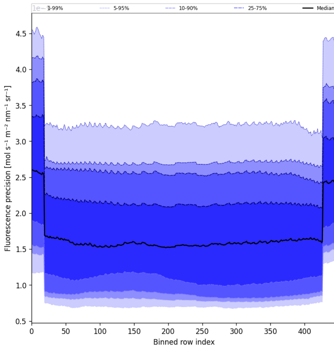
Figure 56: Along track statistics of “Fluorescence precision” for 2025-01-10 to 2025-01-10
