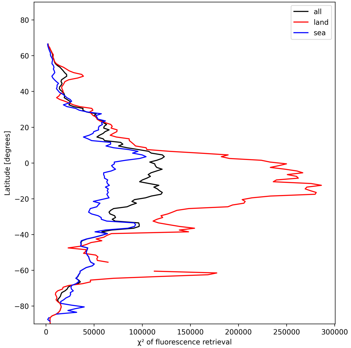
Figure 23: Zonal average of “ \chi^2 of fluorescence retrieval” for 2025-01-10 to 2025-01-10.
