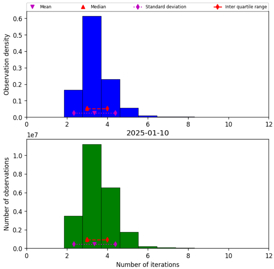
Figure 37: Histogram of “Number of iterations” for 2025-01-10 to 2025-01-10
