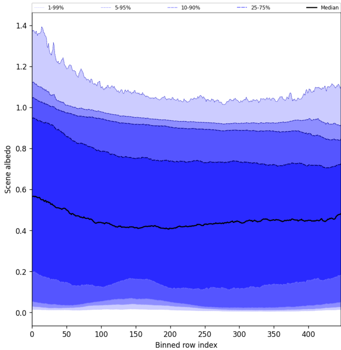
Figure 49: Along track statistics of “Scene albedo” for 2025-01-10 to 2025-01-10
