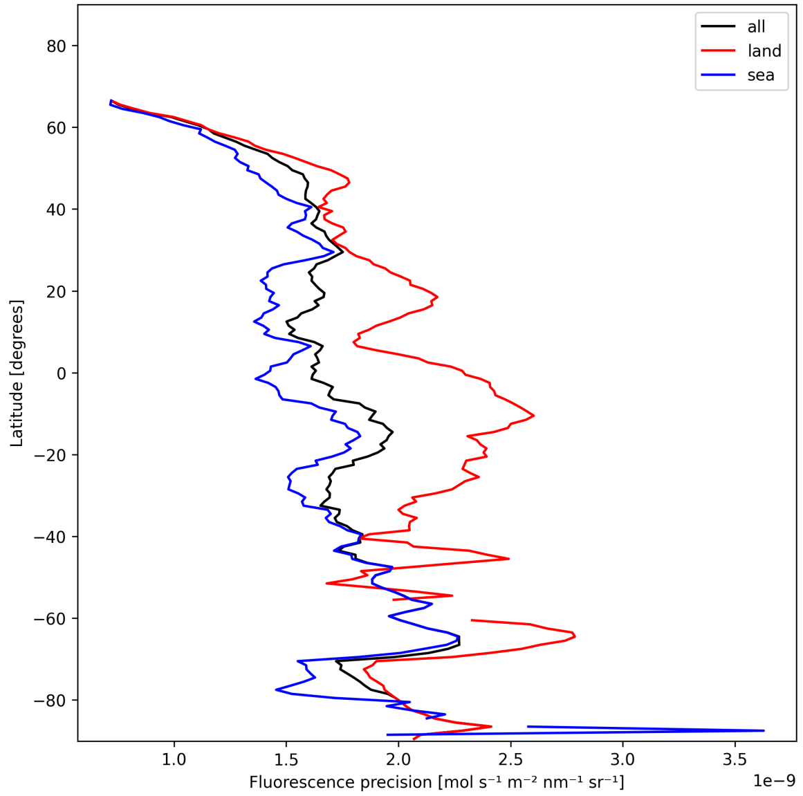
Figure 22: Zonal average of “Fluorescence precision” for 2025-01-10 to 2025-01-10.
