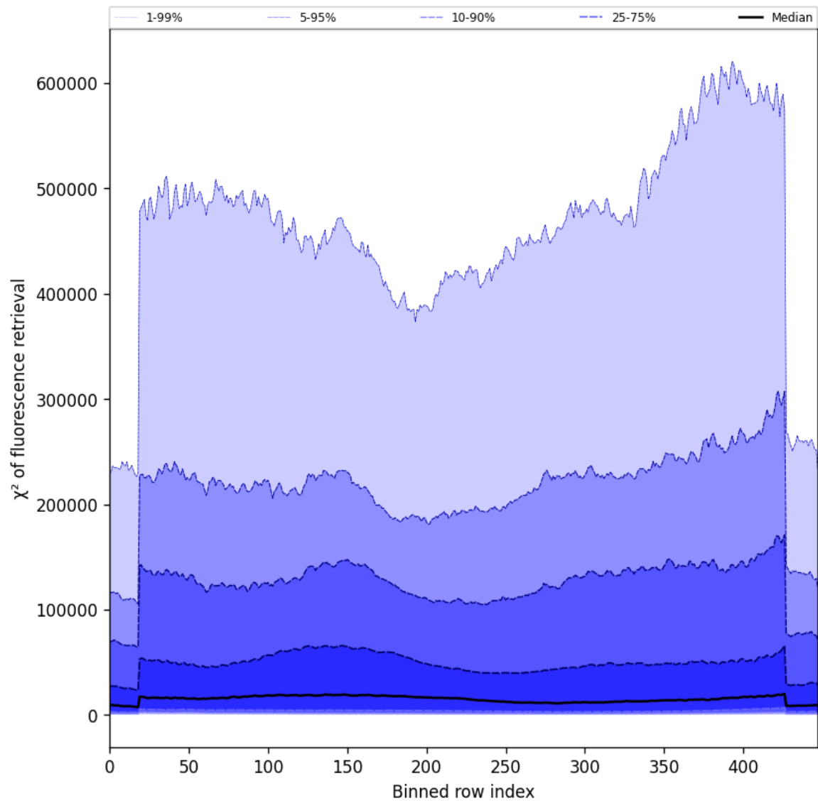
Figure 57: Along track statistics of “ \chi^2 of fluorescence retrieval” for 2025-01-10 to 2025-01-10
