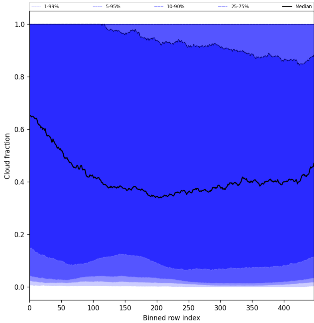
Figure 47: Along track statistics of “Cloud fraction” for 2025-01-10 to 2025-01-10
