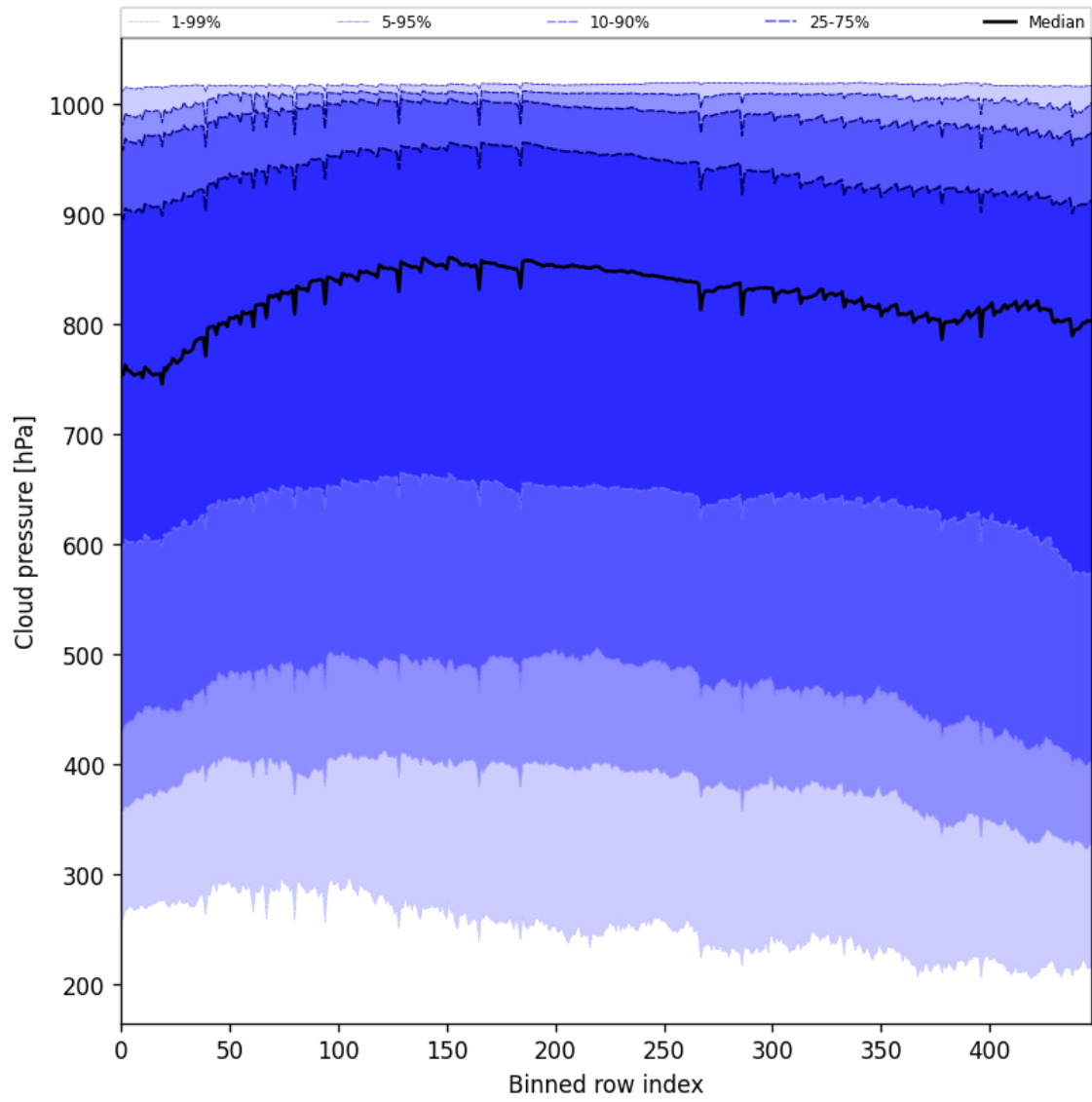
Figure 45: Along track statistics of “Cloud pressure” for 2025-01-10 to 2025-01-10
