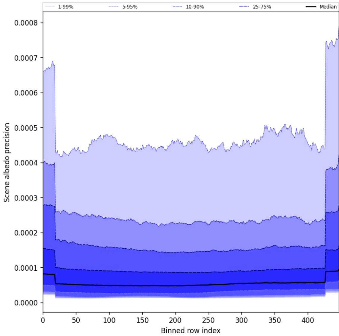
Figure 50: Along track statistics of “Scene albedo precision” for 2025-01-10 to 2025-01-10
