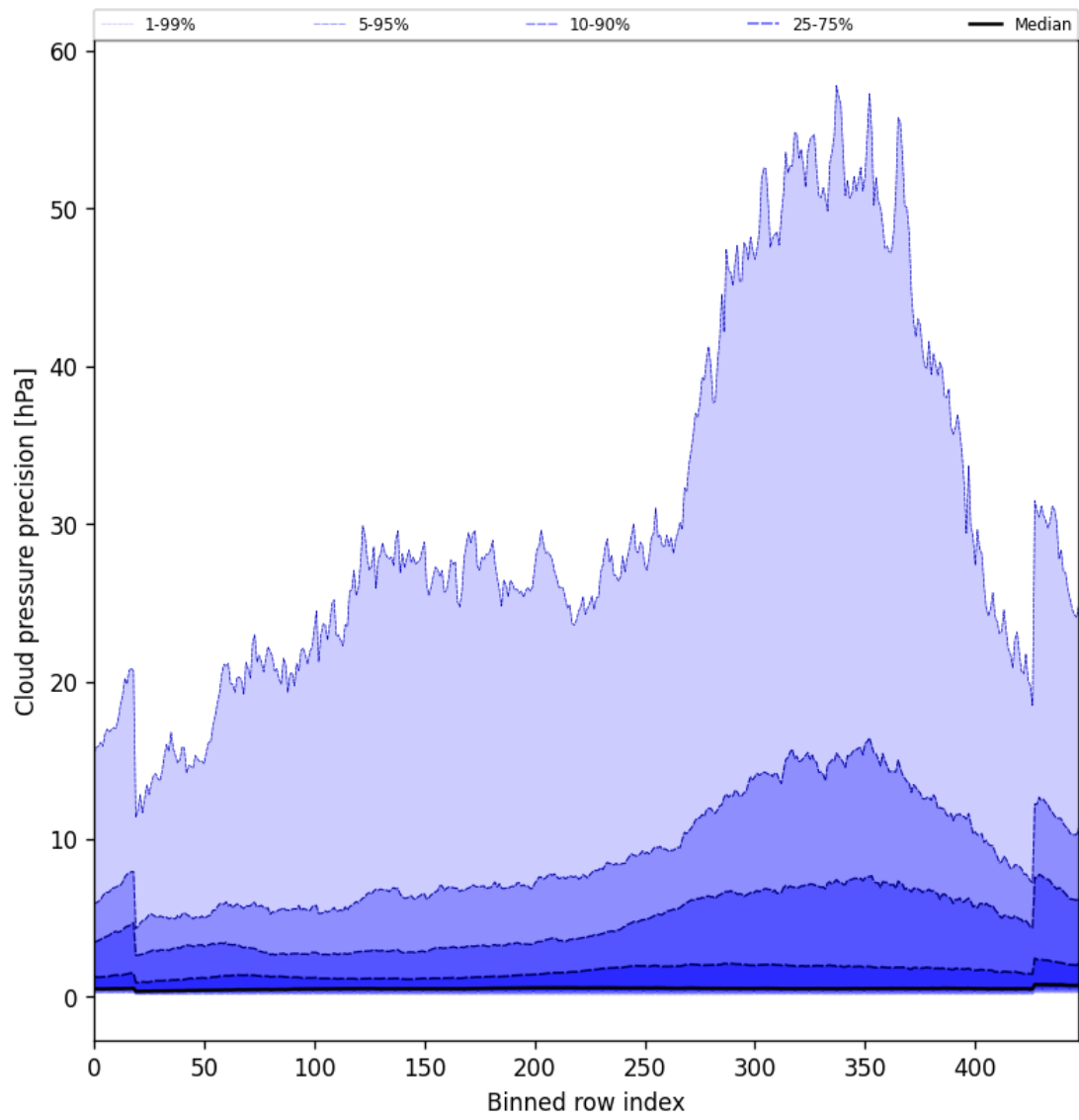
Figure 46: Along track statistics of “Cloud pressure precision” for 2025-01-10 to 2025-01-10
