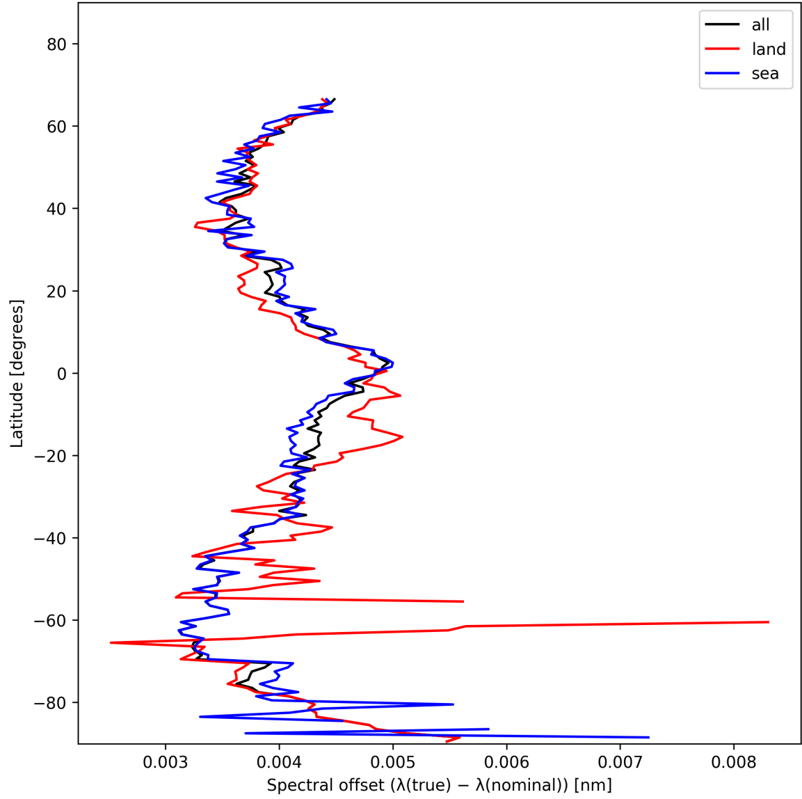
Figure 26: Zonal average of “Spectral offset ( \lambda_{\text{true}} - \lambda_{\text{nominal}} )” for 2025-01-10 to 2025-01-10.
