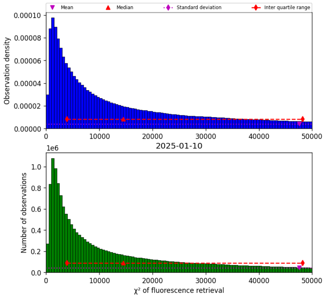
Figure 40: Histogram of “ \chi^2 of fluorescence retrieval” for 2025-01-10 to 2025-01-10
