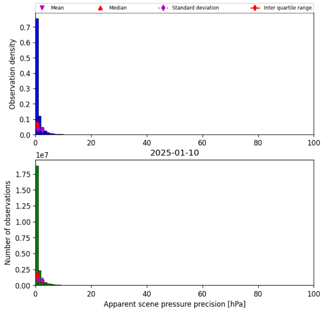
Figure 35: Histogram of “Apparent scene pressure precision” for 2025-01-10 to 2025-01-10
