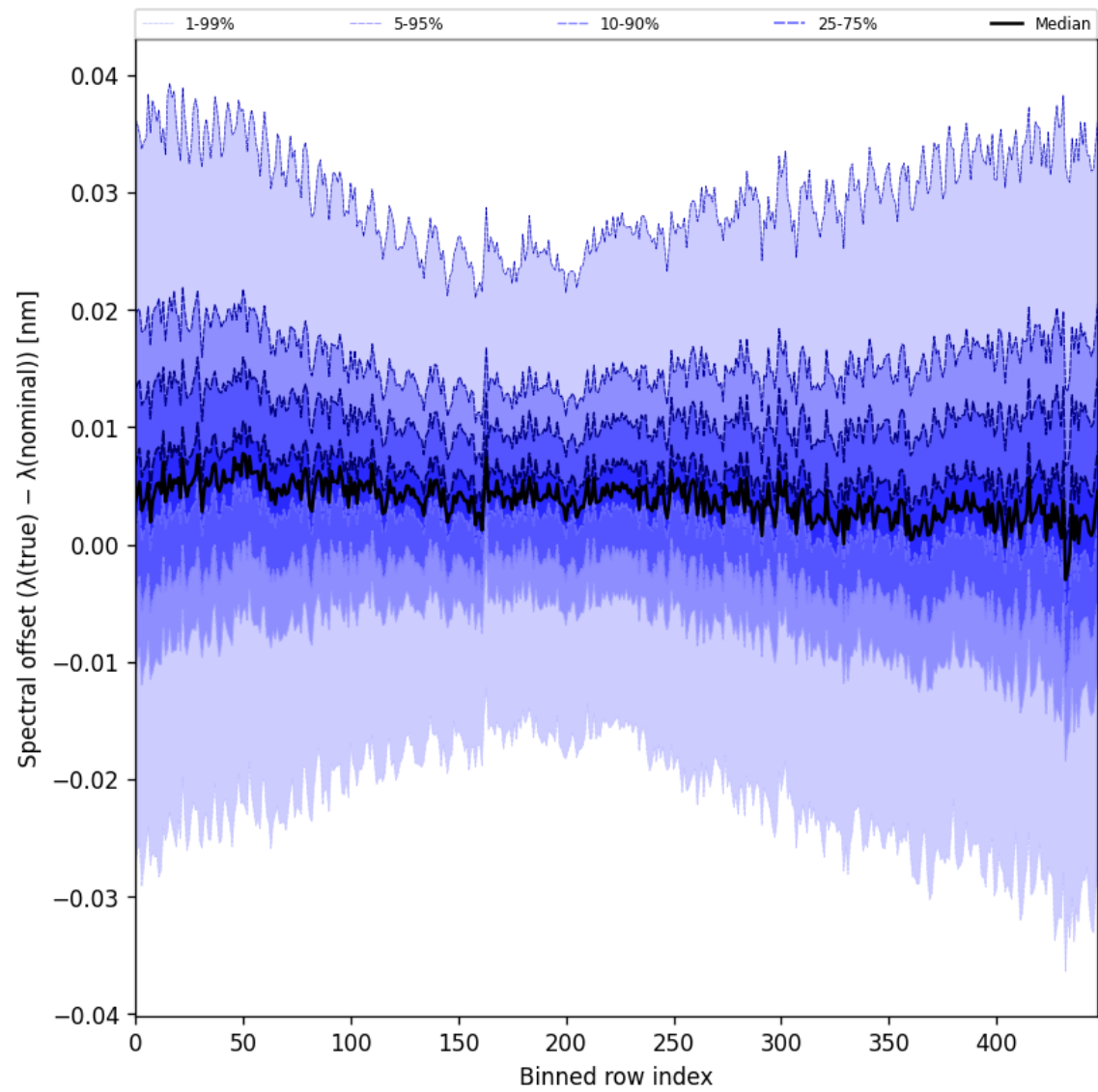
Figure 60: Along track statistics of “Spectral offset ( \lambda_{\text{true}} - \lambda_{\text{nominal}} )” for 2025-01-10 to 2025-01-10
