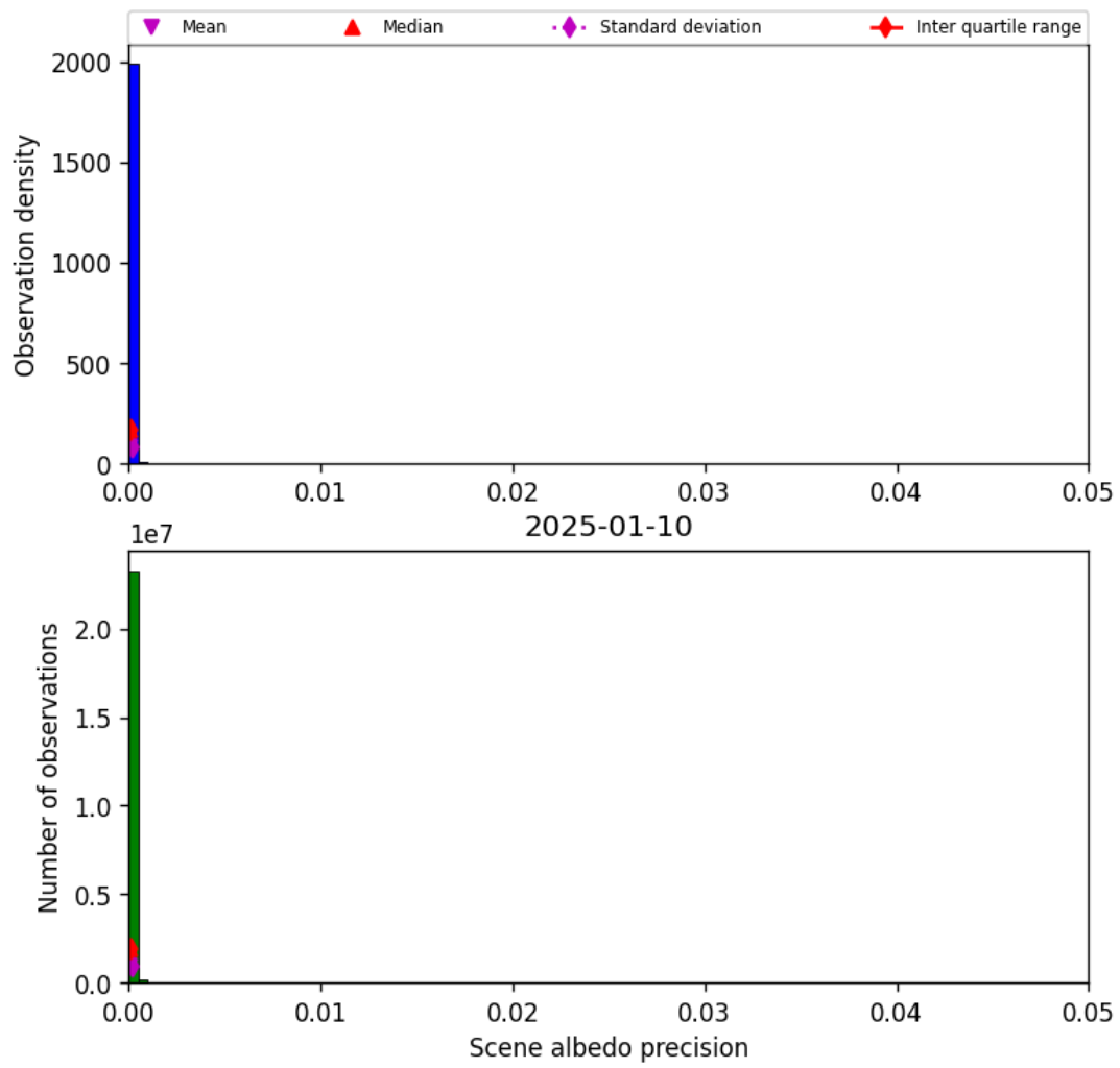
Figure 33: Histogram of “Scene albedo precision” for 2025-01-10 to 2025-01-10
