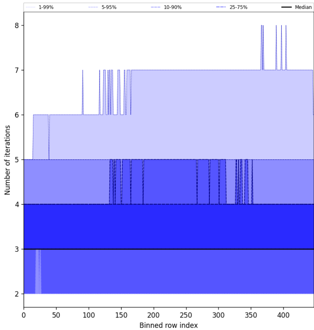
Figure 54: Along track statistics of “Number of iterations” for 2025-01-10 to 2025-01-10
