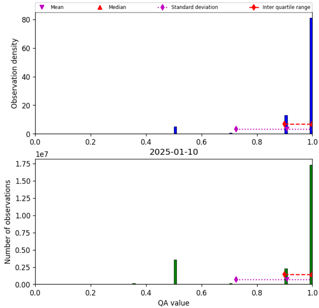
Figure 27: Histogram of “QA value” for 2025-01-10 to 2025-01-10
