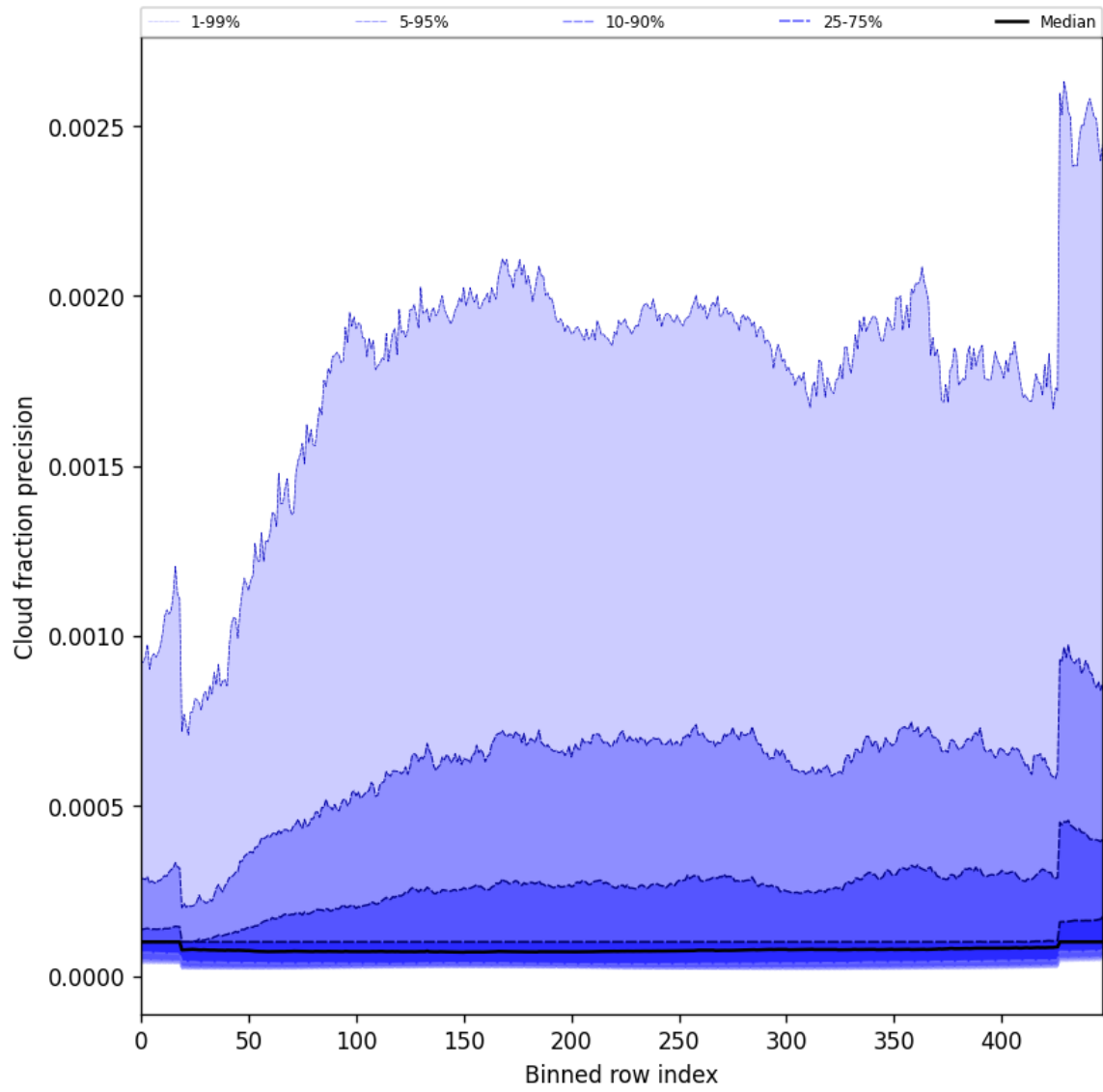
Figure 48: Along track statistics of “Cloud fraction precision” for 2025-01-10 to 2025-01-10
