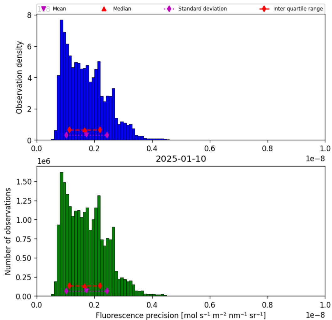
Figure 39: Histogram of “Fluorescence precision” for 2025-01-10 to 2025-01-10
