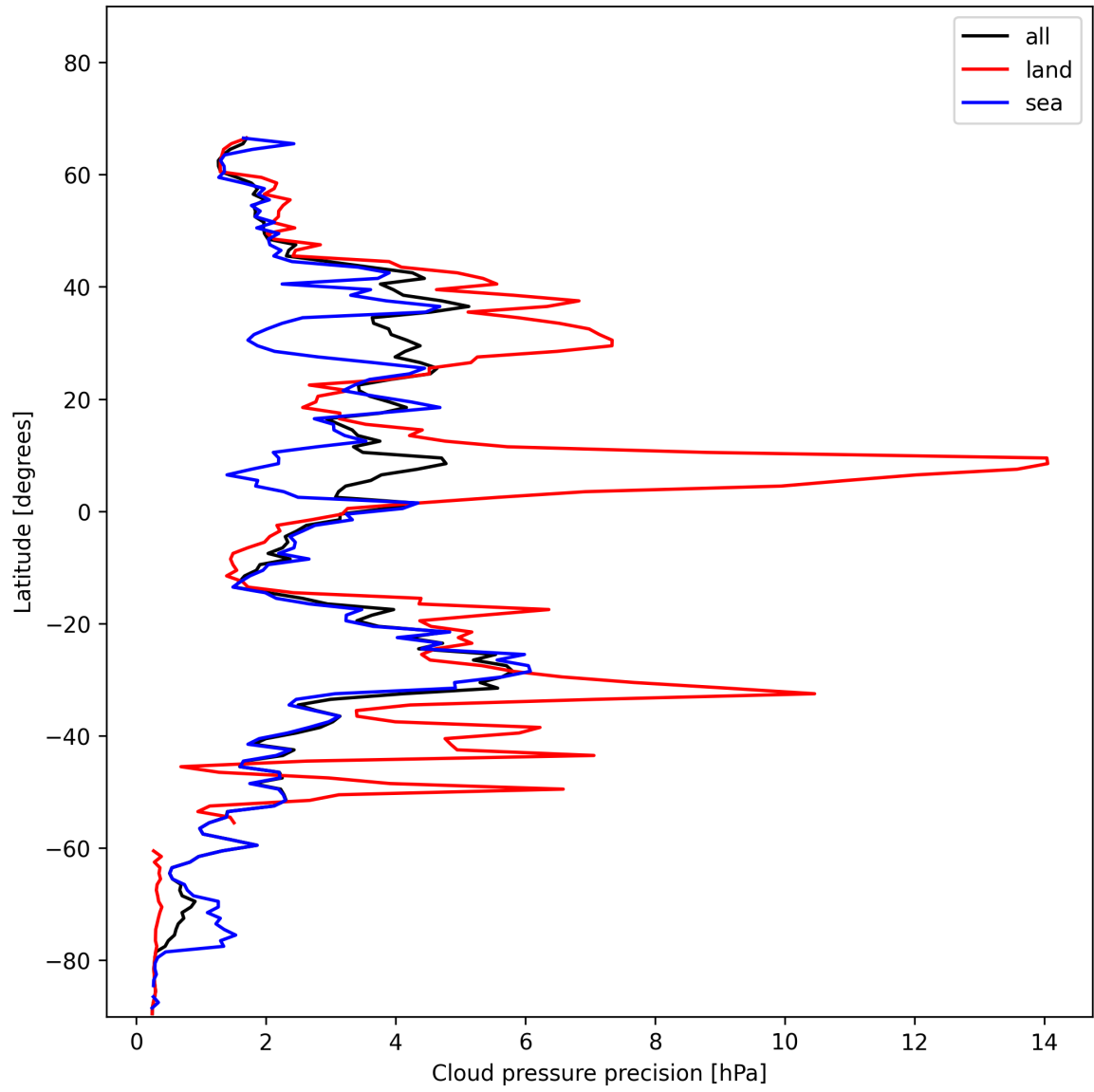
Figure 12: Zonal average of “Cloud pressure precision” for 2025-01-10 to 2025-01-10.
