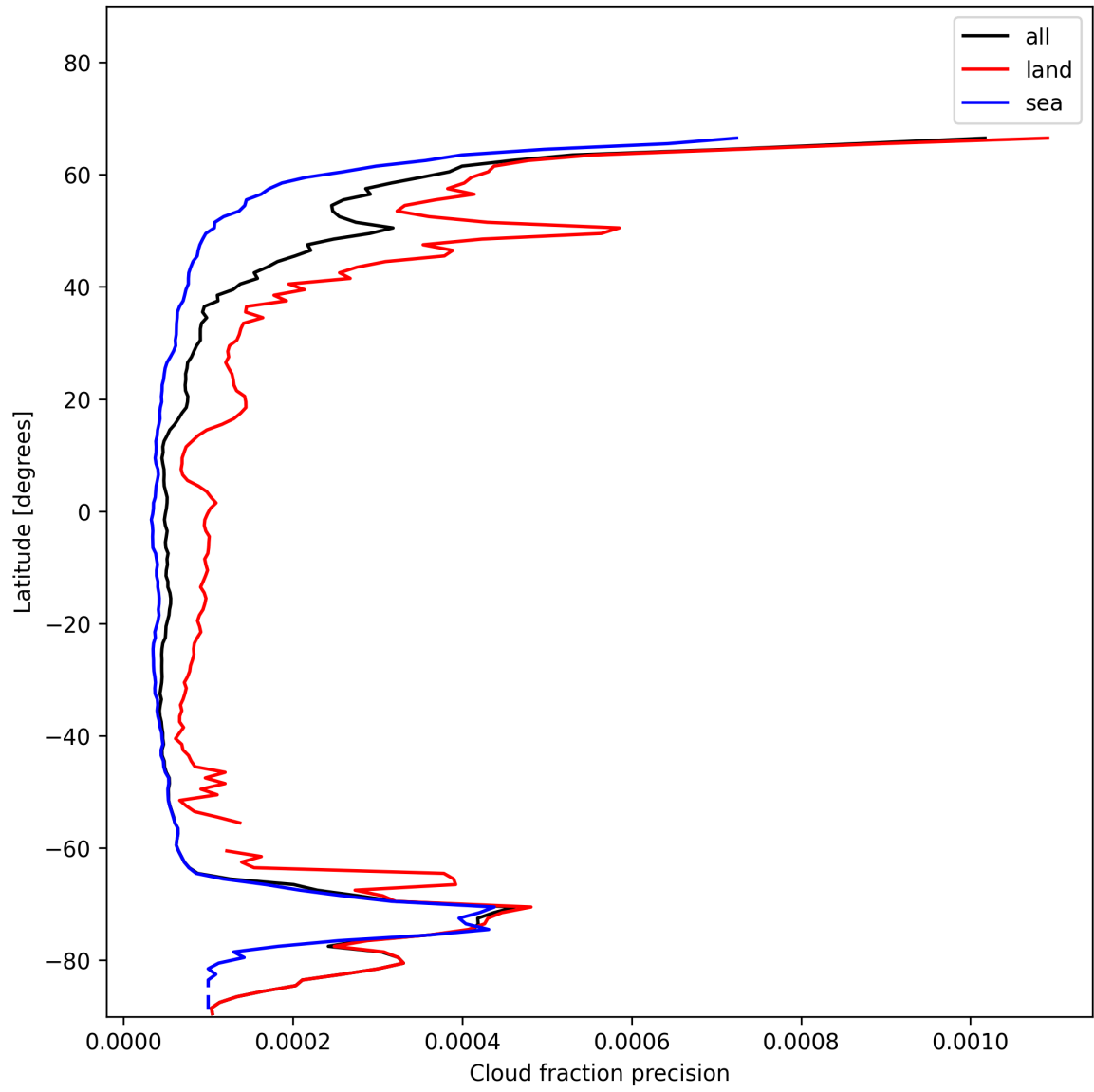
Figure 14: Zonal average of “Cloud fraction precision” for 2025-01-10 to 2025-01-10.
