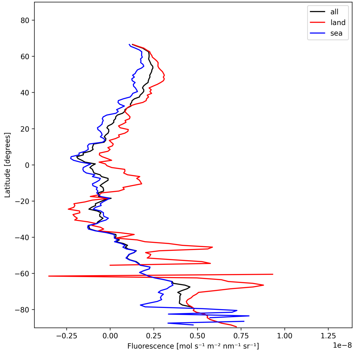
Figure 21: Zonal average of “Fluorescence” for 2025-01-10 to 2025-01-10.
