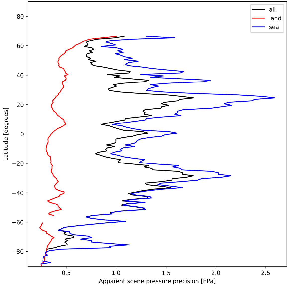
Figure 18: Zonal average of “Apparent scene pressure precision” for 2025-01-10 to 2025-01-10.
