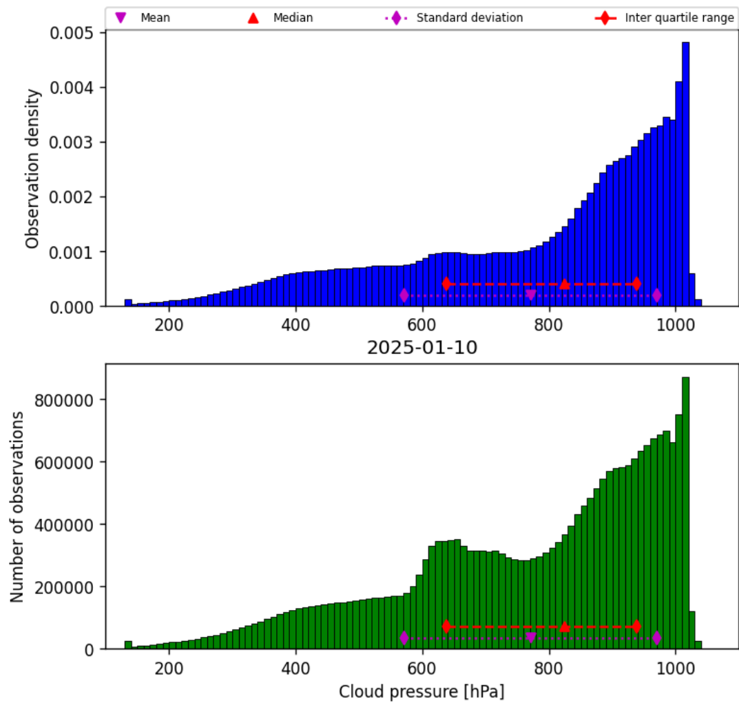
Figure 28: Histogram of “Cloud pressure” for 2025-01-10 to 2025-01-10
