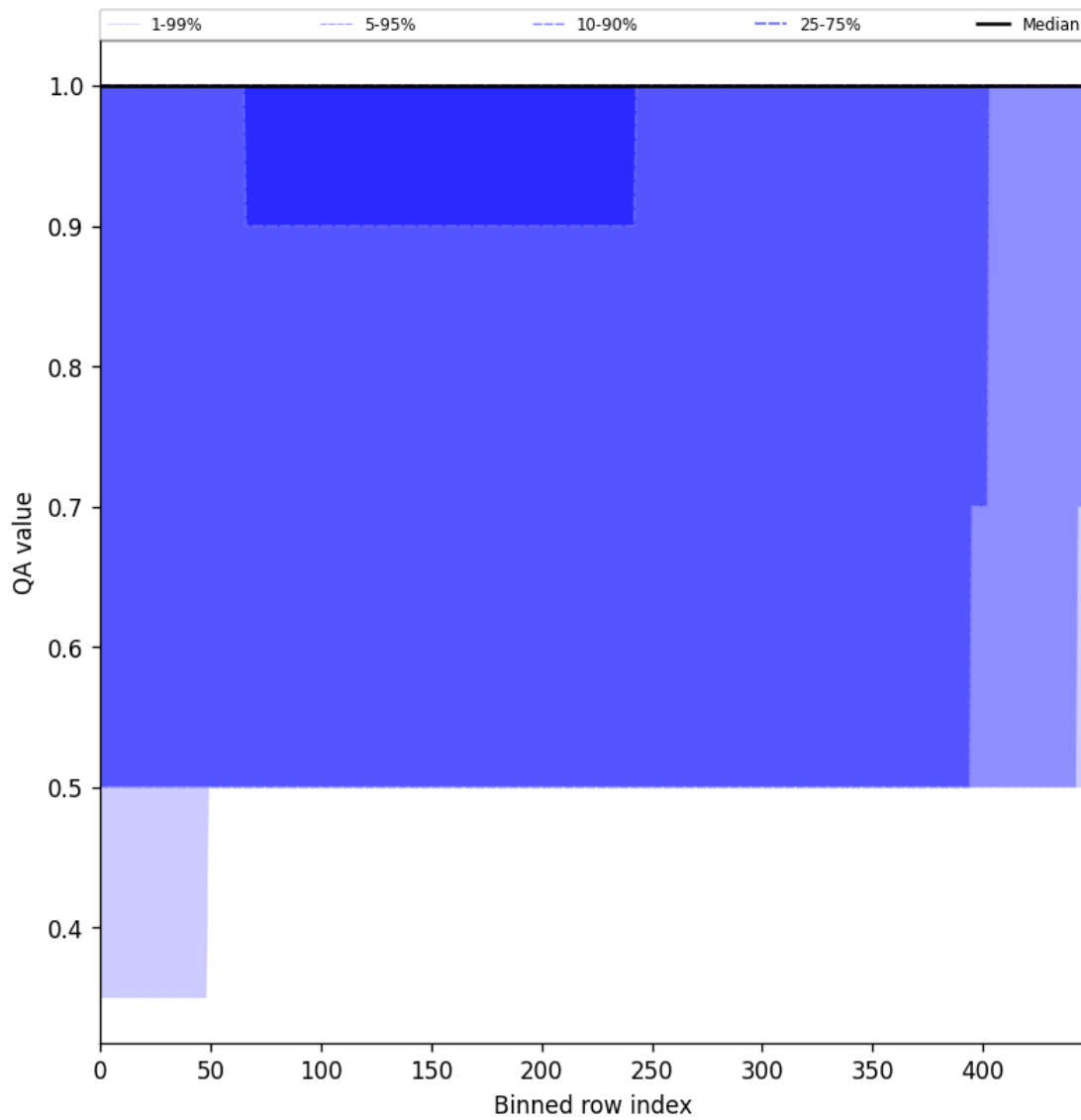
Figure 44: Along track statistics of “QA value” for 2025-01-10 to 2025-01-10
