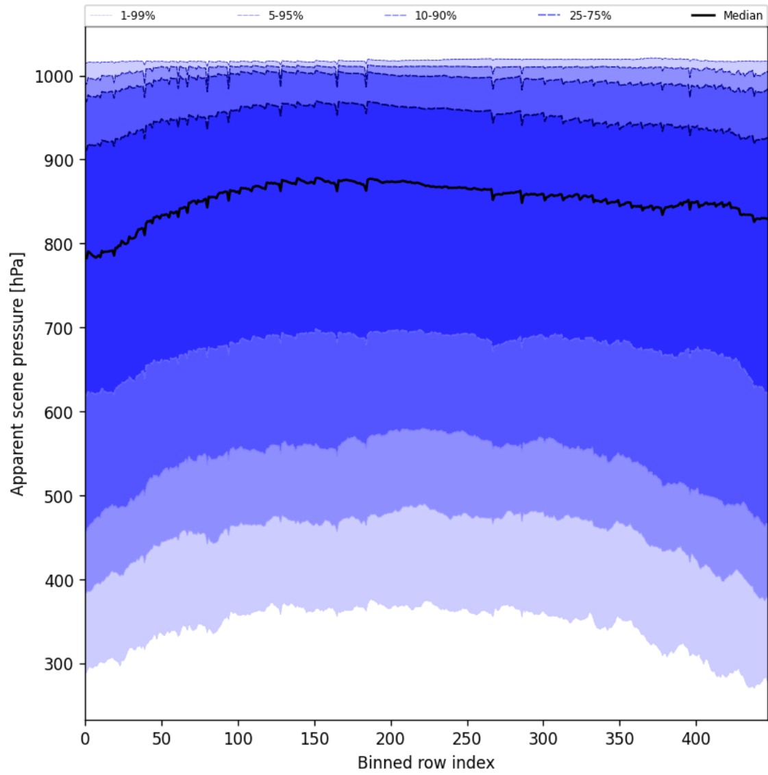
Figure 51: Along track statistics of “Apparent scene pressure” for 2025-01-10 to 2025-01-10
