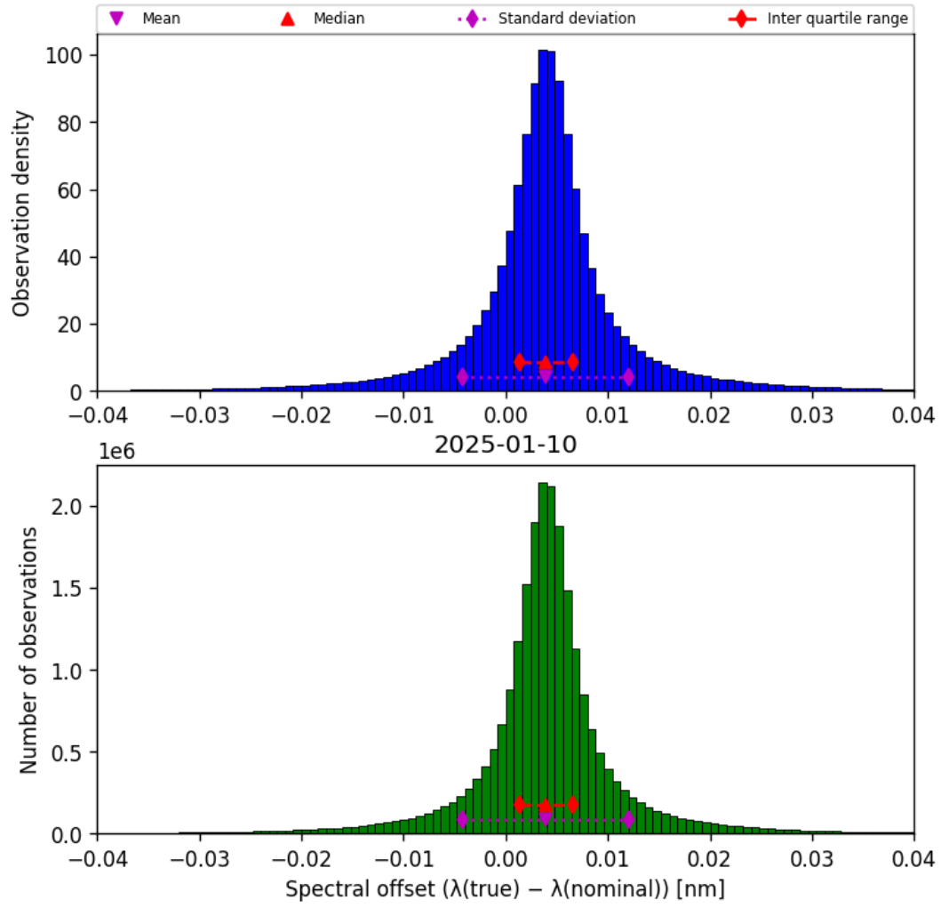
Figure 43: Histogram of “Spectral offset ( \lambda_{\text{true}} - \lambda_{\text{nominal}} )” for 2025-01-10 to 2025-01-10
