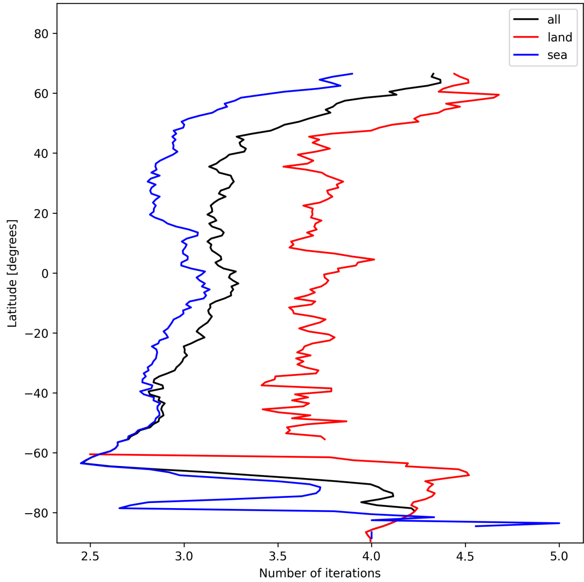
Figure 20: Zonal average of “Number of iterations” for 2025-01-10 to 2025-01-10.
