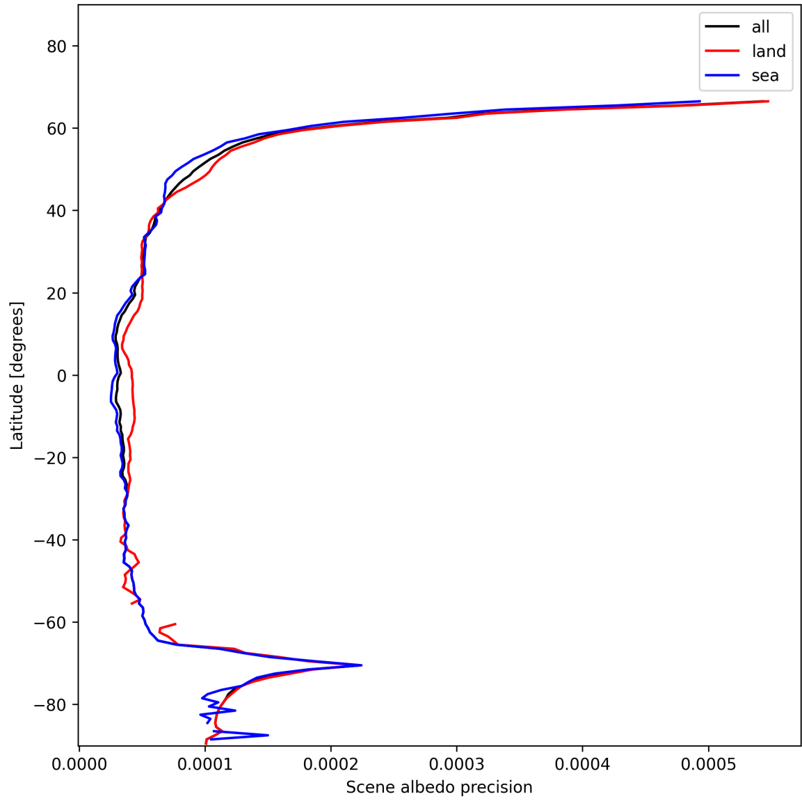
Figure 16: Zonal average of “Scene albedo precision” for 2025-01-10 to 2025-01-10.
