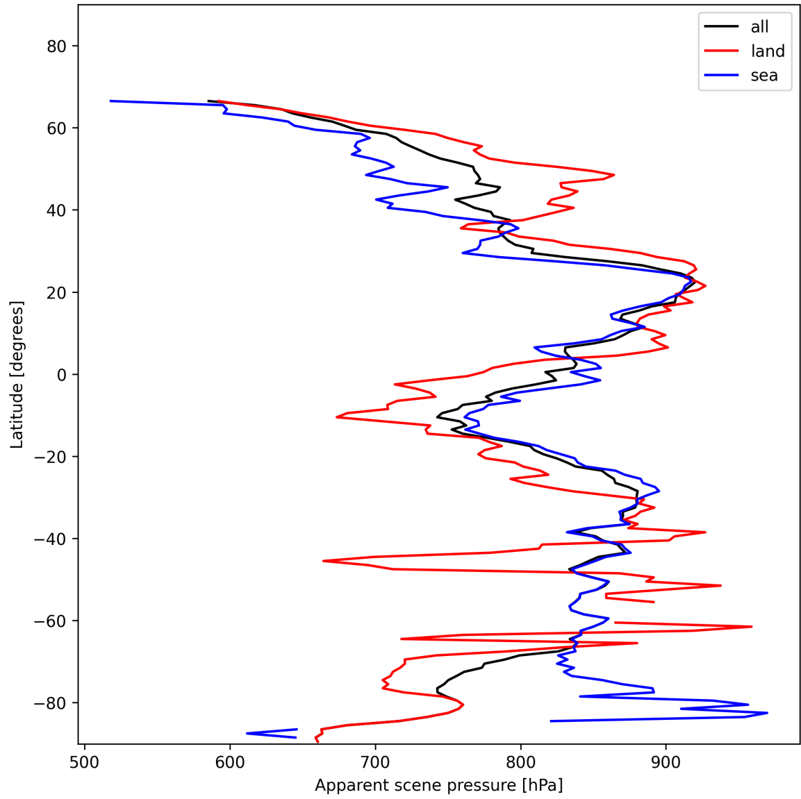
Figure 17: Zonal average of “Apparent scene pressure” for 2025-01-10 to 2025-01-10.
