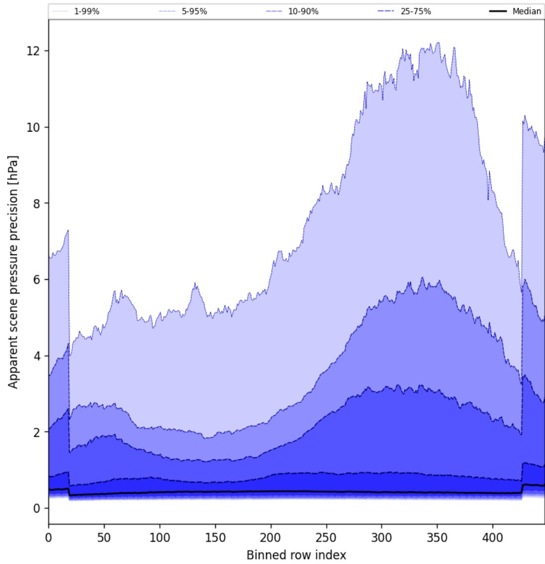
Figure 52: Along track statistics of “Apparent scene pressure precision” for 2025-01-10 to 2025-01-10
