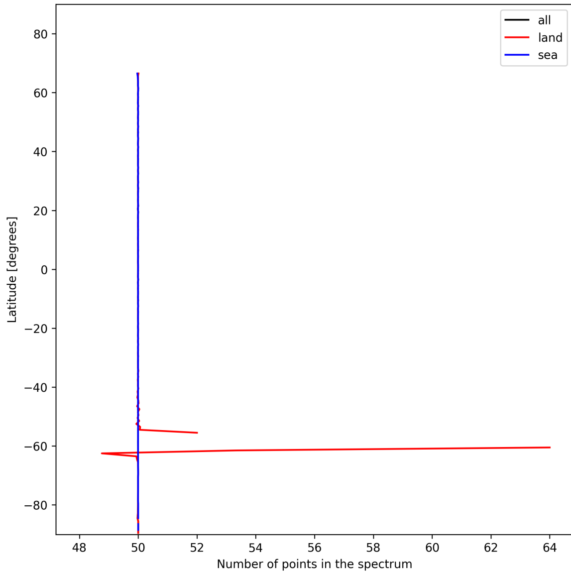
Figure 25: Zonal average of “Number of points in the spectrum” for 2025-01-10 to 2025-01-10.
