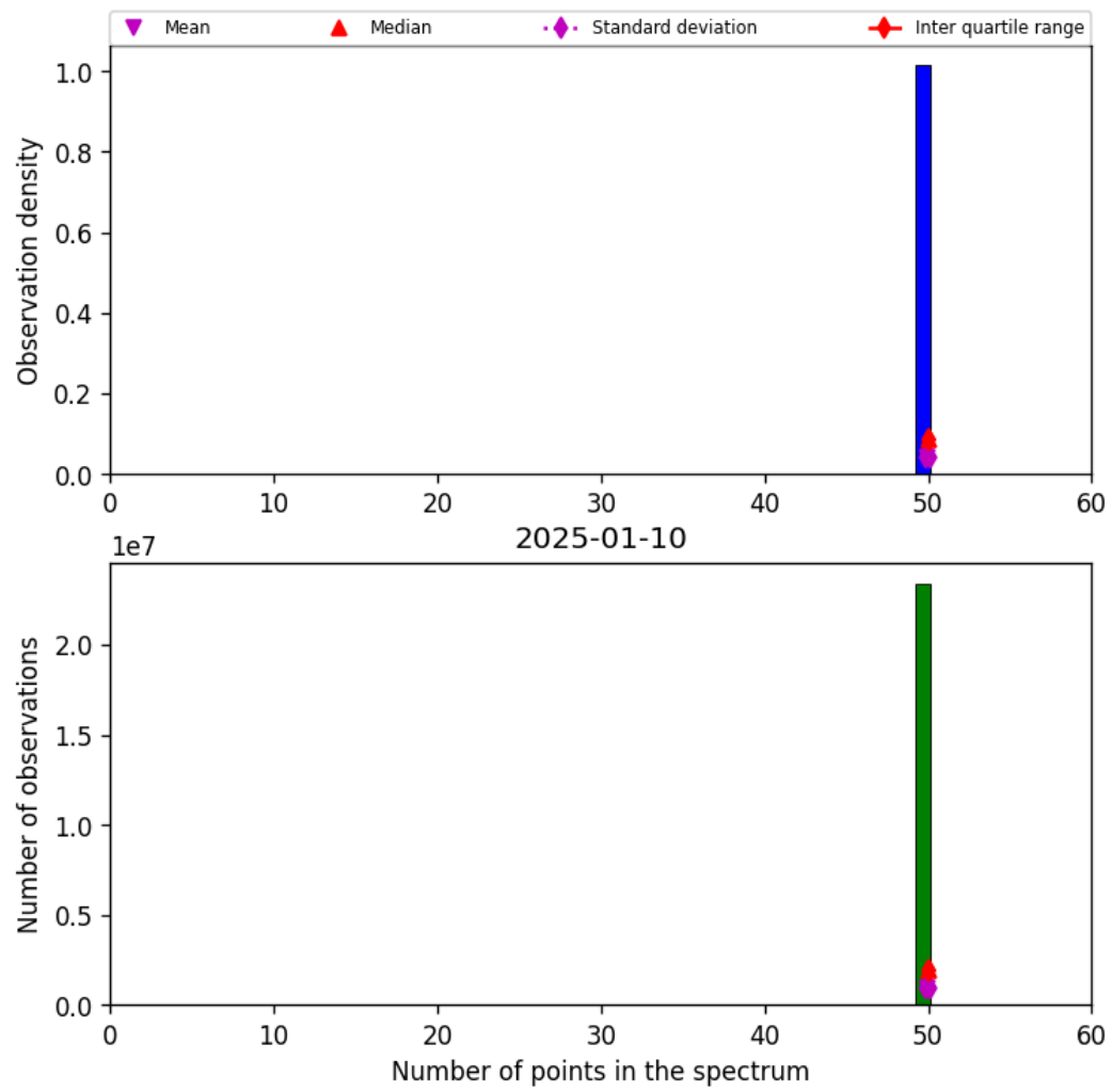
Figure 42: Histogram of “Number of points in the spectrum” for 2025-01-10 to 2025-01-10
