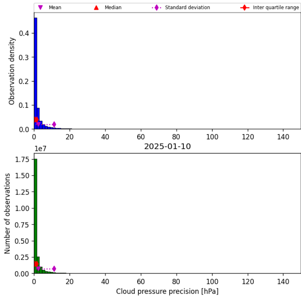
Figure 29: Histogram of “Cloud pressure precision” for 2025-01-10 to 2025-01-10
