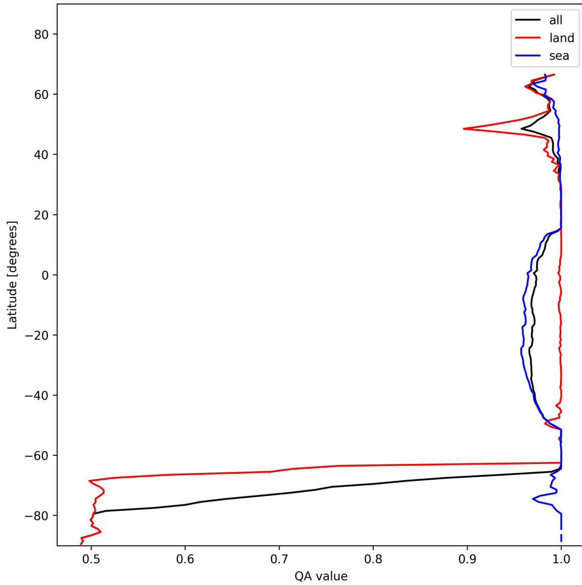
Figure 10: Zonal average of “QA value” for 2025-01-10 to 2025-01-10.
