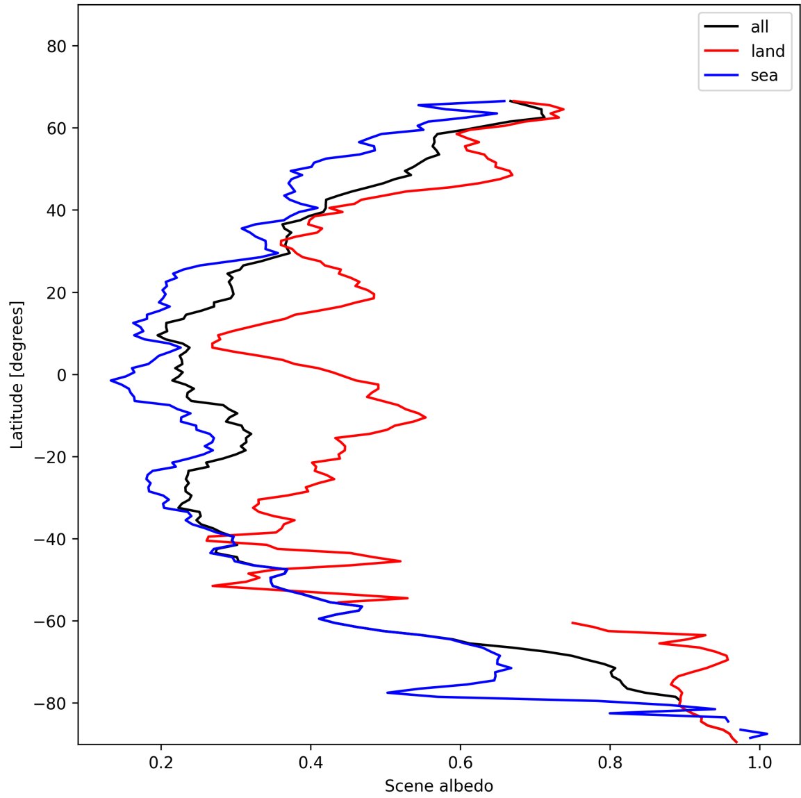
Figure 15: Zonal average of “Scene albedo” for 2025-01-10 to 2025-01-10.
