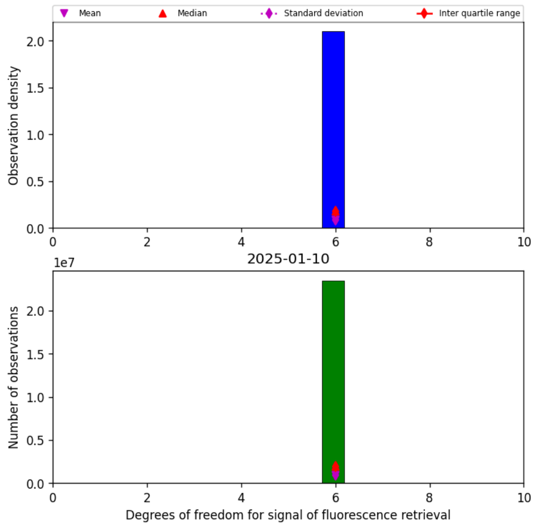
Figure 41: Histogram of “Degrees of freedom for signal of fluorescence retrieval” for 2025-01-10 to 2025-01-10
