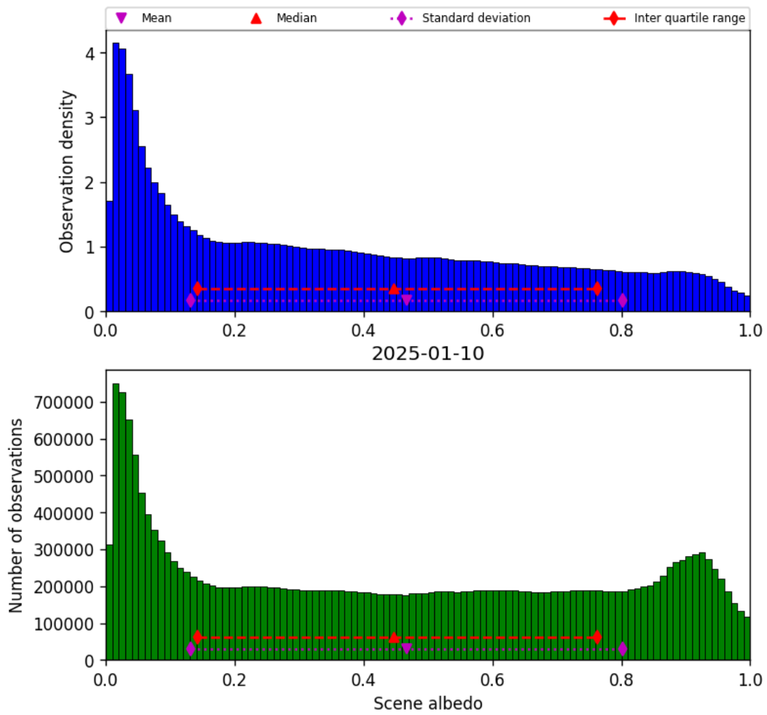
Figure 32: Histogram of “Scene albedo” for 2025-01-10 to 2025-01-10
