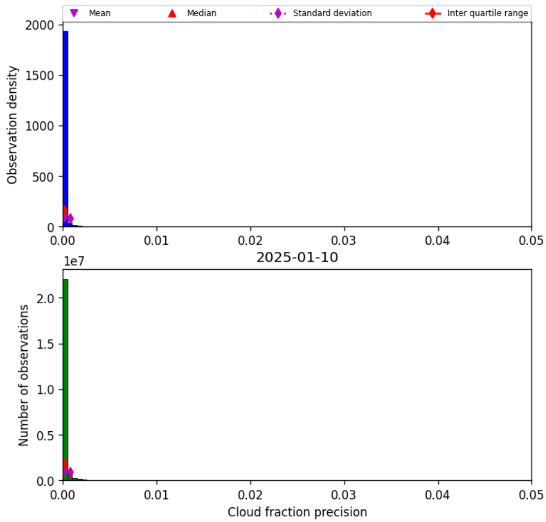
Figure 31: Histogram of “Cloud fraction precision” for 2025-01-10 to 2025-01-10
