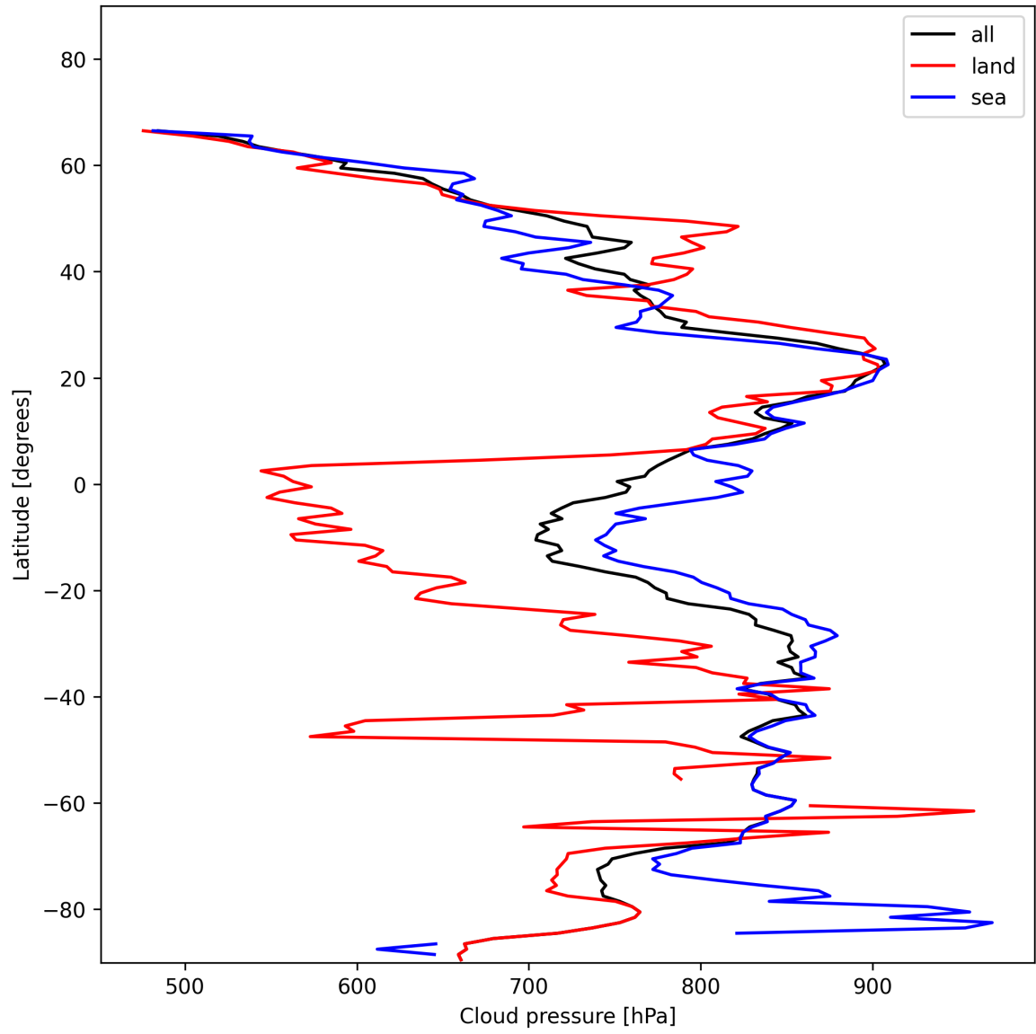
Figure 11: Zonal average of “Cloud pressure” for 2025-01-10 to 2025-01-10.
