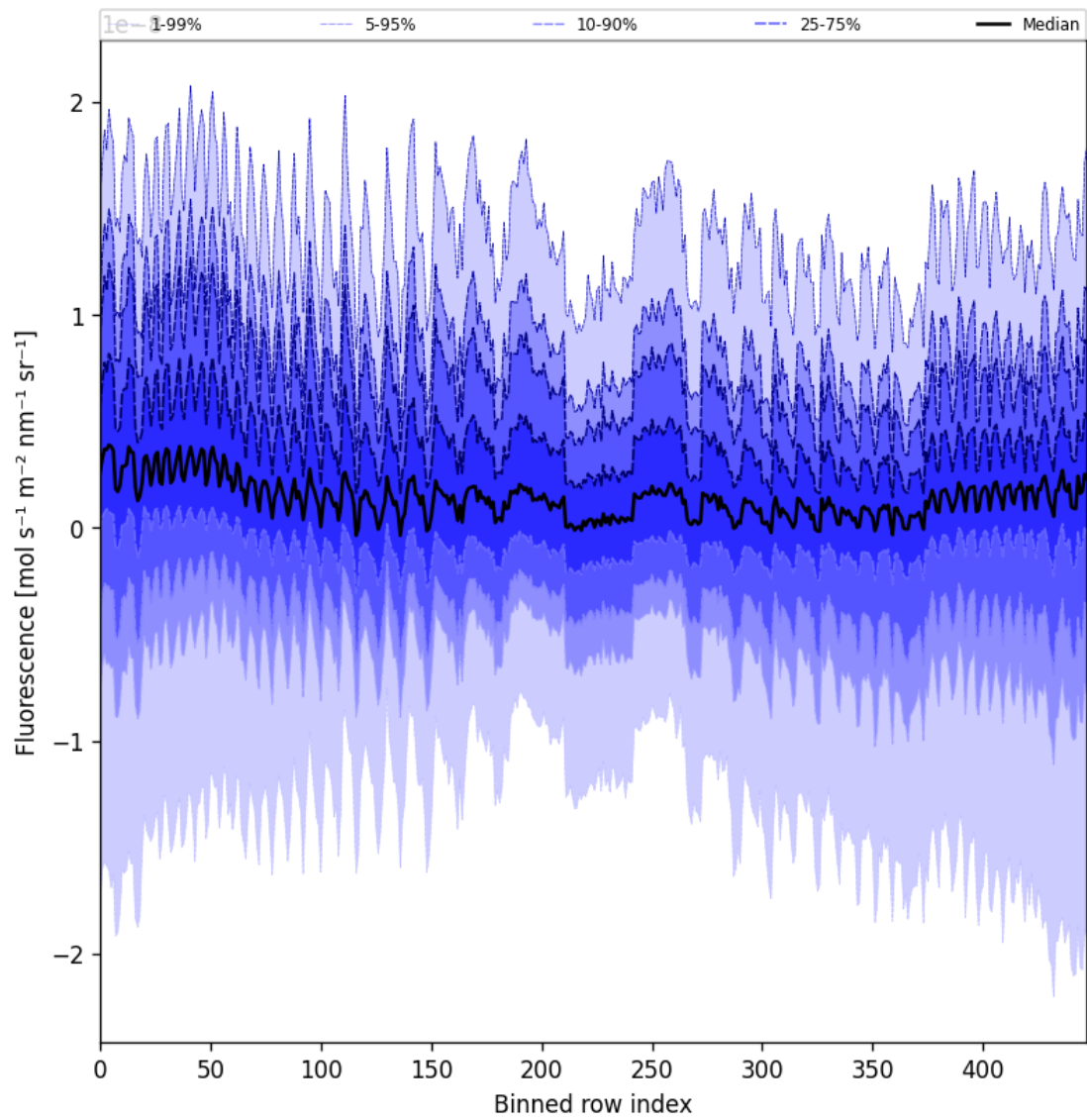
Figure 55: Along track statistics of “Fluorescence” for 2025-01-10 to 2025-01-10
