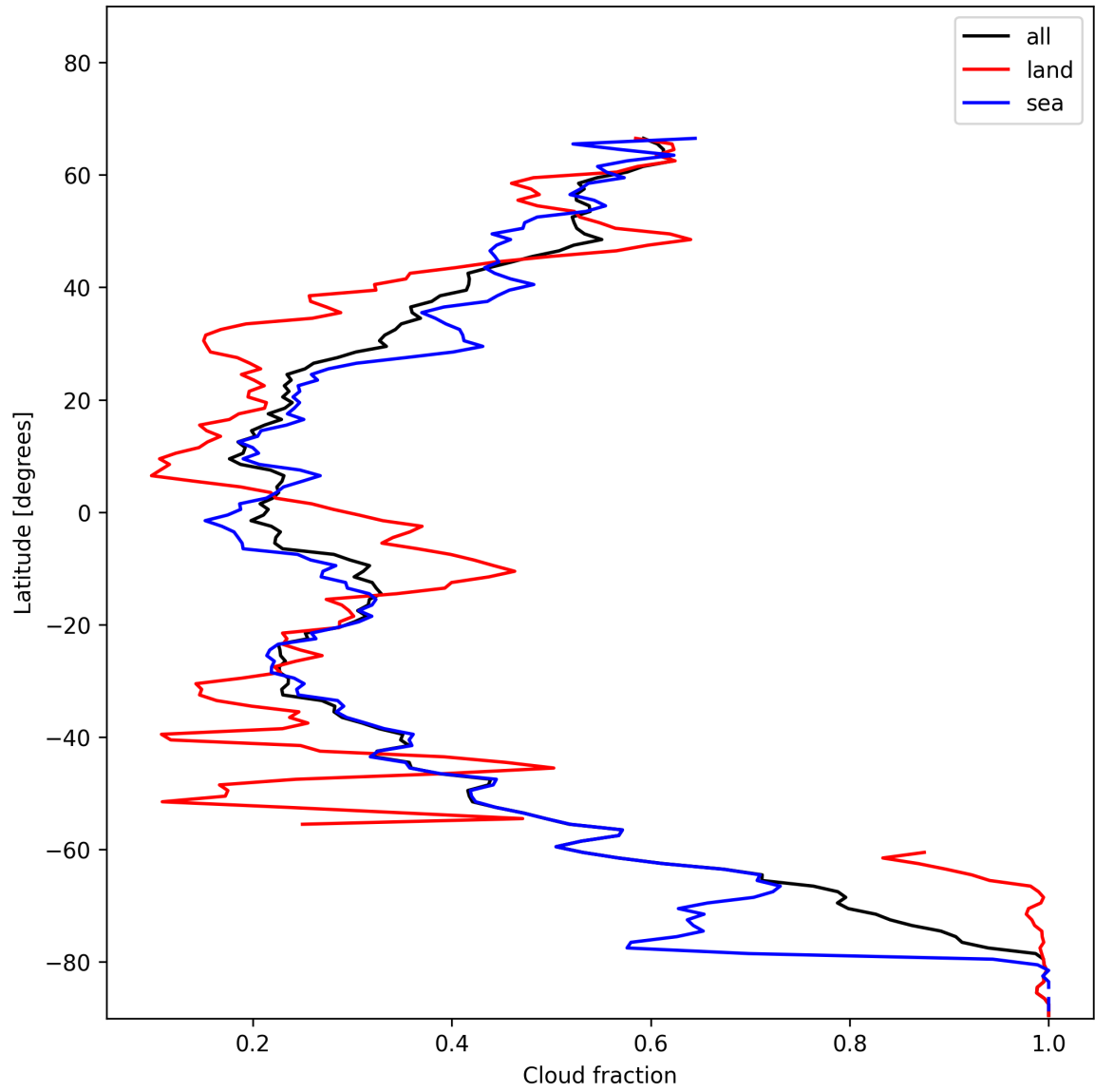
Figure 13: Zonal average of “Cloud fraction” for 2025-01-10 to 2025-01-10.
