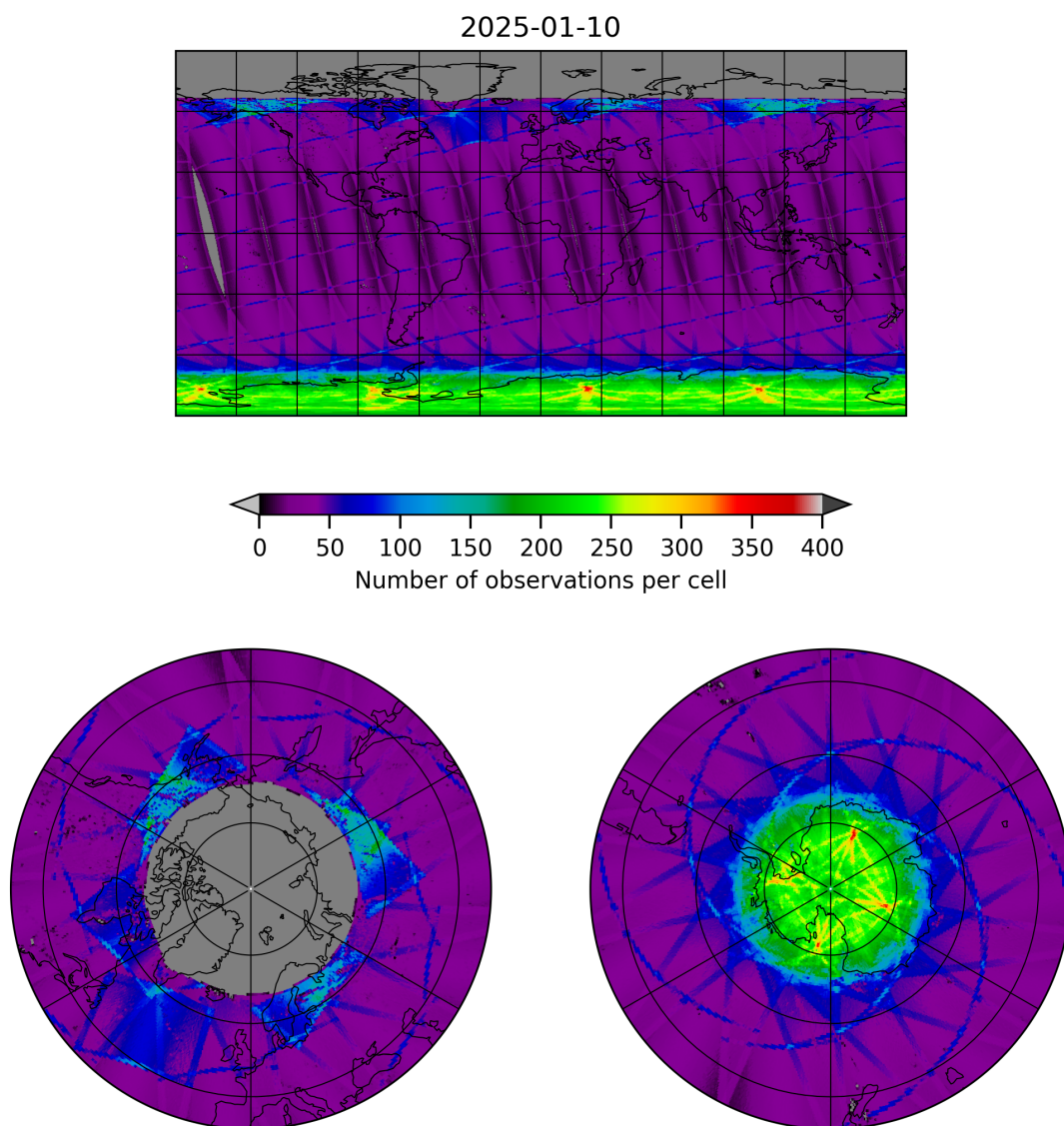
Figure 9: Map of the number of observations for 2025-01-10 to 2025-01-10
