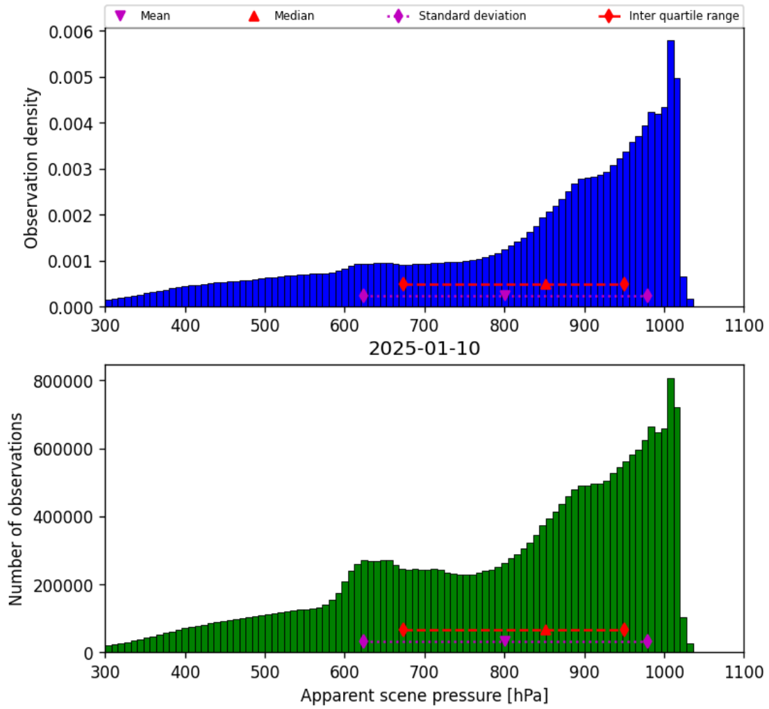
Figure 34: Histogram of “Apparent scene pressure” for 2025-01-10 to 2025-01-10
