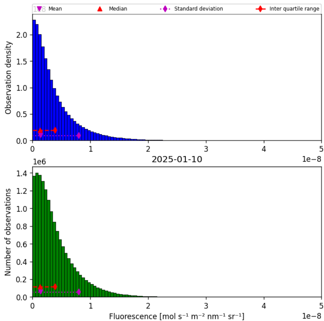
Figure 38: Histogram of “Fluorescence” for 2025-01-10 to 2025-01-10
