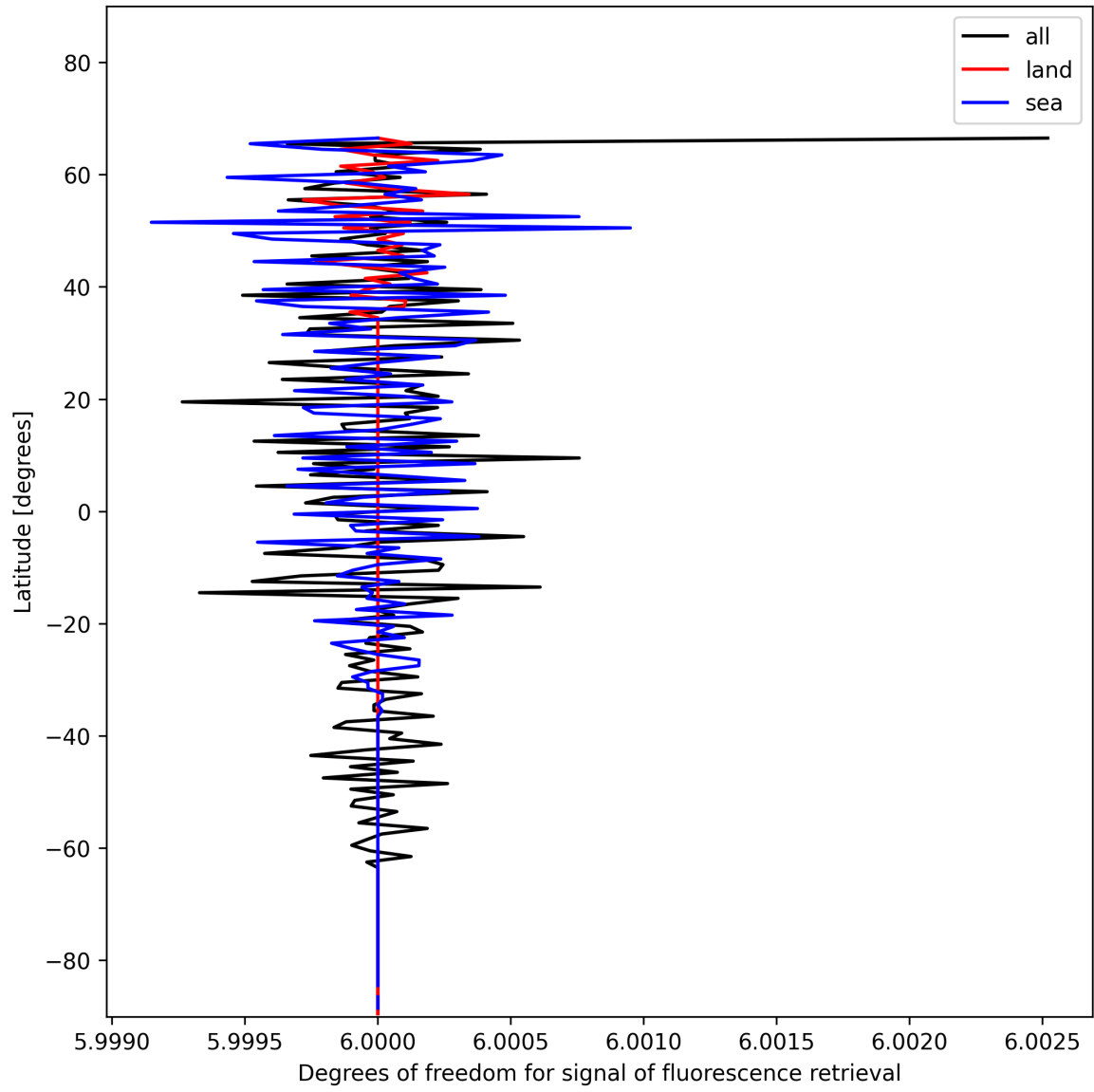
Figure 24: Zonal average of “Degrees of freedom for signal of fluorescence retrieval” for 2025-01-10 to 2025-01-10.
