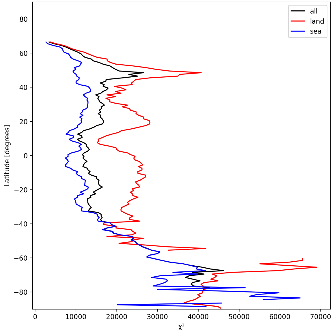
Figure 19: Zonal average of “ \chi^2 ” for 2025-01-10 to 2025-01-10.
