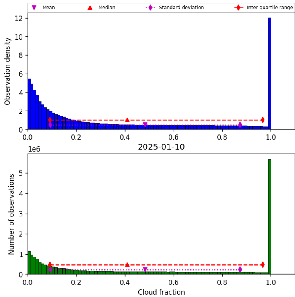
Figure 30: Histogram of “Cloud fraction” for 2025-01-10 to 2025-01-10
