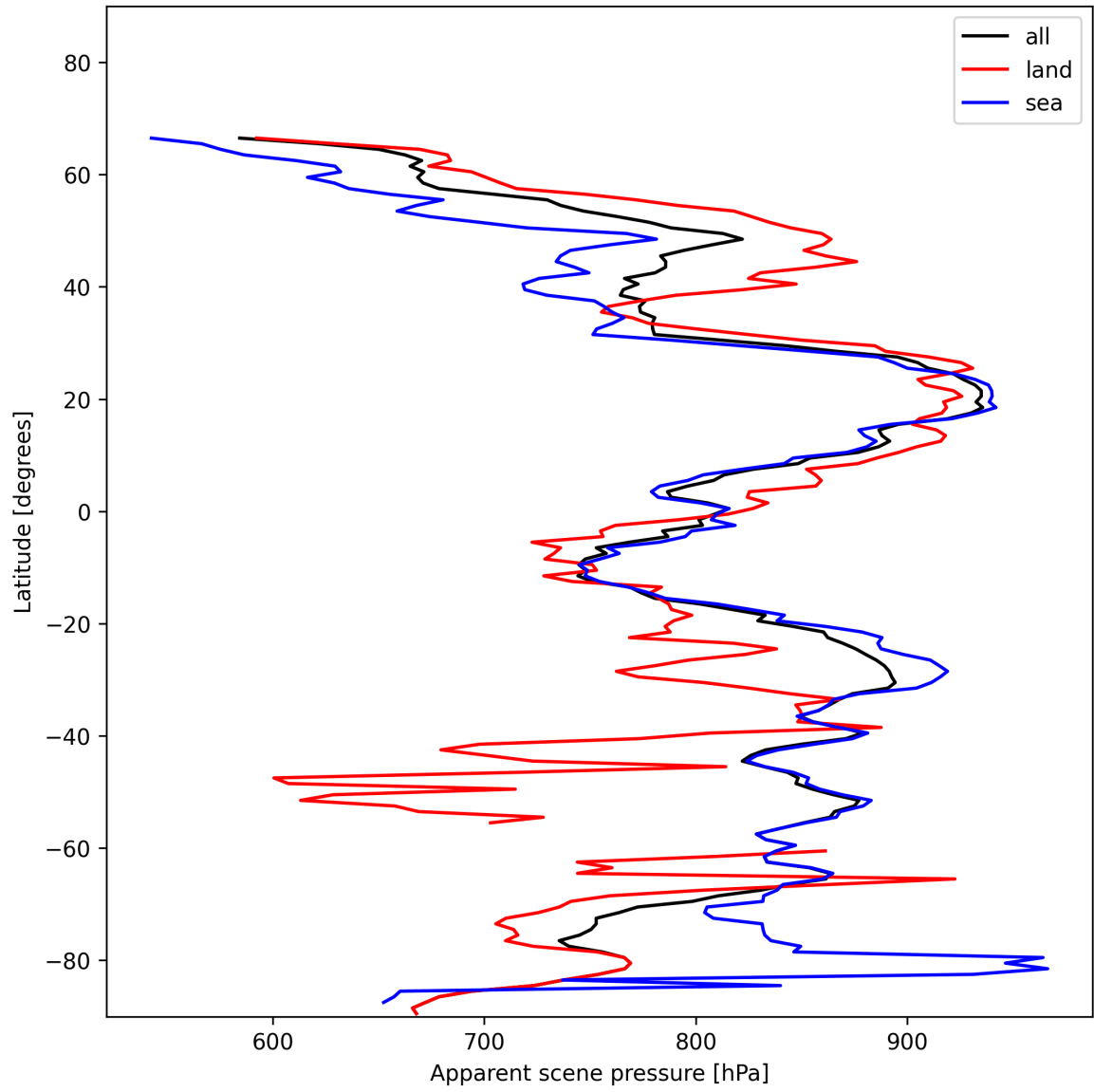
Figure 17: Zonal average of “Apparent scene pressure” for 2025-01-11 to 2025-01-12.
