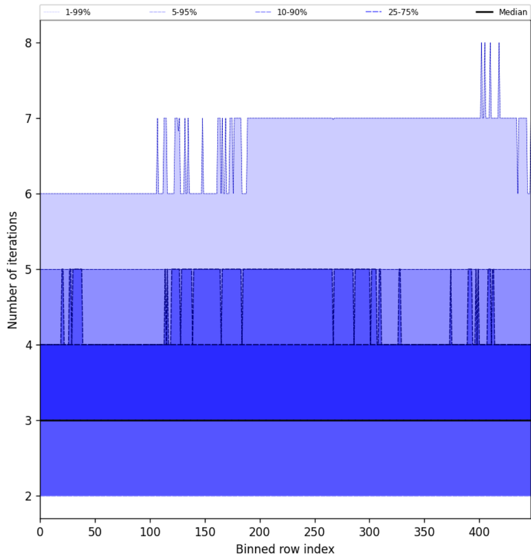
Figure 54: Along track statistics of “Number of iterations” for 2025-01-11 to 2025-01-12
