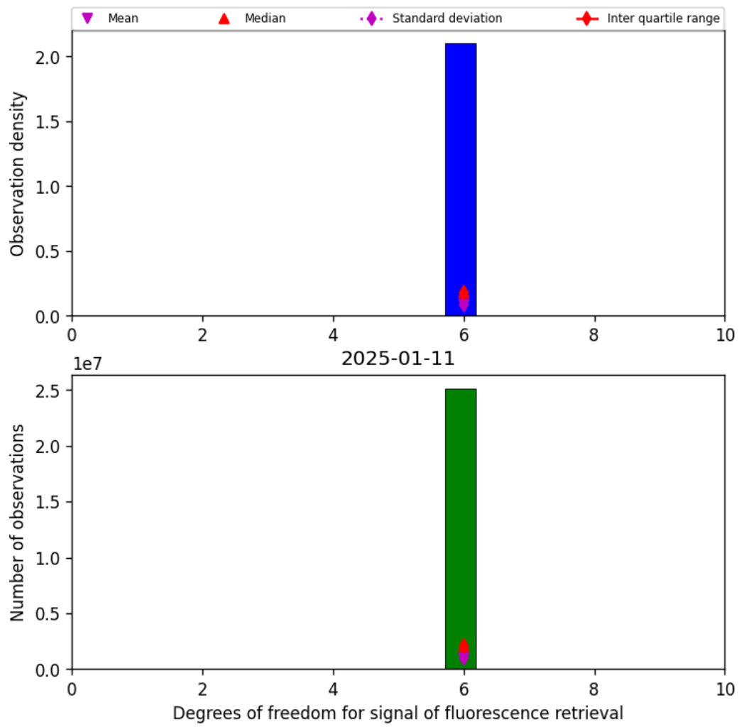
Figure 41: Histogram of “Degrees of freedom for signal of fluorescence retrieval” for 2025-01-11 to 2025-01-12
