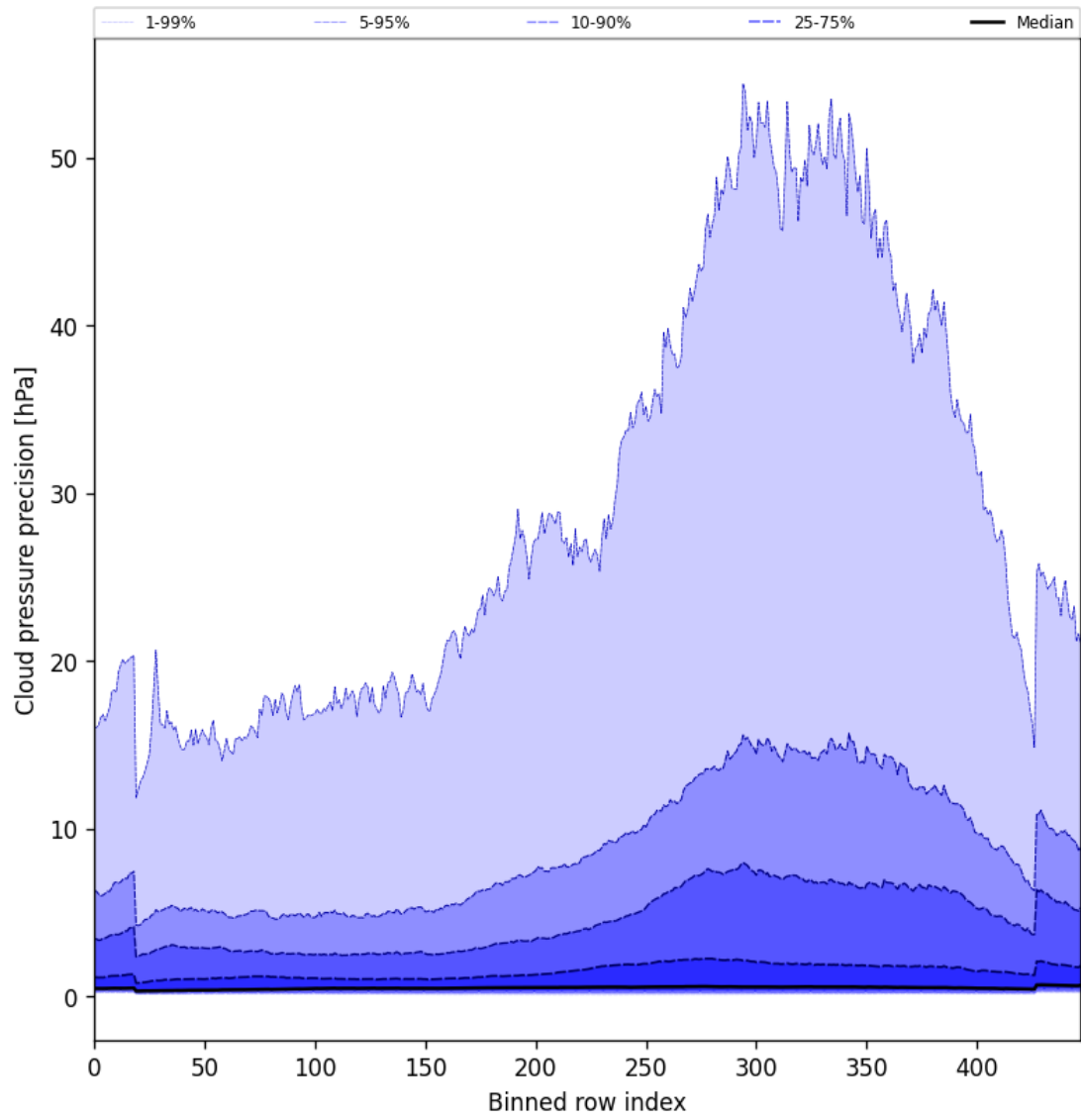
Figure 46: Along track statistics of “Cloud pressure precision” for 2025-01-11 to 2025-01-12
