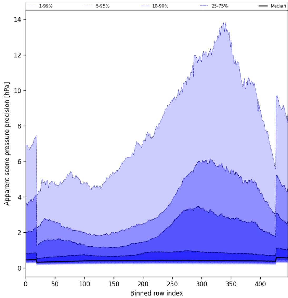
Figure 52: Along track statistics of “Apparent scene pressure precision” for 2025-01-11 to 2025-01-12
