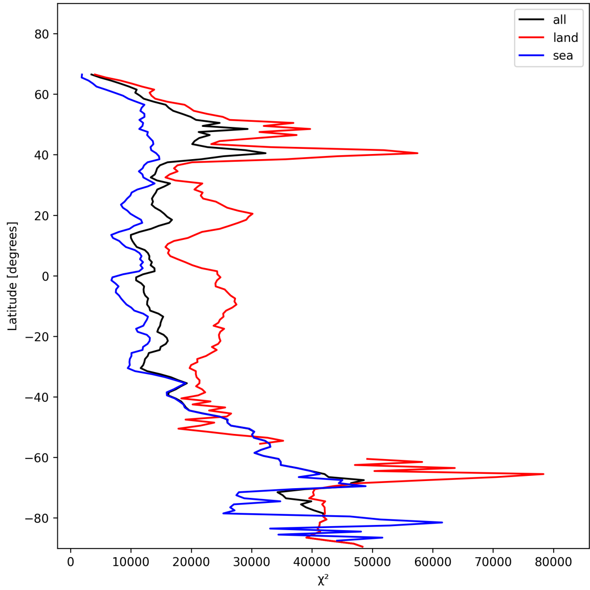
Figure 19: Zonal average of “ \chi^2 ” for 2025-01-11 to 2025-01-12.
