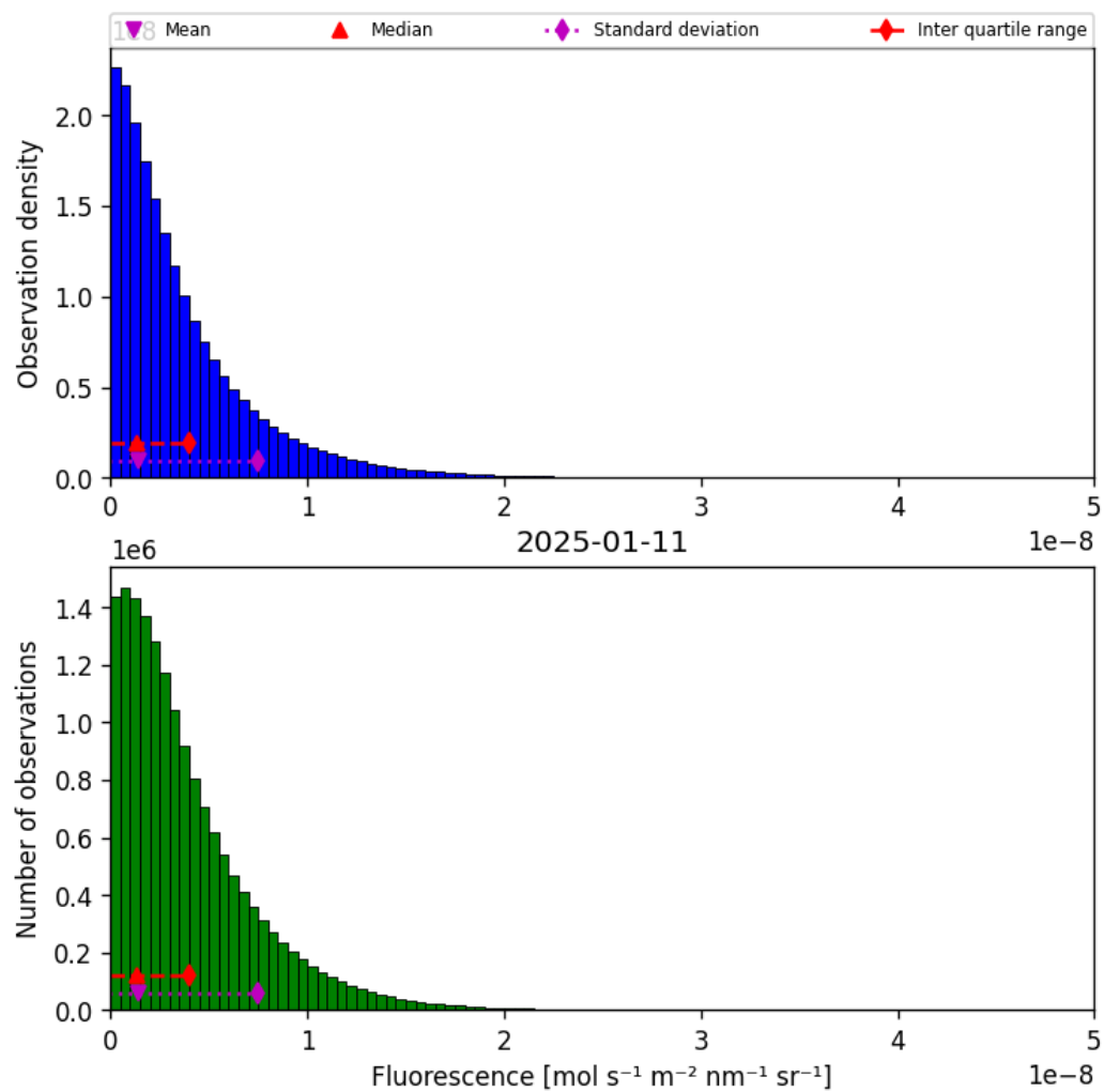
Figure 38: Histogram of “Fluorescence” for 2025-01-11 to 2025-01-12
