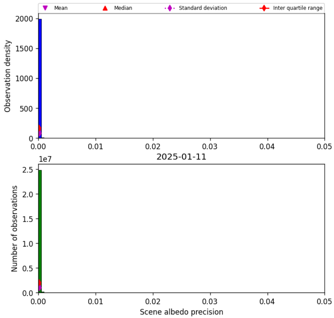
Figure 33: Histogram of “Scene albedo precision” for 2025-01-11 to 2025-01-12
