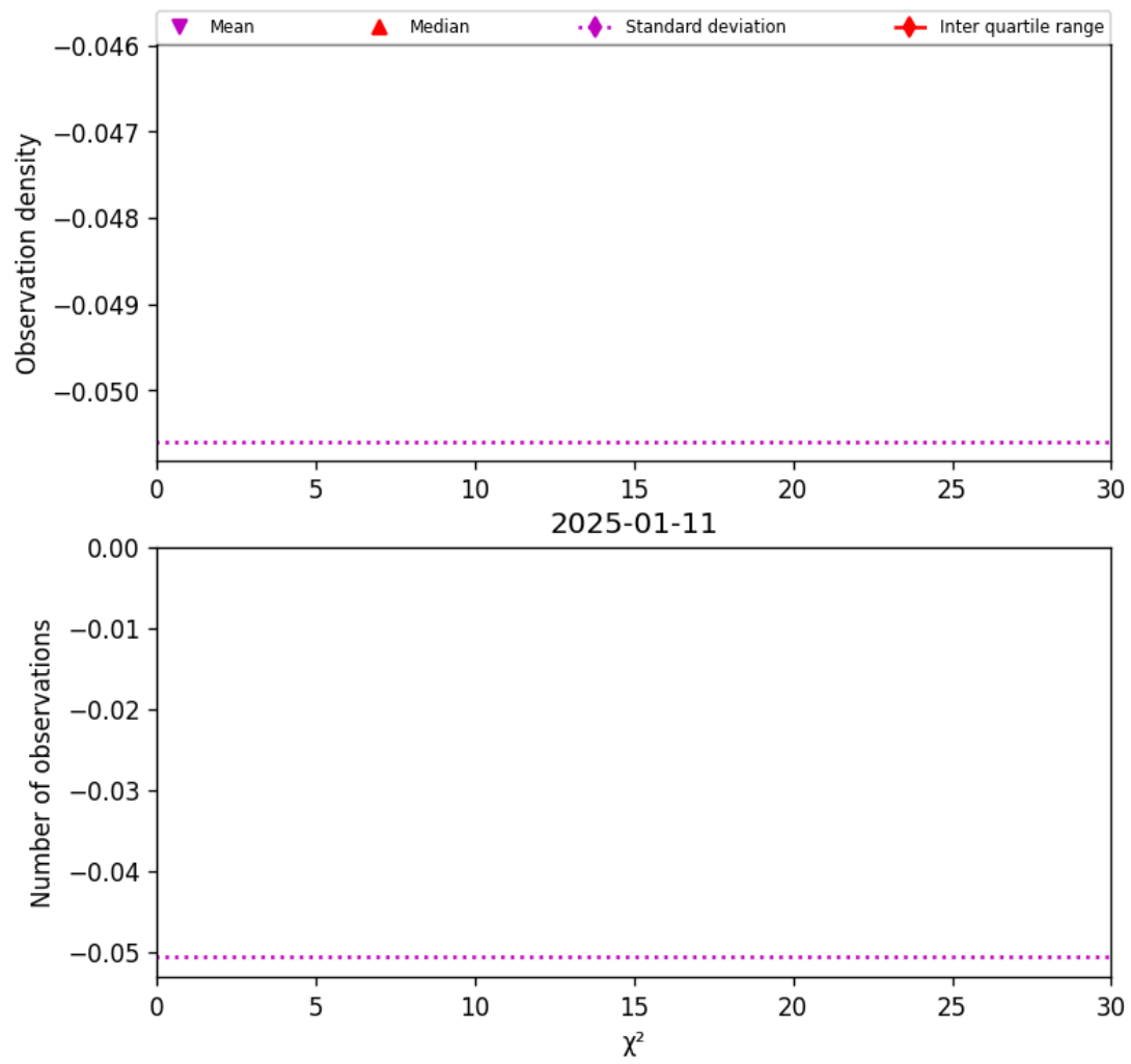
Figure 36: Histogram of " \chi^2 " for 2025-01-11 to 2025-01-12
