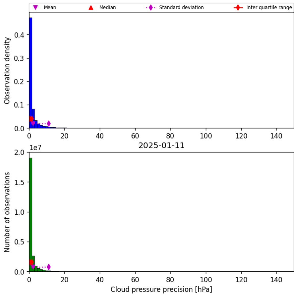
Figure 29: Histogram of “Cloud pressure precision” for 2025-01-11 to 2025-01-12
