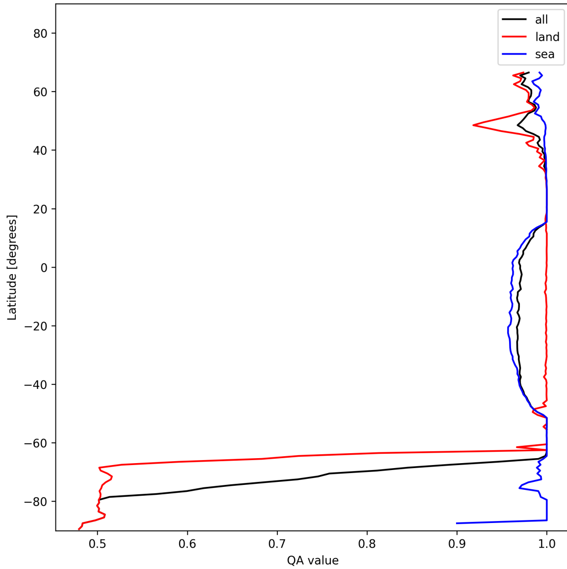
Figure 10: Zonal average of “QA value” for 2025-01-11 to 2025-01-12.
