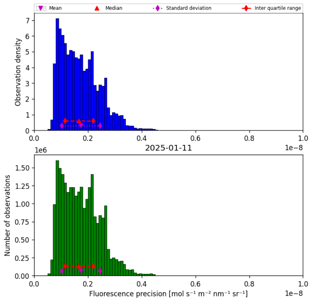
Figure 39: Histogram of “Fluorescence precision” for 2025-01-11 to 2025-01-12
