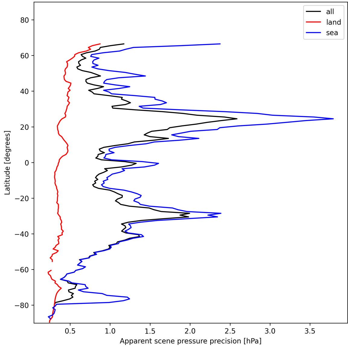
Figure 18: Zonal average of “Apparent scene pressure precision” for 2025-01-11 to 2025-01-12.
