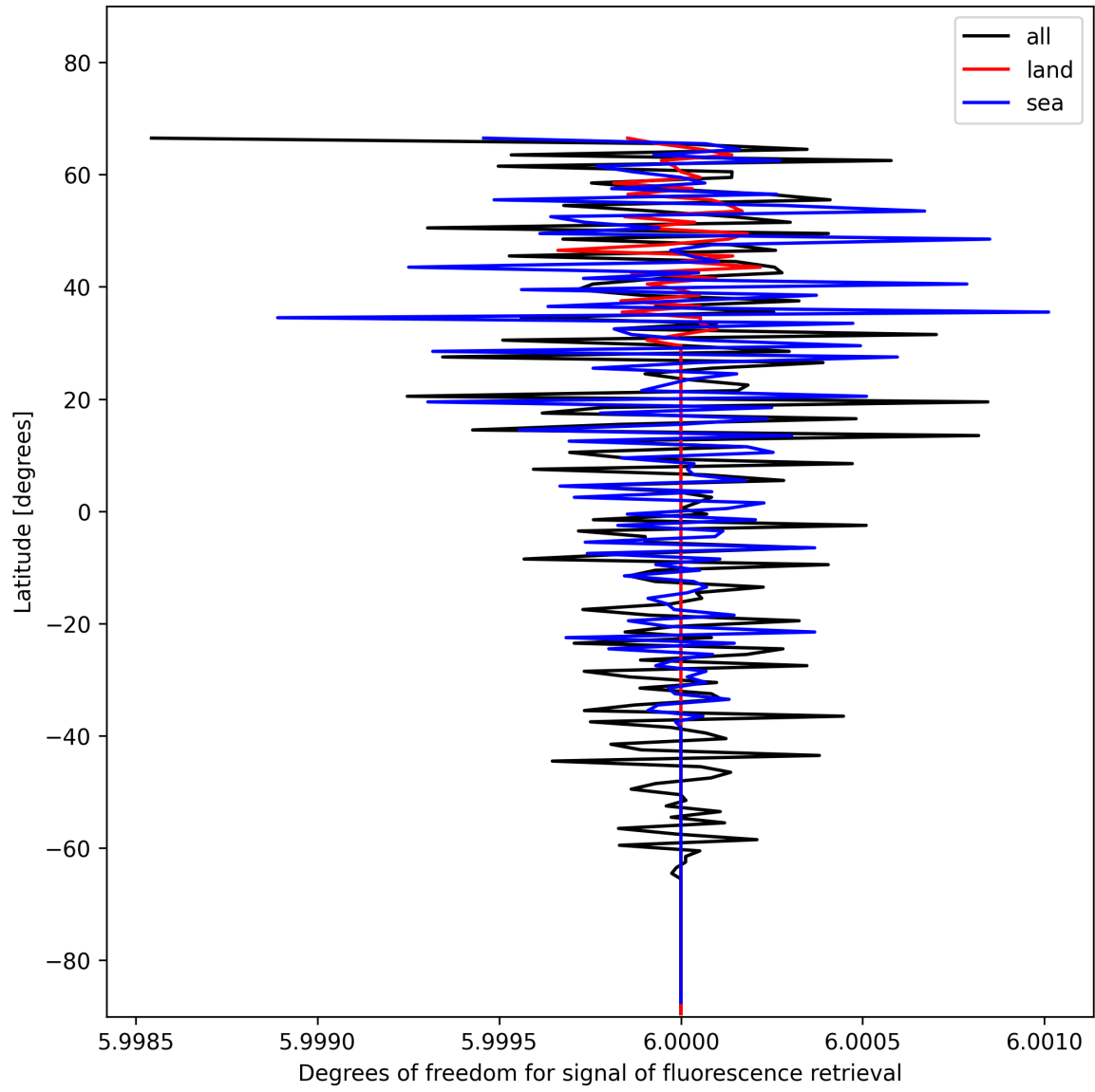
Figure 24: Zonal average of “Degrees of freedom for signal of fluorescence retrieval” for 2025-01-11 to 2025-01-12.
