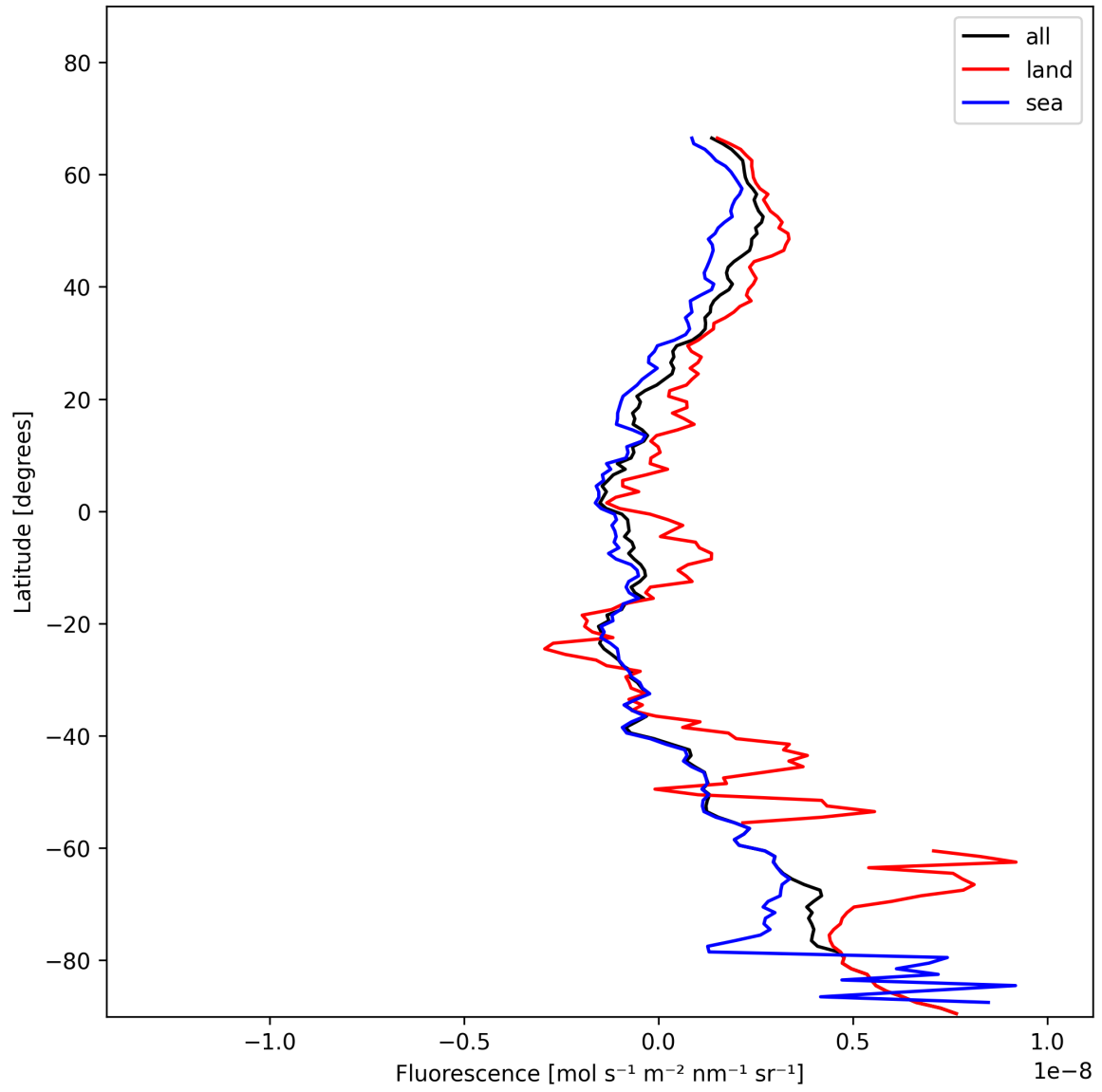
Figure 21: Zonal average of “Fluorescence” for 2025-01-11 to 2025-01-12.
