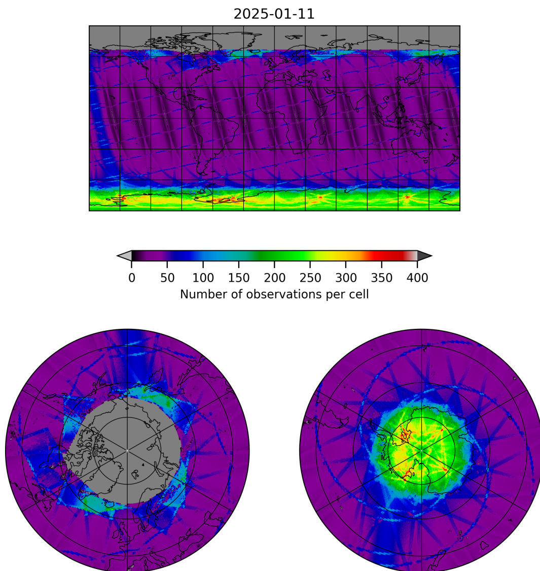
Figure 9: Map of the number of observations for 2025-01-11 to 2025-01-12
