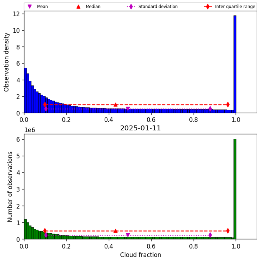
Figure 30: Histogram of “Cloud fraction” for 2025-01-11 to 2025-01-12
