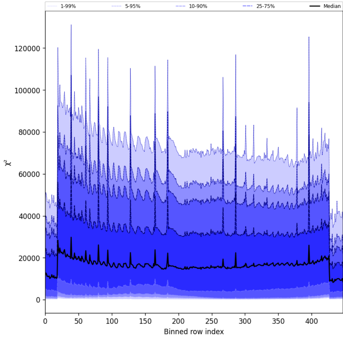
Figure 53: Along track statistics of “ \chi^2 ” for 2025-01-11 to 2025-01-12
