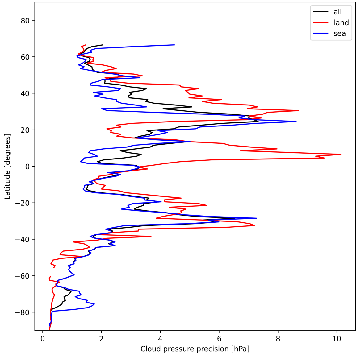
Figure 12: Zonal average of “Cloud pressure precision” for 2025-01-11 to 2025-01-12.
