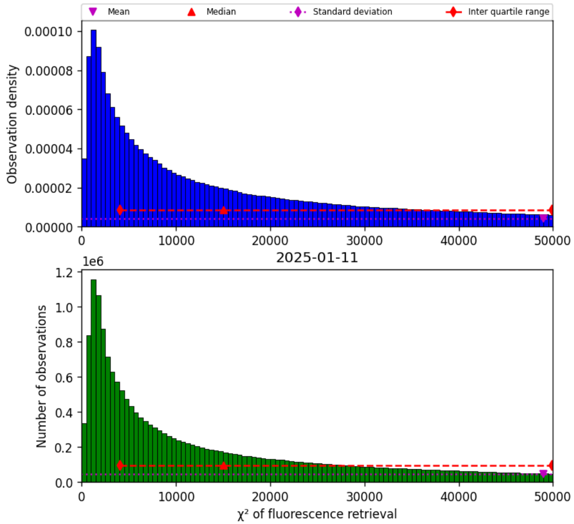
Figure 40: Histogram of “ \chi^2 of fluorescence retrieval” for 2025-01-11 to 2025-01-12
