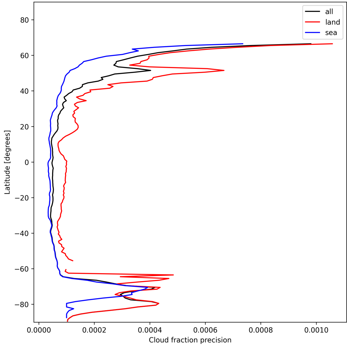
Figure 14: Zonal average of “Cloud fraction precision” for 2025-01-11 to 2025-01-12.
