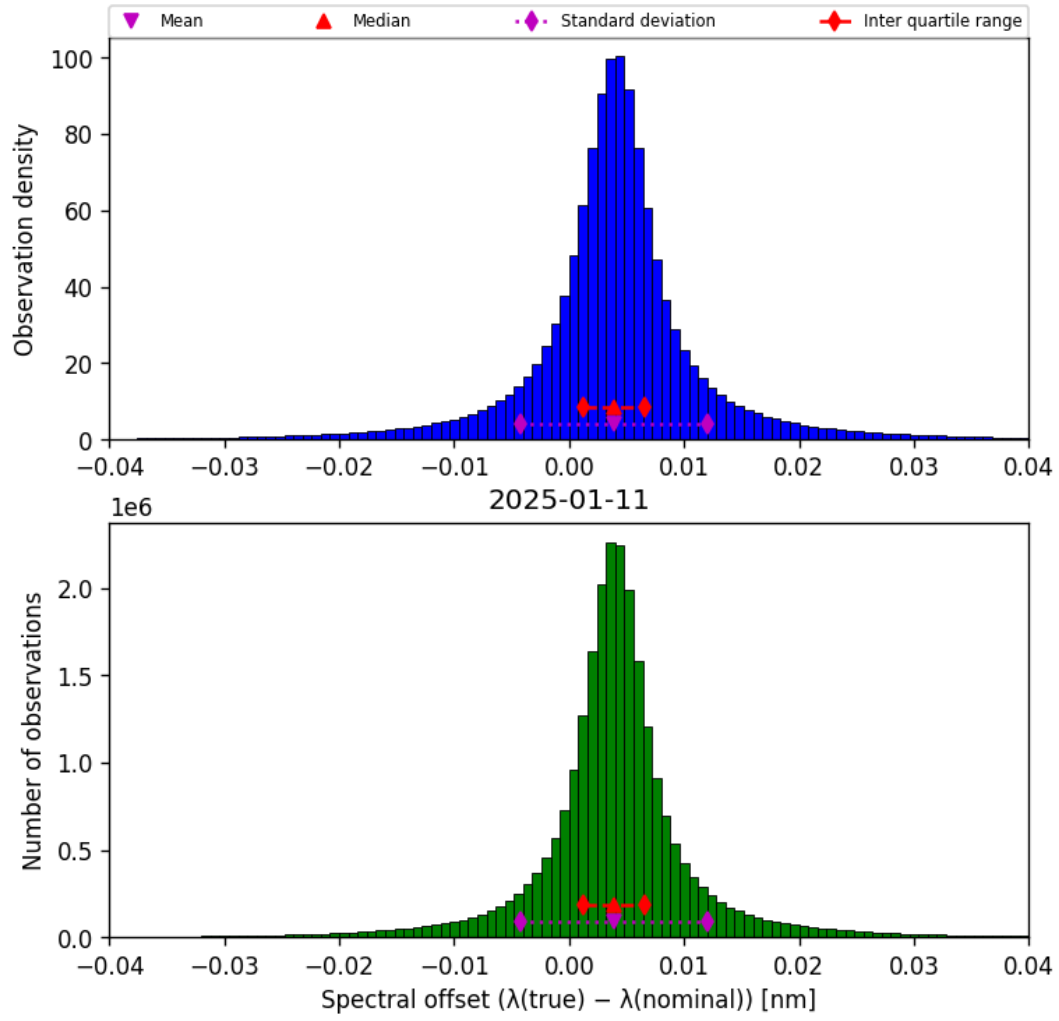
Figure 43: Histogram of “Spectral offset ( \lambda_{\text{true}} - \lambda_{\text{nominal}} )” for 2025-01-11 to 2025-01-12
