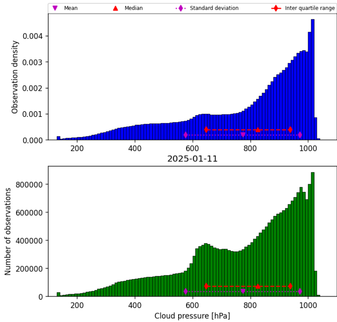
Figure 28: Histogram of “Cloud pressure” for 2025-01-11 to 2025-01-12
