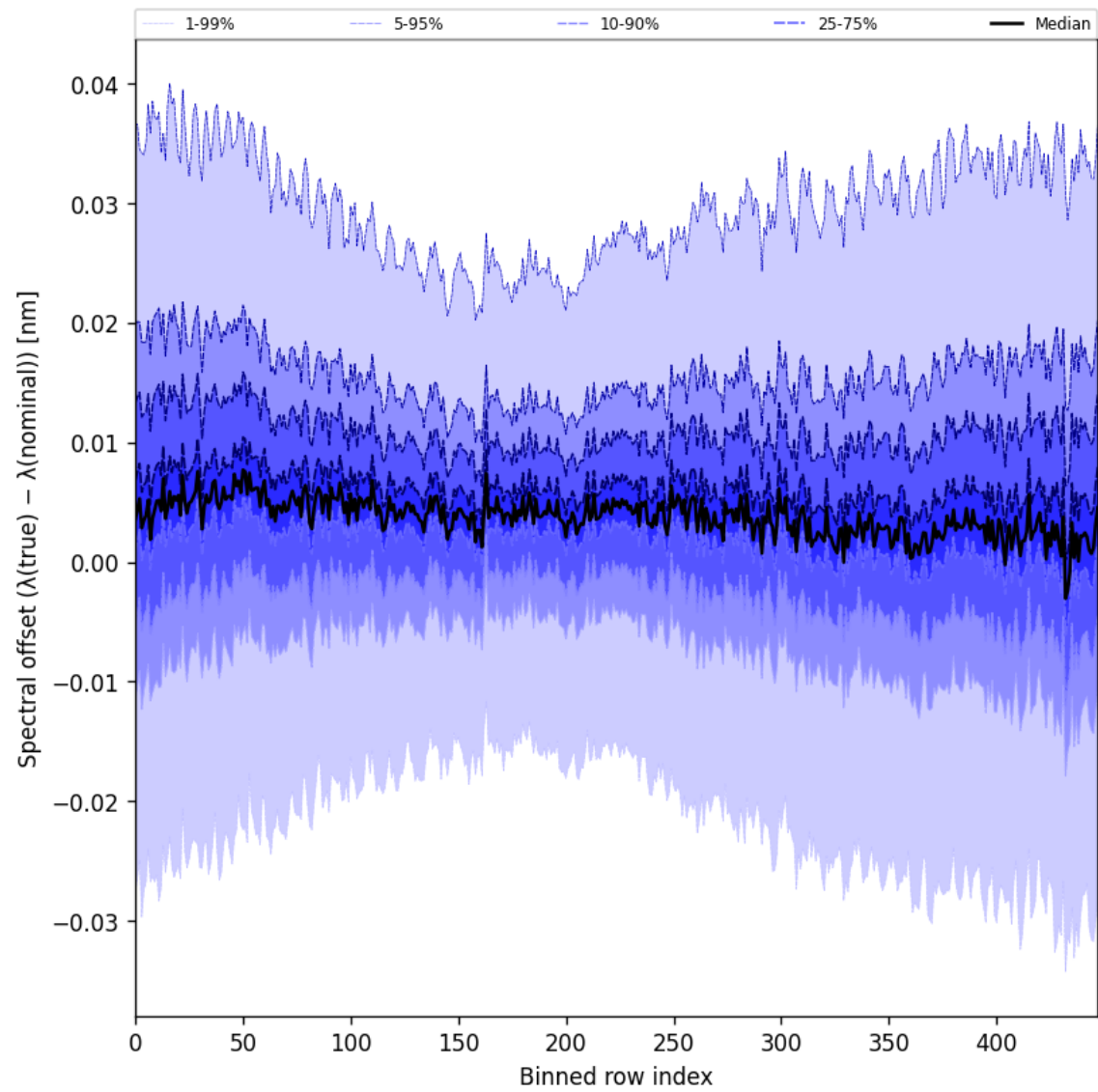
Figure 60: Along track statistics of “Spectral offset ( \lambda_{\text{true}} - \lambda_{\text{nominal}} )” for 2025-01-11 to 2025-01-12
