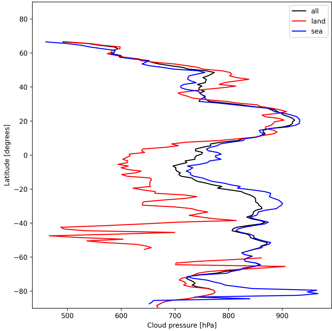
Figure 11: Zonal average of “Cloud pressure” for 2025-01-11 to 2025-01-12.
