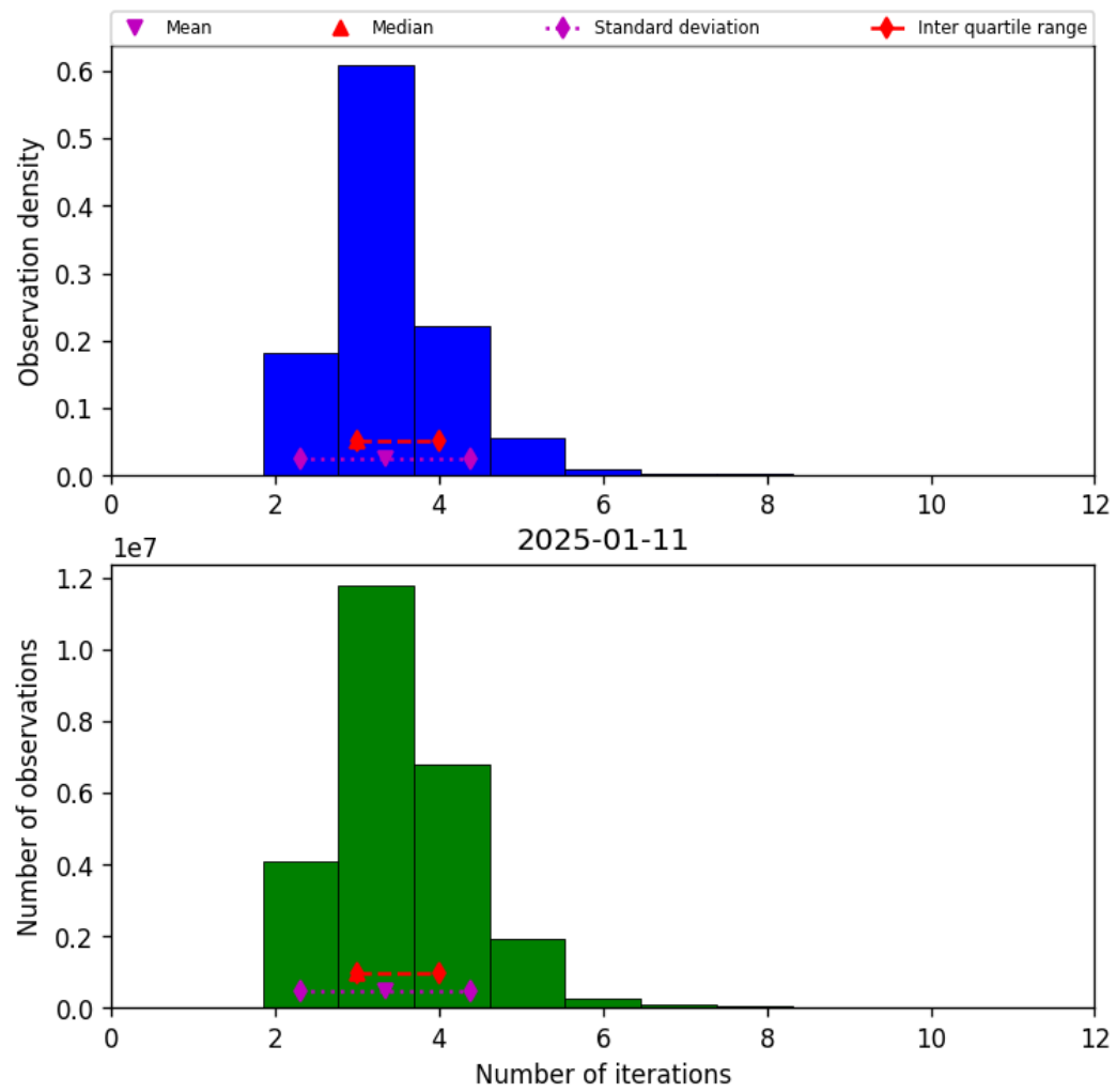
Figure 37: Histogram of “Number of iterations” for 2025-01-11 to 2025-01-12
