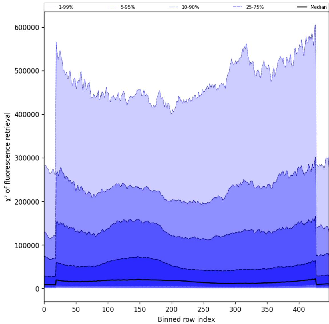
Figure 57: Along track statistics of “ \chi^2 of fluorescence retrieval” for 2025-01-11 to 2025-01-12
