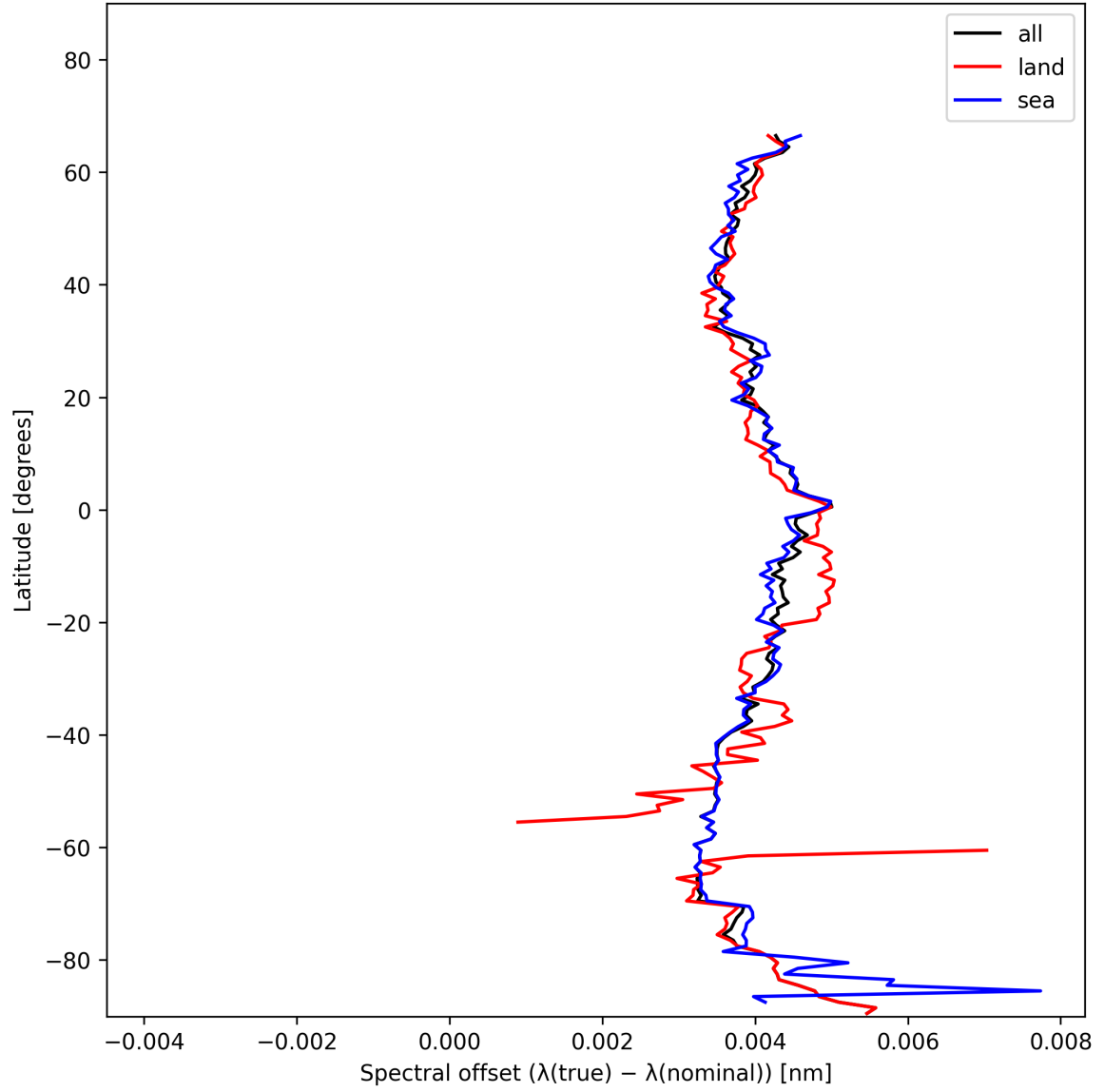
Figure 26: Zonal average of “Spectral offset ( \lambda_{\text{true}} - \lambda_{\text{nominal}} )” for 2025-01-11 to 2025-01-12.
