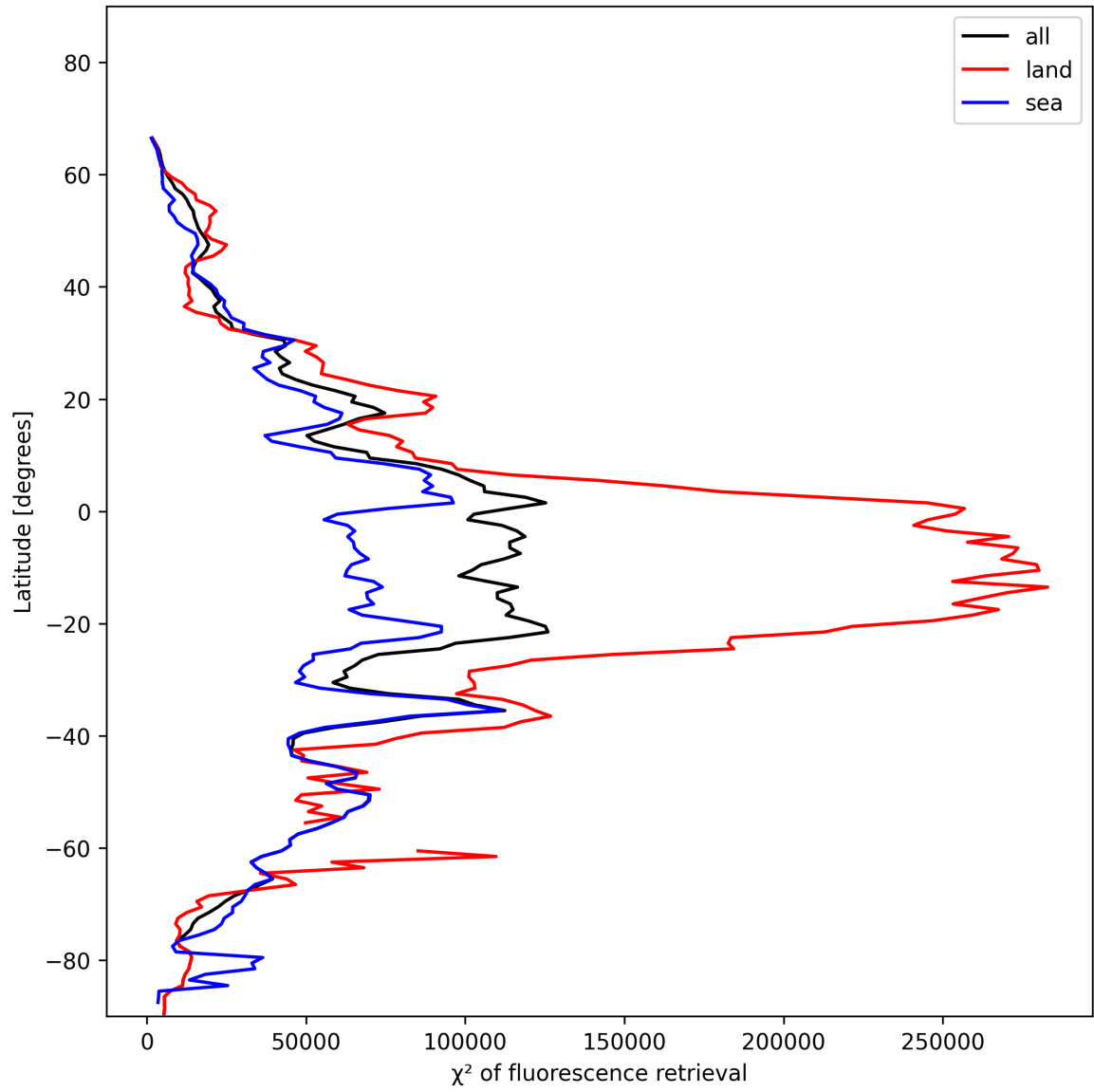
Figure 23: Zonal average of “ \chi^2 of fluorescence retrieval” for 2025-01-11 to 2025-01-12.
