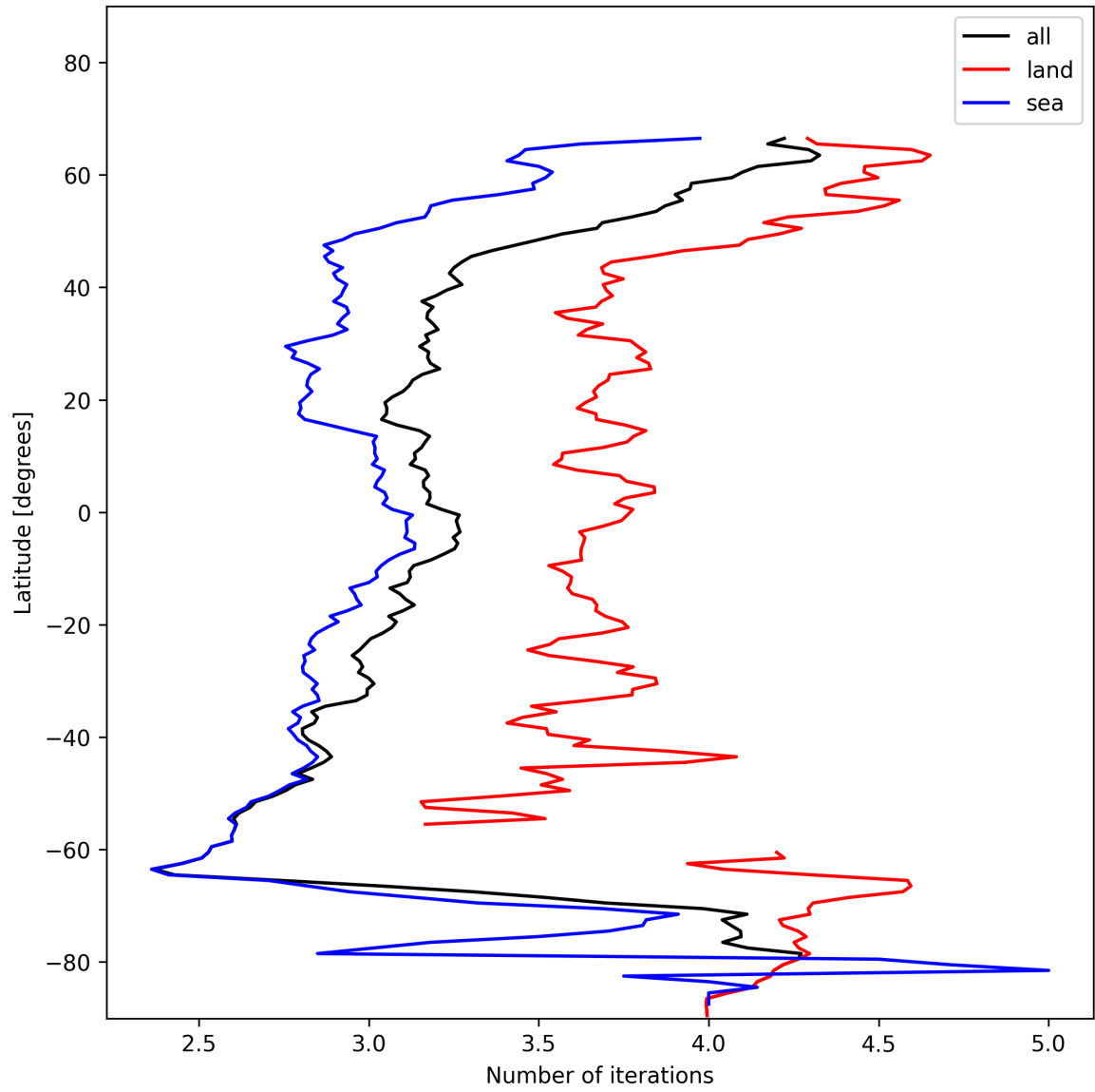
Figure 20: Zonal average of “Number of iterations” for 2025-01-11 to 2025-01-12.
