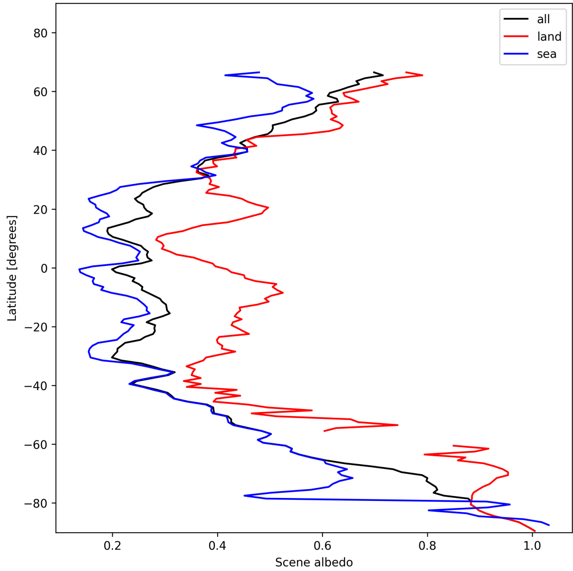
Figure 15: Zonal average of “Scene albedo” for 2025-01-11 to 2025-01-12.
