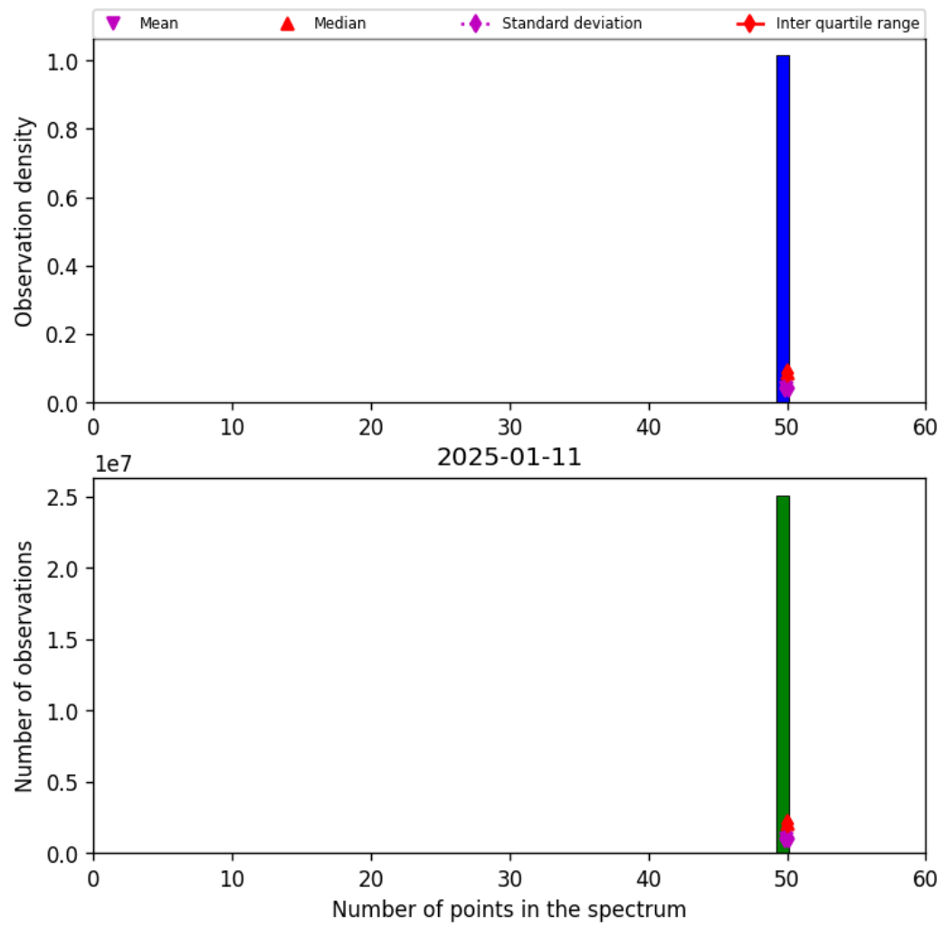
Figure 42: Histogram of “Number of points in the spectrum” for 2025-01-11 to 2025-01-12
