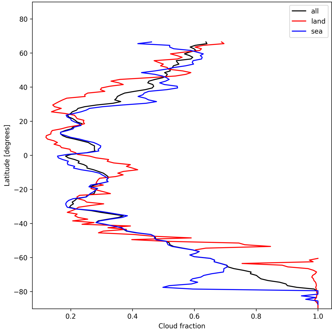
Figure 13: Zonal average of “Cloud fraction” for 2025-01-11 to 2025-01-12.
