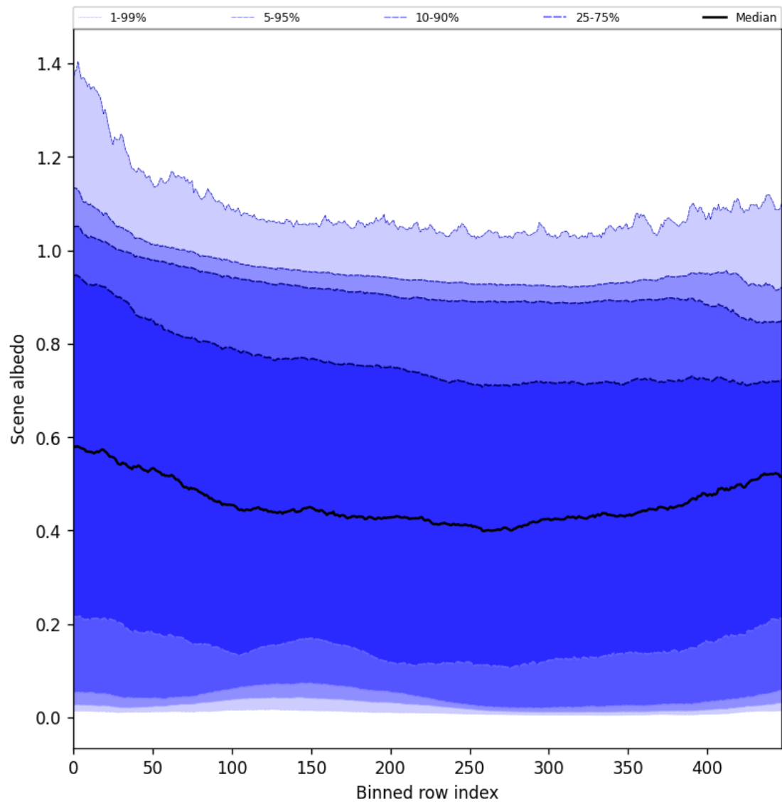
Figure 49: Along track statistics of “Scene albedo” for 2025-01-11 to 2025-01-12
