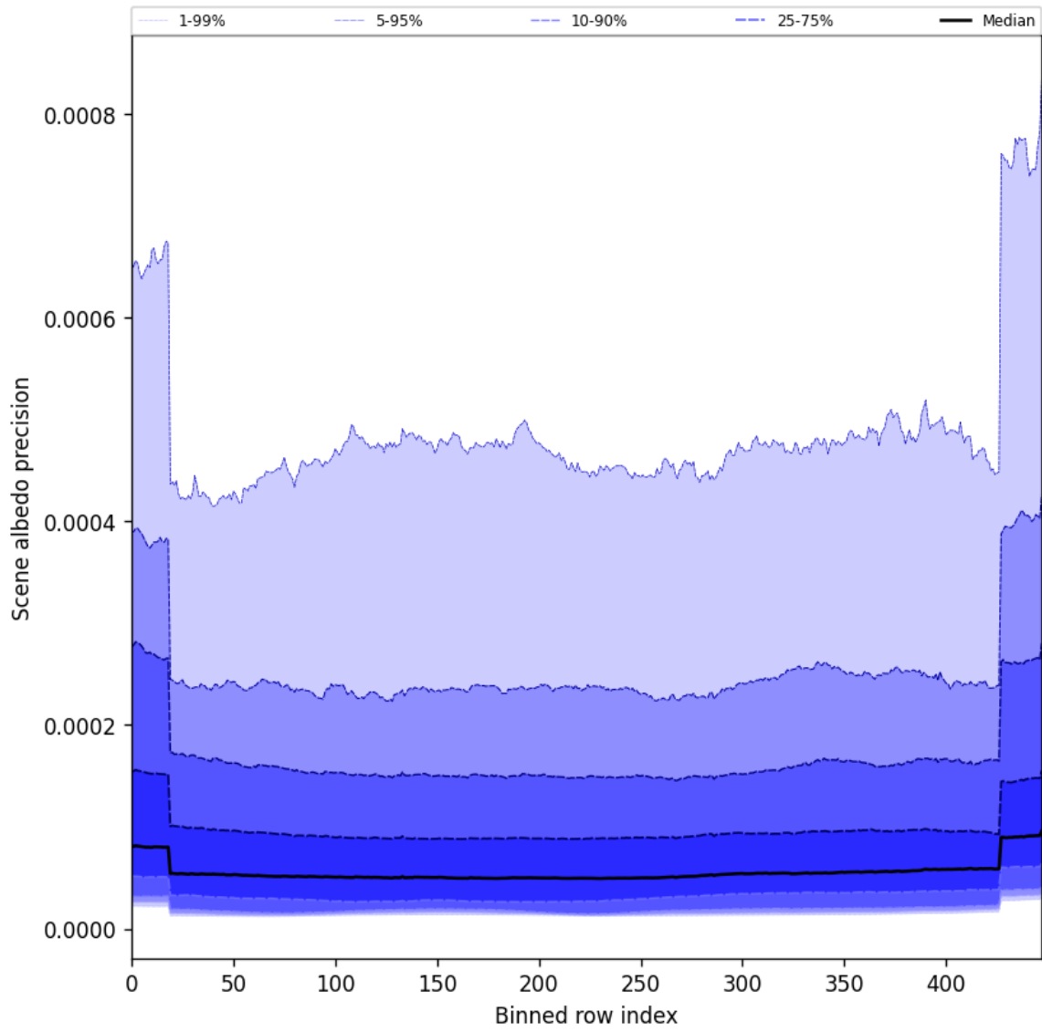
Figure 50: Along track statistics of “Scene albedo precision” for 2025-01-11 to 2025-01-12
