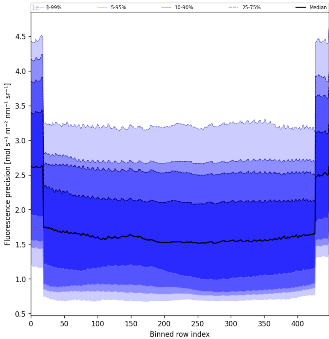
Figure 56: Along track statistics of “Fluorescence precision” for 2025-01-11 to 2025-01-12
