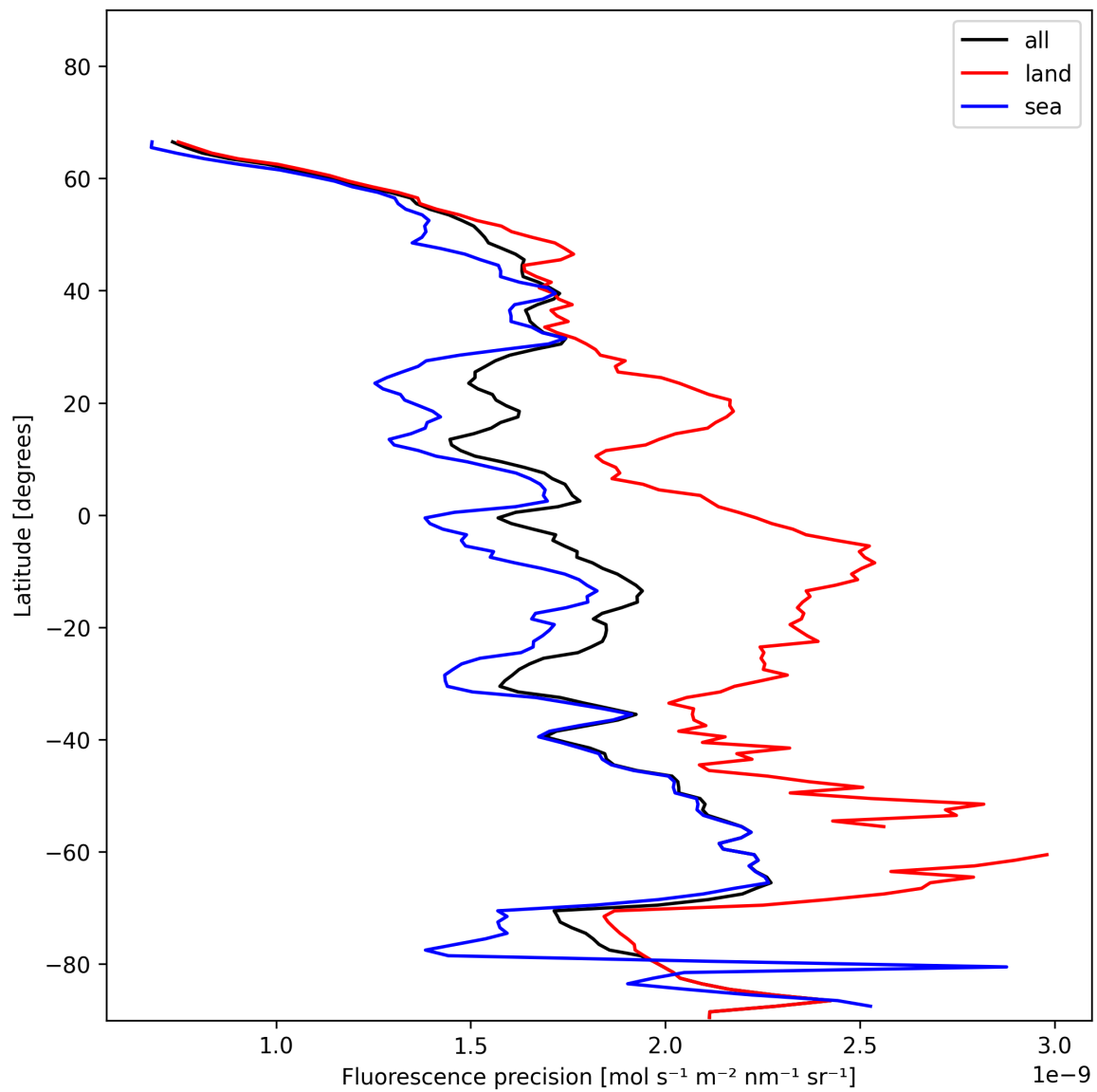
Figure 22: Zonal average of “Fluorescence precision” for 2025-01-11 to 2025-01-12.
