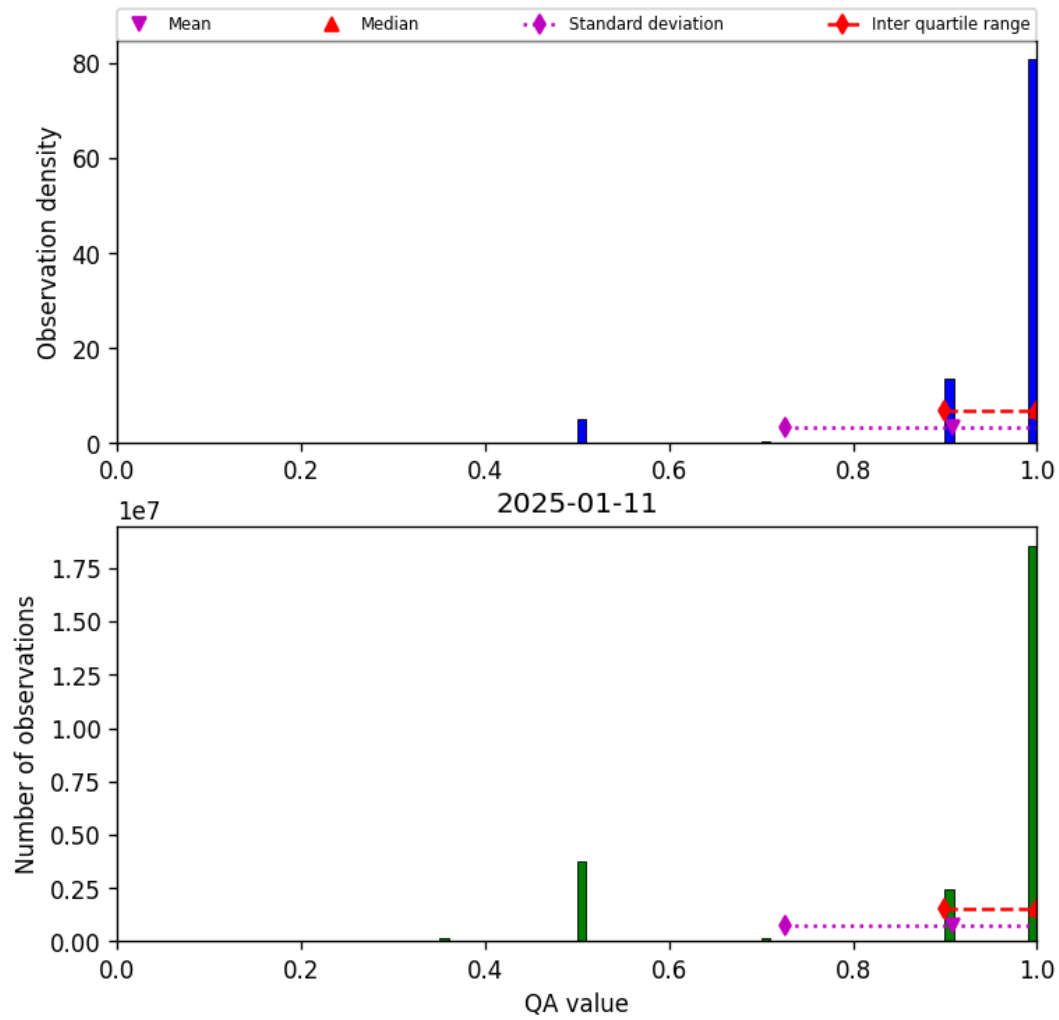
Figure 27: Histogram of “QA value” for 2025-01-11 to 2025-01-12
