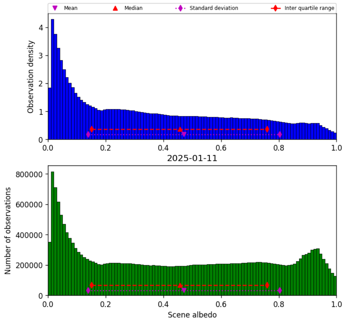
Figure 32: Histogram of “Scene albedo” for 2025-01-11 to 2025-01-12
