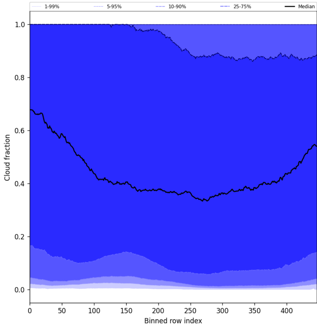
Figure 47: Along track statistics of “Cloud fraction” for 2025-01-11 to 2025-01-12
