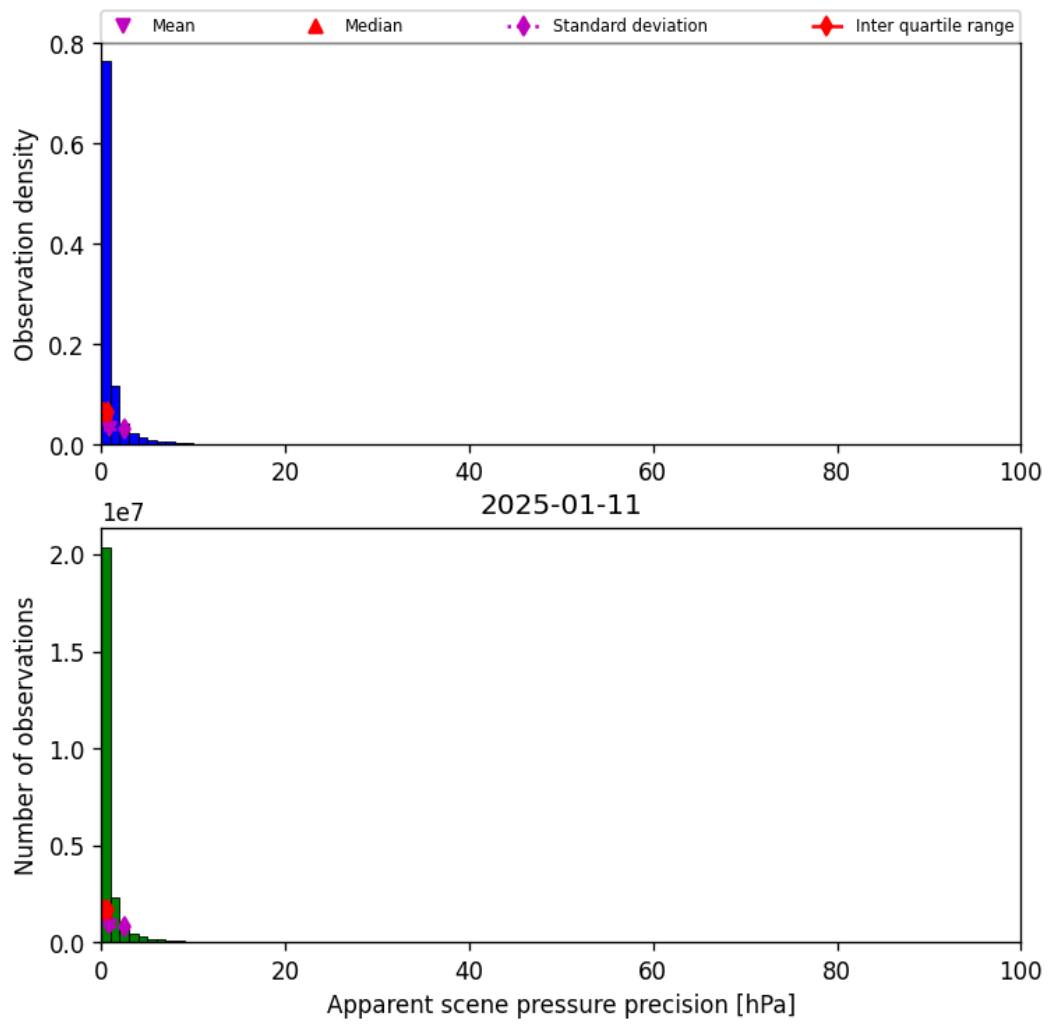
Figure 35: Histogram of “Apparent scene pressure precision” for 2025-01-11 to 2025-01-12
