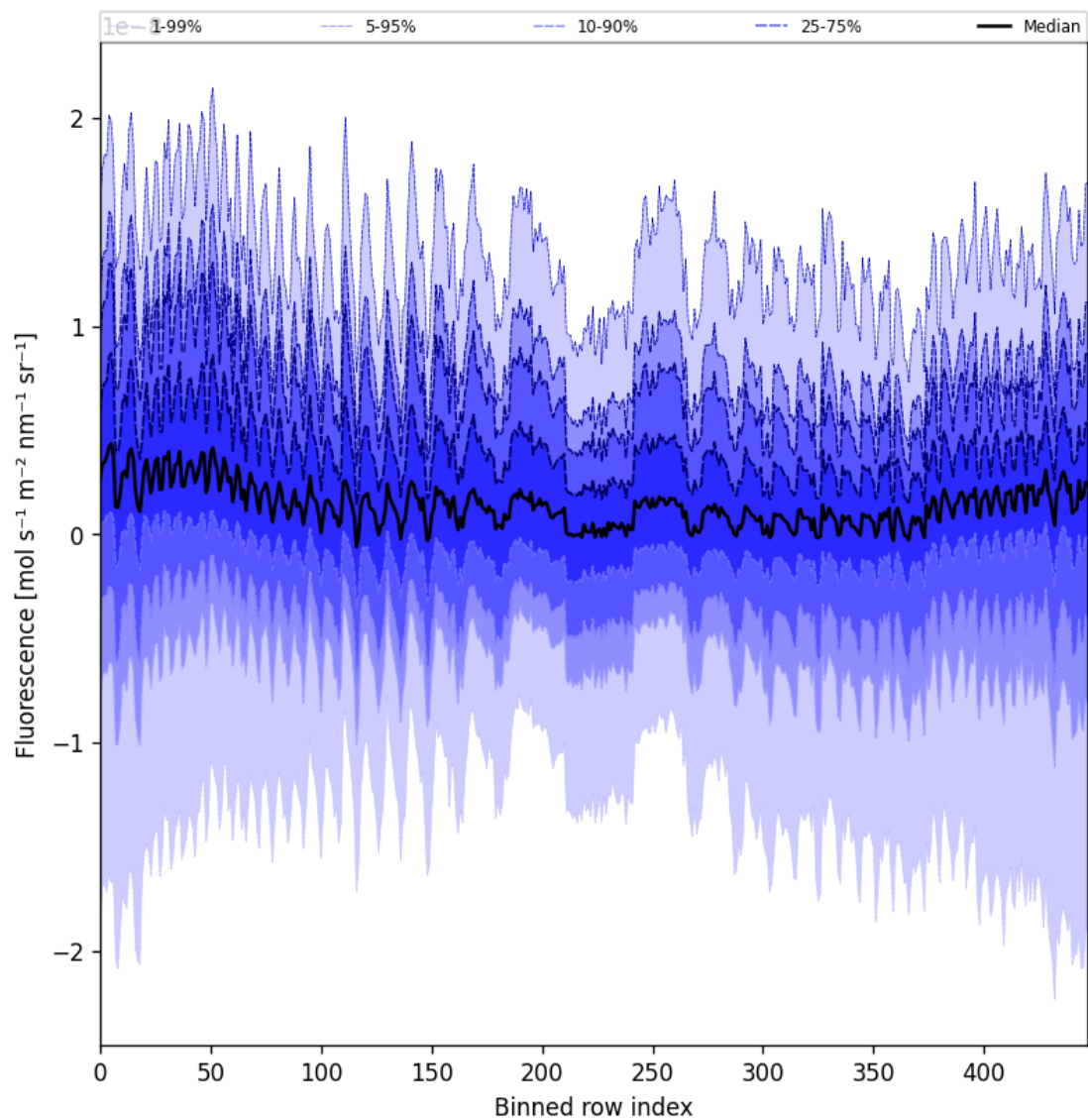
Figure 55: Along track statistics of “Fluorescence” for 2025-01-11 to 2025-01-12
