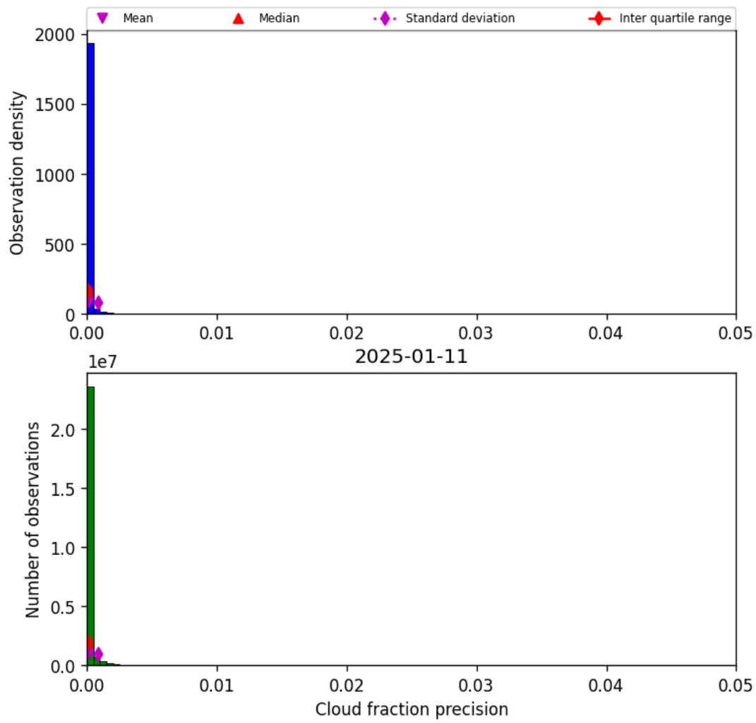
Figure 31: Histogram of “Cloud fraction precision” for 2025-01-11 to 2025-01-12
