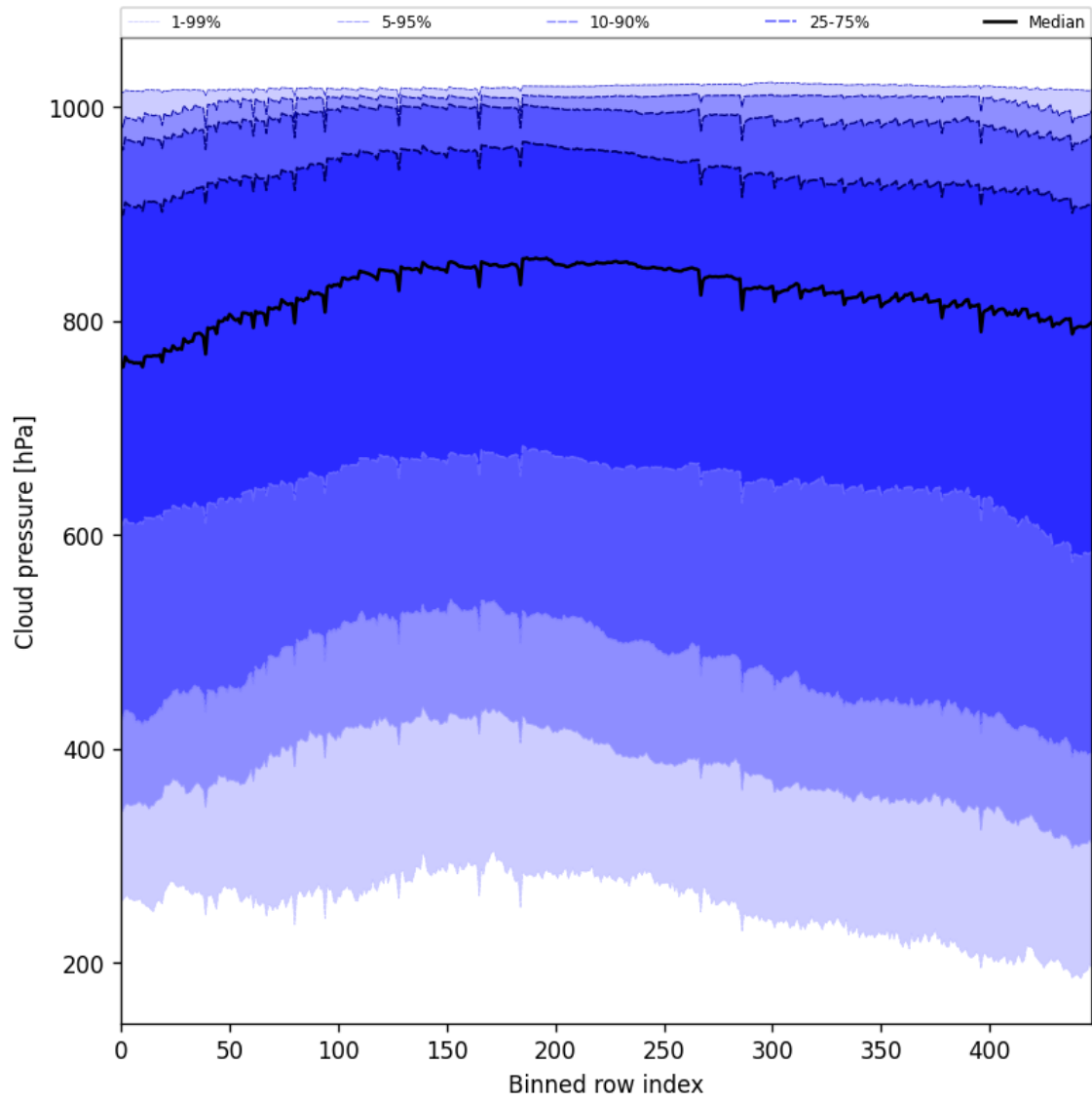
Figure 45: Along track statistics of “Cloud pressure” for 2025-01-11 to 2025-01-12
