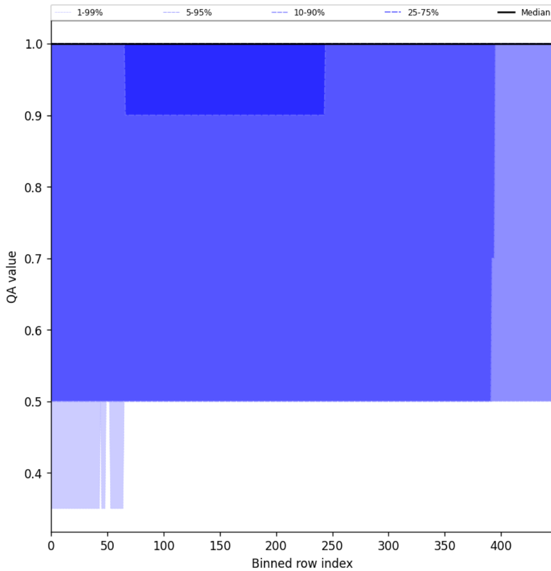
Figure 44: Along track statistics of “QA value” for 2025-01-11 to 2025-01-12
