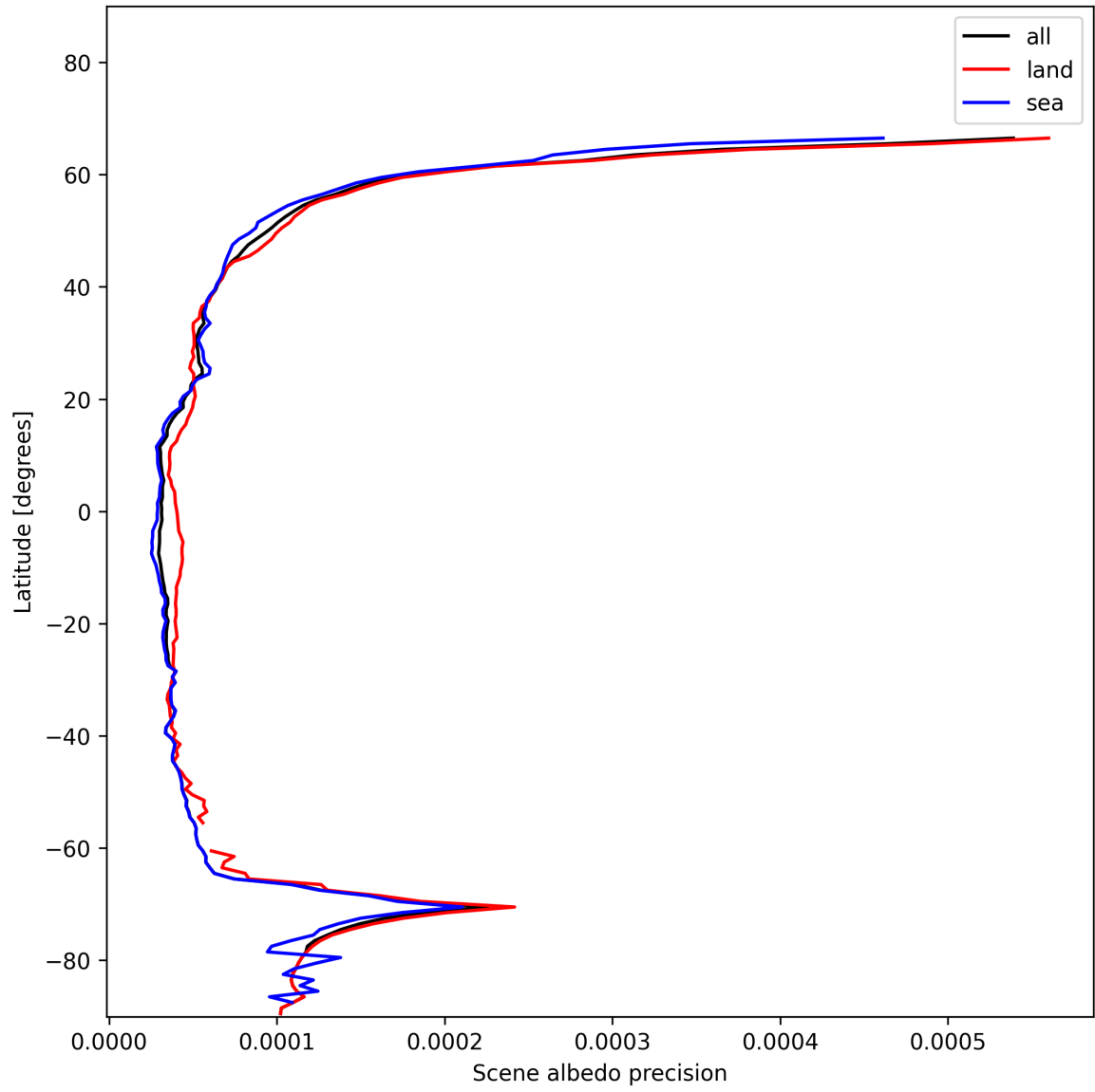
Figure 16: Zonal average of “Scene albedo precision” for 2025-01-11 to 2025-01-12.
