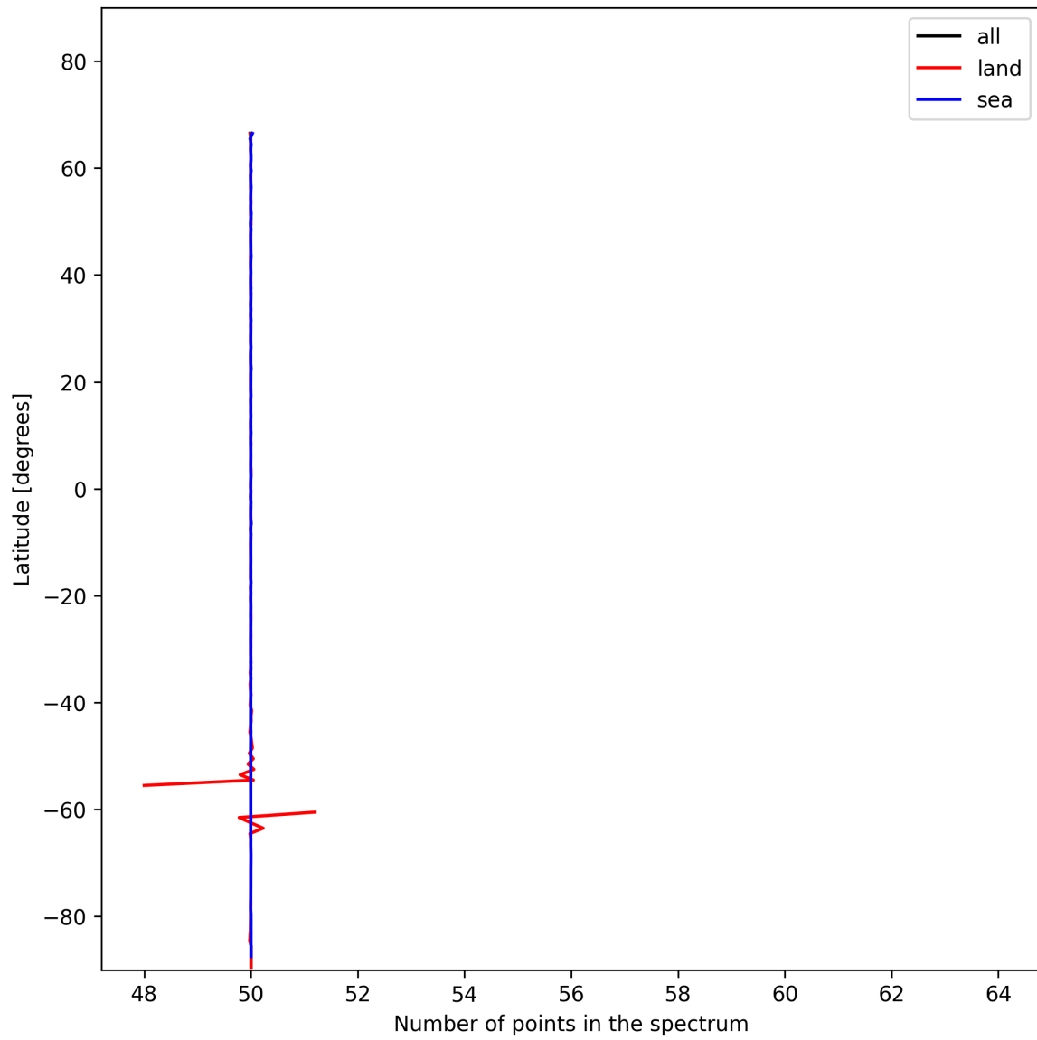
Figure 25: Zonal average of “Number of points in the spectrum” for 2025-01-11 to 2025-01-12.
