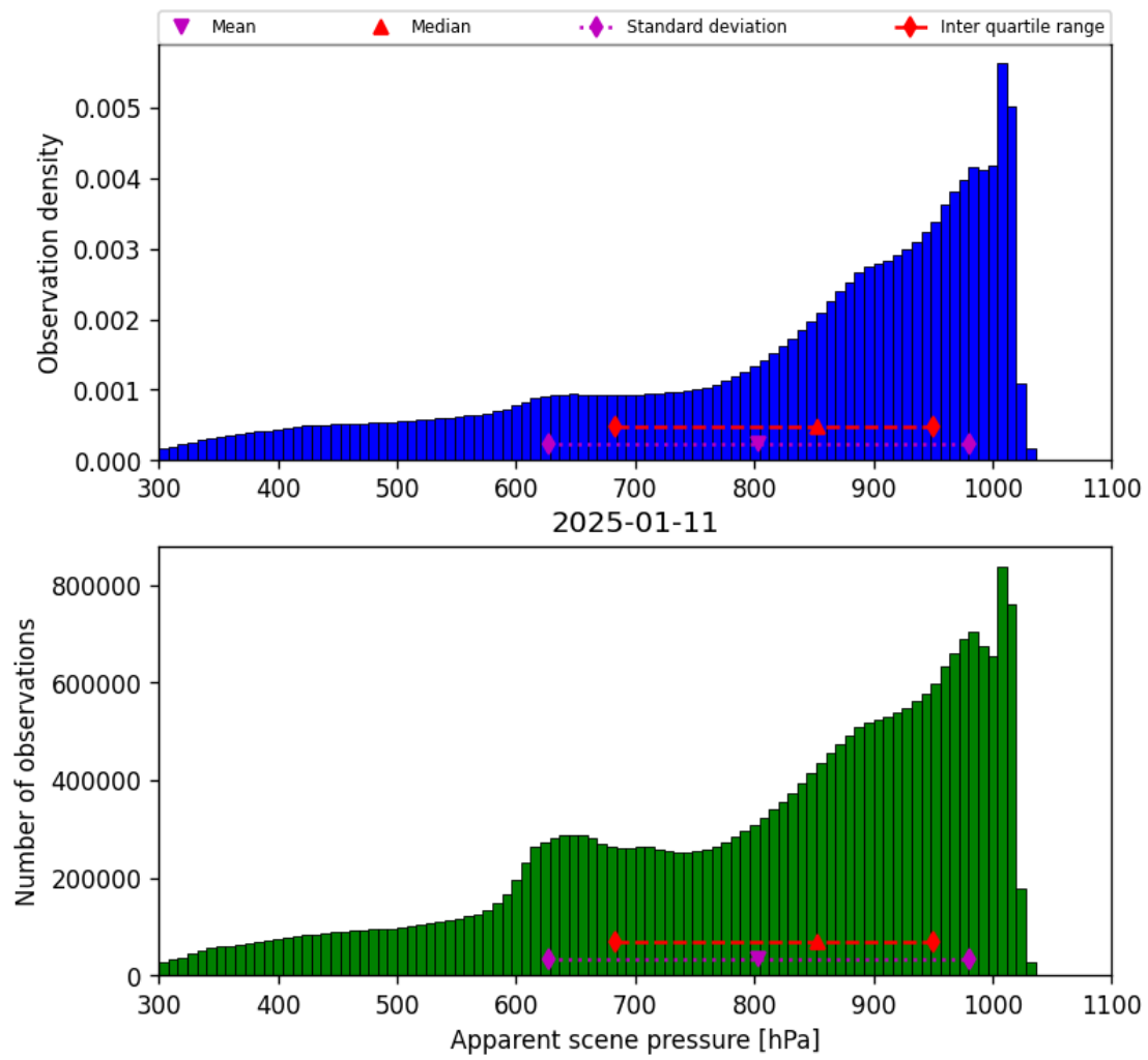
Figure 34: Histogram of “Apparent scene pressure” for 2025-01-11 to 2025-01-12
