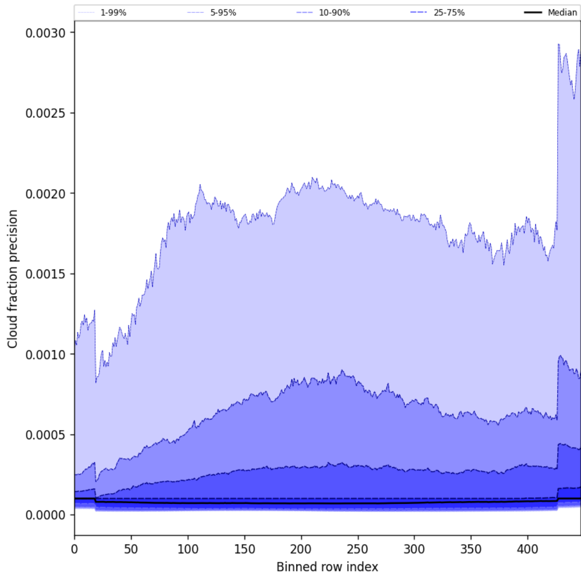
Figure 48: Along track statistics of “Cloud fraction precision” for 2025-01-11 to 2025-01-12
