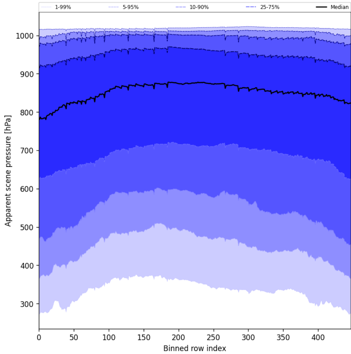
Figure 51: Along track statistics of “Apparent scene pressure” for 2025-01-11 to 2025-01-12
