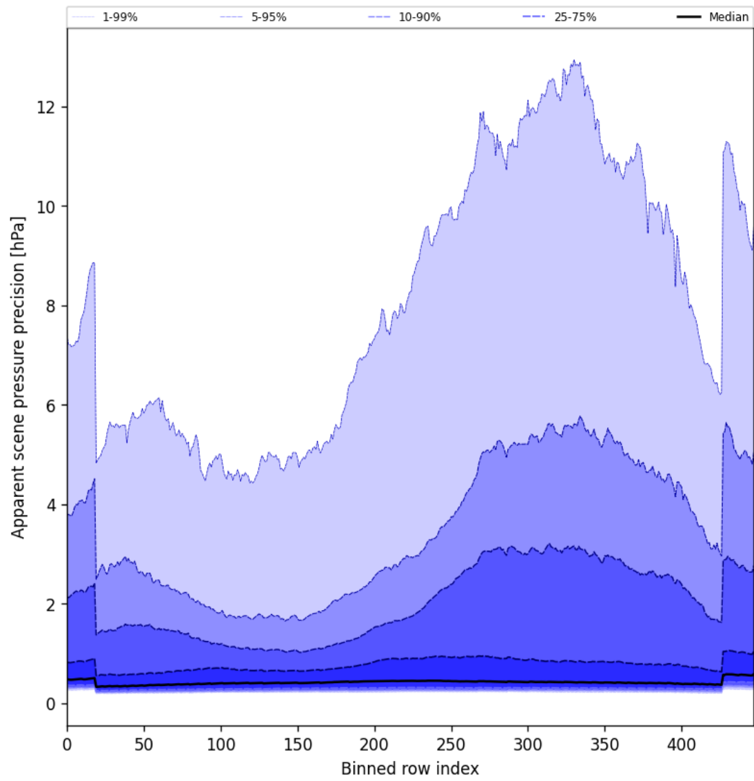
Figure 52: Along track statistics of “Apparent scene pressure precision” for 2025-01-14 to 2025-01-15
