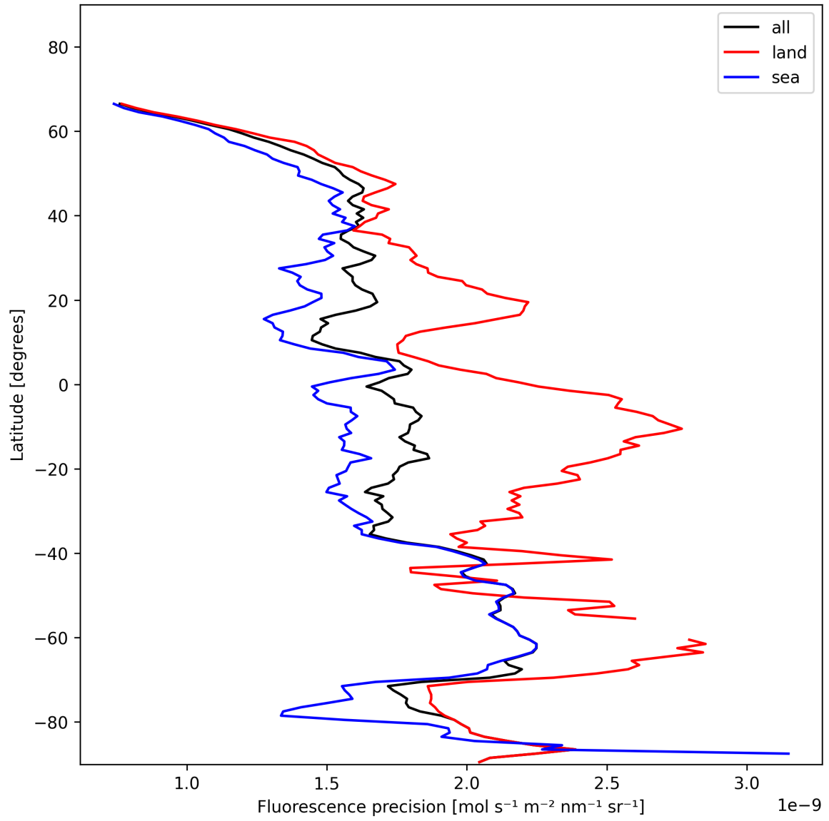
Figure 22: Zonal average of “Fluorescence precision” for 2025-01-14 to 2025-01-15.
