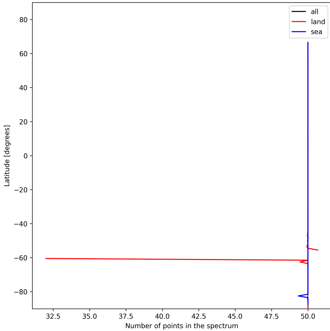
Figure 25: Zonal average of “Number of points in the spectrum” for 2025-01-14 to 2025-01-15.
