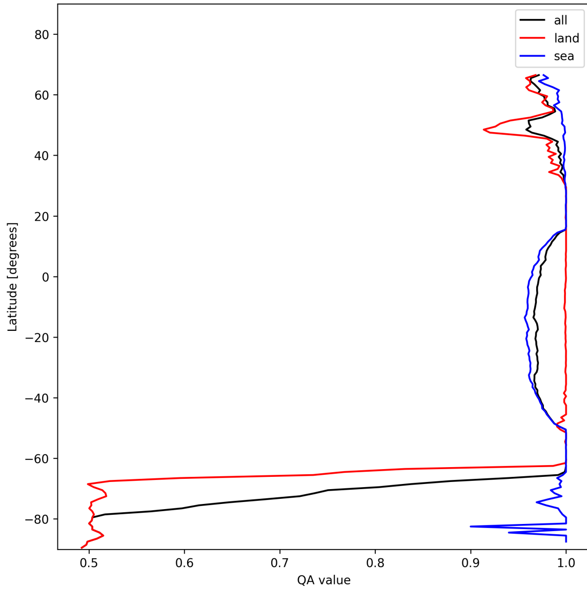
Figure 10: Zonal average of “QA value” for 2025-01-14 to 2025-01-15.
