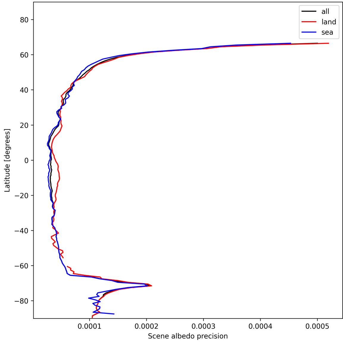
Figure 16: Zonal average of “Scene albedo precision” for 2025-01-14 to 2025-01-15.
