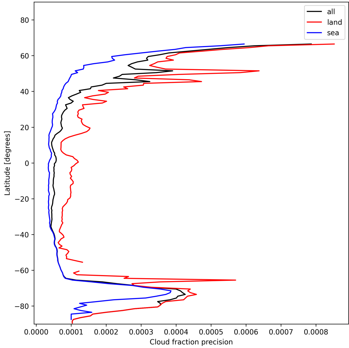
Figure 14: Zonal average of “Cloud fraction precision” for 2025-01-14 to 2025-01-15.
