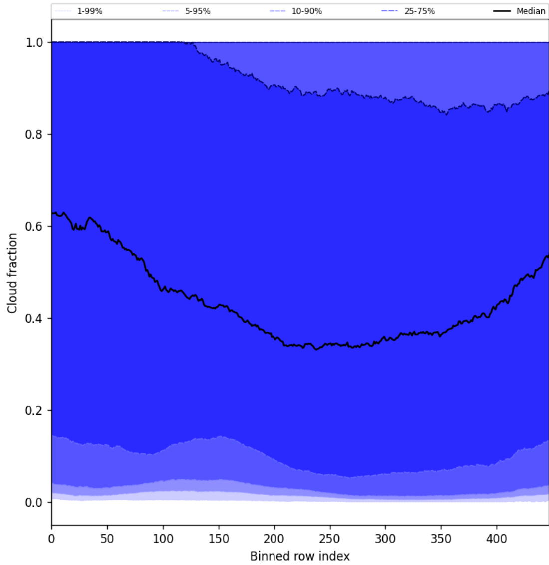
Figure 47: Along track statistics of “Cloud fraction” for 2025-01-14 to 2025-01-15
