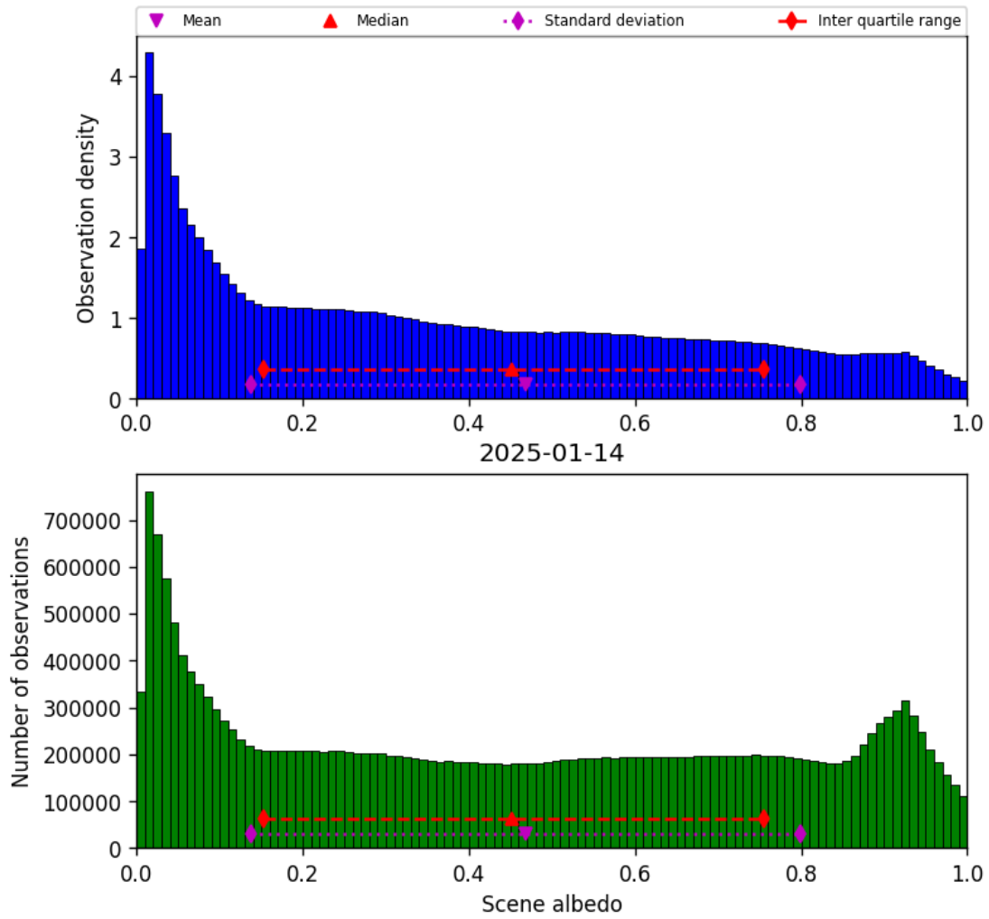
Figure 32: Histogram of “Scene albedo” for 2025-01-14 to 2025-01-15
