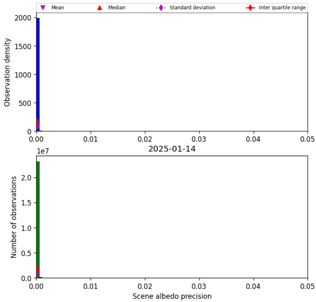
Figure 33: Histogram of “Scene albedo precision” for 2025-01-14 to 2025-01-15
