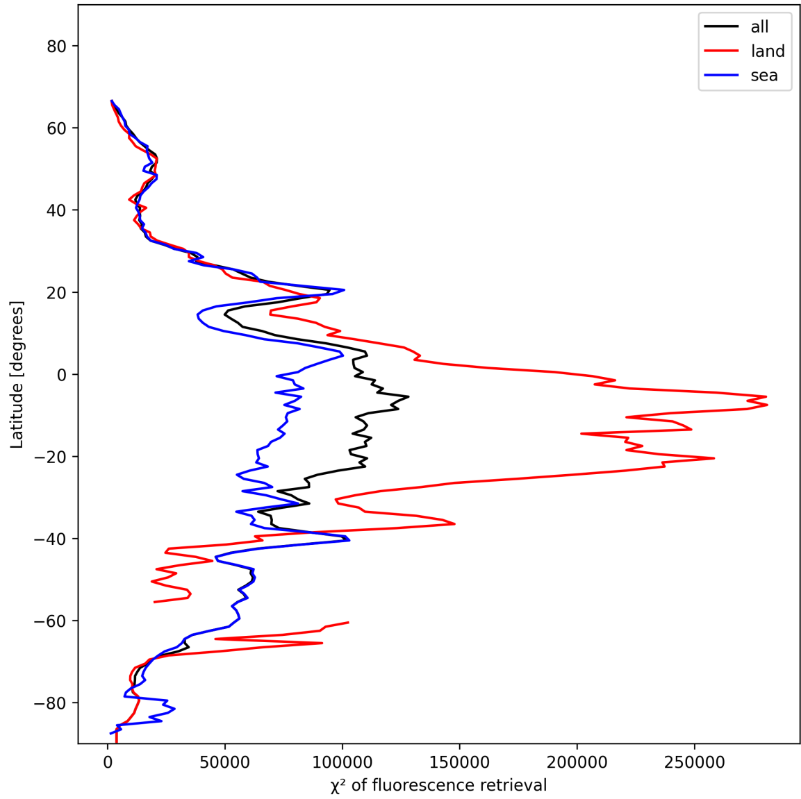
Figure 23: Zonal average of “ \chi^2 of fluorescence retrieval” for 2025-01-14 to 2025-01-15.
