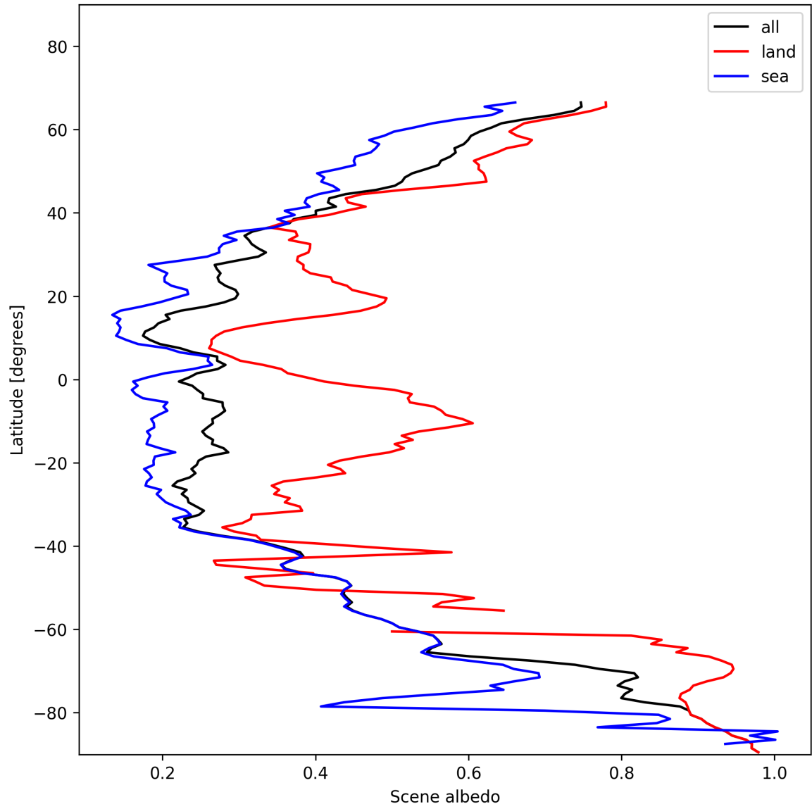
Figure 15: Zonal average of “Scene albedo” for 2025-01-14 to 2025-01-15.
