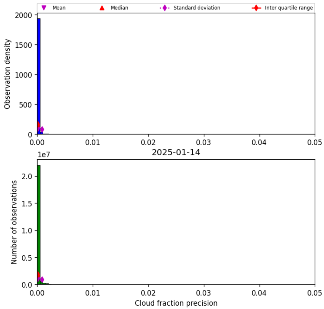
Figure 31: Histogram of “Cloud fraction precision” for 2025-01-14 to 2025-01-15
