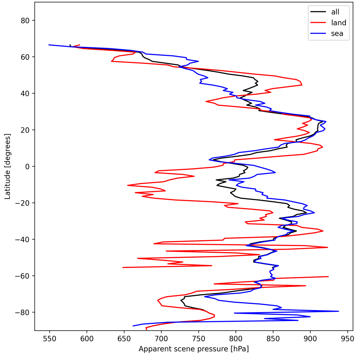
Figure 17: Zonal average of “Apparent scene pressure” for 2025-01-14 to 2025-01-15.
