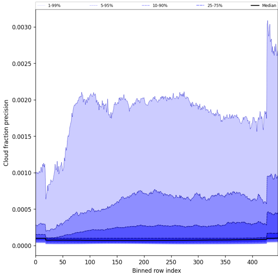
Figure 48: Along track statistics of “Cloud fraction precision” for 2025-01-14 to 2025-01-15
