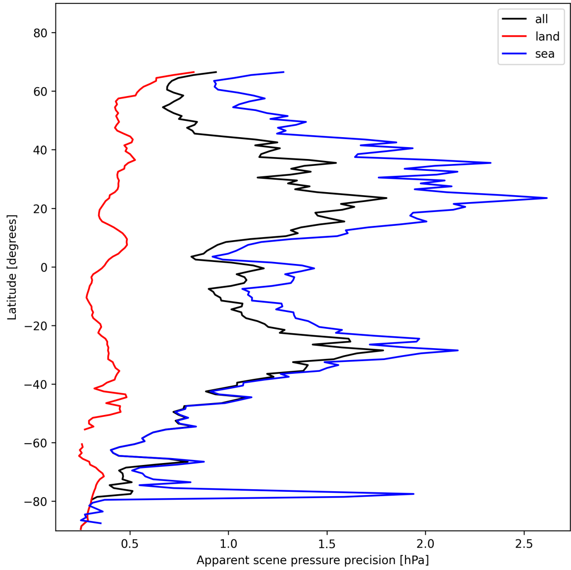
Figure 18: Zonal average of “Apparent scene pressure precision” for 2025-01-14 to 2025-01-15.
