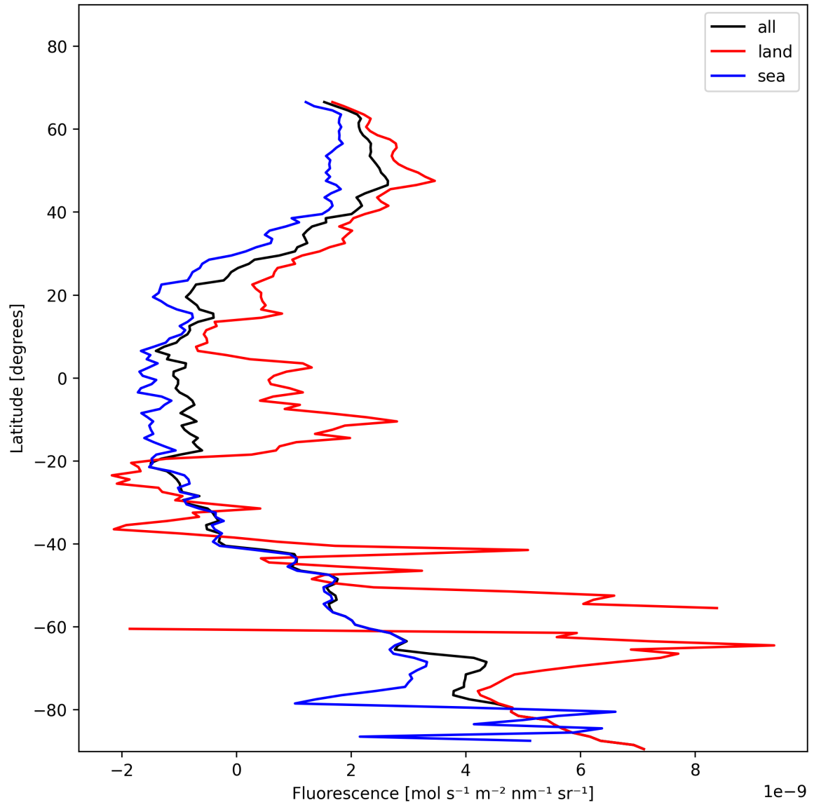
Figure 21: Zonal average of “Fluorescence” for 2025-01-14 to 2025-01-15.
