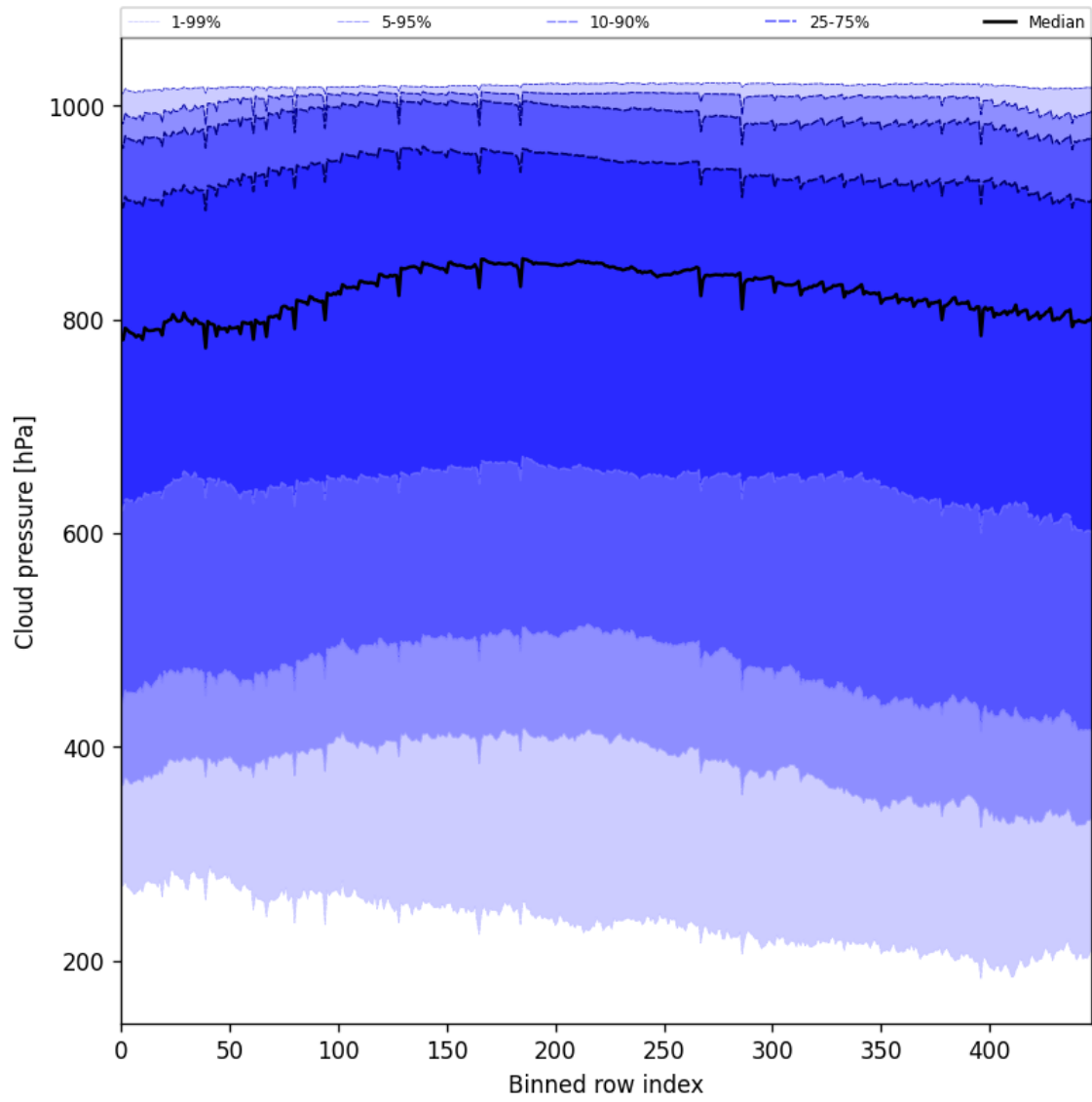
Figure 45: Along track statistics of “Cloud pressure” for 2025-01-14 to 2025-01-15
