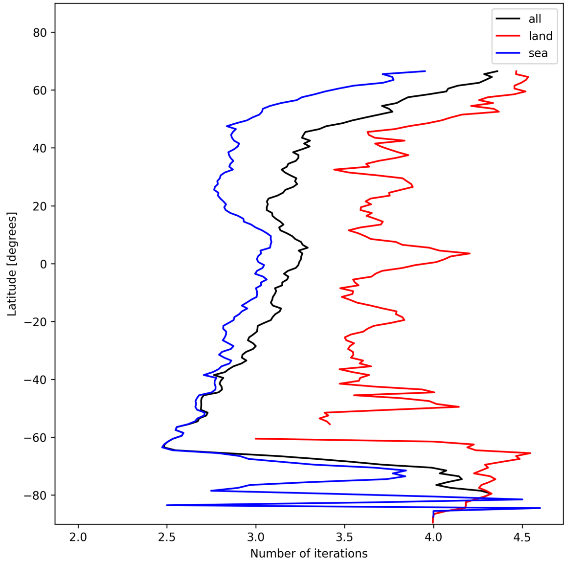
Figure 20: Zonal average of “Number of iterations” for 2025-01-14 to 2025-01-15.
