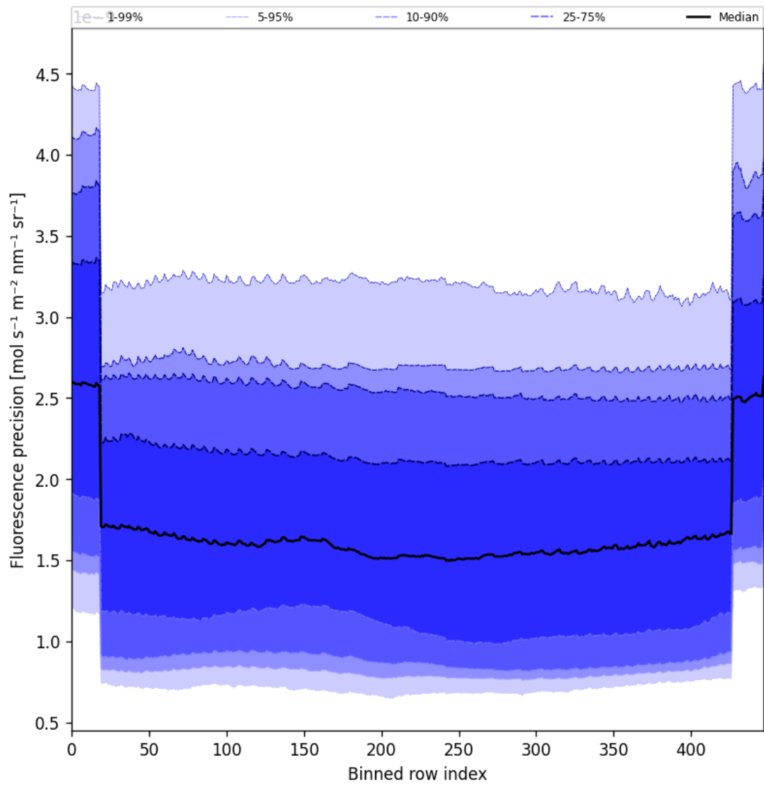
Figure 56: Along track statistics of “Fluorescence precision” for 2025-01-14 to 2025-01-15
