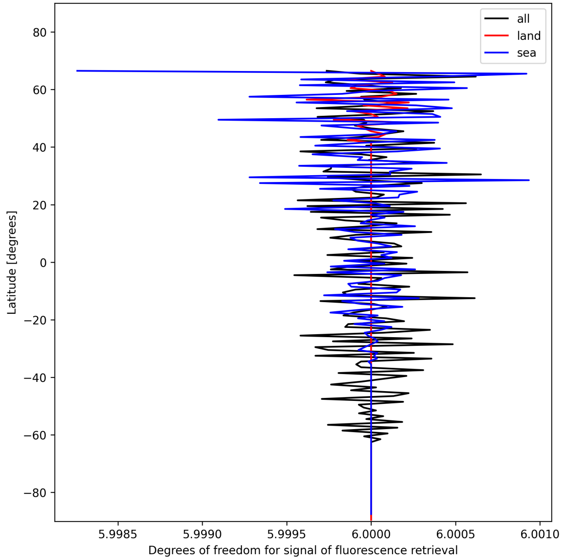
Figure 24: Zonal average of “Degrees of freedom for signal of fluorescence retrieval” for 2025-01-14 to 2025-01-15.
