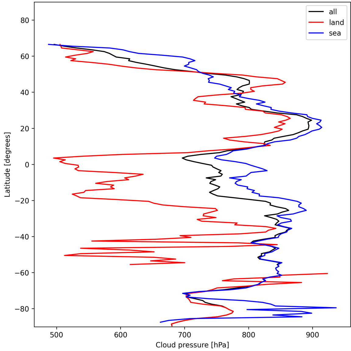
Figure 11: Zonal average of “Cloud pressure” for 2025-01-14 to 2025-01-15.
