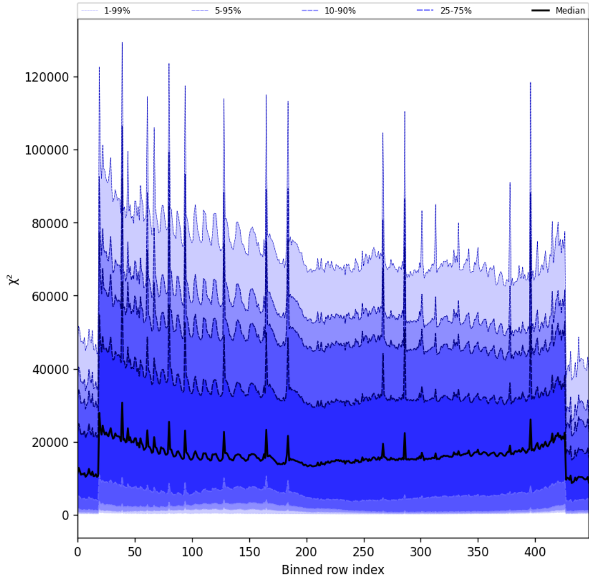
Figure 53: Along track statistics of “ \chi^2 ” for 2025-01-14 to 2025-01-15
