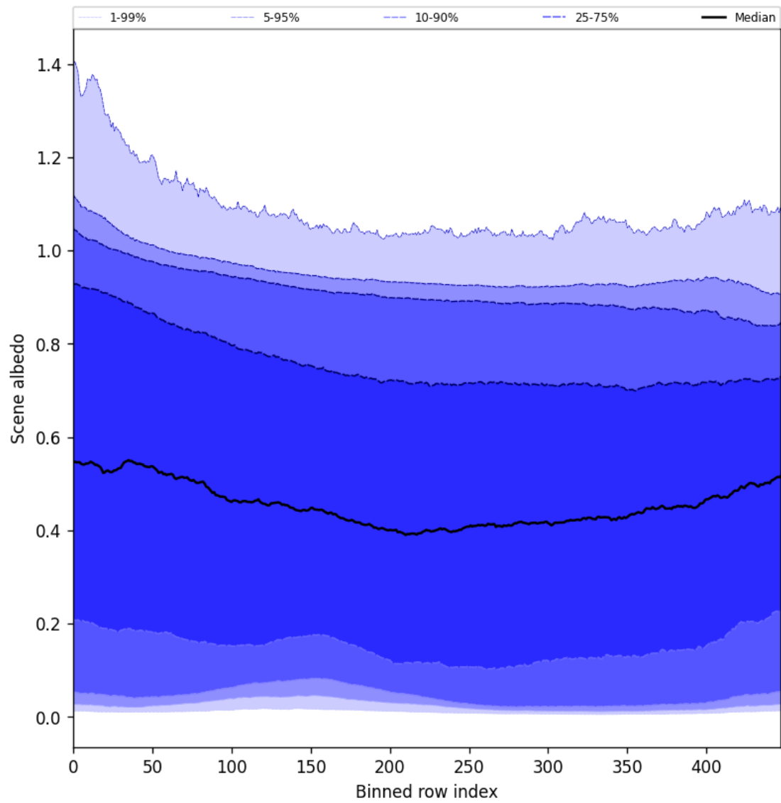
Figure 49: Along track statistics of “Scene albedo” for 2025-01-14 to 2025-01-15
