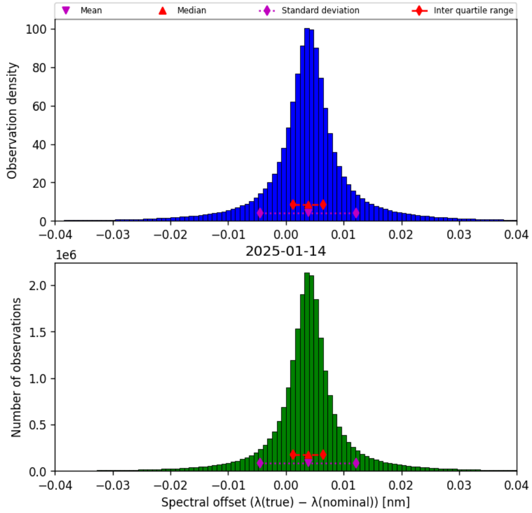
Figure 43: Histogram of “Spectral offset ( \lambda_{\text{true}} - \lambda_{\text{nominal}} )” for 2025-01-14 to 2025-01-15
