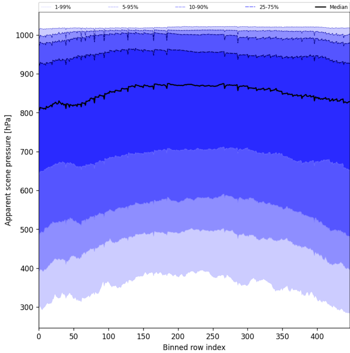
Figure 51: Along track statistics of “Apparent scene pressure” for 2025-01-14 to 2025-01-15
