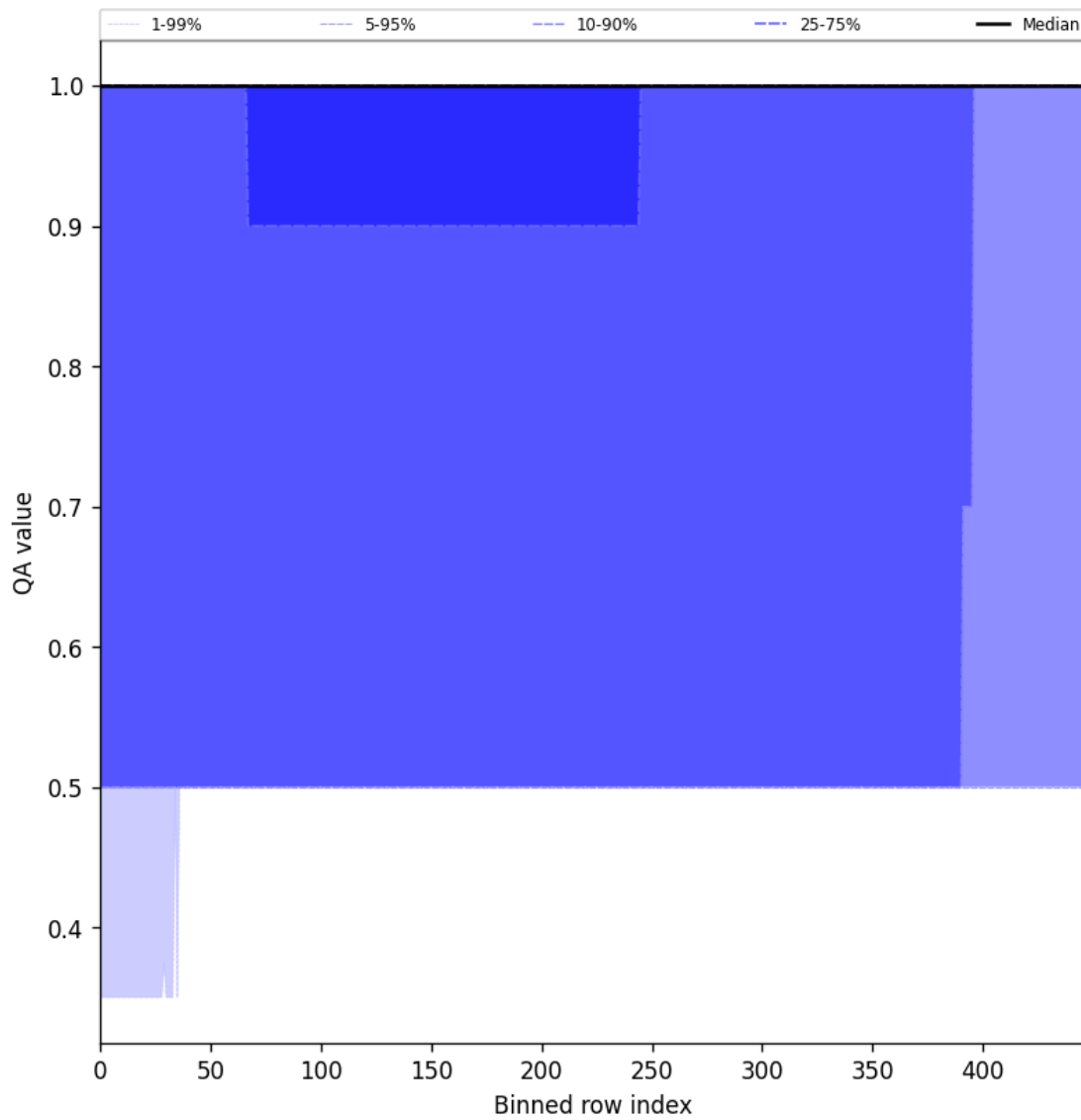
Figure 44: Along track statistics of “QA value” for 2025-01-14 to 2025-01-15
