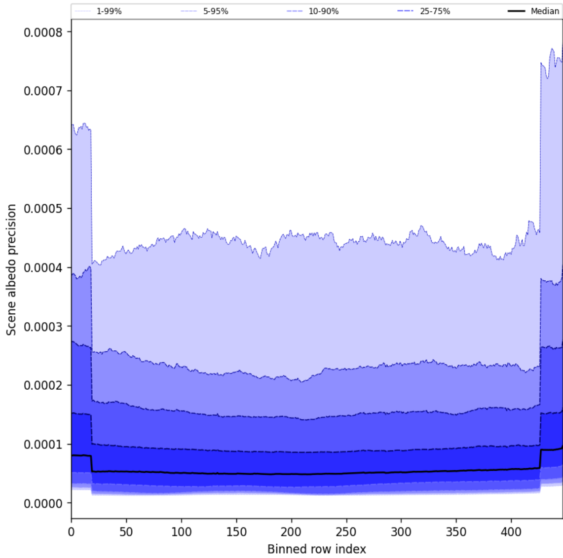
Figure 50: Along track statistics of “Scene albedo precision” for 2025-01-14 to 2025-01-15
