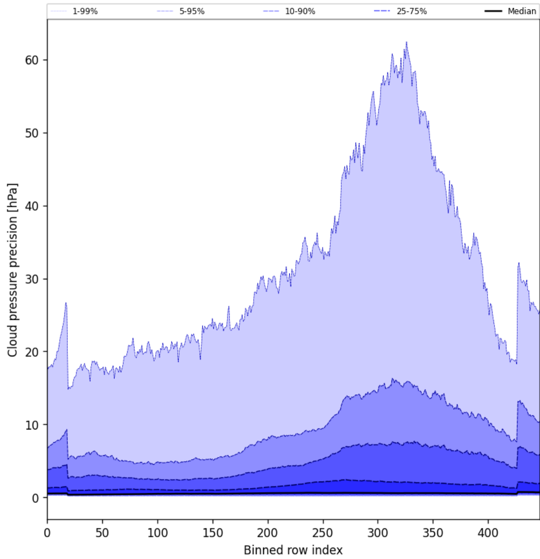
Figure 46: Along track statistics of “Cloud pressure precision” for 2025-01-14 to 2025-01-15
