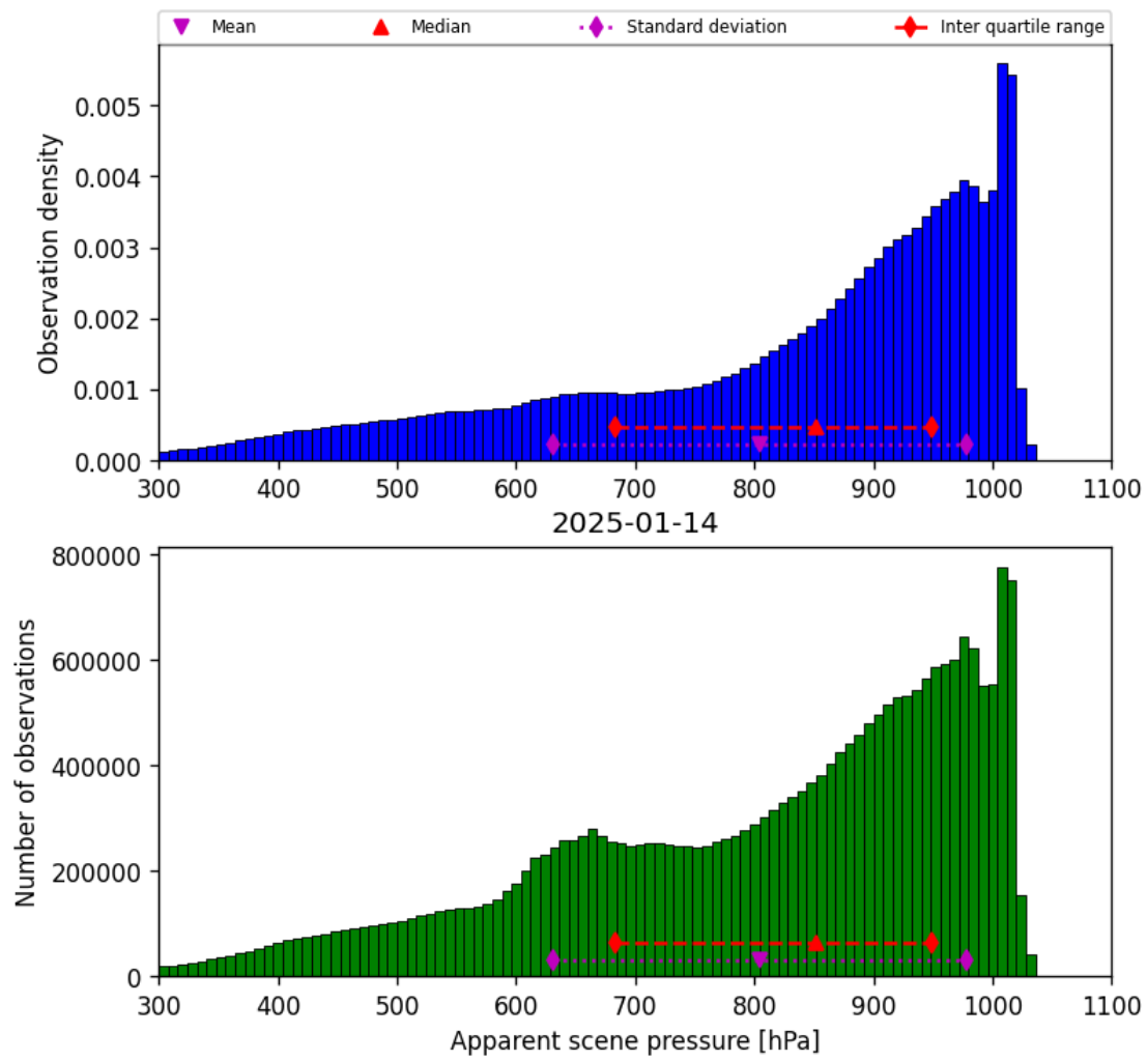
Figure 34: Histogram of “Apparent scene pressure” for 2025-01-14 to 2025-01-15
