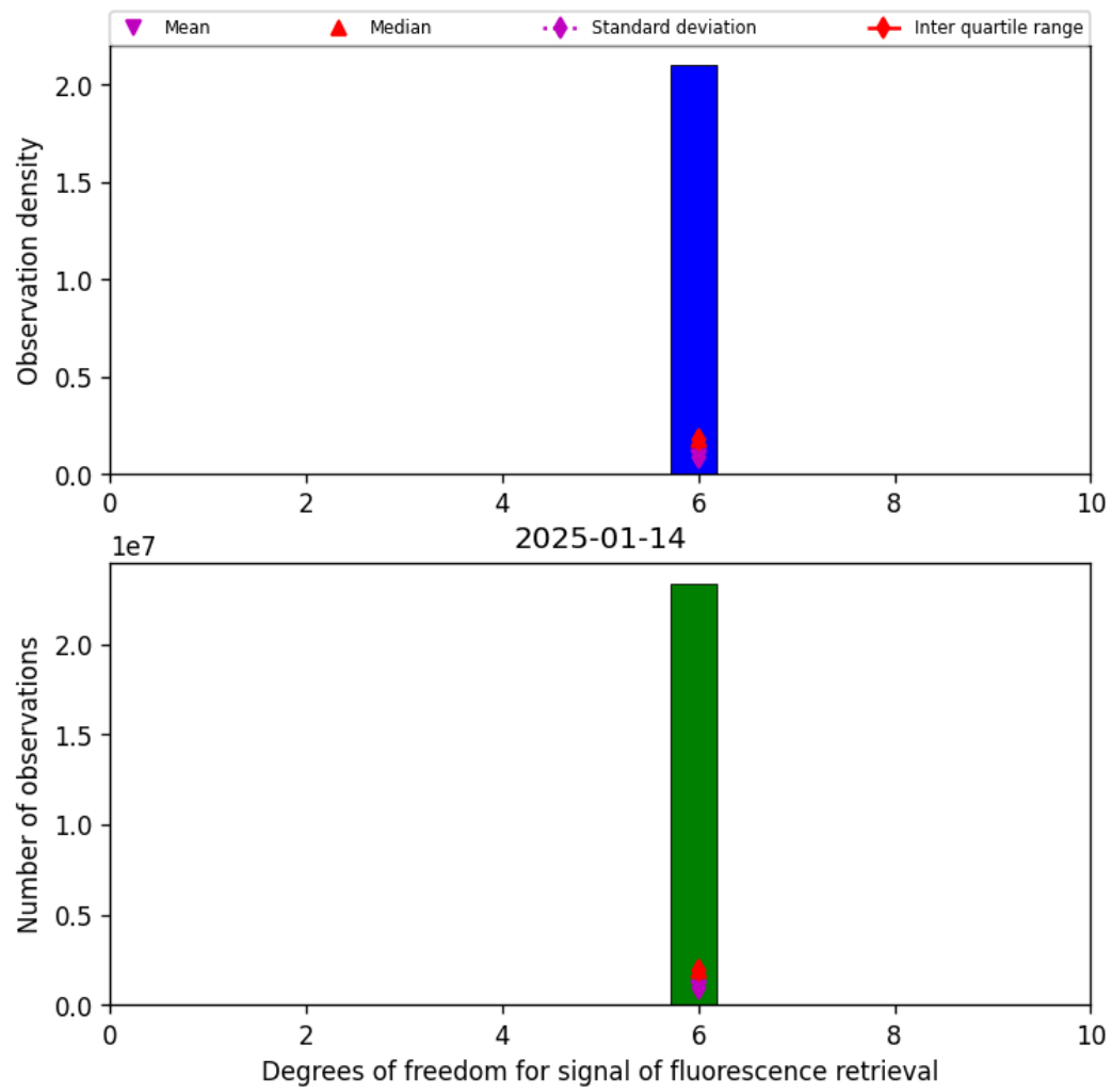
Figure 41: Histogram of “Degrees of freedom for signal of fluorescence retrieval” for 2025-01-14 to 2025-01-15
