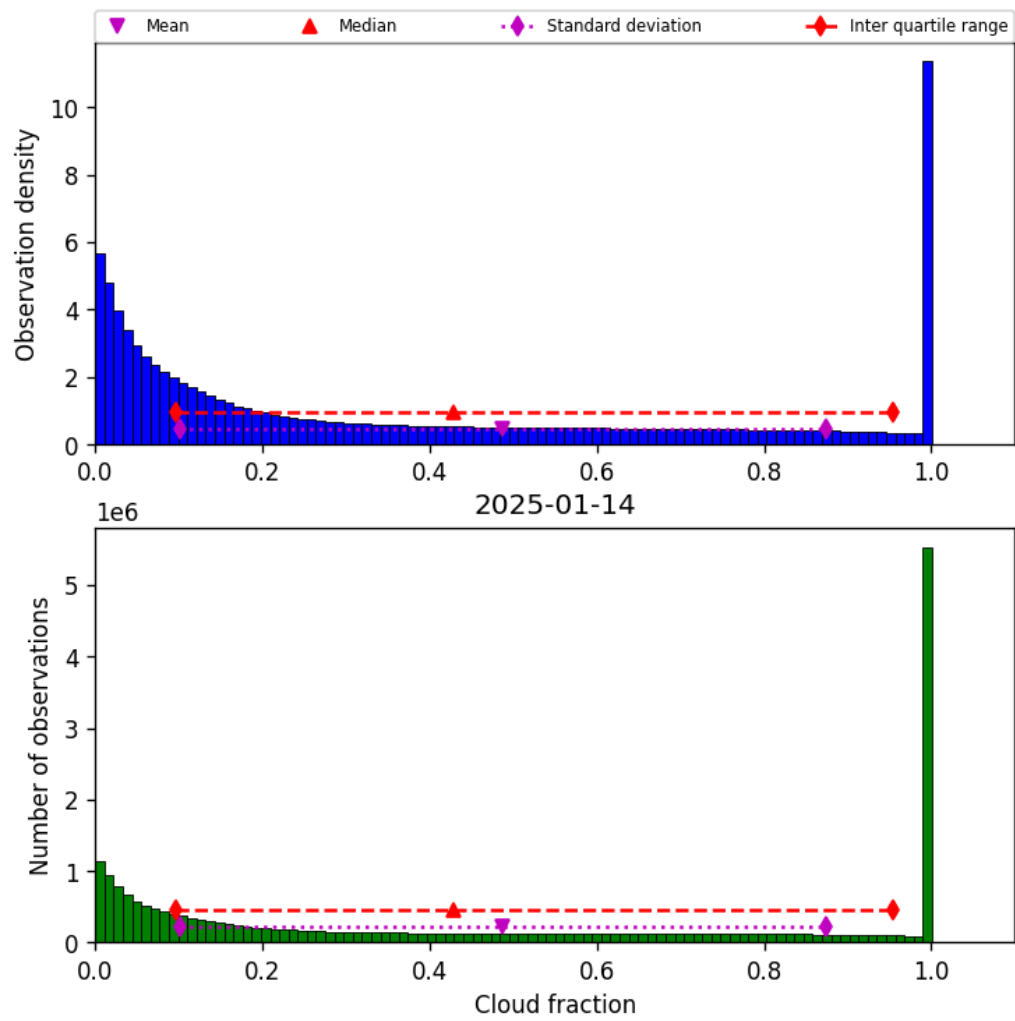
Figure 30: Histogram of “Cloud fraction” for 2025-01-14 to 2025-01-15
