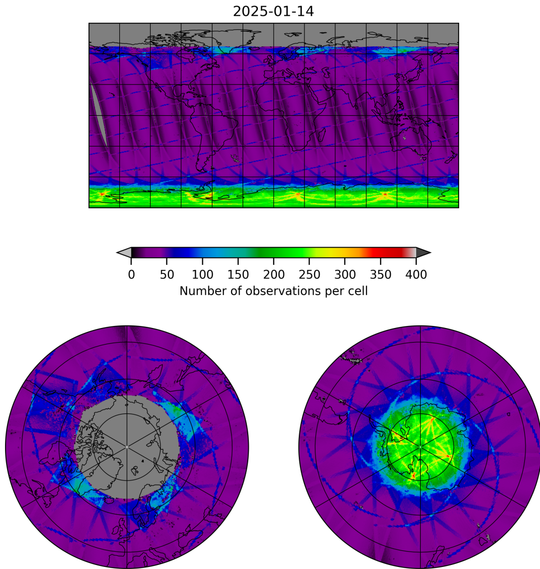
Figure 9: Map of the number of observations for 2025-01-14 to 2025-01-15
