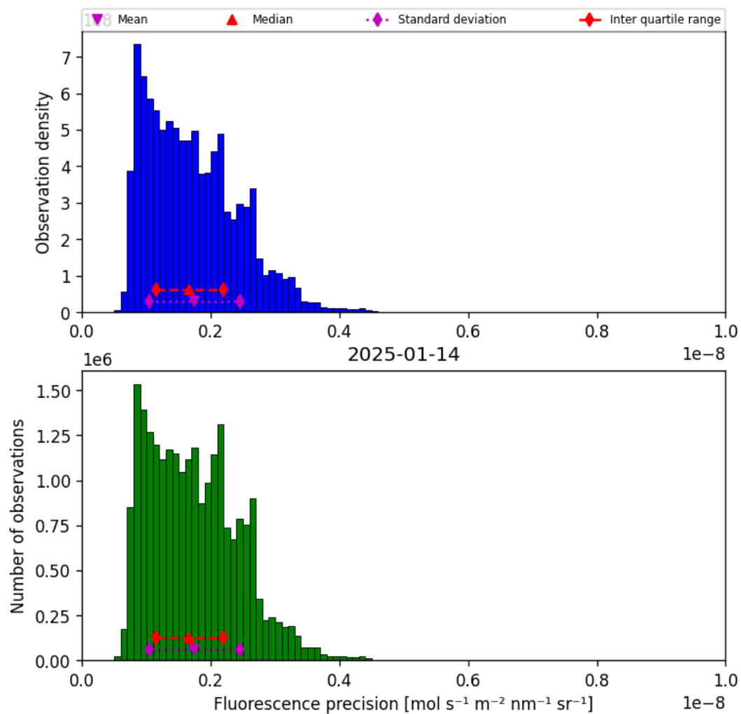
Figure 39: Histogram of “Fluorescence precision” for 2025-01-14 to 2025-01-15
