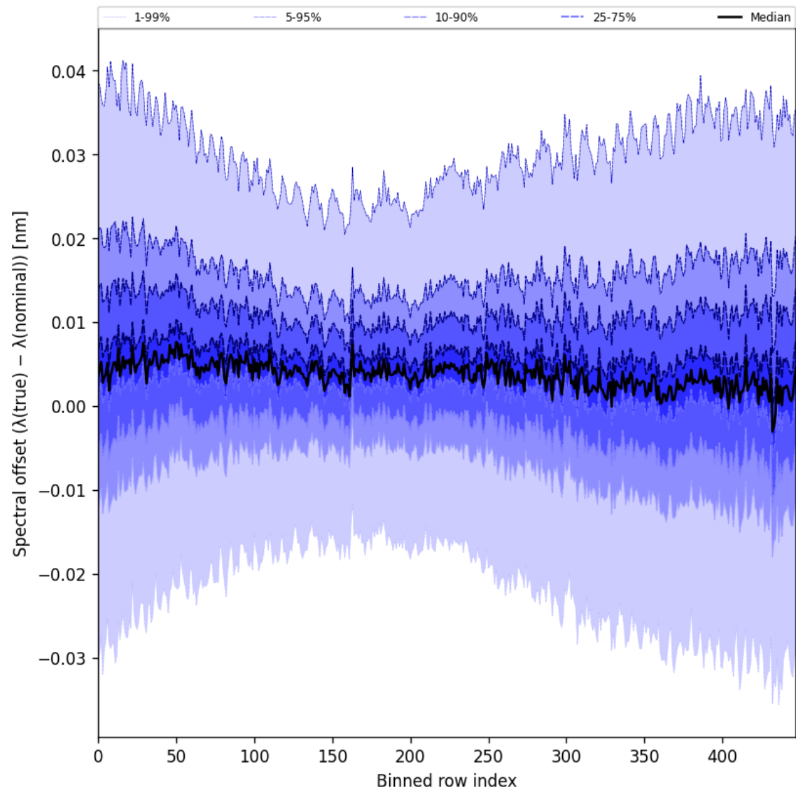
Figure 60: Along track statistics of “Spectral offset ( \lambda_{\text{true}} - \lambda_{\text{nominal}} )” for 2025-01-14 to 2025-01-15
