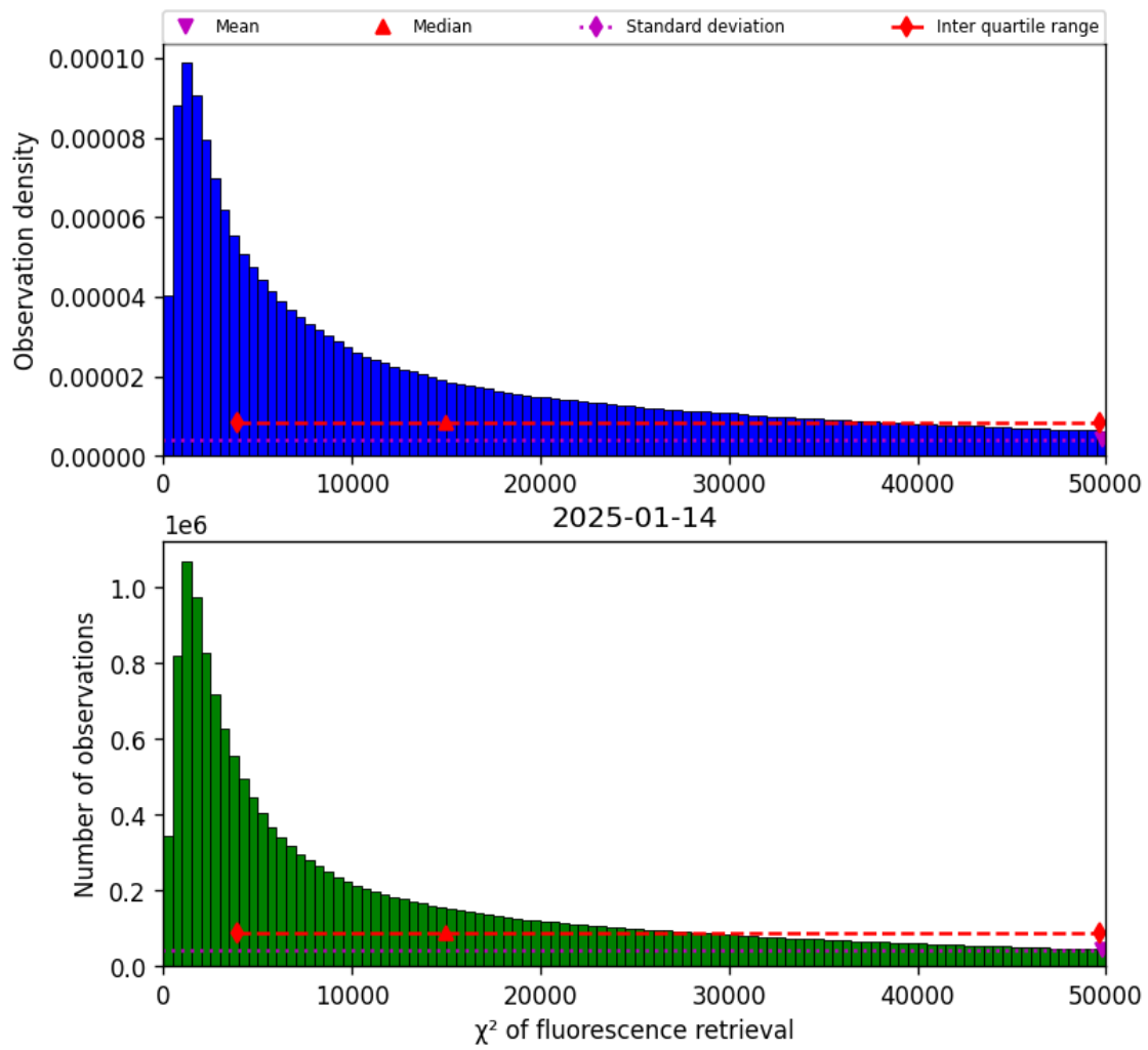
Figure 40: Histogram of “ \chi^2 of fluorescence retrieval” for 2025-01-14 to 2025-01-15
