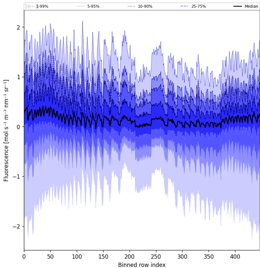
Figure 55: Along track statistics of “Fluorescence” for 2025-01-14 to 2025-01-15
