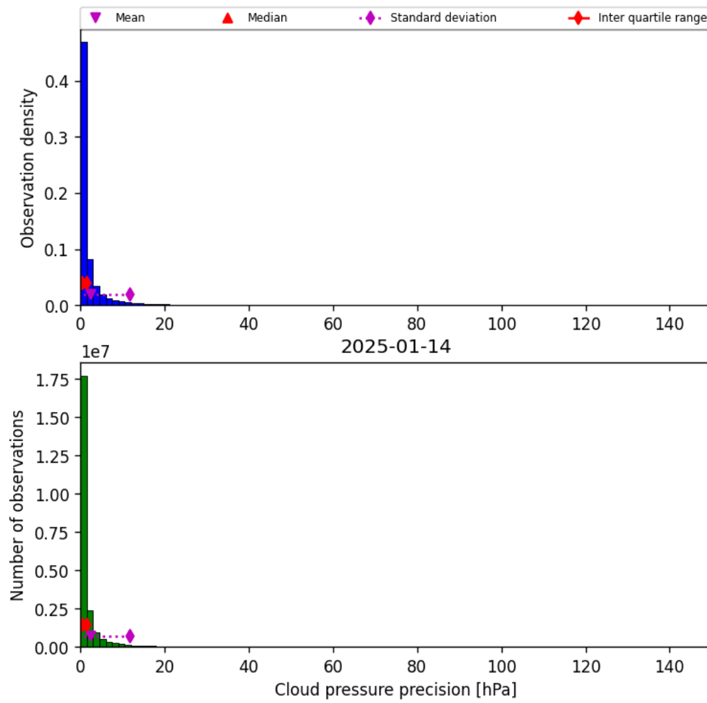
Figure 29: Histogram of “Cloud pressure precision” for 2025-01-14 to 2025-01-15
