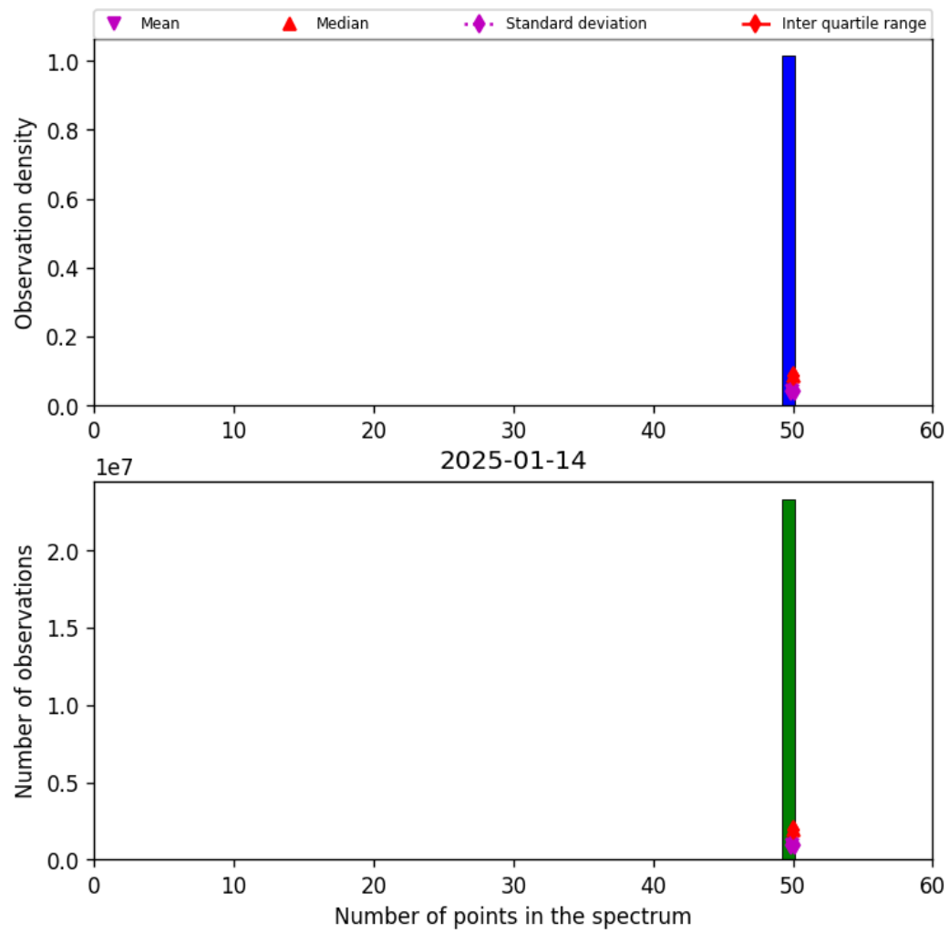
Figure 42: Histogram of “Number of points in the spectrum” for 2025-01-14 to 2025-01-15
