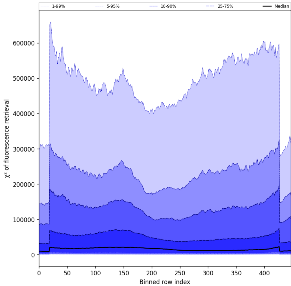
Figure 57: Along track statistics of “ \chi^2 of fluorescence retrieval” for 2025-01-14 to 2025-01-15
