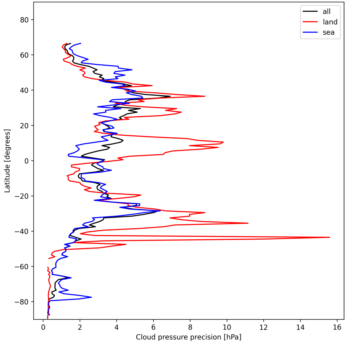
Figure 12: Zonal average of "Cloud pressure precision" for 2025-01-14 to 2025-01-15.
