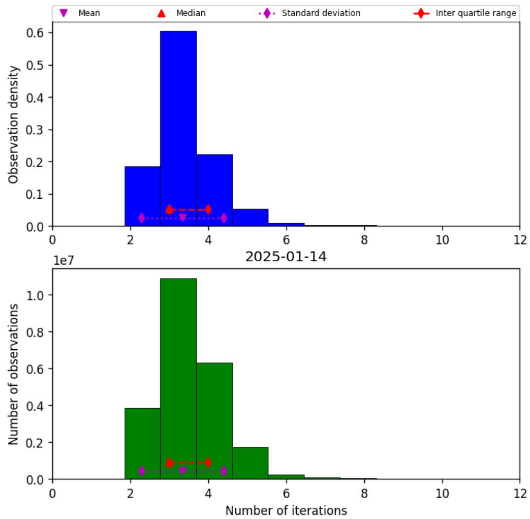
Figure 37: Histogram of “Number of iterations” for 2025-01-14 to 2025-01-15
