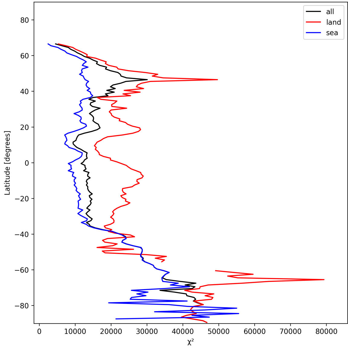
Figure 19: Zonal average of “ \chi^2 ” for 2025-01-14 to 2025-01-15.
