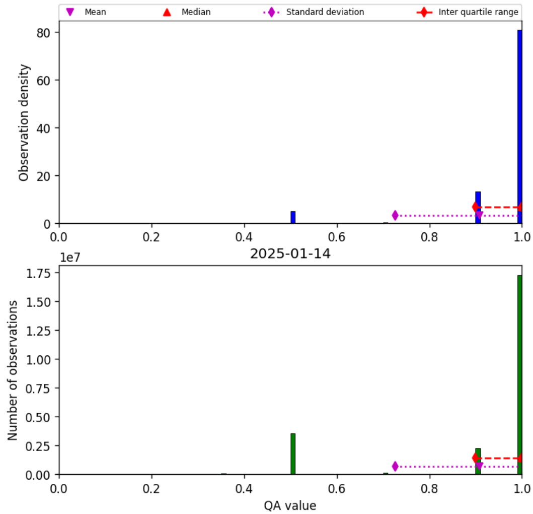
Figure 27: Histogram of “QA value” for 2025-01-14 to 2025-01-15
