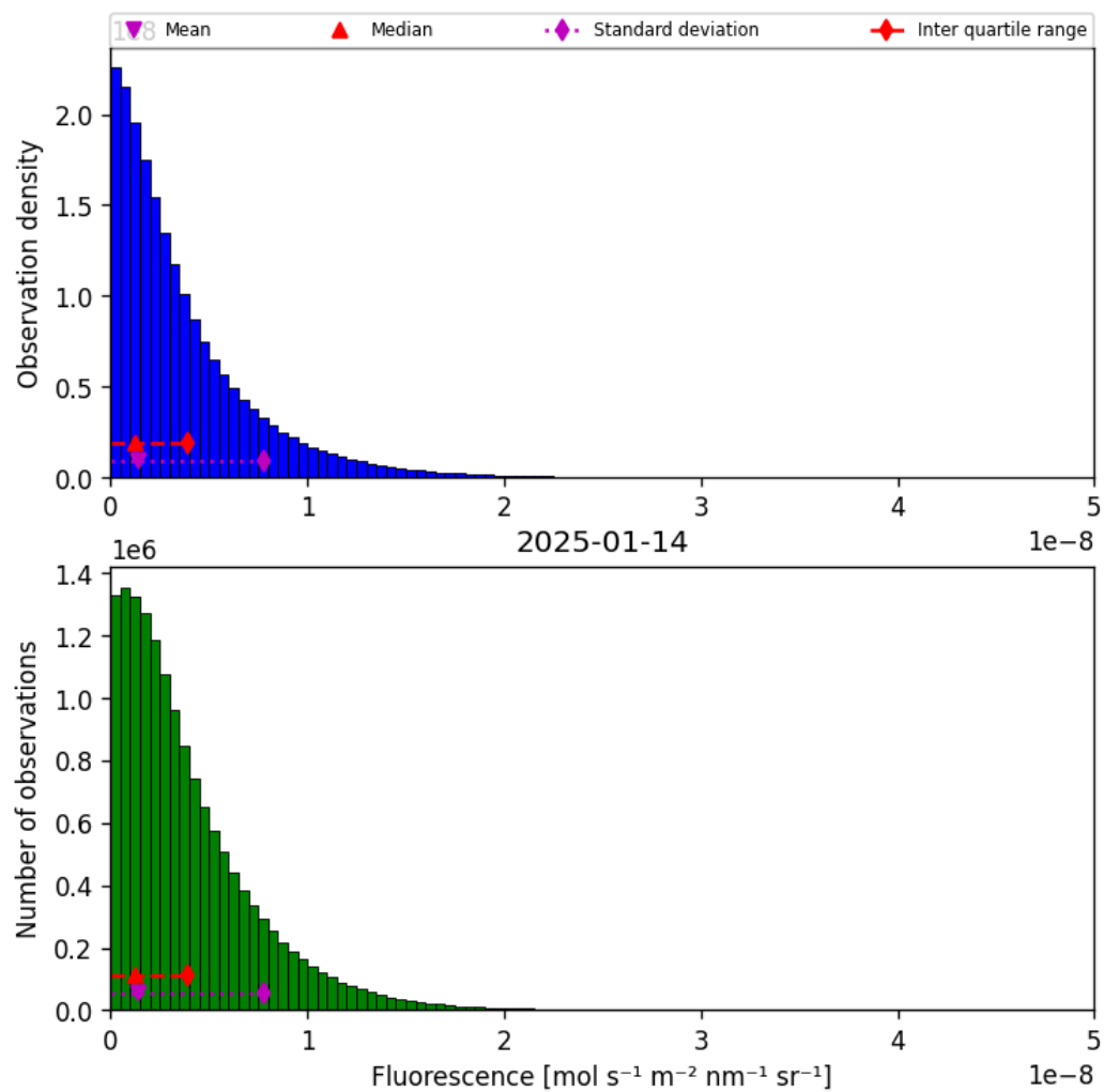
Figure 38: Histogram of “Fluorescence” for 2025-01-14 to 2025-01-15
