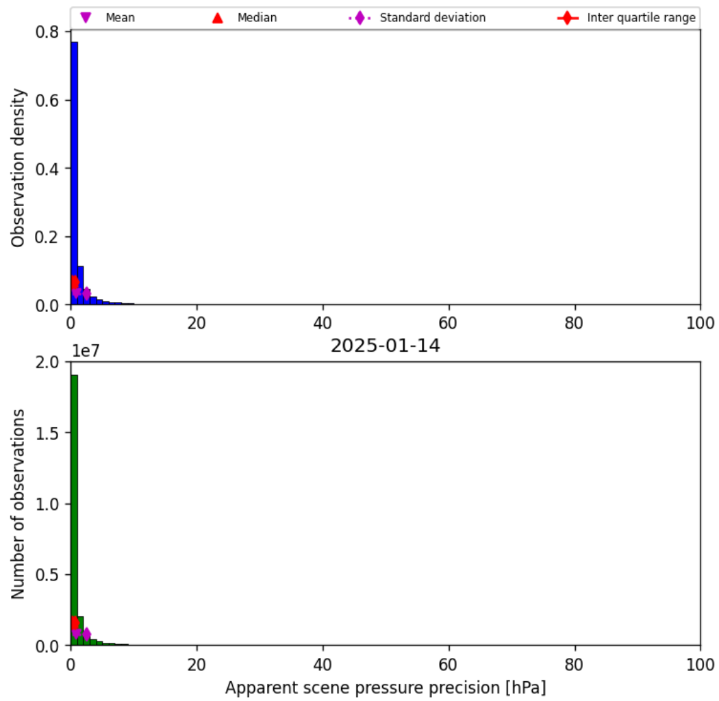
Figure 35: Histogram of “Apparent scene pressure precision” for 2025-01-14 to 2025-01-15
