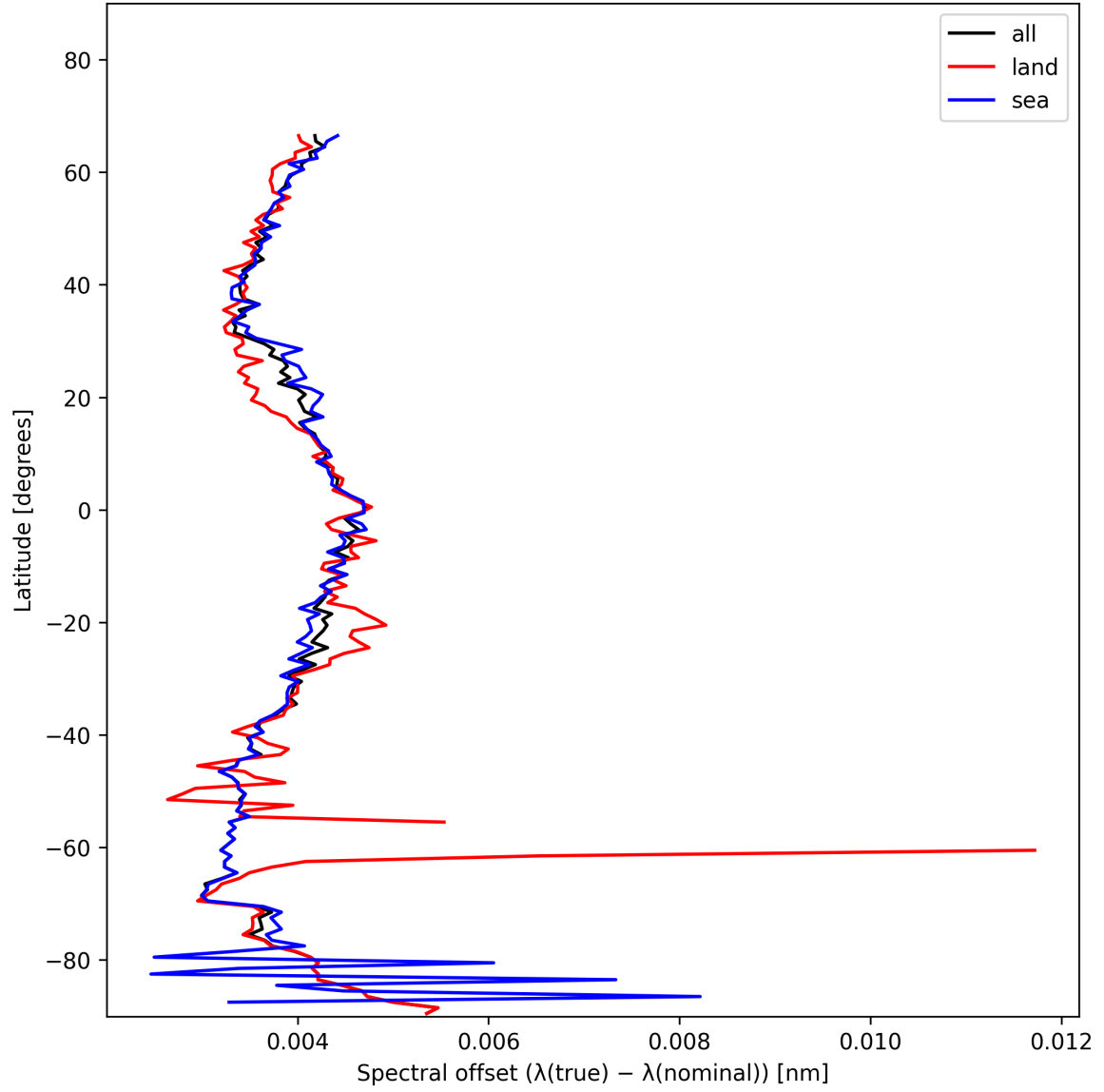
Figure 26: Zonal average of “Spectral offset ( \lambda_{\text{true}} - \lambda_{\text{nominal}} )” for 2025-01-14 to 2025-01-15.
