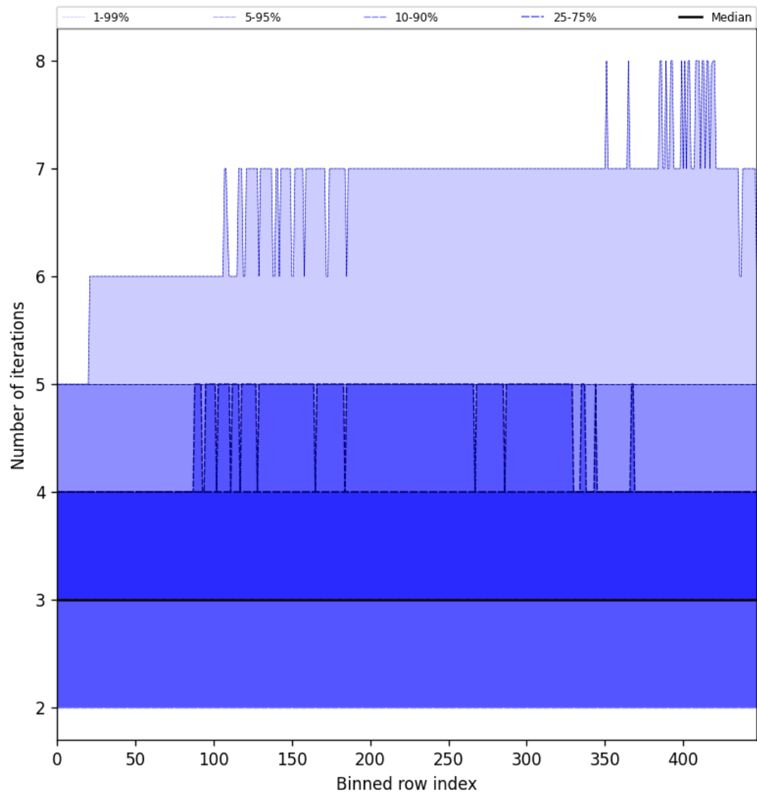
Figure 54: Along track statistics of “Number of iterations” for 2025-01-14 to 2025-01-15
