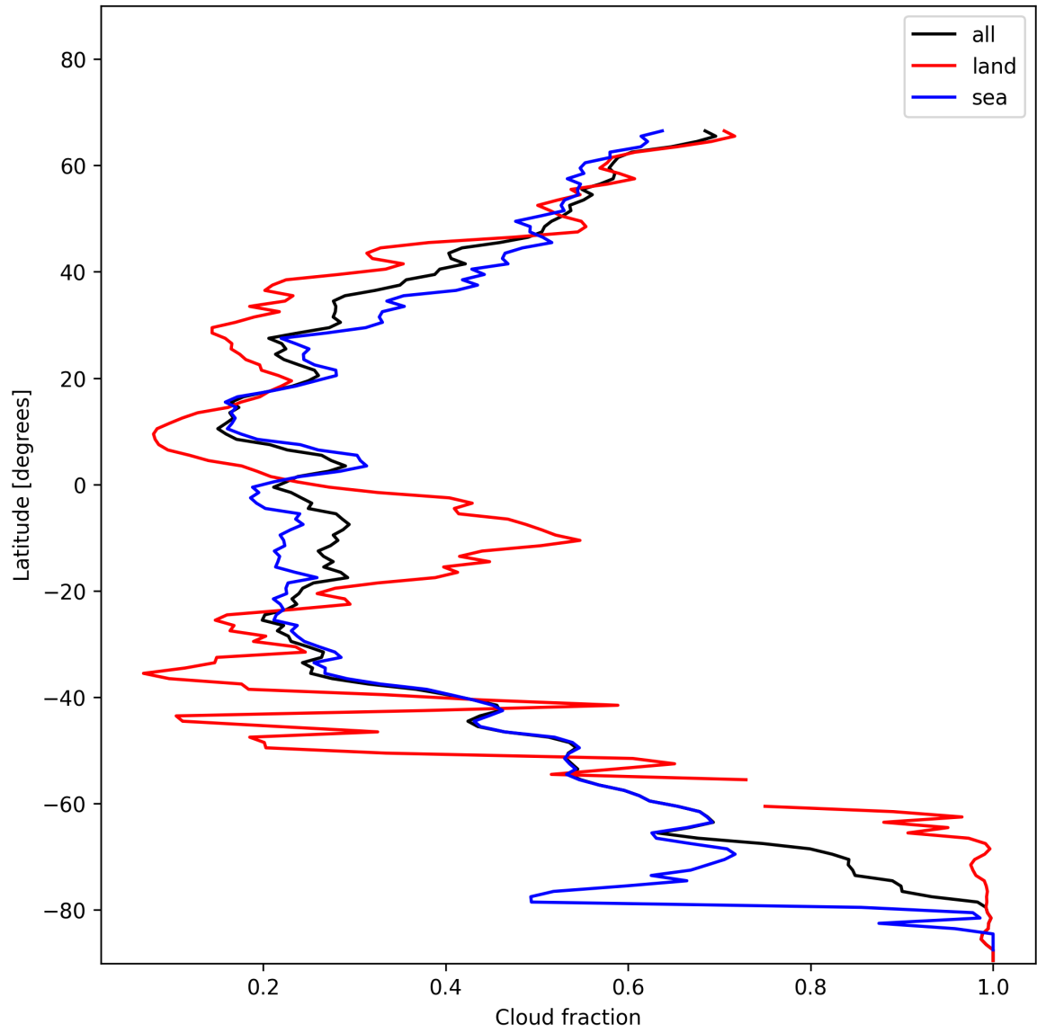
Figure 13: Zonal average of “Cloud fraction” for 2025-01-14 to 2025-01-15.
