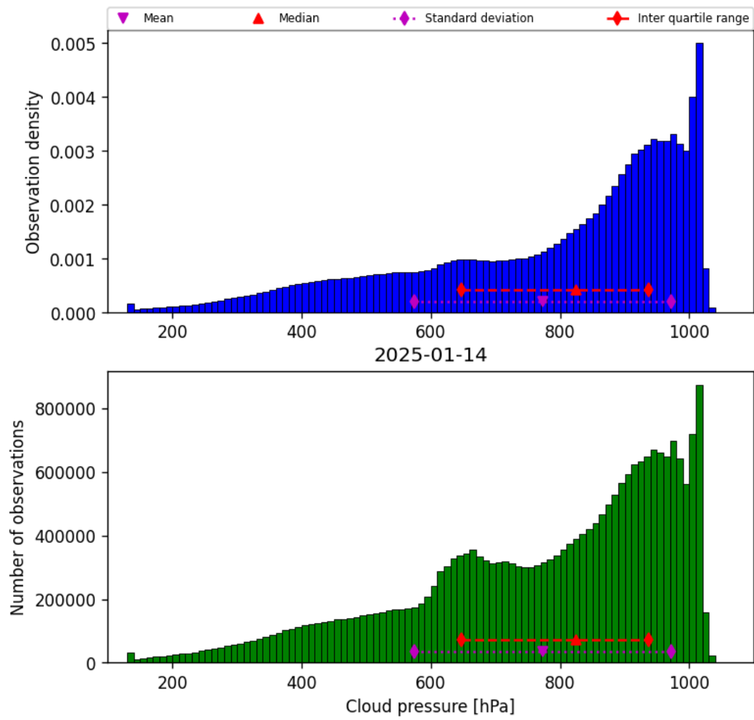
Figure 28: Histogram of “Cloud pressure” for 2025-01-14 to 2025-01-15
