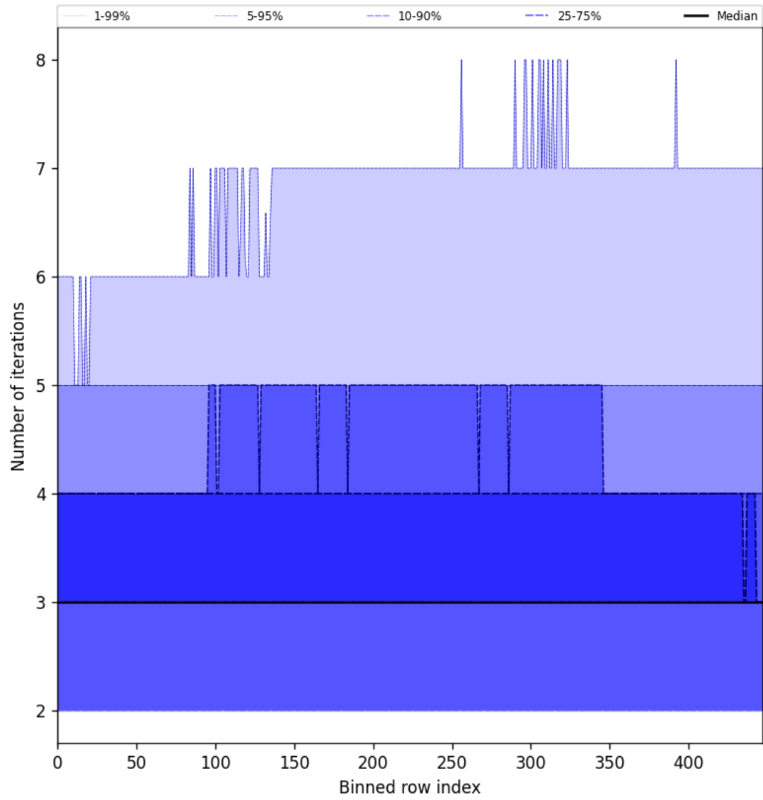
Figure 54: Along track statistics of “Number of iterations” for 2025-01-15 to 2025-01-15
