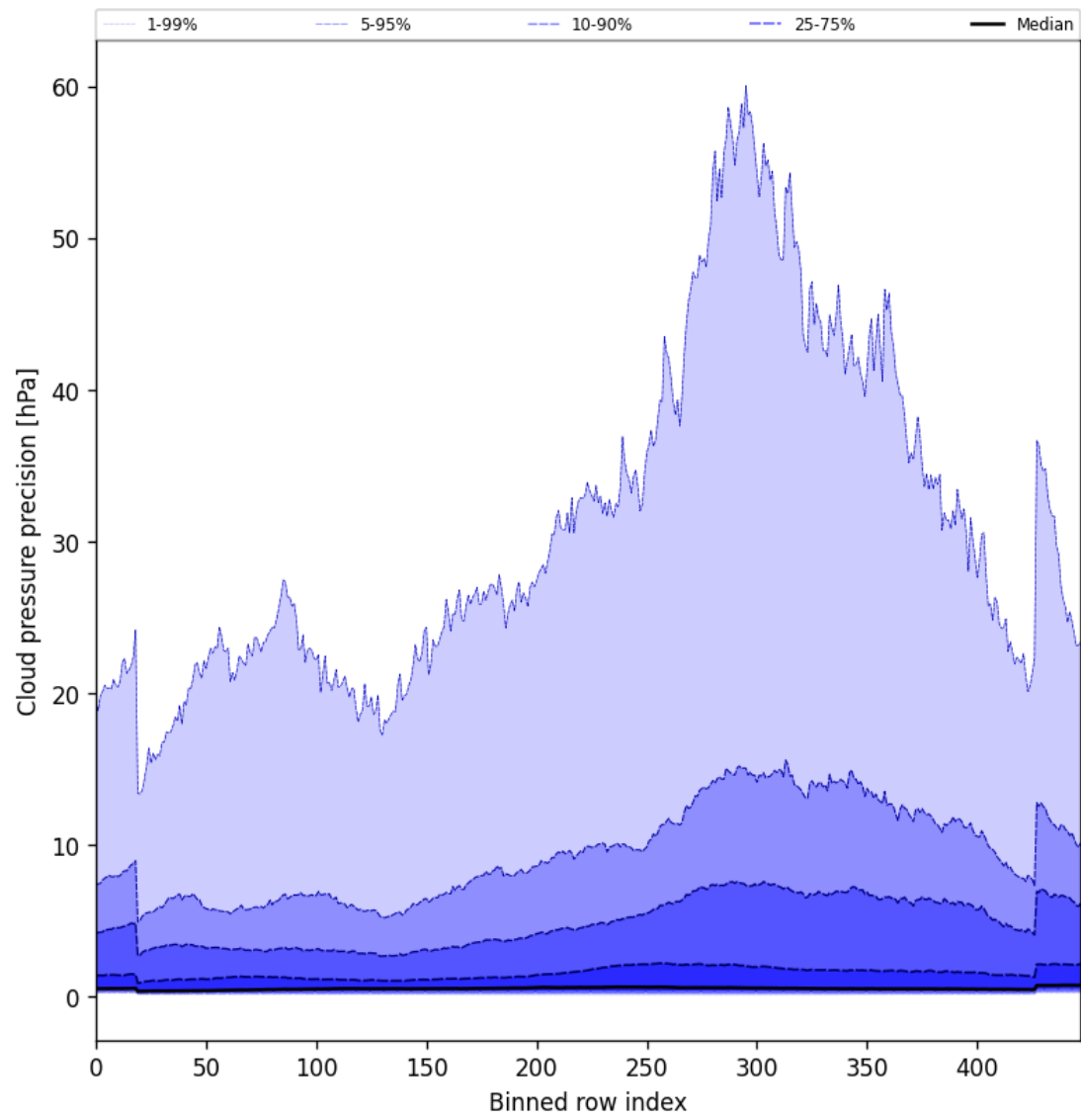
Figure 46: Along track statistics of “Cloud pressure precision” for 2025-01-15 to 2025-01-15
