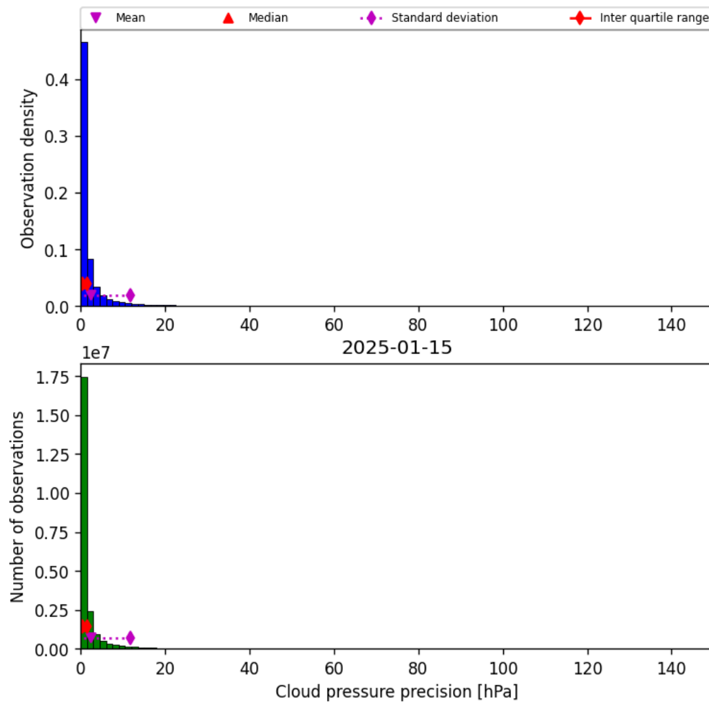
Figure 29: Histogram of “Cloud pressure precision” for 2025-01-15 to 2025-01-15
