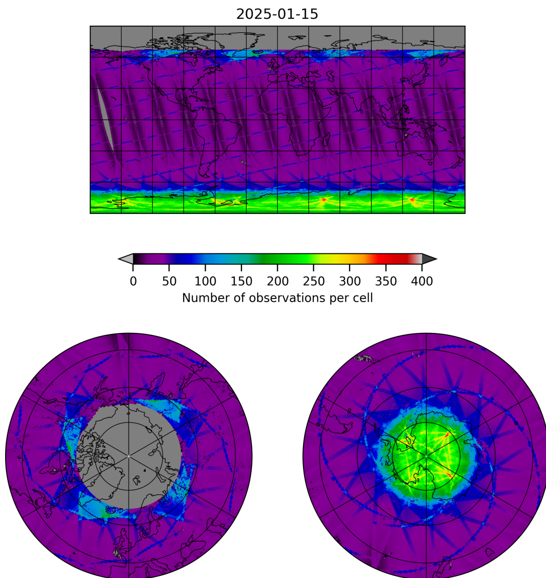
Figure 9: Map of the number of observations for 2025-01-15 to 2025-01-15
