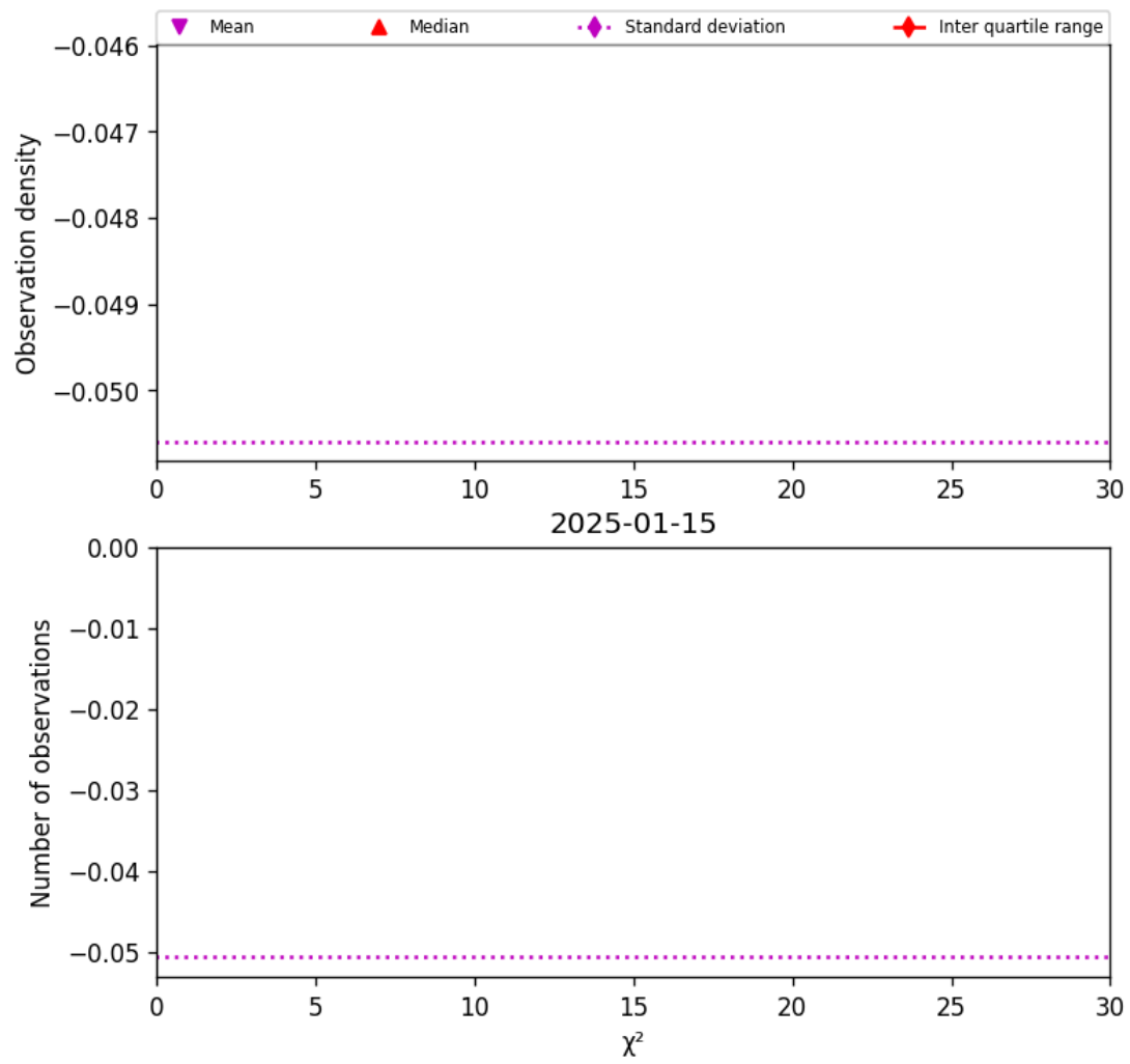
Figure 36: Histogram of " \chi^2 " for 2025-01-15 to 2025-01-15
