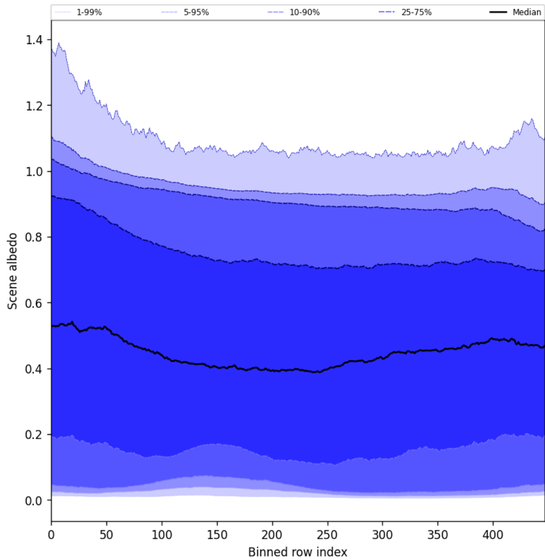
Figure 49: Along track statistics of “Scene albedo” for 2025-01-15 to 2025-01-15
