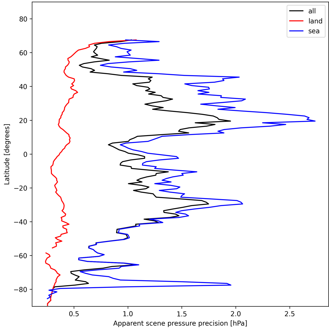
Figure 18: Zonal average of “Apparent scene pressure precision” for 2025-01-15 to 2025-01-15.
