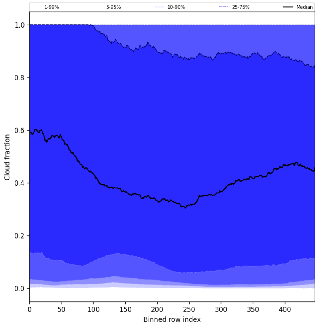
Figure 47: Along track statistics of “Cloud fraction” for 2025-01-15 to 2025-01-15
