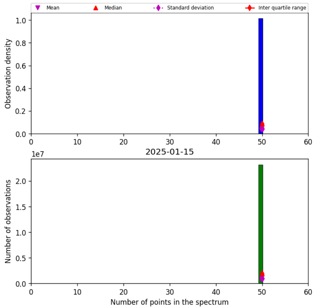
Figure 42: Histogram of “Number of points in the spectrum” for 2025-01-15 to 2025-01-15
