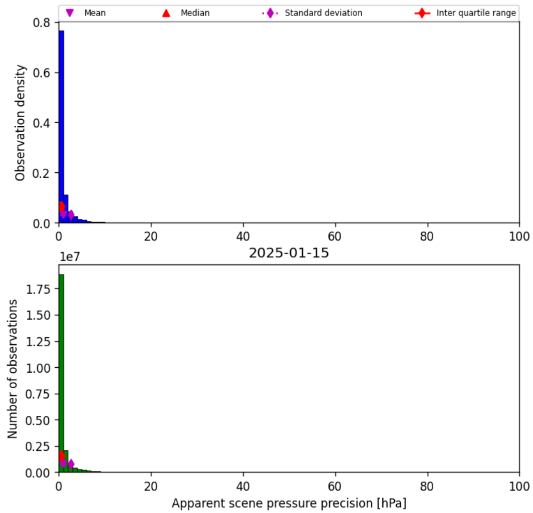
Figure 35: Histogram of “Apparent scene pressure precision” for 2025-01-15 to 2025-01-15
