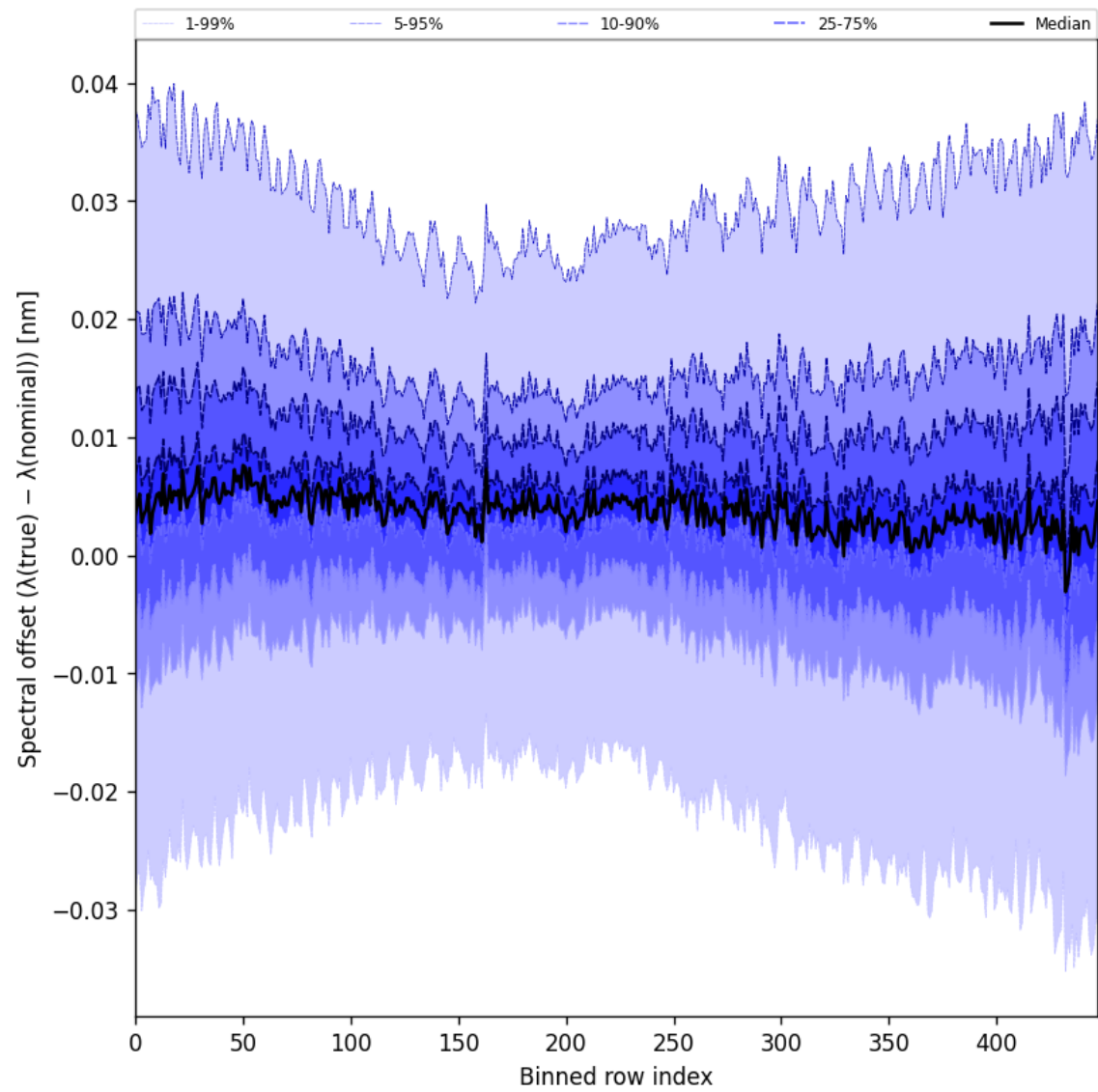
Figure 60: Along track statistics of “Spectral offset ( \lambda_{\text{true}} - \lambda_{\text{nominal}} )” for 2025-01-15 to 2025-01-15
