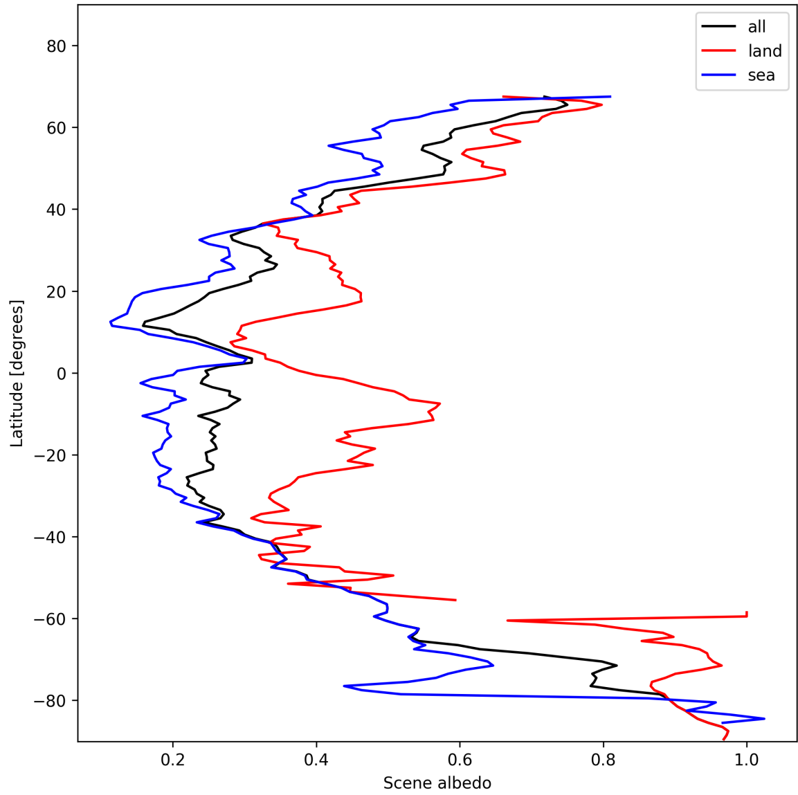
Figure 15: Zonal average of “Scene albedo” for 2025-01-15 to 2025-01-15.
