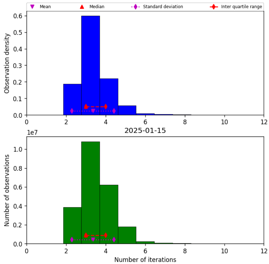
Figure 37: Histogram of “Number of iterations” for 2025-01-15 to 2025-01-15
