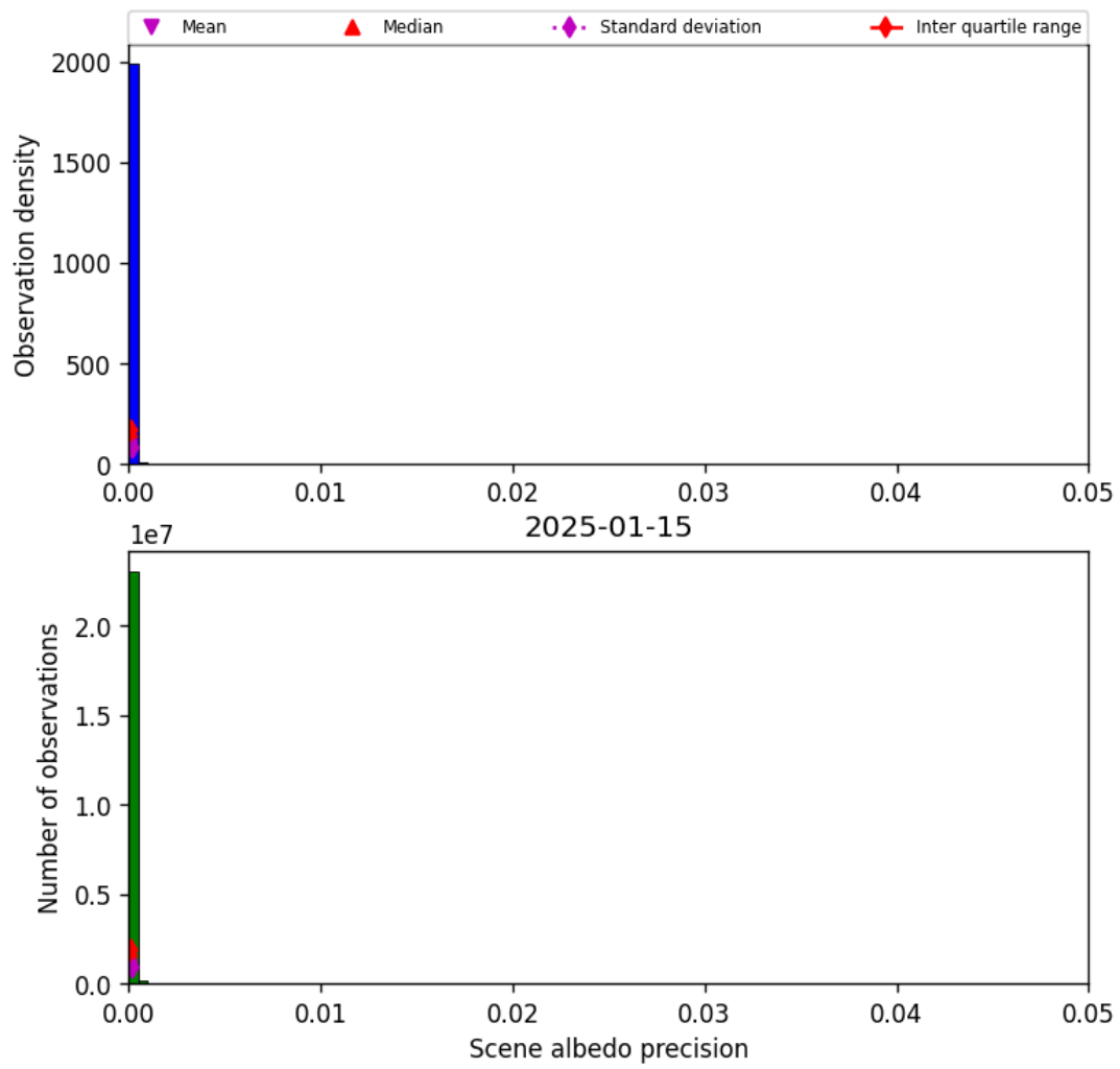
Figure 33: Histogram of “Scene albedo precision” for 2025-01-15 to 2025-01-15
