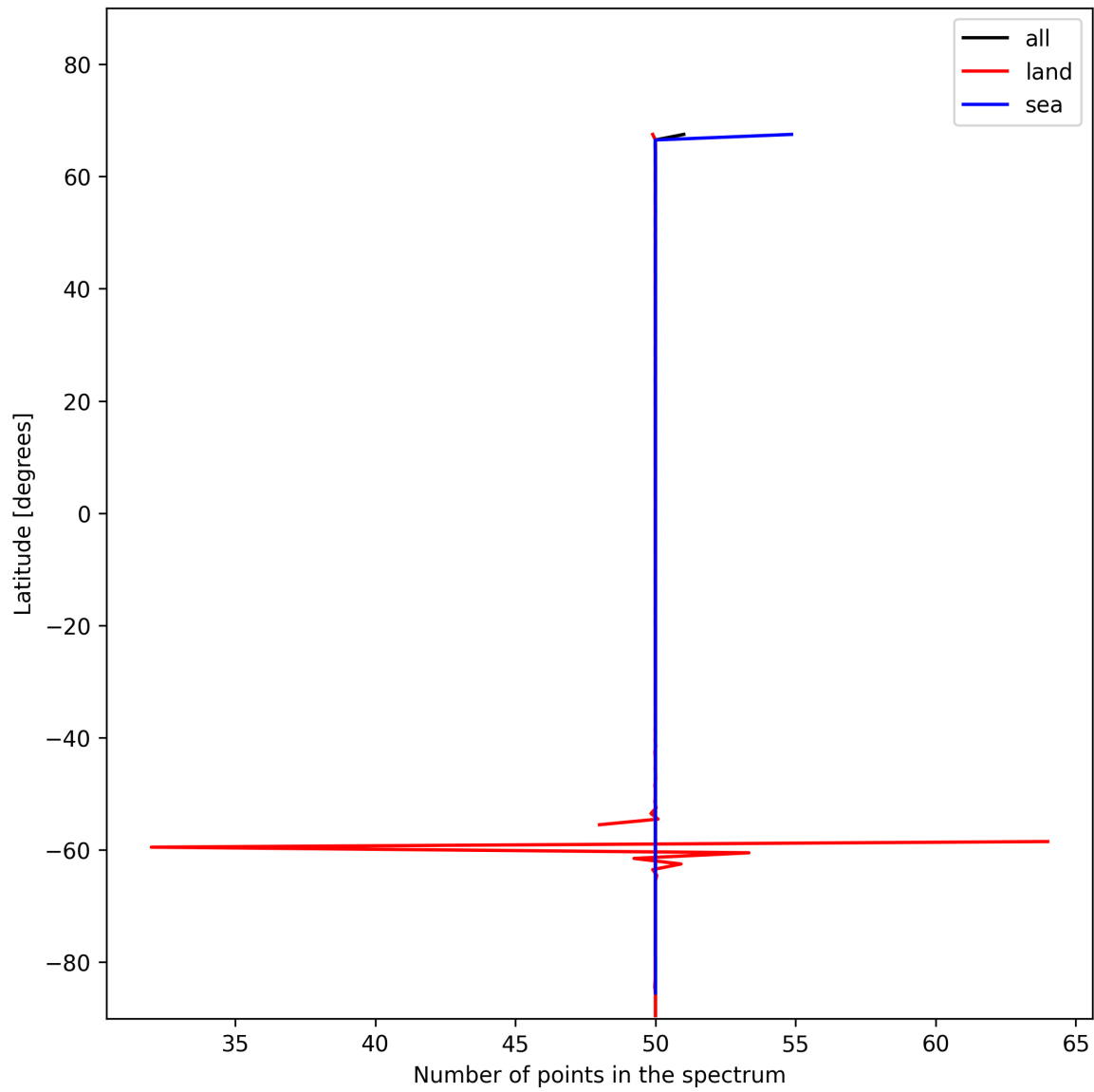
Figure 25: Zonal average of “Number of points in the spectrum” for 2025-01-15 to 2025-01-15.
