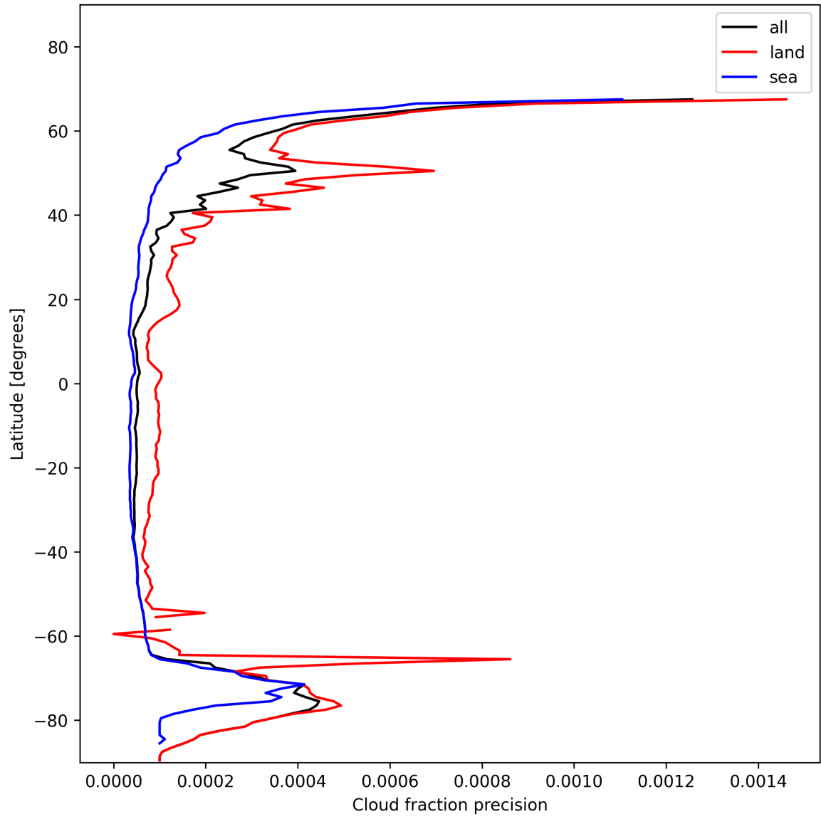
Figure 14: Zonal average of “Cloud fraction precision” for 2025-01-15 to 2025-01-15.
