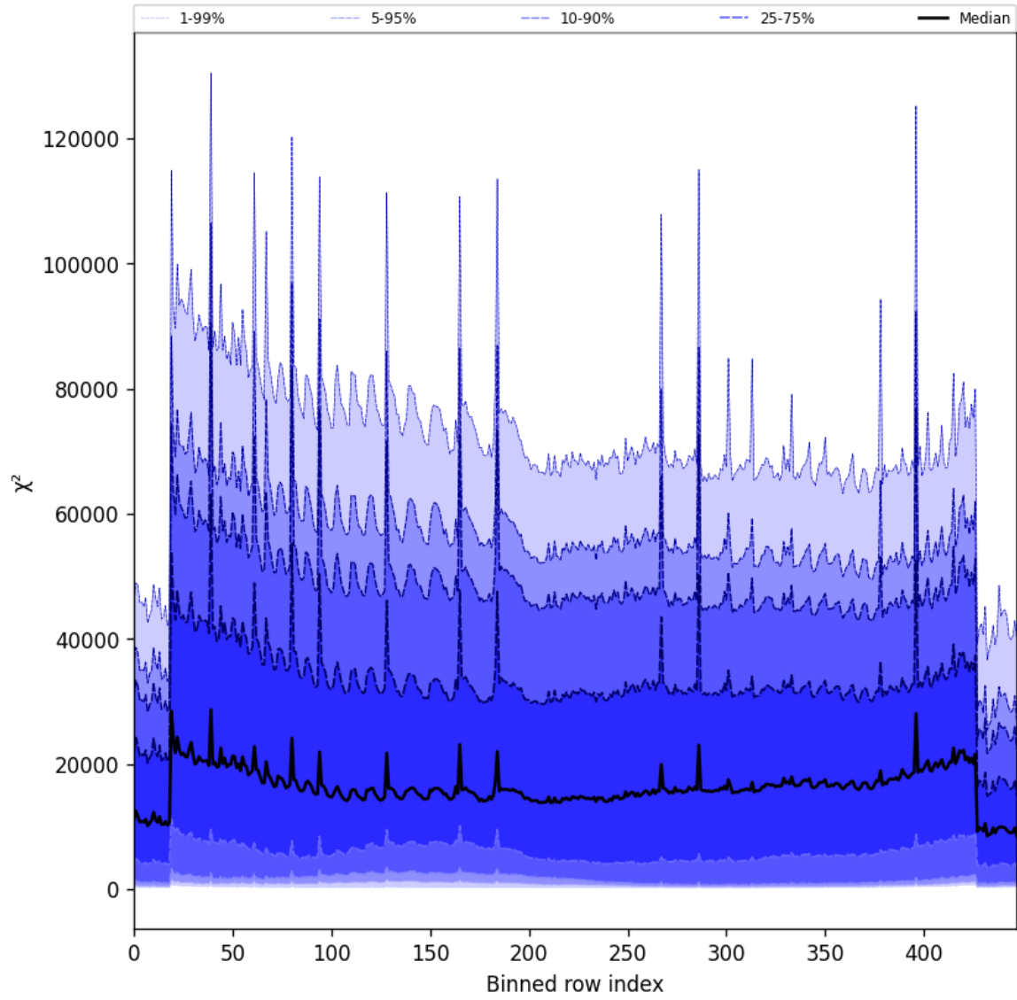
Figure 53: Along track statistics of “ \chi^2 ” for 2025-01-15 to 2025-01-15
