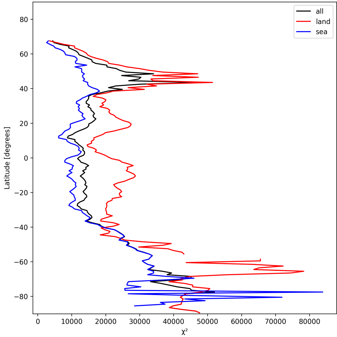
Figure 19: Zonal average of “ \chi^2 ” for 2025-01-15 to 2025-01-15.
