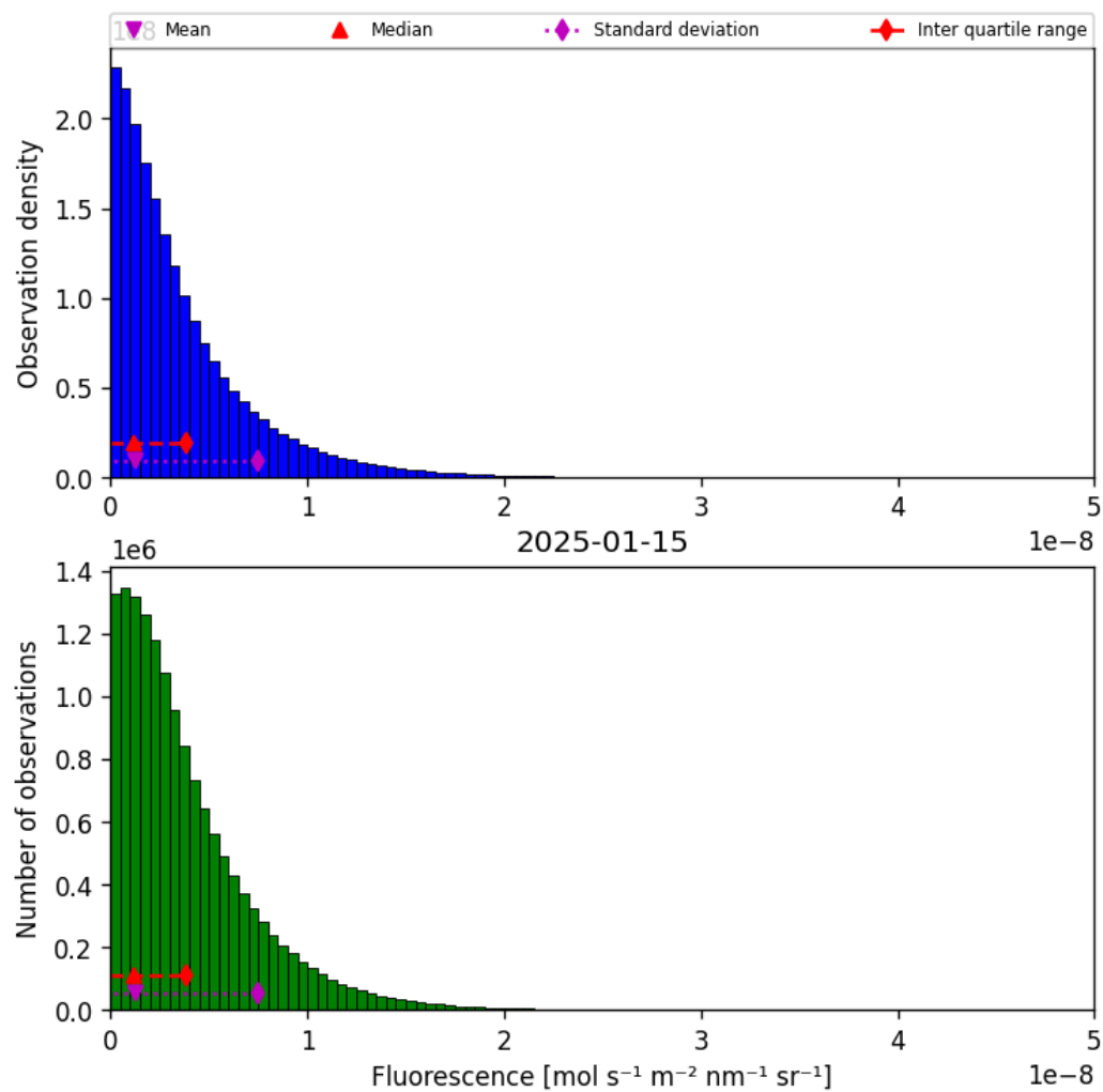
Figure 38: Histogram of “Fluorescence” for 2025-01-15 to 2025-01-15
