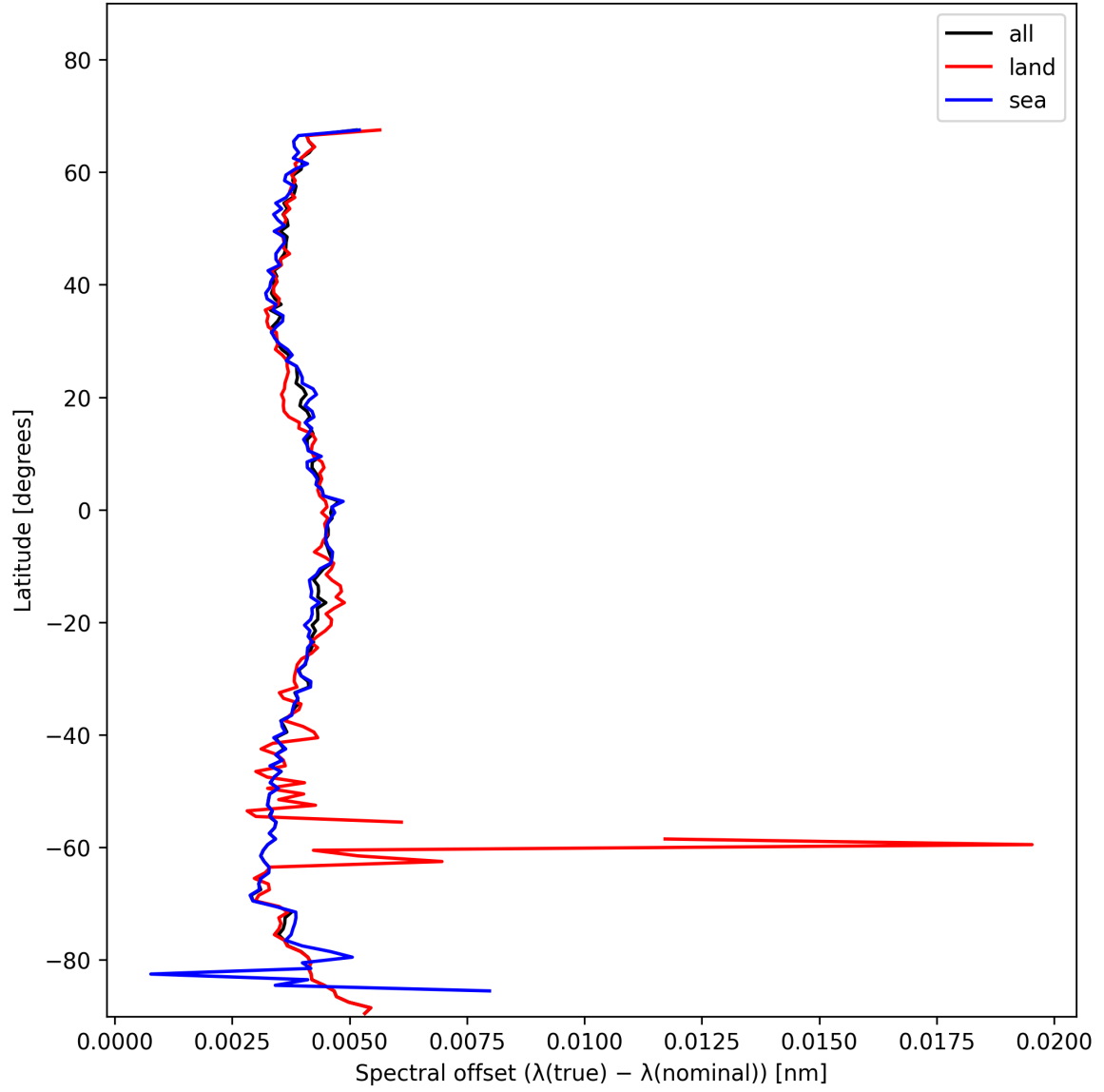
Figure 26: Zonal average of “Spectral offset ( \lambda_{\text{true}} - \lambda_{\text{nominal}} )” for 2025-01-15 to 2025-01-15.
