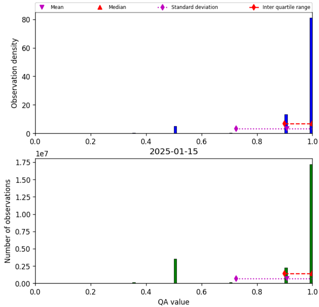
Figure 27: Histogram of “QA value” for 2025-01-15 to 2025-01-15
