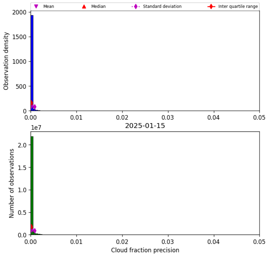
Figure 31: Histogram of “Cloud fraction precision” for 2025-01-15 to 2025-01-15
