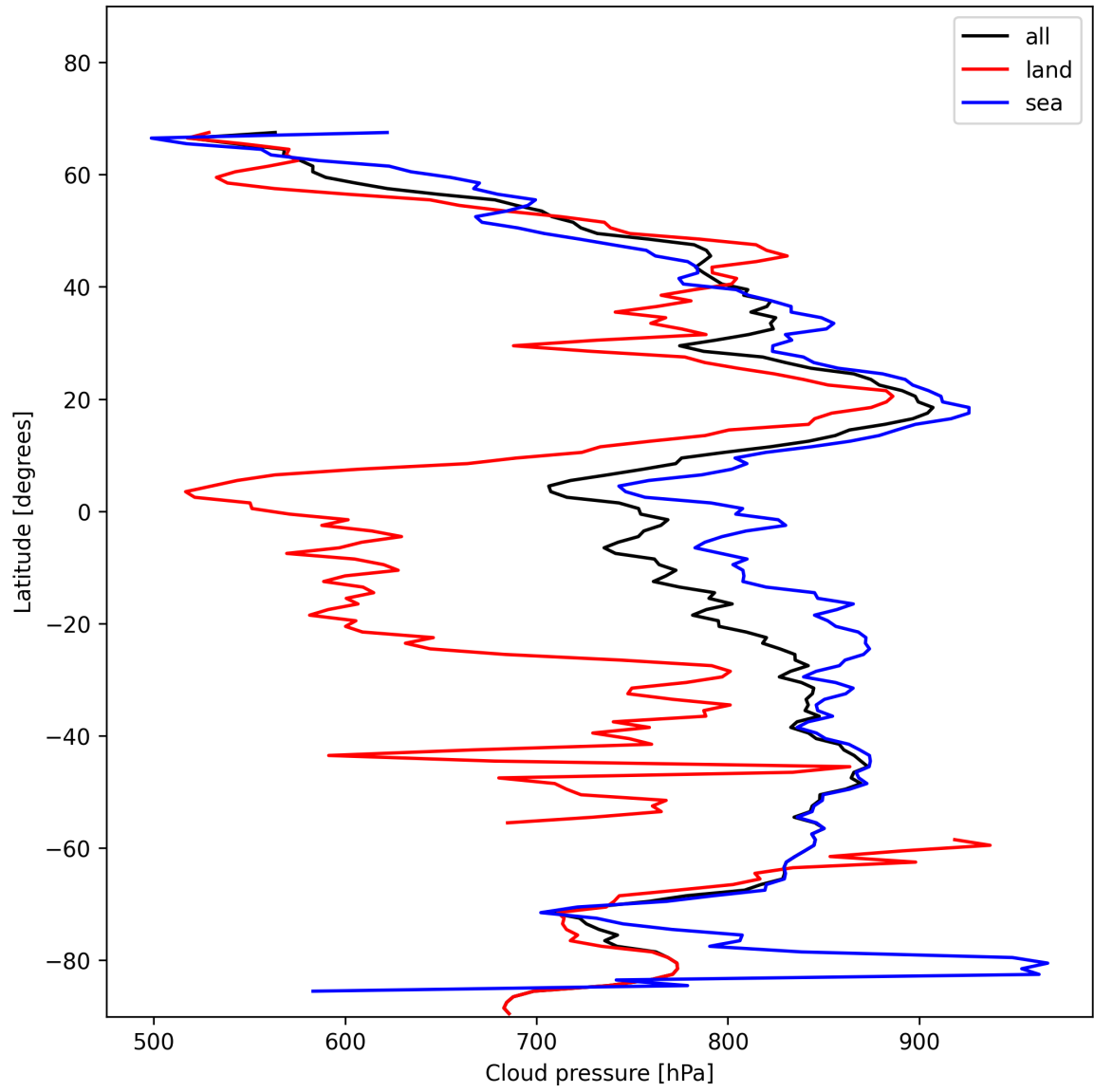
Figure 11: Zonal average of “Cloud pressure” for 2025-01-15 to 2025-01-15.
