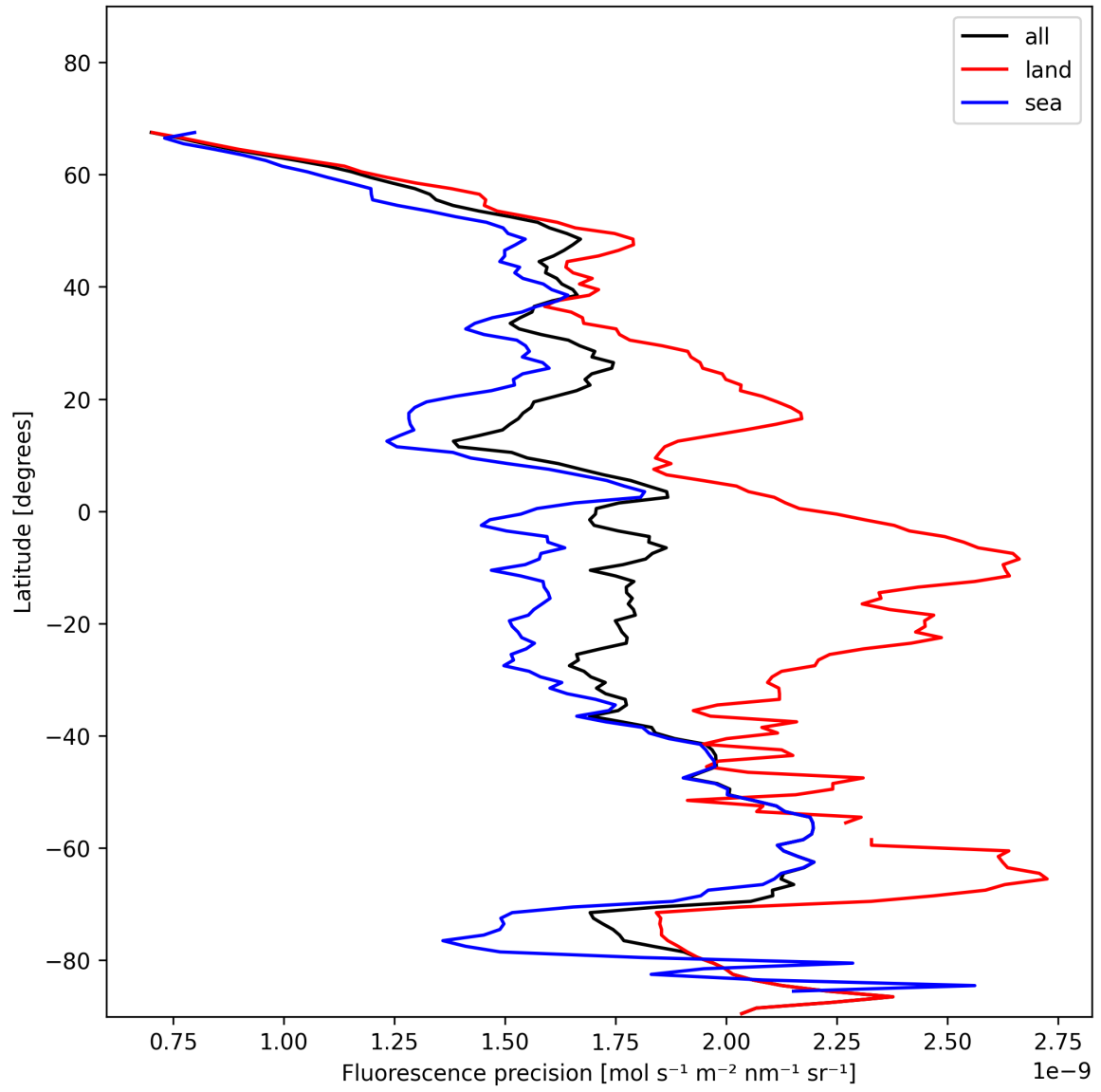
Figure 22: Zonal average of “Fluorescence precision” for 2025-01-15 to 2025-01-15.
