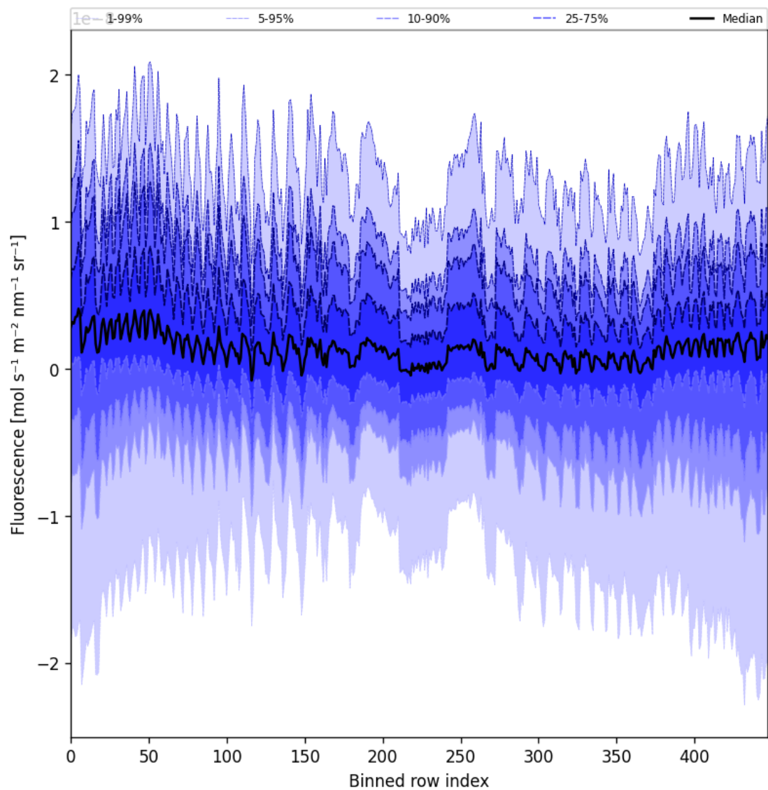
Figure 55: Along track statistics of “Fluorescence” for 2025-01-15 to 2025-01-15
