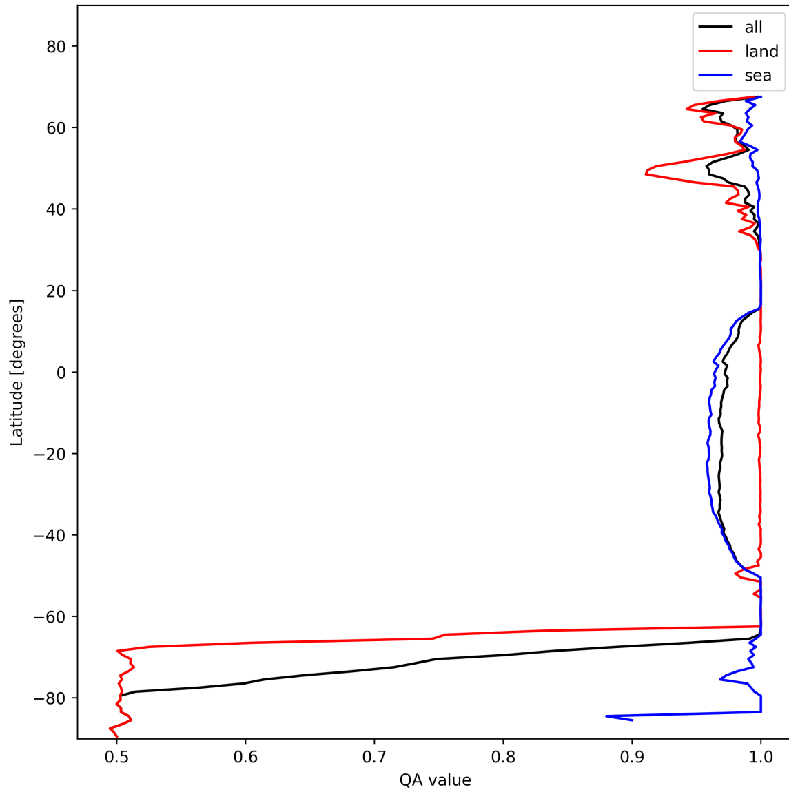
Figure 10: Zonal average of “QA value” for 2025-01-15 to 2025-01-15.
