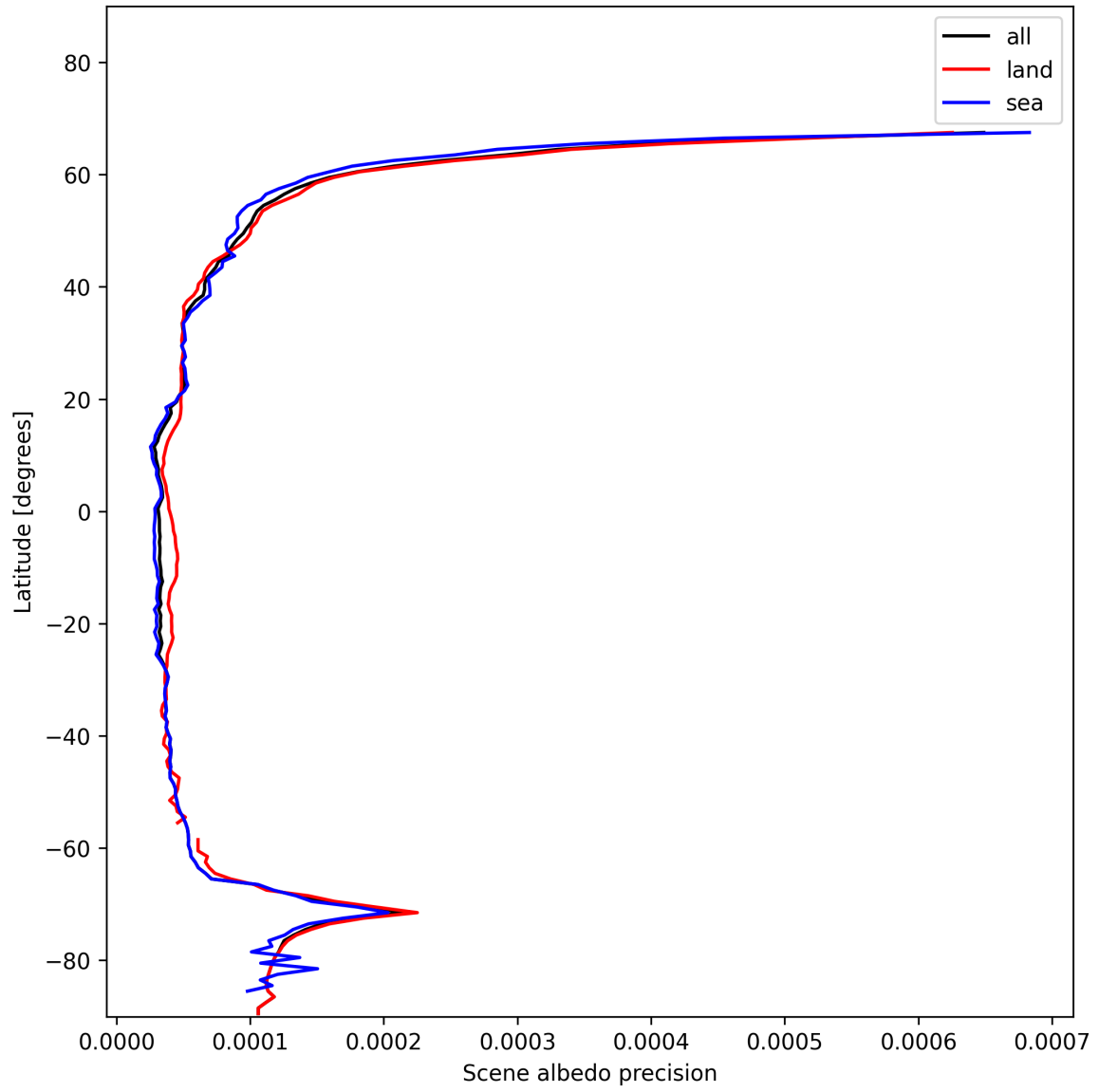
Figure 16: Zonal average of “Scene albedo precision” for 2025-01-15 to 2025-01-15.
