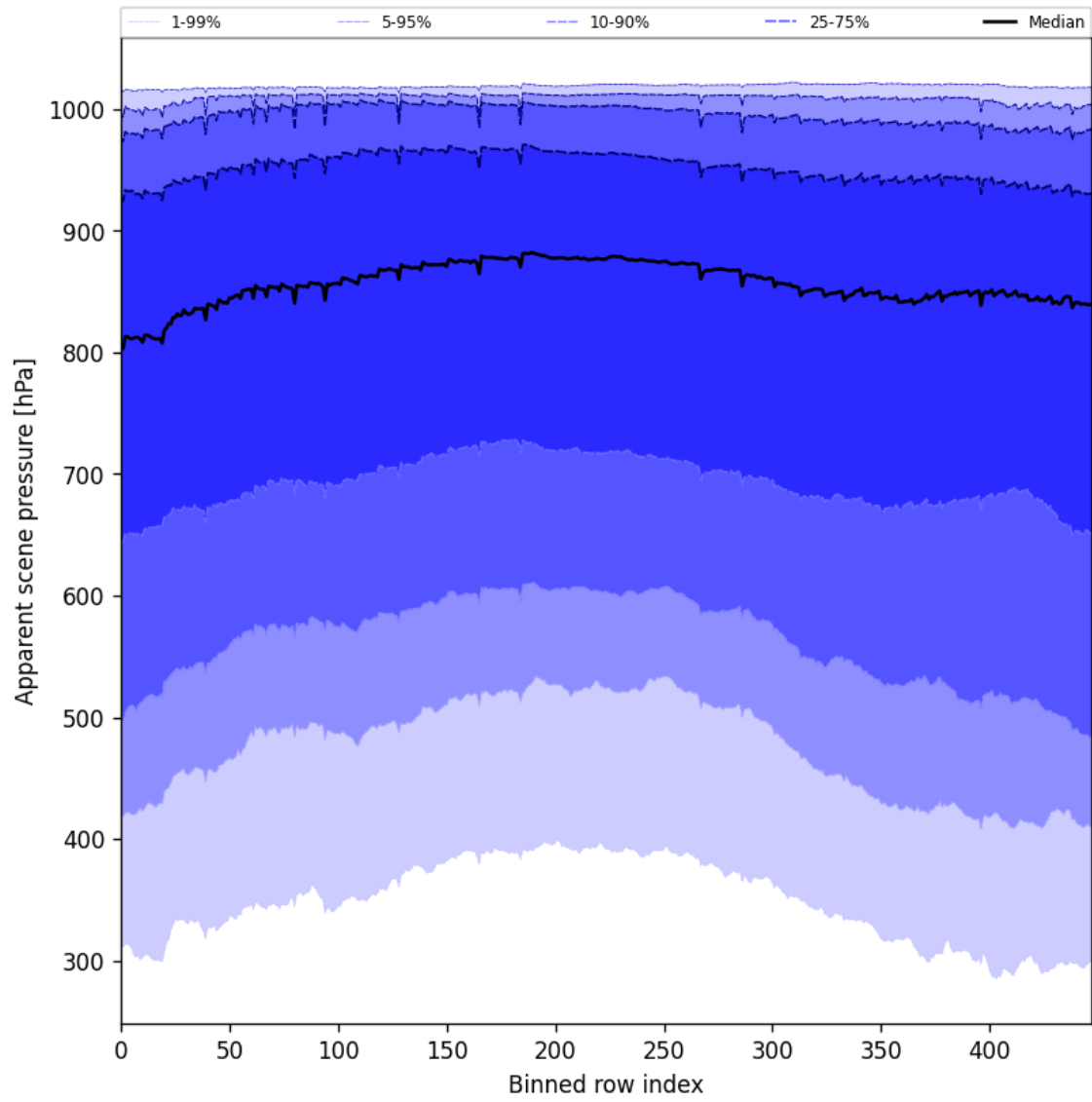
Figure 51: Along track statistics of “Apparent scene pressure” for 2025-01-15 to 2025-01-15
