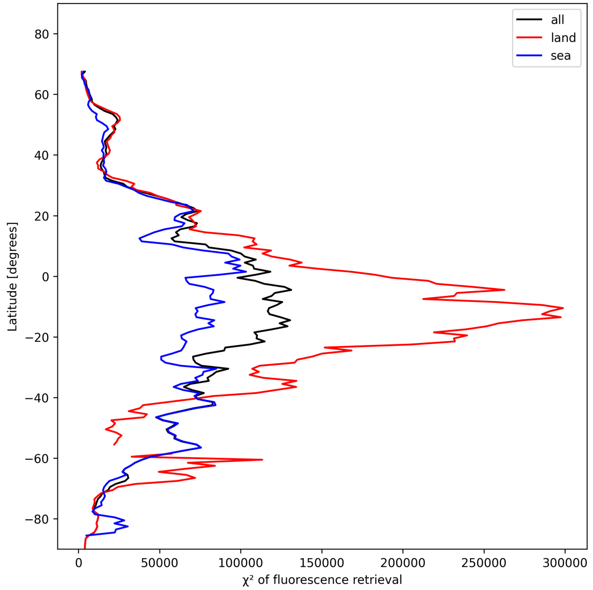
Figure 23: Zonal average of “ \chi^2 of fluorescence retrieval” for 2025-01-15 to 2025-01-15.
