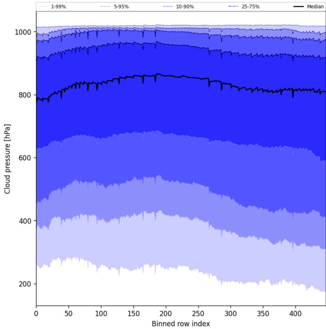
Figure 45: Along track statistics of “Cloud pressure” for 2025-01-15 to 2025-01-15
