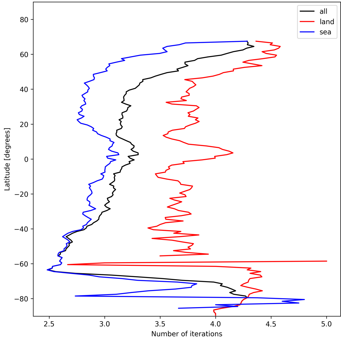
Figure 20: Zonal average of “Number of iterations” for 2025-01-15 to 2025-01-15.
