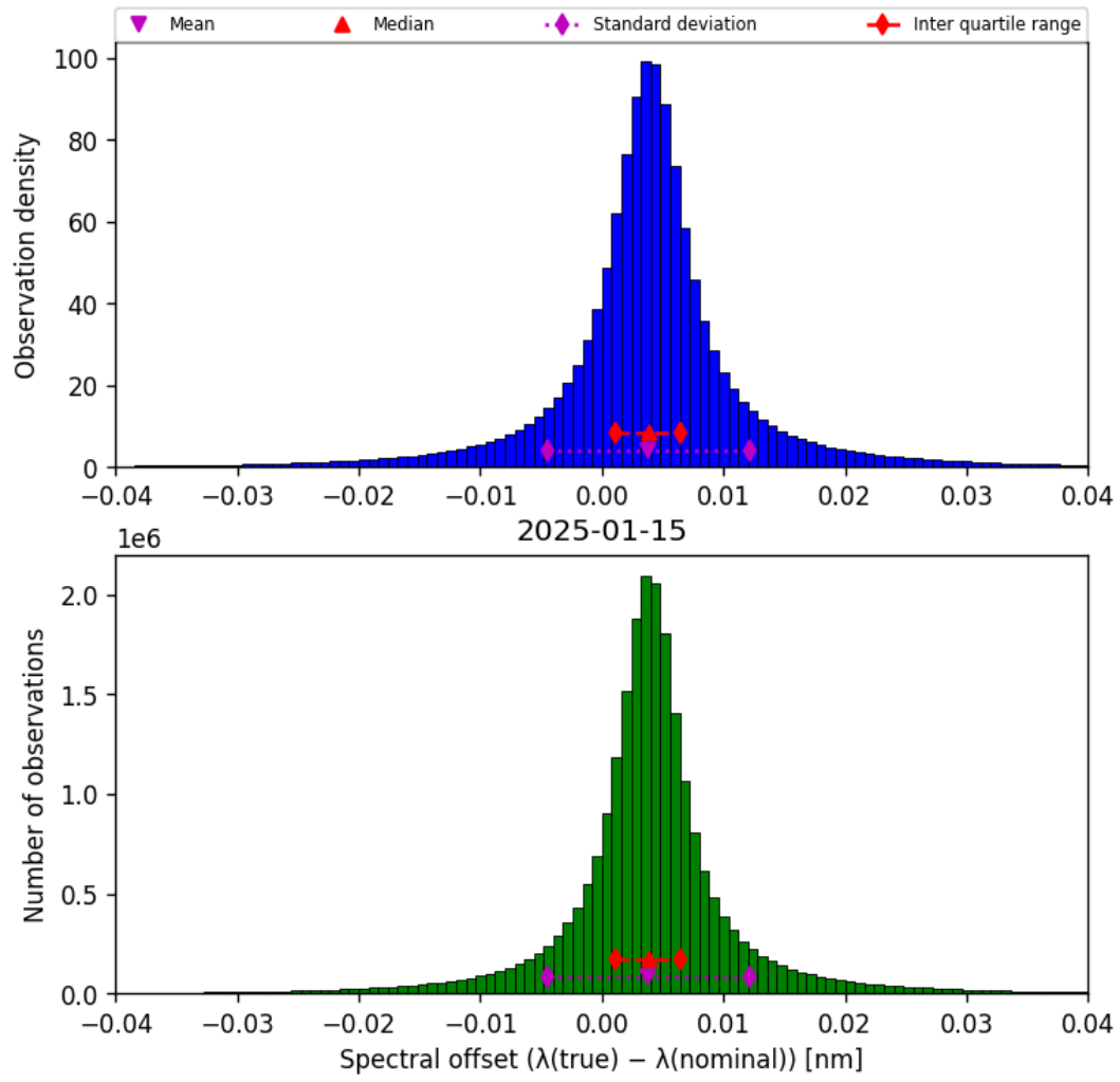
Figure 43: Histogram of “Spectral offset ( \lambda_{\text{true}} - \lambda_{\text{nominal}} )” for 2025-01-15 to 2025-01-15
