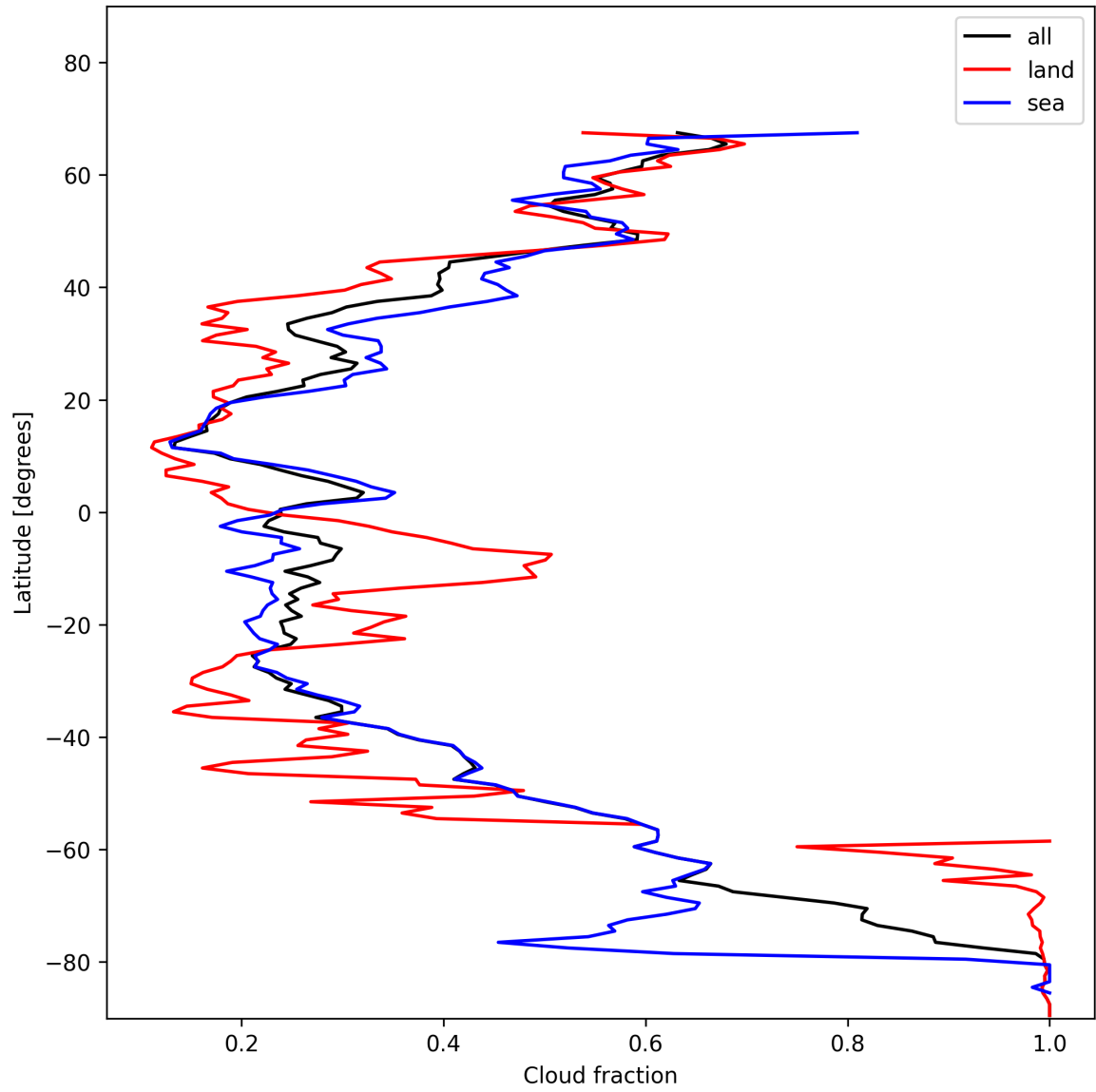
Figure 13: Zonal average of “Cloud fraction” for 2025-01-15 to 2025-01-15.
