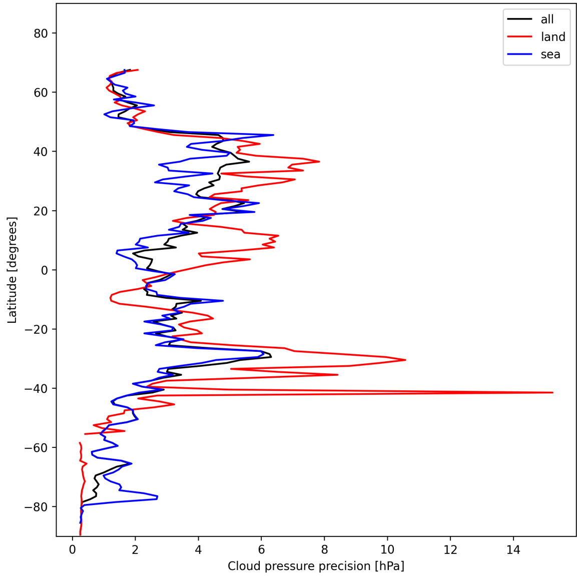
Figure 12: Zonal average of “Cloud pressure precision” for 2025-01-15 to 2025-01-15.
