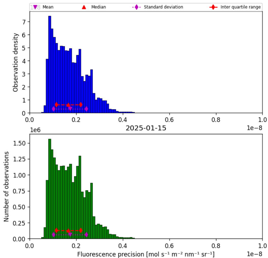
Figure 39: Histogram of “Fluorescence precision” for 2025-01-15 to 2025-01-15
