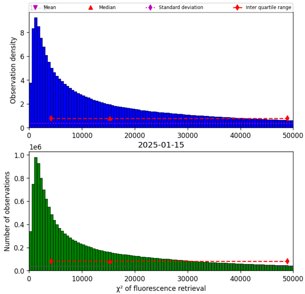
Figure 40: Histogram of “ \chi^2 of fluorescence retrieval” for 2025-01-15 to 2025-01-15
