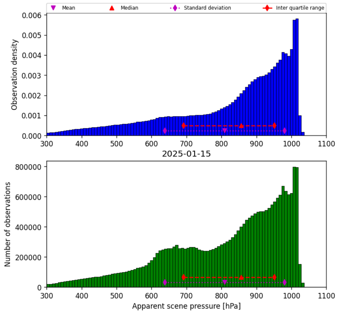
Figure 34: Histogram of “Apparent scene pressure” for 2025-01-15 to 2025-01-15
