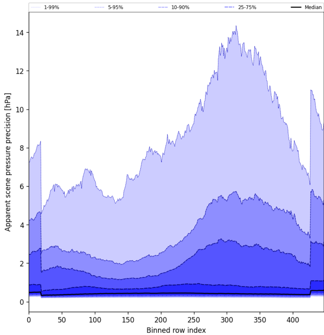
Figure 52: Along track statistics of “Apparent scene pressure precision” for 2025-01-15 to 2025-01-15
