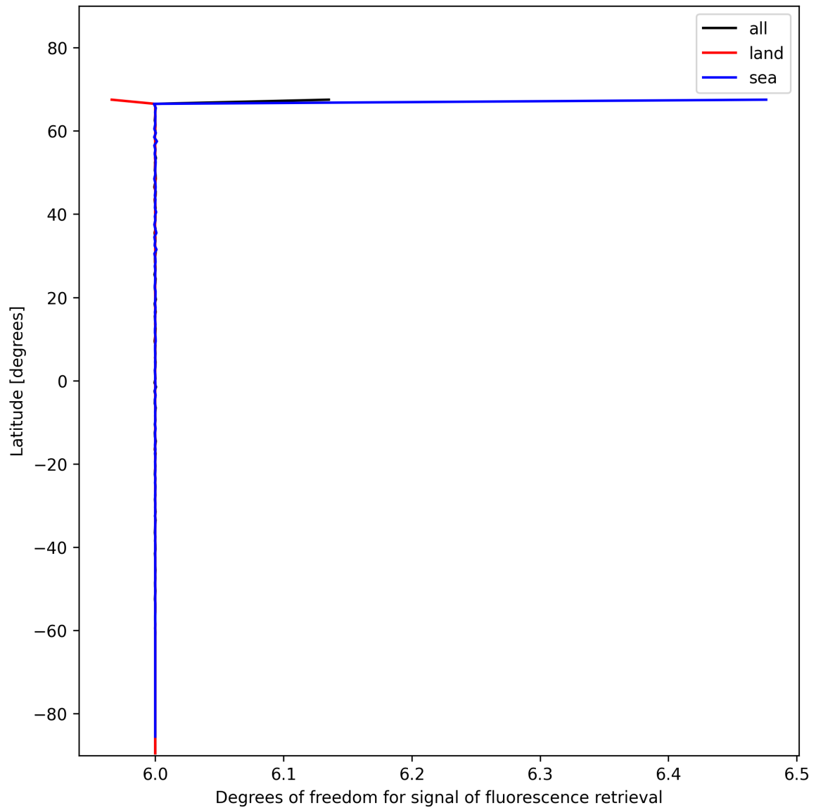
Figure 24: Zonal average of “Degrees of freedom for signal of fluorescence retrieval” for 2025-01-15 to 2025-01-15.
