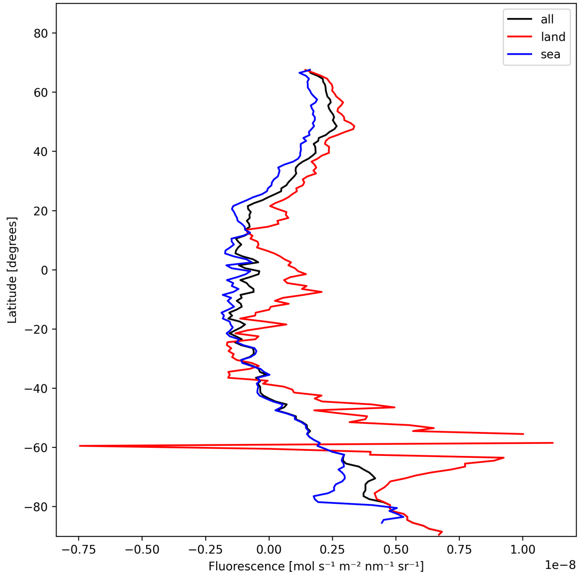
Figure 21: Zonal average of “Fluorescence” for 2025-01-15 to 2025-01-15.
