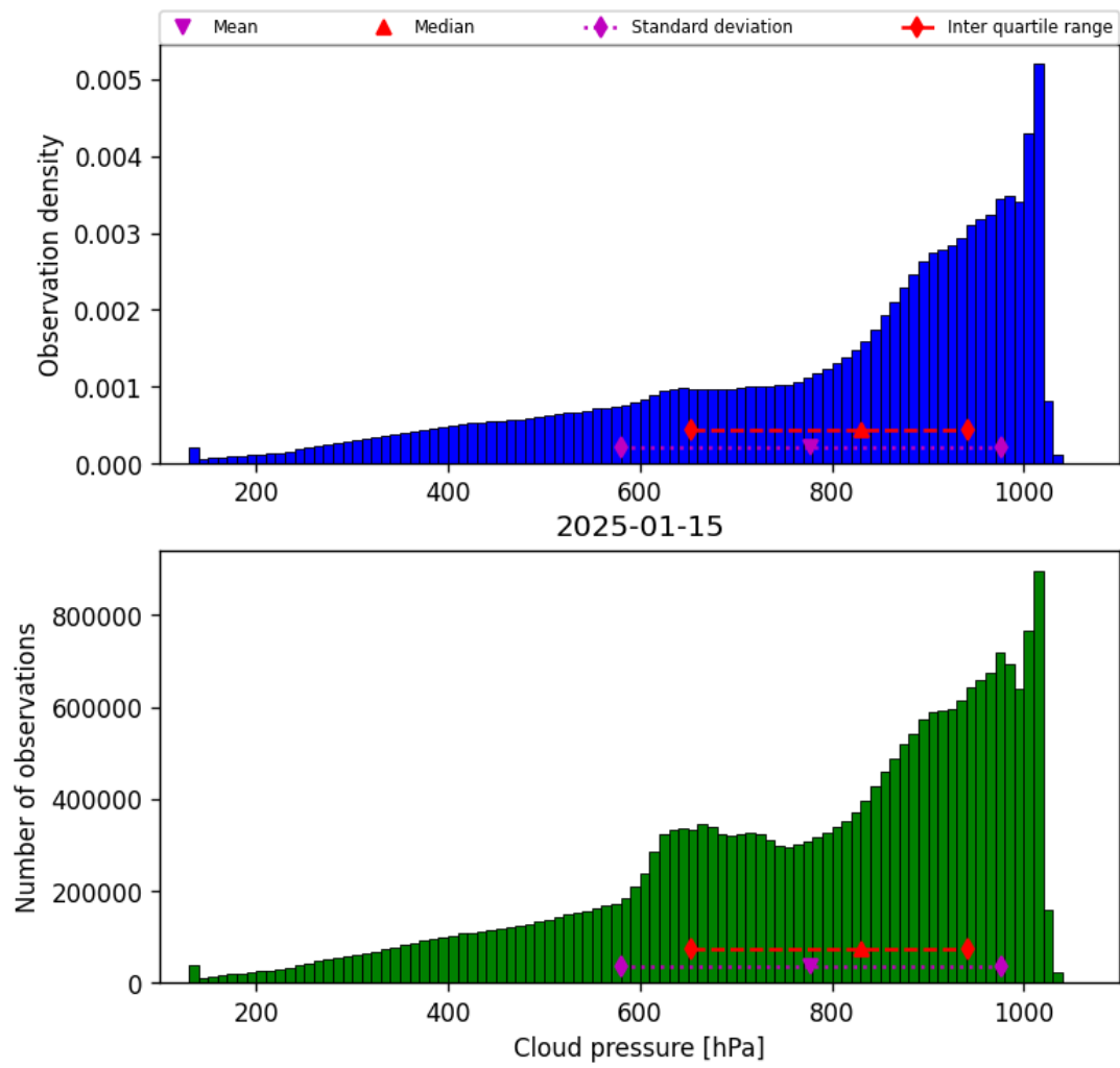
Figure 28: Histogram of “Cloud pressure” for 2025-01-15 to 2025-01-15
