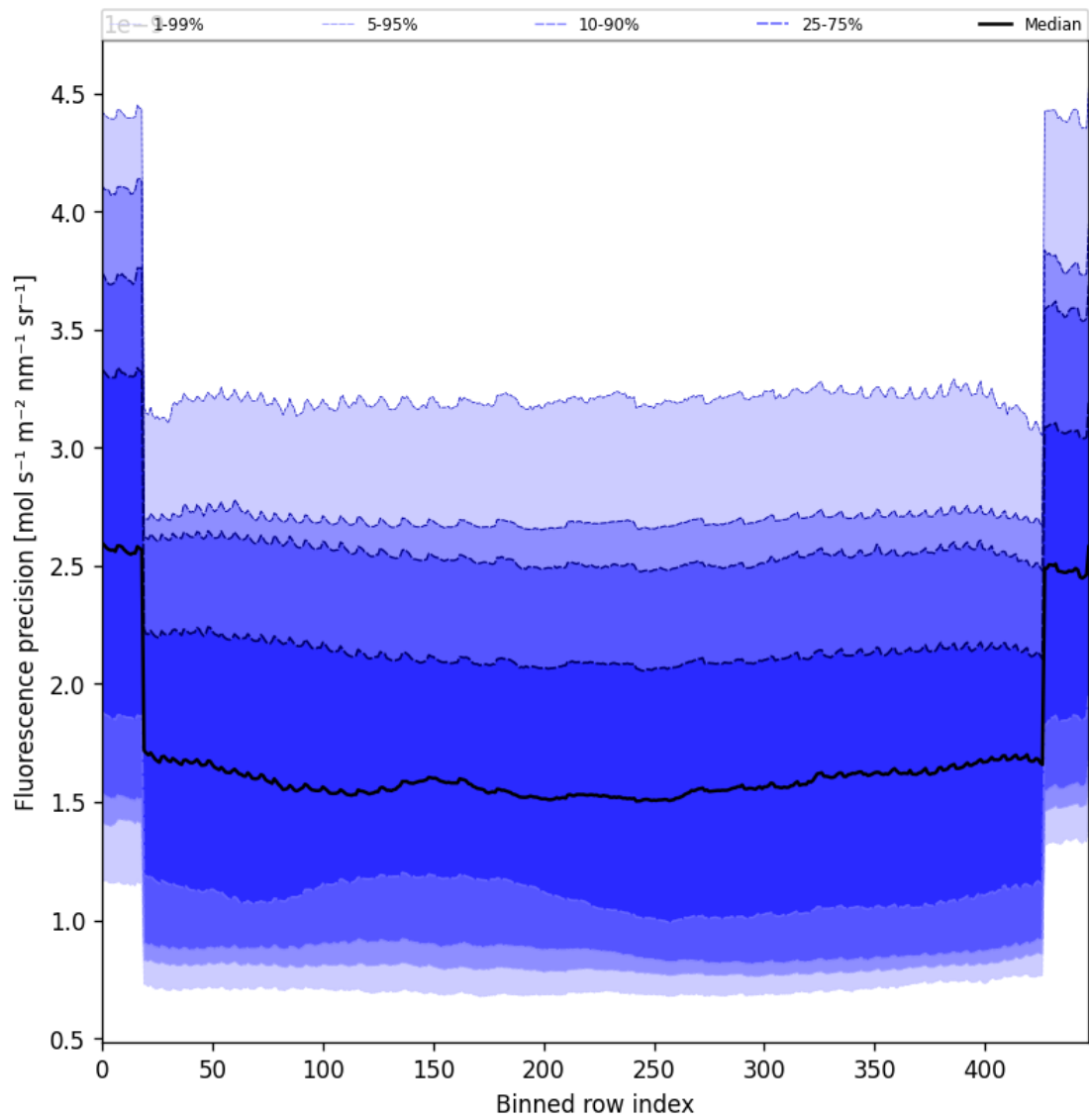
Figure 56: Along track statistics of “Fluorescence precision” for 2025-01-15 to 2025-01-15
