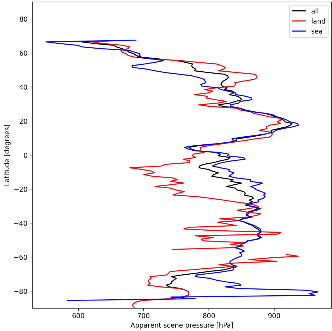
Figure 17: Zonal average of “Apparent scene pressure” for 2025-01-15 to 2025-01-15.
