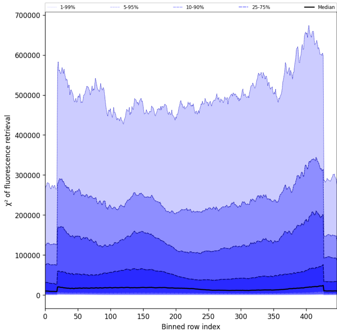
Figure 57: Along track statistics of “ \chi^2 of fluorescence retrieval” for 2025-01-15 to 2025-01-15
