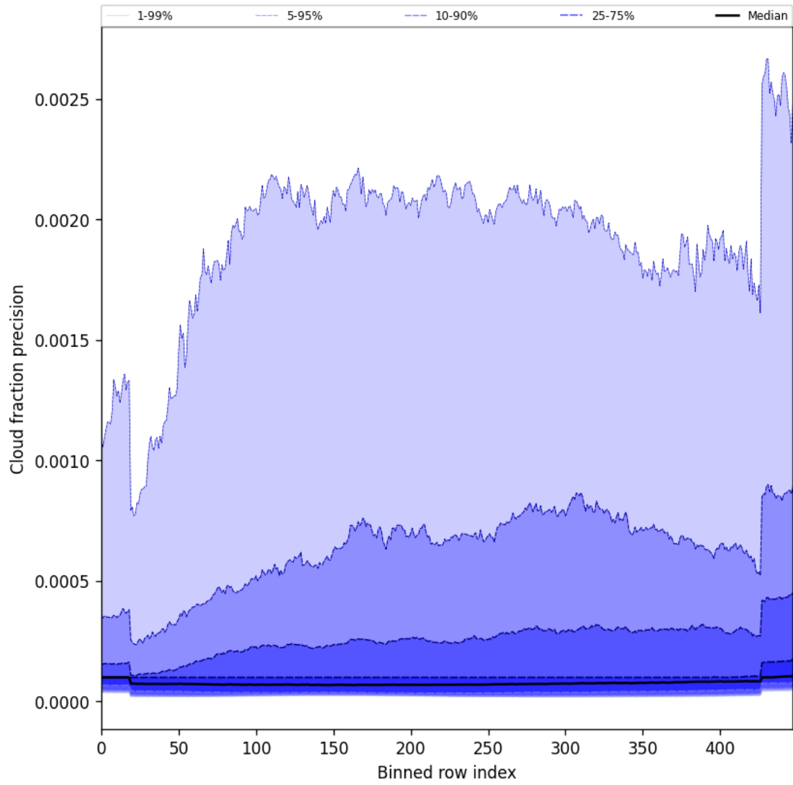
Figure 48: Along track statistics of “Cloud fraction precision” for 2025-01-15 to 2025-01-15
