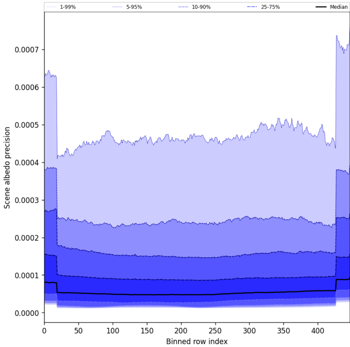
Figure 50: Along track statistics of “Scene albedo precision” for 2025-01-15 to 2025-01-15
