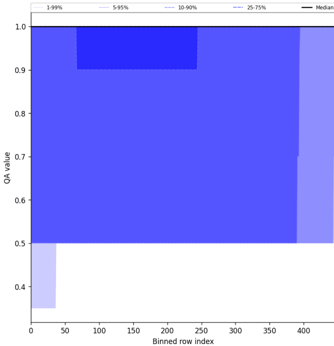
Figure 44: Along track statistics of “QA value” for 2025-01-15 to 2025-01-15
