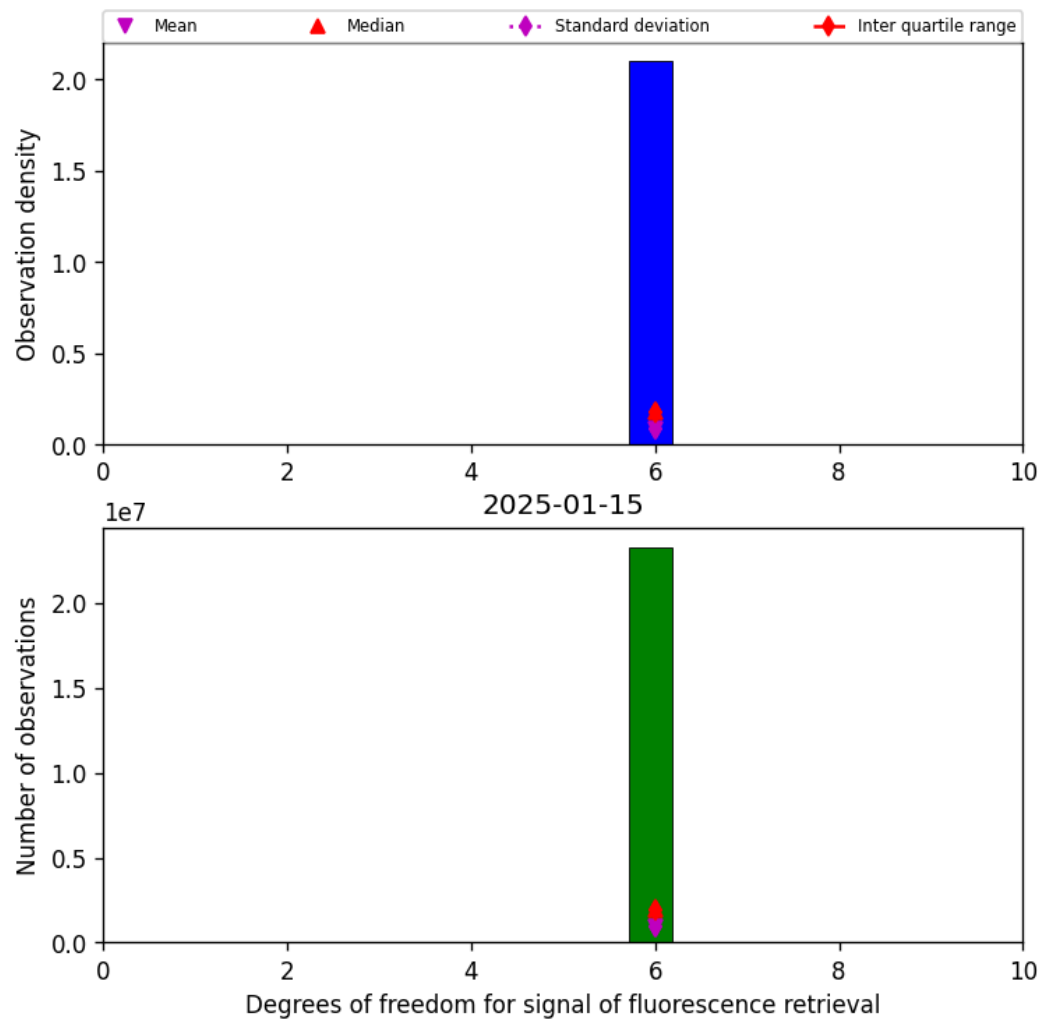
Figure 41: Histogram of “Degrees of freedom for signal of fluorescence retrieval” for 2025-01-15 to 2025-01-15
