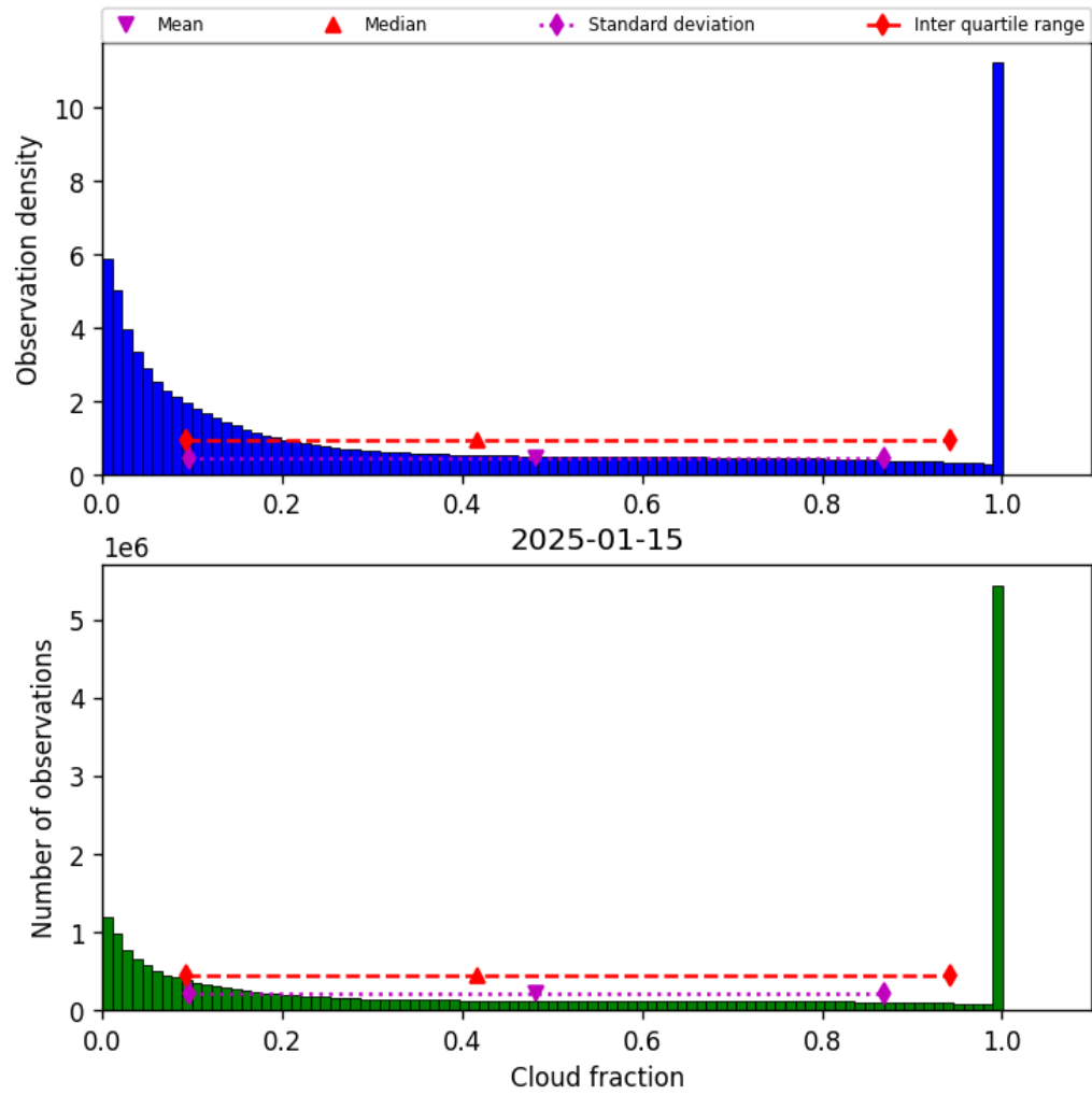
Figure 30: Histogram of "Cloud fraction" for 2025-01-15 to 2025-01-15
