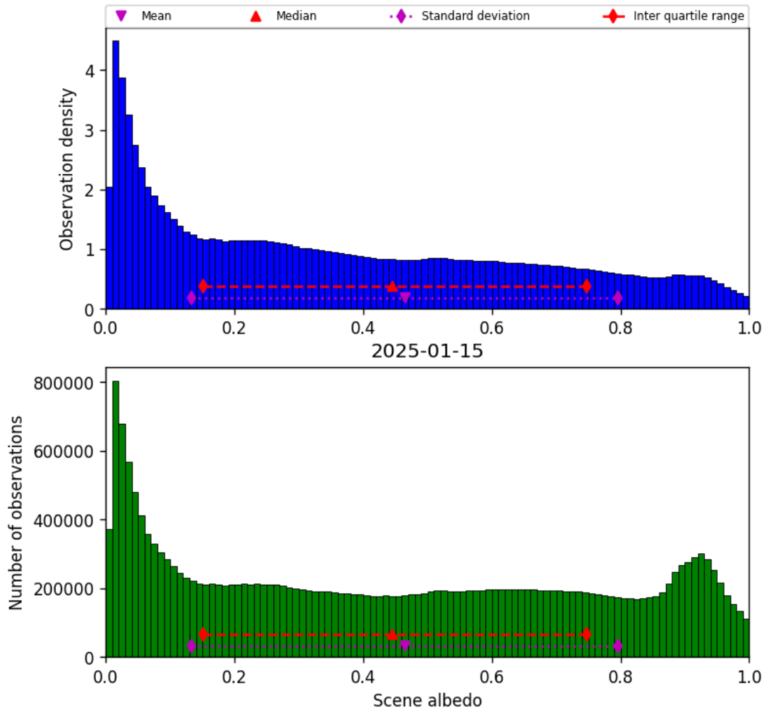
Figure 32: Histogram of “Scene albedo” for 2025-01-15 to 2025-01-15
