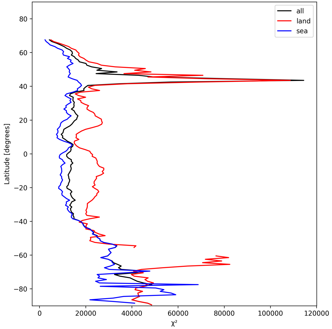
Figure 19: Zonal average of “ \chi^2 ” for 2025-01-16 to 2025-01-17.
