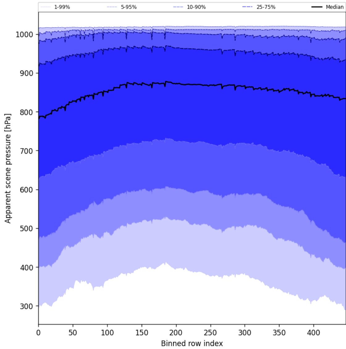
Figure 51: Along track statistics of “Apparent scene pressure” for 2025-01-16 to 2025-01-17
