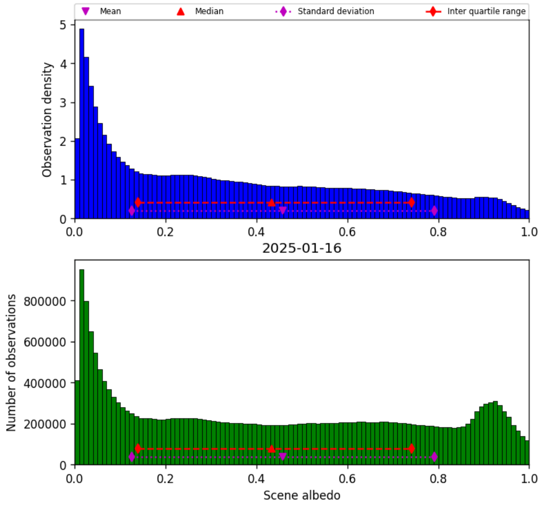
Figure 32: Histogram of “Scene albedo” for 2025-01-16 to 2025-01-17
