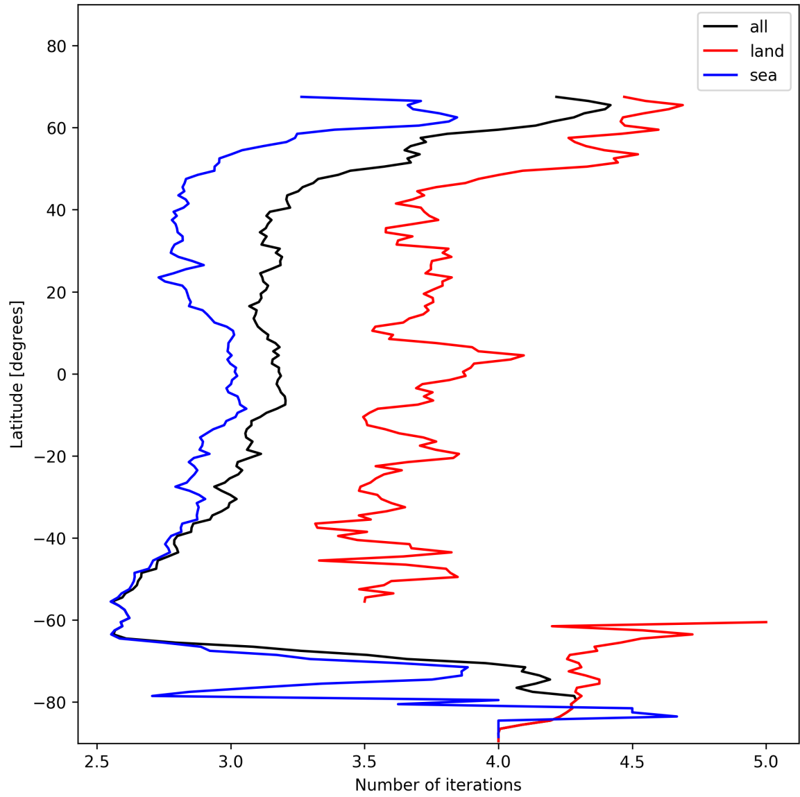
Figure 20: Zonal average of “Number of iterations” for 2025-01-16 to 2025-01-17.
