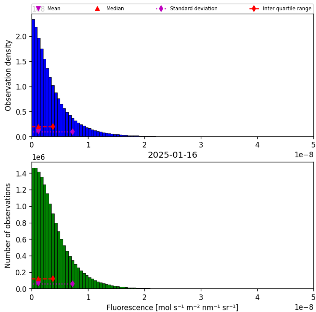
Figure 38: Histogram of “Fluorescence” for 2025-01-16 to 2025-01-17
