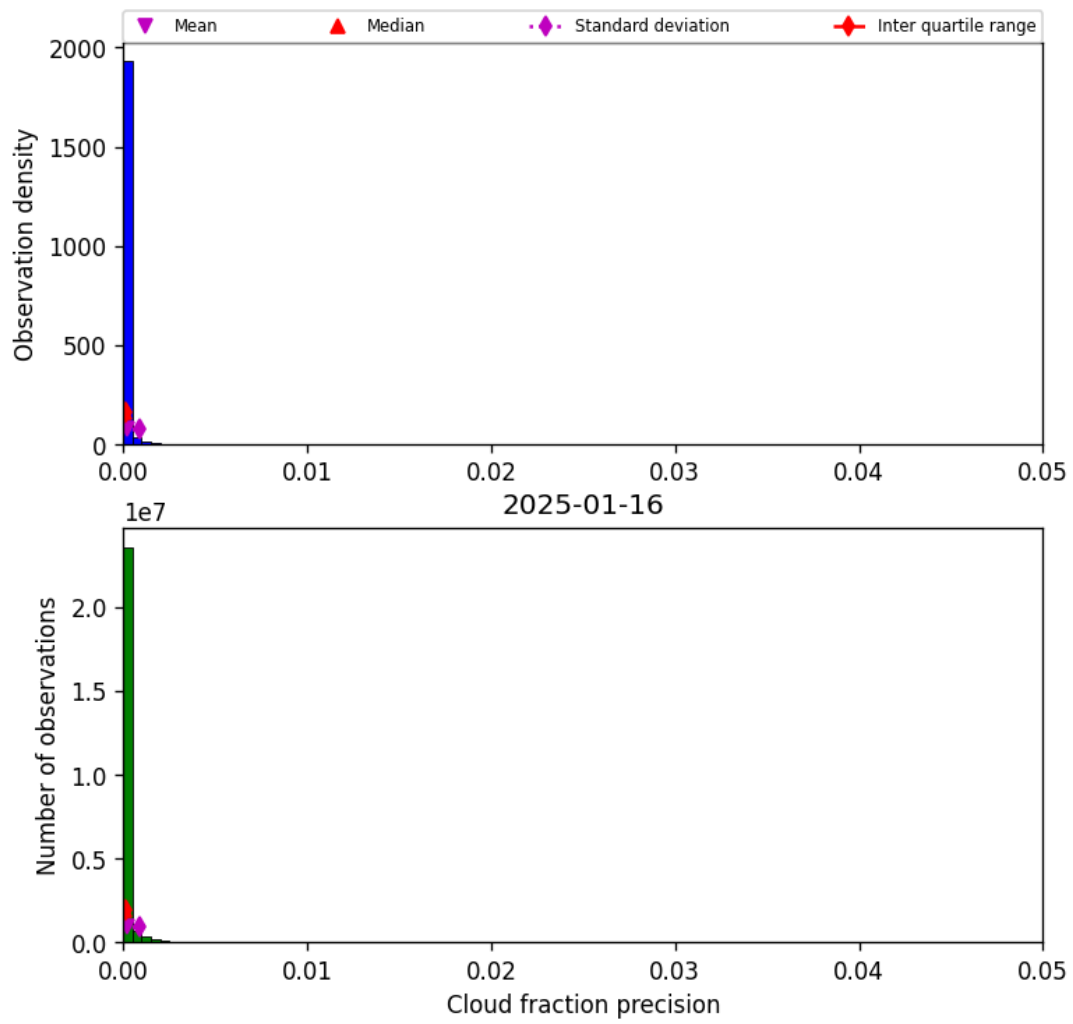
Figure 31: Histogram of “Cloud fraction precision” for 2025-01-16 to 2025-01-17
