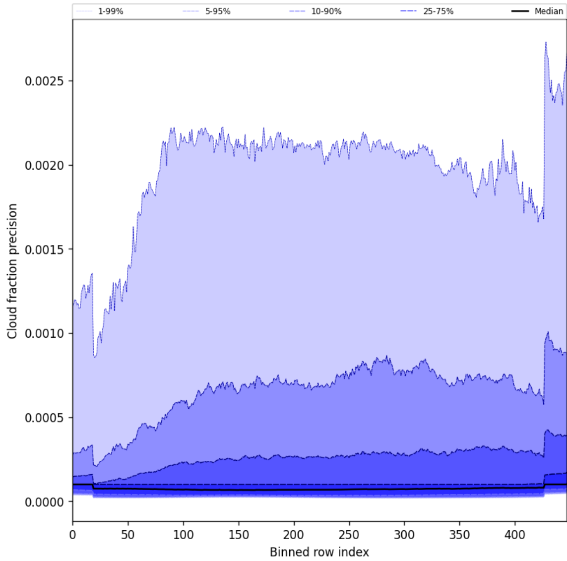
Figure 48: Along track statistics of “Cloud fraction precision” for 2025-01-16 to 2025-01-17
