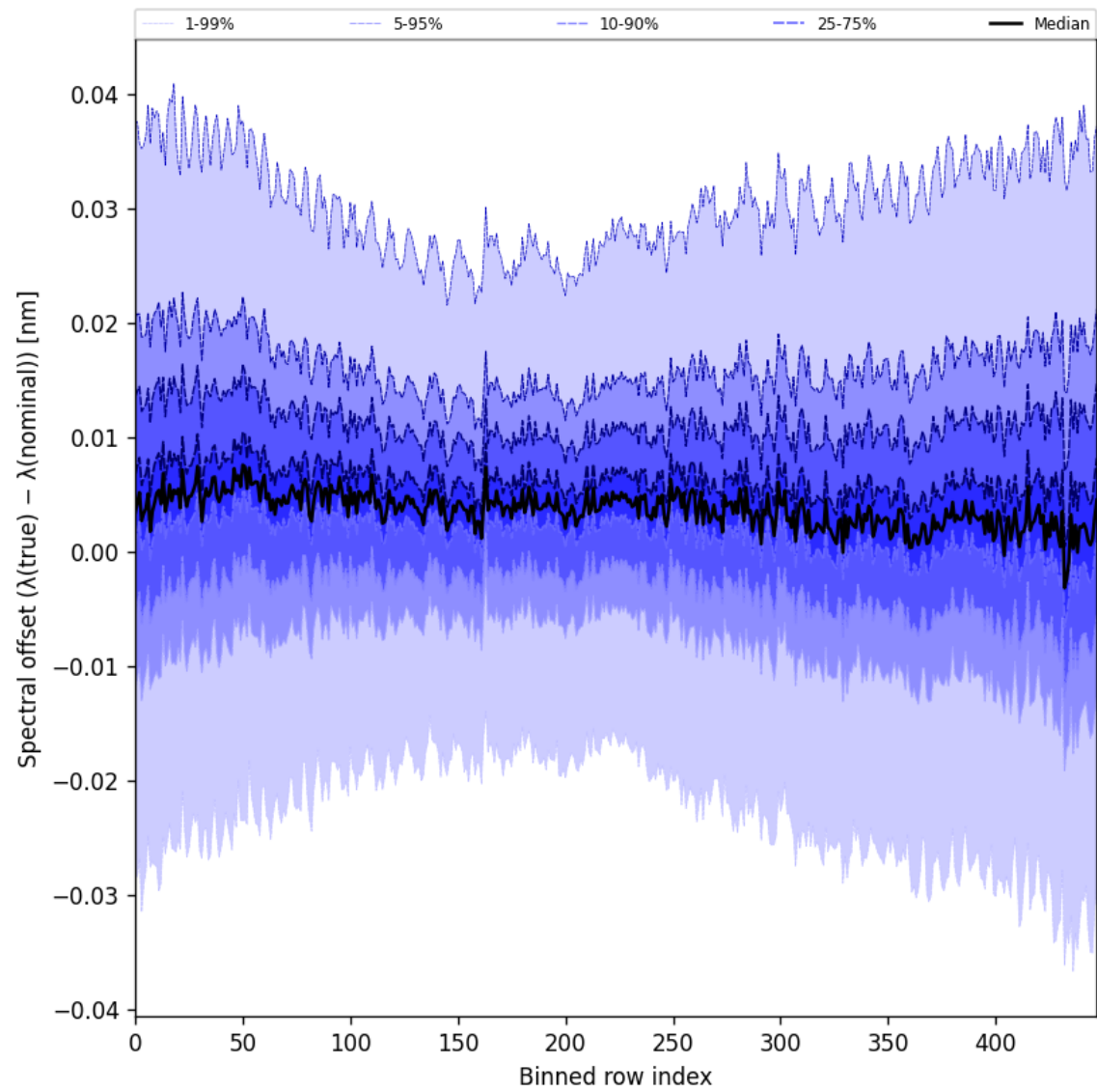
Figure 60: Along track statistics of “Spectral offset ( \lambda_{\text{true}} - \lambda_{\text{nominal}} )” for 2025-01-16 to 2025-01-17
