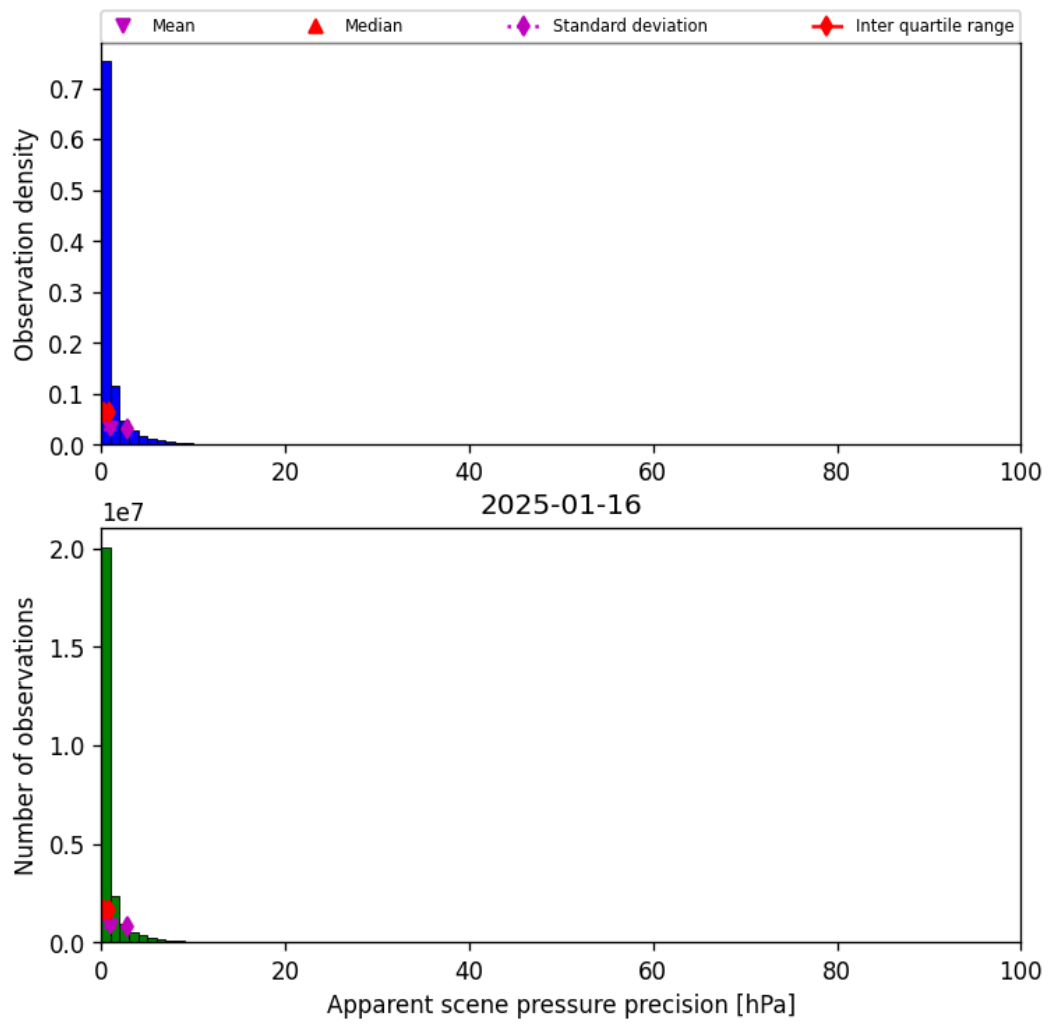
Figure 35: Histogram of “Apparent scene pressure precision” for 2025-01-16 to 2025-01-17
