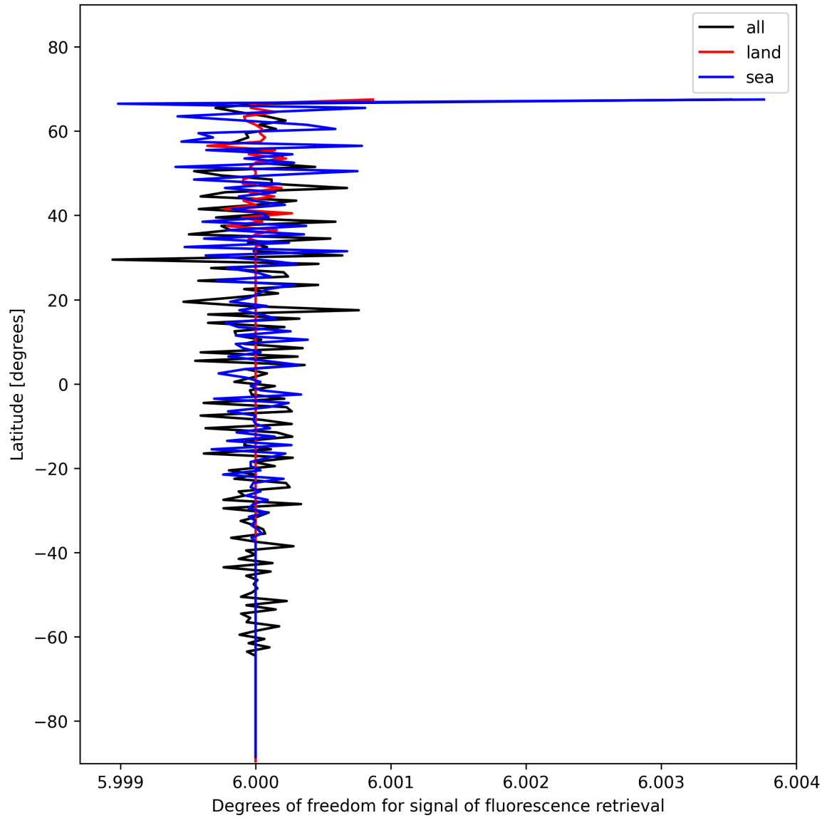
Figure 24: Zonal average of “Degrees of freedom for signal of fluorescence retrieval” for 2025-01-16 to 2025-01-17.
