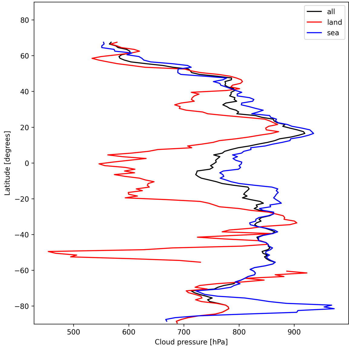
Figure 11: Zonal average of “Cloud pressure” for 2025-01-16 to 2025-01-17.
