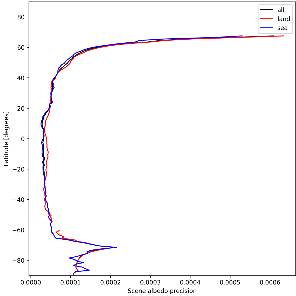
Figure 16: Zonal average of “Scene albedo precision” for 2025-01-16 to 2025-01-17.
