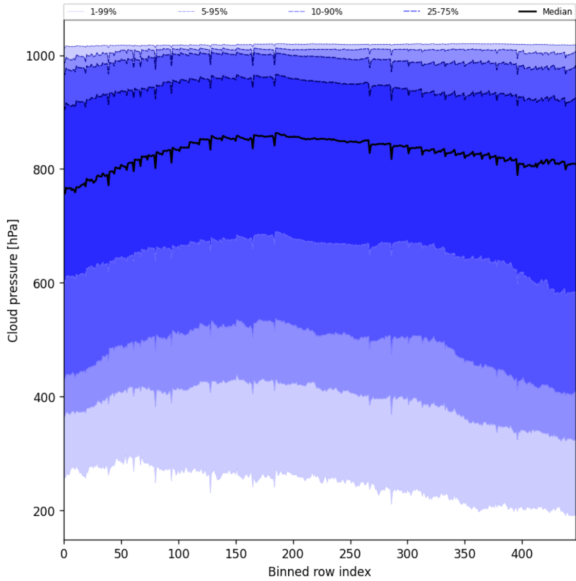
Figure 45: Along track statistics of “Cloud pressure” for 2025-01-16 to 2025-01-17
