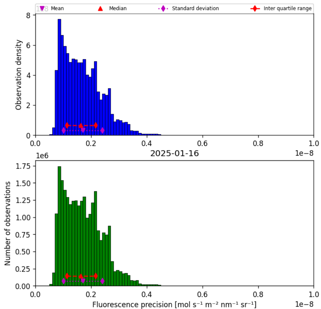
Figure 39: Histogram of “Fluorescence precision” for 2025-01-16 to 2025-01-17
