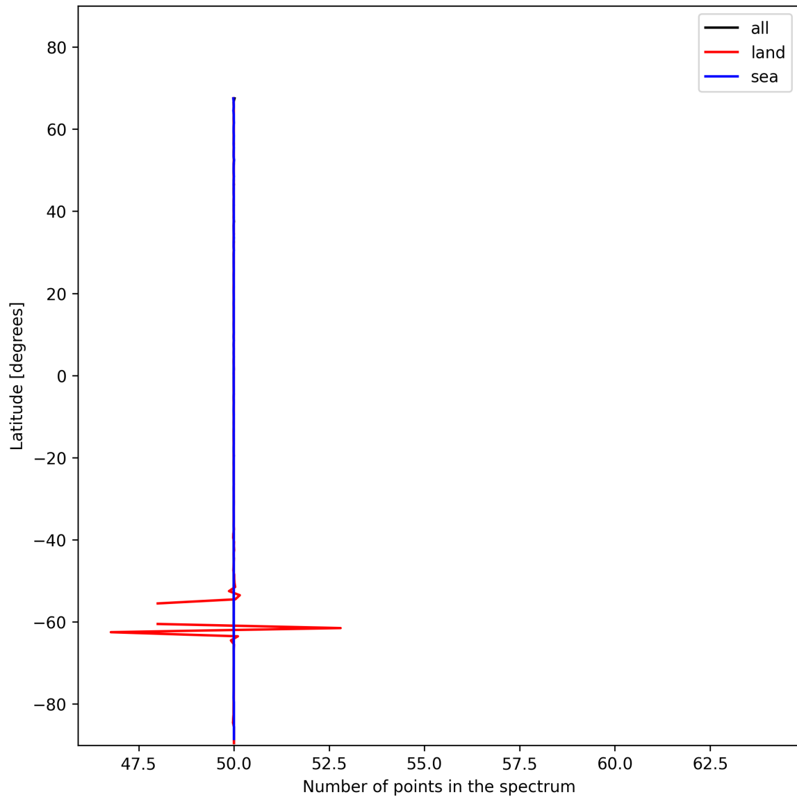
Figure 25: Zonal average of “Number of points in the spectrum” for 2025-01-16 to 2025-01-17.
