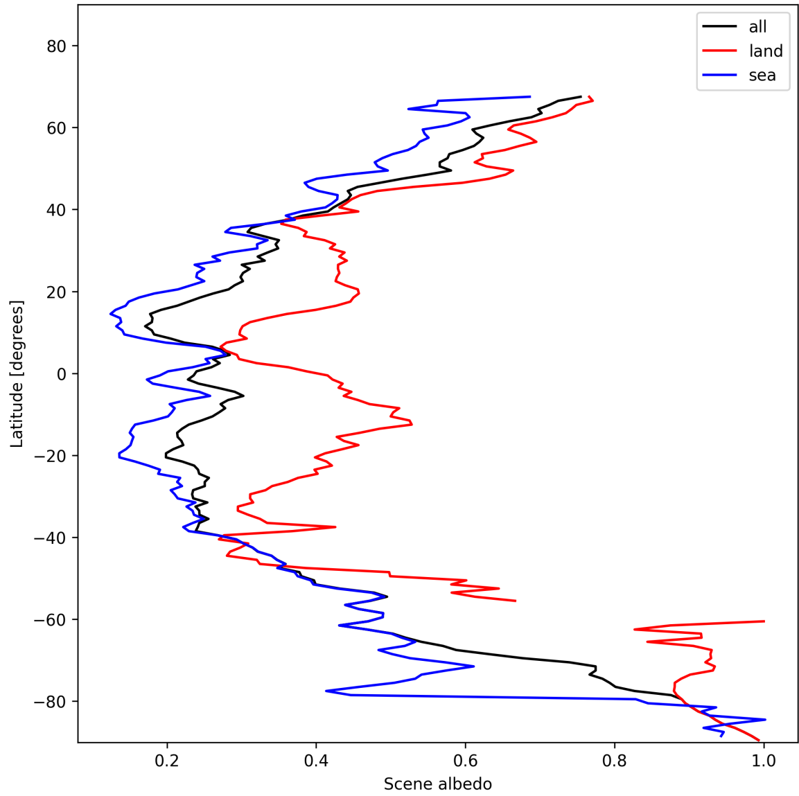
Figure 15: Zonal average of “Scene albedo” for 2025-01-16 to 2025-01-17.
