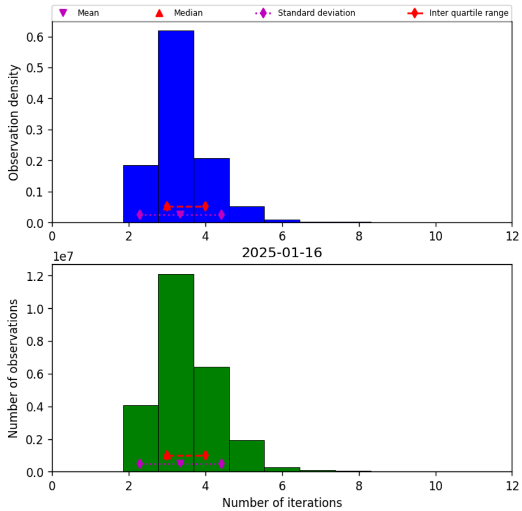
Figure 37: Histogram of “Number of iterations” for 2025-01-16 to 2025-01-17
