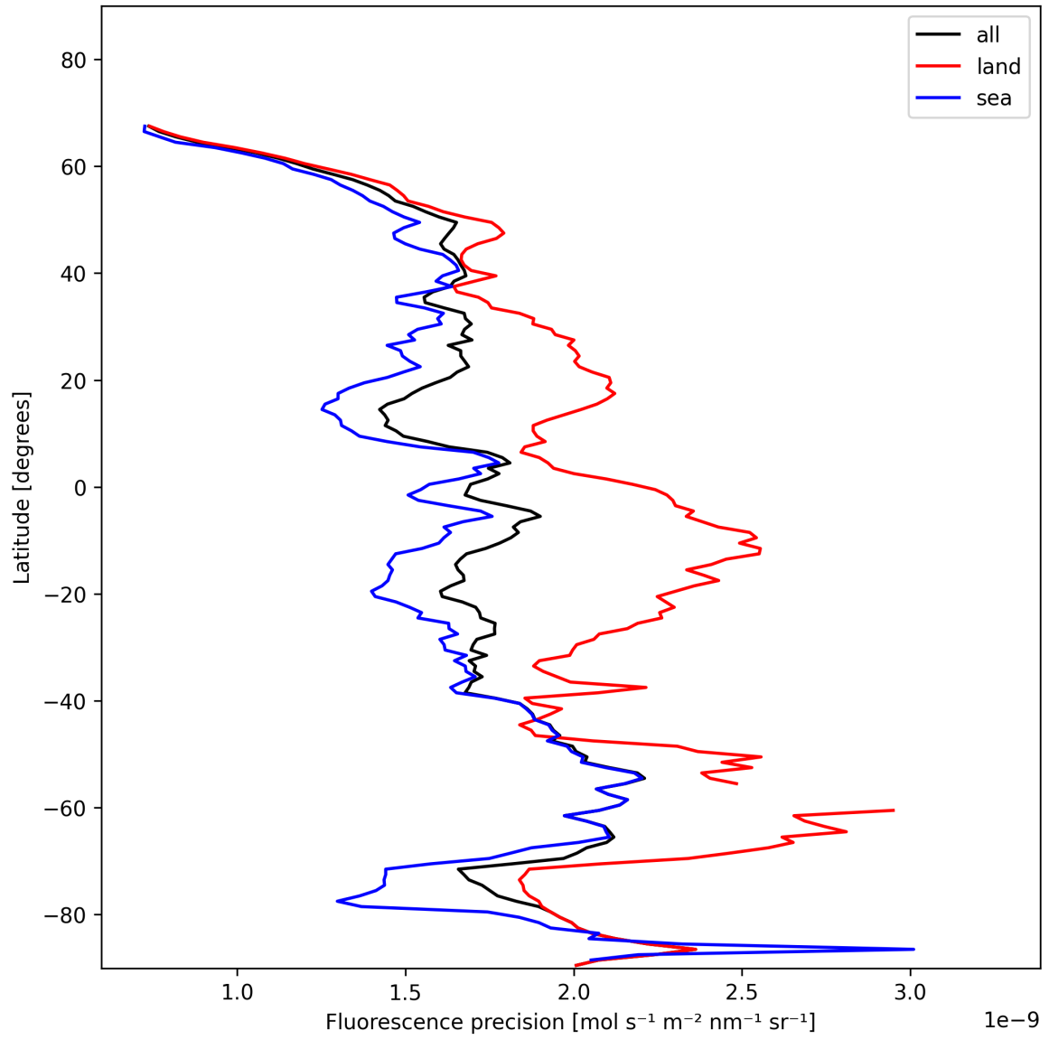
Figure 22: Zonal average of “Fluorescence precision” for 2025-01-16 to 2025-01-17.
