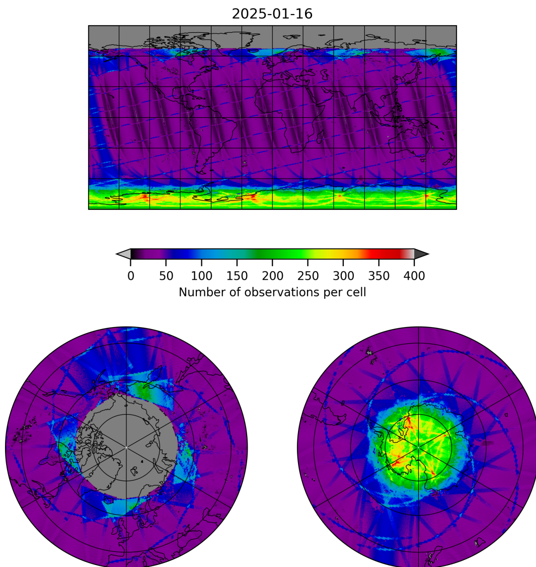
Figure 9: Map of the number of observations for 2025-01-16 to 2025-01-17
