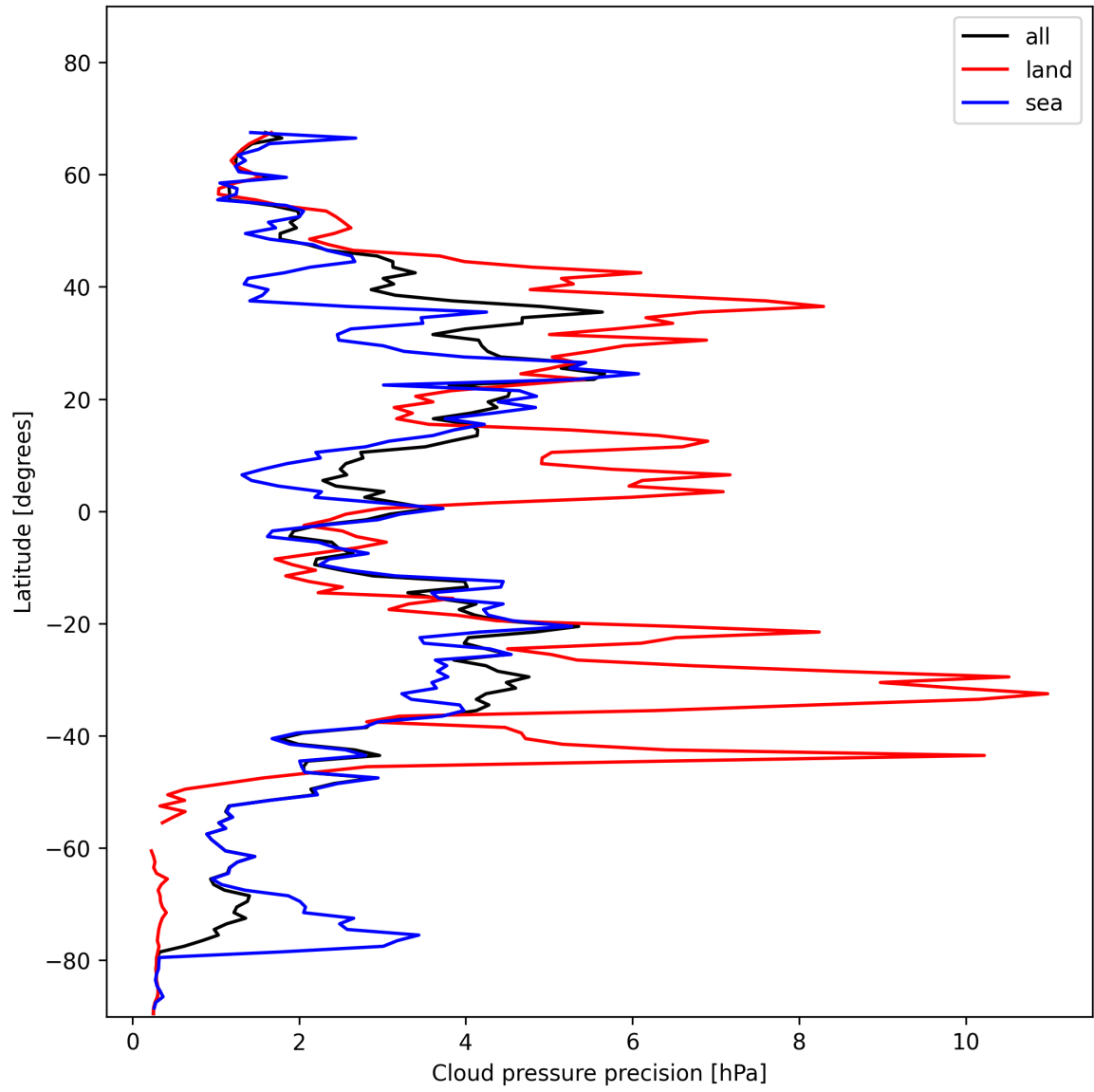
Figure 12: Zonal average of “Cloud pressure precision” for 2025-01-16 to 2025-01-17.
