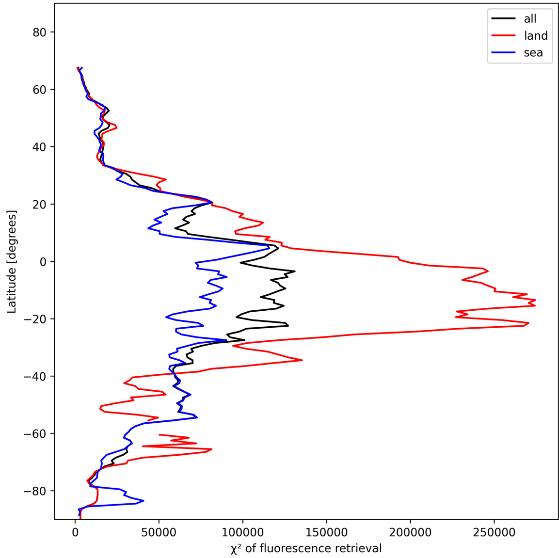
Figure 23: Zonal average of “ \chi^2 of fluorescence retrieval” for 2025-01-16 to 2025-01-17.
