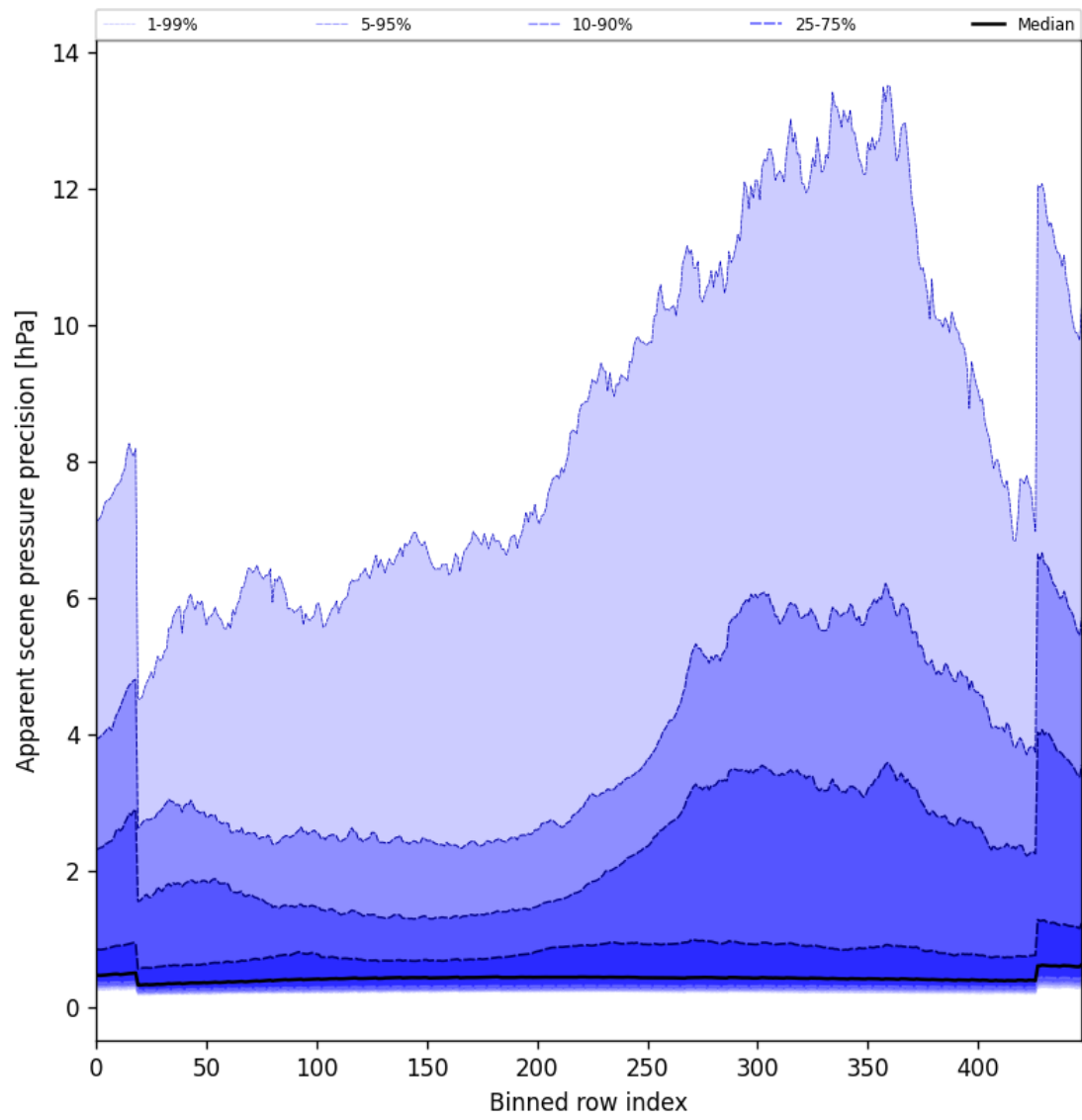
Figure 52: Along track statistics of “Apparent scene pressure precision” for 2025-01-16 to 2025-01-17
