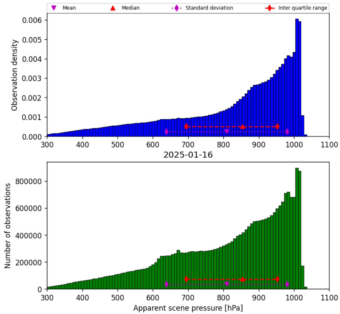
Figure 34: Histogram of “Apparent scene pressure” for 2025-01-16 to 2025-01-17
