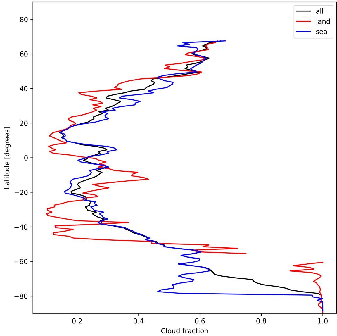
Figure 13: Zonal average of “Cloud fraction” for 2025-01-16 to 2025-01-17.
