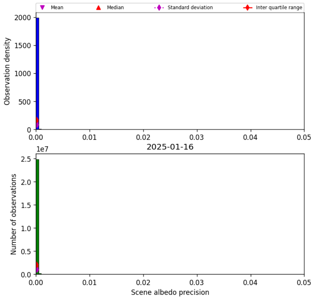
Figure 33: Histogram of “Scene albedo precision” for 2025-01-16 to 2025-01-17
