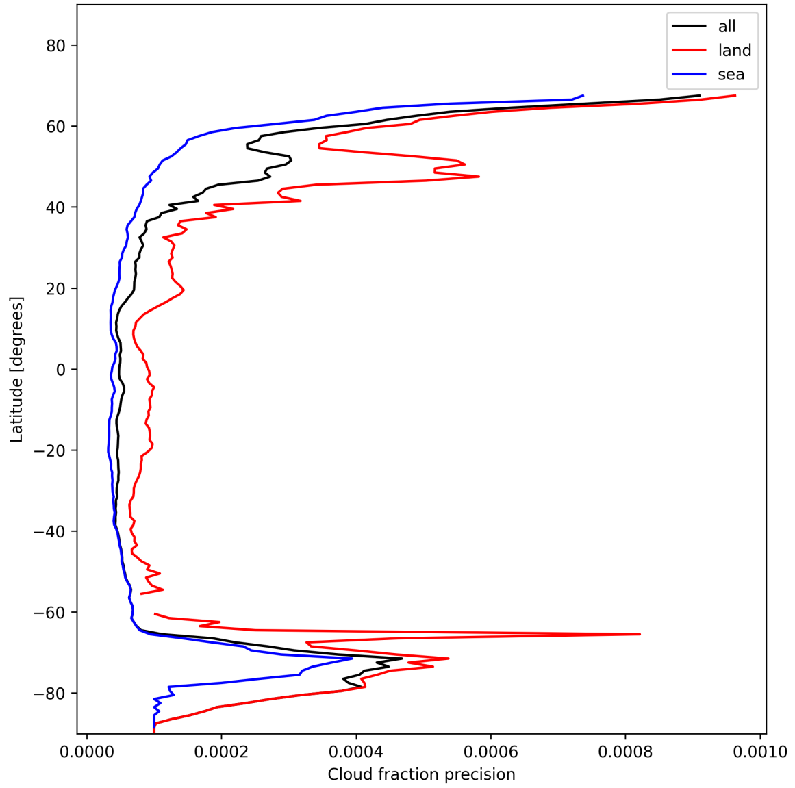
Figure 14: Zonal average of “Cloud fraction precision” for 2025-01-16 to 2025-01-17.
