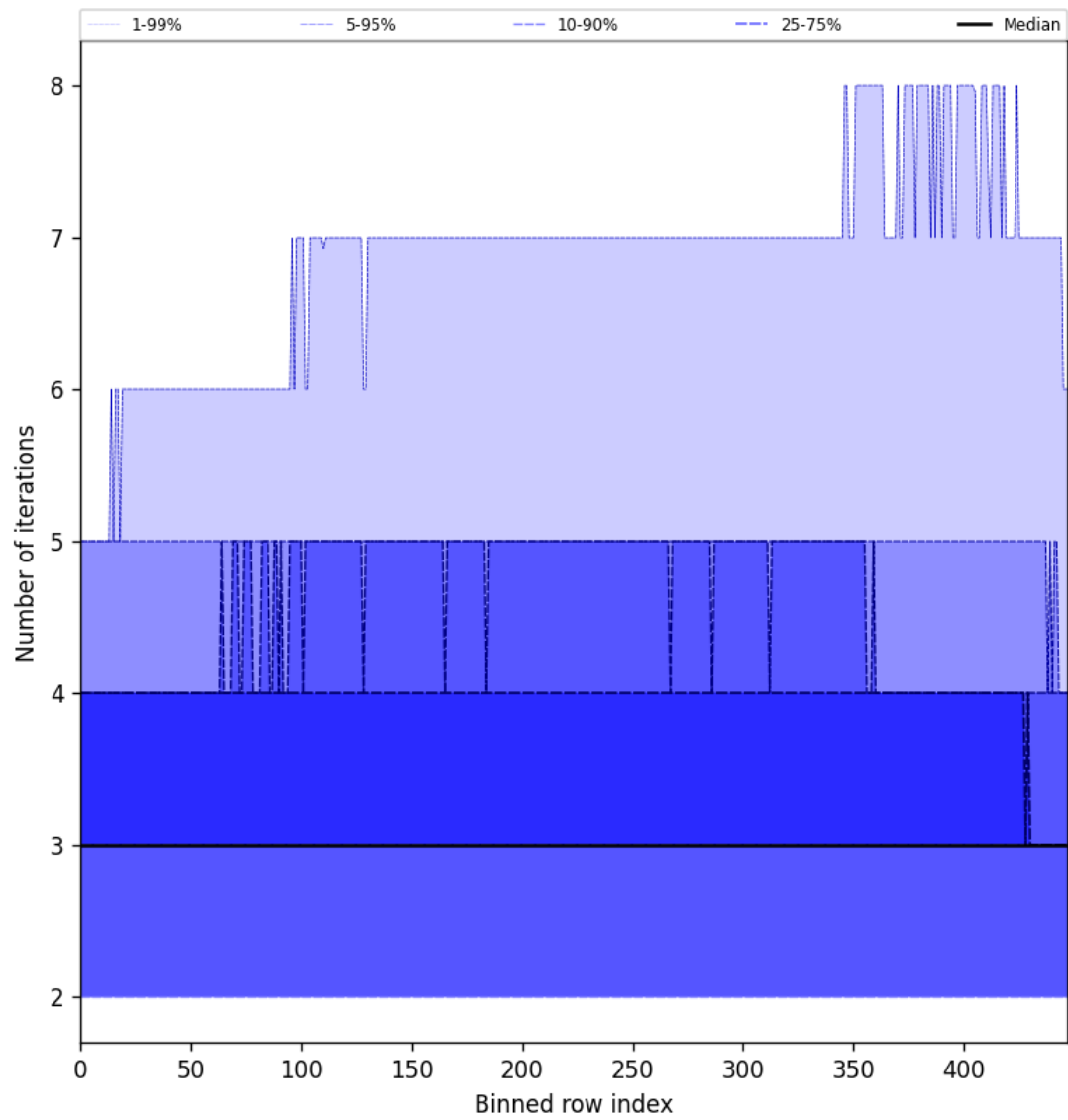
Figure 54: Along track statistics of “Number of iterations” for 2025-01-16 to 2025-01-17
