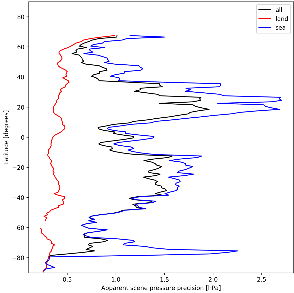
Figure 18: Zonal average of “Apparent scene pressure precision” for 2025-01-16 to 2025-01-17.
