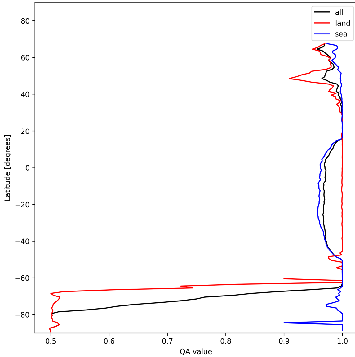
Figure 10: Zonal average of “QA value” for 2025-01-16 to 2025-01-17.
