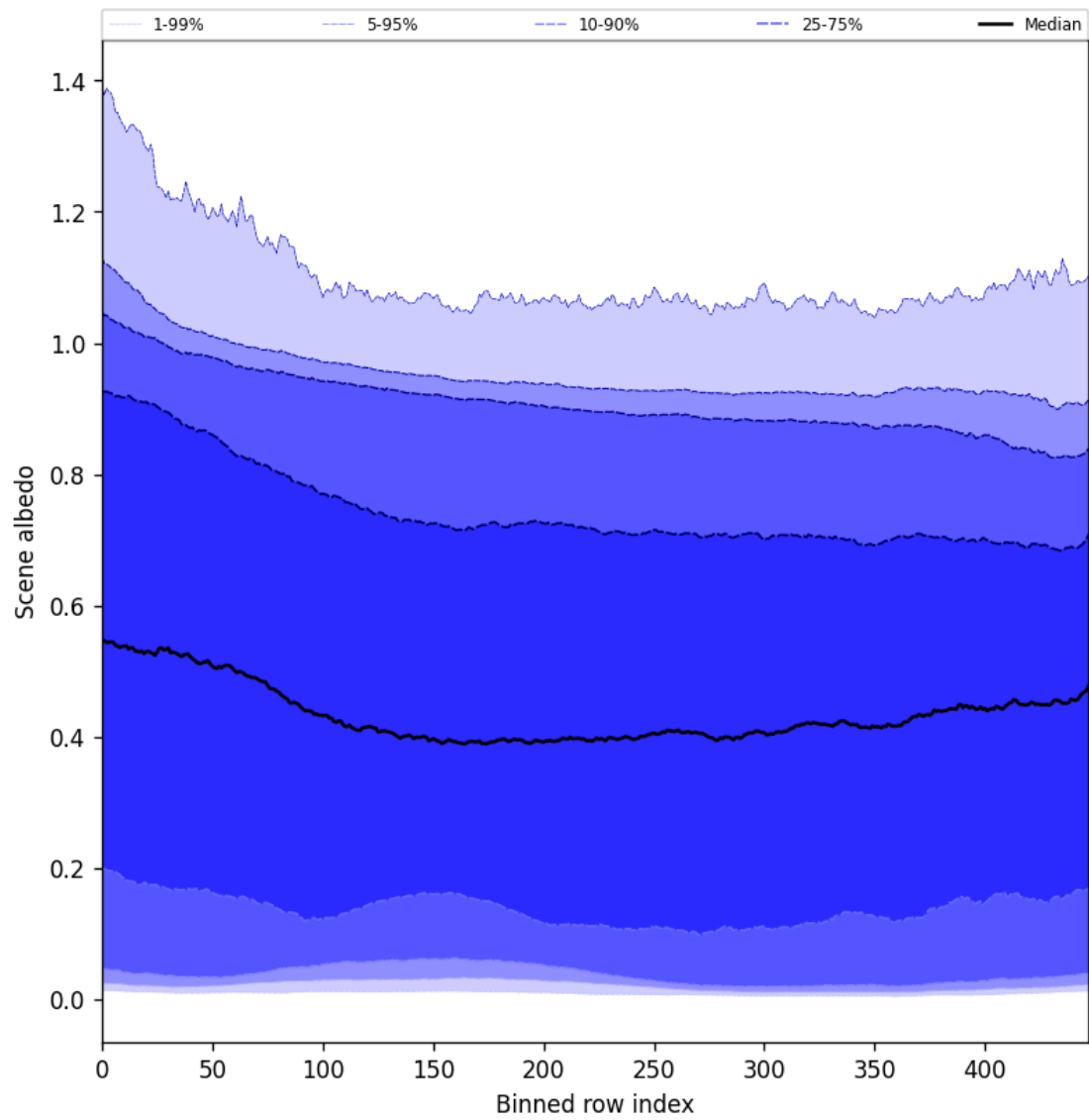
Figure 49: Along track statistics of "Scene albedo" for 2025-01-16 to 2025-01-17
