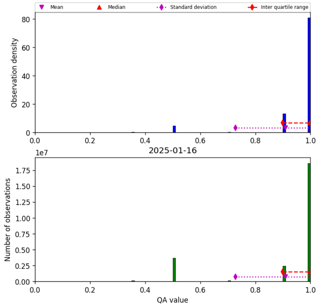
Figure 27: Histogram of “QA value” for 2025-01-16 to 2025-01-17
