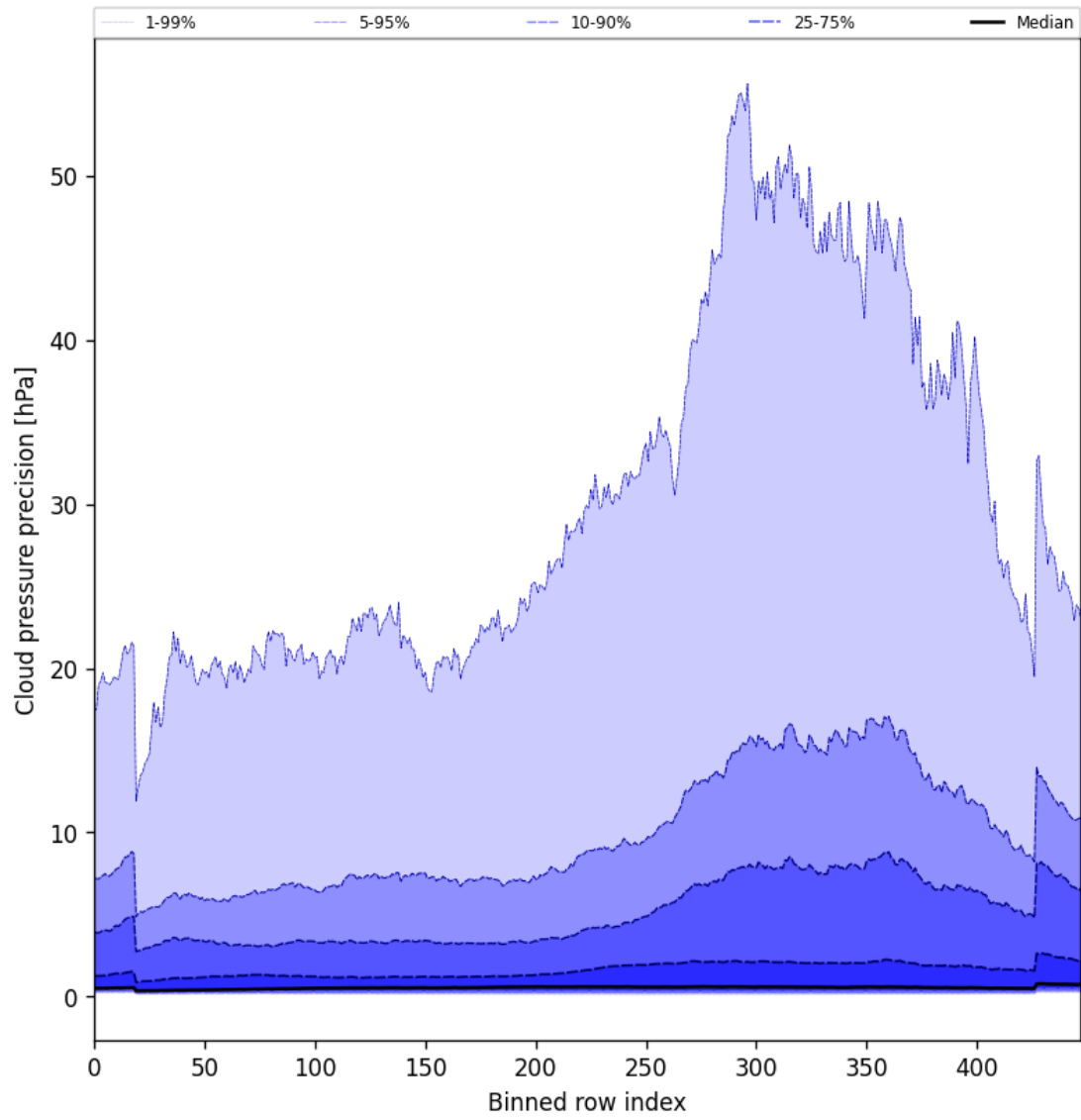
Figure 46: Along track statistics of “Cloud pressure precision” for 2025-01-16 to 2025-01-17
