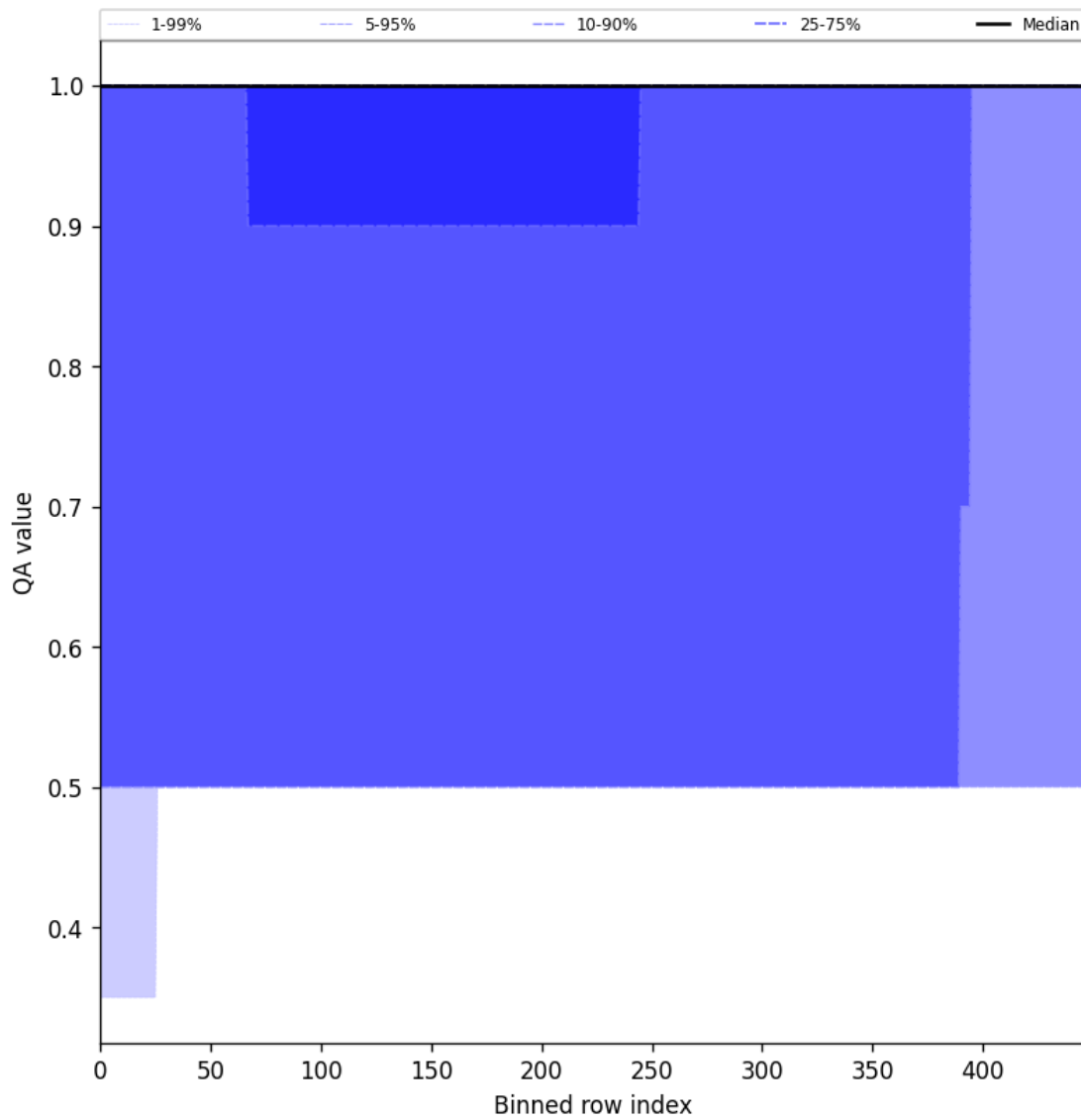
Figure 44: Along track statistics of “QA value” for 2025-01-16 to 2025-01-17
