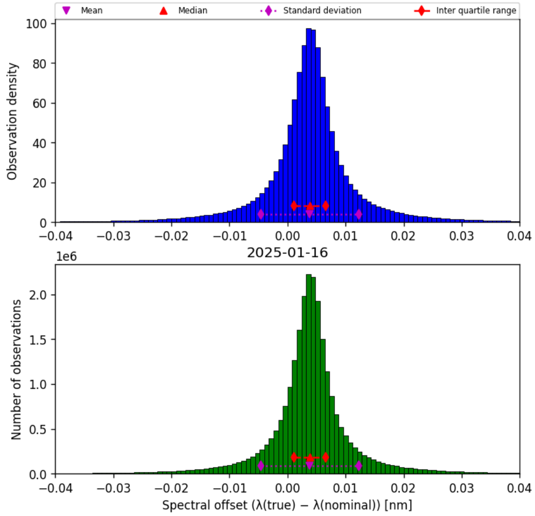
Figure 43: Histogram of “Spectral offset ( \lambda_{\text{true}} - \lambda_{\text{nominal}} )” for 2025-01-16 to 2025-01-17
