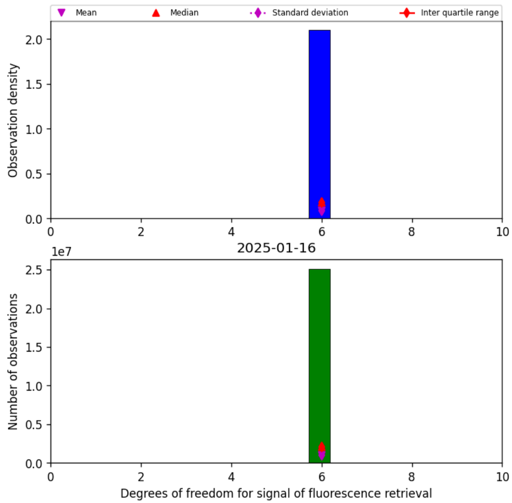
Figure 41: Histogram of “Degrees of freedom for signal of fluorescence retrieval” for 2025-01-16 to 2025-01-17
