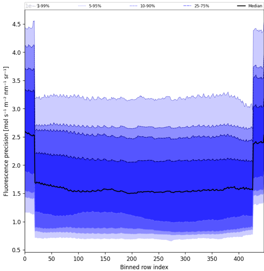
Figure 56: Along track statistics of “Fluorescence precision” for 2025-01-16 to 2025-01-17
