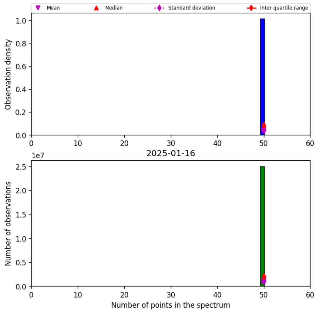
Figure 42: Histogram of “Number of points in the spectrum” for 2025-01-16 to 2025-01-17
