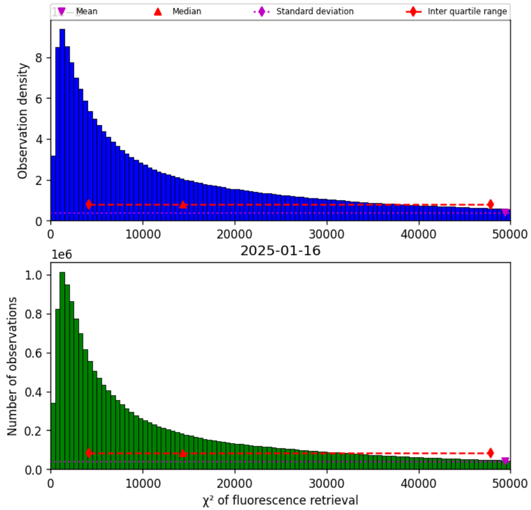
Figure 40: Histogram of “ \chi^2 of fluorescence retrieval” for 2025-01-16 to 2025-01-17
