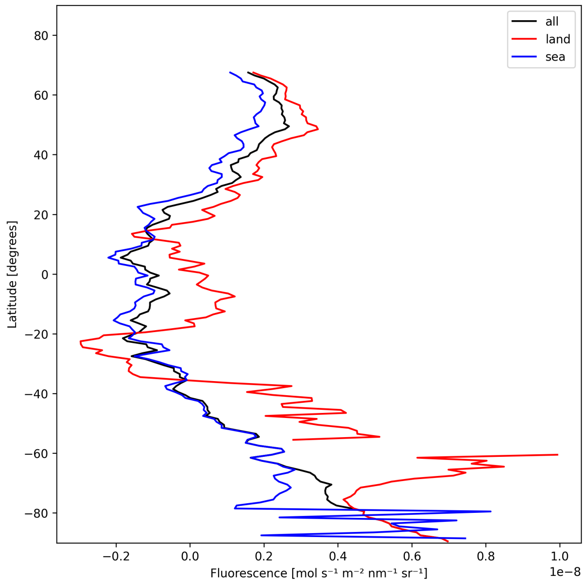
Figure 21: Zonal average of “Fluorescence” for 2025-01-16 to 2025-01-17.
