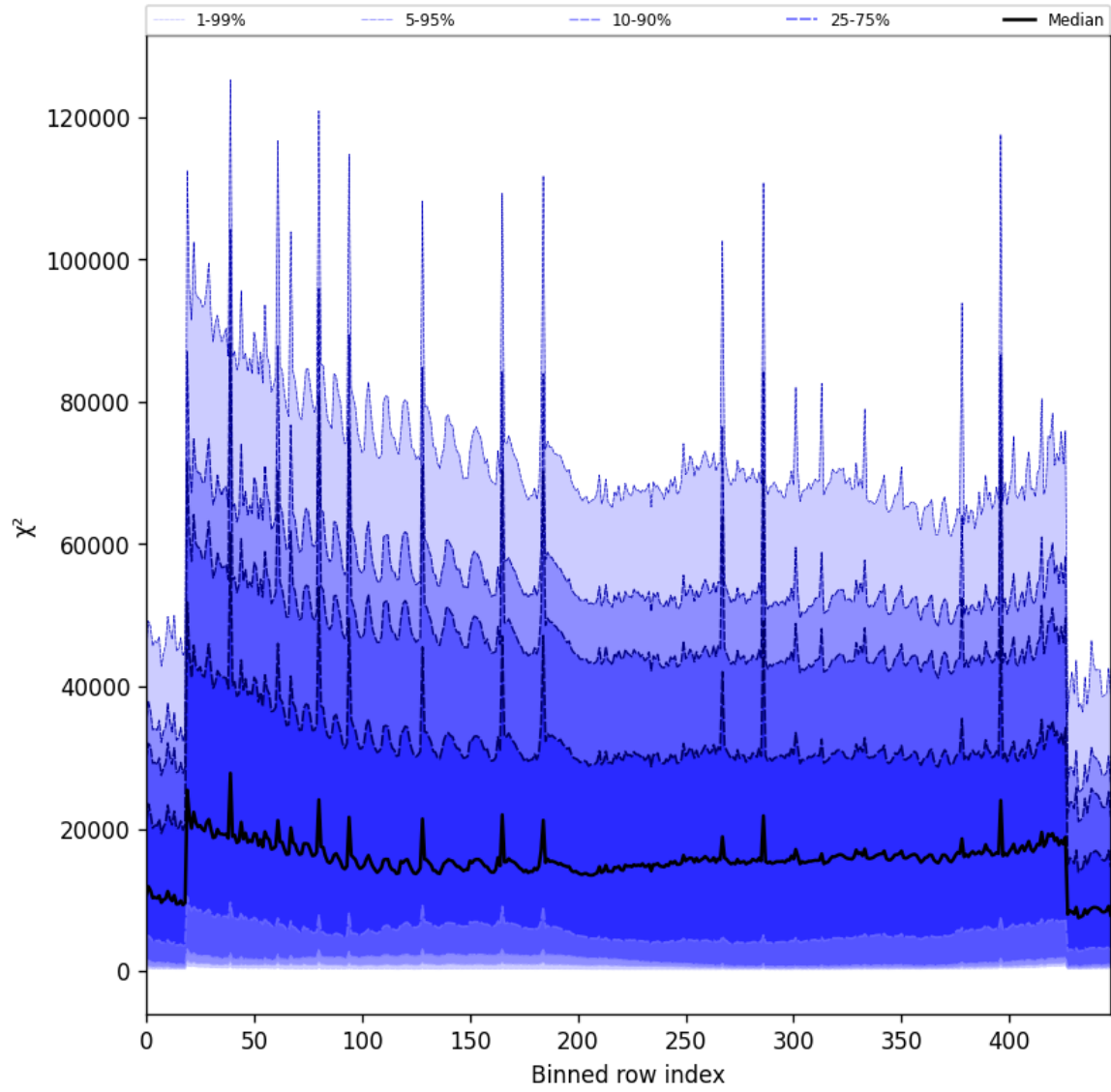
Figure 53: Along track statistics of “ \chi^2 ” for 2025-01-16 to 2025-01-17
