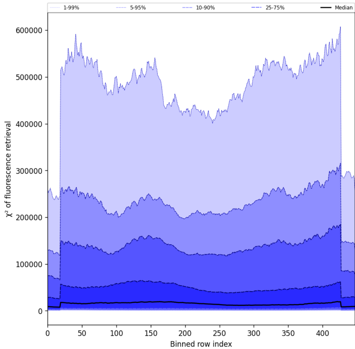
Figure 57: Along track statistics of “ \chi^2 of fluorescence retrieval” for 2025-01-16 to 2025-01-17
