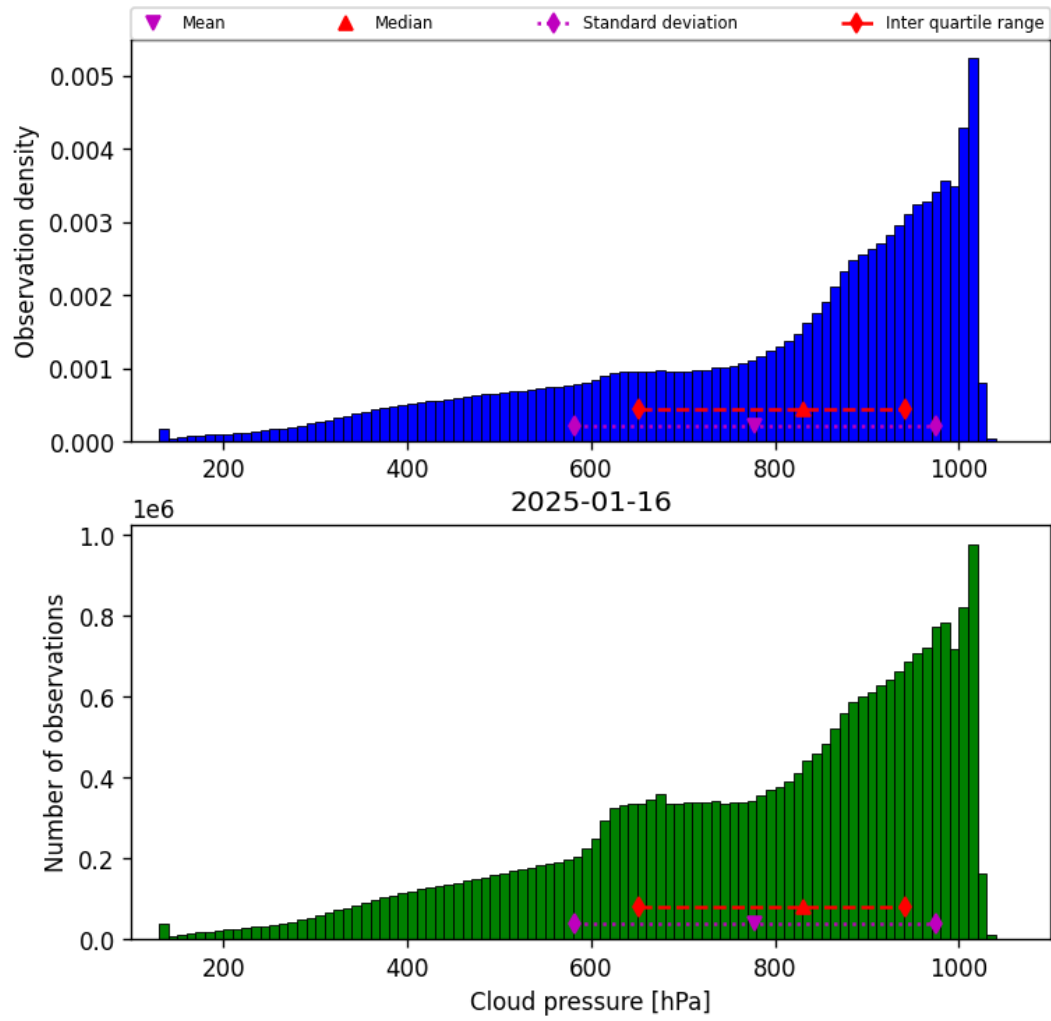
Figure 28: Histogram of “Cloud pressure” for 2025-01-16 to 2025-01-17
