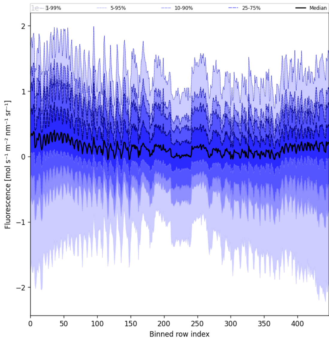
Figure 55: Along track statistics of “Fluorescence” for 2025-01-16 to 2025-01-17
