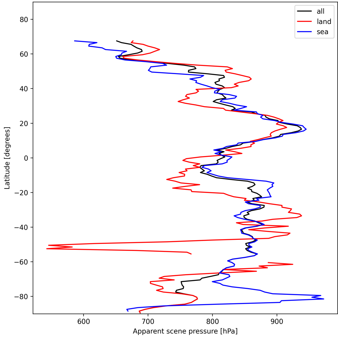
Figure 17: Zonal average of “Apparent scene pressure” for 2025-01-16 to 2025-01-17.
