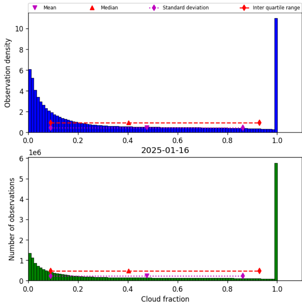
Figure 30: Histogram of “Cloud fraction” for 2025-01-16 to 2025-01-17
