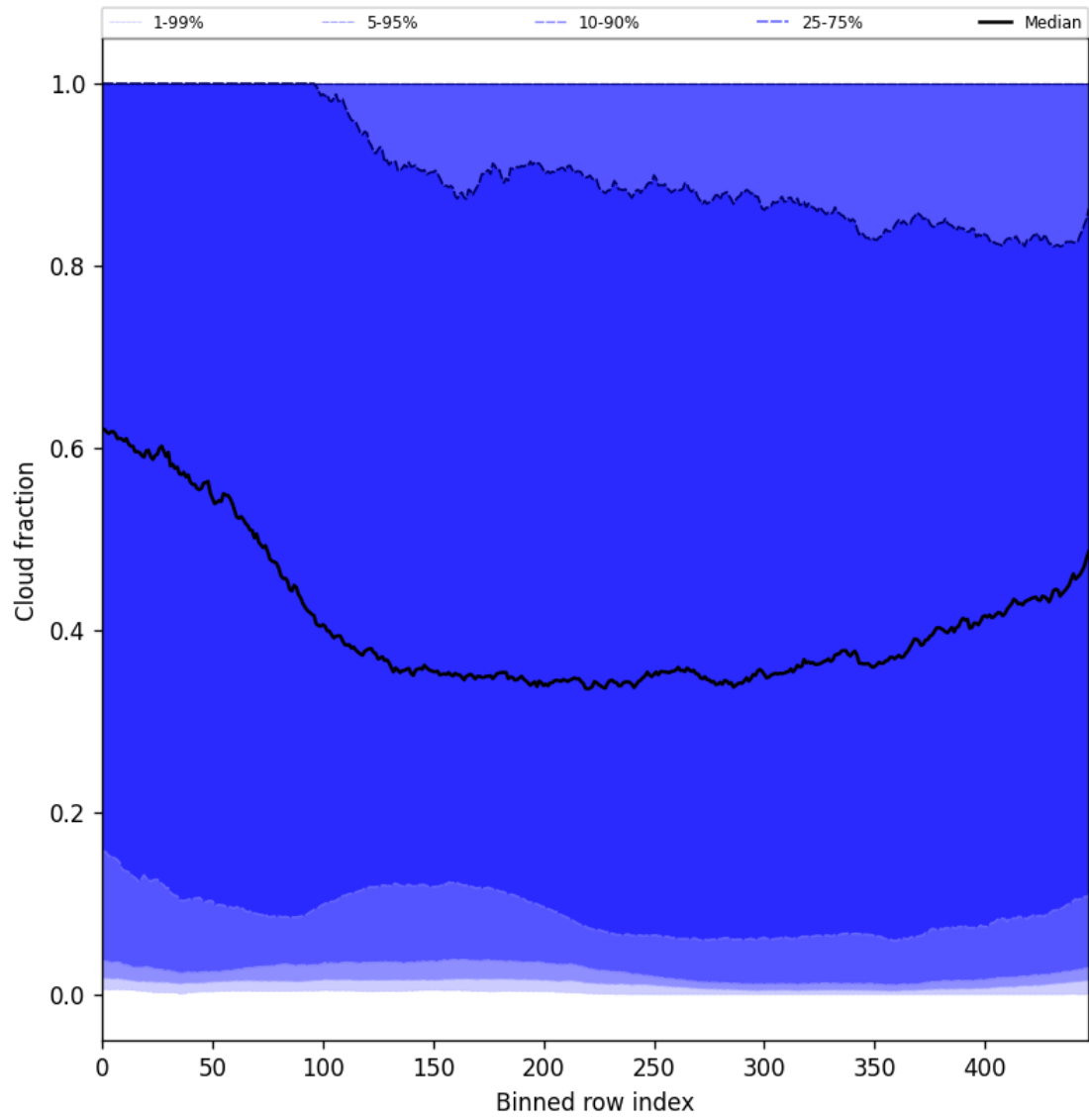
Figure 47: Along track statistics of “Cloud fraction” for 2025-01-16 to 2025-01-17
