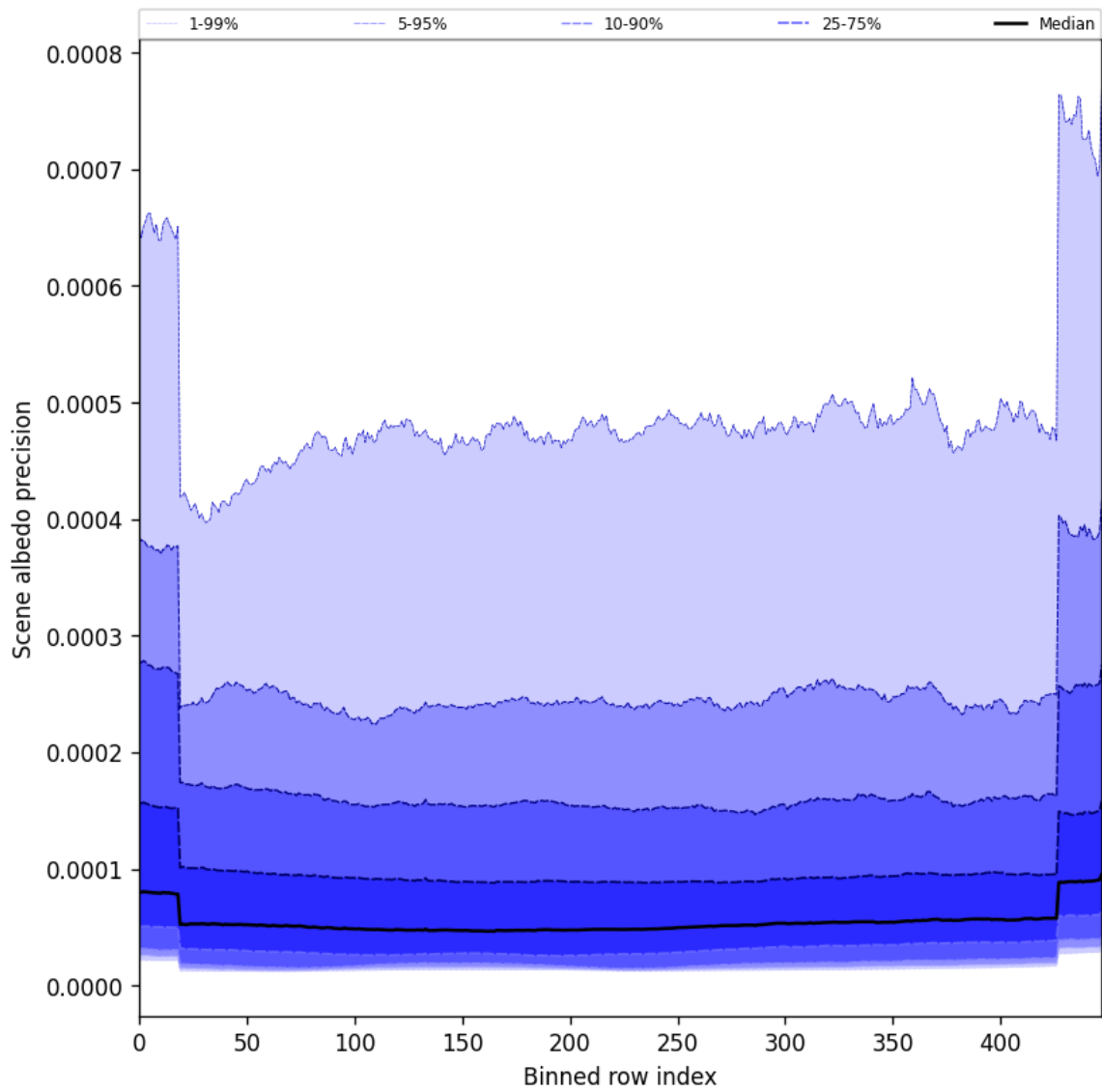
Figure 50: Along track statistics of “Scene albedo precision” for 2025-01-16 to 2025-01-17
