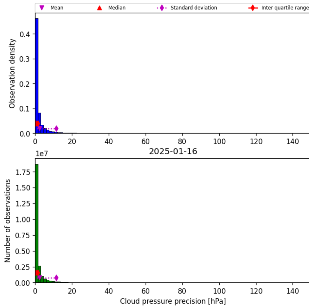
Figure 29: Histogram of “Cloud pressure precision” for 2025-01-16 to 2025-01-17
