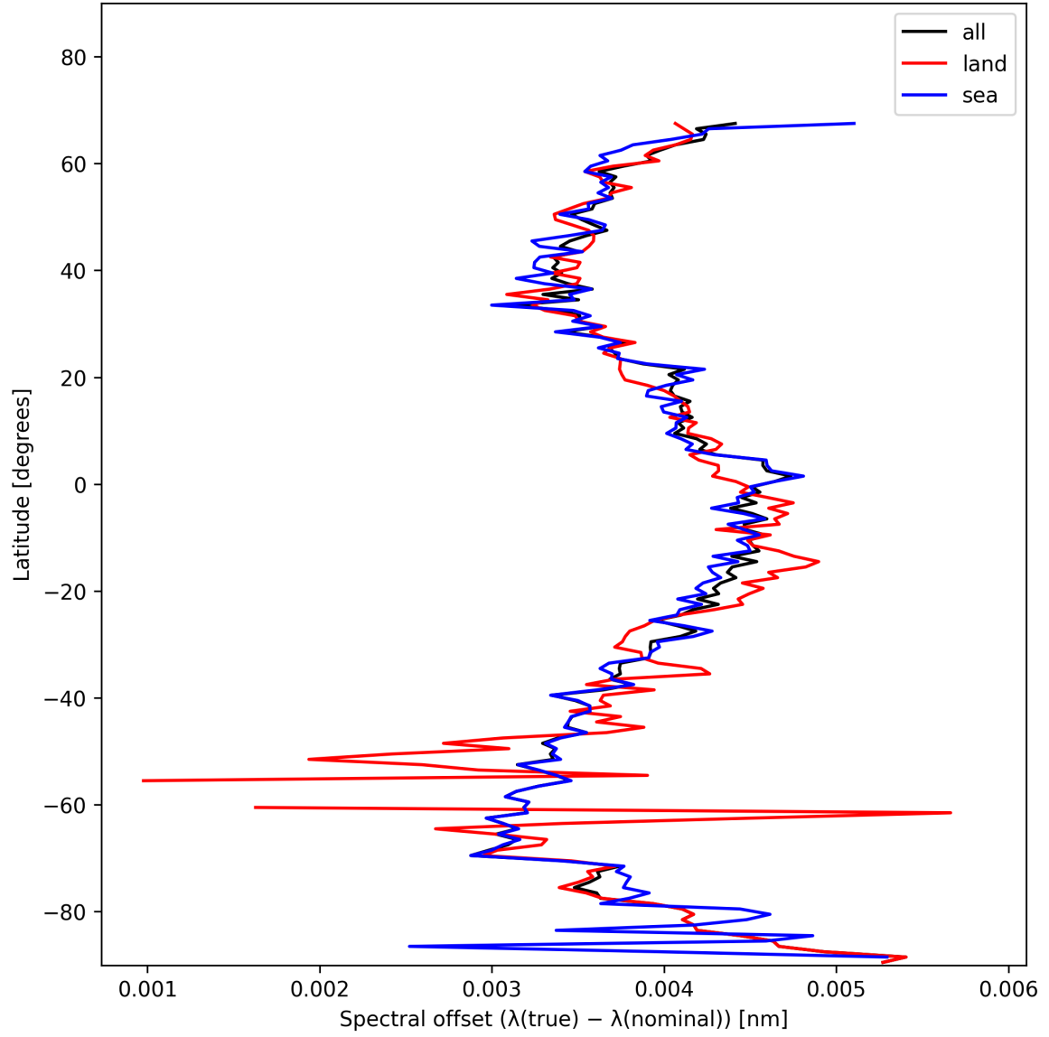
Figure 26: Zonal average of “Spectral offset ( \lambda_{\text{true}} - \lambda_{\text{nominal}} )” for 2025-01-16 to 2025-01-17.
