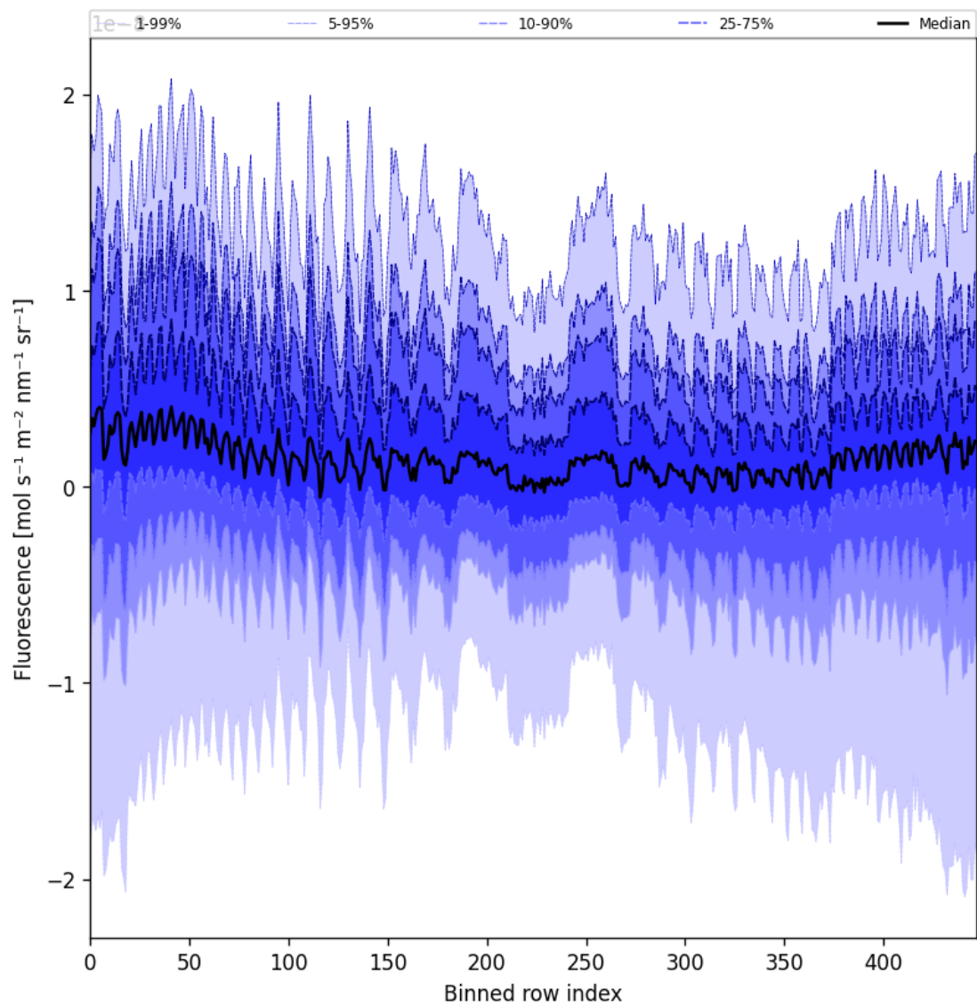
Figure 55: Along track statistics of “Fluorescence” for 2025-01-19 to 2025-01-20
