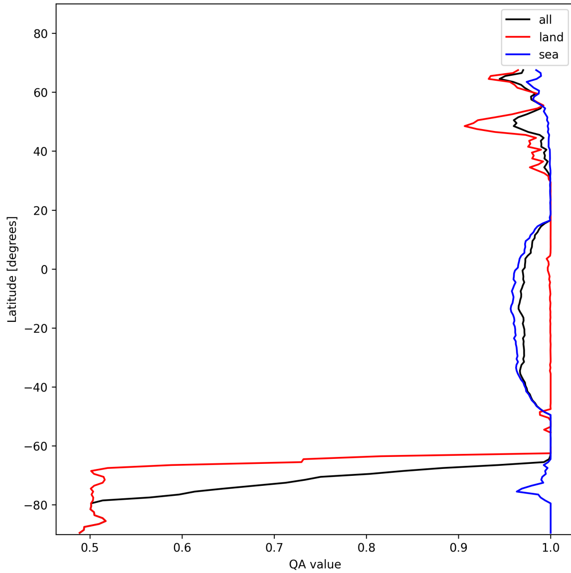
Figure 10: Zonal average of “QA value” for 2025-01-19 to 2025-01-20.
