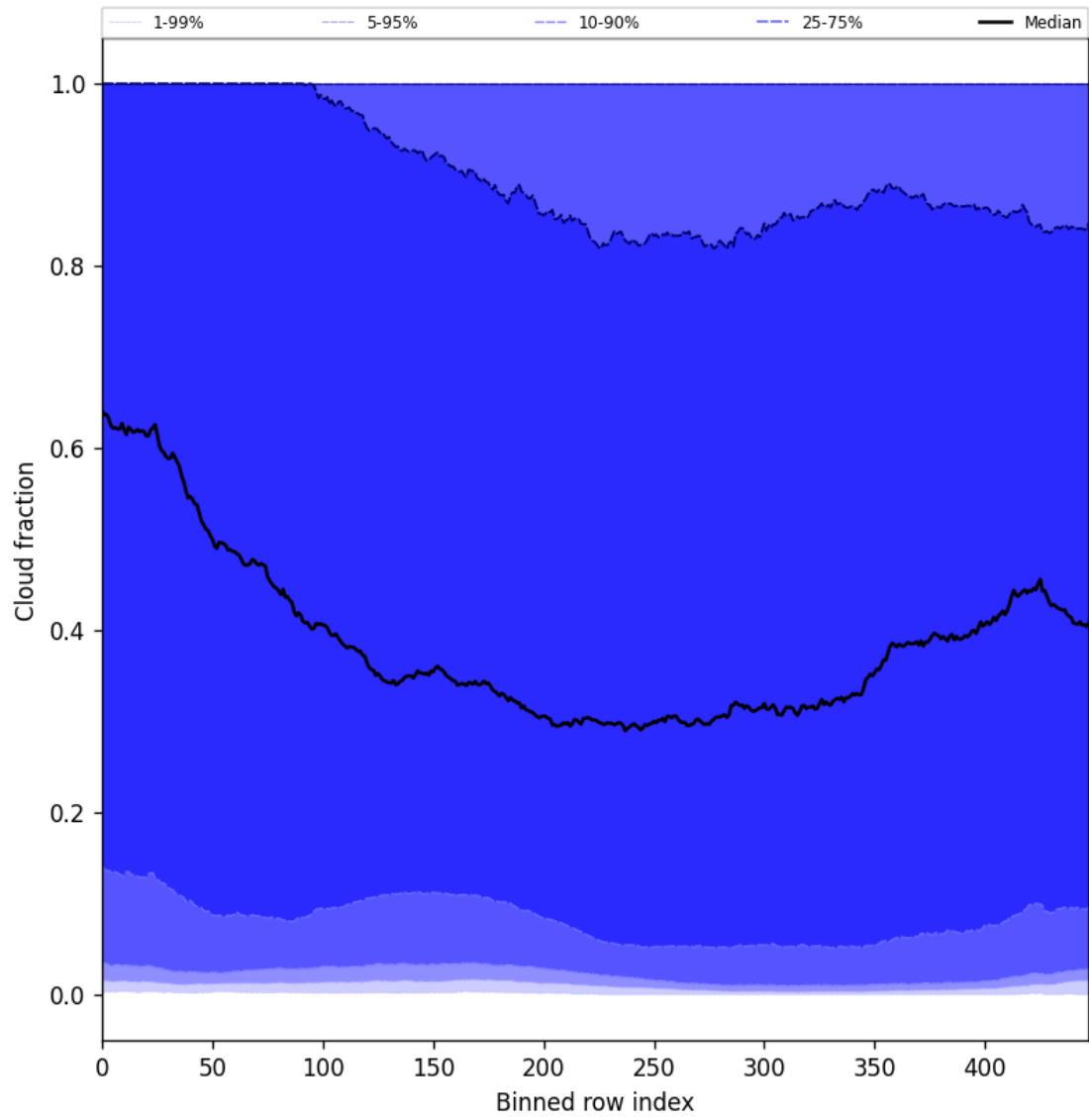
Figure 47: Along track statistics of “Cloud fraction” for 2025-01-19 to 2025-01-20
