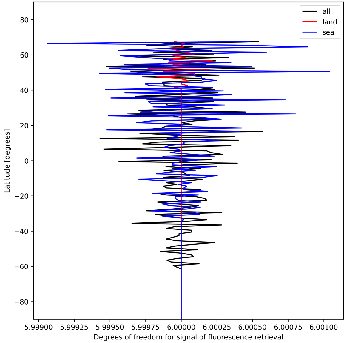
Figure 24: Zonal average of “Degrees of freedom for signal of fluorescence retrieval” for 2025-01-19 to 2025-01-20.
