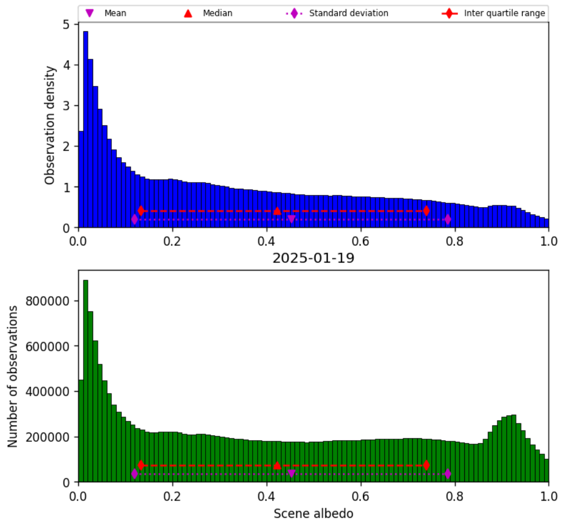
Figure 32: Histogram of “Scene albedo” for 2025-01-19 to 2025-01-20
