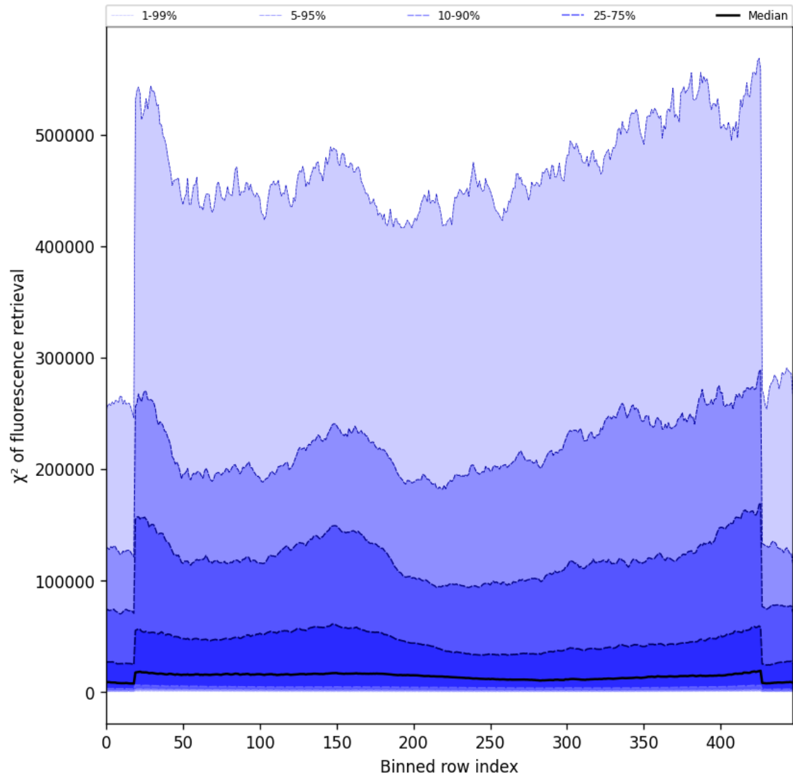
Figure 57: Along track statistics of “ \chi^2 of fluorescence retrieval” for 2025-01-19 to 2025-01-20
