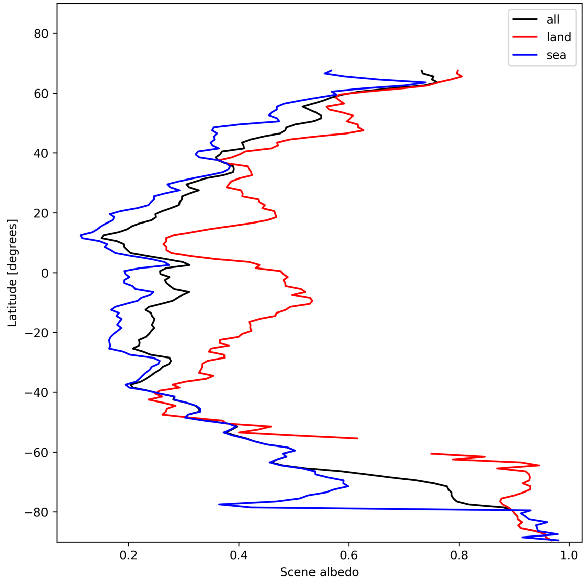
Figure 15: Zonal average of “Scene albedo” for 2025-01-19 to 2025-01-20.
