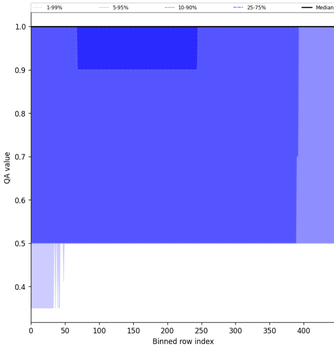
Figure 44: Along track statistics of “QA value” for 2025-01-19 to 2025-01-20
