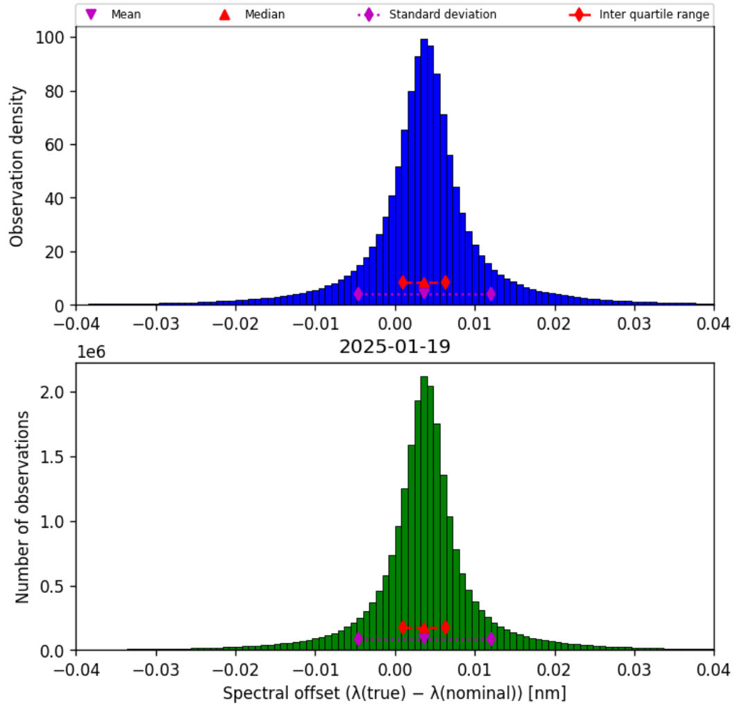
Figure 43: Histogram of “Spectral offset ( \lambda_{\text{true}} - \lambda_{\text{nominal}} )” for 2025-01-19 to 2025-01-20
