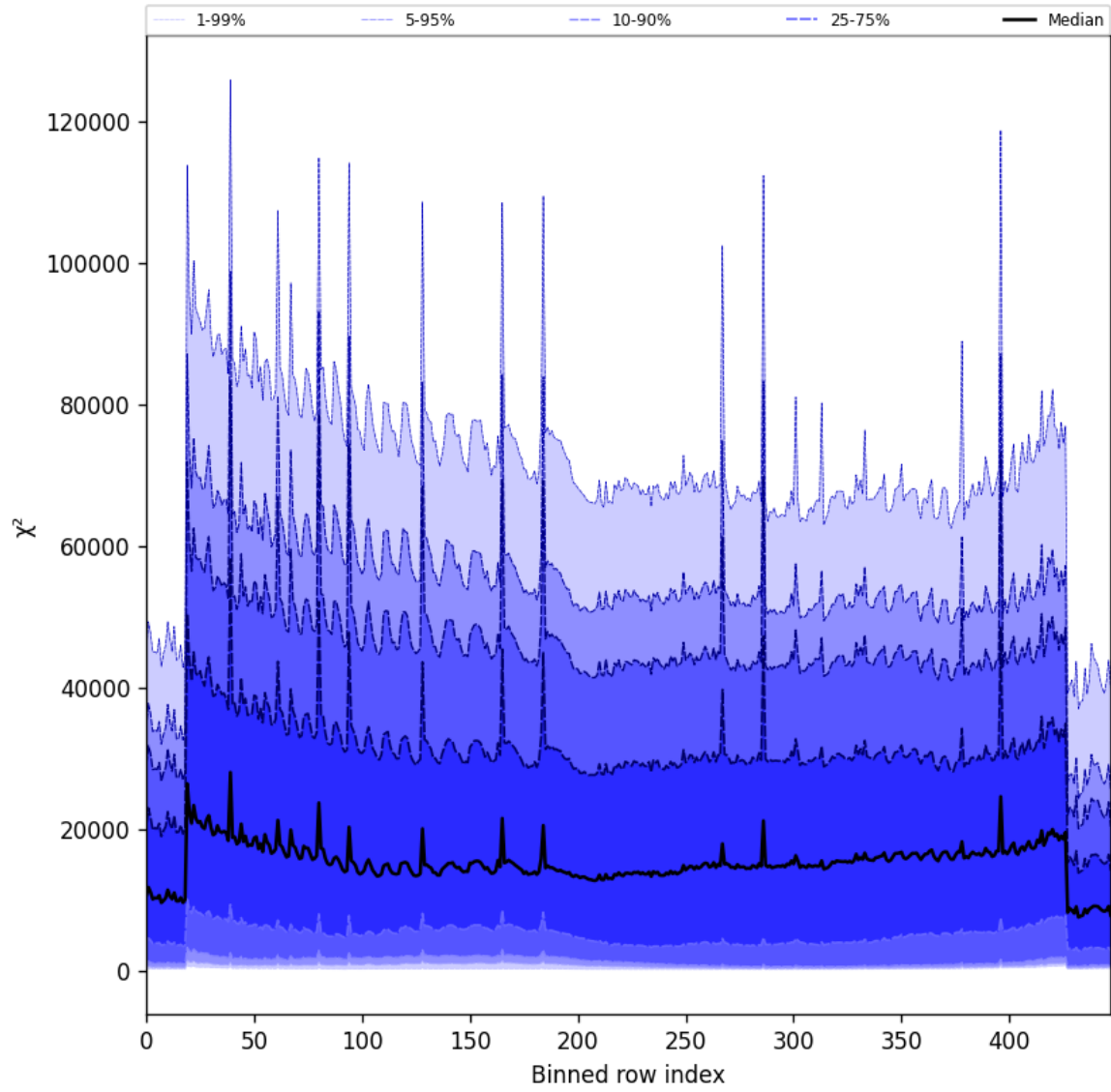
Figure 53: Along track statistics of “ \chi^2 ” for 2025-01-19 to 2025-01-20
