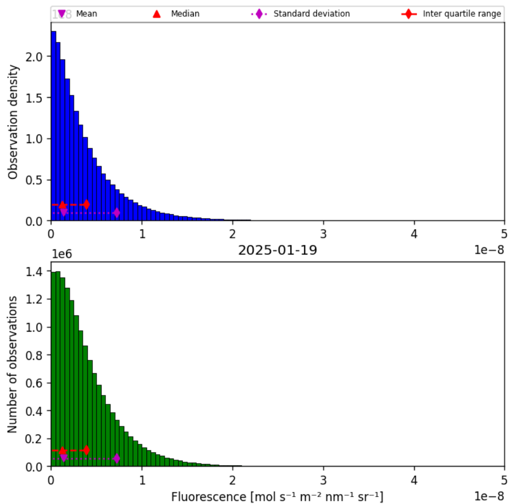
Figure 38: Histogram of “Fluorescence” for 2025-01-19 to 2025-01-20
