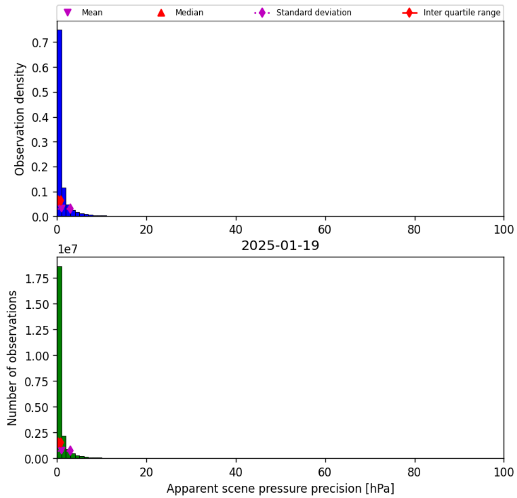
Figure 35: Histogram of “Apparent scene pressure precision” for 2025-01-19 to 2025-01-20
