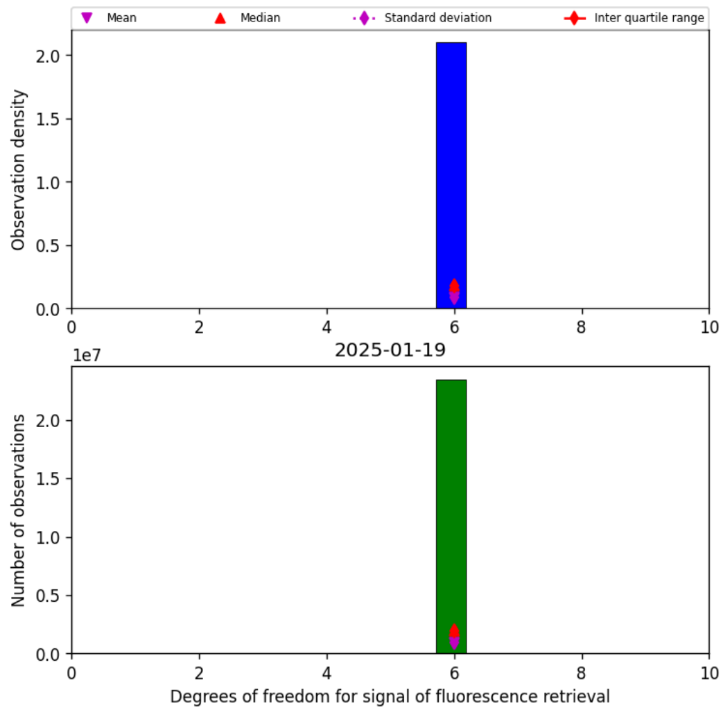
Figure 41: Histogram of “Degrees of freedom for signal of fluorescence retrieval” for 2025-01-19 to 2025-01-20
