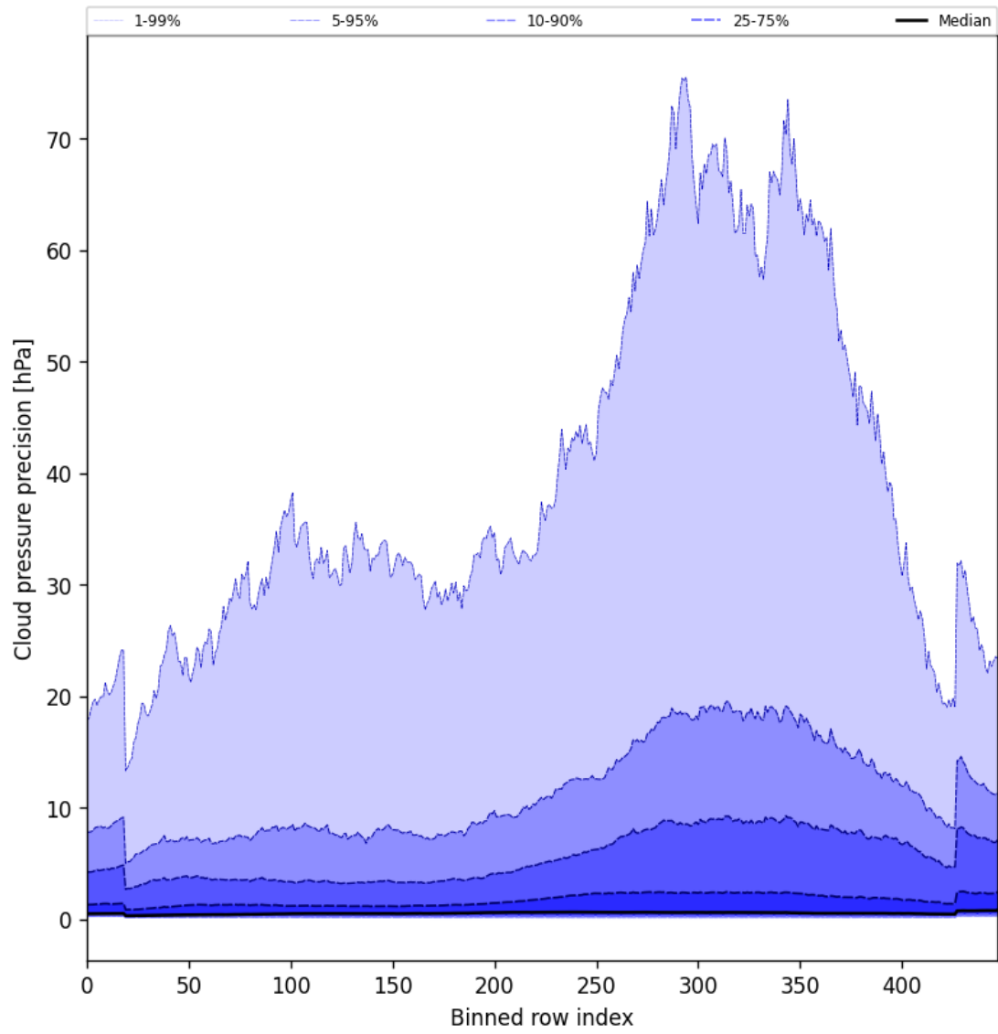
Figure 46: Along track statistics of “Cloud pressure precision” for 2025-01-19 to 2025-01-20
