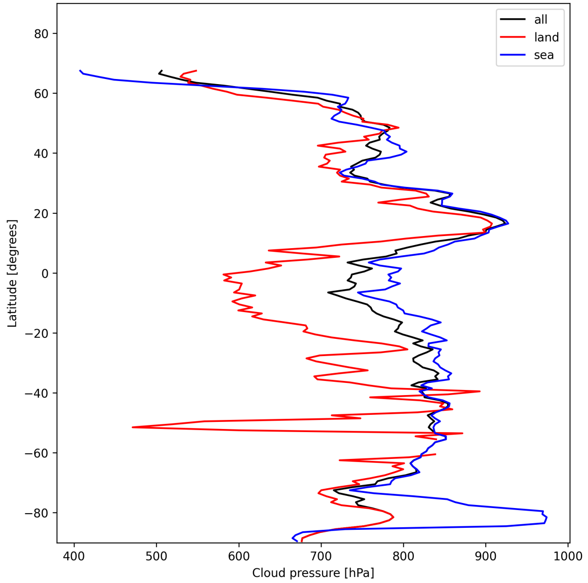
Figure 11: Zonal average of “Cloud pressure” for 2025-01-19 to 2025-01-20.
