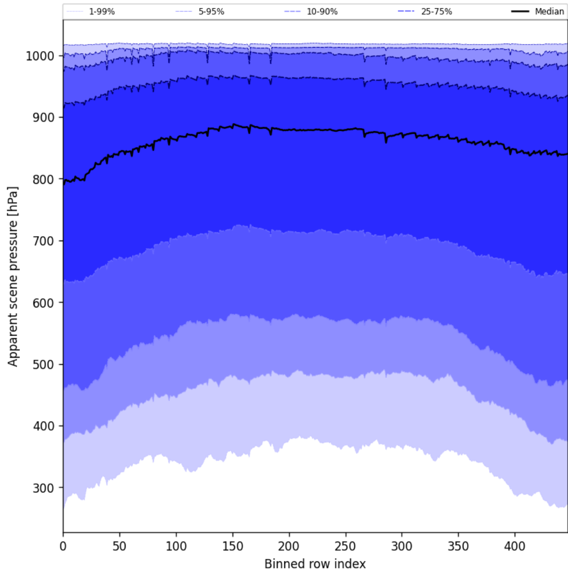
Figure 51: Along track statistics of “Apparent scene pressure” for 2025-01-19 to 2025-01-20
