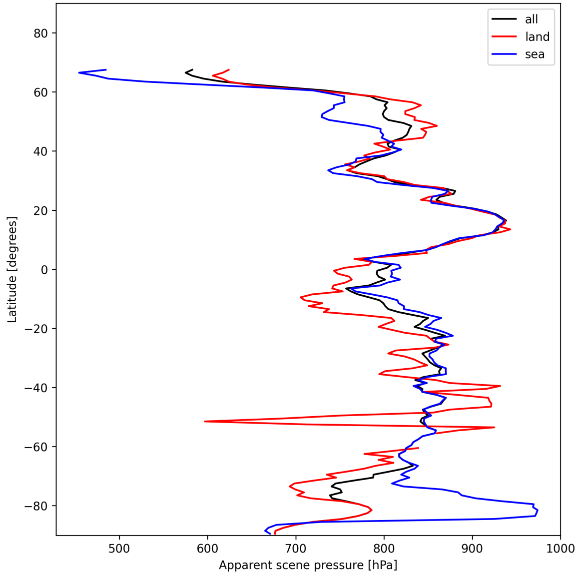
Figure 17: Zonal average of “Apparent scene pressure” for 2025-01-19 to 2025-01-20.
