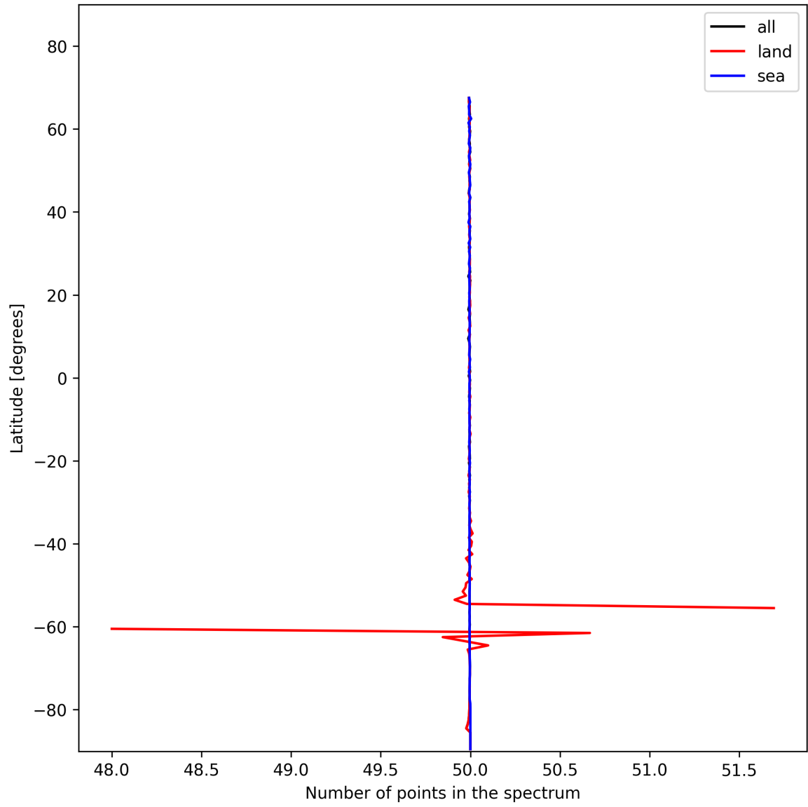
Figure 25: Zonal average of “Number of points in the spectrum” for 2025-01-19 to 2025-01-20.
