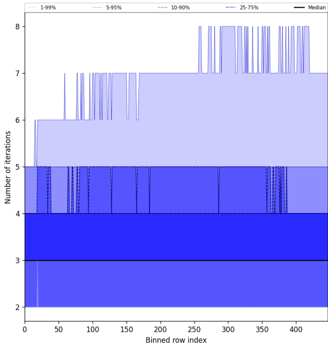
Figure 54: Along track statistics of “Number of iterations” for 2025-01-19 to 2025-01-20
