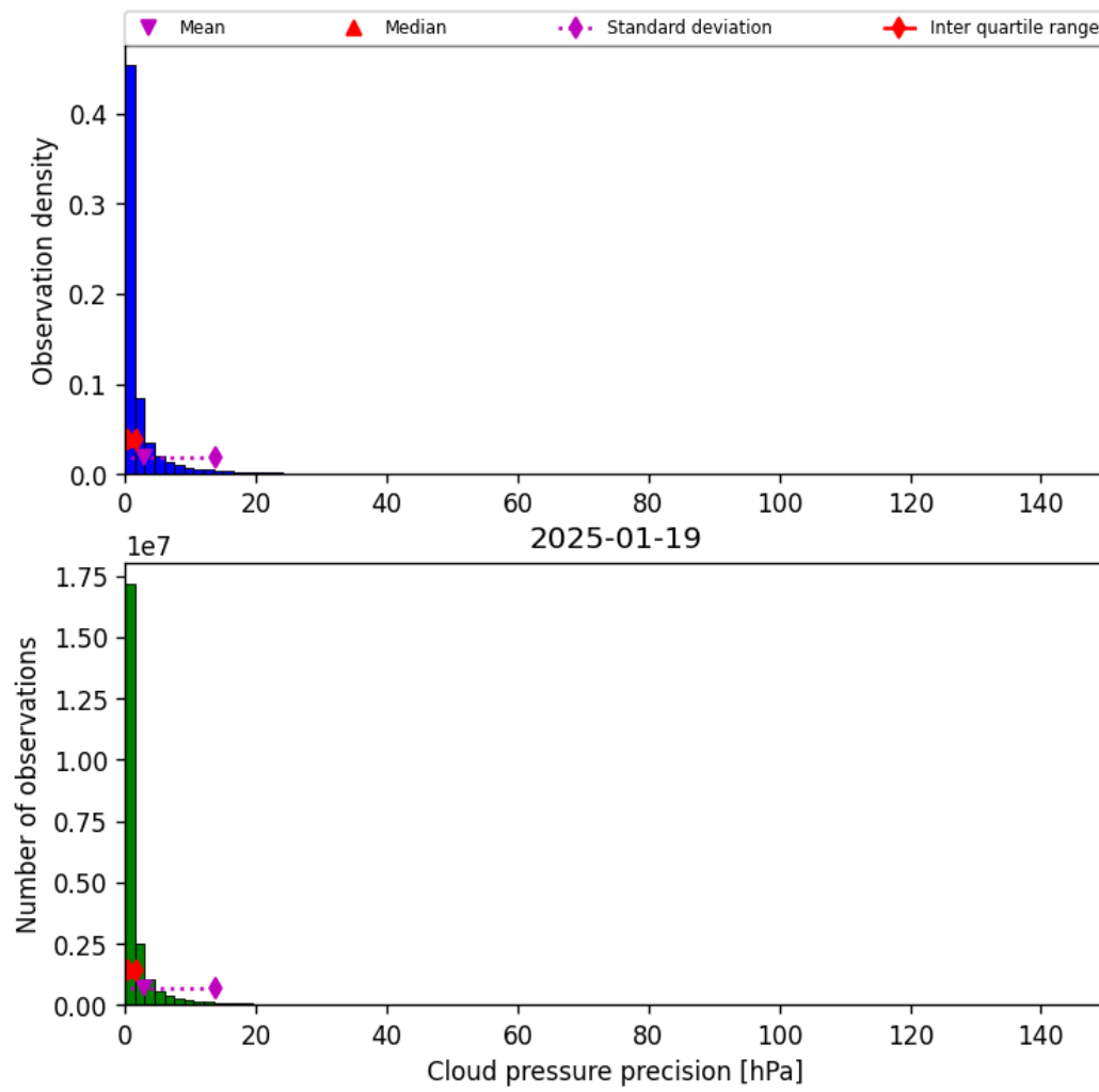
Figure 29: Histogram of “Cloud pressure precision” for 2025-01-19 to 2025-01-20
