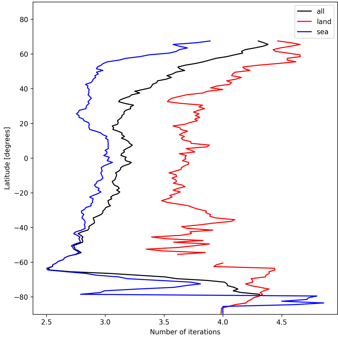
Figure 20: Zonal average of “Number of iterations” for 2025-01-19 to 2025-01-20.
