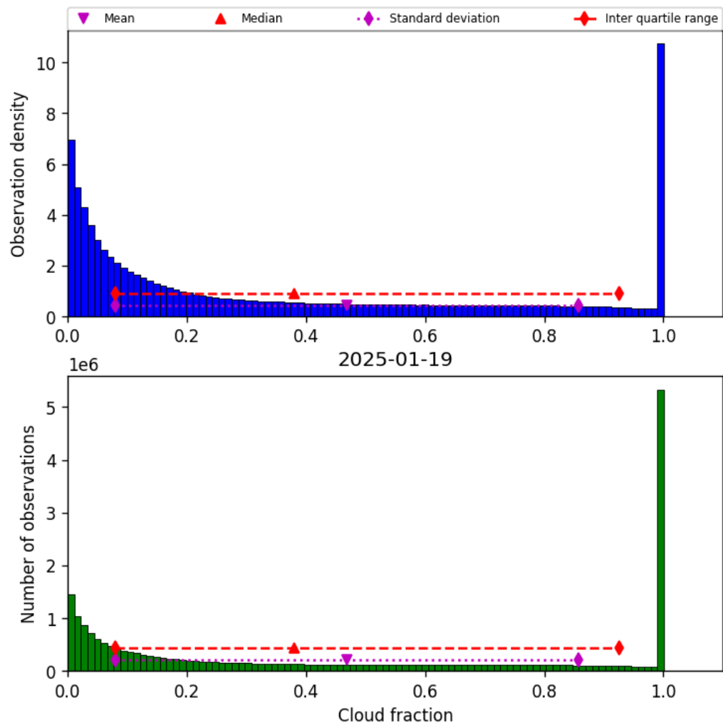
Figure 30: Histogram of “Cloud fraction” for 2025-01-19 to 2025-01-20
