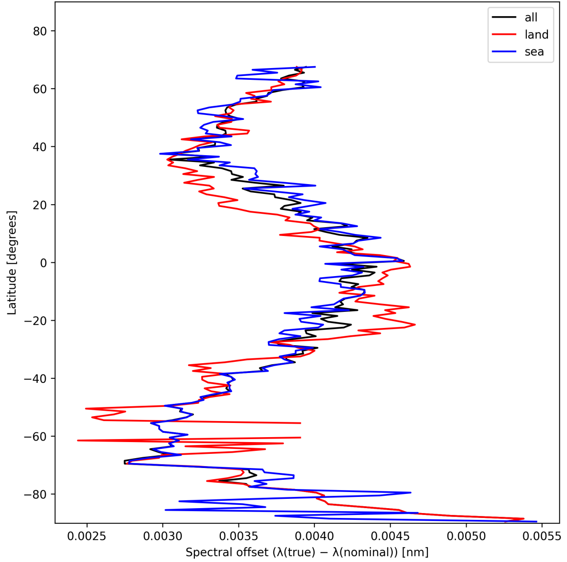
Figure 26: Zonal average of “Spectral offset ( \lambda_{\text{true}} - \lambda_{\text{nominal}} )” for 2025-01-19 to 2025-01-20.
