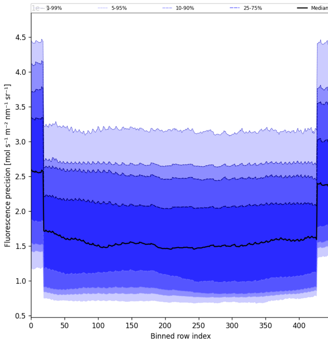
Figure 56: Along track statistics of “Fluorescence precision” for 2025-01-19 to 2025-01-20
