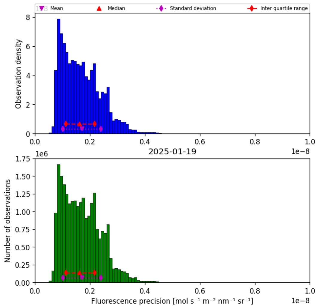
Figure 39: Histogram of “Fluorescence precision” for 2025-01-19 to 2025-01-20
