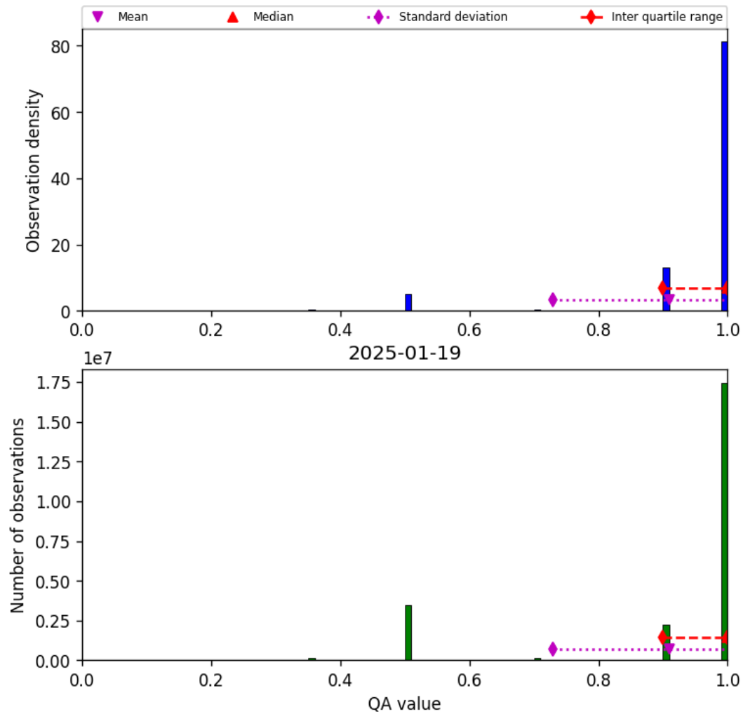
Figure 27: Histogram of “QA value” for 2025-01-19 to 2025-01-20
