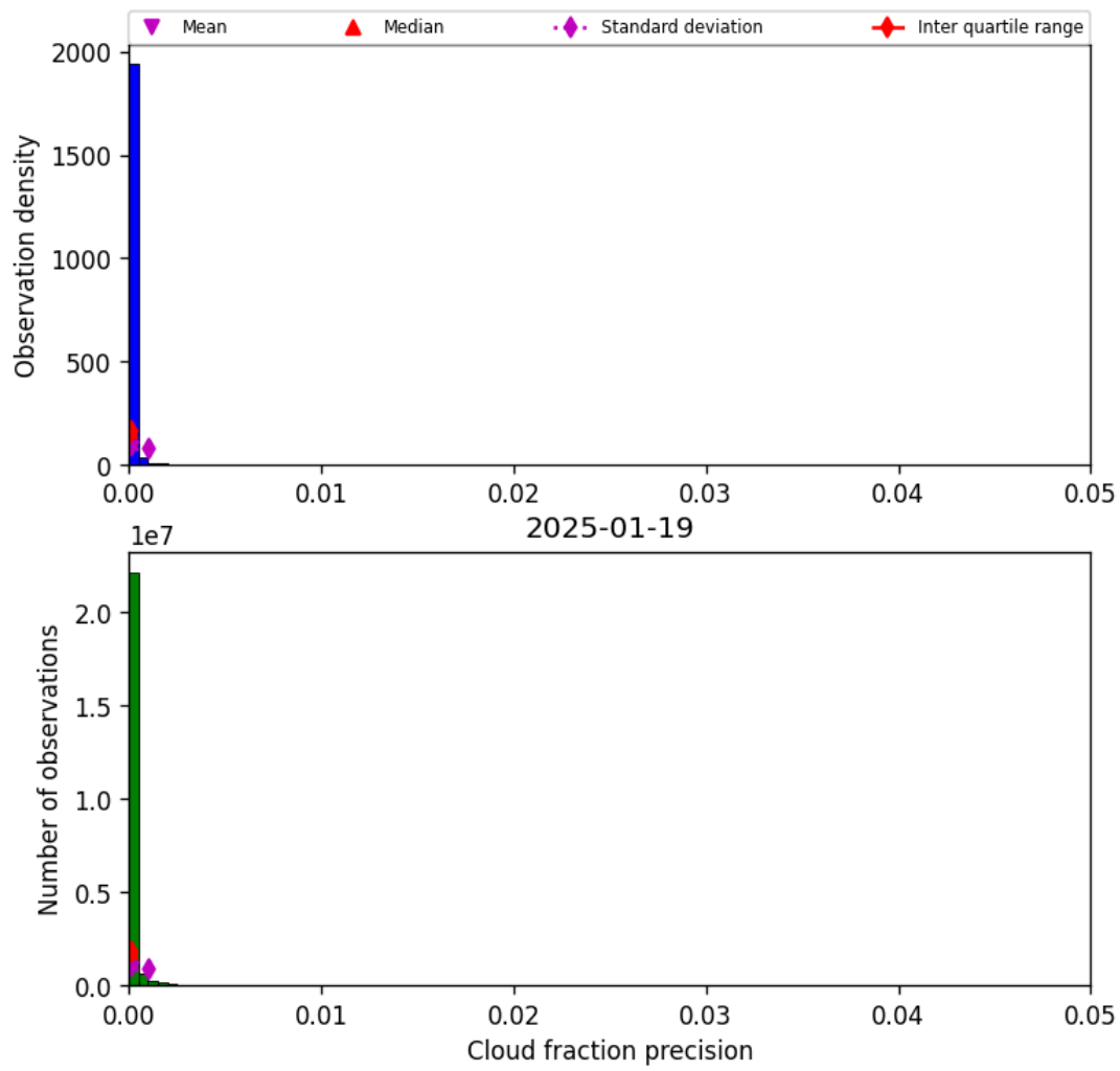
Figure 31: Histogram of “Cloud fraction precision” for 2025-01-19 to 2025-01-20
