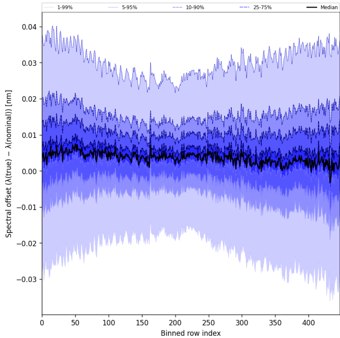
Figure 60: Along track statistics of “Spectral offset ( \lambda_{\text{true}} - \lambda_{\text{nominal}} )” for 2025-01-19 to 2025-01-20
