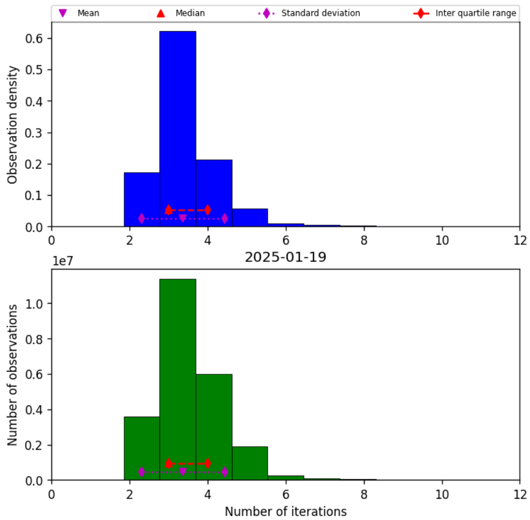
Figure 37: Histogram of “Number of iterations” for 2025-01-19 to 2025-01-20
