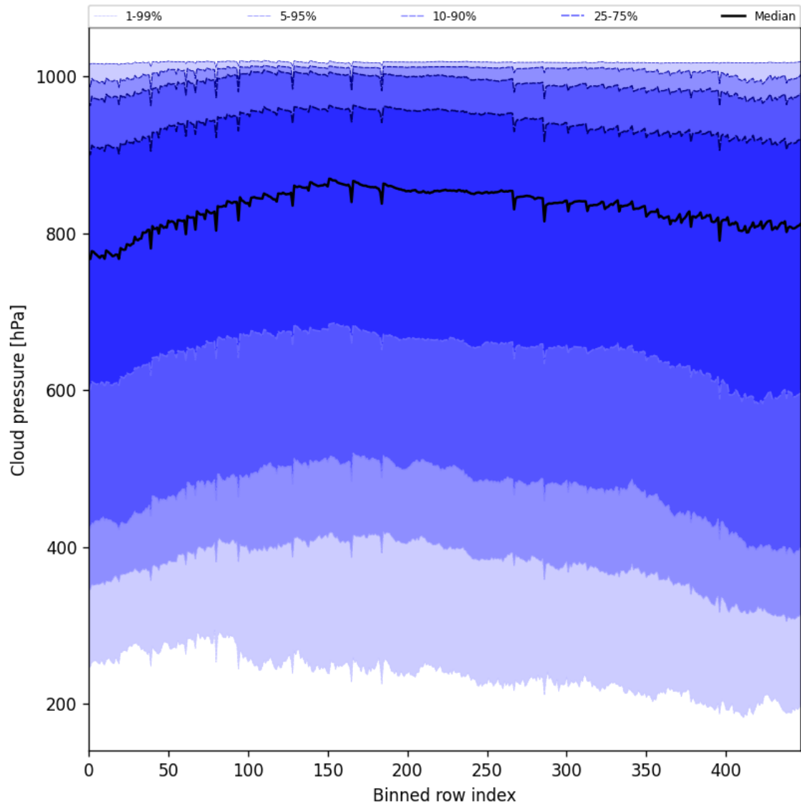
Figure 45: Along track statistics of “Cloud pressure” for 2025-01-19 to 2025-01-20
