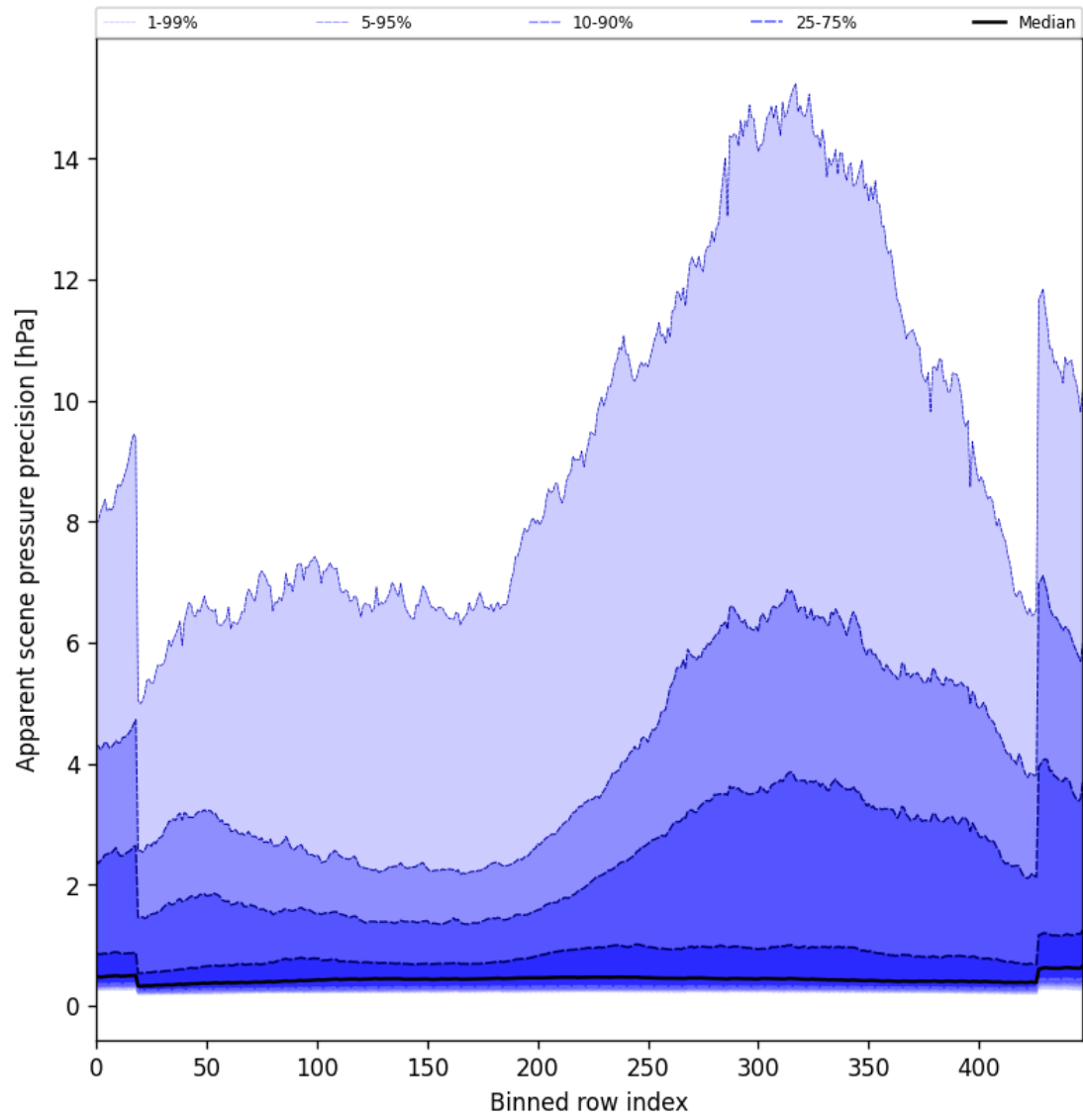
Figure 52: Along track statistics of “Apparent scene pressure precision” for 2025-01-19 to 2025-01-20
