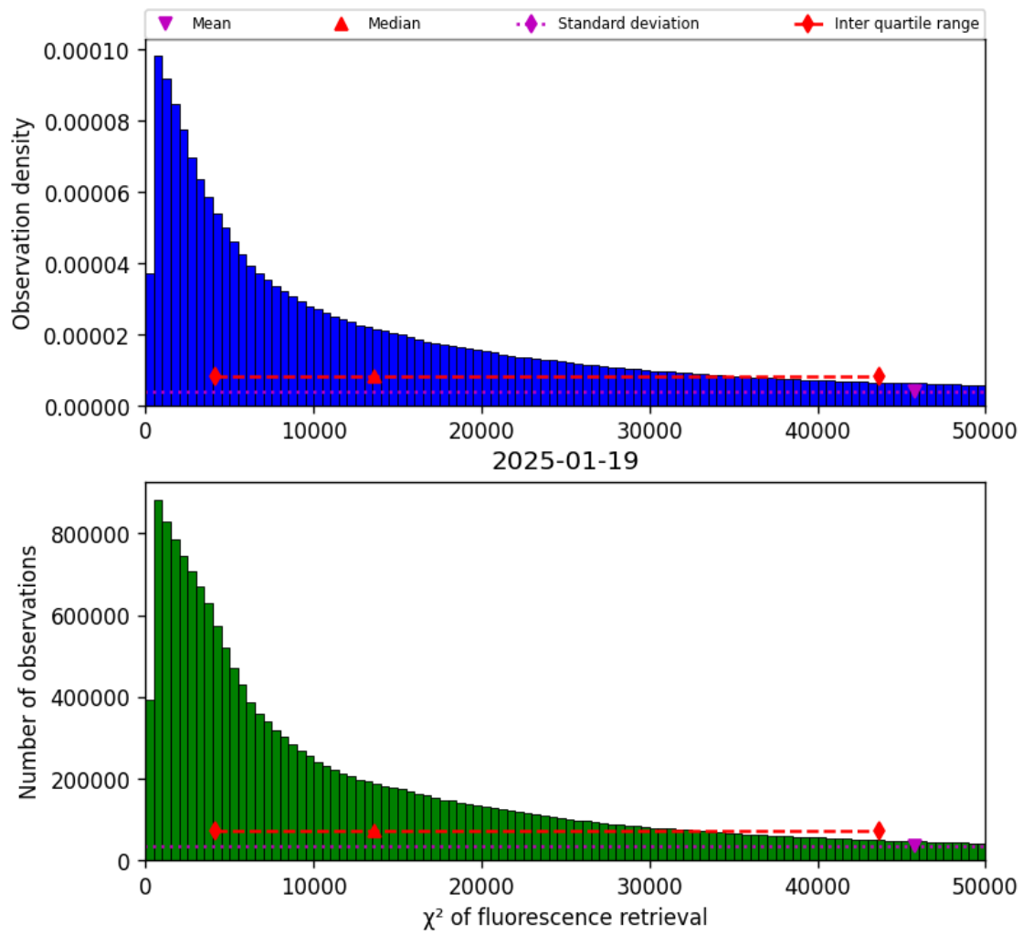
Figure 40: Histogram of “ \chi^2 of fluorescence retrieval” for 2025-01-19 to 2025-01-20
