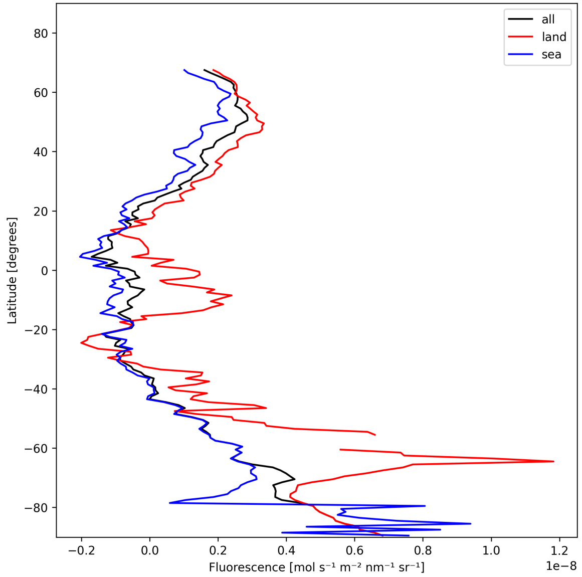
Figure 21: Zonal average of “Fluorescence” for 2025-01-19 to 2025-01-20.
