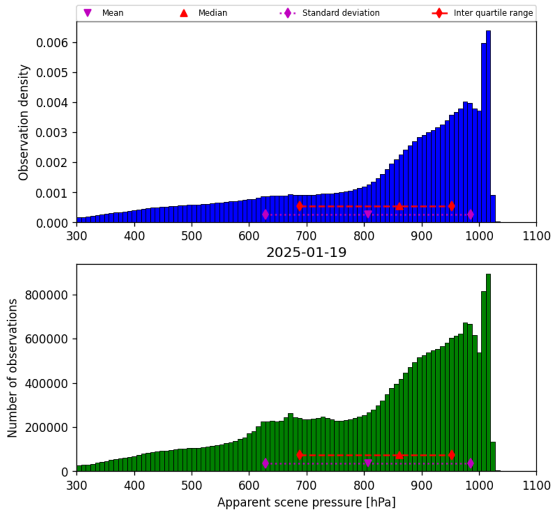
Figure 34: Histogram of “Apparent scene pressure” for 2025-01-19 to 2025-01-20
