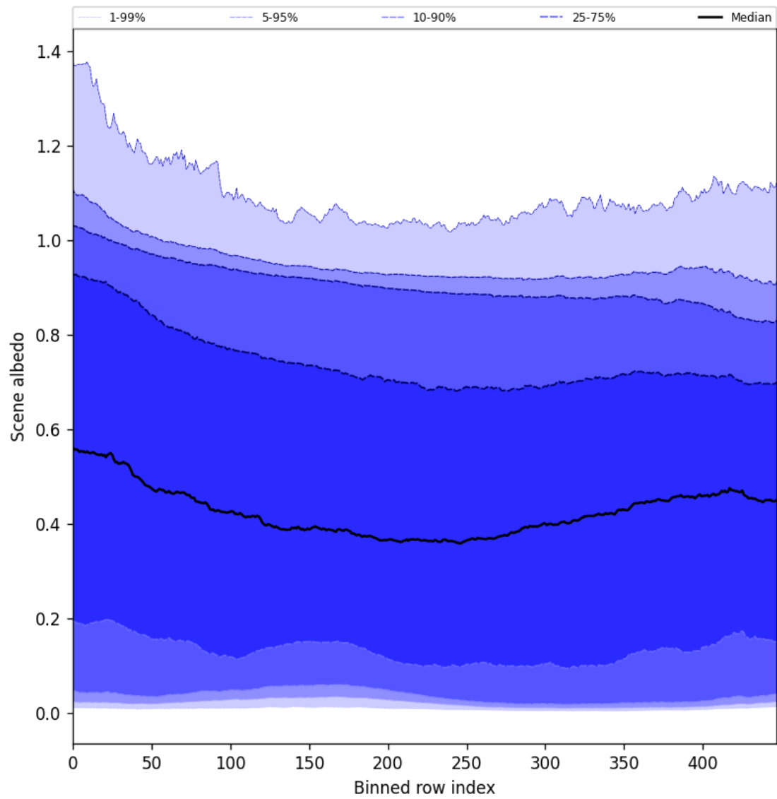
Figure 49: Along track statistics of “Scene albedo” for 2025-01-19 to 2025-01-20
