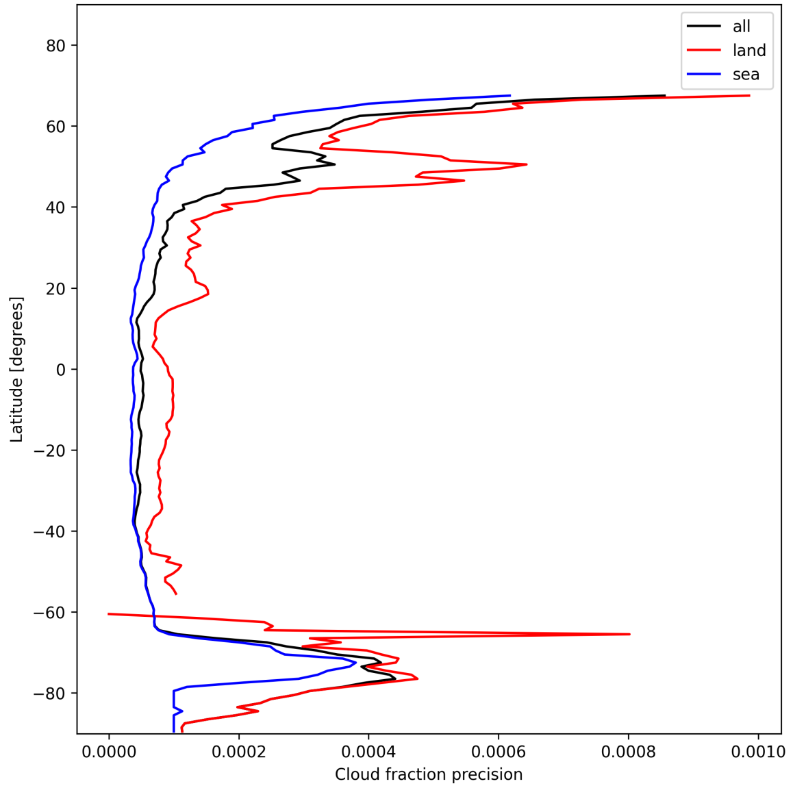
Figure 14: Zonal average of “Cloud fraction precision” for 2025-01-19 to 2025-01-20.
