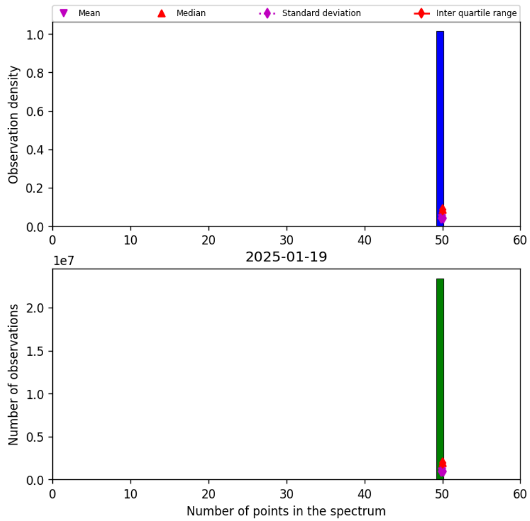
Figure 42: Histogram of “Number of points in the spectrum” for 2025-01-19 to 2025-01-20
