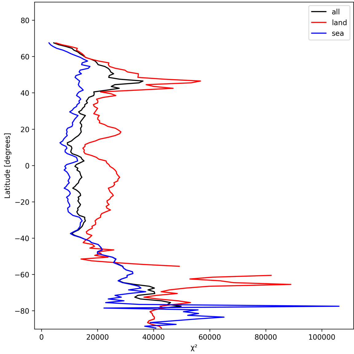
Figure 19: Zonal average of “ \chi^2 ” for 2025-01-19 to 2025-01-20.
