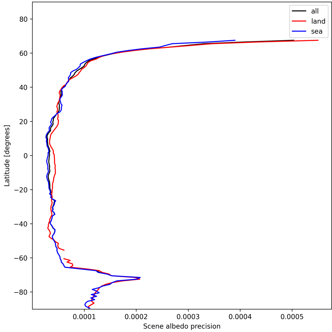
Figure 16: Zonal average of “Scene albedo precision” for 2025-01-19 to 2025-01-20.
