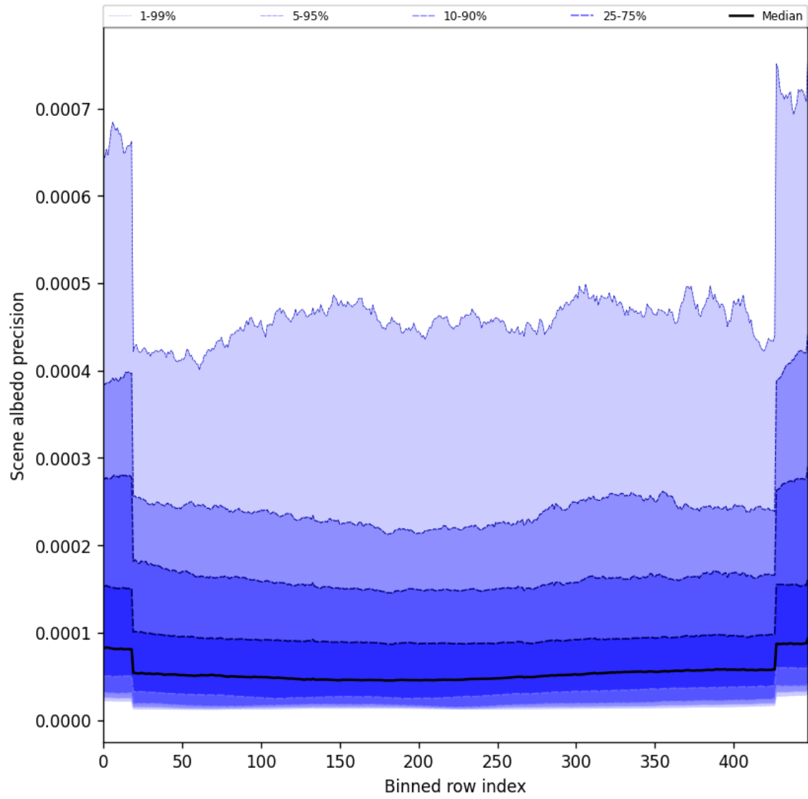
Figure 50: Along track statistics of “Scene albedo precision” for 2025-01-19 to 2025-01-20
