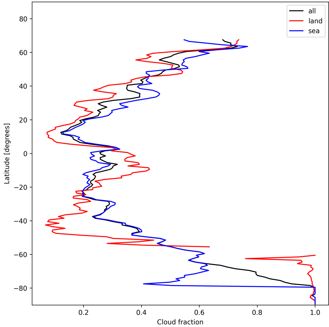
Figure 13: Zonal average of “Cloud fraction” for 2025-01-19 to 2025-01-20.
