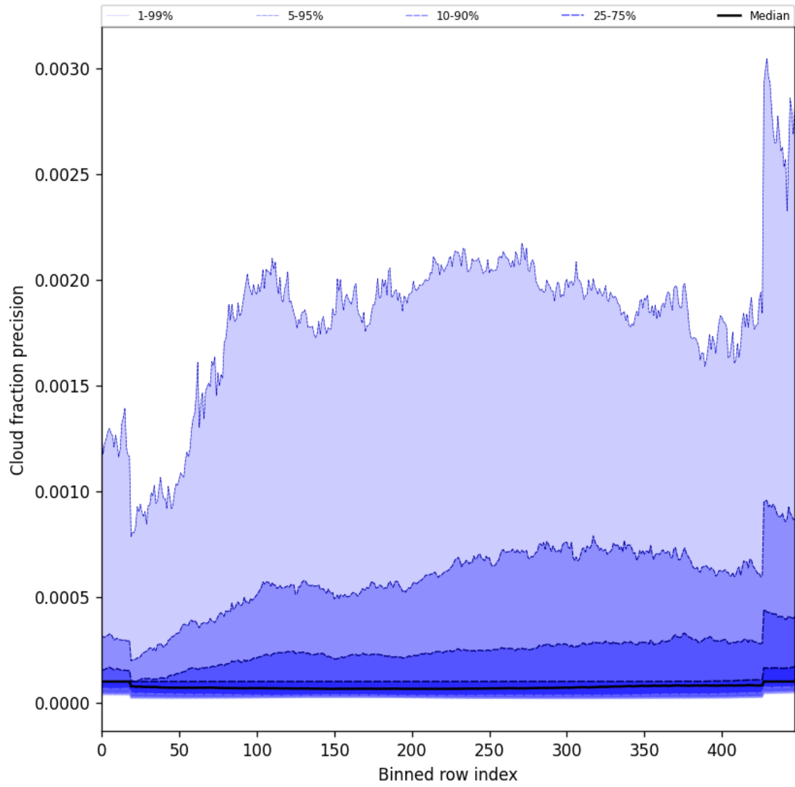
Figure 48: Along track statistics of “Cloud fraction precision” for 2025-01-19 to 2025-01-20
