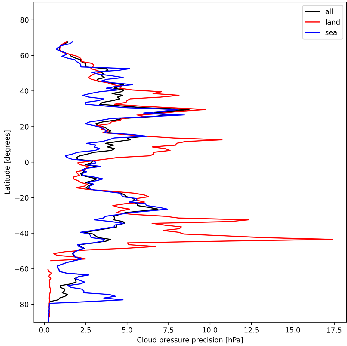
Figure 12: Zonal average of “Cloud pressure precision” for 2025-01-19 to 2025-01-20.
