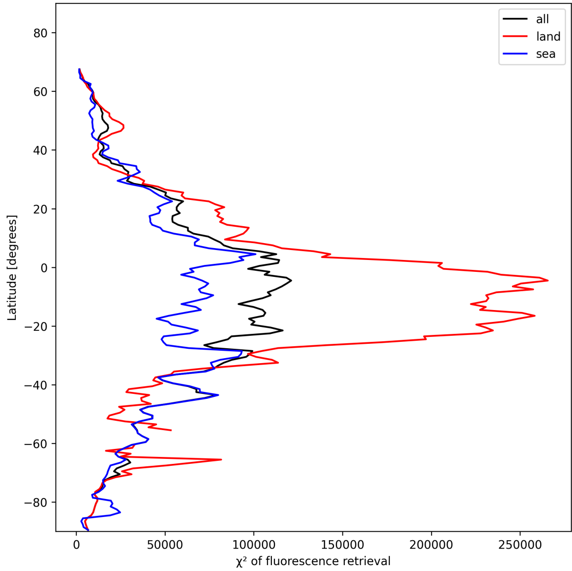
Figure 23: Zonal average of “ \chi^2 of fluorescence retrieval” for 2025-01-19 to 2025-01-20.
