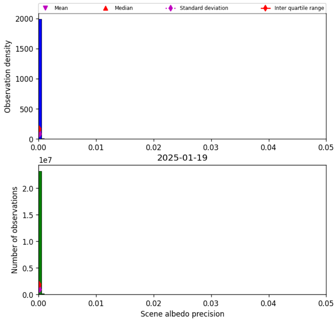
Figure 33: Histogram of “Scene albedo precision” for 2025-01-19 to 2025-01-20
