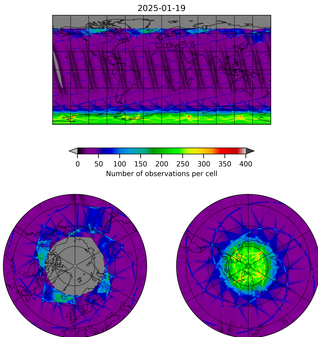
Figure 9: Map of the number of observations for 2025-01-19 to 2025-01-20
