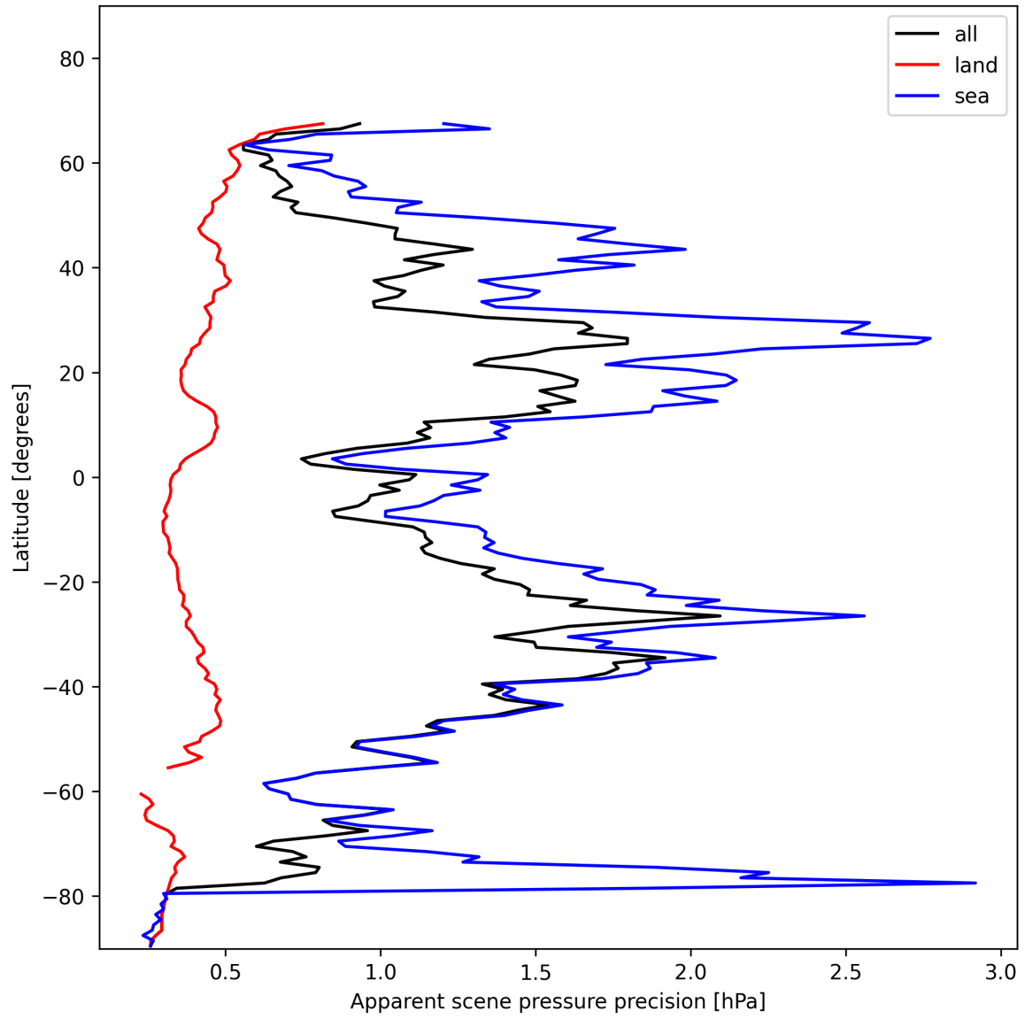
Figure 18: Zonal average of “Apparent scene pressure precision” for 2025-01-19 to 2025-01-20.
