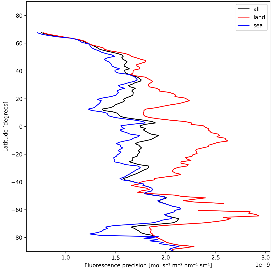
Figure 22: Zonal average of “Fluorescence precision” for 2025-01-19 to 2025-01-20.
