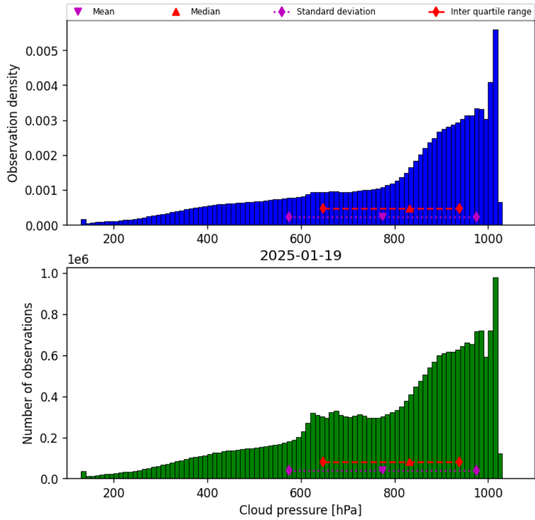
Figure 28: Histogram of “Cloud pressure” for 2025-01-19 to 2025-01-20
