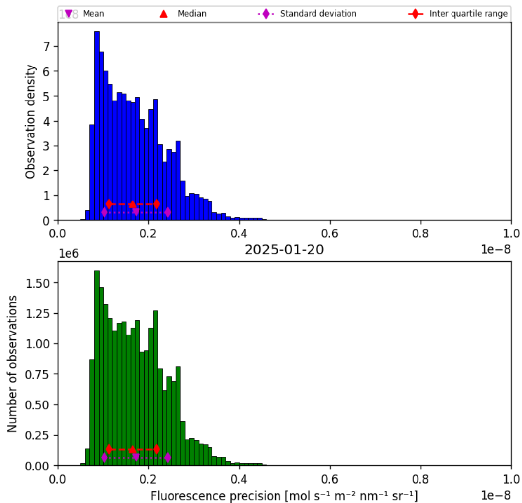
Figure 39: Histogram of “Fluorescence precision” for 2025-01-20 to 2025-01-21
