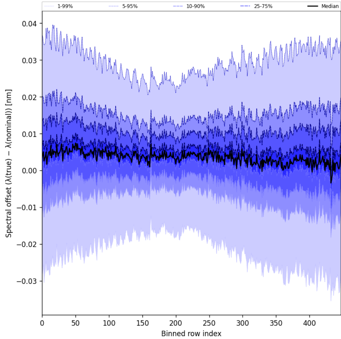
Figure 60: Along track statistics of “Spectral offset ( \lambda_{\text{true}} - \lambda_{\text{nominal}} )” for 2025-01-20 to 2025-01-21
