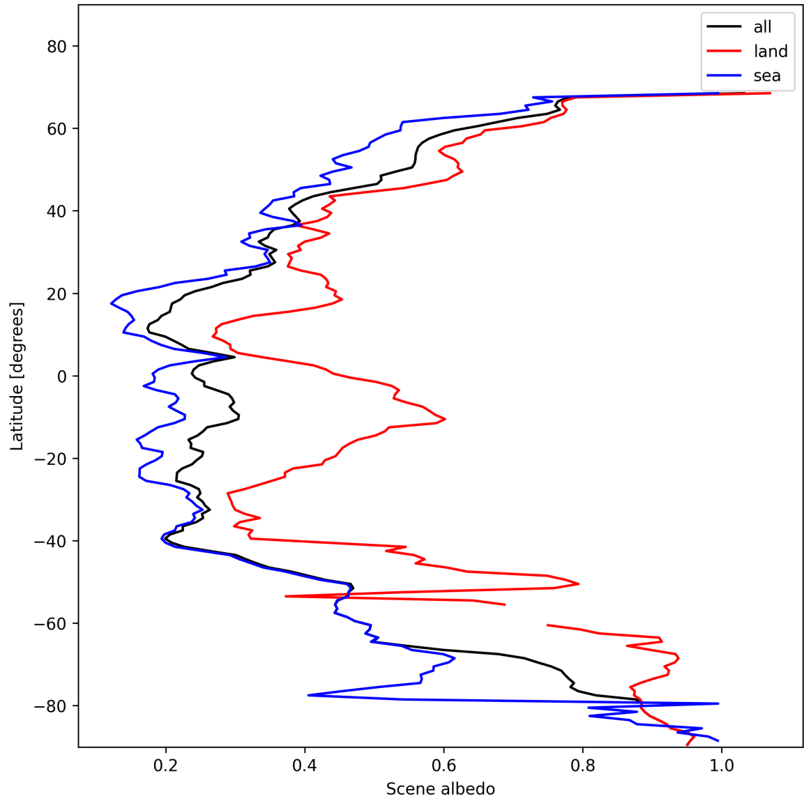
Figure 15: Zonal average of “Scene albedo” for 2025-01-20 to 2025-01-21.
