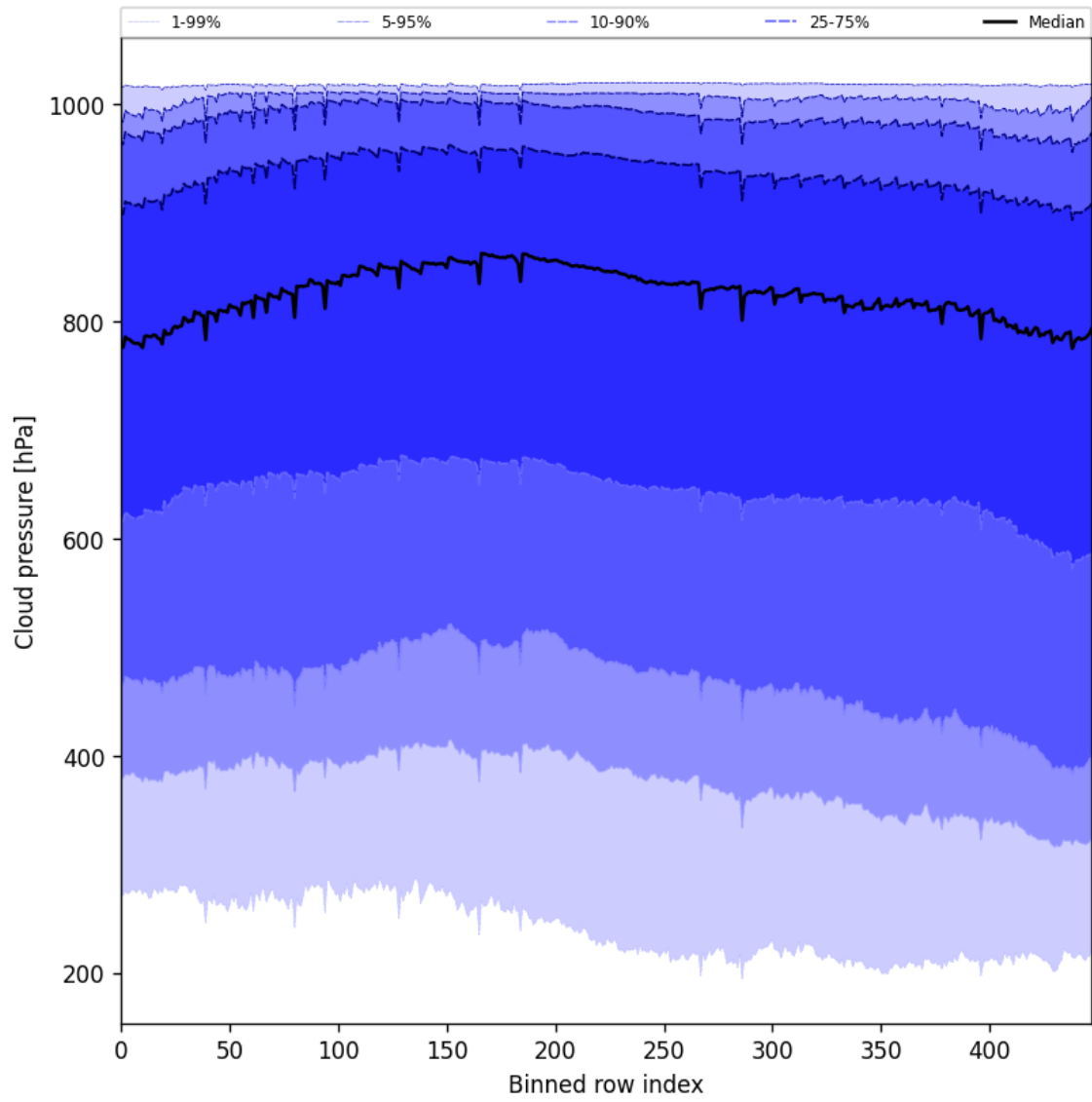
Figure 45: Along track statistics of “Cloud pressure” for 2025-01-20 to 2025-01-21
