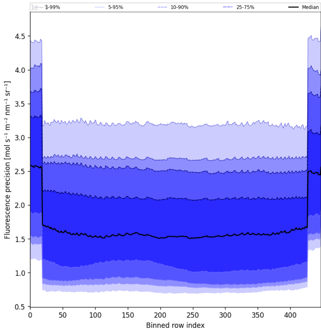
Figure 56: Along track statistics of “Fluorescence precision” for 2025-01-20 to 2025-01-21
