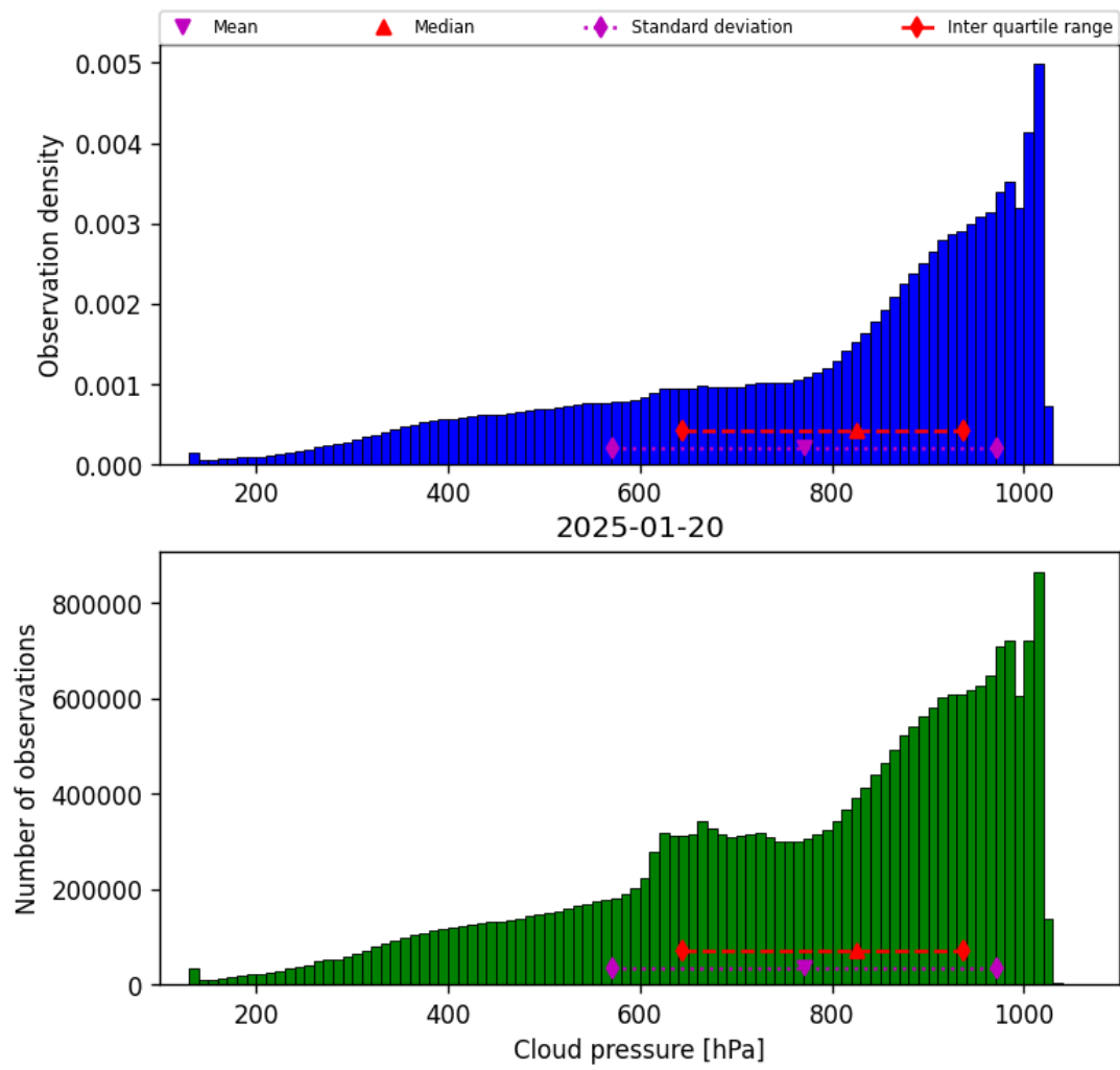
Figure 28: Histogram of “Cloud pressure” for 2025-01-20 to 2025-01-21
