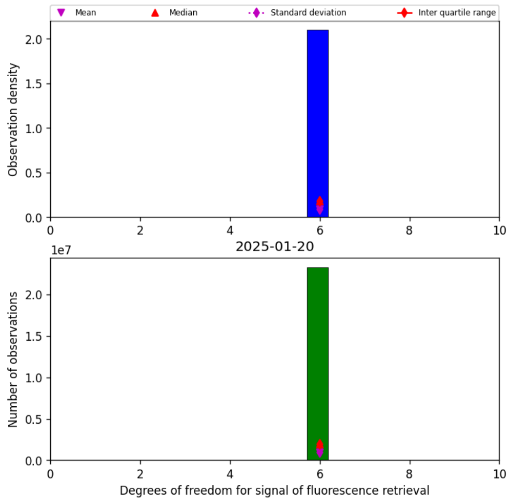
Figure 41: Histogram of “Degrees of freedom for signal of fluorescence retrieval” for 2025-01-20 to 2025-01-21
