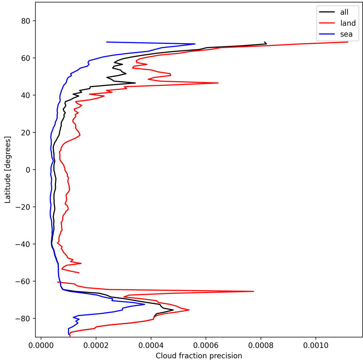
Figure 14: Zonal average of “Cloud fraction precision” for 2025-01-20 to 2025-01-21.
