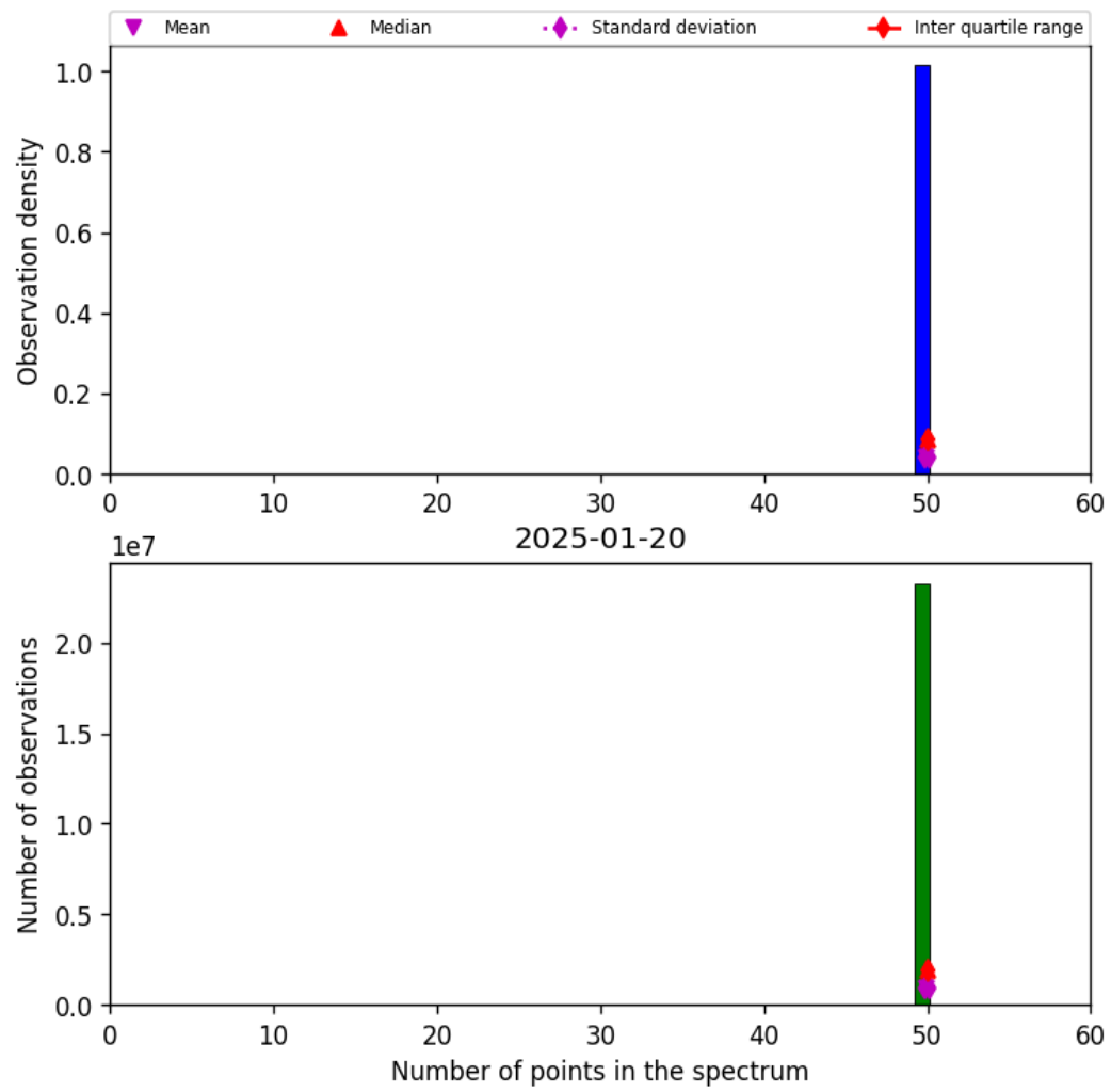
Figure 42: Histogram of “Number of points in the spectrum” for 2025-01-20 to 2025-01-21
