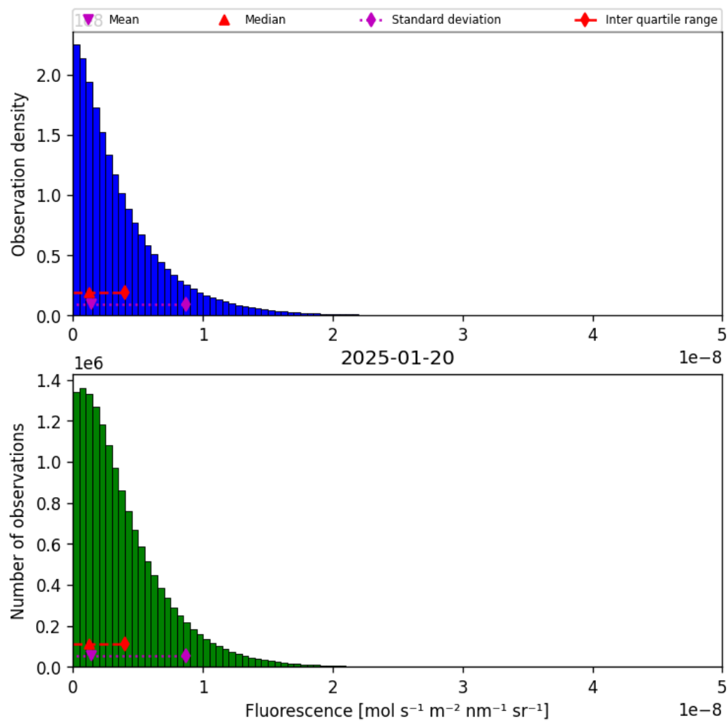
Figure 38: Histogram of “Fluorescence” for 2025-01-20 to 2025-01-21
