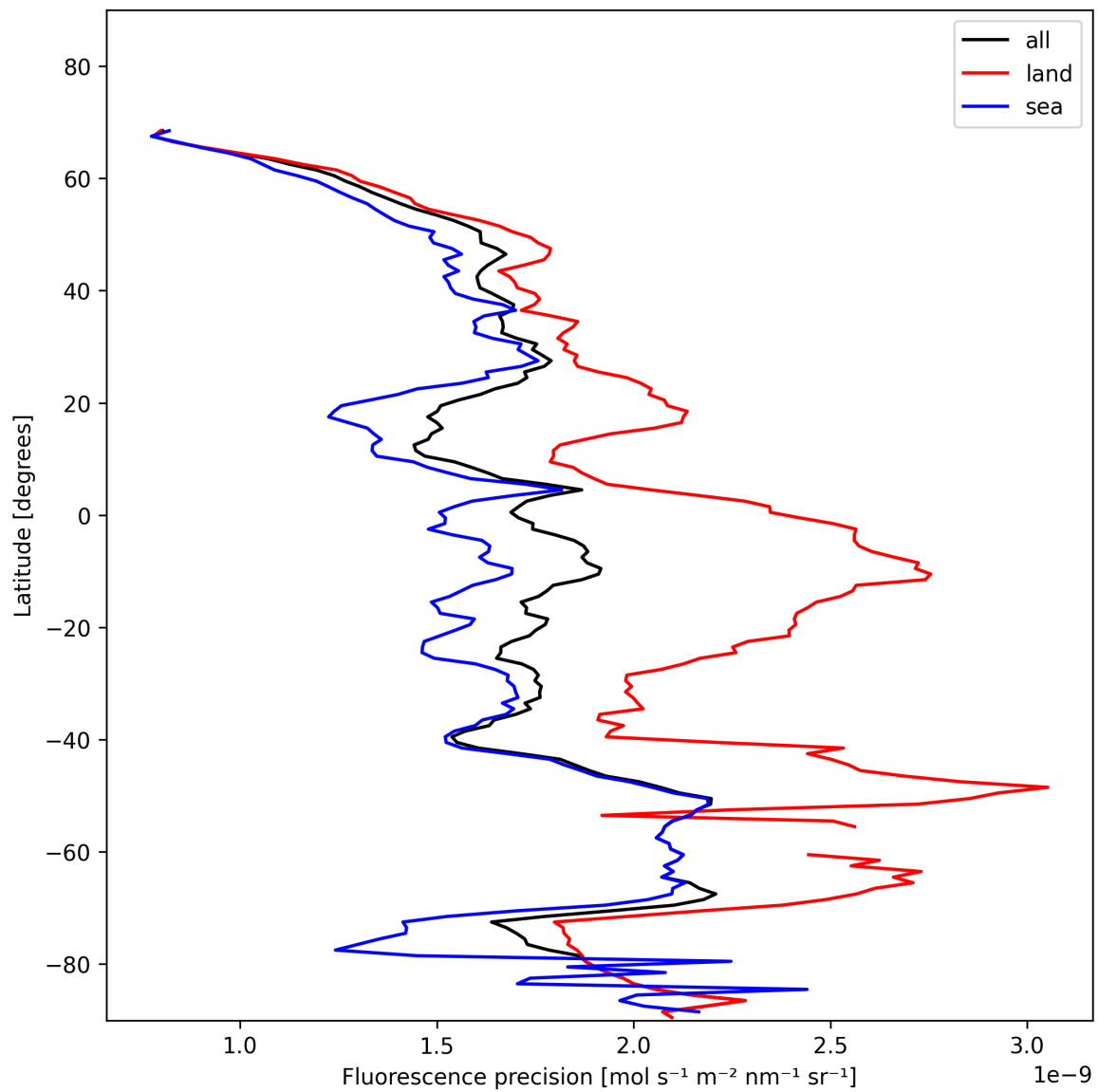
Figure 22: Zonal average of “Fluorescence precision” for 2025-01-20 to 2025-01-21.
