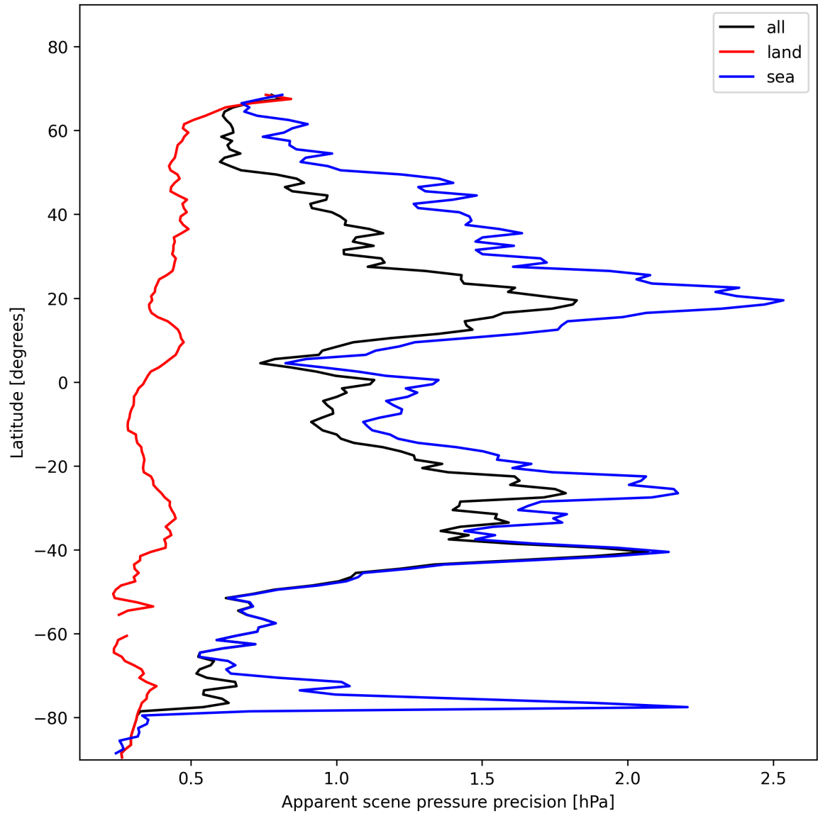
Figure 18: Zonal average of “Apparent scene pressure precision” for 2025-01-20 to 2025-01-21.
