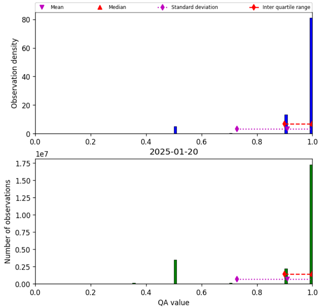
Figure 27: Histogram of “QA value” for 2025-01-20 to 2025-01-21
