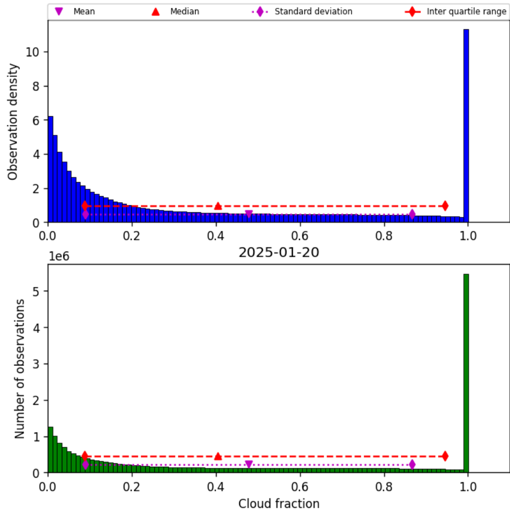
Figure 30: Histogram of “Cloud fraction” for 2025-01-20 to 2025-01-21
