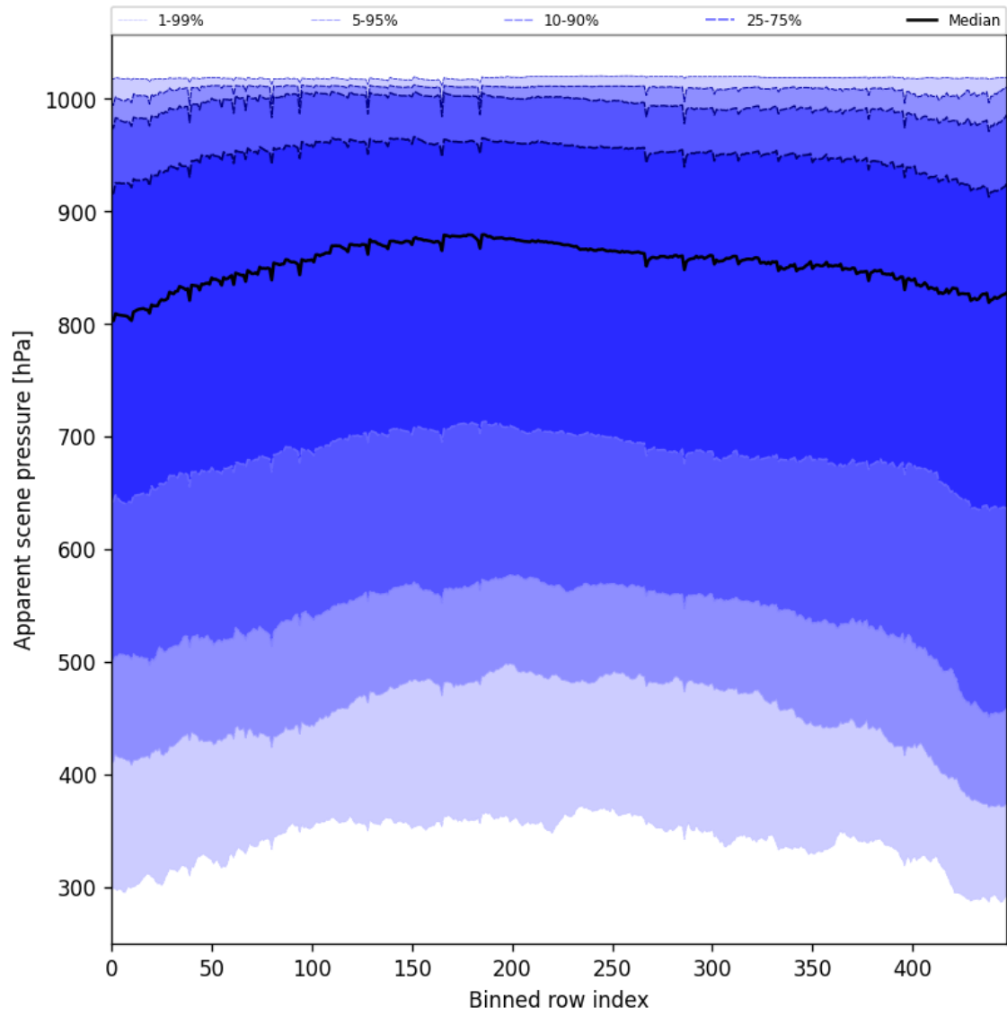
Figure 51: Along track statistics of “Apparent scene pressure” for 2025-01-20 to 2025-01-21
