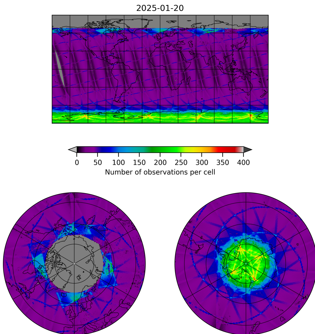
Figure 9: Map of the number of observations for 2025-01-20 to 2025-01-21
