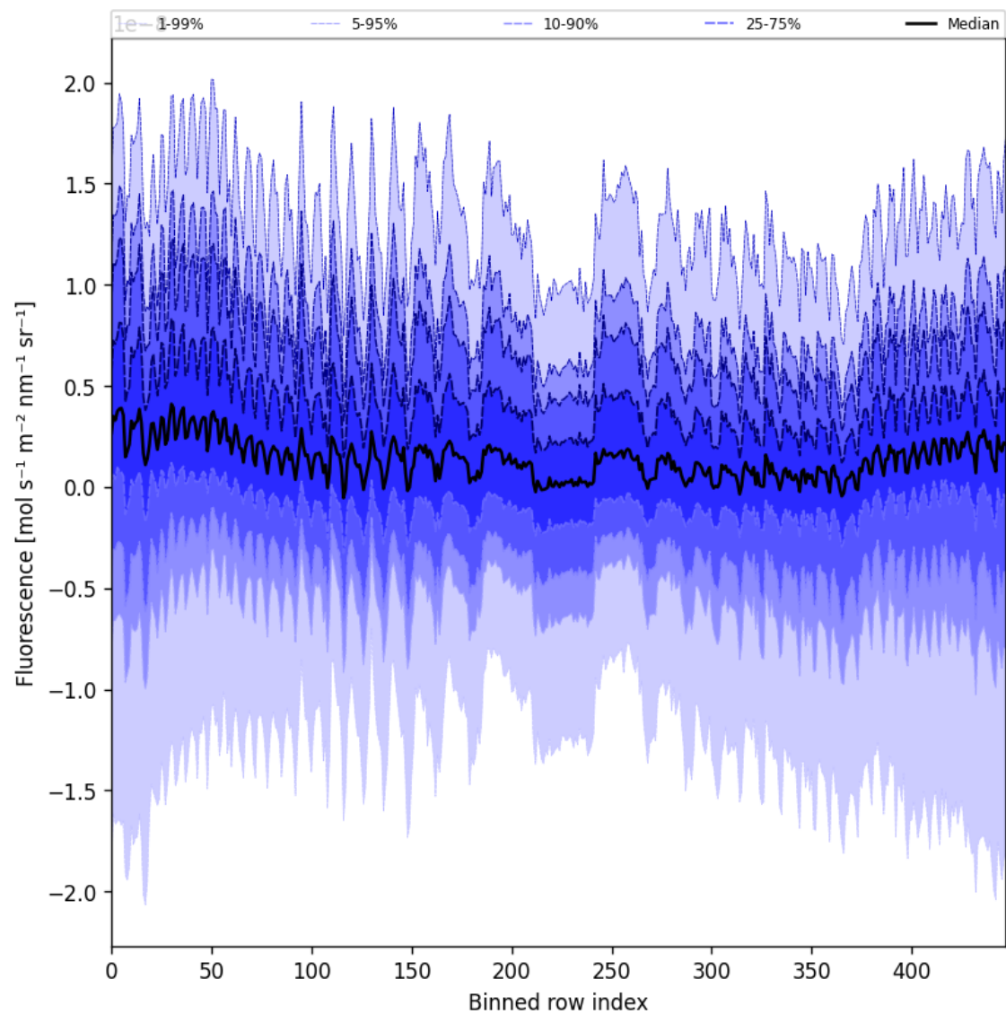
Figure 55: Along track statistics of “Fluorescence” for 2025-01-20 to 2025-01-21
