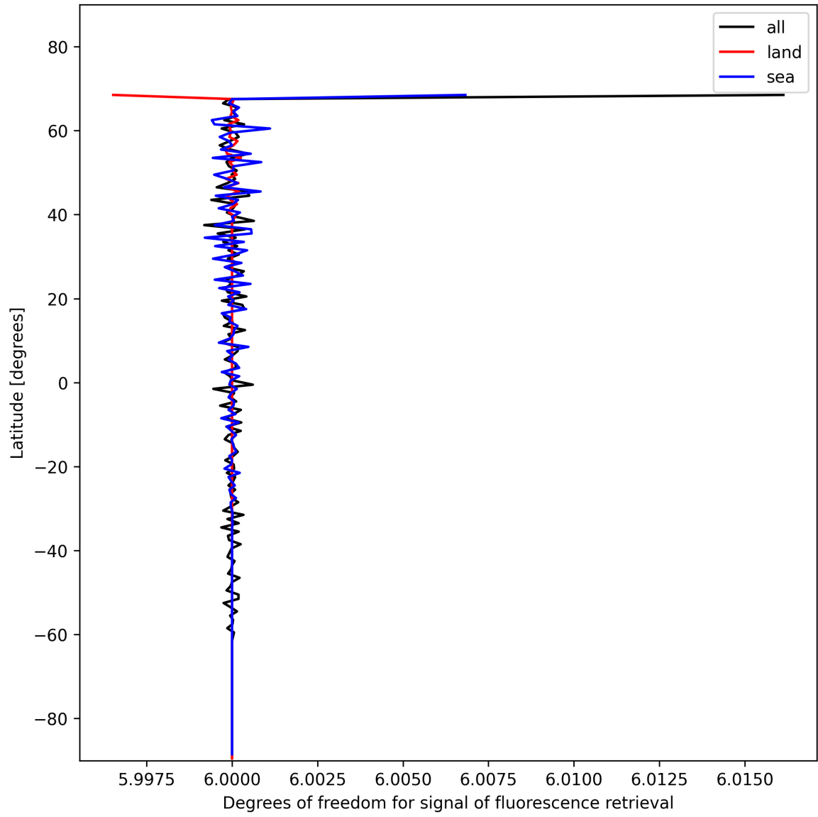
Figure 24: Zonal average of “Degrees of freedom for signal of fluorescence retrieval” for 2025-01-20 to 2025-01-21.
