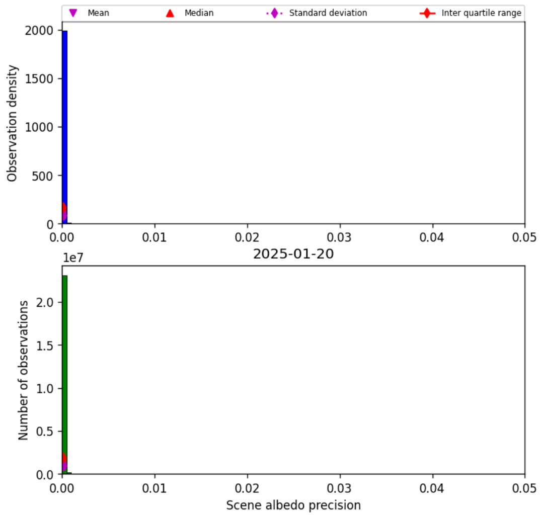
Figure 33: Histogram of “Scene albedo precision” for 2025-01-20 to 2025-01-21
