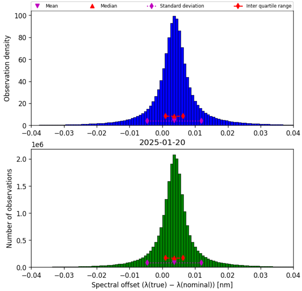
Figure 43: Histogram of “Spectral offset ( \lambda_{\text{true}} - \lambda_{\text{nominal}} )” for 2025-01-20 to 2025-01-21
