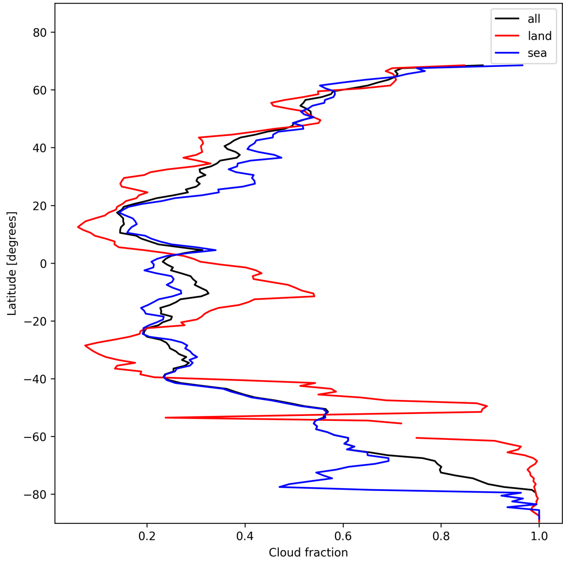
Figure 13: Zonal average of “Cloud fraction” for 2025-01-20 to 2025-01-21.
