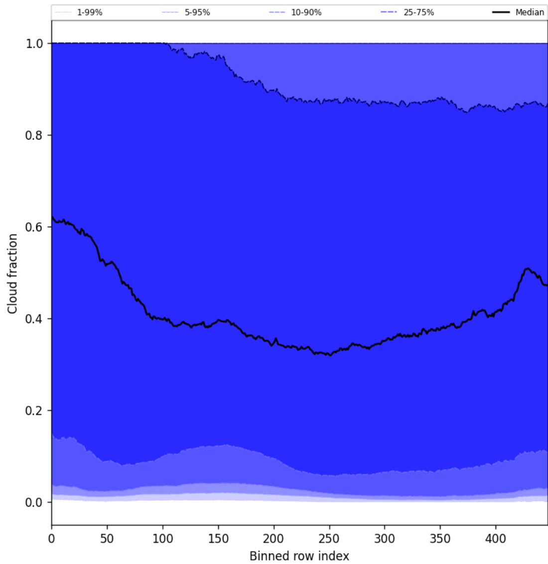
Figure 47: Along track statistics of “Cloud fraction” for 2025-01-20 to 2025-01-21
