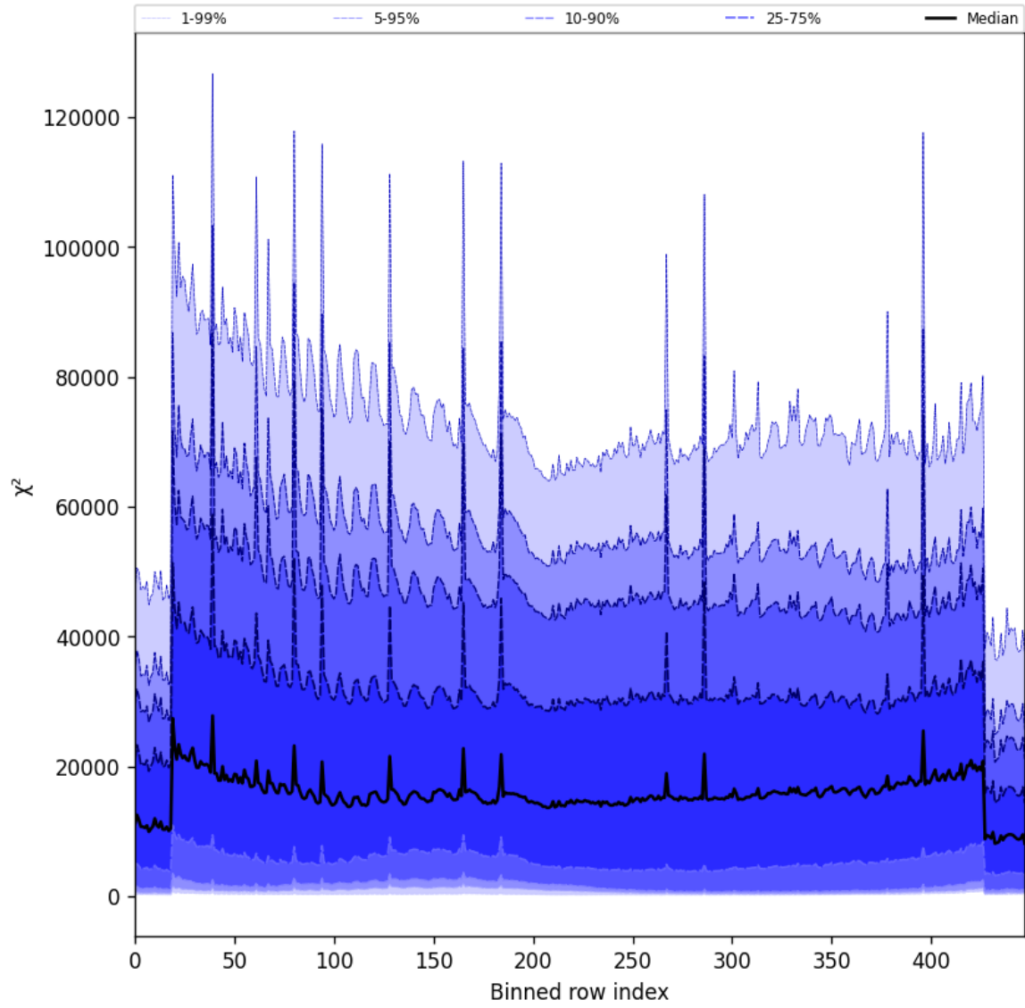
Figure 53: Along track statistics of “ \chi^2 ” for 2025-01-20 to 2025-01-21
