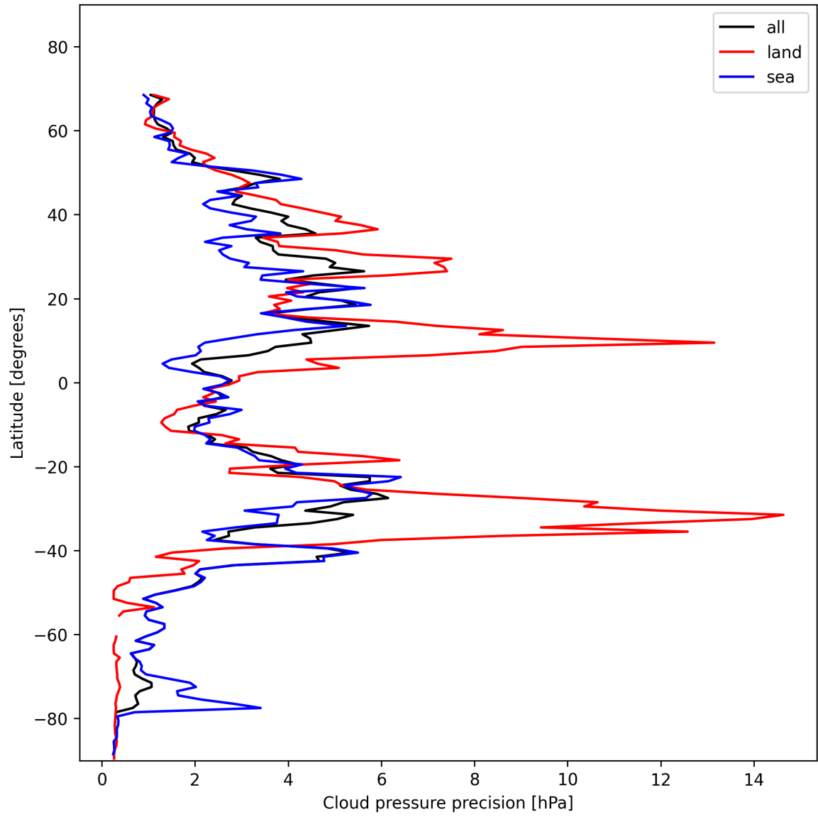
Figure 12: Zonal average of "Cloud pressure precision" for 2025-01-20 to 2025-01-21.
