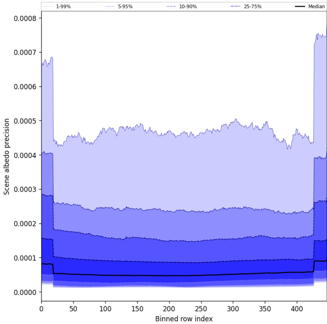
Figure 50: Along track statistics of “Scene albedo precision” for 2025-01-20 to 2025-01-21
