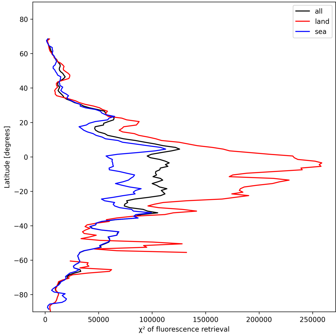
Figure 23: Zonal average of “ \chi^2 of fluorescence retrieval” for 2025-01-20 to 2025-01-21.
