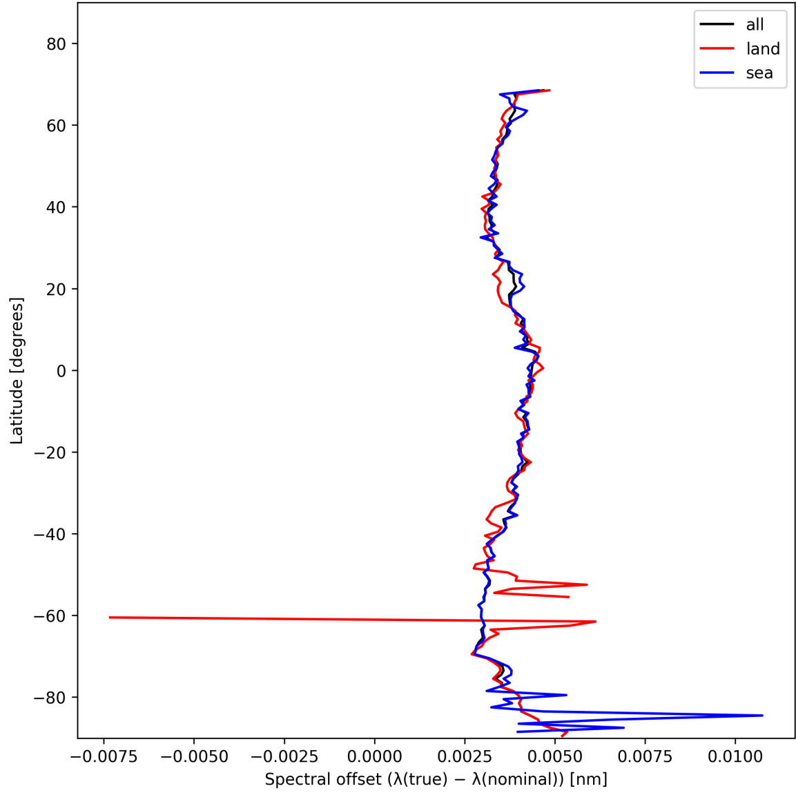
Figure 26: Zonal average of “Spectral offset ( \lambda_{\text{true}} - \lambda_{\text{nominal}} )” for 2025-01-20 to 2025-01-21.
