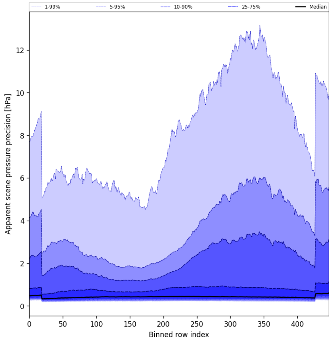
Figure 52: Along track statistics of “Apparent scene pressure precision” for 2025-01-20 to 2025-01-21
