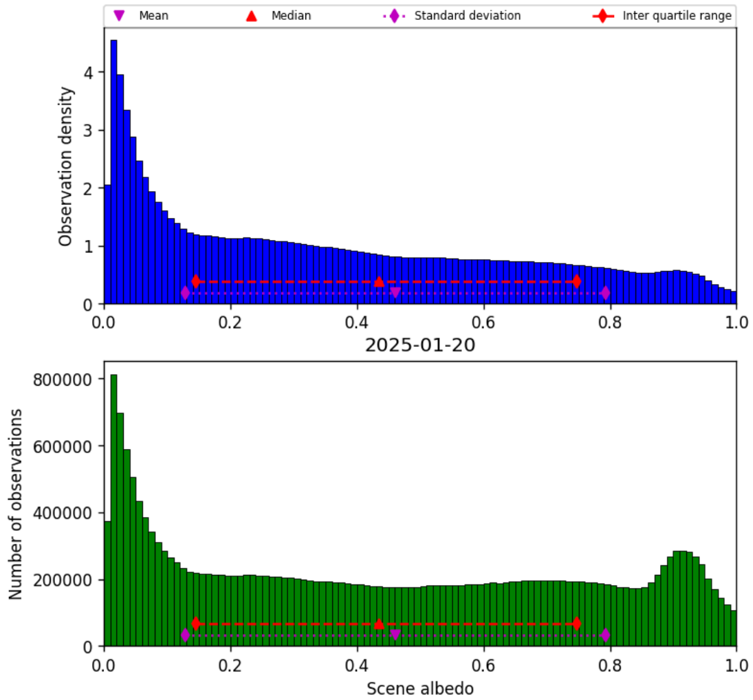
Figure 32: Histogram of “Scene albedo” for 2025-01-20 to 2025-01-21
