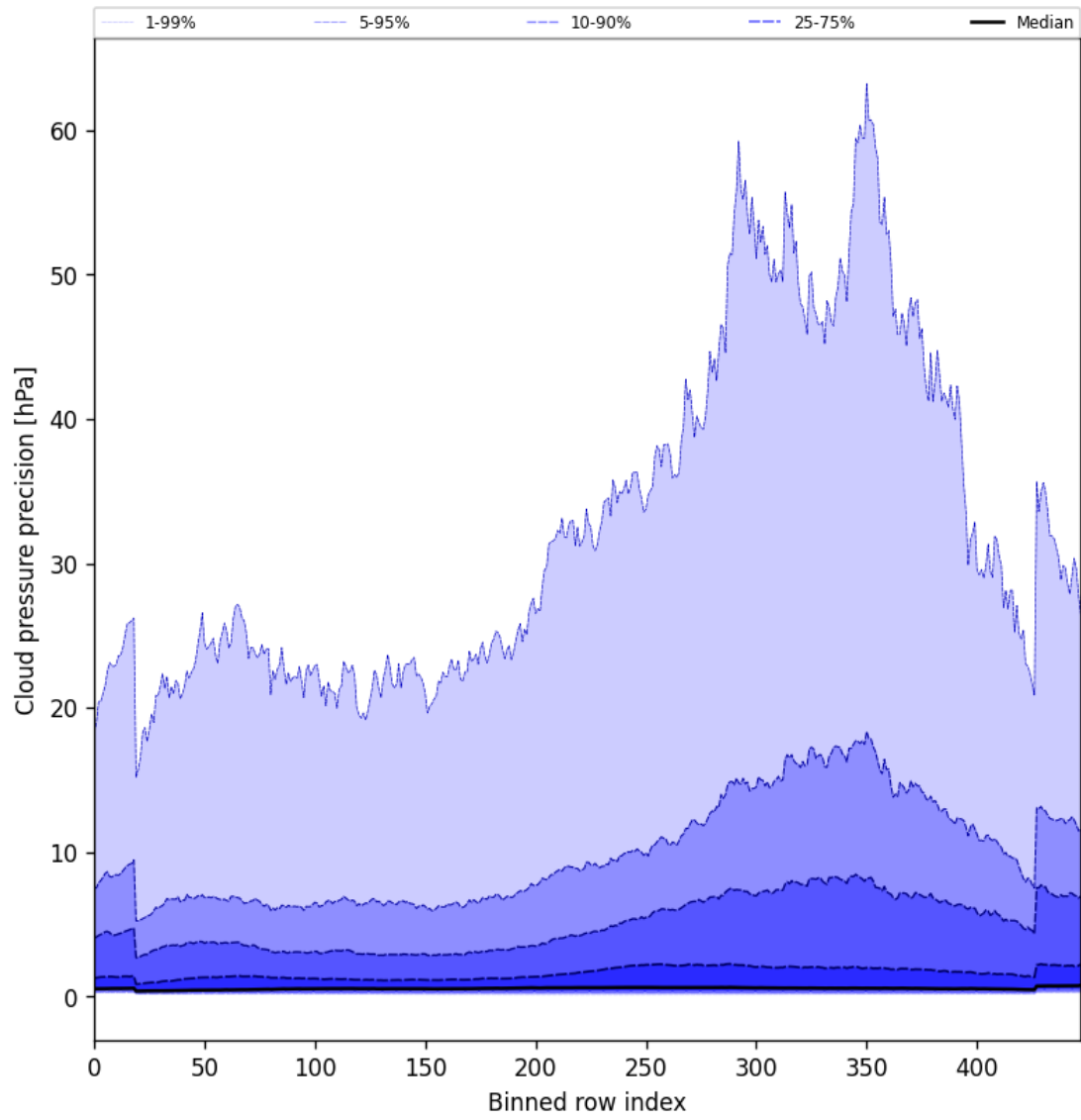
Figure 46: Along track statistics of “Cloud pressure precision” for 2025-01-20 to 2025-01-21
