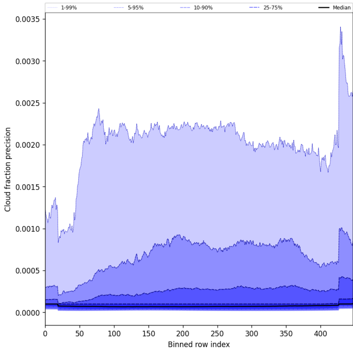
Figure 48: Along track statistics of “Cloud fraction precision” for 2025-01-20 to 2025-01-21
