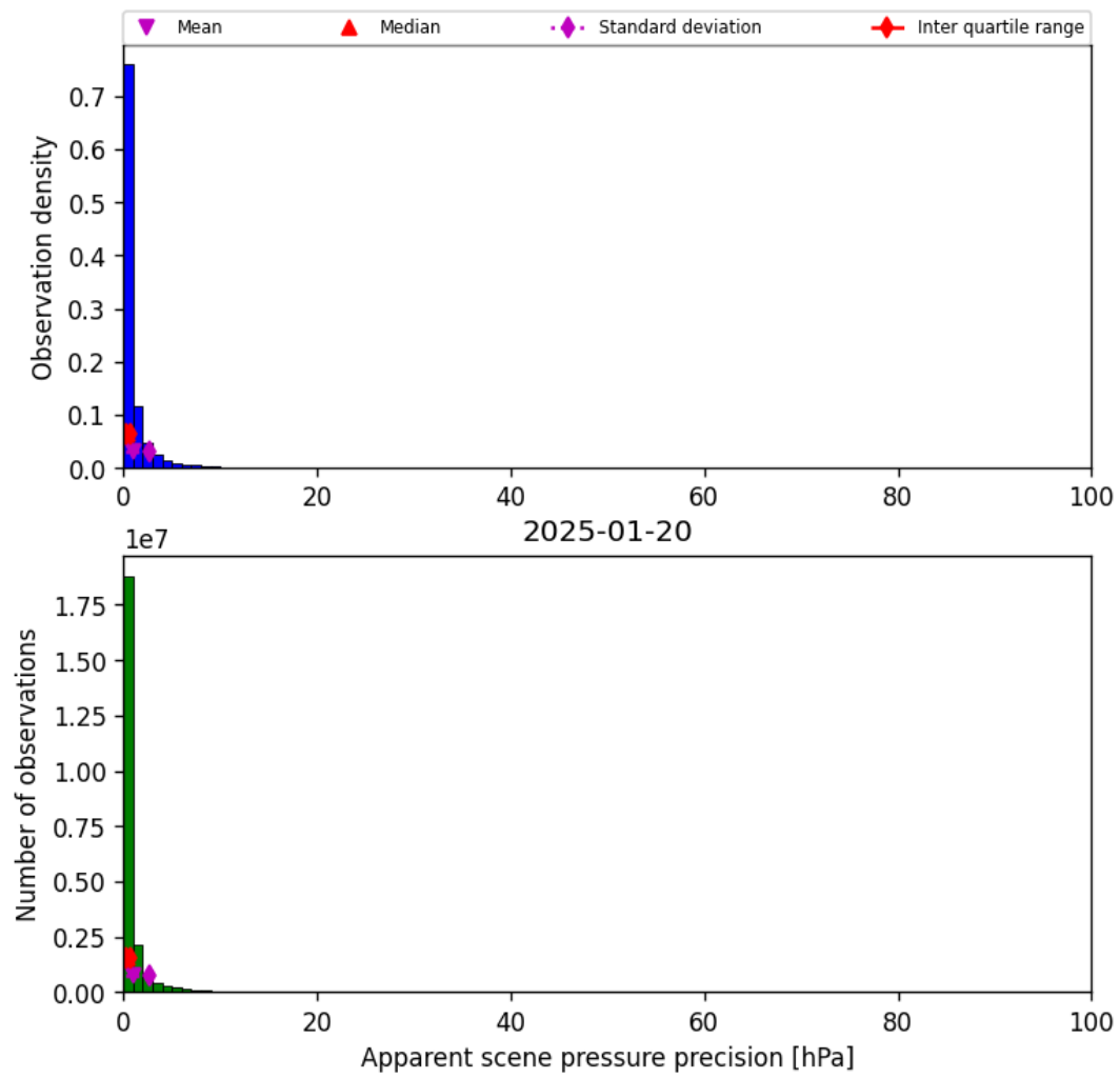
Figure 35: Histogram of “Apparent scene pressure precision” for 2025-01-20 to 2025-01-21
