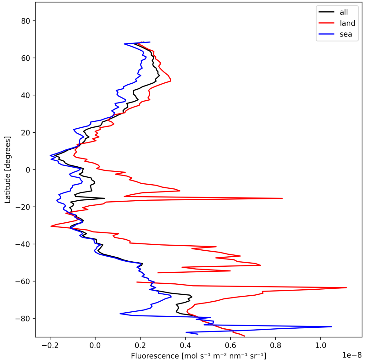
Figure 21: Zonal average of “Fluorescence” for 2025-01-20 to 2025-01-21.
