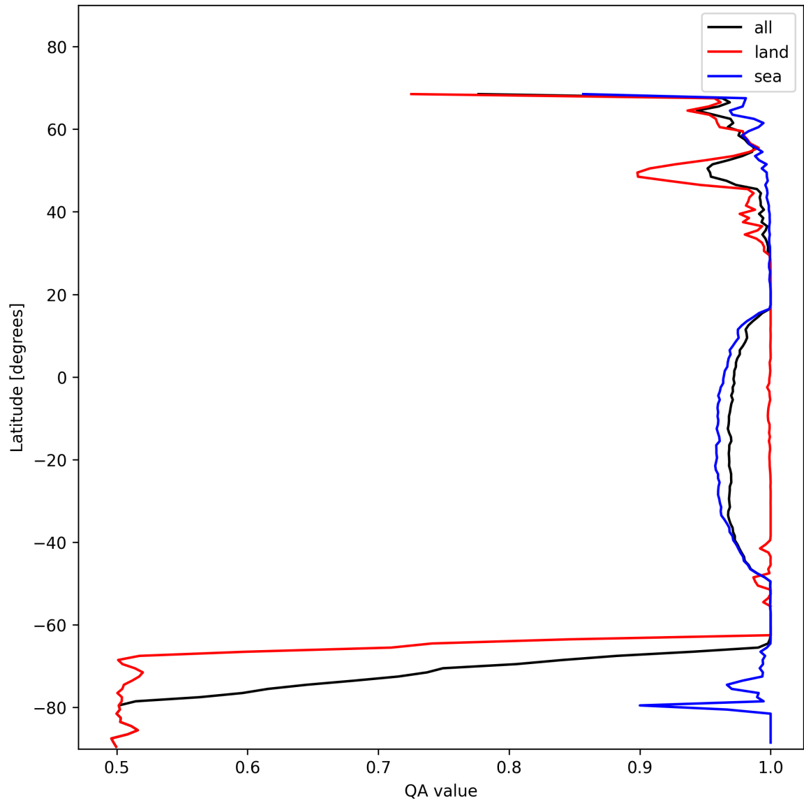
Figure 10: Zonal average of “QA value” for 2025-01-20 to 2025-01-21.
