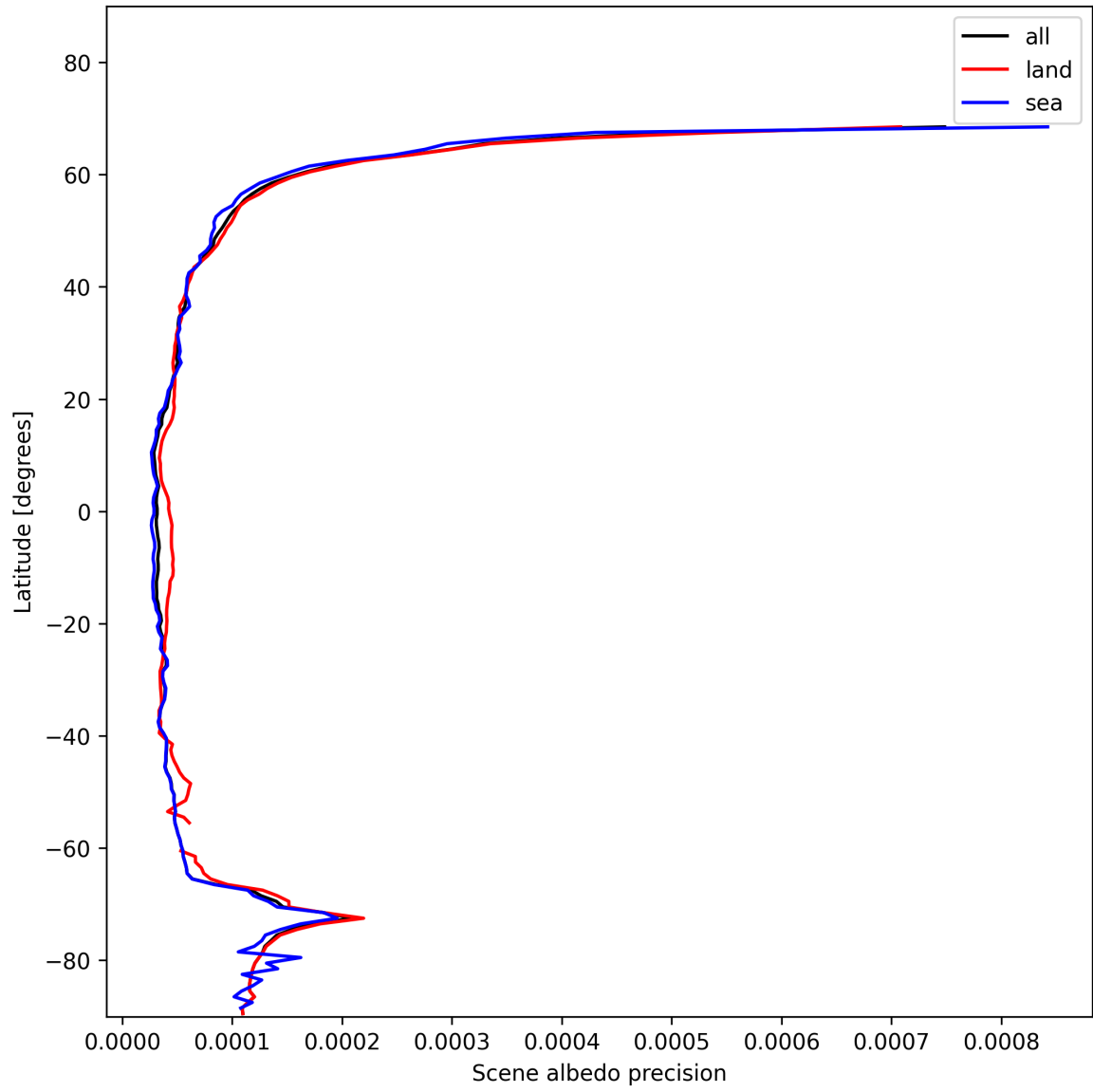
Figure 16: Zonal average of “Scene albedo precision” for 2025-01-20 to 2025-01-21.
