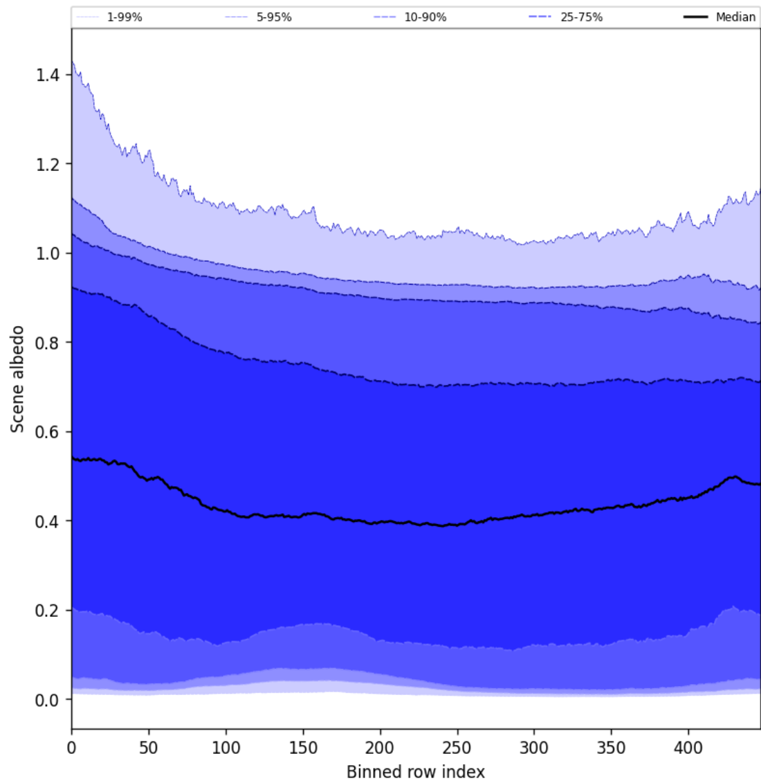
Figure 49: Along track statistics of “Scene albedo” for 2025-01-20 to 2025-01-21
