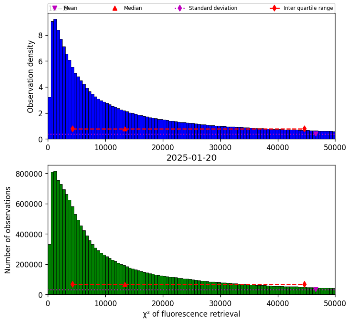
Figure 40: Histogram of “ \chi^2 of fluorescence retrieval” for 2025-01-20 to 2025-01-21
