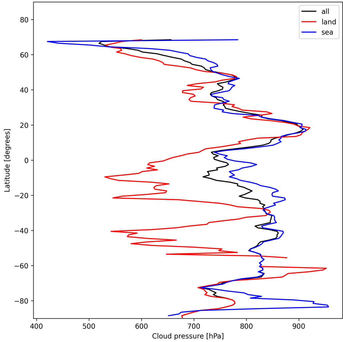
Figure 11: Zonal average of “Cloud pressure” for 2025-01-20 to 2025-01-21.
