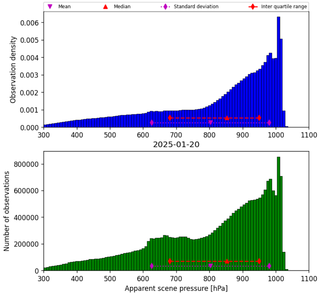
Figure 34: Histogram of “Apparent scene pressure” for 2025-01-20 to 2025-01-21
