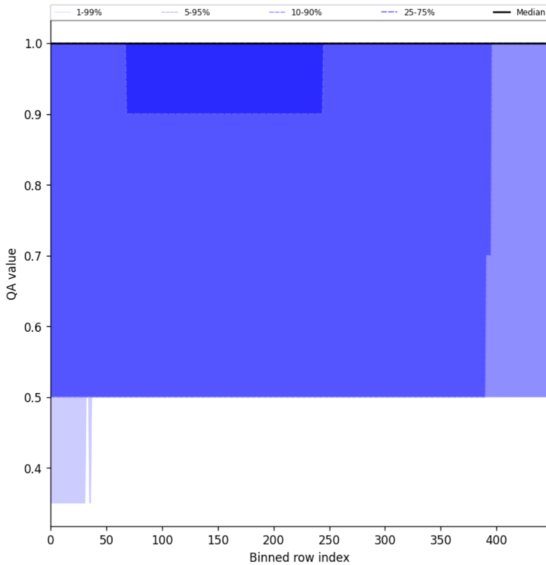
Figure 44: Along track statistics of “QA value” for 2025-01-20 to 2025-01-21
