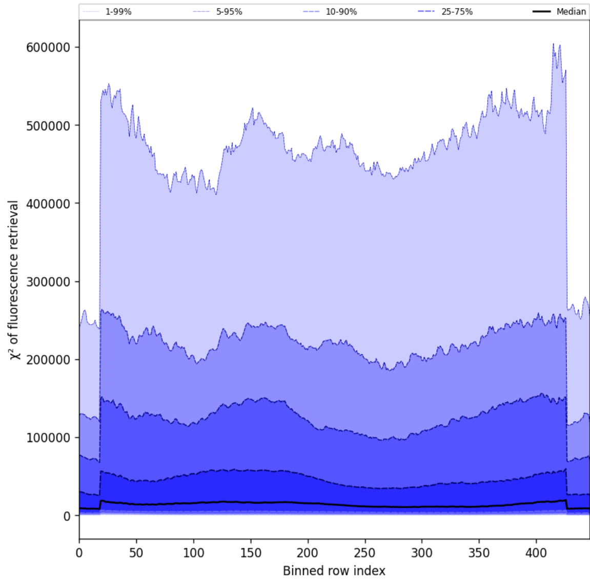
Figure 57: Along track statistics of “ \chi^2 of fluorescence retrieval” for 2025-01-20 to 2025-01-21
