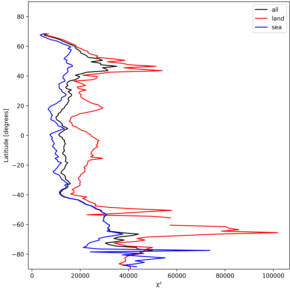
Figure 19: Zonal average of “ \chi^2 ” for 2025-01-20 to 2025-01-21.
