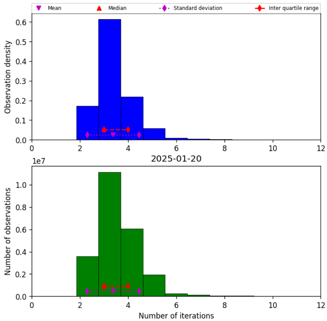
Figure 37: Histogram of “Number of iterations” for 2025-01-20 to 2025-01-21
