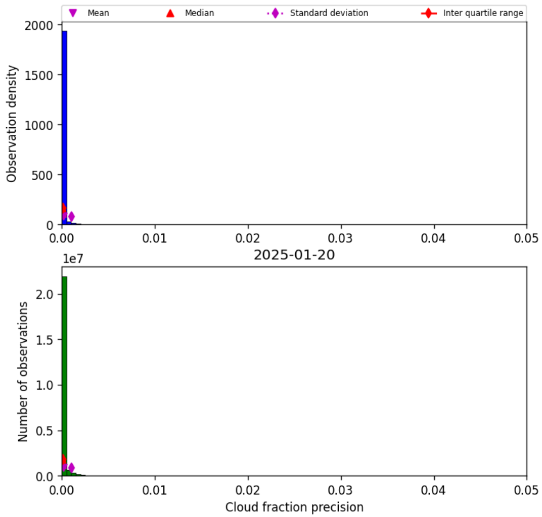
Figure 31: Histogram of “Cloud fraction precision” for 2025-01-20 to 2025-01-21
