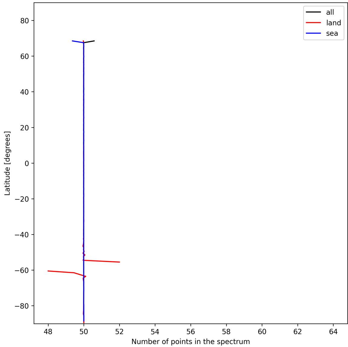
Figure 25: Zonal average of “Number of points in the spectrum” for 2025-01-20 to 2025-01-21.
