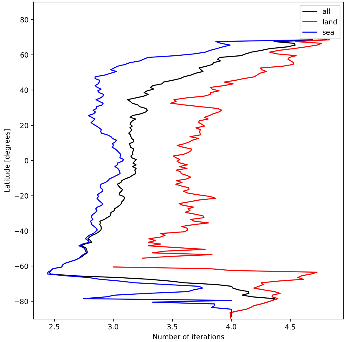
Figure 20: Zonal average of “Number of iterations” for 2025-01-20 to 2025-01-21.
