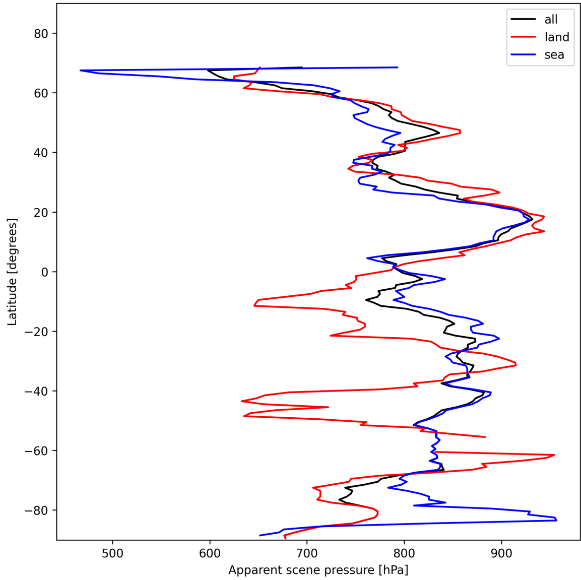
Figure 17: Zonal average of “Apparent scene pressure” for 2025-01-20 to 2025-01-21.
