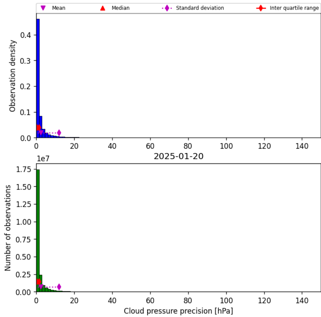
Figure 29: Histogram of “Cloud pressure precision” for 2025-01-20 to 2025-01-21
