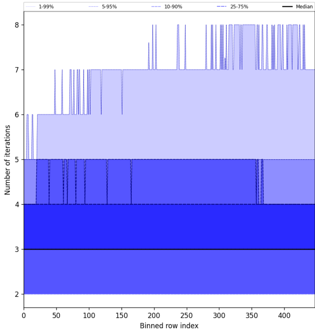
Figure 54: Along track statistics of “Number of iterations” for 2025-01-20 to 2025-01-21
