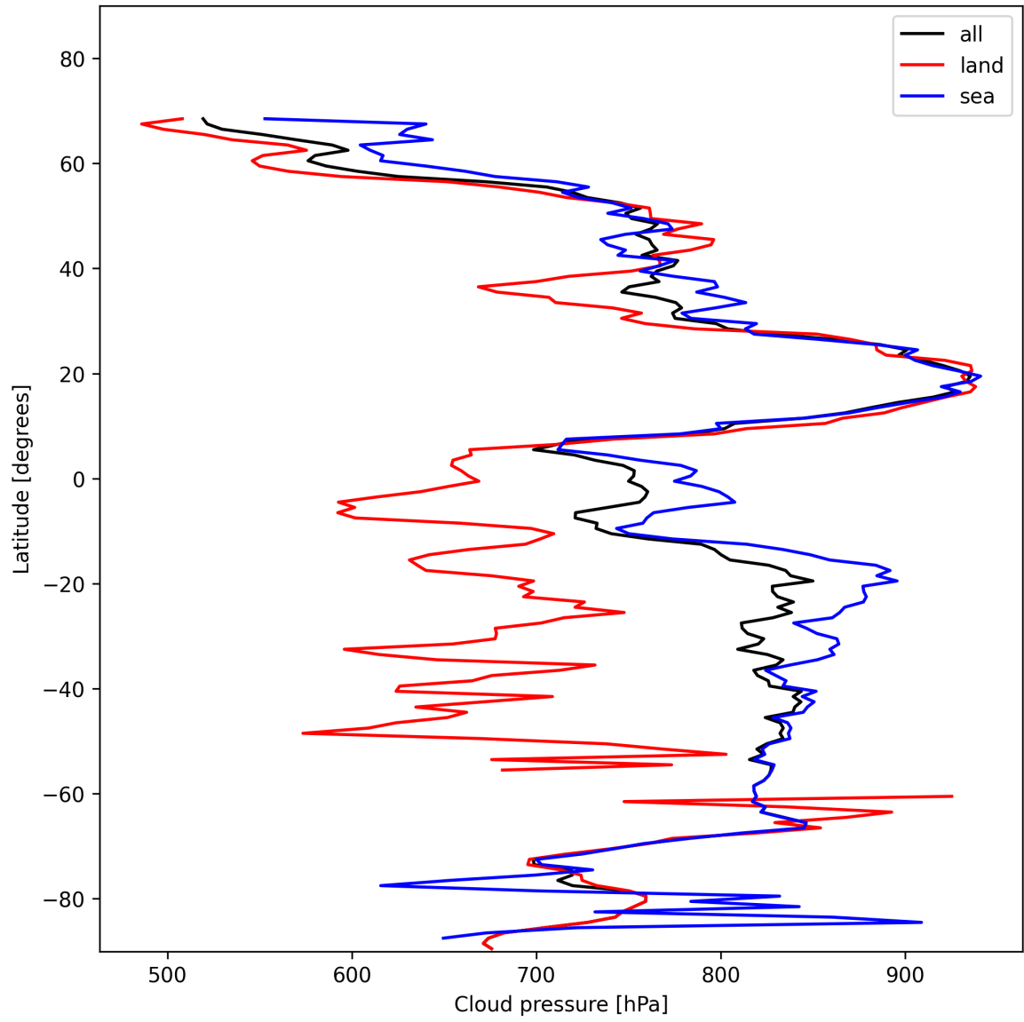
Figure 11: Zonal average of “Cloud pressure” for 2025-01-23 to 2025-01-24.
