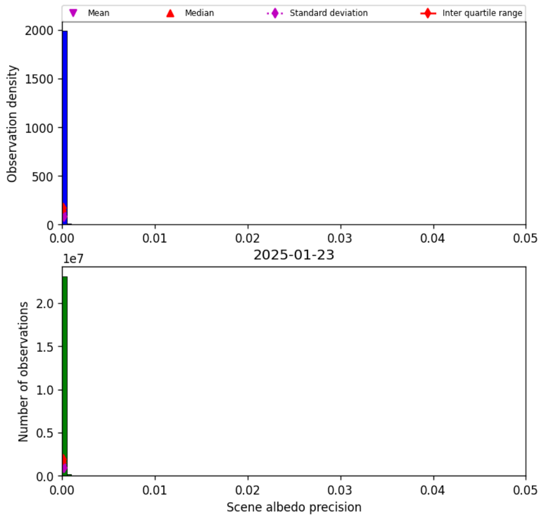
Figure 33: Histogram of “Scene albedo precision” for 2025-01-23 to 2025-01-24
