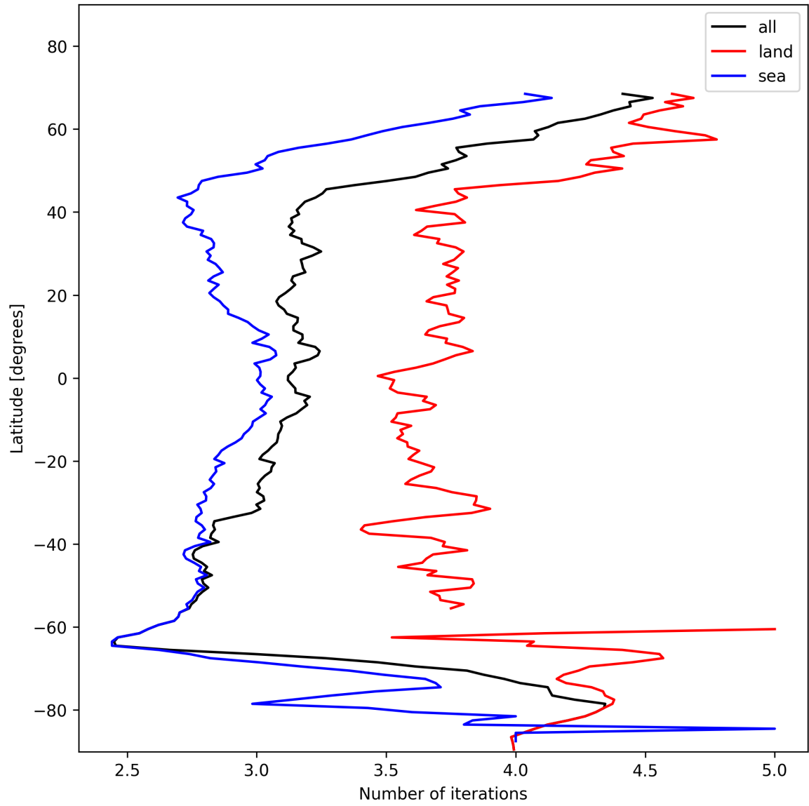
Figure 20: Zonal average of “Number of iterations” for 2025-01-23 to 2025-01-24.
