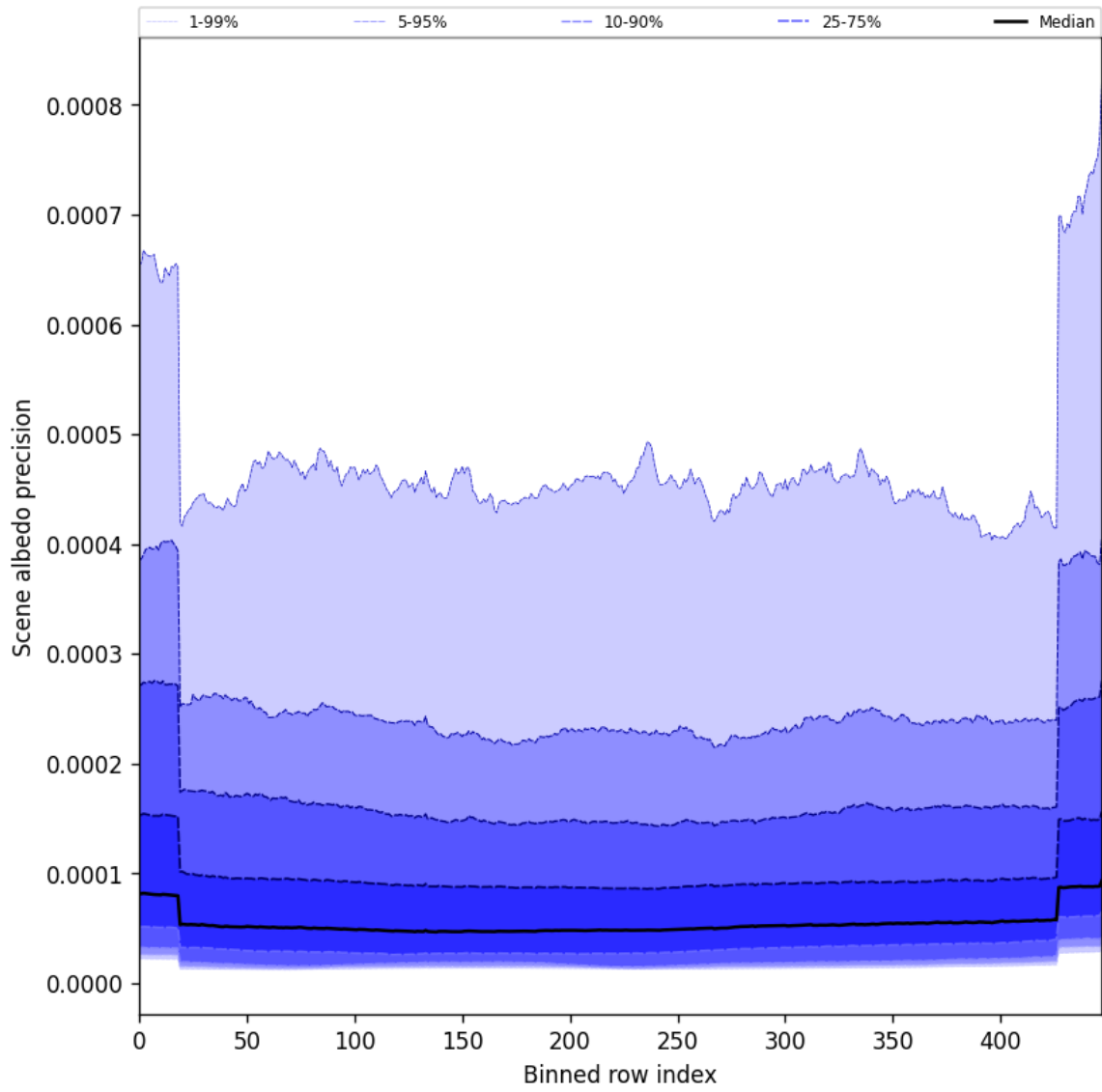
Figure 50: Along track statistics of “Scene albedo precision” for 2025-01-23 to 2025-01-24
