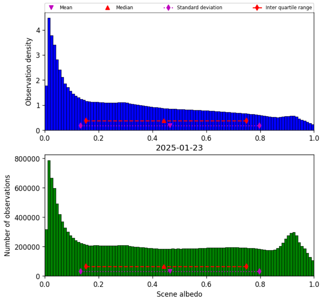
Figure 32: Histogram of “Scene albedo” for 2025-01-23 to 2025-01-24
