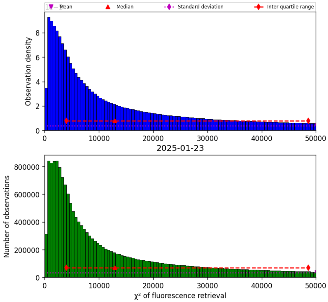
Figure 40: Histogram of “ \chi^2 of fluorescence retrieval” for 2025-01-23 to 2025-01-24
