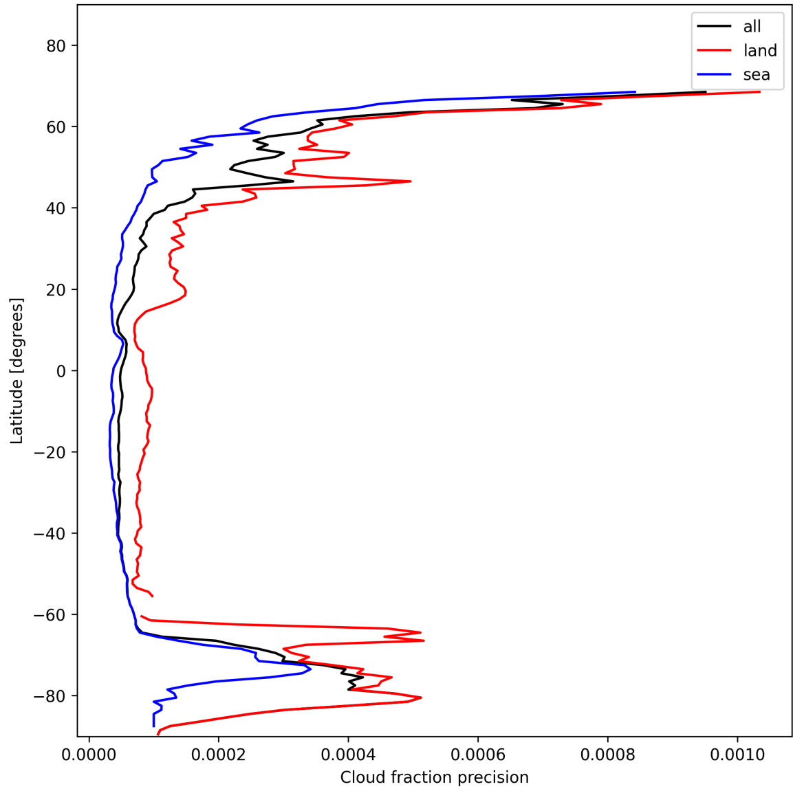
Figure 14: Zonal average of “Cloud fraction precision” for 2025-01-23 to 2025-01-24.
