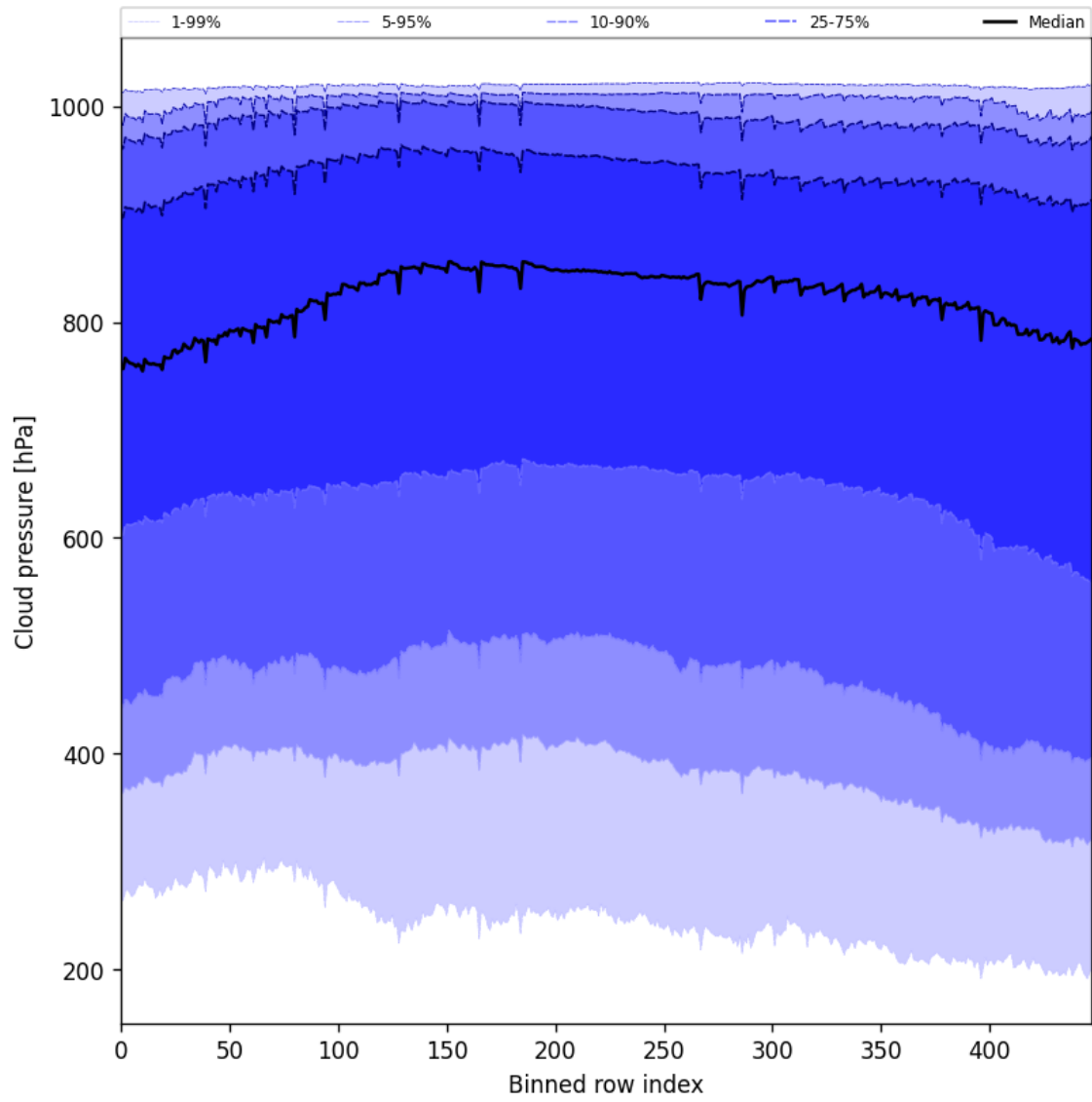
Figure 45: Along track statistics of “Cloud pressure” for 2025-01-23 to 2025-01-24
