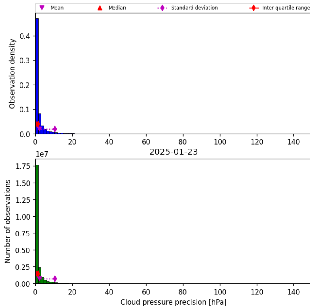
Figure 29: Histogram of “Cloud pressure precision” for 2025-01-23 to 2025-01-24
