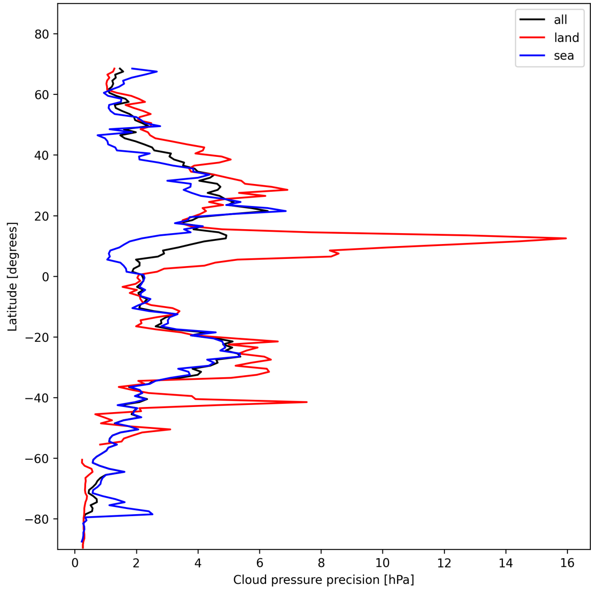
Figure 12: Zonal average of “Cloud pressure precision” for 2025-01-23 to 2025-01-24.
