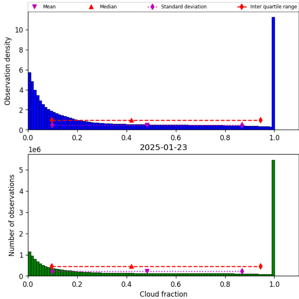
Figure 30: Histogram of “Cloud fraction” for 2025-01-23 to 2025-01-24
