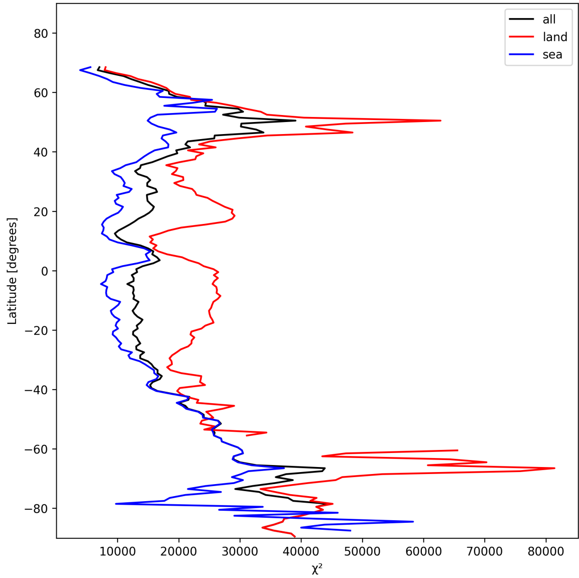
Figure 19: Zonal average of “ \chi^2 ” for 2025-01-23 to 2025-01-24.
