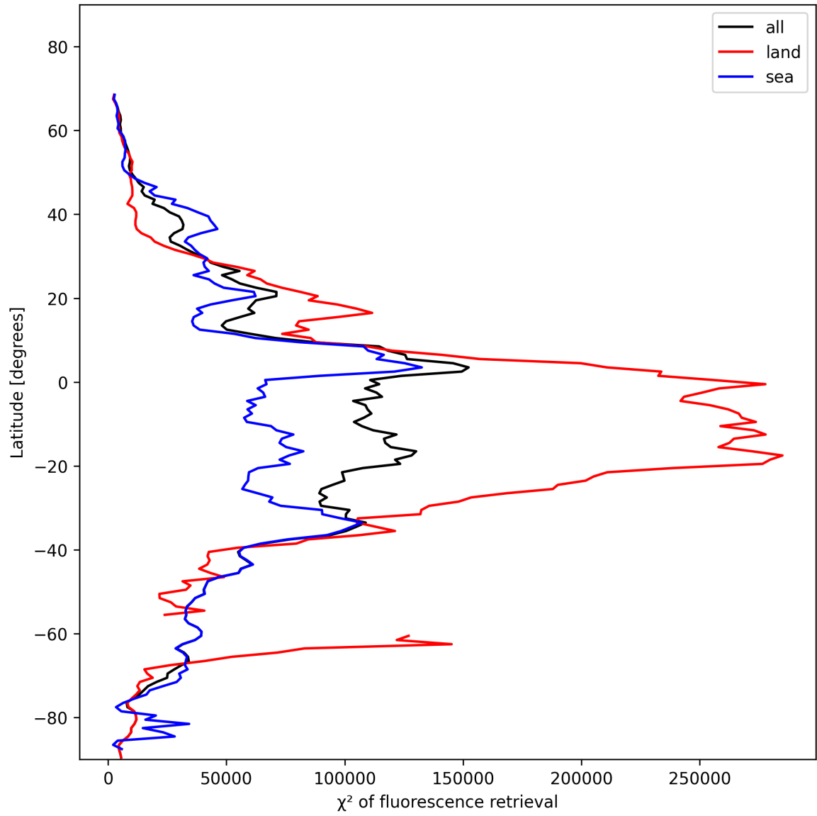
Figure 23: Zonal average of “ \chi^2 of fluorescence retrieval” for 2025-01-23 to 2025-01-24.
