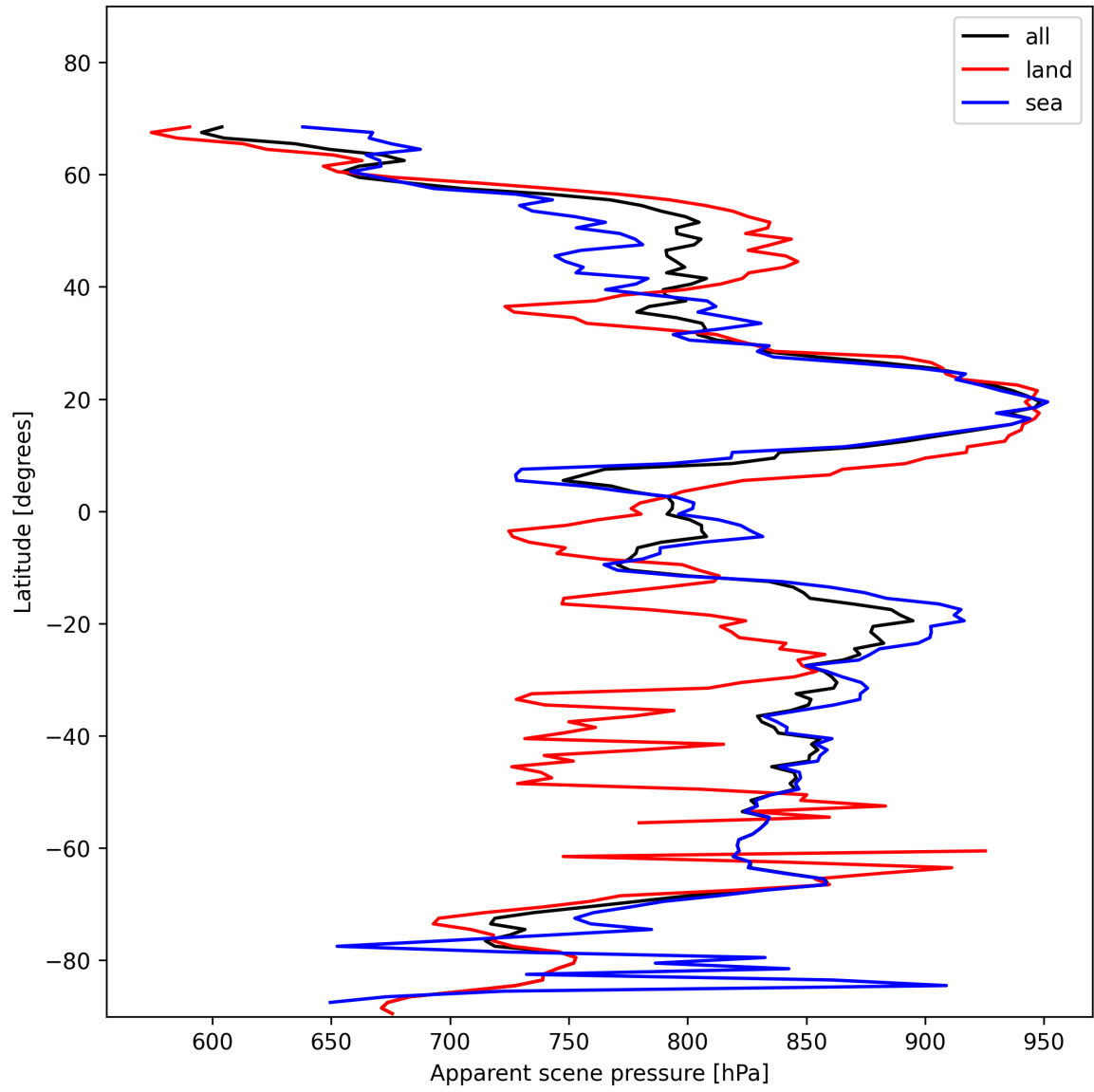
Figure 17: Zonal average of “Apparent scene pressure” for 2025-01-23 to 2025-01-24.
