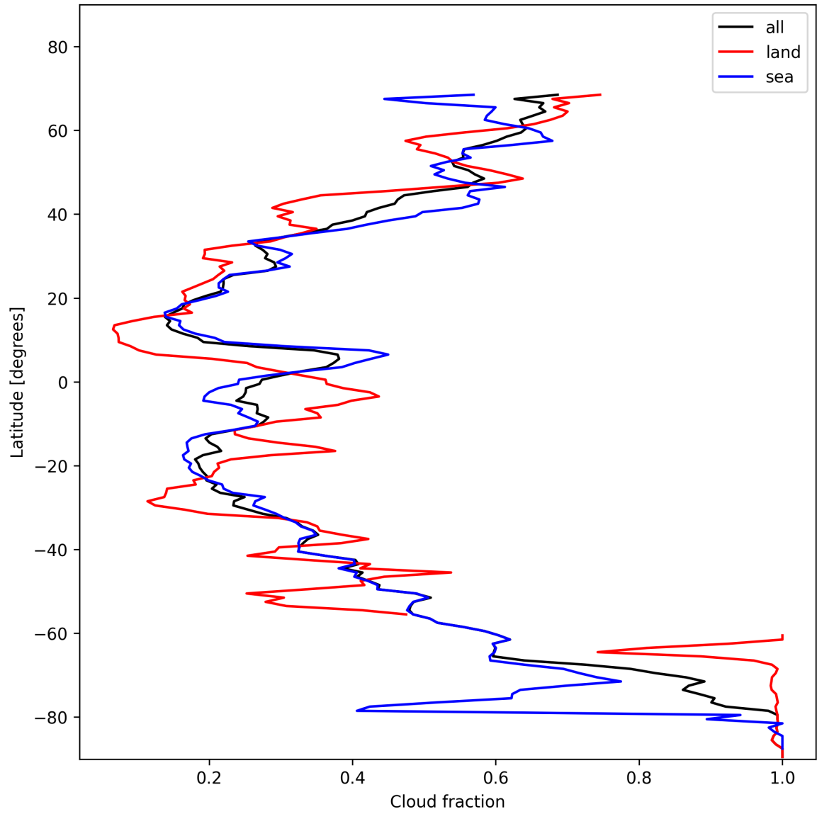
Figure 13: Zonal average of “Cloud fraction” for 2025-01-23 to 2025-01-24.
