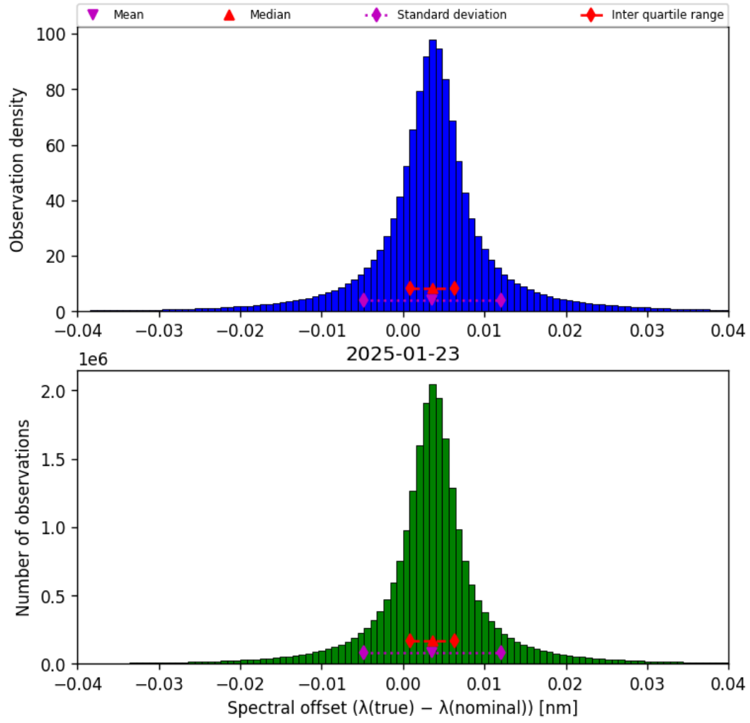
Figure 43: Histogram of “Spectral offset ( \lambda_{\text{true}} - \lambda_{\text{nominal}} )” for 2025-01-23 to 2025-01-24
