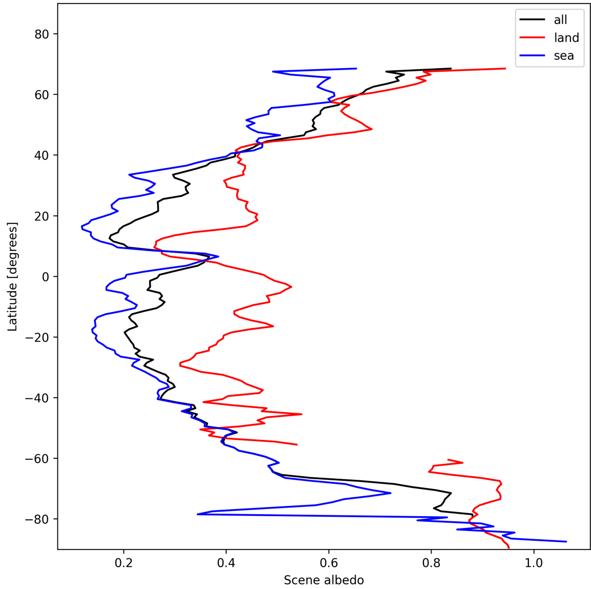
Figure 15: Zonal average of “Scene albedo” for 2025-01-23 to 2025-01-24.
