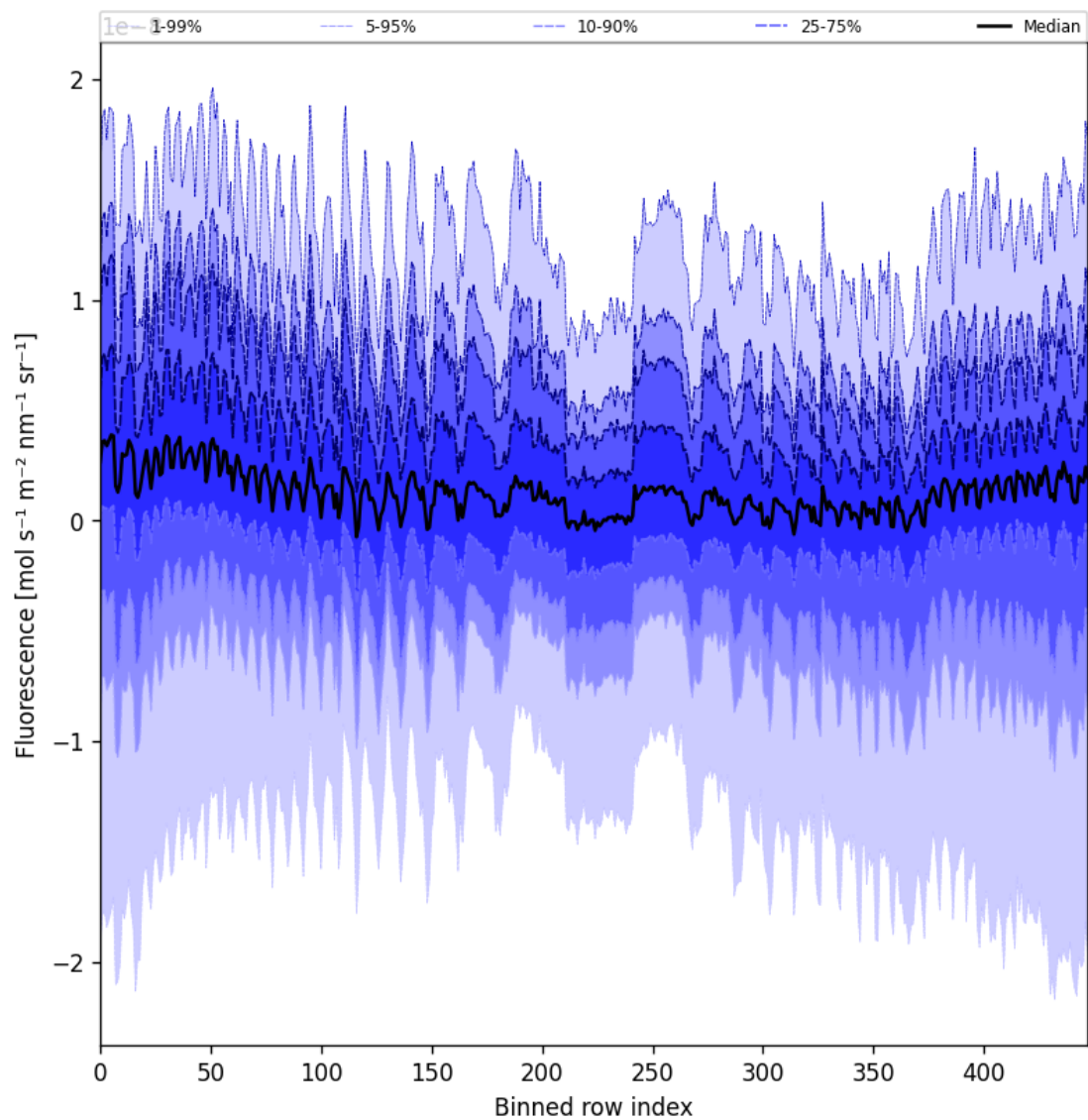
Figure 55: Along track statistics of “Fluorescence” for 2025-01-23 to 2025-01-24
