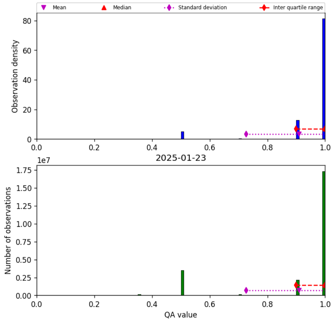
Figure 27: Histogram of “QA value” for 2025-01-23 to 2025-01-24
