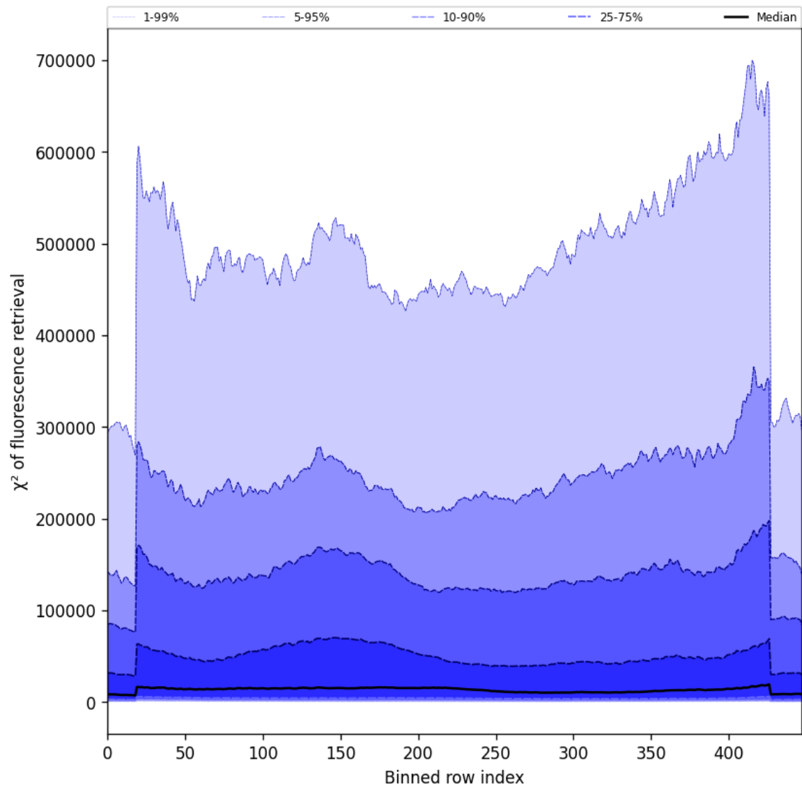
Figure 57: Along track statistics of “ \chi^2 of fluorescence retrieval” for 2025-01-23 to 2025-01-24
