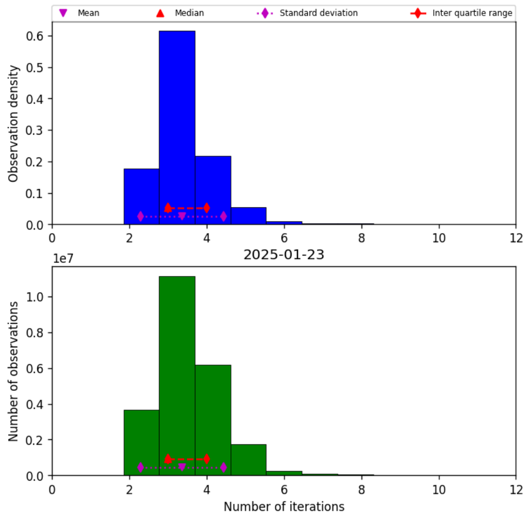
Figure 37: Histogram of “Number of iterations” for 2025-01-23 to 2025-01-24
