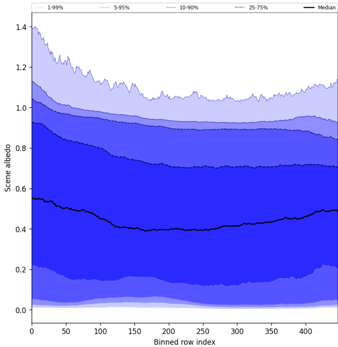
Figure 49: Along track statistics of “Scene albedo” for 2025-01-23 to 2025-01-24
