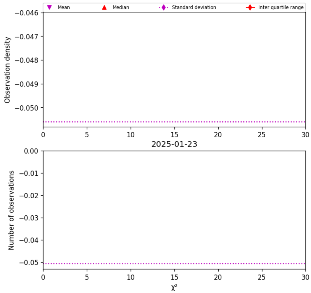
Figure 36: Histogram of " \chi^2 " for 2025-01-23 to 2025-01-24
