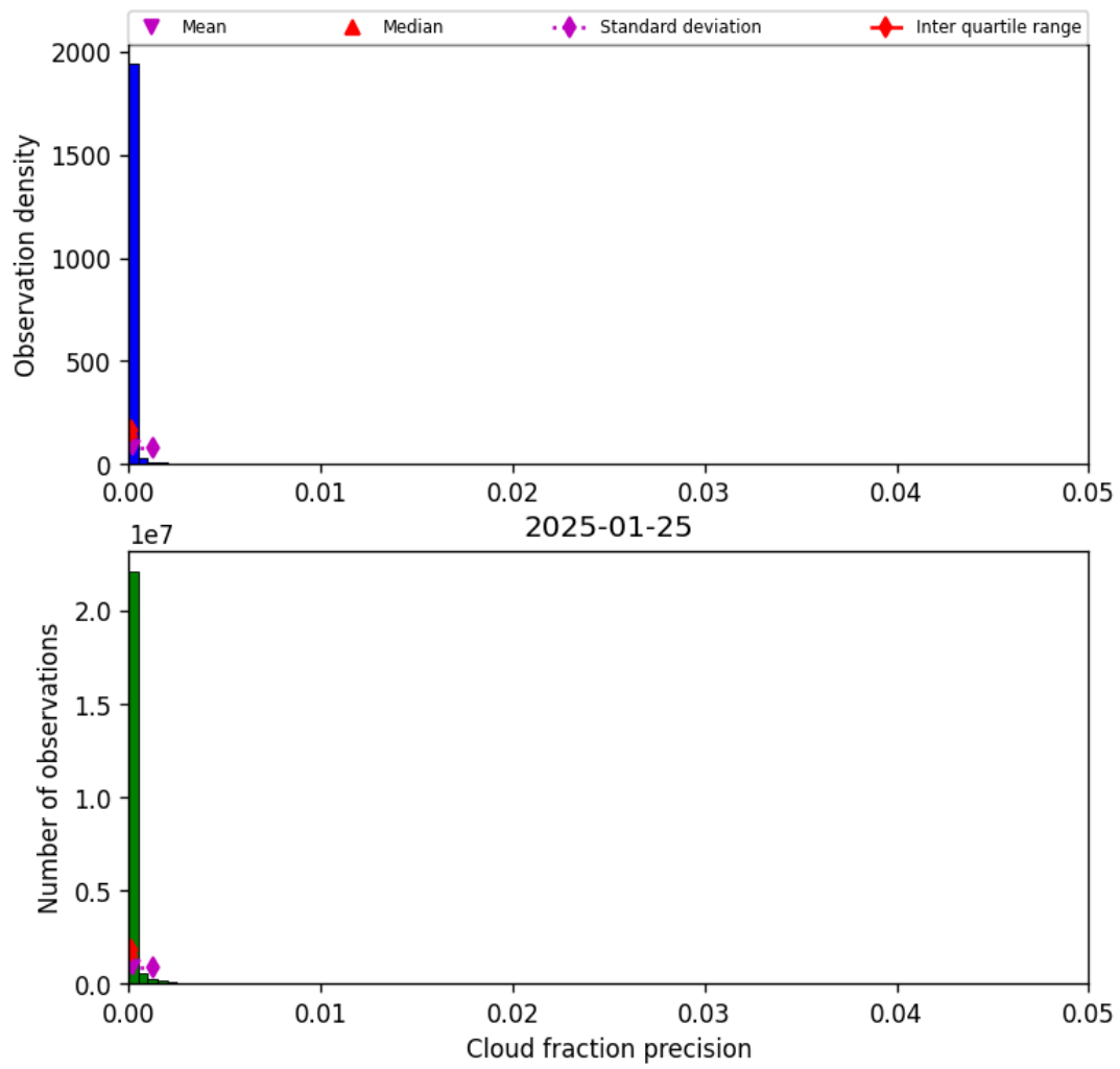
Figure 31: Histogram of “Cloud fraction precision” for 2025-01-25 to 2025-01-26
