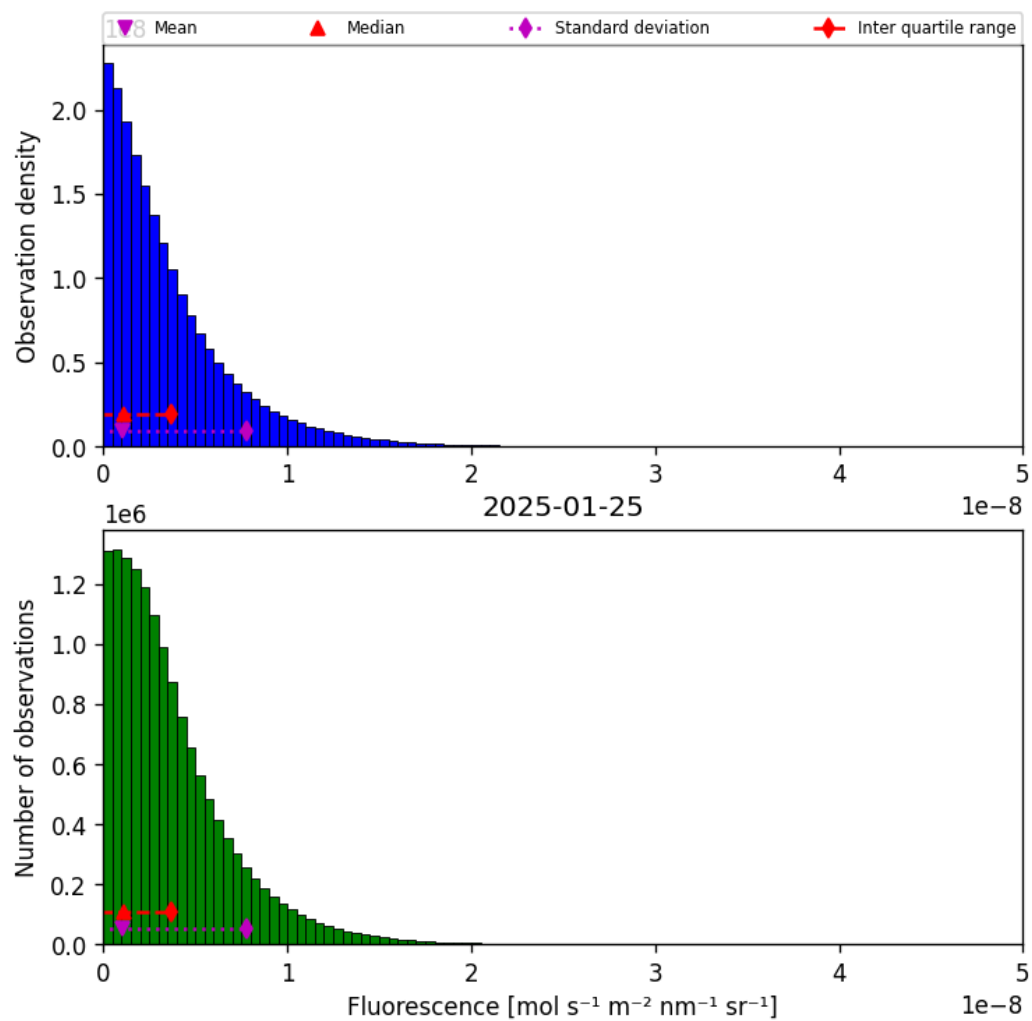
Figure 38: Histogram of “Fluorescence” for 2025-01-25 to 2025-01-26
