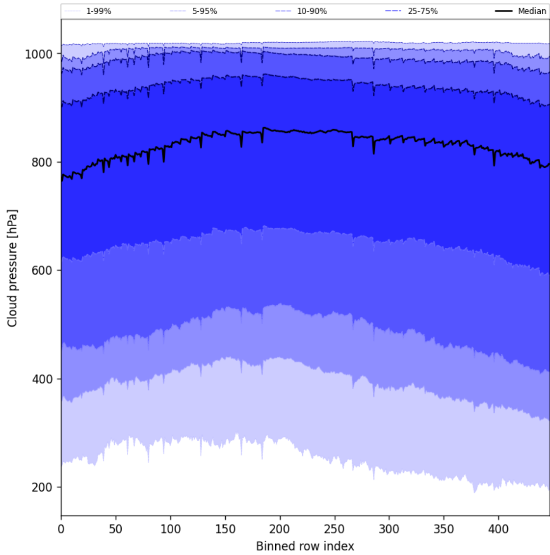
Figure 45: Along track statistics of “Cloud pressure” for 2025-01-25 to 2025-01-26
