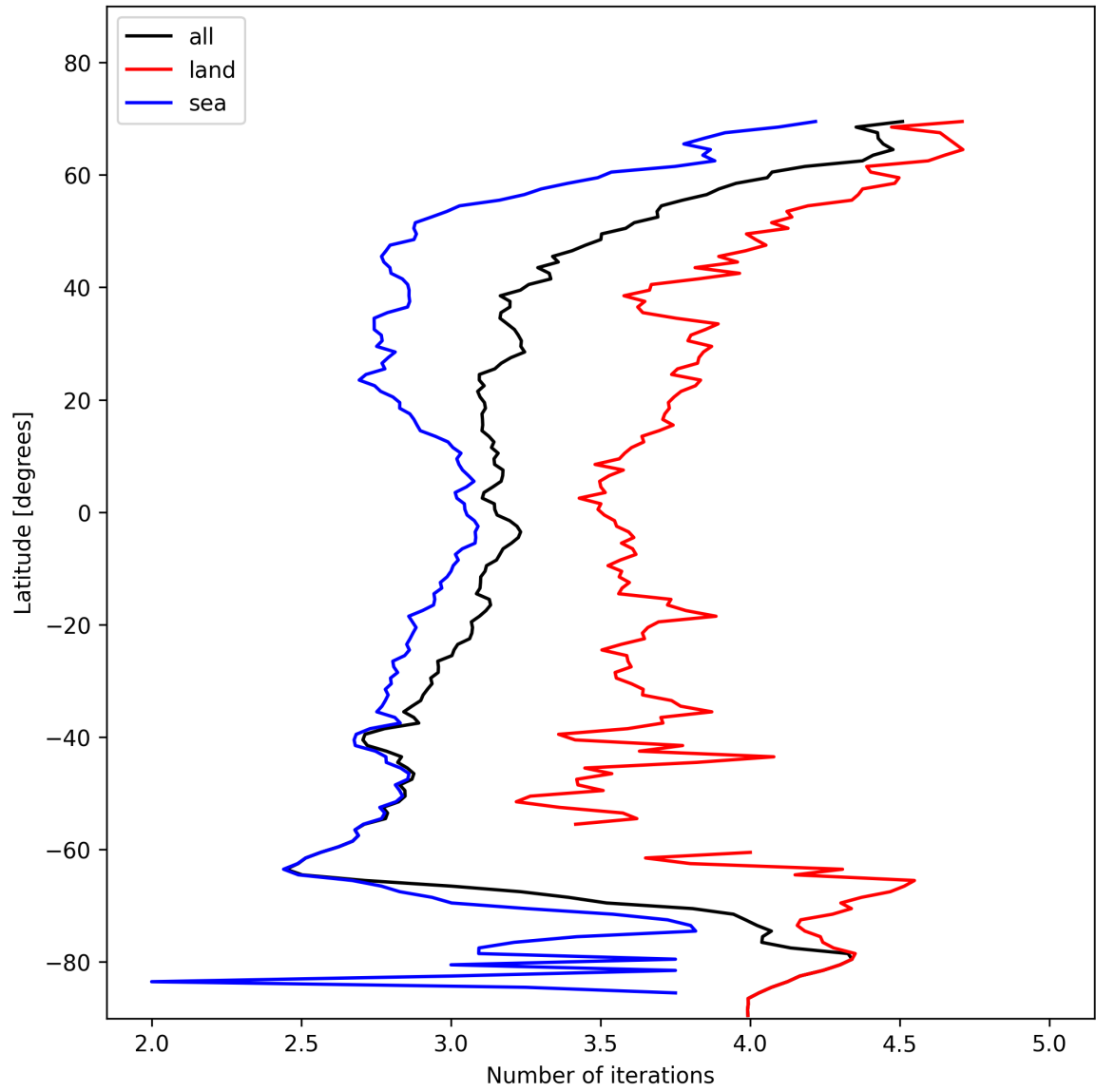
Figure 20: Zonal average of “Number of iterations” for 2025-01-25 to 2025-01-26.
