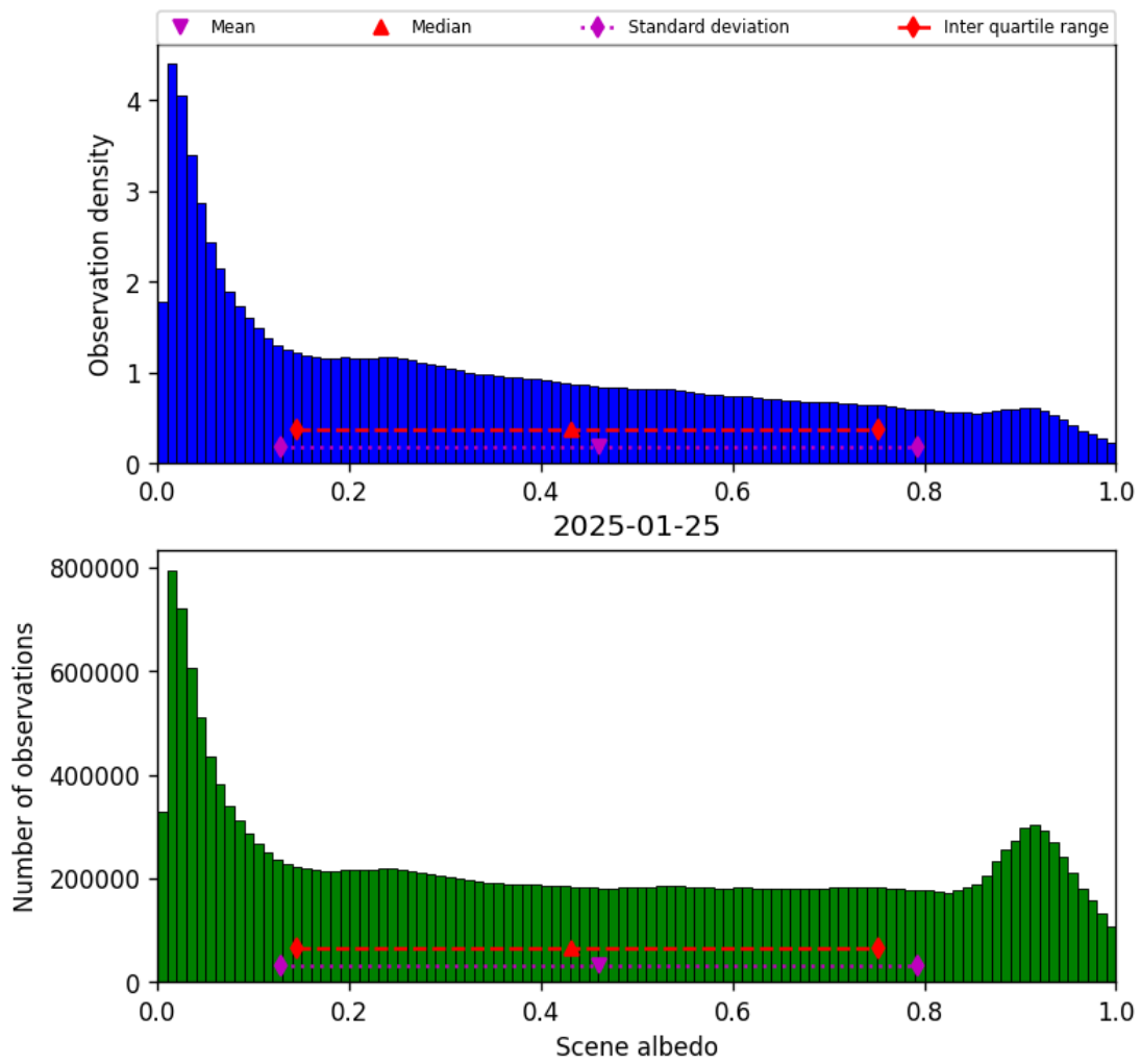
Figure 32: Histogram of “Scene albedo” for 2025-01-25 to 2025-01-26
