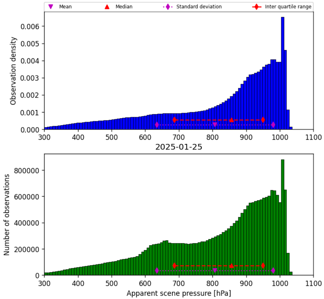
Figure 34: Histogram of “Apparent scene pressure” for 2025-01-25 to 2025-01-26
