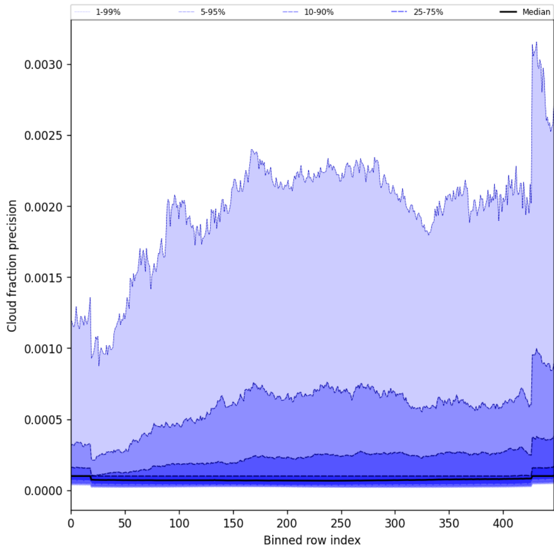
Figure 48: Along track statistics of “Cloud fraction precision” for 2025-01-25 to 2025-01-26
