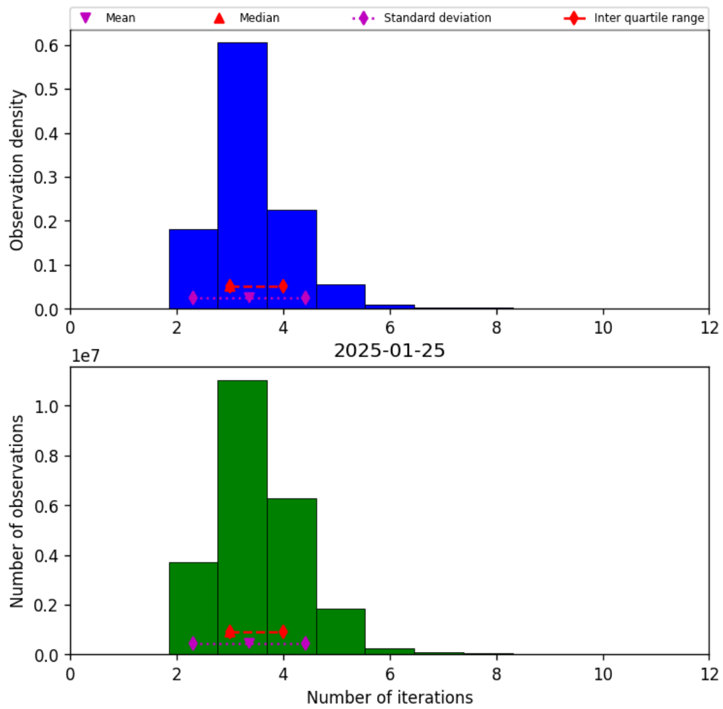
Figure 37: Histogram of “Number of iterations” for 2025-01-25 to 2025-01-26
