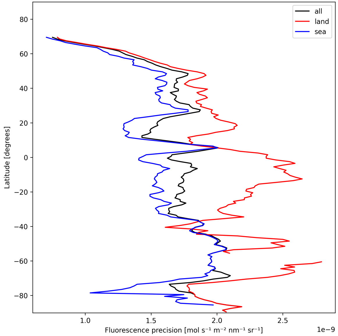
Figure 22: Zonal average of “Fluorescence precision” for 2025-01-25 to 2025-01-26.
