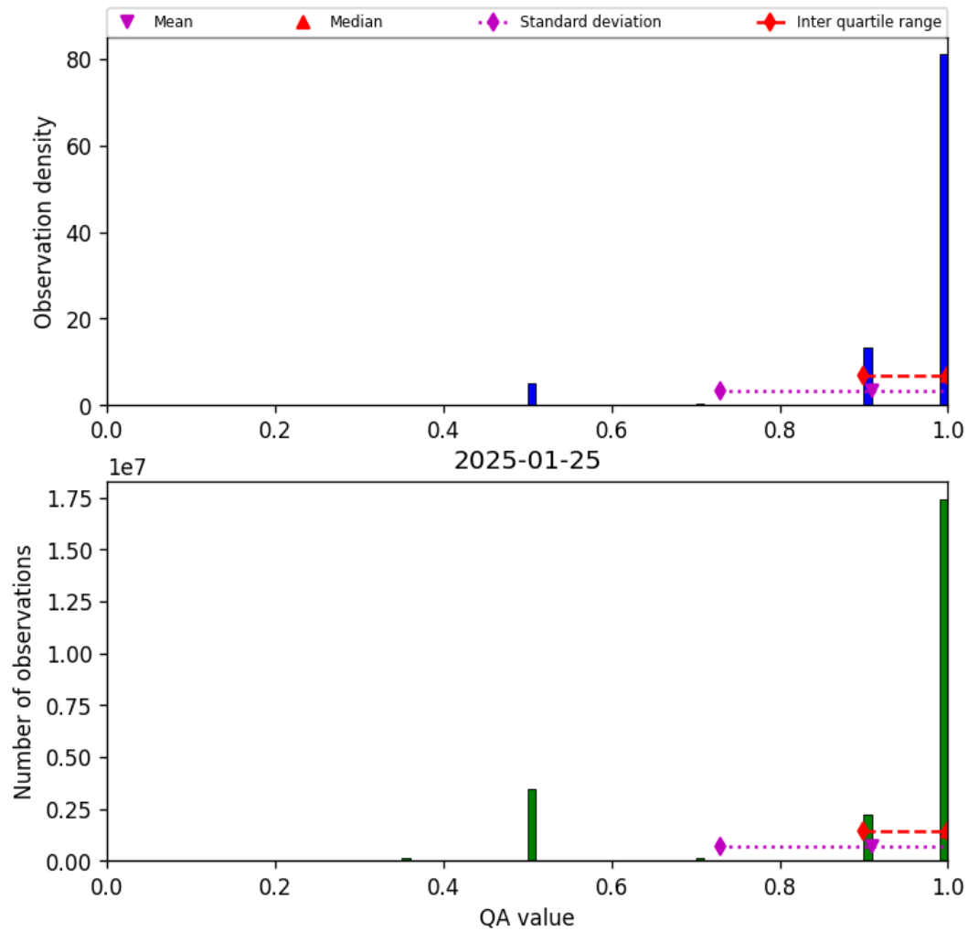
Figure 27: Histogram of “QA value” for 2025-01-25 to 2025-01-26
