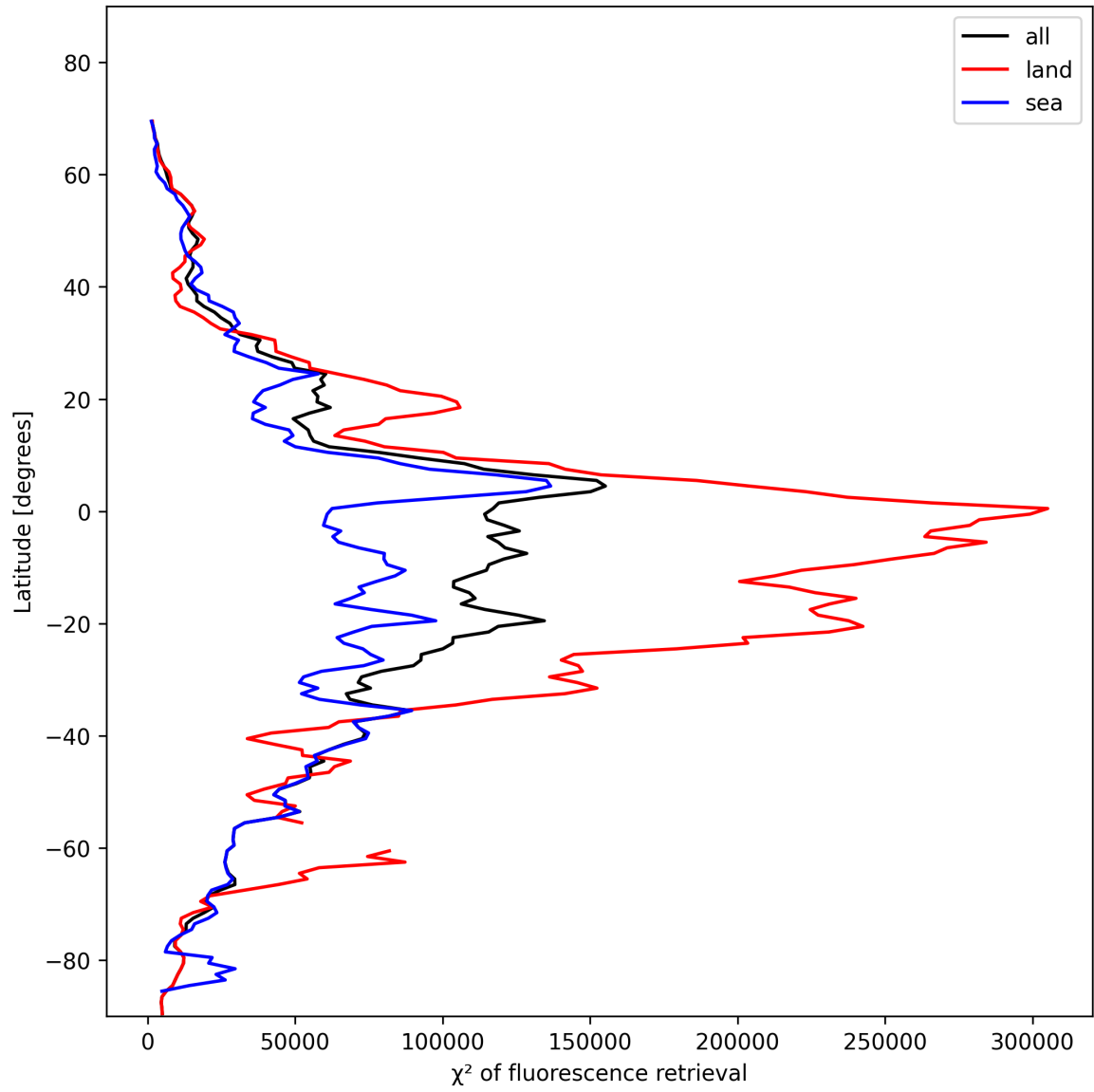
Figure 23: Zonal average of “ \chi^2 of fluorescence retrieval” for 2025-01-25 to 2025-01-26.
