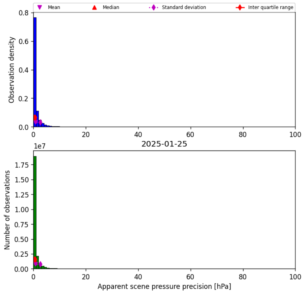
Figure 35: Histogram of “Apparent scene pressure precision” for 2025-01-25 to 2025-01-26
