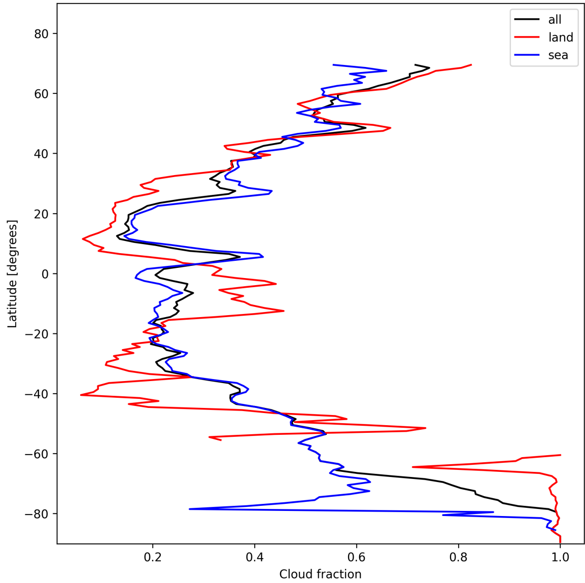
Figure 13: Zonal average of “Cloud fraction” for 2025-01-25 to 2025-01-26.
