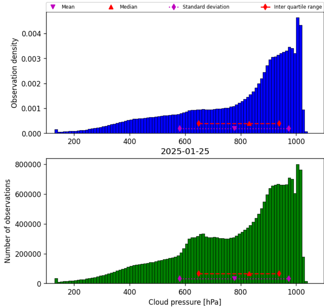
Figure 28: Histogram of “Cloud pressure” for 2025-01-25 to 2025-01-26
