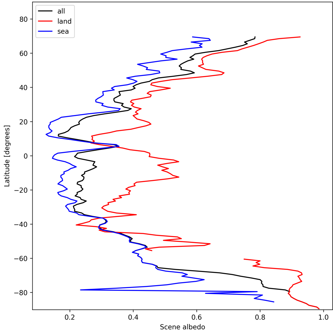
Figure 15: Zonal average of “Scene albedo” for 2025-01-25 to 2025-01-26.
