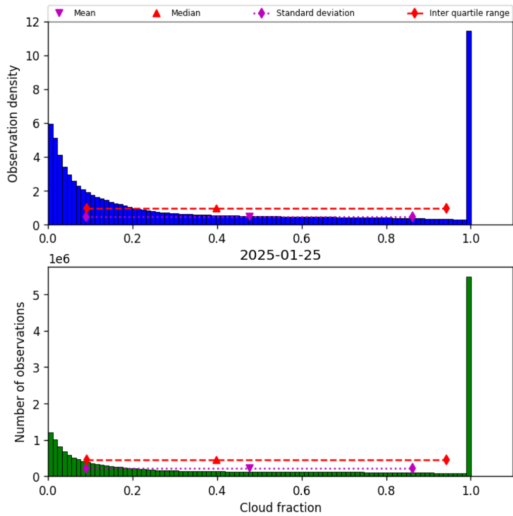
Figure 30: Histogram of “Cloud fraction” for 2025-01-25 to 2025-01-26
