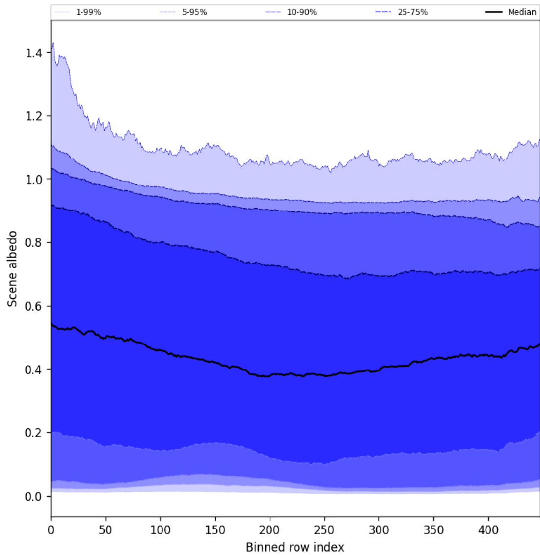
Figure 49: Along track statistics of “Scene albedo” for 2025-01-25 to 2025-01-26
