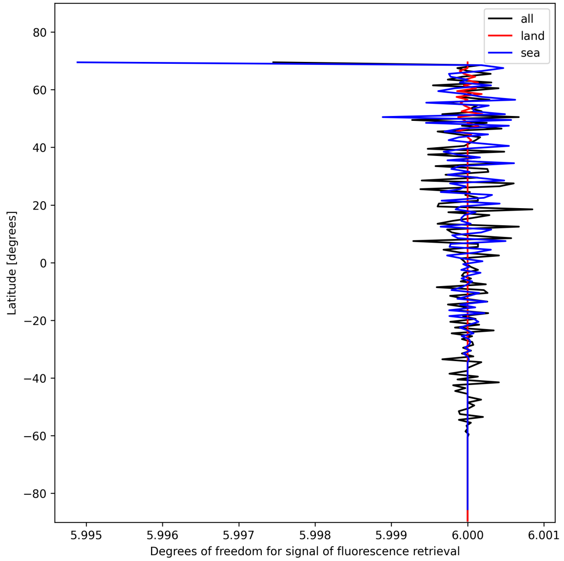
Figure 24: Zonal average of “Degrees of freedom for signal of fluorescence retrieval” for 2025-01-25 to 2025-01-26.
