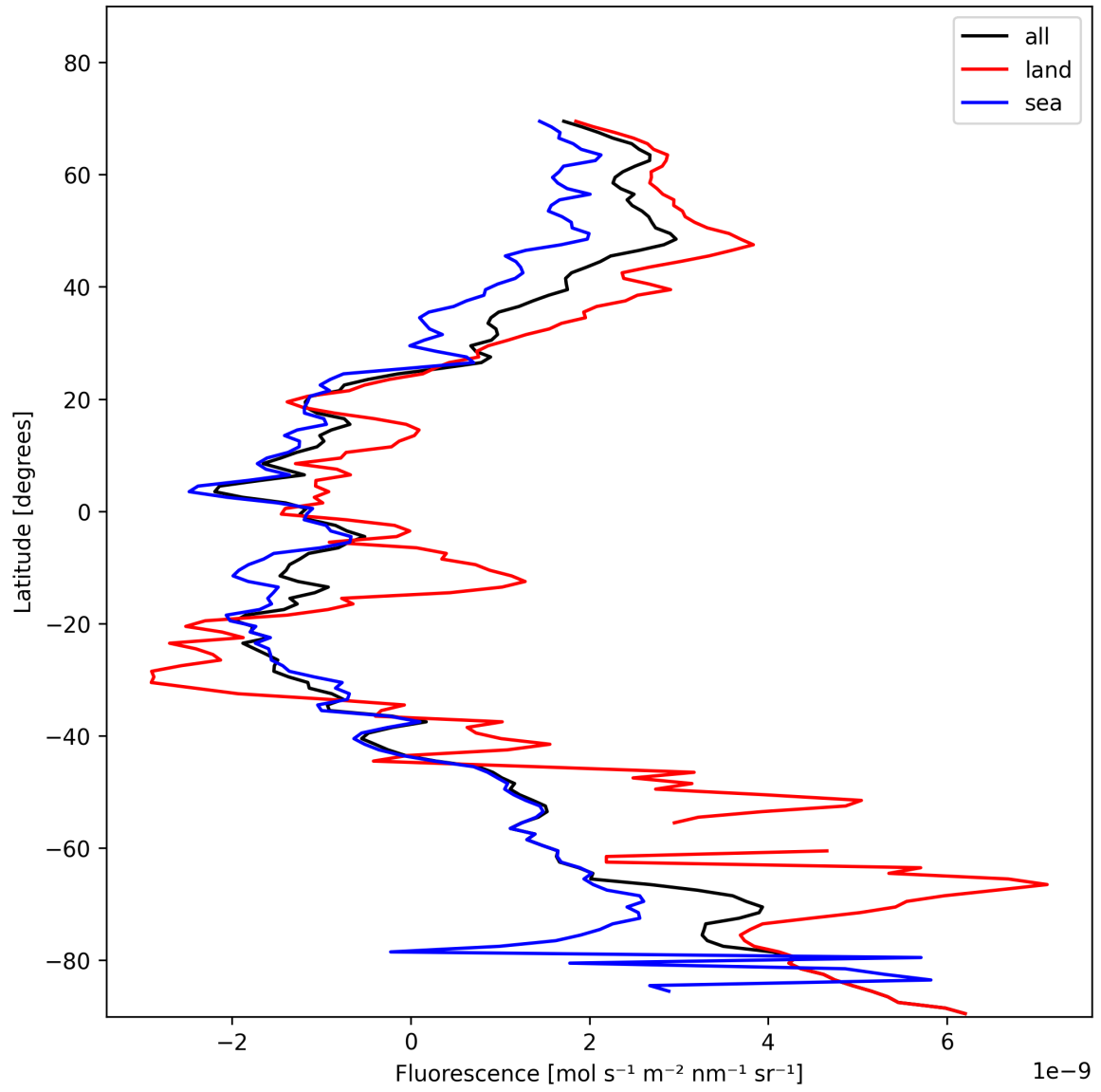
Figure 21: Zonal average of “Fluorescence” for 2025-01-25 to 2025-01-26.
