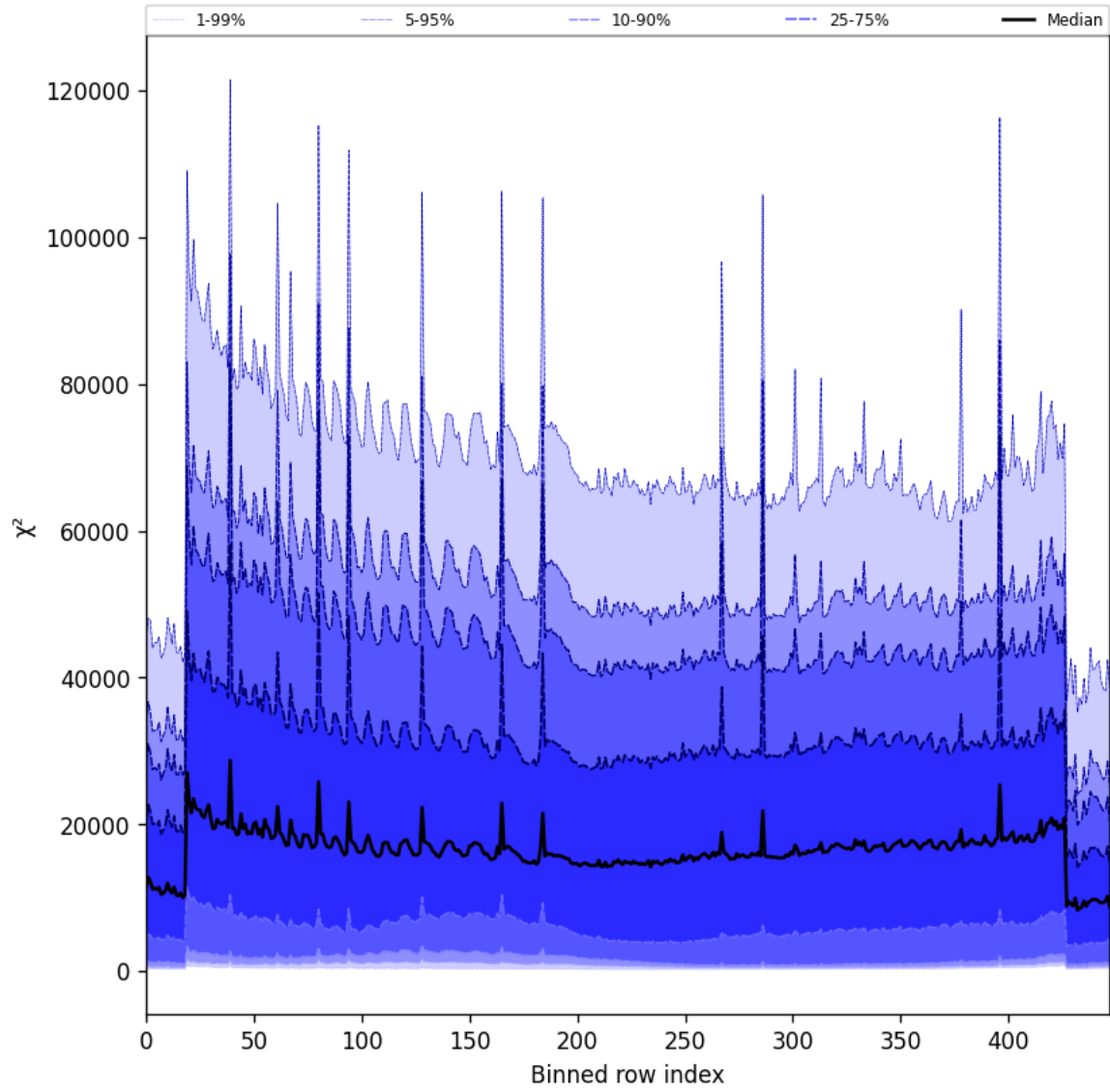
Figure 53: Along track statistics of “ \chi^2 ” for 2025-01-25 to 2025-01-26
