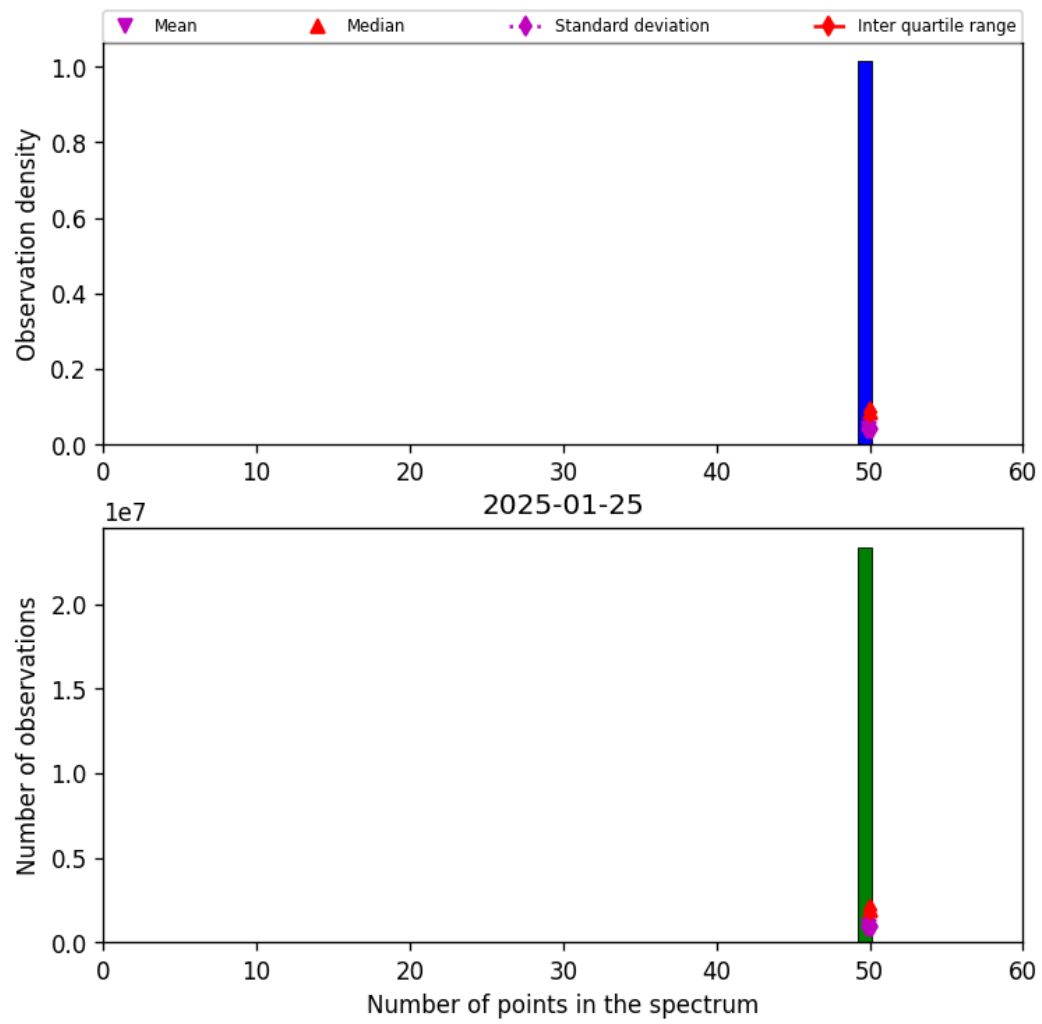
Figure 42: Histogram of “Number of points in the spectrum” for 2025-01-25 to 2025-01-26
