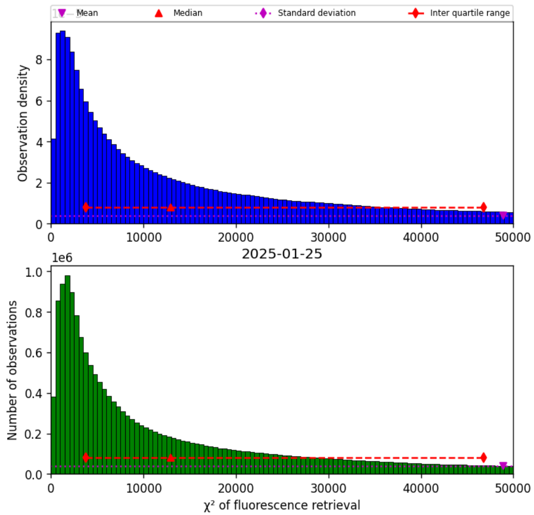
Figure 40: Histogram of “ \chi^2 of fluorescence retrieval” for 2025-01-25 to 2025-01-26
