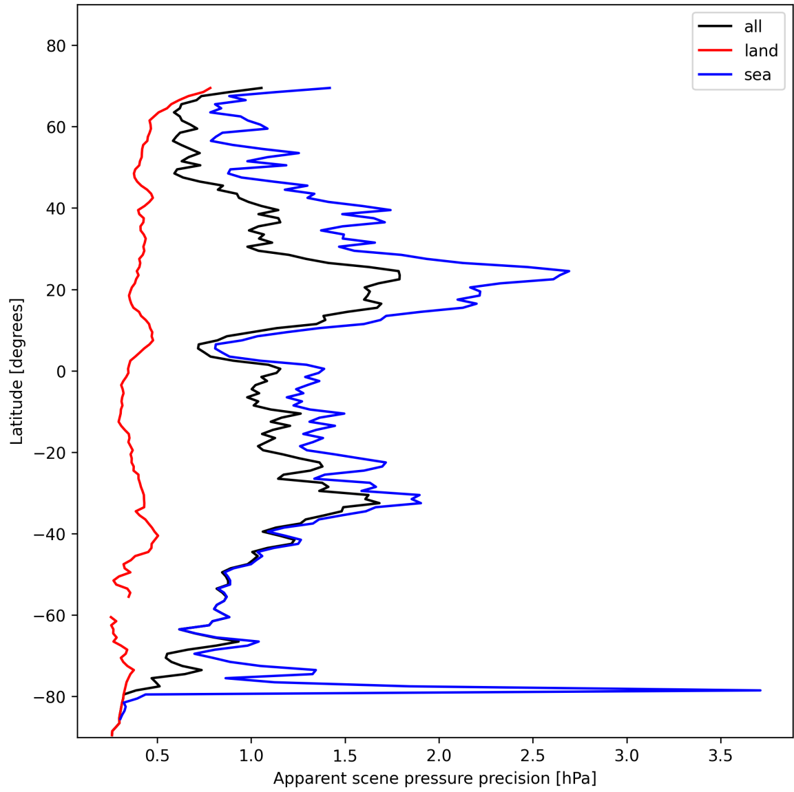
Figure 18: Zonal average of “Apparent scene pressure precision” for 2025-01-25 to 2025-01-26.
