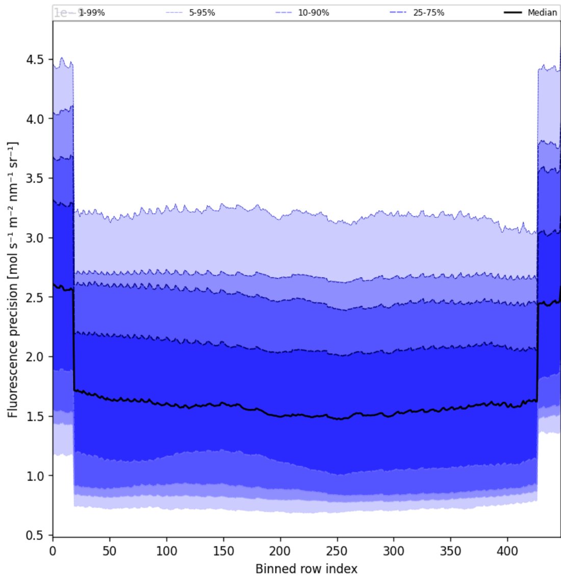
Figure 56: Along track statistics of “Fluorescence precision” for 2025-01-25 to 2025-01-26
