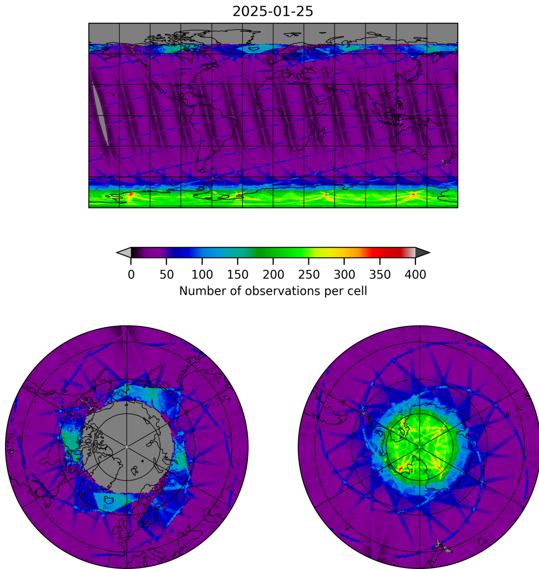
Figure 9: Map of the number of observations for 2025-01-25 to 2025-01-26
