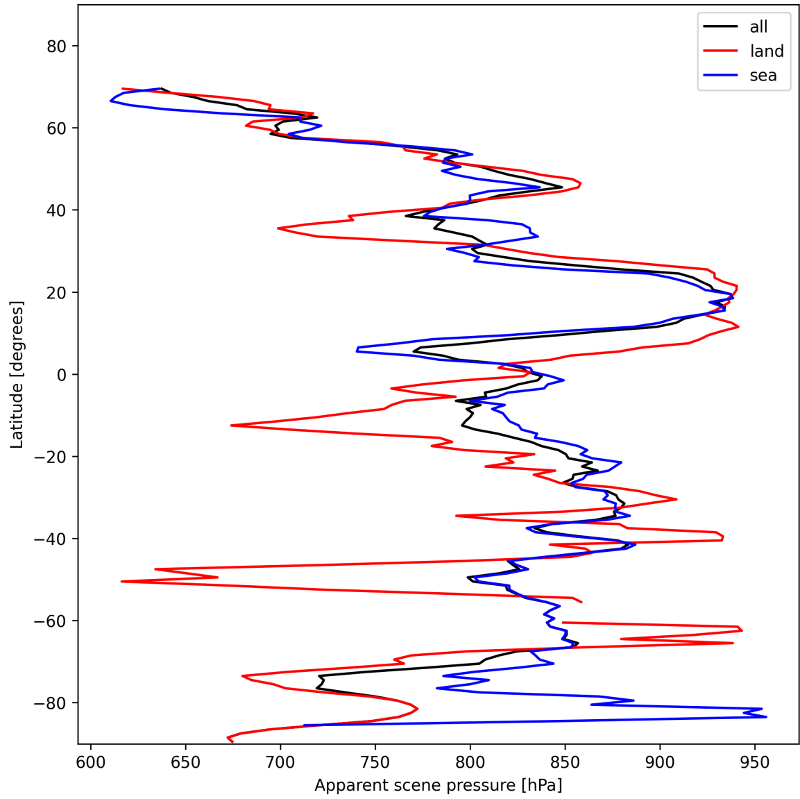
Figure 17: Zonal average of “Apparent scene pressure” for 2025-01-25 to 2025-01-26.
