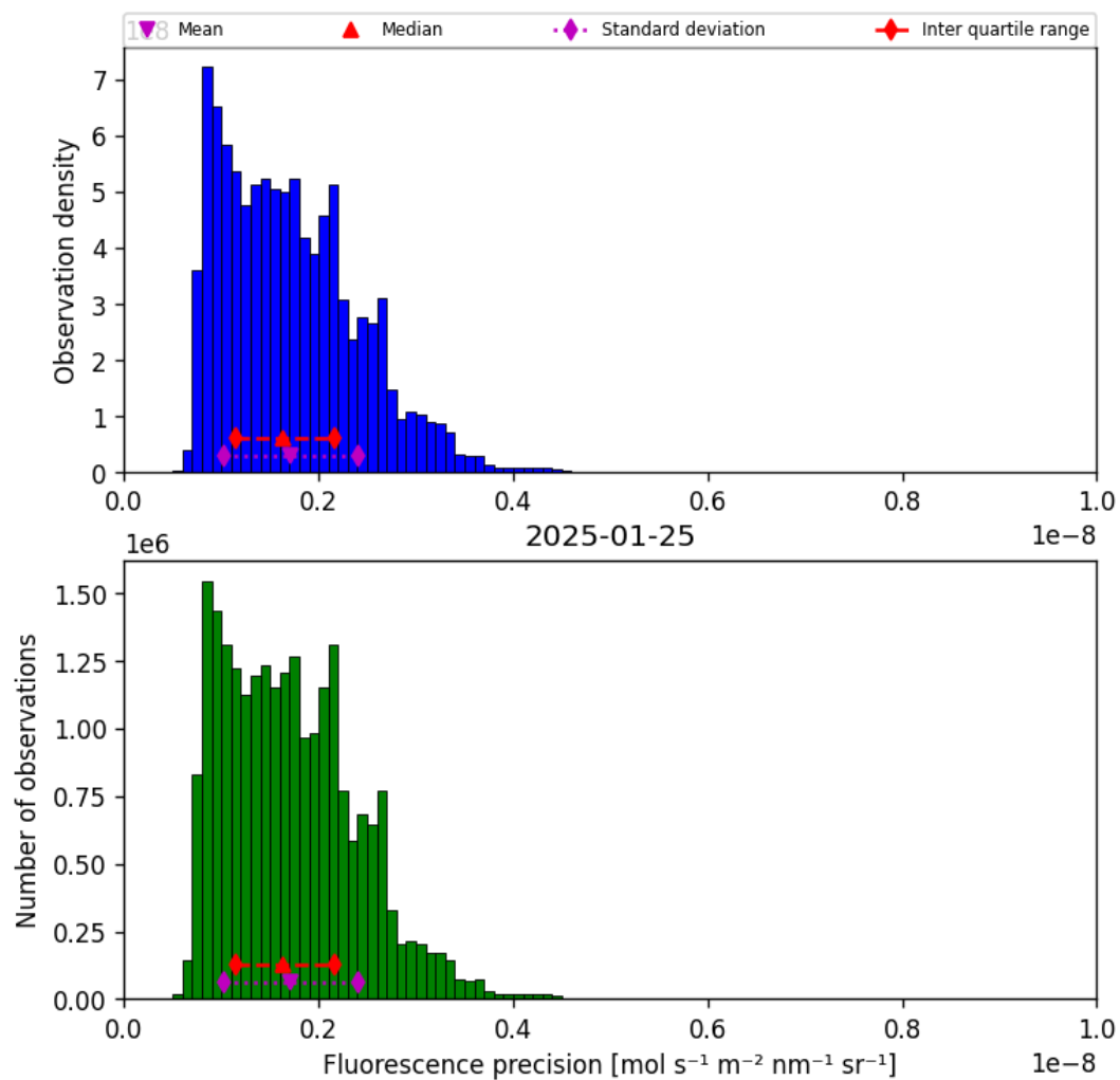
Figure 39: Histogram of “Fluorescence precision” for 2025-01-25 to 2025-01-26
