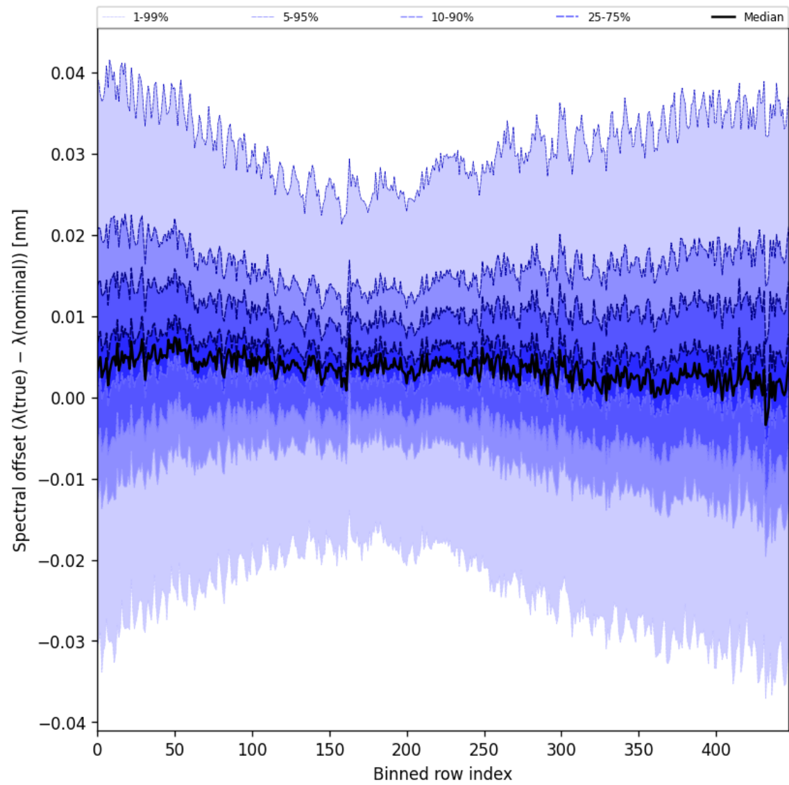
Figure 60: Along track statistics of “Spectral offset ( \lambda_{\text{true}} - \lambda_{\text{nominal}} )” for 2025-01-25 to 2025-01-26
