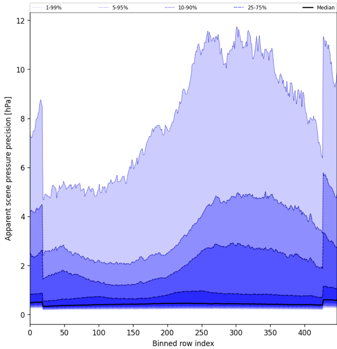
Figure 52: Along track statistics of “Apparent scene pressure precision” for 2025-01-25 to 2025-01-26
