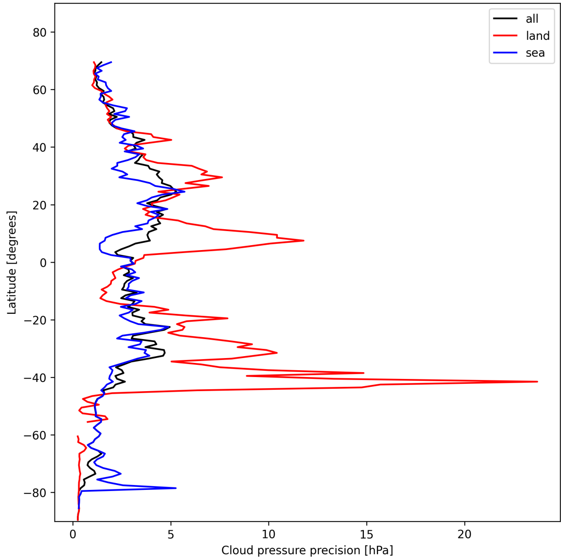
Figure 12: Zonal average of "Cloud pressure precision" for 2025-01-25 to 2025-01-26.
