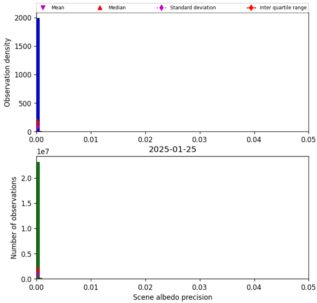
Figure 33: Histogram of “Scene albedo precision” for 2025-01-25 to 2025-01-26
