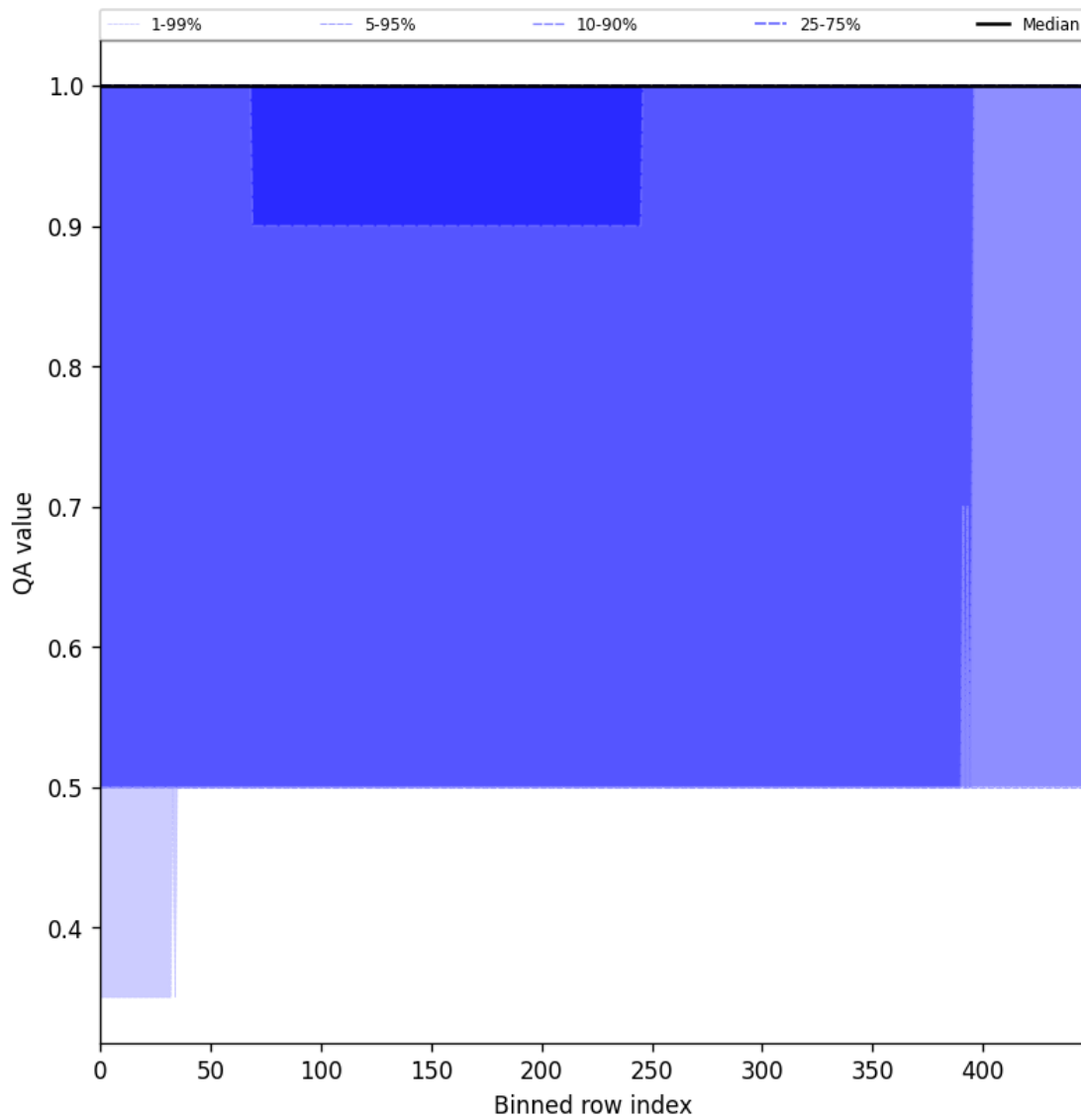
Figure 44: Along track statistics of “QA value” for 2025-01-25 to 2025-01-26
