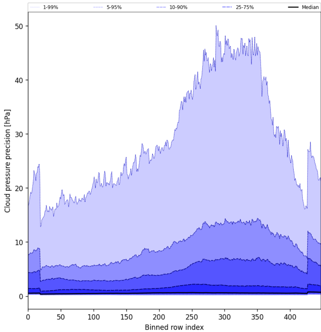
Figure 46: Along track statistics of “Cloud pressure precision” for 2025-01-25 to 2025-01-26
