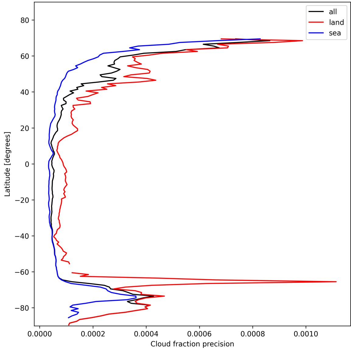
Figure 14: Zonal average of “Cloud fraction precision” for 2025-01-25 to 2025-01-26.
