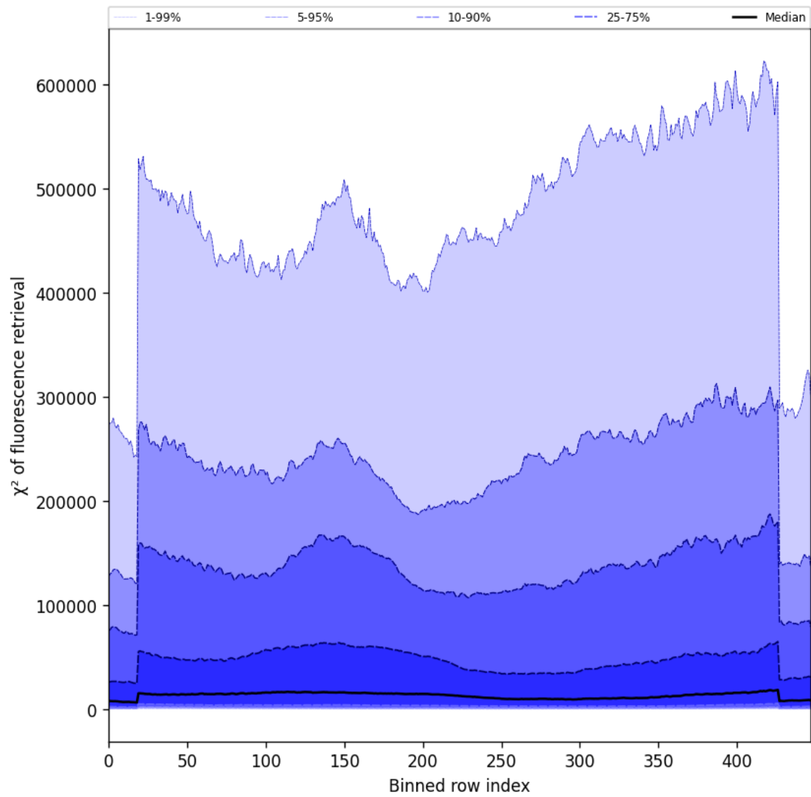
Figure 57: Along track statistics of “ \chi^2 of fluorescence retrieval” for 2025-01-25 to 2025-01-26
