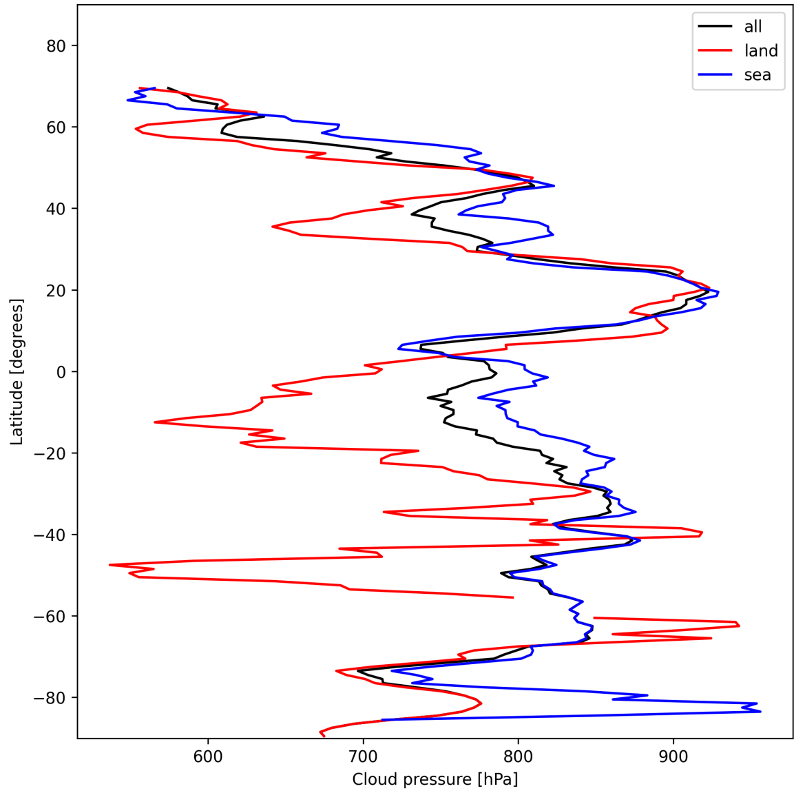
Figure 11: Zonal average of “Cloud pressure” for 2025-01-25 to 2025-01-26.
