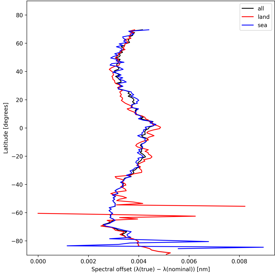
Figure 26: Zonal average of “Spectral offset ( \lambda_{\text{true}} - \lambda_{\text{nominal}} )” for 2025-01-25 to 2025-01-26.
