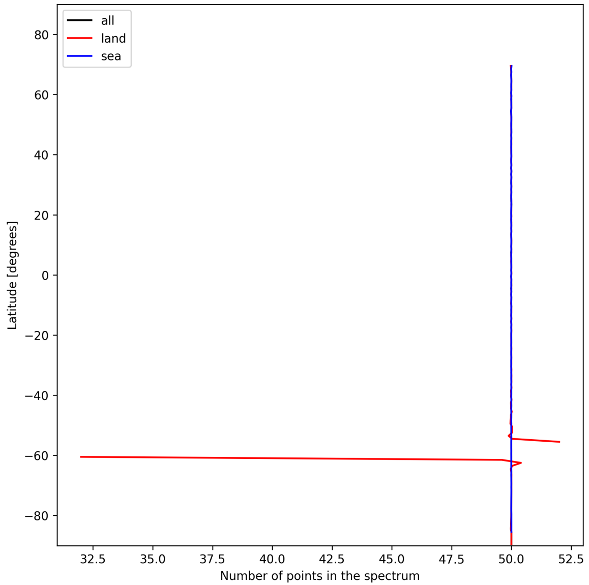
Figure 25: Zonal average of “Number of points in the spectrum” for 2025-01-25 to 2025-01-26.
