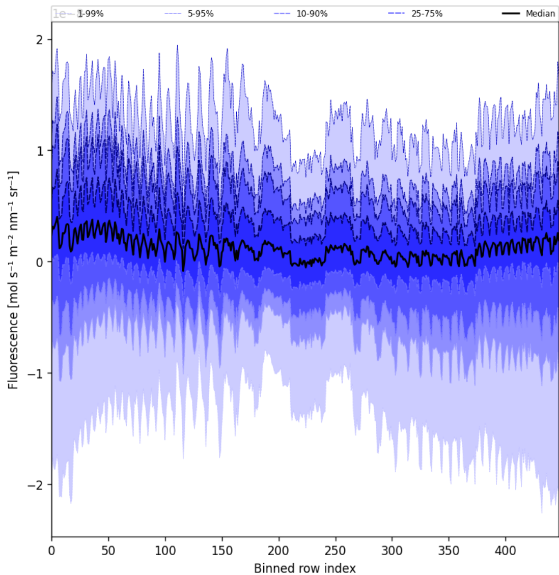
Figure 55: Along track statistics of “Fluorescence” for 2025-01-25 to 2025-01-26
