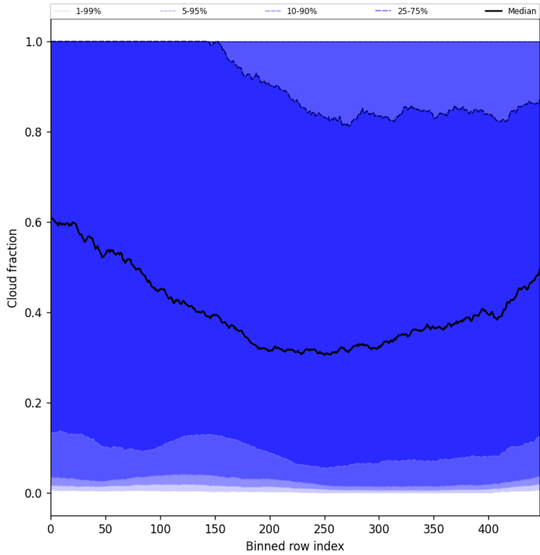
Figure 47: Along track statistics of “Cloud fraction” for 2025-01-25 to 2025-01-26
