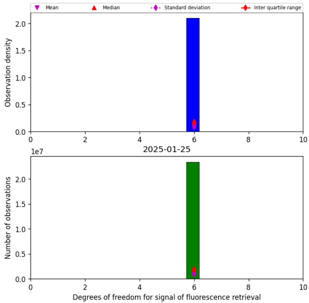
Figure 41: Histogram of “Degrees of freedom for signal of fluorescence retrieval” for 2025-01-25 to 2025-01-26
