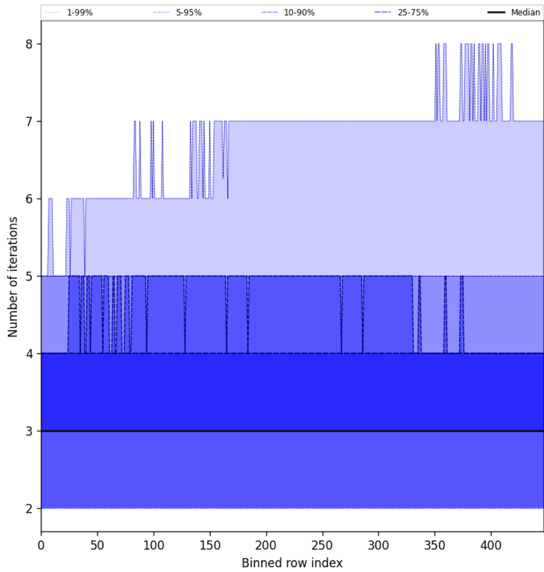
Figure 54: Along track statistics of “Number of iterations” for 2025-01-25 to 2025-01-26
