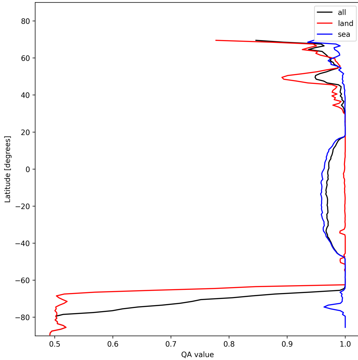
Figure 10: Zonal average of “QA value” for 2025-01-25 to 2025-01-26.
