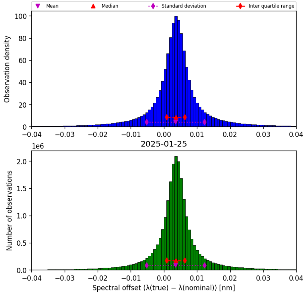
Figure 43: Histogram of “Spectral offset ( \lambda_{\text{true}} - \lambda_{\text{nominal}} )” for 2025-01-25 to 2025-01-26
