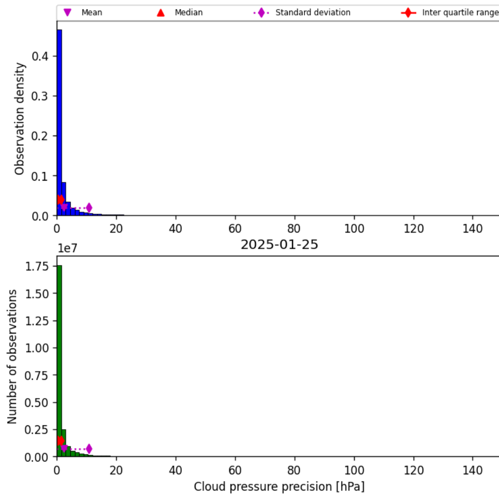
Figure 29: Histogram of “Cloud pressure precision” for 2025-01-25 to 2025-01-26
