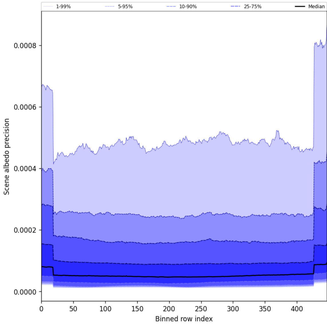
Figure 50: Along track statistics of “Scene albedo precision” for 2025-01-25 to 2025-01-26
