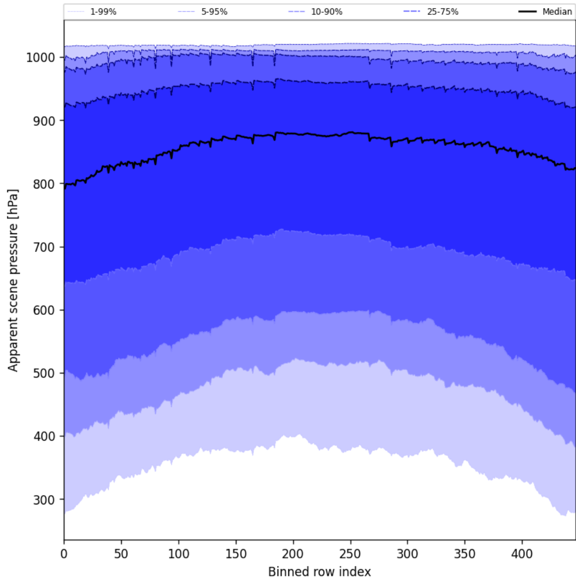
Figure 51: Along track statistics of “Apparent scene pressure” for 2025-01-25 to 2025-01-26
