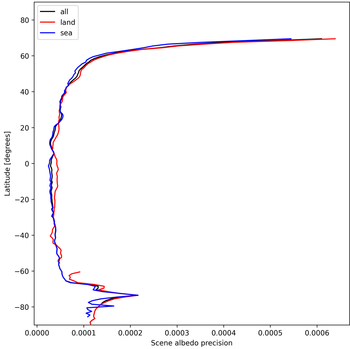
Figure 16: Zonal average of “Scene albedo precision” for 2025-01-25 to 2025-01-26.
