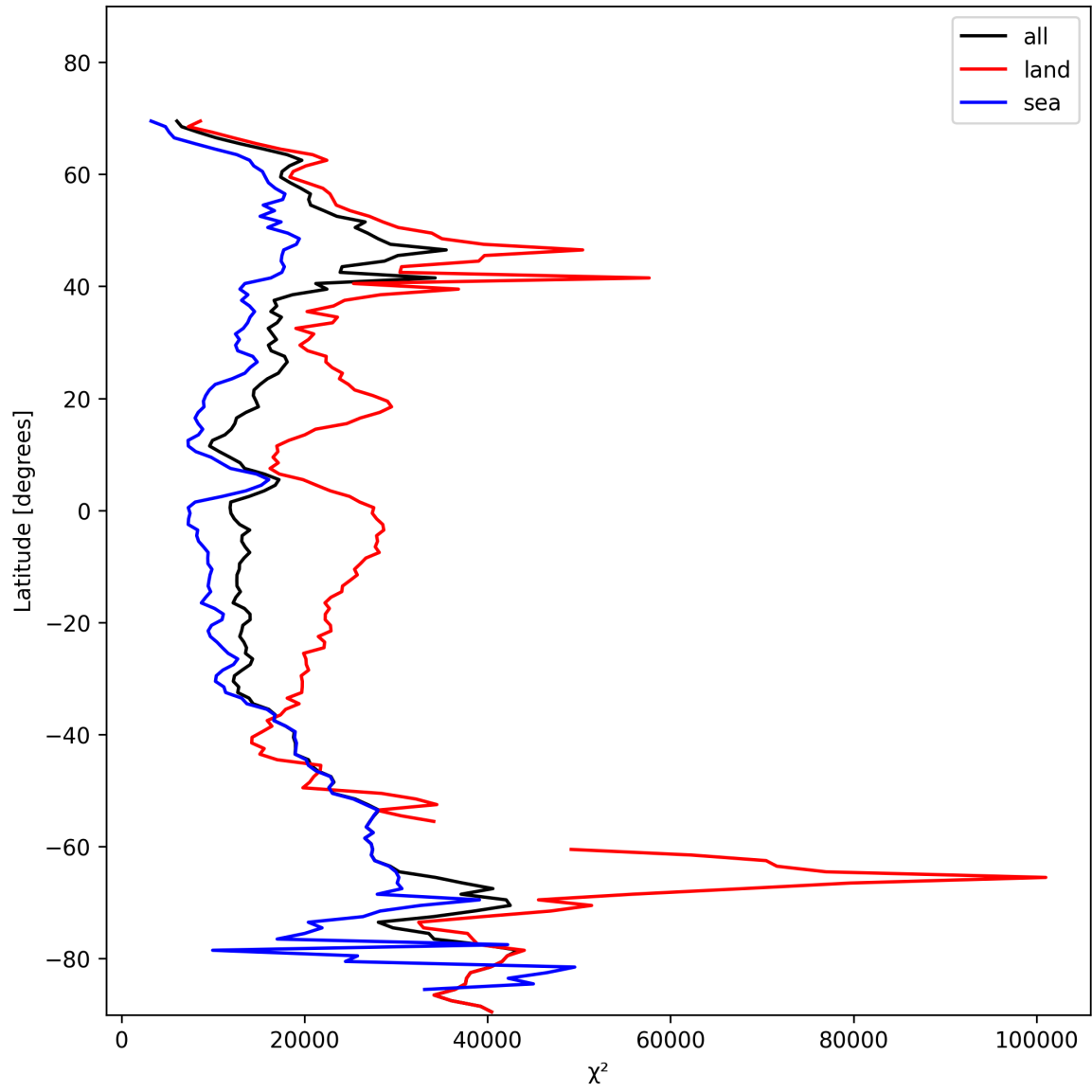
Figure 19: Zonal average of “ \chi^2 ” for 2025-01-25 to 2025-01-26.
