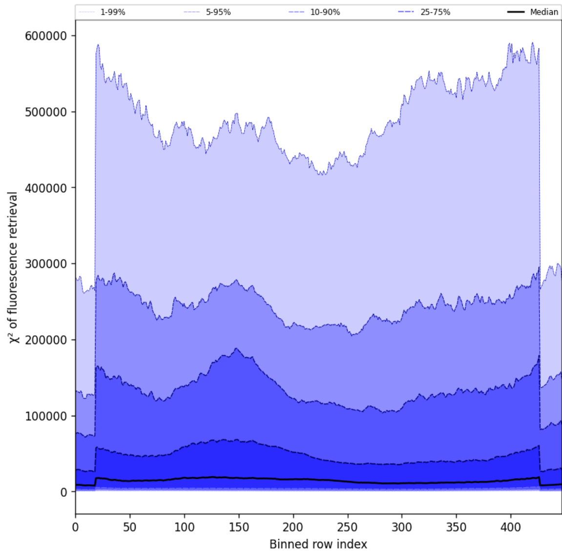
Figure 57: Along track statistics of “ \chi^2 of fluorescence retrieval” for 2025-01-28 to 2025-01-29
