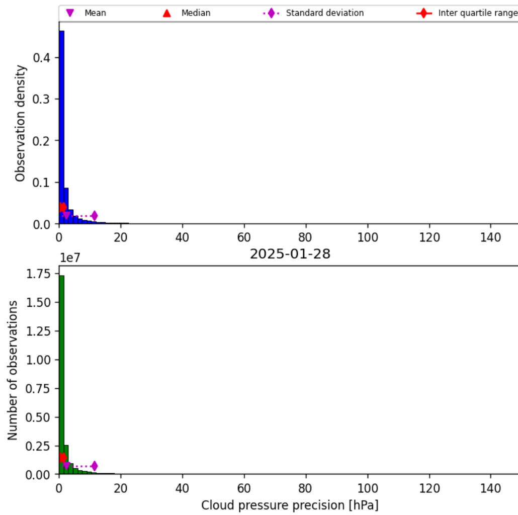
Figure 29: Histogram of “Cloud pressure precision” for 2025-01-28 to 2025-01-29
