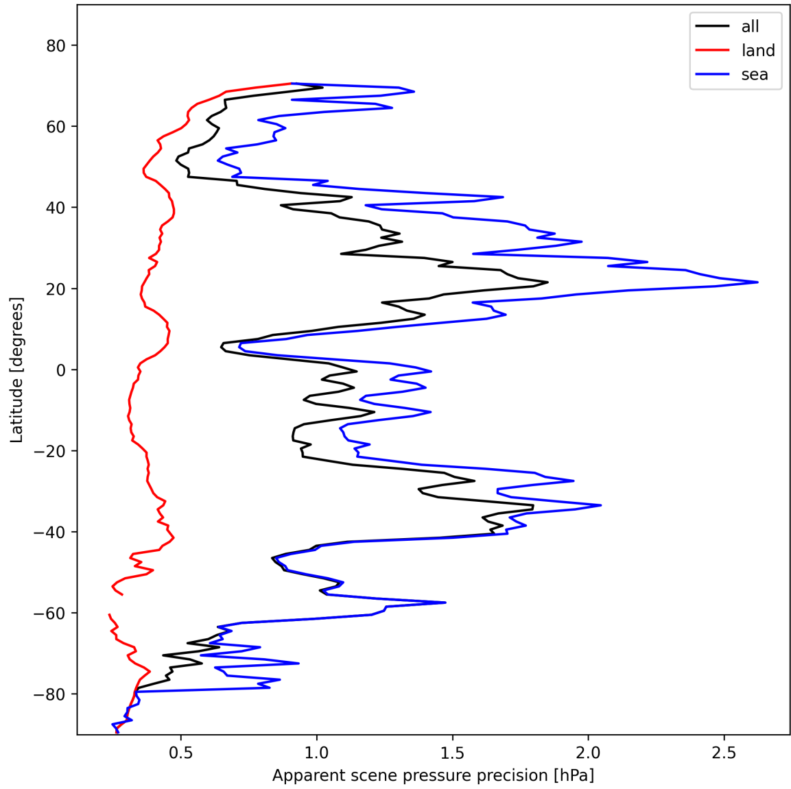
Figure 18: Zonal average of “Apparent scene pressure precision” for 2025-01-28 to 2025-01-29.
