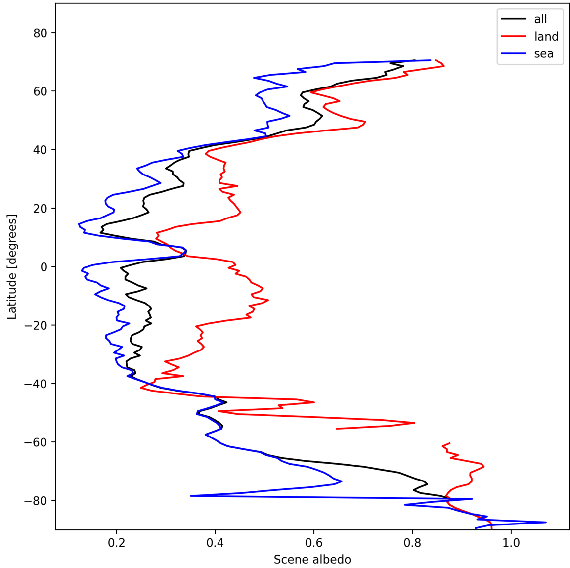
Figure 15: Zonal average of "Scene albedo" for 2025-01-28 to 2025-01-29.
