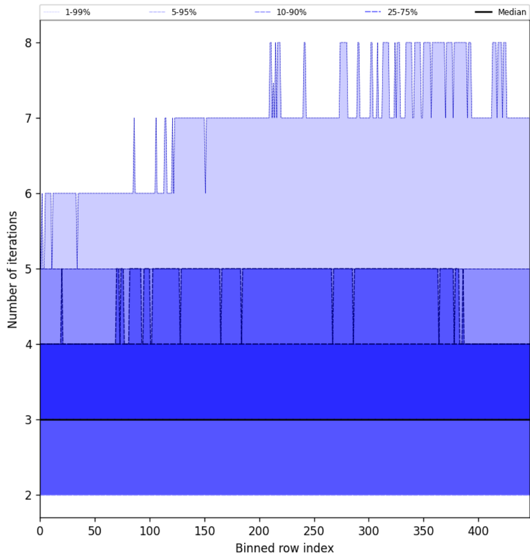
Figure 54: Along track statistics of “Number of iterations” for 2025-01-28 to 2025-01-29
