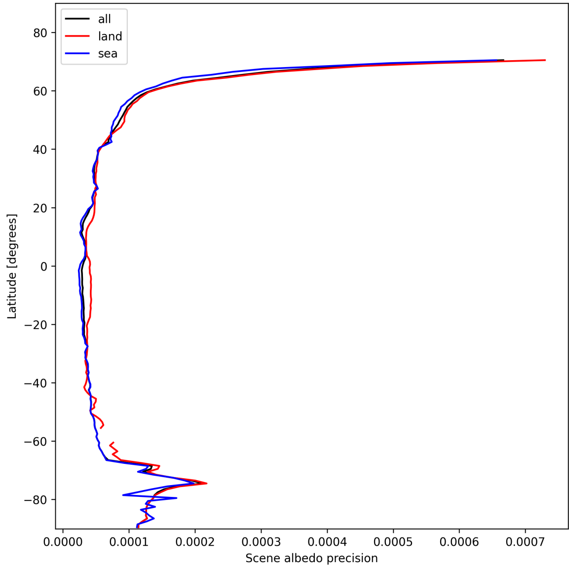
Figure 16: Zonal average of “Scene albedo precision” for 2025-01-28 to 2025-01-29.
