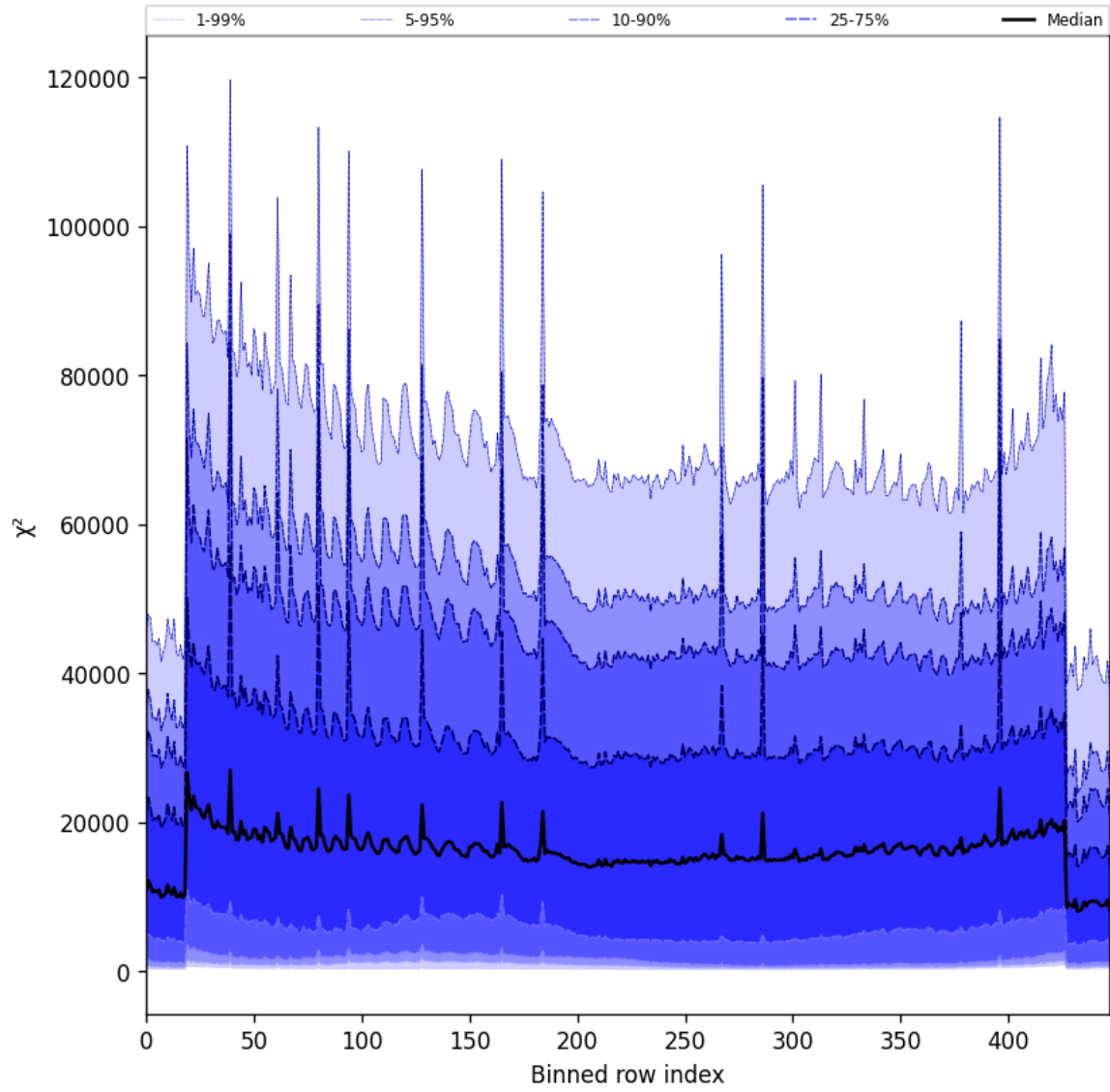
Figure 53: Along track statistics of “ \chi^2 ” for 2025-01-28 to 2025-01-29
