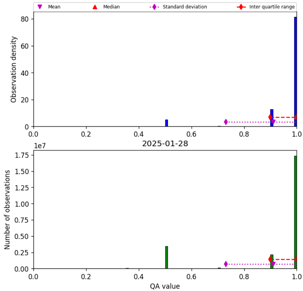
Figure 27: Histogram of “QA value” for 2025-01-28 to 2025-01-29
