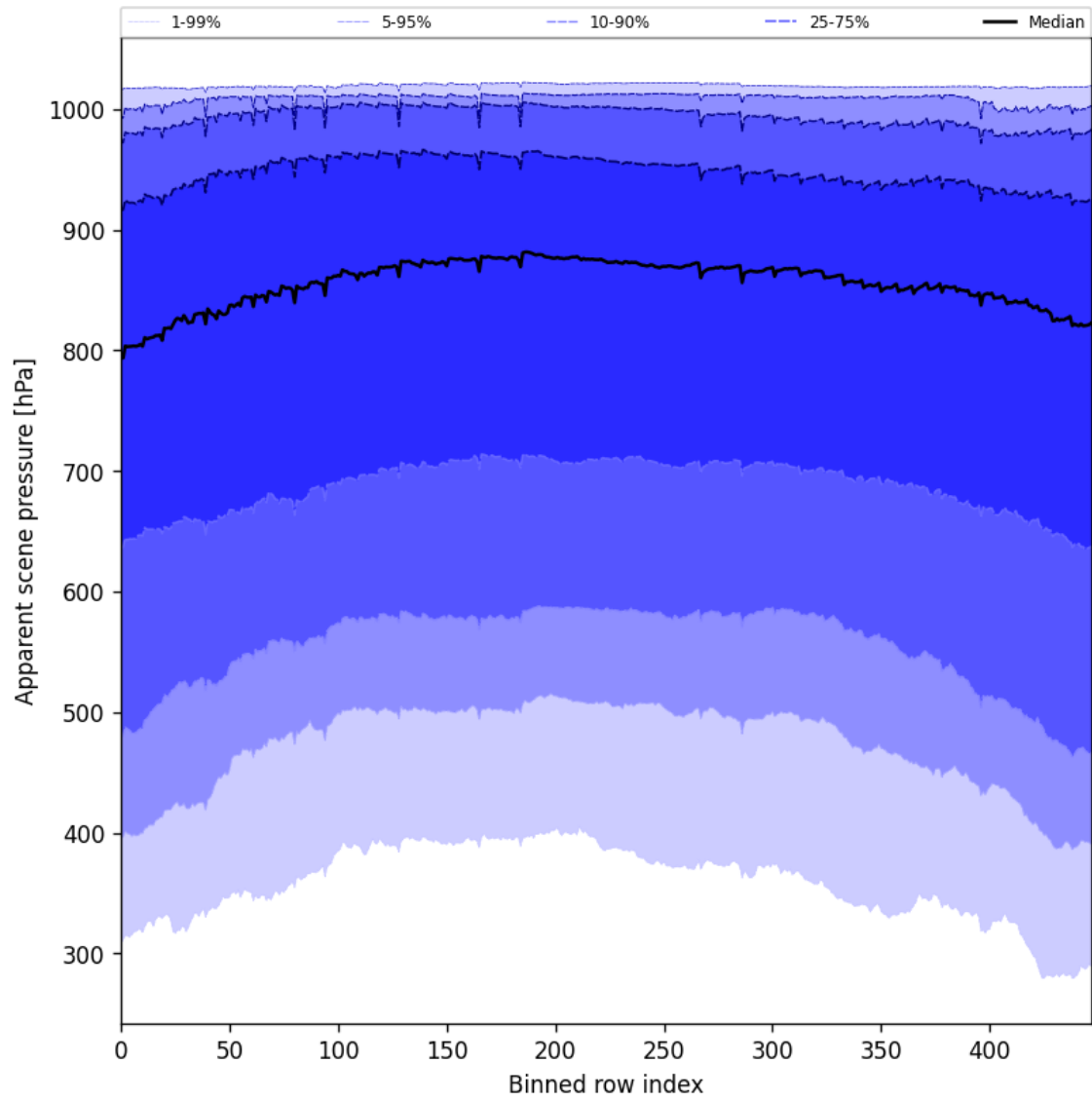
Figure 51: Along track statistics of “Apparent scene pressure” for 2025-01-28 to 2025-01-29
