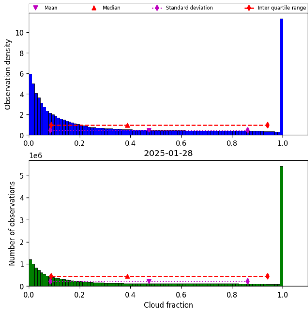
Figure 30: Histogram of “Cloud fraction” for 2025-01-28 to 2025-01-29
