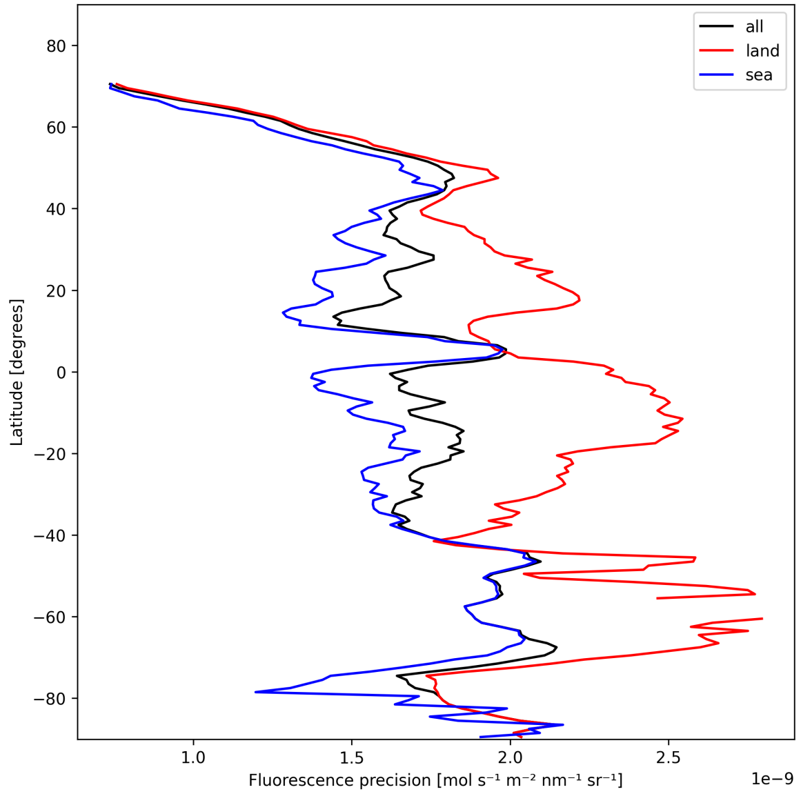
Figure 22: Zonal average of “Fluorescence precision” for 2025-01-28 to 2025-01-29.
