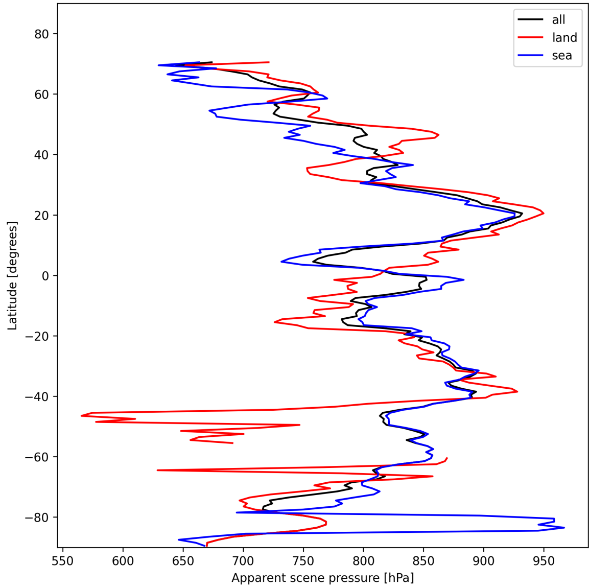
Figure 17: Zonal average of “Apparent scene pressure” for 2025-01-28 to 2025-01-29.
