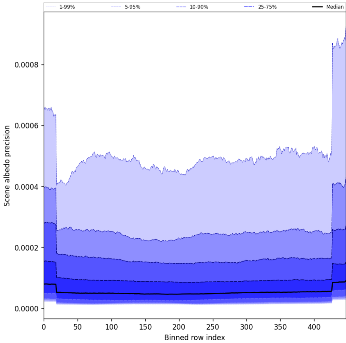
Figure 50: Along track statistics of “Scene albedo precision” for 2025-01-28 to 2025-01-29
