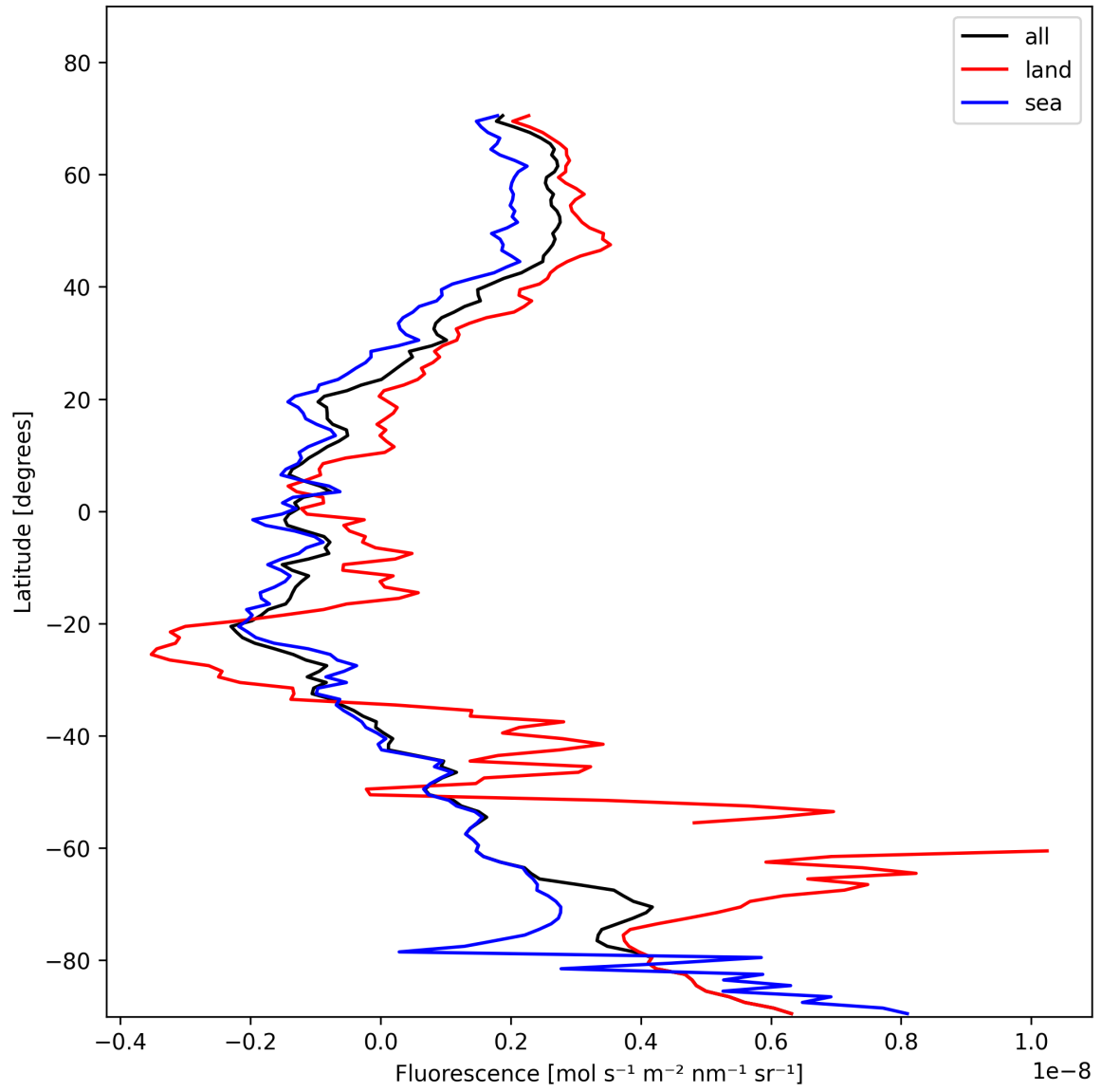
Figure 21: Zonal average of “Fluorescence” for 2025-01-28 to 2025-01-29.
