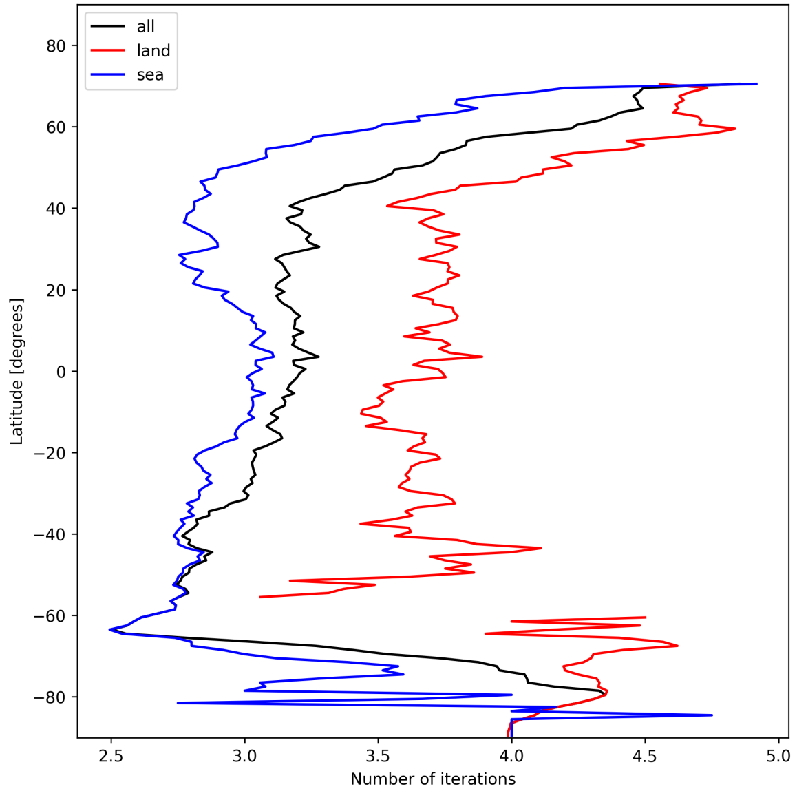
Figure 20: Zonal average of “Number of iterations” for 2025-01-28 to 2025-01-29.
