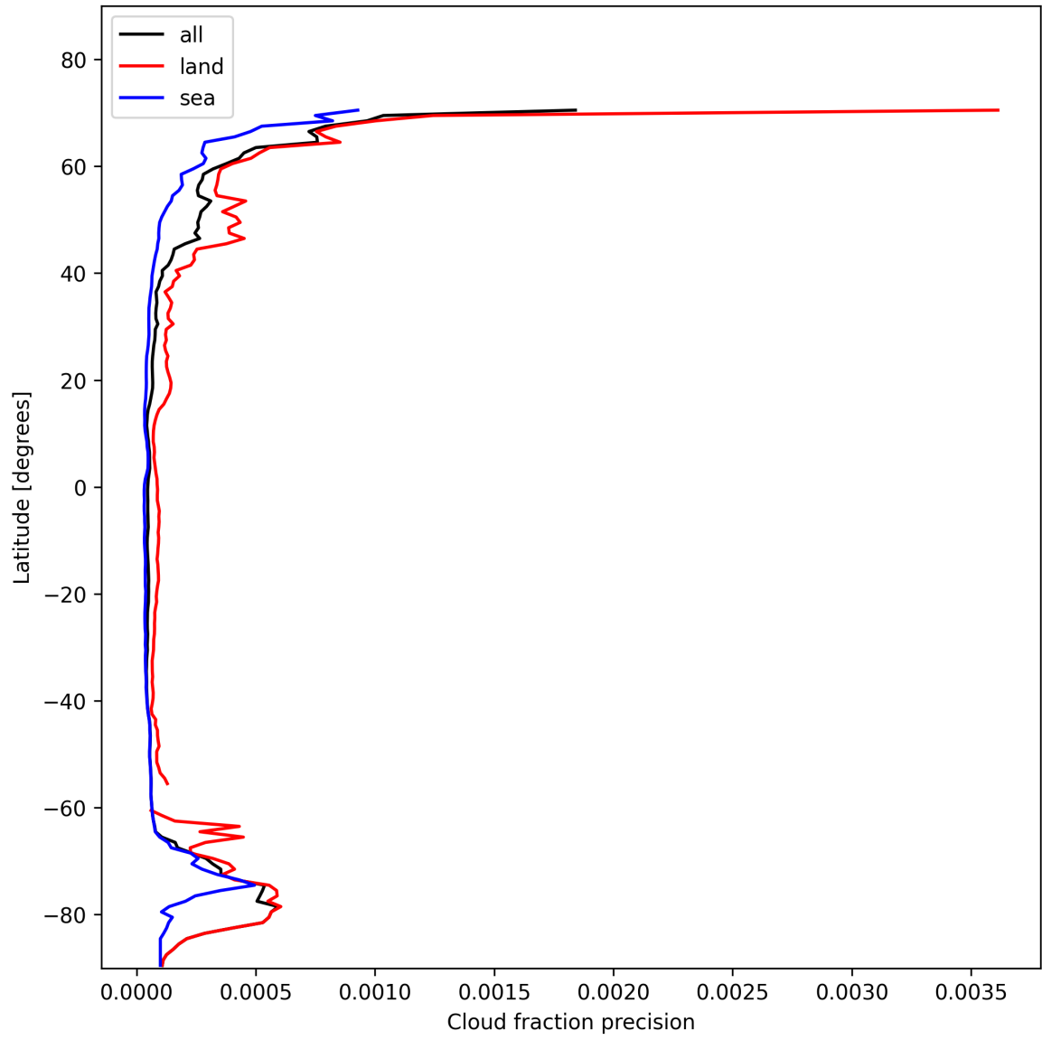
Figure 14: Zonal average of “Cloud fraction precision” for 2025-01-28 to 2025-01-29.
