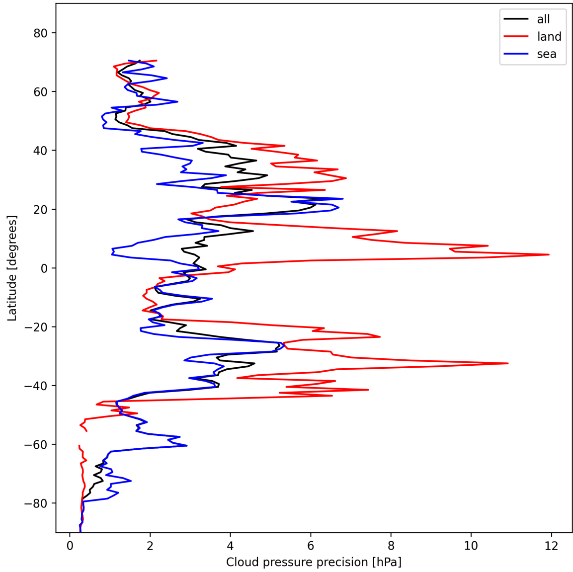
Figure 12: Zonal average of “Cloud pressure precision” for 2025-01-28 to 2025-01-29.
