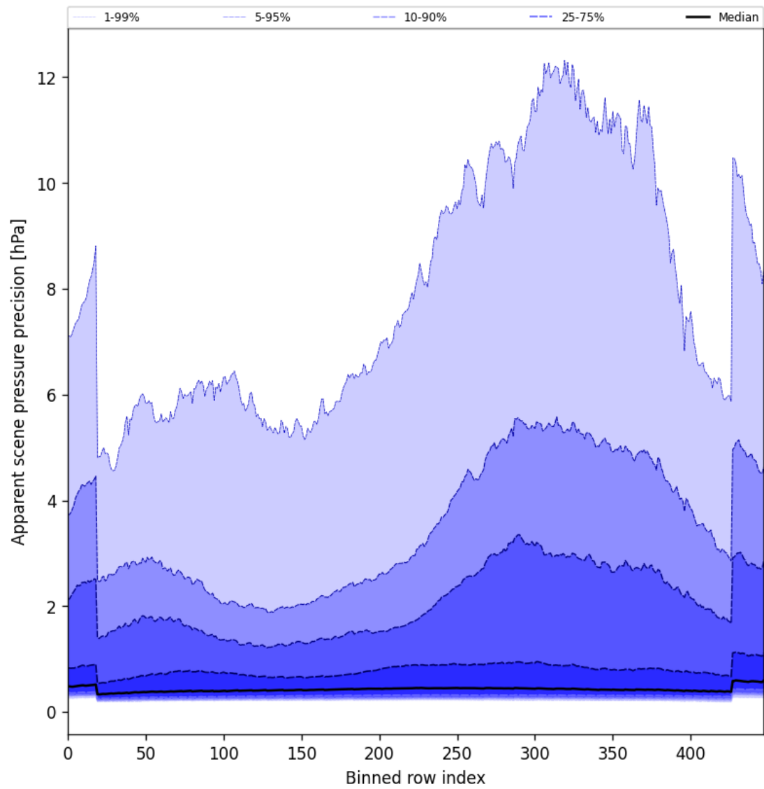
Figure 52: Along track statistics of “Apparent scene pressure precision” for 2025-01-28 to 2025-01-29
