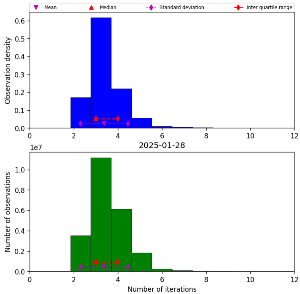
Figure 37: Histogram of “Number of iterations” for 2025-01-28 to 2025-01-29
