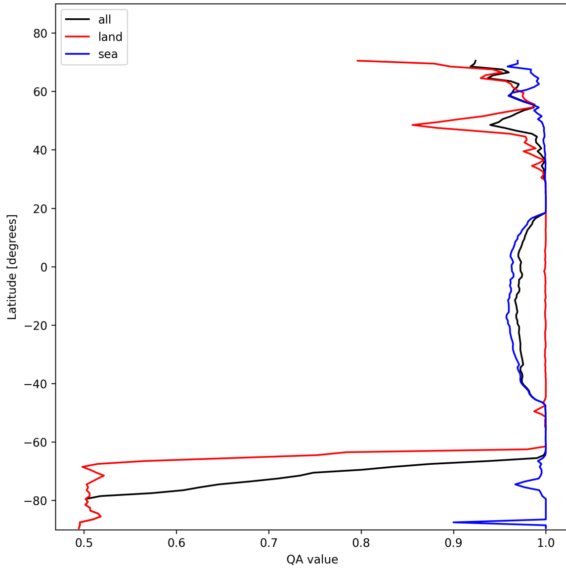
Figure 10: Zonal average of “QA value” for 2025-01-28 to 2025-01-29.
