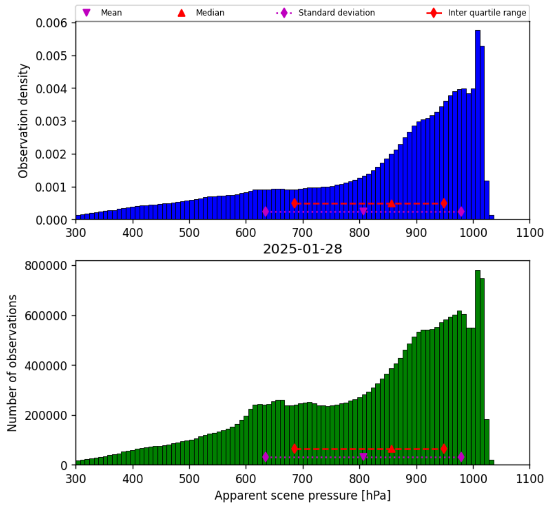
Figure 34: Histogram of “Apparent scene pressure” for 2025-01-28 to 2025-01-29
