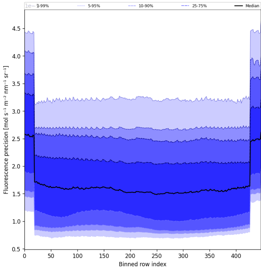
Figure 56: Along track statistics of “Fluorescence precision” for 2025-01-28 to 2025-01-29
