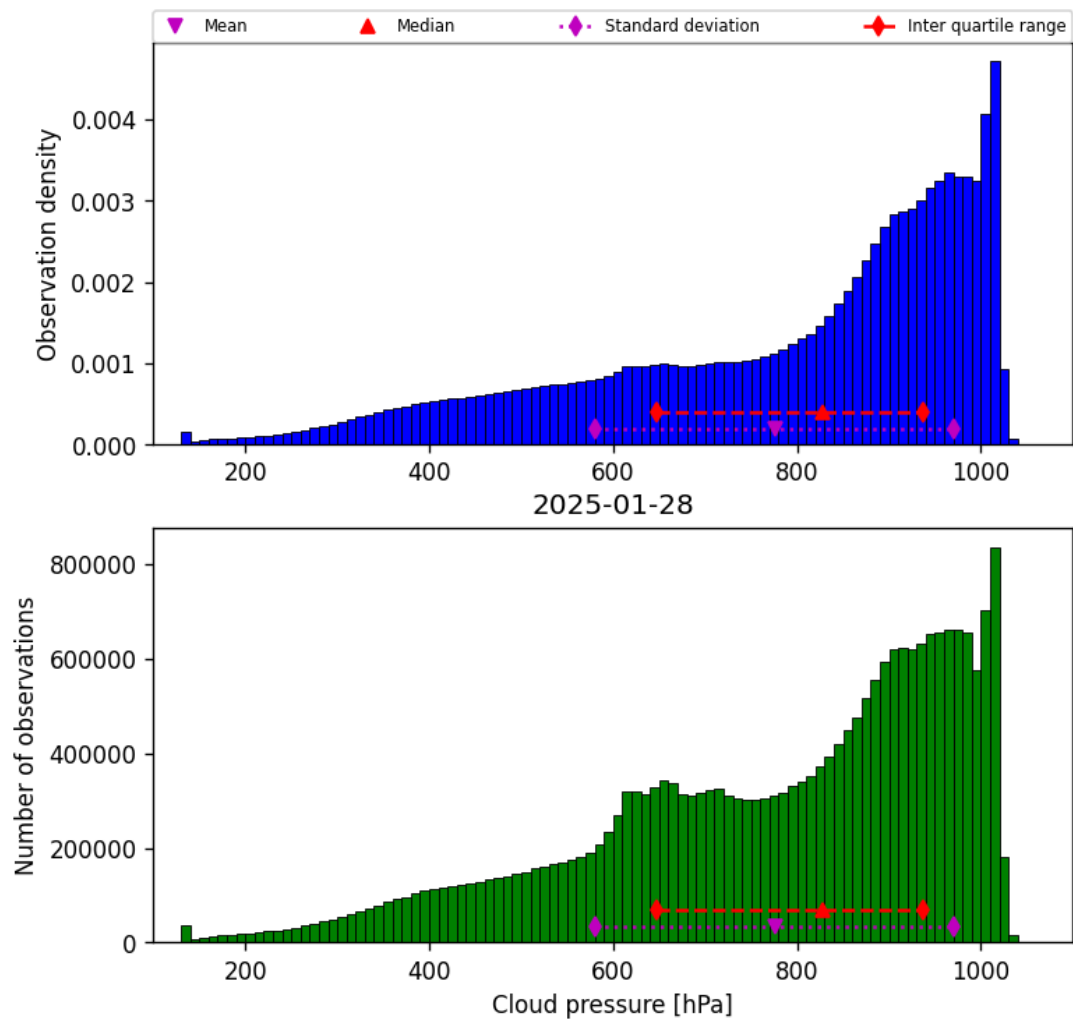
Figure 28: Histogram of “Cloud pressure” for 2025-01-28 to 2025-01-29
