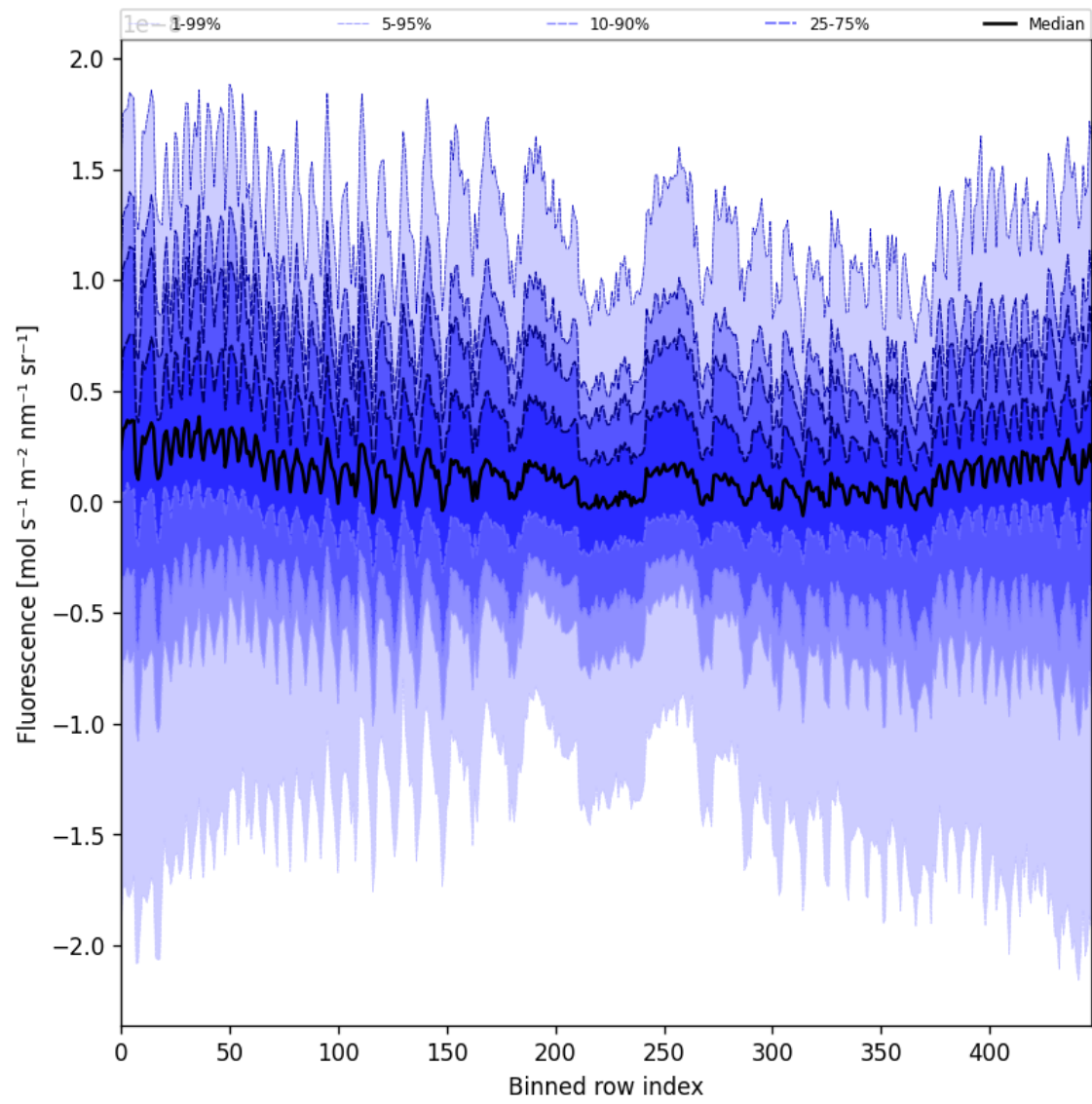
Figure 55: Along track statistics of “Fluorescence” for 2025-01-28 to 2025-01-29
