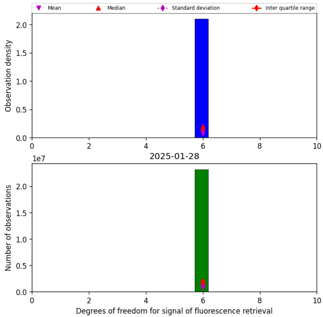
Figure 41: Histogram of “Degrees of freedom for signal of fluorescence retrieval” for 2025-01-28 to 2025-01-29
