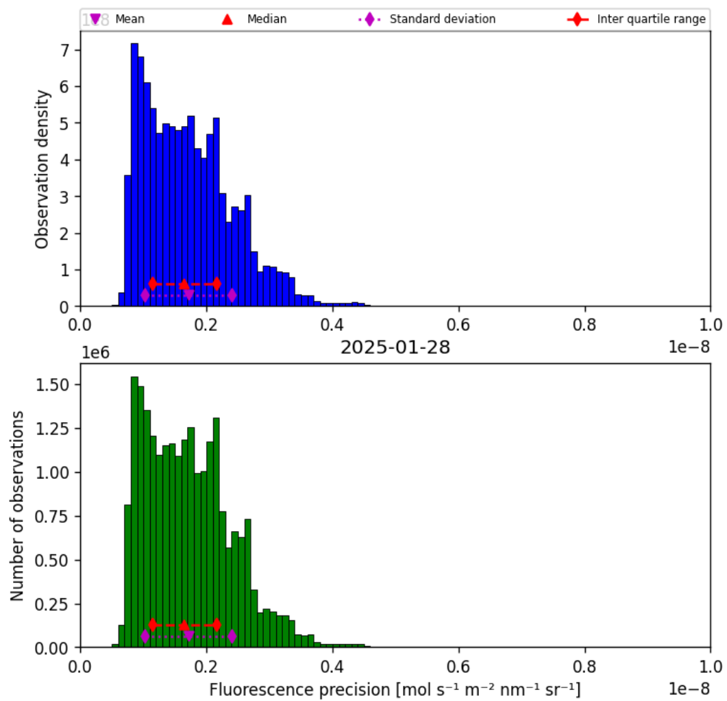
Figure 39: Histogram of “Fluorescence precision” for 2025-01-28 to 2025-01-29
