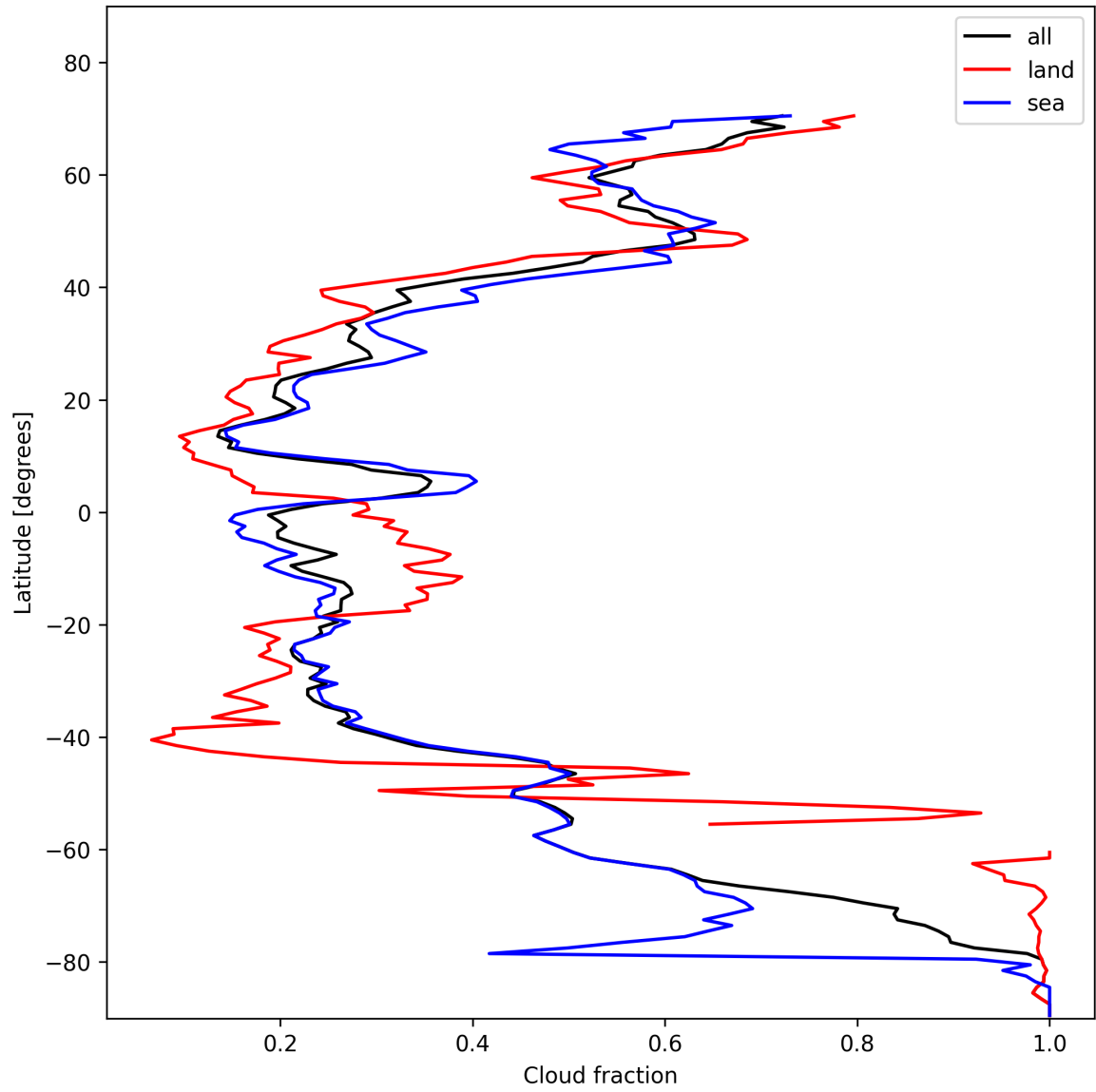
Figure 13: Zonal average of “Cloud fraction” for 2025-01-28 to 2025-01-29.
