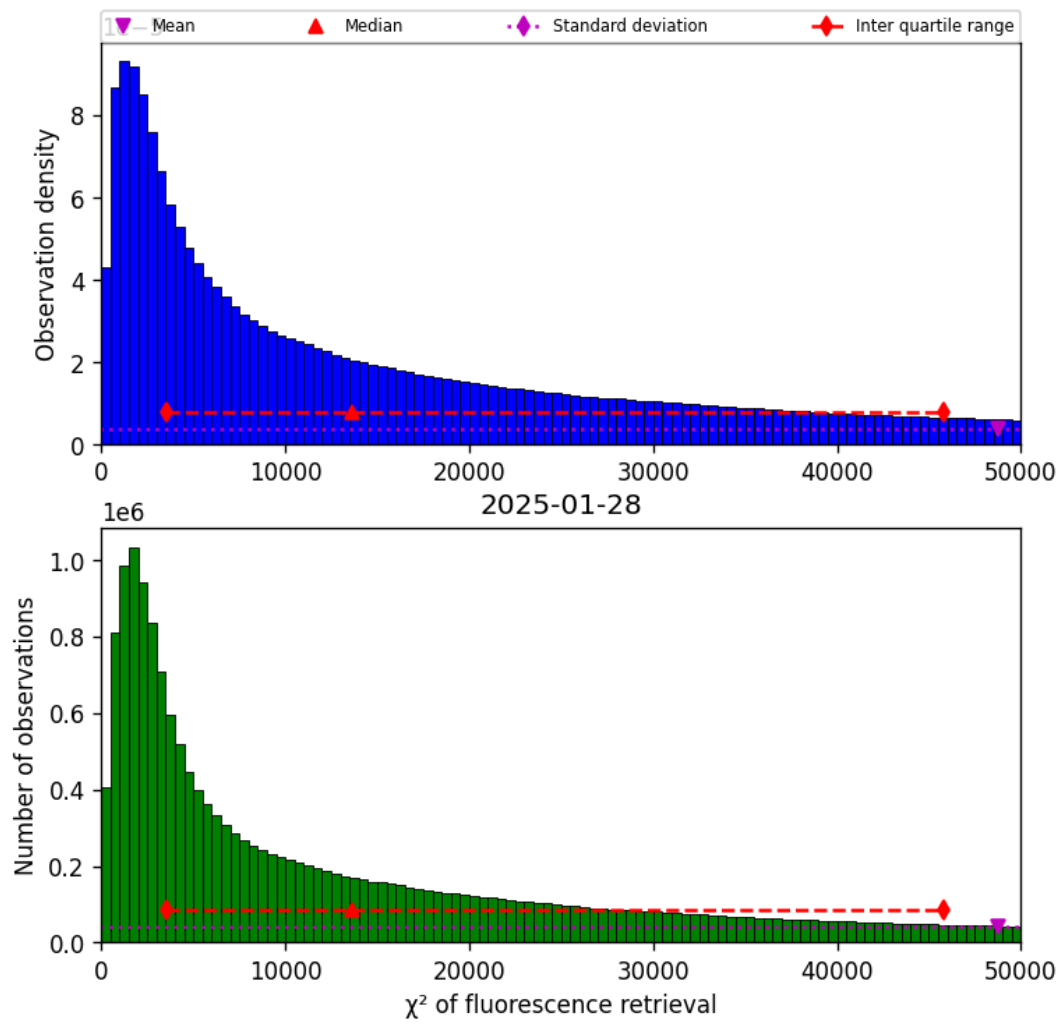
Figure 40: Histogram of “ \chi^2 of fluorescence retrieval” for 2025-01-28 to 2025-01-29
