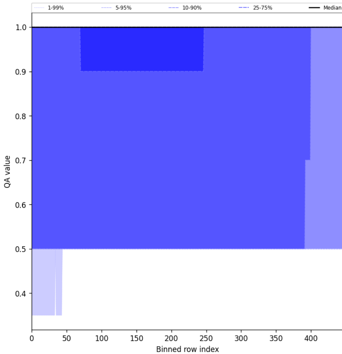
Figure 44: Along track statistics of “QA value” for 2025-01-28 to 2025-01-29
