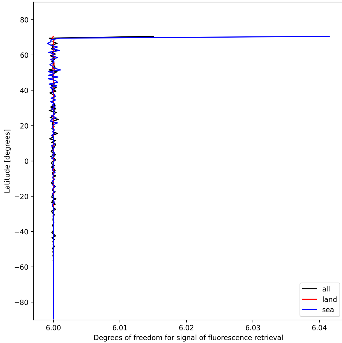
Figure 24: Zonal average of “Degrees of freedom for signal of fluorescence retrieval” for 2025-01-28 to 2025-01-29.
