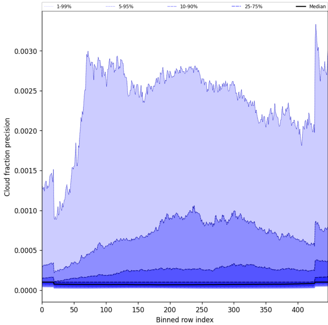
Figure 48: Along track statistics of “Cloud fraction precision” for 2025-01-28 to 2025-01-29
