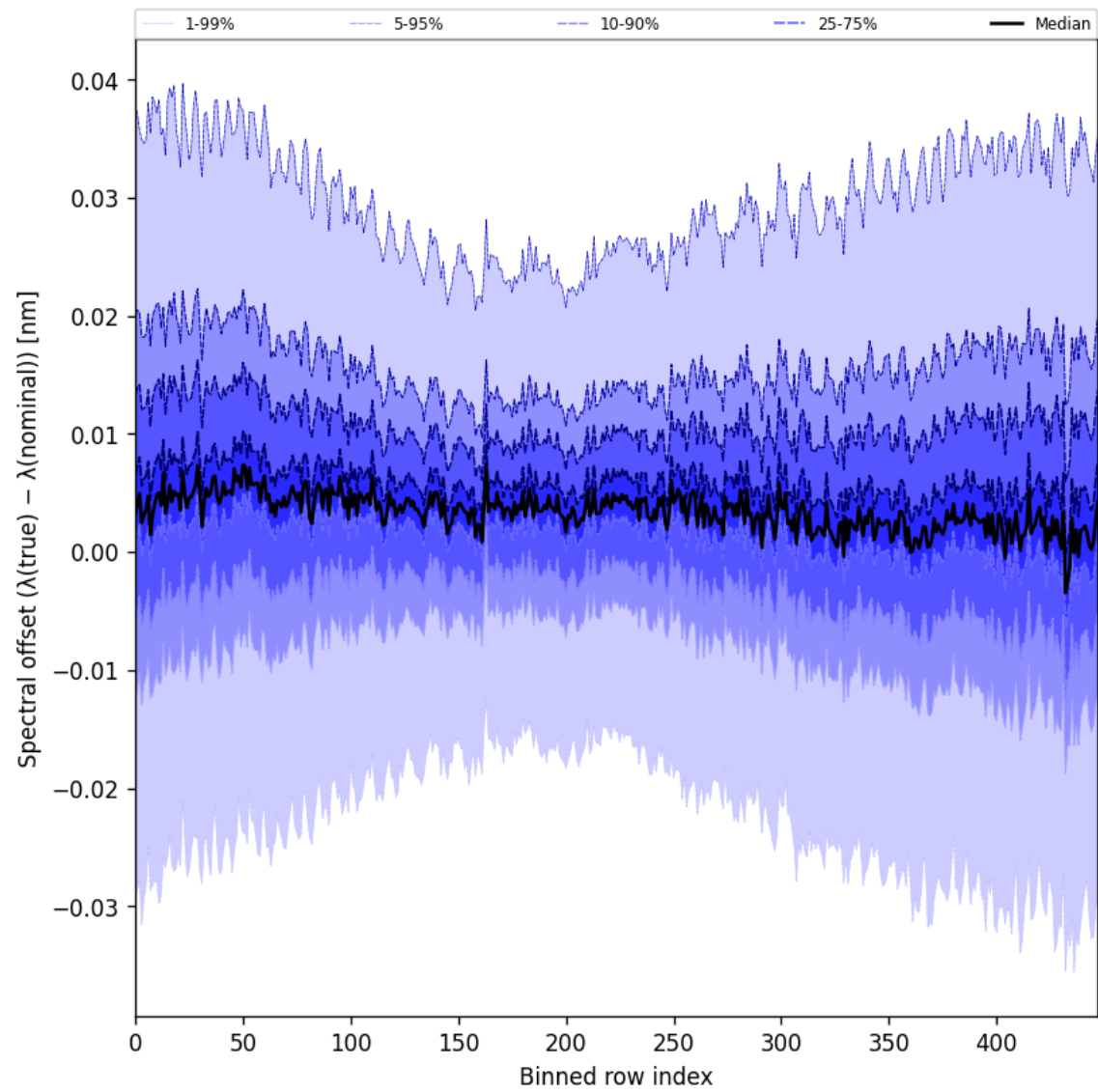
Figure 60: Along track statistics of “Spectral offset ( \lambda_{\text{true}} - \lambda_{\text{nominal}} )” for 2025-01-28 to 2025-01-29
