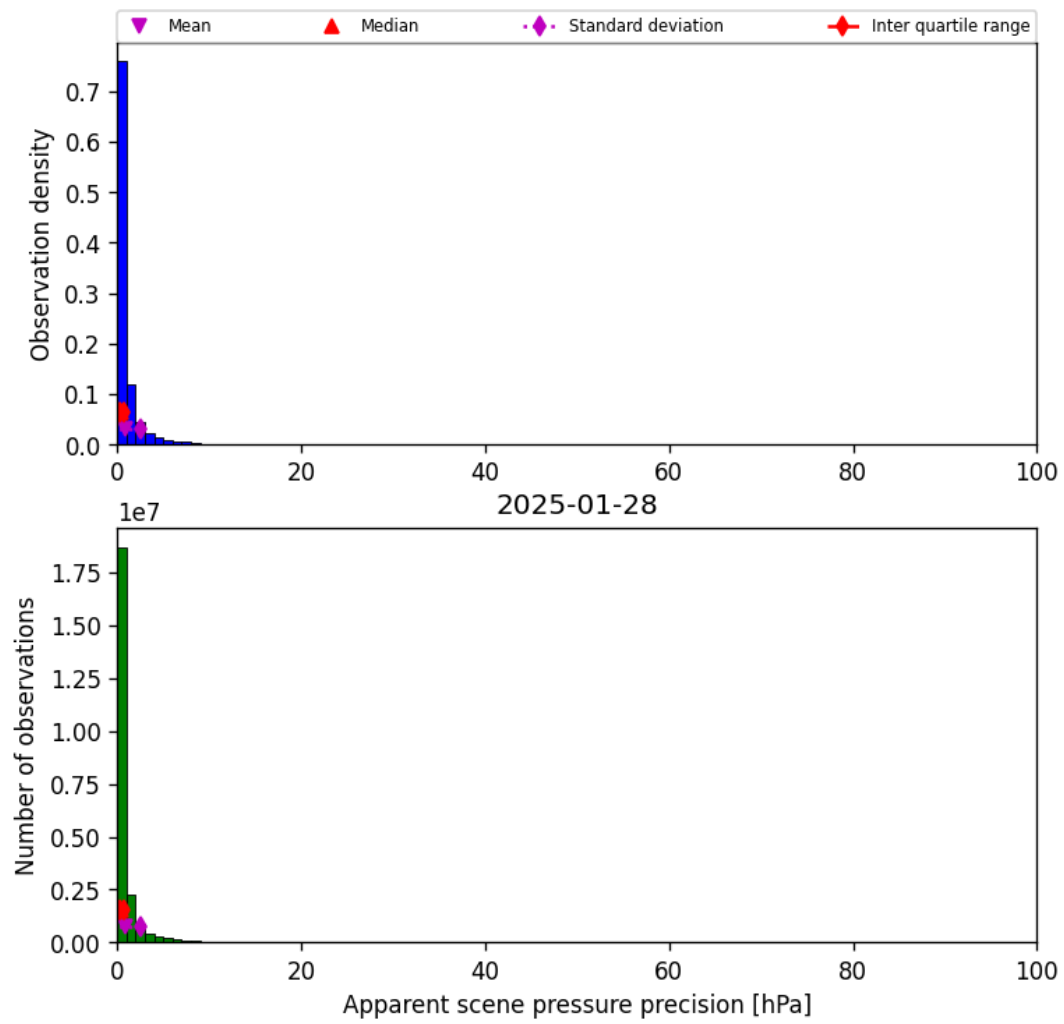
Figure 35: Histogram of “Apparent scene pressure precision” for 2025-01-28 to 2025-01-29
