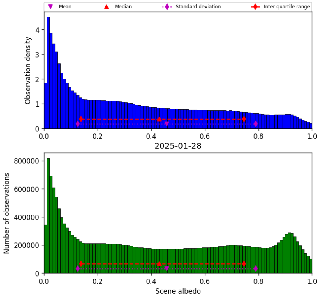
Figure 32: Histogram of “Scene albedo” for 2025-01-28 to 2025-01-29
