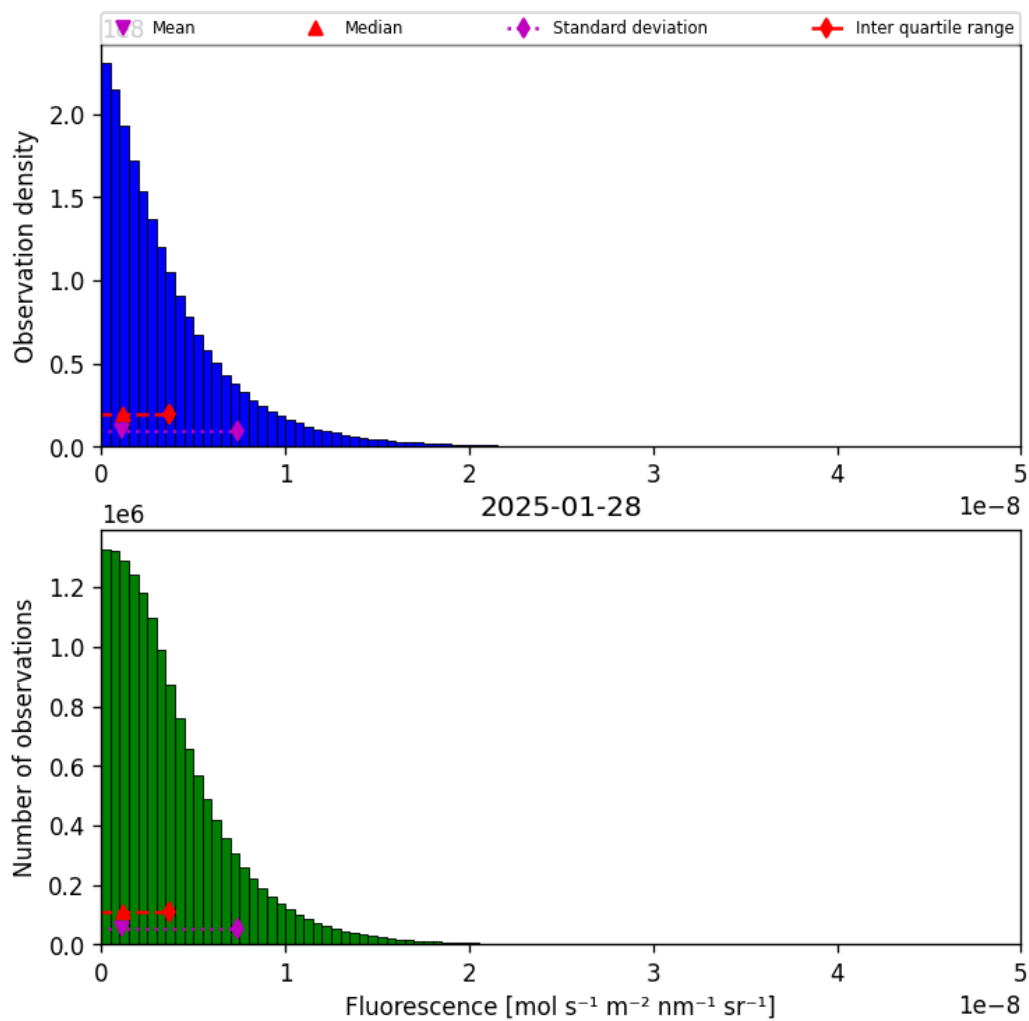
Figure 38: Histogram of “Fluorescence” for 2025-01-28 to 2025-01-29
