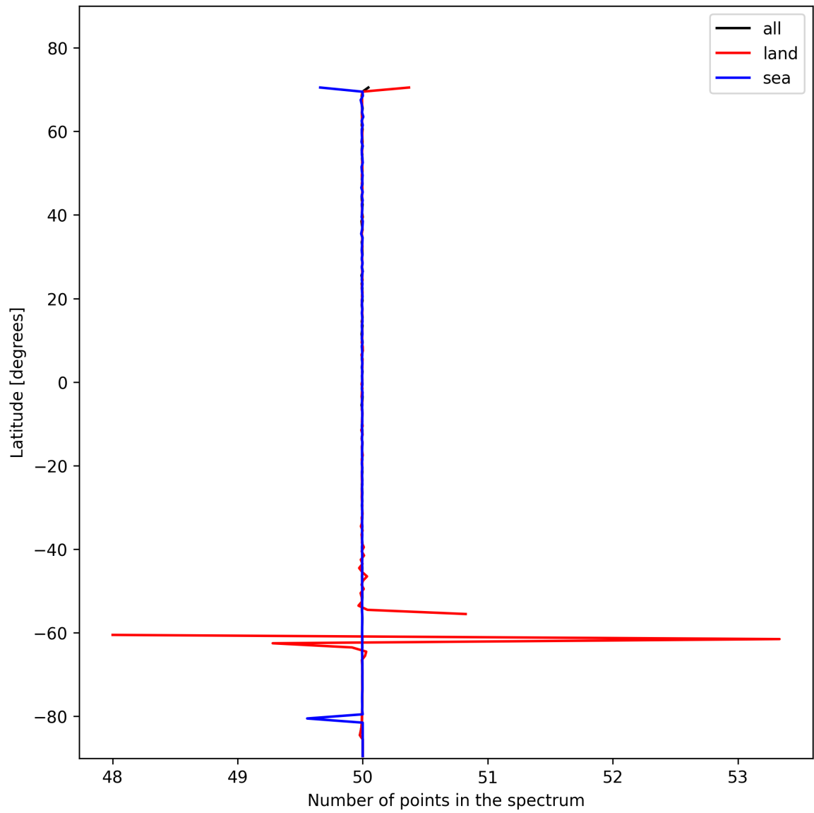
Figure 25: Zonal average of “Number of points in the spectrum” for 2025-01-28 to 2025-01-29.
