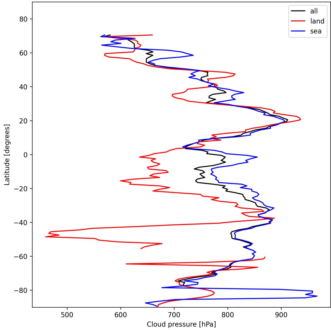
Figure 11: Zonal average of “Cloud pressure” for 2025-01-28 to 2025-01-29.
