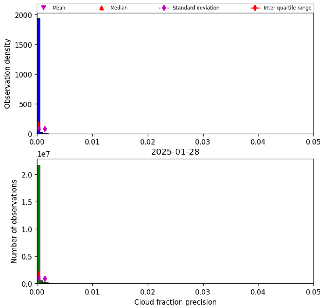
Figure 31: Histogram of “Cloud fraction precision” for 2025-01-28 to 2025-01-29
