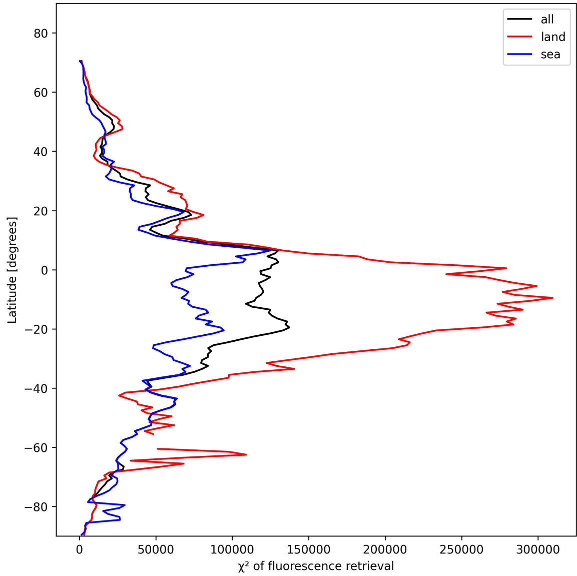
Figure 23: Zonal average of “ \chi^2 of fluorescence retrieval” for 2025-01-28 to 2025-01-29.
