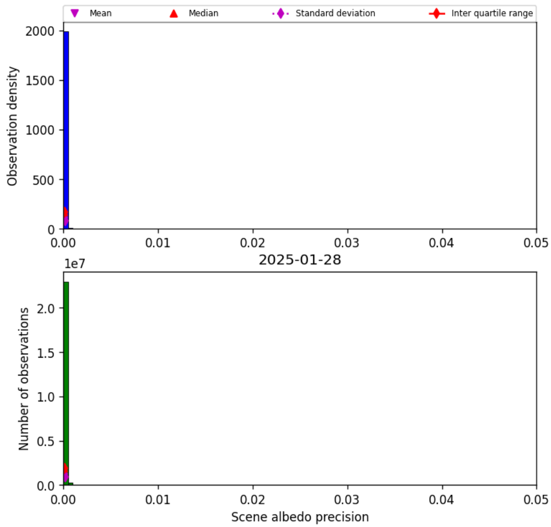
Figure 33: Histogram of “Scene albedo precision” for 2025-01-28 to 2025-01-29
