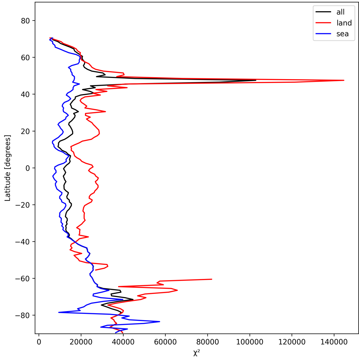
Figure 19: Zonal average of “ \chi^2 ” for 2025-01-28 to 2025-01-29.
