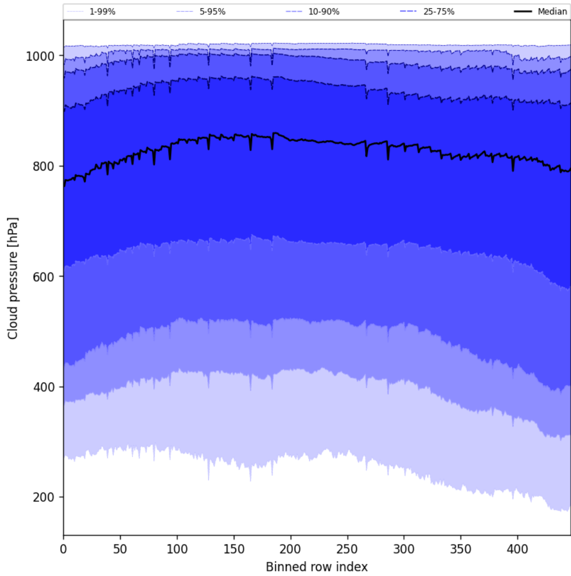
Figure 45: Along track statistics of “Cloud pressure” for 2025-01-28 to 2025-01-29
