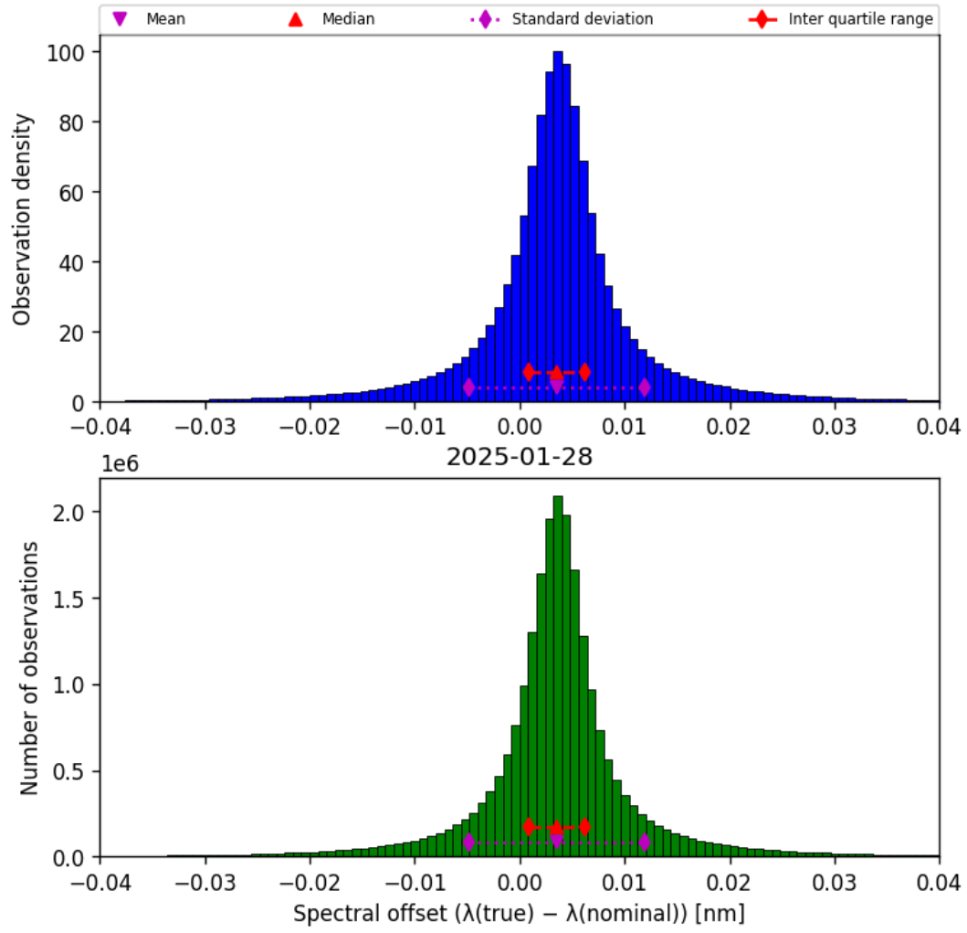
Figure 43: Histogram of “Spectral offset ( \lambda_{\text{true}} - \lambda_{\text{nominal}} )” for 2025-01-28 to 2025-01-29
