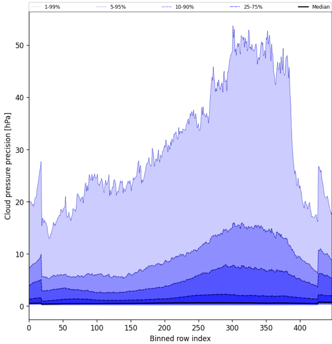
Figure 46: Along track statistics of “Cloud pressure precision” for 2025-01-28 to 2025-01-29
