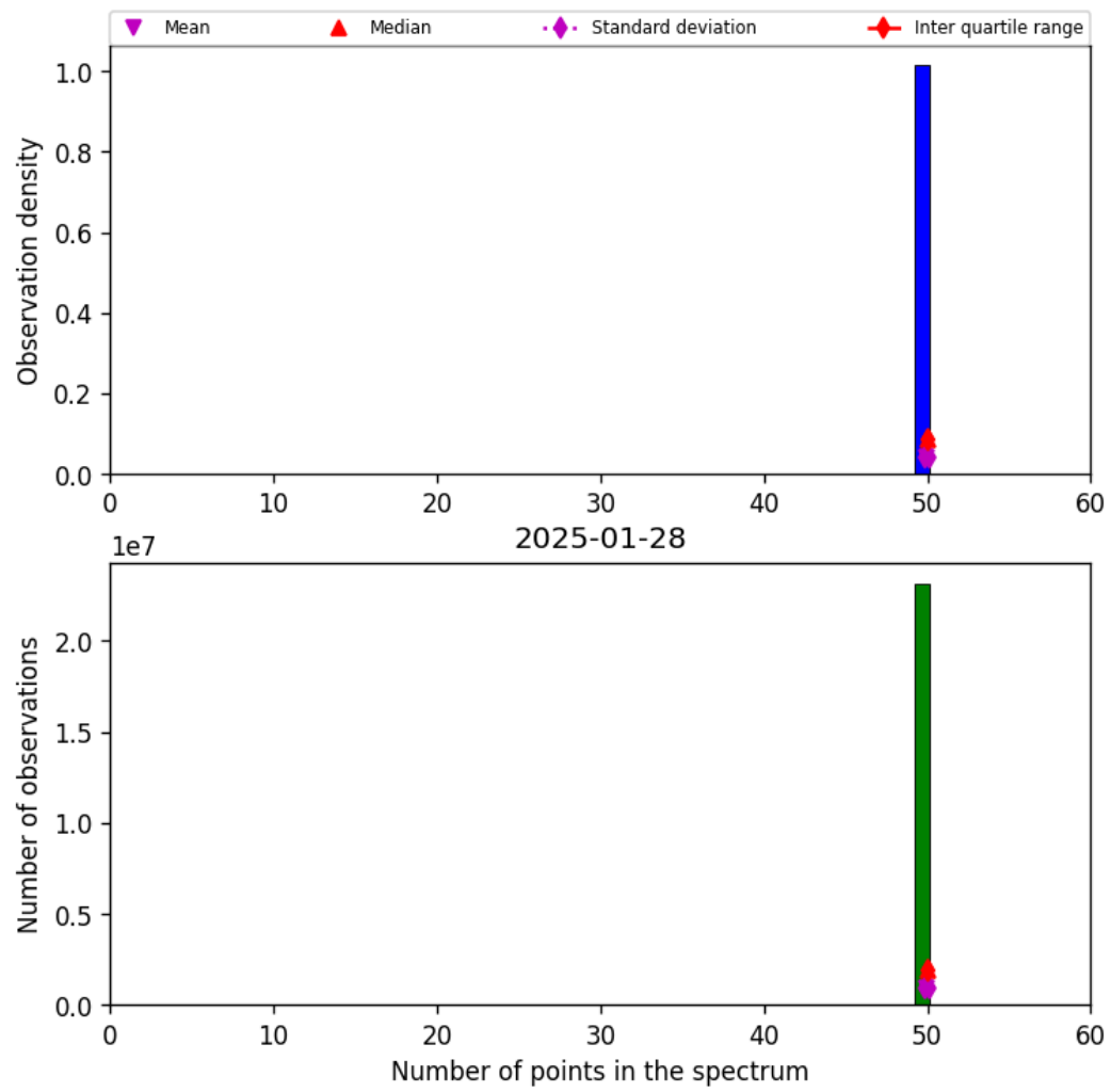
Figure 42: Histogram of “Number of points in the spectrum” for 2025-01-28 to 2025-01-29
