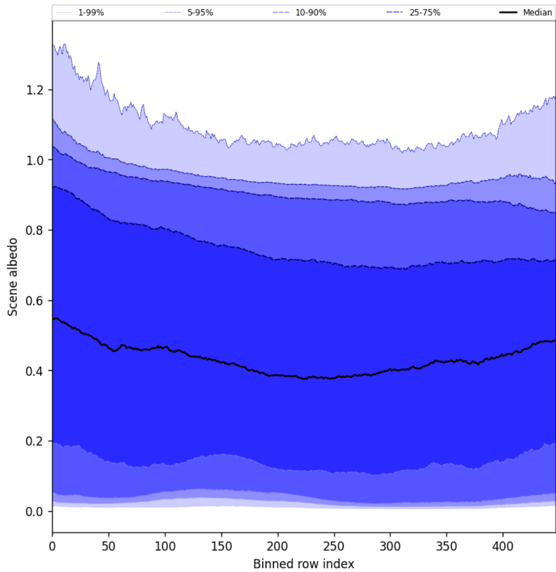
Figure 49: Along track statistics of “Scene albedo” for 2025-01-28 to 2025-01-29
