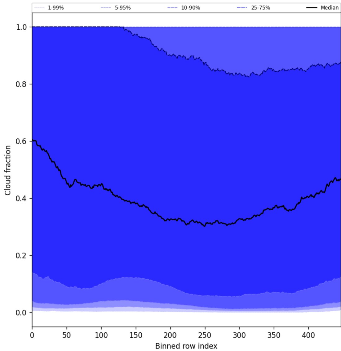
Figure 47: Along track statistics of “Cloud fraction” for 2025-01-28 to 2025-01-29
