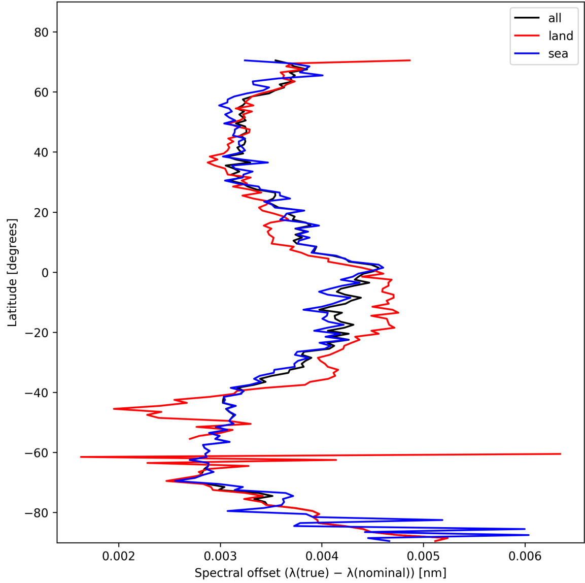
Figure 26: Zonal average of “Spectral offset ( \lambda_{\text{true}} - \lambda_{\text{nominal}} )” for 2025-01-28 to 2025-01-29.
