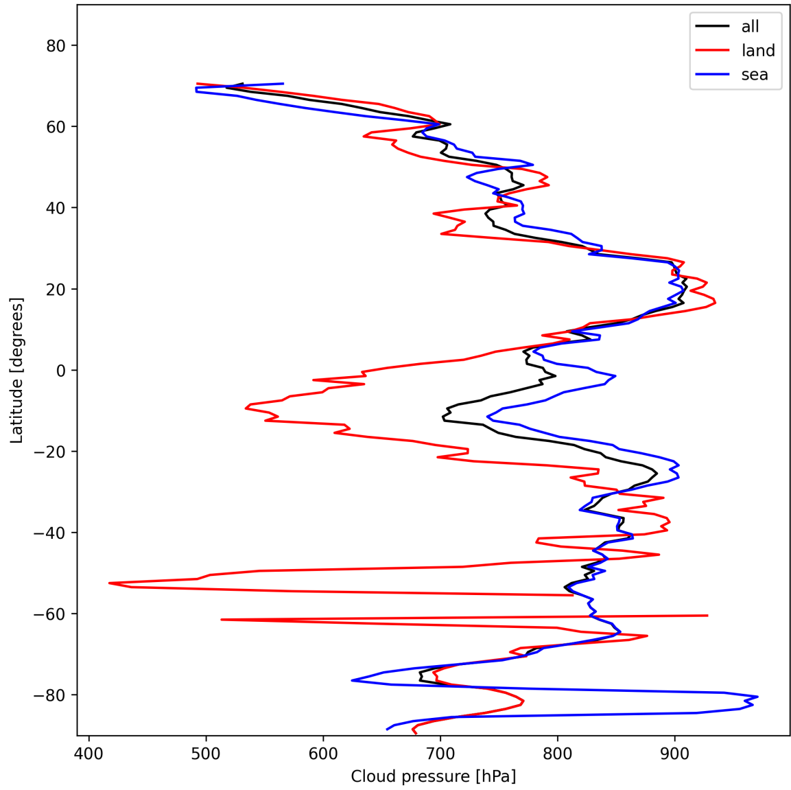
Figure 11: Zonal average of “Cloud pressure” for 2025-01-30 to 2025-01-31.
