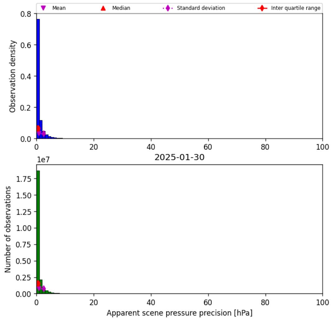
Figure 35: Histogram of “Apparent scene pressure precision” for 2025-01-30 to 2025-01-31
