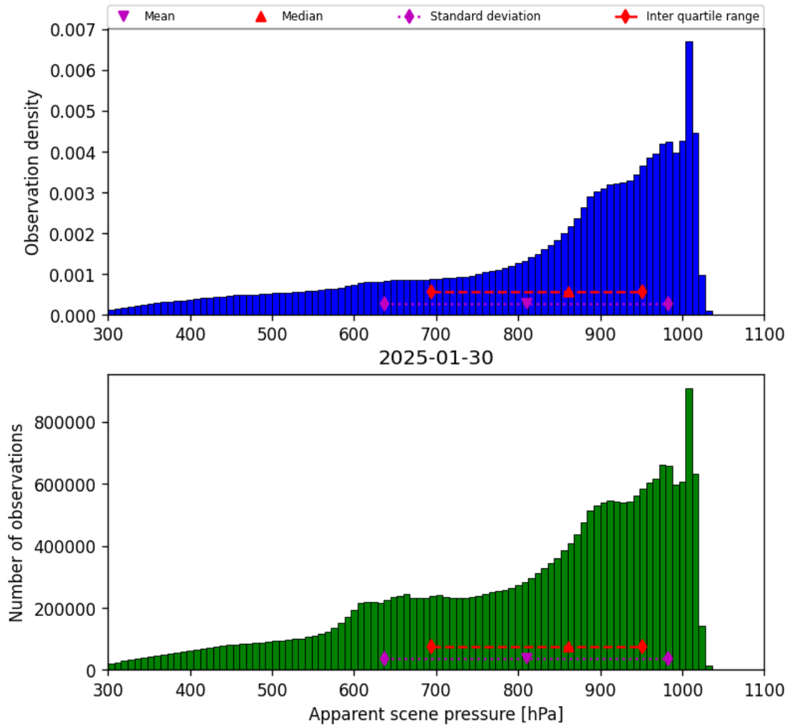
Figure 34: Histogram of “Apparent scene pressure” for 2025-01-30 to 2025-01-31
