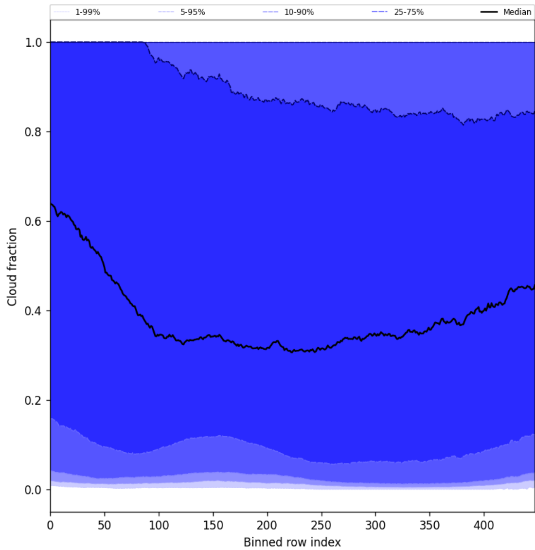
Figure 47: Along track statistics of “Cloud fraction” for 2025-01-30 to 2025-01-31
