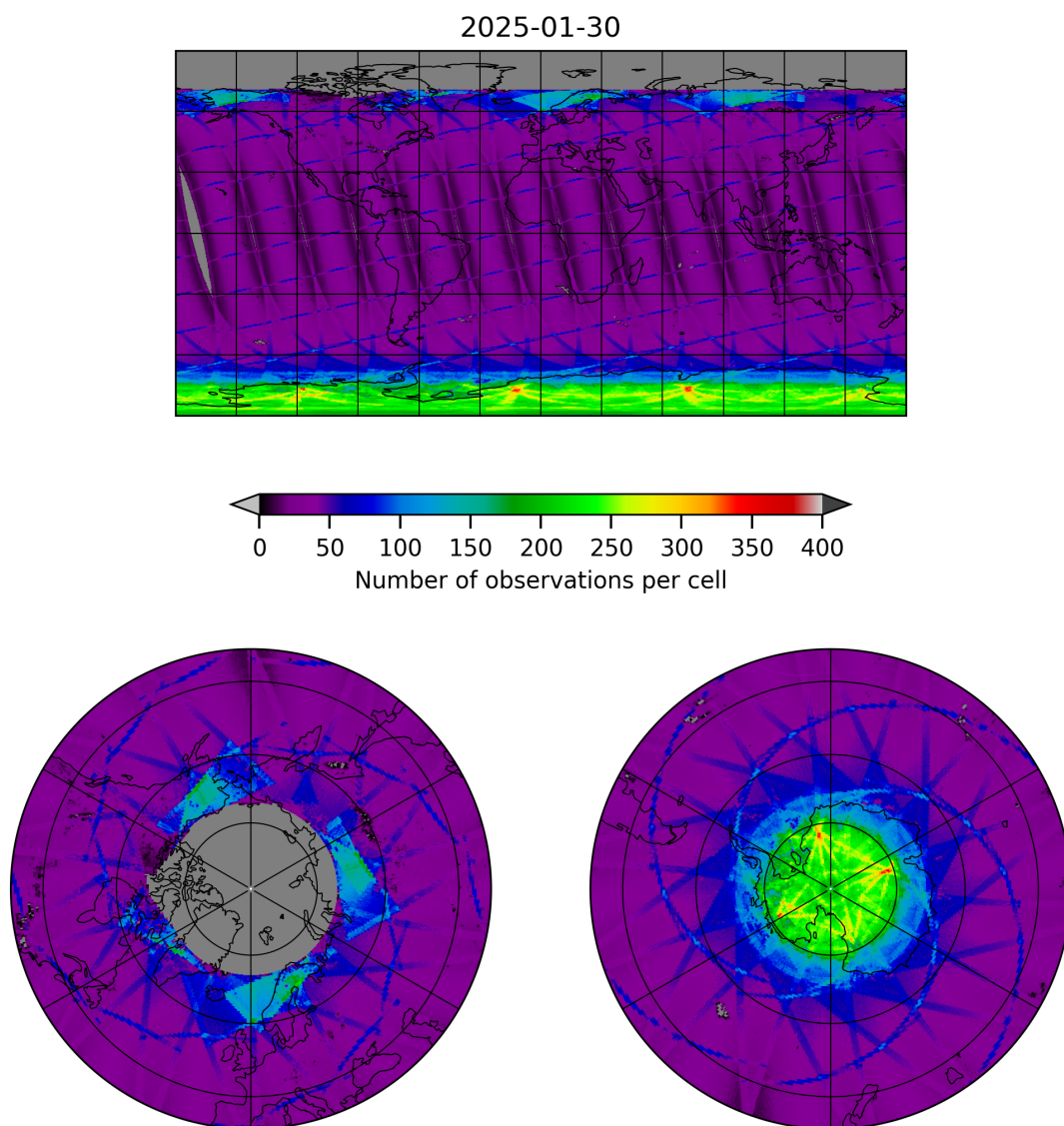
Figure 9: Map of the number of observations for 2025-01-30 to 2025-01-31
