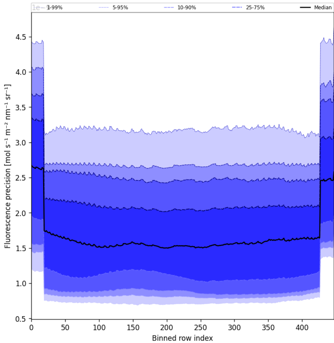
Figure 56: Along track statistics of “Fluorescence precision” for 2025-01-30 to 2025-01-31
