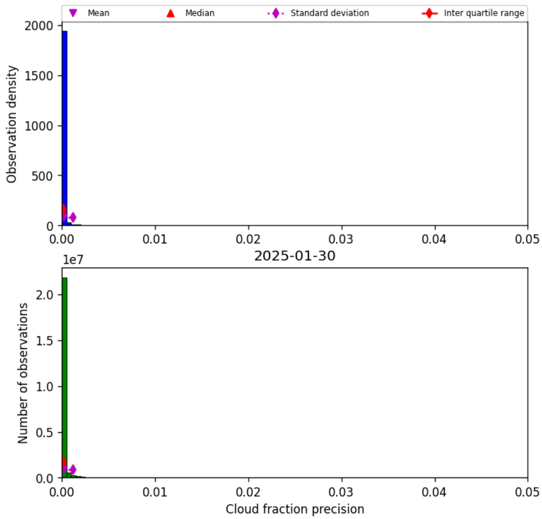
Figure 31: Histogram of “Cloud fraction precision” for 2025-01-30 to 2025-01-31
