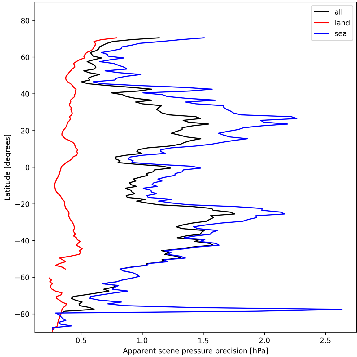
Figure 18: Zonal average of “Apparent scene pressure precision” for 2025-01-30 to 2025-01-31.
