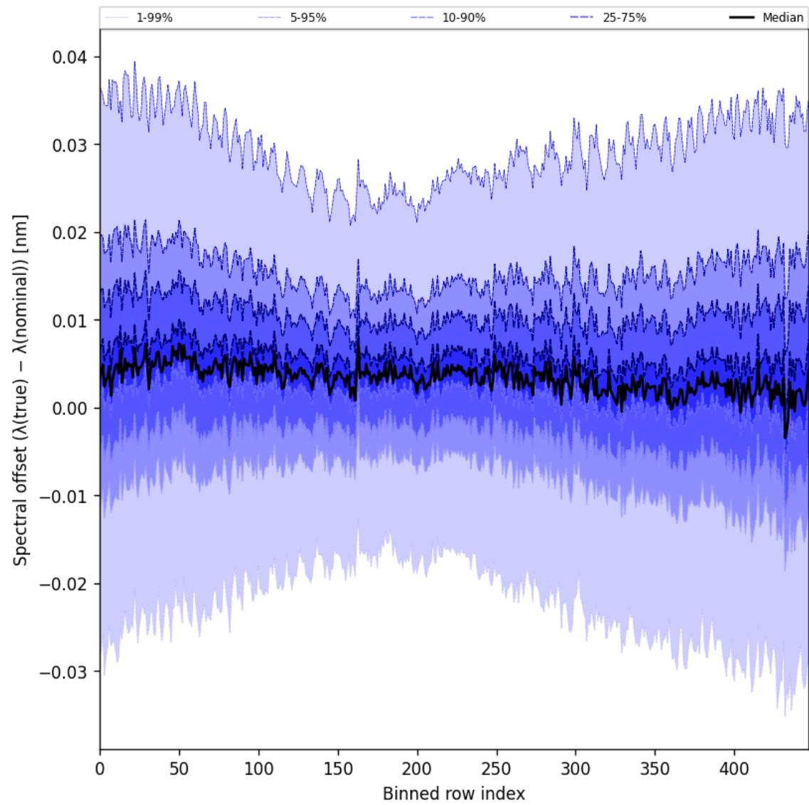
Figure 60: Along track statistics of “Spectral offset ( \lambda_{\text{true}} - \lambda_{\text{nominal}} )” for 2025-01-30 to 2025-01-31
