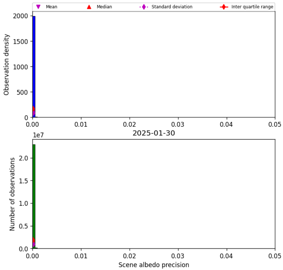
Figure 33: Histogram of “Scene albedo precision” for 2025-01-30 to 2025-01-31
