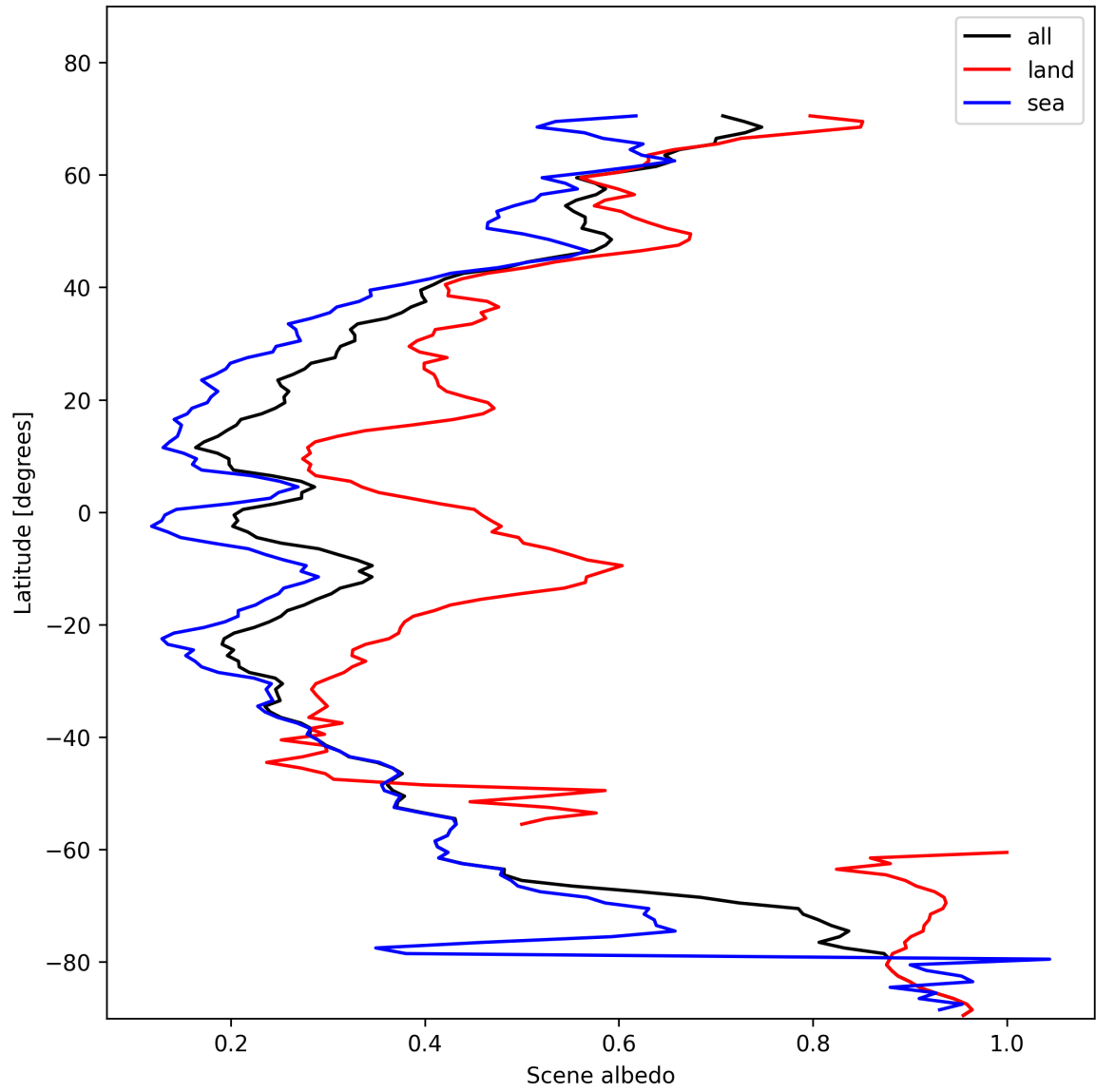
Figure 15: Zonal average of “Scene albedo” for 2025-01-30 to 2025-01-31.
