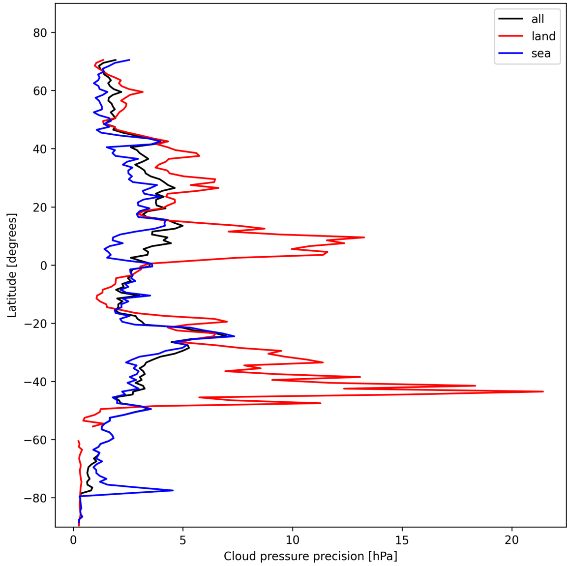
Figure 12: Zonal average of "Cloud pressure precision" for 2025-01-30 to 2025-01-31.
