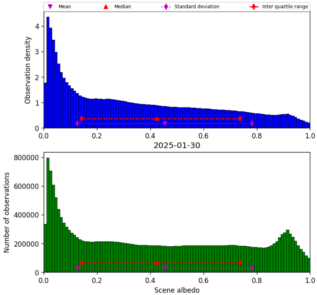
Figure 32: Histogram of “Scene albedo” for 2025-01-30 to 2025-01-31
