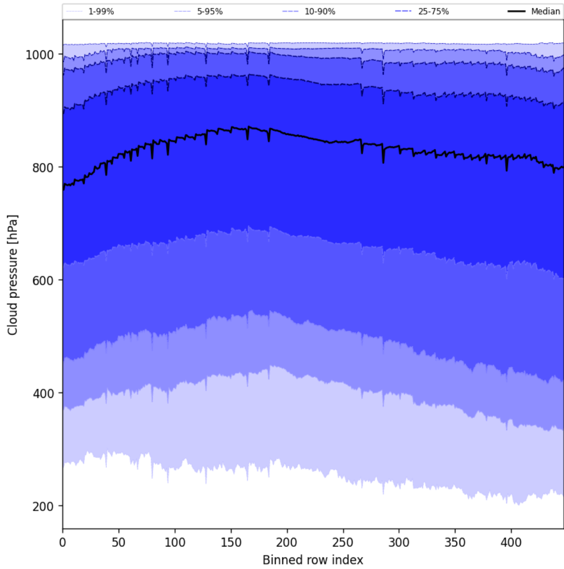
Figure 45: Along track statistics of “Cloud pressure” for 2025-01-30 to 2025-01-31
