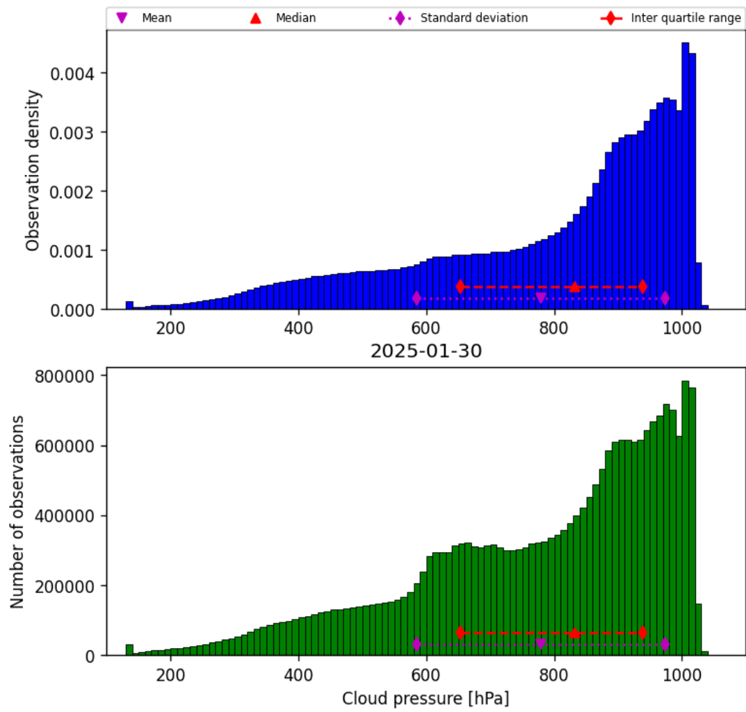
Figure 28: Histogram of “Cloud pressure” for 2025-01-30 to 2025-01-31
