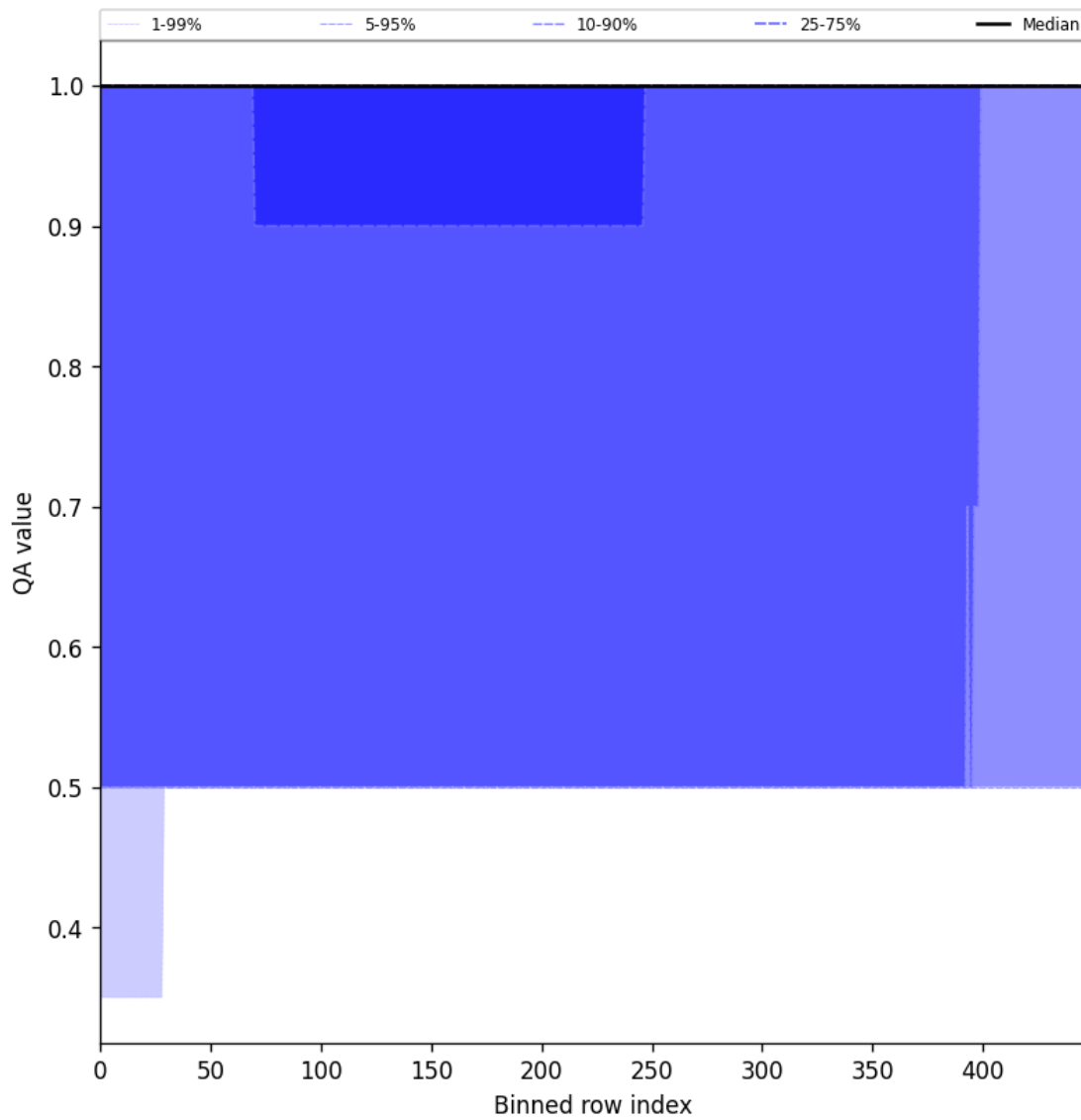
Figure 44: Along track statistics of “QA value” for 2025-01-30 to 2025-01-31
