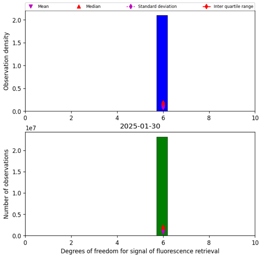
Figure 41: Histogram of “Degrees of freedom for signal of fluorescence retrieval” for 2025-01-30 to 2025-01-31
