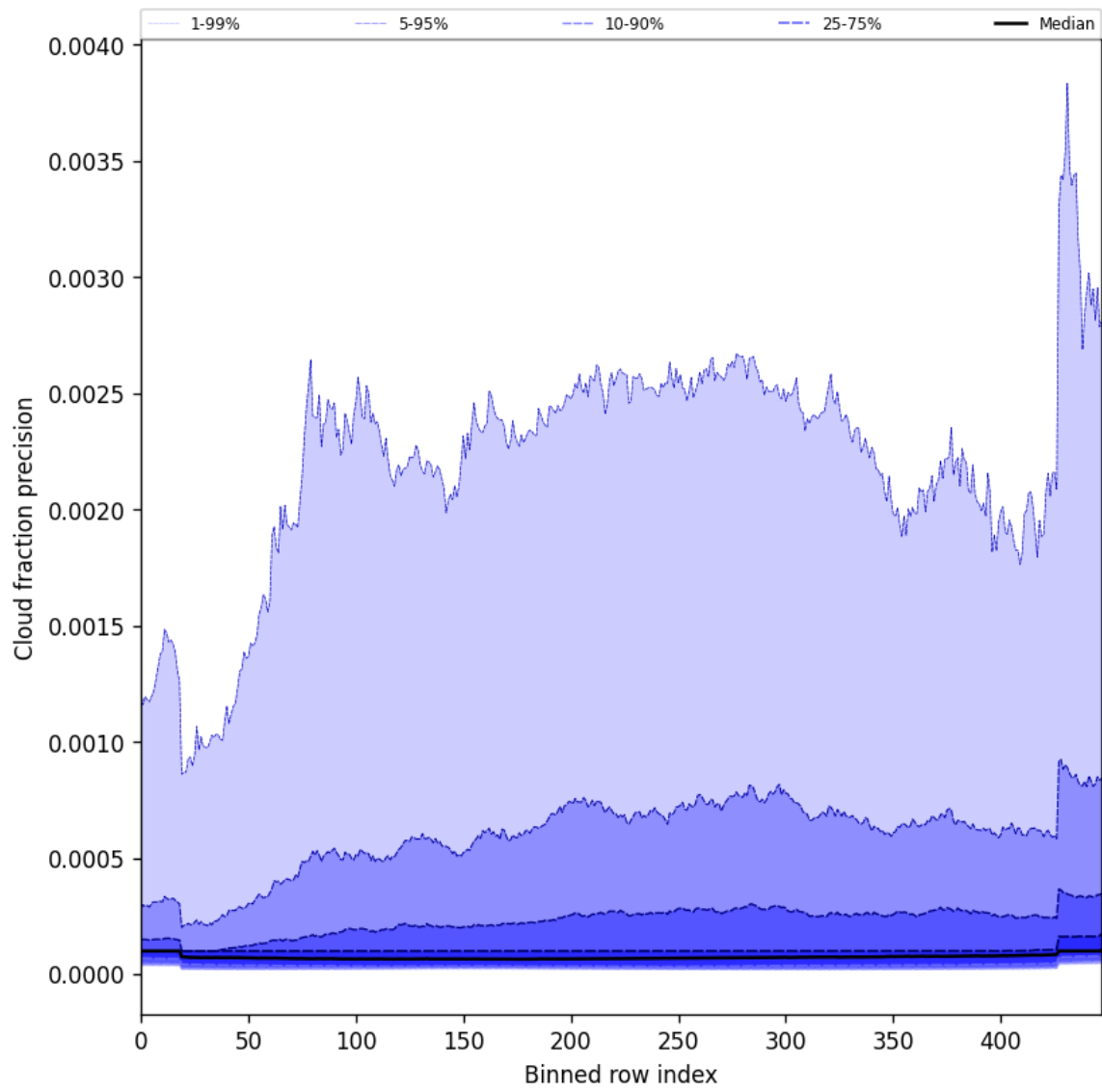
Figure 48: Along track statistics of “Cloud fraction precision” for 2025-01-30 to 2025-01-31
