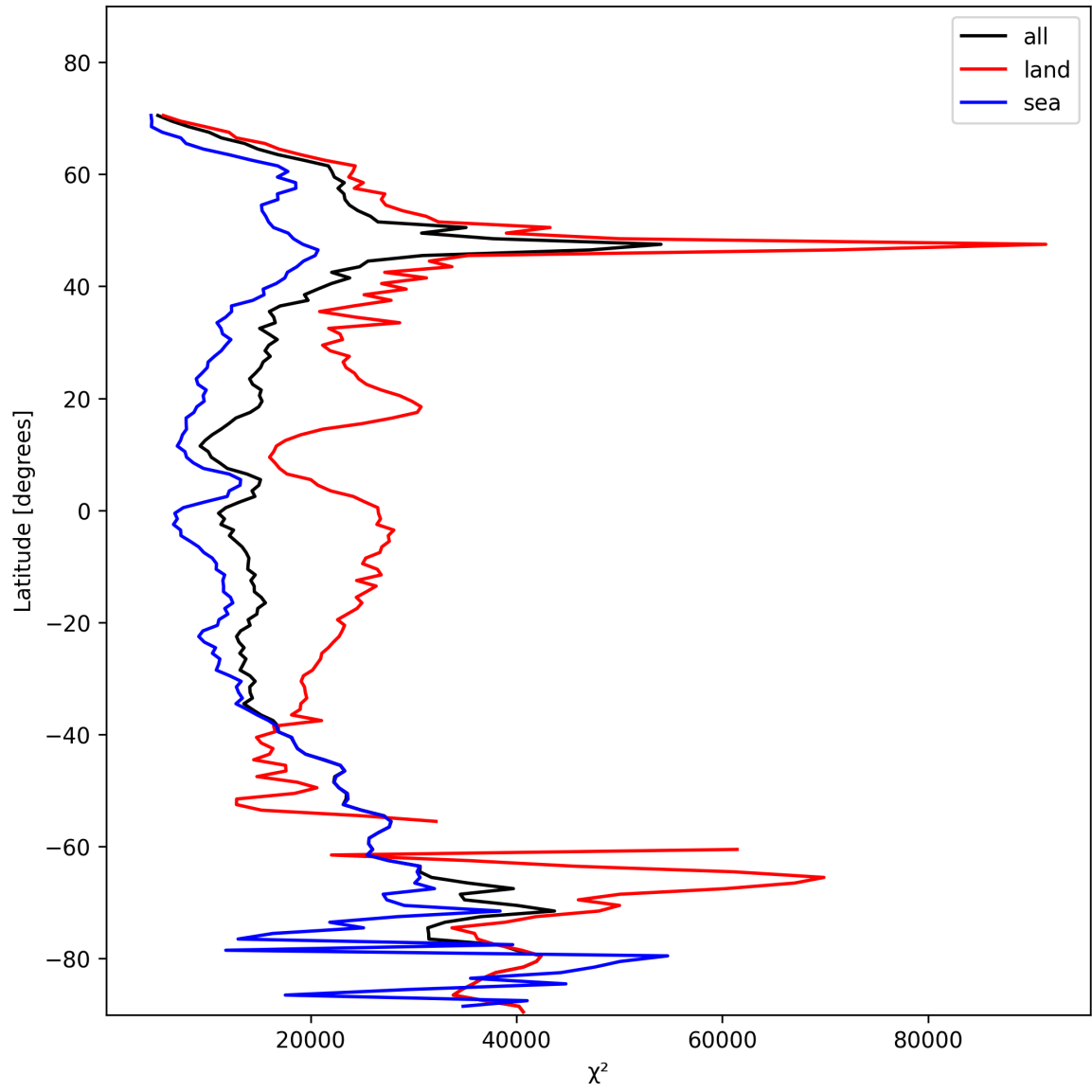
Figure 19: Zonal average of “ \chi^2 ” for 2025-01-30 to 2025-01-31.
