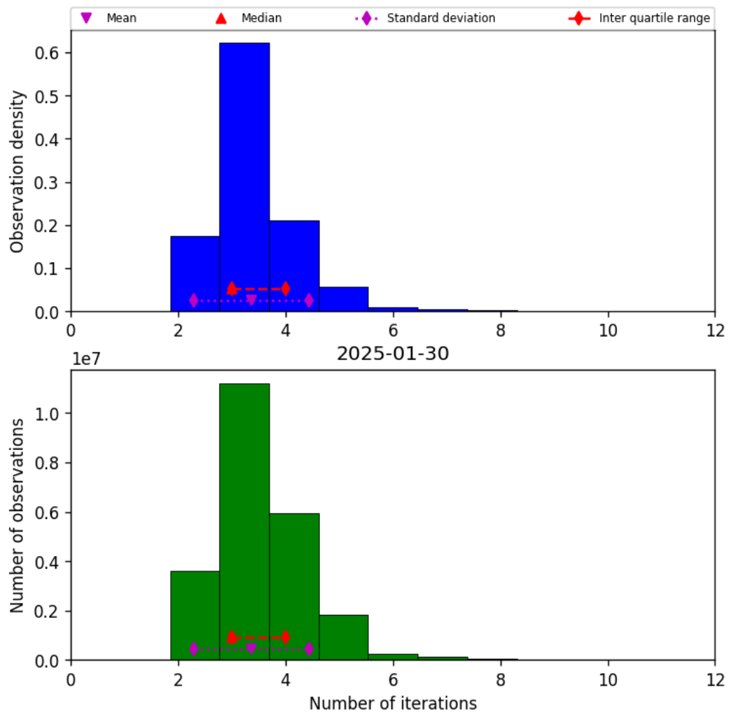
Figure 37: Histogram of “Number of iterations” for 2025-01-30 to 2025-01-31
