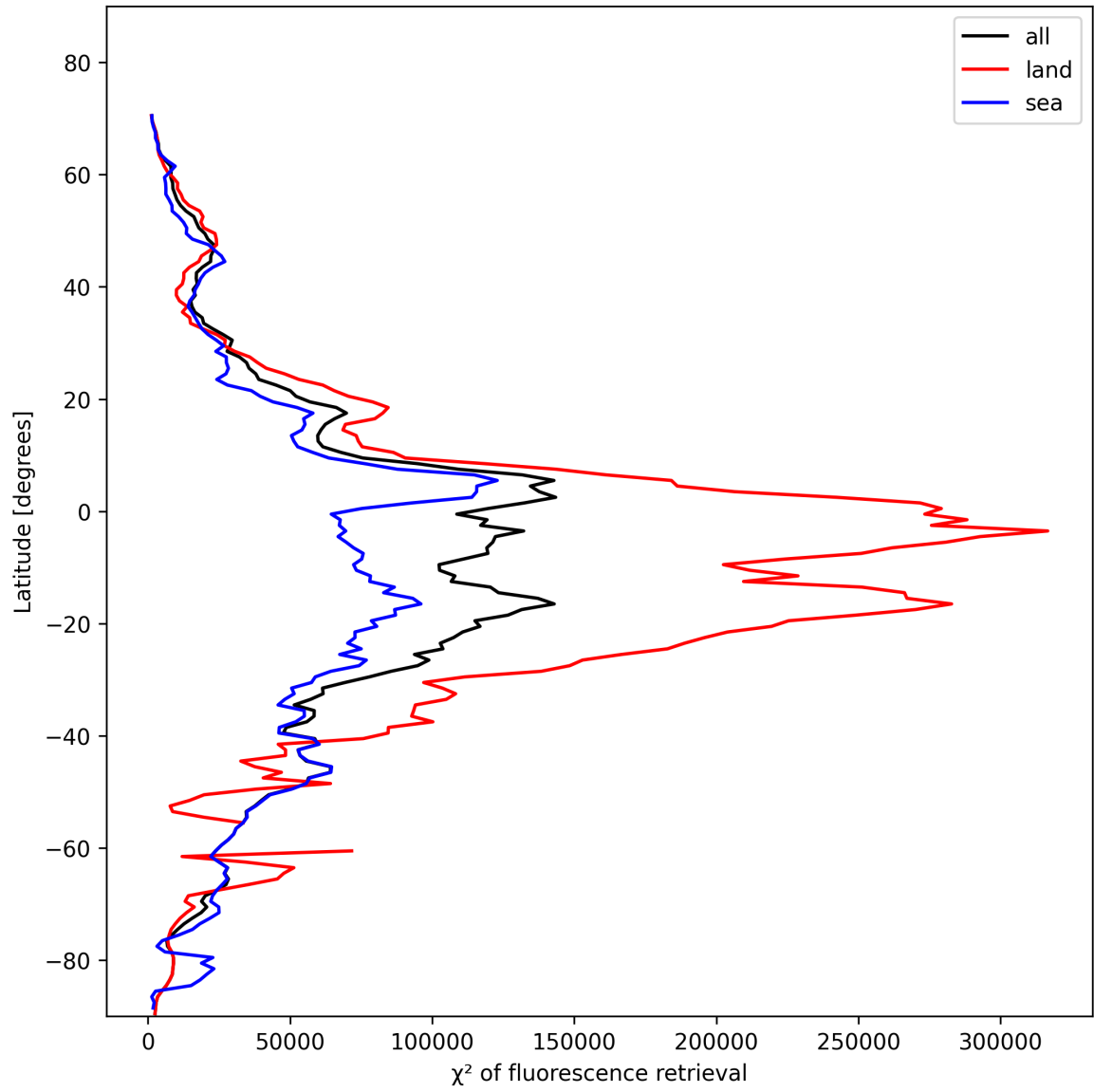
Figure 23: Zonal average of “ \chi^2 of fluorescence retrieval” for 2025-01-30 to 2025-01-31.
