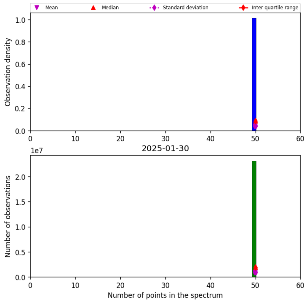
Figure 42: Histogram of "Number of points in the spectrum" for 2025-01-30 to 2025-01-31
