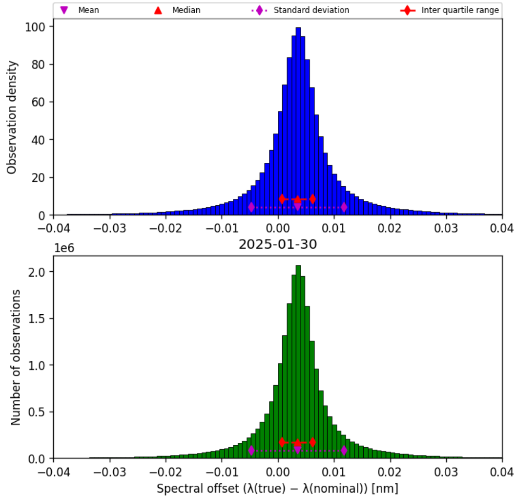
Figure 43: Histogram of “Spectral offset ( \lambda_{\text{true}} - \lambda_{\text{nominal}} )” for 2025-01-30 to 2025-01-31
