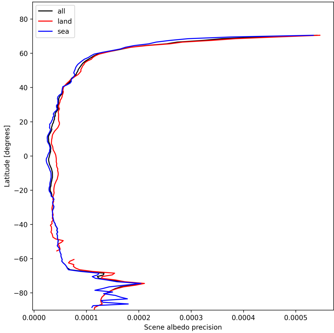
Figure 16: Zonal average of “Scene albedo precision” for 2025-01-30 to 2025-01-31.
