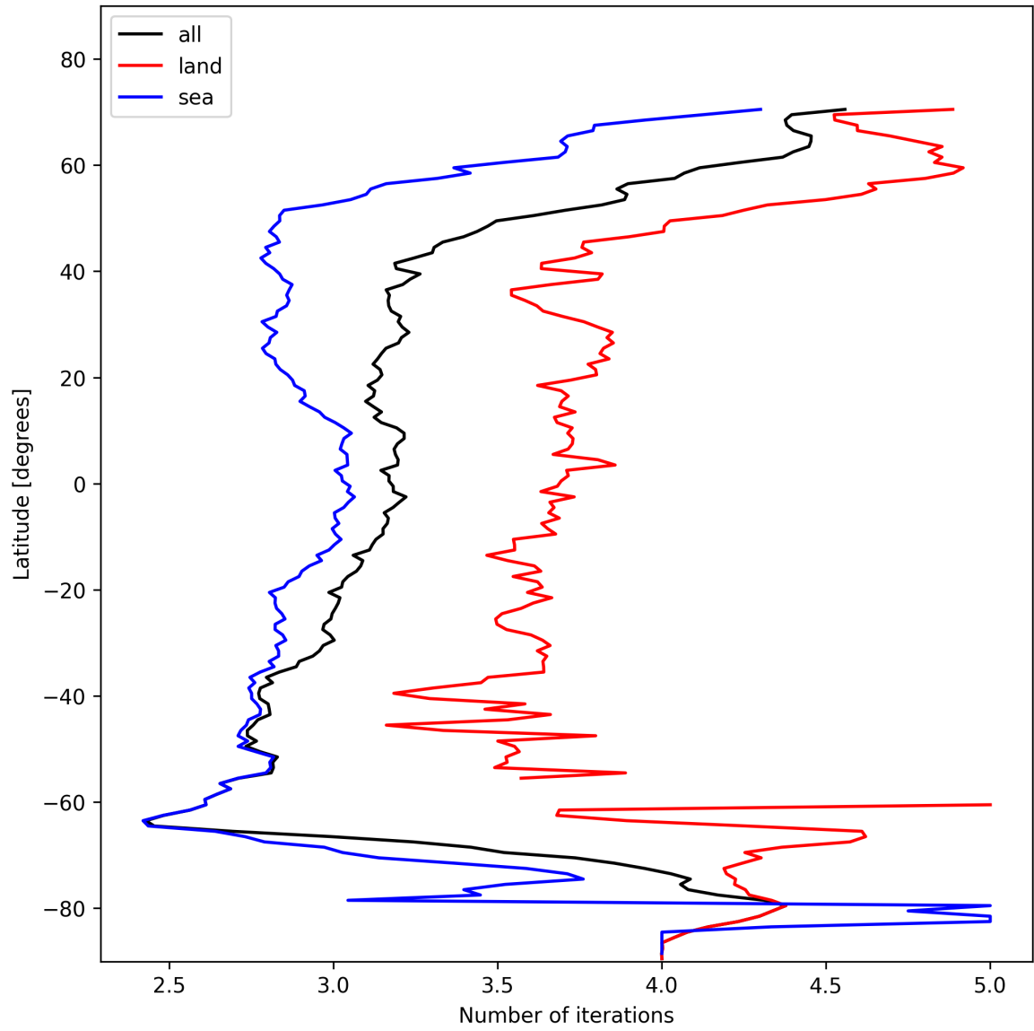
Figure 20: Zonal average of “Number of iterations” for 2025-01-30 to 2025-01-31.
