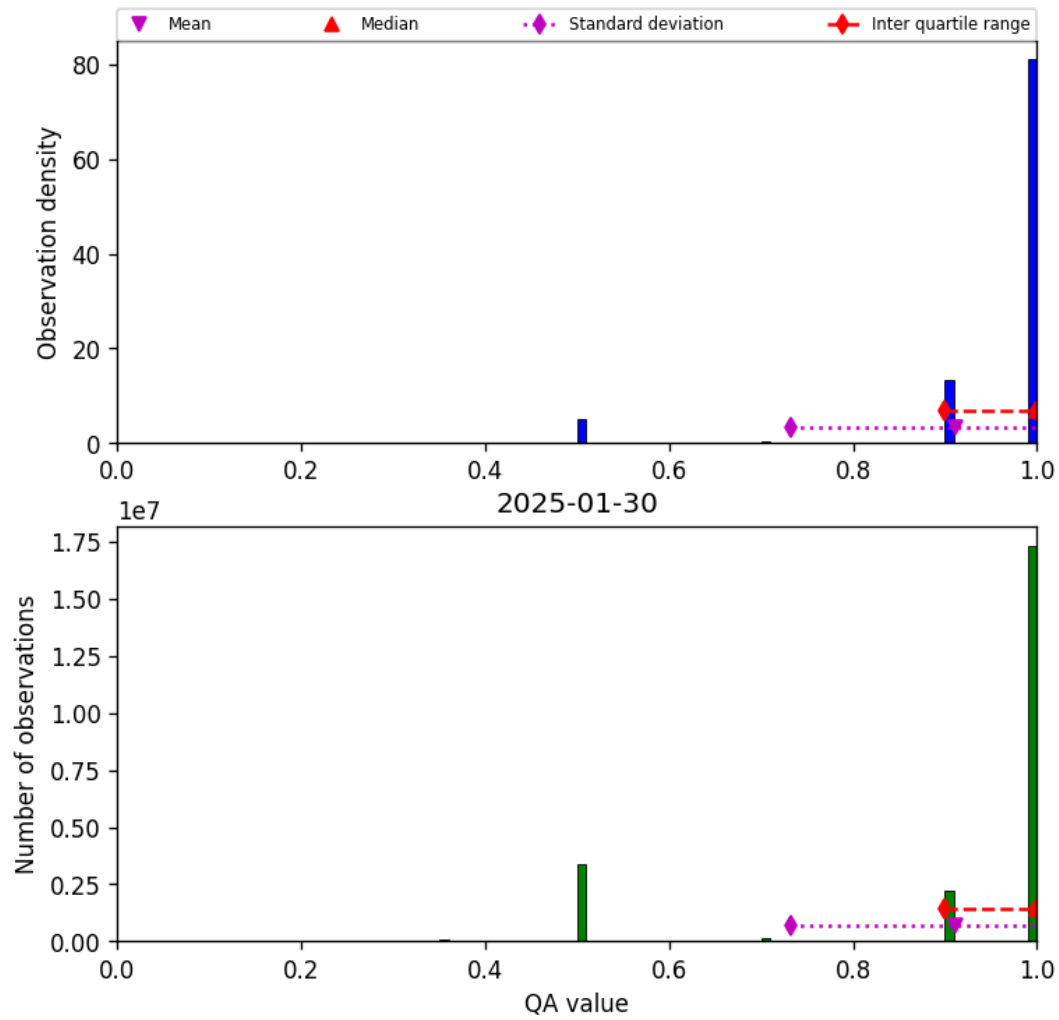
Figure 27: Histogram of “QA value” for 2025-01-30 to 2025-01-31
