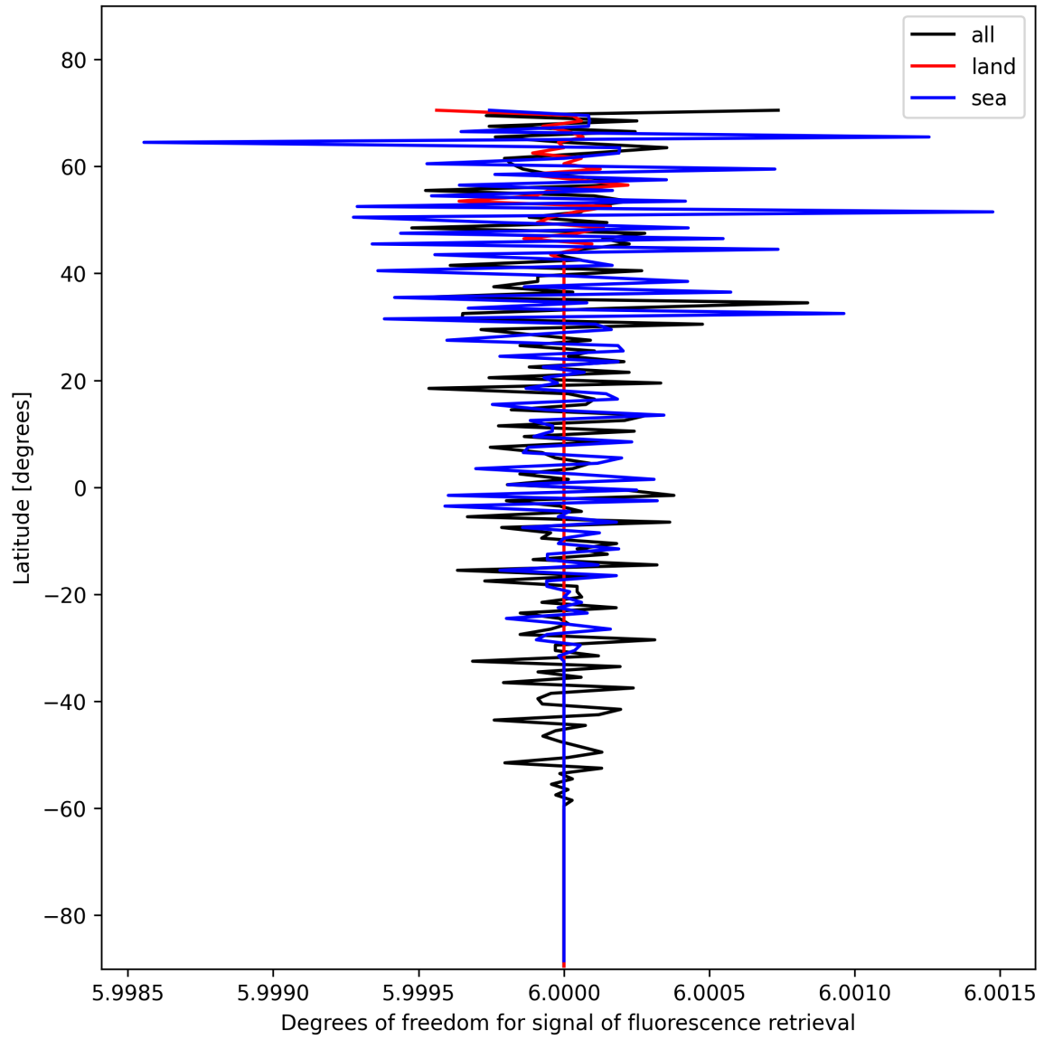
Figure 24: Zonal average of “Degrees of freedom for signal of fluorescence retrieval” for 2025-01-30 to 2025-01-31.
