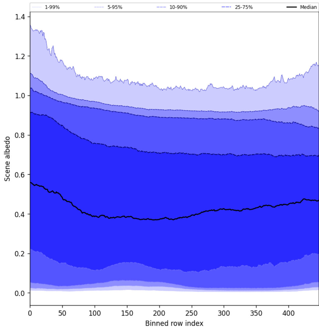
Figure 49: Along track statistics of “Scene albedo” for 2025-01-30 to 2025-01-31
