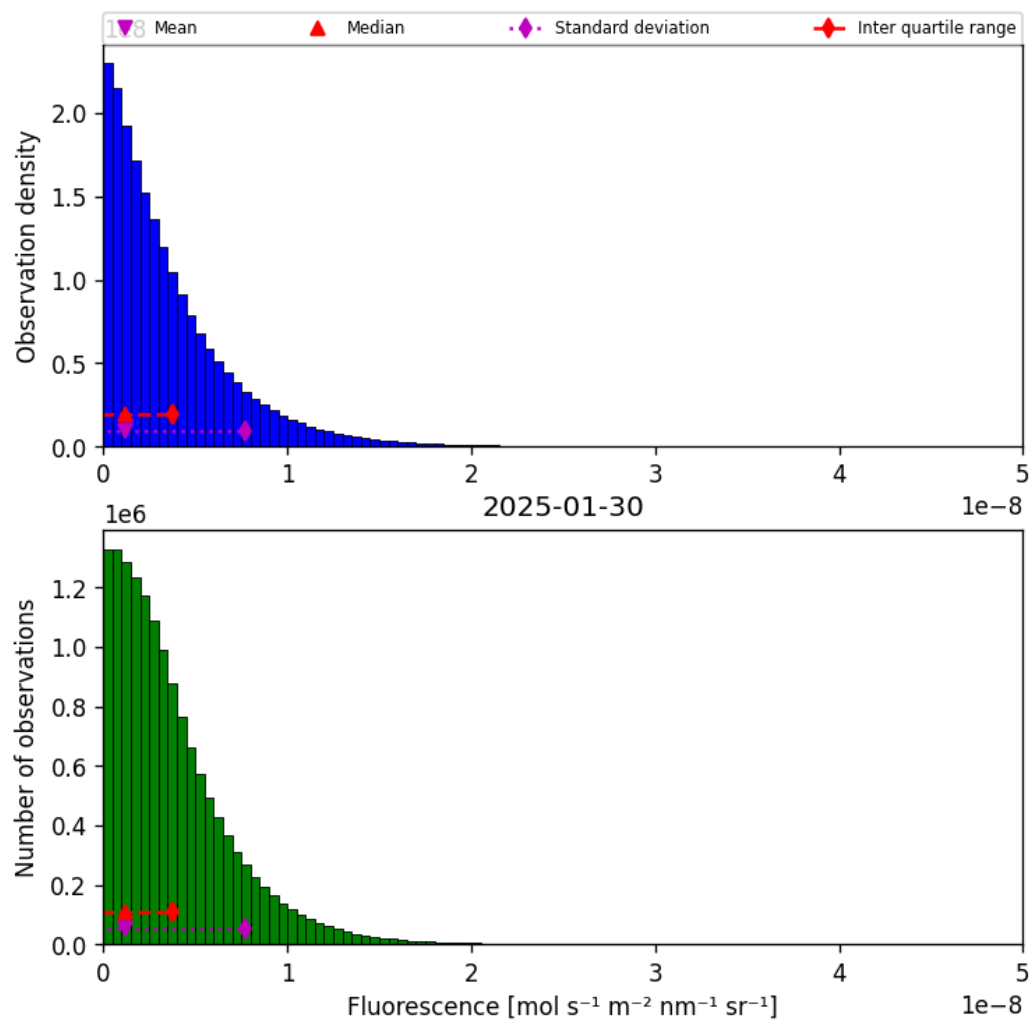
Figure 38: Histogram of “Fluorescence” for 2025-01-30 to 2025-01-31
