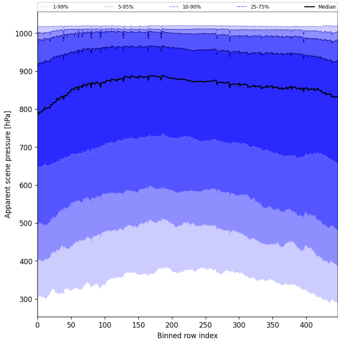
Figure 51: Along track statistics of “Apparent scene pressure” for 2025-01-30 to 2025-01-31
