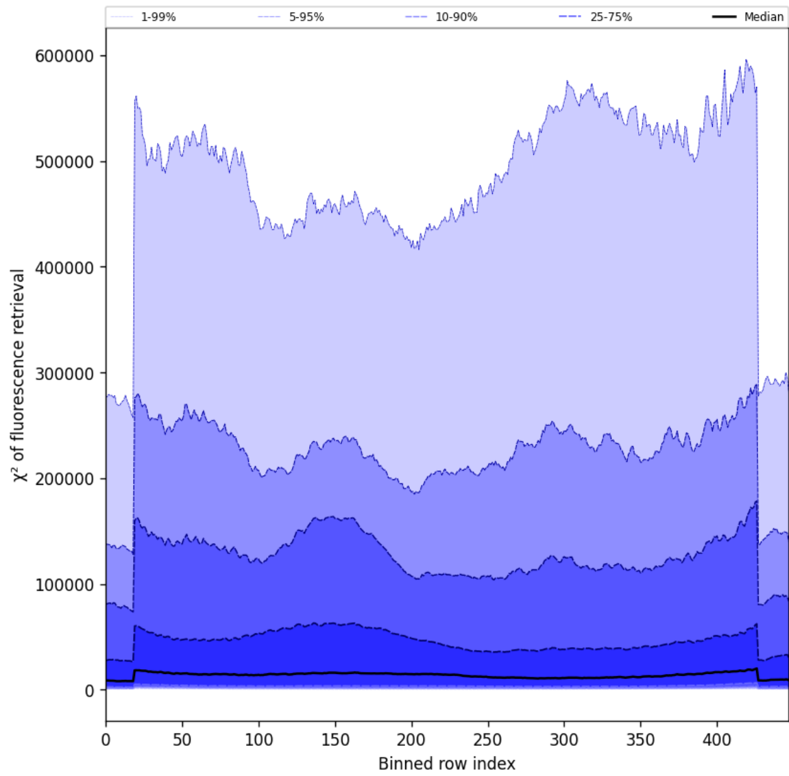
Figure 57: Along track statistics of “ \chi^2 of fluorescence retrieval” for 2025-01-30 to 2025-01-31
