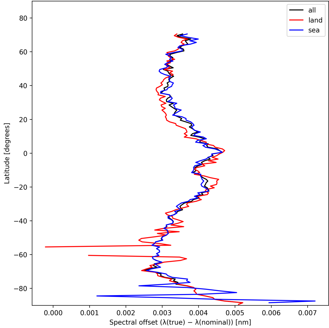
Figure 26: Zonal average of “Spectral offset ( \lambda_{\text{true}} - \lambda_{\text{nominal}} )” for 2025-01-30 to 2025-01-31.
