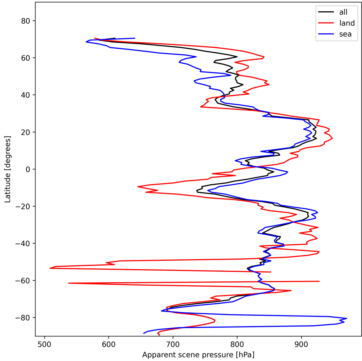
Figure 17: Zonal average of “Apparent scene pressure” for 2025-01-30 to 2025-01-31.
