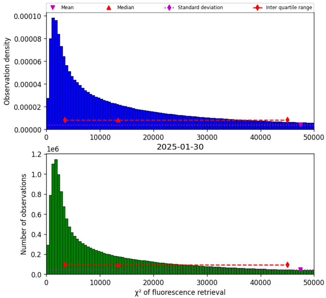
Figure 40: Histogram of “ \chi^2 of fluorescence retrieval” for 2025-01-30 to 2025-01-31
