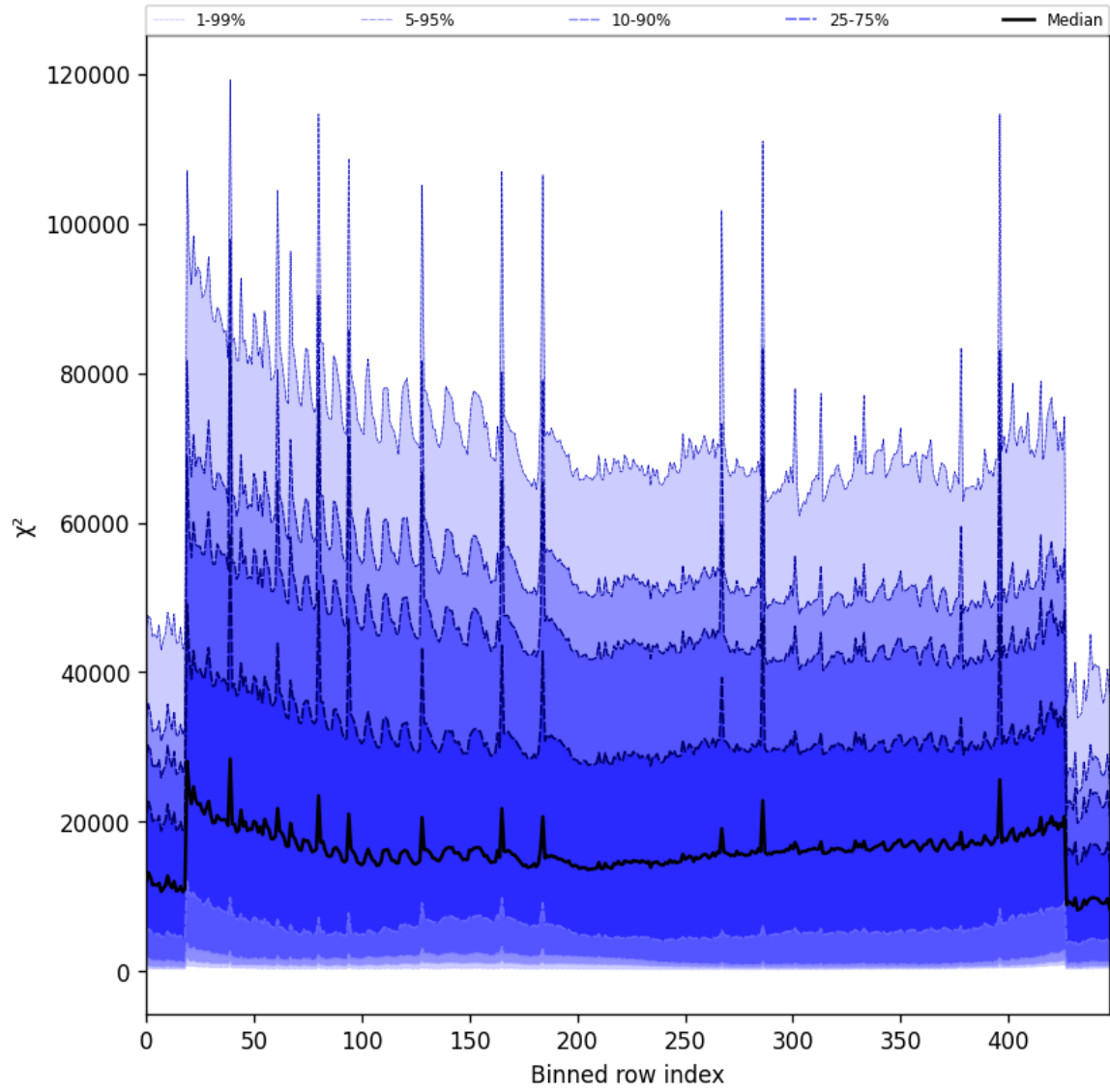
Figure 53: Along track statistics of “ \chi^2 ” for 2025-01-30 to 2025-01-31
