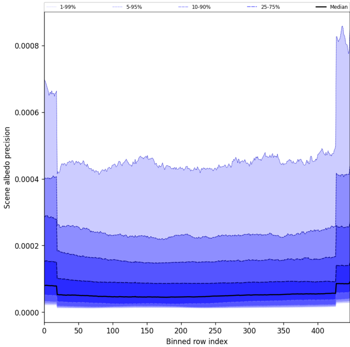
Figure 50: Along track statistics of “Scene albedo precision” for 2025-01-30 to 2025-01-31
