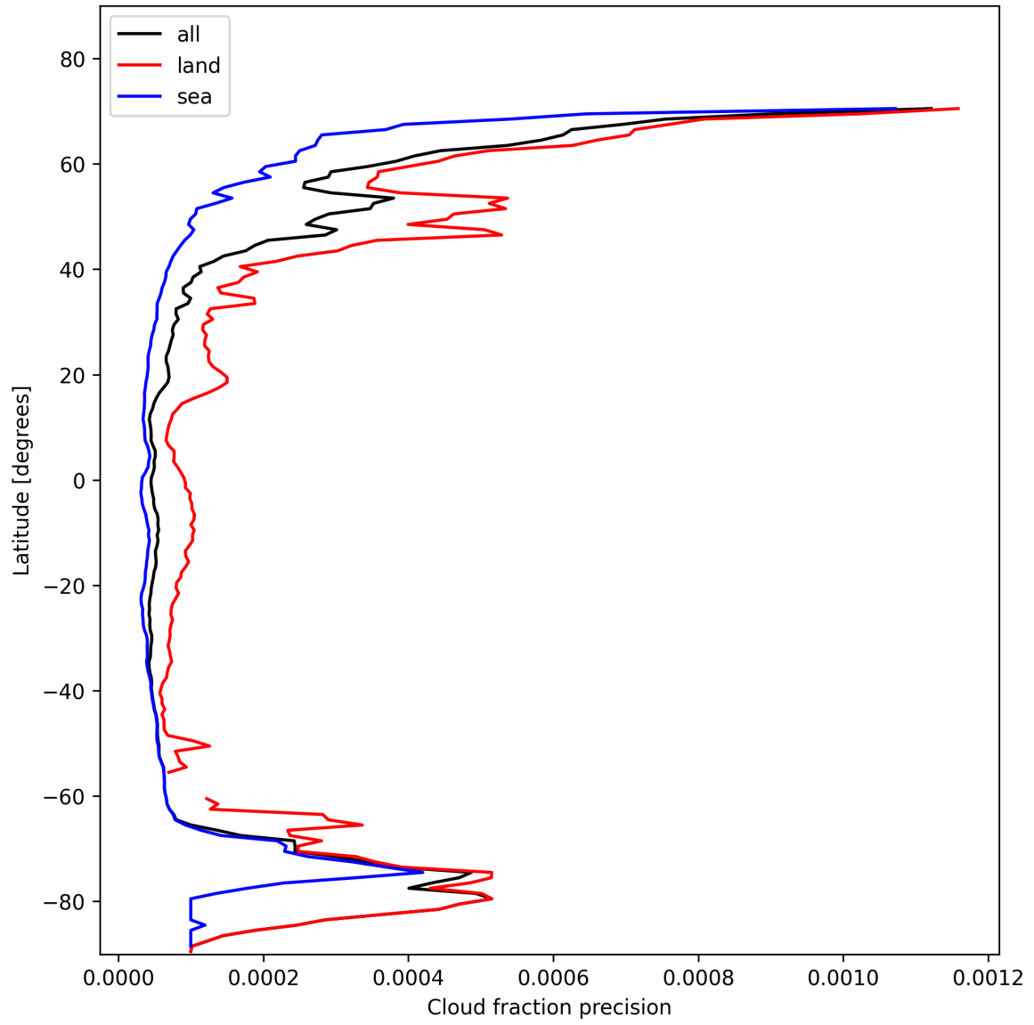
Figure 14: Zonal average of “Cloud fraction precision” for 2025-01-30 to 2025-01-31.
