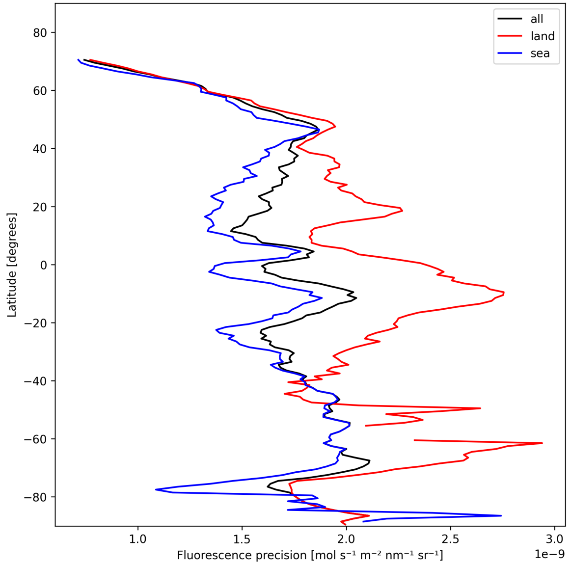
Figure 22: Zonal average of “Fluorescence precision” for 2025-01-30 to 2025-01-31.
