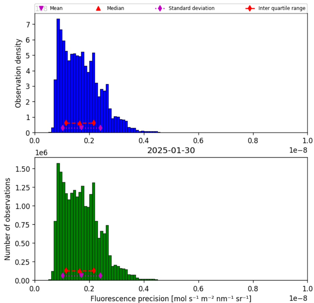
Figure 39: Histogram of “Fluorescence precision” for 2025-01-30 to 2025-01-31
