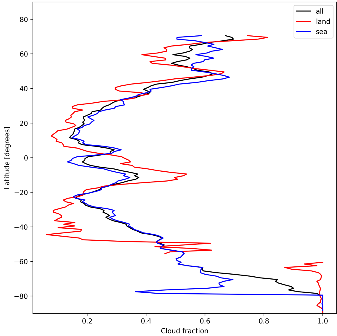
Figure 13: Zonal average of “Cloud fraction” for 2025-01-30 to 2025-01-31.
