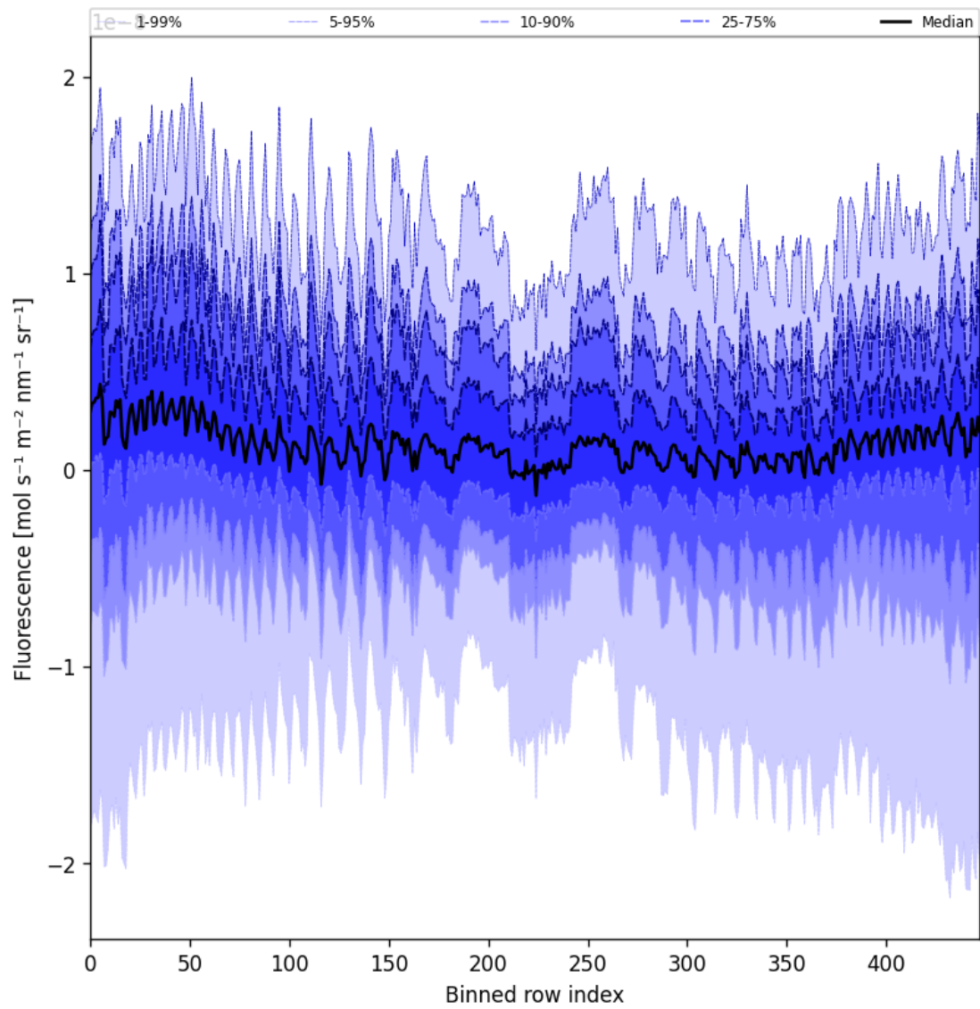
Figure 55: Along track statistics of “Fluorescence” for 2025-01-30 to 2025-01-31
