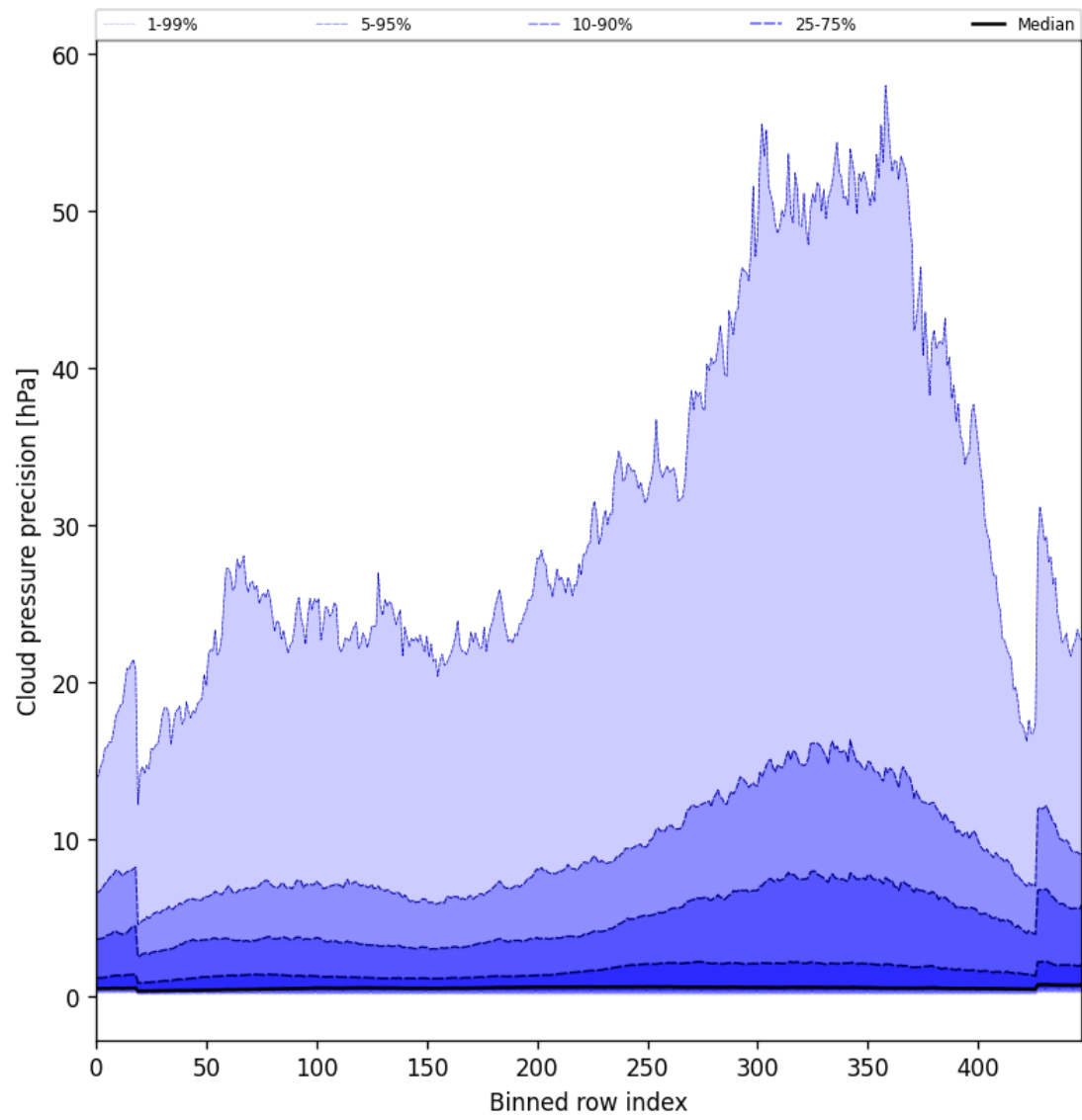
Figure 46: Along track statistics of “Cloud pressure precision” for 2025-01-30 to 2025-01-31
