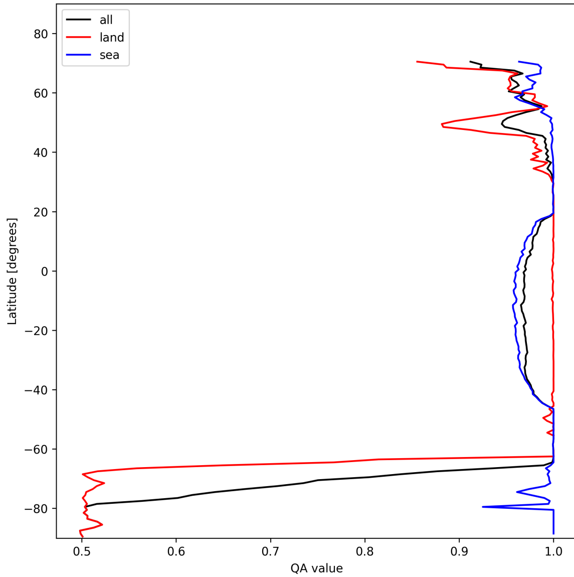
Figure 10: Zonal average of “QA value” for 2025-01-30 to 2025-01-31.
