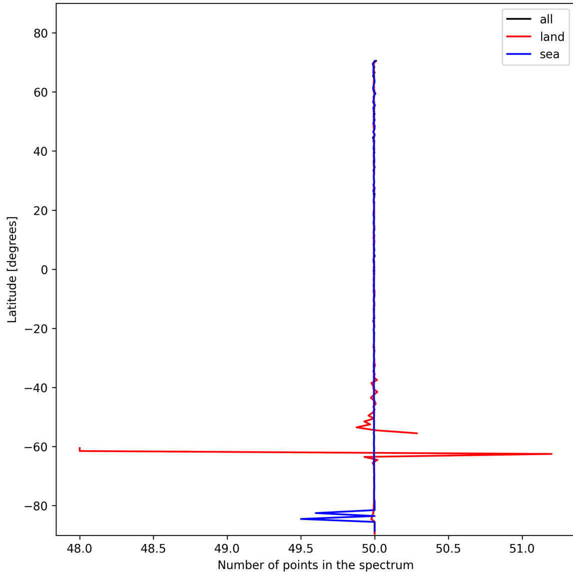
Figure 25: Zonal average of “Number of points in the spectrum” for 2025-01-30 to 2025-01-31.
