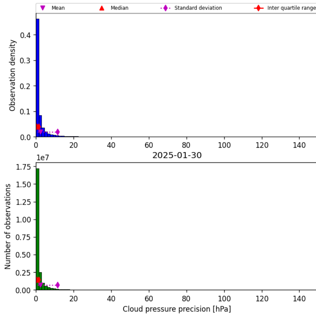
Figure 29: Histogram of “Cloud pressure precision” for 2025-01-30 to 2025-01-31
