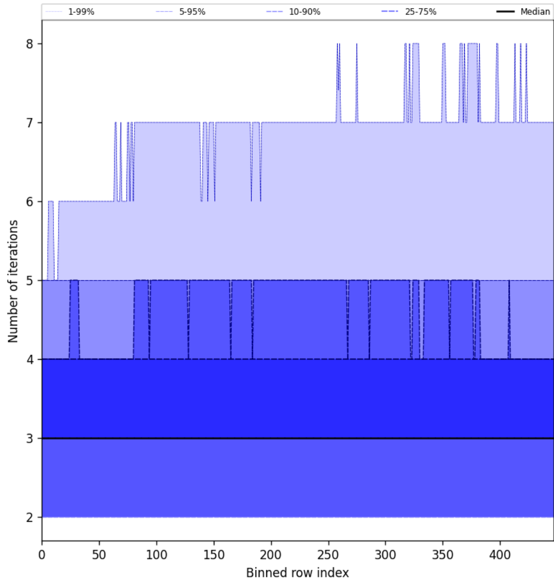
Figure 54: Along track statistics of “Number of iterations” for 2025-01-30 to 2025-01-31
