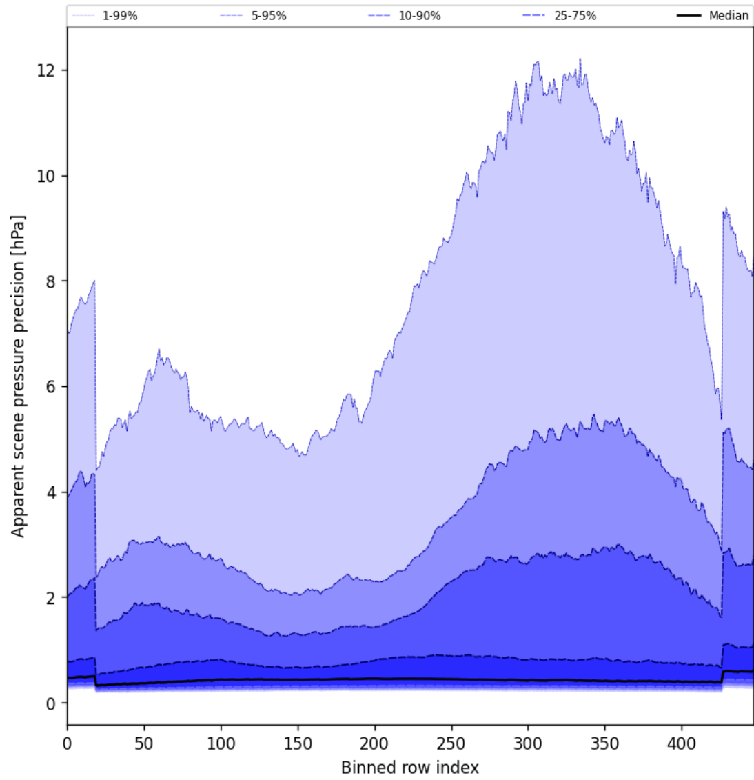
Figure 52: Along track statistics of “Apparent scene pressure precision” for 2025-01-30 to 2025-01-31
