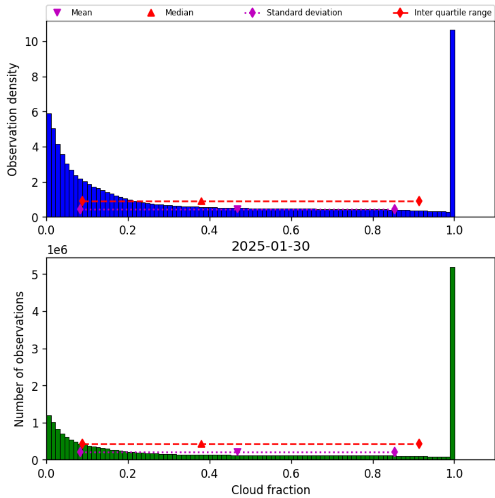
Figure 30: Histogram of “Cloud fraction” for 2025-01-30 to 2025-01-31
