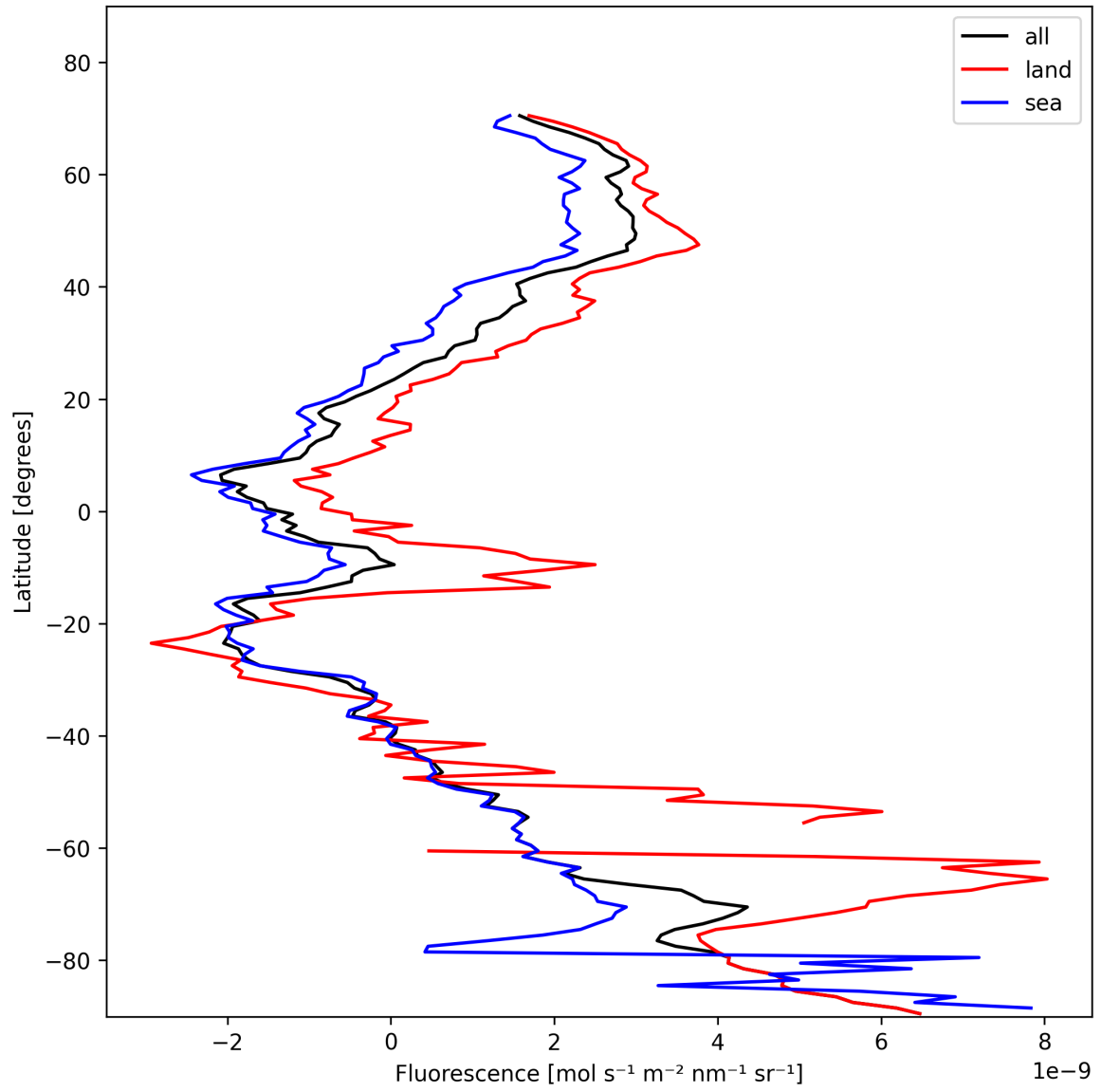
Figure 21: Zonal average of “Fluorescence” for 2025-01-30 to 2025-01-31.
