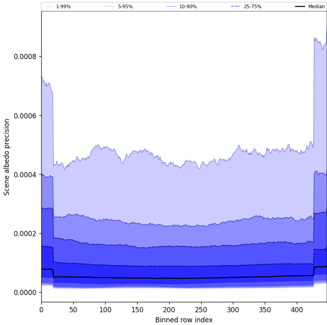
Figure 50: Along track statistics of “Scene albedo precision” for 2025-01-31 to 2025-01-31
