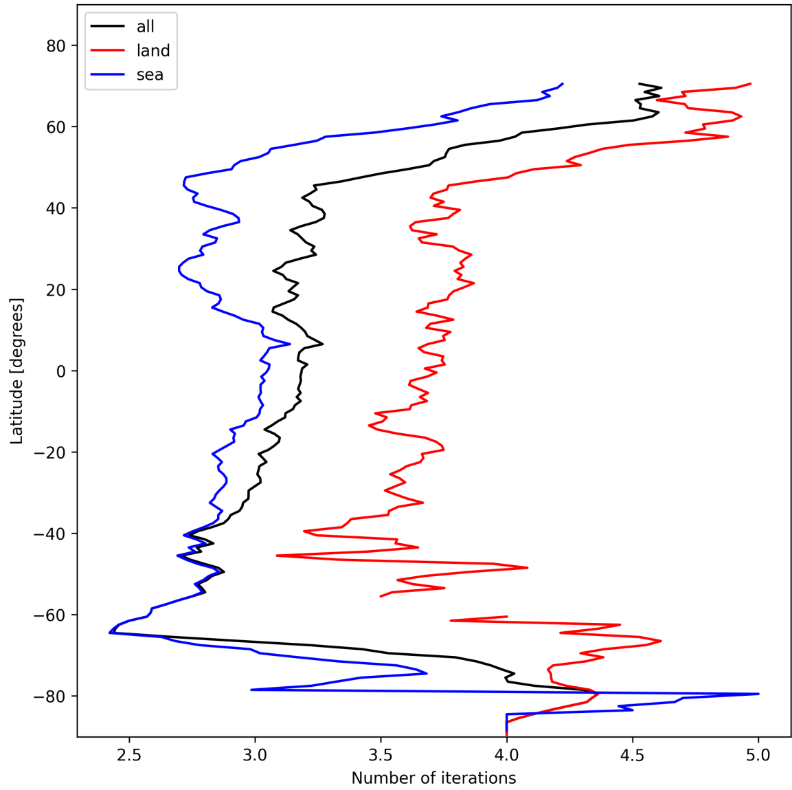
Figure 20: Zonal average of “Number of iterations” for 2025-01-31 to 2025-01-31.
