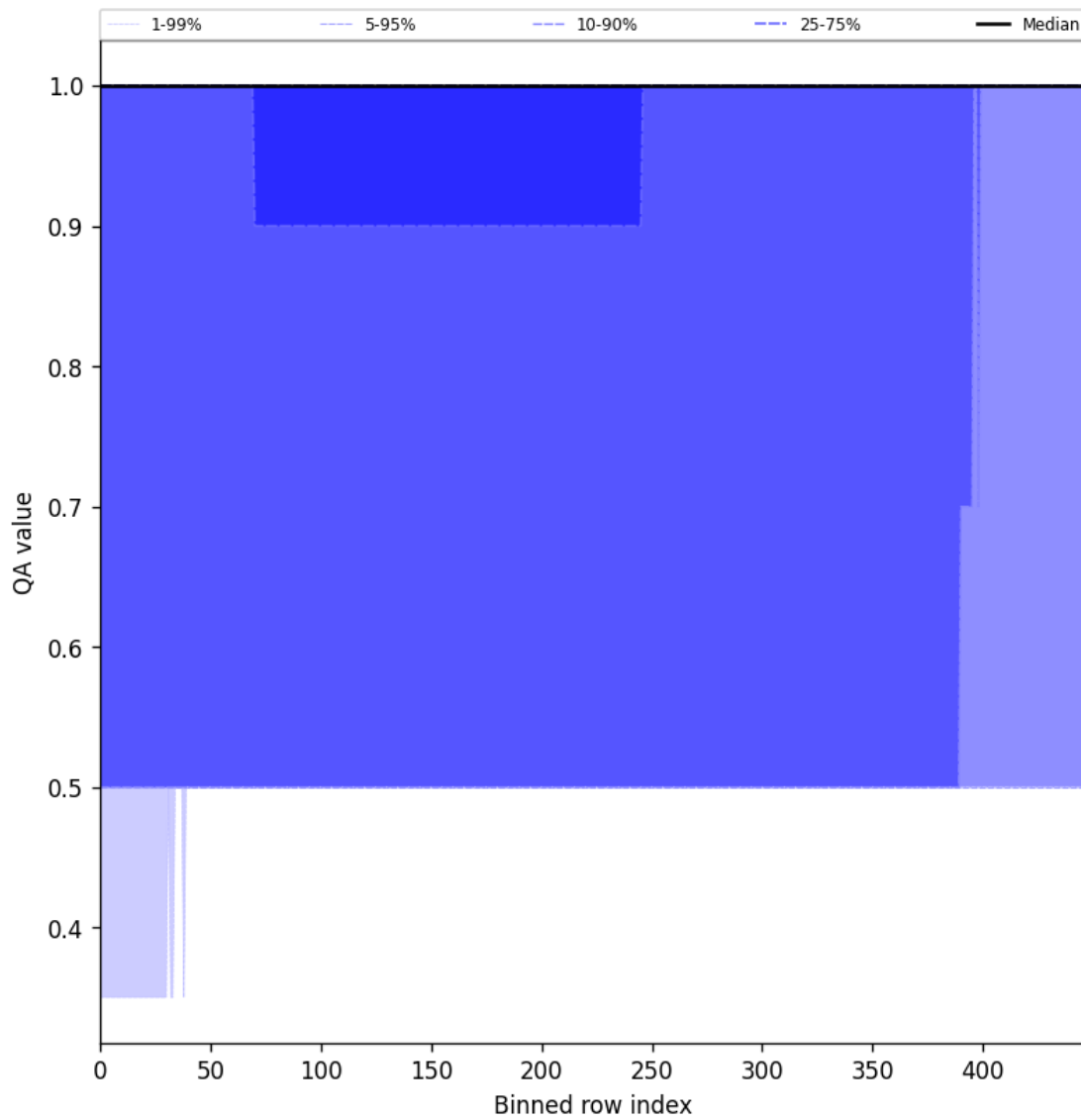
Figure 44: Along track statistics of “QA value” for 2025-01-31 to 2025-01-31
