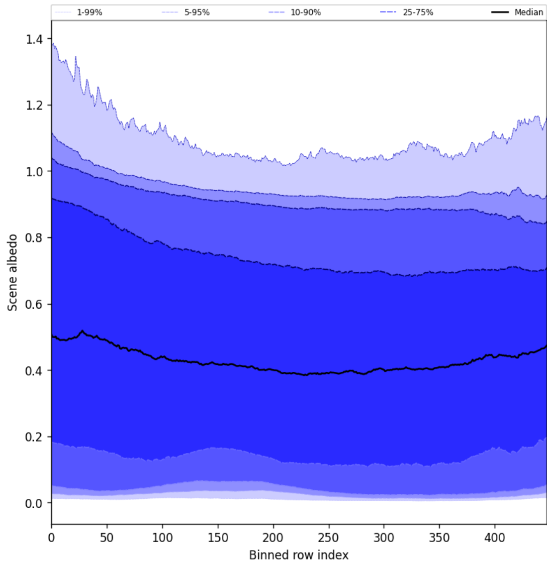
Figure 49: Along track statistics of “Scene albedo” for 2025-01-31 to 2025-01-31
