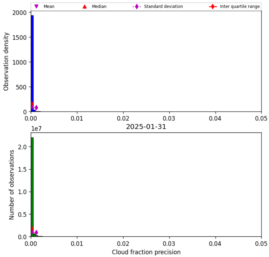
Figure 31: Histogram of “Cloud fraction precision” for 2025-01-31 to 2025-01-31
