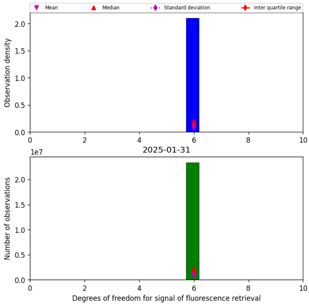
Figure 41: Histogram of “Degrees of freedom for signal of fluorescence retrieval” for 2025-01-31 to 2025-01-31
