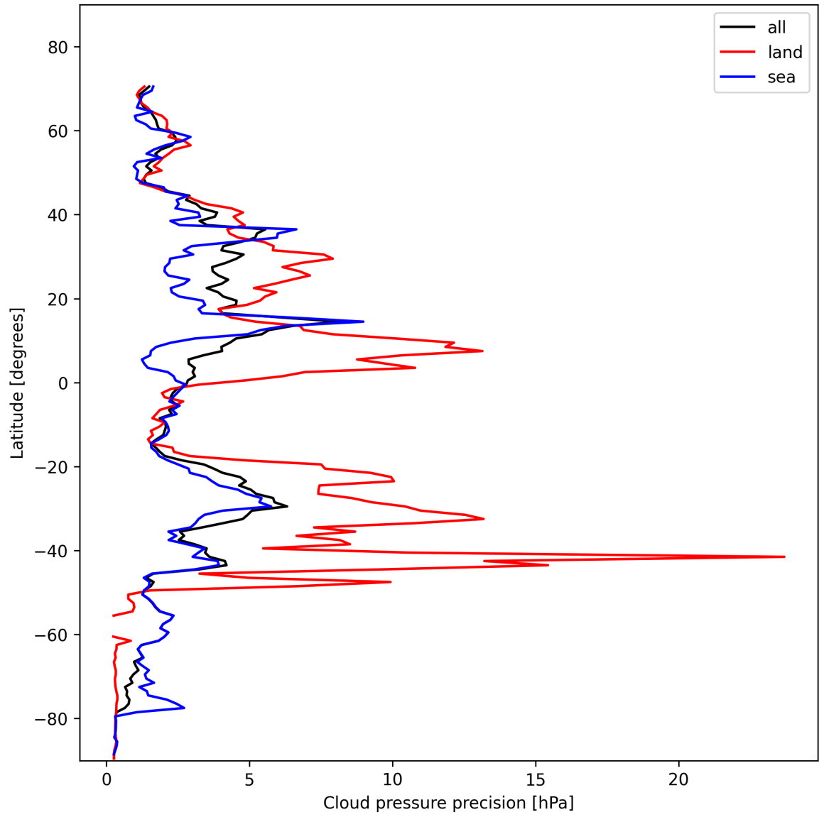
Figure 12: Zonal average of “Cloud pressure precision” for 2025-01-31 to 2025-01-31.
