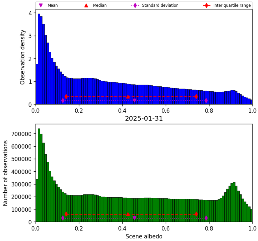
Figure 32: Histogram of “Scene albedo” for 2025-01-31 to 2025-01-31
