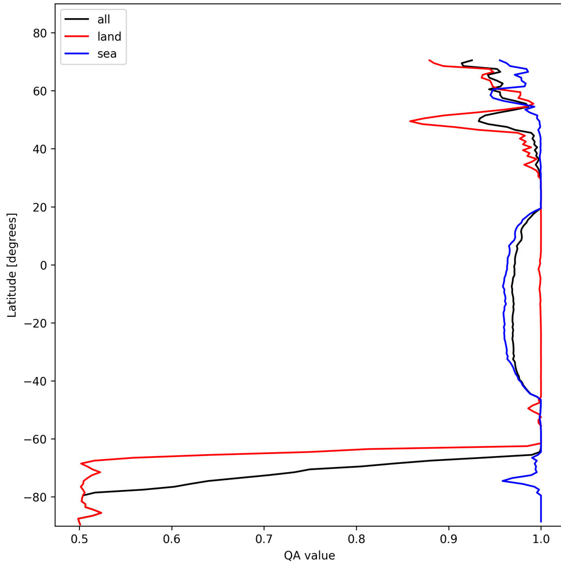
Figure 10: Zonal average of “QA value” for 2025-01-31 to 2025-01-31.
