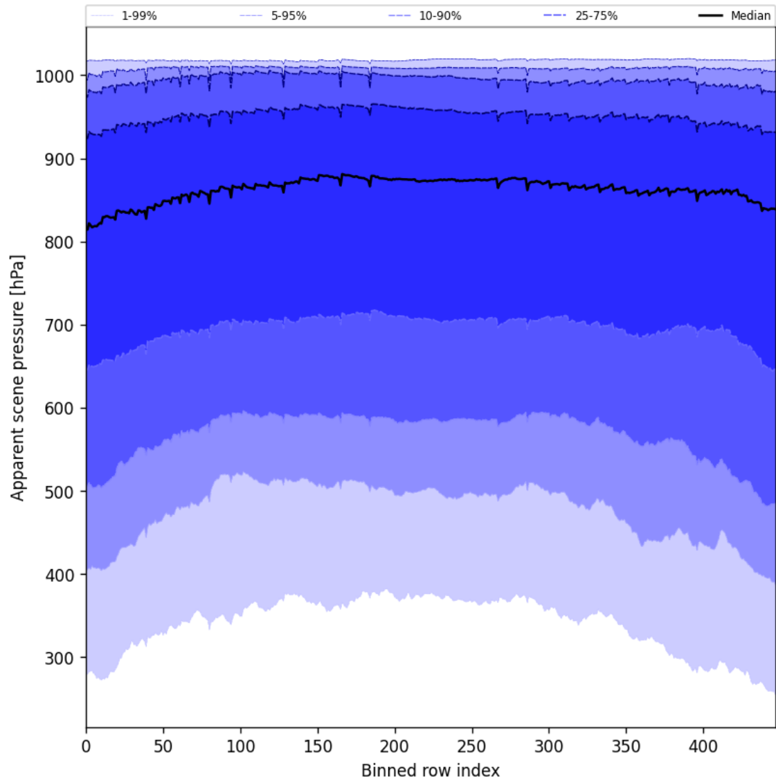
Figure 51: Along track statistics of “Apparent scene pressure” for 2025-01-31 to 2025-01-31
