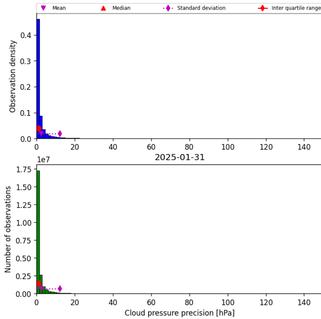
Figure 29: Histogram of “Cloud pressure precision” for 2025-01-31 to 2025-01-31
