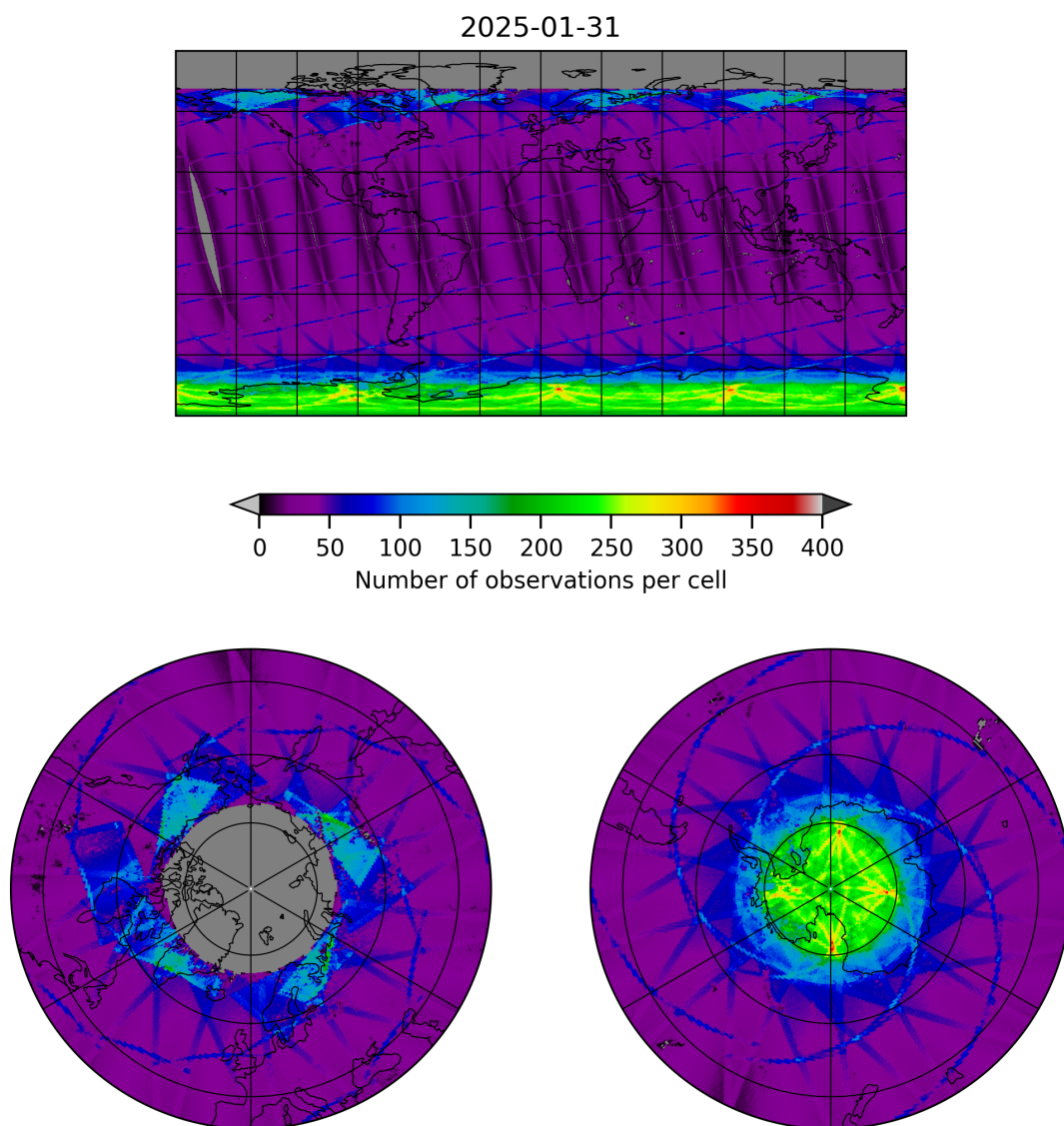
Figure 9: Map of the number of observations for 2025-01-31 to 2025-01-31
