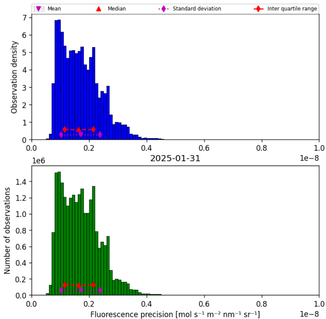
Figure 39: Histogram of “Fluorescence precision” for 2025-01-31 to 2025-01-31
