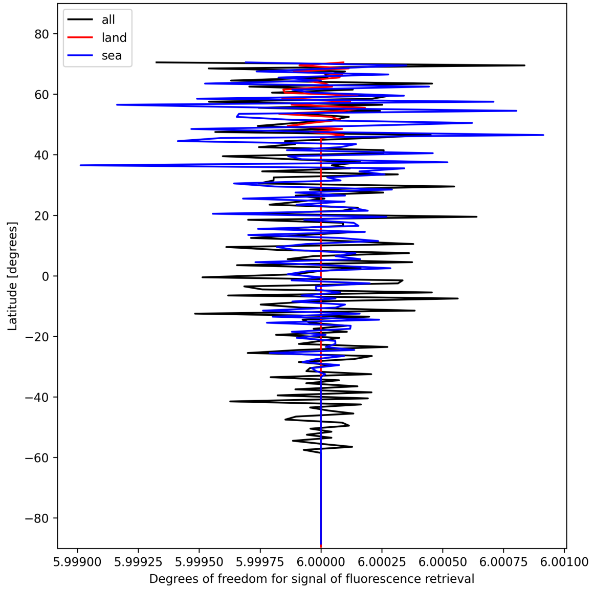
Figure 24: Zonal average of “Degrees of freedom for signal of fluorescence retrieval” for 2025-01-31 to 2025-01-31.
