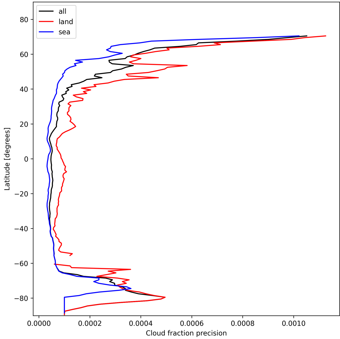
Figure 14: Zonal average of “Cloud fraction precision” for 2025-01-31 to 2025-01-31.
