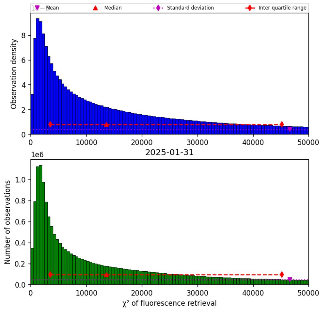
Figure 40: Histogram of “ \chi^2 of fluorescence retrieval” for 2025-01-31 to 2025-01-31
