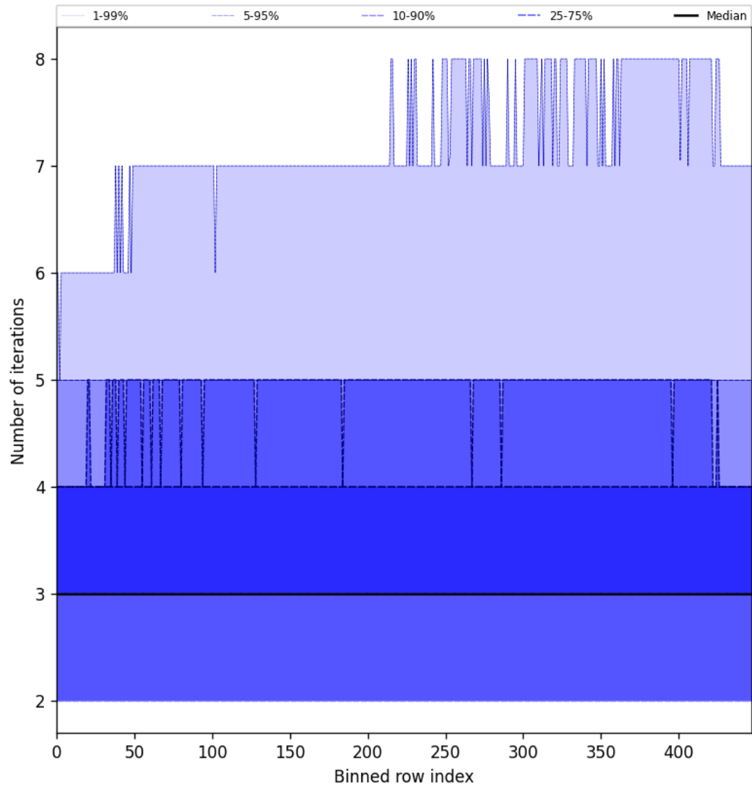
Figure 54: Along track statistics of “Number of iterations” for 2025-01-31 to 2025-01-31
