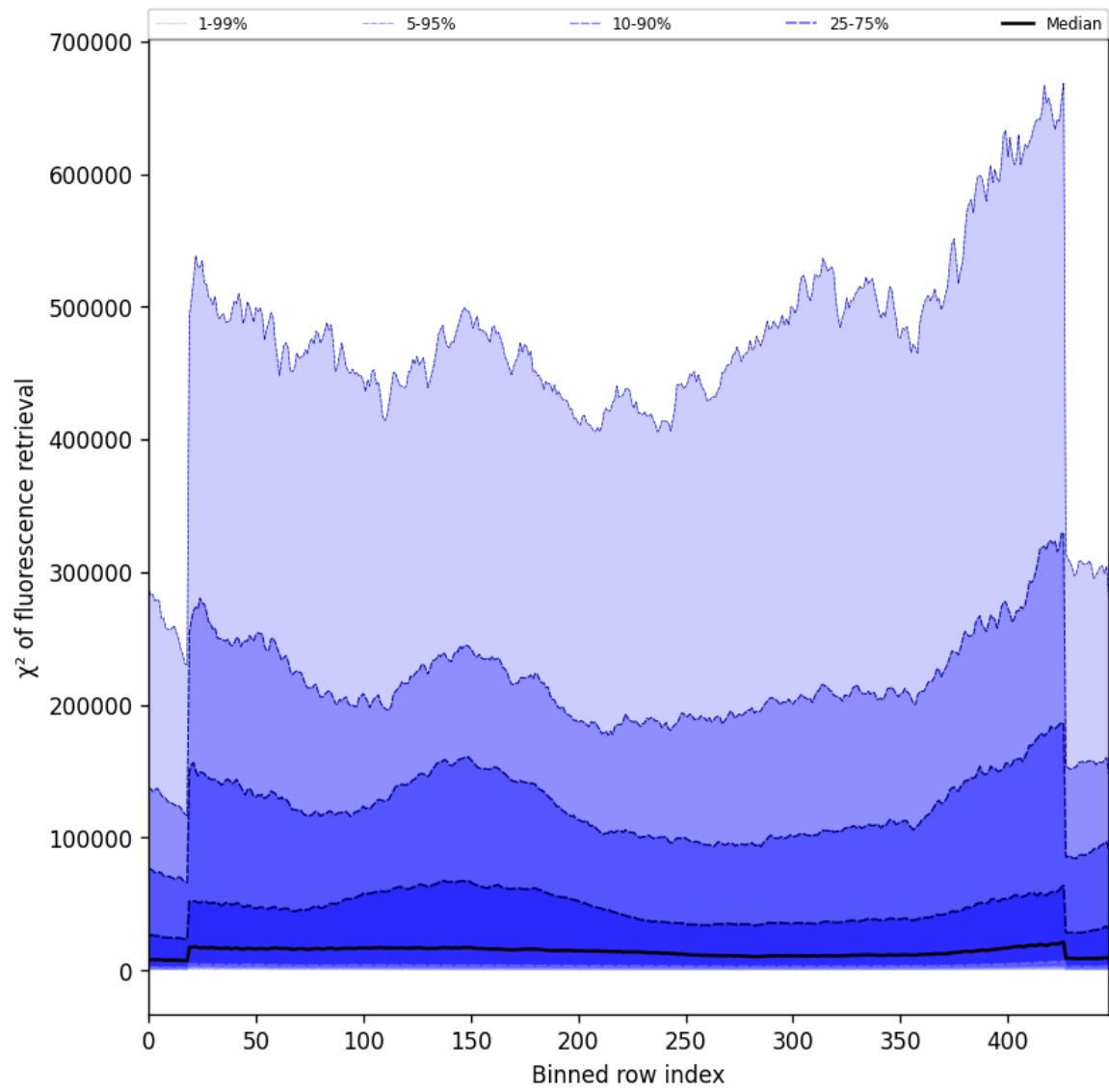
Figure 57: Along track statistics of “ \chi^2 of fluorescence retrieval” for 2025-01-31 to 2025-01-31
