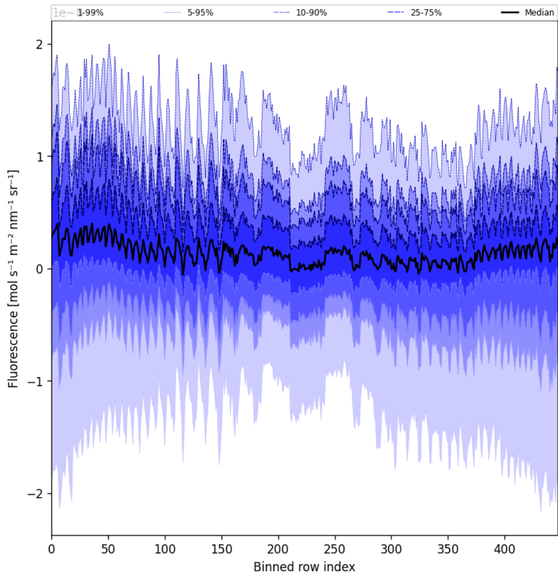
Figure 55: Along track statistics of “Fluorescence” for 2025-01-31 to 2025-01-31
