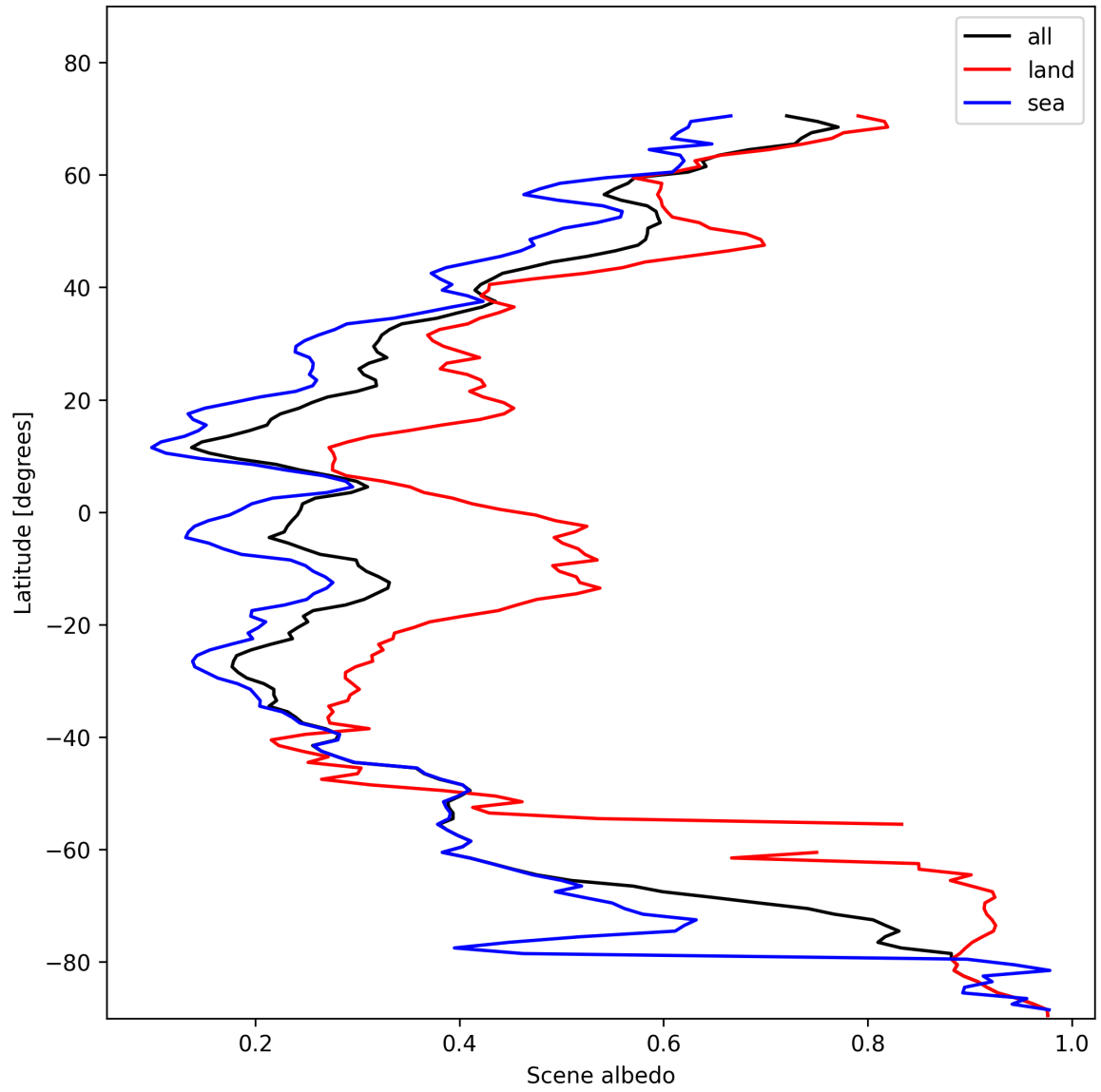
Figure 15: Zonal average of “Scene albedo” for 2025-01-31 to 2025-01-31.
