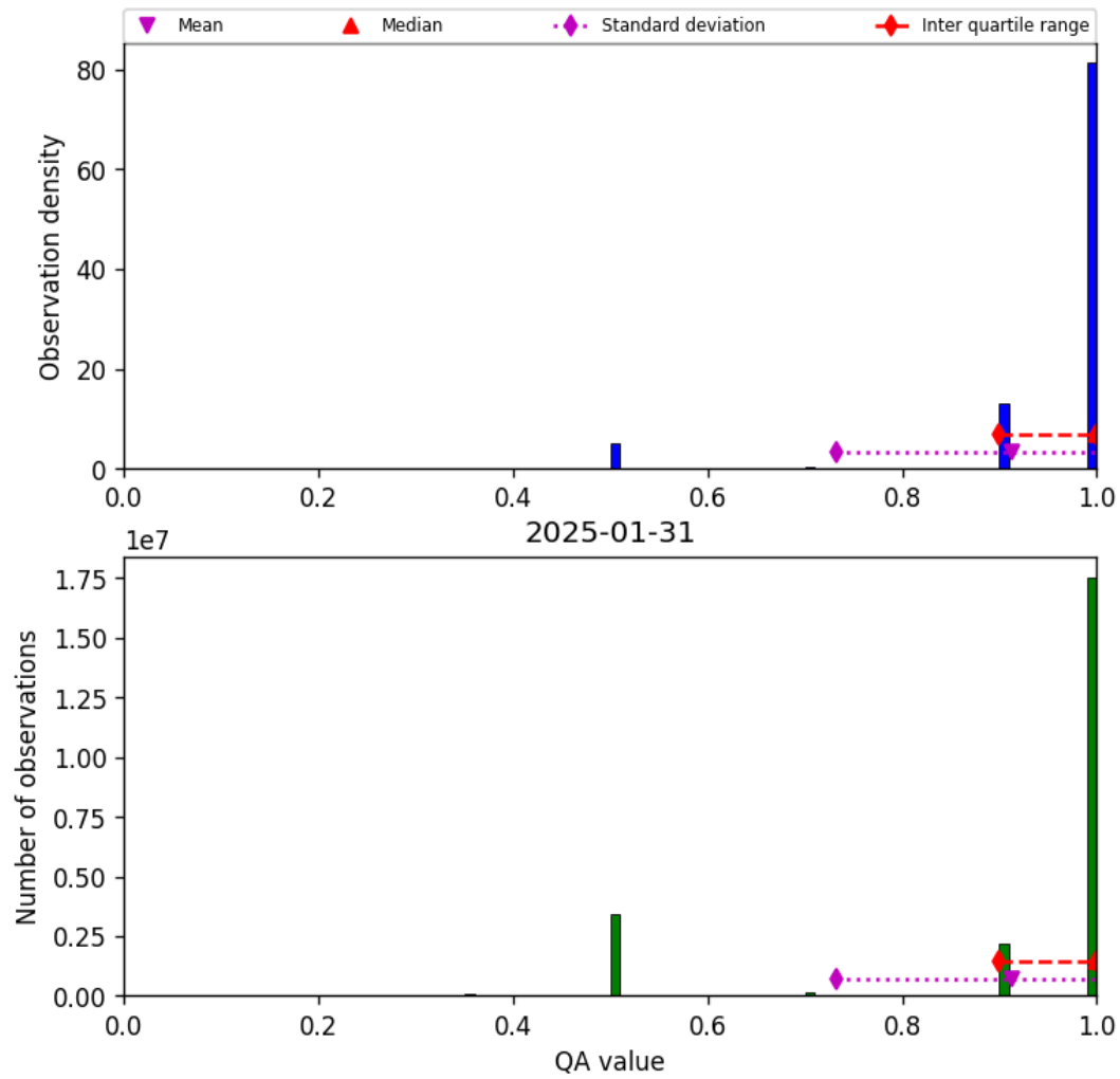
Figure 27: Histogram of “QA value” for 2025-01-31 to 2025-01-31
