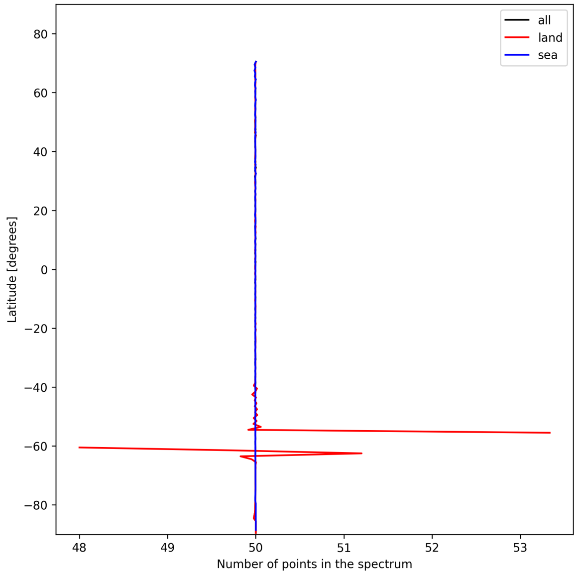
Figure 25: Zonal average of “Number of points in the spectrum” for 2025-01-31 to 2025-01-31.
