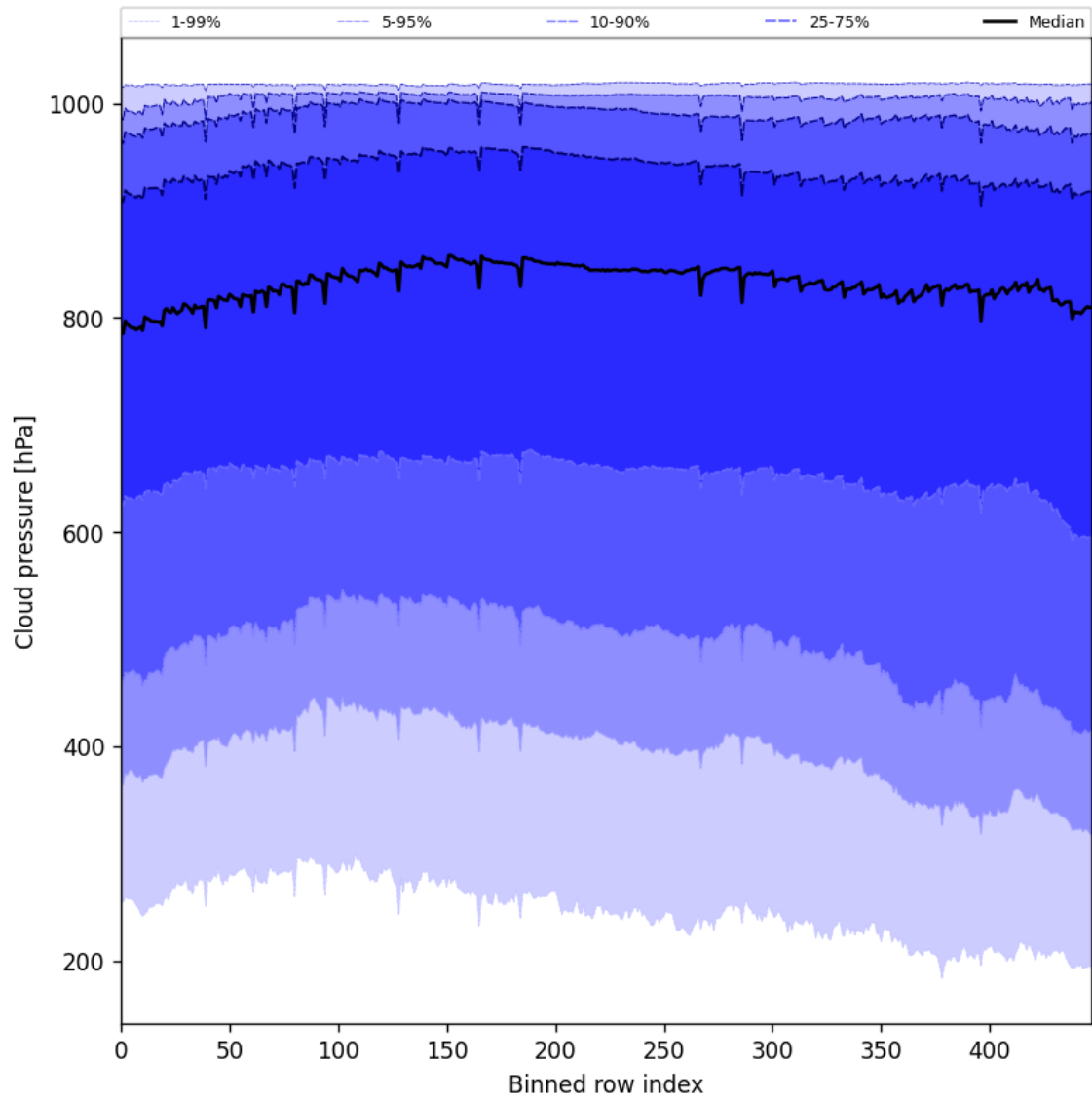
Figure 45: Along track statistics of “Cloud pressure” for 2025-01-31 to 2025-01-31
