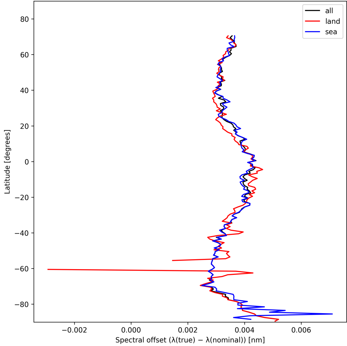
Figure 26: Zonal average of “Spectral offset ( \lambda_{\text{true}} - \lambda_{\text{nominal}} )” for 2025-01-31 to 2025-01-31.
