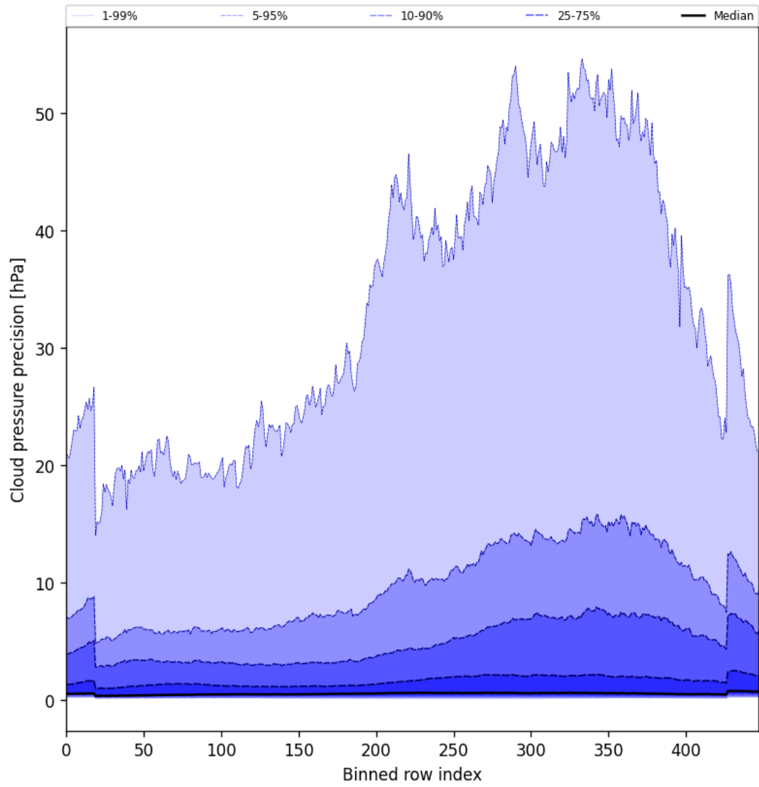
Figure 46: Along track statistics of “Cloud pressure precision” for 2025-01-31 to 2025-01-31
