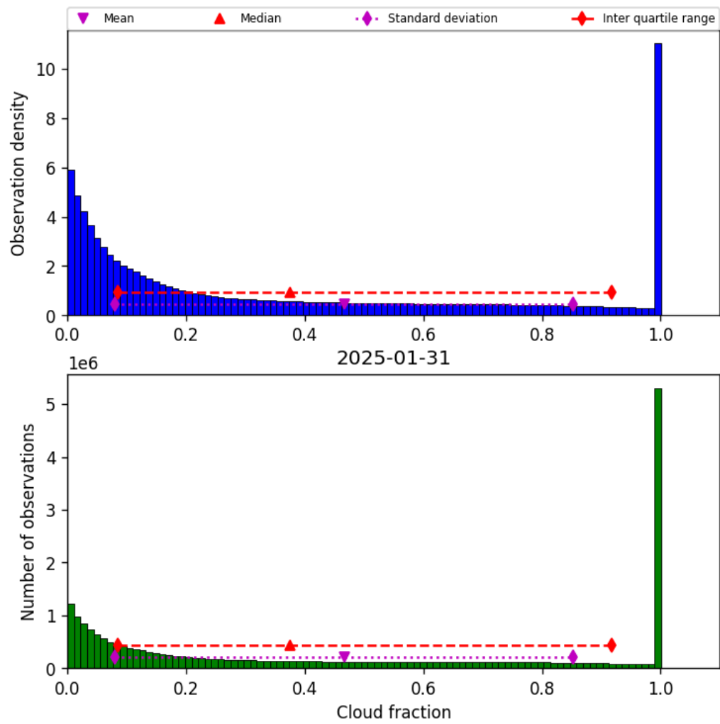
Figure 30: Histogram of “Cloud fraction” for 2025-01-31 to 2025-01-31
