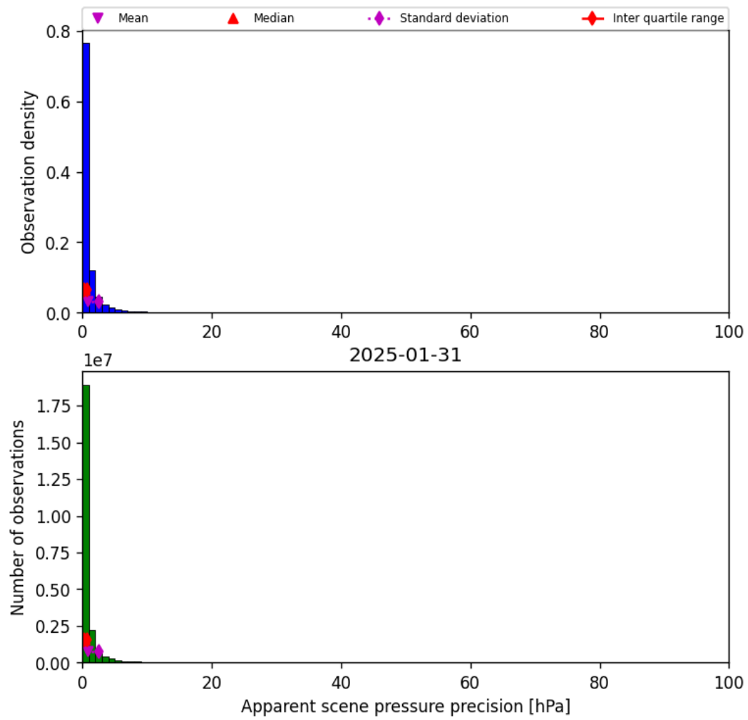
Figure 35: Histogram of “Apparent scene pressure precision” for 2025-01-31 to 2025-01-31
