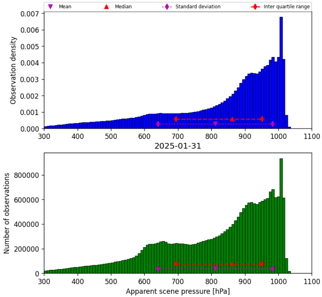
Figure 34: Histogram of “Apparent scene pressure” for 2025-01-31 to 2025-01-31
