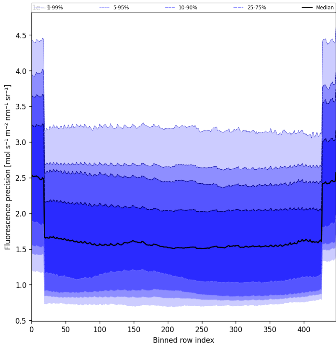
Figure 56: Along track statistics of “Fluorescence precision” for 2025-01-31 to 2025-01-31
