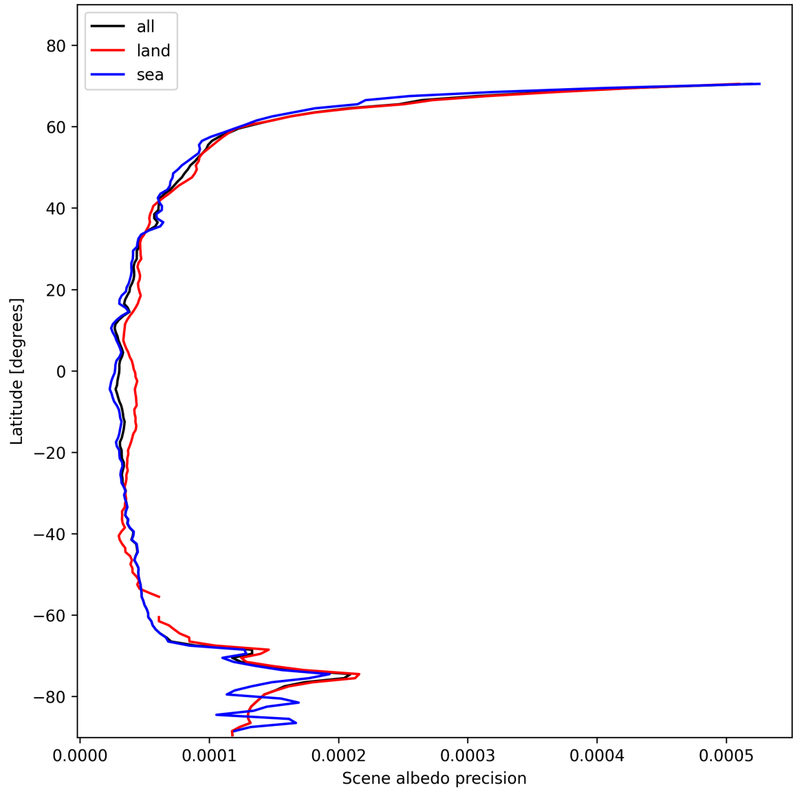
Figure 16: Zonal average of “Scene albedo precision” for 2025-01-31 to 2025-01-31.
