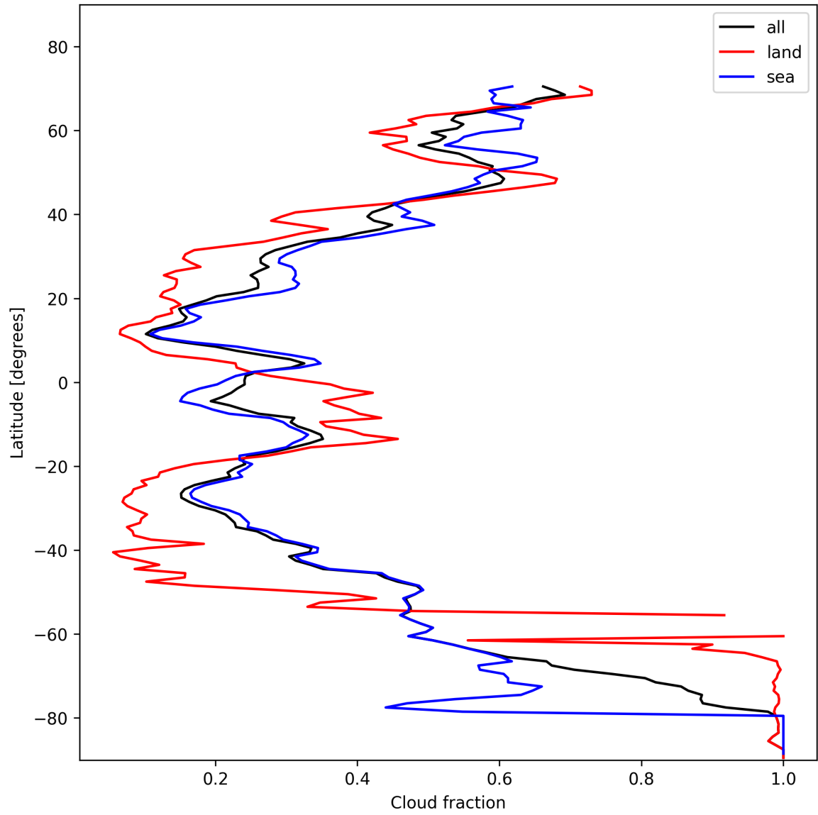
Figure 13: Zonal average of “Cloud fraction” for 2025-01-31 to 2025-01-31.
