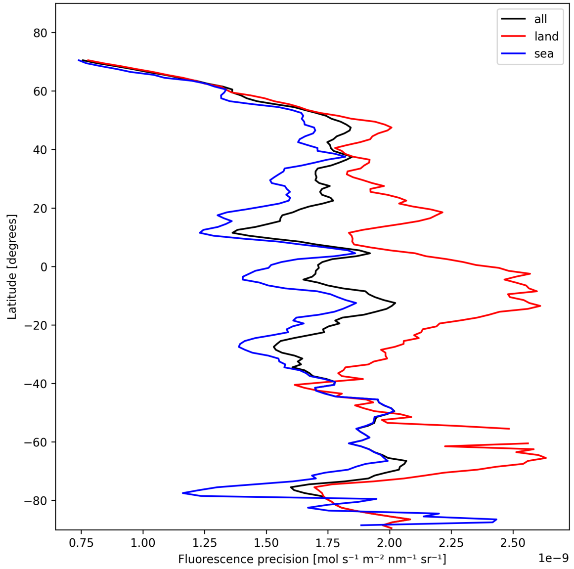
Figure 22: Zonal average of "Fluorescence precision" for 2025-01-31 to 2025-01-31.
