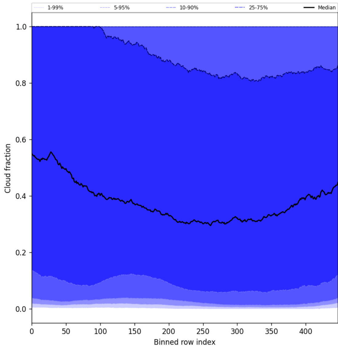
Figure 47: Along track statistics of “Cloud fraction” for 2025-01-31 to 2025-01-31
