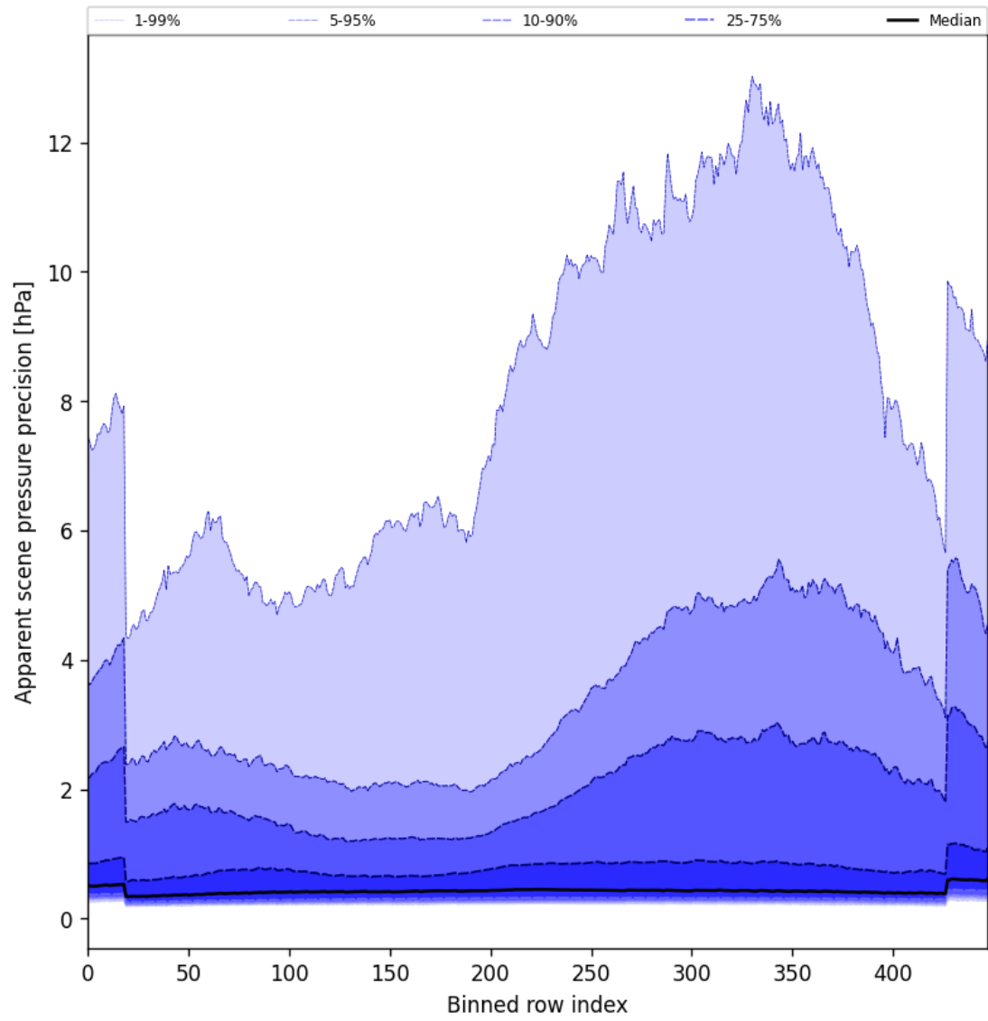
Figure 52: Along track statistics of “Apparent scene pressure precision” for 2025-01-31 to 2025-01-31
