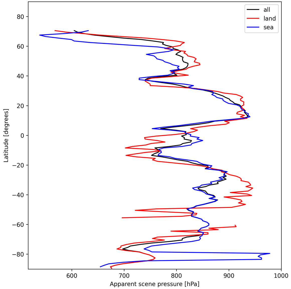
Figure 17: Zonal average of “Apparent scene pressure” for 2025-01-31 to 2025-01-31.
