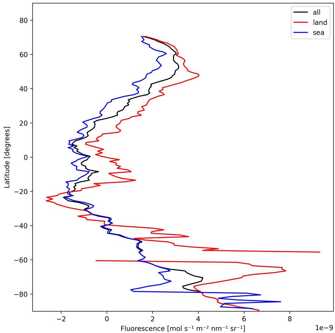
Figure 21: Zonal average of “Fluorescence” for 2025-01-31 to 2025-01-31.
