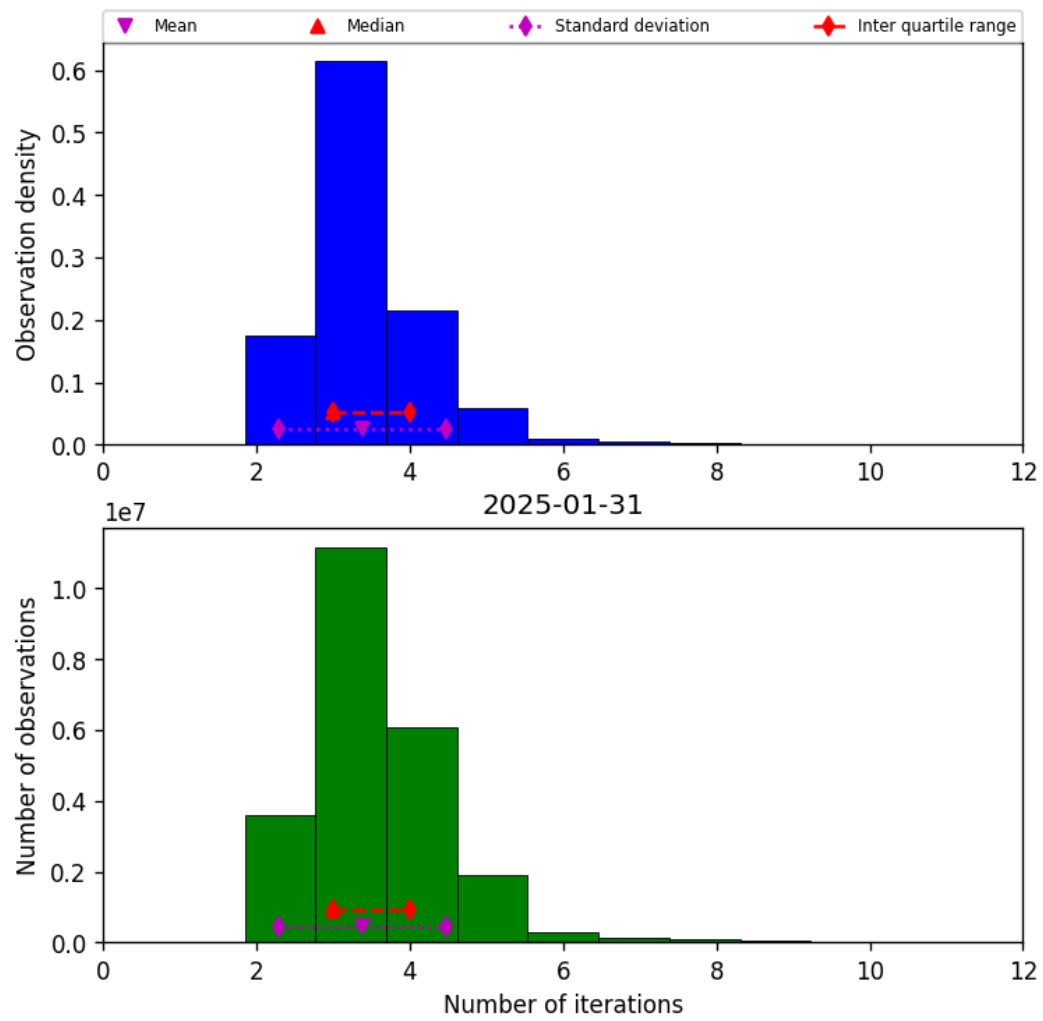
Figure 37: Histogram of “Number of iterations” for 2025-01-31 to 2025-01-31
