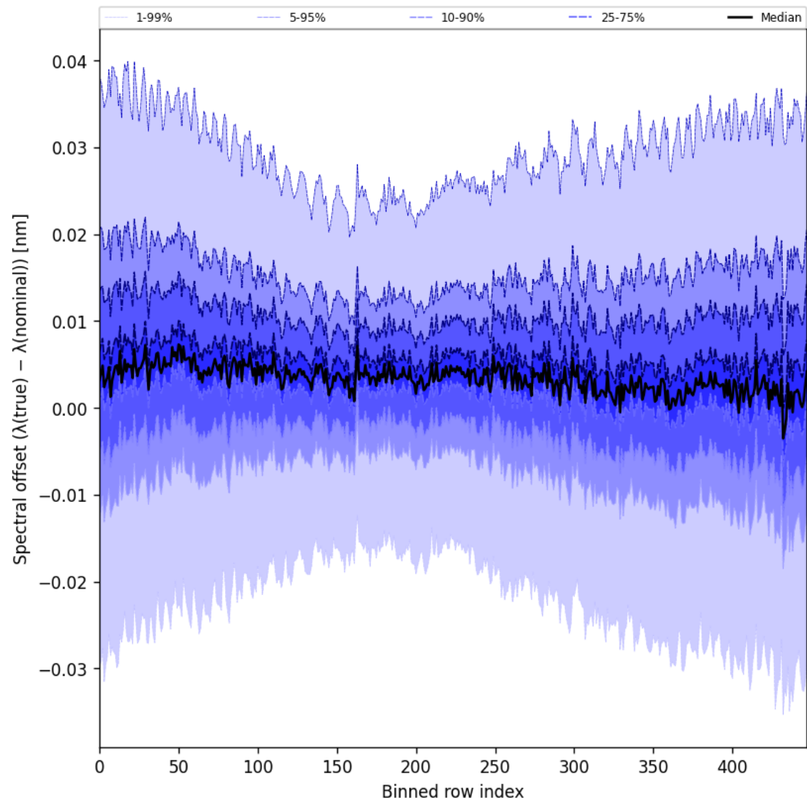
Figure 60: Along track statistics of “Spectral offset ( \lambda_{\text{true}} - \lambda_{\text{nominal}} )” for 2025-01-31 to 2025-01-31
