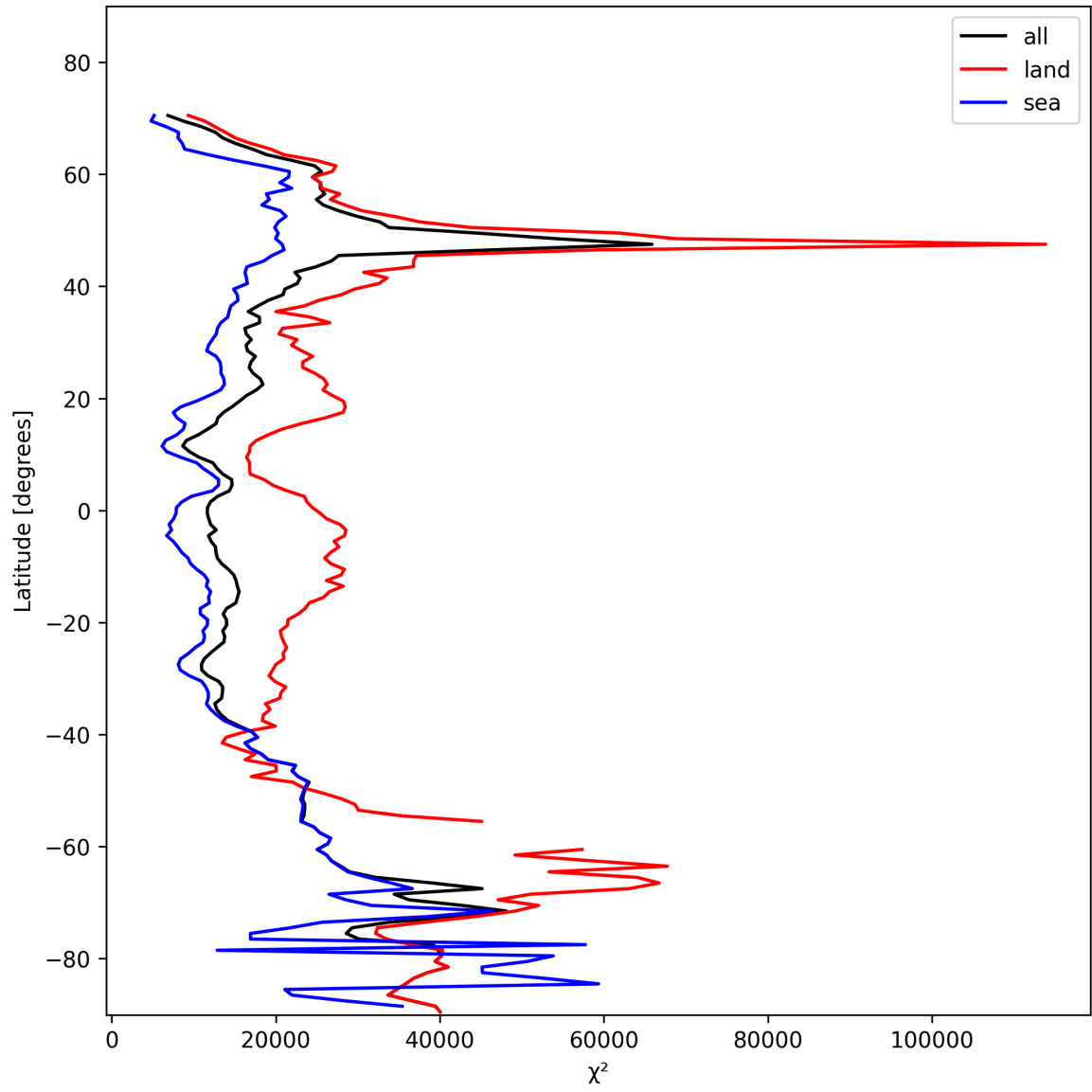
Figure 19: Zonal average of “ \chi^2 ” for 2025-01-31 to 2025-01-31.
