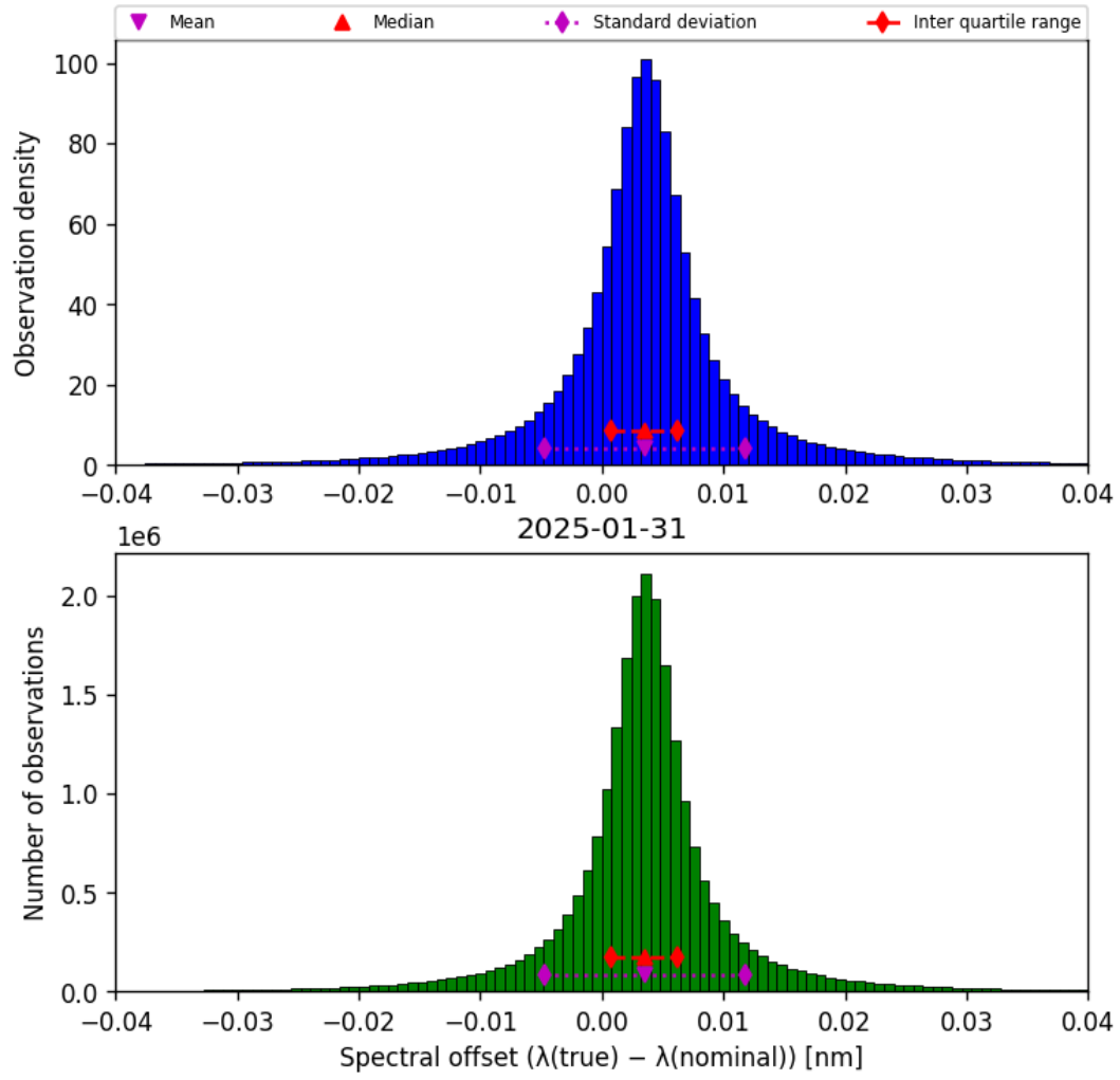
Figure 43: Histogram of “Spectral offset ( \lambda_{\text{true}} - \lambda_{\text{nominal}} )” for 2025-01-31 to 2025-01-31
