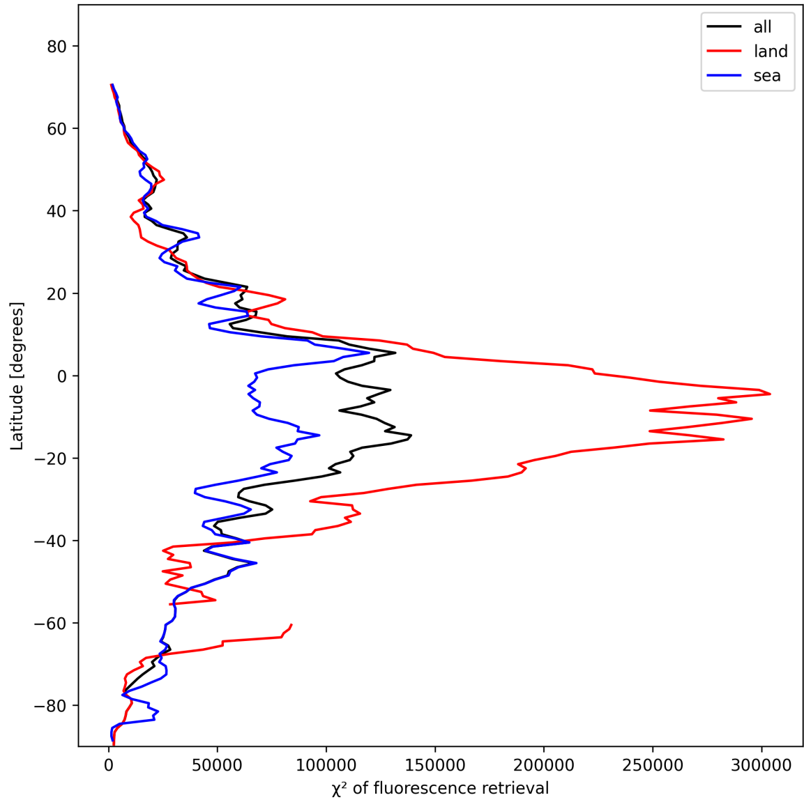
Figure 23: Zonal average of “ \chi^2 of fluorescence retrieval” for 2025-01-31 to 2025-01-31.
