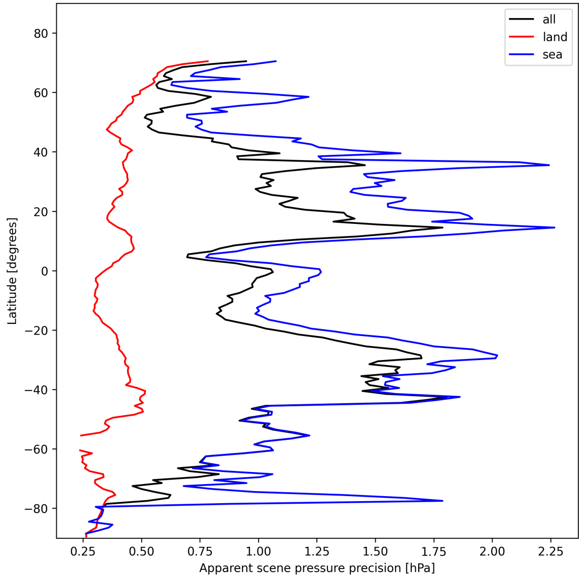
Figure 18: Zonal average of “Apparent scene pressure precision” for 2025-01-31 to 2025-01-31.
