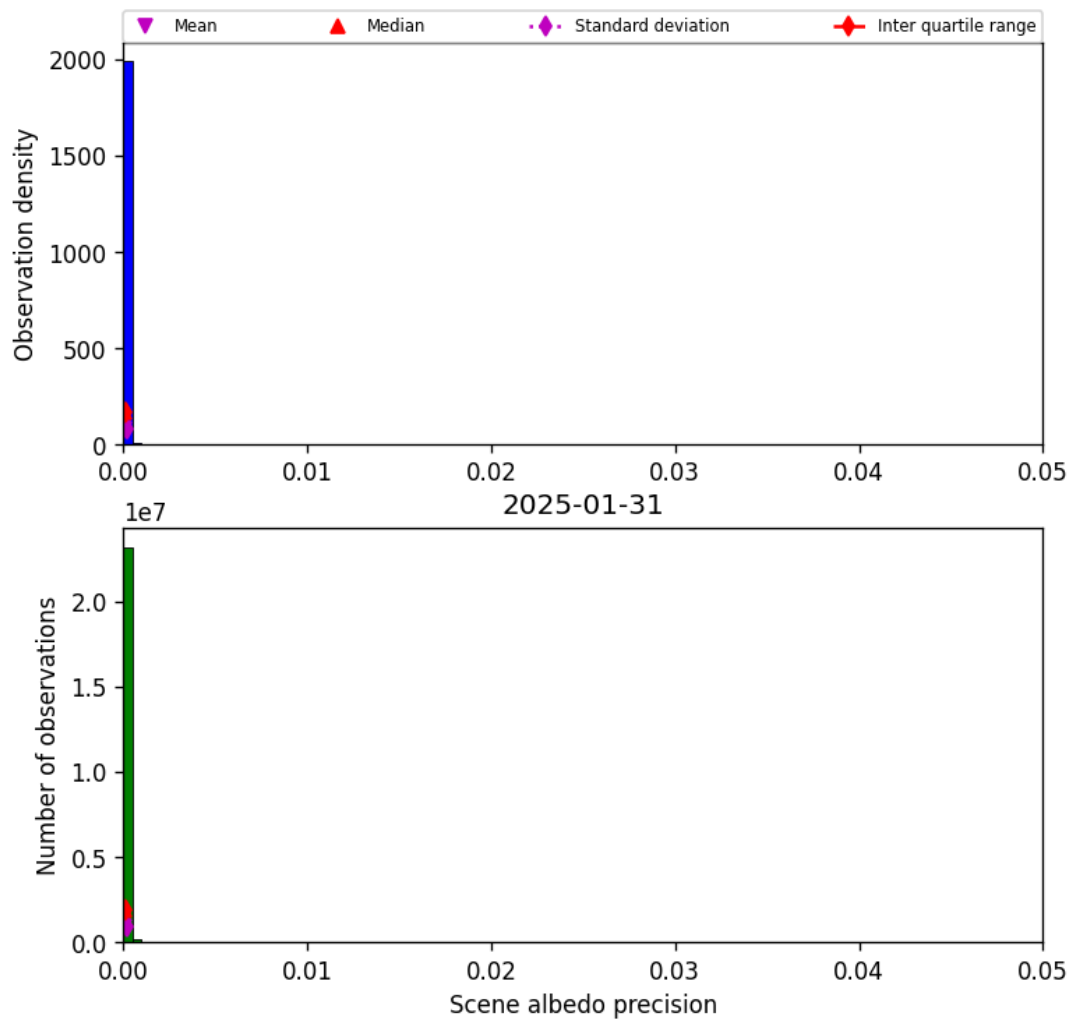
Figure 33: Histogram of “Scene albedo precision” for 2025-01-31 to 2025-01-31
