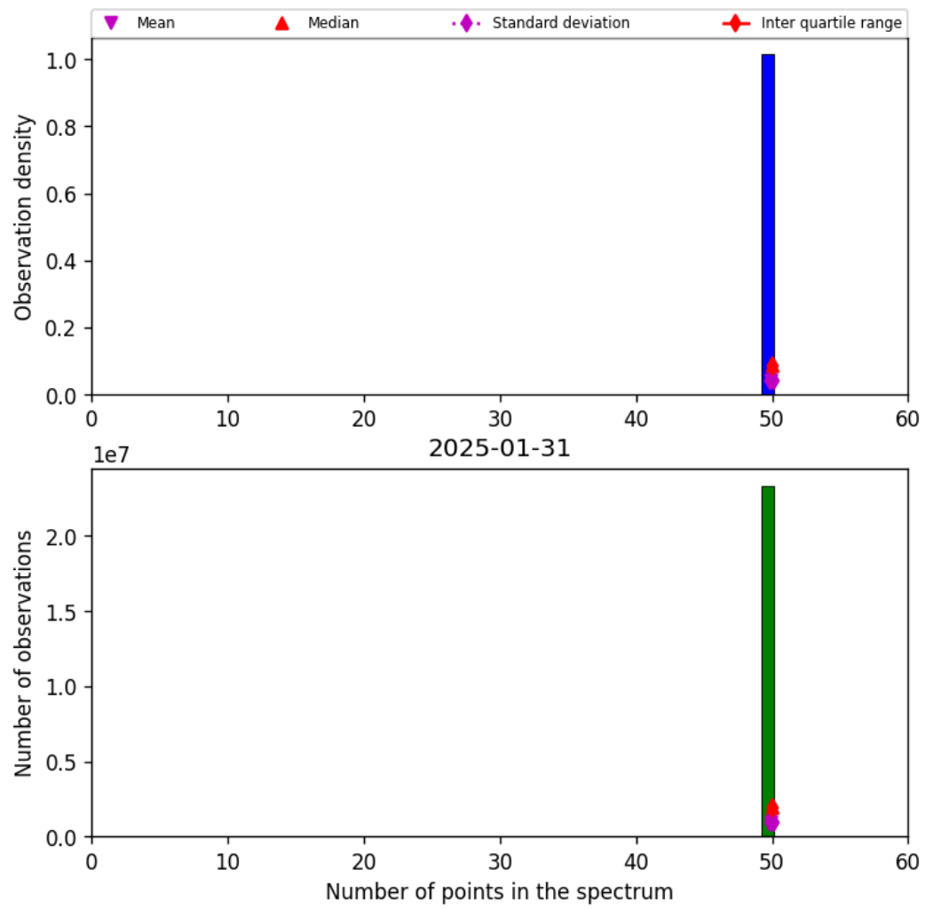
Figure 42: Histogram of “Number of points in the spectrum” for 2025-01-31 to 2025-01-31
