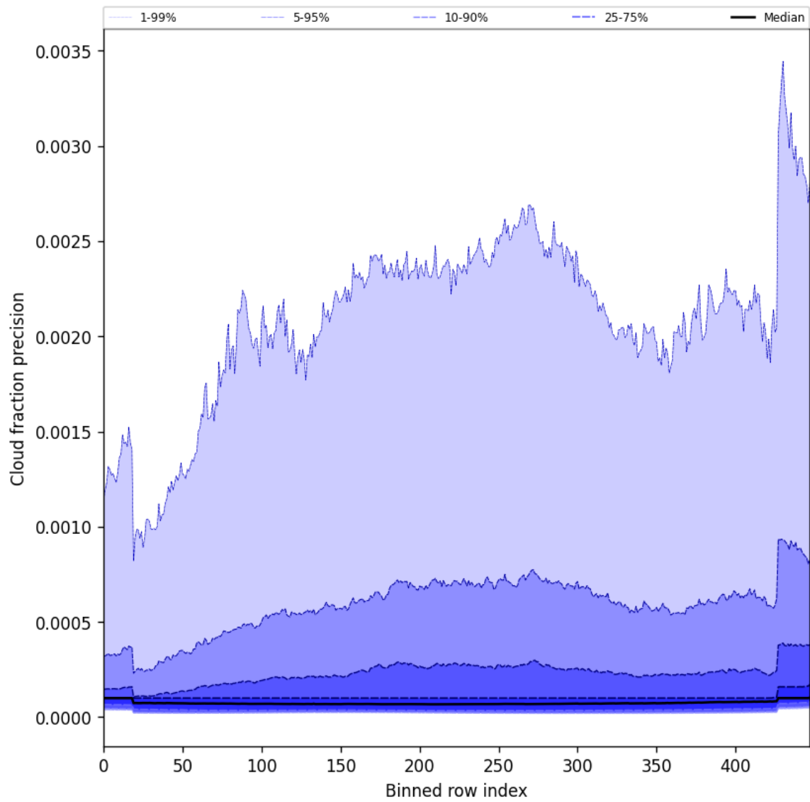
Figure 48: Along track statistics of “Cloud fraction precision” for 2025-01-31 to 2025-01-31
