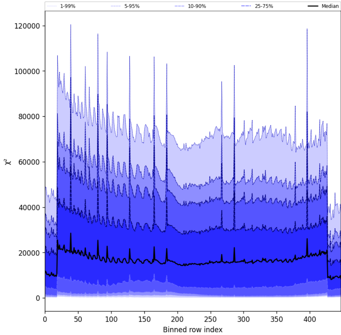
Figure 53: Along track statistics of “ \chi^2 ” for 2025-01-31 to 2025-01-31
