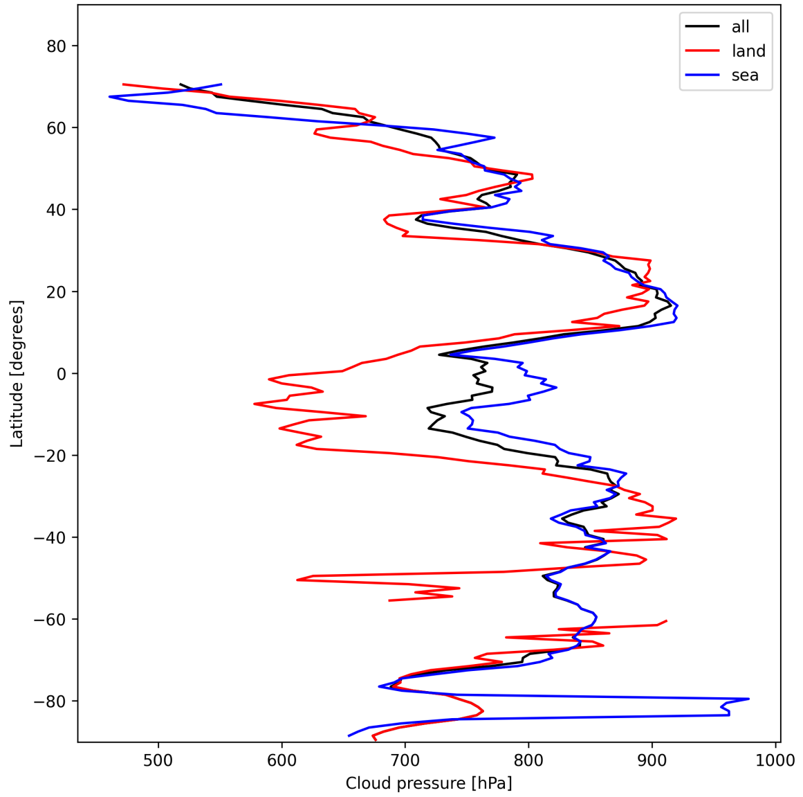
Figure 11: Zonal average of “Cloud pressure” for 2025-01-31 to 2025-01-31.
