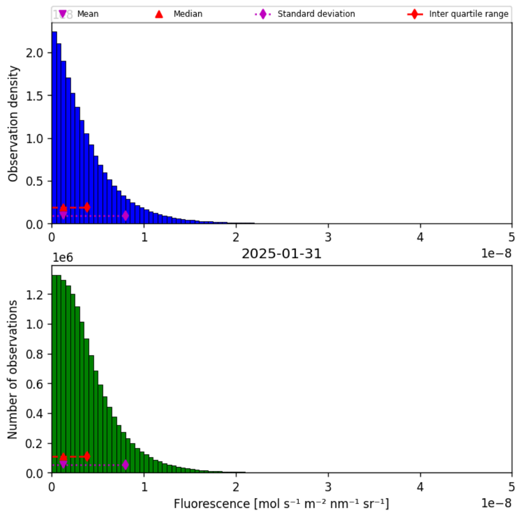
Figure 38: Histogram of “Fluorescence” for 2025-01-31 to 2025-01-31
