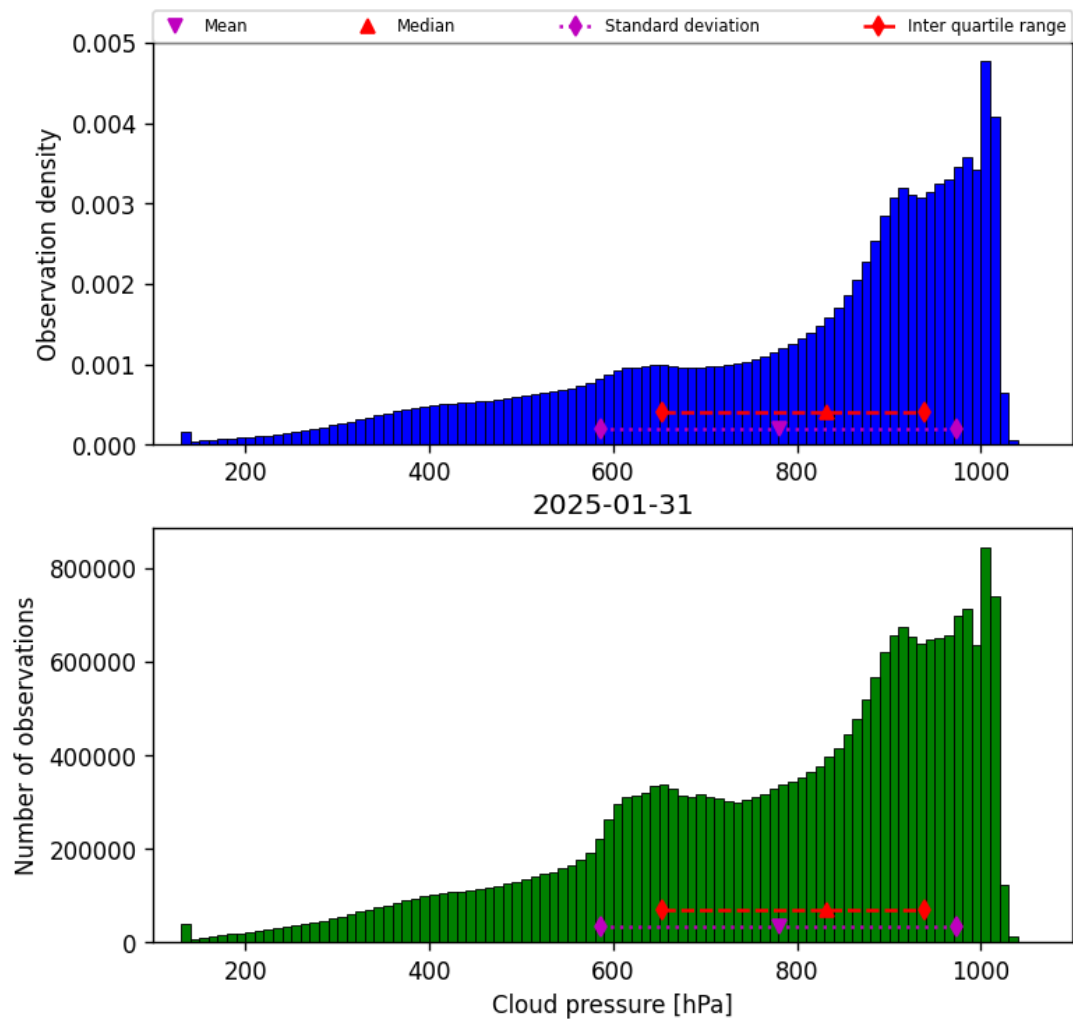
Figure 28: Histogram of “Cloud pressure” for 2025-01-31 to 2025-01-31
