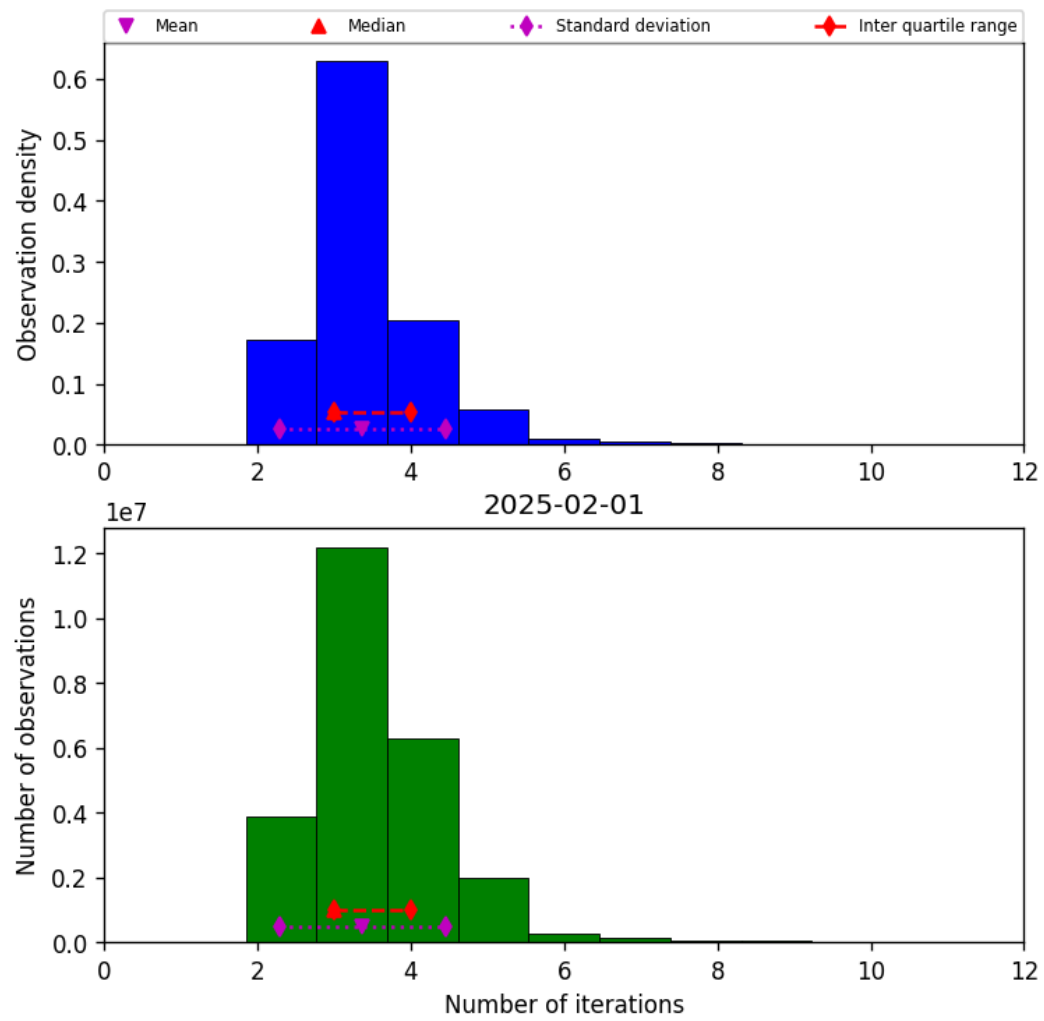
Figure 37: Histogram of “Number of iterations” for 2025-02-01 to 2025-02-02
