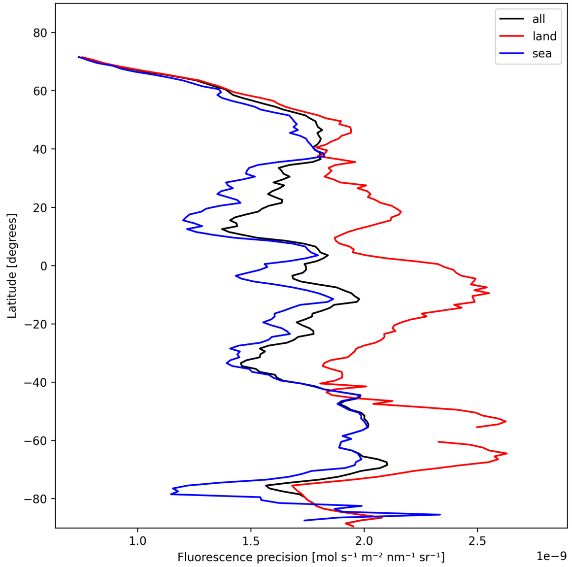
Figure 22: Zonal average of “Fluorescence precision” for 2025-02-01 to 2025-02-02.
