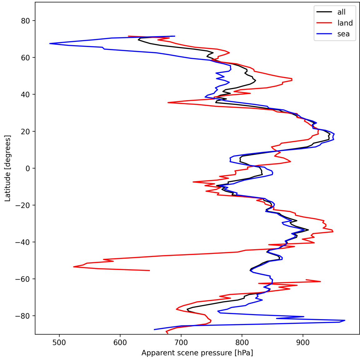
Figure 17: Zonal average of “Apparent scene pressure” for 2025-02-01 to 2025-02-02.
