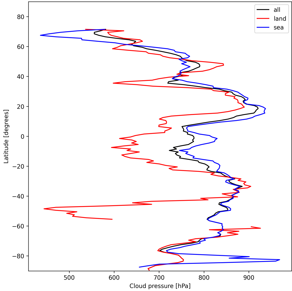
Figure 11: Zonal average of “Cloud pressure” for 2025-02-01 to 2025-02-02.
