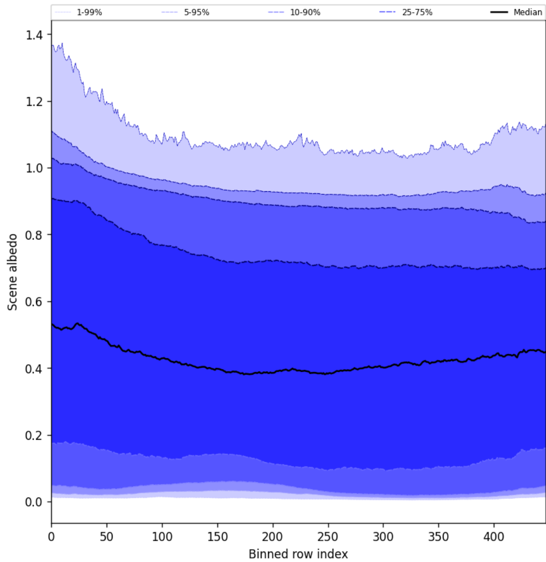
Figure 49: Along track statistics of “Scene albedo” for 2025-02-01 to 2025-02-02
