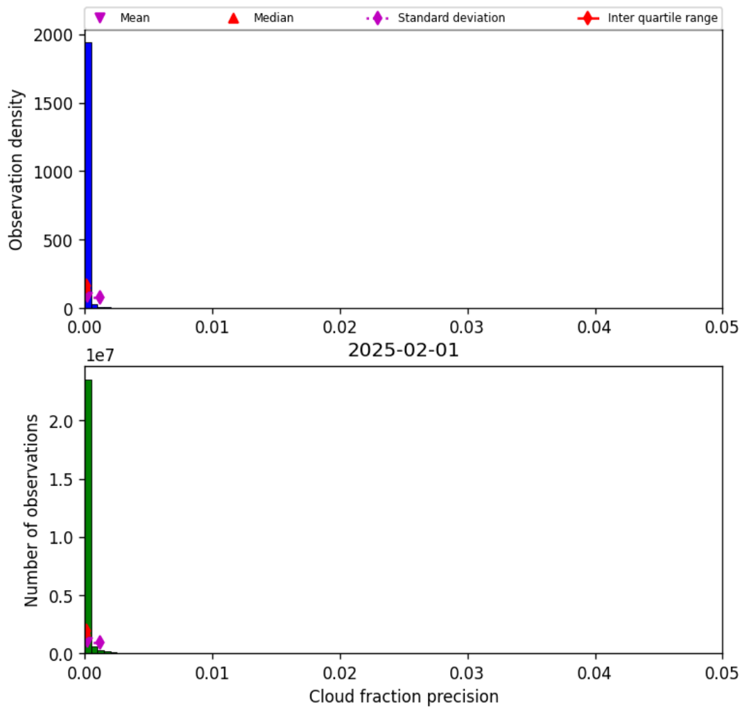
Figure 31: Histogram of “Cloud fraction precision” for 2025-02-01 to 2025-02-02
