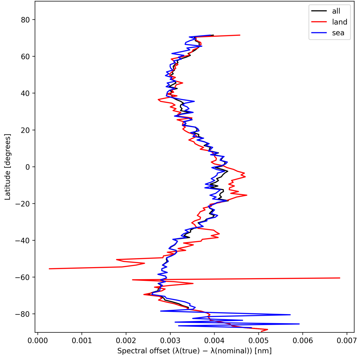
Figure 26: Zonal average of “Spectral offset ( \lambda_{\text{true}} - \lambda_{\text{nominal}} )” for 2025-02-01 to 2025-02-02.
