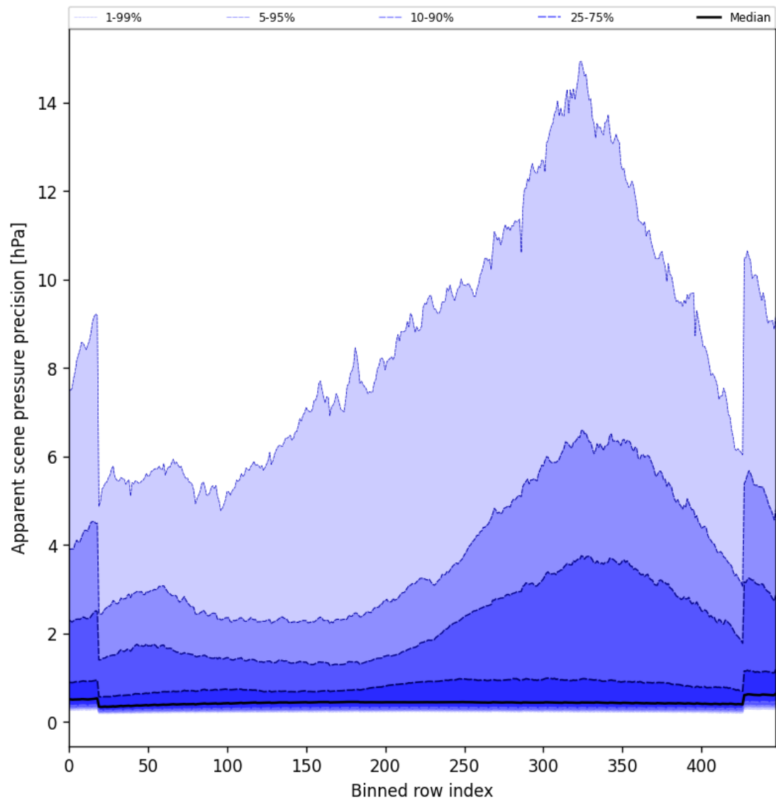
Figure 52: Along track statistics of “Apparent scene pressure precision” for 2025-02-01 to 2025-02-02
