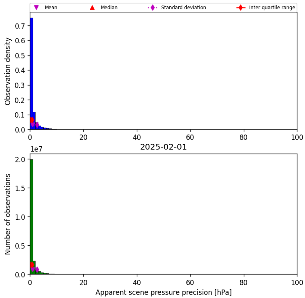
Figure 35: Histogram of “Apparent scene pressure precision” for 2025-02-01 to 2025-02-02
