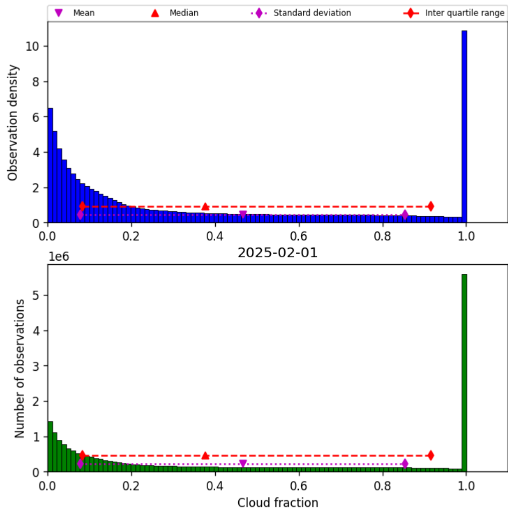
Figure 30: Histogram of “Cloud fraction” for 2025-02-01 to 2025-02-02
