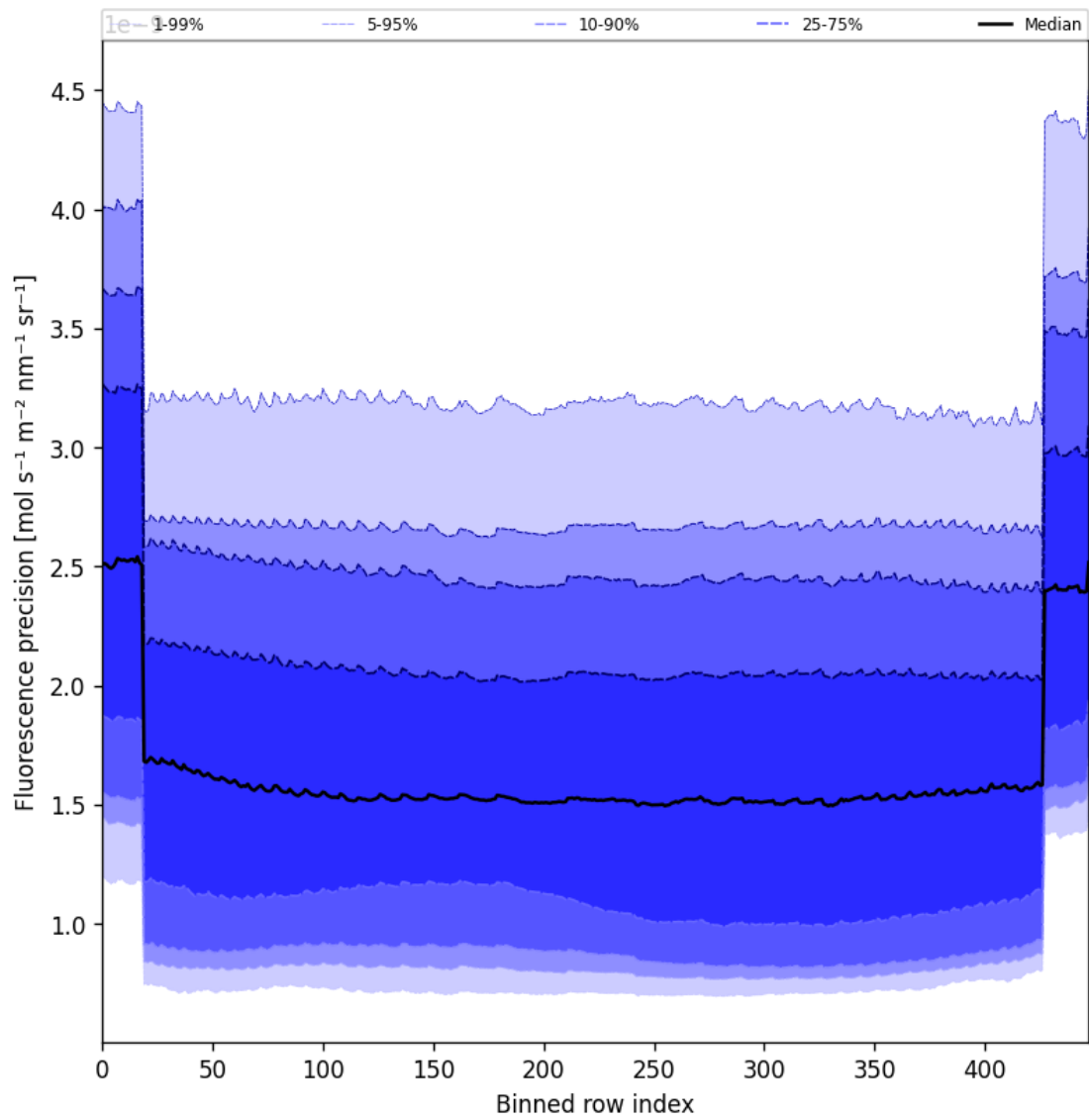
Figure 56: Along track statistics of “Fluorescence precision” for 2025-02-01 to 2025-02-02
