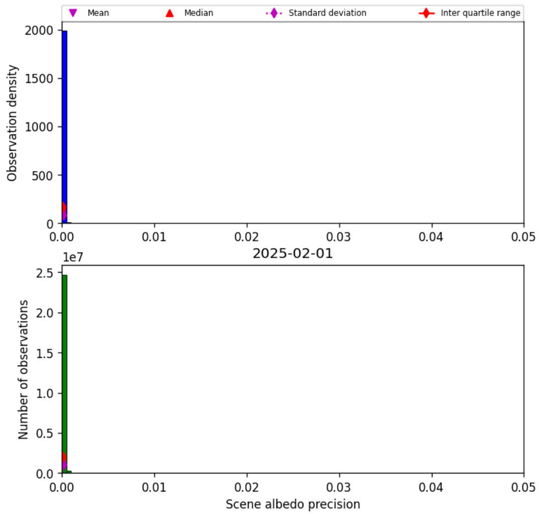
Figure 33: Histogram of “Scene albedo precision” for 2025-02-01 to 2025-02-02
