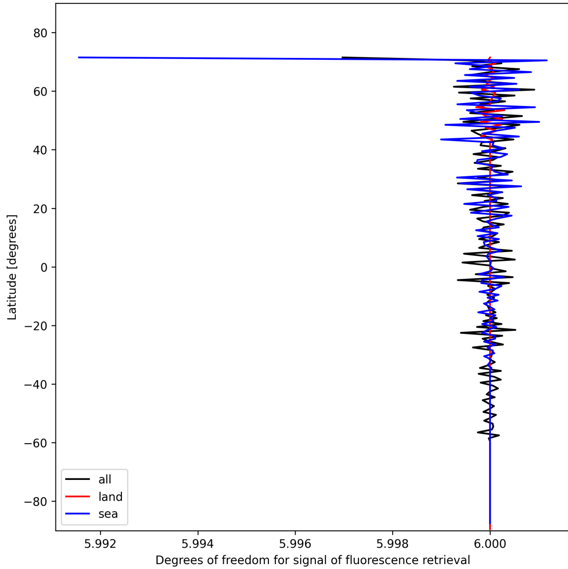
Figure 24: Zonal average of “Degrees of freedom for signal of fluorescence retrieval” for 2025-02-01 to 2025-02-02.
