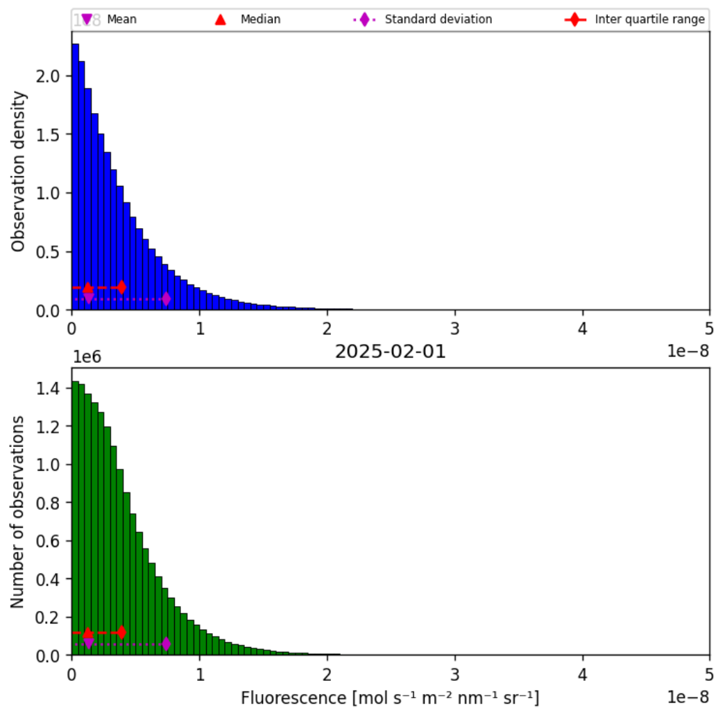
Figure 38: Histogram of “Fluorescence” for 2025-02-01 to 2025-02-02
