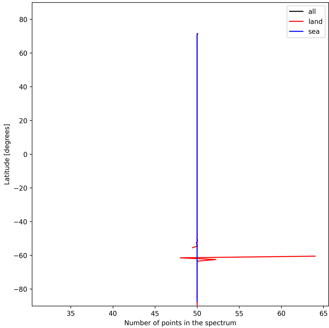
Figure 25: Zonal average of “Number of points in the spectrum” for 2025-02-01 to 2025-02-02.
