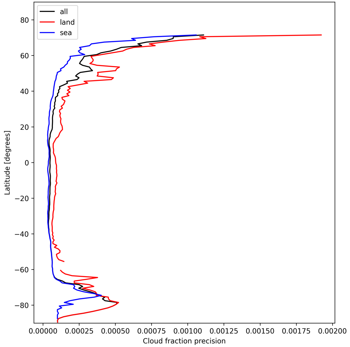
Figure 14: Zonal average of “Cloud fraction precision” for 2025-02-01 to 2025-02-02.
