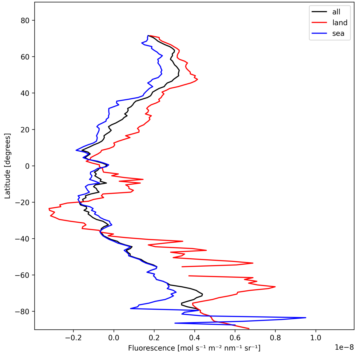
Figure 21: Zonal average of “Fluorescence” for 2025-02-01 to 2025-02-02.
