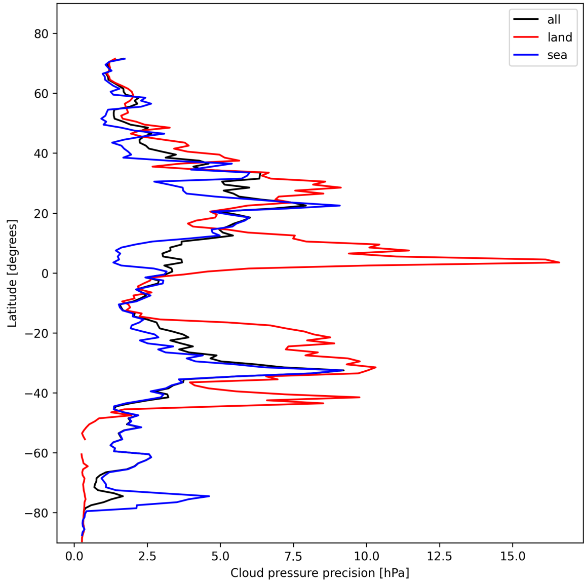
Figure 12: Zonal average of "Cloud pressure precision" for 2025-02-01 to 2025-02-02.
