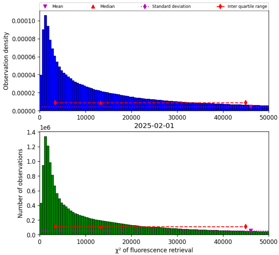
Figure 40: Histogram of “ \chi^2 of fluorescence retrieval” for 2025-02-01 to 2025-02-02
