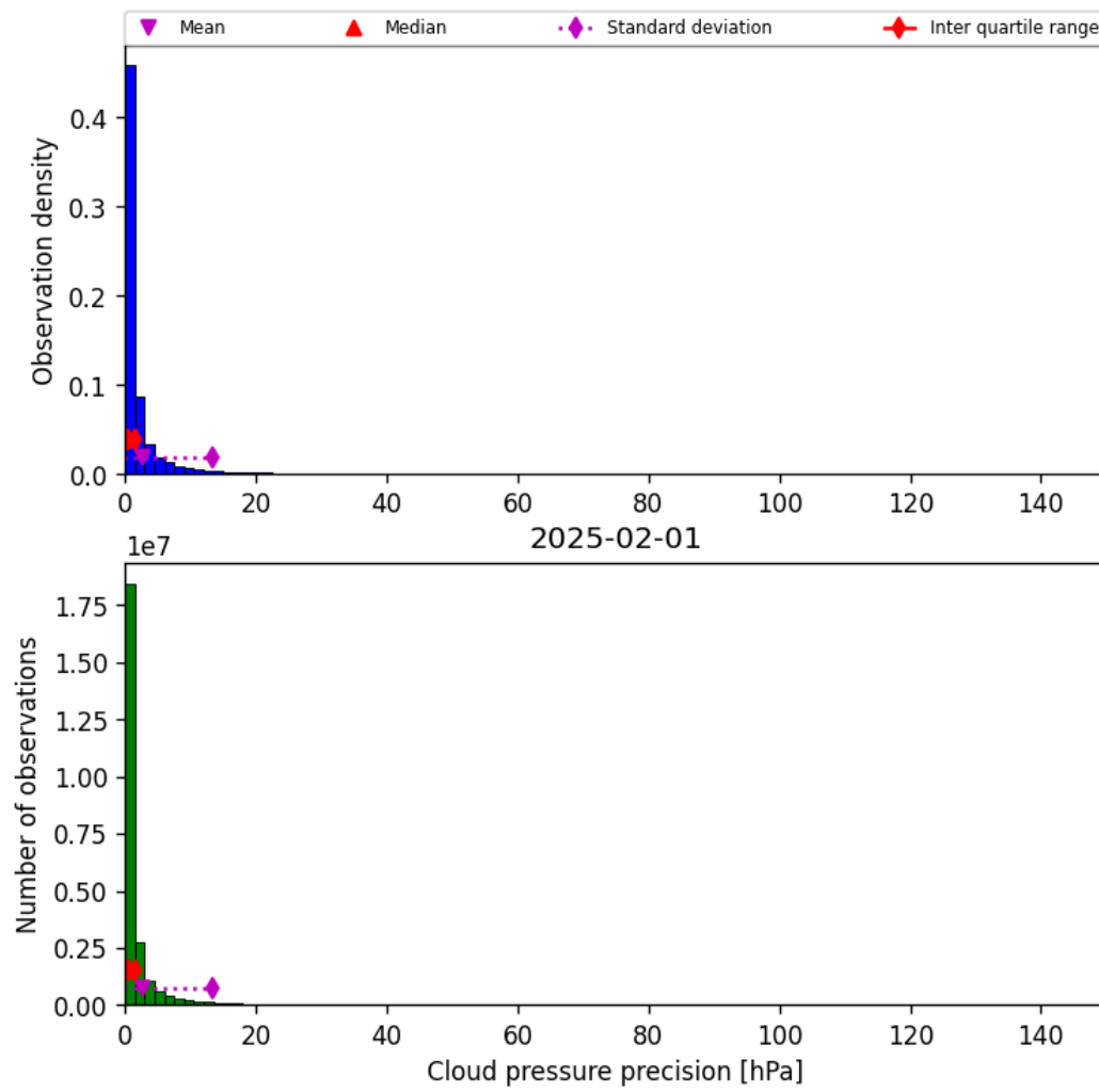
Figure 29: Histogram of “Cloud pressure precision” for 2025-02-01 to 2025-02-02
