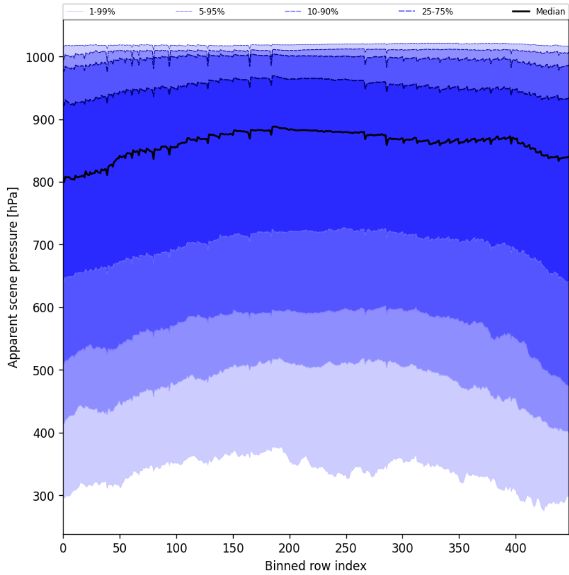
Figure 51: Along track statistics of “Apparent scene pressure” for 2025-02-01 to 2025-02-02
