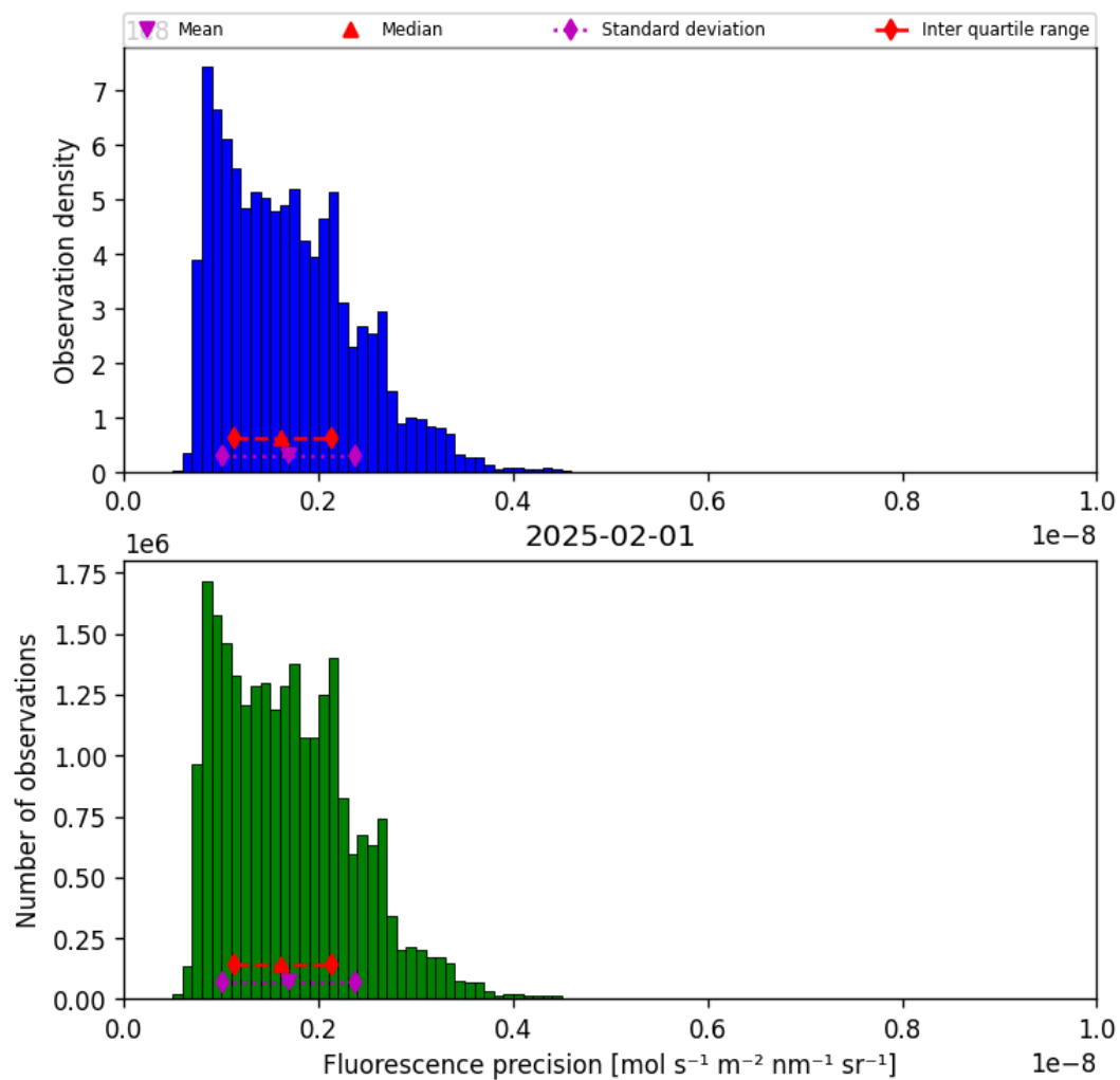
Figure 39: Histogram of “Fluorescence precision” for 2025-02-01 to 2025-02-02
