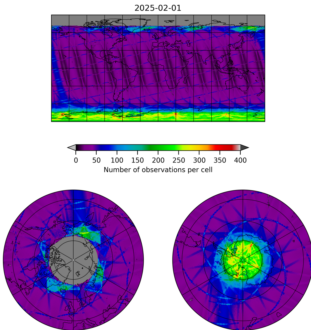
Figure 9: Map of the number of observations for 2025-02-01 to 2025-02-02
