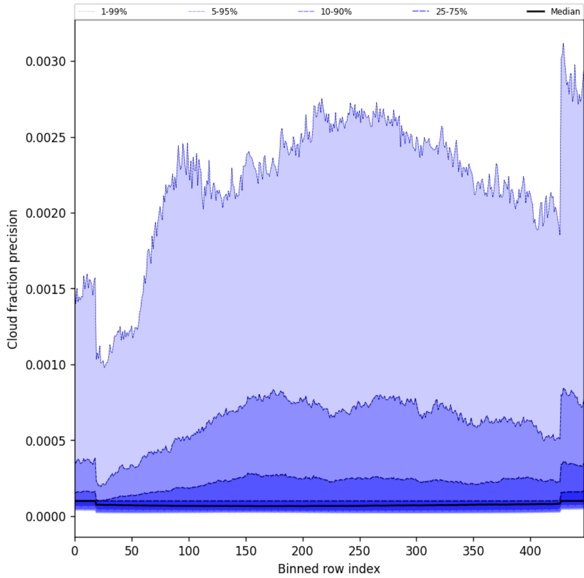
Figure 48: Along track statistics of “Cloud fraction precision” for 2025-02-01 to 2025-02-02
