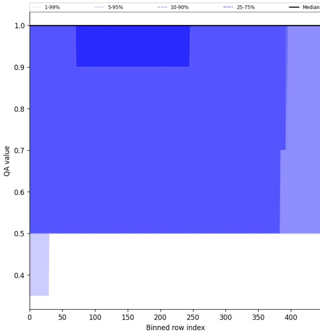
Figure 44: Along track statistics of “QA value” for 2025-02-01 to 2025-02-02
