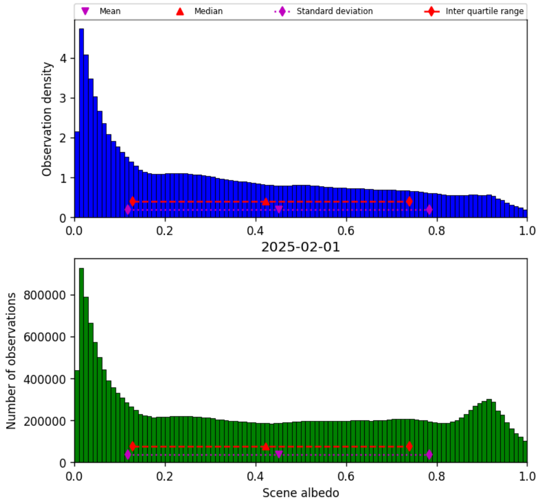
Figure 32: Histogram of “Scene albedo” for 2025-02-01 to 2025-02-02
