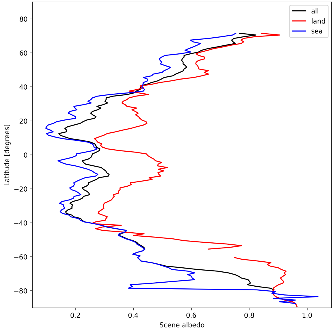
Figure 15: Zonal average of “Scene albedo” for 2025-02-01 to 2025-02-02.
