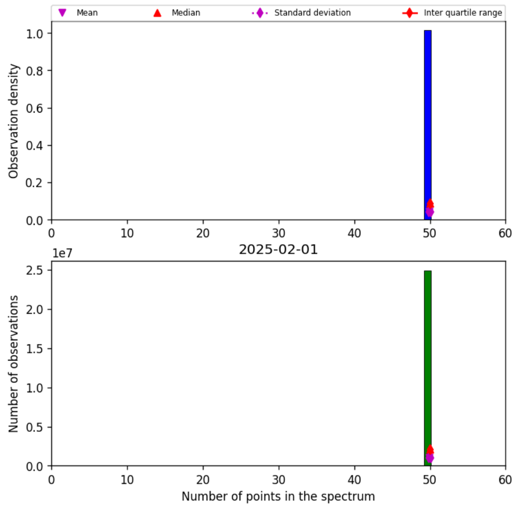
Figure 42: Histogram of “Number of points in the spectrum” for 2025-02-01 to 2025-02-02
