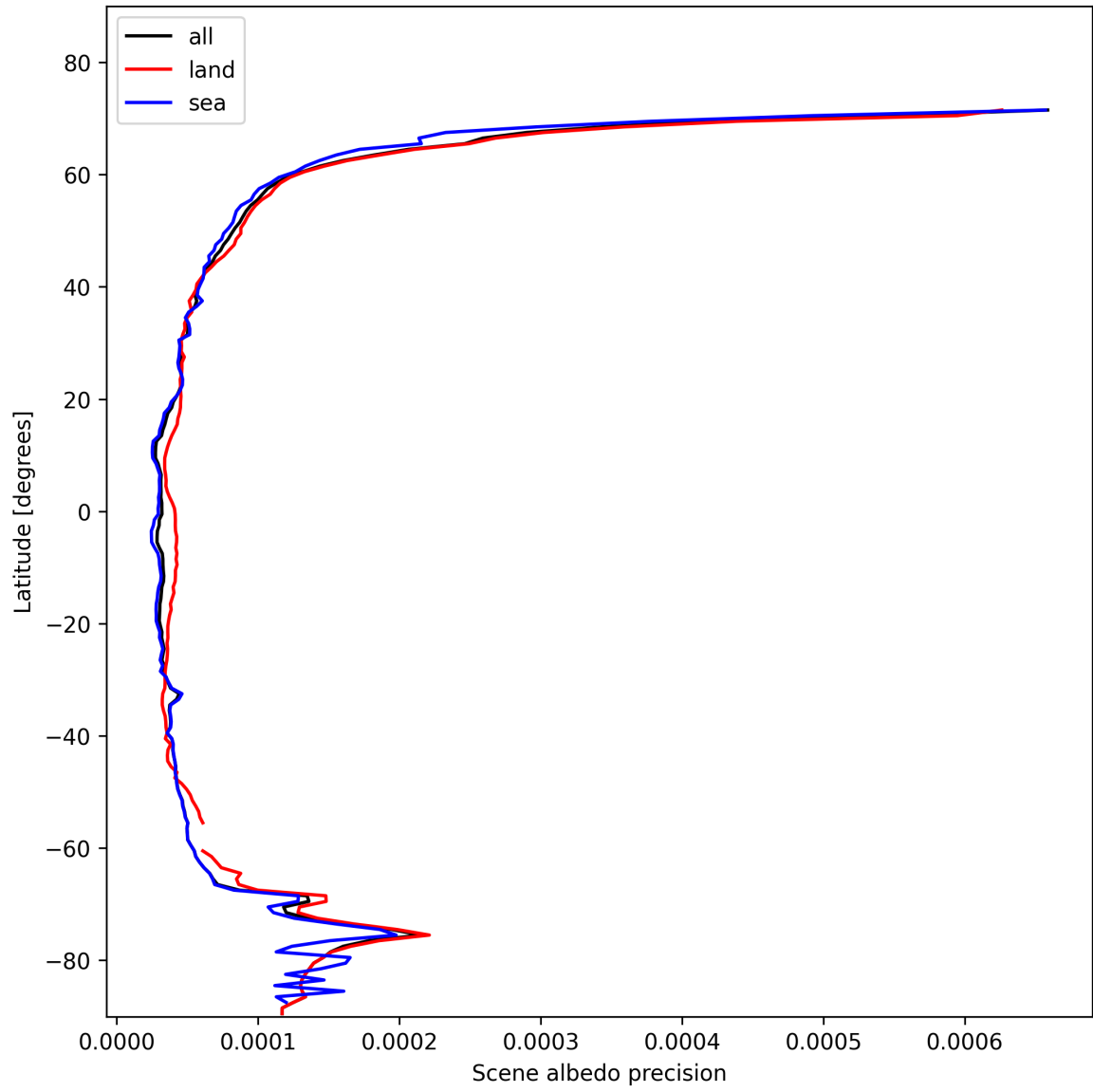
Figure 16: Zonal average of “Scene albedo precision” for 2025-02-01 to 2025-02-02.
