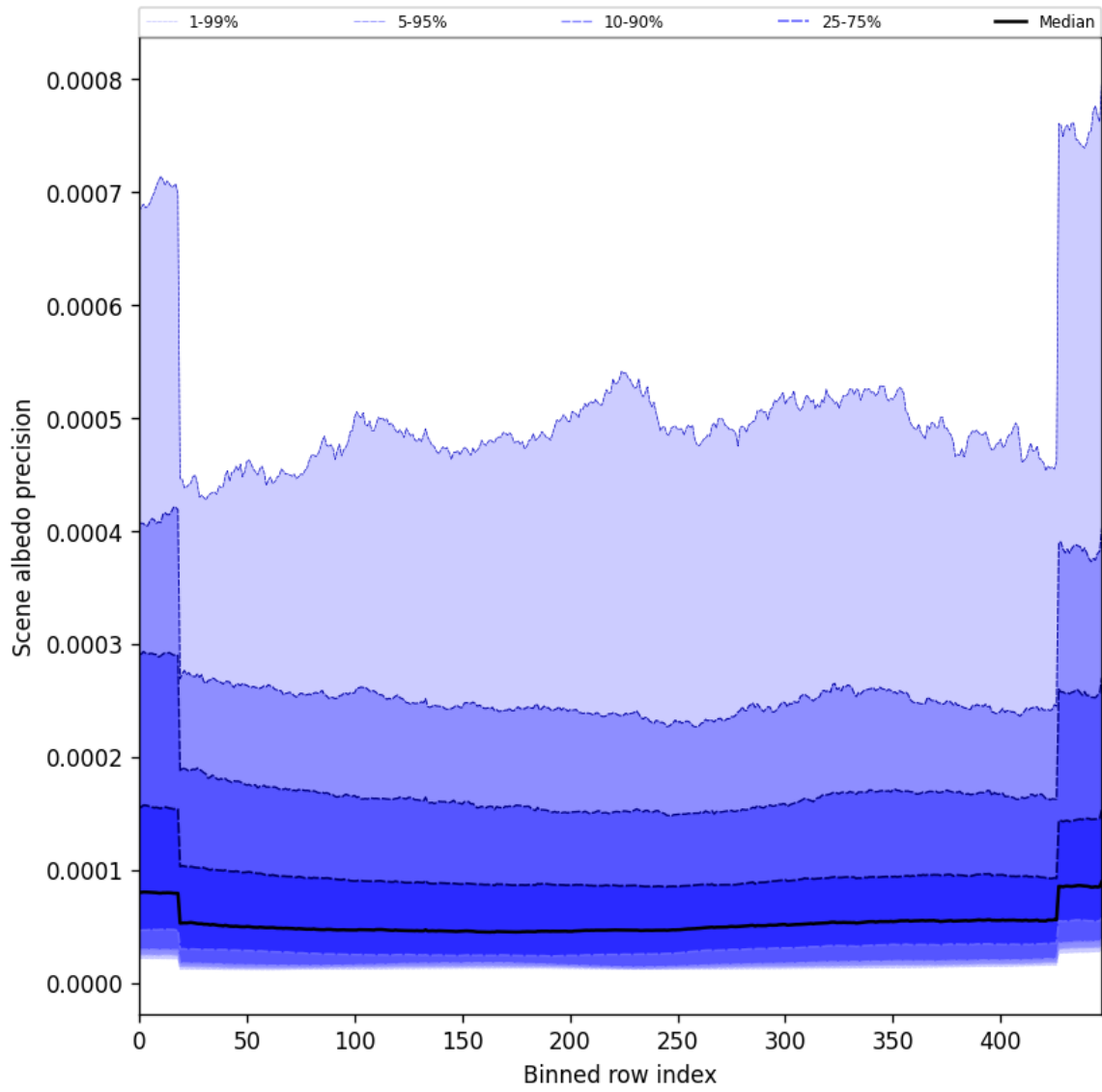
Figure 50: Along track statistics of “Scene albedo precision” for 2025-02-01 to 2025-02-02
