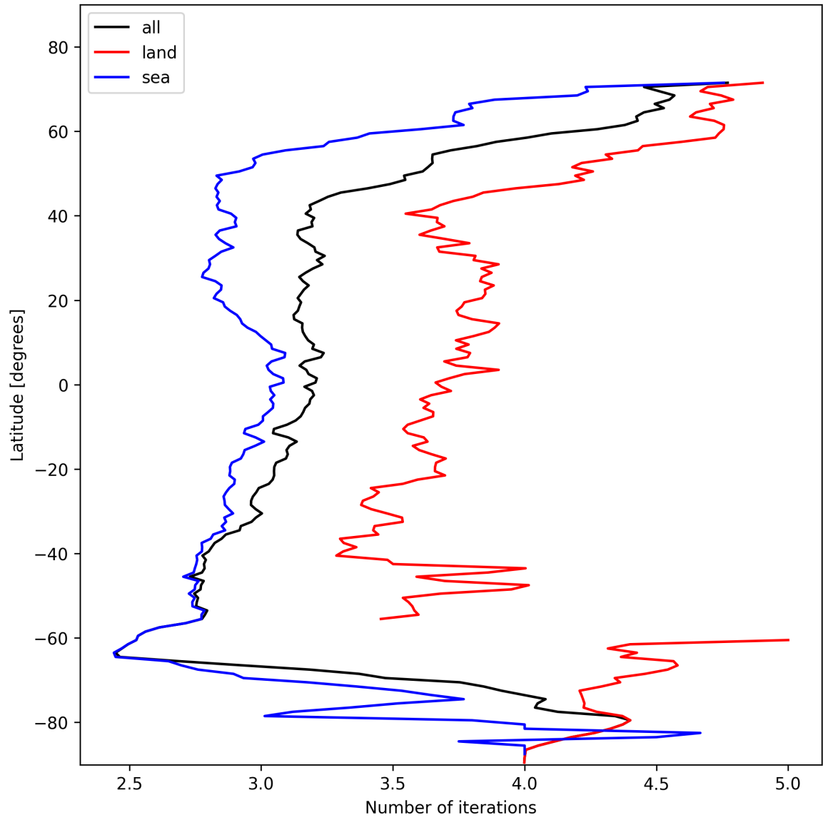
Figure 20: Zonal average of “Number of iterations” for 2025-02-01 to 2025-02-02.
