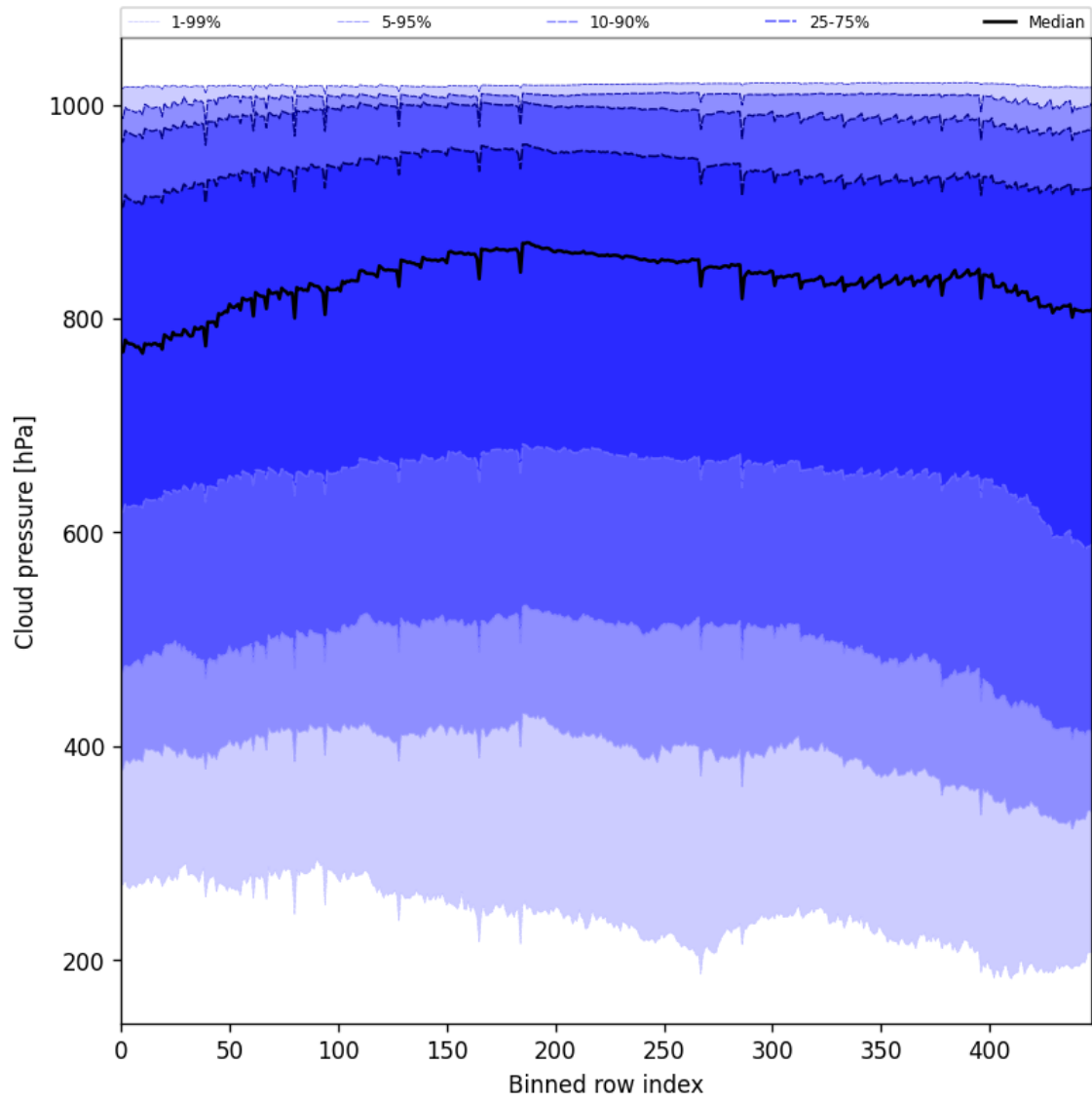
Figure 45: Along track statistics of “Cloud pressure” for 2025-02-01 to 2025-02-02
