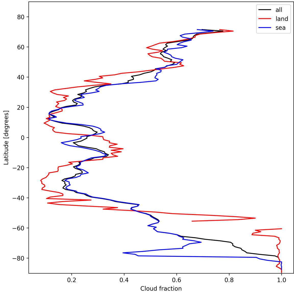
Figure 13: Zonal average of “Cloud fraction” for 2025-02-01 to 2025-02-02.
