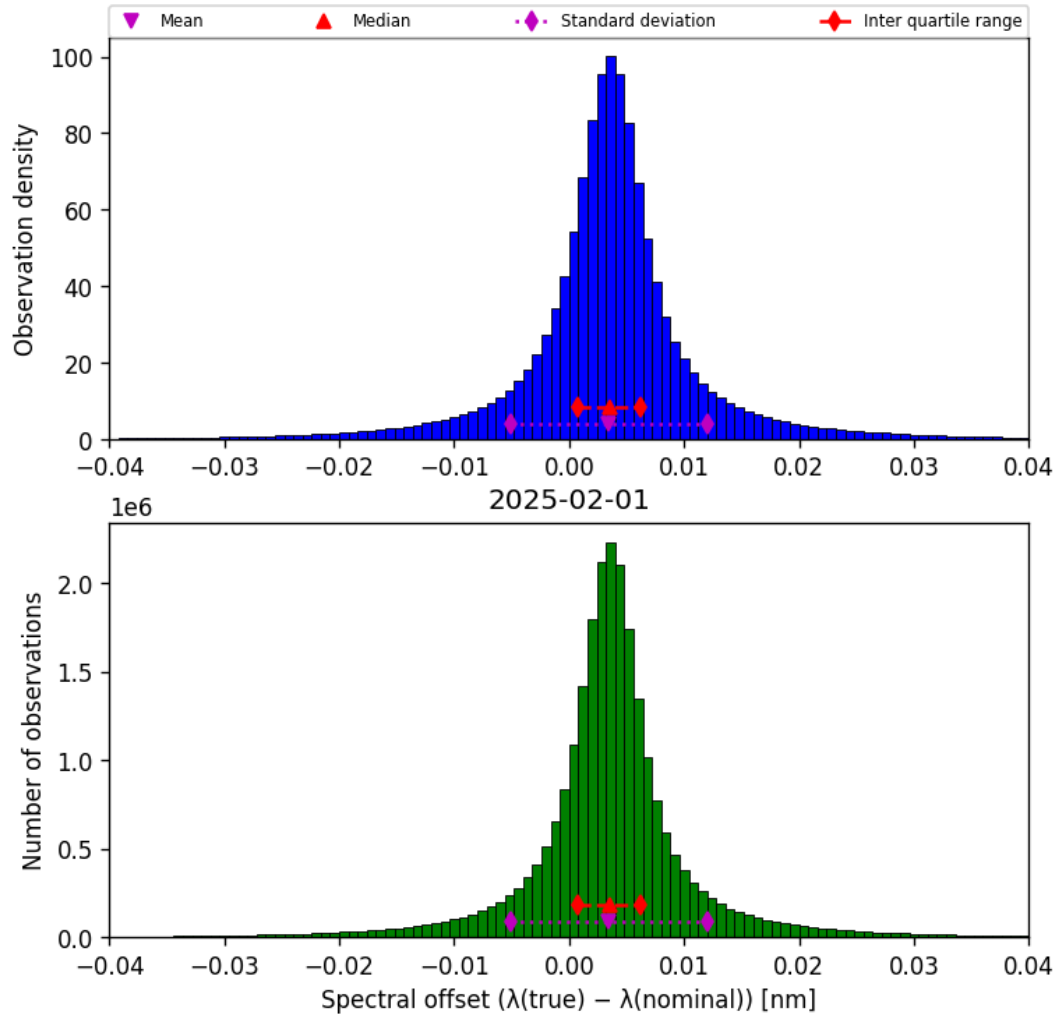
Figure 43: Histogram of “Spectral offset ( \lambda_{\text{true}} - \lambda_{\text{nominal}} )” for 2025-02-01 to 2025-02-02
