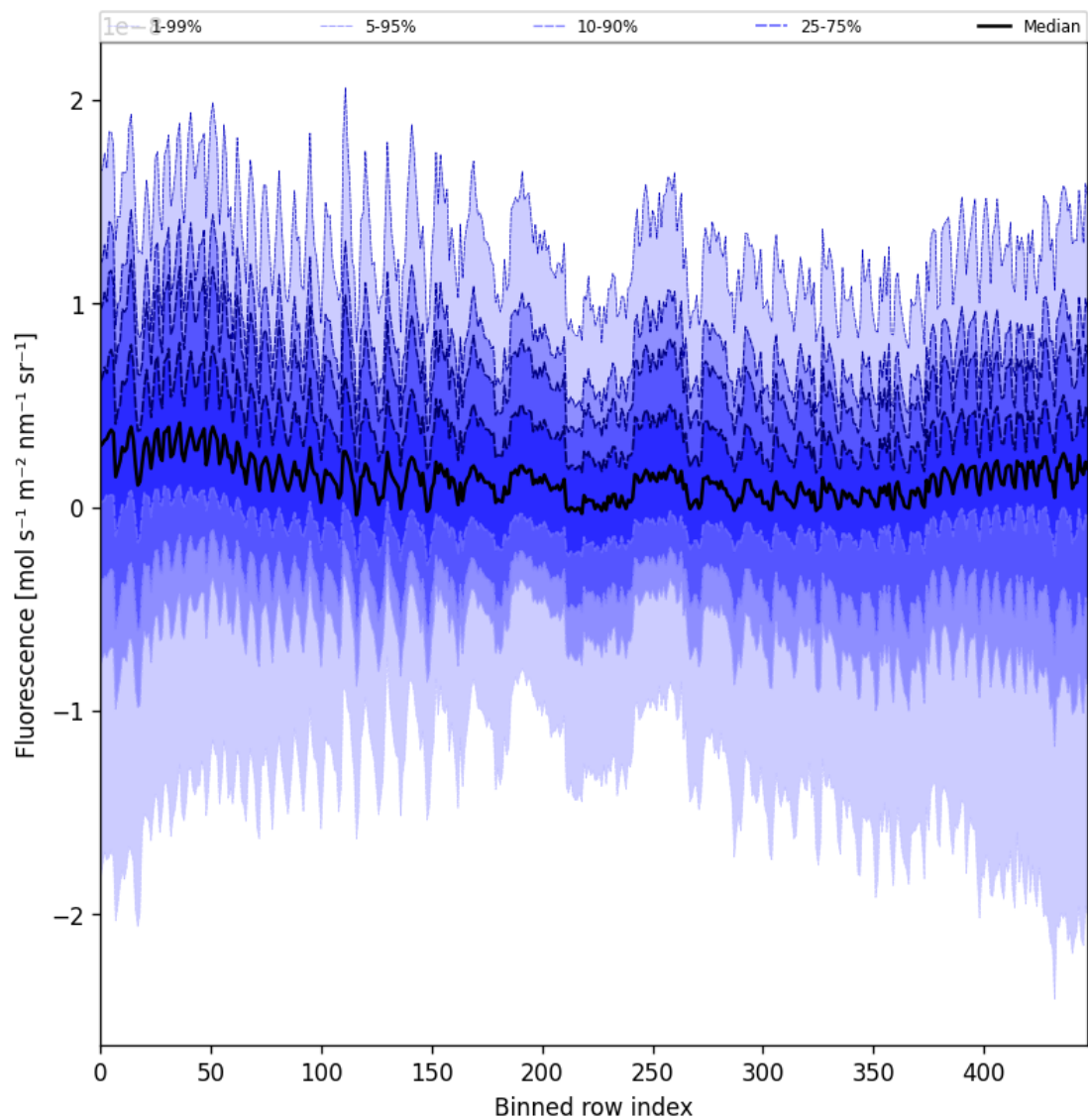
Figure 55: Along track statistics of “Fluorescence” for 2025-02-01 to 2025-02-02
