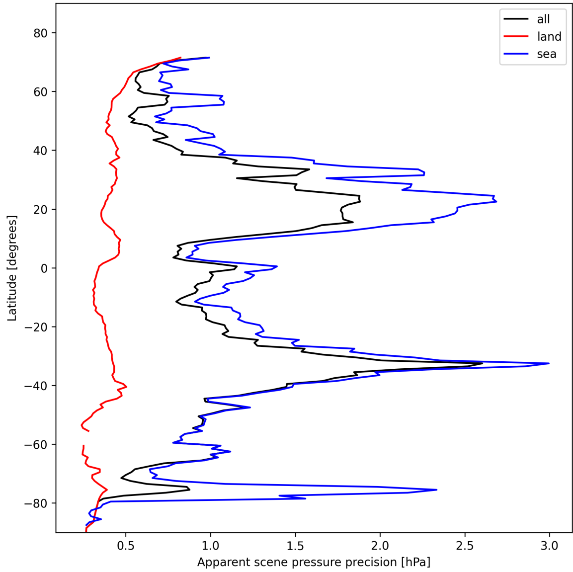
Figure 18: Zonal average of “Apparent scene pressure precision” for 2025-02-01 to 2025-02-02.
