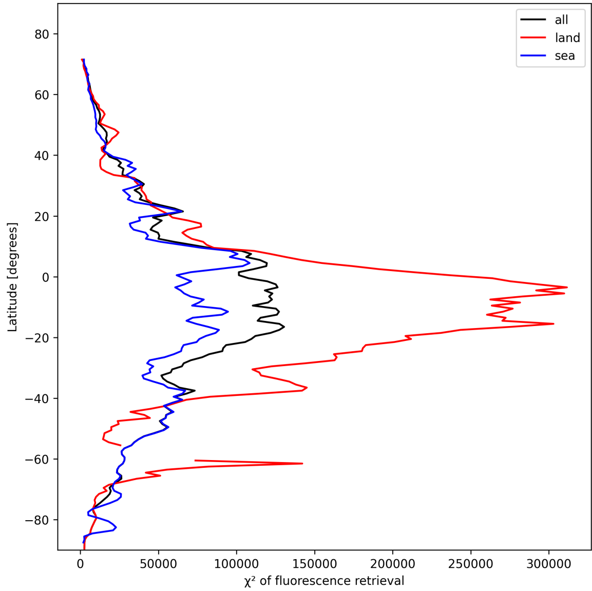
Figure 23: Zonal average of “ \chi^2 of fluorescence retrieval” for 2025-02-01 to 2025-02-02.
