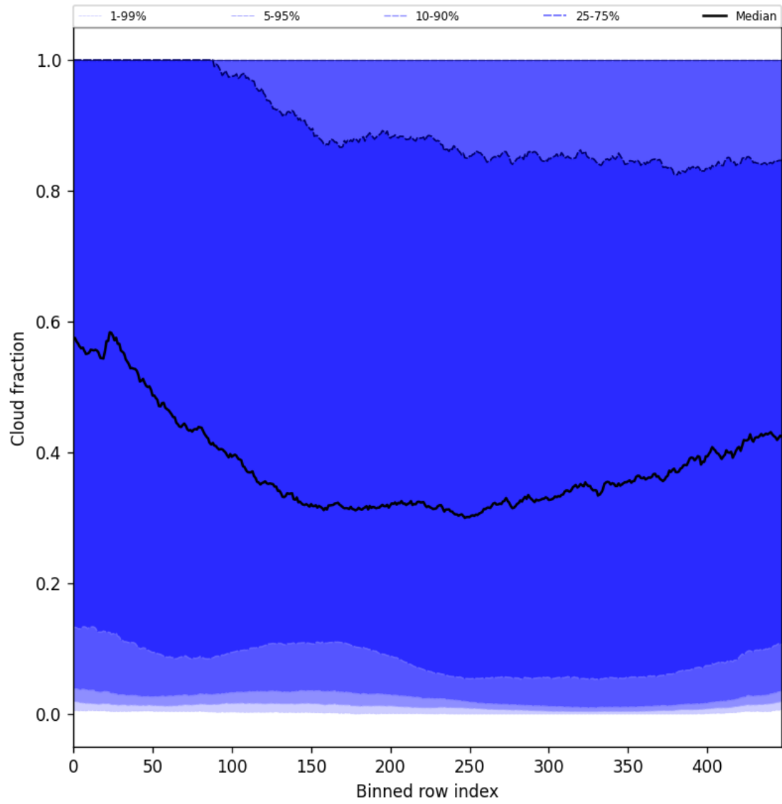
Figure 47: Along track statistics of “Cloud fraction” for 2025-02-01 to 2025-02-02
