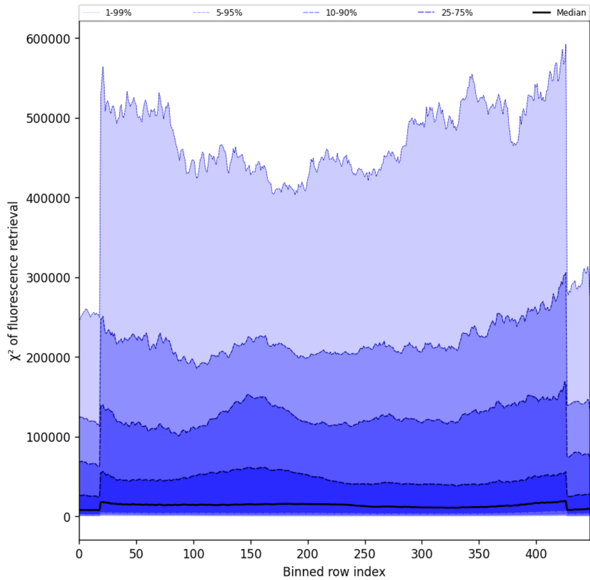
Figure 57: Along track statistics of “ \chi^2 of fluorescence retrieval” for 2025-02-01 to 2025-02-02
