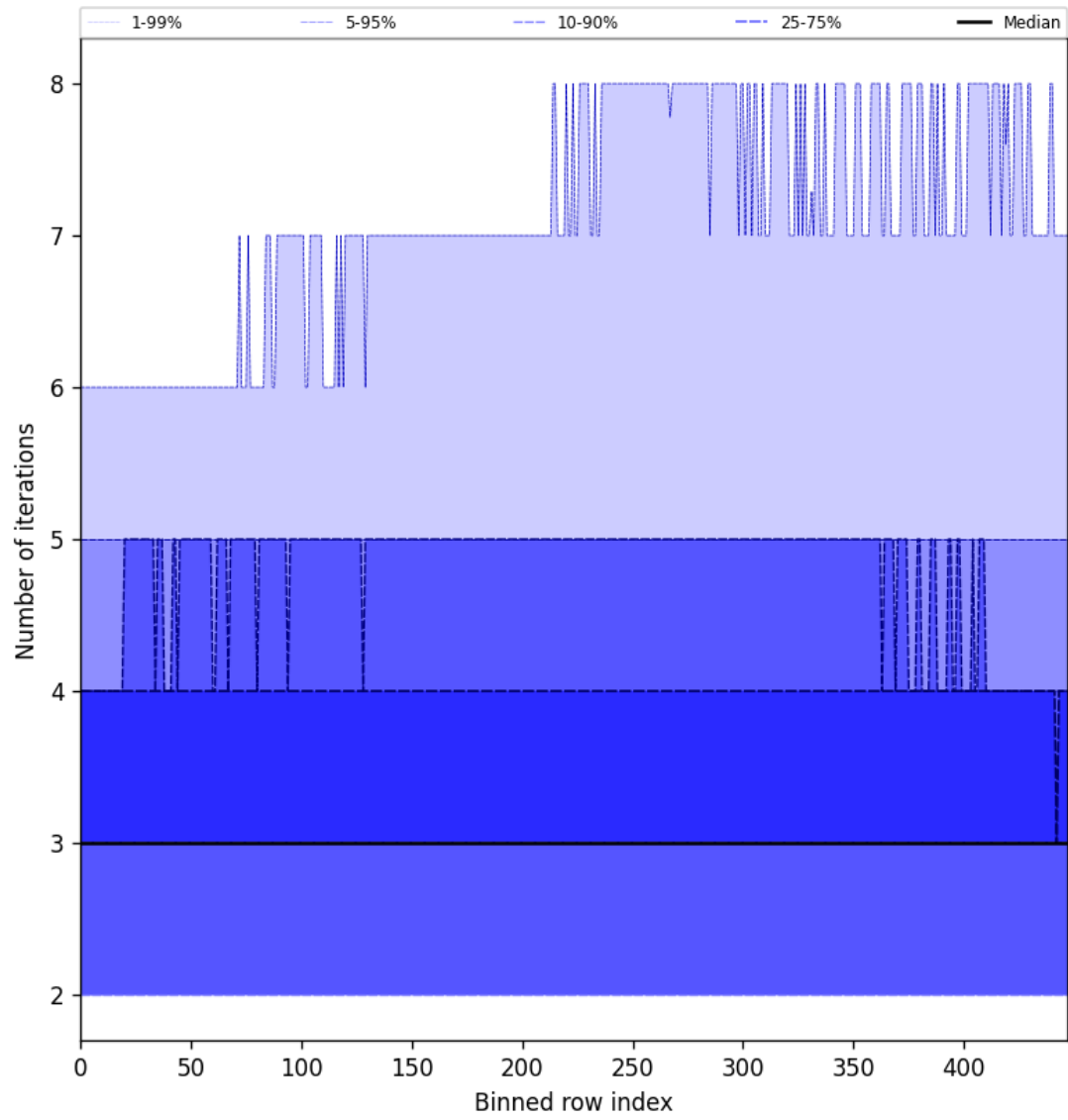
Figure 54: Along track statistics of “Number of iterations” for 2025-02-01 to 2025-02-02
