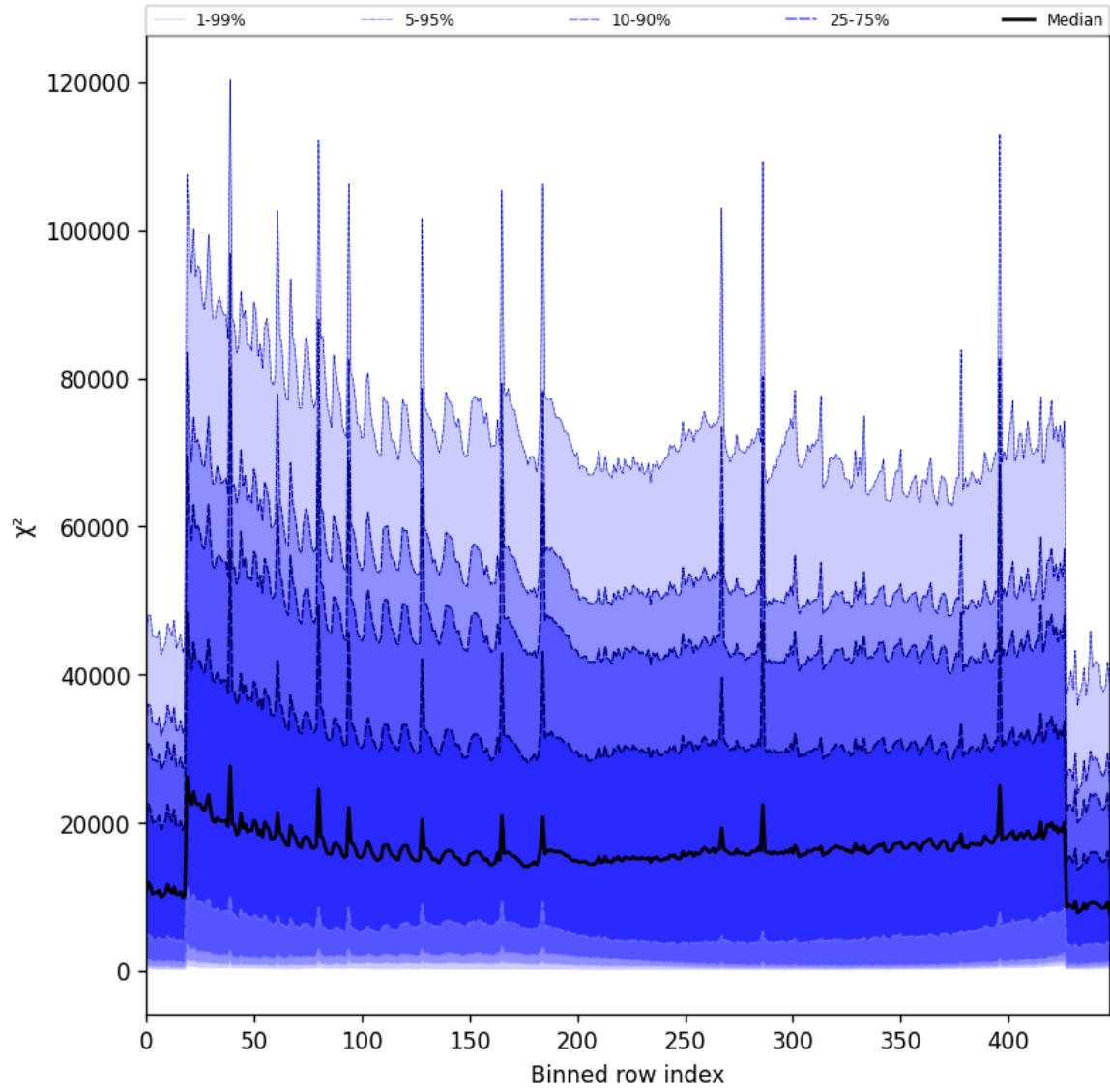
Figure 53: Along track statistics of “ \chi^2 ” for 2025-02-01 to 2025-02-02
