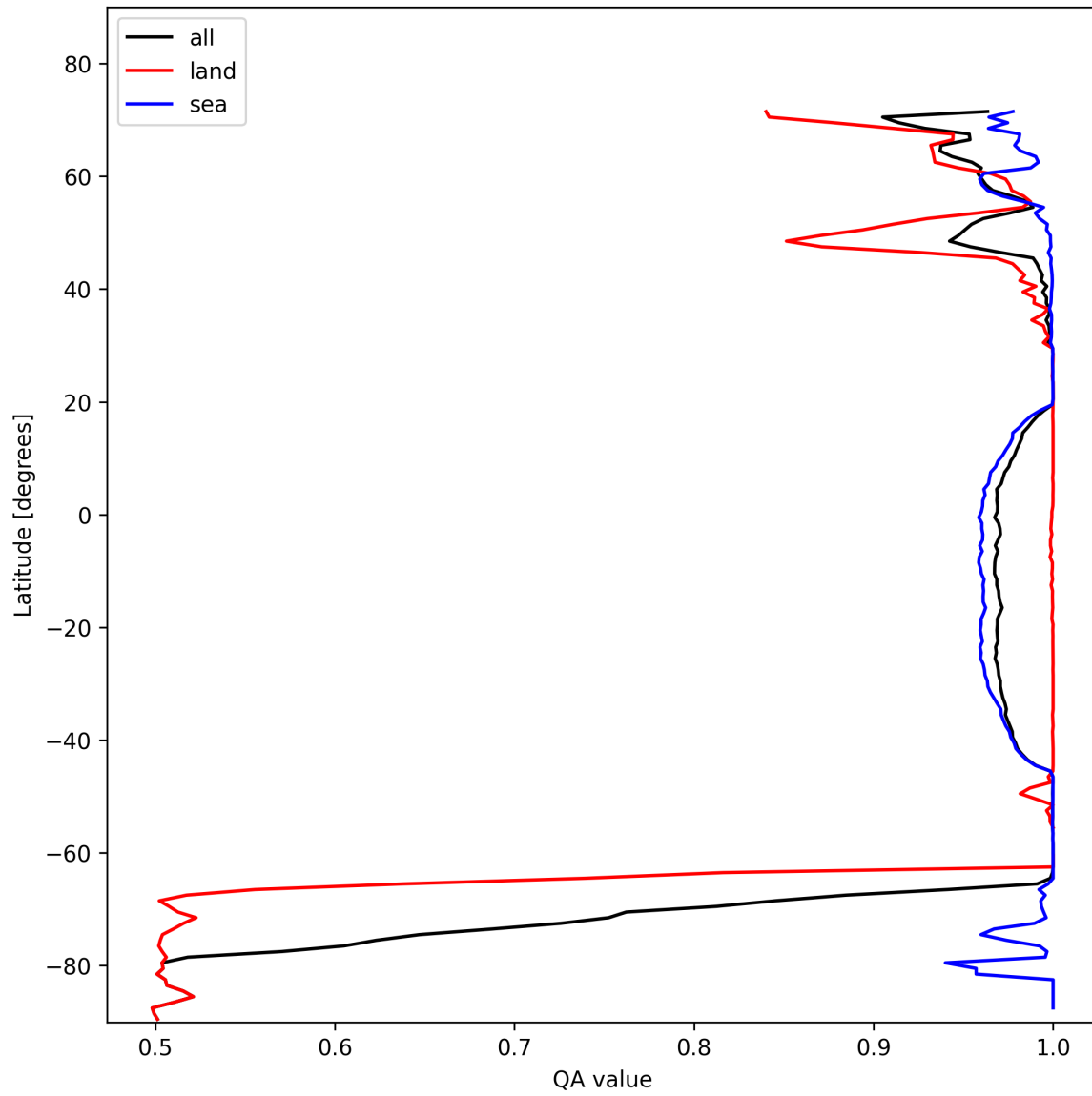
Figure 10: Zonal average of “QA value” for 2025-02-01 to 2025-02-02.
