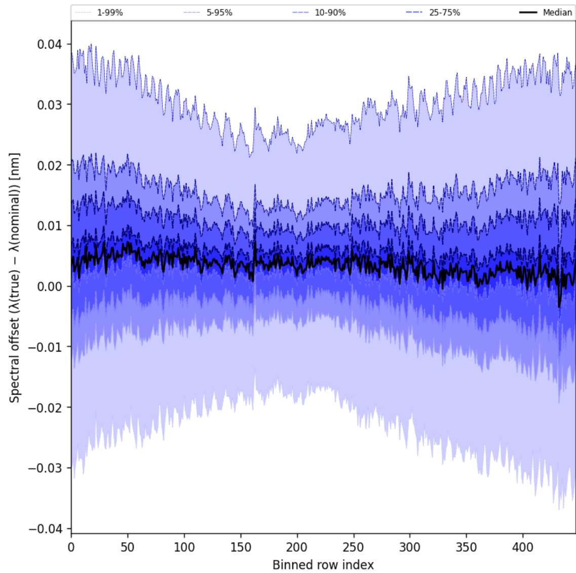
Figure 60: Along track statistics of “Spectral offset ( \lambda_{\text{true}} - \lambda_{\text{nominal}} )” for 2025-02-01 to 2025-02-02
