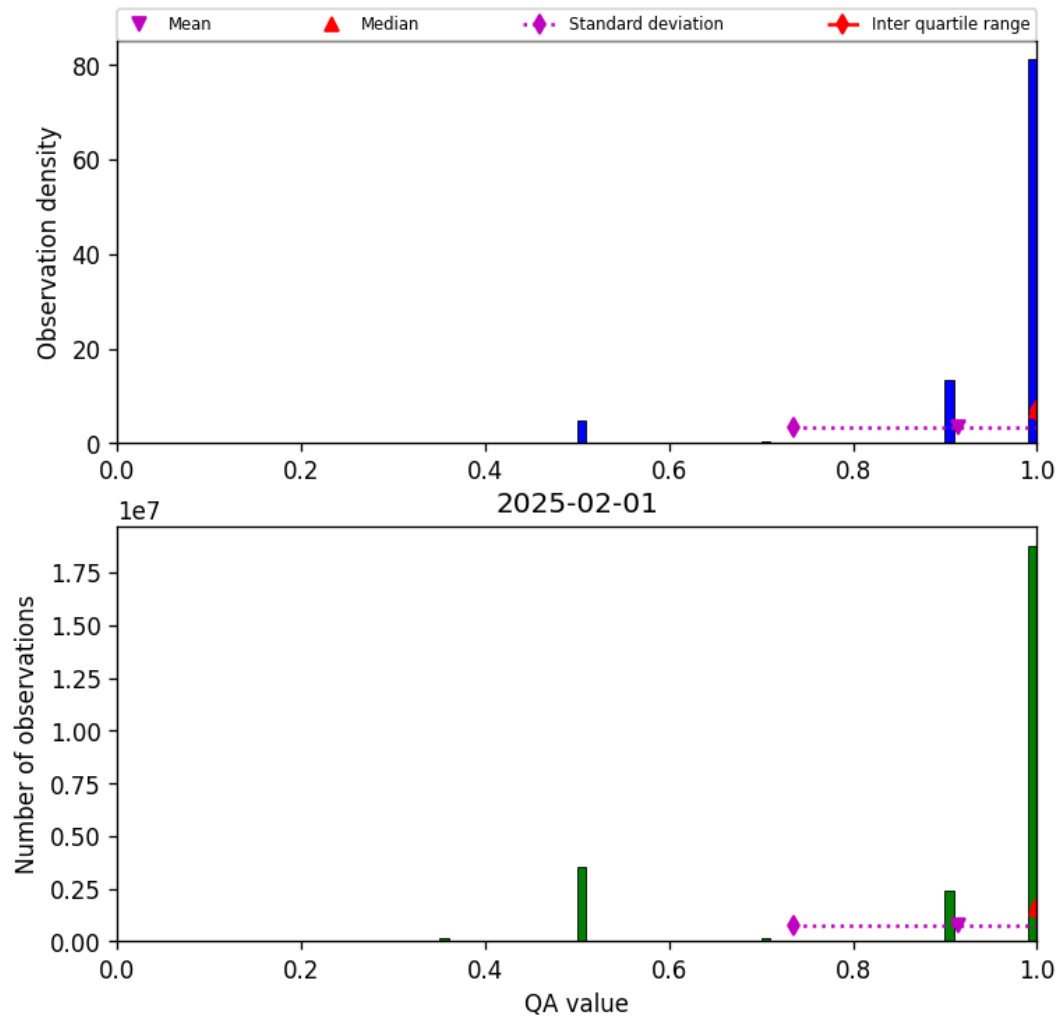
Figure 27: Histogram of “QA value” for 2025-02-01 to 2025-02-02
