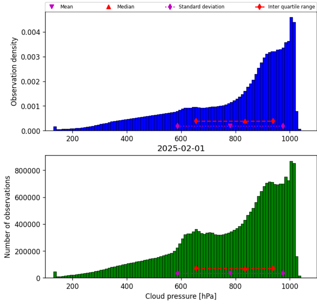
Figure 28: Histogram of “Cloud pressure” for 2025-02-01 to 2025-02-02
