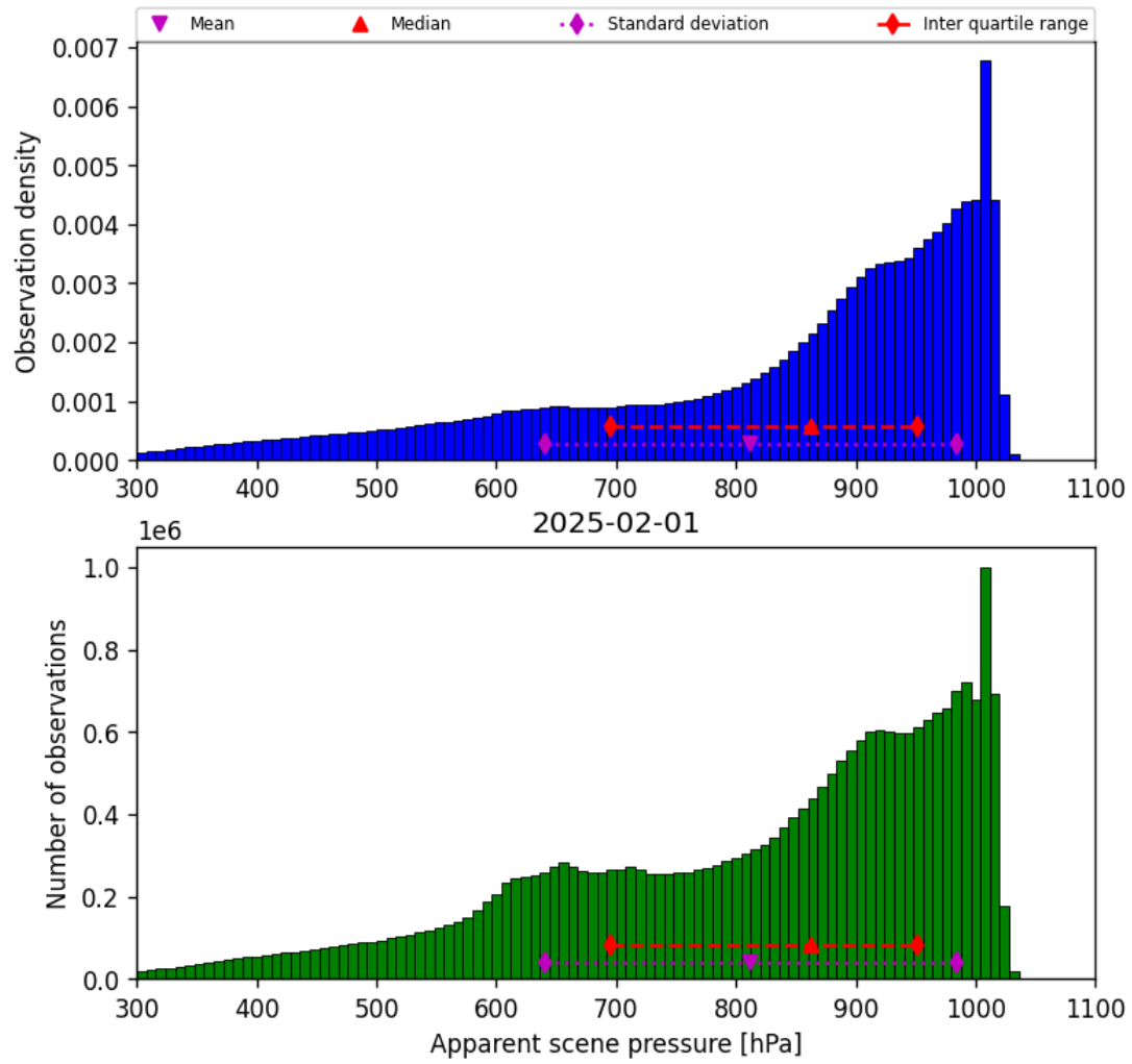
Figure 34: Histogram of “Apparent scene pressure” for 2025-02-01 to 2025-02-02
