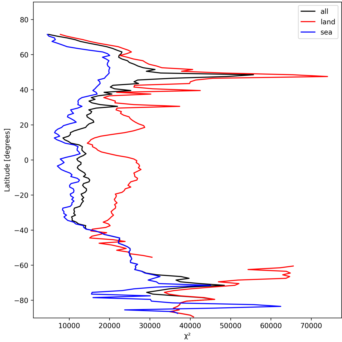
Figure 19: Zonal average of “ \chi^2 ” for 2025-02-01 to 2025-02-02.
