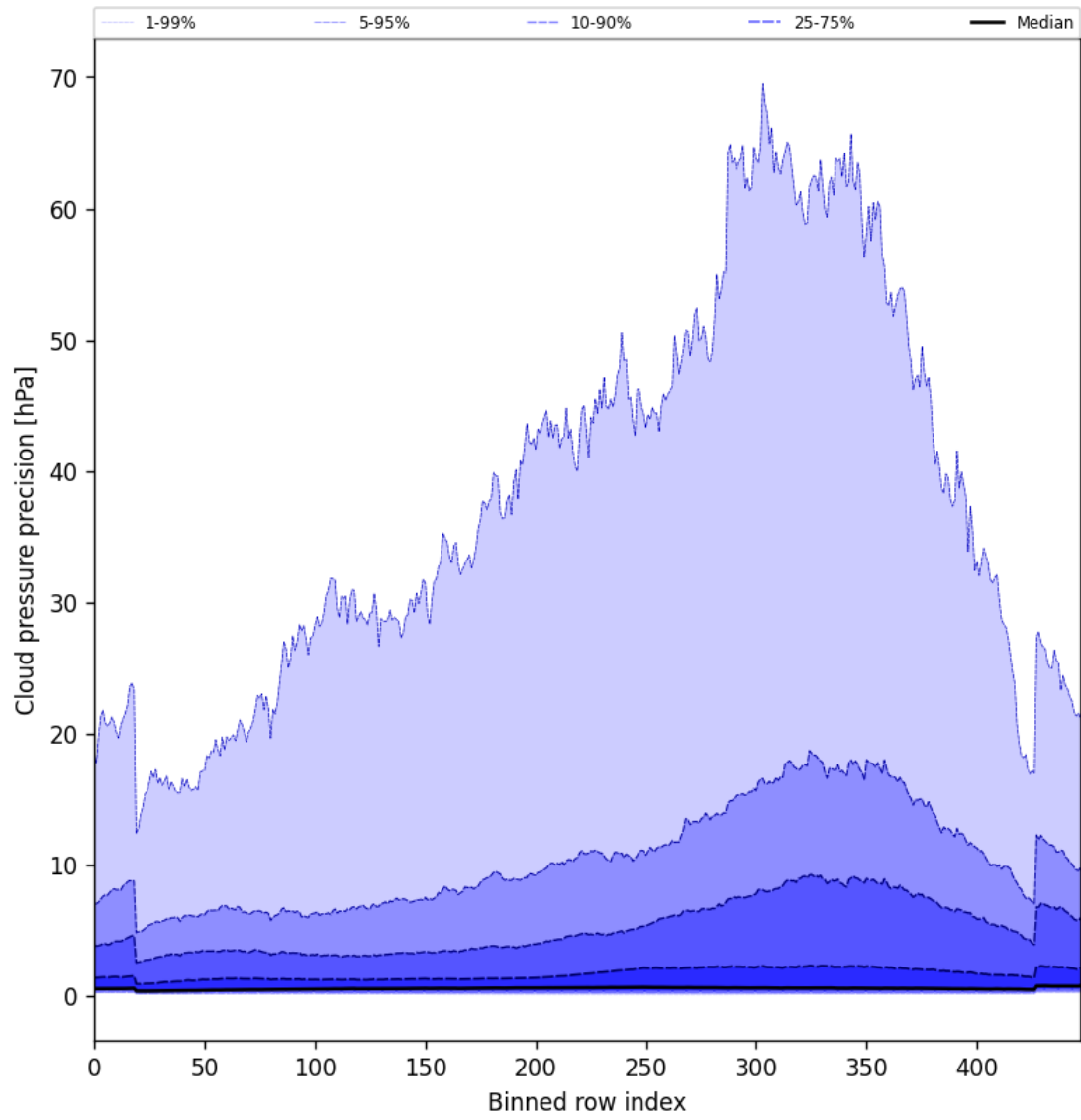
Figure 46: Along track statistics of “Cloud pressure precision” for 2025-02-01 to 2025-02-02
