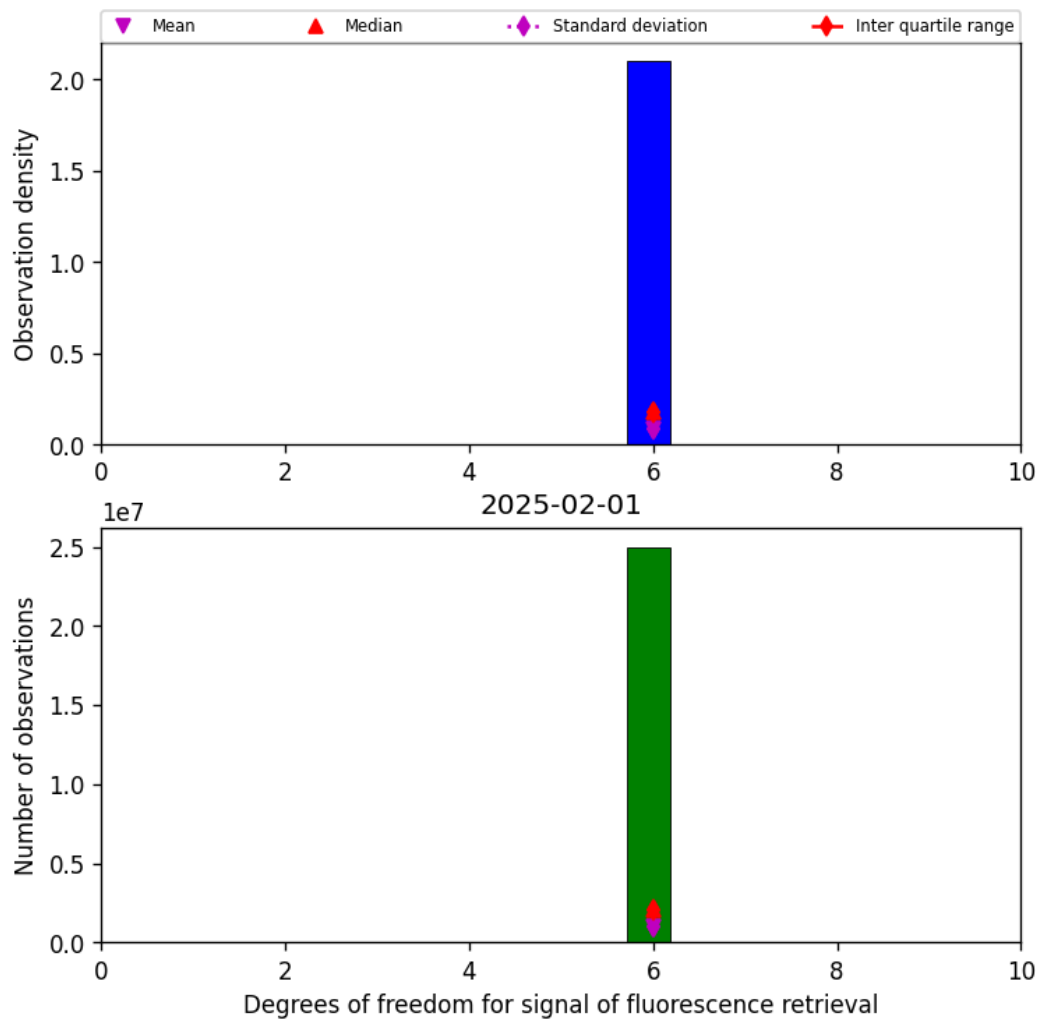
Figure 41: Histogram of “Degrees of freedom for signal of fluorescence retrieval” for 2025-02-01 to 2025-02-02
