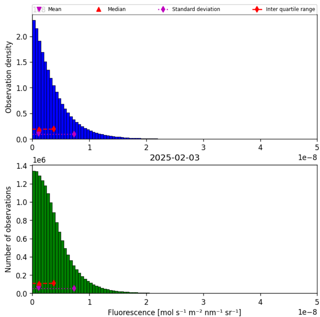
Figure 38: Histogram of “Fluorescence” for 2025-02-03 to 2025-02-04
