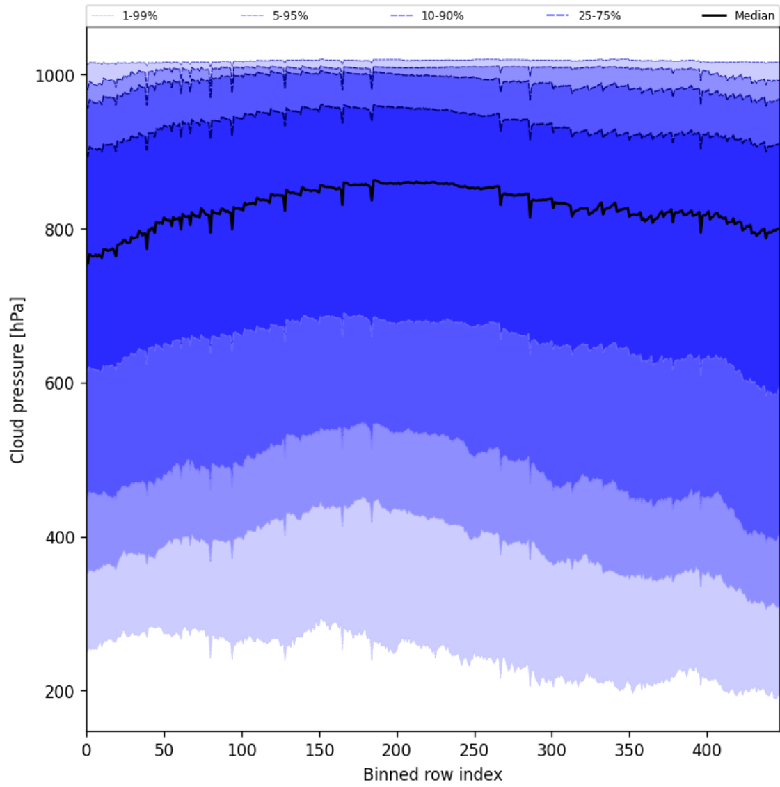
Figure 45: Along track statistics of “Cloud pressure” for 2025-02-03 to 2025-02-04
