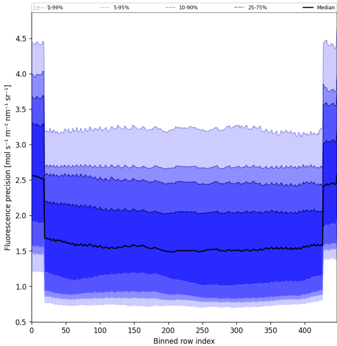
Figure 56: Along track statistics of “Fluorescence precision” for 2025-02-03 to 2025-02-04
