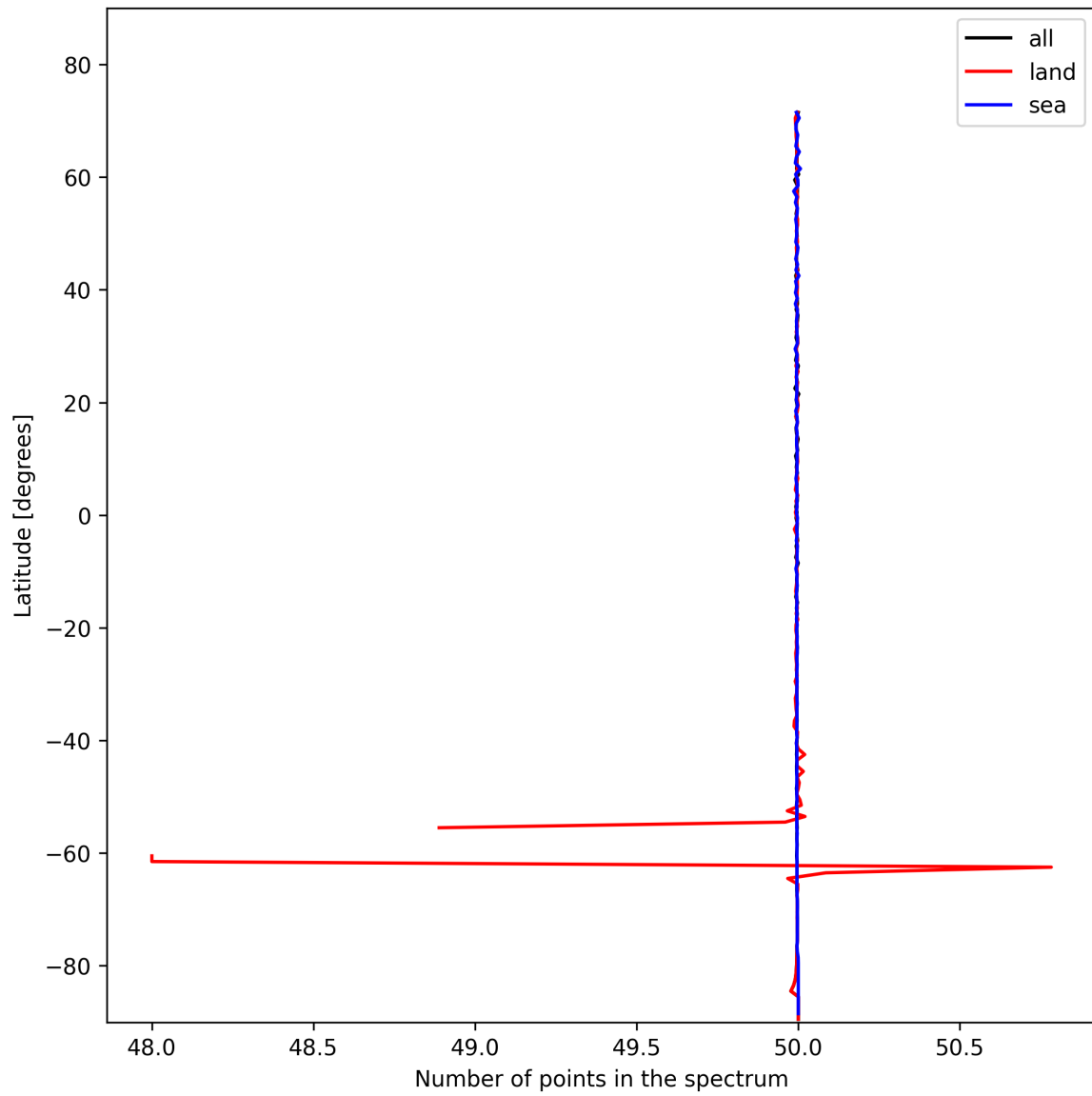
Figure 25: Zonal average of “Number of points in the spectrum” for 2025-02-03 to 2025-02-04.
