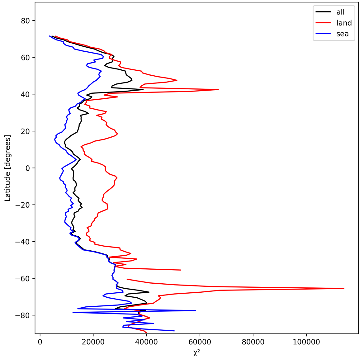
Figure 19: Zonal average of “ \chi^2 ” for 2025-02-03 to 2025-02-04.
