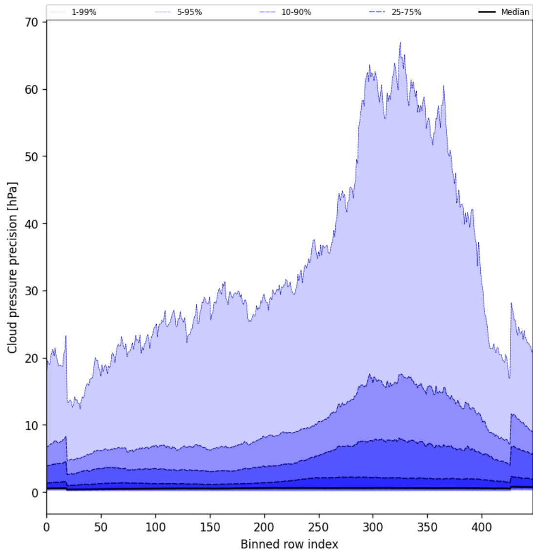
Figure 46: Along track statistics of “Cloud pressure precision” for 2025-02-03 to 2025-02-04
