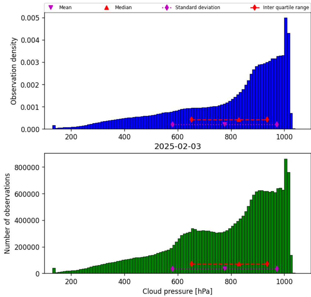
Figure 28: Histogram of “Cloud pressure” for 2025-02-03 to 2025-02-04
