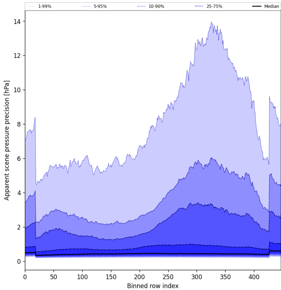
Figure 52: Along track statistics of “Apparent scene pressure precision” for 2025-02-03 to 2025-02-04
