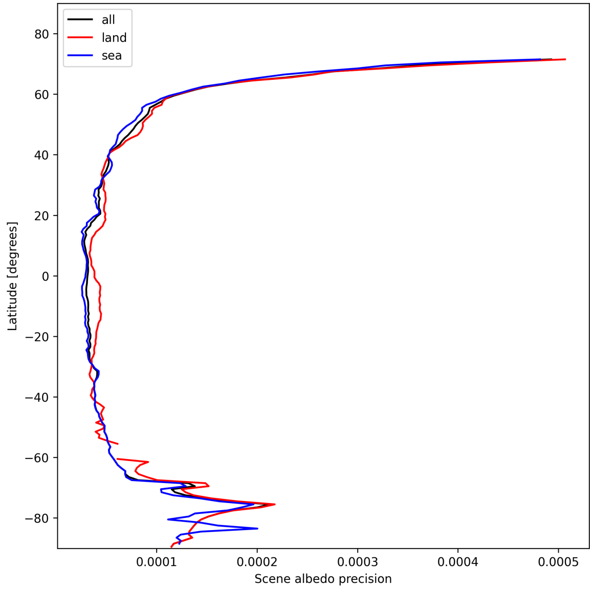
Figure 16: Zonal average of “Scene albedo precision” for 2025-02-03 to 2025-02-04.
