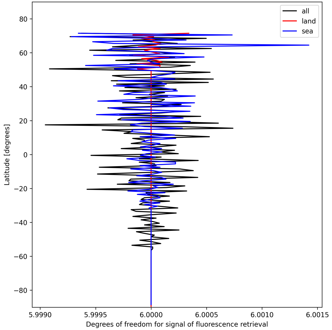
Figure 24: Zonal average of “Degrees of freedom for signal of fluorescence retrieval” for 2025-02-03 to 2025-02-04.
