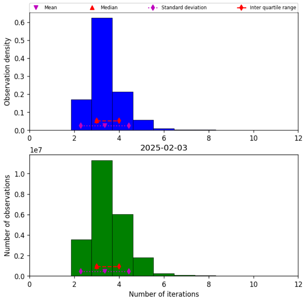
Figure 37: Histogram of “Number of iterations” for 2025-02-03 to 2025-02-04
