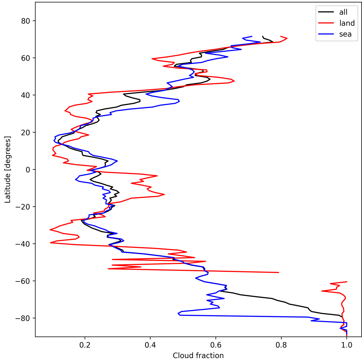
Figure 13: Zonal average of “Cloud fraction” for 2025-02-03 to 2025-02-04.
