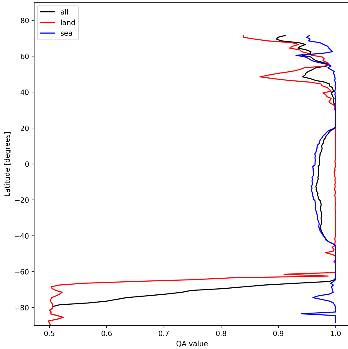
Figure 10: Zonal average of “QA value” for 2025-02-03 to 2025-02-04.
