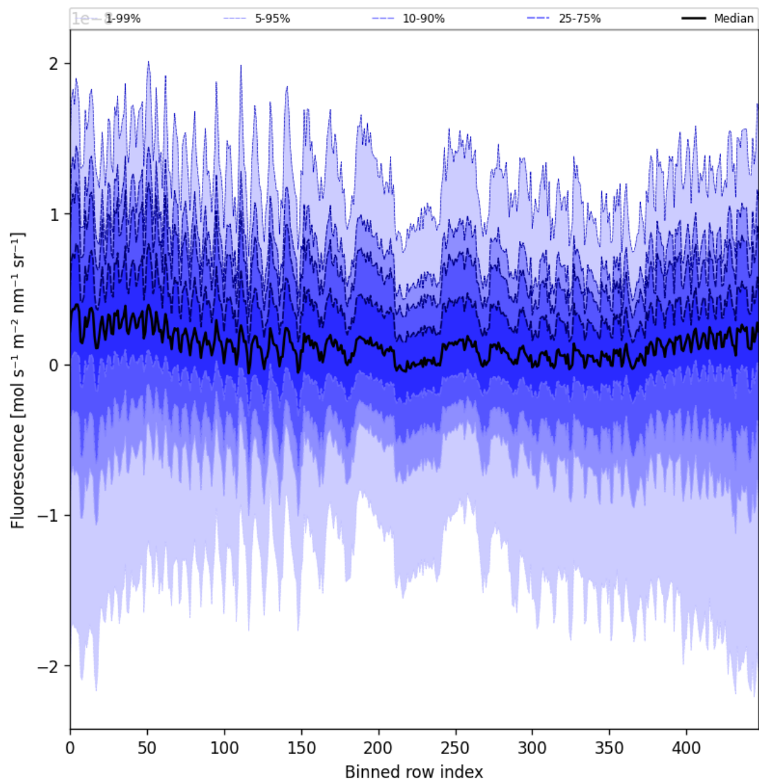
Figure 55: Along track statistics of “Fluorescence” for 2025-02-03 to 2025-02-04
