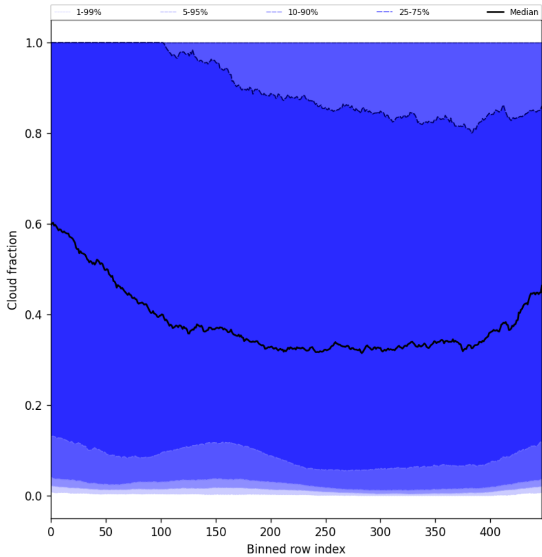
Figure 47: Along track statistics of “Cloud fraction” for 2025-02-03 to 2025-02-04
