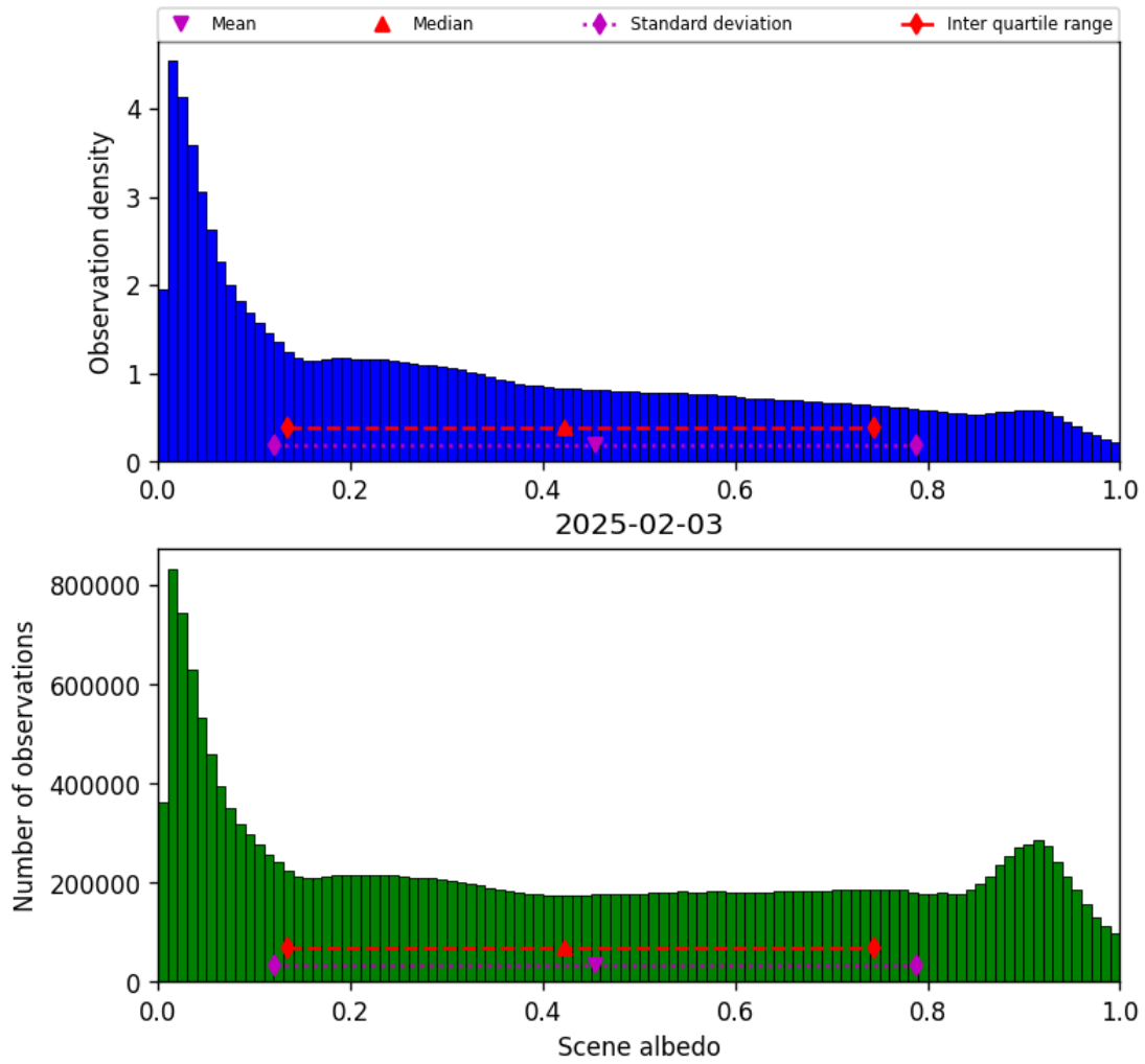
Figure 32: Histogram of “Scene albedo” for 2025-02-03 to 2025-02-04
