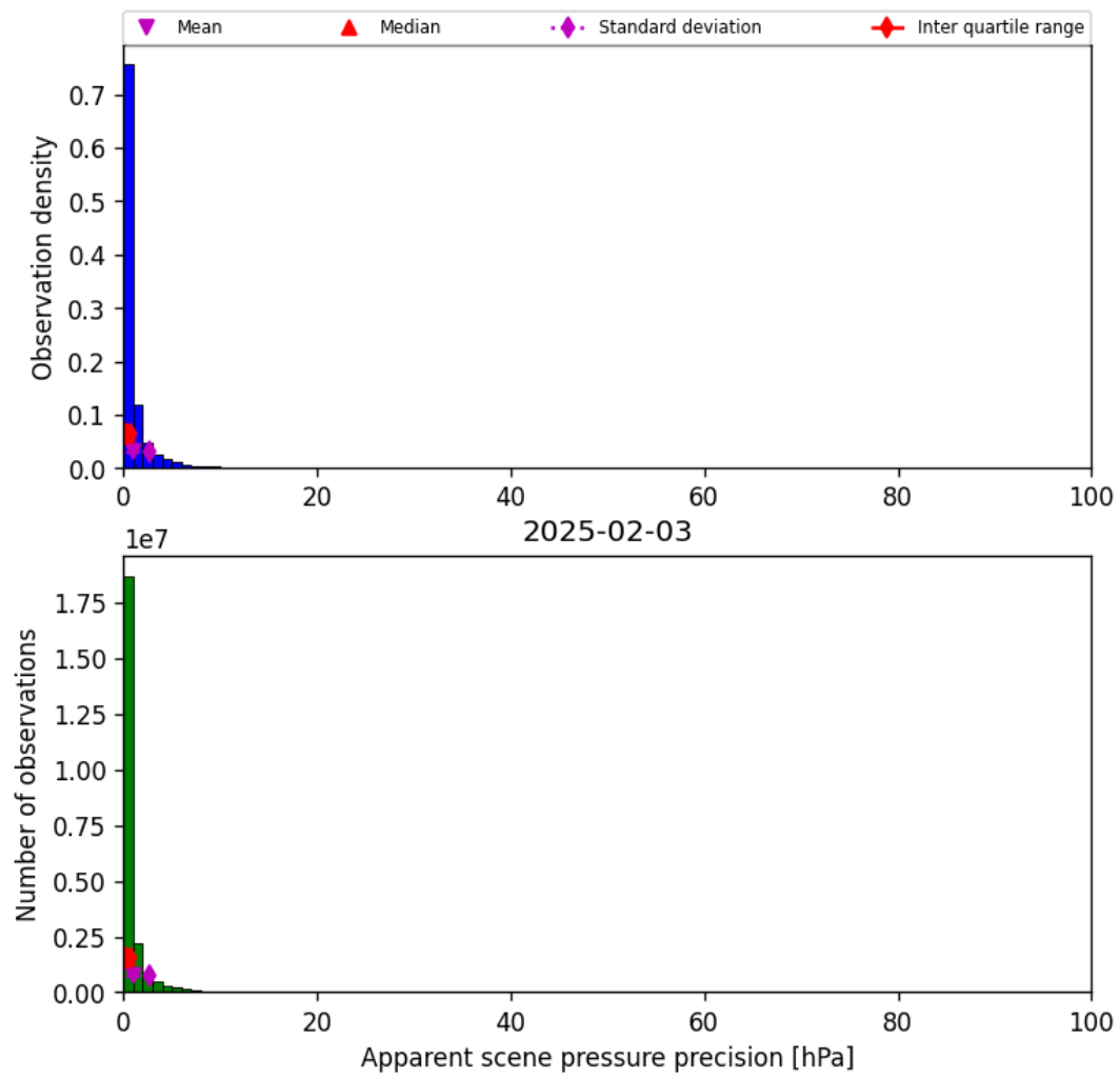
Figure 35: Histogram of “Apparent scene pressure precision” for 2025-02-03 to 2025-02-04
