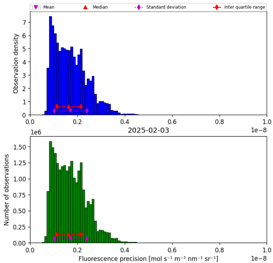
Figure 39: Histogram of “Fluorescence precision” for 2025-02-03 to 2025-02-04
