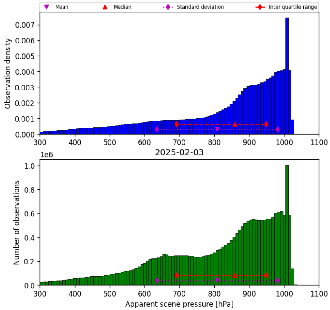
Figure 34: Histogram of “Apparent scene pressure” for 2025-02-03 to 2025-02-04
