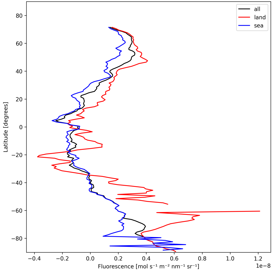
Figure 21: Zonal average of “Fluorescence” for 2025-02-03 to 2025-02-04.
