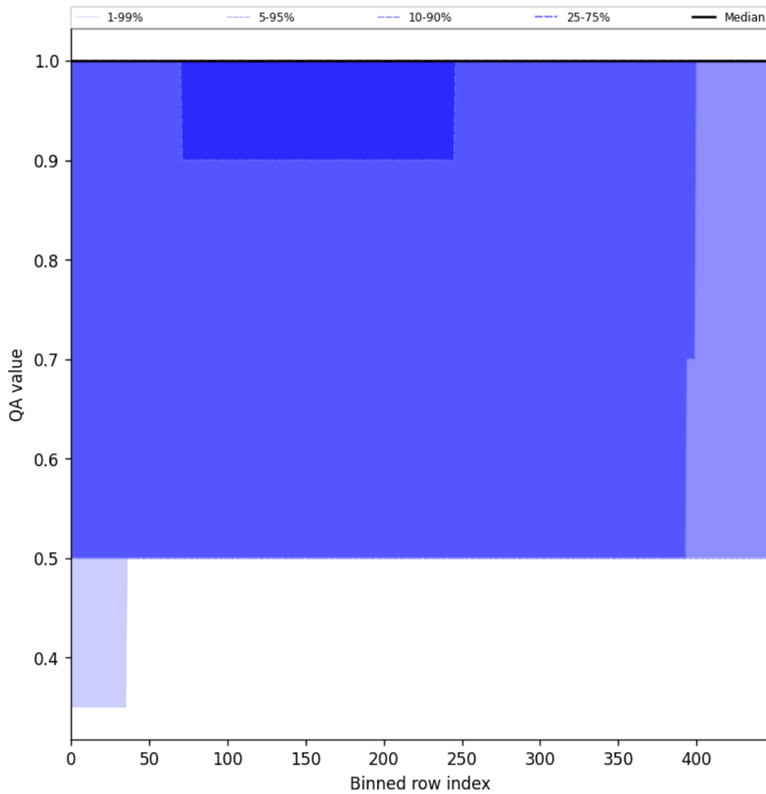
Figure 44: Along track statistics of “QA value” for 2025-02-03 to 2025-02-04
