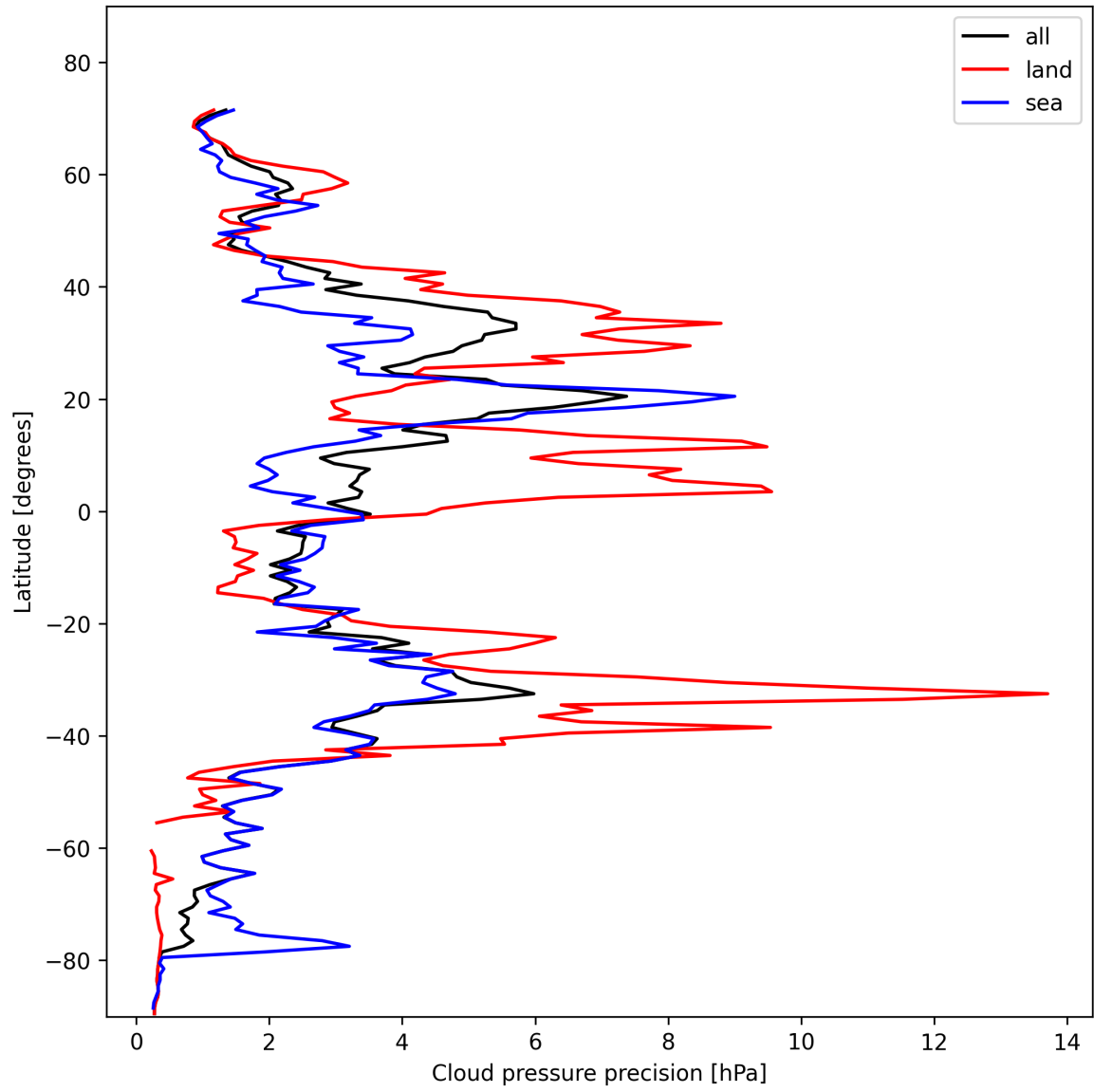
Figure 12: Zonal average of "Cloud pressure precision" for 2025-02-03 to 2025-02-04.
