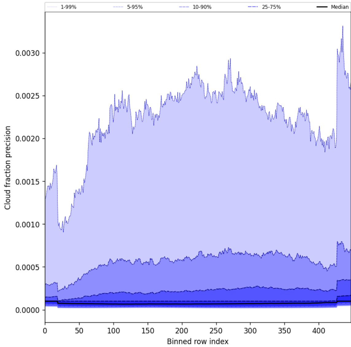
Figure 48: Along track statistics of “Cloud fraction precision” for 2025-02-03 to 2025-02-04
