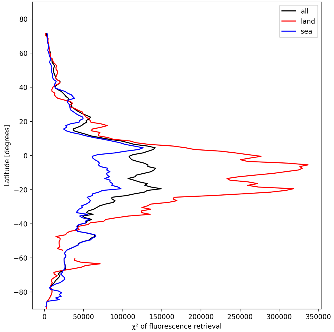
Figure 23: Zonal average of “ \chi^2 of fluorescence retrieval” for 2025-02-03 to 2025-02-04.
