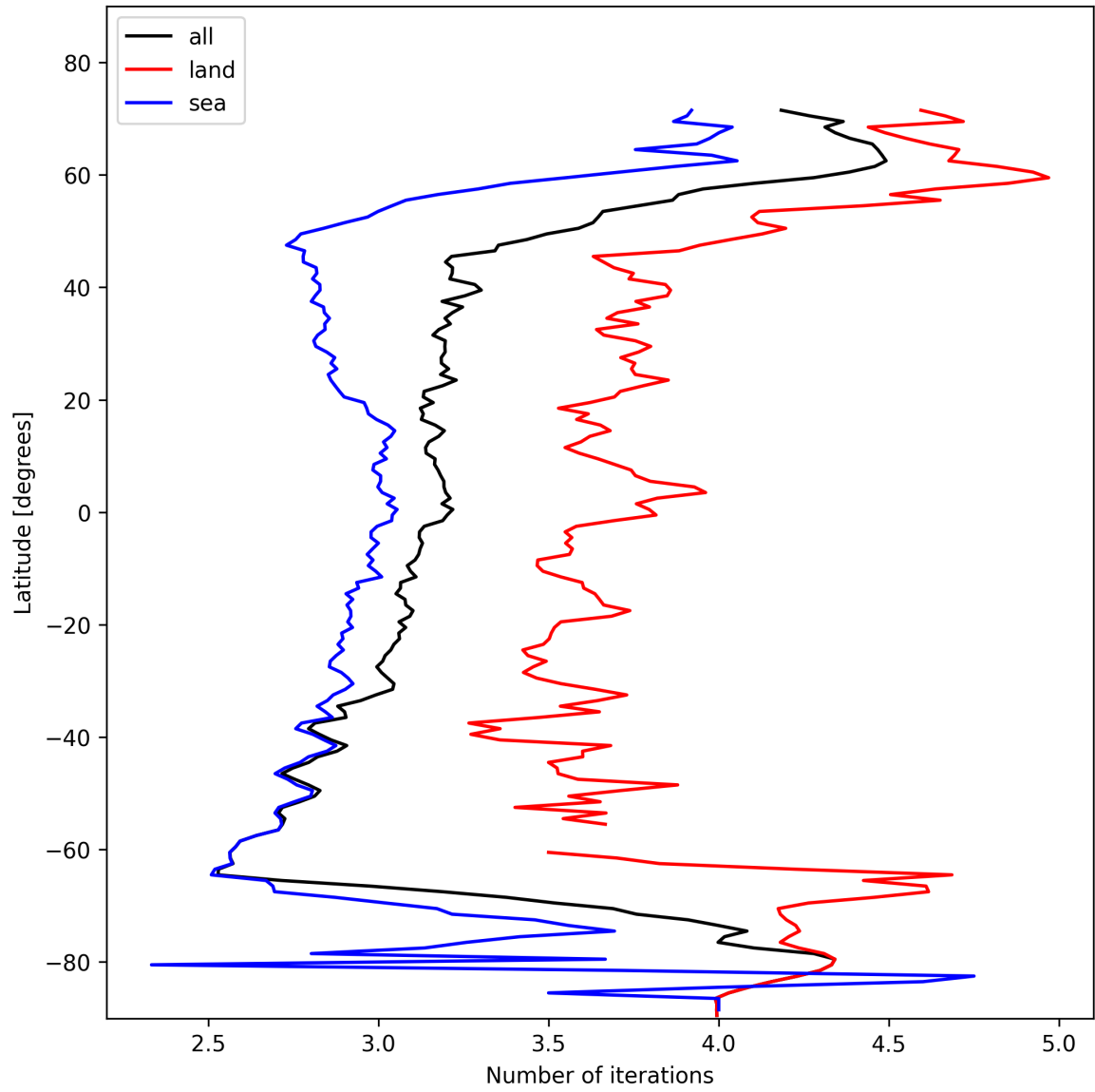
Figure 20: Zonal average of “Number of iterations” for 2025-02-03 to 2025-02-04.
