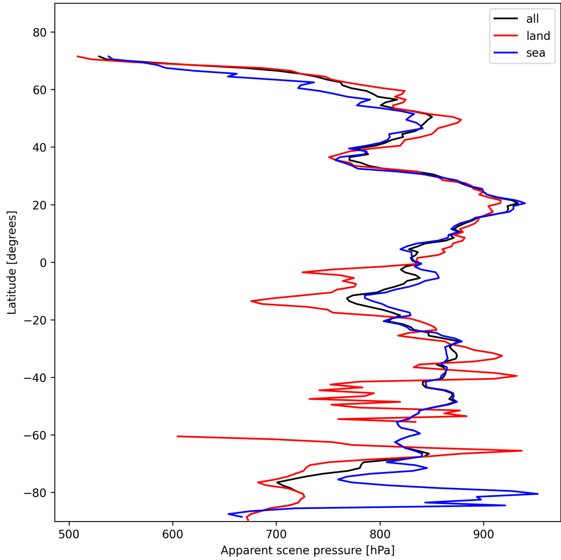
Figure 17: Zonal average of “Apparent scene pressure” for 2025-02-03 to 2025-02-04.
