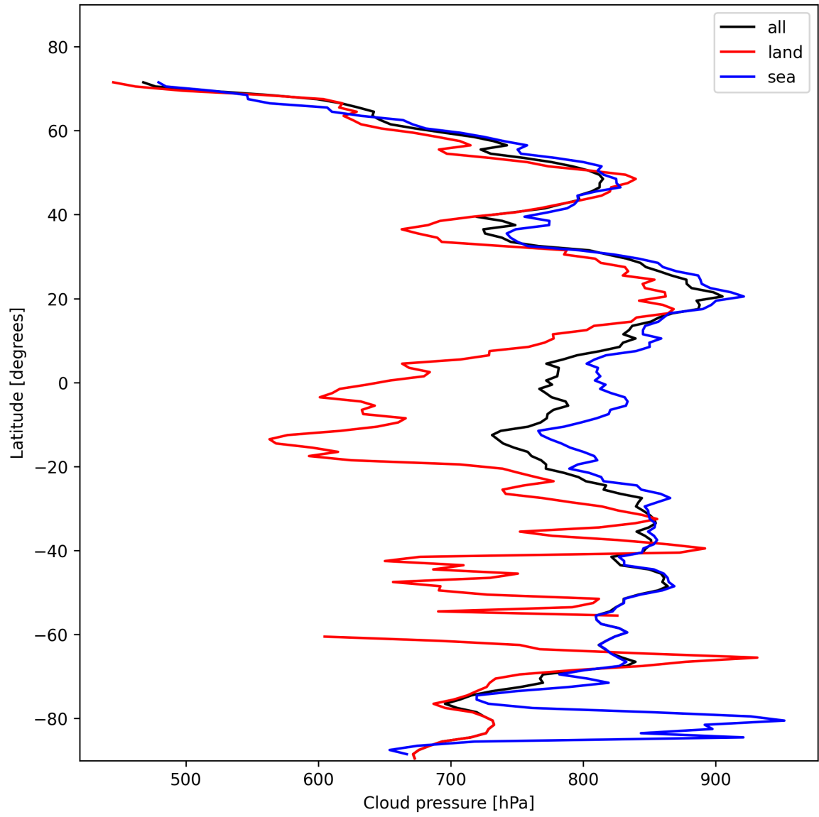
Figure 11: Zonal average of “Cloud pressure” for 2025-02-03 to 2025-02-04.
