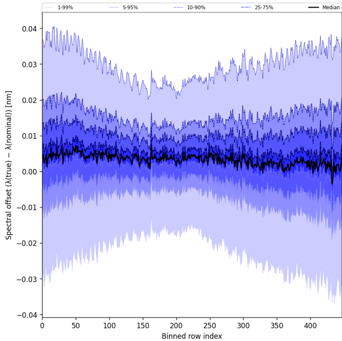
Figure 60: Along track statistics of “Spectral offset ( \lambda_{\text{true}} - \lambda_{\text{nominal}} )” for 2025-02-03 to 2025-02-04
