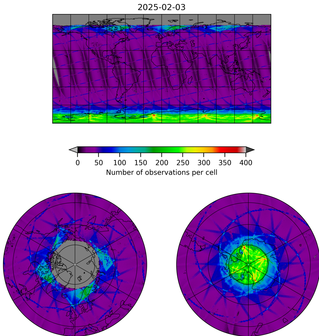
Figure 9: Map of the number of observations for 2025-02-03 to 2025-02-04
