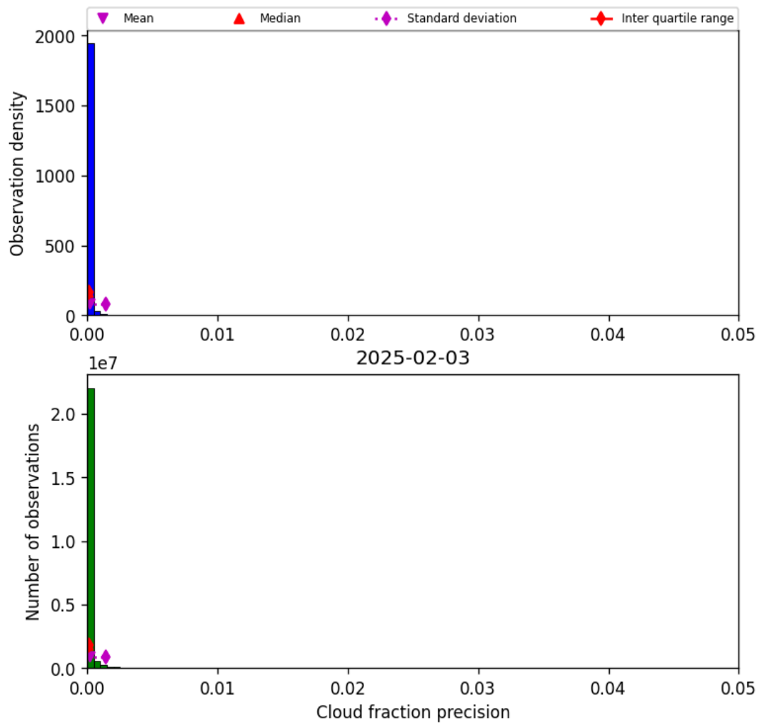
Figure 31: Histogram of “Cloud fraction precision” for 2025-02-03 to 2025-02-04
