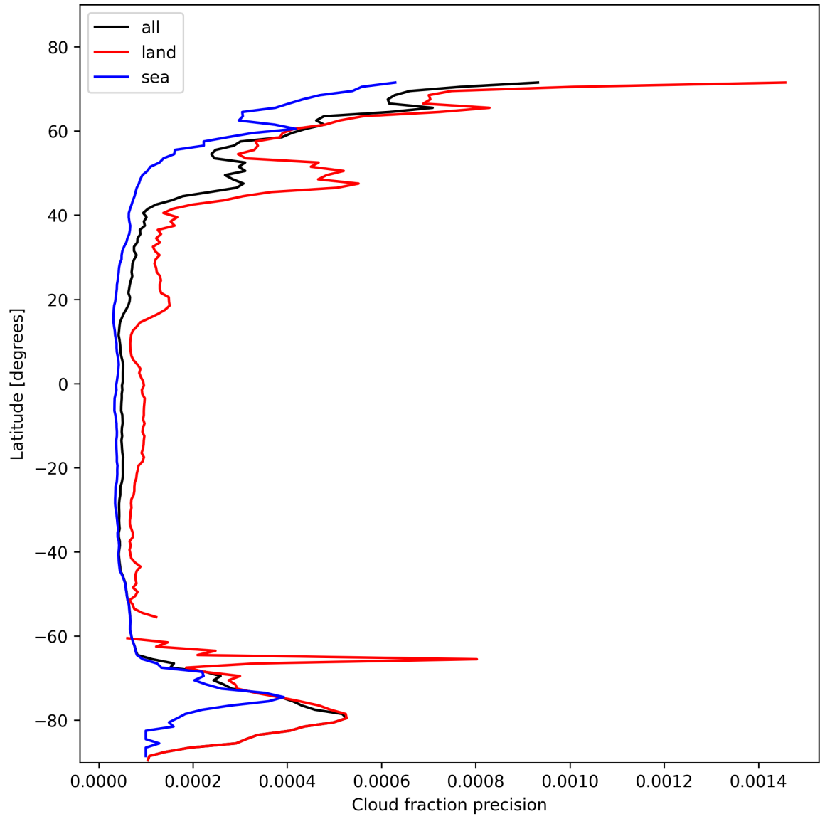
Figure 14: Zonal average of “Cloud fraction precision” for 2025-02-03 to 2025-02-04.
