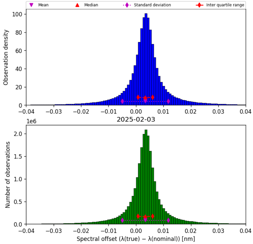
Figure 43: Histogram of “Spectral offset ( \lambda_{\text{true}} - \lambda_{\text{nominal}} )” for 2025-02-03 to 2025-02-04
