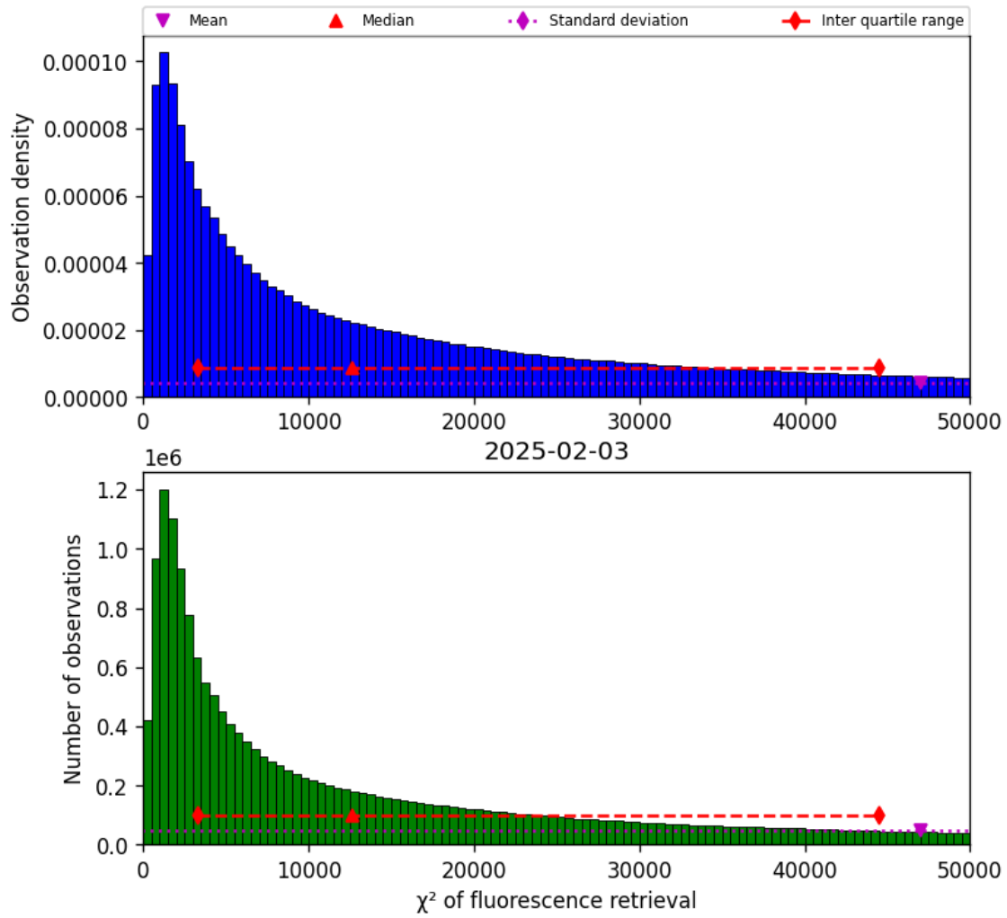
Figure 40: Histogram of “ \chi^2 of fluorescence retrieval” for 2025-02-03 to 2025-02-04
