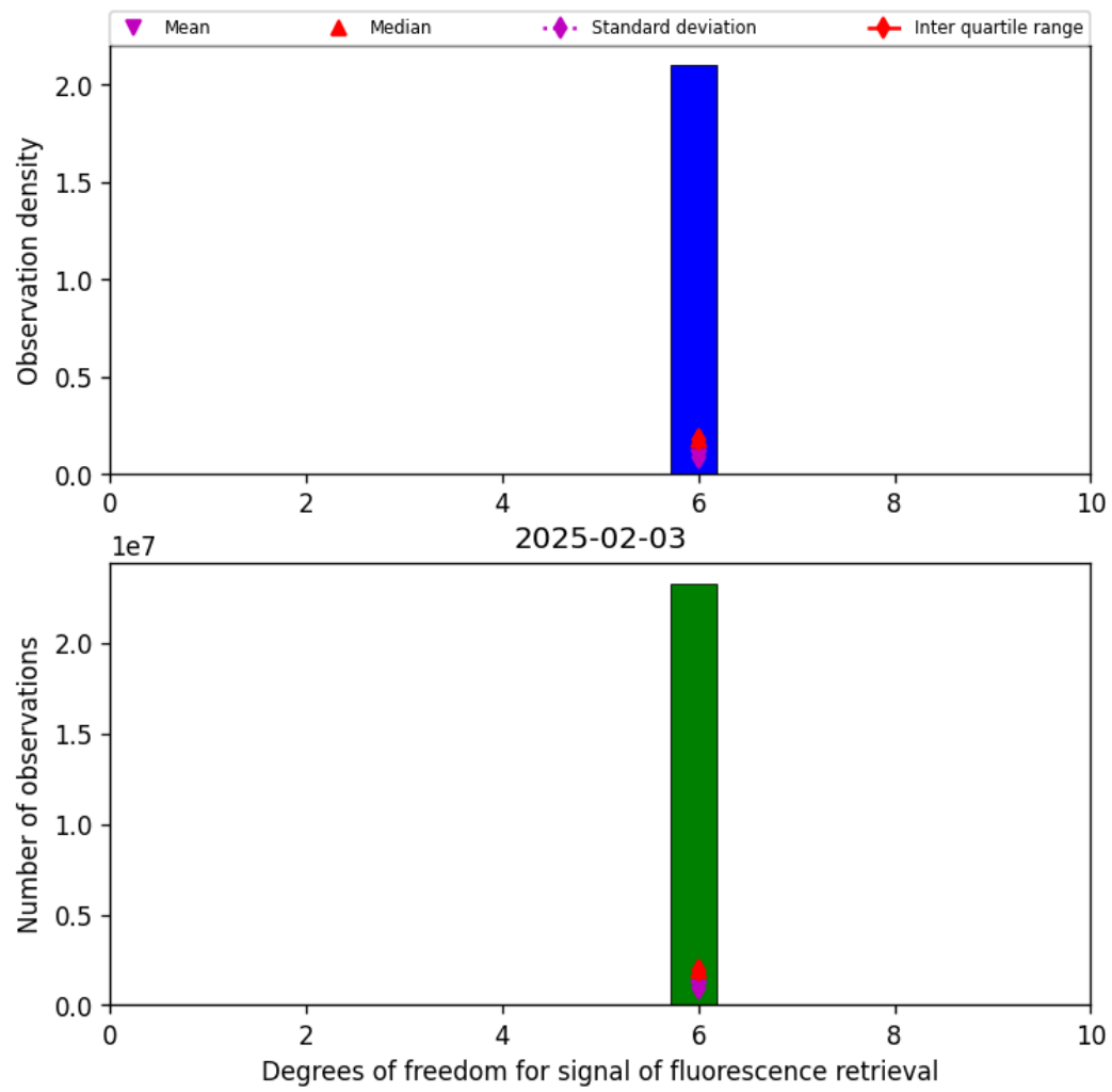
Figure 41: Histogram of “Degrees of freedom for signal of fluorescence retrieval” for 2025-02-03 to 2025-02-04
