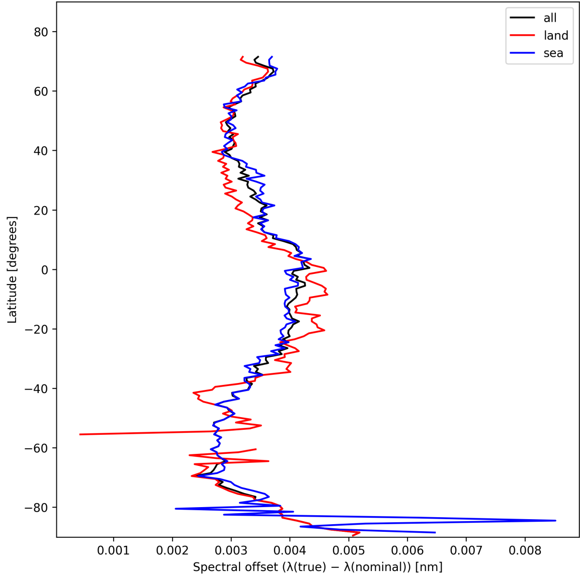
Figure 26: Zonal average of “Spectral offset ( \lambda_{\text{true}} - \lambda_{\text{nominal}} )” for 2025-02-03 to 2025-02-04.
