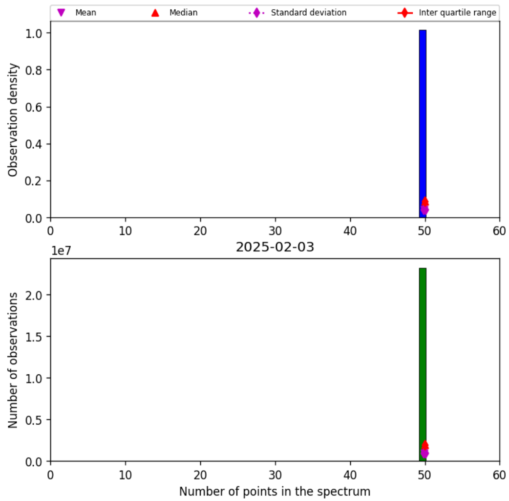
Figure 42: Histogram of “Number of points in the spectrum” for 2025-02-03 to 2025-02-04
