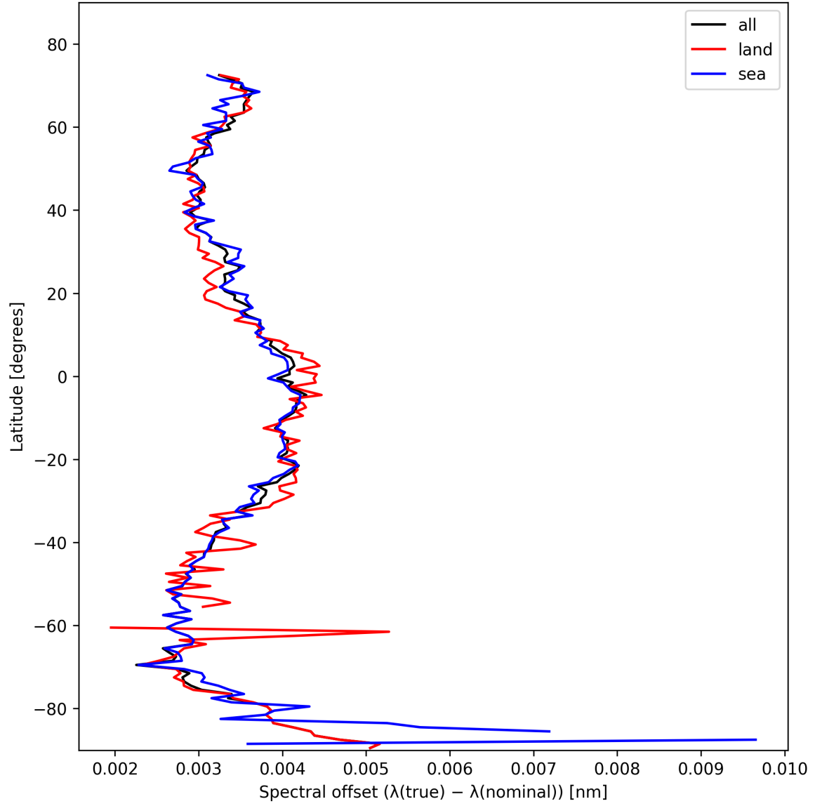
Figure 26: Zonal average of “Spectral offset ( \lambda_{\text{true}} - \lambda_{\text{nominal}} )” for 2025-02-05 to 2025-02-06.
