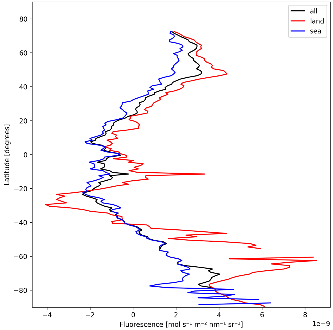
Figure 21: Zonal average of “Fluorescence” for 2025-02-05 to 2025-02-06.
