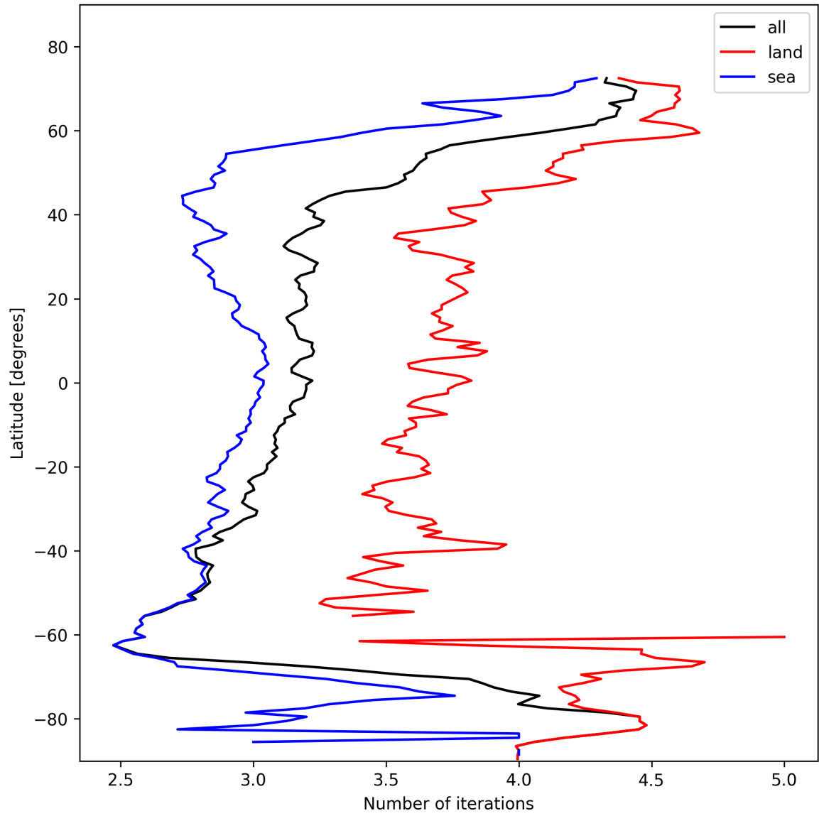
Figure 20: Zonal average of “Number of iterations” for 2025-02-05 to 2025-02-06.
