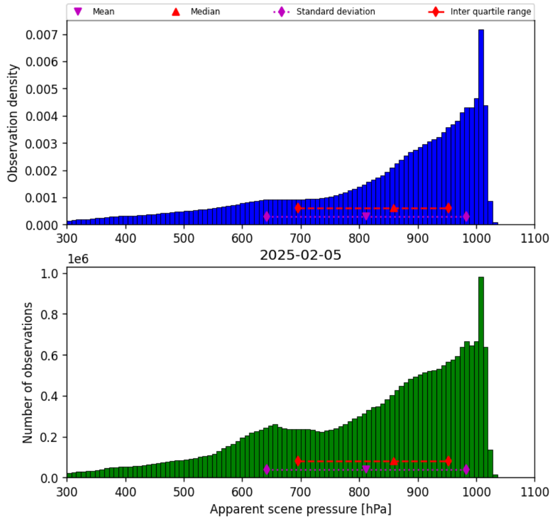
Figure 34: Histogram of “Apparent scene pressure” for 2025-02-05 to 2025-02-06
