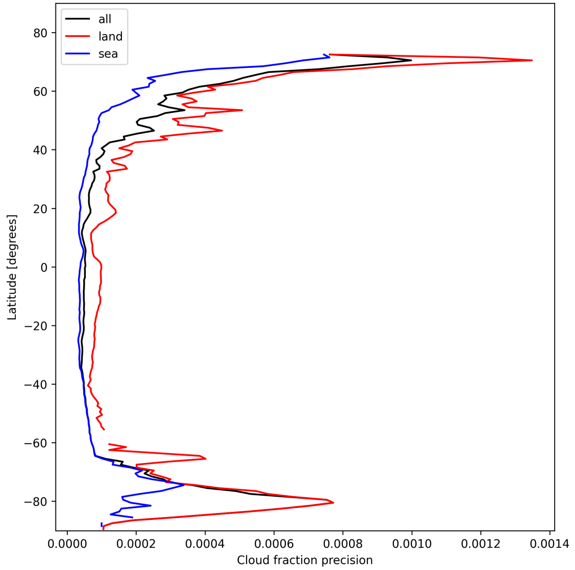
Figure 14: Zonal average of “Cloud fraction precision” for 2025-02-05 to 2025-02-06.
