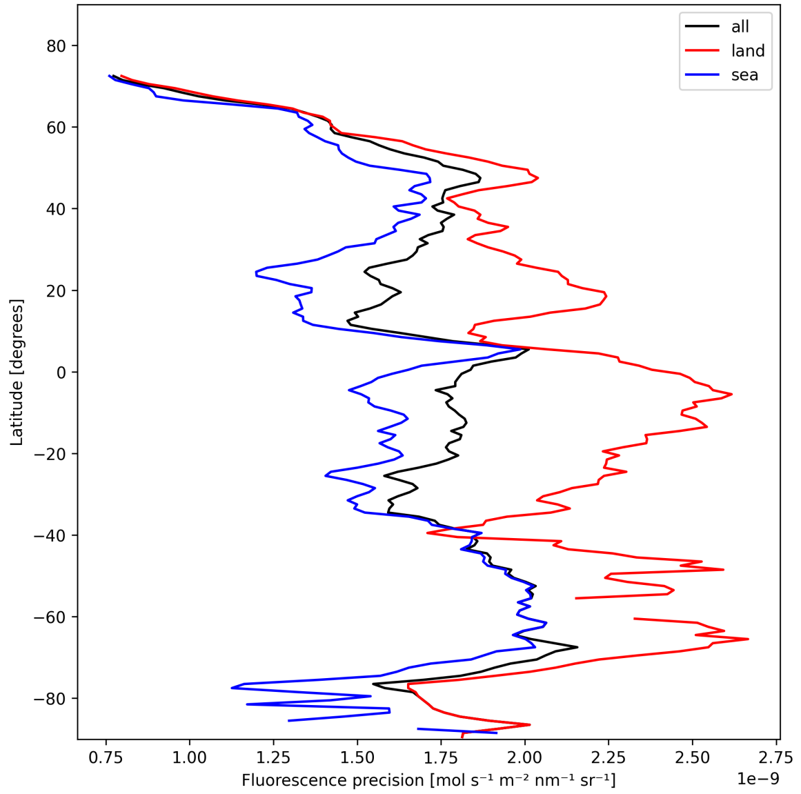
Figure 22: Zonal average of “Fluorescence precision” for 2025-02-05 to 2025-02-06.
