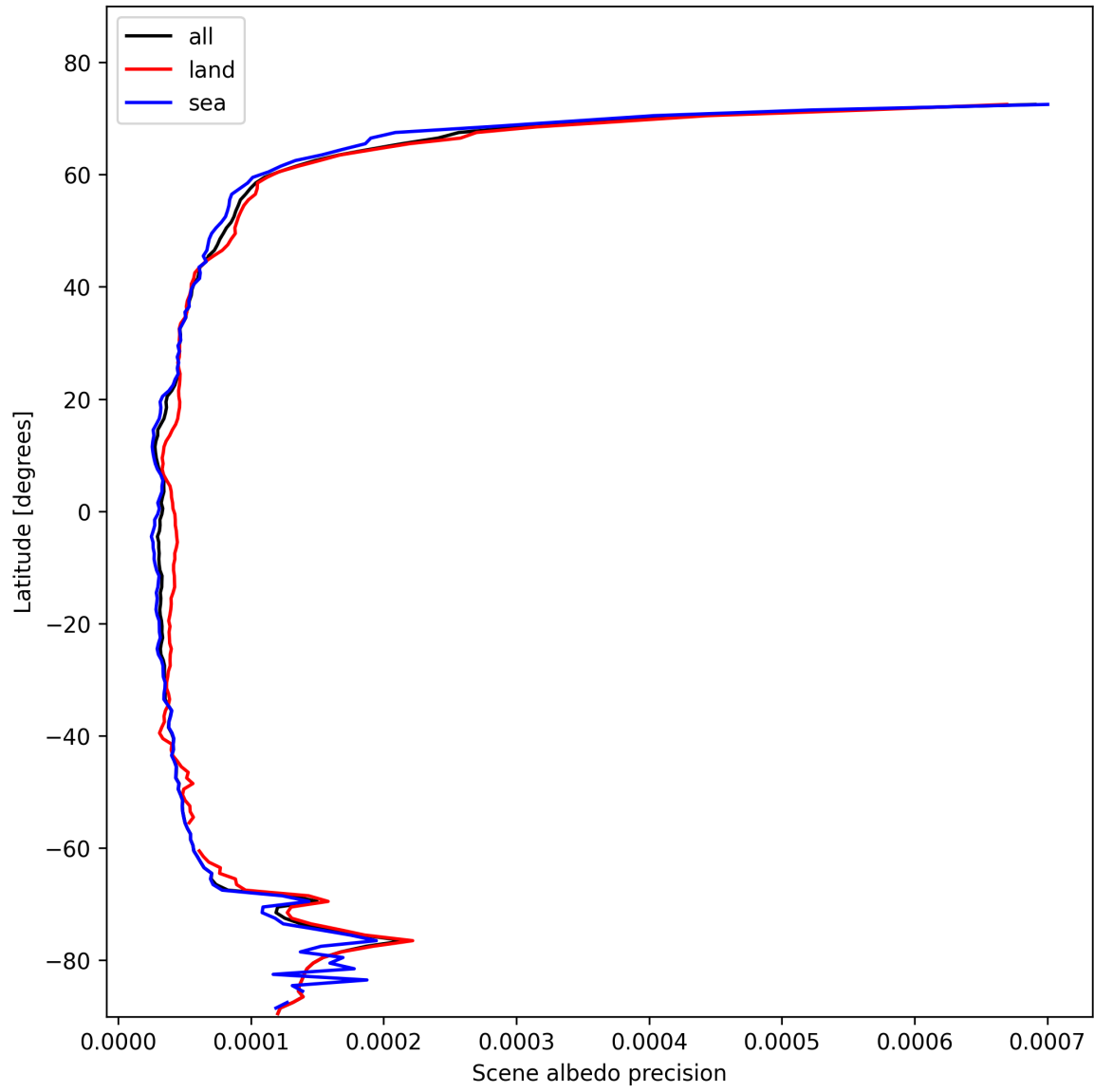
Figure 16: Zonal average of “Scene albedo precision” for 2025-02-05 to 2025-02-06.
