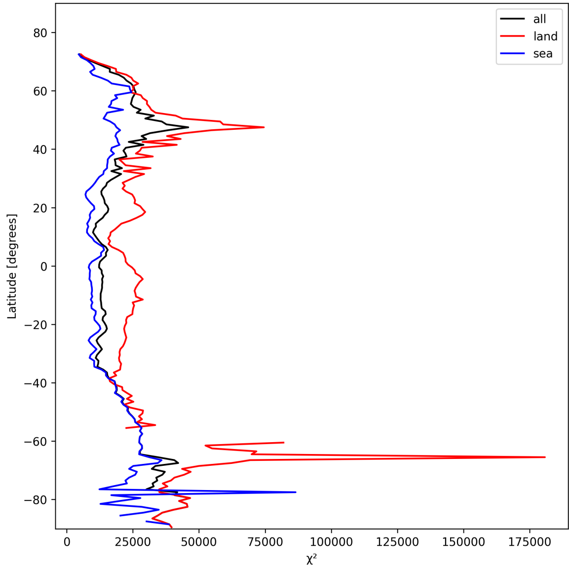
Figure 19: Zonal average of “ \chi^2 ” for 2025-02-05 to 2025-02-06.
