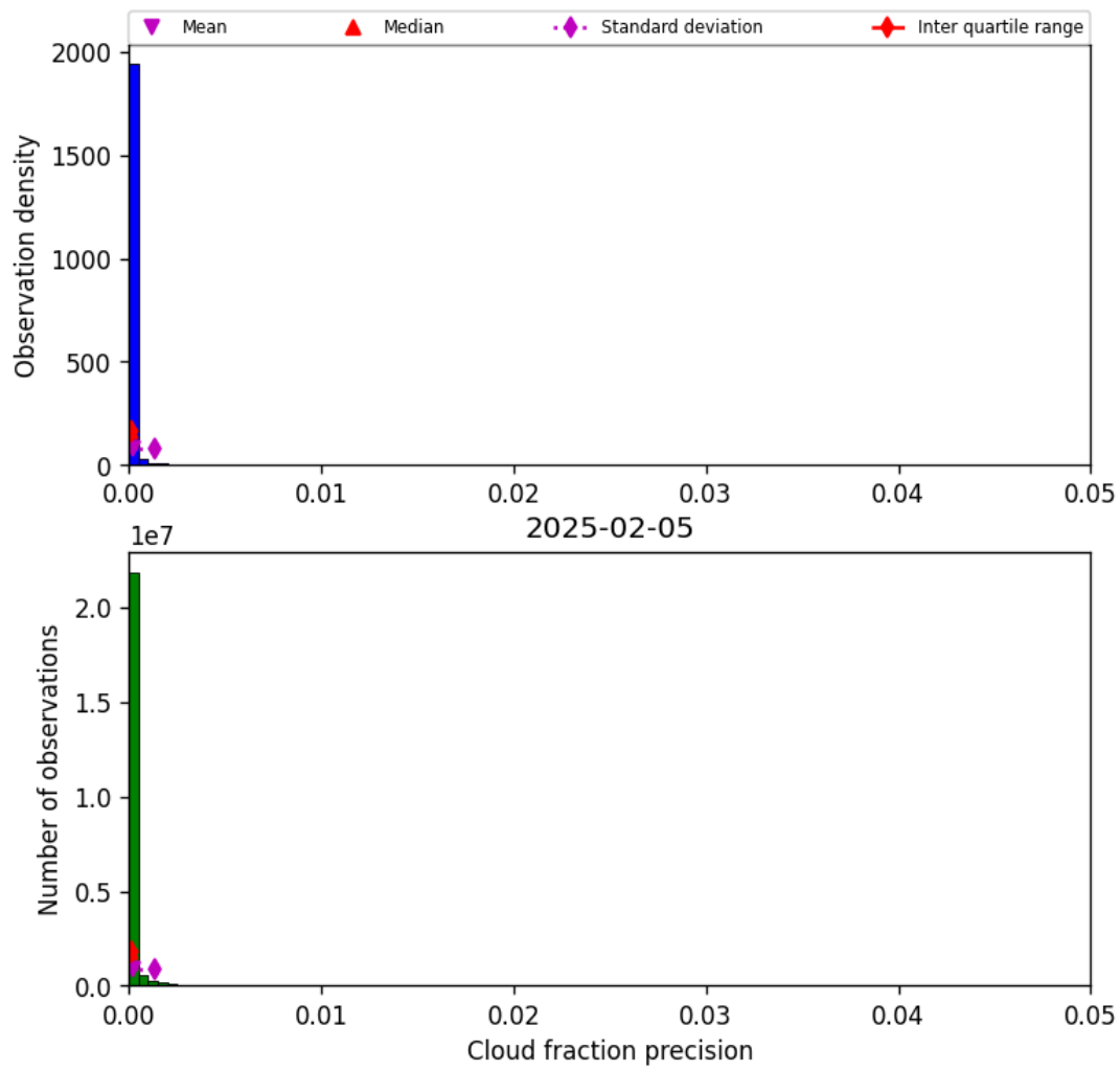
Figure 31: Histogram of “Cloud fraction precision” for 2025-02-05 to 2025-02-06
