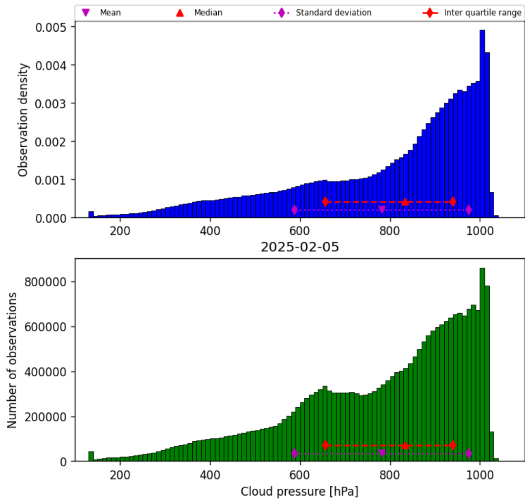
Figure 28: Histogram of “Cloud pressure” for 2025-02-05 to 2025-02-06
