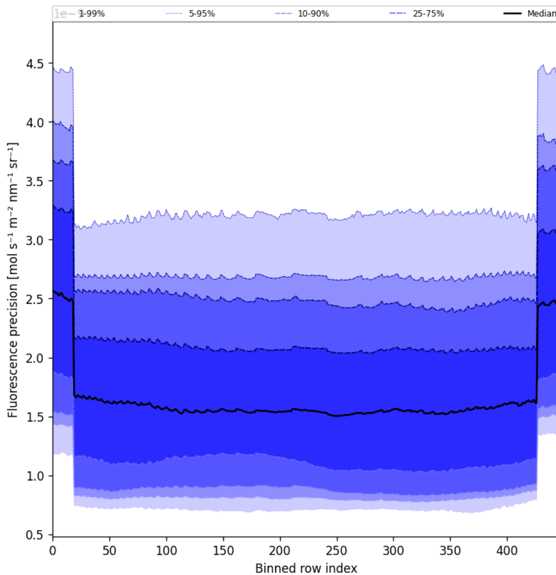
Figure 56: Along track statistics of “Fluorescence precision” for 2025-02-05 to 2025-02-06
