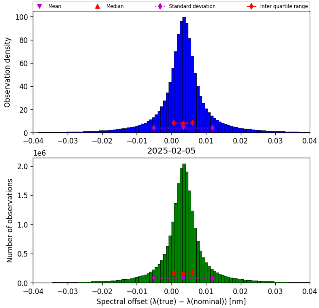
Figure 43: Histogram of “Spectral offset ( \lambda_{\text{true}} - \lambda_{\text{nominal}} )” for 2025-02-05 to 2025-02-06
