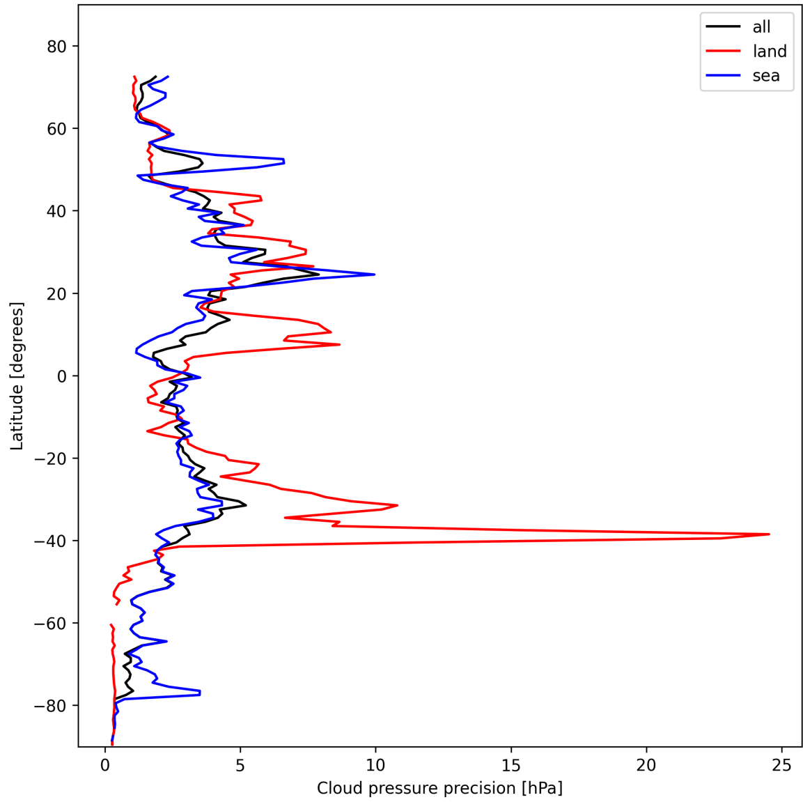
Figure 12: Zonal average of “Cloud pressure precision” for 2025-02-05 to 2025-02-06.
