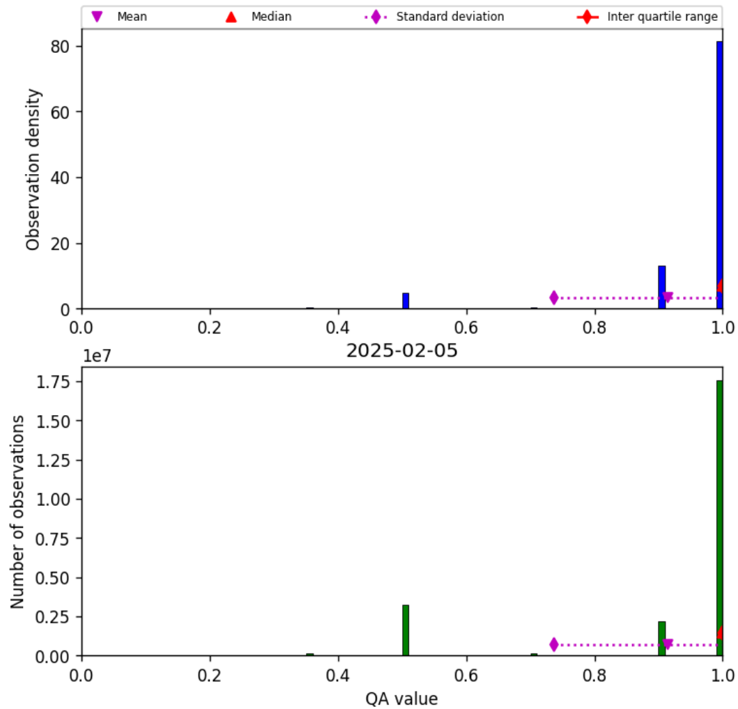
Figure 27: Histogram of “QA value” for 2025-02-05 to 2025-02-06
