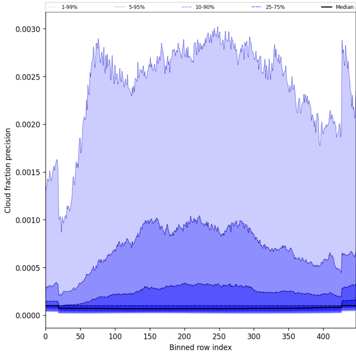
Figure 48: Along track statistics of “Cloud fraction precision” for 2025-02-05 to 2025-02-06
