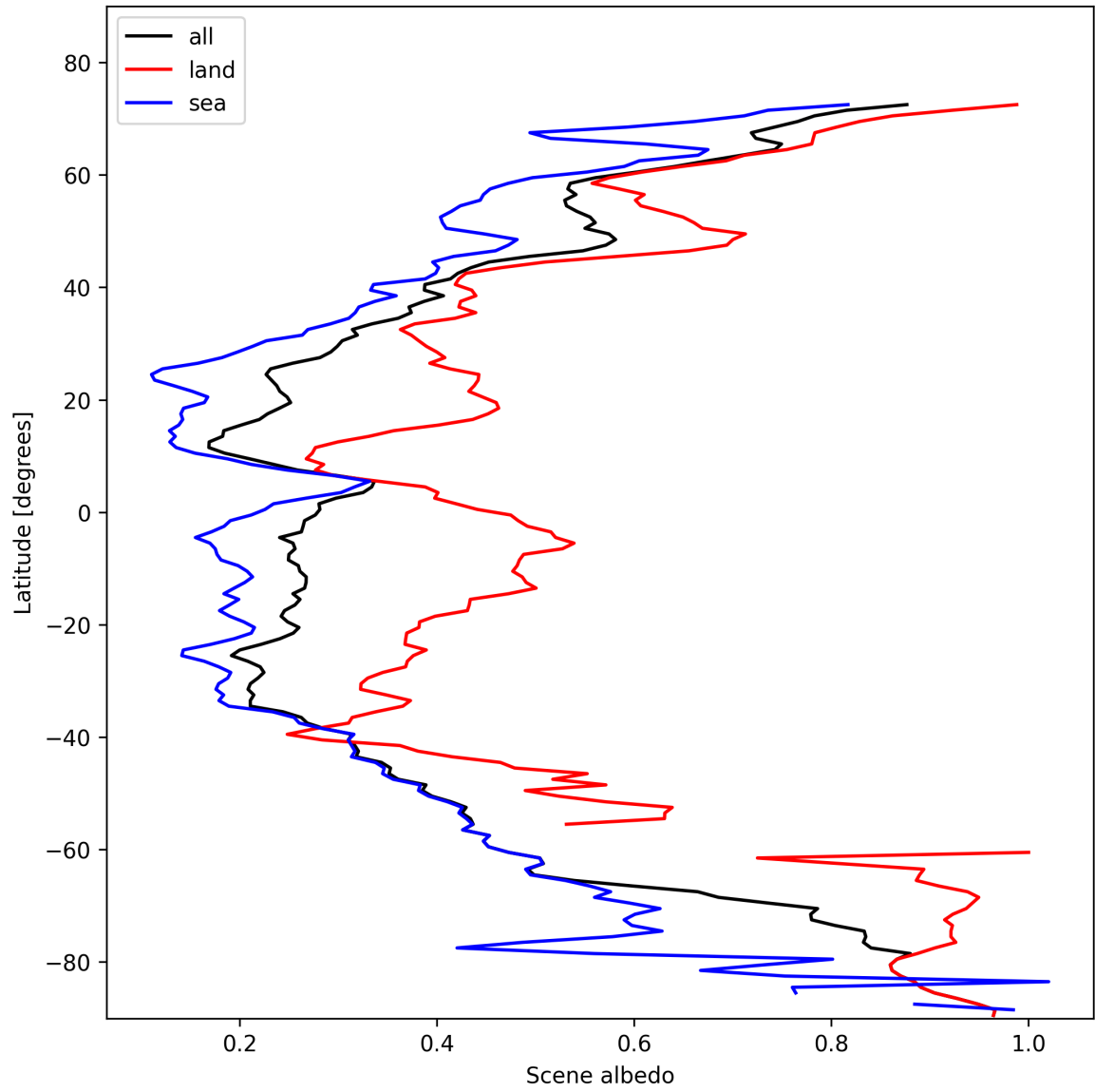
Figure 15: Zonal average of “Scene albedo” for 2025-02-05 to 2025-02-06.
