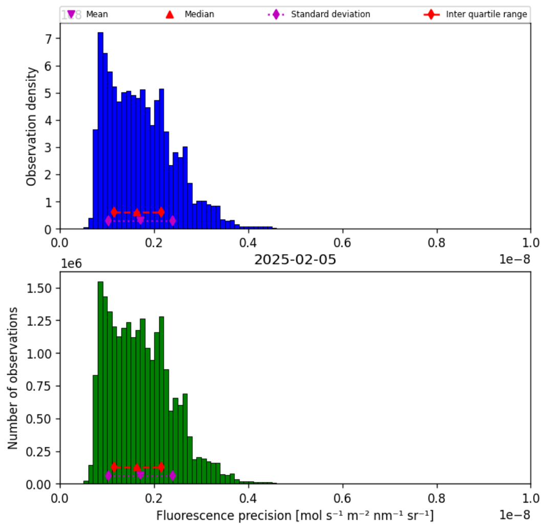
Figure 39: Histogram of “Fluorescence precision” for 2025-02-05 to 2025-02-06
