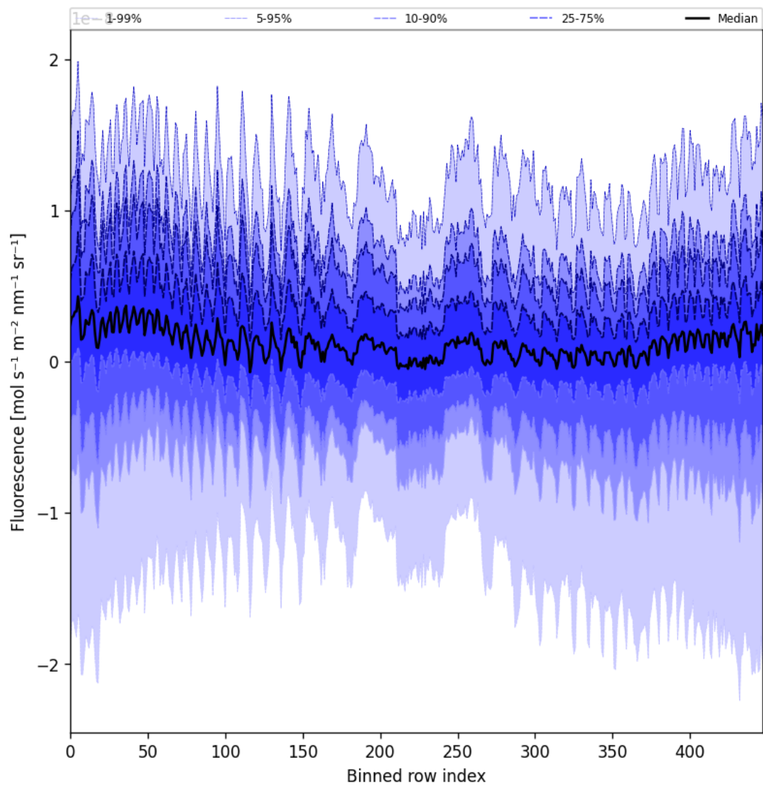
Figure 55: Along track statistics of “Fluorescence” for 2025-02-05 to 2025-02-06
