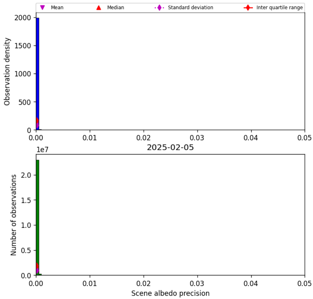
Figure 33: Histogram of “Scene albedo precision” for 2025-02-05 to 2025-02-06
