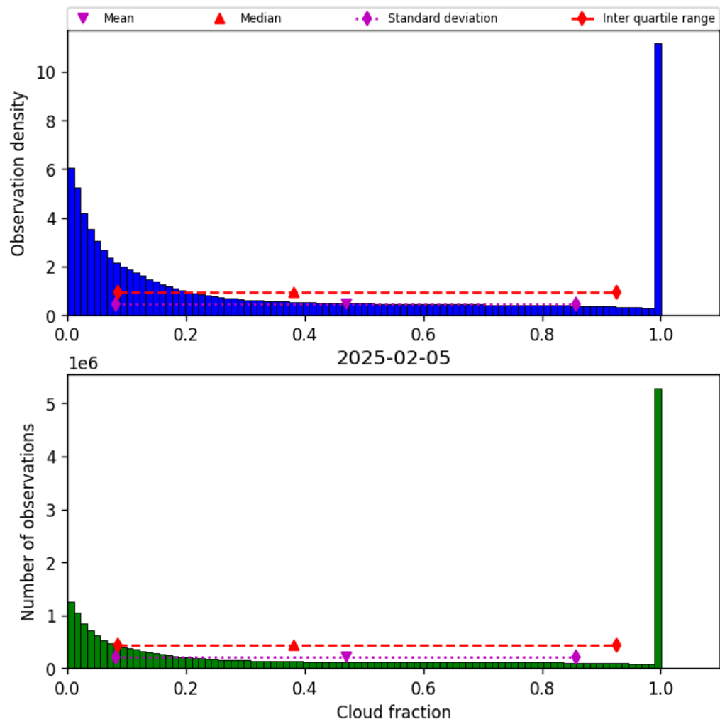
Figure 30: Histogram of “Cloud fraction” for 2025-02-05 to 2025-02-06
