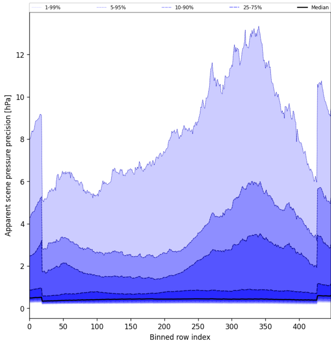
Figure 52: Along track statistics of “Apparent scene pressure precision” for 2025-02-05 to 2025-02-06
