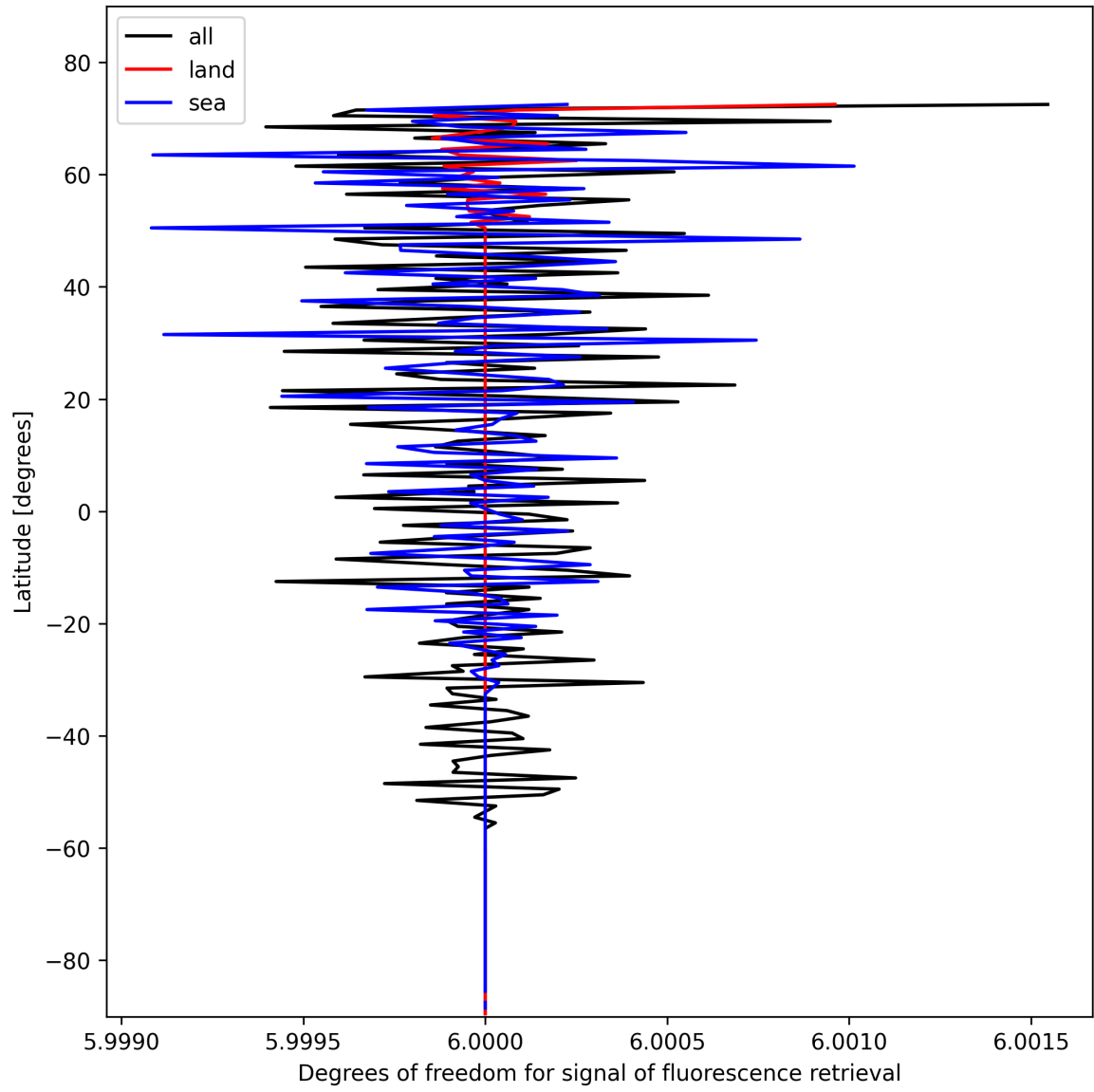
Figure 24: Zonal average of “Degrees of freedom for signal of fluorescence retrieval” for 2025-02-05 to 2025-02-06.
