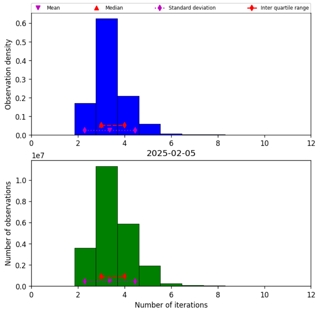
Figure 37: Histogram of “Number of iterations” for 2025-02-05 to 2025-02-06
