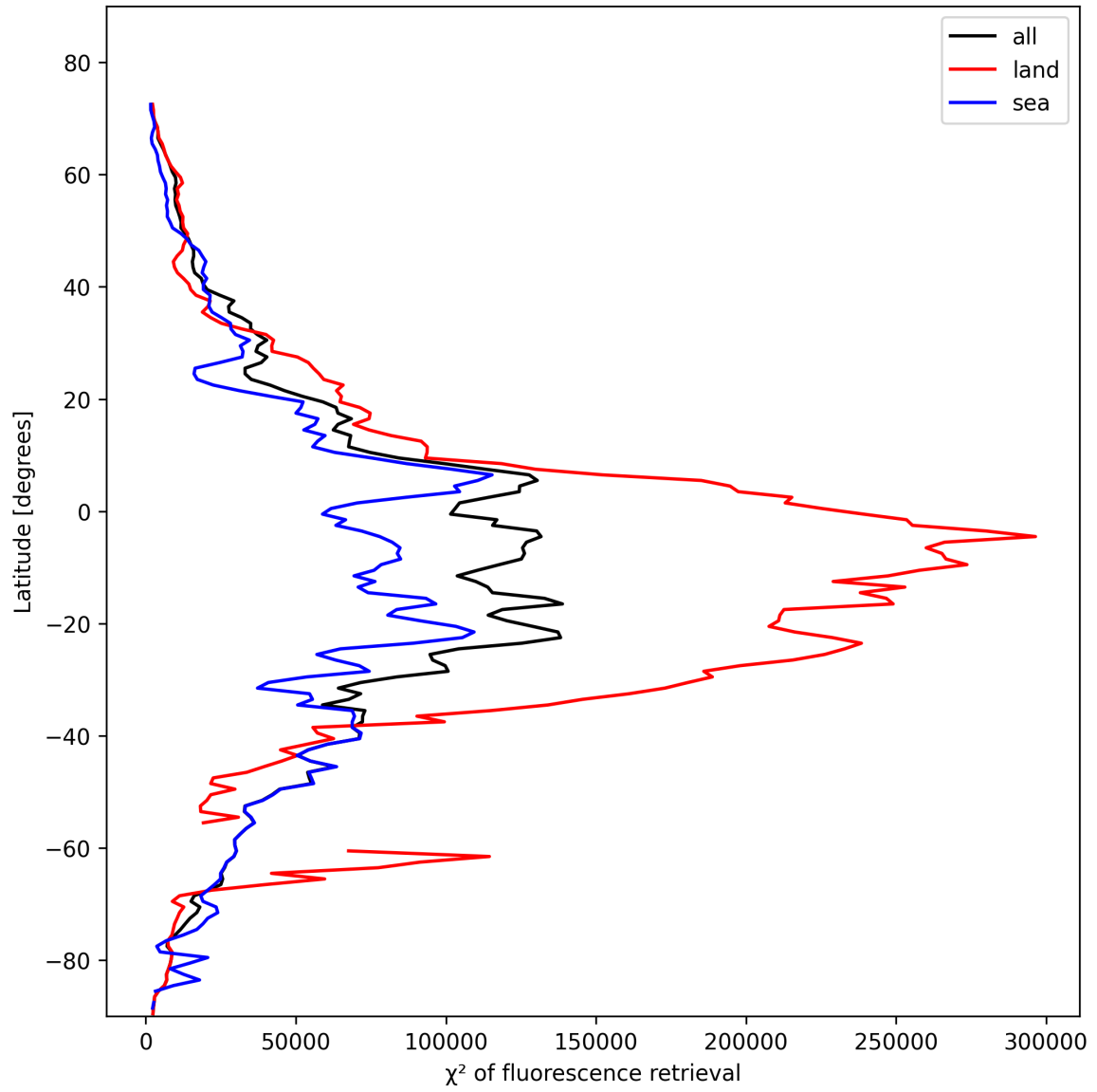
Figure 23: Zonal average of “ \chi^2 of fluorescence retrieval” for 2025-02-05 to 2025-02-06.
