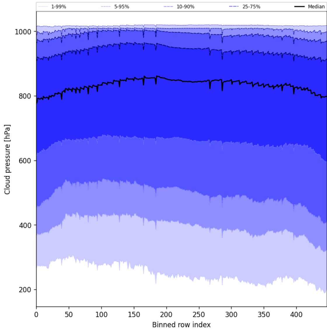
Figure 45: Along track statistics of “Cloud pressure” for 2025-02-05 to 2025-02-06
