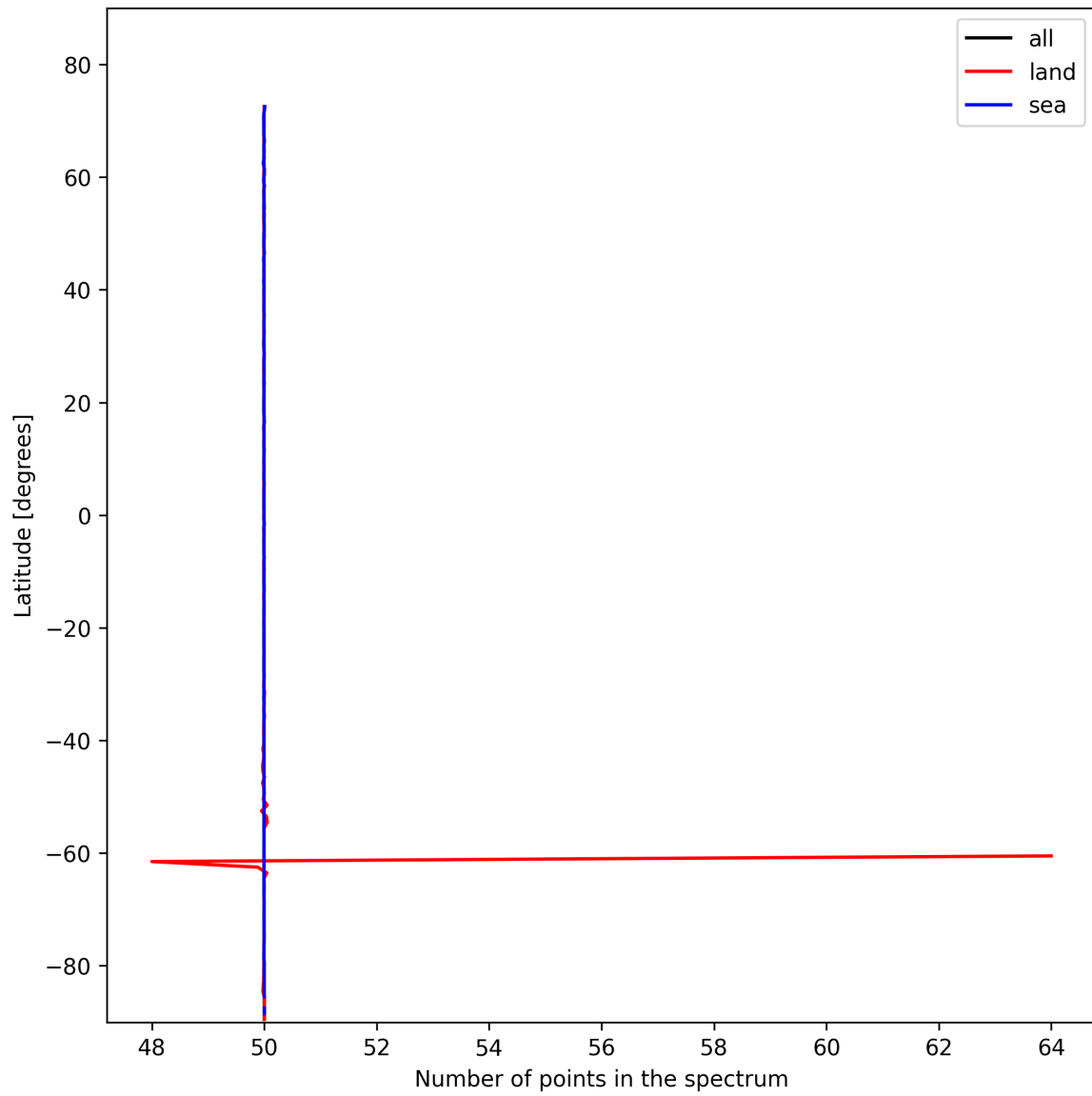
Figure 25: Zonal average of “Number of points in the spectrum” for 2025-02-05 to 2025-02-06.
