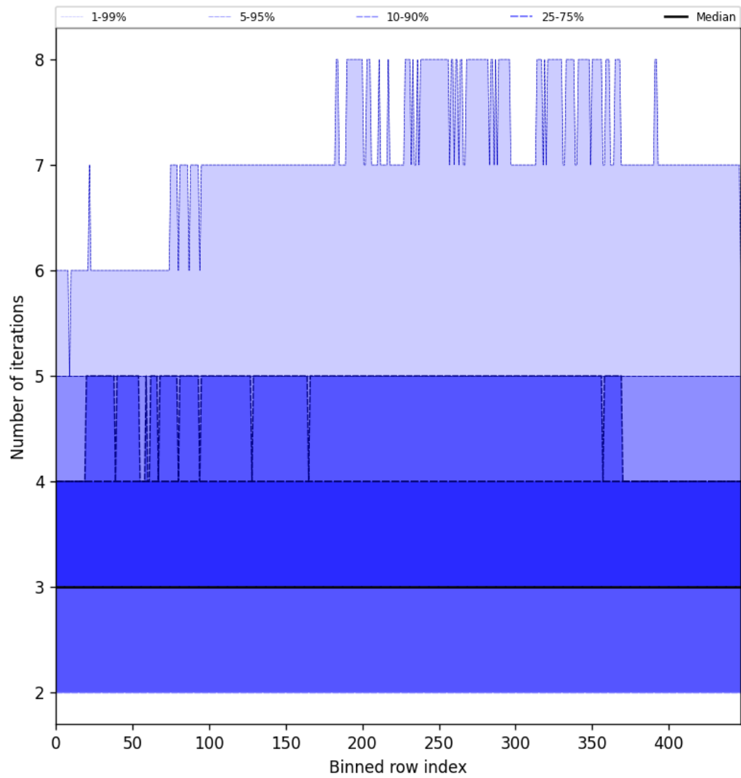
Figure 54: Along track statistics of “Number of iterations” for 2025-02-05 to 2025-02-06
