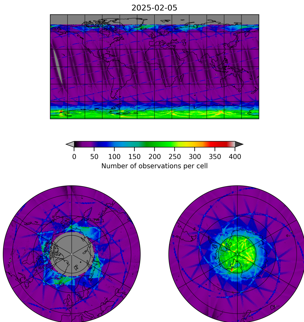
Figure 9: Map of the number of observations for 2025-02-05 to 2025-02-06
