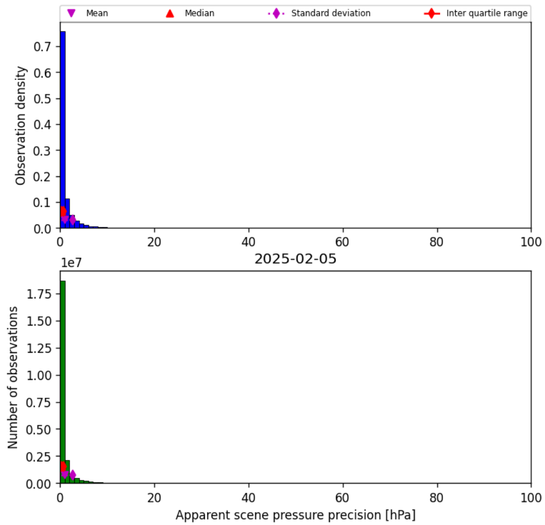
Figure 35: Histogram of “Apparent scene pressure precision” for 2025-02-05 to 2025-02-06
