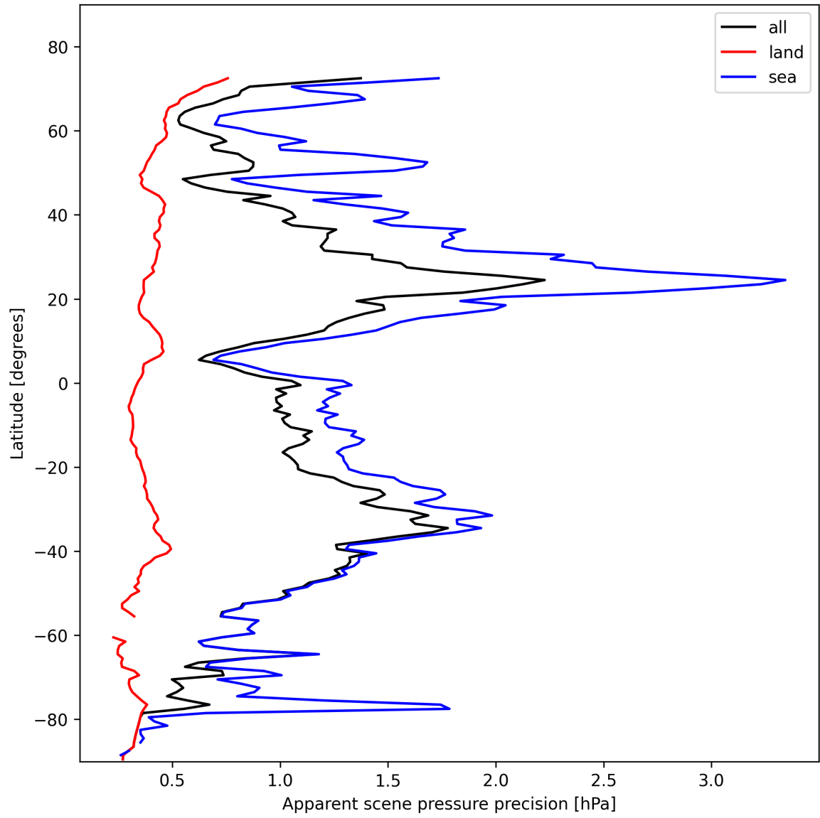
Figure 18: Zonal average of “Apparent scene pressure precision” for 2025-02-05 to 2025-02-06.
