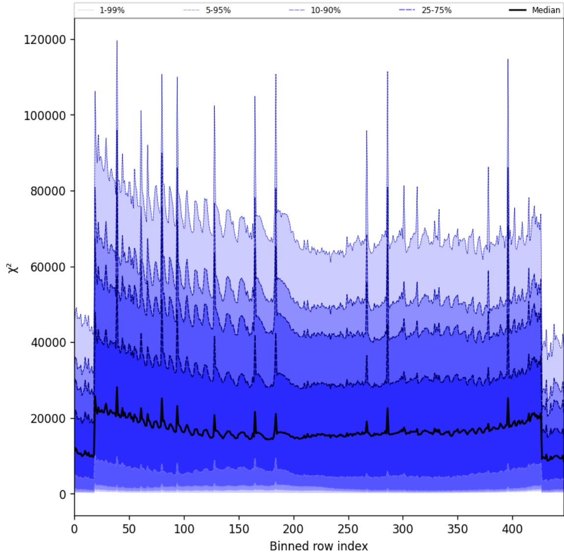
Figure 53: Along track statistics of “ \chi^2 ” for 2025-02-05 to 2025-02-06
