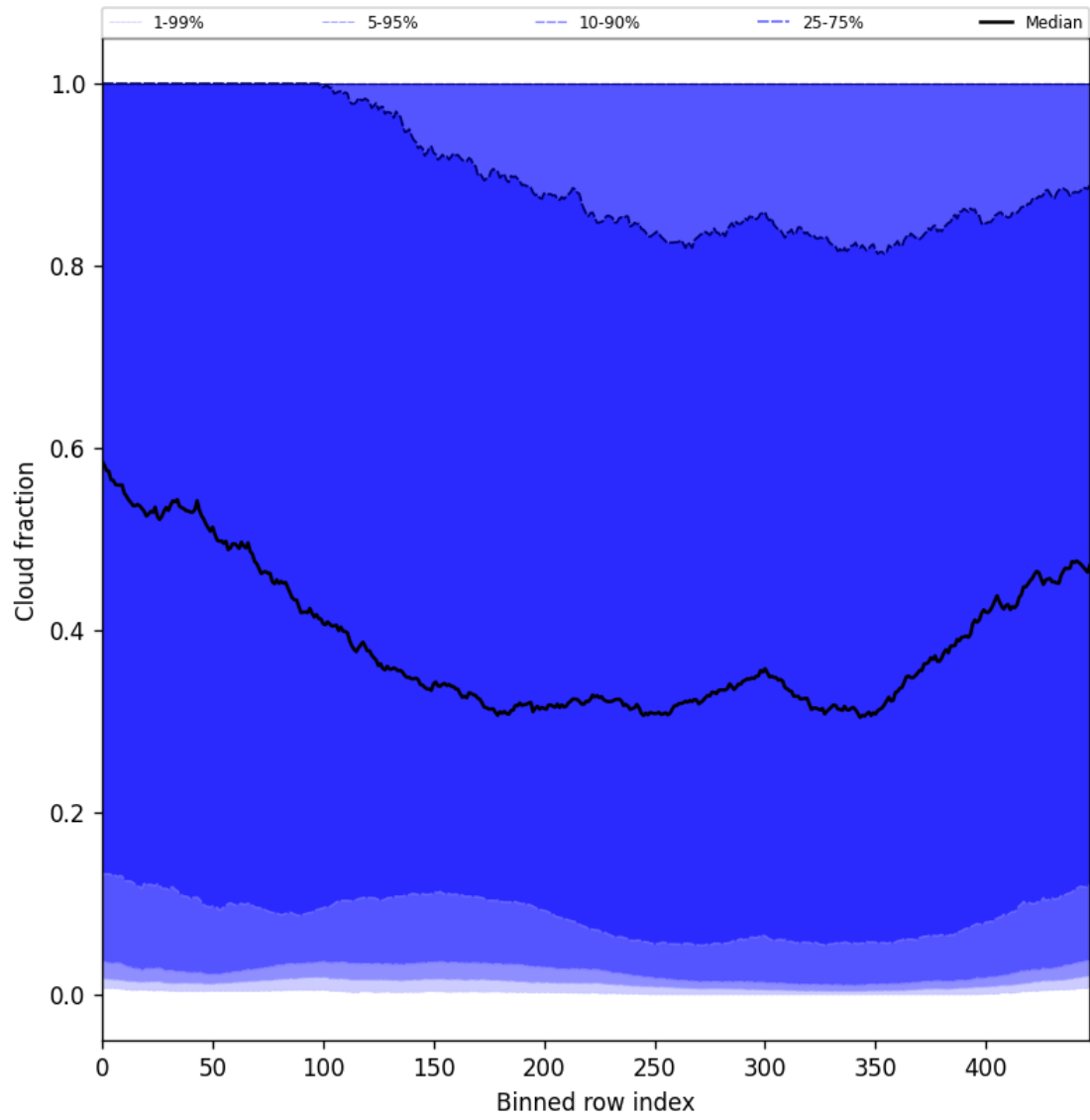
Figure 47: Along track statistics of “Cloud fraction” for 2025-02-05 to 2025-02-06
