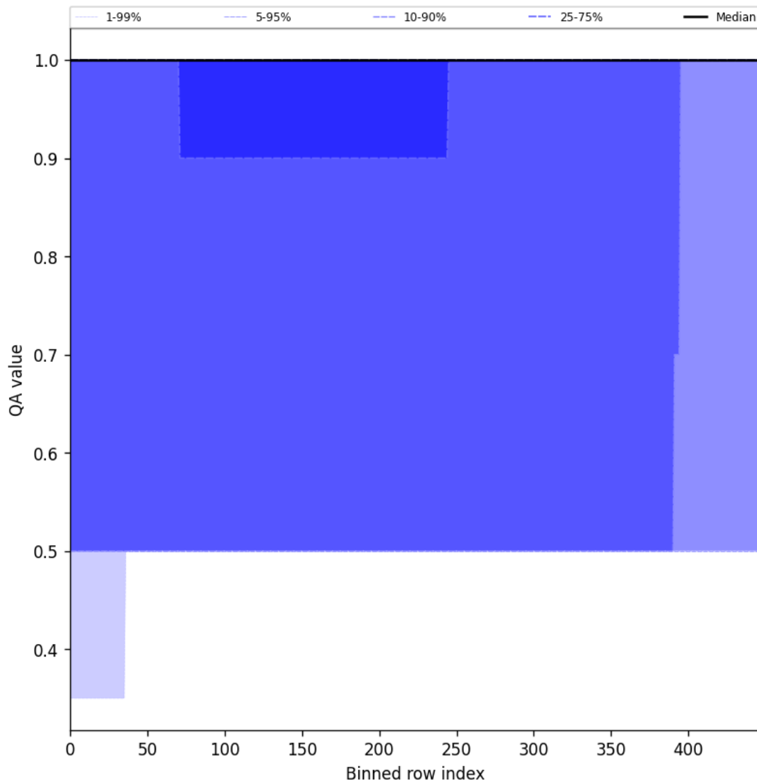
Figure 44: Along track statistics of “QA value” for 2025-02-05 to 2025-02-06
