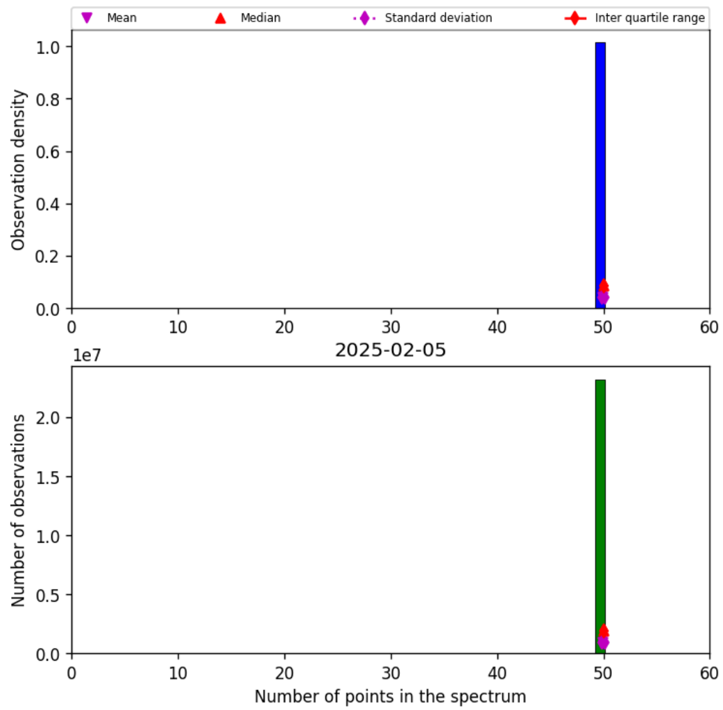
Figure 42: Histogram of “Number of points in the spectrum” for 2025-02-05 to 2025-02-06
