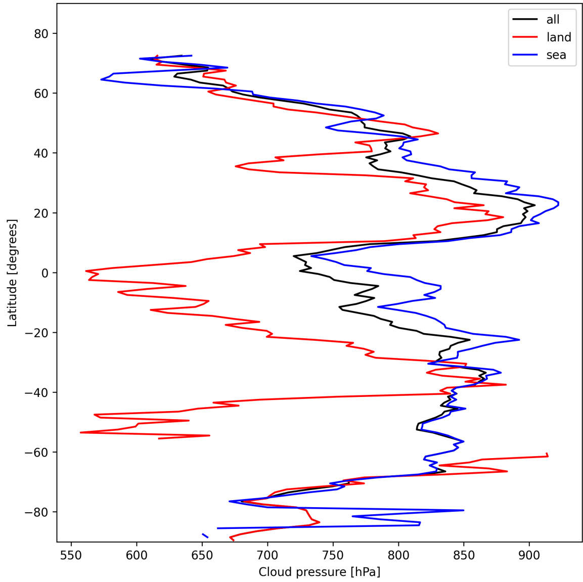
Figure 11: Zonal average of “Cloud pressure” for 2025-02-05 to 2025-02-06.
