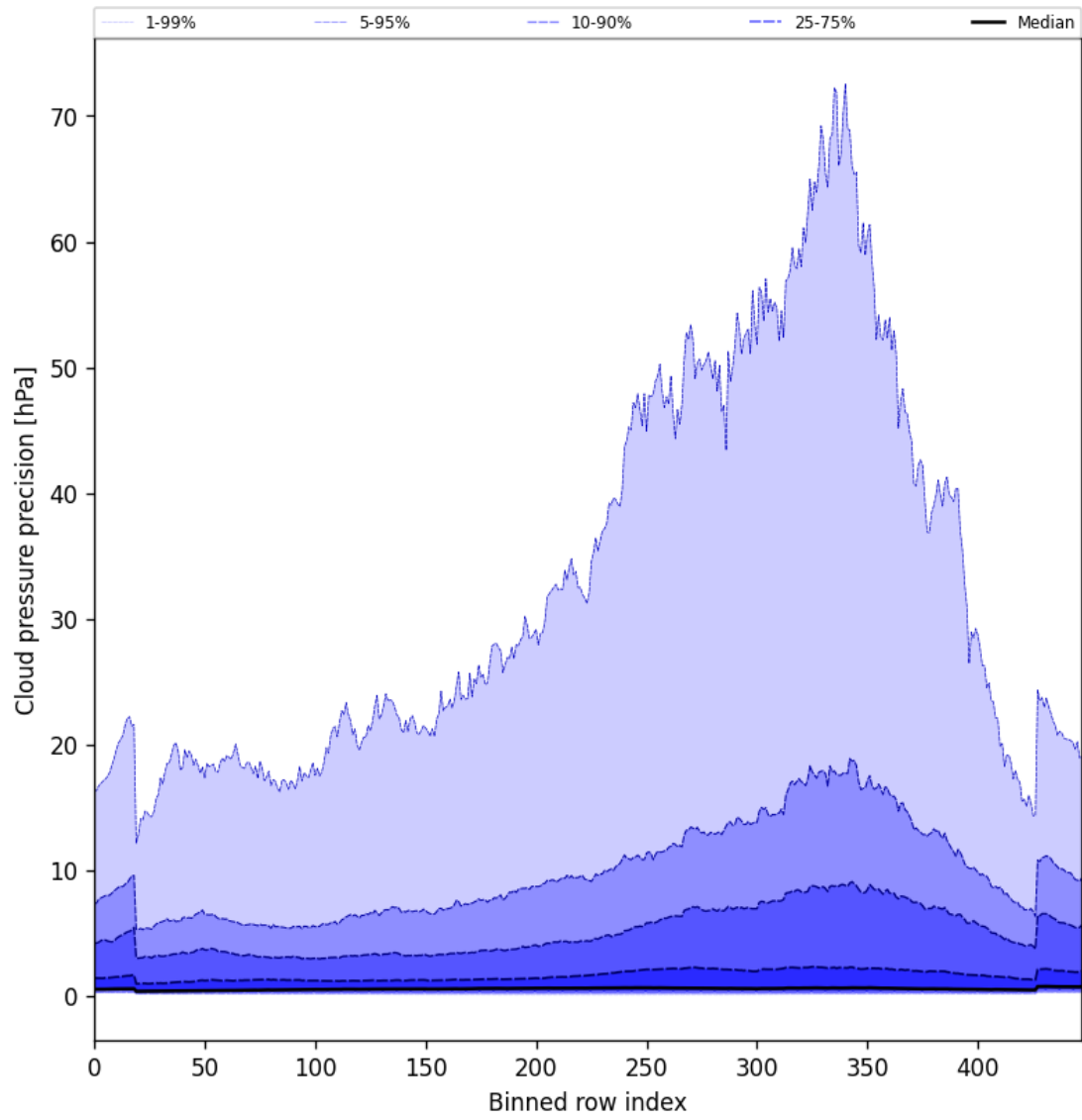
Figure 46: Along track statistics of “Cloud pressure precision” for 2025-02-05 to 2025-02-06
