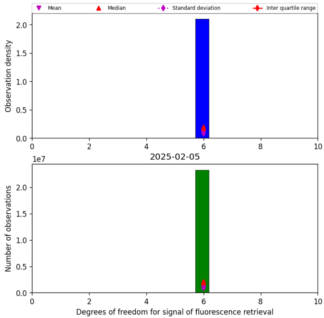
Figure 41: Histogram of “Degrees of freedom for signal of fluorescence retrieval” for 2025-02-05 to 2025-02-06
