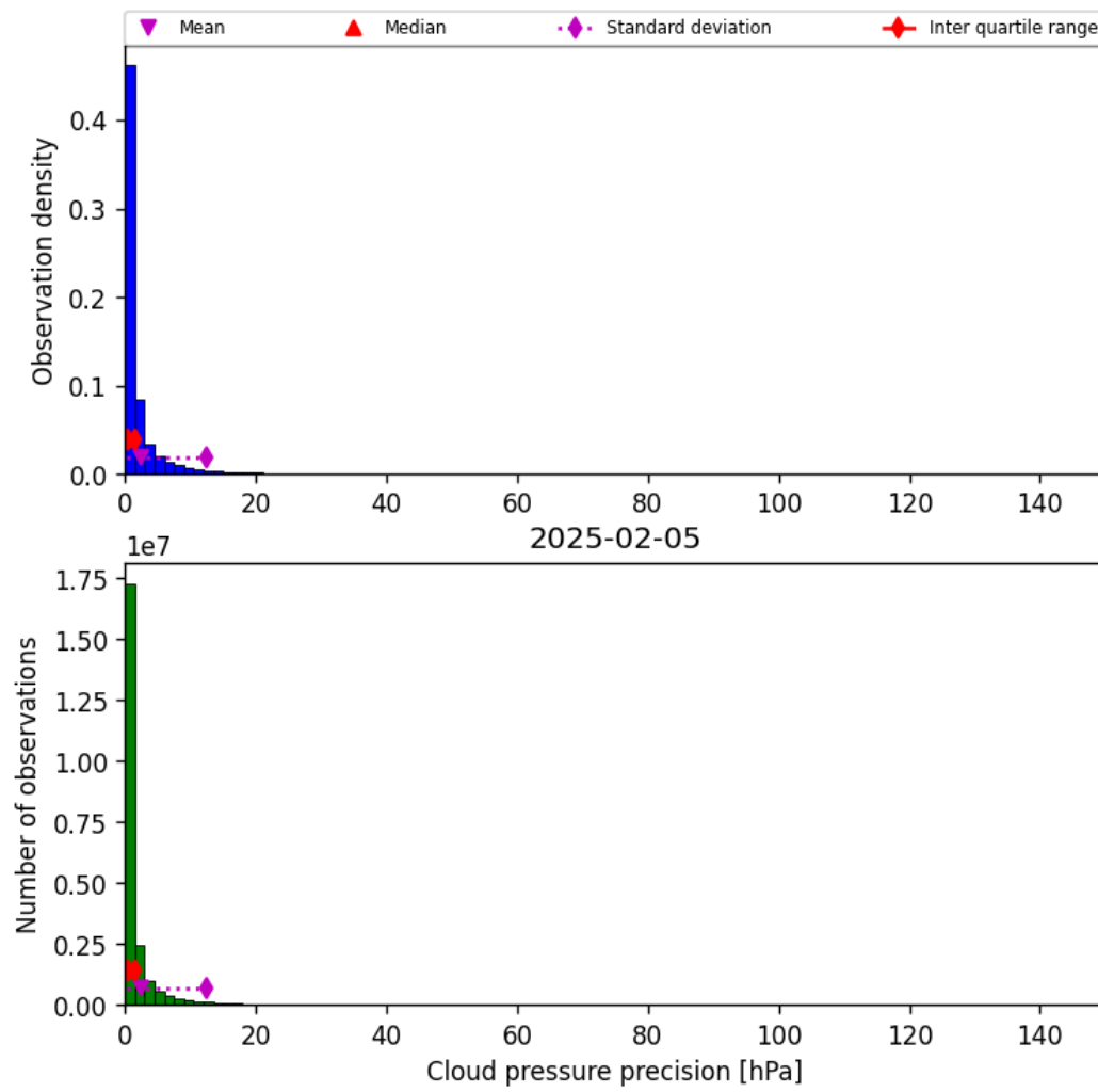
Figure 29: Histogram of “Cloud pressure precision” for 2025-02-05 to 2025-02-06
