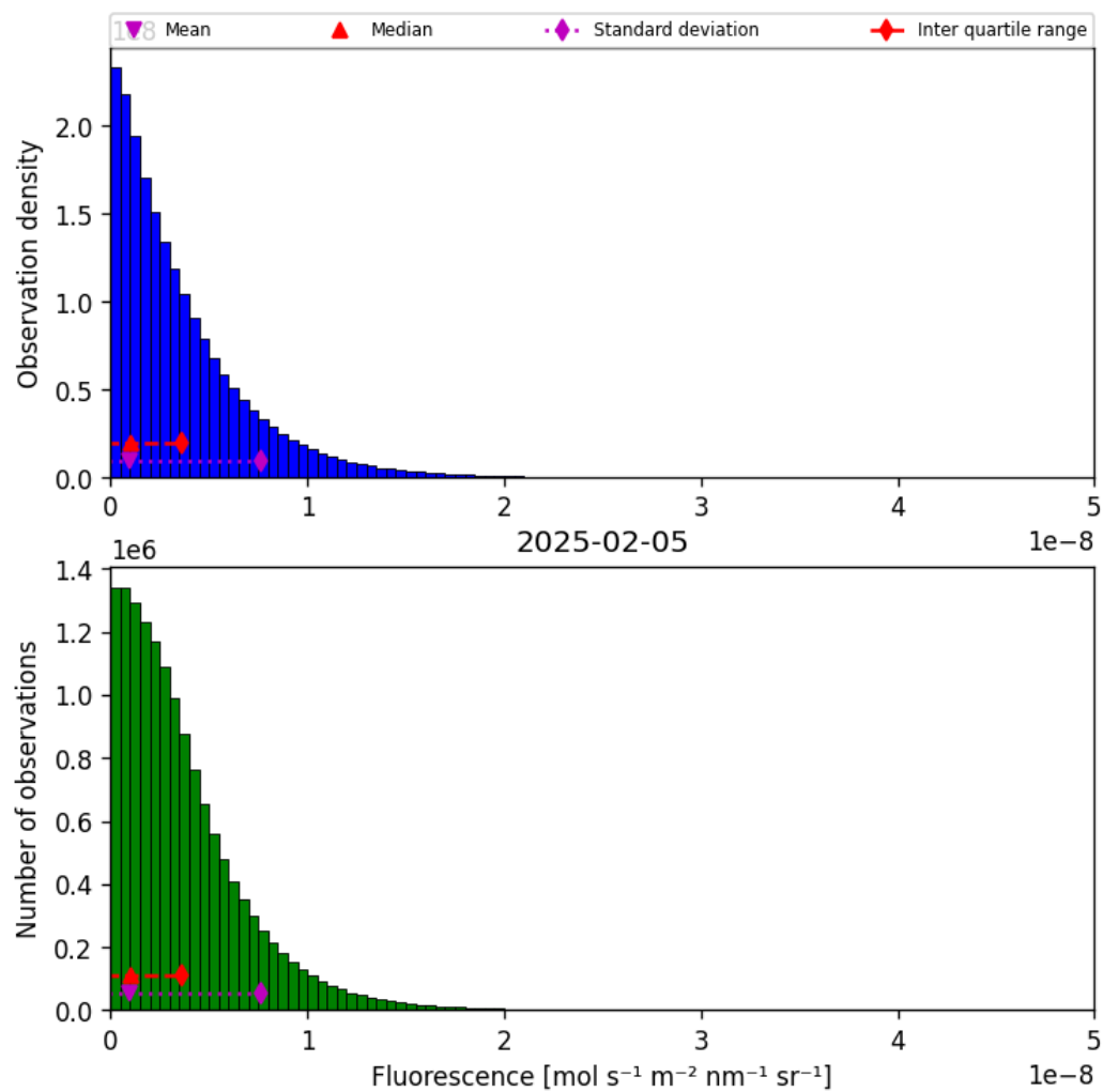
Figure 38: Histogram of “Fluorescence” for 2025-02-05 to 2025-02-06
