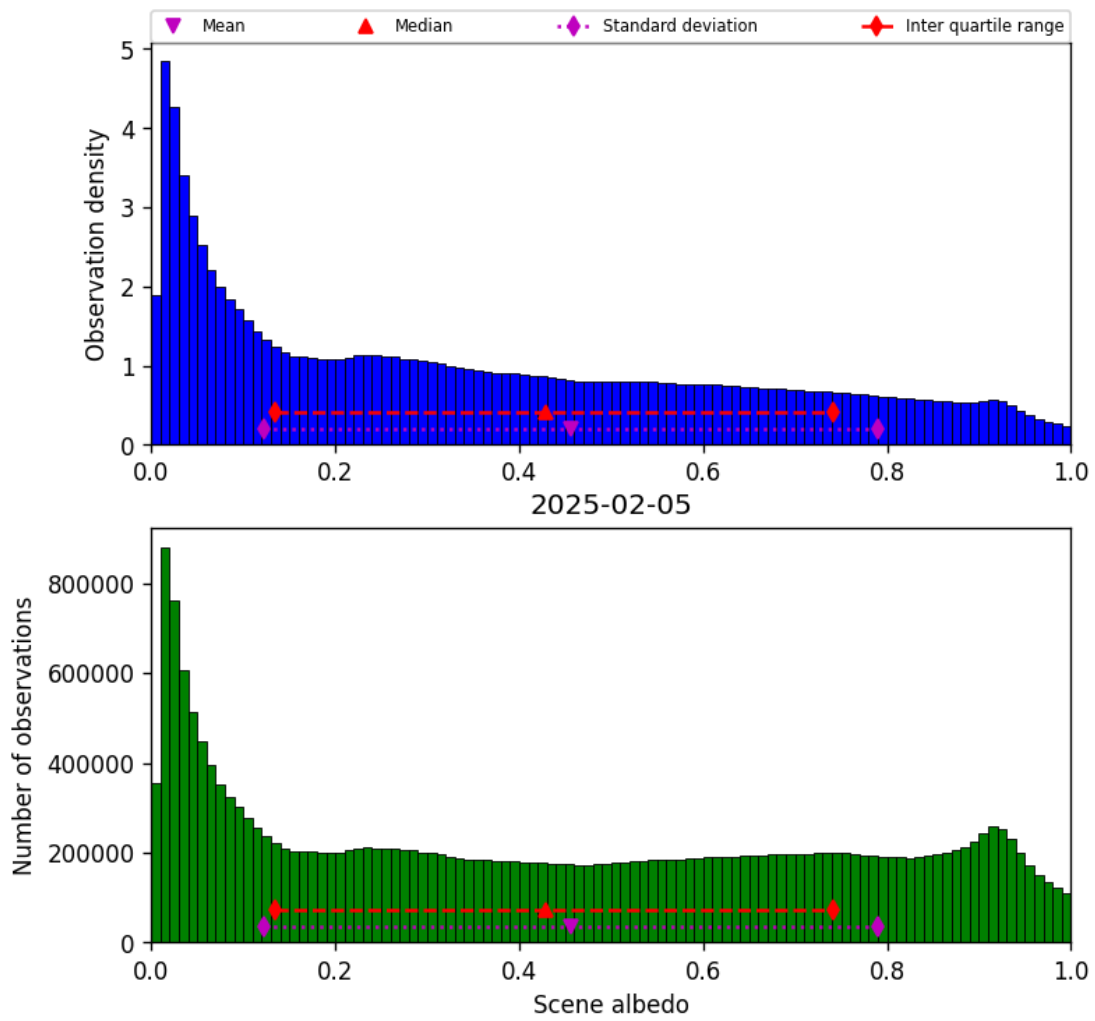
Figure 32: Histogram of “Scene albedo” for 2025-02-05 to 2025-02-06
