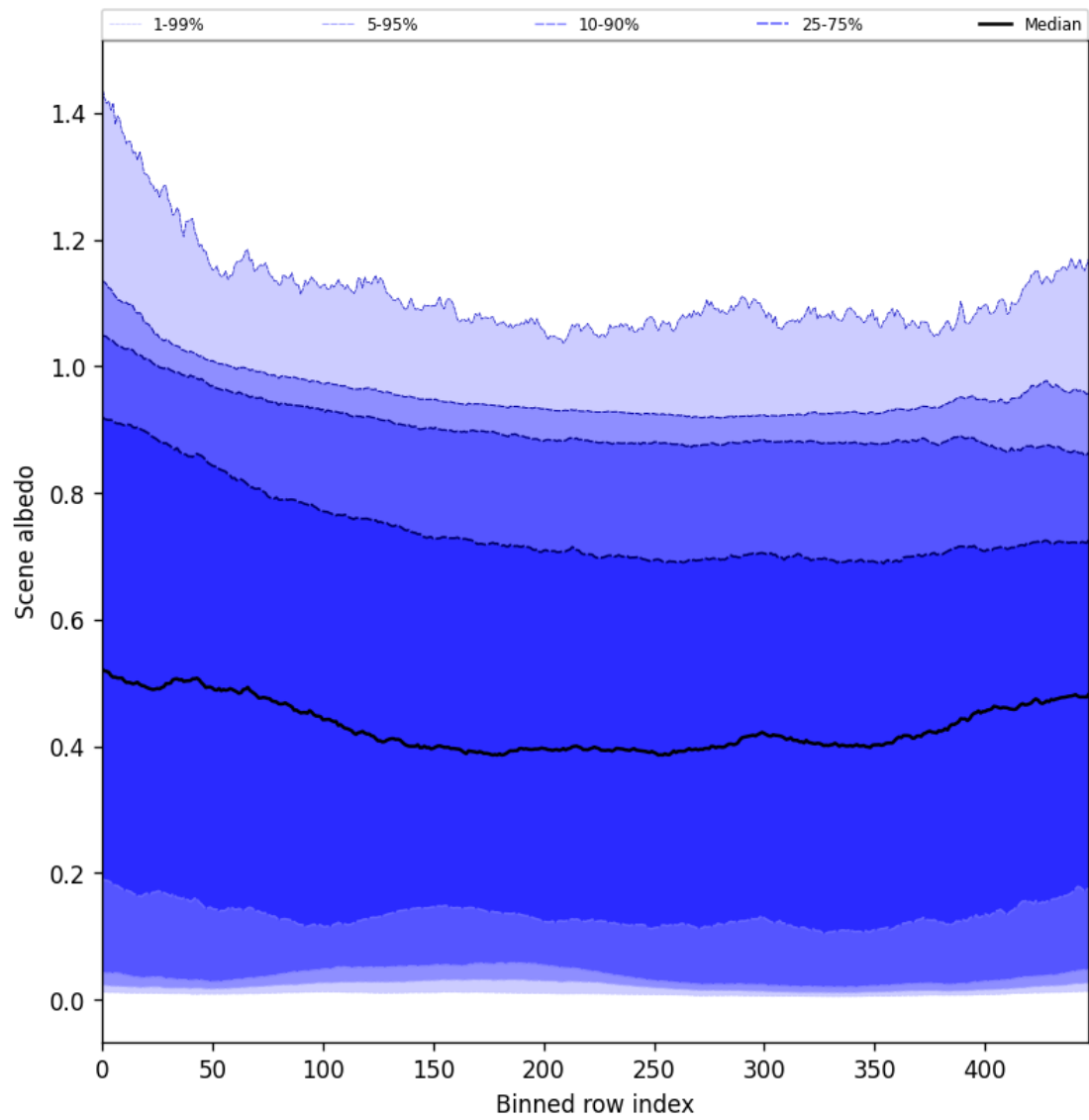
Figure 49: Along track statistics of “Scene albedo” for 2025-02-05 to 2025-02-06
