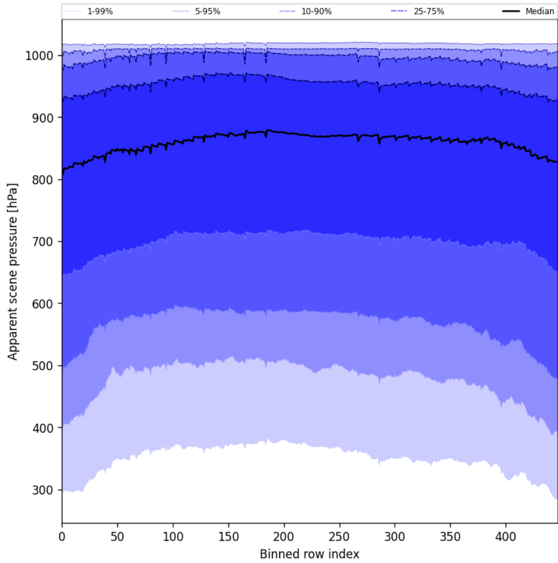
Figure 51: Along track statistics of “Apparent scene pressure” for 2025-02-05 to 2025-02-06
