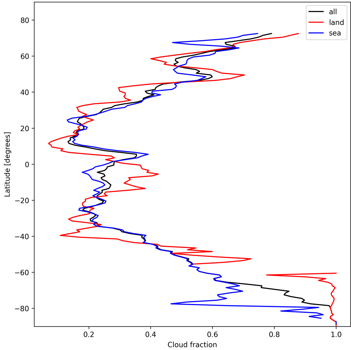
Figure 13: Zonal average of “Cloud fraction” for 2025-02-05 to 2025-02-06.
