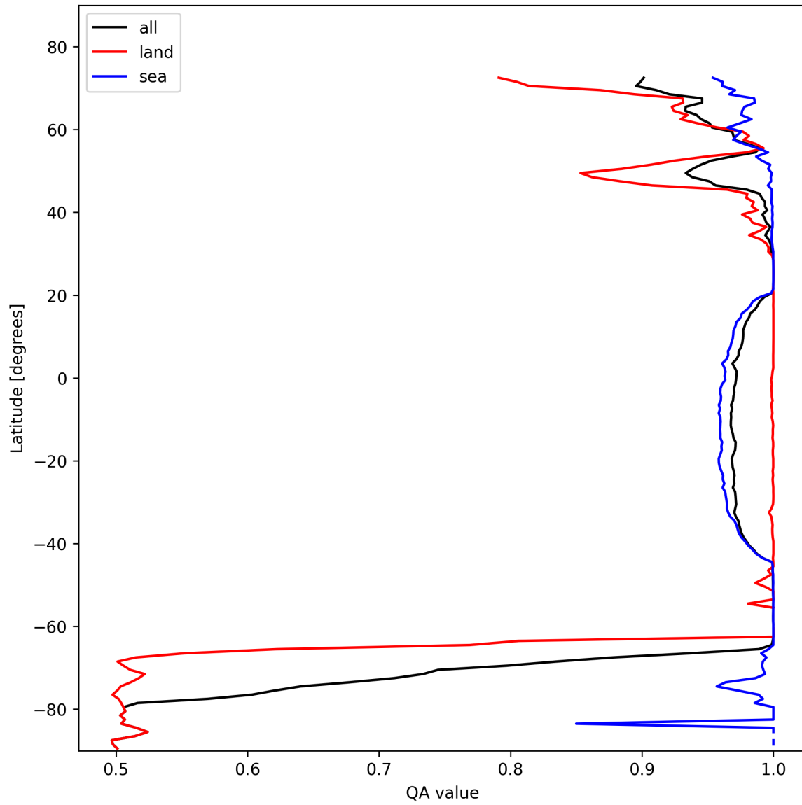
Figure 10: Zonal average of “QA value” for 2025-02-05 to 2025-02-06.
