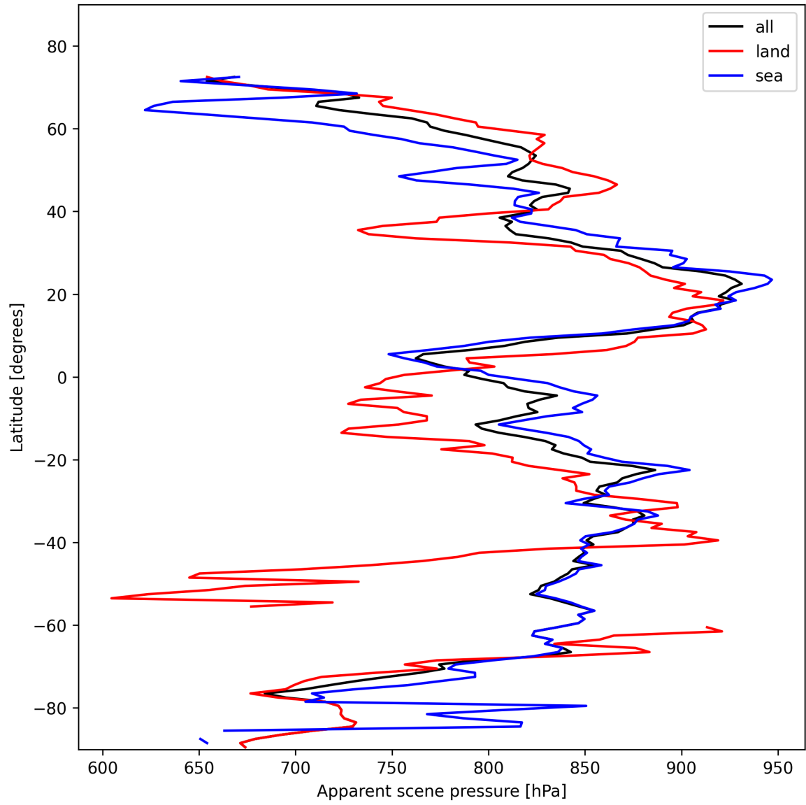
Figure 17: Zonal average of “Apparent scene pressure” for 2025-02-05 to 2025-02-06.
