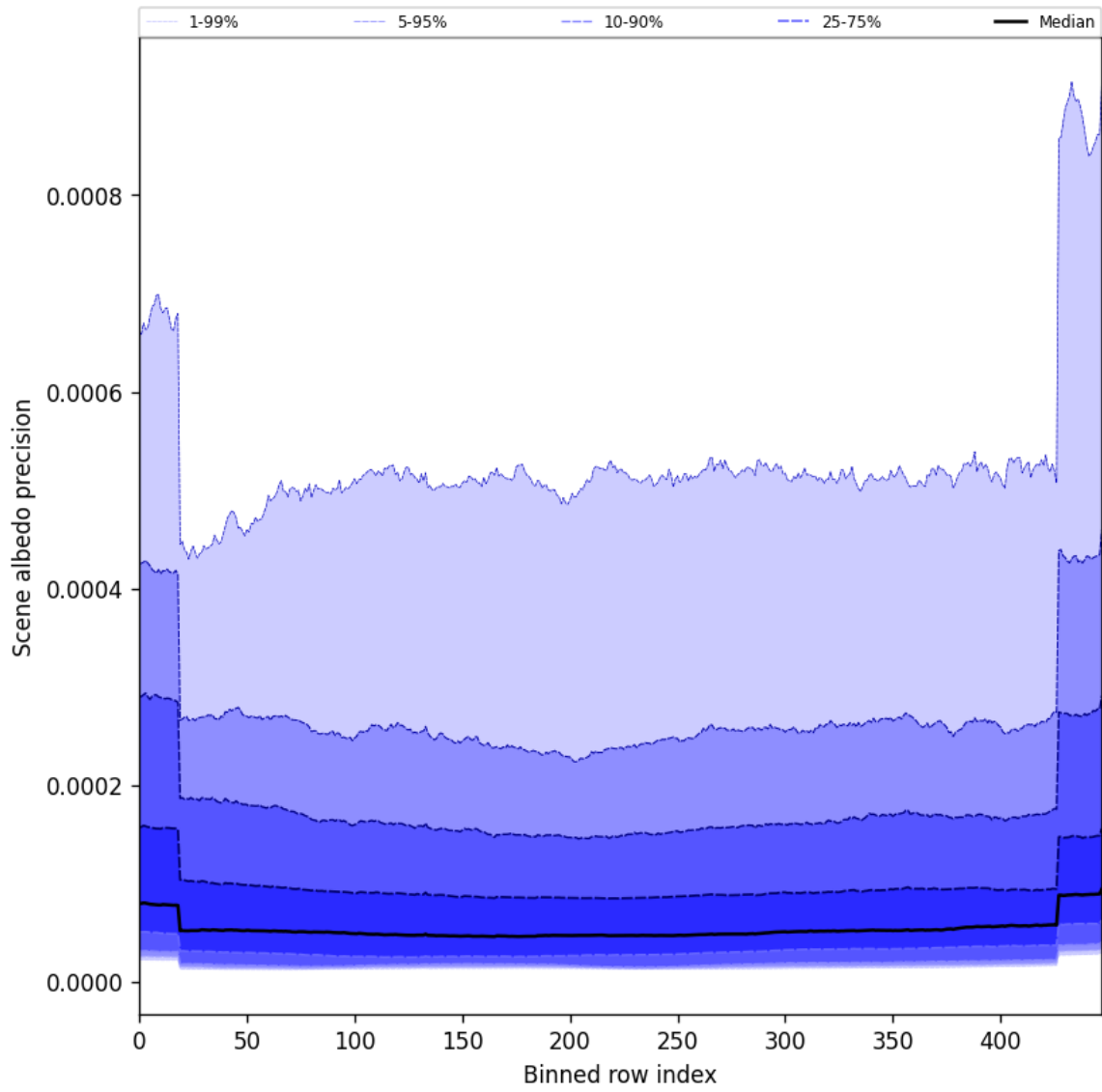
Figure 50: Along track statistics of “Scene albedo precision” for 2025-02-05 to 2025-02-06
