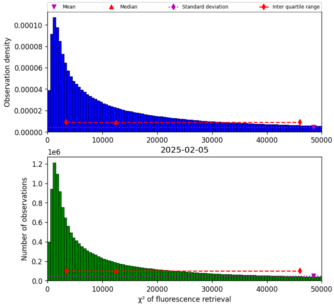
Figure 40: Histogram of “ \chi^2 of fluorescence retrieval” for 2025-02-05 to 2025-02-06
