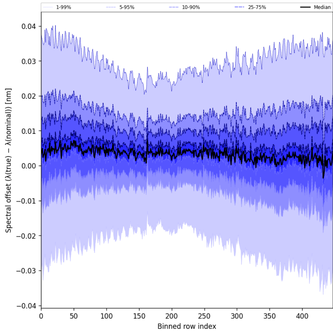
Figure 60: Along track statistics of “Spectral offset ( \lambda_{\text{true}} - \lambda_{\text{nominal}} )” for 2025-02-05 to 2025-02-06
