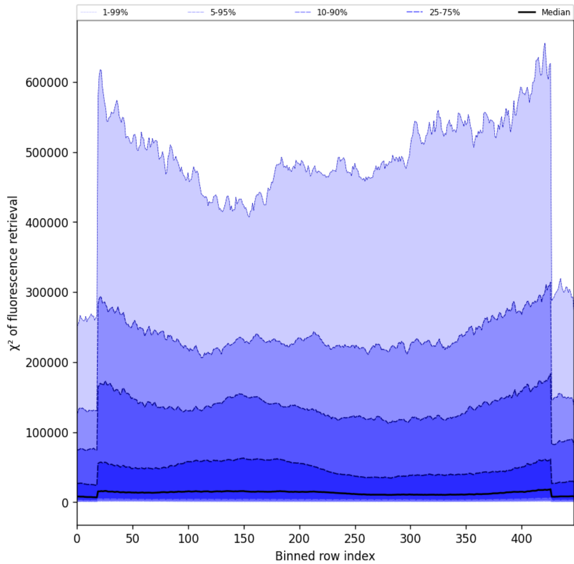
Figure 57: Along track statistics of “ \chi^2 of fluorescence retrieval” for 2025-02-05 to 2025-02-06
