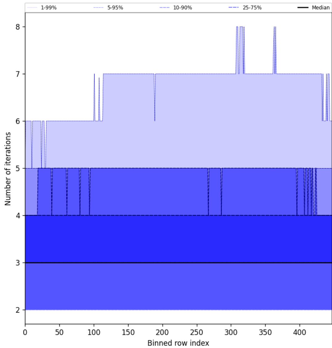
Figure 54: Along track statistics of “Number of iterations” for 2025-02-07 to 2025-02-08
