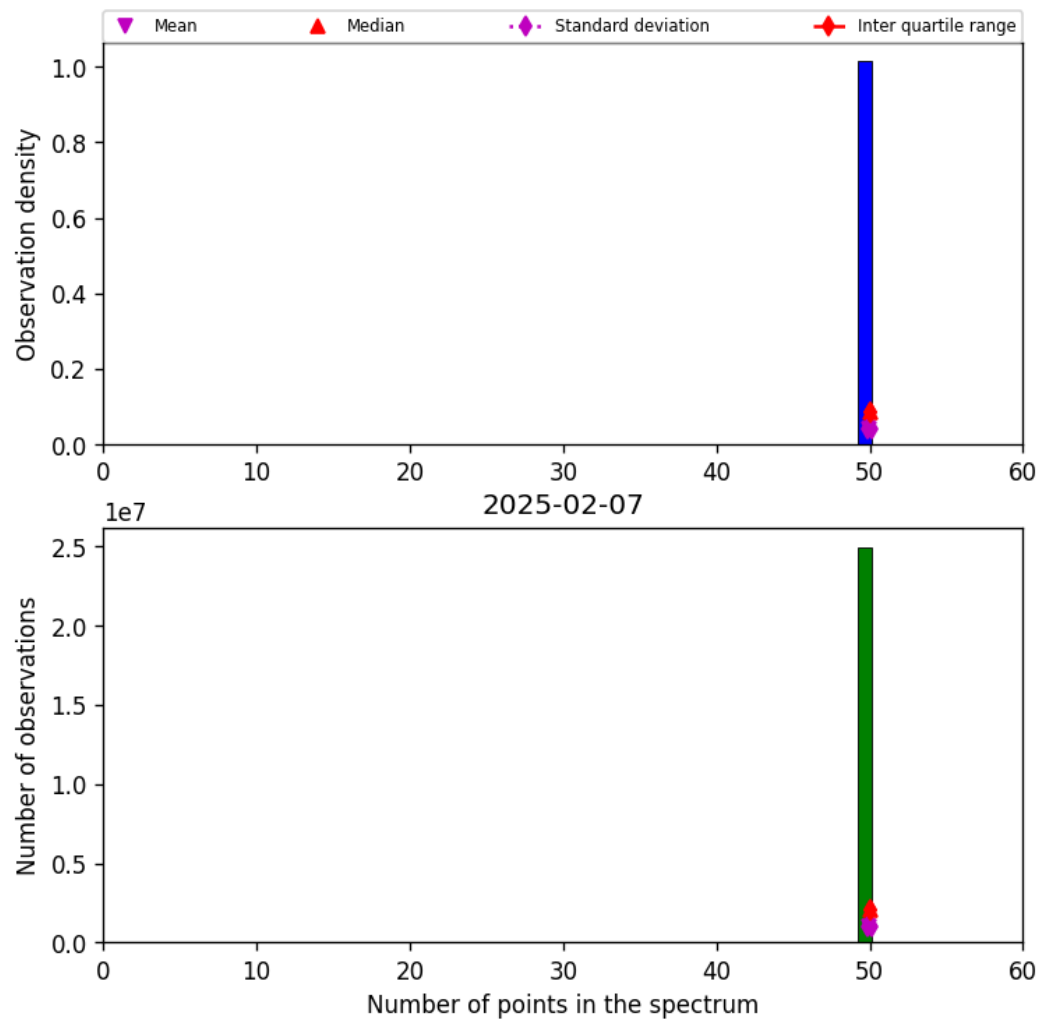
Figure 42: Histogram of “Number of points in the spectrum” for 2025-02-07 to 2025-02-08
