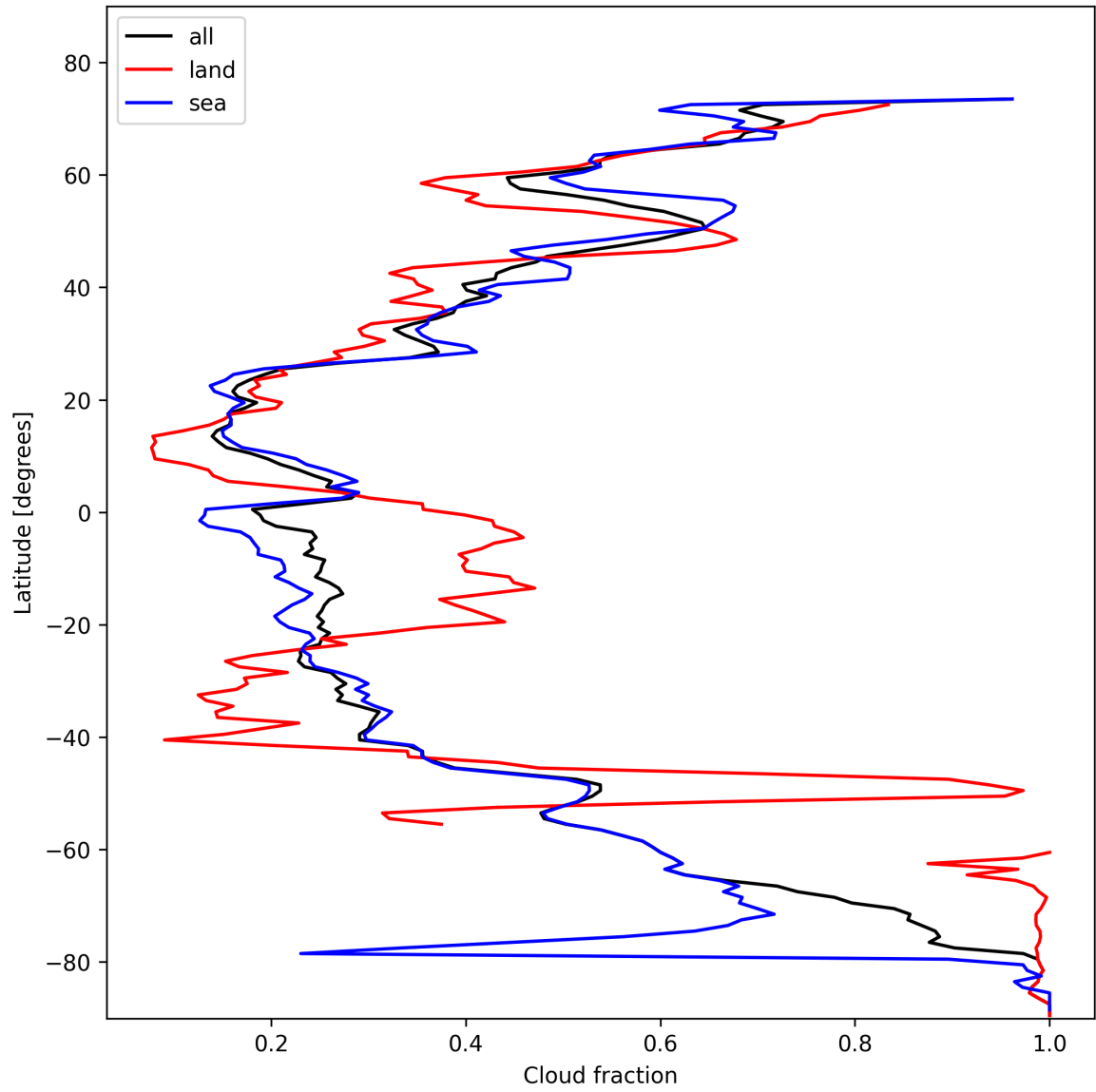
Figure 13: Zonal average of “Cloud fraction” for 2025-02-07 to 2025-02-08.
