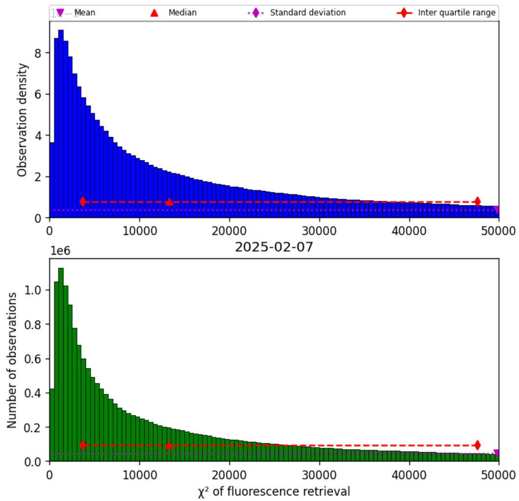
Figure 40: Histogram of “ \chi^2 of fluorescence retrieval” for 2025-02-07 to 2025-02-08
