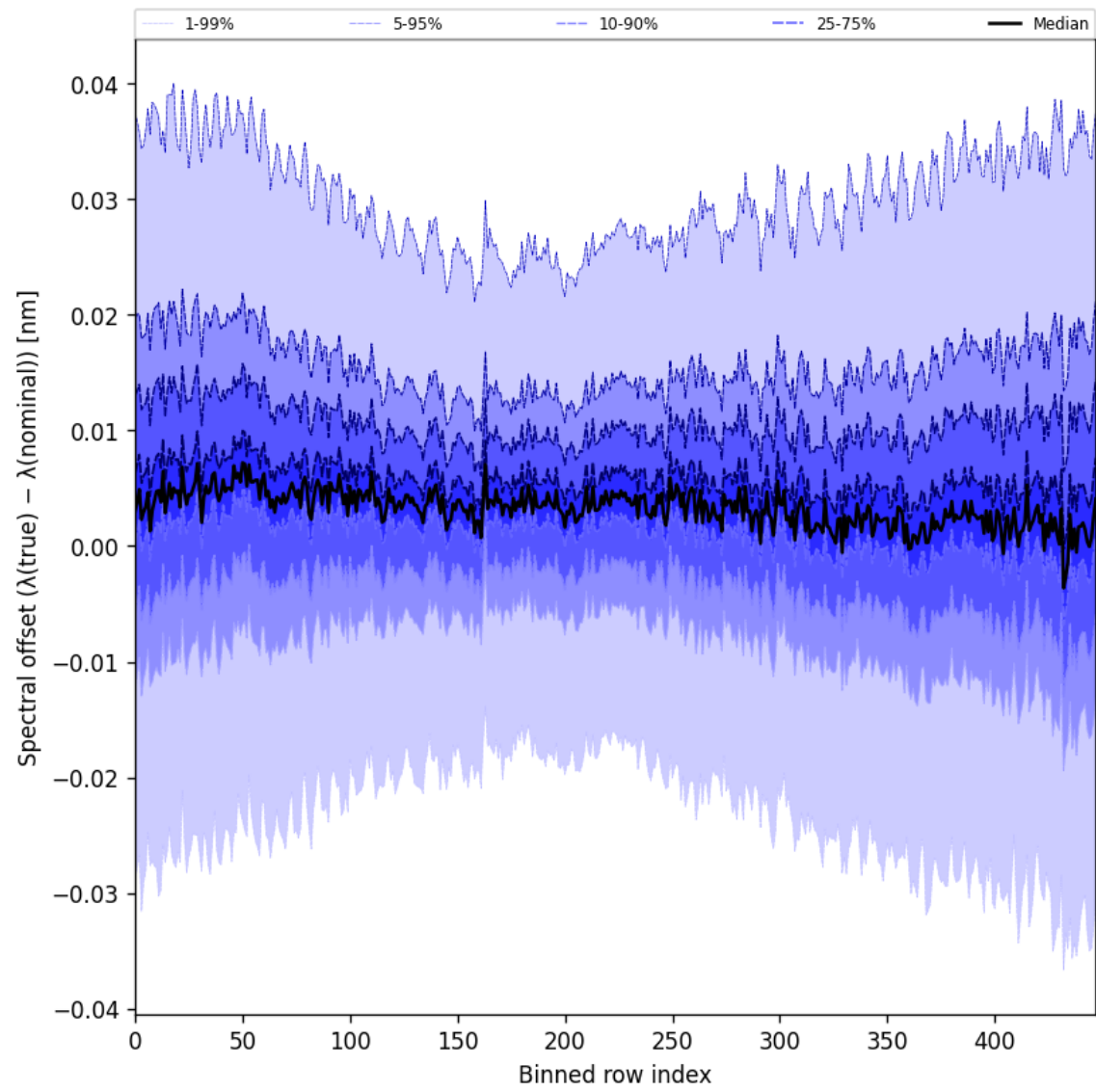
Figure 60: Along track statistics of “Spectral offset ( \lambda_{\text{true}} - \lambda_{\text{nominal}} )” for 2025-02-07 to 2025-02-08
