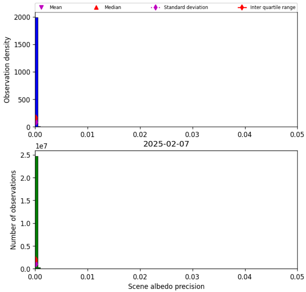
Figure 33: Histogram of “Scene albedo precision” for 2025-02-07 to 2025-02-08
