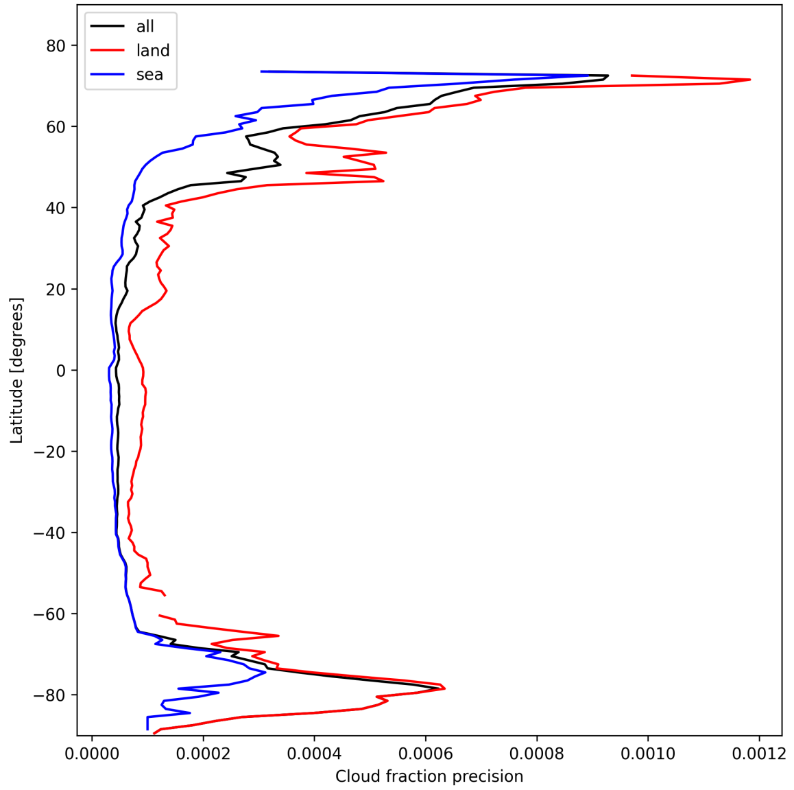
Figure 14: Zonal average of “Cloud fraction precision” for 2025-02-07 to 2025-02-08.
