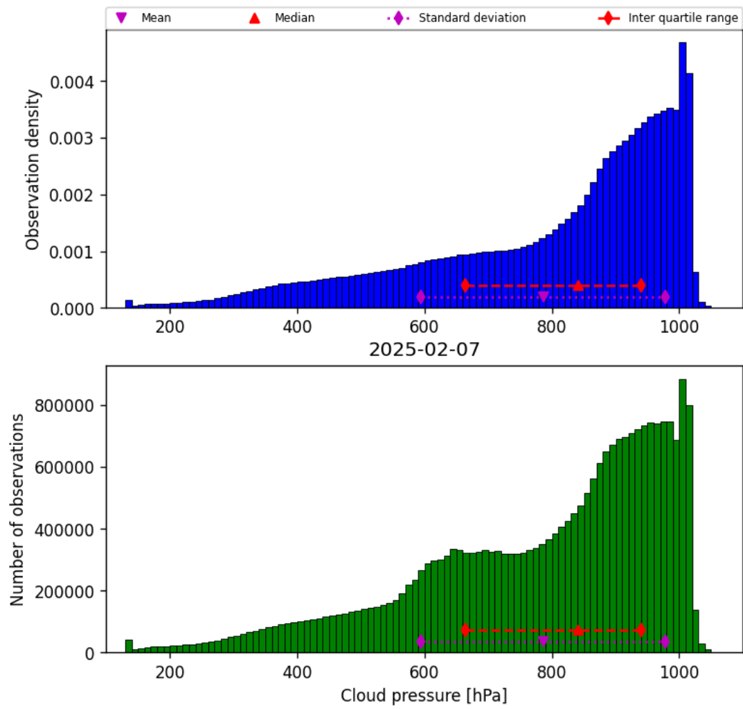
Figure 28: Histogram of “Cloud pressure” for 2025-02-07 to 2025-02-08
