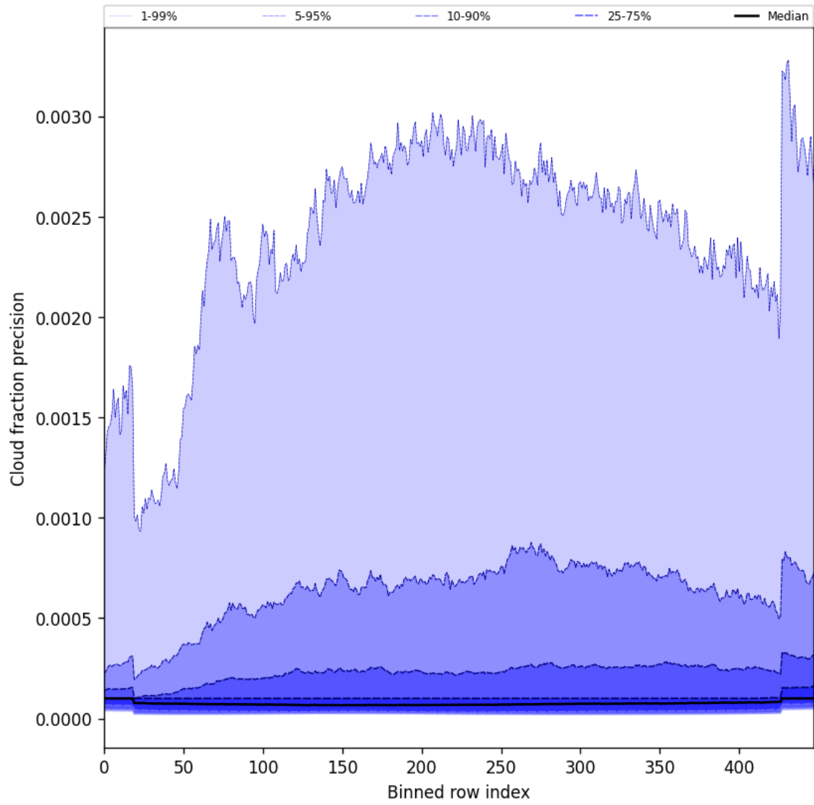
Figure 48: Along track statistics of “Cloud fraction precision” for 2025-02-07 to 2025-02-08
