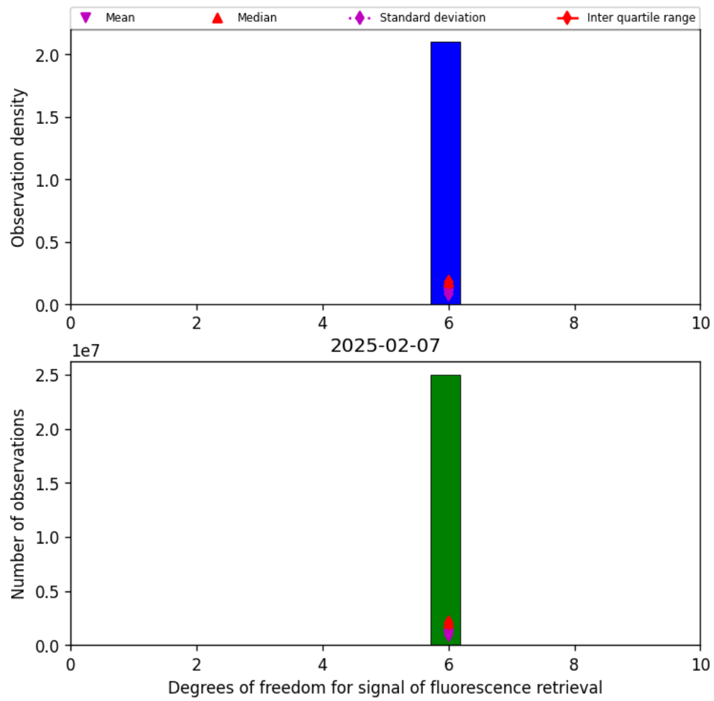
Figure 41: Histogram of “Degrees of freedom for signal of fluorescence retrieval” for 2025-02-07 to 2025-02-08
