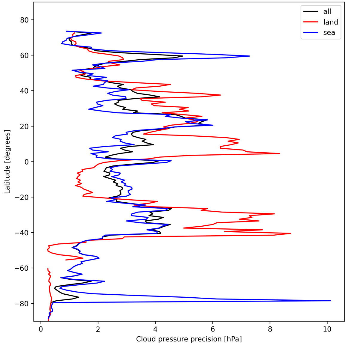
Figure 12: Zonal average of “Cloud pressure precision” for 2025-02-07 to 2025-02-08.
