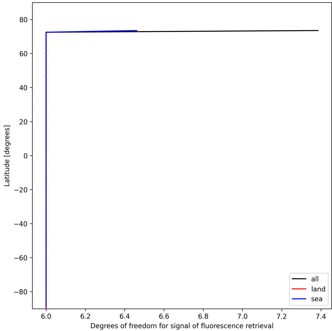
Figure 24: Zonal average of “Degrees of freedom for signal of fluorescence retrieval” for 2025-02-07 to 2025-02-08.
