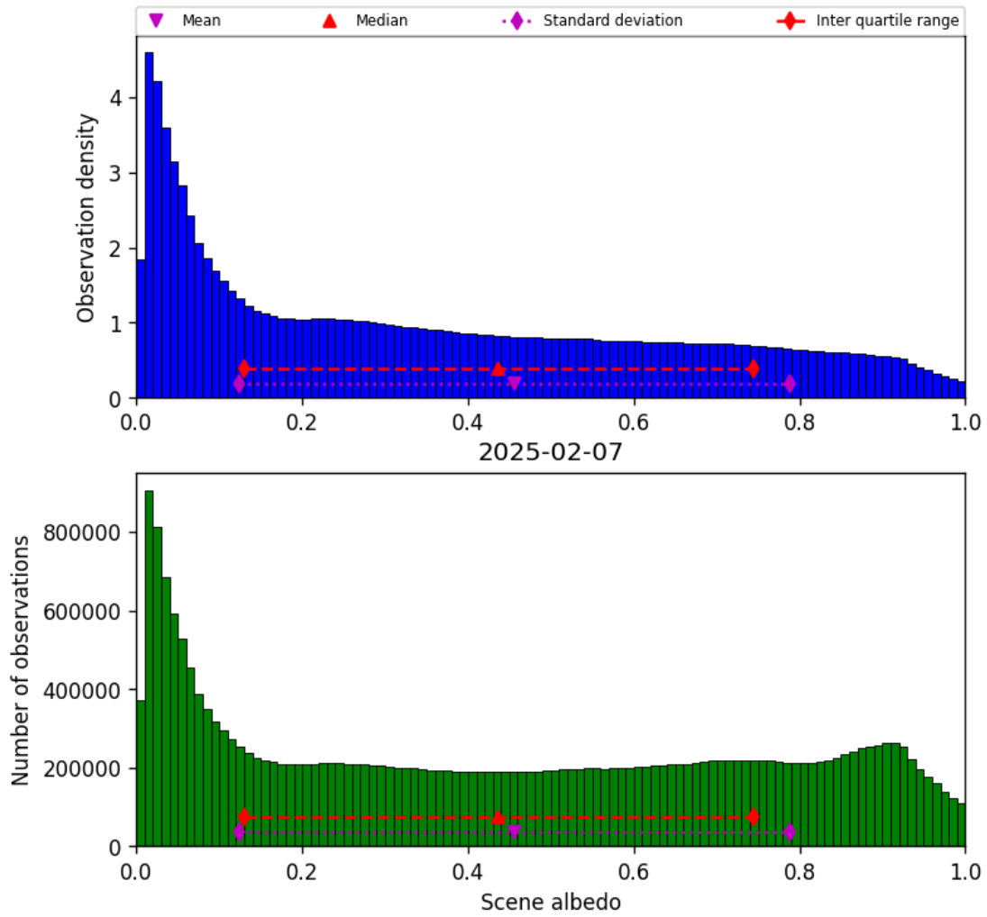
Figure 32: Histogram of “Scene albedo” for 2025-02-07 to 2025-02-08
