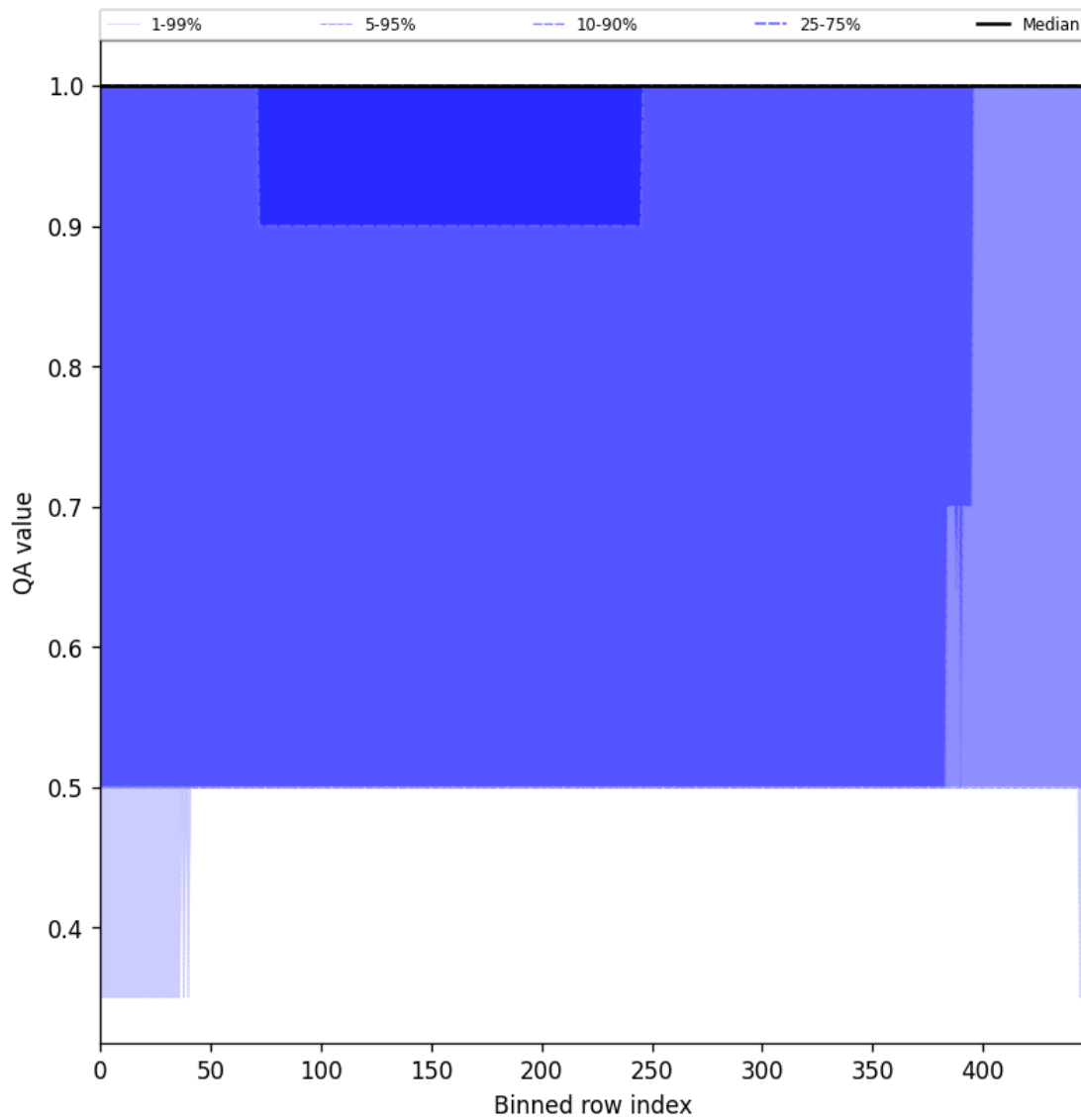
Figure 44: Along track statistics of “QA value” for 2025-02-07 to 2025-02-08
