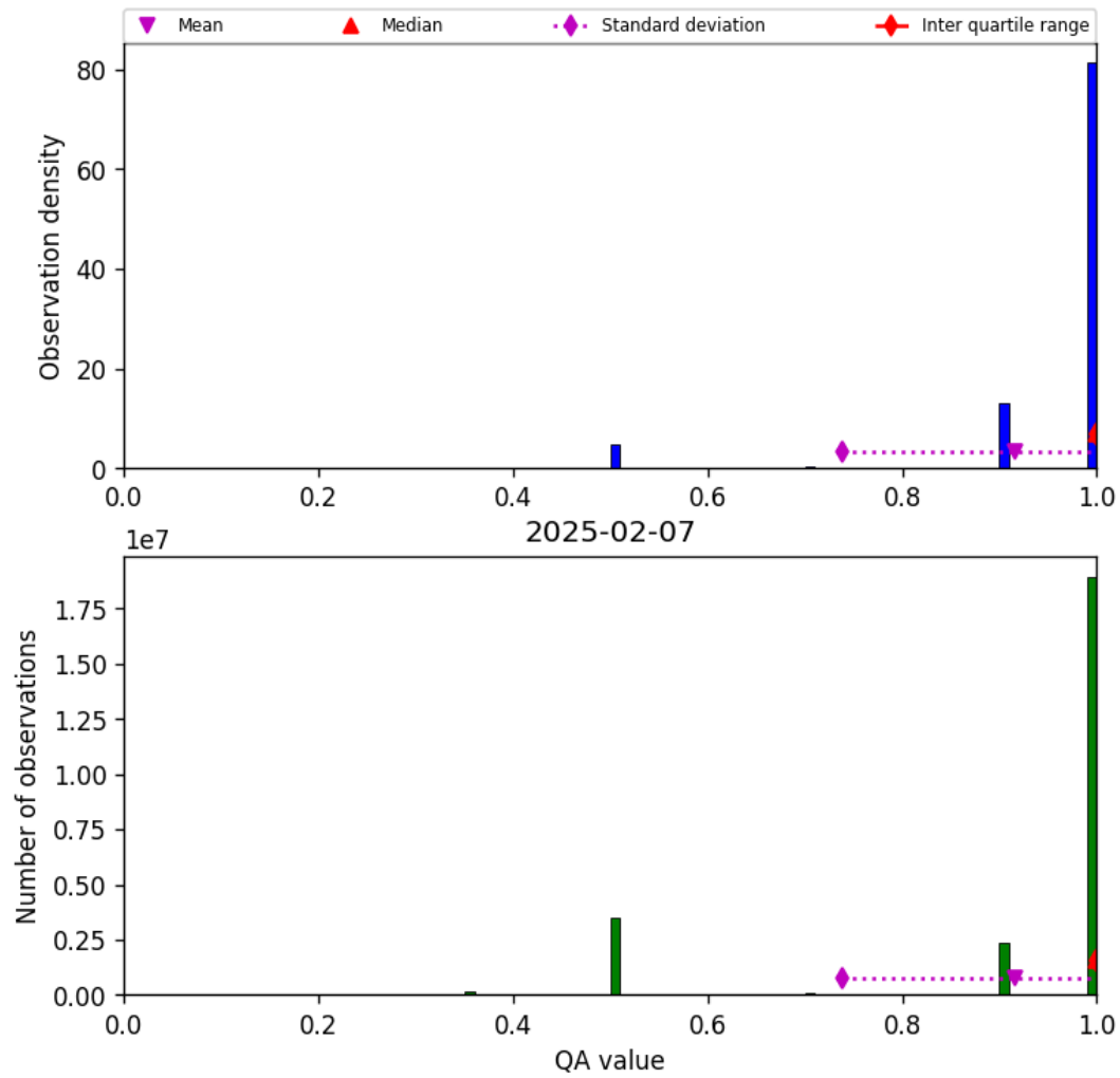
Figure 27: Histogram of “QA value” for 2025-02-07 to 2025-02-08
