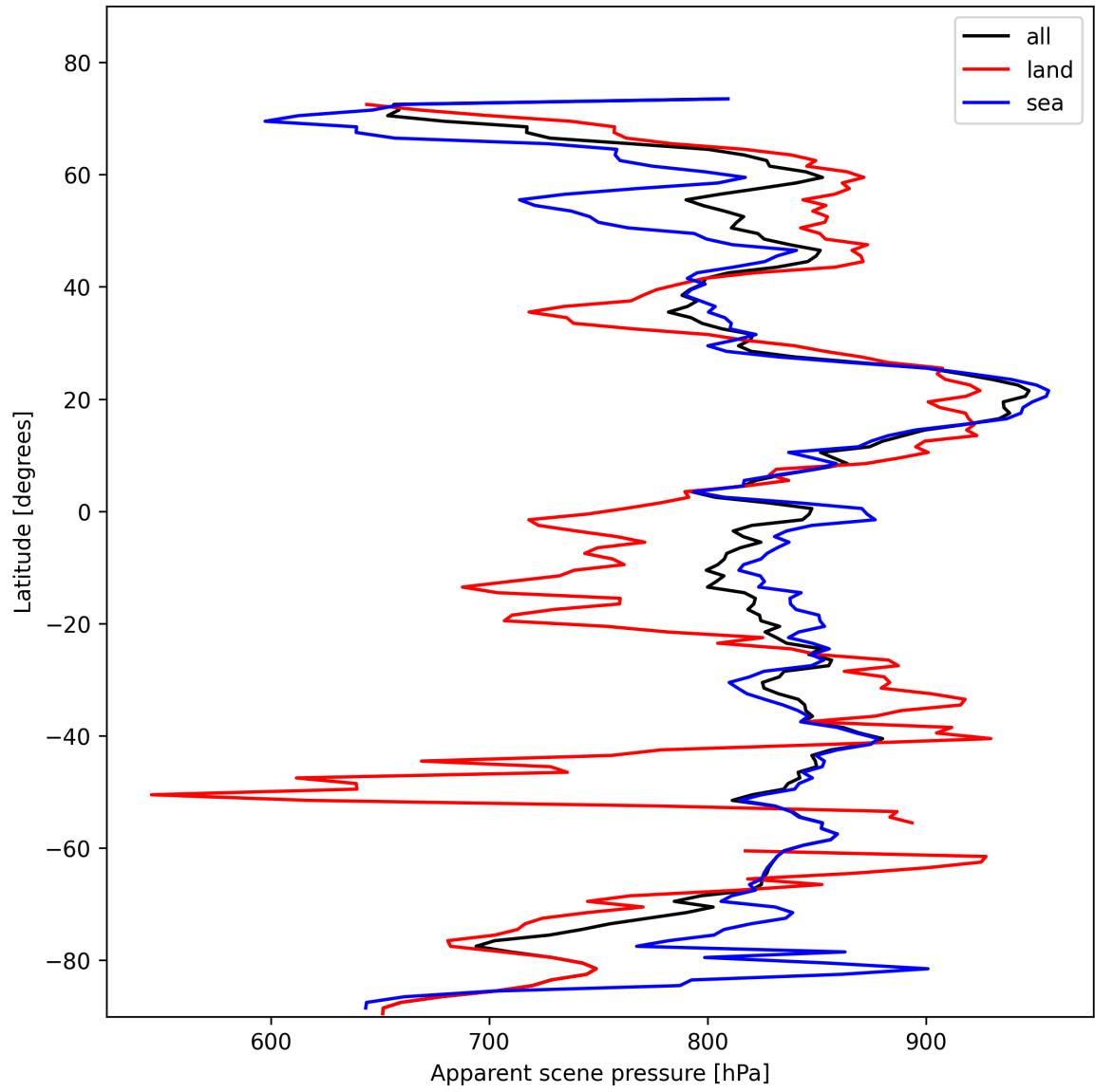
Figure 17: Zonal average of “Apparent scene pressure” for 2025-02-07 to 2025-02-08.
