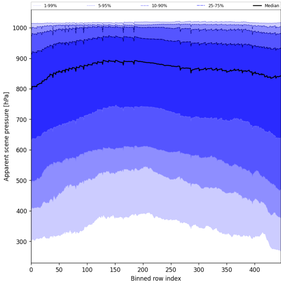
Figure 51: Along track statistics of “Apparent scene pressure” for 2025-02-07 to 2025-02-08
