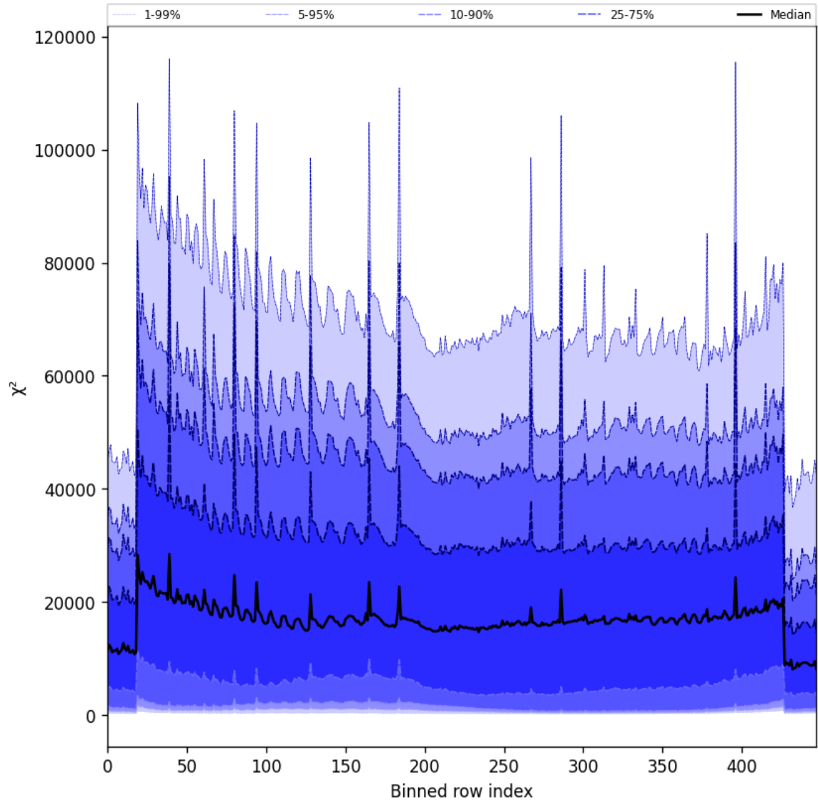
Figure 53: Along track statistics of “ \chi^2 ” for 2025-02-07 to 2025-02-08
