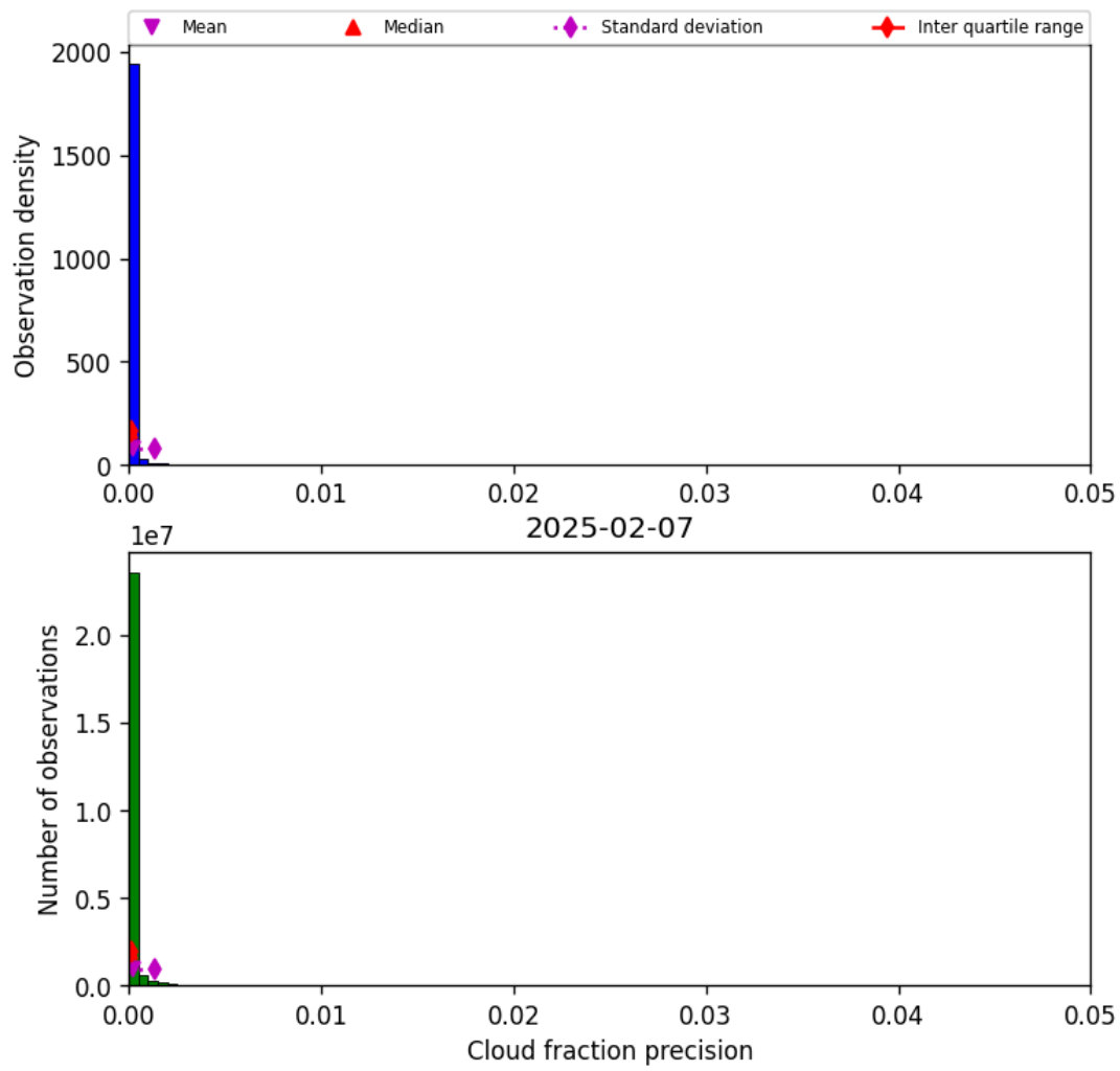
Figure 31: Histogram of “Cloud fraction precision” for 2025-02-07 to 2025-02-08
