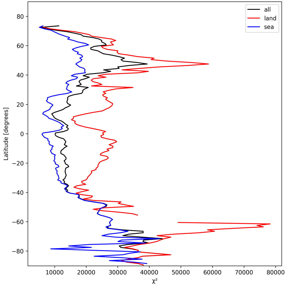
Figure 19: Zonal average of “ \chi^2 ” for 2025-02-07 to 2025-02-08.
