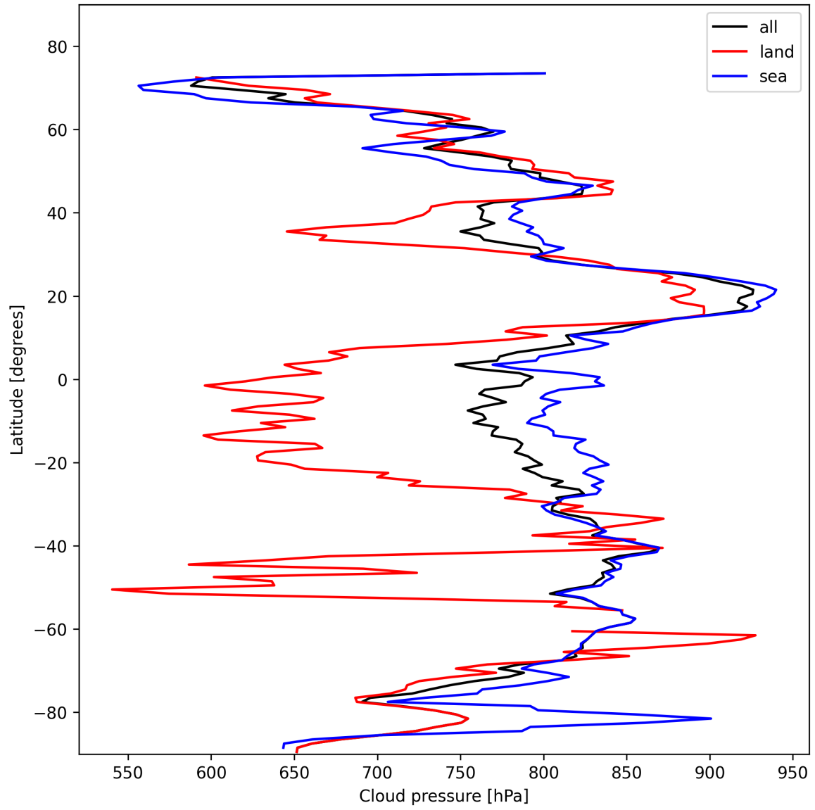
Figure 11: Zonal average of “Cloud pressure” for 2025-02-07 to 2025-02-08.
