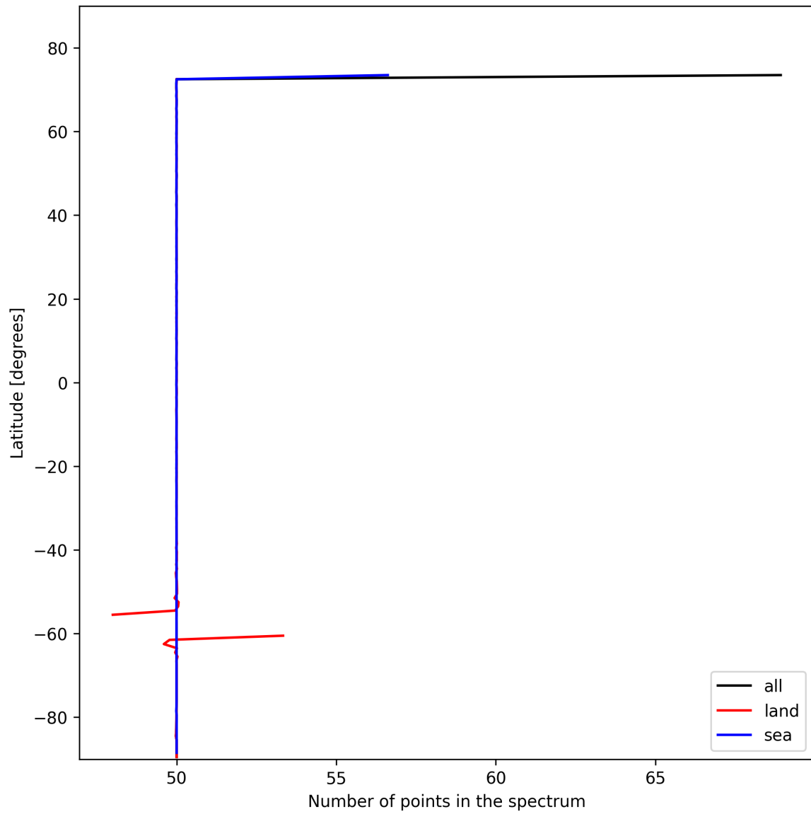
Figure 25: Zonal average of “Number of points in the spectrum” for 2025-02-07 to 2025-02-08.
