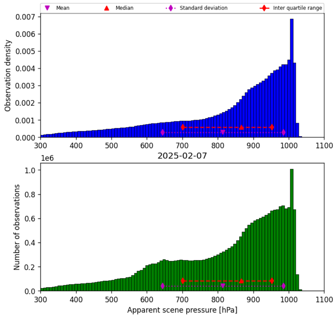
Figure 34: Histogram of “Apparent scene pressure” for 2025-02-07 to 2025-02-08
