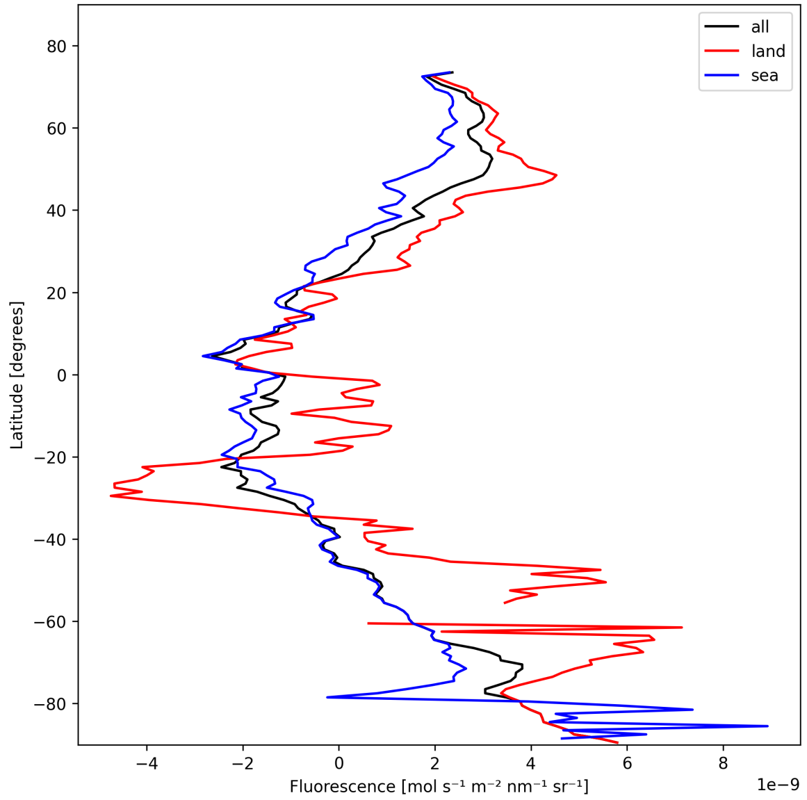
Figure 21: Zonal average of “Fluorescence” for 2025-02-07 to 2025-02-08.
