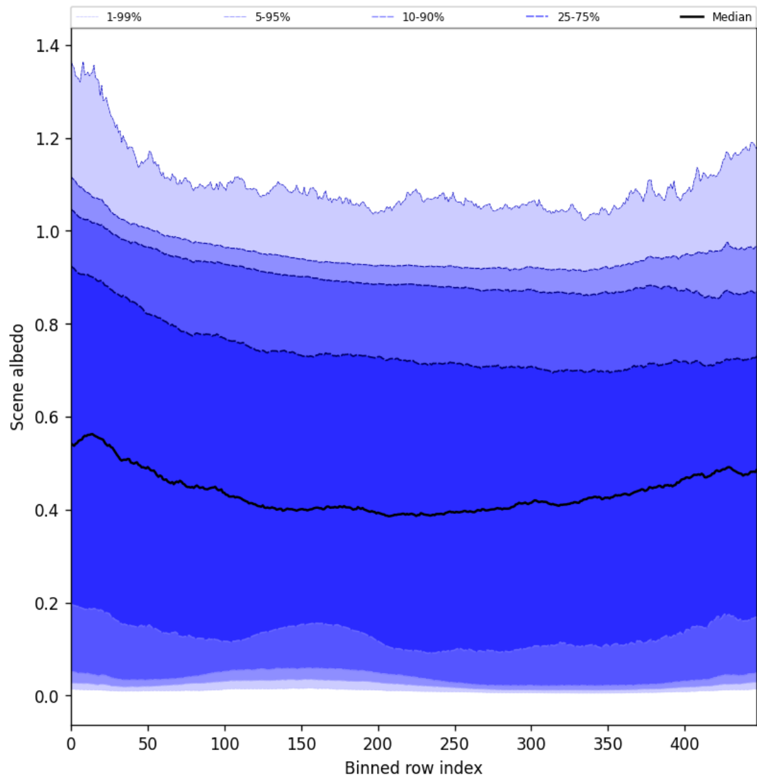
Figure 49: Along track statistics of “Scene albedo” for 2025-02-07 to 2025-02-08
