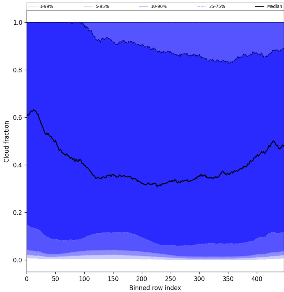
Figure 47: Along track statistics of “Cloud fraction” for 2025-02-07 to 2025-02-08
