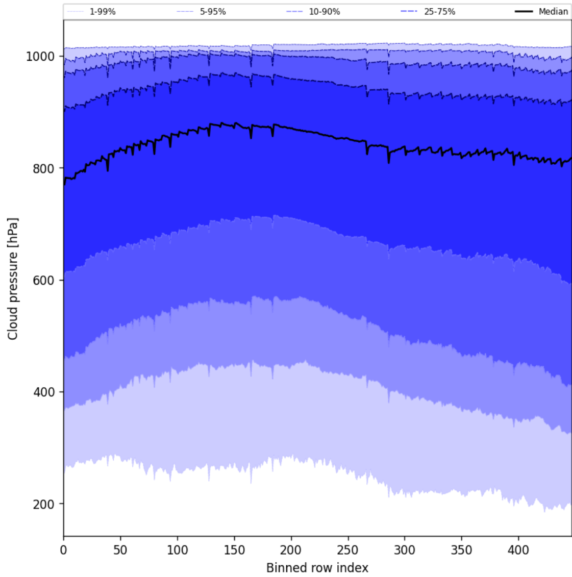
Figure 45: Along track statistics of “Cloud pressure” for 2025-02-07 to 2025-02-08
