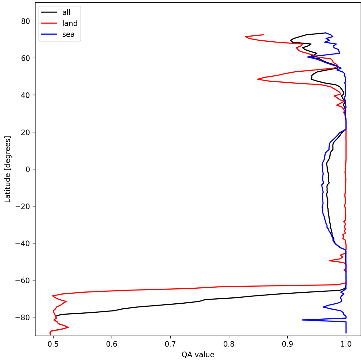
Figure 10: Zonal average of “QA value” for 2025-02-07 to 2025-02-08.
