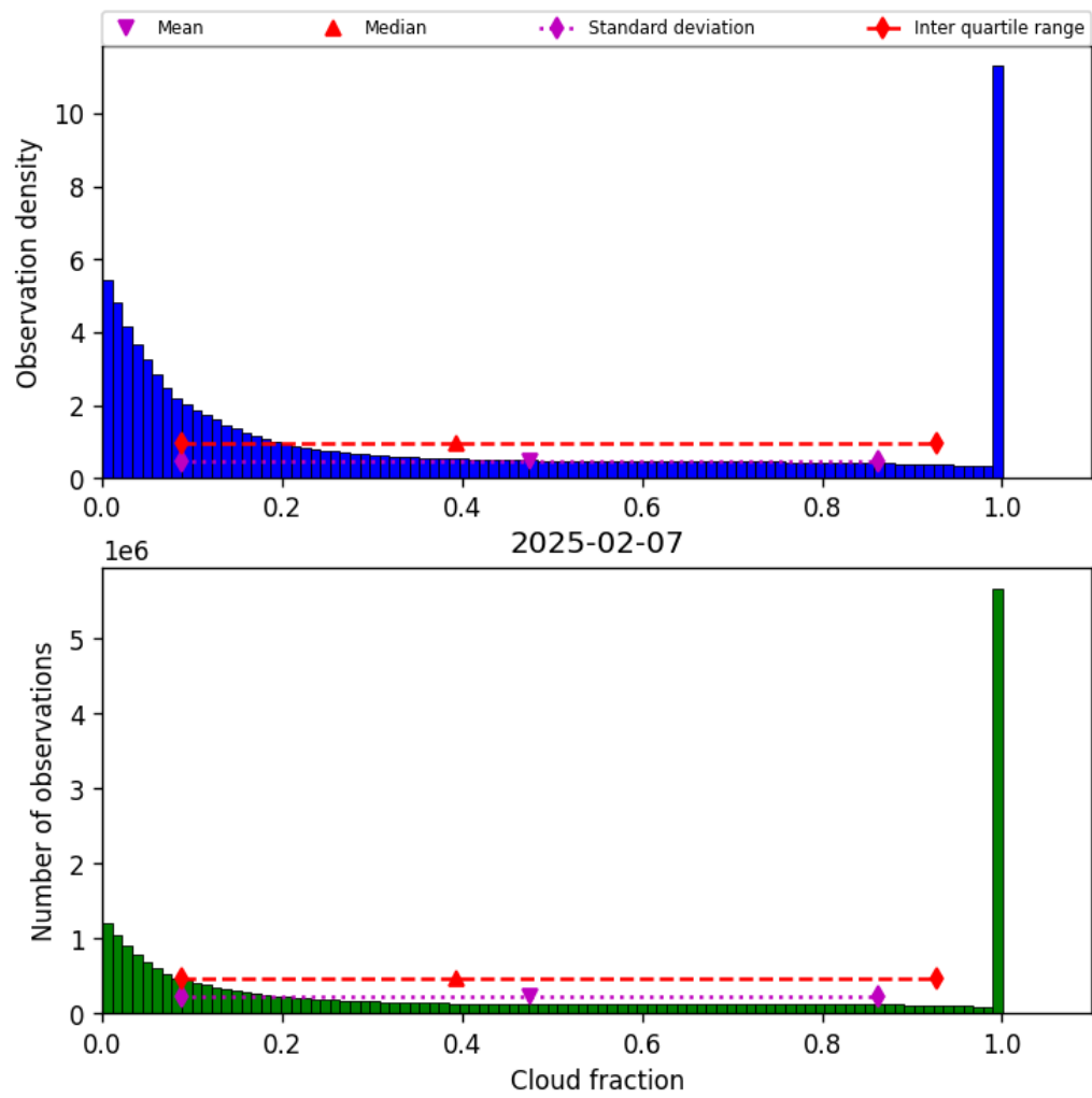
Figure 30: Histogram of “Cloud fraction” for 2025-02-07 to 2025-02-08
