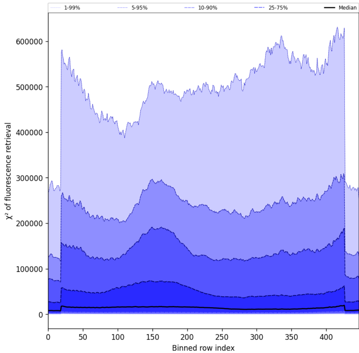
Figure 57: Along track statistics of “ \chi^2 of fluorescence retrieval” for 2025-02-07 to 2025-02-08
