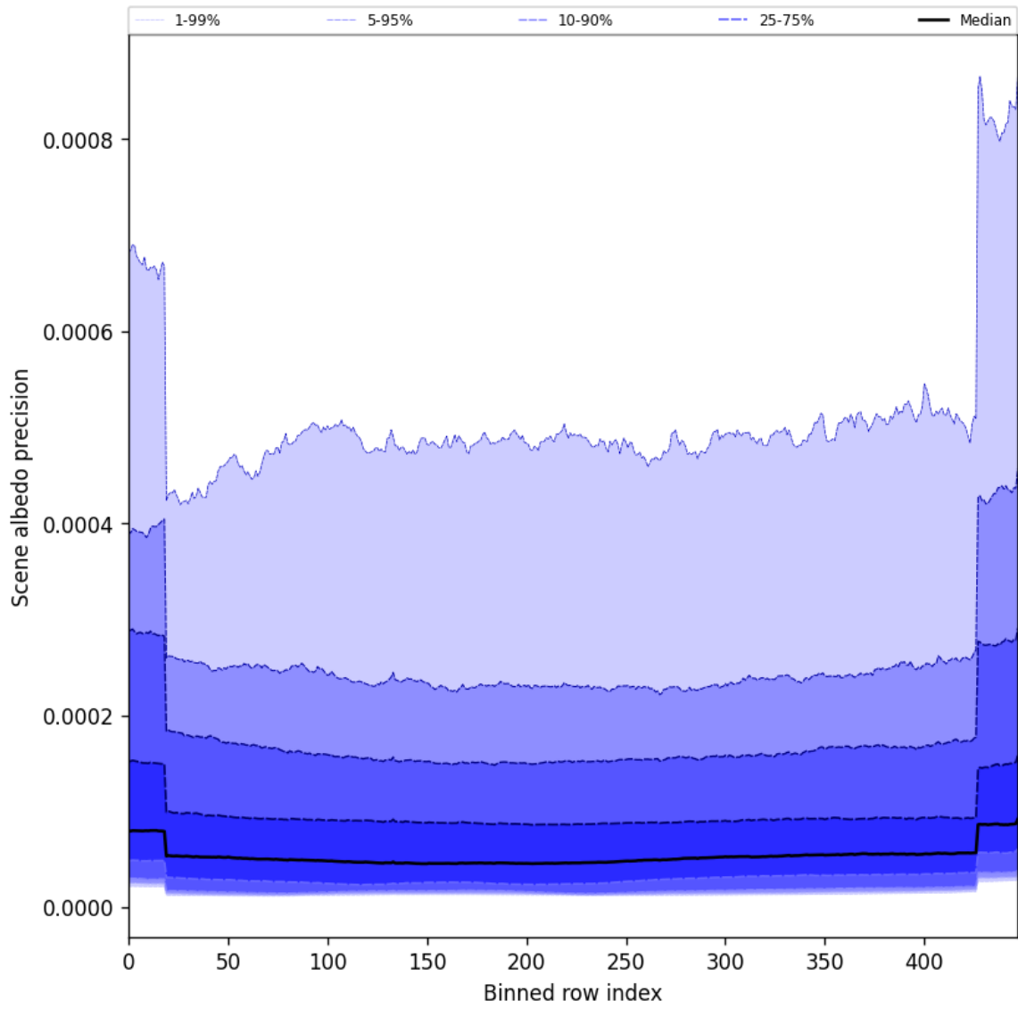
Figure 50: Along track statistics of “Scene albedo precision” for 2025-02-07 to 2025-02-08
