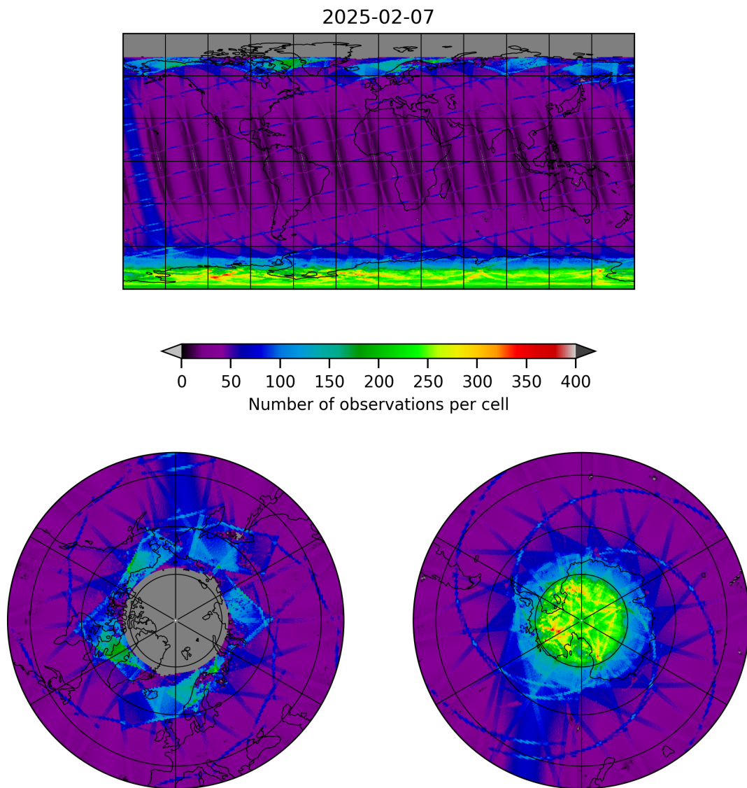
Figure 9: Map of the number of observations for 2025-02-07 to 2025-02-08
