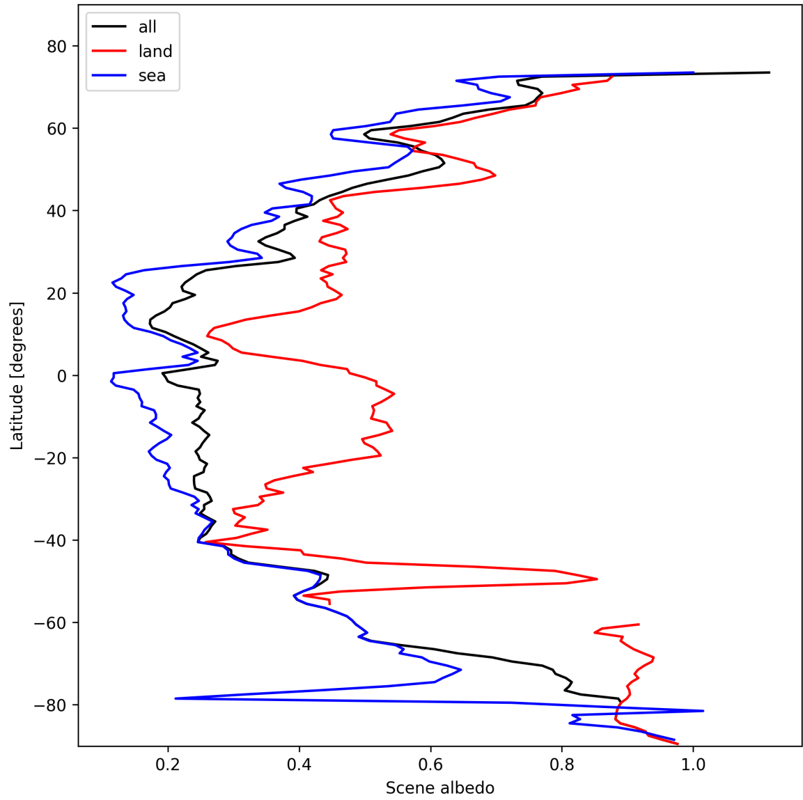
Figure 15: Zonal average of “Scene albedo” for 2025-02-07 to 2025-02-08.
