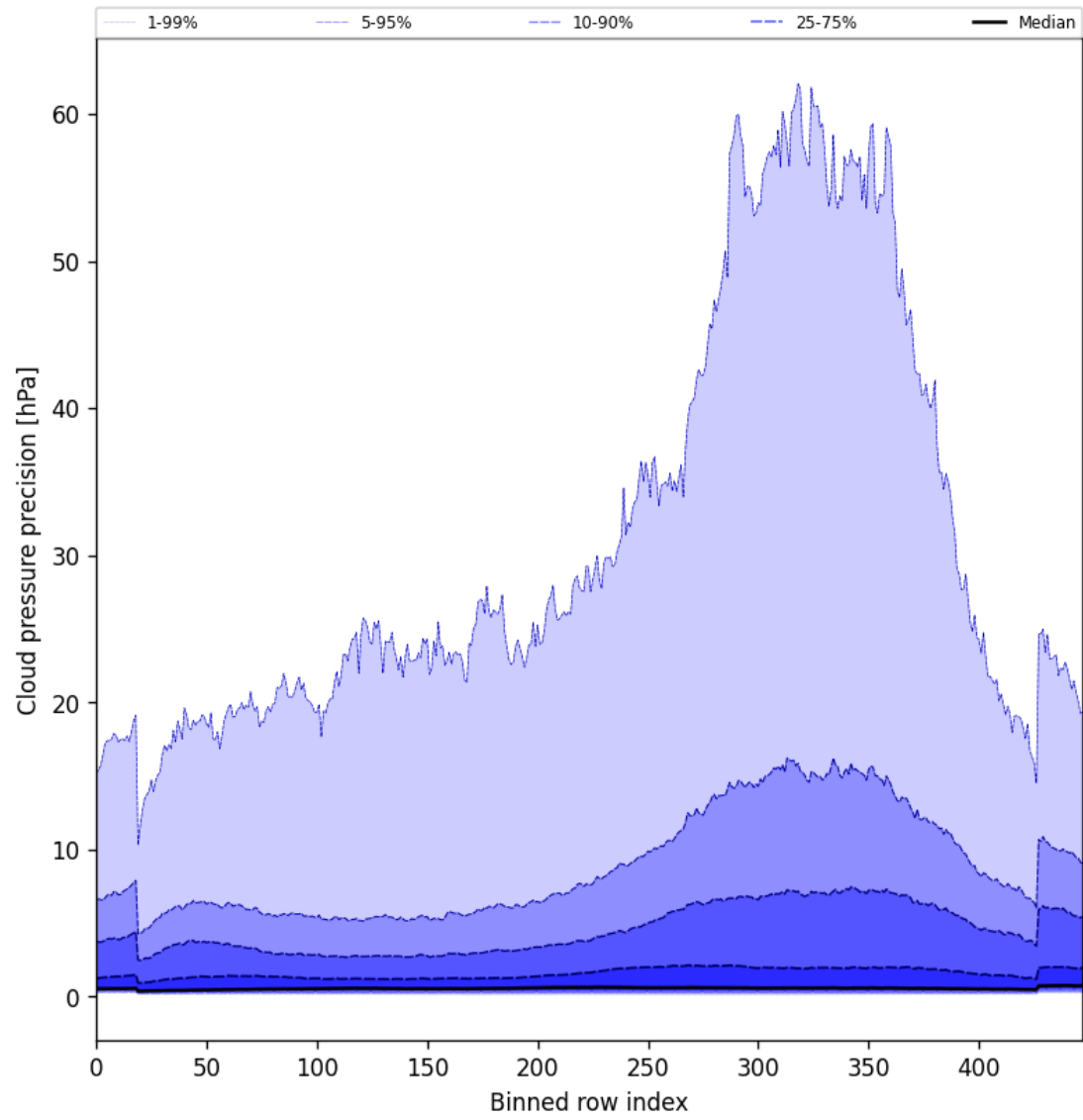
Figure 46: Along track statistics of “Cloud pressure precision” for 2025-02-07 to 2025-02-08
