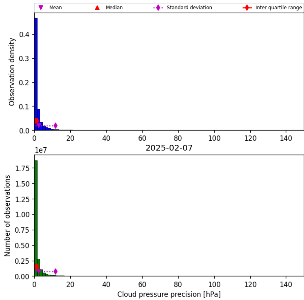
Figure 29: Histogram of “Cloud pressure precision” for 2025-02-07 to 2025-02-08
