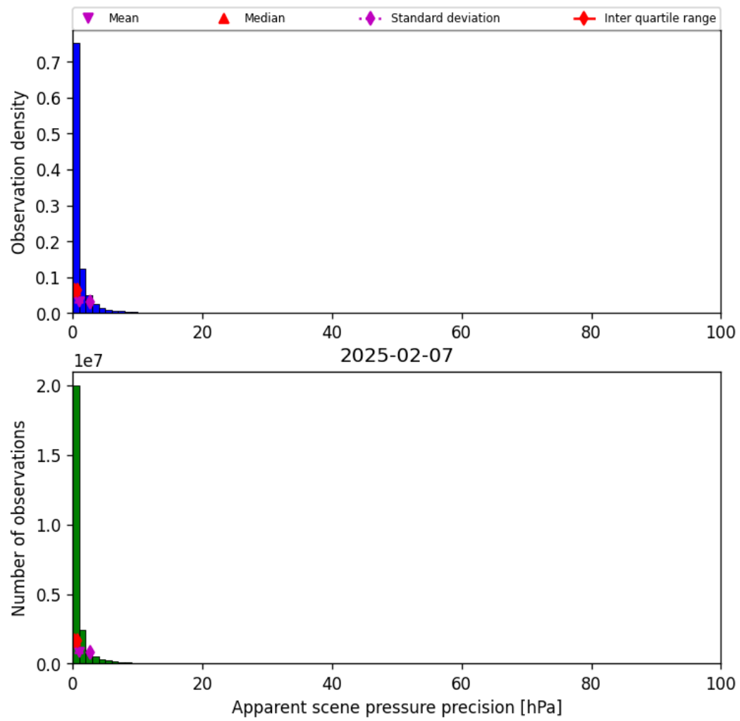
Figure 35: Histogram of “Apparent scene pressure precision” for 2025-02-07 to 2025-02-08
