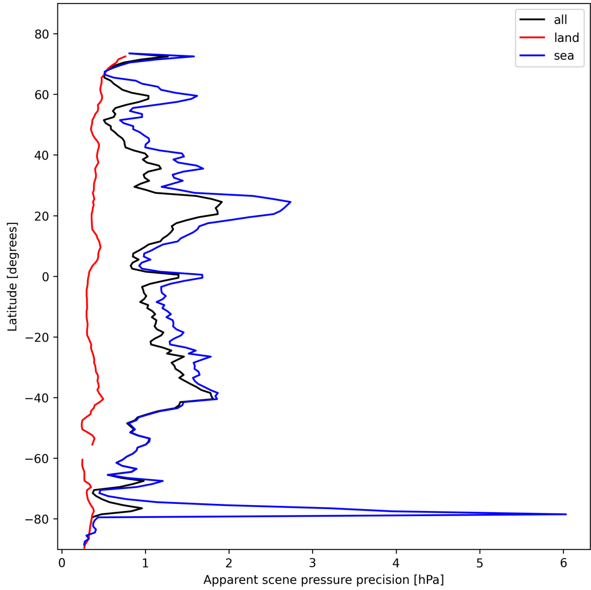
Figure 18: Zonal average of “Apparent scene pressure precision” for 2025-02-07 to 2025-02-08.
