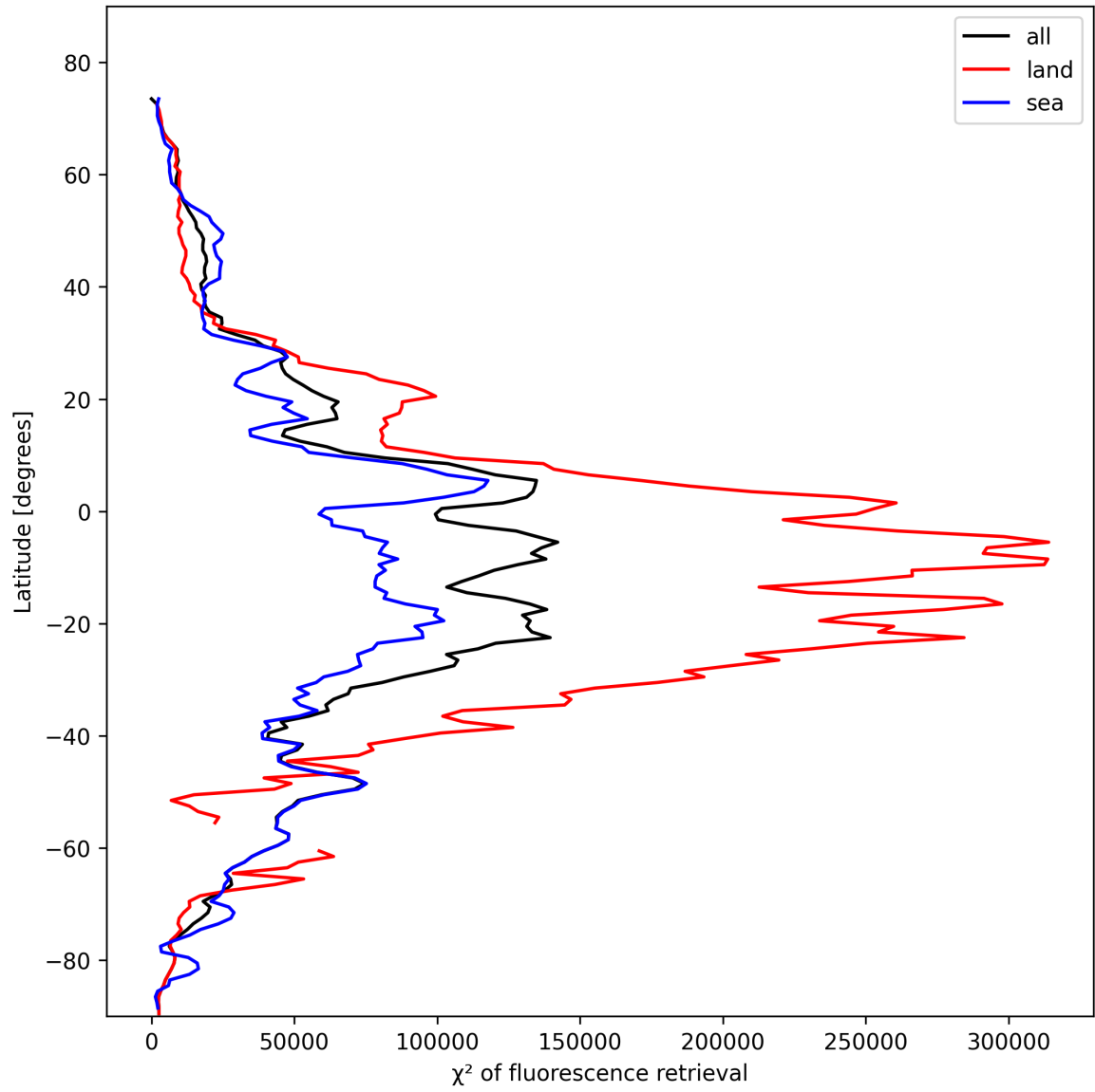
Figure 23: Zonal average of “ \chi^2 of fluorescence retrieval” for 2025-02-07 to 2025-02-08.
