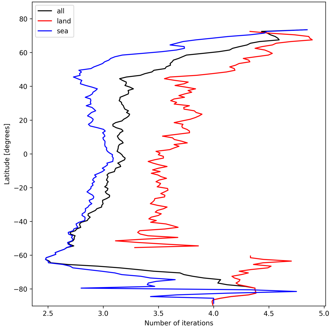
Figure 20: Zonal average of “Number of iterations” for 2025-02-07 to 2025-02-08.
