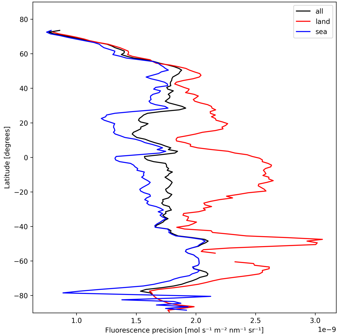
Figure 22: Zonal average of “Fluorescence precision” for 2025-02-07 to 2025-02-08.
