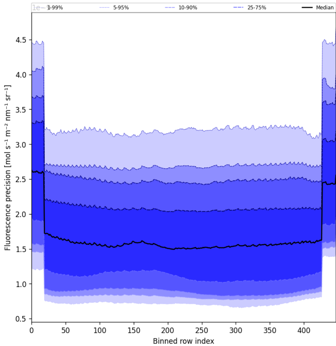
Figure 56: Along track statistics of “Fluorescence precision” for 2025-02-07 to 2025-02-08
