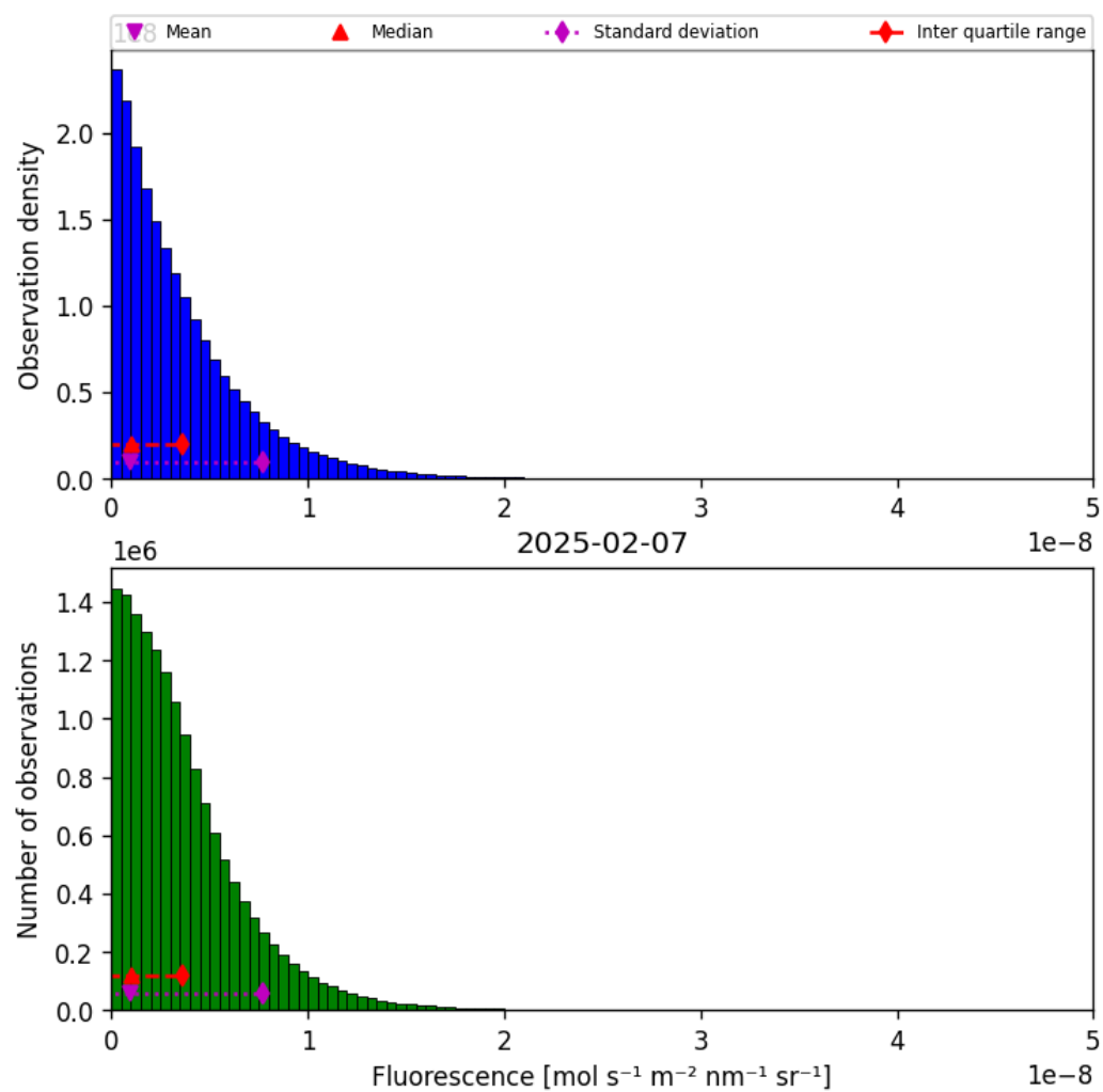
Figure 38: Histogram of “Fluorescence” for 2025-02-07 to 2025-02-08
