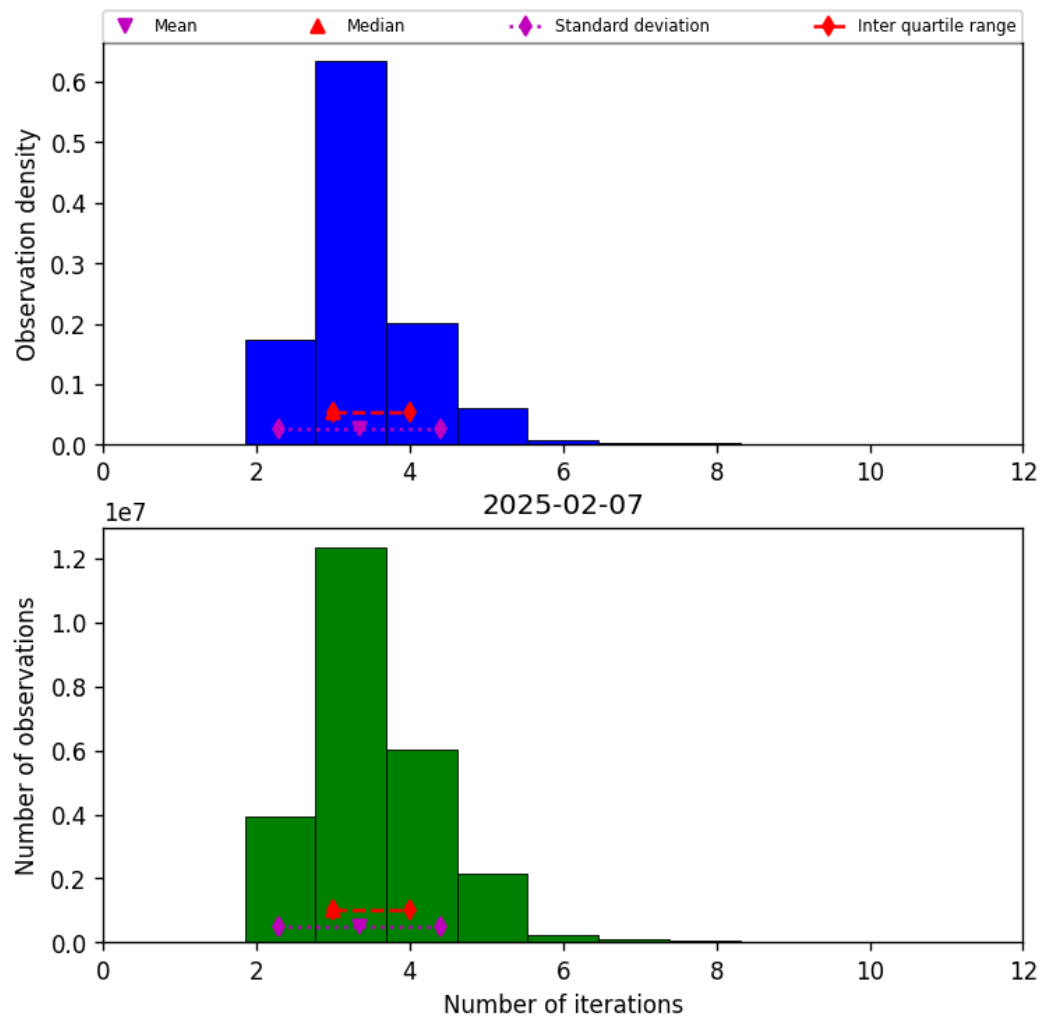
Figure 37: Histogram of “Number of iterations” for 2025-02-07 to 2025-02-08
