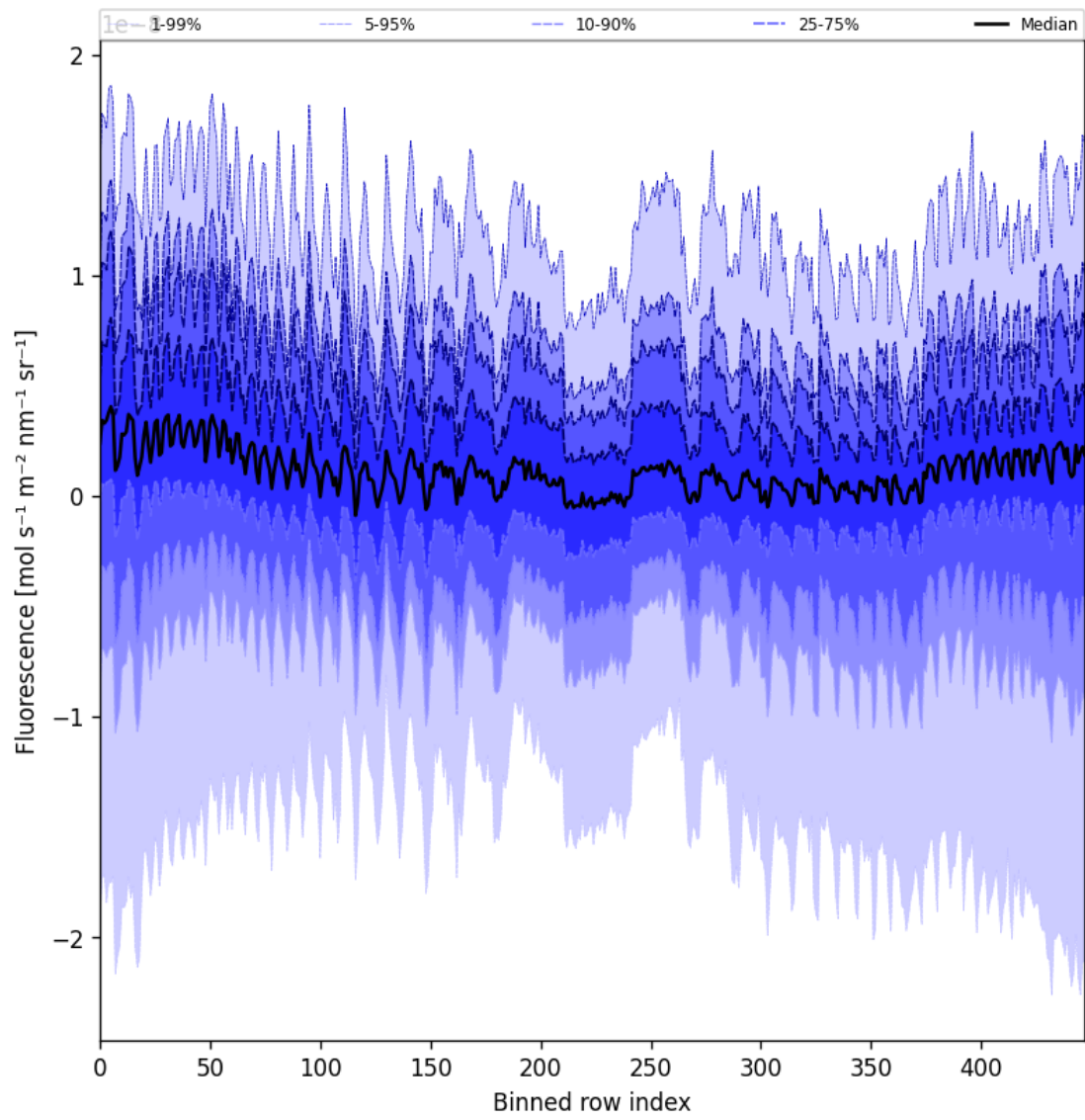
Figure 55: Along track statistics of “Fluorescence” for 2025-02-07 to 2025-02-08
