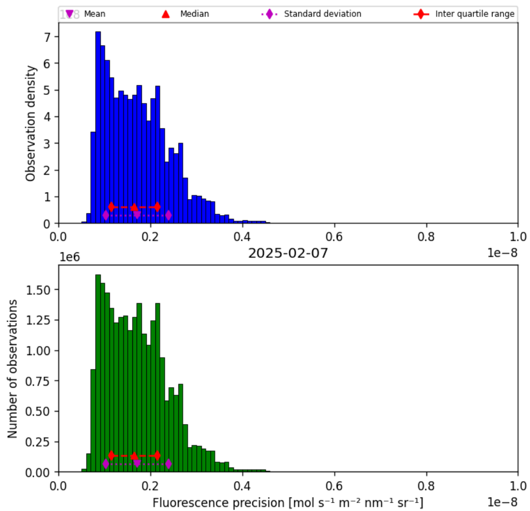
Figure 39: Histogram of “Fluorescence precision” for 2025-02-07 to 2025-02-08
