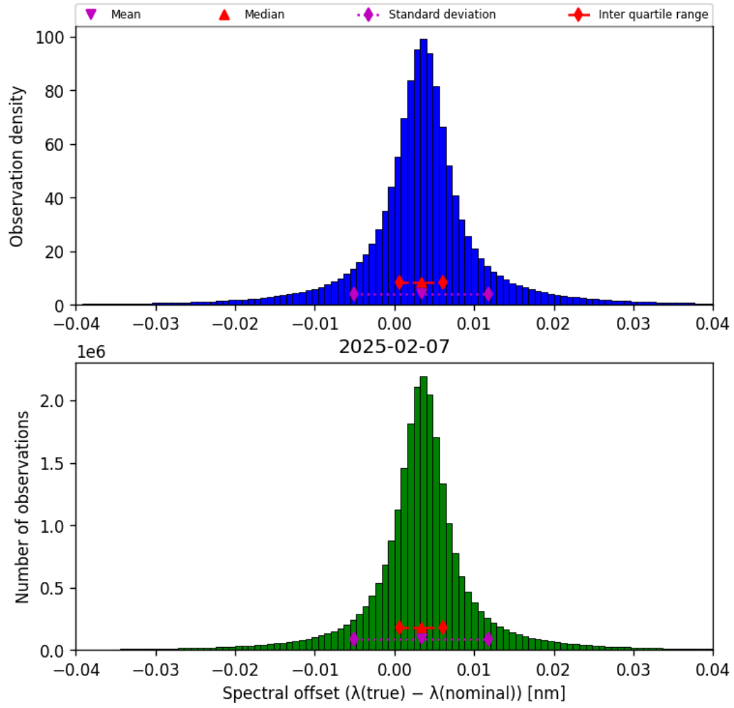
Figure 43: Histogram of “Spectral offset ( \lambda_{\text{true}} - \lambda_{\text{nominal}} )” for 2025-02-07 to 2025-02-08
