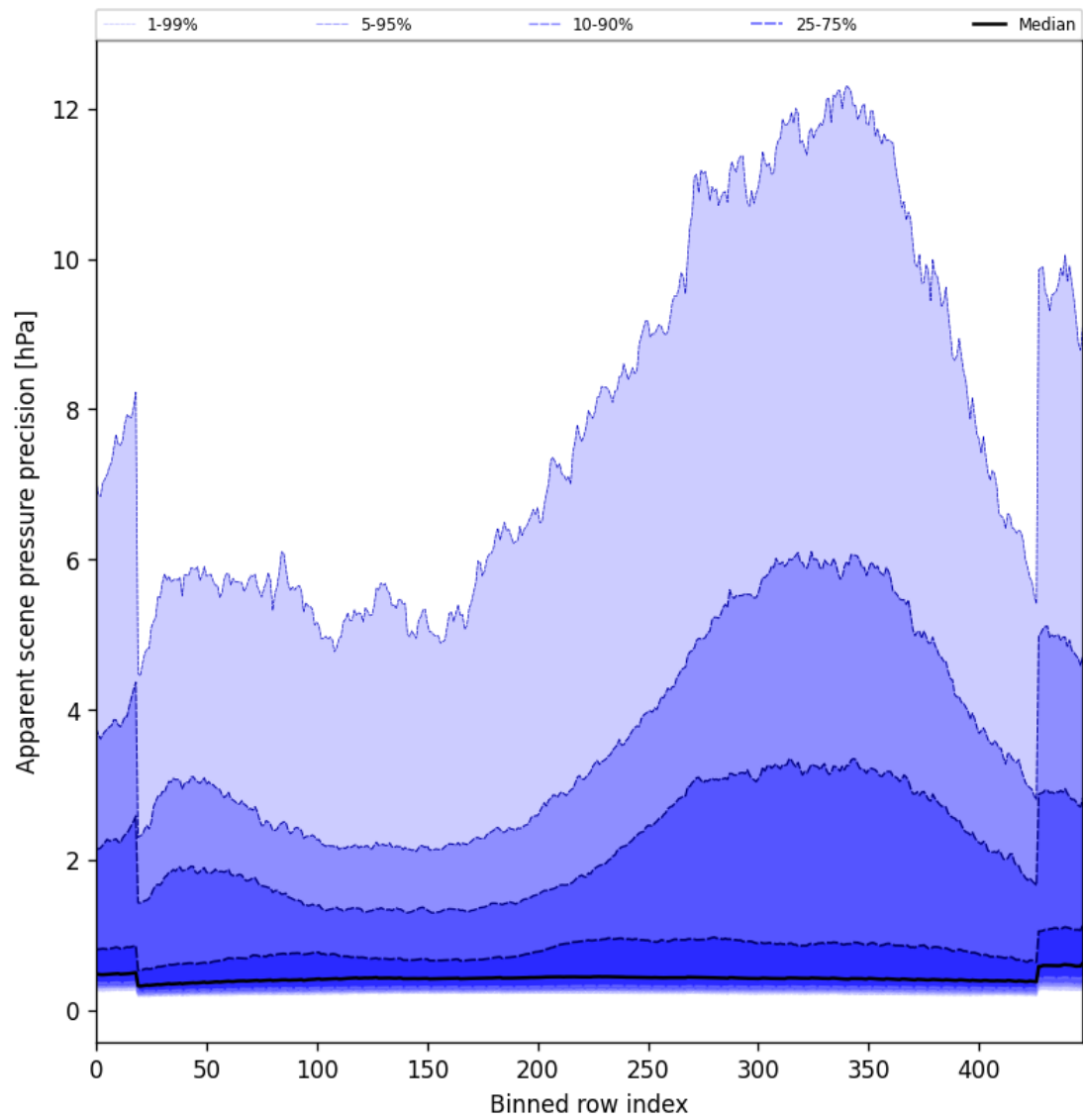
Figure 52: Along track statistics of “Apparent scene pressure precision” for 2025-02-07 to 2025-02-08
