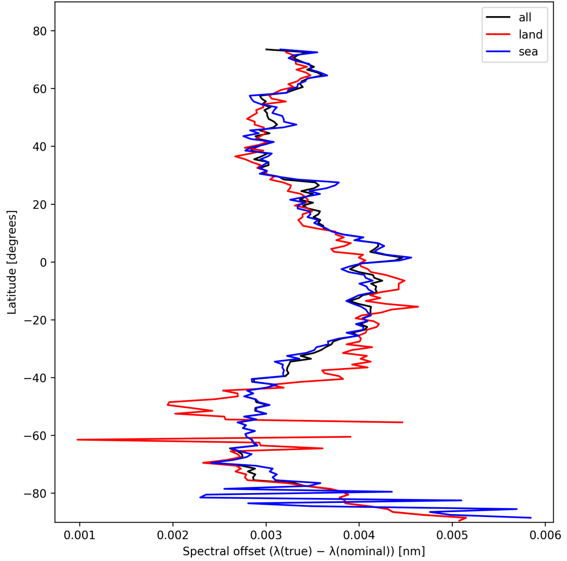
Figure 26: Zonal average of “Spectral offset ( \lambda_{\text{true}} - \lambda_{\text{nominal}} )” for 2025-02-07 to 2025-02-08.
