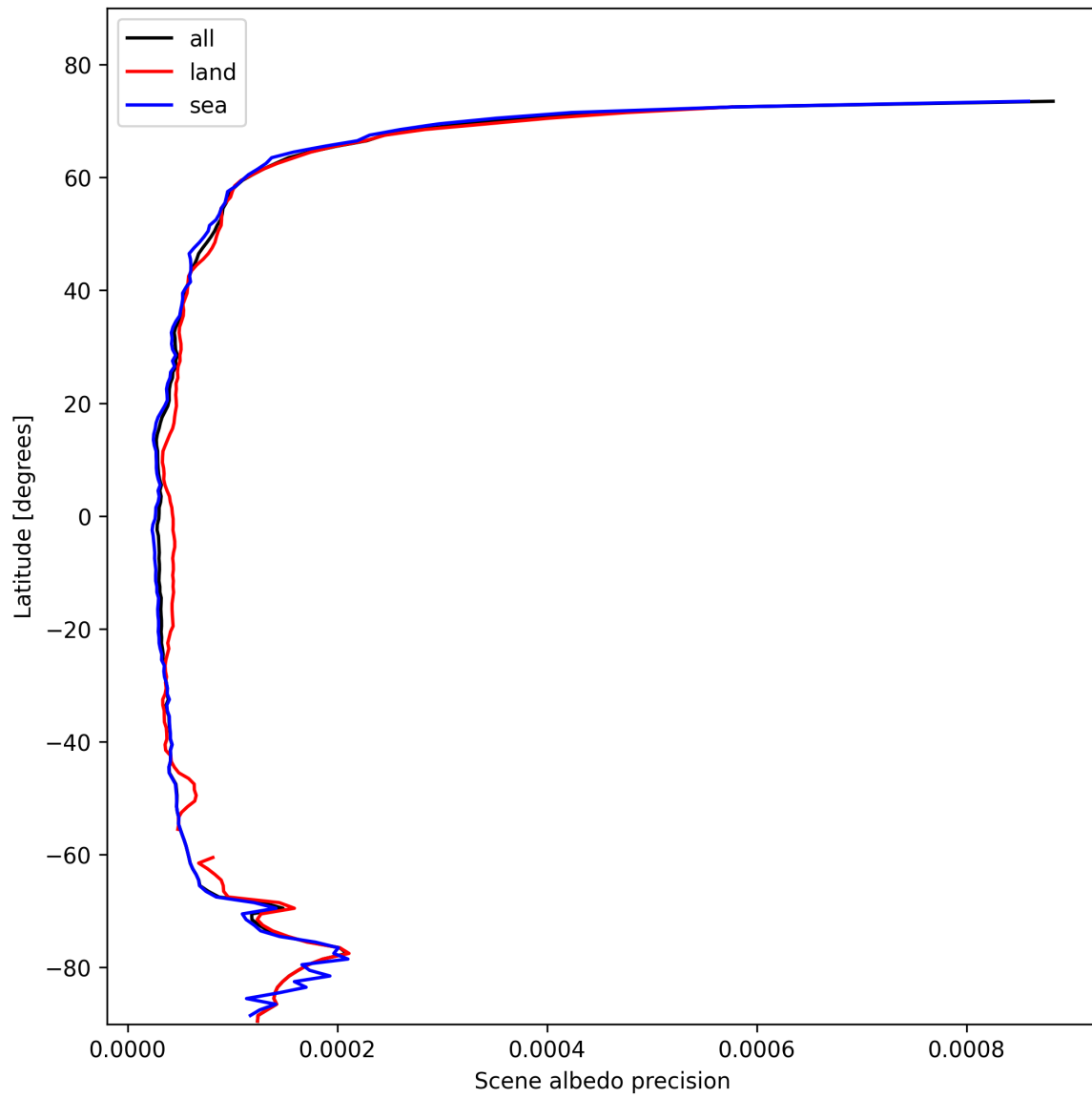
Figure 16: Zonal average of “Scene albedo precision” for 2025-02-07 to 2025-02-08.
