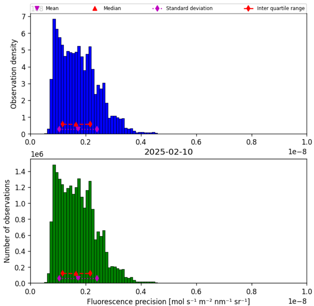
Figure 39: Histogram of “Fluorescence precision” for 2025-02-10 to 2025-02-11
