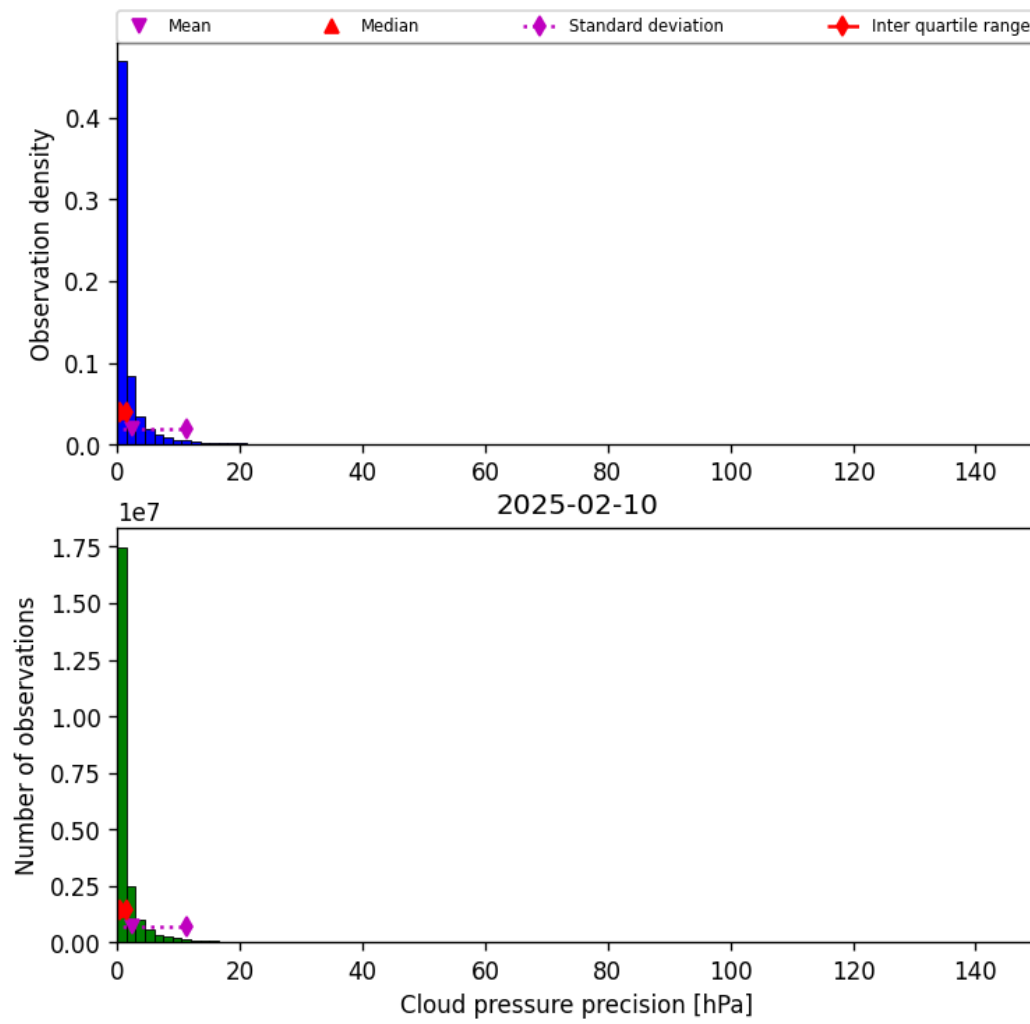
Figure 29: Histogram of “Cloud pressure precision” for 2025-02-10 to 2025-02-11
