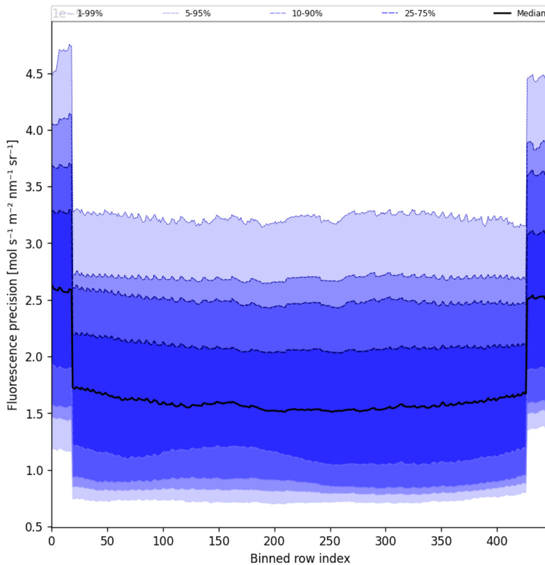
Figure 56: Along track statistics of “Fluorescence precision” for 2025-02-10 to 2025-02-11
