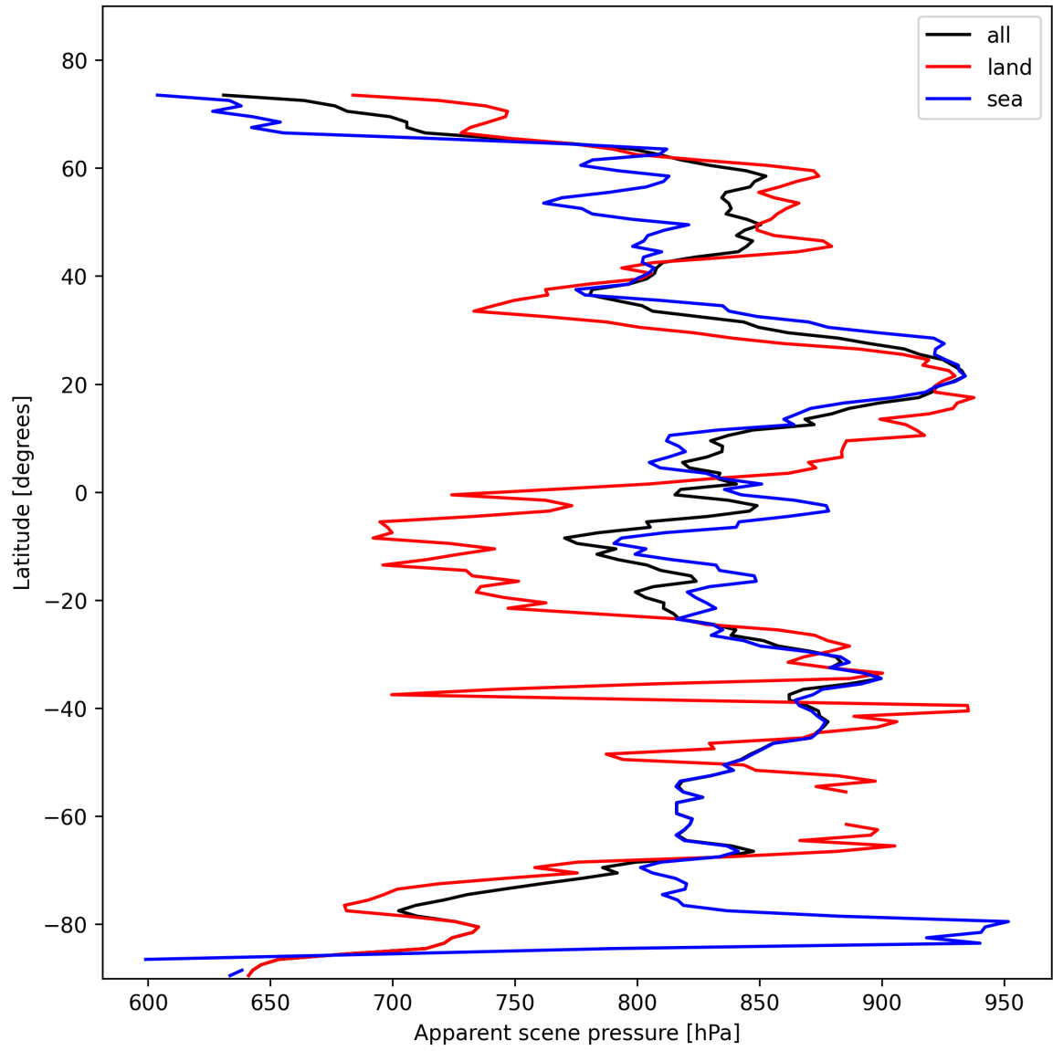
Figure 17: Zonal average of “Apparent scene pressure” for 2025-02-10 to 2025-02-11.
