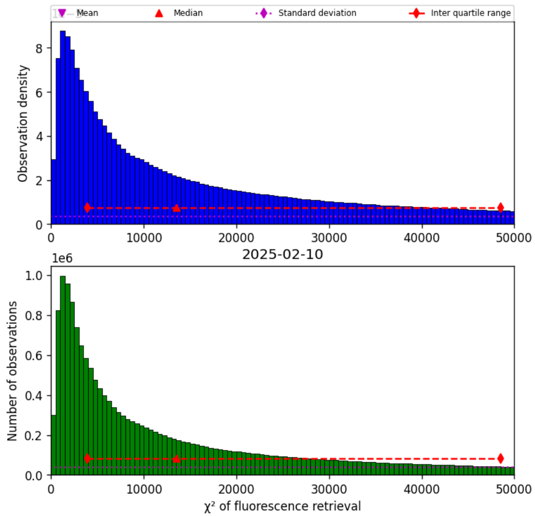
Figure 40: Histogram of “ \chi^2 of fluorescence retrieval” for 2025-02-10 to 2025-02-11
