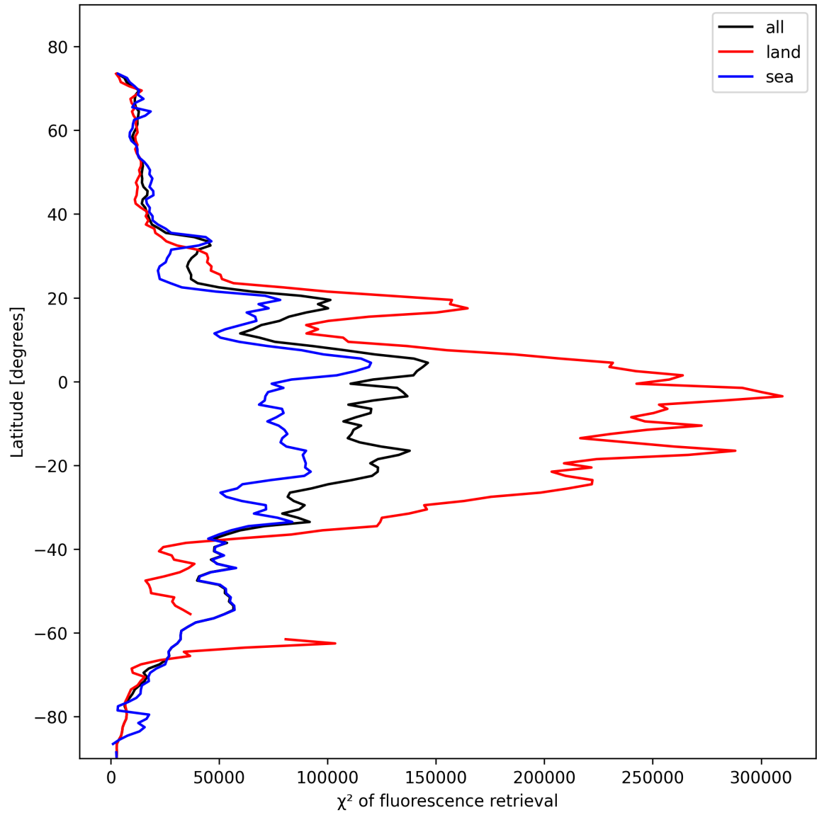
Figure 23: Zonal average of “ \chi^2 of fluorescence retrieval” for 2025-02-10 to 2025-02-11.
