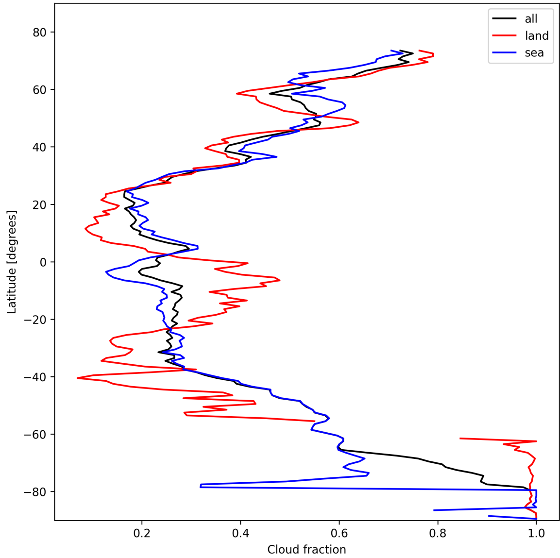
Figure 13: Zonal average of “Cloud fraction” for 2025-02-10 to 2025-02-11.
