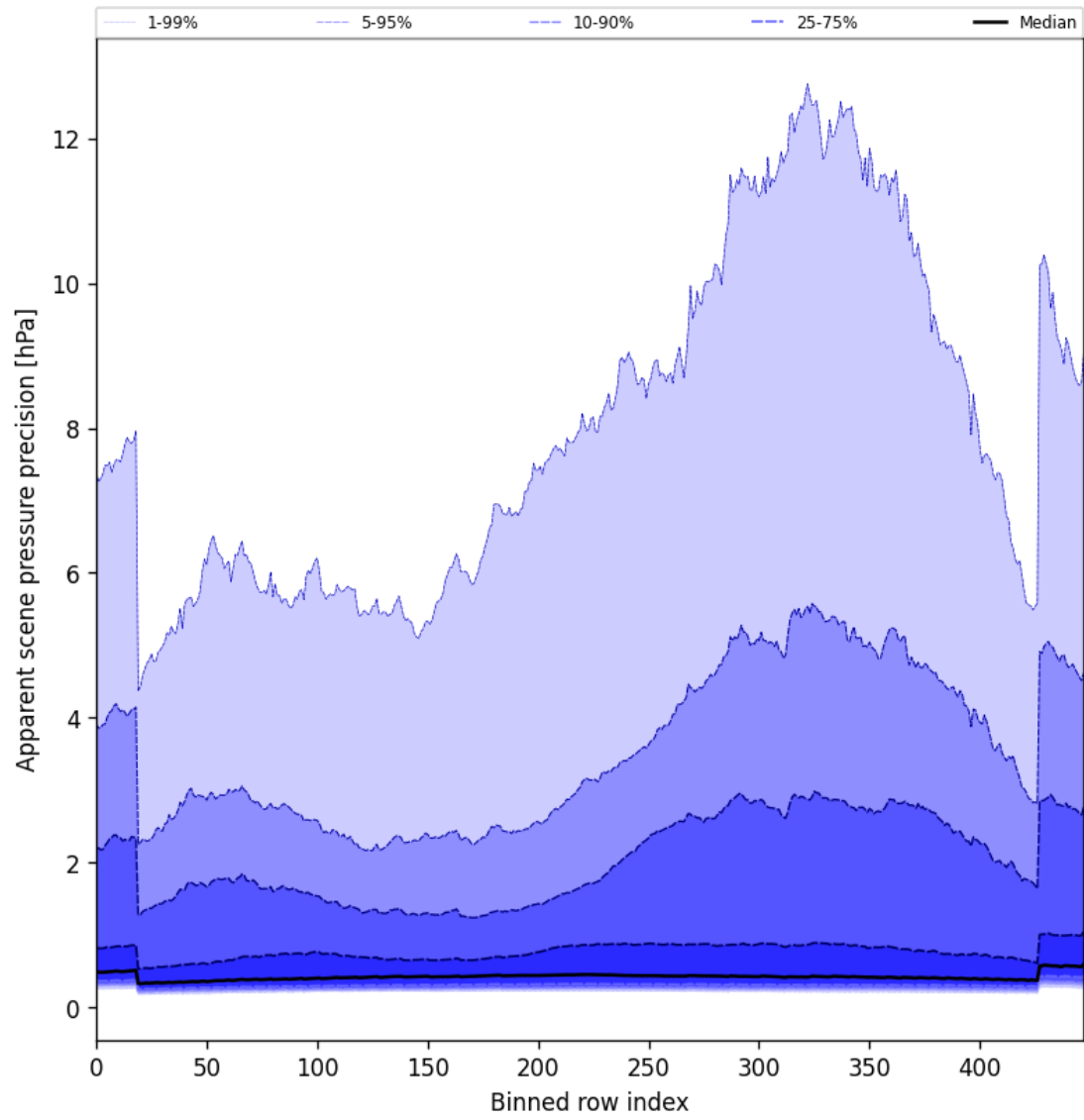
Figure 52: Along track statistics of “Apparent scene pressure precision” for 2025-02-10 to 2025-02-11
