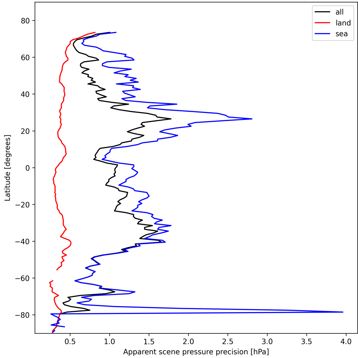
Figure 18: Zonal average of “Apparent scene pressure precision” for 2025-02-10 to 2025-02-11.
