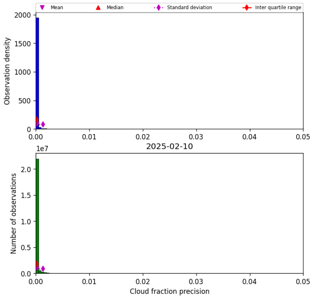
Figure 31: Histogram of “Cloud fraction precision” for 2025-02-10 to 2025-02-11
