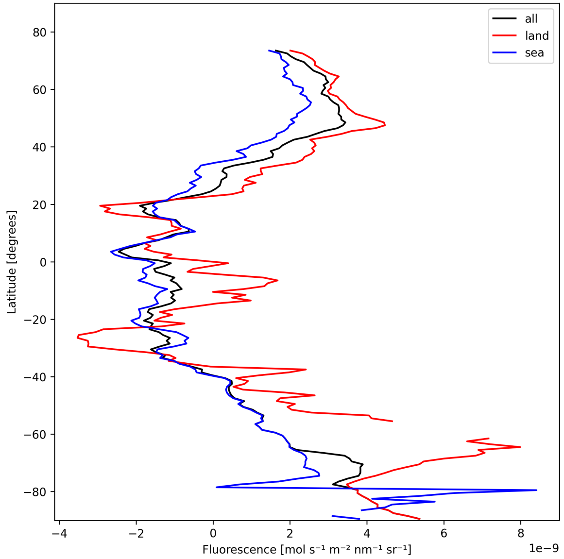
Figure 21: Zonal average of “Fluorescence” for 2025-02-10 to 2025-02-11.
