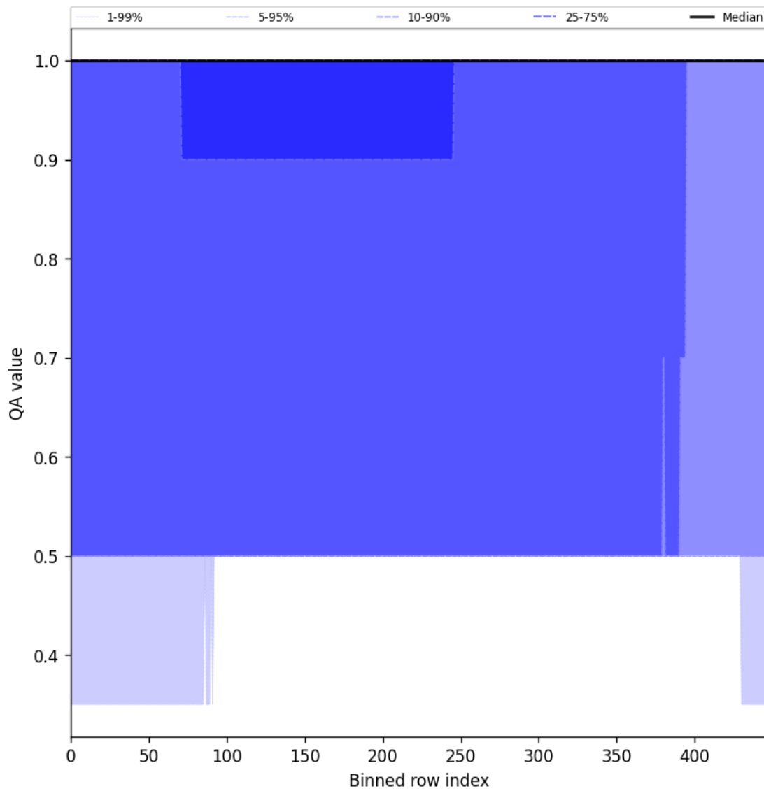
Figure 44: Along track statistics of “QA value” for 2025-02-10 to 2025-02-11
