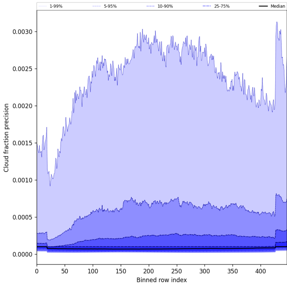
Figure 48: Along track statistics of “Cloud fraction precision” for 2025-02-10 to 2025-02-11
