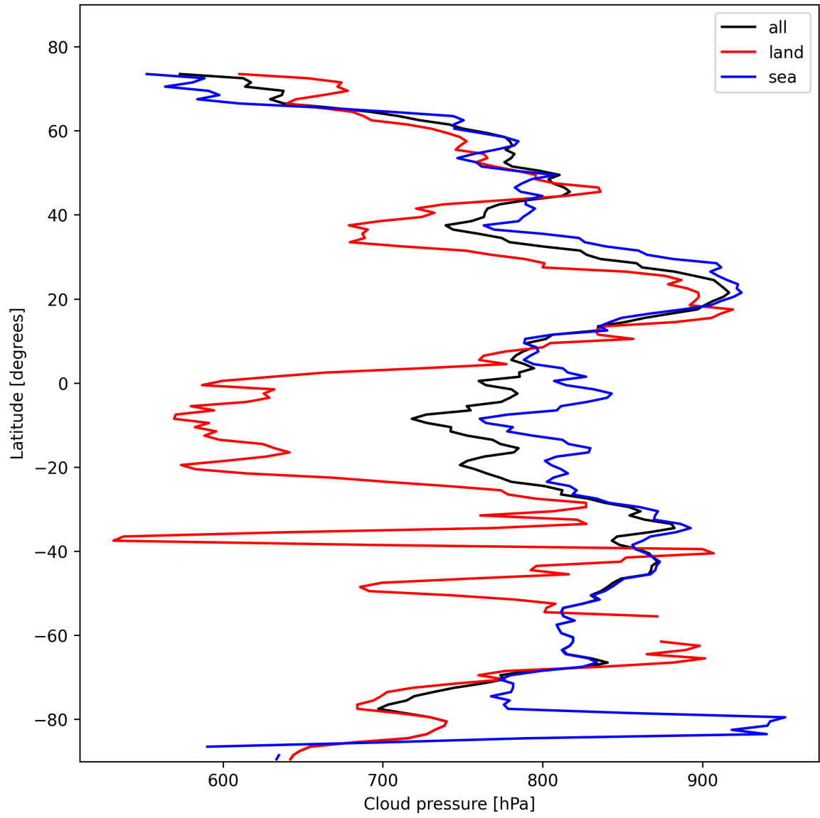
Figure 11: Zonal average of “Cloud pressure” for 2025-02-10 to 2025-02-11.
