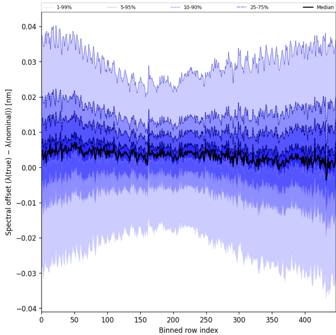
Figure 60: Along track statistics of “Spectral offset ( \lambda_{\text{true}} - \lambda_{\text{nominal}} )” for 2025-02-10 to 2025-02-11
