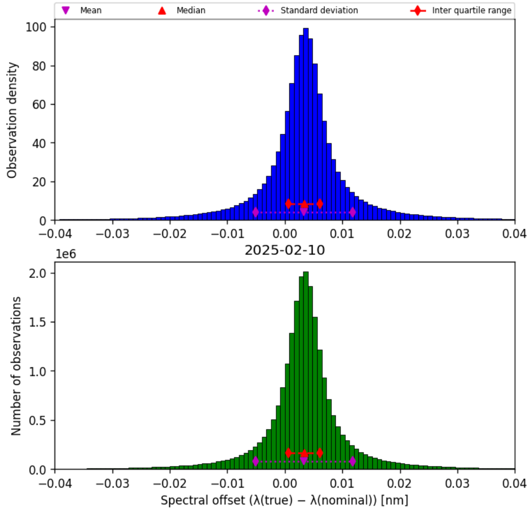
Figure 43: Histogram of “Spectral offset ( \lambda_{\text{true}} - \lambda_{\text{nominal}} )” for 2025-02-10 to 2025-02-11
