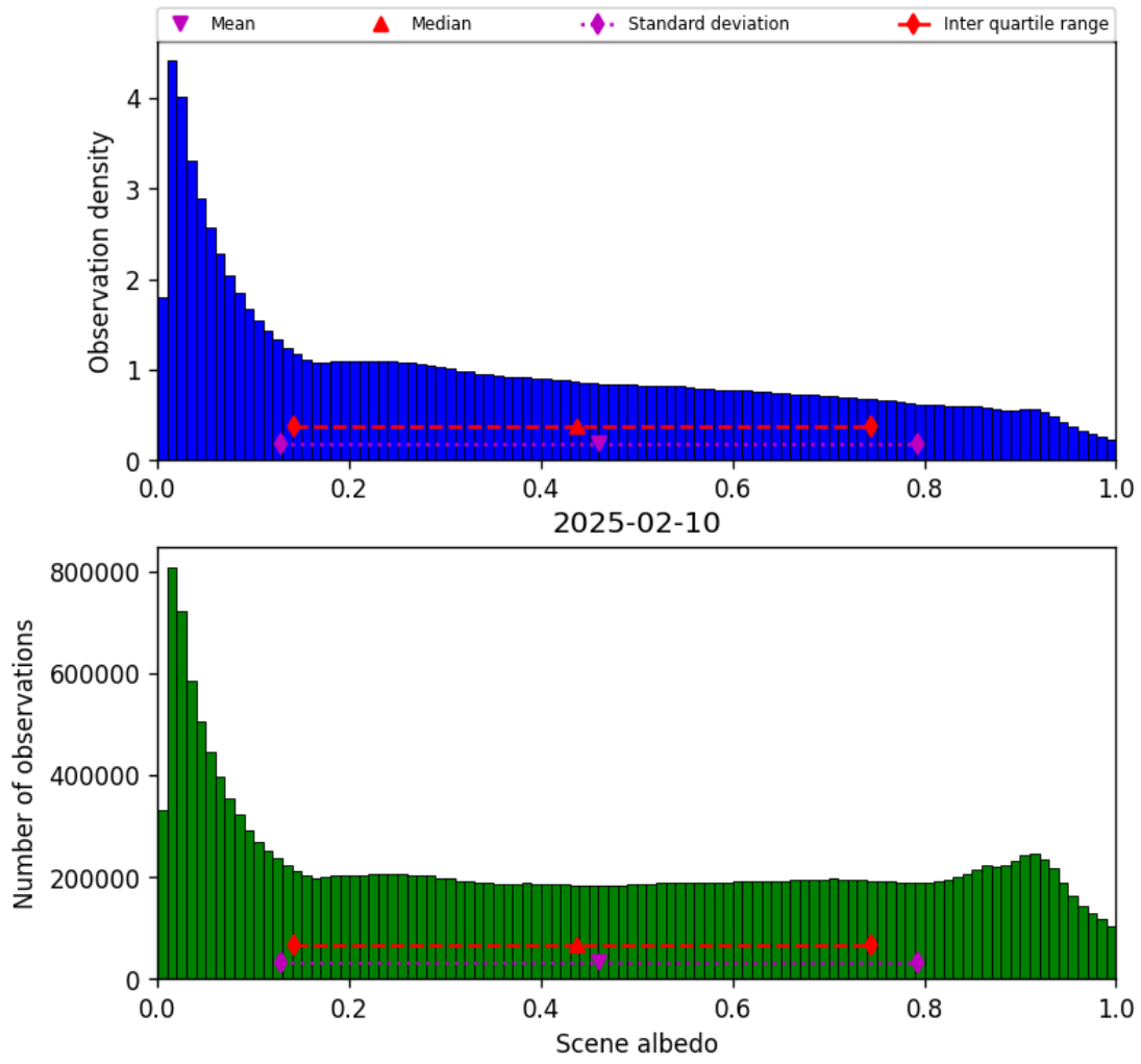
Figure 32: Histogram of “Scene albedo” for 2025-02-10 to 2025-02-11
