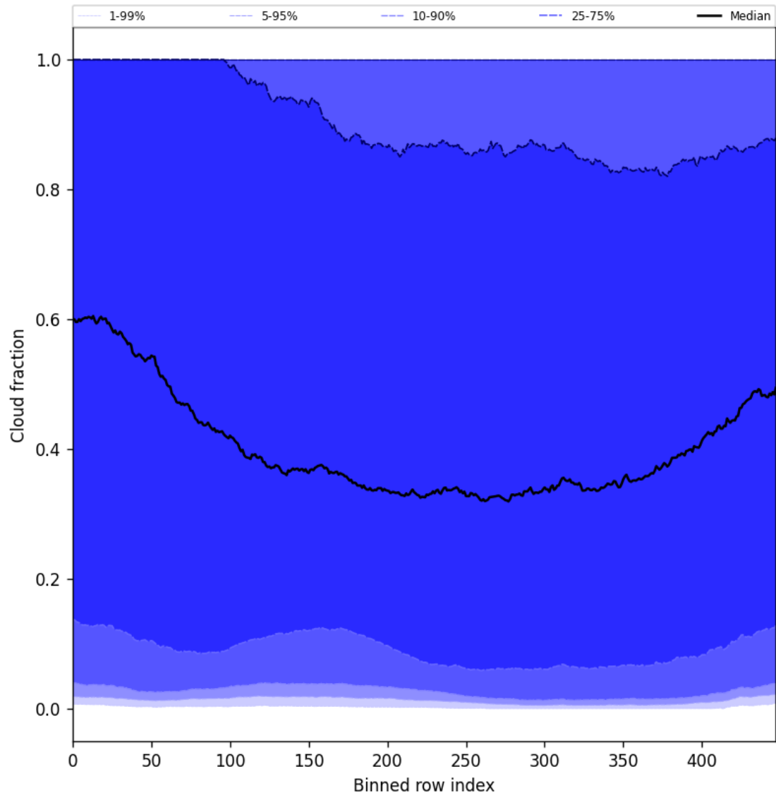
Figure 47: Along track statistics of “Cloud fraction” for 2025-02-10 to 2025-02-11
