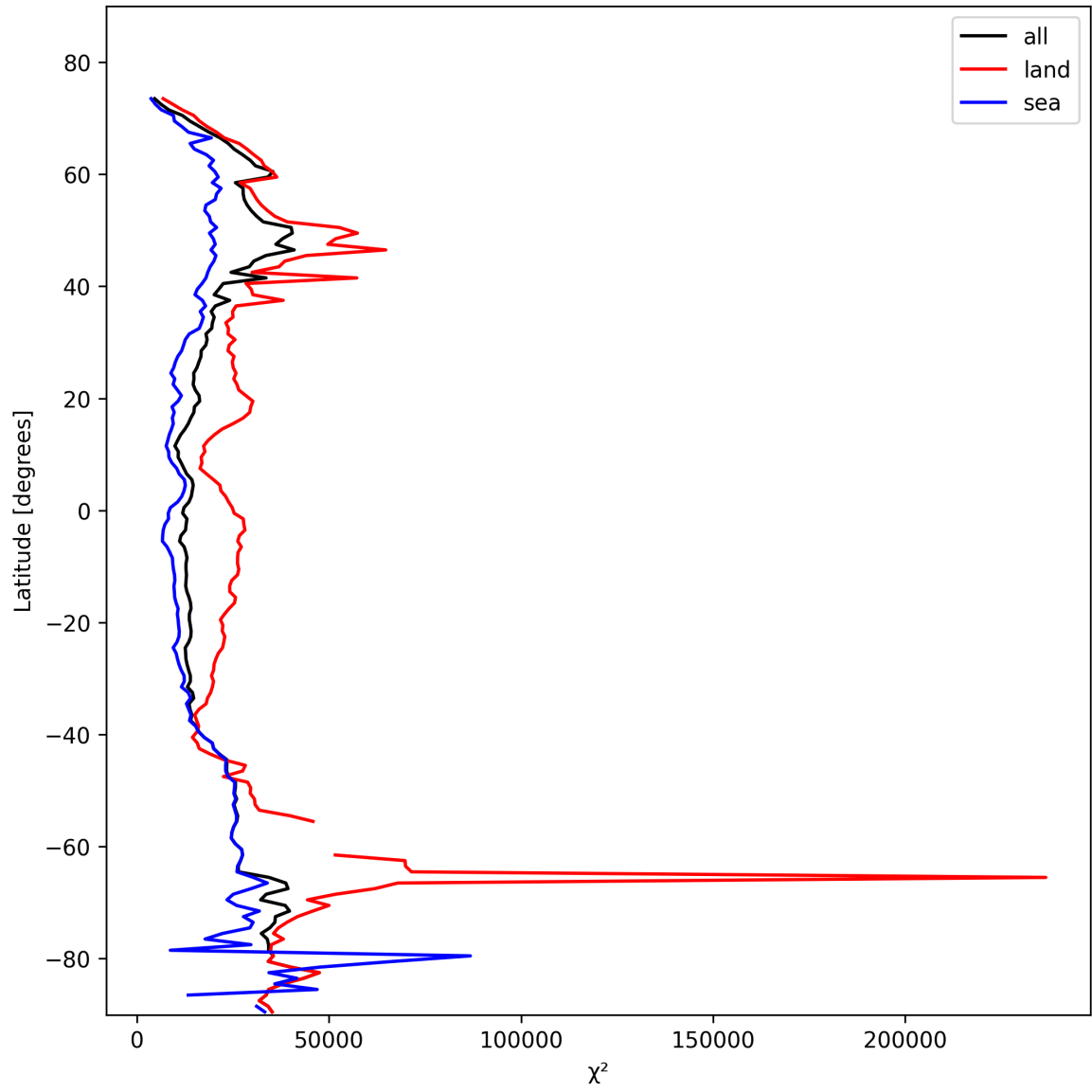
Figure 19: Zonal average of “ \chi^2 ” for 2025-02-10 to 2025-02-11.
