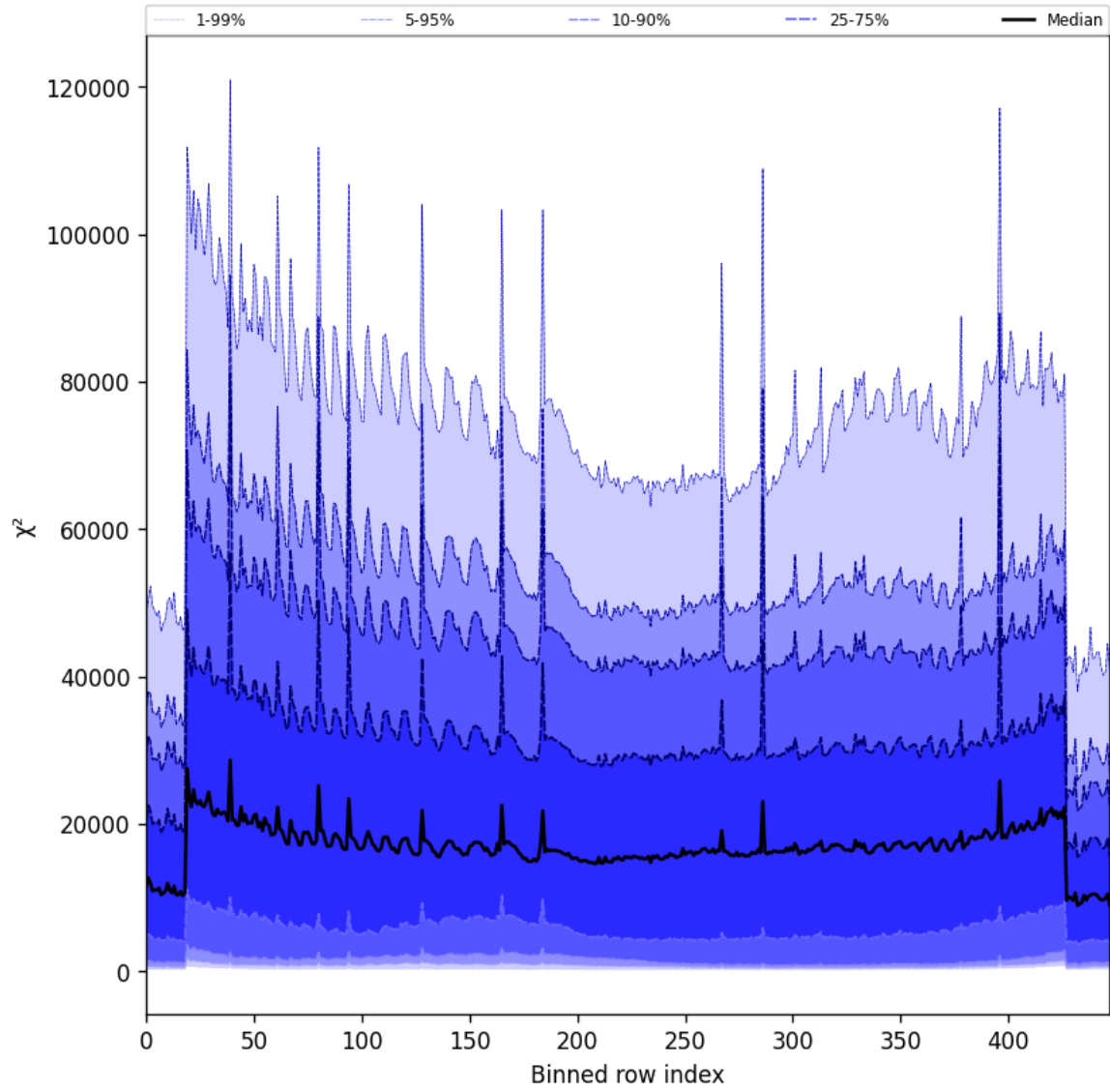
Figure 53: Along track statistics of “ \chi^2 ” for 2025-02-10 to 2025-02-11
