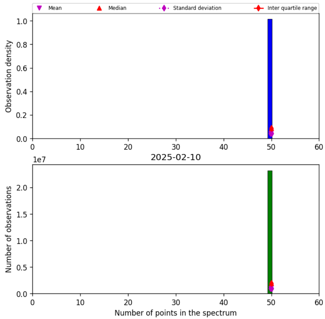
Figure 42: Histogram of “Number of points in the spectrum” for 2025-02-10 to 2025-02-11
