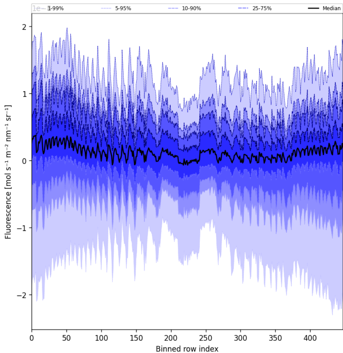
Figure 55: Along track statistics of “Fluorescence” for 2025-02-10 to 2025-02-11
