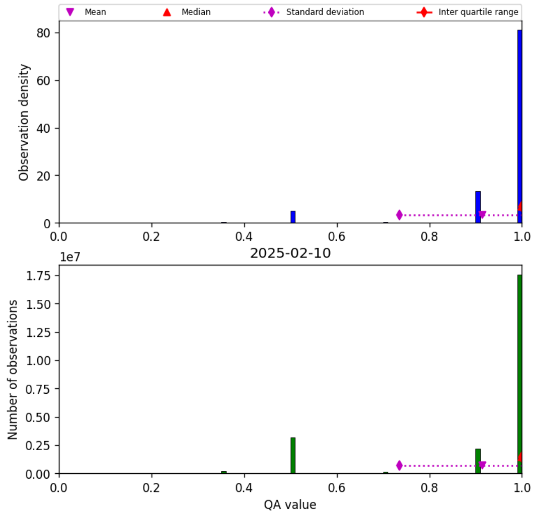
Figure 27: Histogram of “QA value” for 2025-02-10 to 2025-02-11
