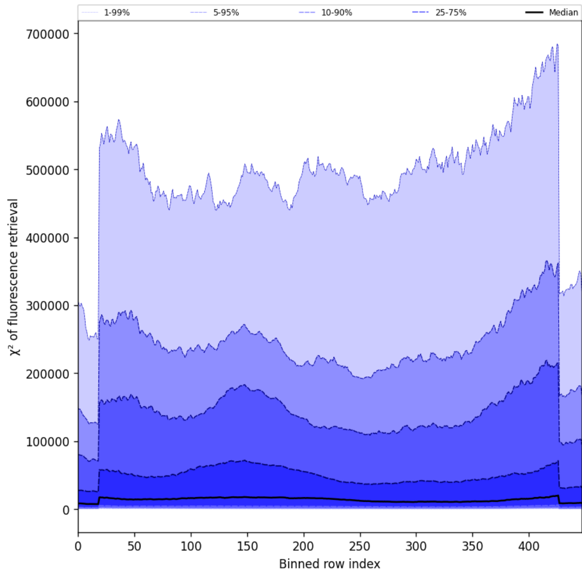
Figure 57: Along track statistics of “ \chi^2 of fluorescence retrieval” for 2025-02-10 to 2025-02-11
