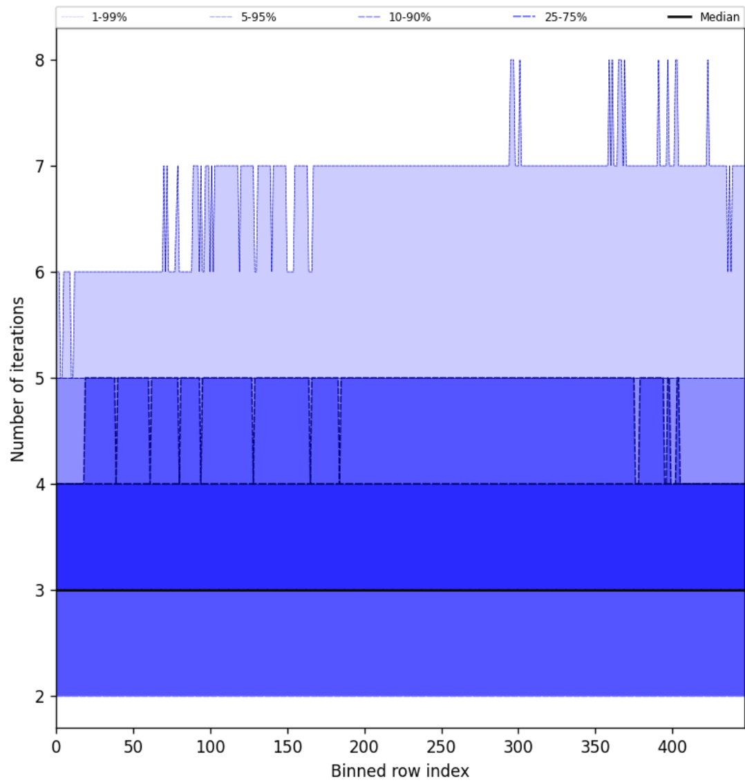
Figure 54: Along track statistics of “Number of iterations” for 2025-02-10 to 2025-02-11
