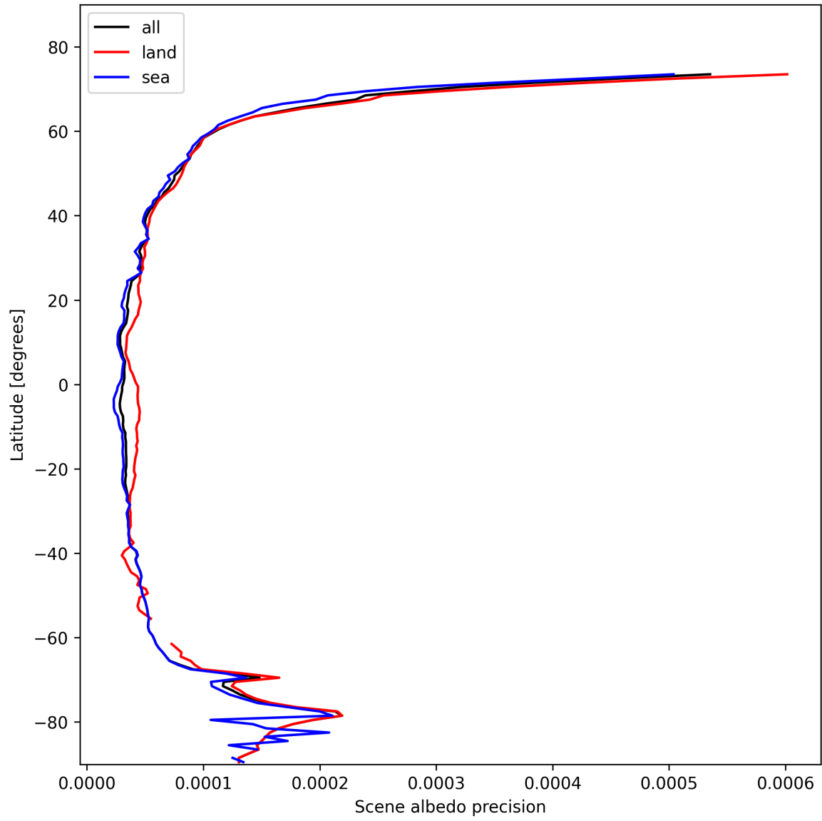
Figure 16: Zonal average of “Scene albedo precision” for 2025-02-10 to 2025-02-11.
