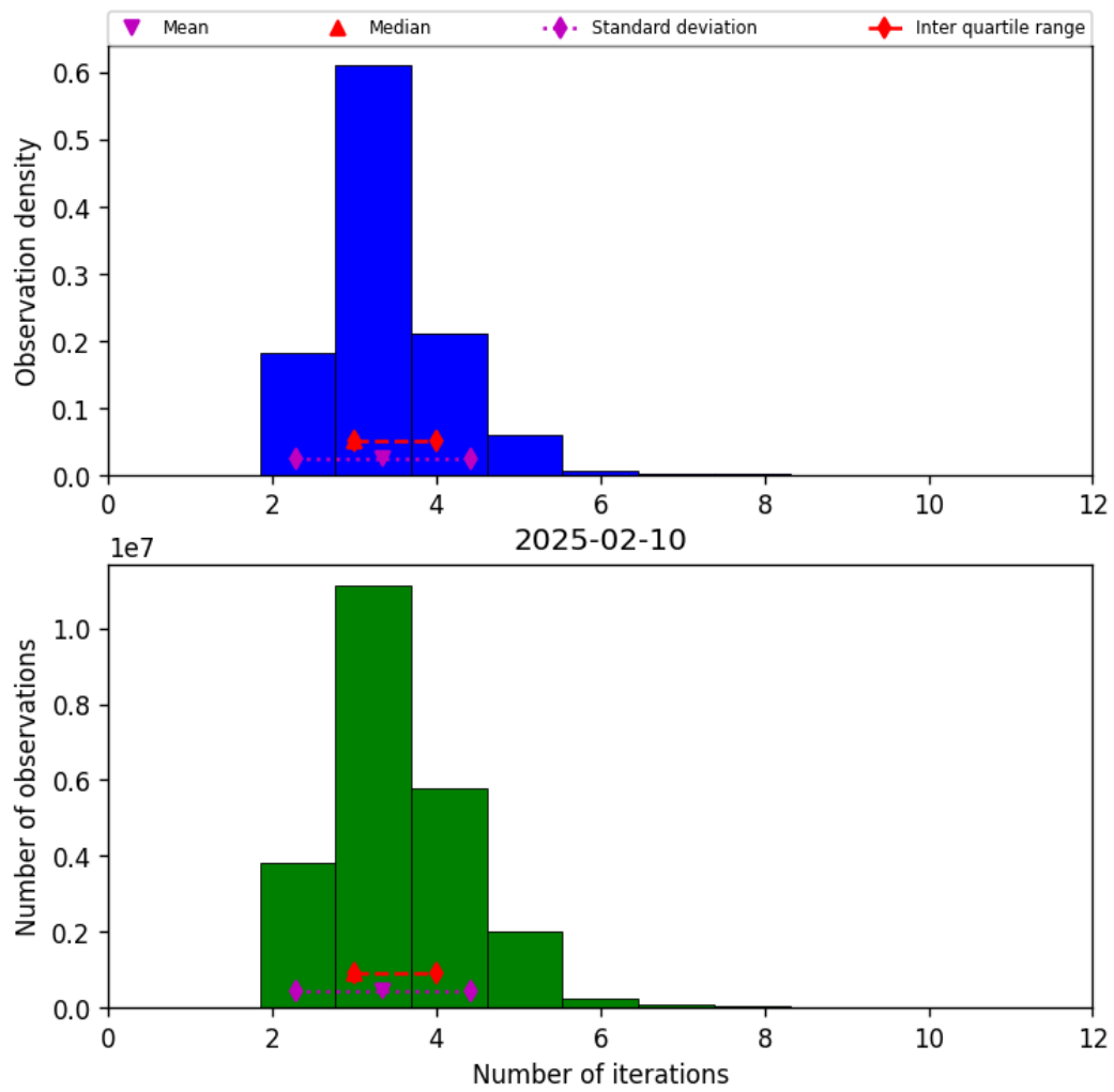
Figure 37: Histogram of “Number of iterations” for 2025-02-10 to 2025-02-11
