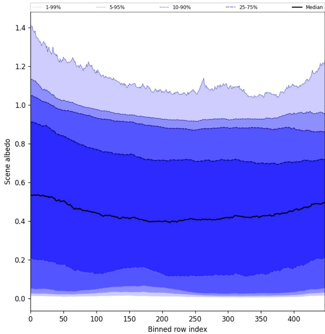
Figure 49: Along track statistics of “Scene albedo” for 2025-02-10 to 2025-02-11
