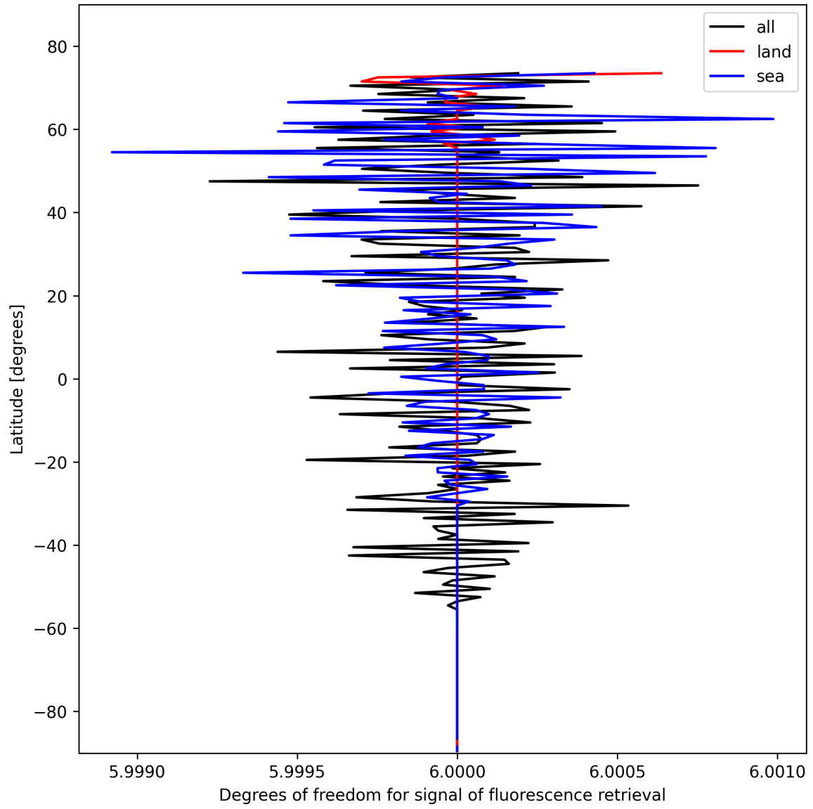
Figure 24: Zonal average of “Degrees of freedom for signal of fluorescence retrieval” for 2025-02-10 to 2025-02-11.
