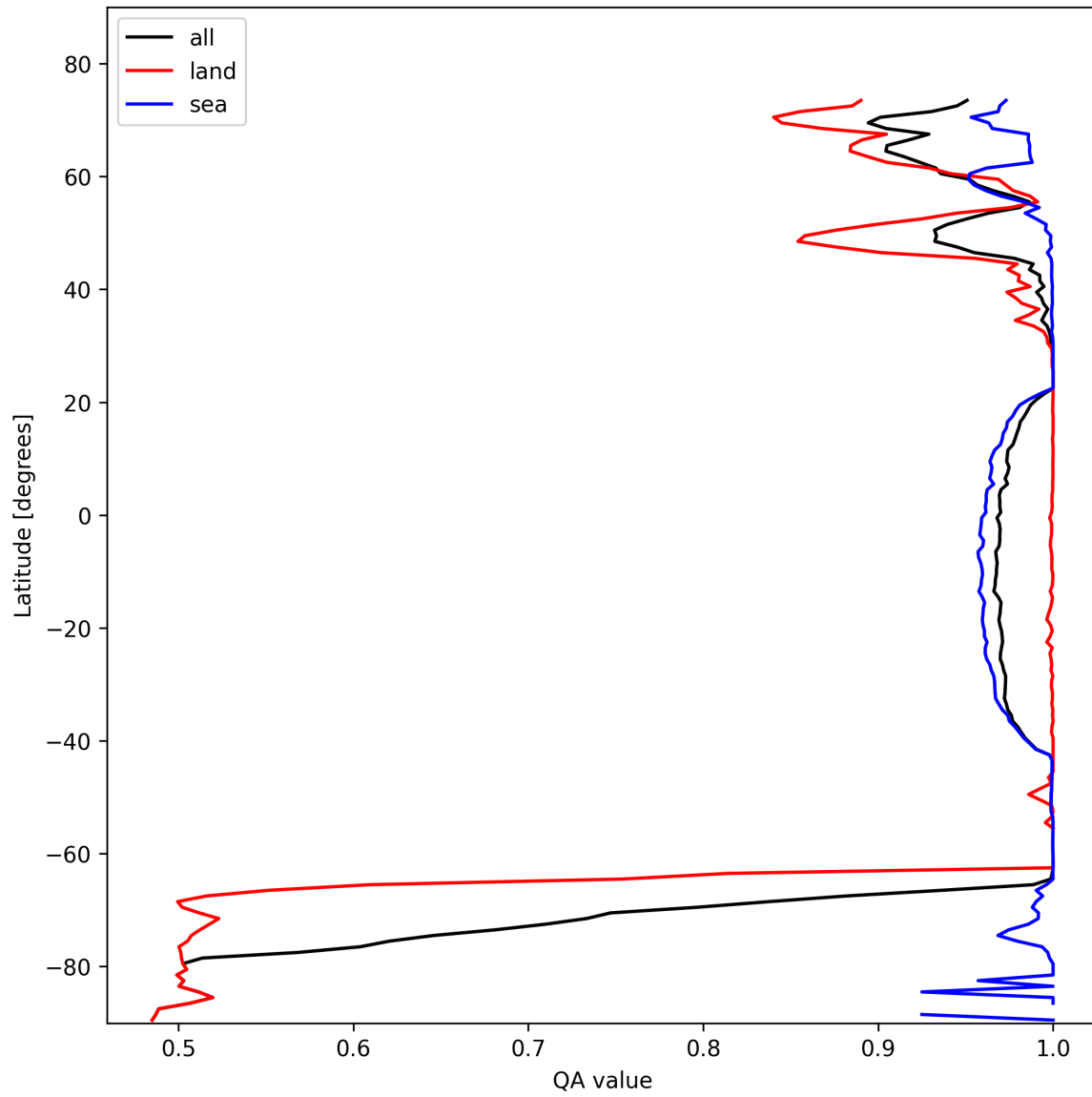
Figure 10: Zonal average of “QA value” for 2025-02-10 to 2025-02-11.
