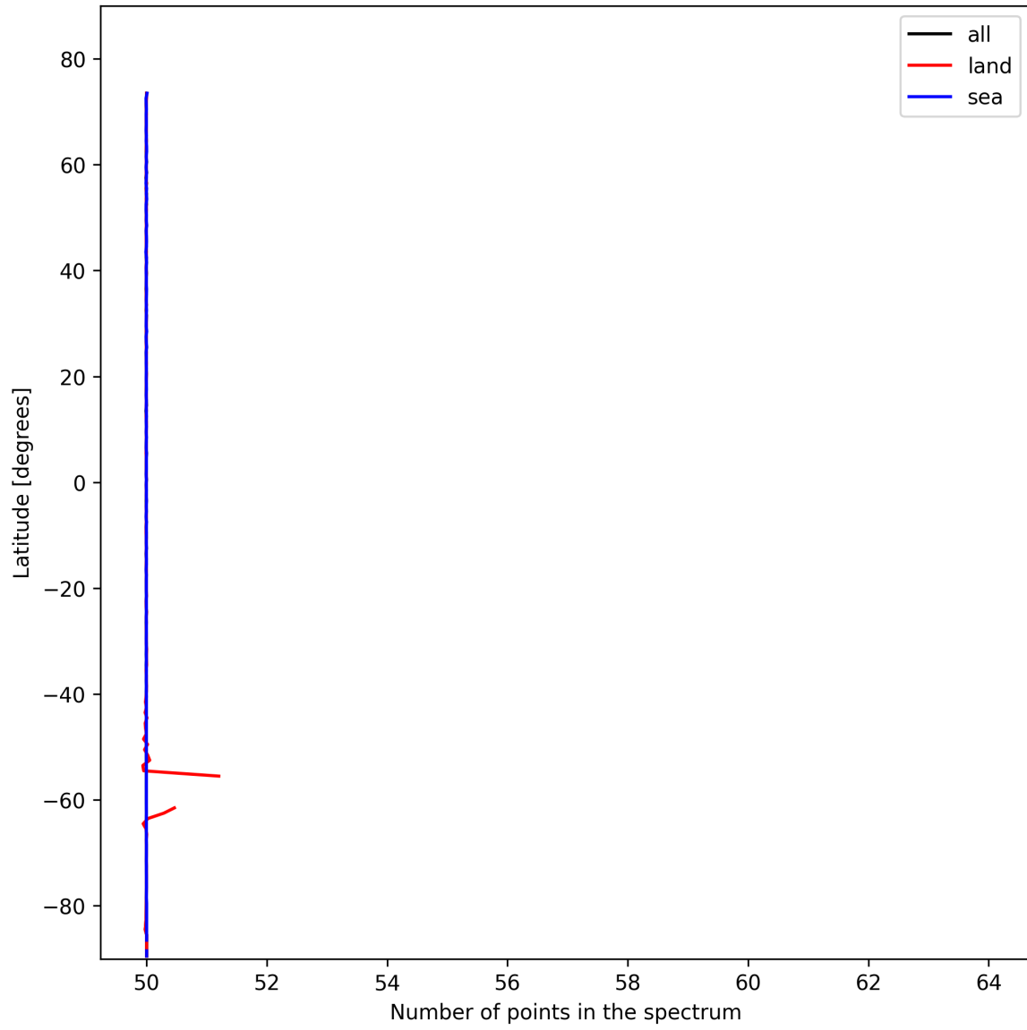
Figure 25: Zonal average of “Number of points in the spectrum” for 2025-02-10 to 2025-02-11.
