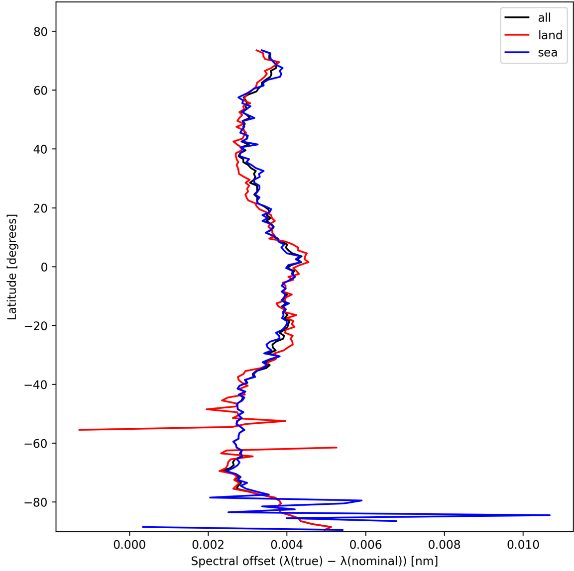
Figure 26: Zonal average of “Spectral offset ( \lambda_{\text{true}} - \lambda_{\text{nominal}} )” for 2025-02-10 to 2025-02-11.
