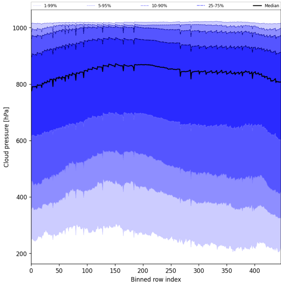
Figure 45: Along track statistics of “Cloud pressure” for 2025-02-10 to 2025-02-11
