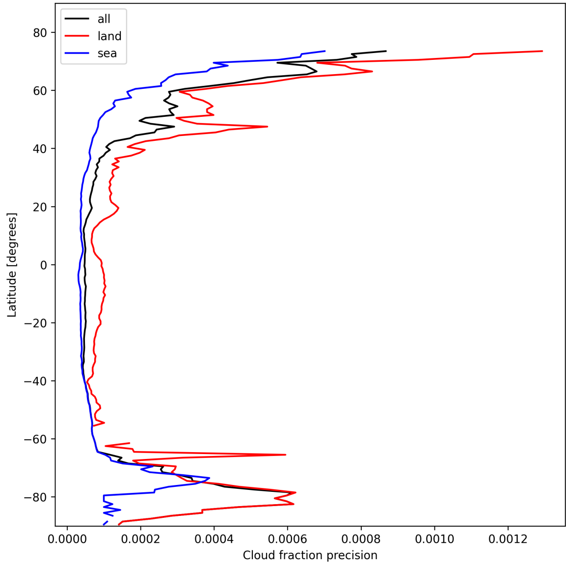
Figure 14: Zonal average of “Cloud fraction precision” for 2025-02-10 to 2025-02-11.
