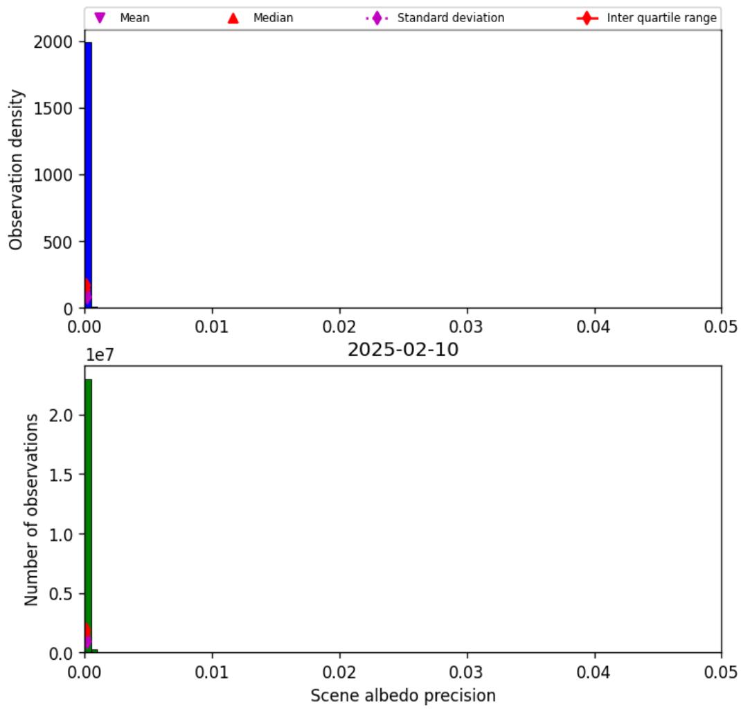
Figure 33: Histogram of “Scene albedo precision” for 2025-02-10 to 2025-02-11
