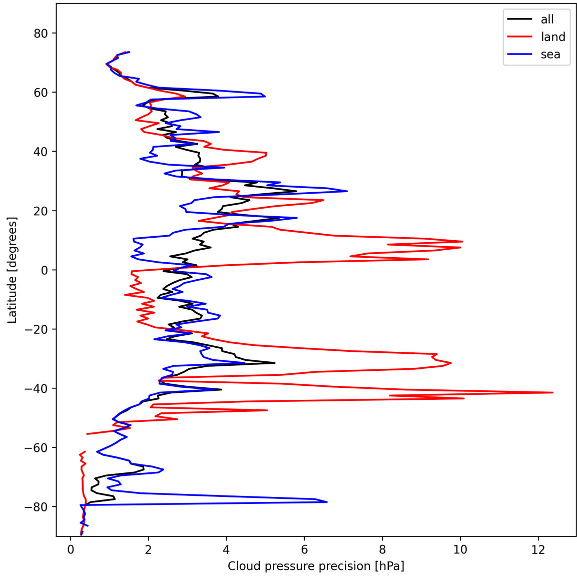
Figure 12: Zonal average of “Cloud pressure precision” for 2025-02-10 to 2025-02-11.
