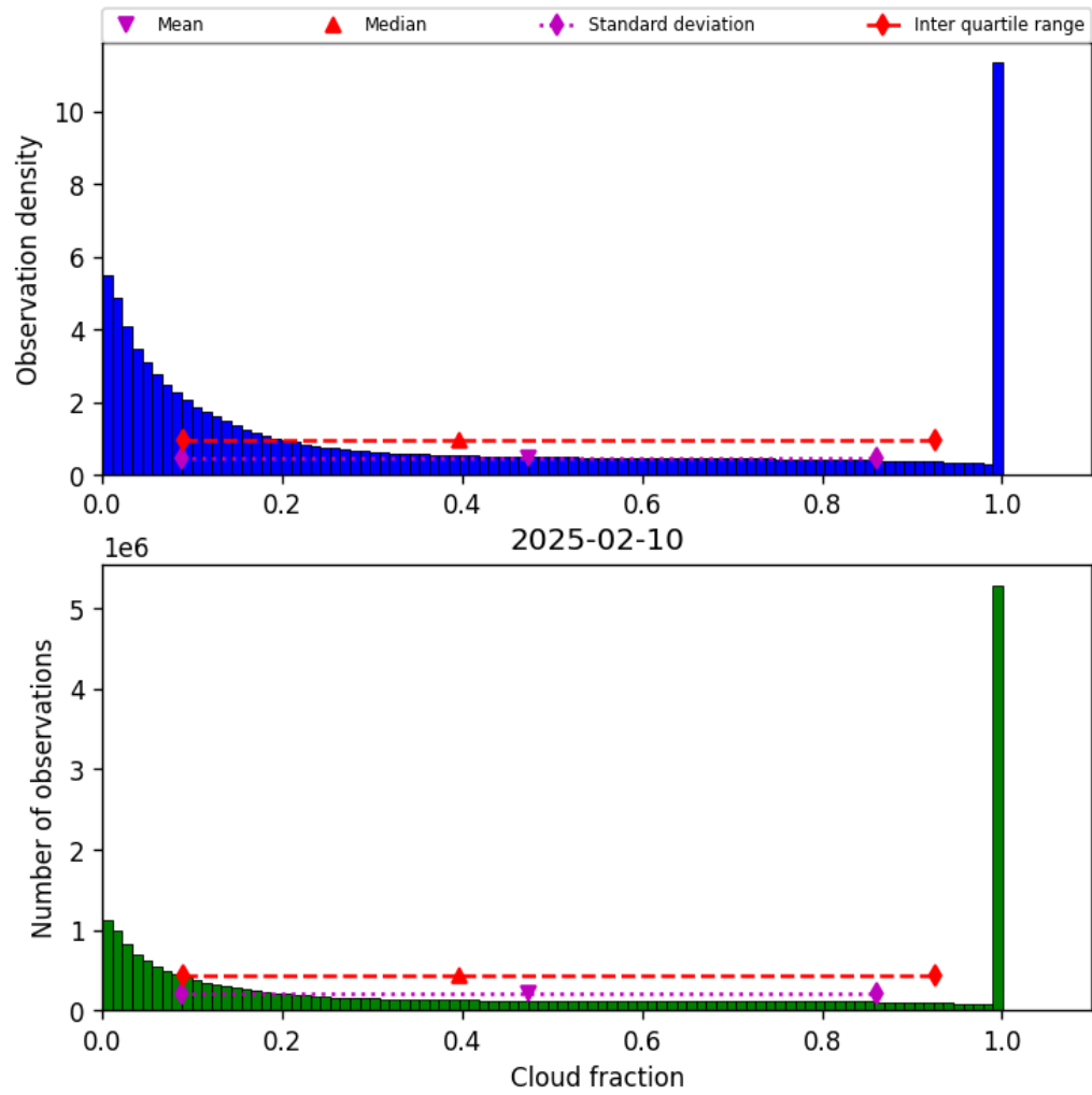
Figure 30: Histogram of “Cloud fraction” for 2025-02-10 to 2025-02-11
