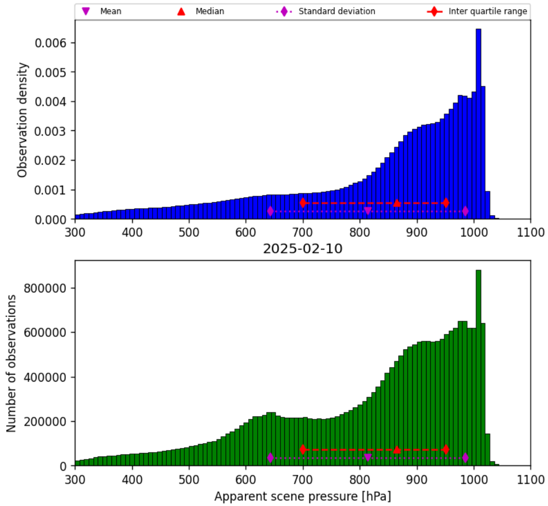
Figure 34: Histogram of “Apparent scene pressure” for 2025-02-10 to 2025-02-11
