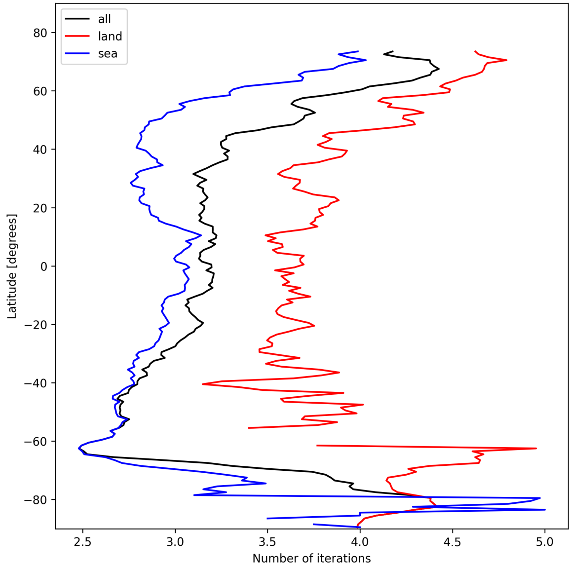
Figure 20: Zonal average of “Number of iterations” for 2025-02-10 to 2025-02-11.
