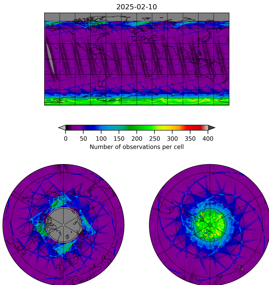
Figure 9: Map of the number of observations for 2025-02-10 to 2025-02-11
