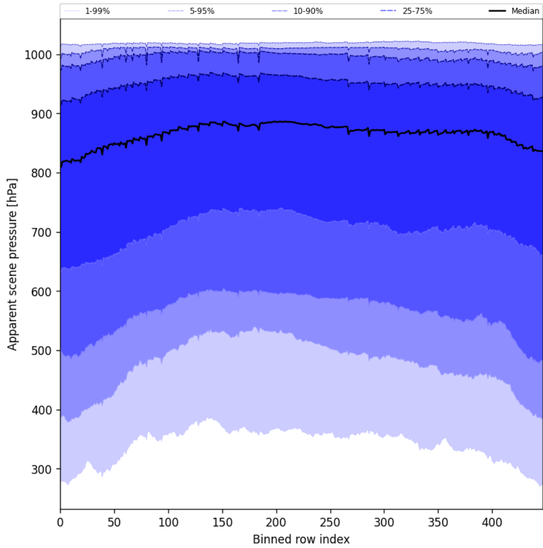
Figure 51: Along track statistics of “Apparent scene pressure” for 2025-02-10 to 2025-02-11
