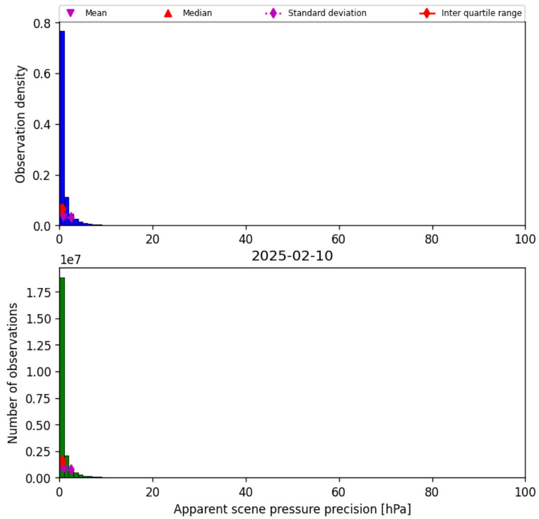
Figure 35: Histogram of “Apparent scene pressure precision” for 2025-02-10 to 2025-02-11
