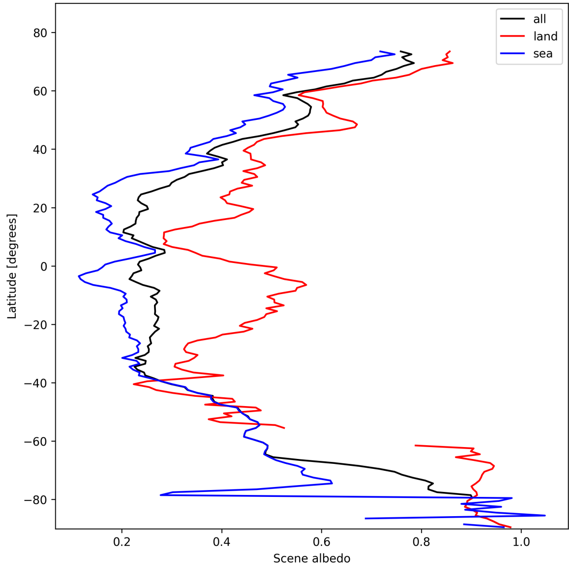
Figure 15: Zonal average of “Scene albedo” for 2025-02-10 to 2025-02-11.
