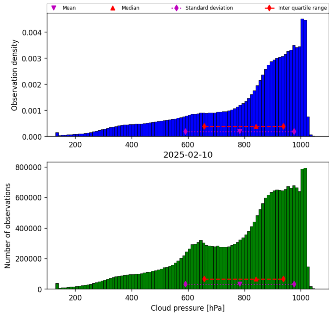
Figure 28: Histogram of “Cloud pressure” for 2025-02-10 to 2025-02-11
