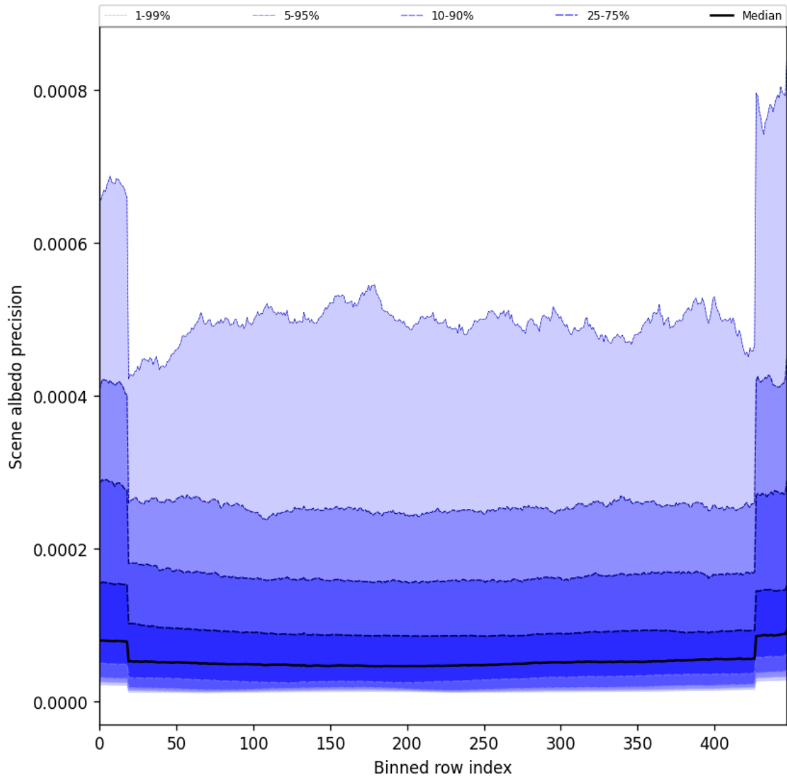
Figure 50: Along track statistics of “Scene albedo precision” for 2025-02-10 to 2025-02-11
