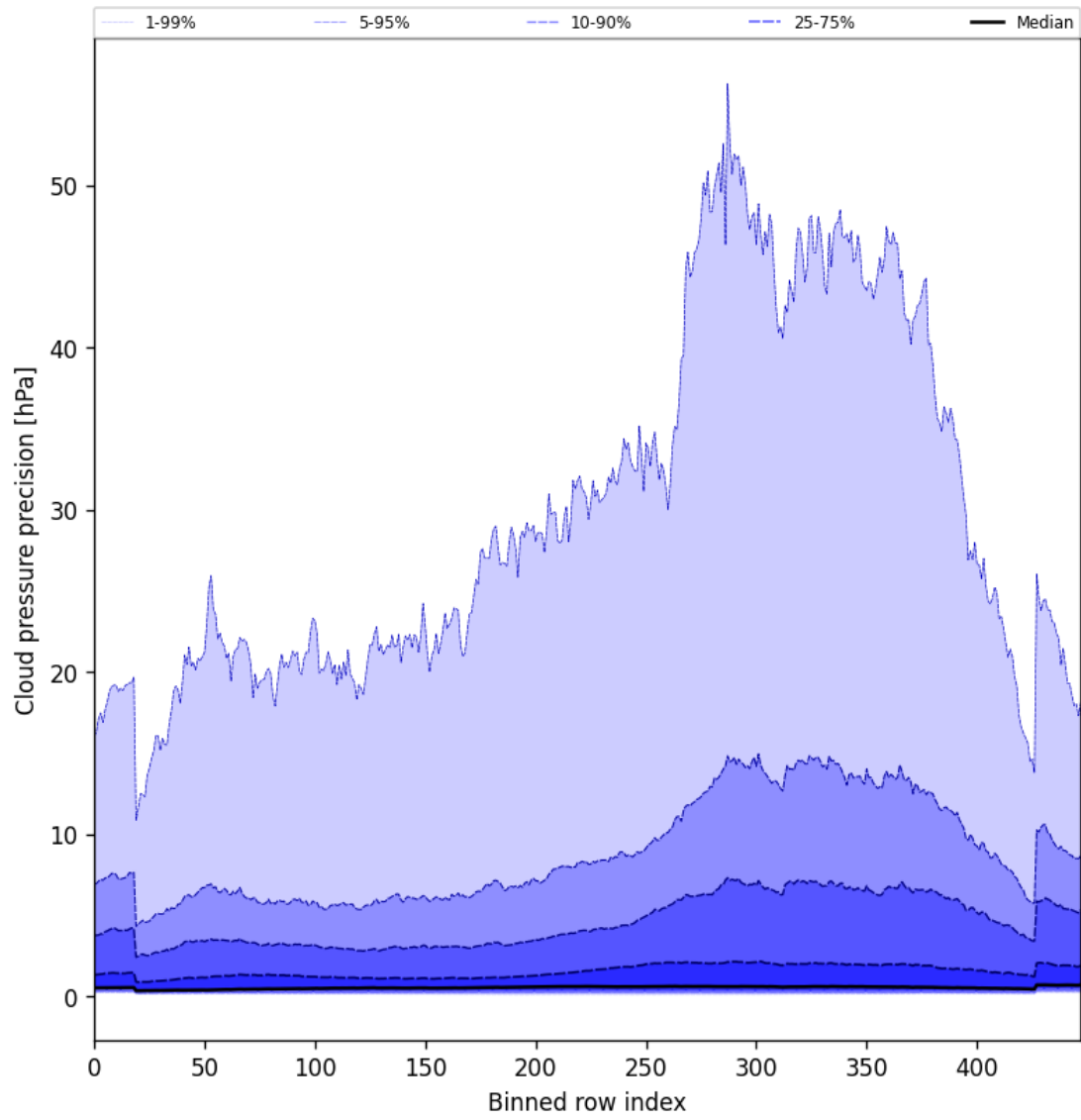
Figure 46: Along track statistics of “Cloud pressure precision” for 2025-02-10 to 2025-02-11
