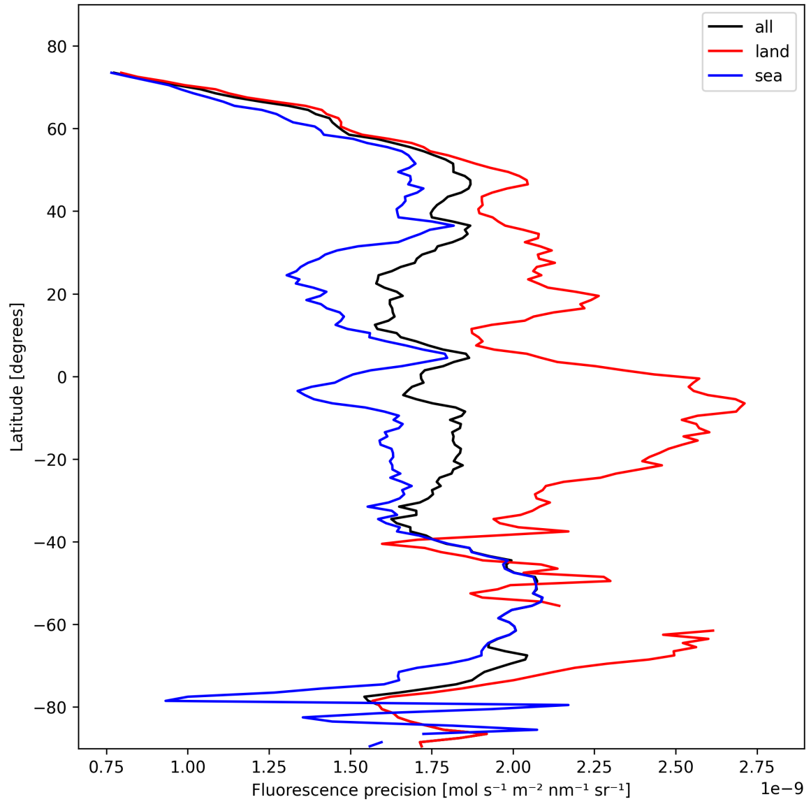
Figure 22: Zonal average of “Fluorescence precision” for 2025-02-10 to 2025-02-11.
