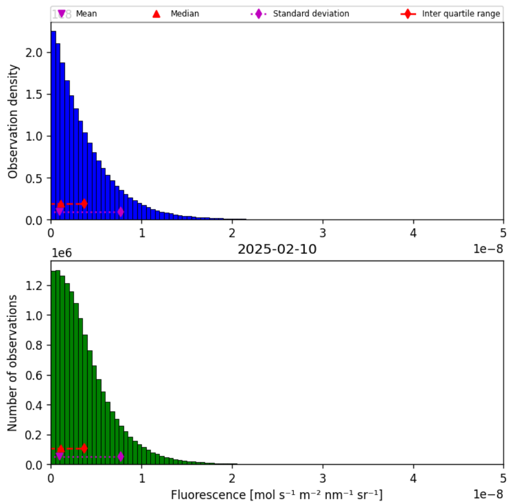
Figure 38: Histogram of “Fluorescence” for 2025-02-10 to 2025-02-11
