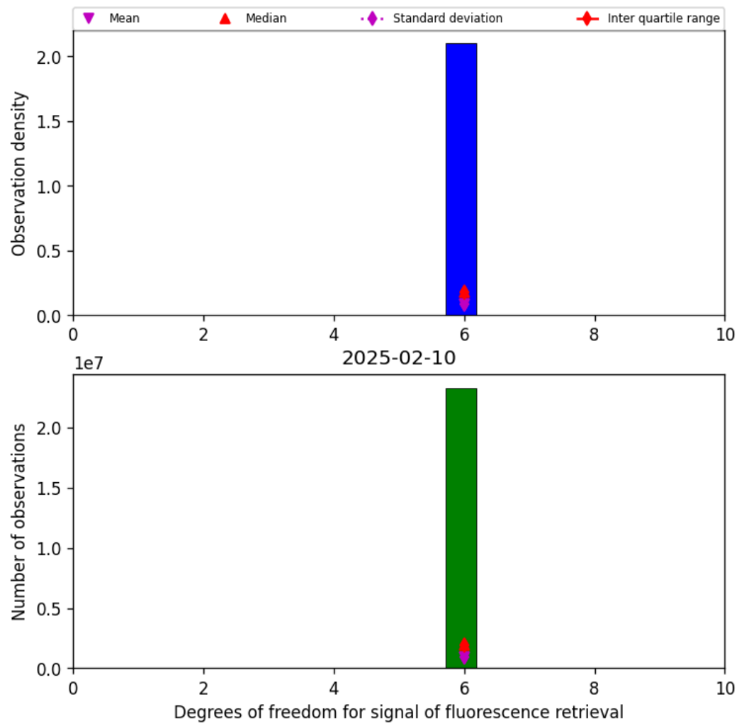
Figure 41: Histogram of “Degrees of freedom for signal of fluorescence retrieval” for 2025-02-10 to 2025-02-11
