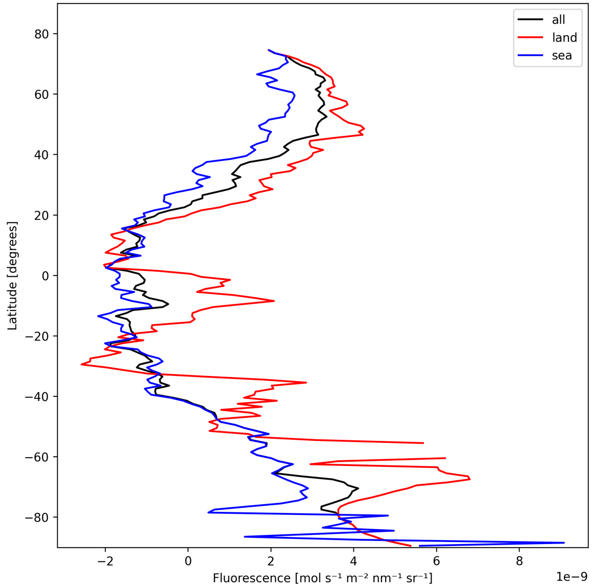
Figure 21: Zonal average of “Fluorescence” for 2025-02-13 to 2025-02-14.
