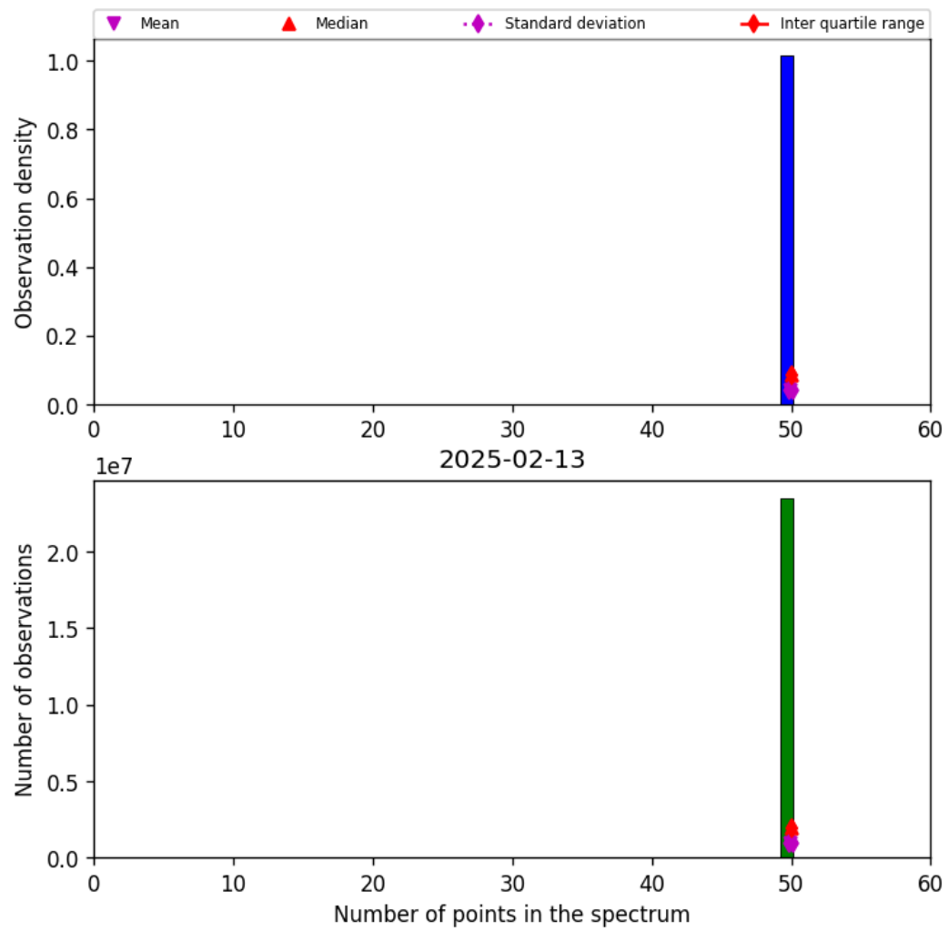
Figure 42: Histogram of “Number of points in the spectrum” for 2025-02-13 to 2025-02-14
