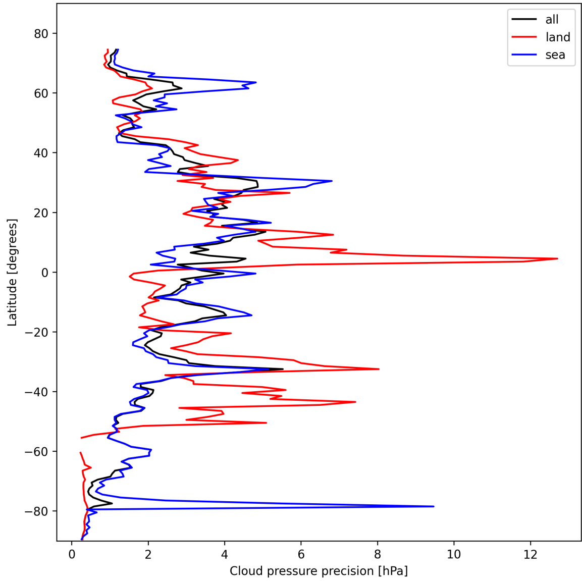
Figure 12: Zonal average of “Cloud pressure precision” for 2025-02-13 to 2025-02-14.
