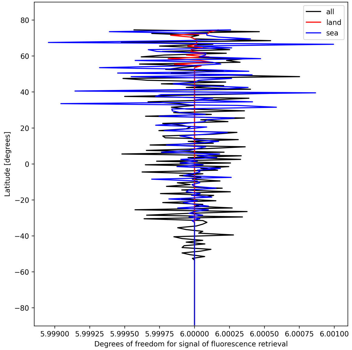
Figure 24: Zonal average of “Degrees of freedom for signal of fluorescence retrieval” for 2025-02-13 to 2025-02-14.
