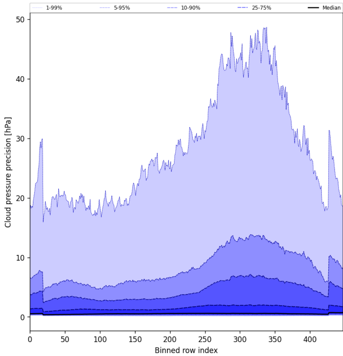
Figure 46: Along track statistics of “Cloud pressure precision” for 2025-02-13 to 2025-02-14
