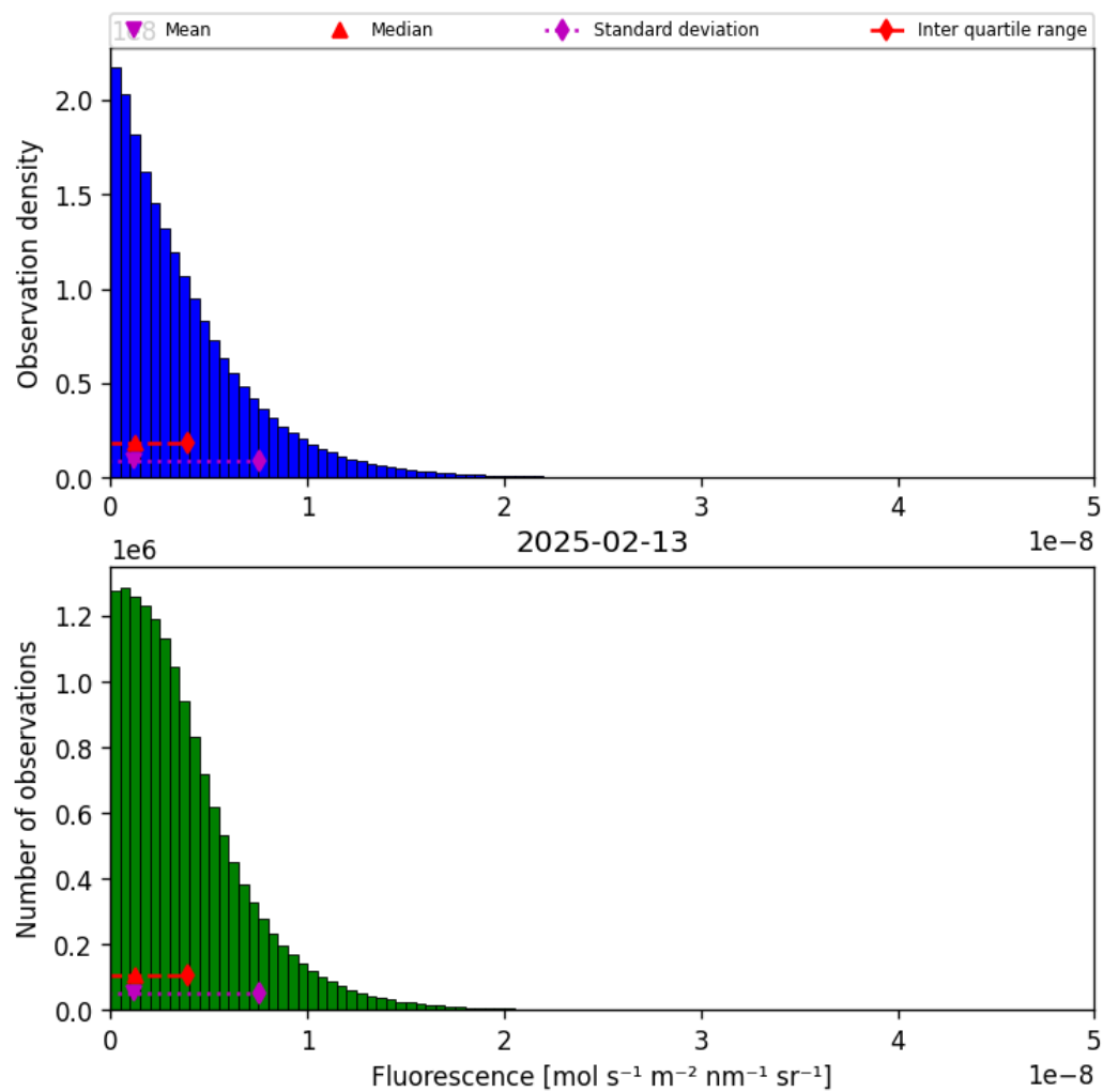
Figure 38: Histogram of “Fluorescence” for 2025-02-13 to 2025-02-14
