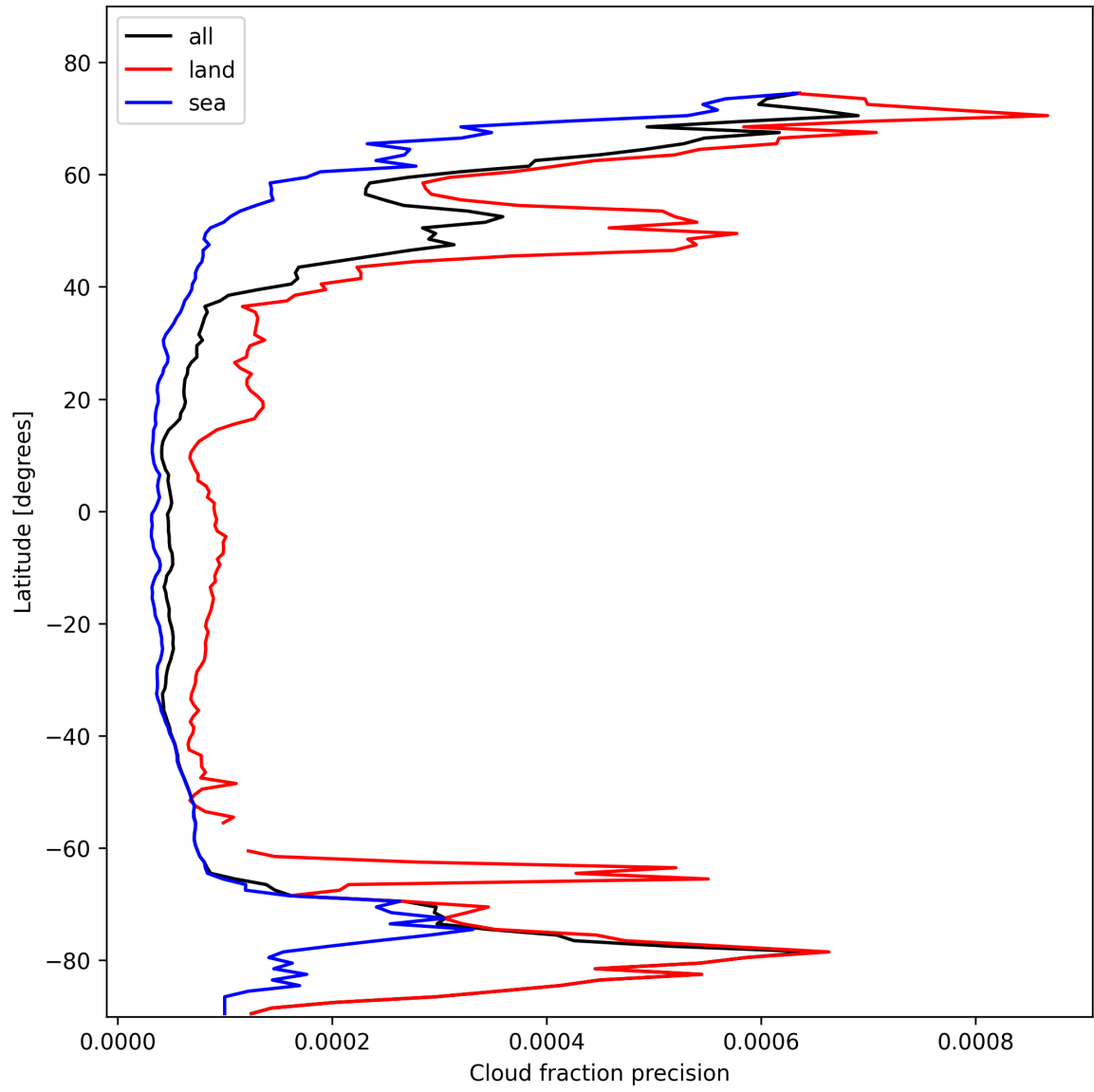
Figure 14: Zonal average of “Cloud fraction precision” for 2025-02-13 to 2025-02-14.
