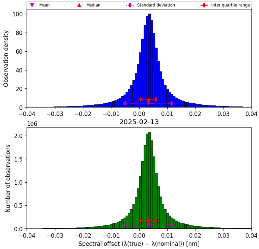
Figure 43: Histogram of “Spectral offset ( \lambda_{\text{true}} - \lambda_{\text{nominal}} )” for 2025-02-13 to 2025-02-14
