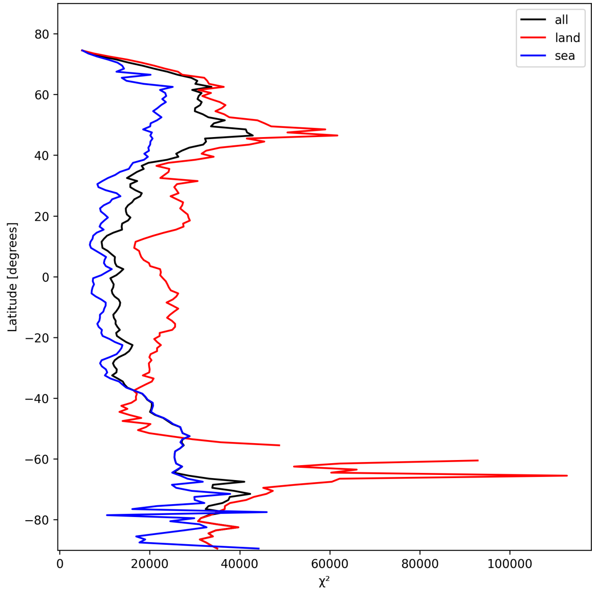
Figure 19: Zonal average of “ \chi^2 ” for 2025-02-13 to 2025-02-14.
