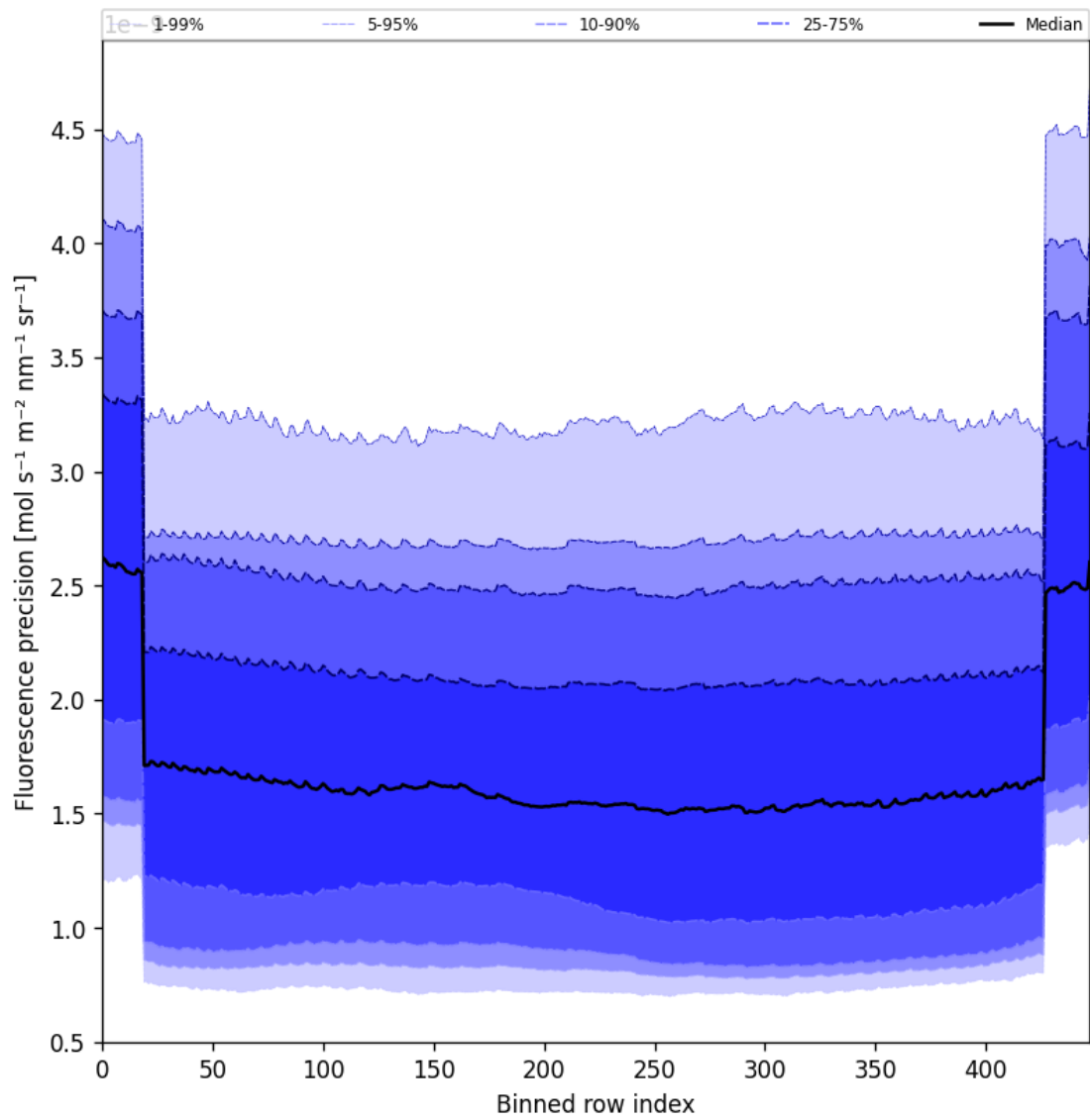
Figure 56: Along track statistics of “Fluorescence precision” for 2025-02-13 to 2025-02-14
