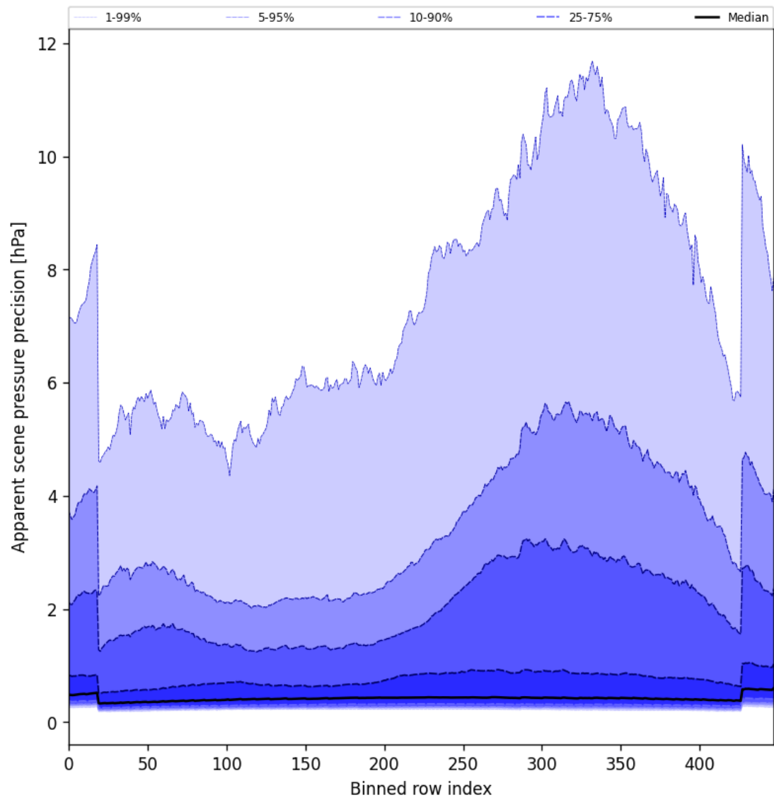
Figure 52: Along track statistics of “Apparent scene pressure precision” for 2025-02-13 to 2025-02-14
