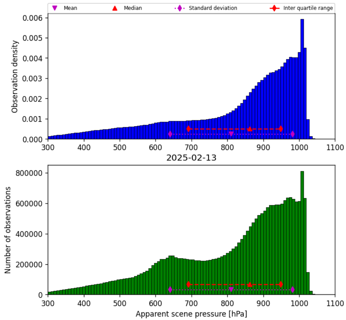
Figure 34: Histogram of “Apparent scene pressure” for 2025-02-13 to 2025-02-14
