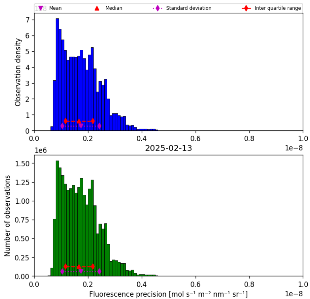
Figure 39: Histogram of “Fluorescence precision” for 2025-02-13 to 2025-02-14
