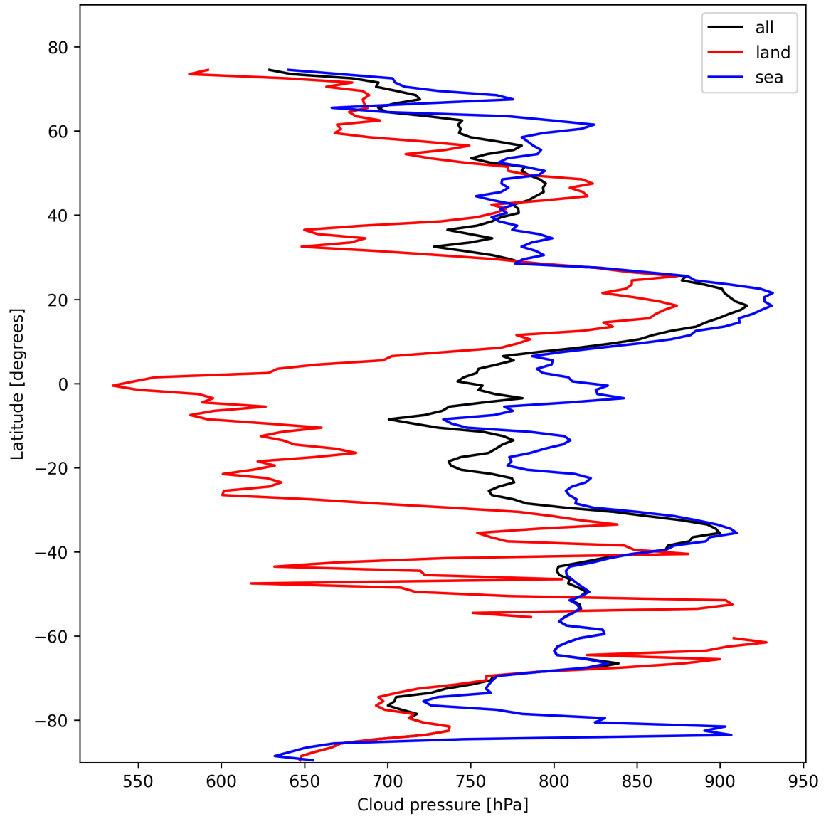
Figure 11: Zonal average of “Cloud pressure” for 2025-02-13 to 2025-02-14.
