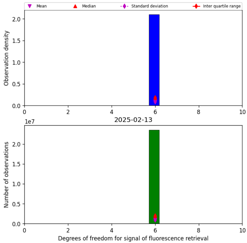
Figure 41: Histogram of “Degrees of freedom for signal of fluorescence retrieval” for 2025-02-13 to 2025-02-14
