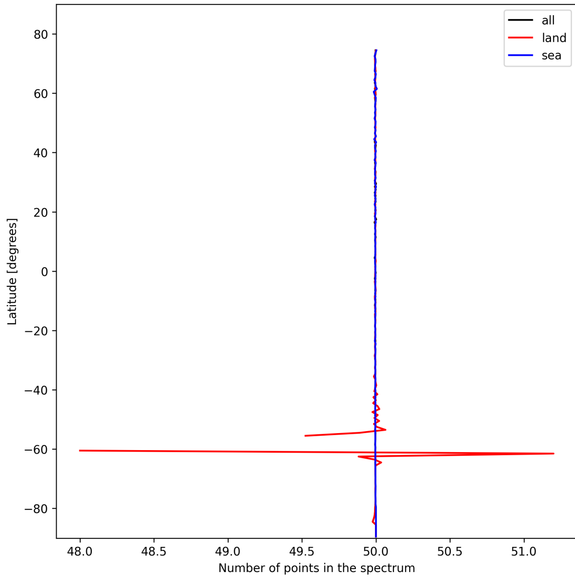
Figure 25: Zonal average of “Number of points in the spectrum” for 2025-02-13 to 2025-02-14.
