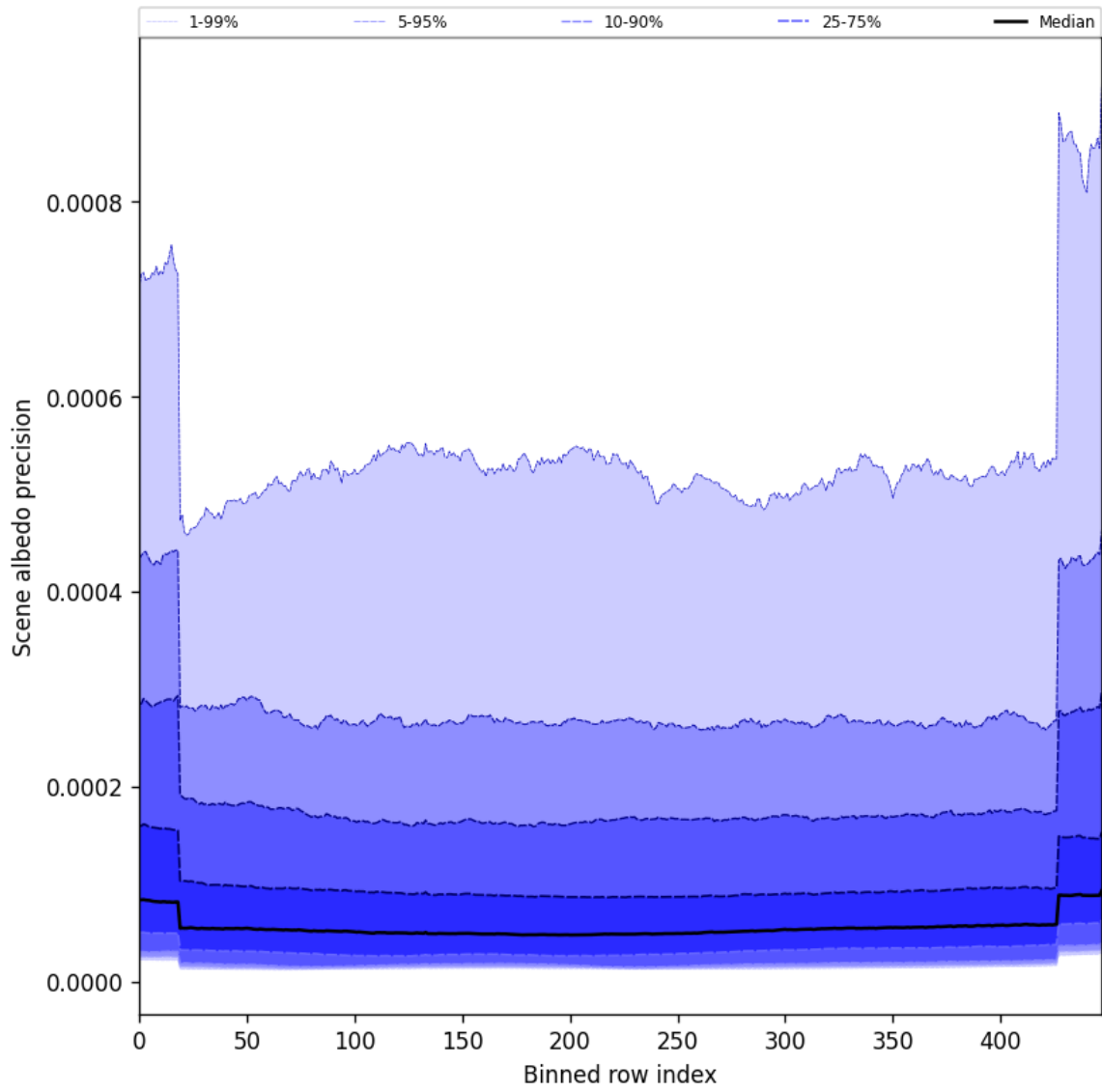
Figure 50: Along track statistics of “Scene albedo precision” for 2025-02-13 to 2025-02-14
