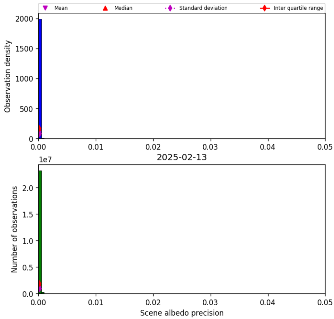
Figure 33: Histogram of “Scene albedo precision” for 2025-02-13 to 2025-02-14
