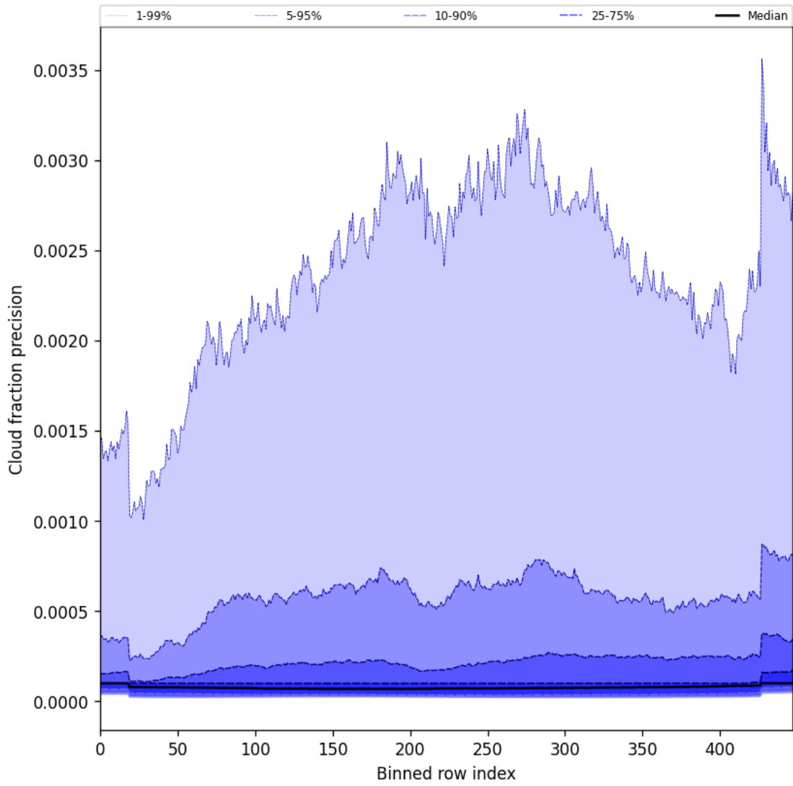
Figure 48: Along track statistics of “Cloud fraction precision” for 2025-02-13 to 2025-02-14
