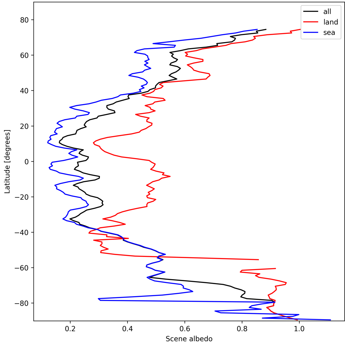
Figure 15: Zonal average of “Scene albedo” for 2025-02-13 to 2025-02-14.
