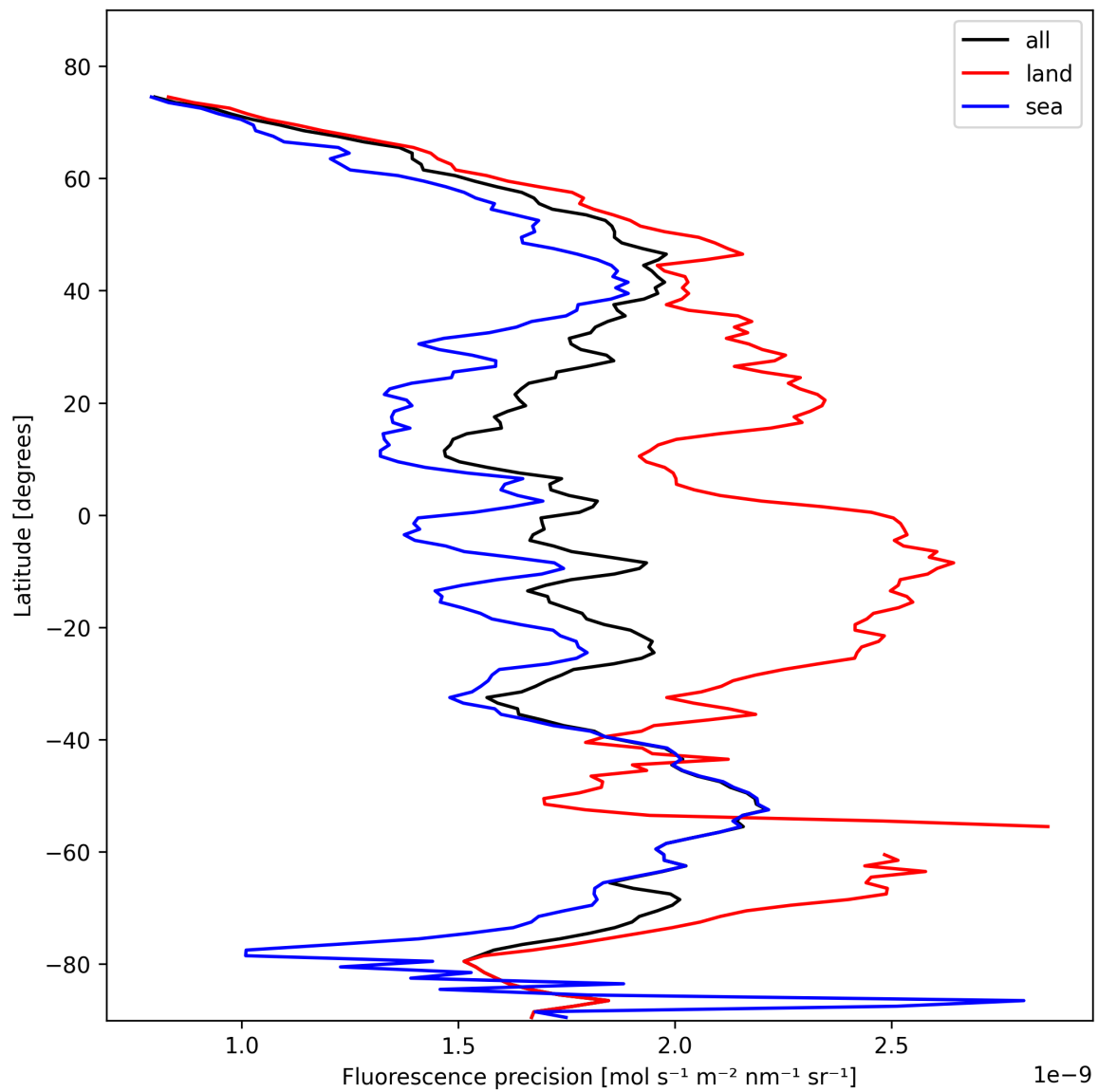
Figure 22: Zonal average of “Fluorescence precision” for 2025-02-13 to 2025-02-14.
