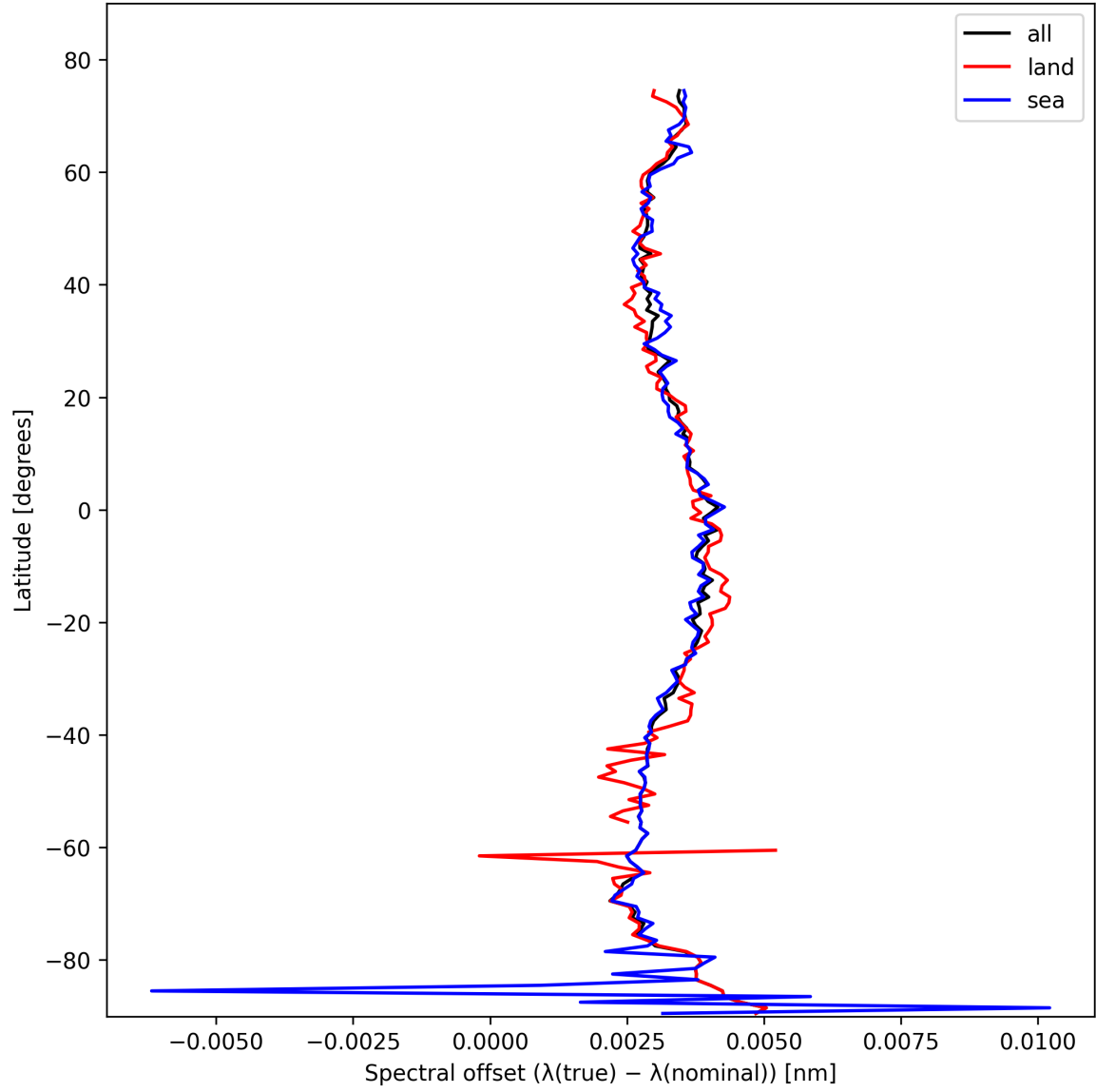
Figure 26: Zonal average of “Spectral offset ( \lambda_{\text{true}} - \lambda_{\text{nominal}} )” for 2025-02-13 to 2025-02-14.
