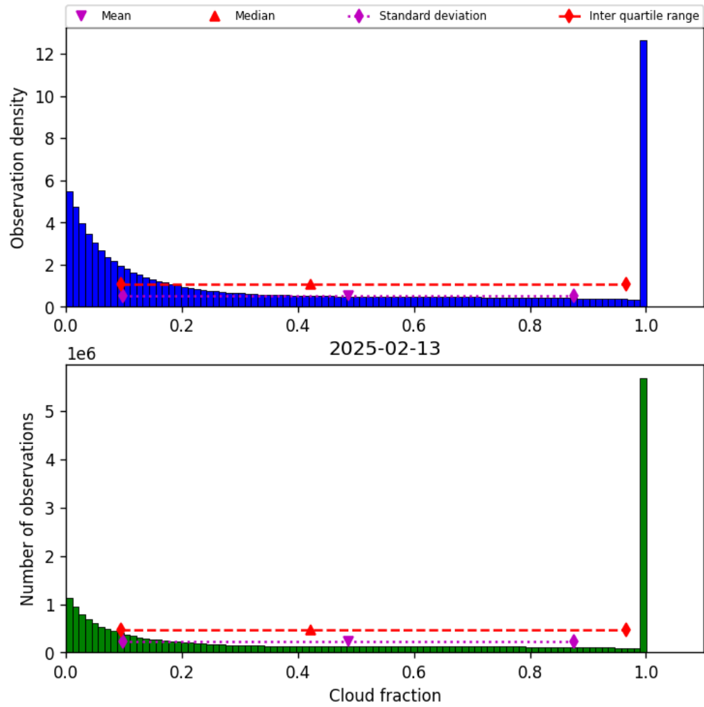
Figure 30: Histogram of “Cloud fraction” for 2025-02-13 to 2025-02-14
