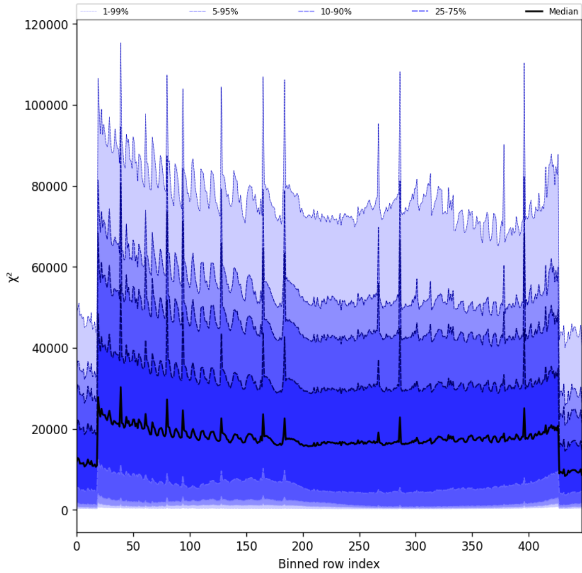
Figure 53: Along track statistics of “ \chi^2 ” for 2025-02-13 to 2025-02-14
