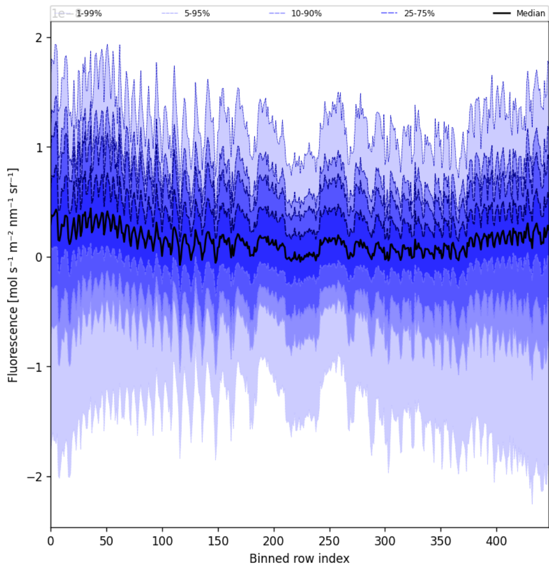
Figure 55: Along track statistics of “Fluorescence” for 2025-02-13 to 2025-02-14
