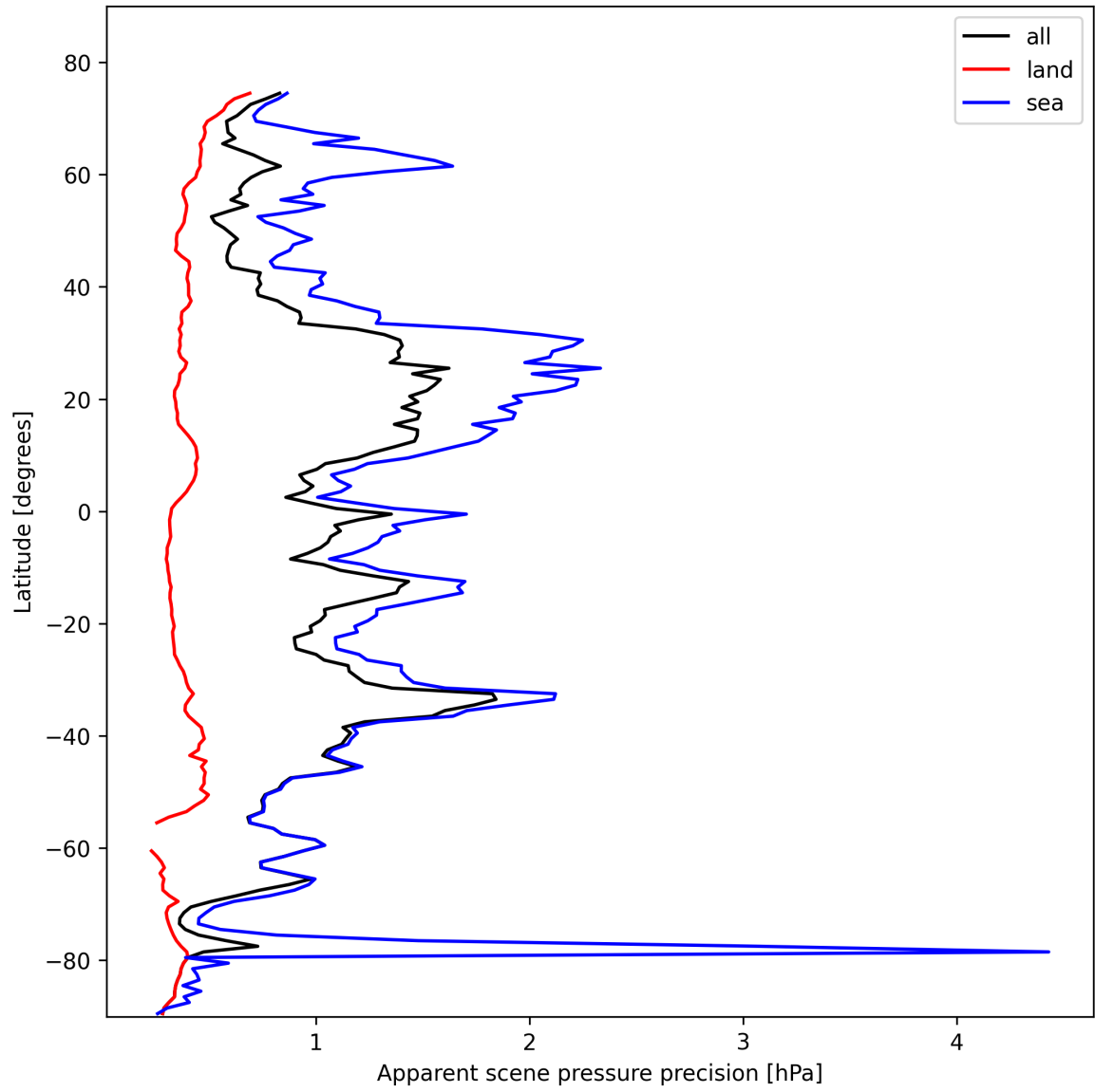
Figure 18: Zonal average of “Apparent scene pressure precision” for 2025-02-13 to 2025-02-14.
