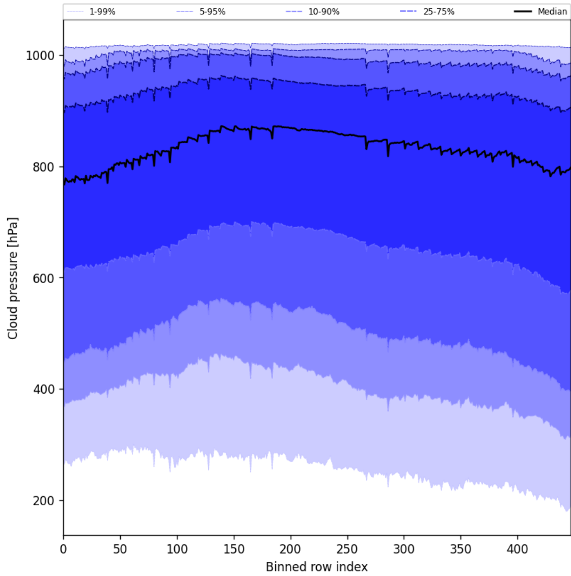
Figure 45: Along track statistics of “Cloud pressure” for 2025-02-13 to 2025-02-14
