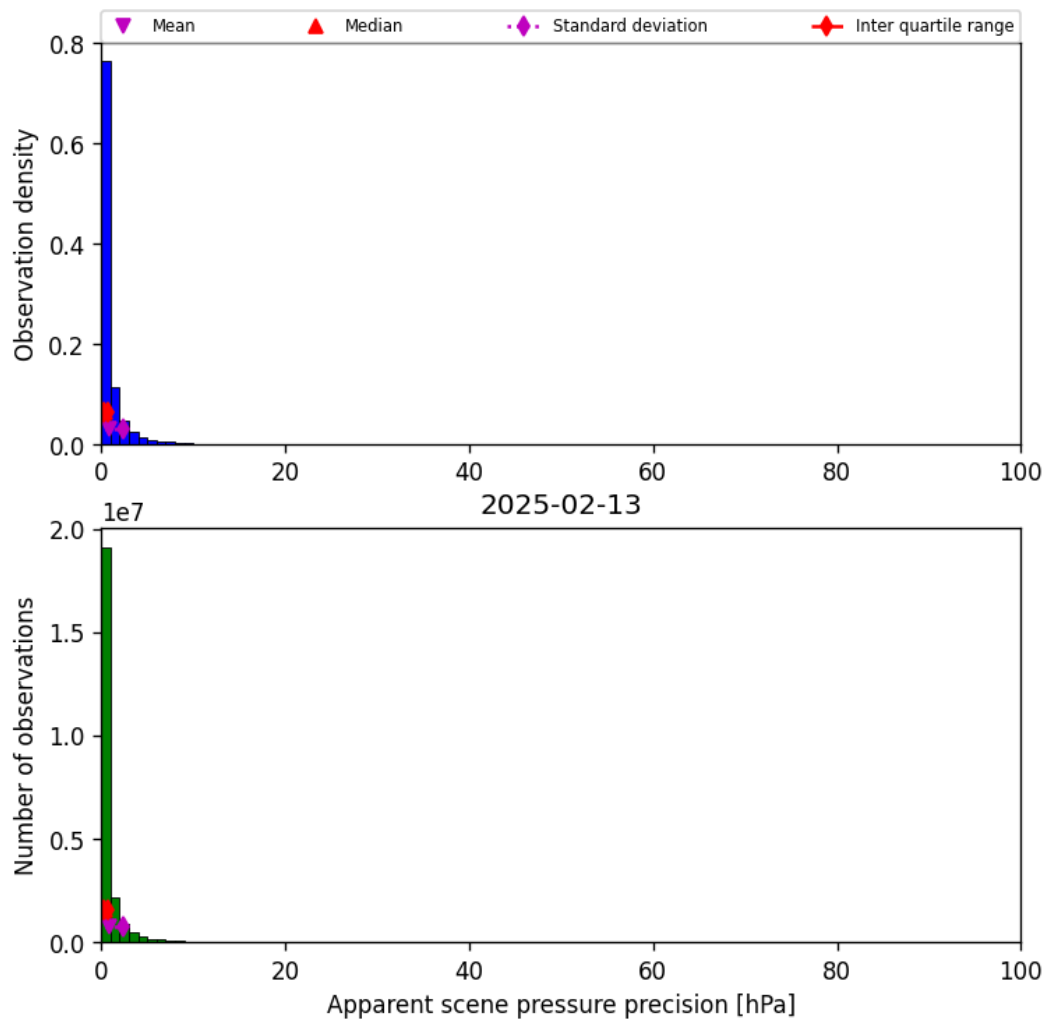
Figure 35: Histogram of “Apparent scene pressure precision” for 2025-02-13 to 2025-02-14
