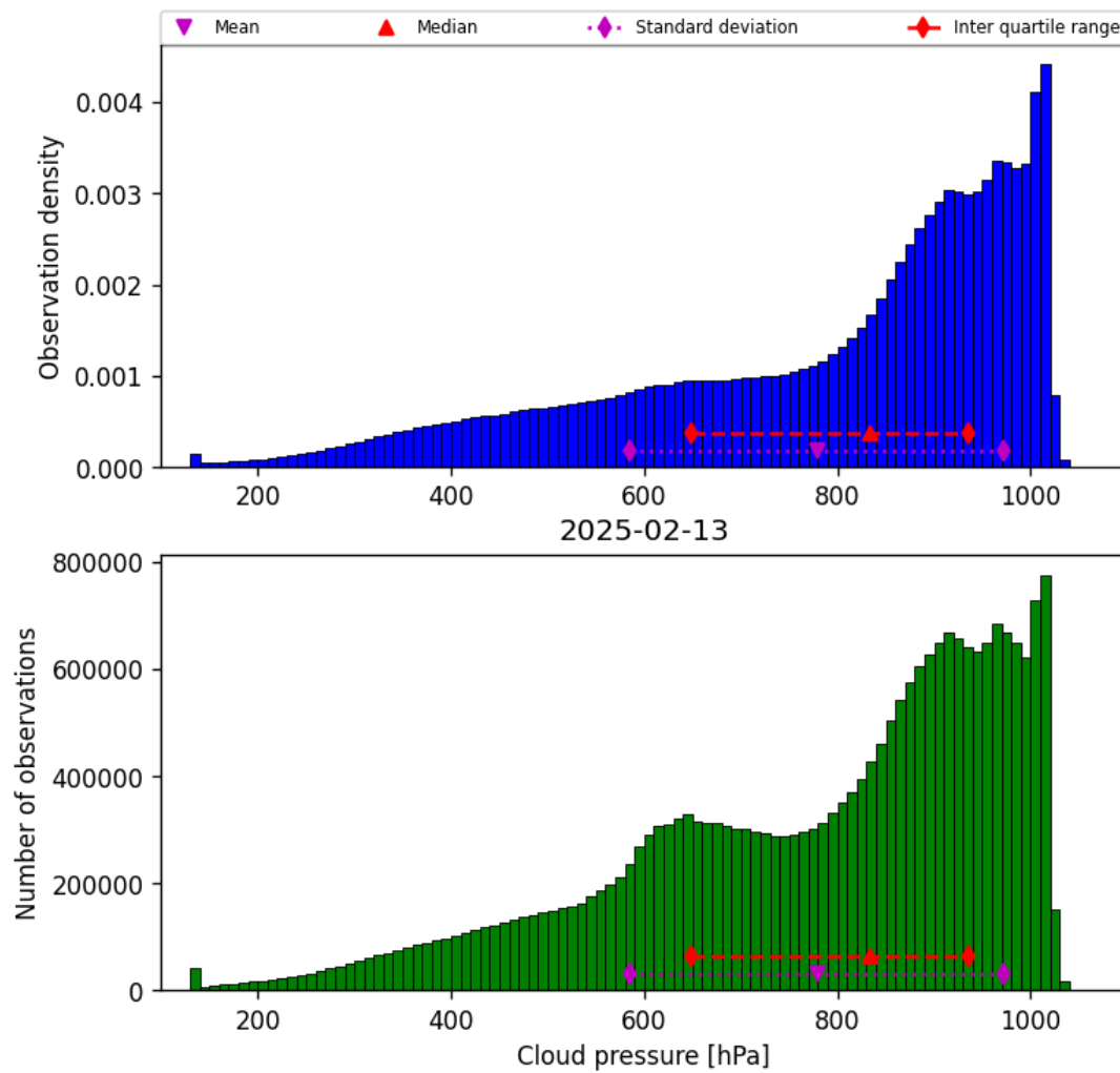
Figure 28: Histogram of “Cloud pressure” for 2025-02-13 to 2025-02-14
