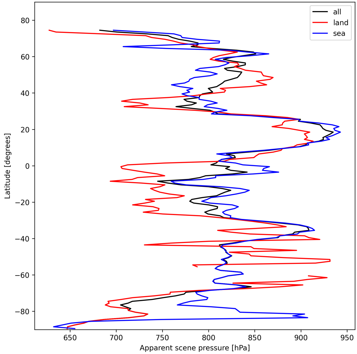
Figure 17: Zonal average of “Apparent scene pressure” for 2025-02-13 to 2025-02-14.
