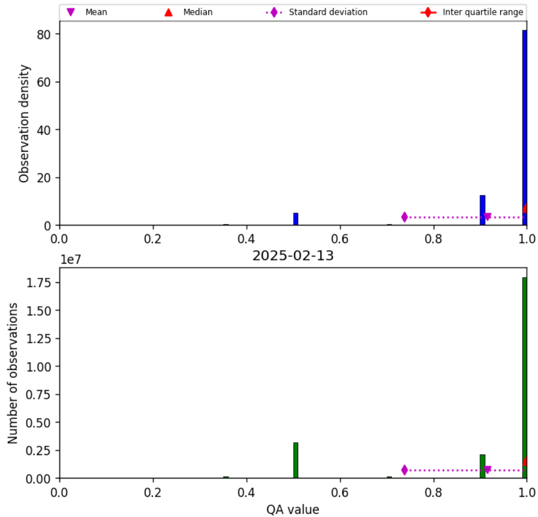
Figure 27: Histogram of “QA value” for 2025-02-13 to 2025-02-14
