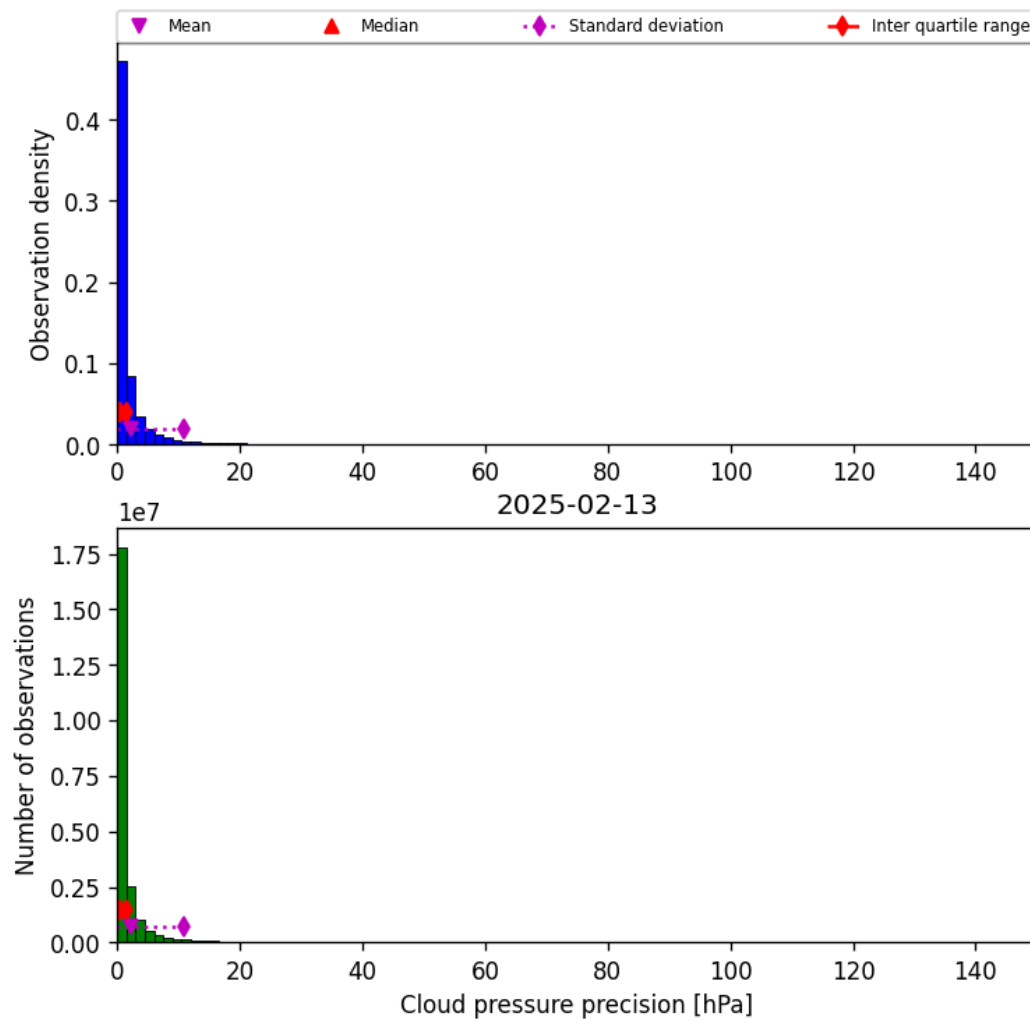
Figure 29: Histogram of “Cloud pressure precision” for 2025-02-13 to 2025-02-14
