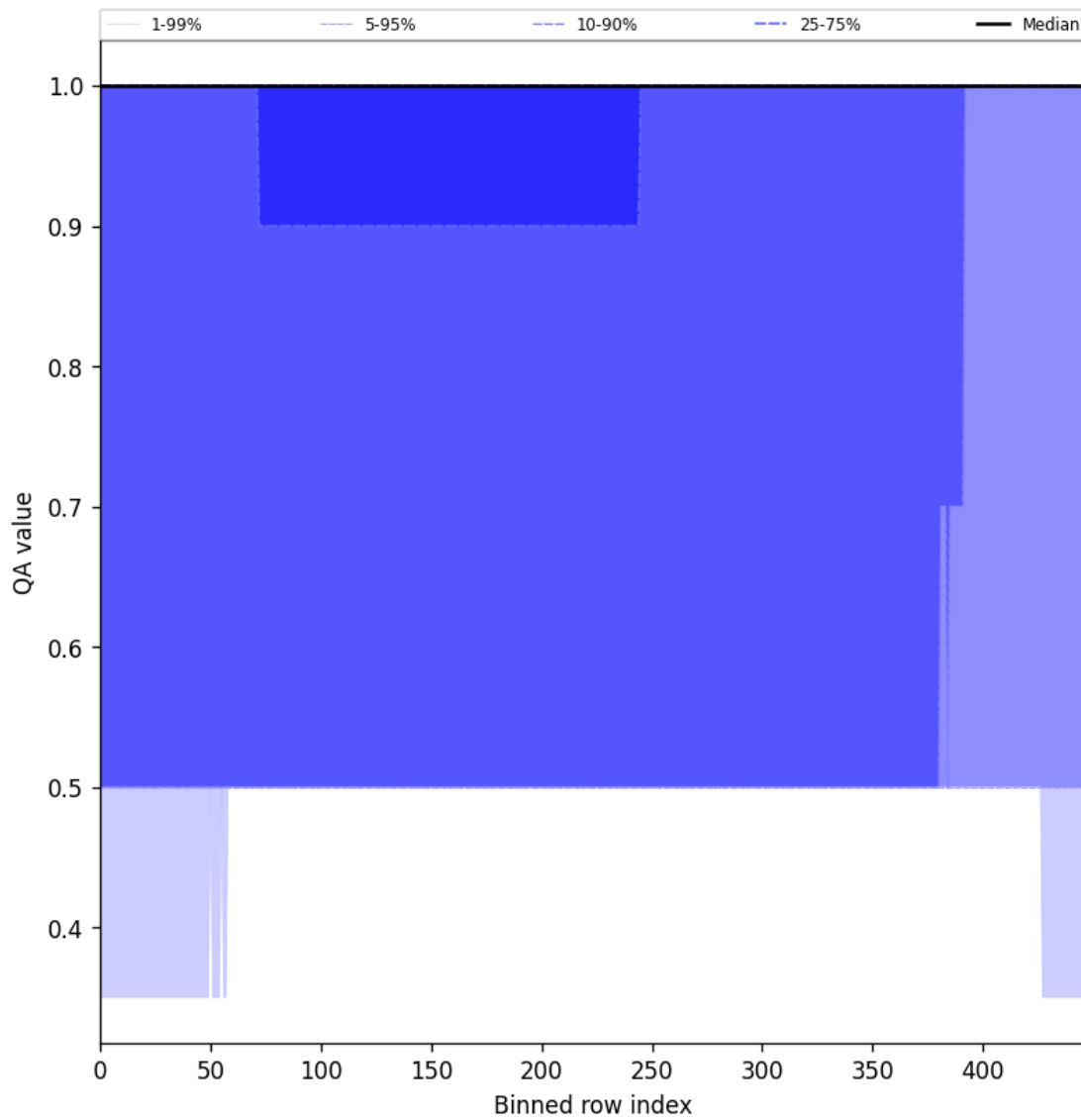
Figure 44: Along track statistics of “QA value” for 2025-02-13 to 2025-02-14
