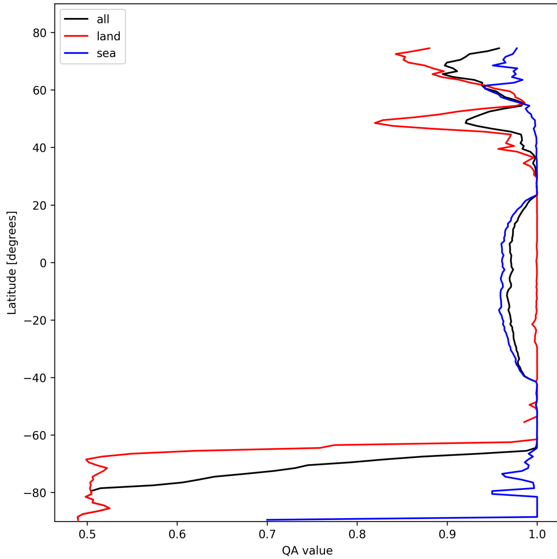
Figure 10: Zonal average of “QA value” for 2025-02-13 to 2025-02-14.
