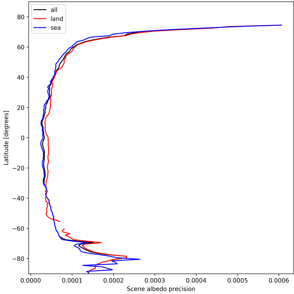
Figure 16: Zonal average of “Scene albedo precision” for 2025-02-13 to 2025-02-14.
