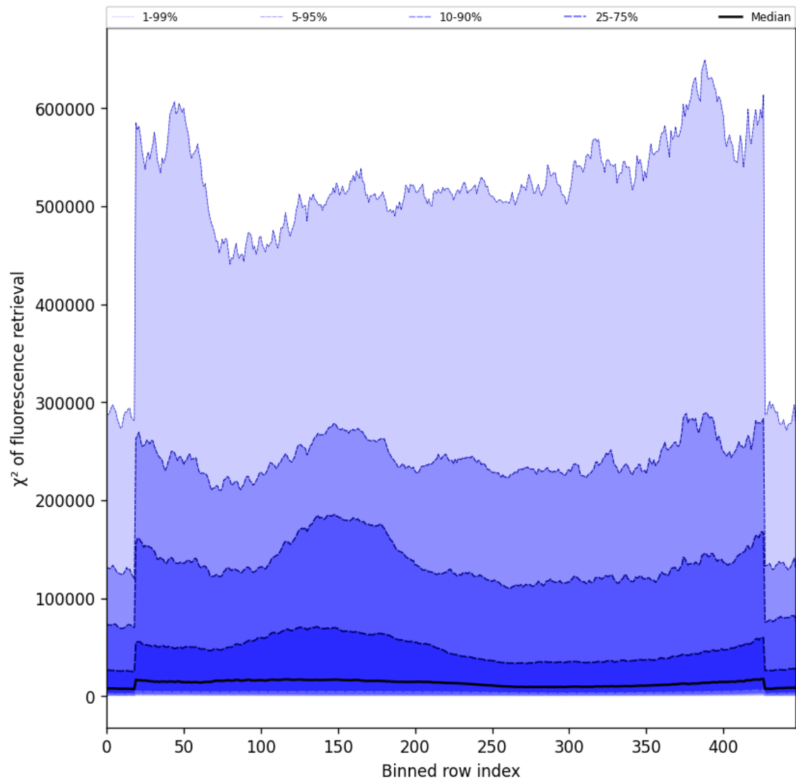
Figure 57: Along track statistics of " \chi^2 of fluorescence retrieval" for 2025-02-13 to 2025-02-14
