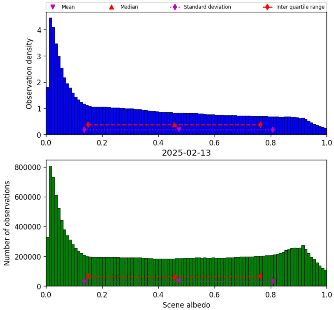
Figure 32: Histogram of “Scene albedo” for 2025-02-13 to 2025-02-14
