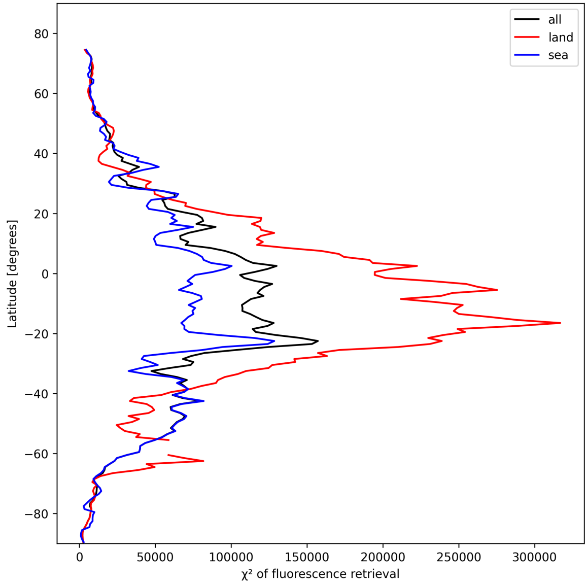
Figure 23: Zonal average of “ \chi^2 of fluorescence retrieval” for 2025-02-13 to 2025-02-14.
