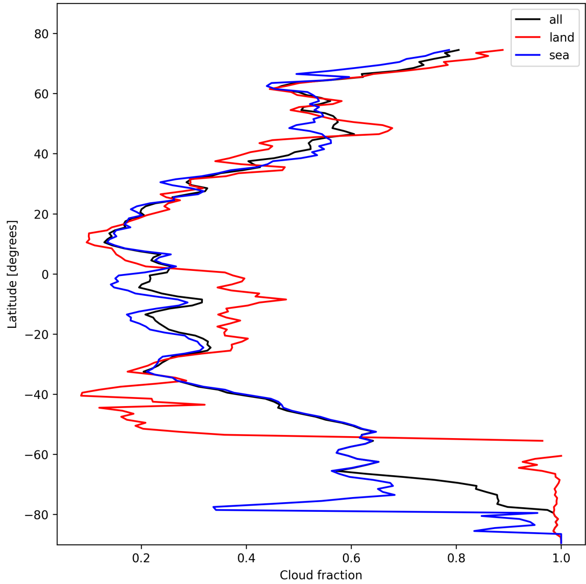
Figure 13: Zonal average of “Cloud fraction” for 2025-02-13 to 2025-02-14.
