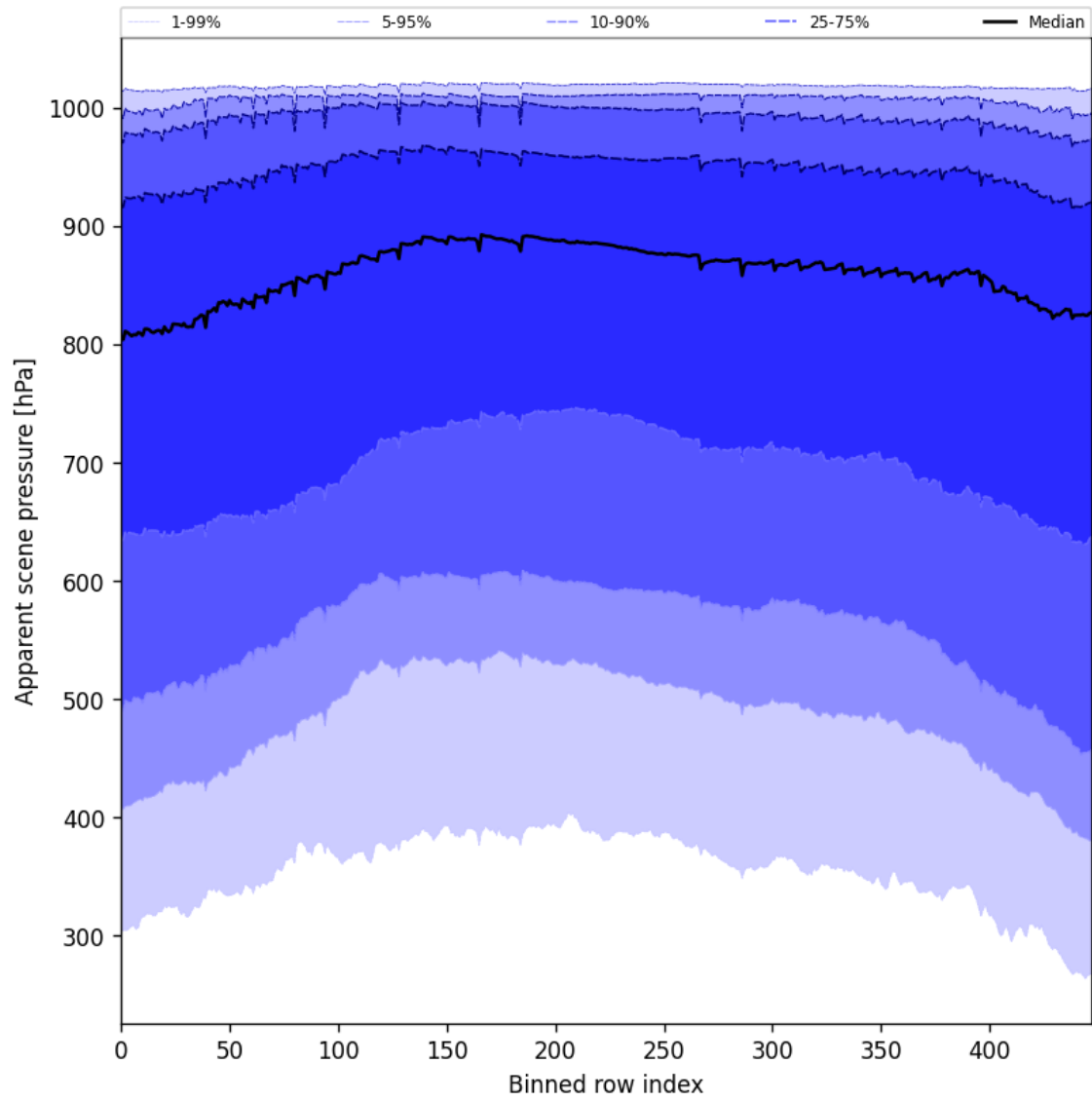
Figure 51: Along track statistics of “Apparent scene pressure” for 2025-02-13 to 2025-02-14
