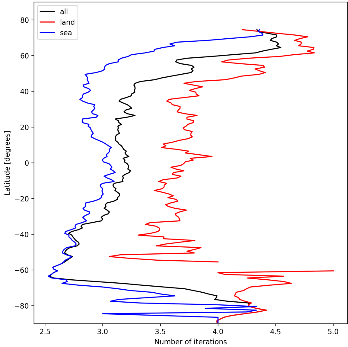
Figure 20: Zonal average of “Number of iterations” for 2025-02-13 to 2025-02-14.
