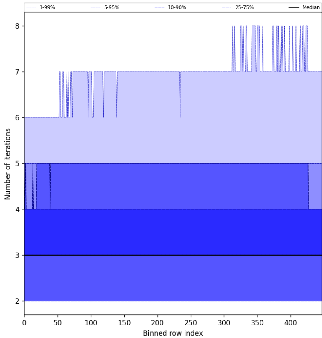
Figure 54: Along track statistics of “Number of iterations” for 2025-02-13 to 2025-02-14
