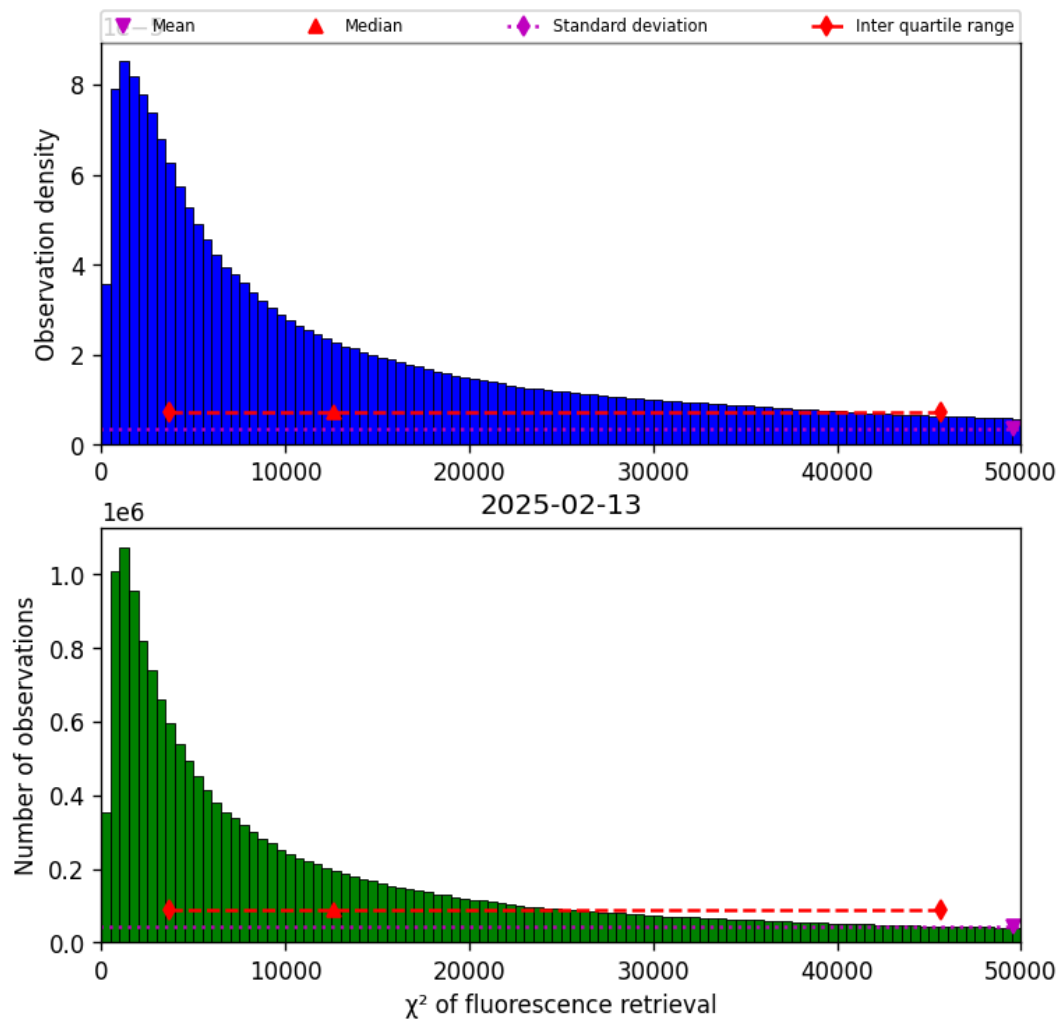
Figure 40: Histogram of “ \chi^2 of fluorescence retrieval” for 2025-02-13 to 2025-02-14
