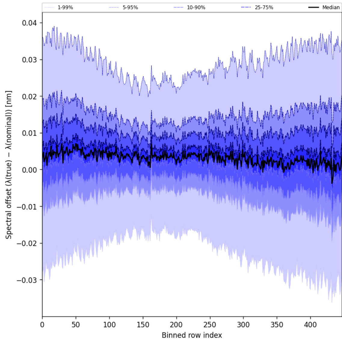
Figure 60: Along track statistics of “Spectral offset ( \lambda_{\text{true}} - \lambda_{\text{nominal}} )” for 2025-02-13 to 2025-02-14
