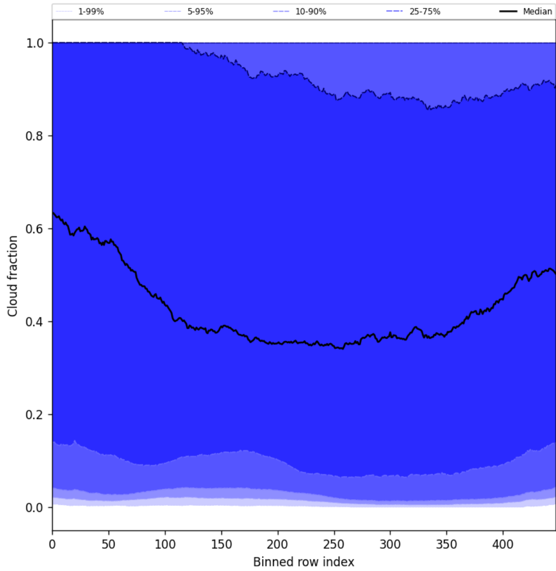
Figure 47: Along track statistics of “Cloud fraction” for 2025-02-13 to 2025-02-14
