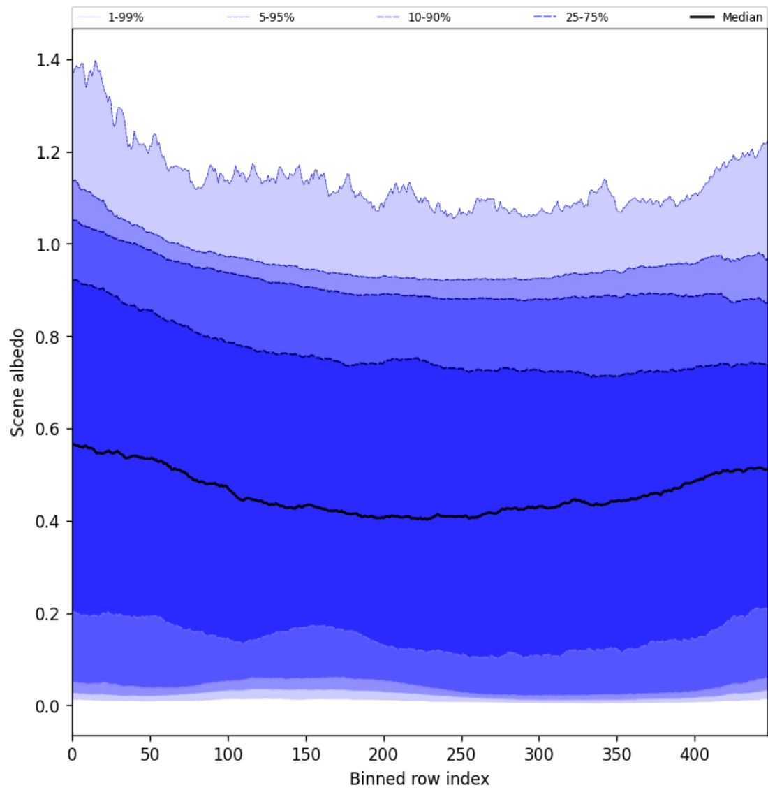
Figure 49: Along track statistics of “Scene albedo” for 2025-02-13 to 2025-02-14
