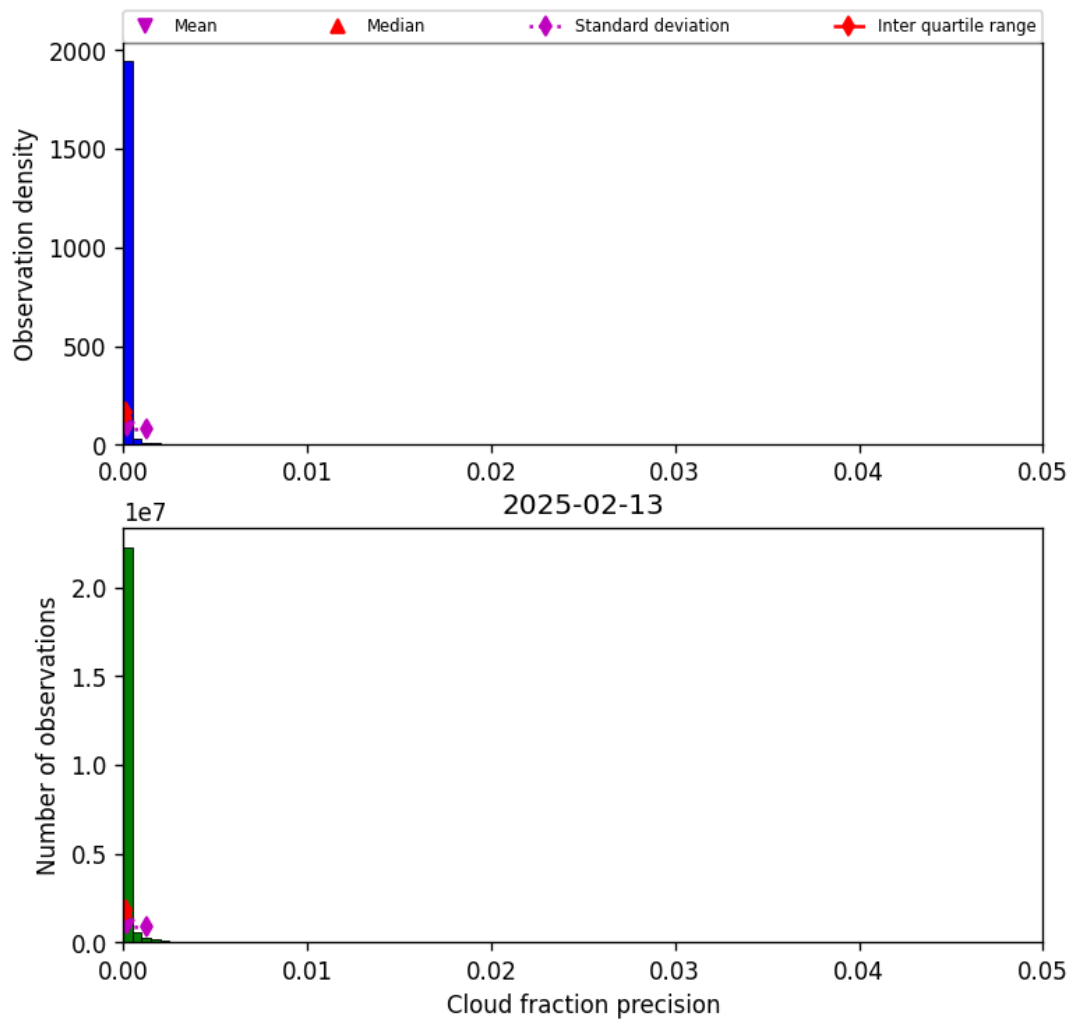
Figure 31: Histogram of “Cloud fraction precision” for 2025-02-13 to 2025-02-14
