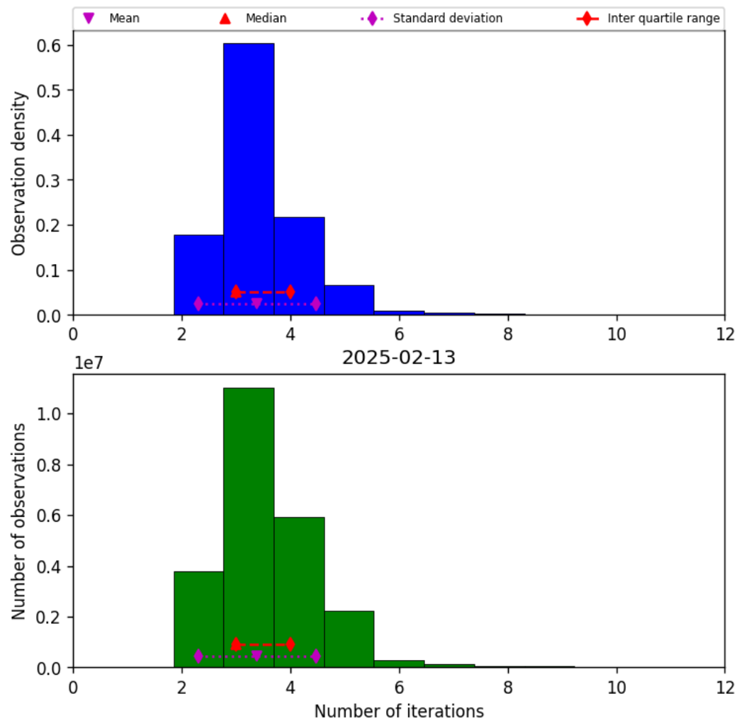
Figure 37: Histogram of “Number of iterations” for 2025-02-13 to 2025-02-14
