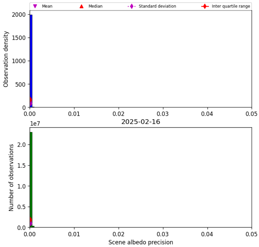
Figure 33: Histogram of “Scene albedo precision” for 2025-02-16 to 2025-02-16
