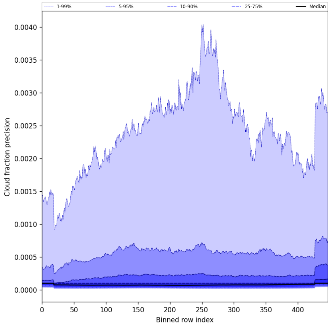
Figure 48: Along track statistics of “Cloud fraction precision” for 2025-02-16 to 2025-02-16
