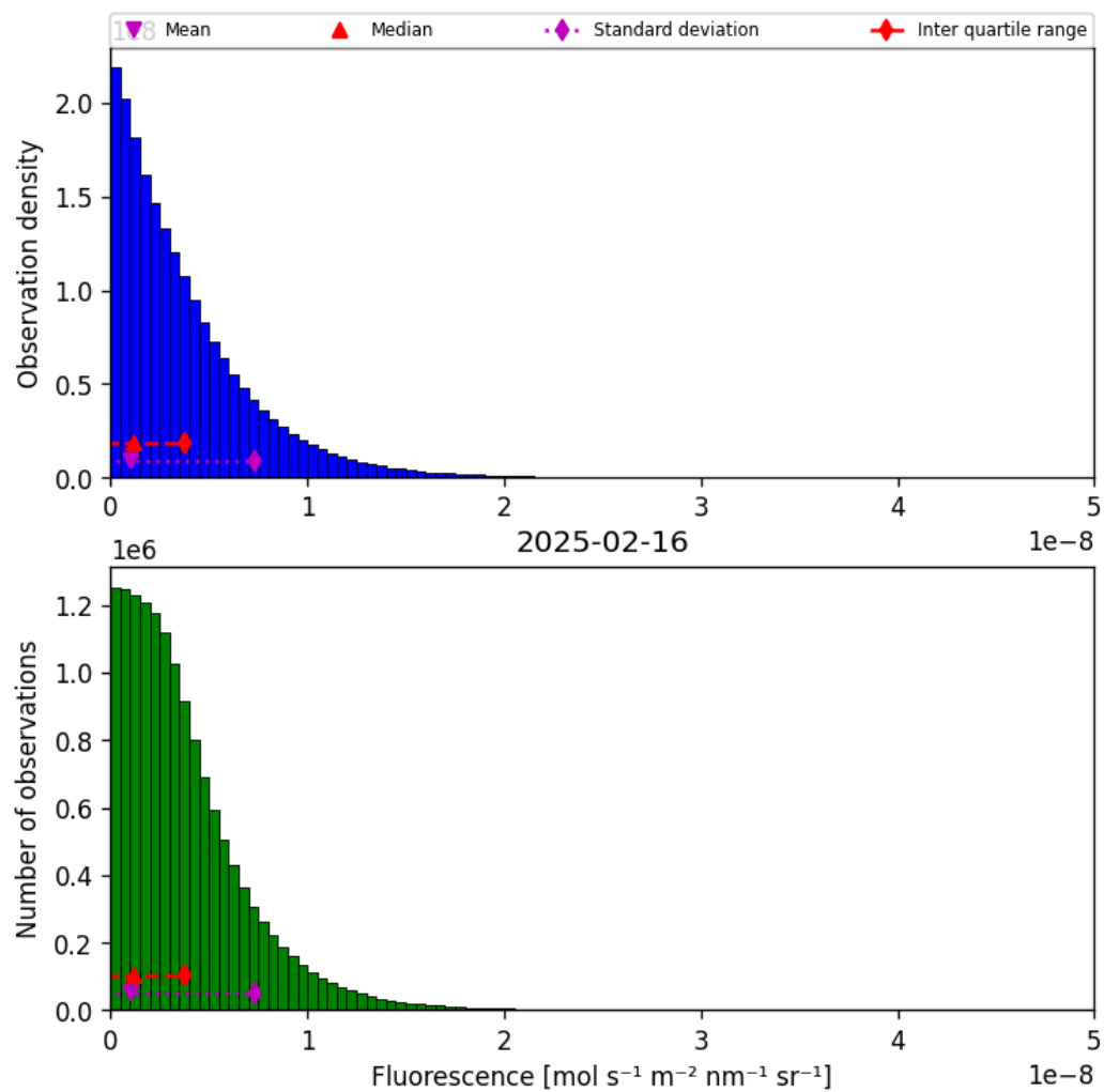
Figure 38: Histogram of “Fluorescence” for 2025-02-16 to 2025-02-16
