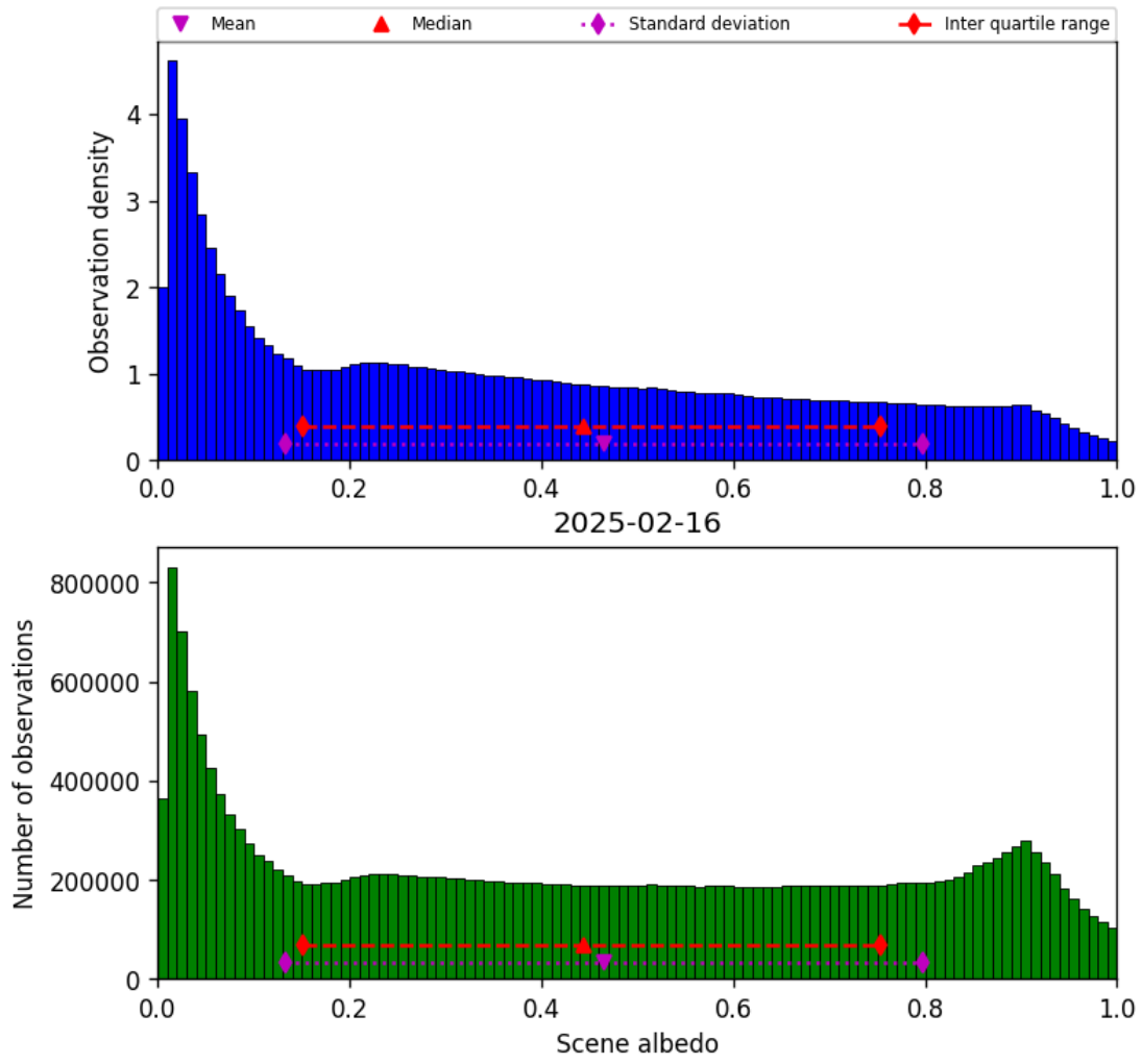
Figure 32: Histogram of “Scene albedo” for 2025-02-16 to 2025-02-16
