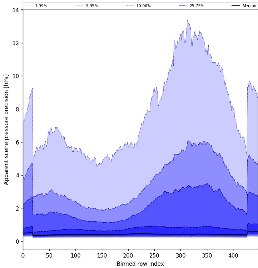
Figure 52: Along track statistics of “Apparent scene pressure precision” for 2025-02-16 to 2025-02-16
