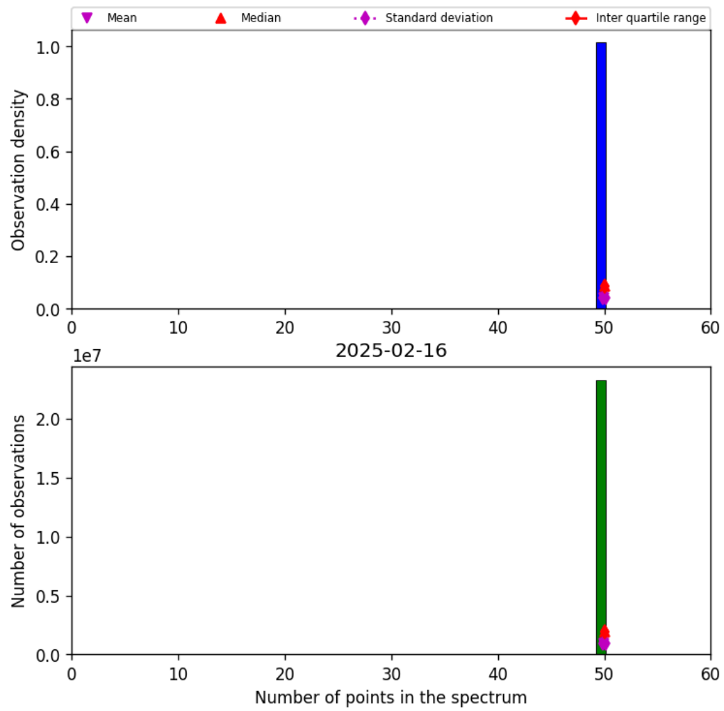
Figure 42: Histogram of "Number of points in the spectrum" for 2025-02-16 to 2025-02-16
