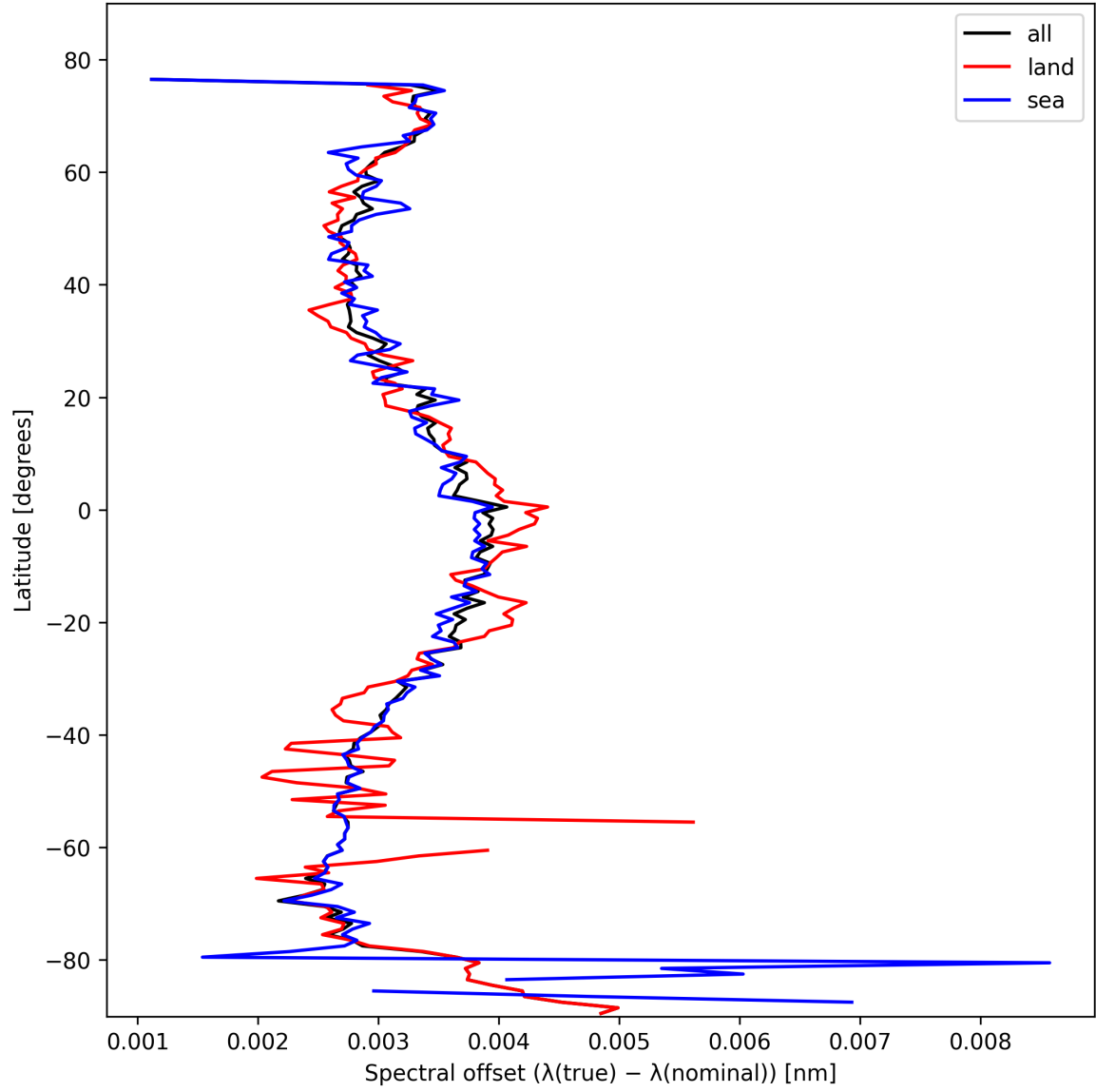
Figure 26: Zonal average of “Spectral offset ( \lambda_{\text{true}} - \lambda_{\text{nominal}} )” for 2025-02-16 to 2025-02-16.
