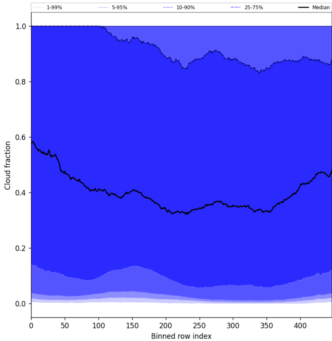
Figure 47: Along track statistics of “Cloud fraction” for 2025-02-16 to 2025-02-16
