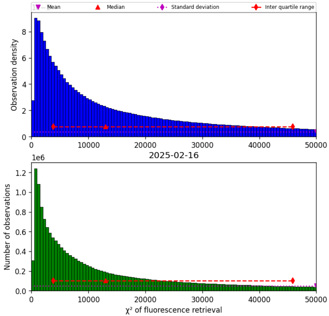
Figure 40: Histogram of “ \chi^2 of fluorescence retrieval” for 2025-02-16 to 2025-02-16
