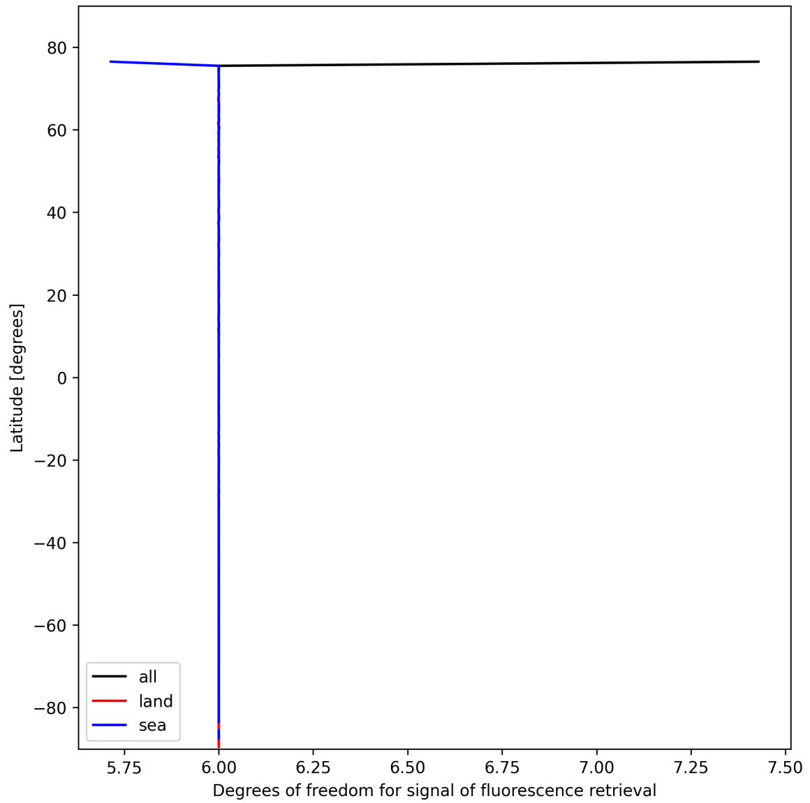
Figure 24: Zonal average of “Degrees of freedom for signal of fluorescence retrieval” for 2025-02-16 to 2025-02-16.
