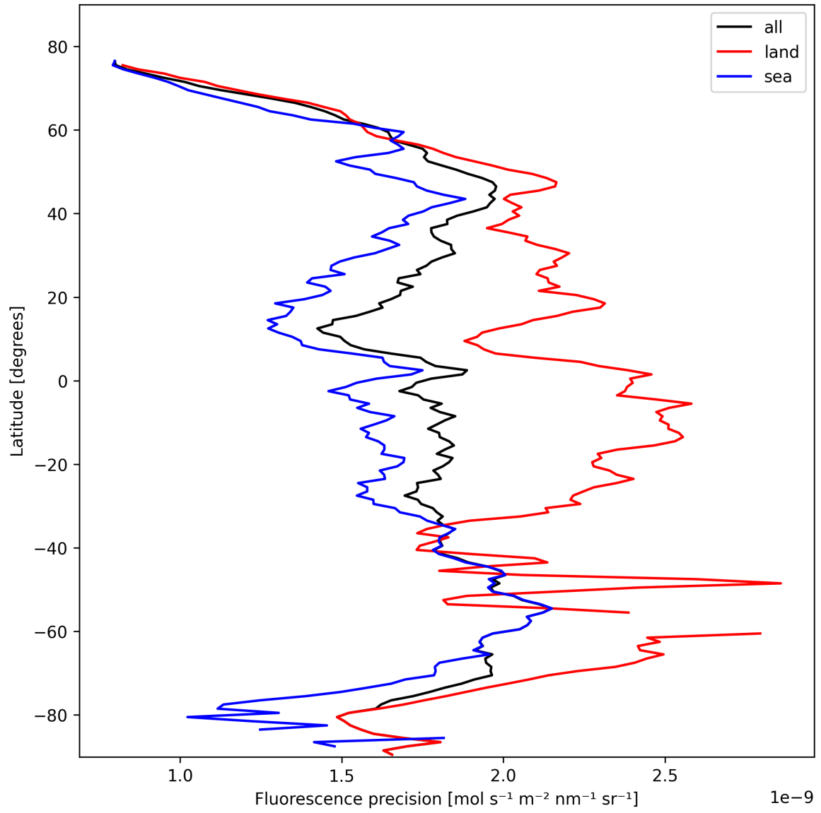
Figure 22: Zonal average of “Fluorescence precision” for 2025-02-16 to 2025-02-16.
