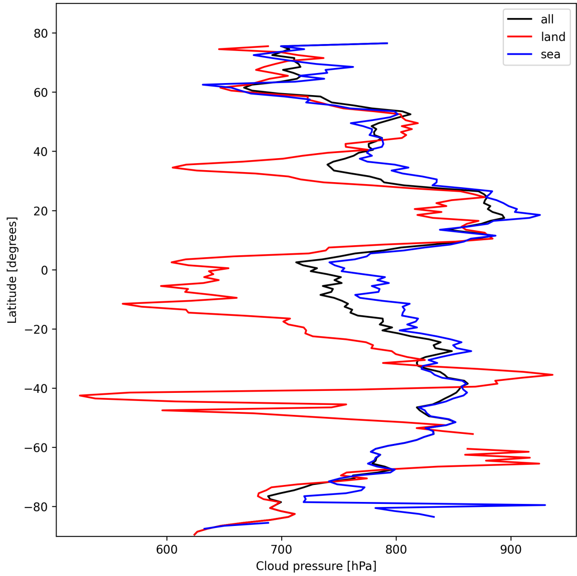
Figure 11: Zonal average of “Cloud pressure” for 2025-02-16 to 2025-02-16.
