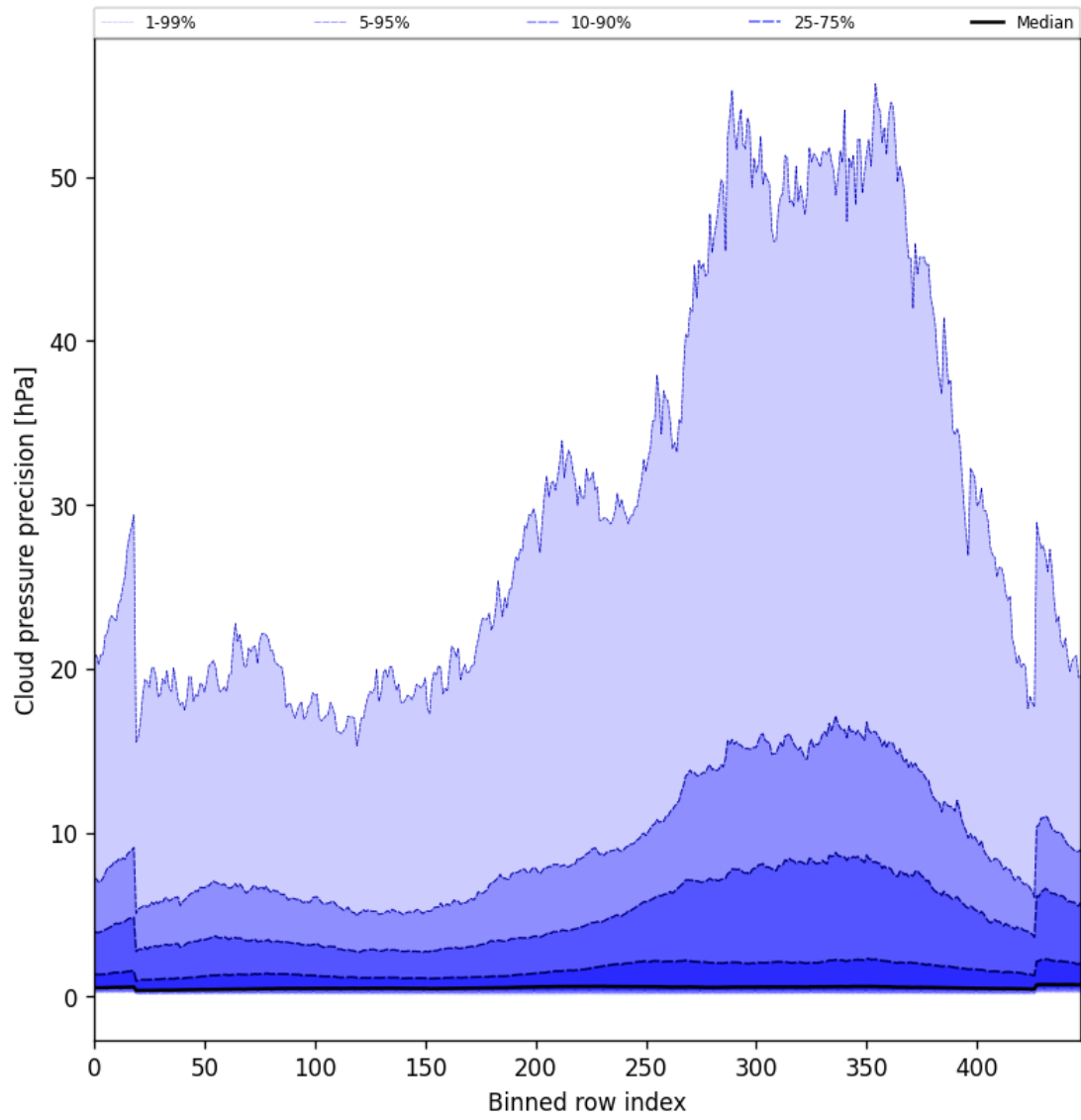
Figure 46: Along track statistics of “Cloud pressure precision” for 2025-02-16 to 2025-02-16
