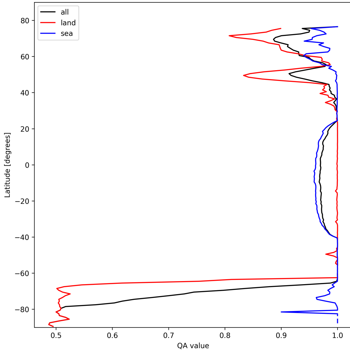
Figure 10: Zonal average of “QA value” for 2025-02-16 to 2025-02-16.
