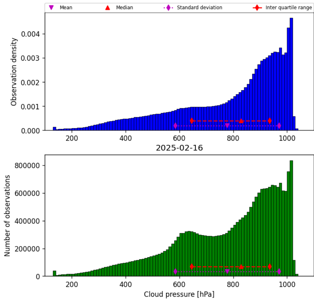
Figure 28: Histogram of “Cloud pressure” for 2025-02-16 to 2025-02-16
