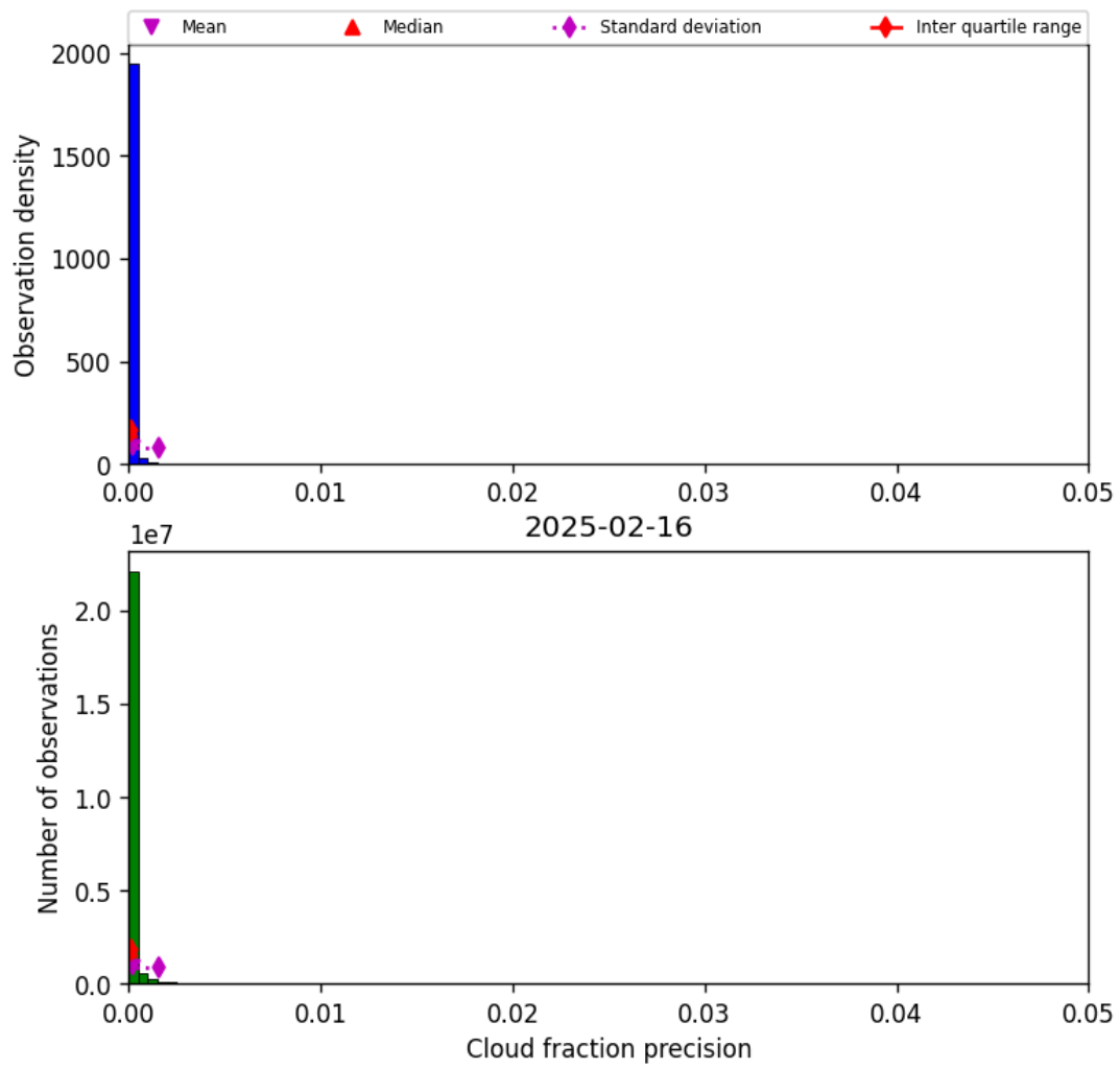
Figure 31: Histogram of “Cloud fraction precision” for 2025-02-16 to 2025-02-16
