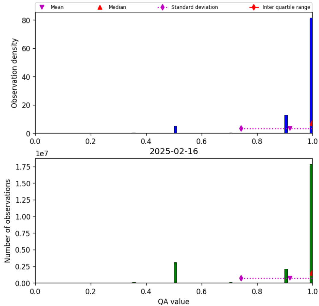
Figure 27: Histogram of “QA value” for 2025-02-16 to 2025-02-16
