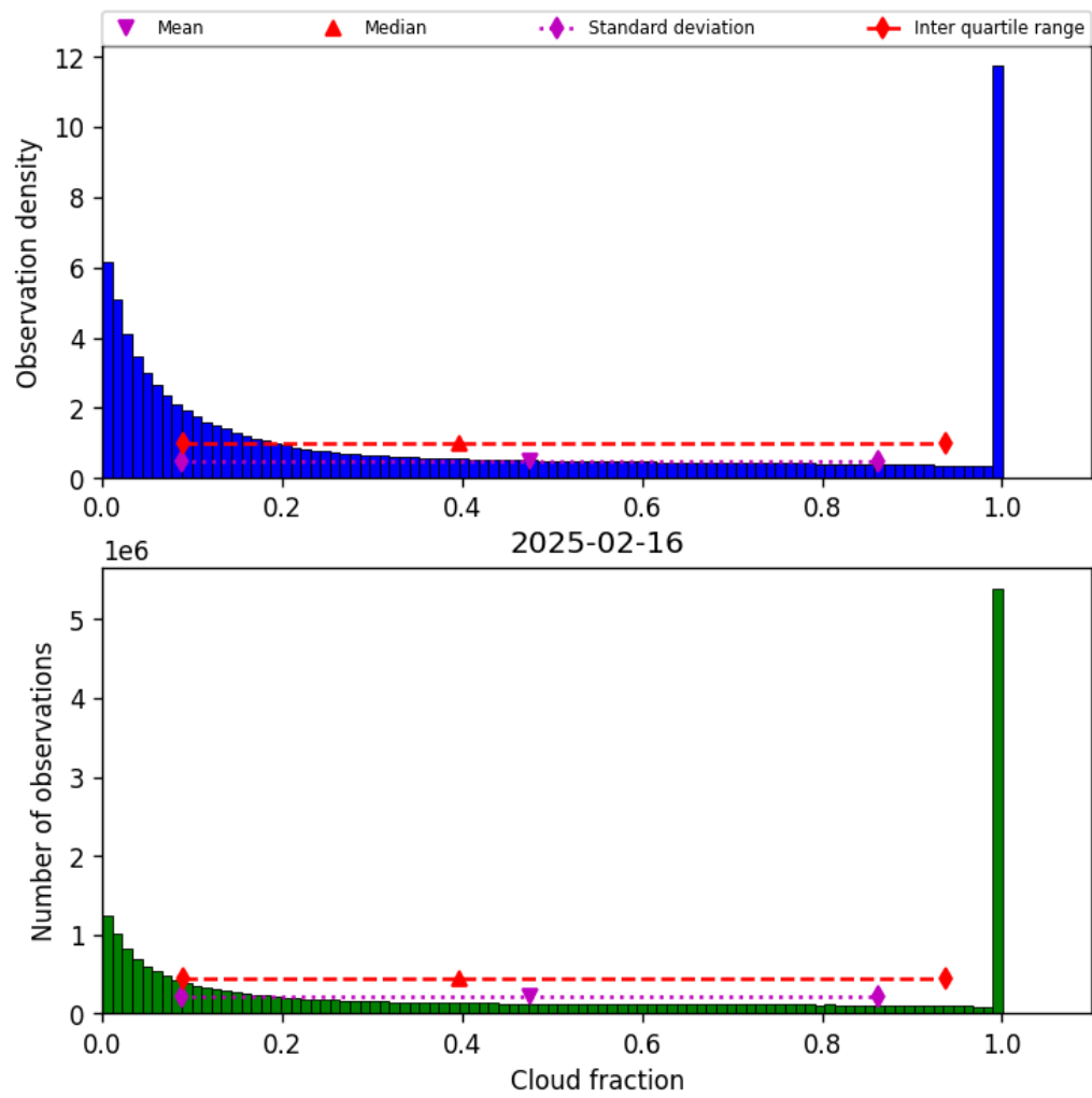
Figure 30: Histogram of “Cloud fraction” for 2025-02-16 to 2025-02-16
