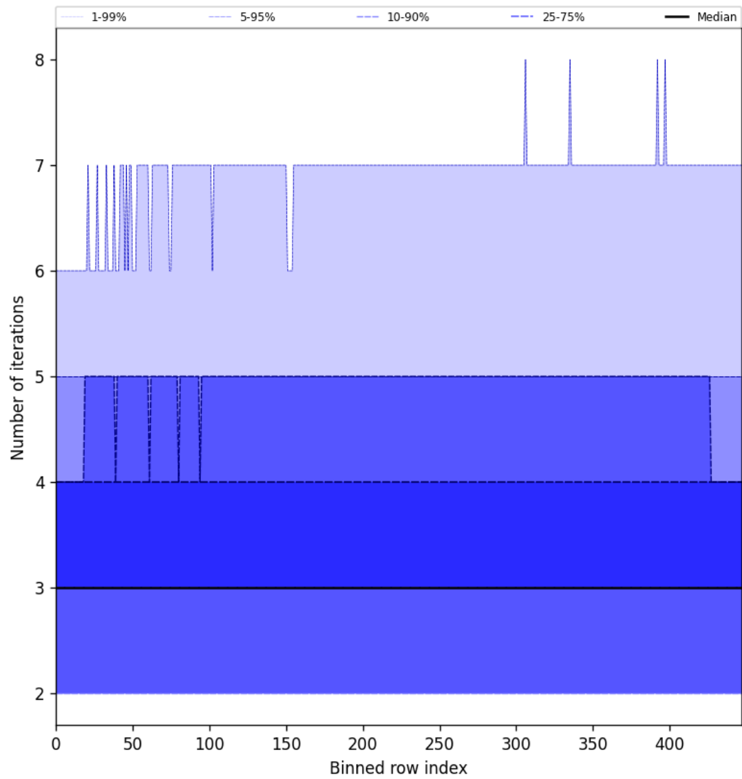
Figure 54: Along track statistics of “Number of iterations” for 2025-02-16 to 2025-02-16
