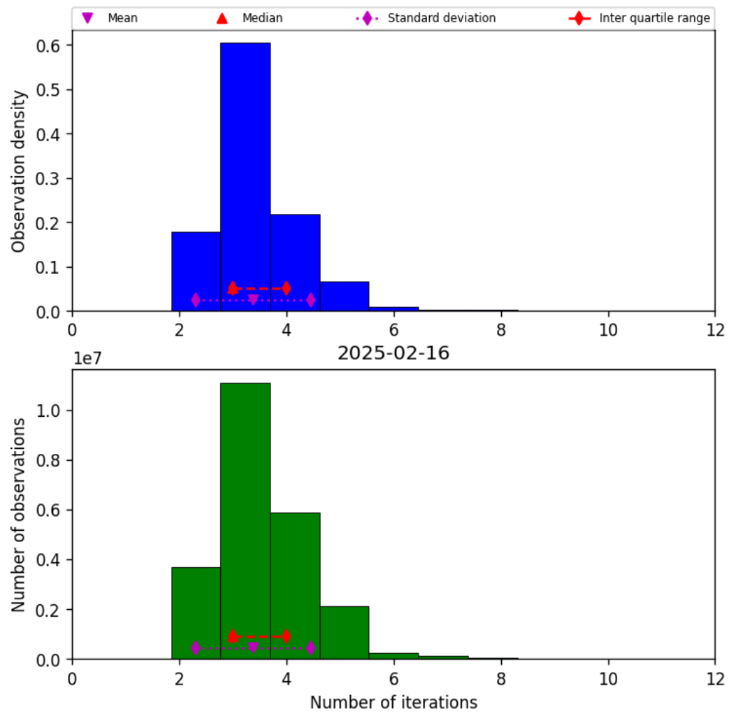
Figure 37: Histogram of “Number of iterations” for 2025-02-16 to 2025-02-16
