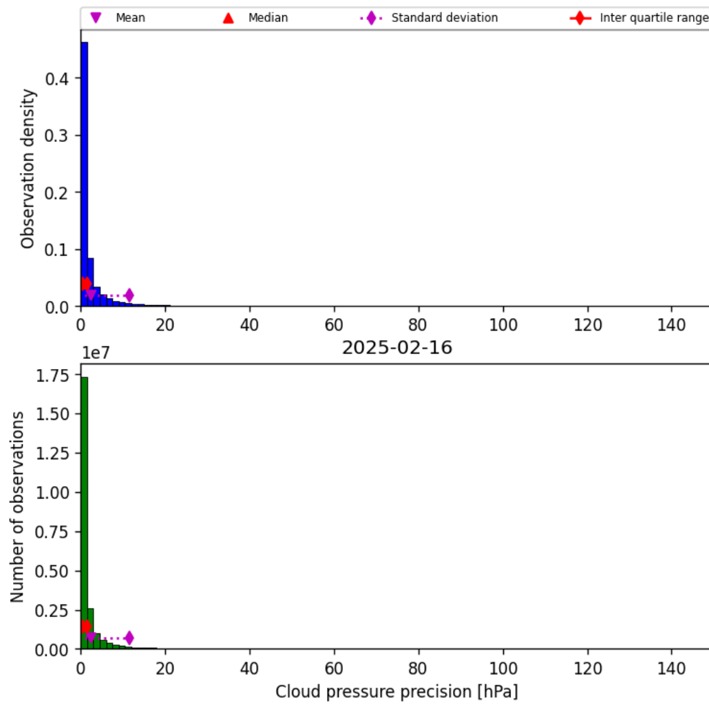
Figure 29: Histogram of “Cloud pressure precision” for 2025-02-16 to 2025-02-16
