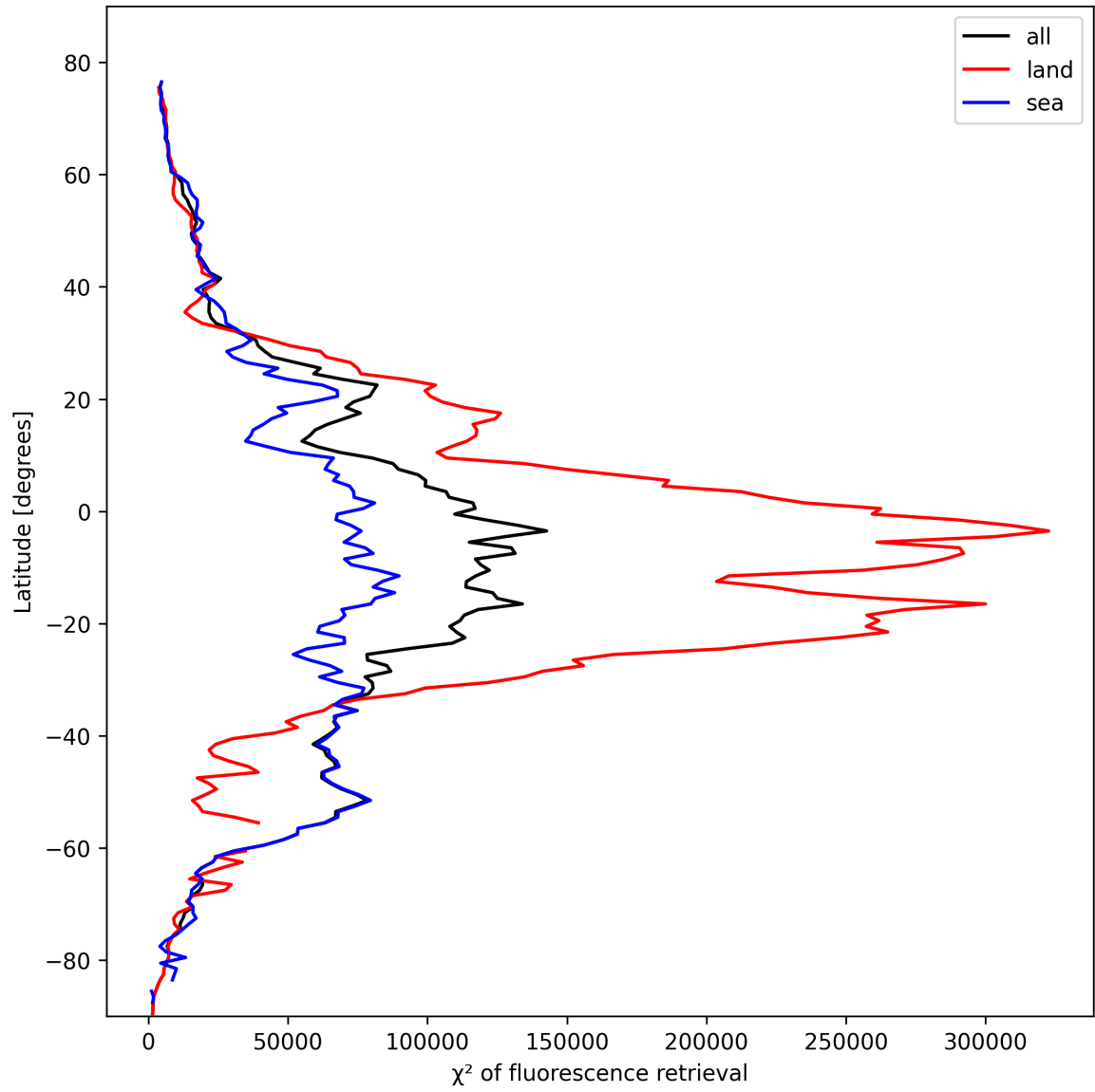
Figure 23: Zonal average of “ \chi^2 of fluorescence retrieval” for 2025-02-16 to 2025-02-16.
