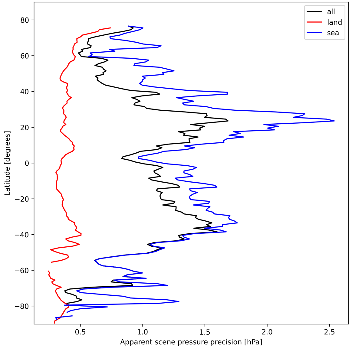
Figure 18: Zonal average of “Apparent scene pressure precision” for 2025-02-16 to 2025-02-16.
