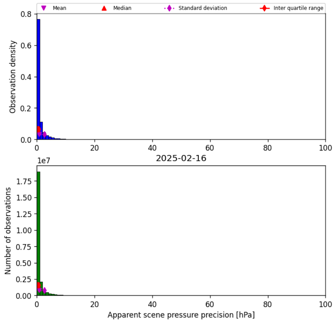
Figure 35: Histogram of "Apparent scene pressure precision" for 2025-02-16 to 2025-02-16
