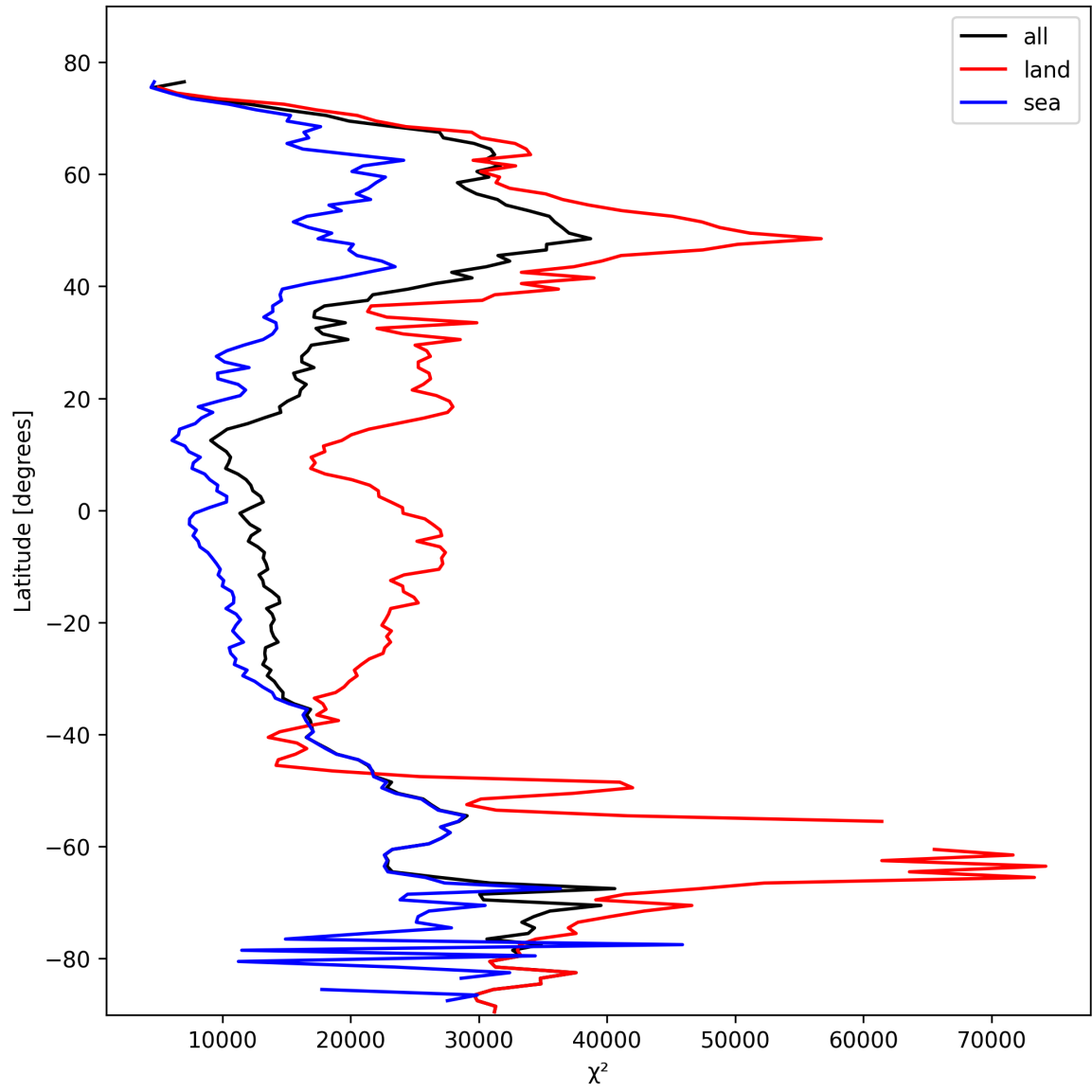
Figure 19: Zonal average of “ \chi^2 ” for 2025-02-16 to 2025-02-16.
