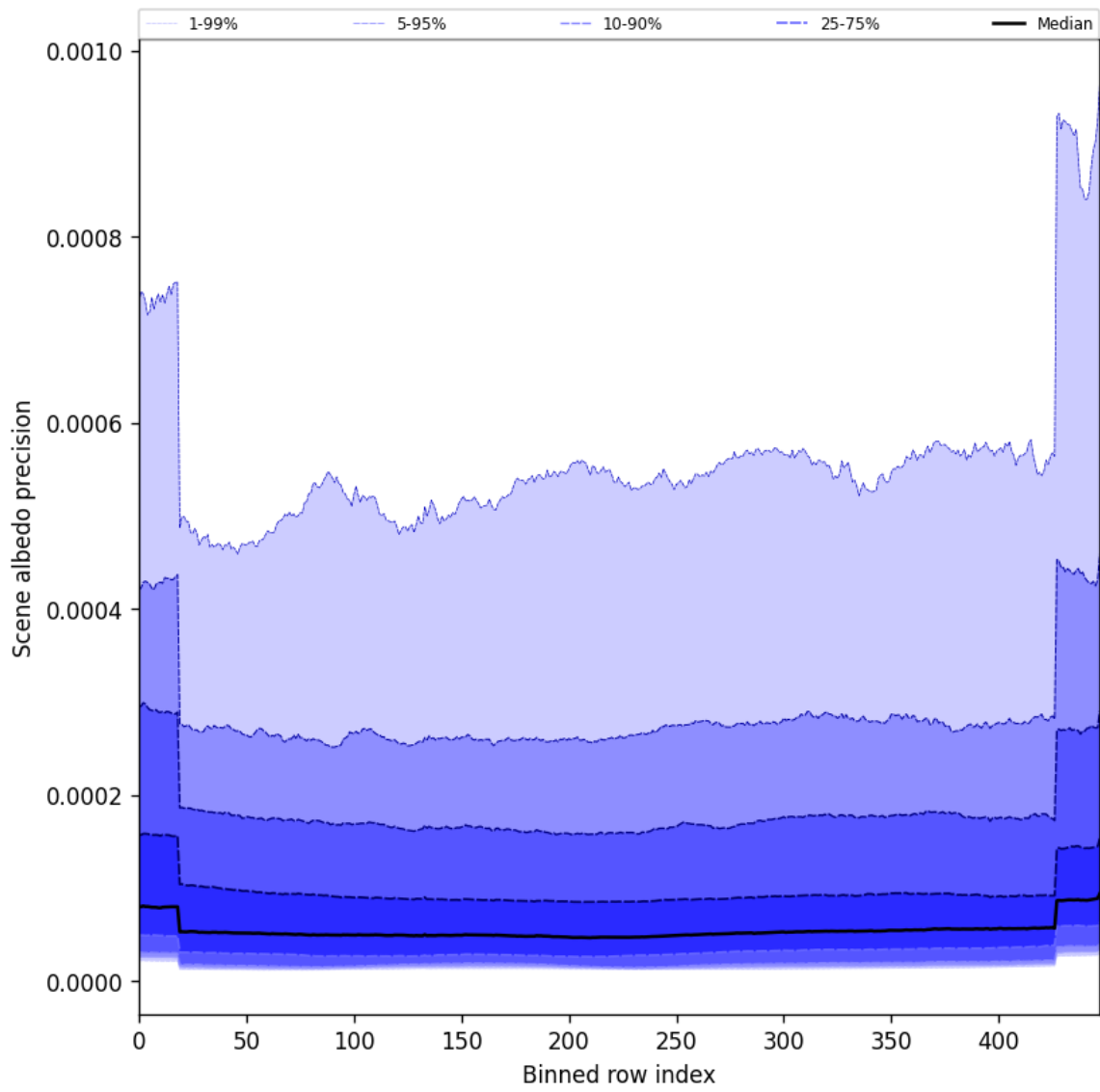
Figure 50: Along track statistics of “Scene albedo precision” for 2025-02-16 to 2025-02-16
