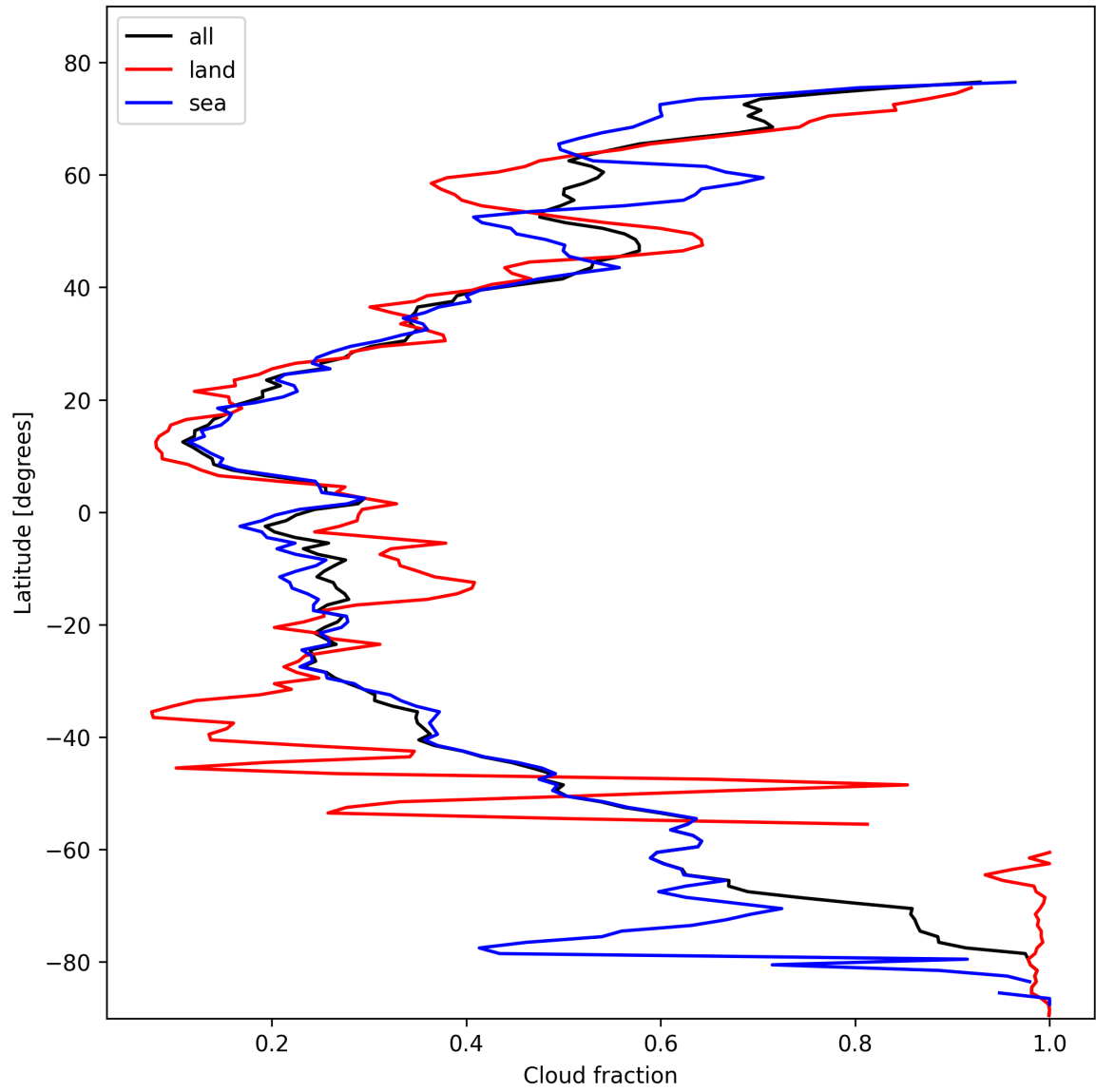
Figure 13: Zonal average of “Cloud fraction” for 2025-02-16 to 2025-02-16.
