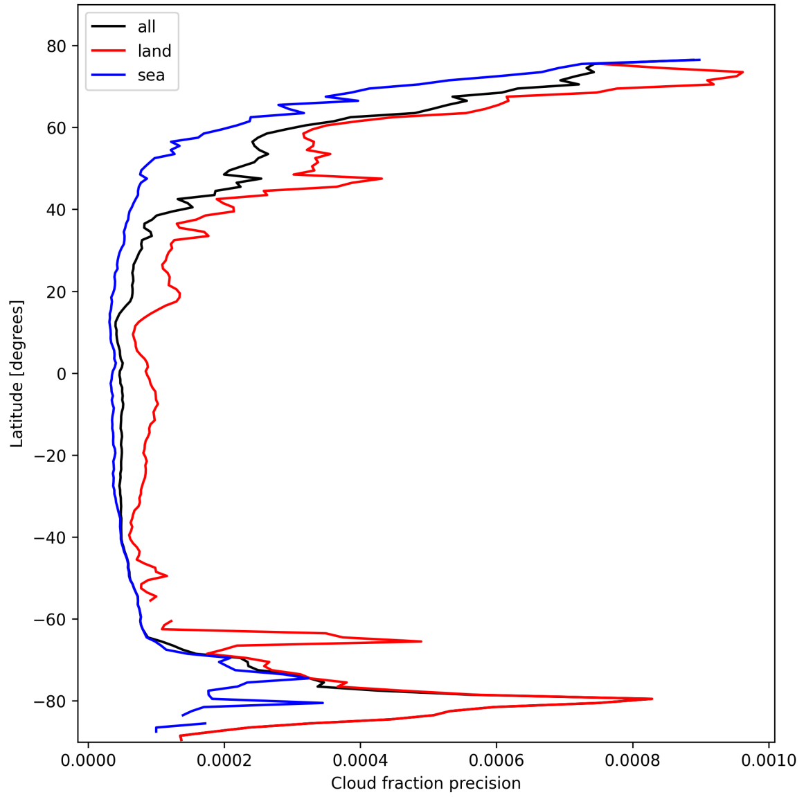
Figure 14: Zonal average of “Cloud fraction precision” for 2025-02-16 to 2025-02-16.
