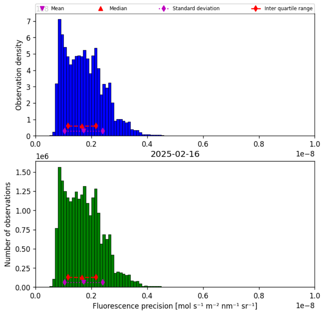
Figure 39: Histogram of “Fluorescence precision” for 2025-02-16 to 2025-02-16
