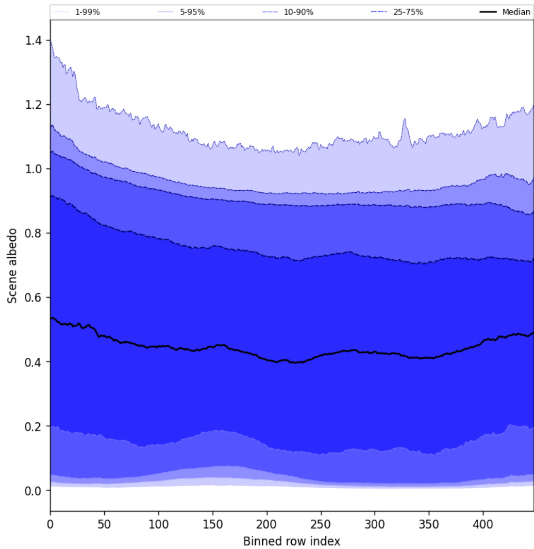
Figure 49: Along track statistics of “Scene albedo” for 2025-02-16 to 2025-02-16
