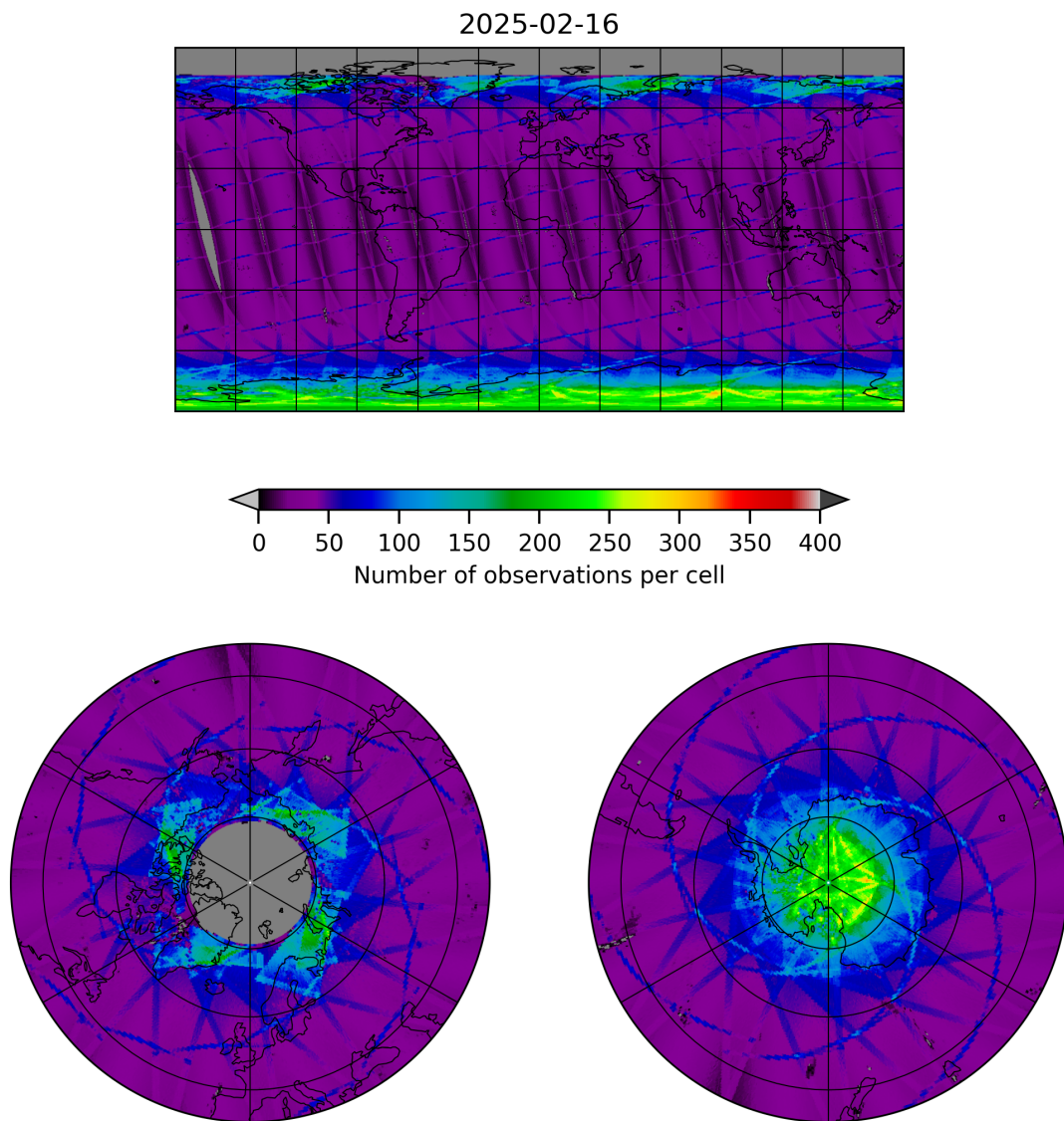
Figure 9: Map of the number of observations for 2025-02-16 to 2025-02-16
