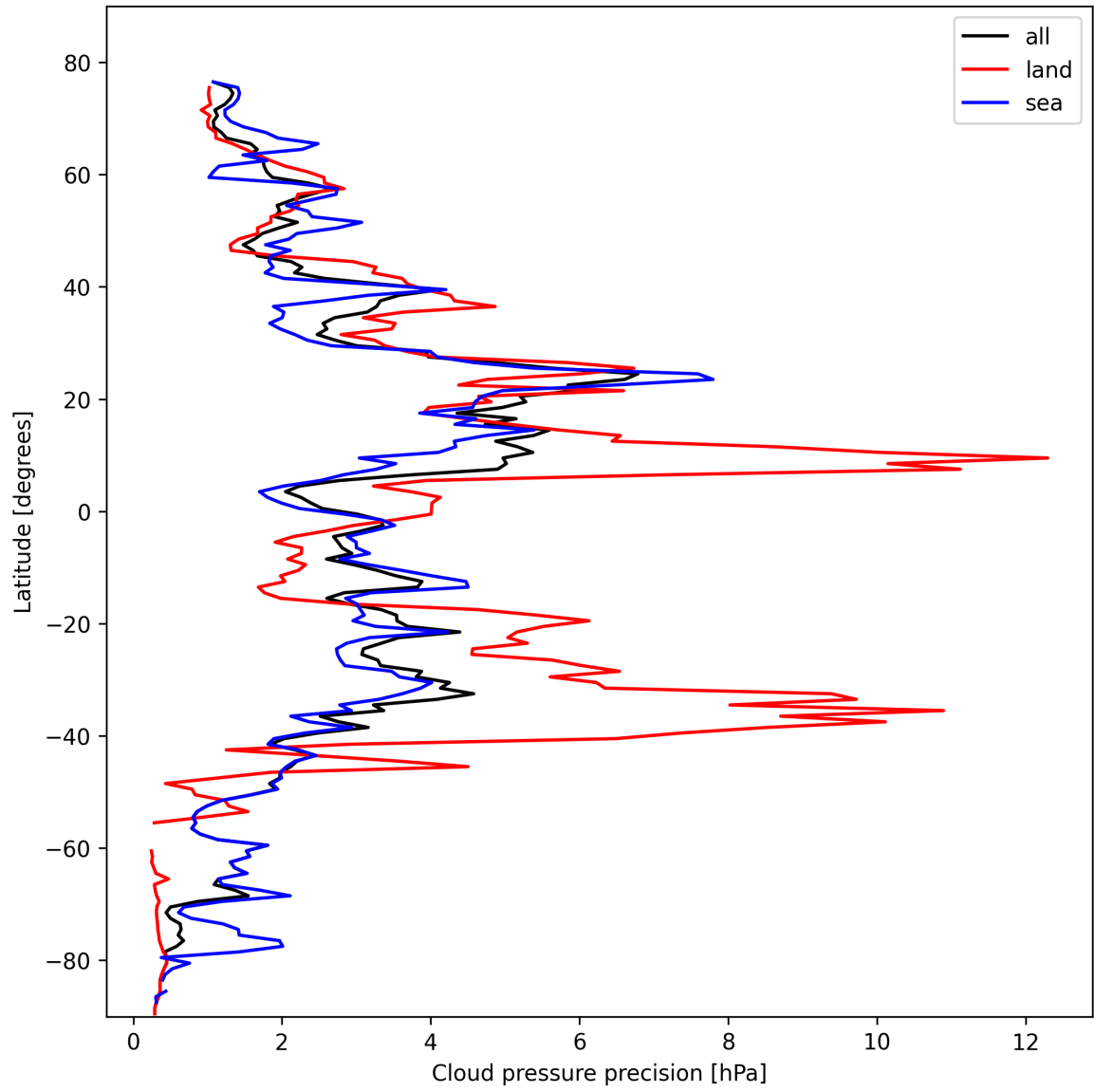
Figure 12: Zonal average of “Cloud pressure precision” for 2025-02-16 to 2025-02-16.
