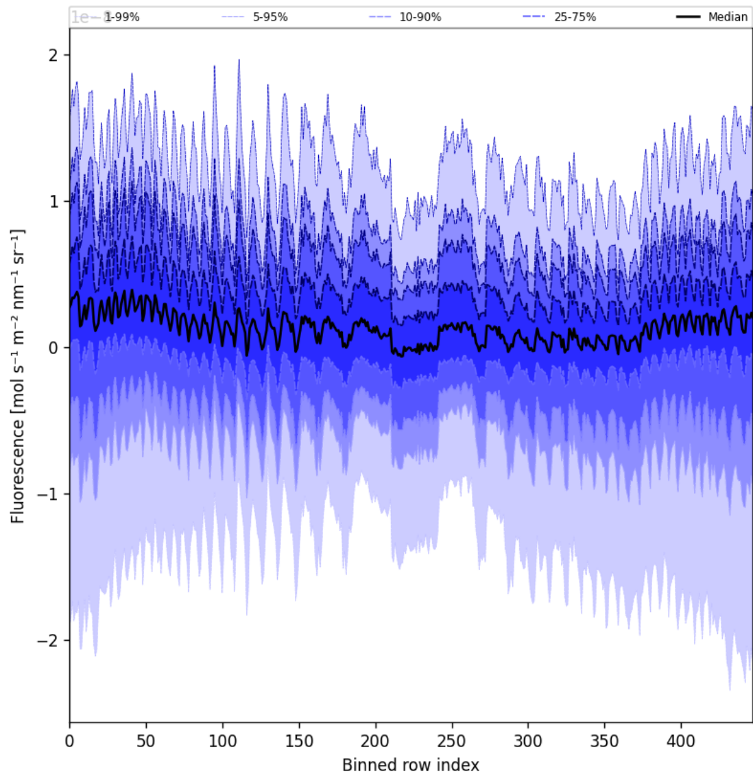
Figure 55: Along track statistics of “Fluorescence” for 2025-02-16 to 2025-02-16
