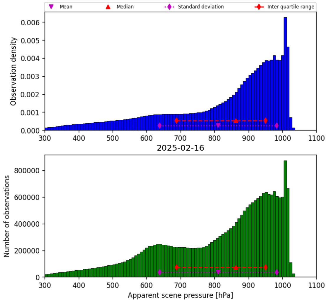
Figure 34: Histogram of “Apparent scene pressure” for 2025-02-16 to 2025-02-16
