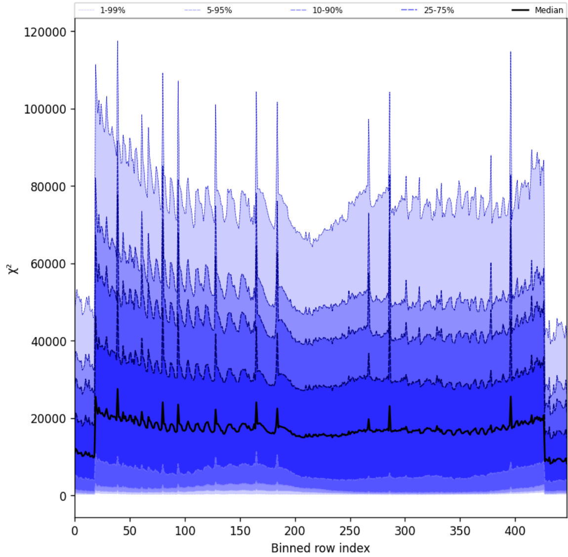
Figure 53: Along track statistics of “ \chi^2 ” for 2025-02-16 to 2025-02-16
