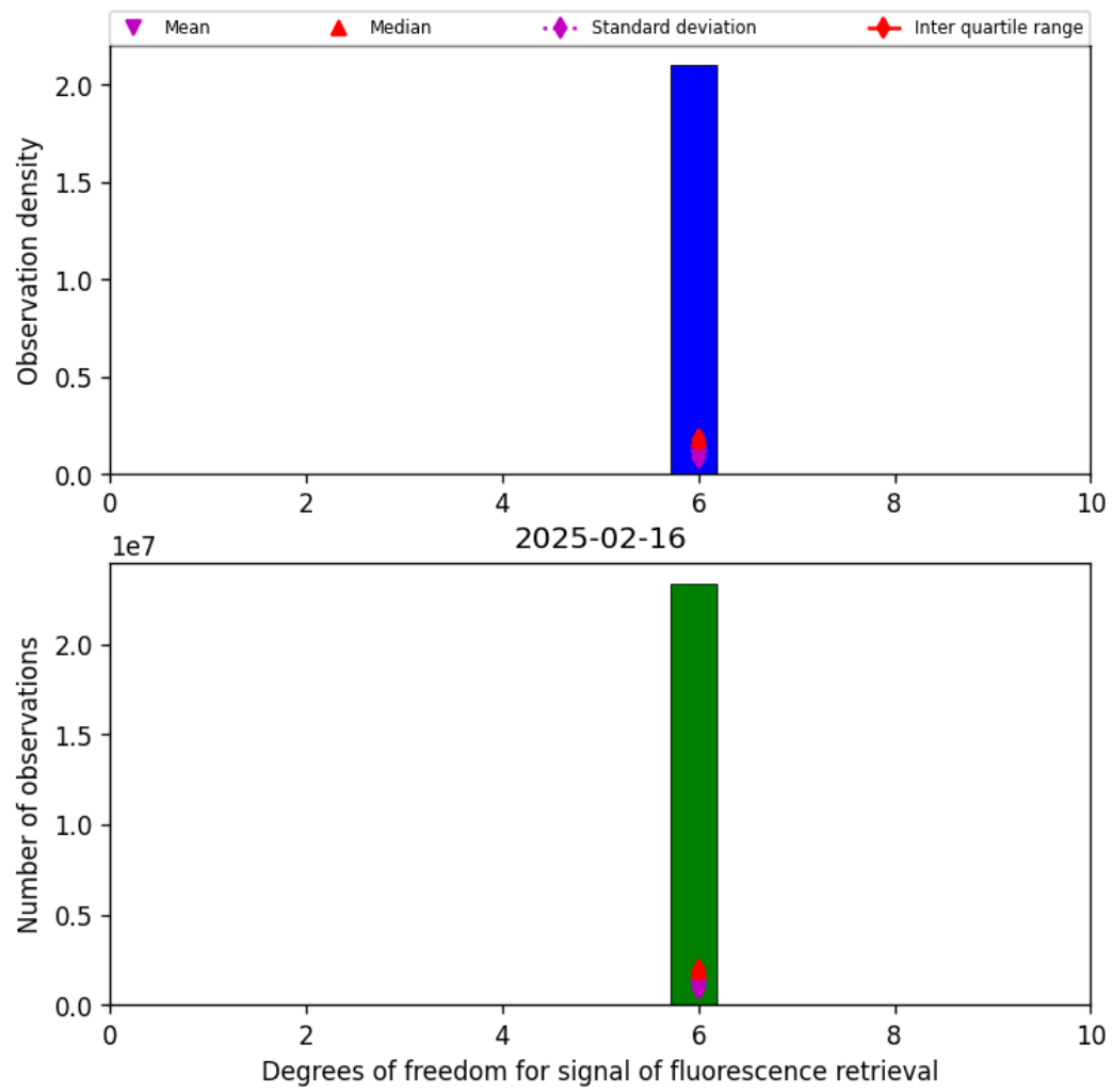
Figure 41: Histogram of “Degrees of freedom for signal of fluorescence retrieval” for 2025-02-16 to 2025-02-16
