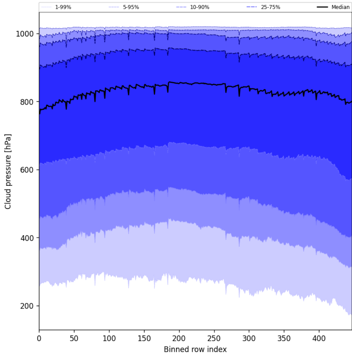
Figure 45: Along track statistics of “Cloud pressure” for 2025-02-16 to 2025-02-16
