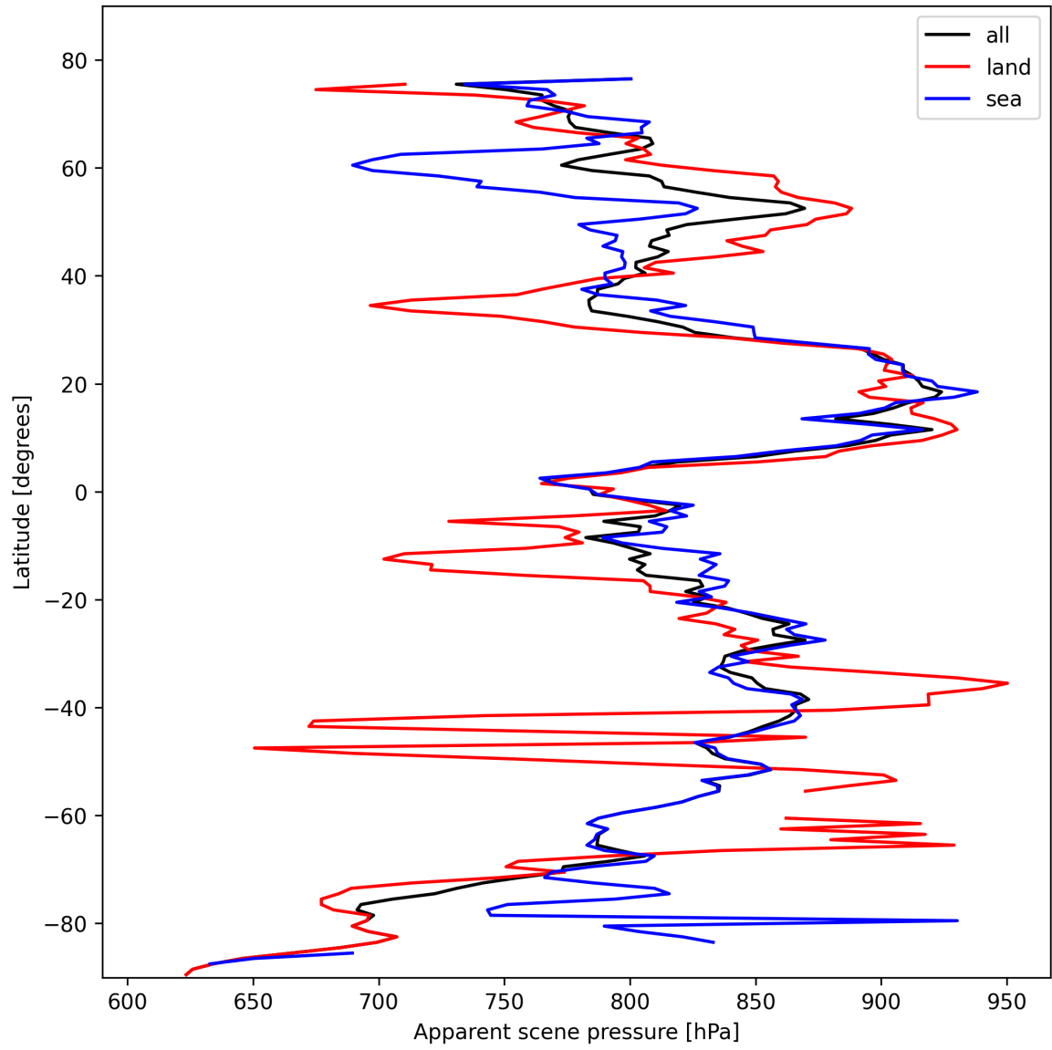
Figure 17: Zonal average of “Apparent scene pressure” for 2025-02-16 to 2025-02-16.
