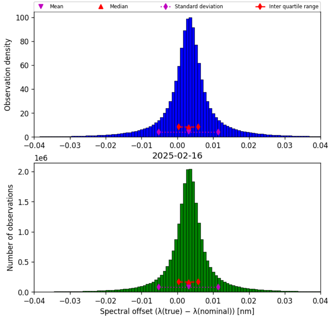
Figure 43: Histogram of “Spectral offset ( \lambda_{\text{true}} - \lambda_{\text{nominal}} )” for 2025-02-16 to 2025-02-16
