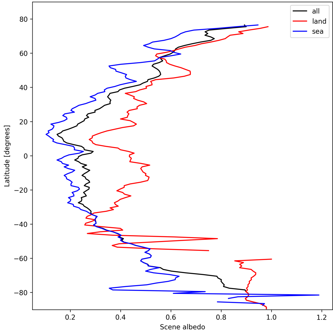
Figure 15: Zonal average of “Scene albedo” for 2025-02-16 to 2025-02-16.
