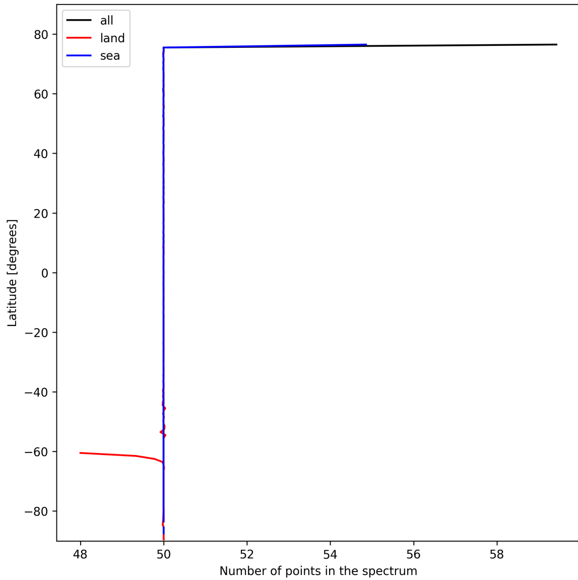
Figure 25: Zonal average of “Number of points in the spectrum” for 2025-02-16 to 2025-02-16.
