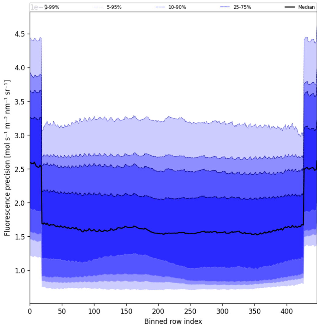
Figure 56: Along track statistics of “Fluorescence precision” for 2025-02-16 to 2025-02-16
