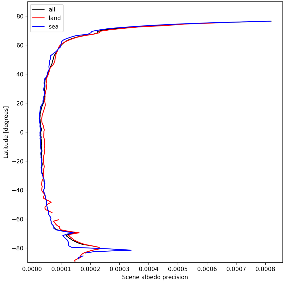
Figure 16: Zonal average of “Scene albedo precision” for 2025-02-16 to 2025-02-16.
