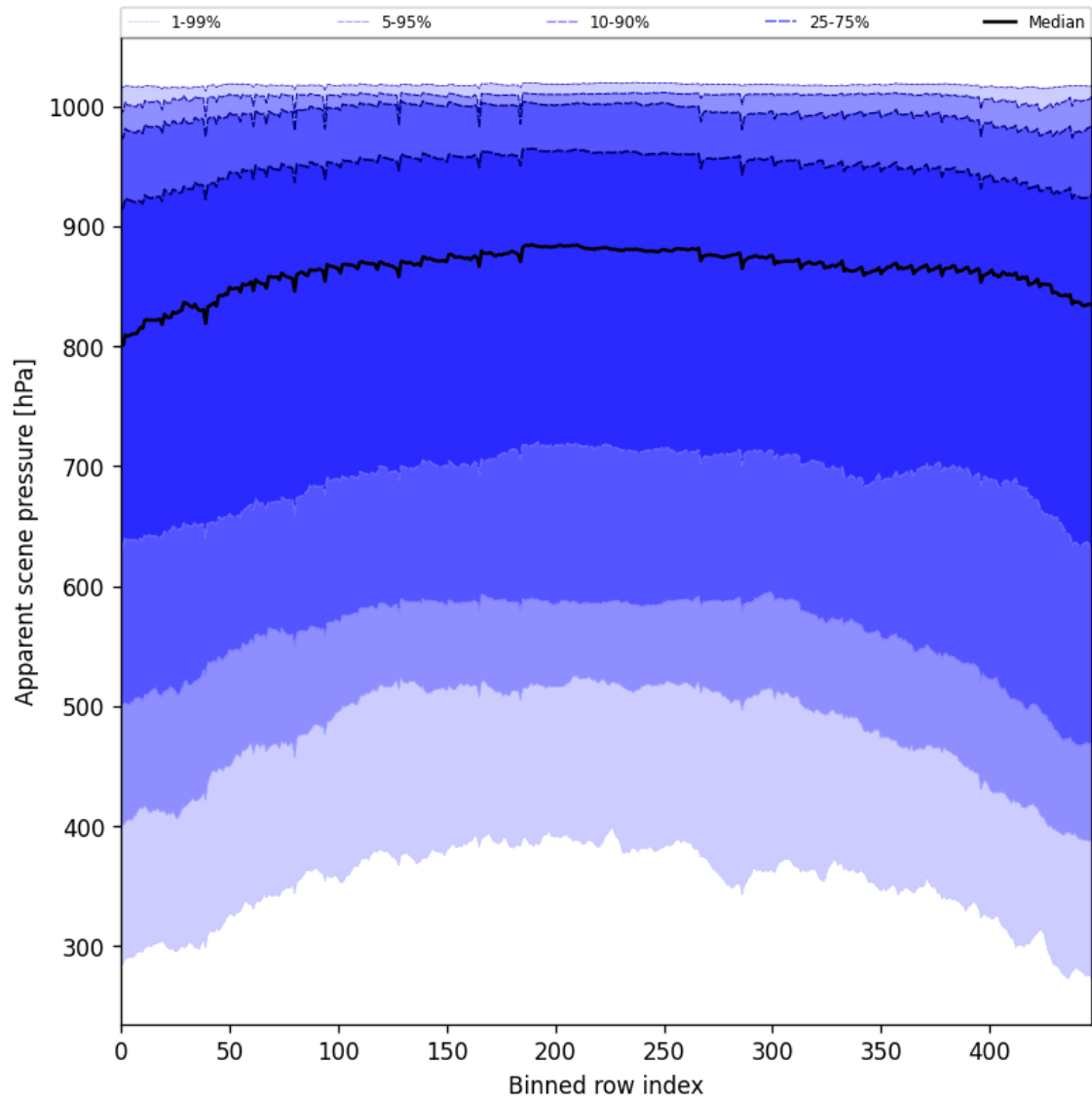
Figure 51: Along track statistics of “Apparent scene pressure” for 2025-02-16 to 2025-02-16
