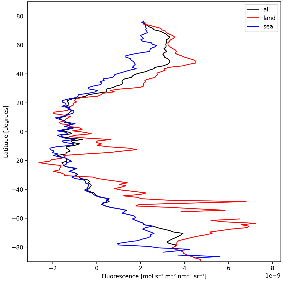
Figure 21: Zonal average of “Fluorescence” for 2025-02-16 to 2025-02-16.
