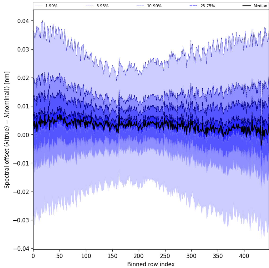
Figure 60: Along track statistics of “Spectral offset ( \lambda_{\text{true}} - \lambda_{\text{nominal}} )” for 2025-02-16 to 2025-02-16
