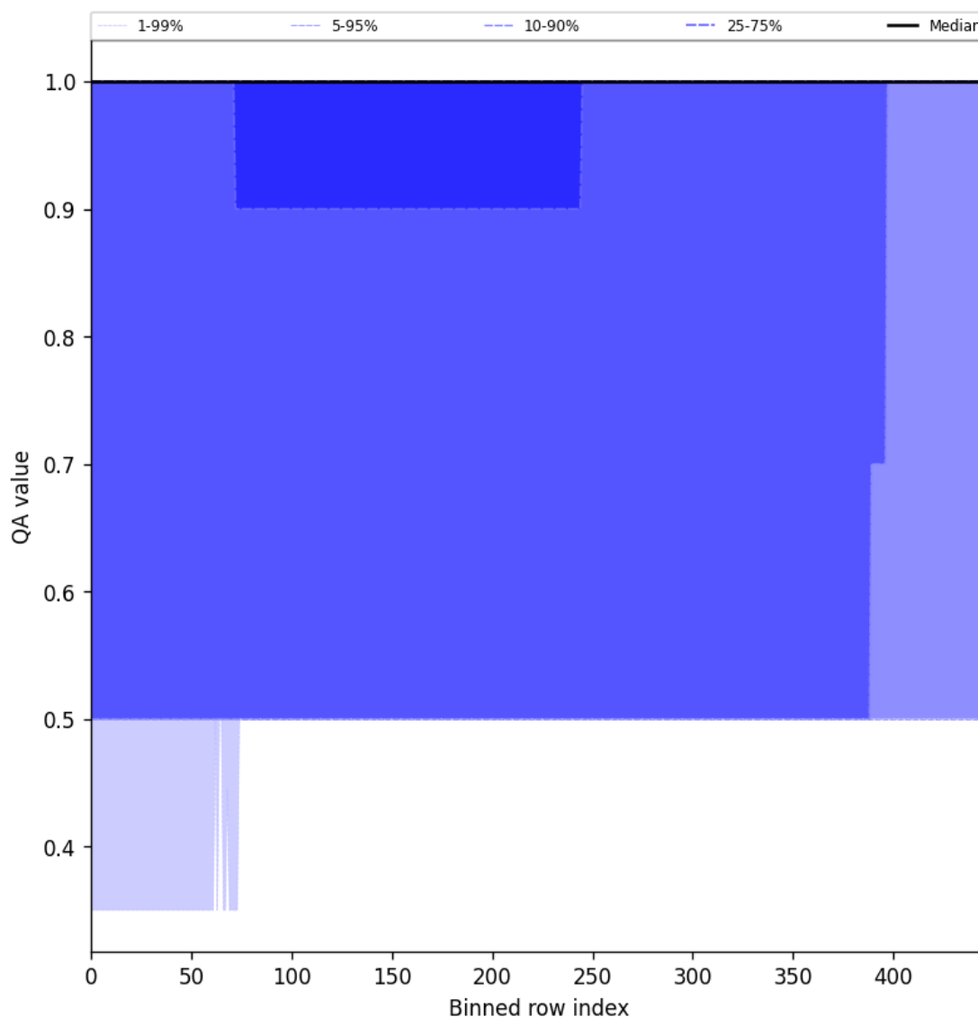
Figure 44: Along track statistics of “QA value” for 2025-02-16 to 2025-02-16
