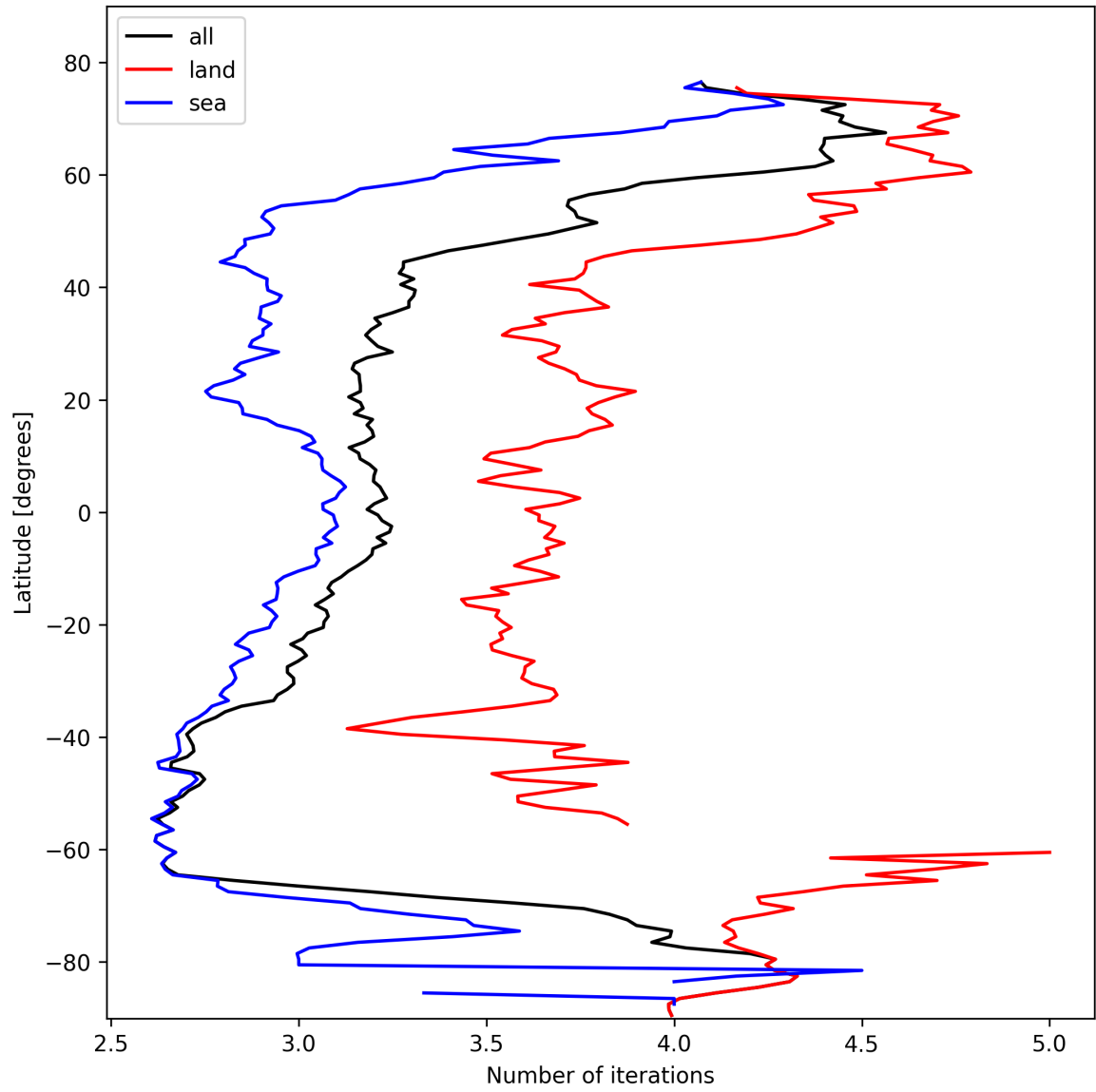
Figure 20: Zonal average of “Number of iterations” for 2025-02-16 to 2025-02-16.
