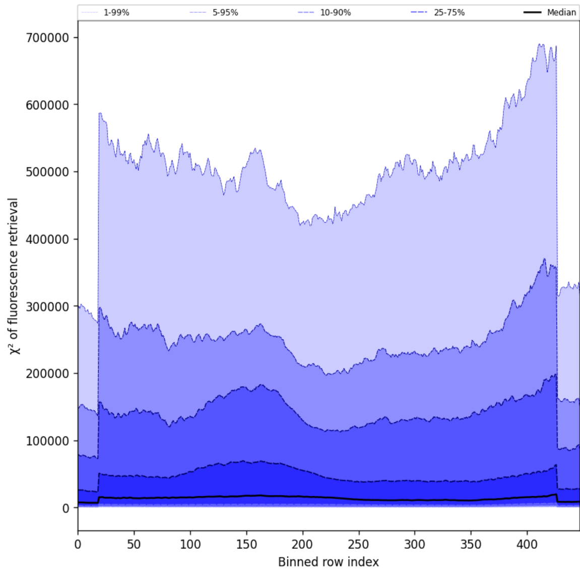
Figure 57: Along track statistics of “ \chi^2 of fluorescence retrieval” for 2025-02-16 to 2025-02-16
