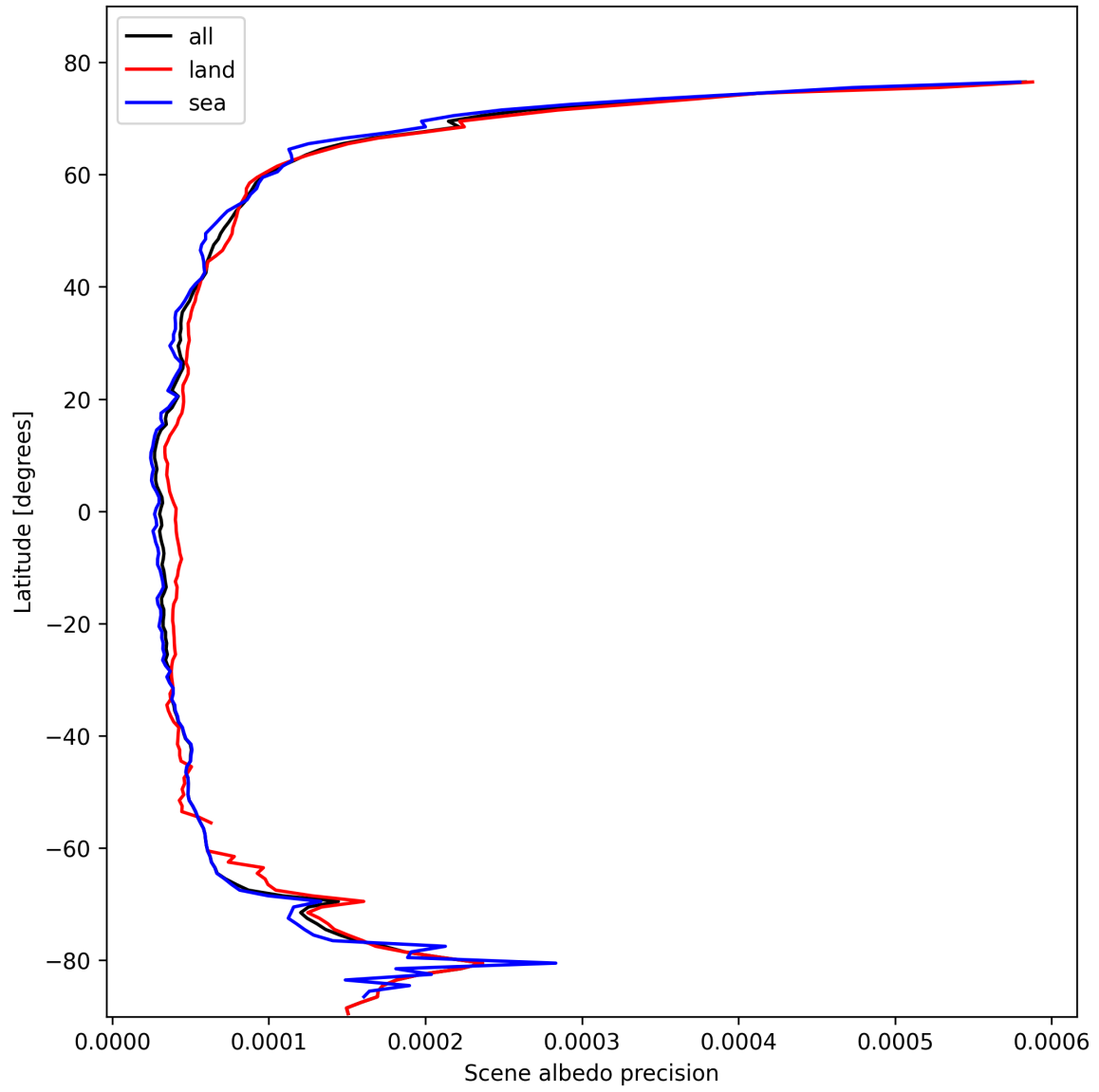
Figure 16: Zonal average of “Scene albedo precision” for 2025-02-18 to 2025-02-19.
