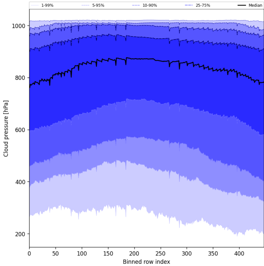
Figure 45: Along track statistics of “Cloud pressure” for 2025-02-18 to 2025-02-19
