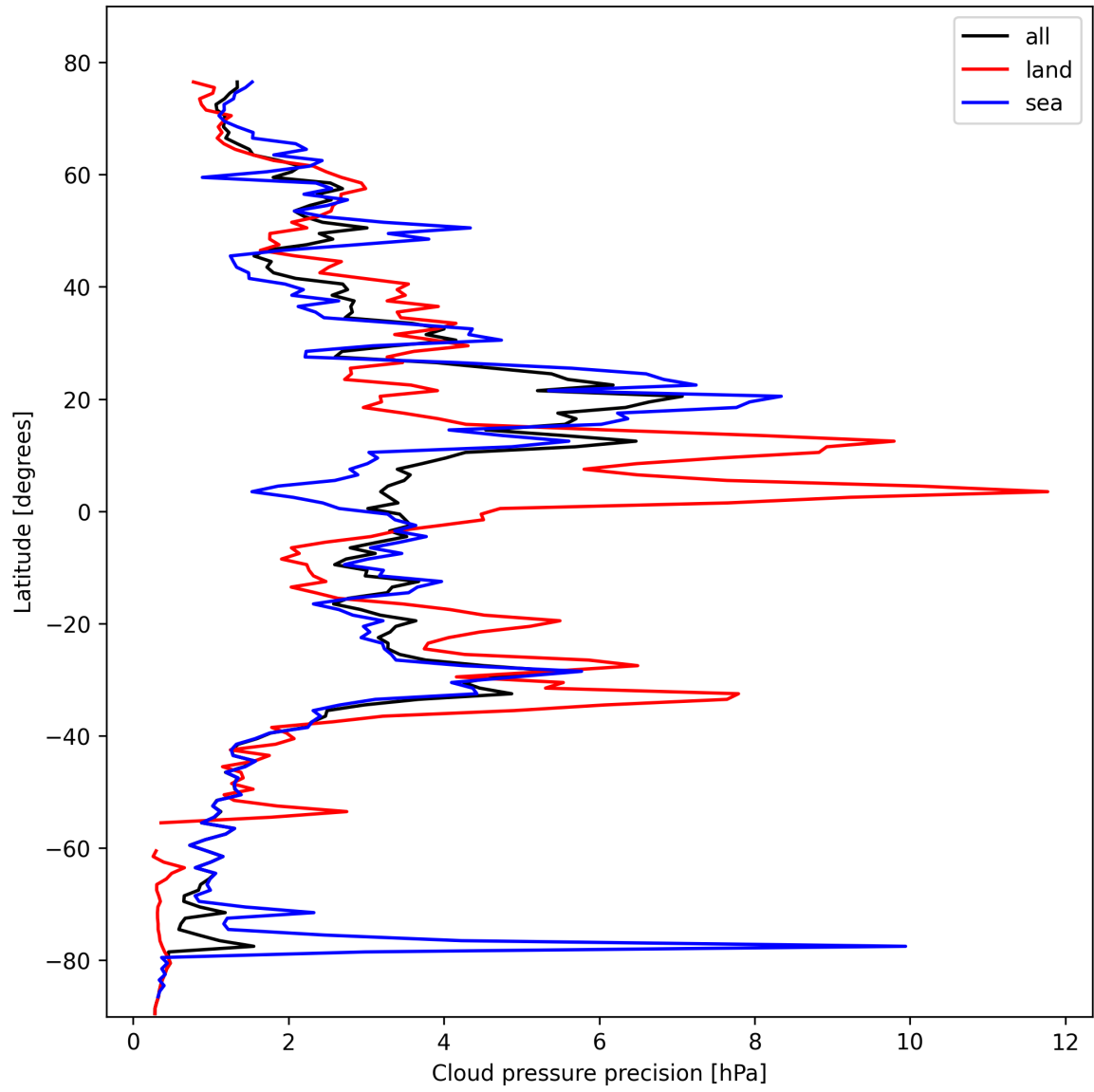
Figure 12: Zonal average of “Cloud pressure precision” for 2025-02-18 to 2025-02-19.
