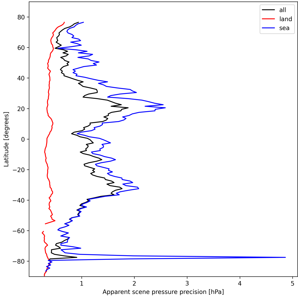
Figure 18: Zonal average of “Apparent scene pressure precision” for 2025-02-18 to 2025-02-19.
