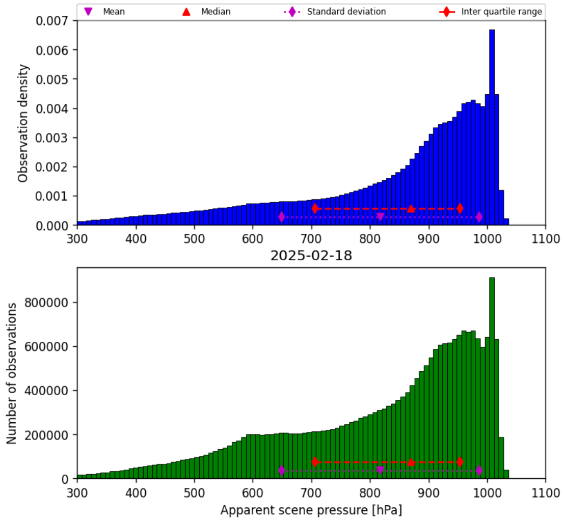
Figure 34: Histogram of “Apparent scene pressure” for 2025-02-18 to 2025-02-19
