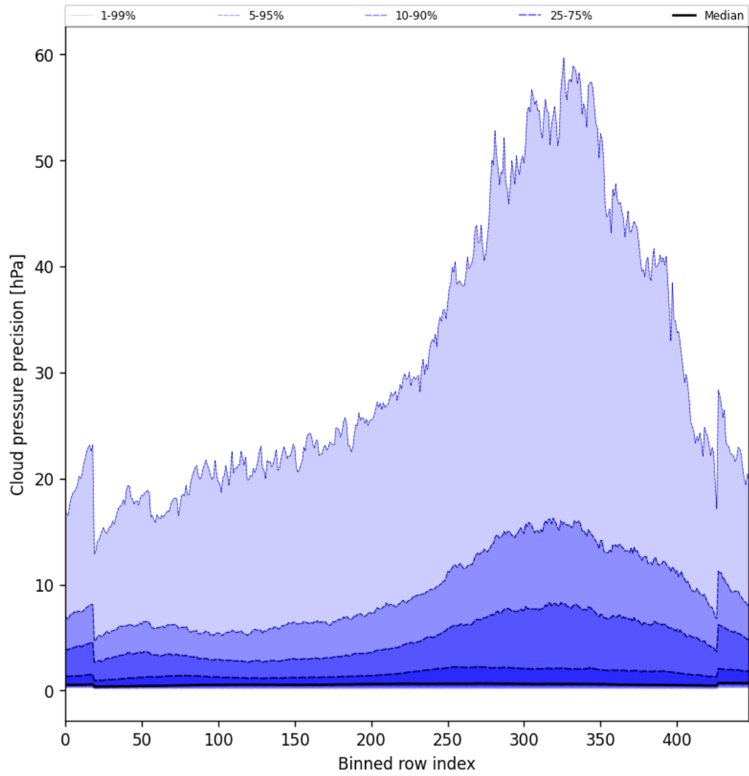
Figure 46: Along track statistics of “Cloud pressure precision” for 2025-02-18 to 2025-02-19
