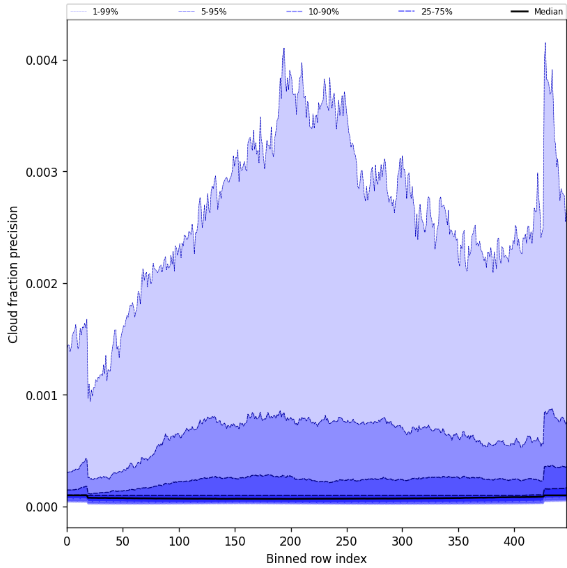
Figure 48: Along track statistics of “Cloud fraction precision” for 2025-02-18 to 2025-02-19
