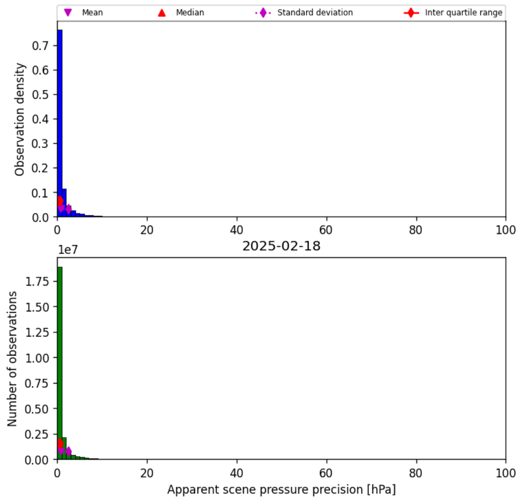
Figure 35: Histogram of “Apparent scene pressure precision” for 2025-02-18 to 2025-02-19
