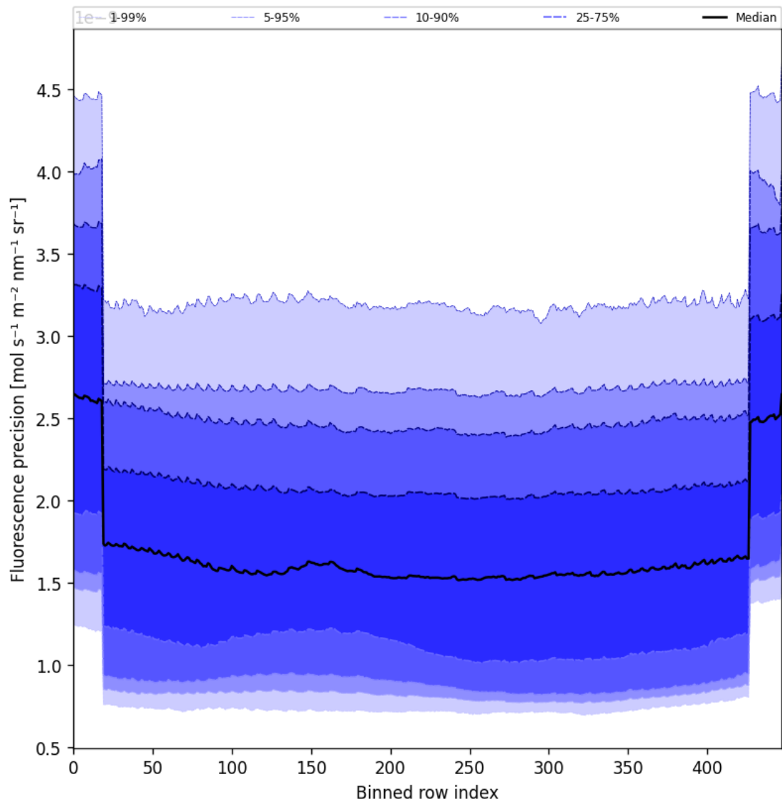
Figure 56: Along track statistics of “Fluorescence precision” for 2025-02-18 to 2025-02-19
