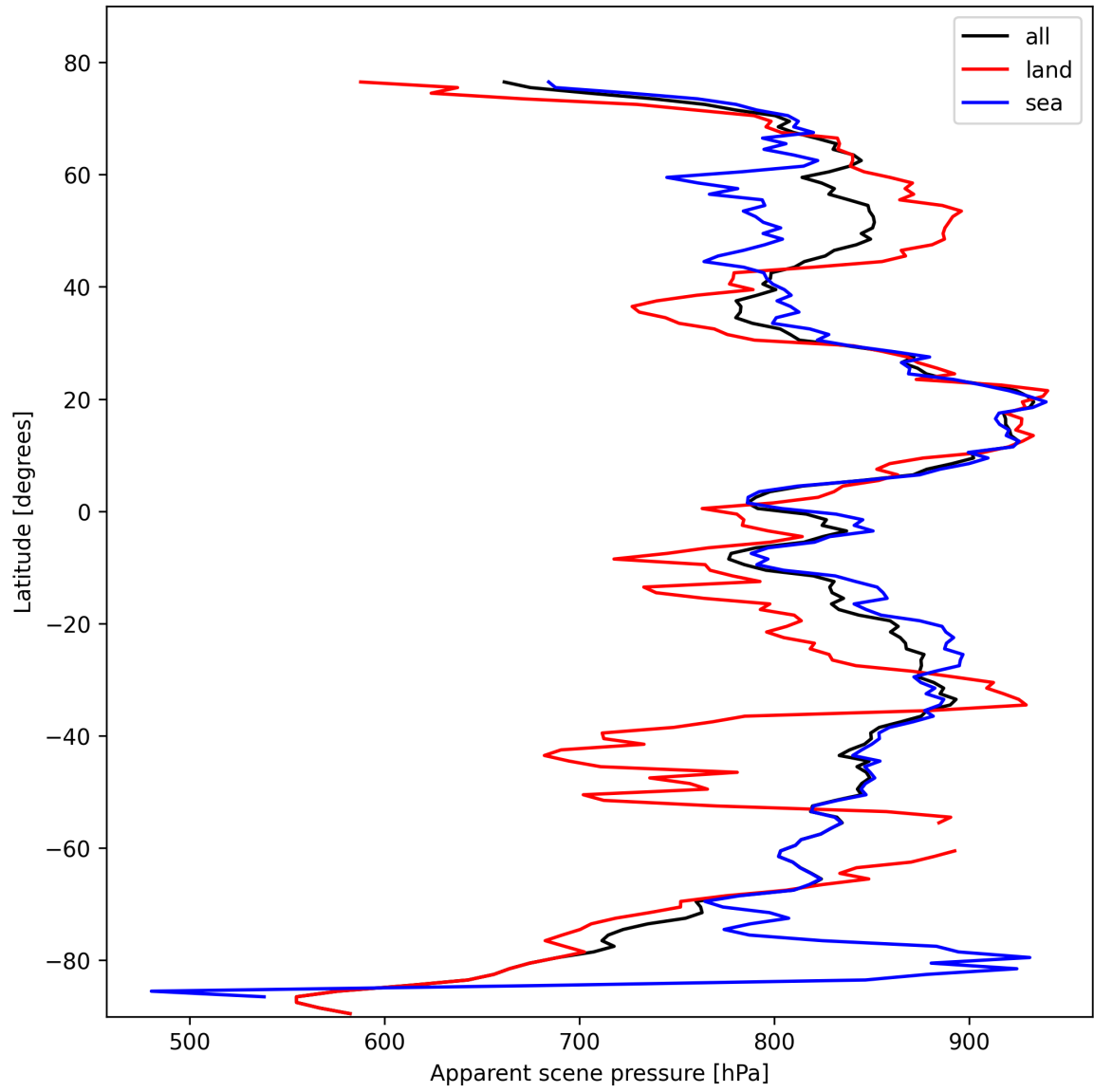
Figure 17: Zonal average of “Apparent scene pressure” for 2025-02-18 to 2025-02-19.
