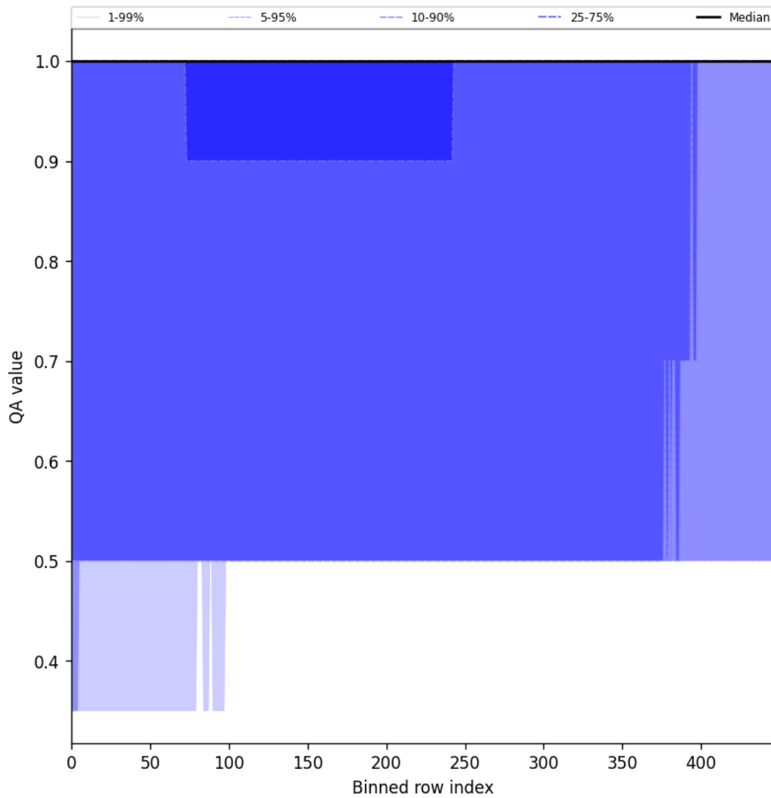
Figure 44: Along track statistics of “QA value” for 2025-02-18 to 2025-02-19
