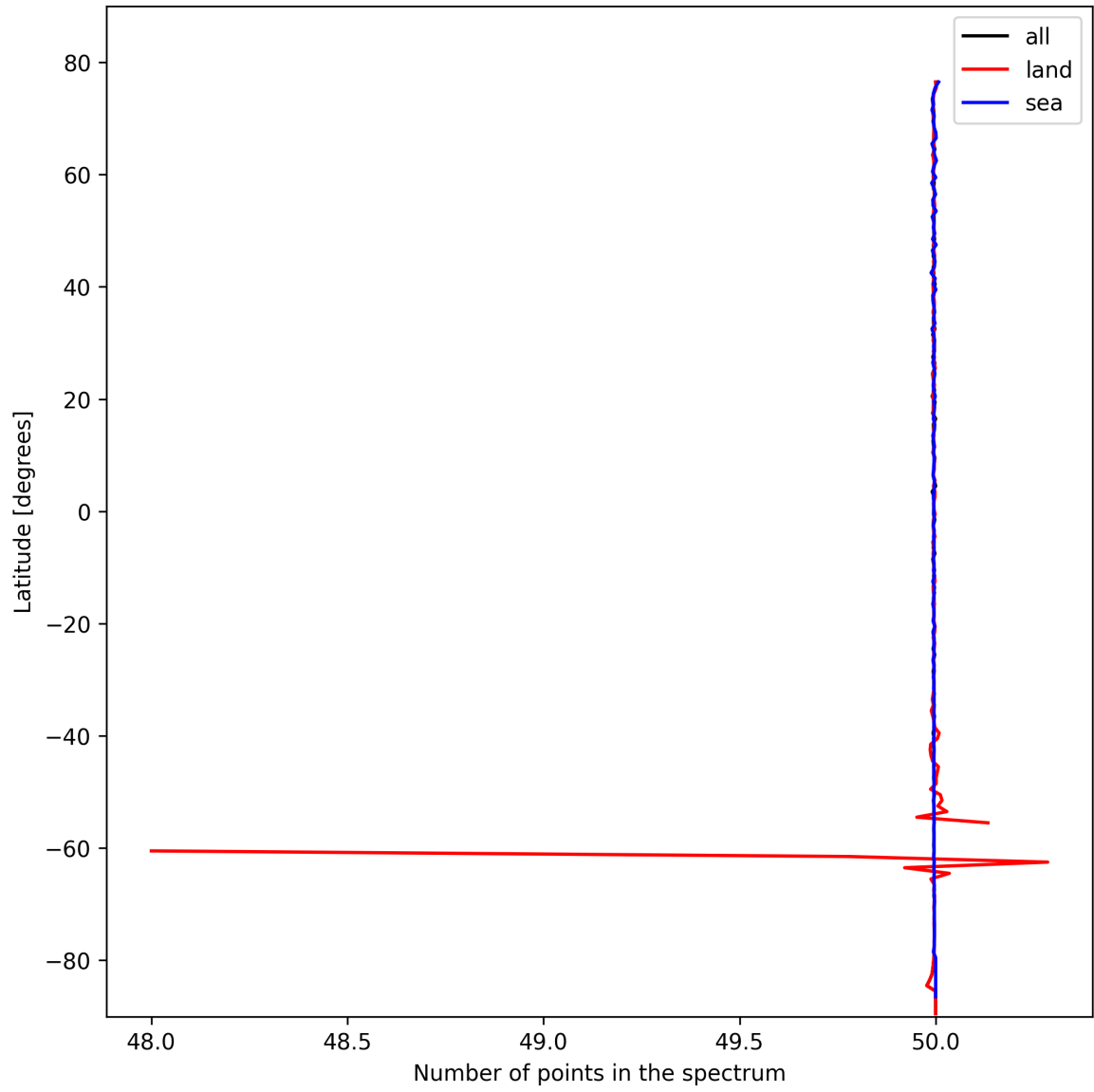
Figure 25: Zonal average of “Number of points in the spectrum” for 2025-02-18 to 2025-02-19.
