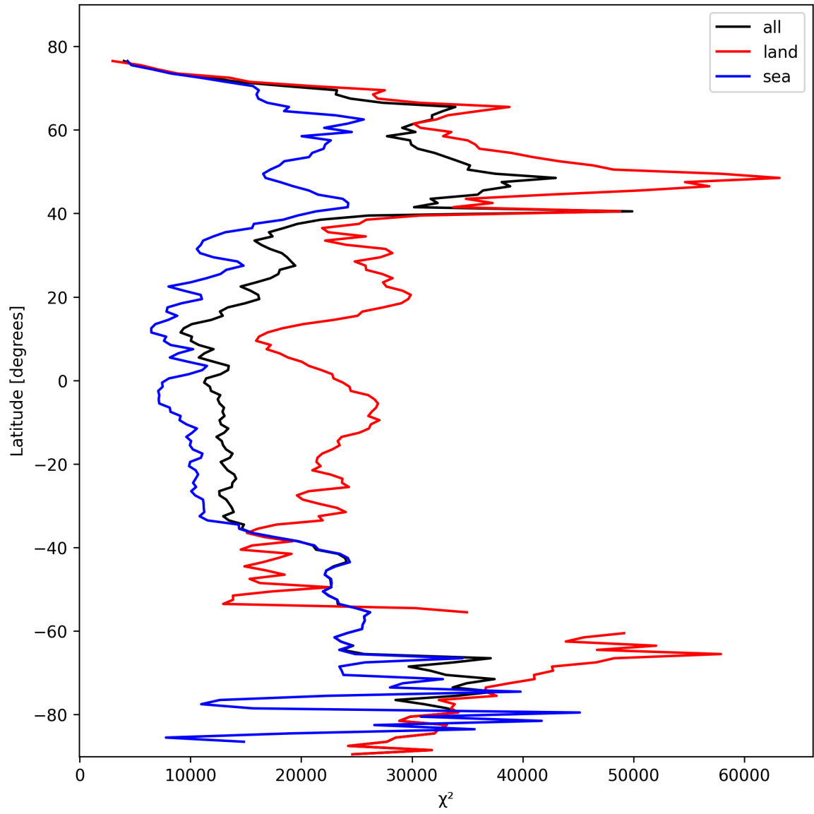
Figure 19: Zonal average of “ \chi^2 ” for 2025-02-18 to 2025-02-19.
