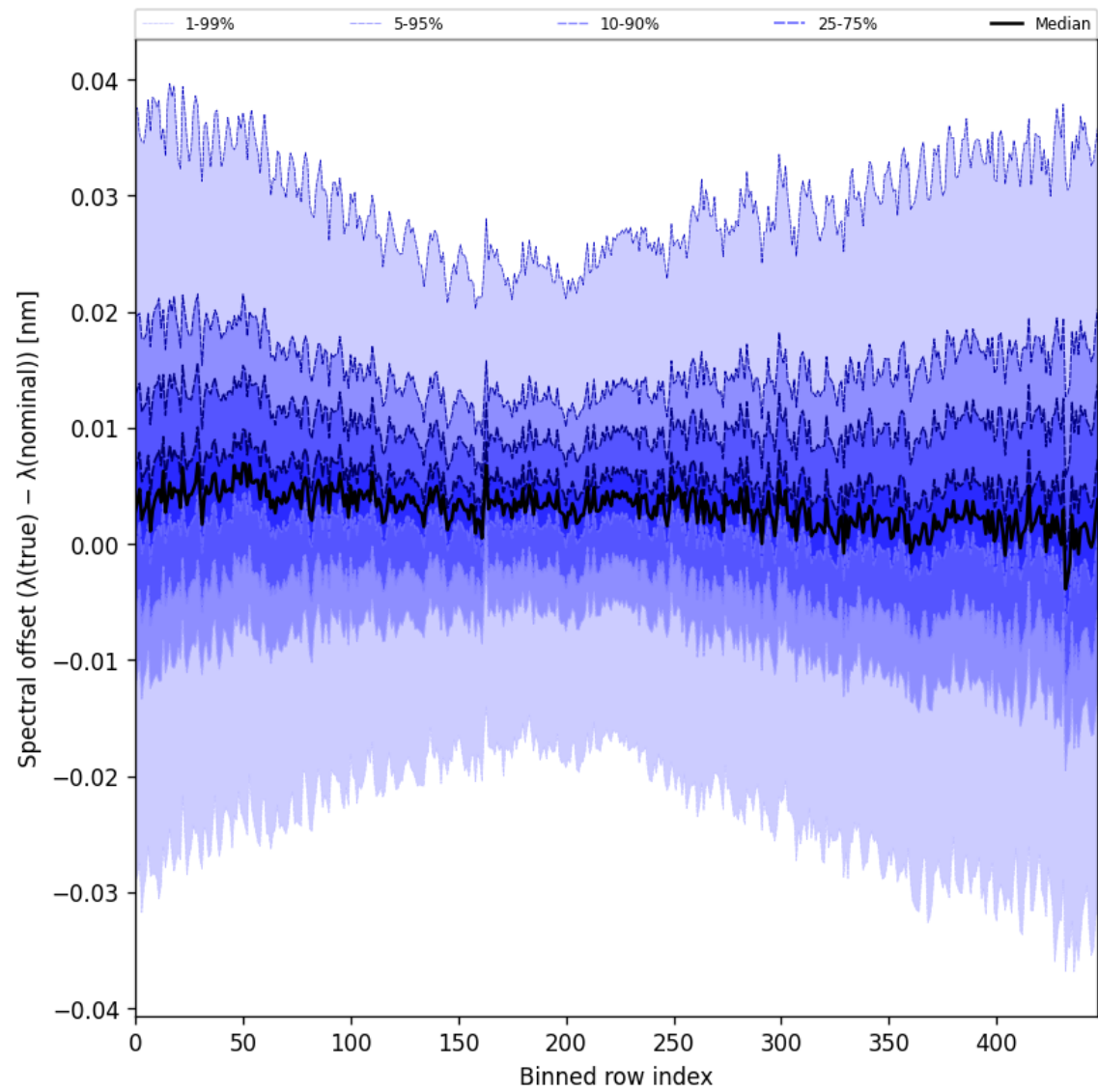
Figure 60: Along track statistics of “Spectral offset (\lambda_{\text{true}} - \lambda_{\text{nominal}}) ” for 2025-02-18 to 2025-02-19
