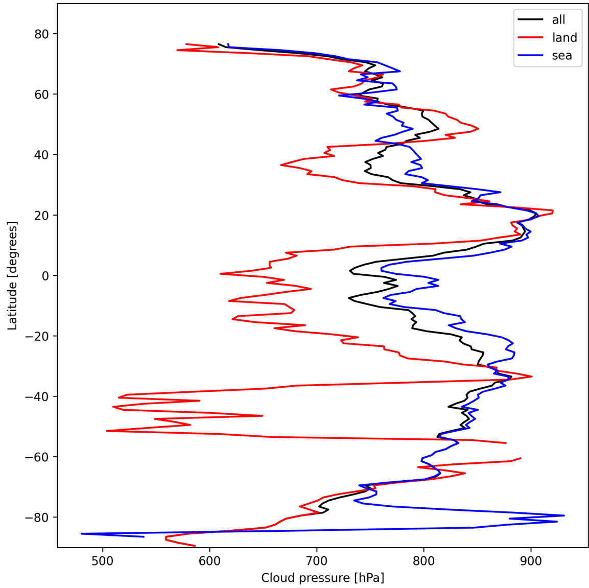
Figure 11: Zonal average of “Cloud pressure” for 2025-02-18 to 2025-02-19.
