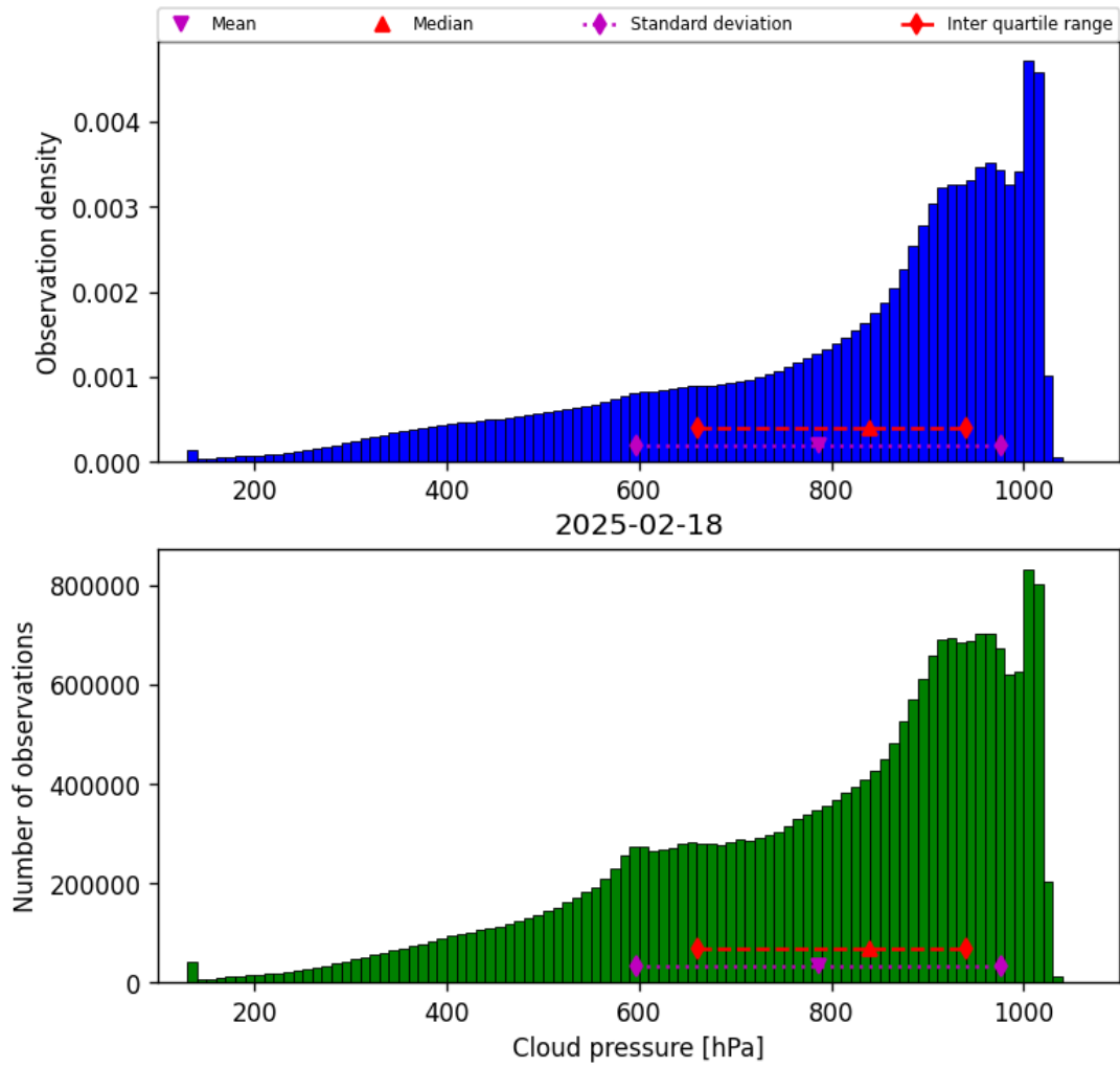
Figure 28: Histogram of “Cloud pressure” for 2025-02-18 to 2025-02-19
