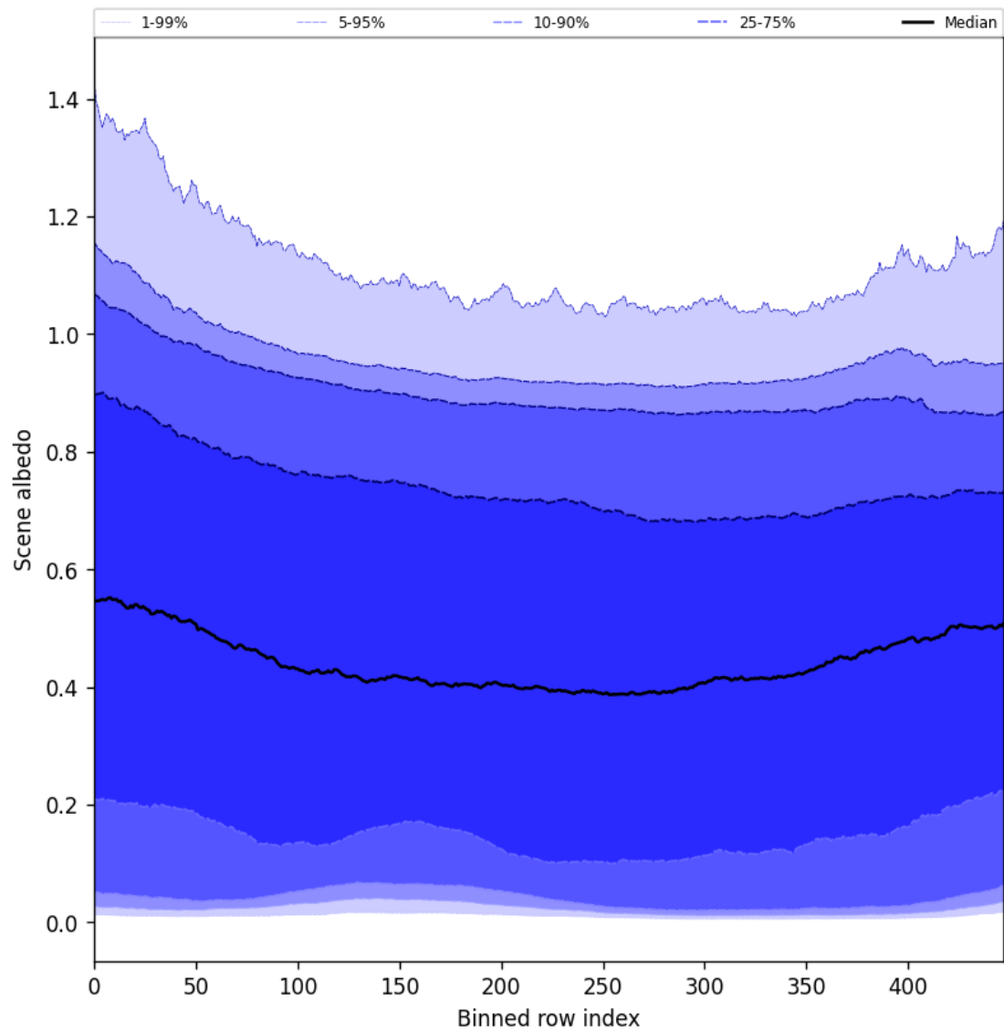
Figure 49: Along track statistics of “Scene albedo” for 2025-02-18 to 2025-02-19
