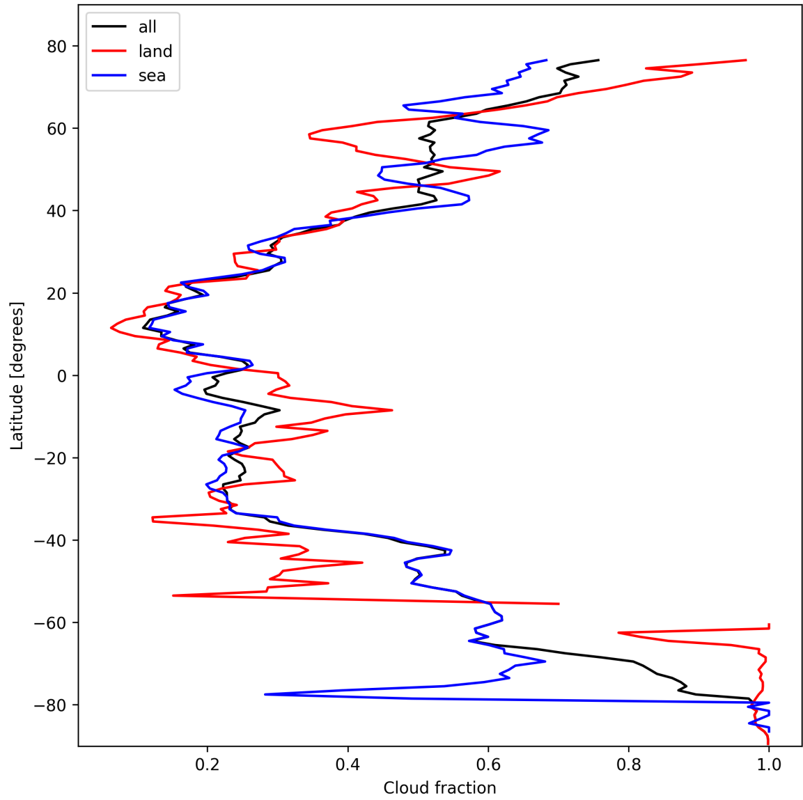
Figure 13: Zonal average of “Cloud fraction” for 2025-02-18 to 2025-02-19.
