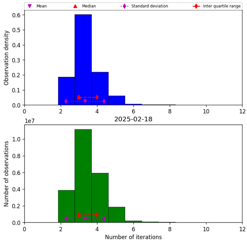
Figure 37: Histogram of “Number of iterations” for 2025-02-18 to 2025-02-19
