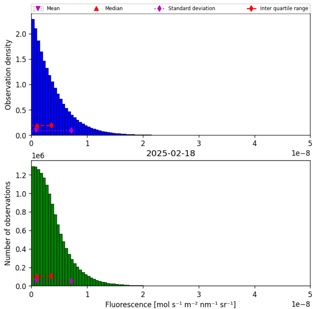
Figure 38: Histogram of “Fluorescence” for 2025-02-18 to 2025-02-19
