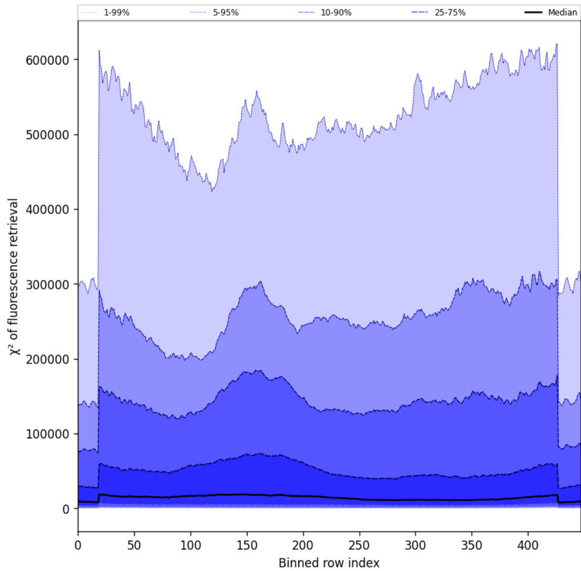
Figure 57: Along track statistics of “ \chi^2 of fluorescence retrieval” for 2025-02-18 to 2025-02-19
