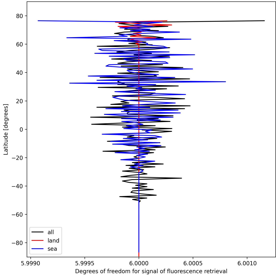
Figure 24: Zonal average of “Degrees of freedom for signal of fluorescence retrieval” for 2025-02-18 to 2025-02-19.
