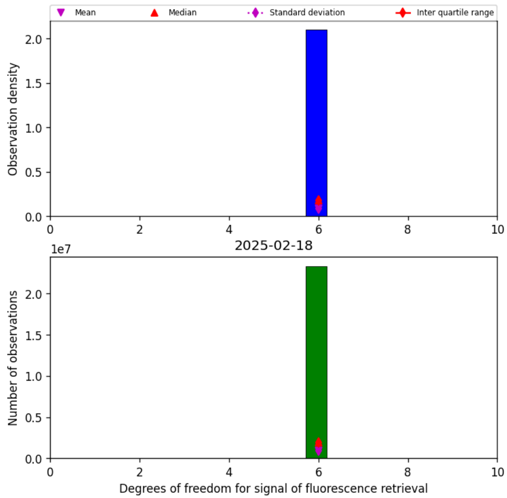
Figure 41: Histogram of “Degrees of freedom for signal of fluorescence retrieval” for 2025-02-18 to 2025-02-19
