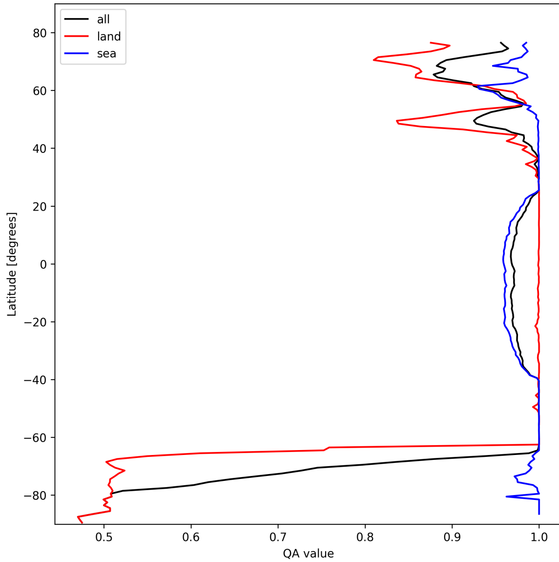
Figure 10: Zonal average of “QA value” for 2025-02-18 to 2025-02-19.
