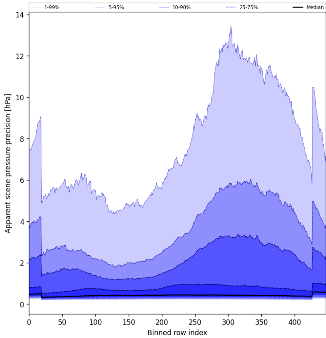
Figure 52: Along track statistics of “Apparent scene pressure precision” for 2025-02-18 to 2025-02-19
