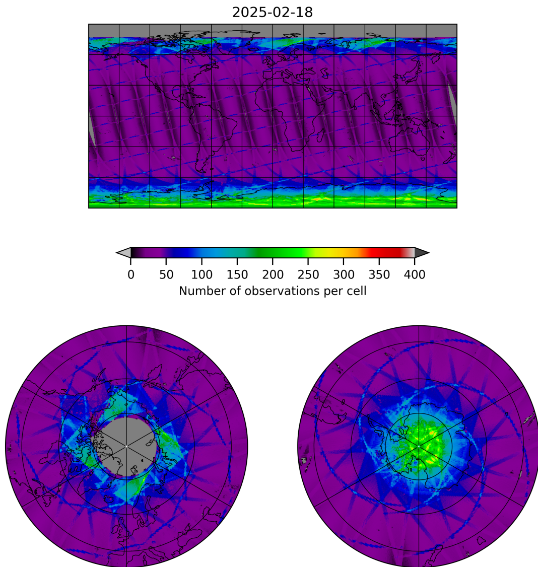
Figure 9: Map of the number of observations for 2025-02-18 to 2025-02-19
