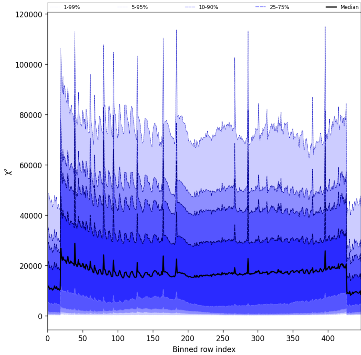
Figure 53: Along track statistics of “ \chi^2 ” for 2025-02-18 to 2025-02-19
