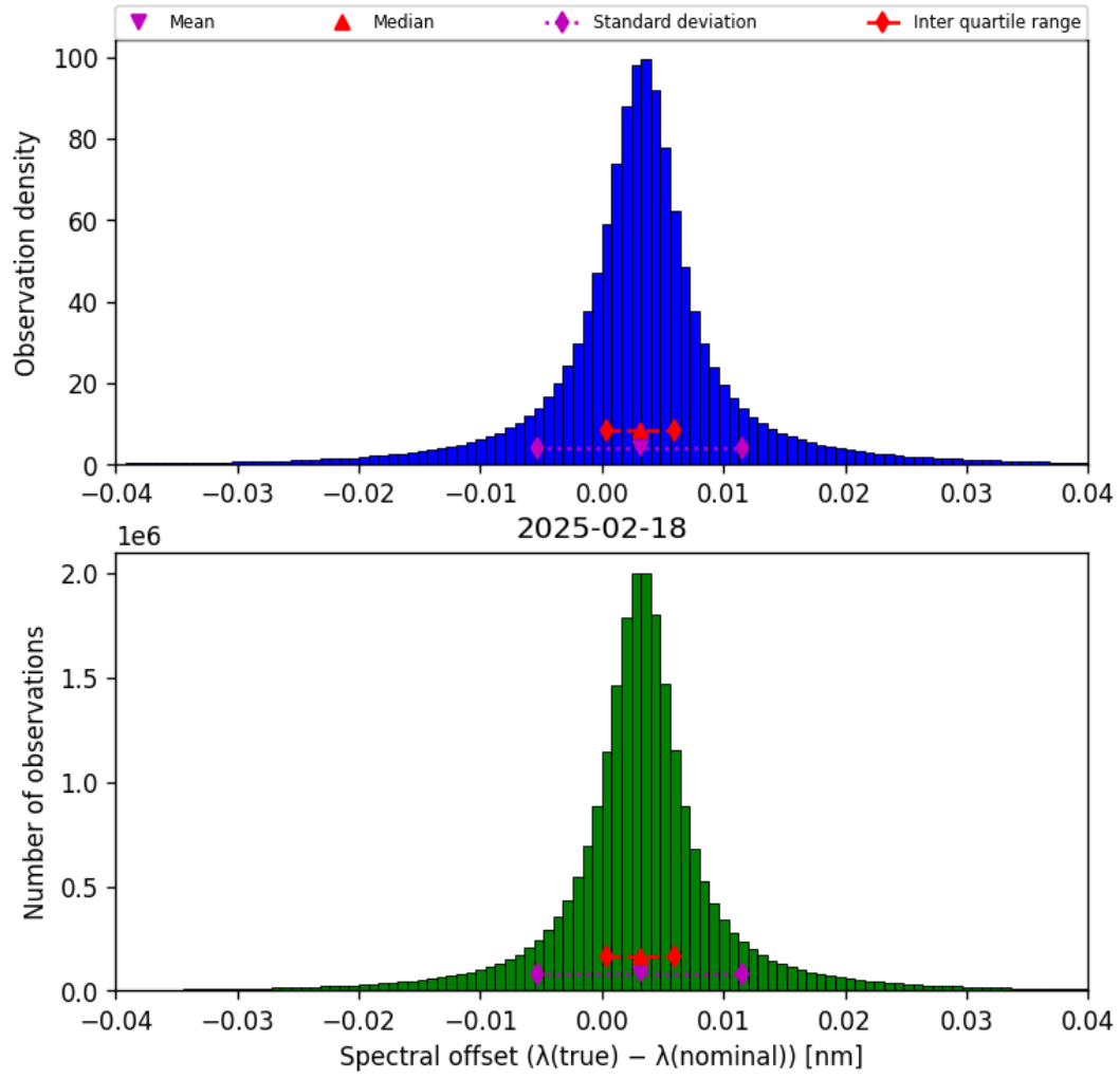
Figure 43: Histogram of “Spectral offset ( \lambda_{\text{true}} - \lambda_{\text{nominal}} )” for 2025-02-18 to 2025-02-19
