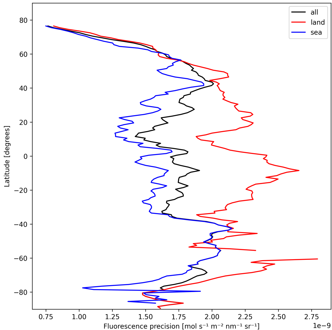
Figure 22: Zonal average of “Fluorescence precision” for 2025-02-18 to 2025-02-19.
