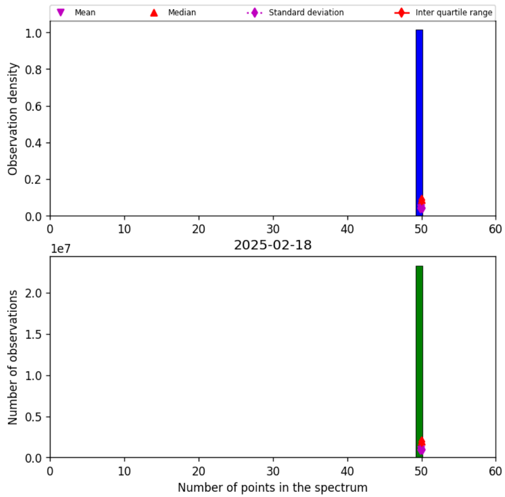
Figure 42: Histogram of “Number of points in the spectrum” for 2025-02-18 to 2025-02-19
