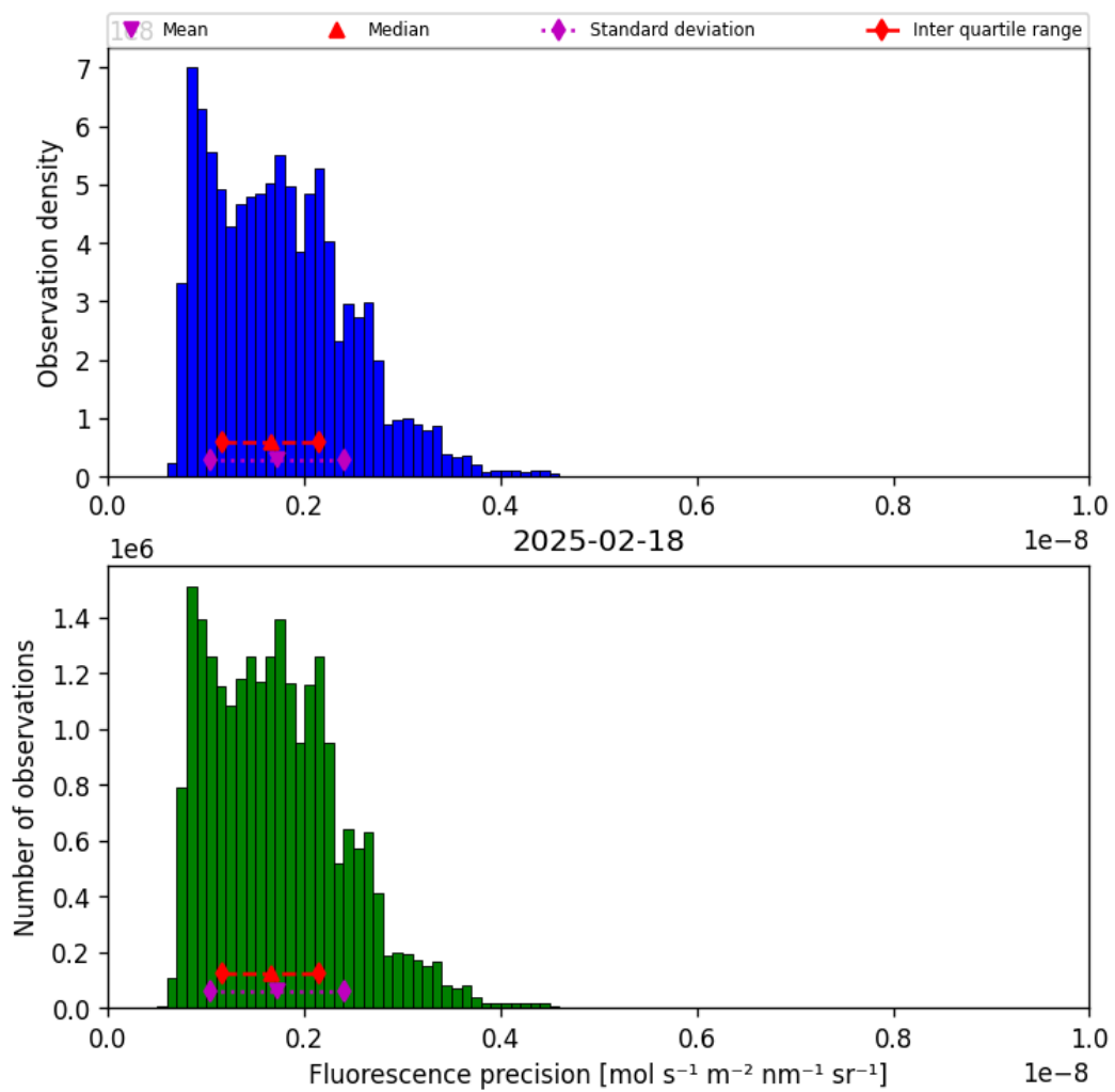
Figure 39: Histogram of “Fluorescence precision” for 2025-02-18 to 2025-02-19
