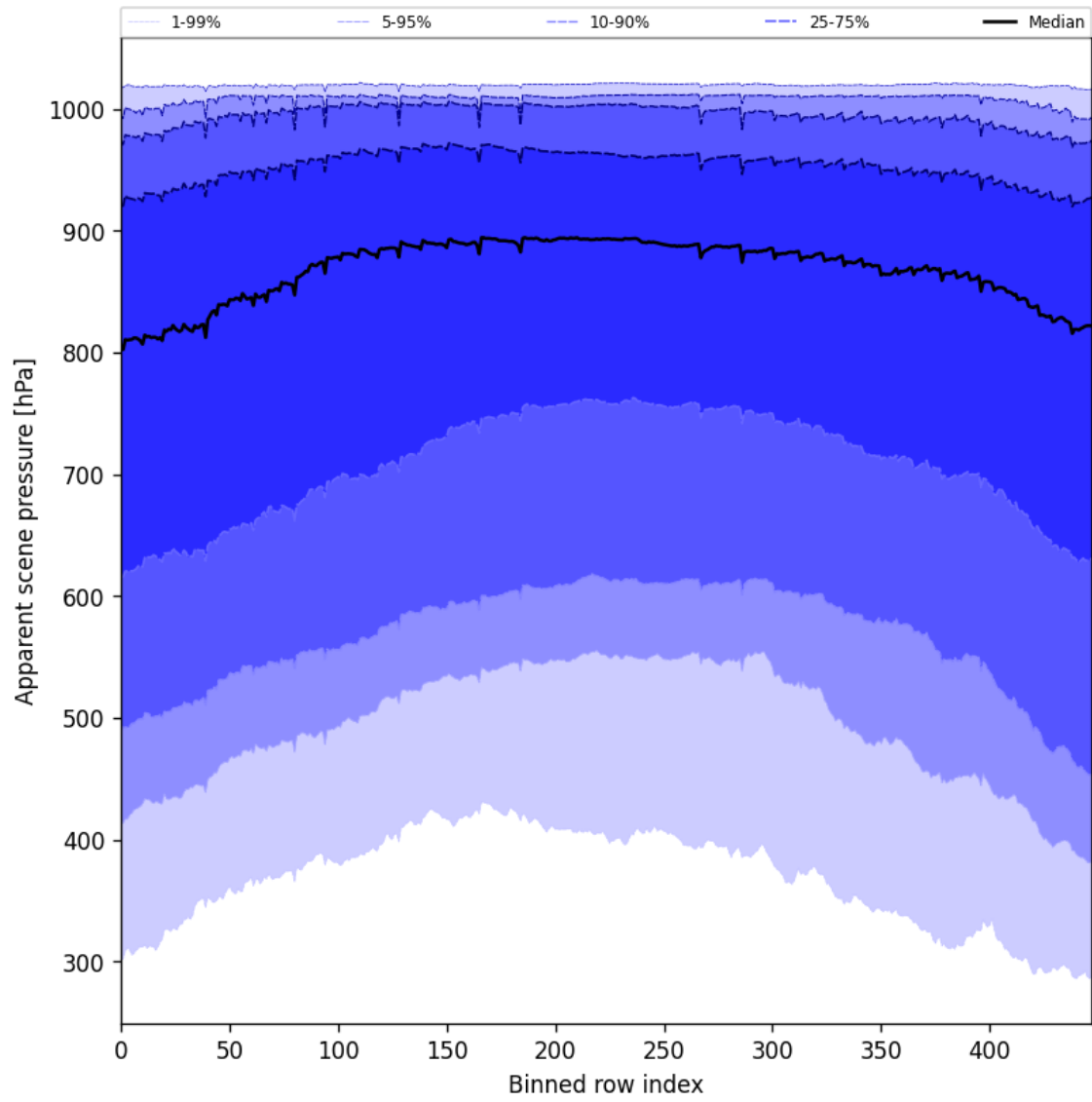
Figure 51: Along track statistics of “Apparent scene pressure” for 2025-02-18 to 2025-02-19
