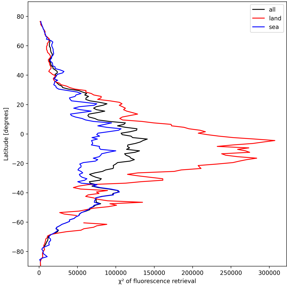
Figure 23: Zonal average of “ \chi^2 of fluorescence retrieval” for 2025-02-18 to 2025-02-19.
