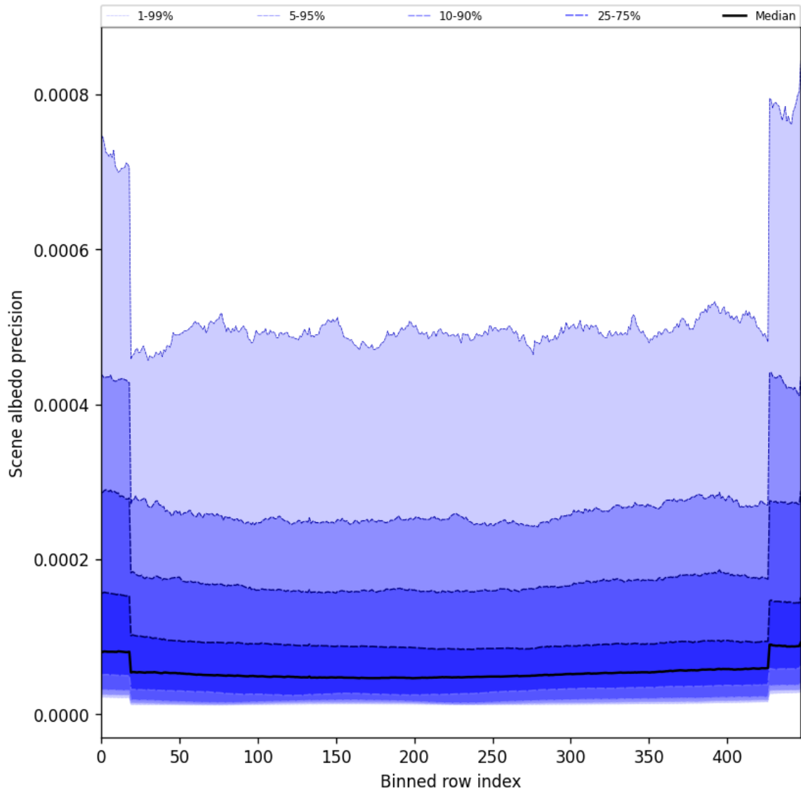
Figure 50: Along track statistics of “Scene albedo precision” for 2025-02-18 to 2025-02-19
