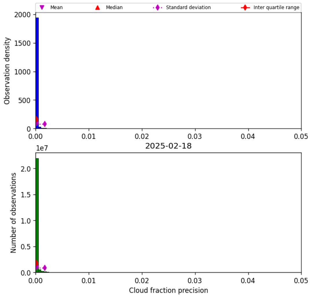
Figure 31: Histogram of “Cloud fraction precision” for 2025-02-18 to 2025-02-19
