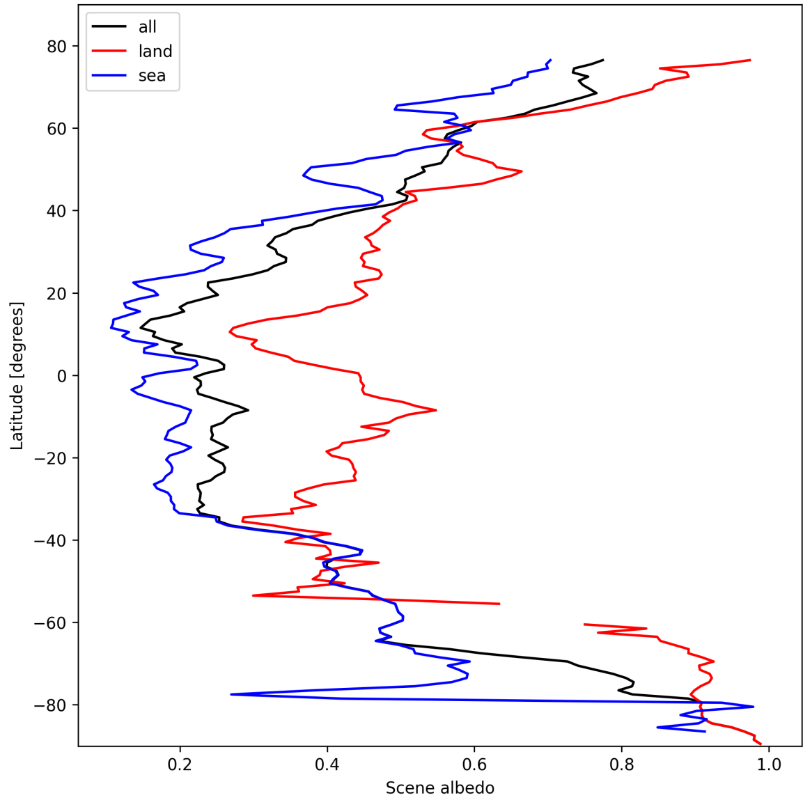
Figure 15: Zonal average of “Scene albedo” for 2025-02-18 to 2025-02-19.
