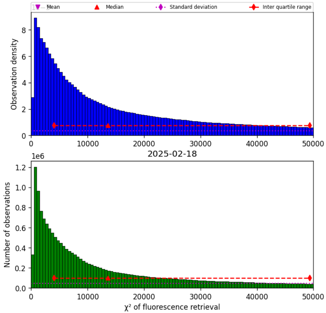
Figure 40: Histogram of “ \chi^2 of fluorescence retrieval” for 2025-02-18 to 2025-02-19
