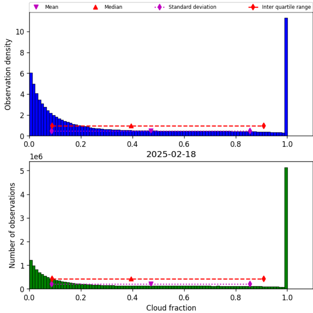
Figure 30: Histogram of “Cloud fraction” for 2025-02-18 to 2025-02-19
