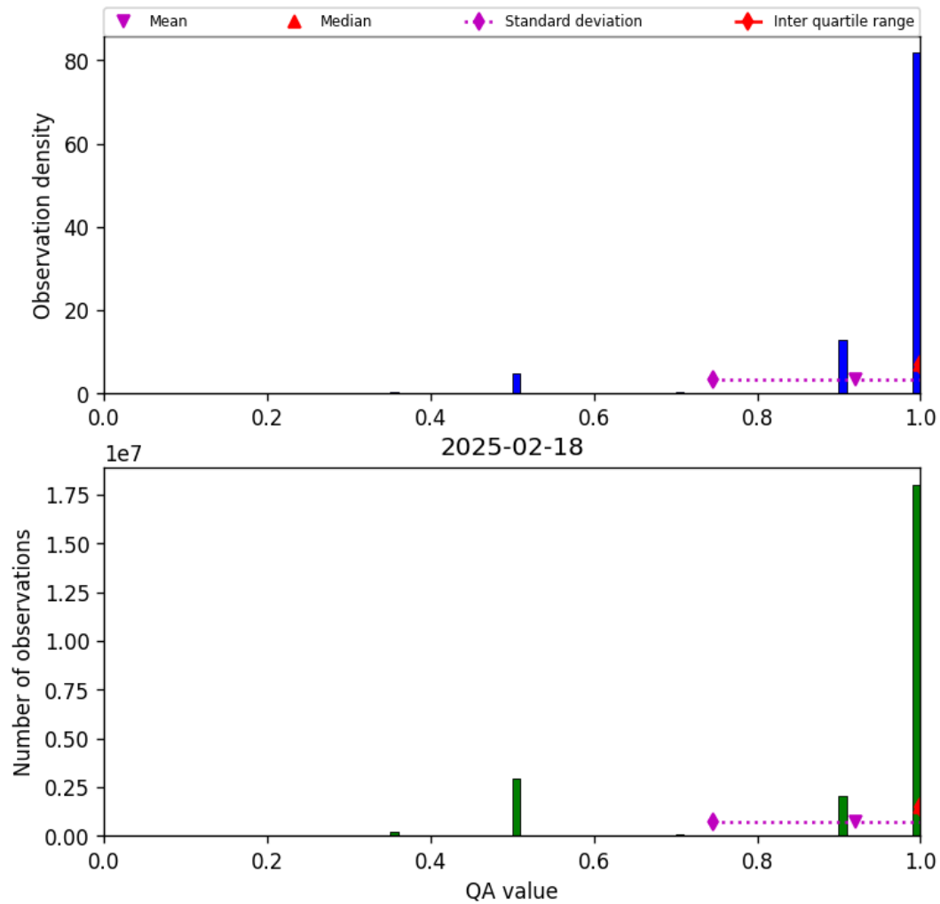
Figure 27: Histogram of “QA value” for 2025-02-18 to 2025-02-19
