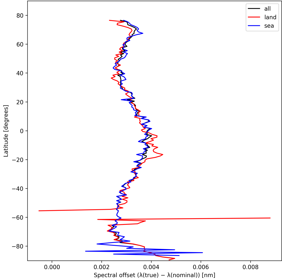
Figure 26: Zonal average of “Spectral offset ( \lambda_{\text{true}} - \lambda_{\text{nominal}} )” for 2025-02-18 to 2025-02-19.
