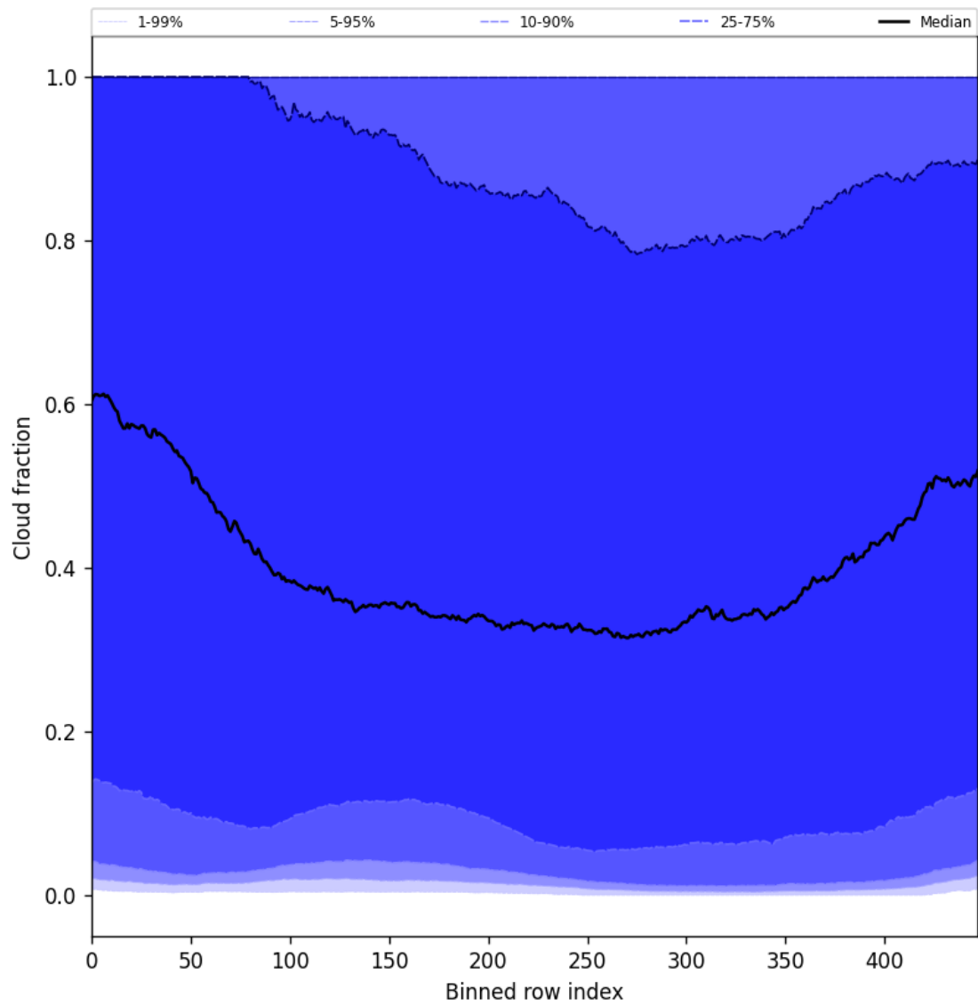
Figure 47: Along track statistics of “Cloud fraction” for 2025-02-18 to 2025-02-19
