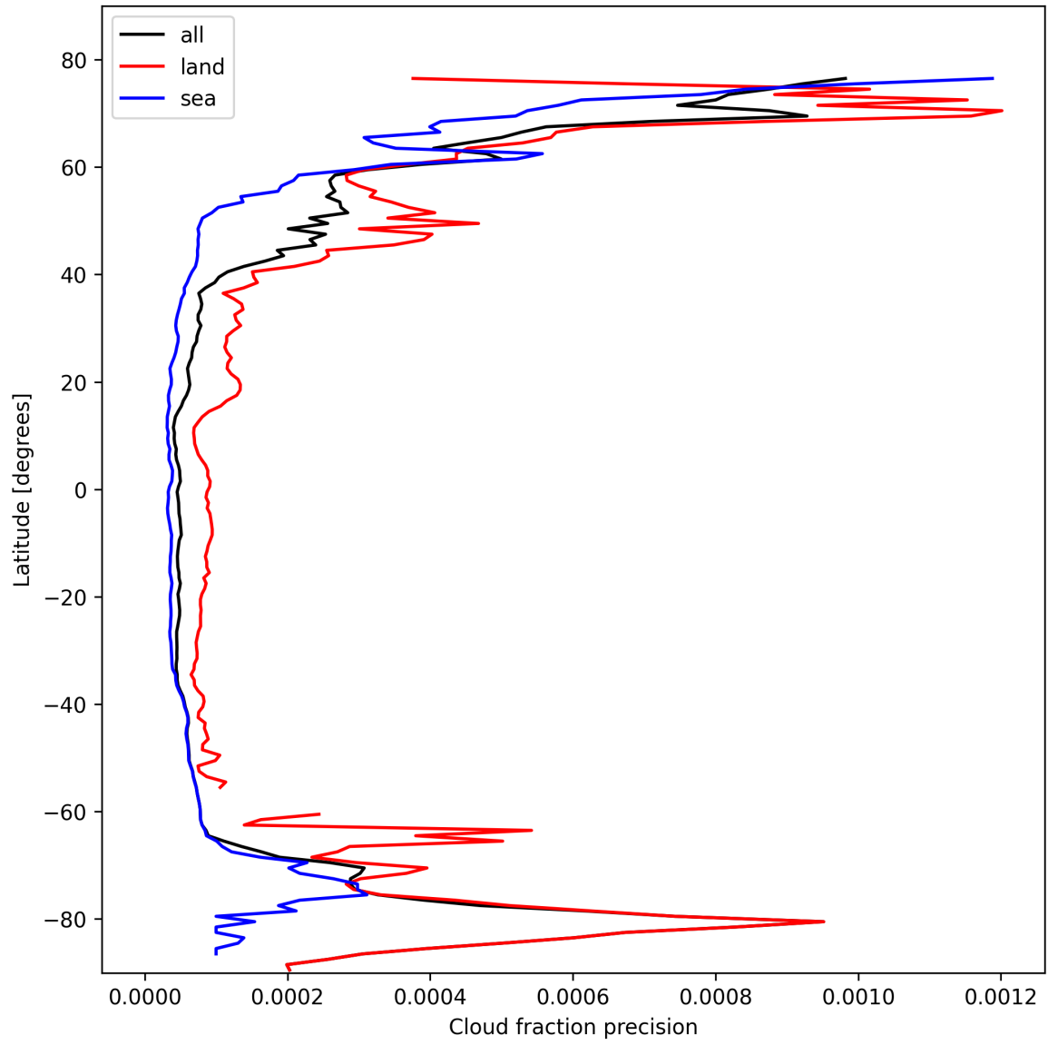
Figure 14: Zonal average of “Cloud fraction precision” for 2025-02-18 to 2025-02-19.
