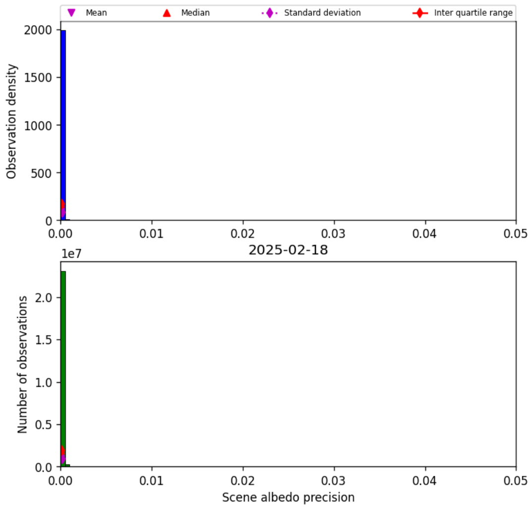
Figure 33: Histogram of “Scene albedo precision” for 2025-02-18 to 2025-02-19
