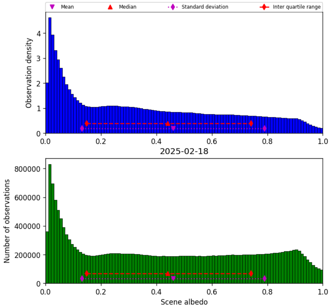
Figure 32: Histogram of “Scene albedo” for 2025-02-18 to 2025-02-19
