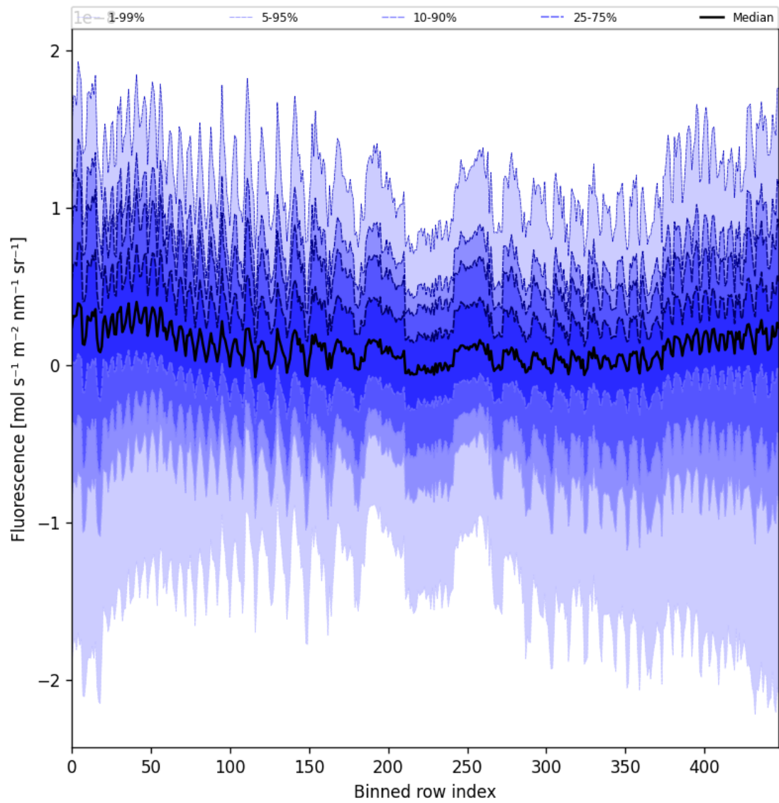
Figure 55: Along track statistics of “Fluorescence” for 2025-02-18 to 2025-02-19
