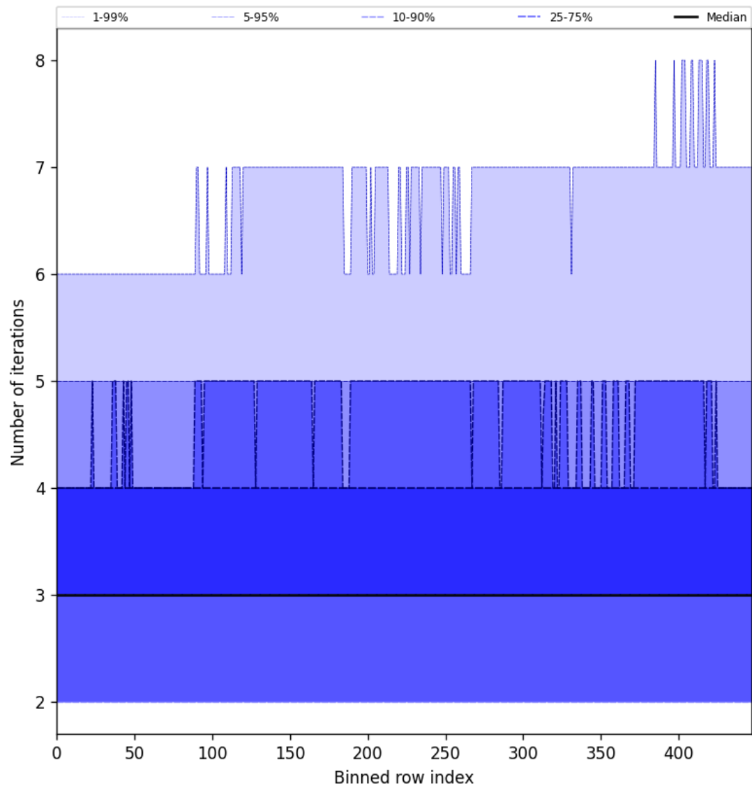
Figure 54: Along track statistics of “Number of iterations” for 2025-02-18 to 2025-02-19
