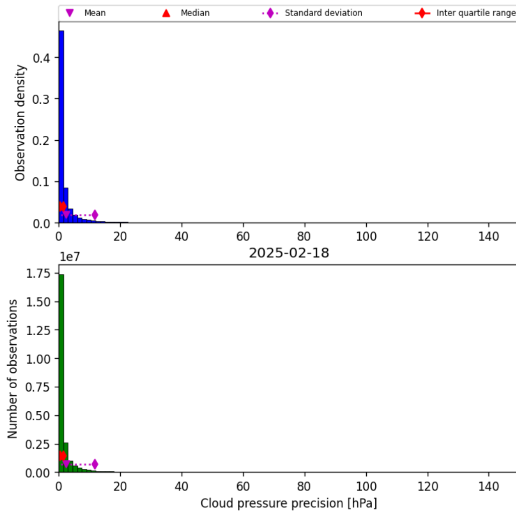
Figure 29: Histogram of “Cloud pressure precision” for 2025-02-18 to 2025-02-19
