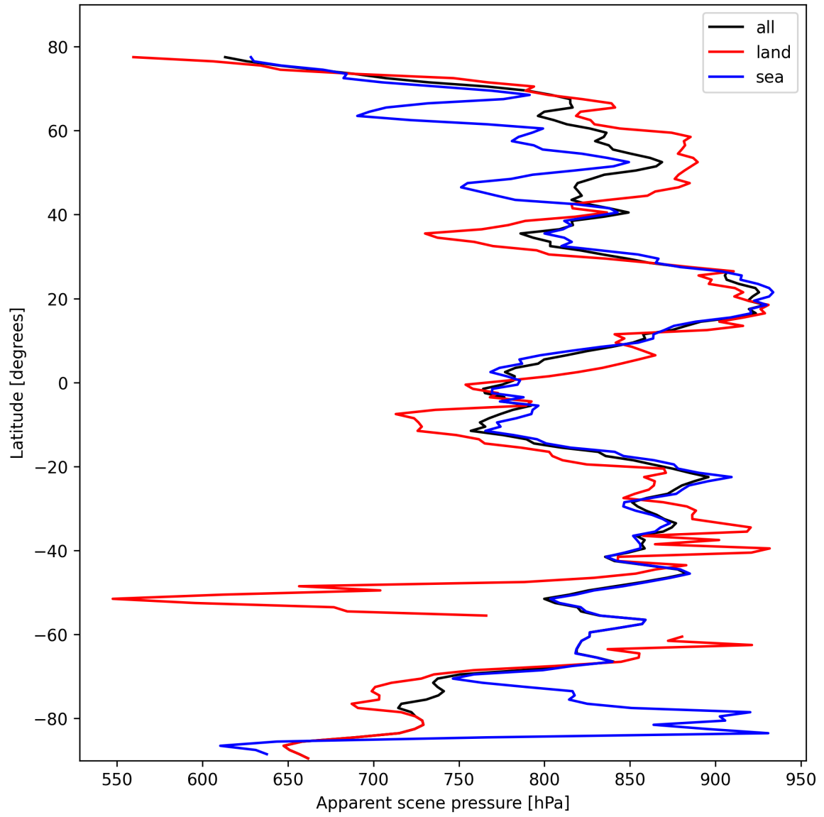
Figure 17: Zonal average of “Apparent scene pressure” for 2025-02-21 to 2025-02-22.
