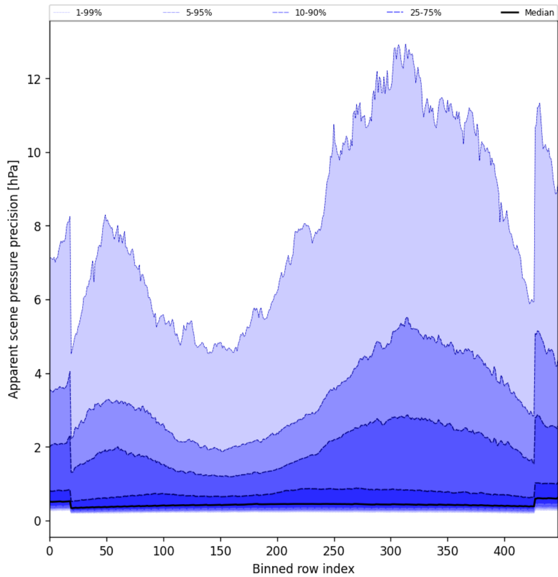
Figure 52: Along track statistics of “Apparent scene pressure precision” for 2025-02-21 to 2025-02-22
