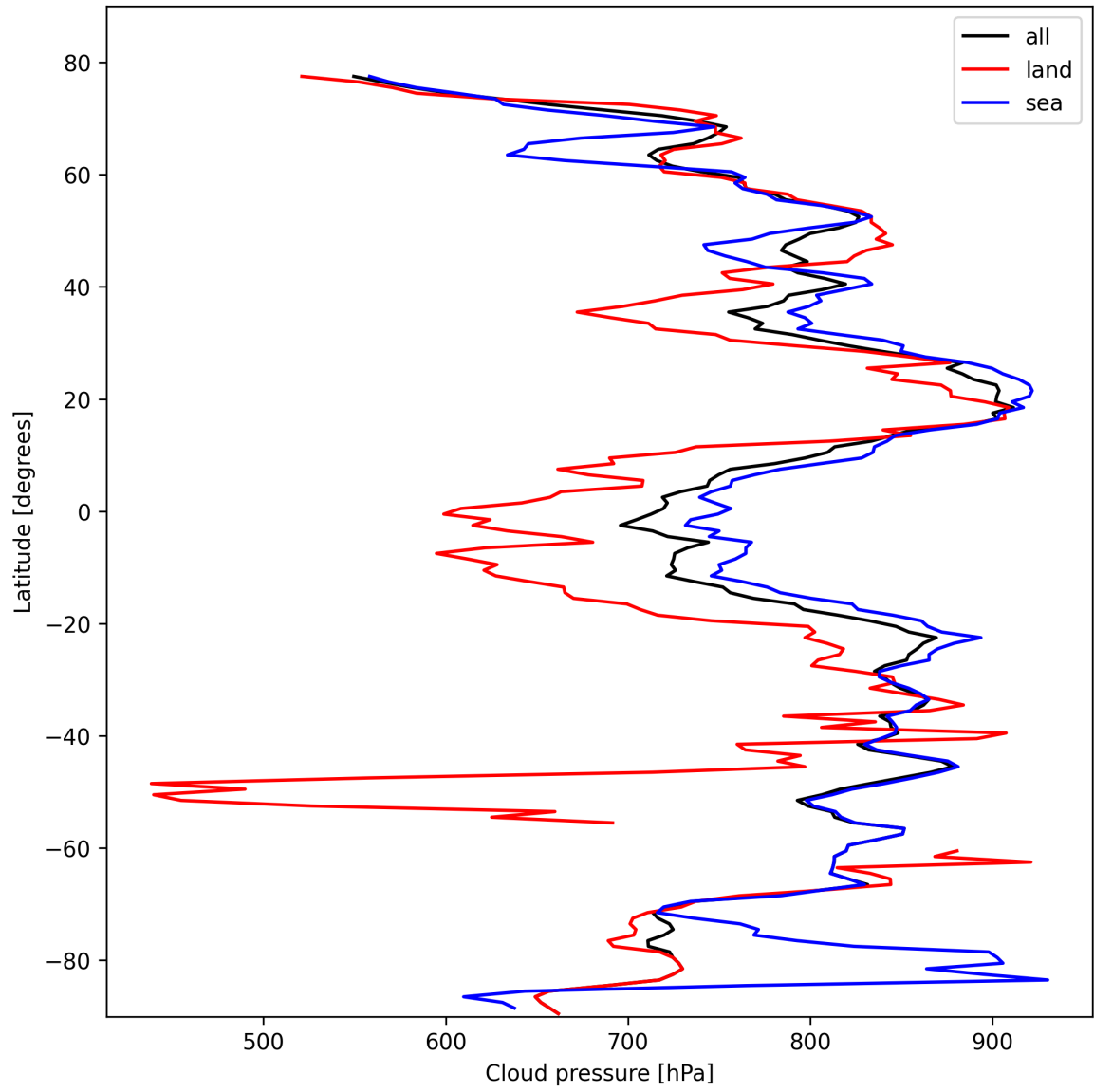
Figure 11: Zonal average of “Cloud pressure” for 2025-02-21 to 2025-02-22.
