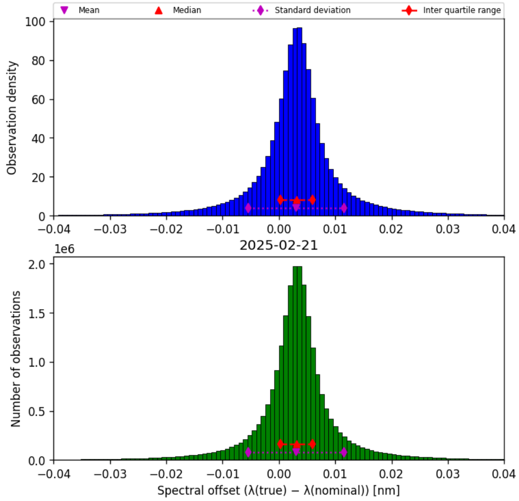
Figure 43: Histogram of “Spectral offset ( \lambda_{\text{true}} - \lambda_{\text{nominal}} )” for 2025-02-21 to 2025-02-22
