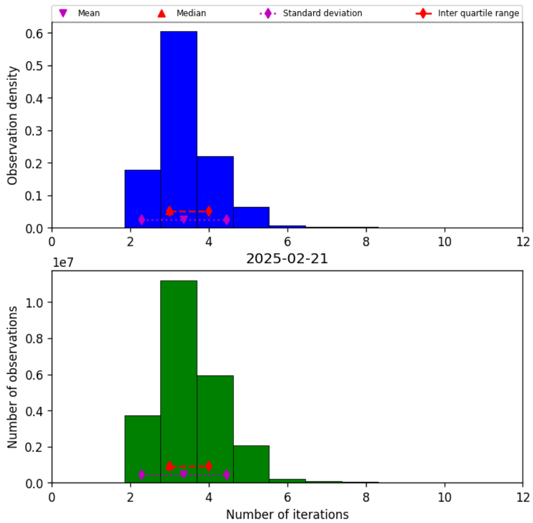
Figure 37: Histogram of “Number of iterations” for 2025-02-21 to 2025-02-22
