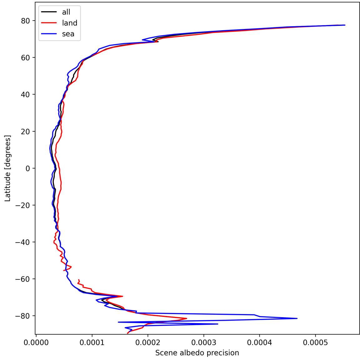
Figure 16: Zonal average of “Scene albedo precision” for 2025-02-21 to 2025-02-22.
