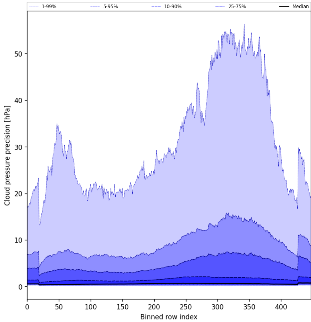
Figure 46: Along track statistics of “Cloud pressure precision” for 2025-02-21 to 2025-02-22
