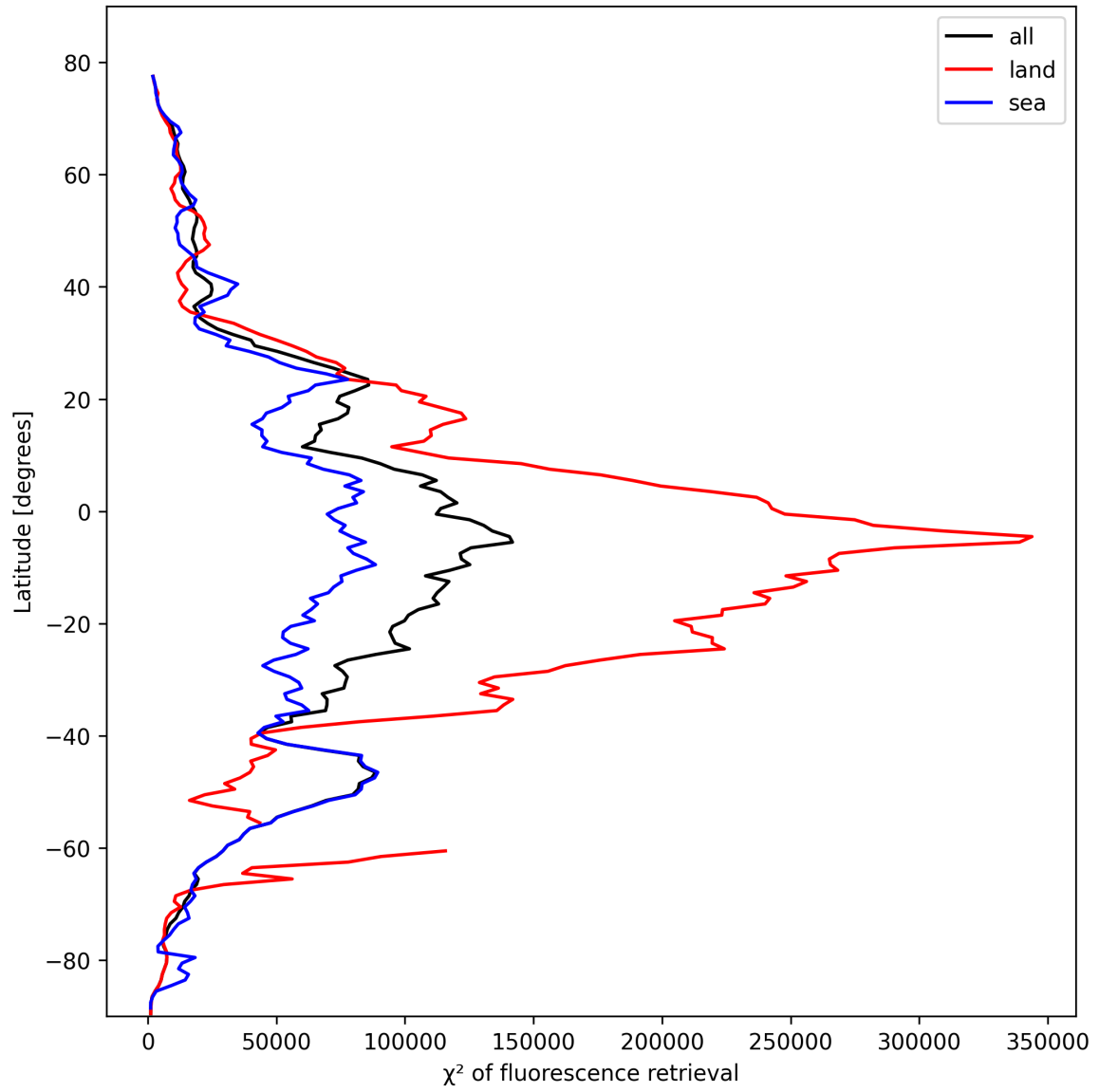
Figure 23: Zonal average of “ \chi^2 of fluorescence retrieval” for 2025-02-21 to 2025-02-22.
