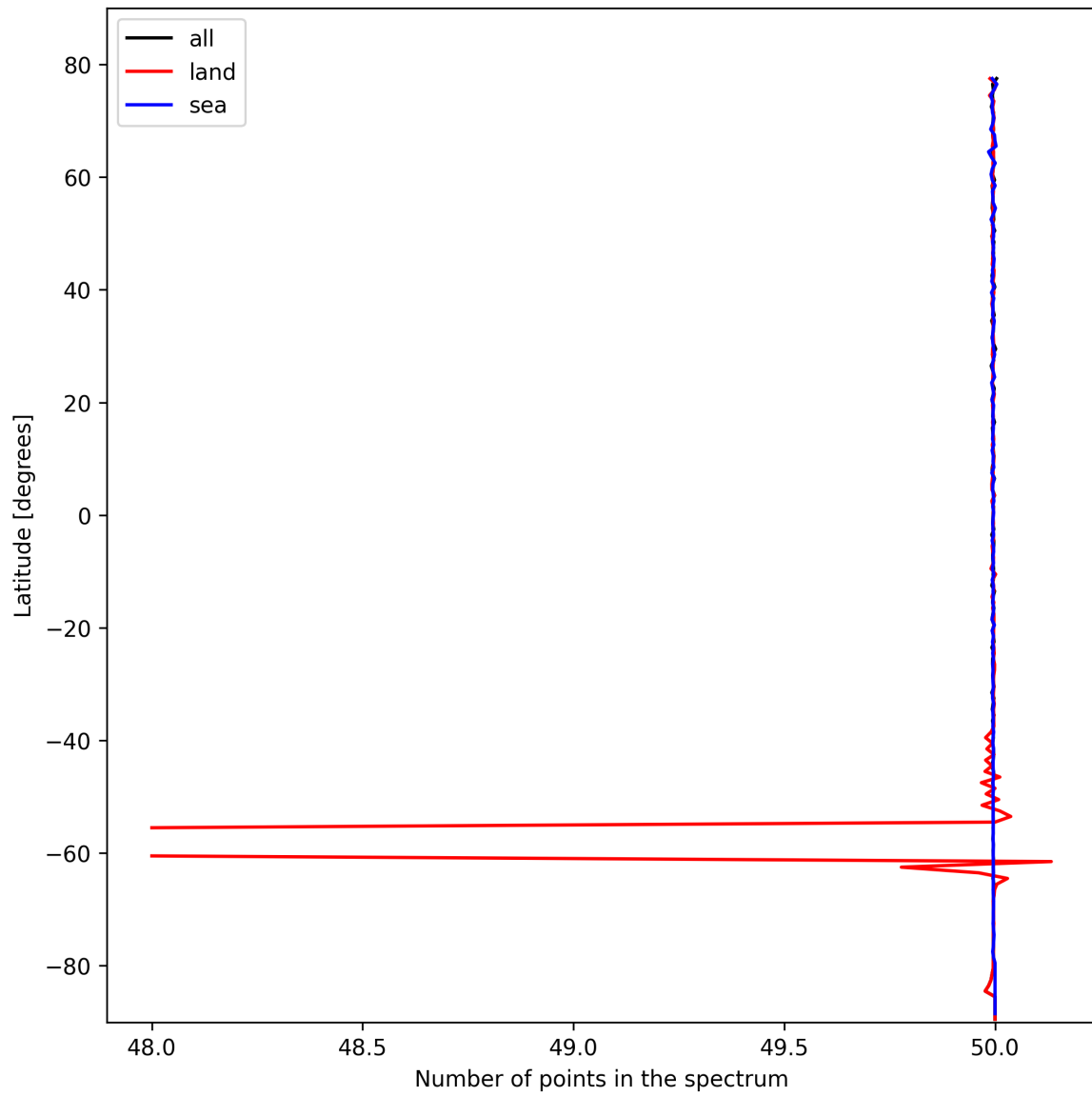
Figure 25: Zonal average of “Number of points in the spectrum” for 2025-02-21 to 2025-02-22.
