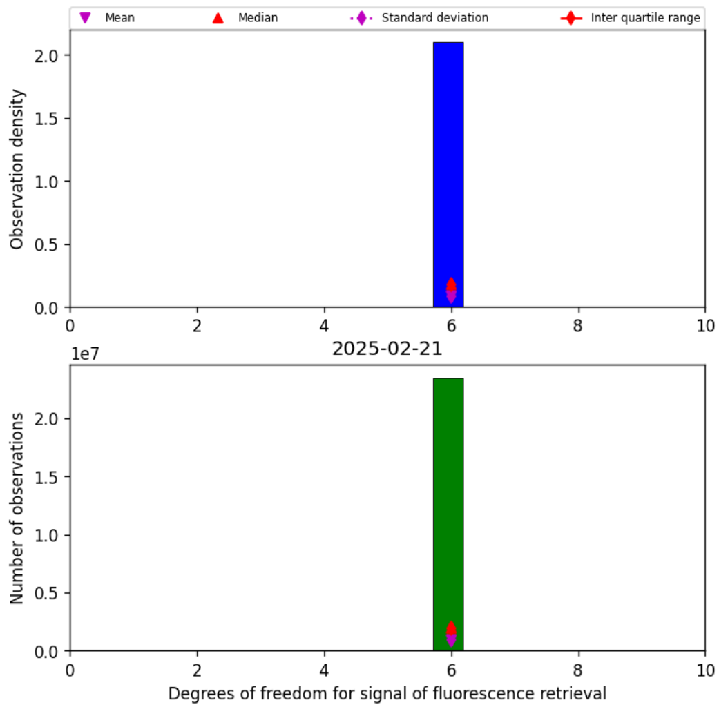
Figure 41: Histogram of “Degrees of freedom for signal of fluorescence retrieval” for 2025-02-21 to 2025-02-22
