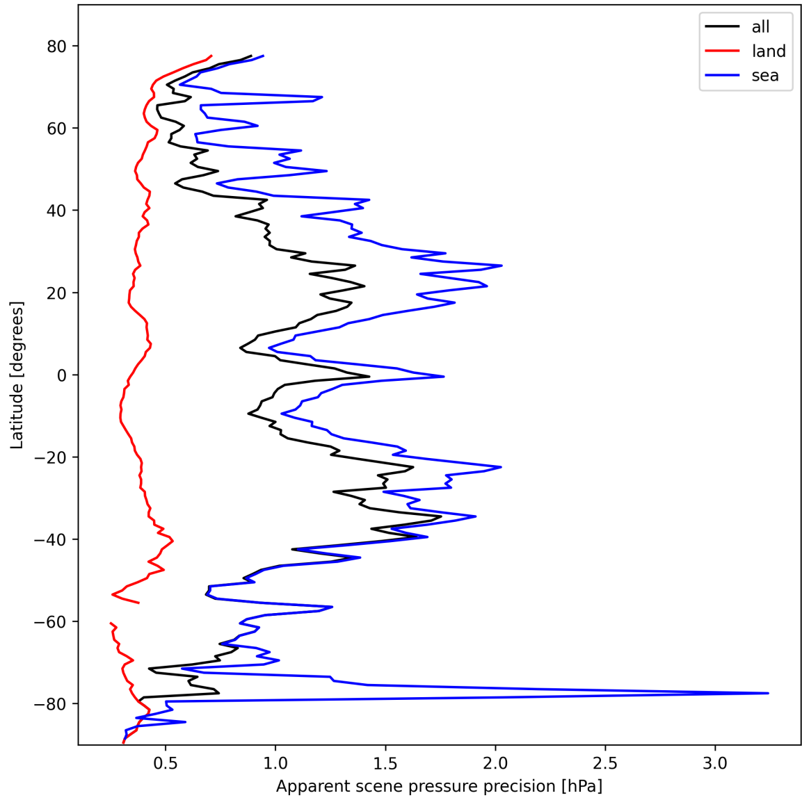
Figure 18: Zonal average of “Apparent scene pressure precision” for 2025-02-21 to 2025-02-22.
