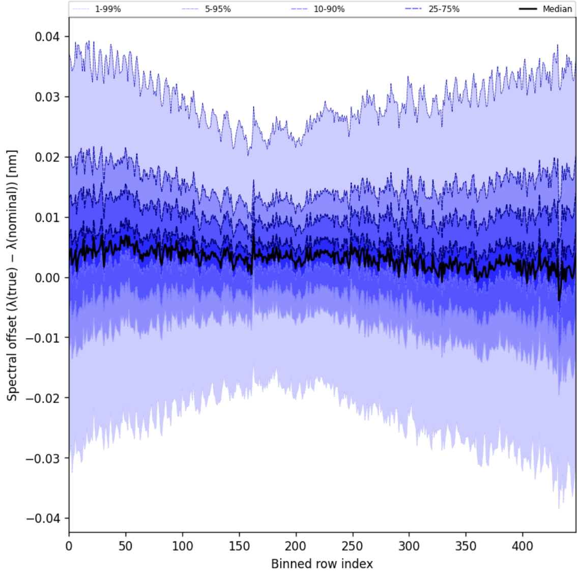
Figure 60: Along track statistics of “Spectral offset ( \lambda_{\text{true}} - \lambda_{\text{nominal}} )” for 2025-02-21 to 2025-02-22
