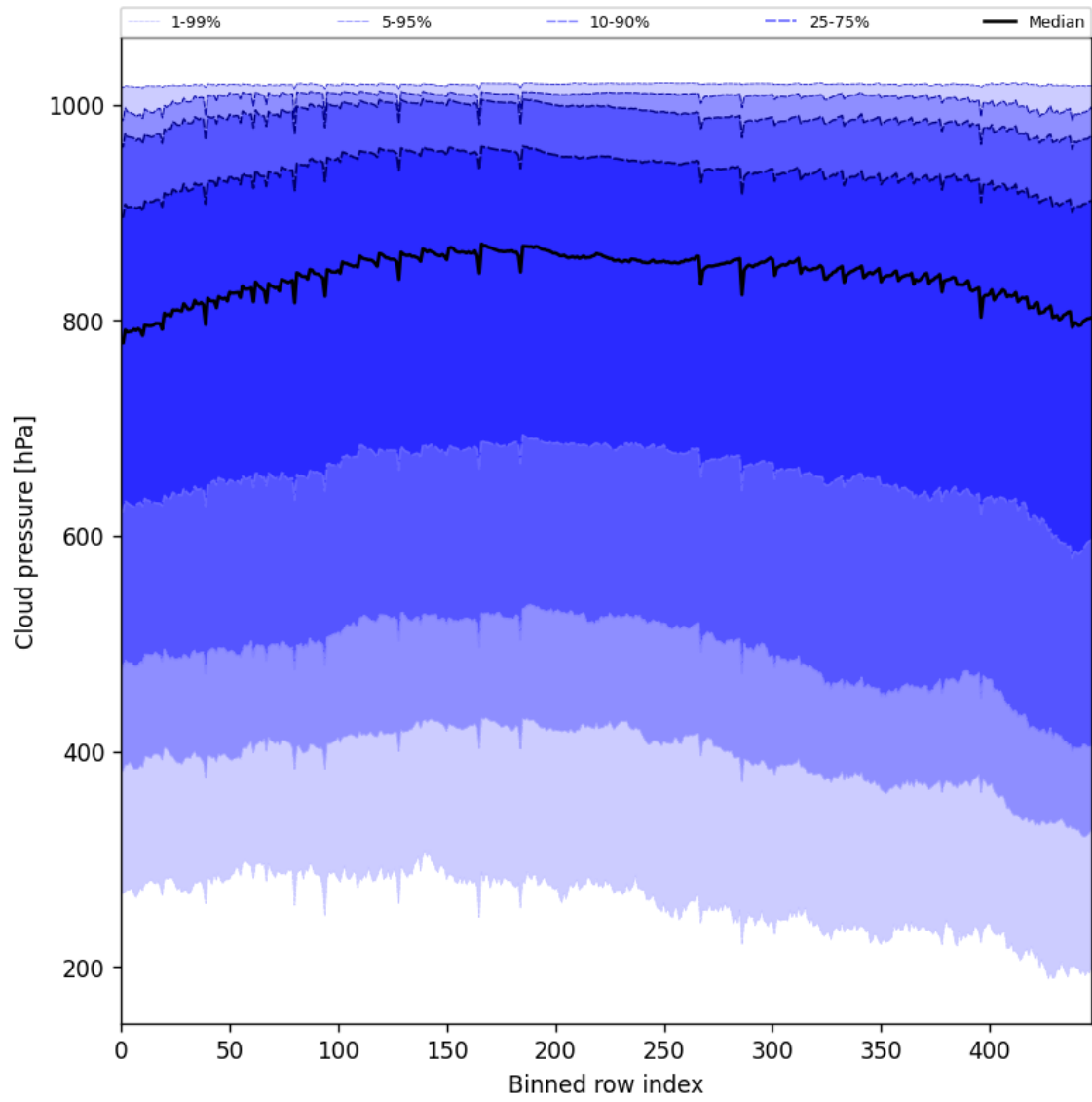
Figure 45: Along track statistics of “Cloud pressure” for 2025-02-21 to 2025-02-22
