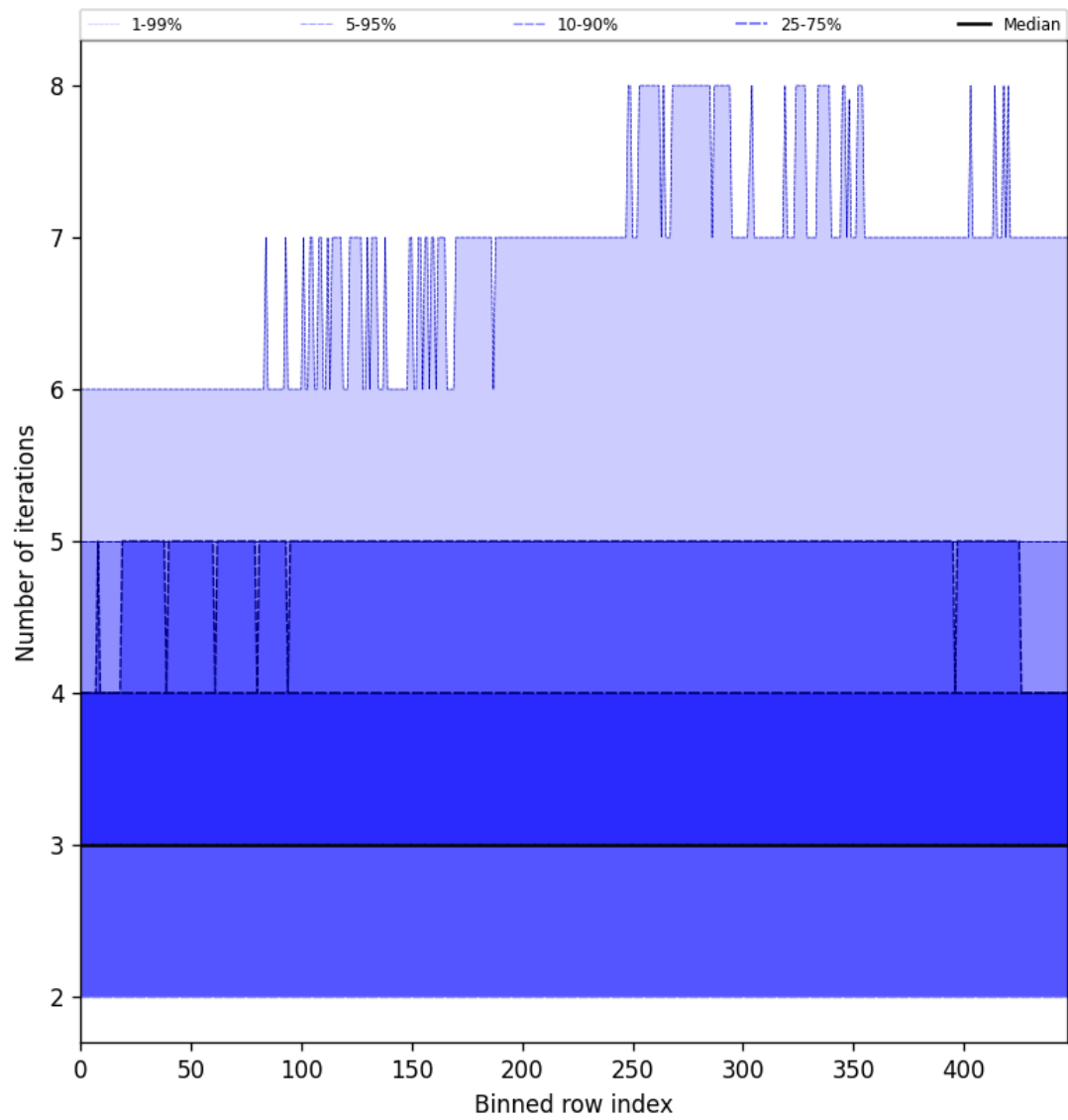
Figure 54: Along track statistics of “Number of iterations” for 2025-02-21 to 2025-02-22
