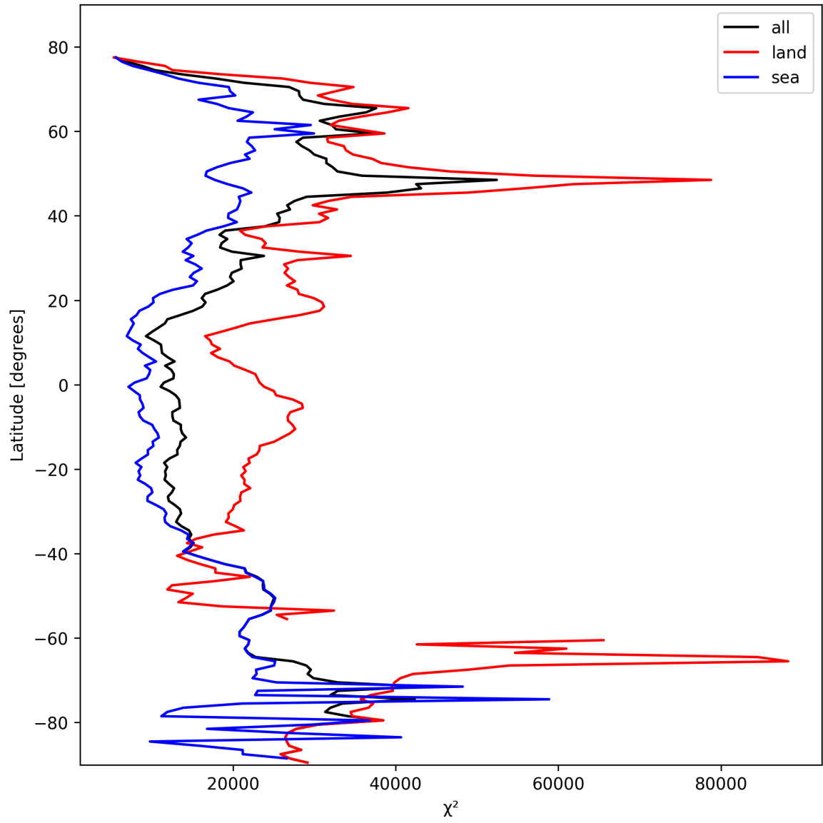
Figure 19: Zonal average of “ \chi^2 ” for 2025-02-21 to 2025-02-22.
