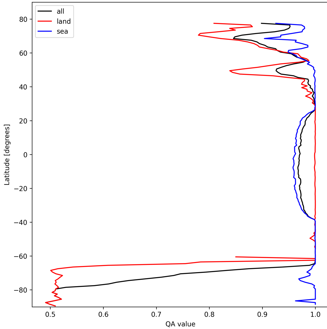
Figure 10: Zonal average of “QA value” for 2025-02-21 to 2025-02-22.
