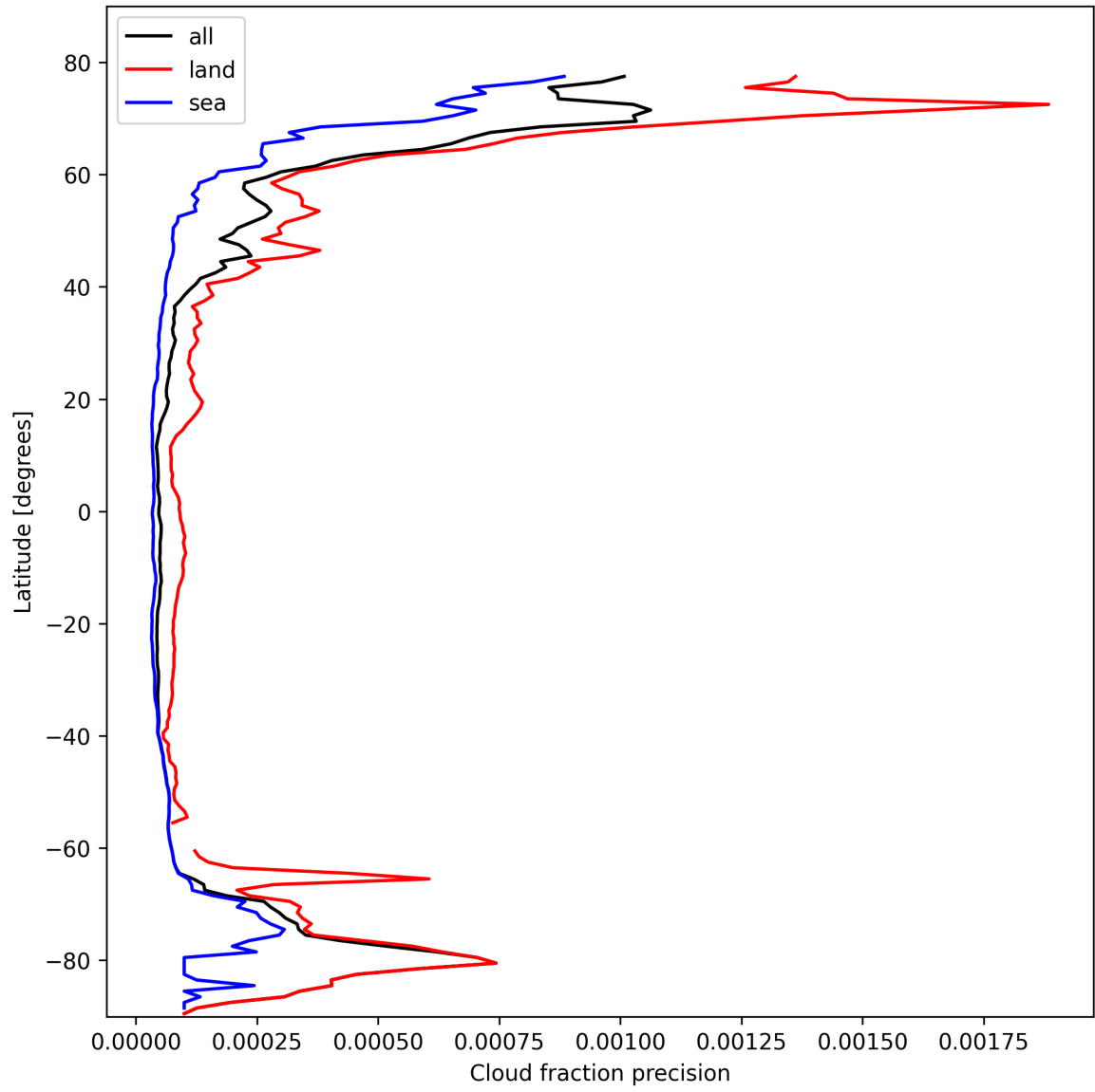
Figure 14: Zonal average of “Cloud fraction precision” for 2025-02-21 to 2025-02-22.
