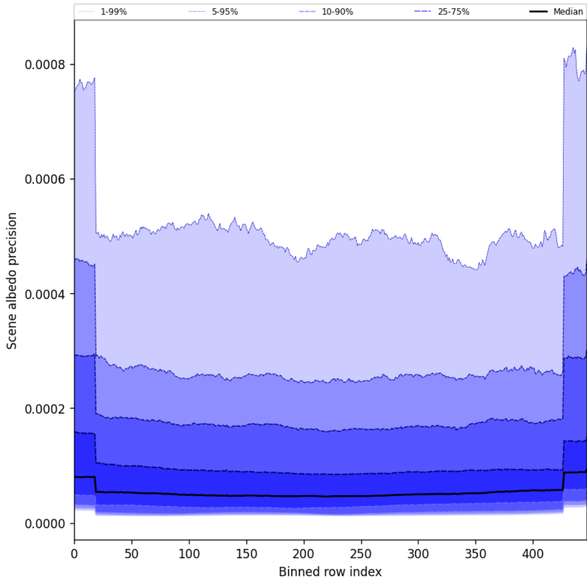
Figure 50: Along track statistics of “Scene albedo precision” for 2025-02-21 to 2025-02-22
