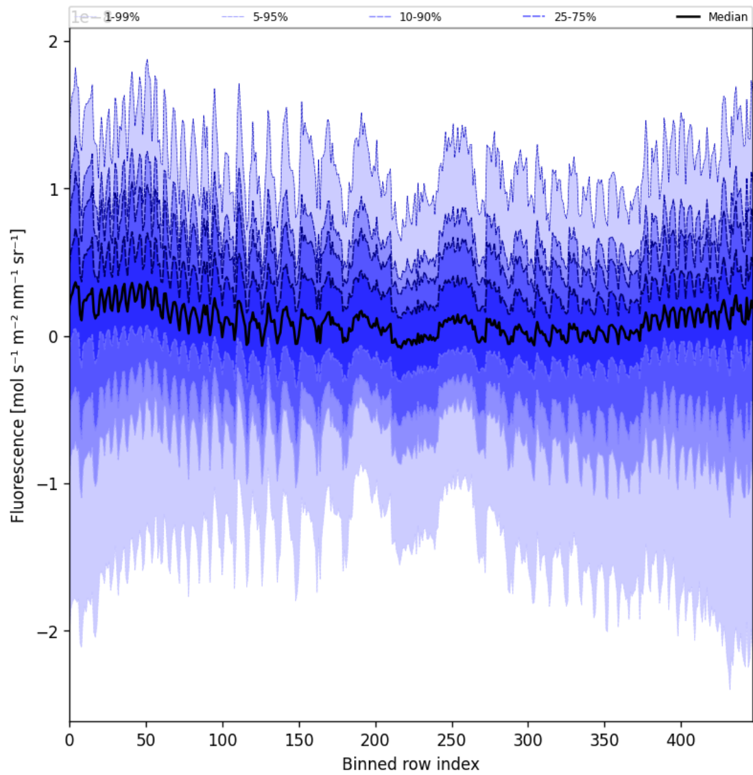
Figure 55: Along track statistics of “Fluorescence” for 2025-02-21 to 2025-02-22
