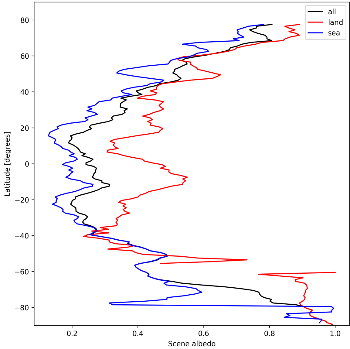
Figure 15: Zonal average of "Scene albedo" for 2025-02-21 to 2025-02-22.
