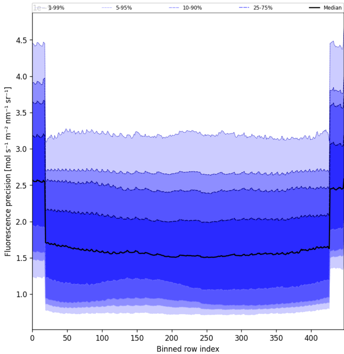
Figure 56: Along track statistics of “Fluorescence precision” for 2025-02-21 to 2025-02-22
