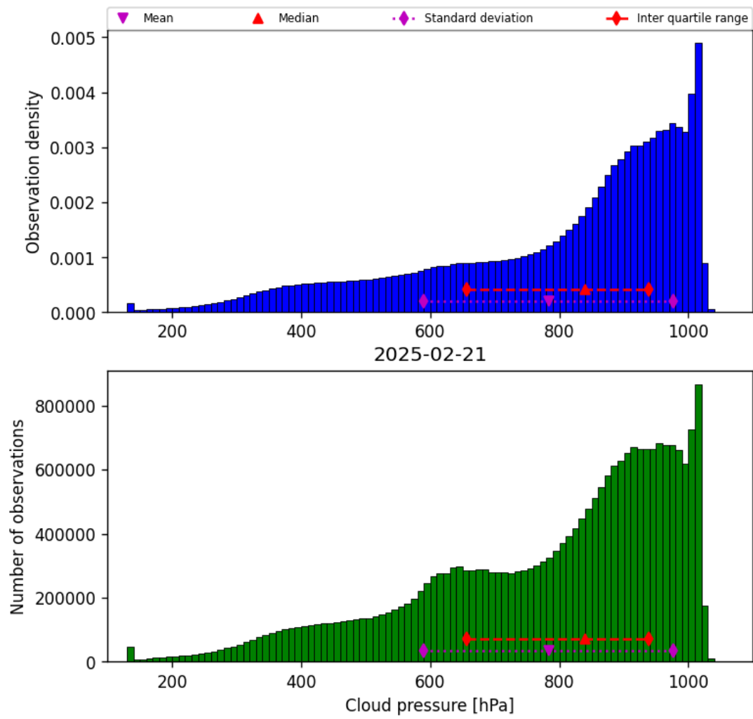
Figure 28: Histogram of “Cloud pressure” for 2025-02-21 to 2025-02-22
