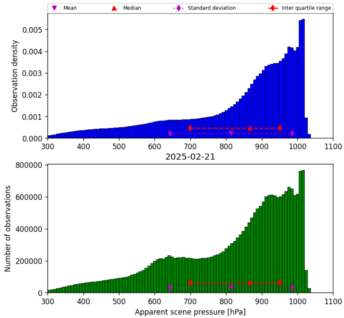
Figure 34: Histogram of “Apparent scene pressure” for 2025-02-21 to 2025-02-22
