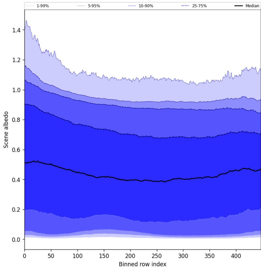
Figure 49: Along track statistics of “Scene albedo” for 2025-02-21 to 2025-02-22
