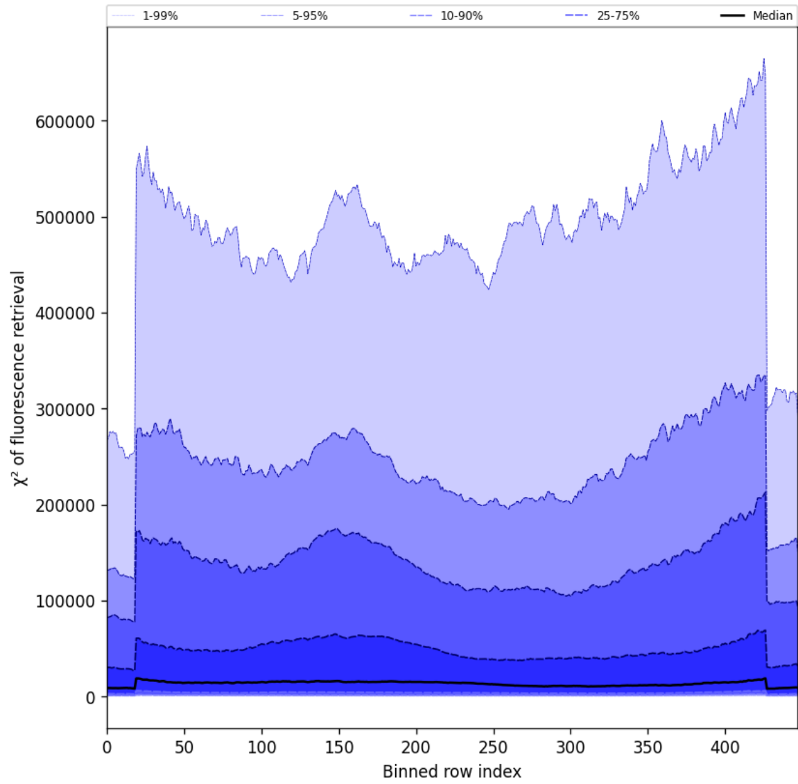
Figure 57: Along track statistics of “ \chi^2 of fluorescence retrieval” for 2025-02-21 to 2025-02-22
