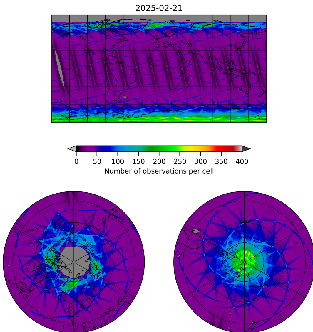
Figure 9: Map of the number of observations for 2025-02-21 to 2025-02-22
