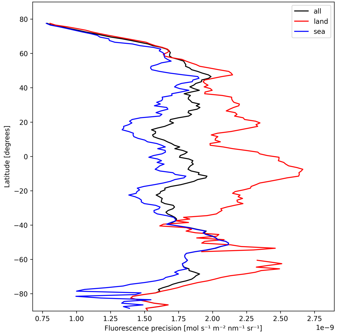
Figure 22: Zonal average of “Fluorescence precision” for 2025-02-21 to 2025-02-22.
