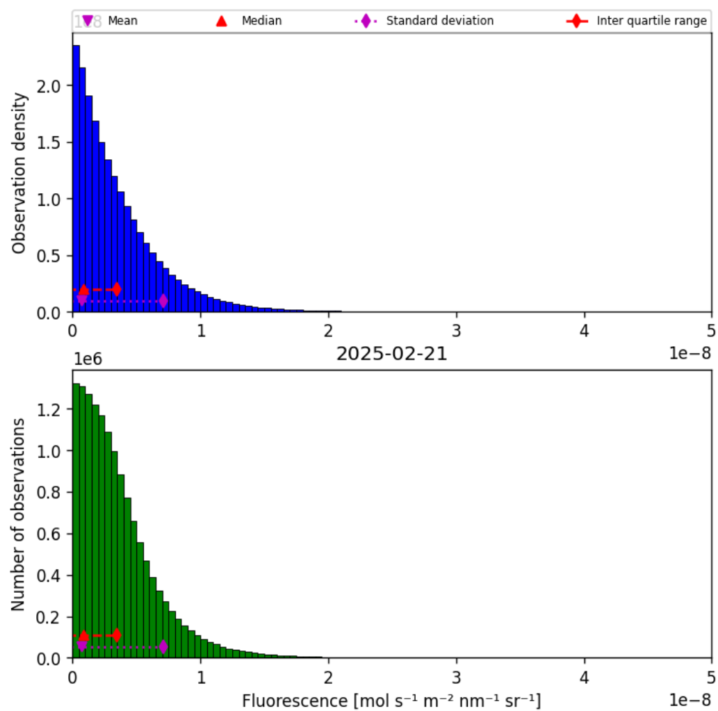
Figure 38: Histogram of “Fluorescence” for 2025-02-21 to 2025-02-22
