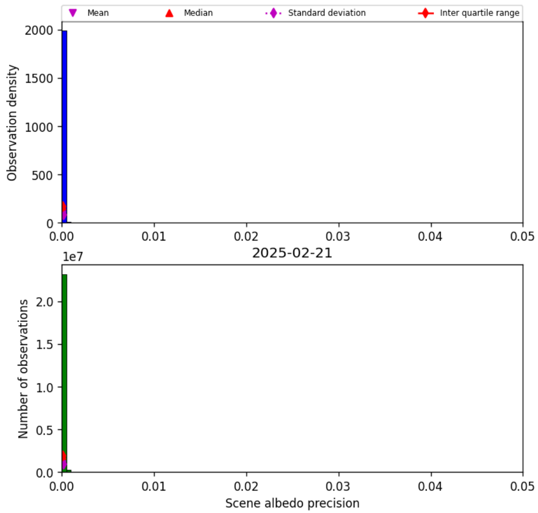
Figure 33: Histogram of “Scene albedo precision” for 2025-02-21 to 2025-02-22
