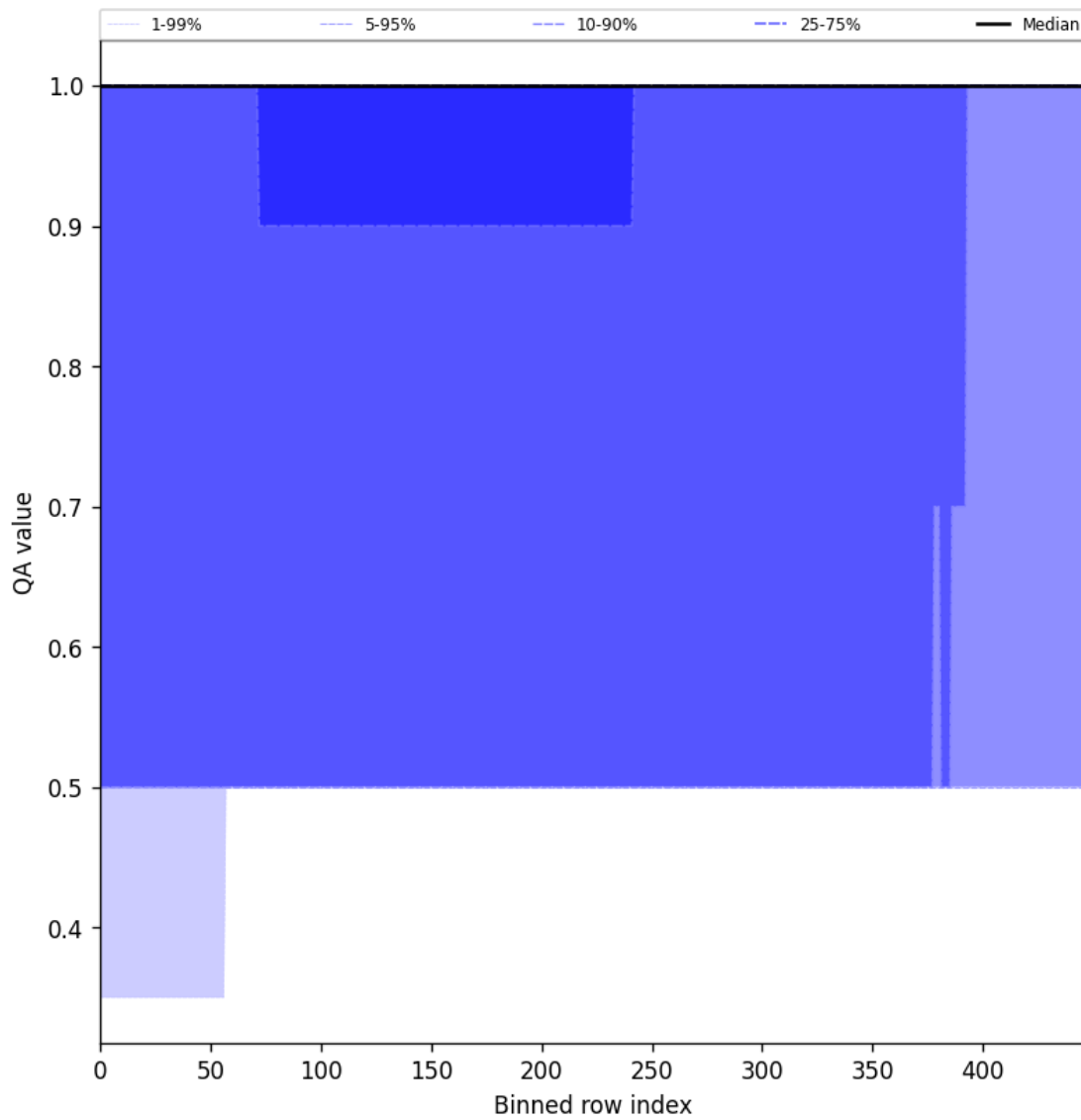
Figure 44: Along track statistics of “QA value” for 2025-02-21 to 2025-02-22
