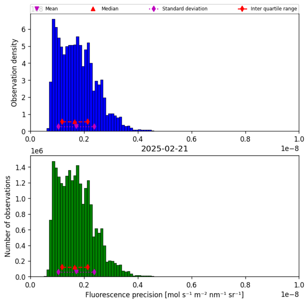
Figure 39: Histogram of “Fluorescence precision” for 2025-02-21 to 2025-02-22
