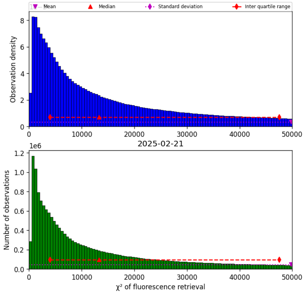
Figure 40: Histogram of “ \chi^2 of fluorescence retrieval” for 2025-02-21 to 2025-02-22
