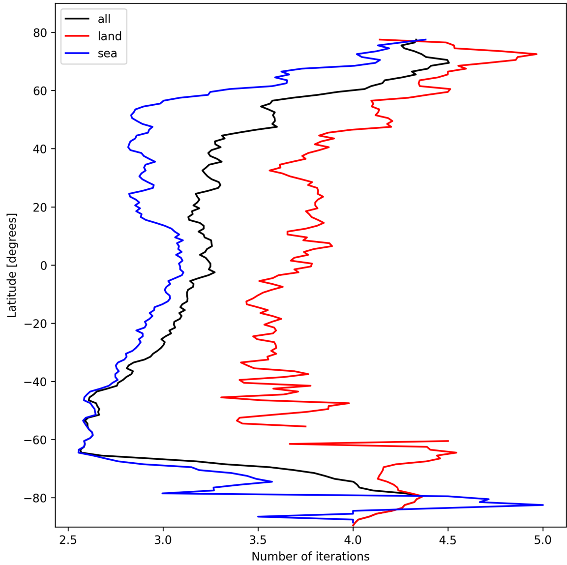
Figure 20: Zonal average of “Number of iterations” for 2025-02-21 to 2025-02-22.
