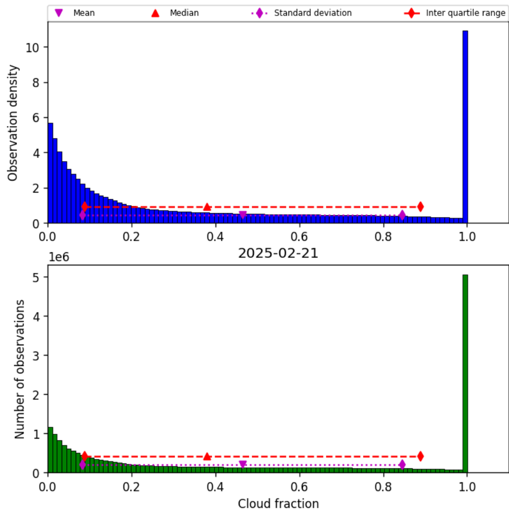
Figure 30: Histogram of “Cloud fraction” for 2025-02-21 to 2025-02-22
