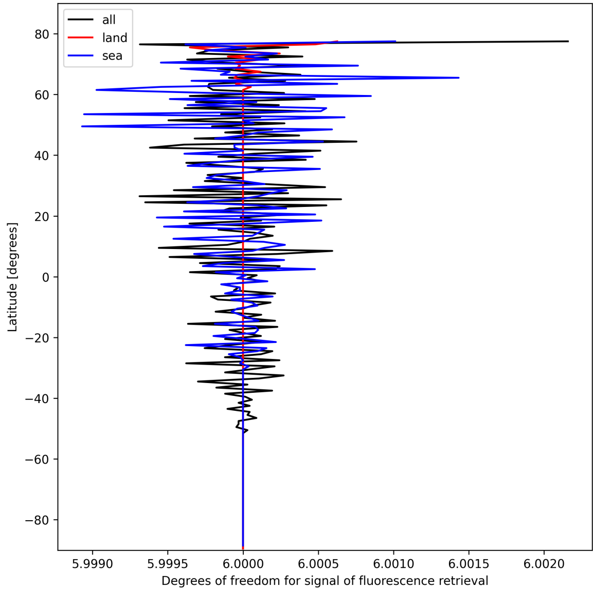
Figure 24: Zonal average of “Degrees of freedom for signal of fluorescence retrieval” for 2025-02-21 to 2025-02-22.
