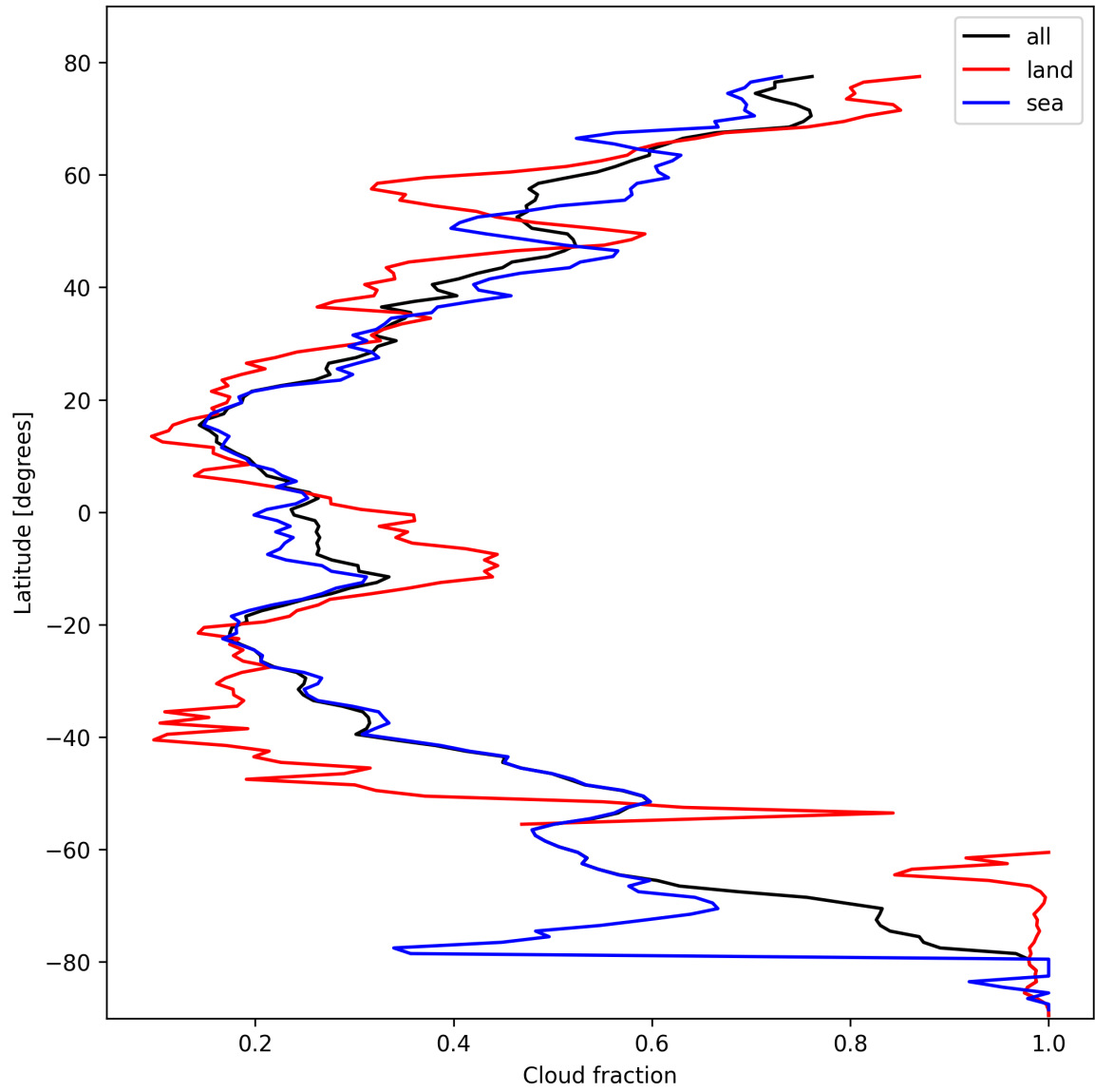
Figure 13: Zonal average of “Cloud fraction” for 2025-02-21 to 2025-02-22.
