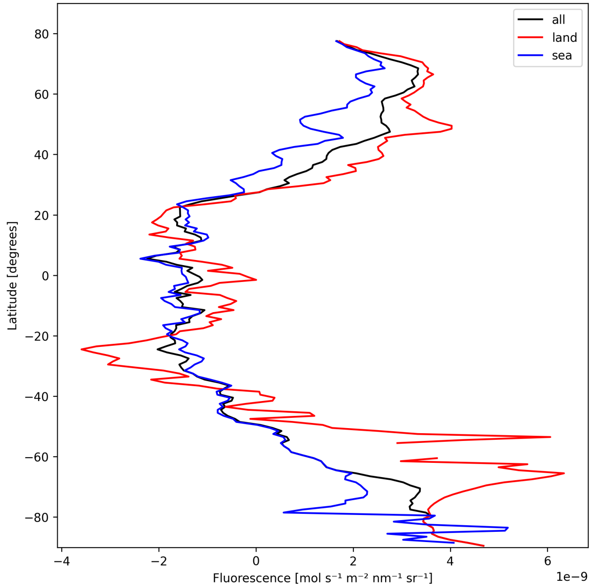
Figure 21: Zonal average of “Fluorescence” for 2025-02-21 to 2025-02-22.
