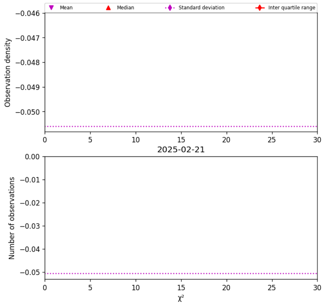
Figure 36: Histogram of " \chi^2 " for 2025-02-21 to 2025-02-22
