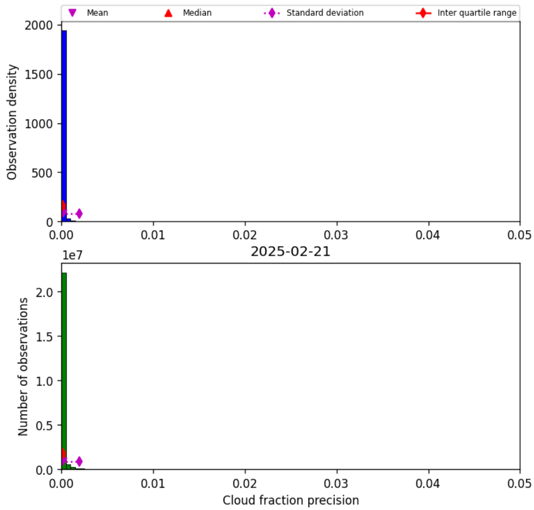
Figure 31: Histogram of “Cloud fraction precision” for 2025-02-21 to 2025-02-22
