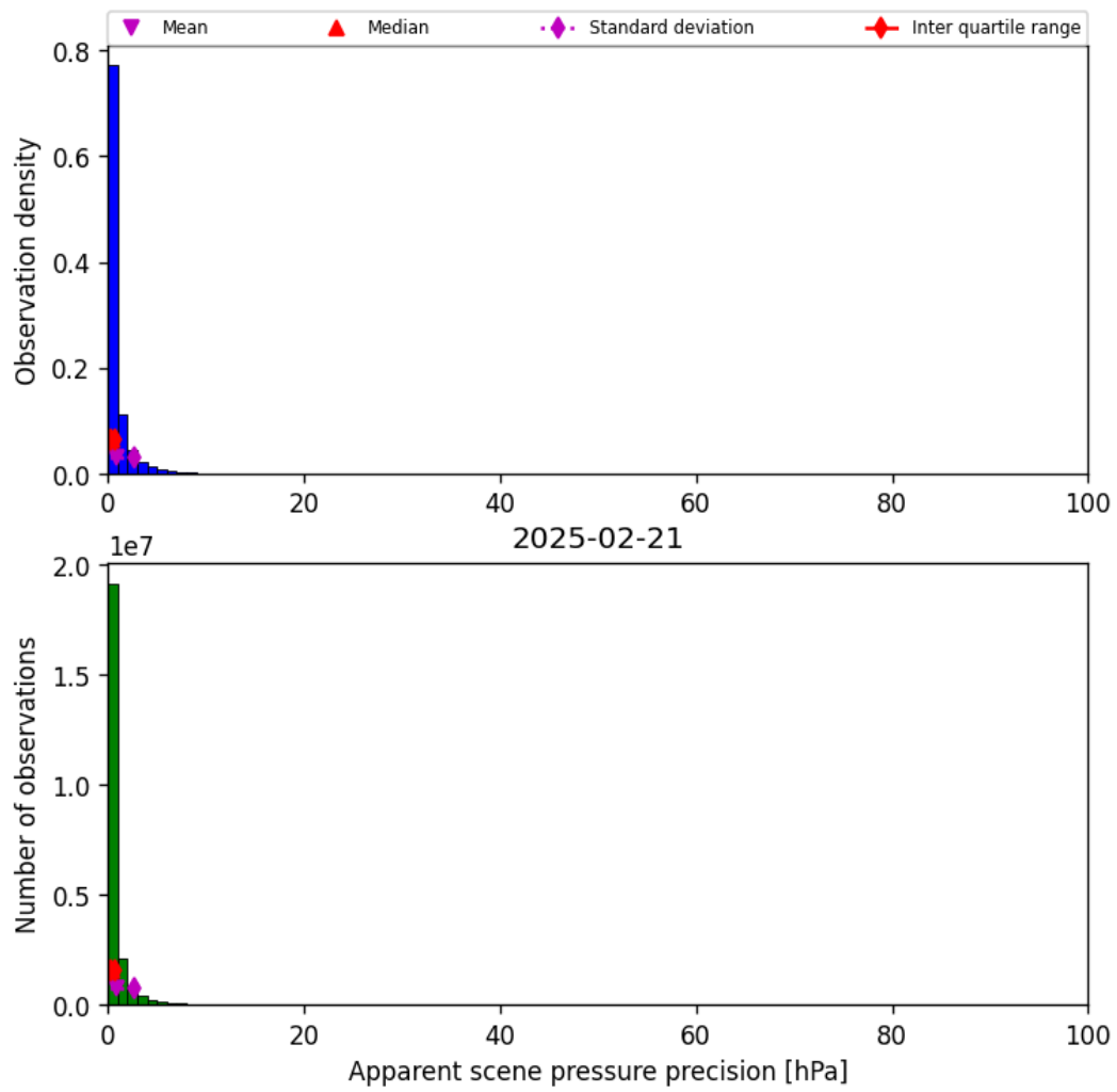
Figure 35: Histogram of “Apparent scene pressure precision” for 2025-02-21 to 2025-02-22
