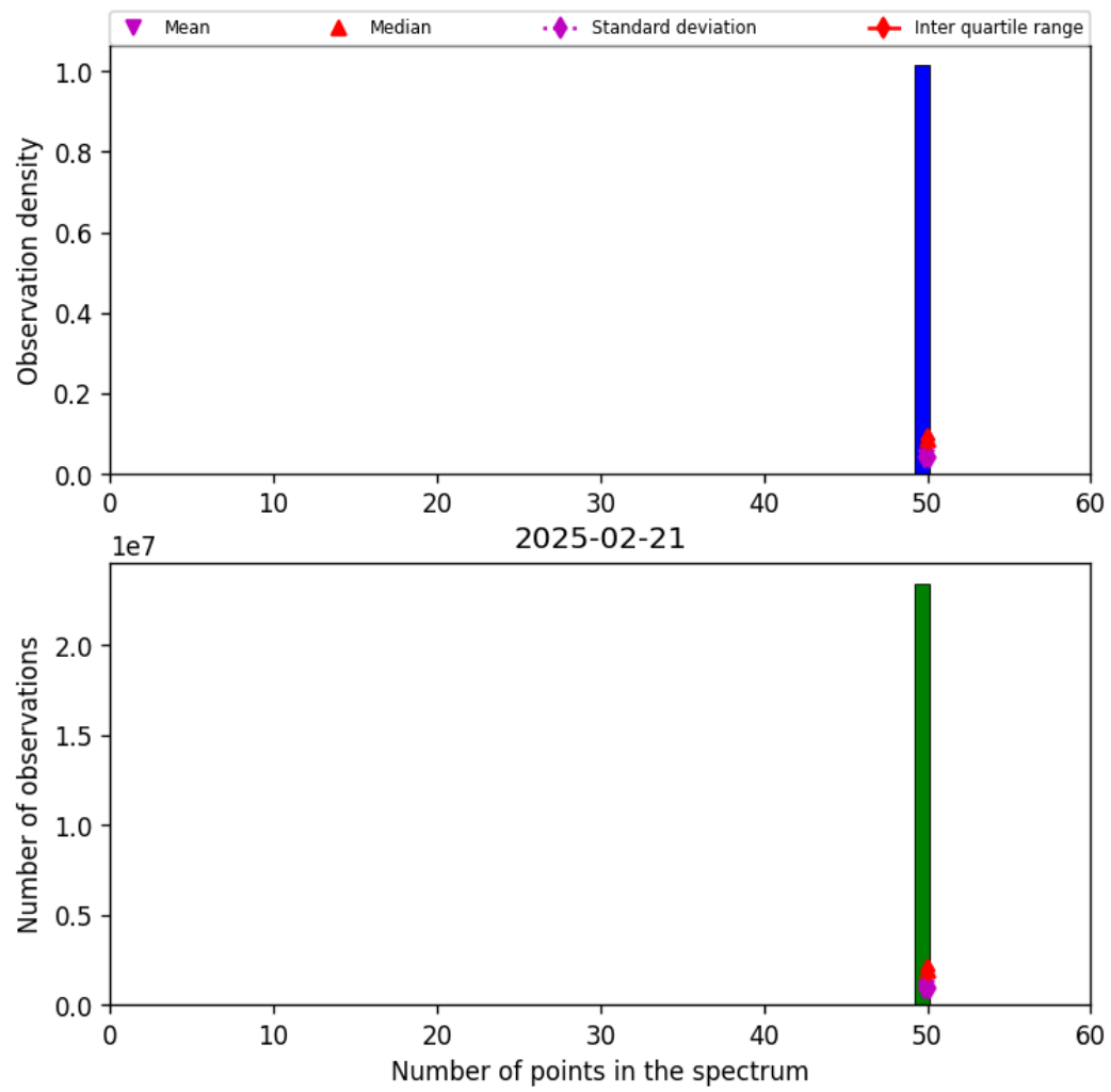
Figure 42: Histogram of “Number of points in the spectrum” for 2025-02-21 to 2025-02-22
