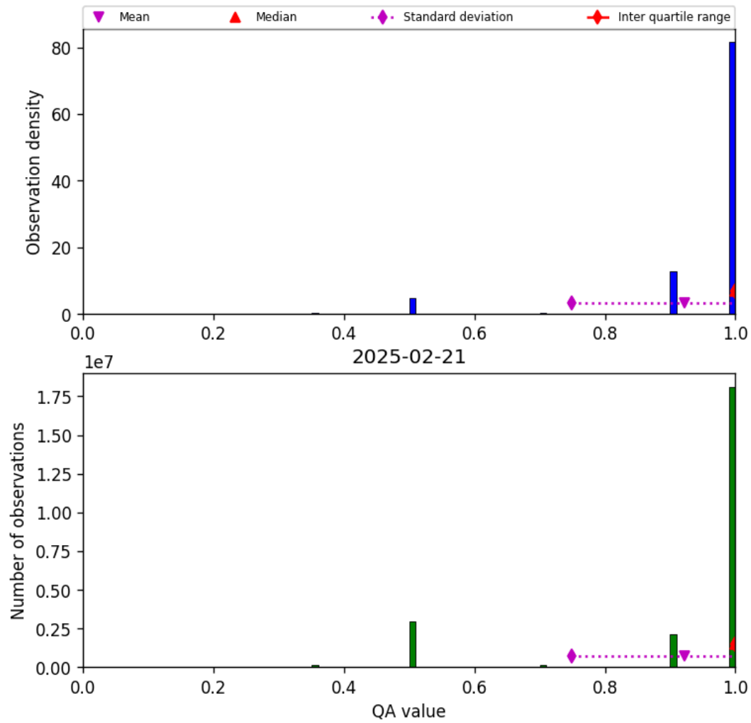
Figure 27: Histogram of “QA value” for 2025-02-21 to 2025-02-22
