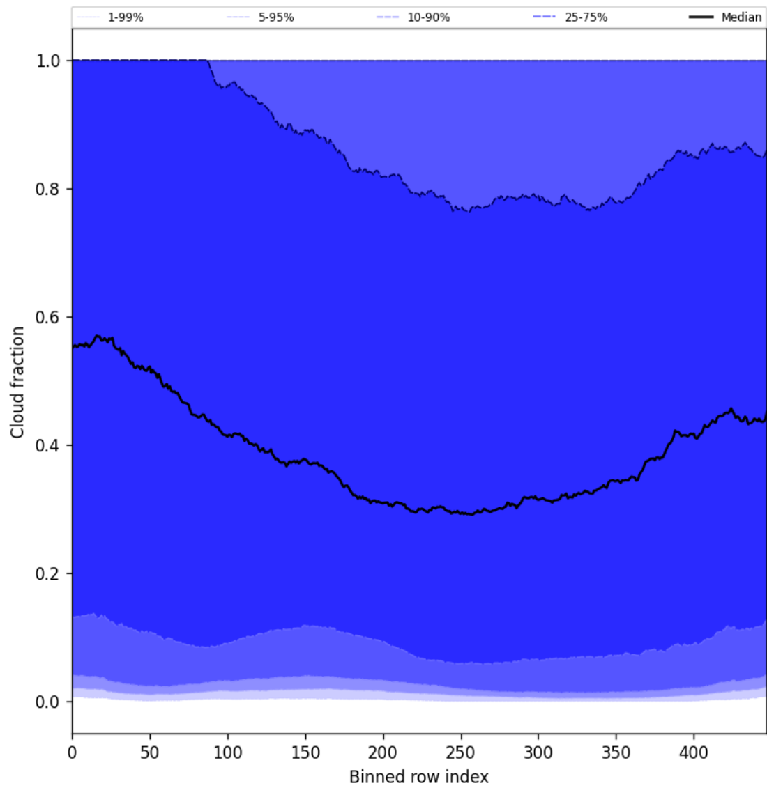
Figure 47: Along track statistics of “Cloud fraction” for 2025-02-21 to 2025-02-22
