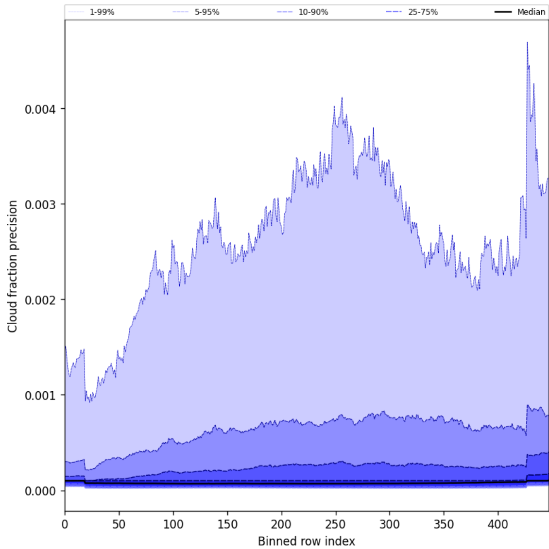
Figure 48: Along track statistics of “Cloud fraction precision” for 2025-02-21 to 2025-02-22
