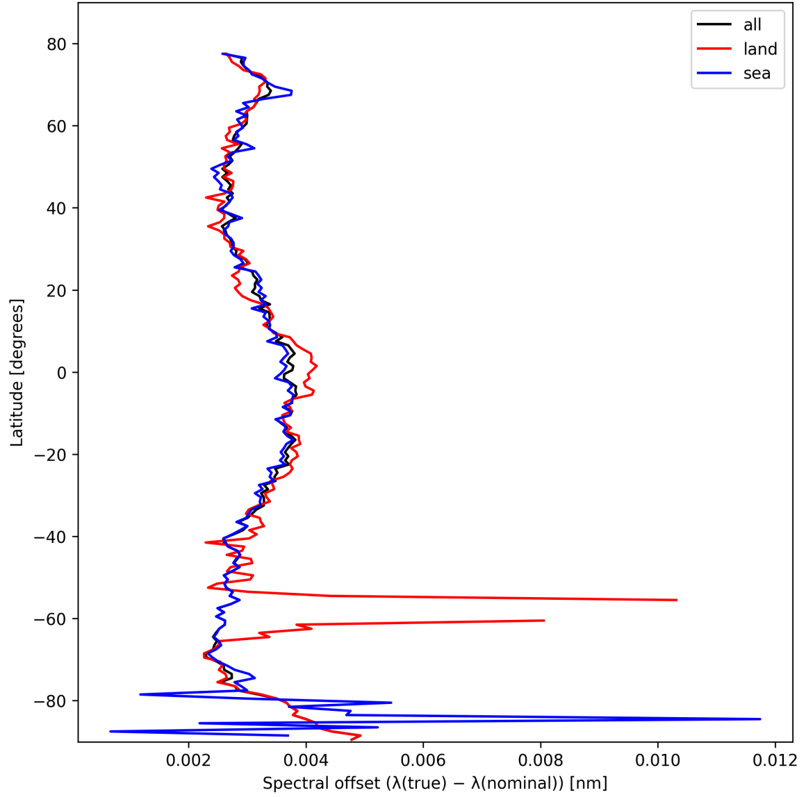
Figure 26: Zonal average of “Spectral offset ( \lambda_{\text{true}} - \lambda_{\text{nominal}} )” for 2025-02-21 to 2025-02-22.
