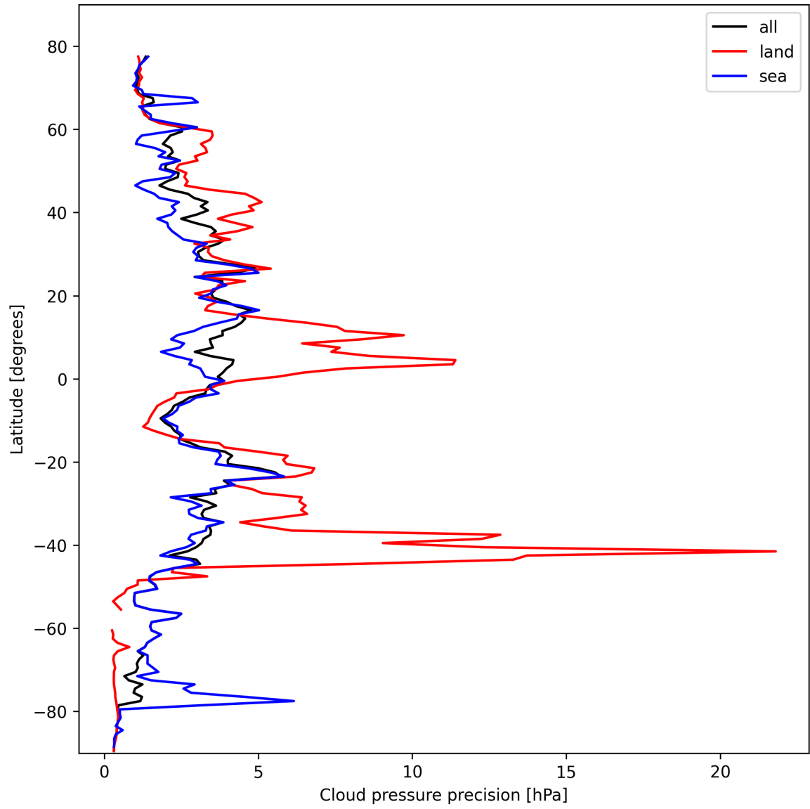
Figure 12: Zonal average of "Cloud pressure precision" for 2025-02-21 to 2025-02-22.
