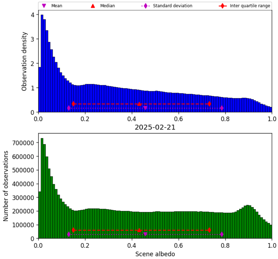
Figure 32: Histogram of “Scene albedo” for 2025-02-21 to 2025-02-22
