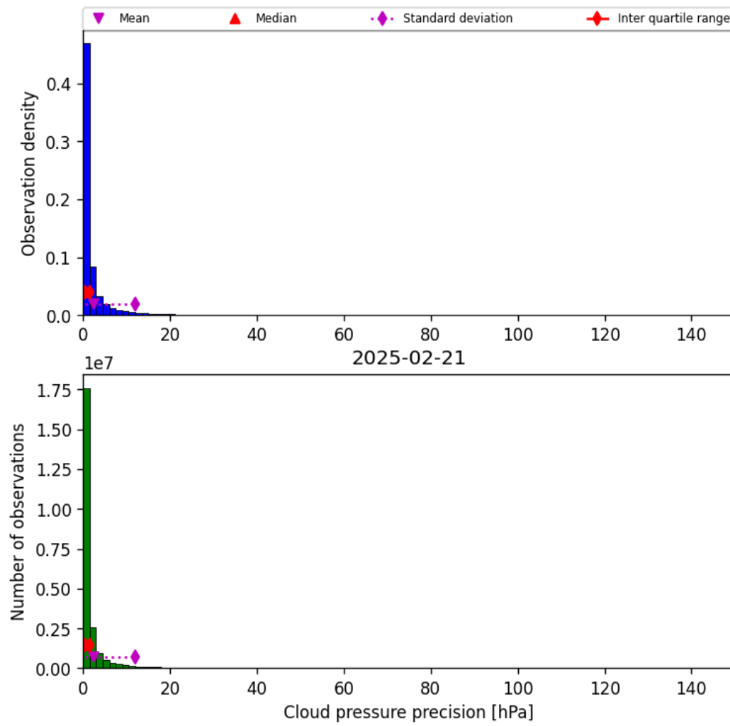
Figure 29: Histogram of “Cloud pressure precision” for 2025-02-21 to 2025-02-22
