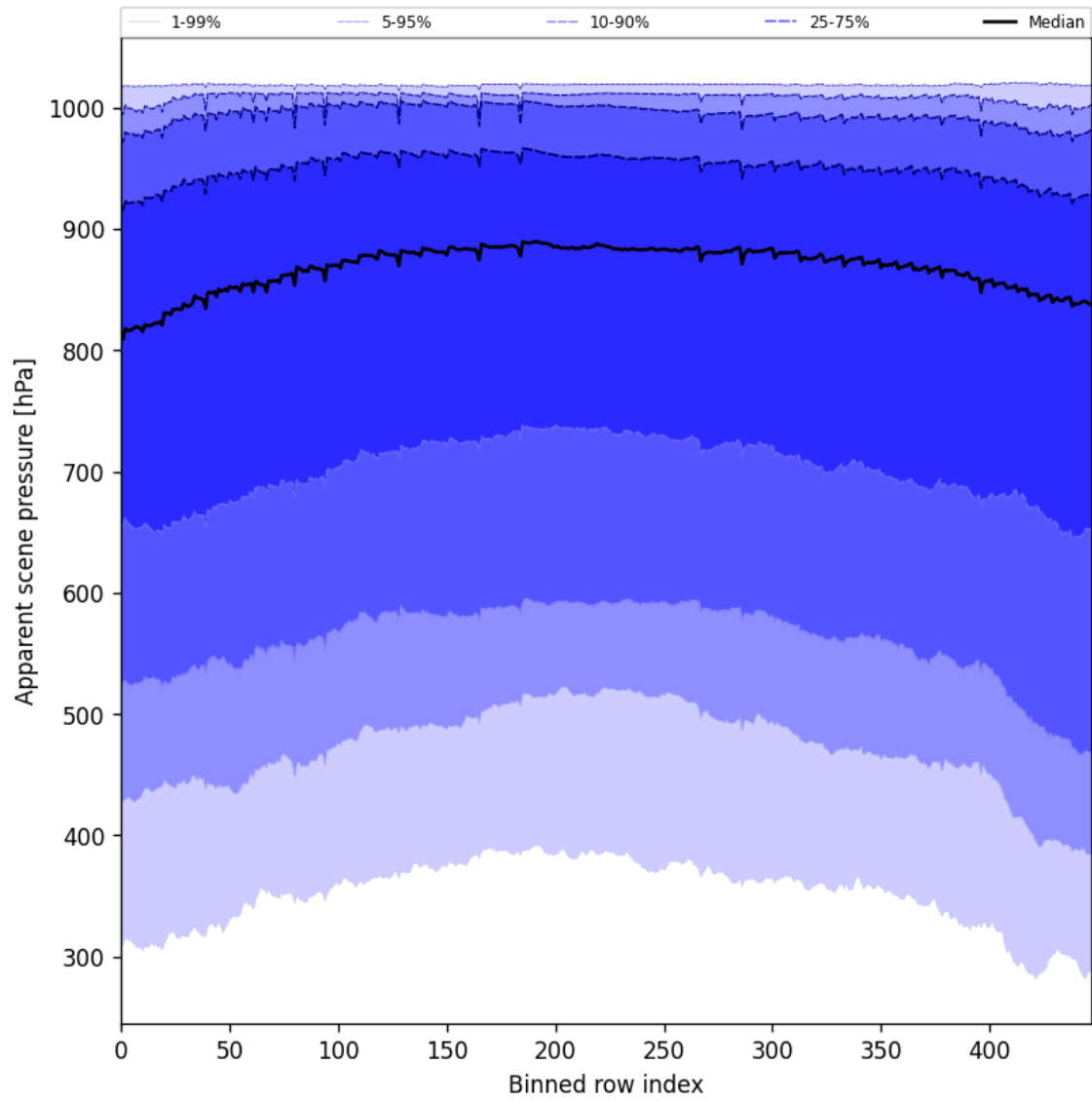
Figure 51: Along track statistics of “Apparent scene pressure” for 2025-02-21 to 2025-02-22
