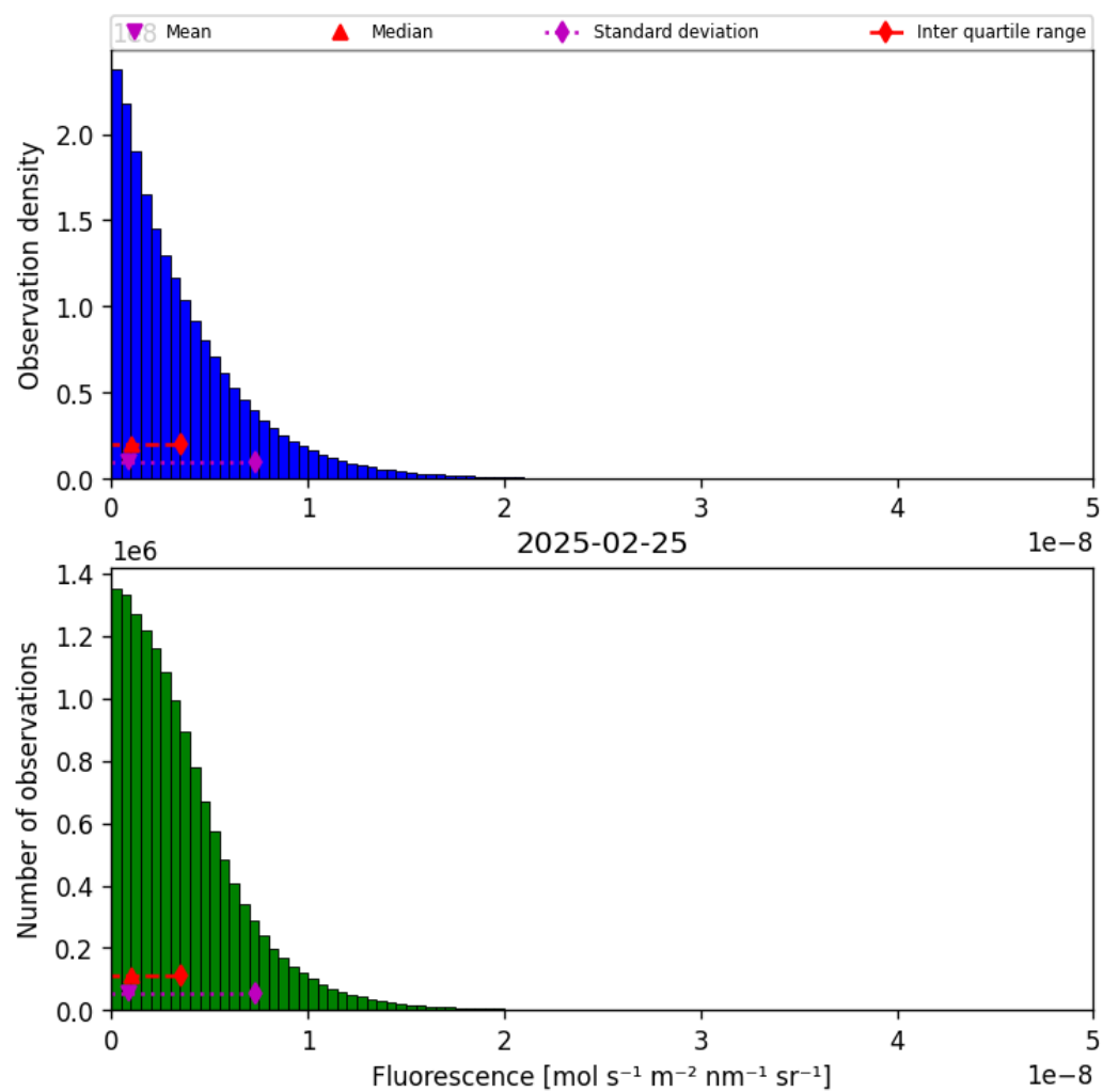
Figure 38: Histogram of “Fluorescence” for 2025-02-25 to 2025-02-26
