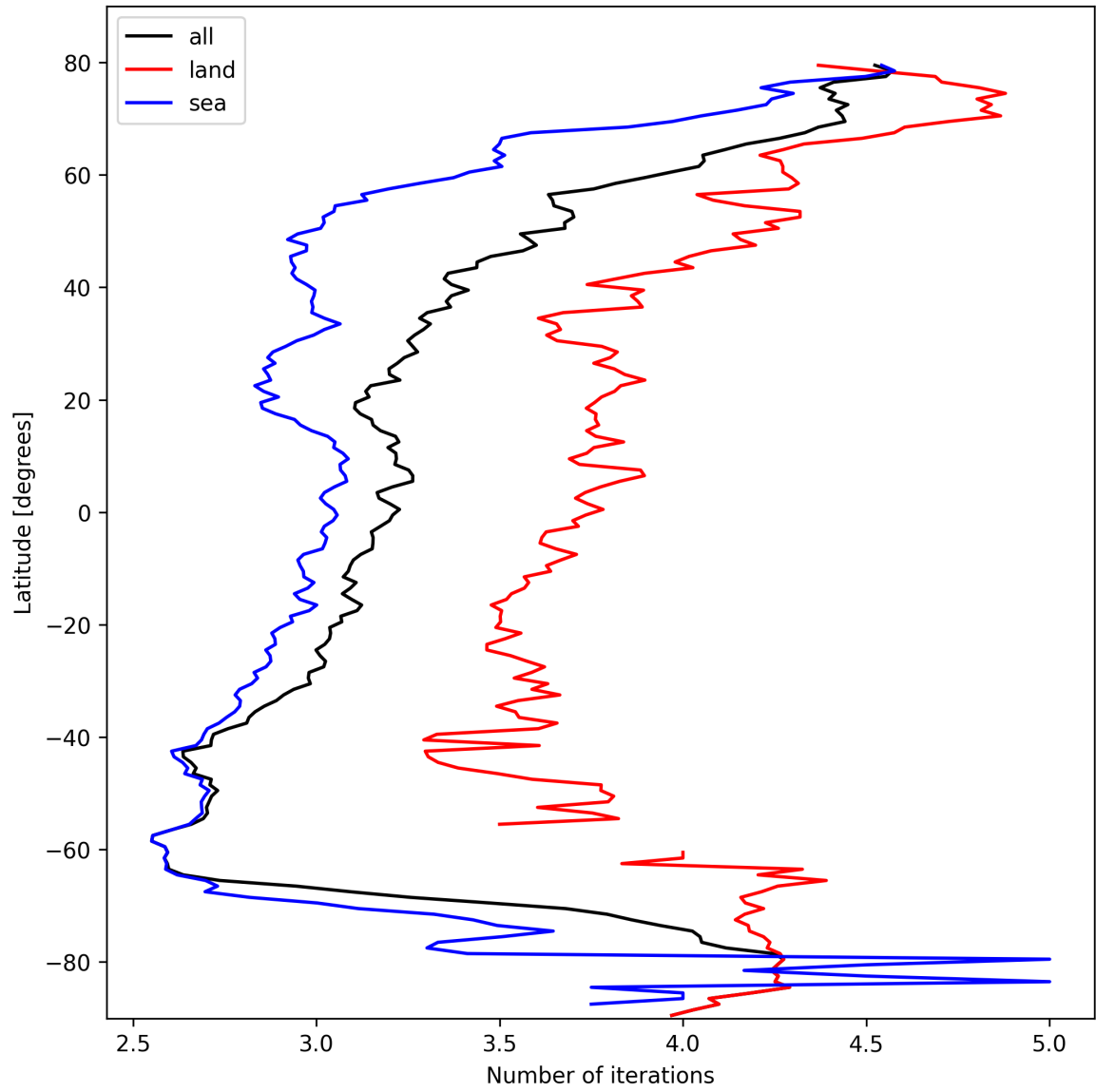
Figure 20: Zonal average of “Number of iterations” for 2025-02-25 to 2025-02-26.
