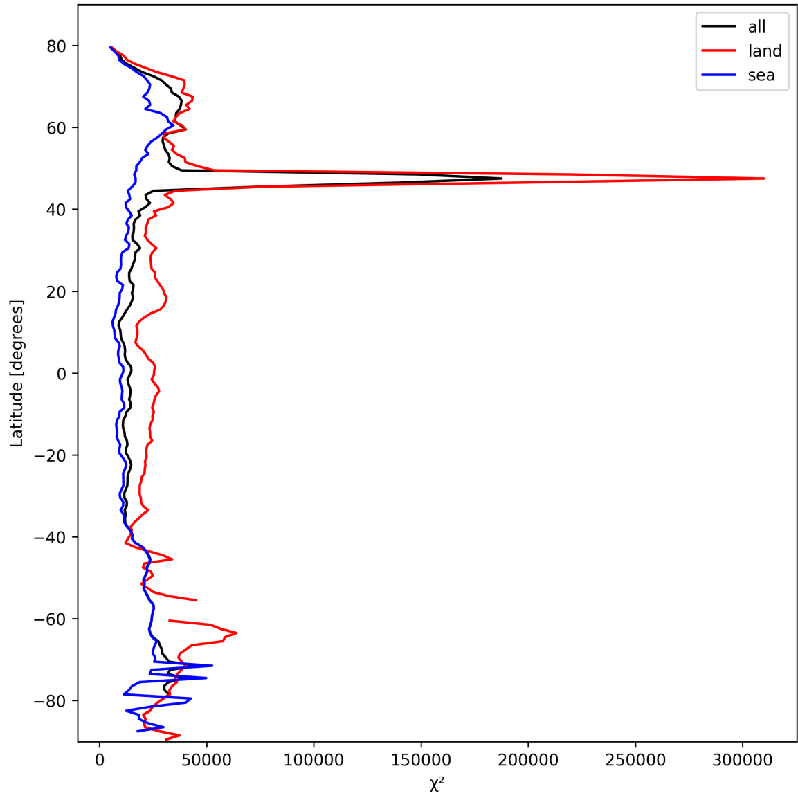
Figure 19: Zonal average of “ \chi^2 ” for 2025-02-25 to 2025-02-26.
