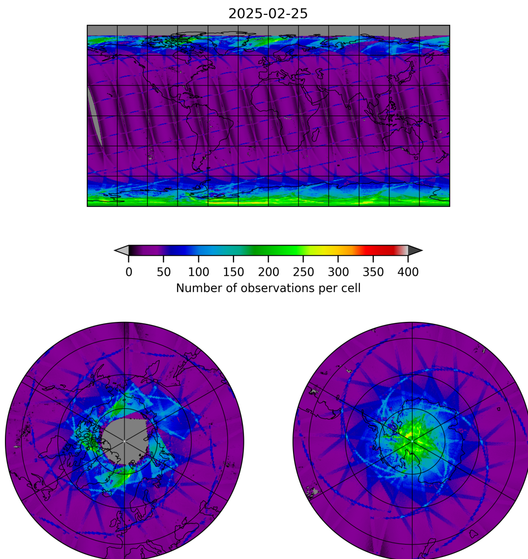
Figure 9: Map of the number of observations for 2025-02-25 to 2025-02-26
