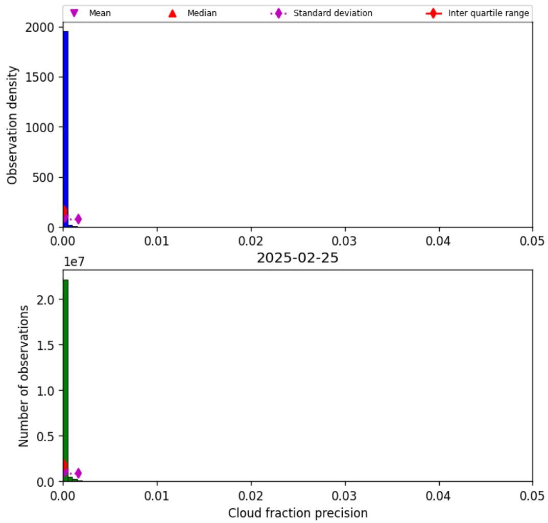
Figure 31: Histogram of “Cloud fraction precision” for 2025-02-25 to 2025-02-26
