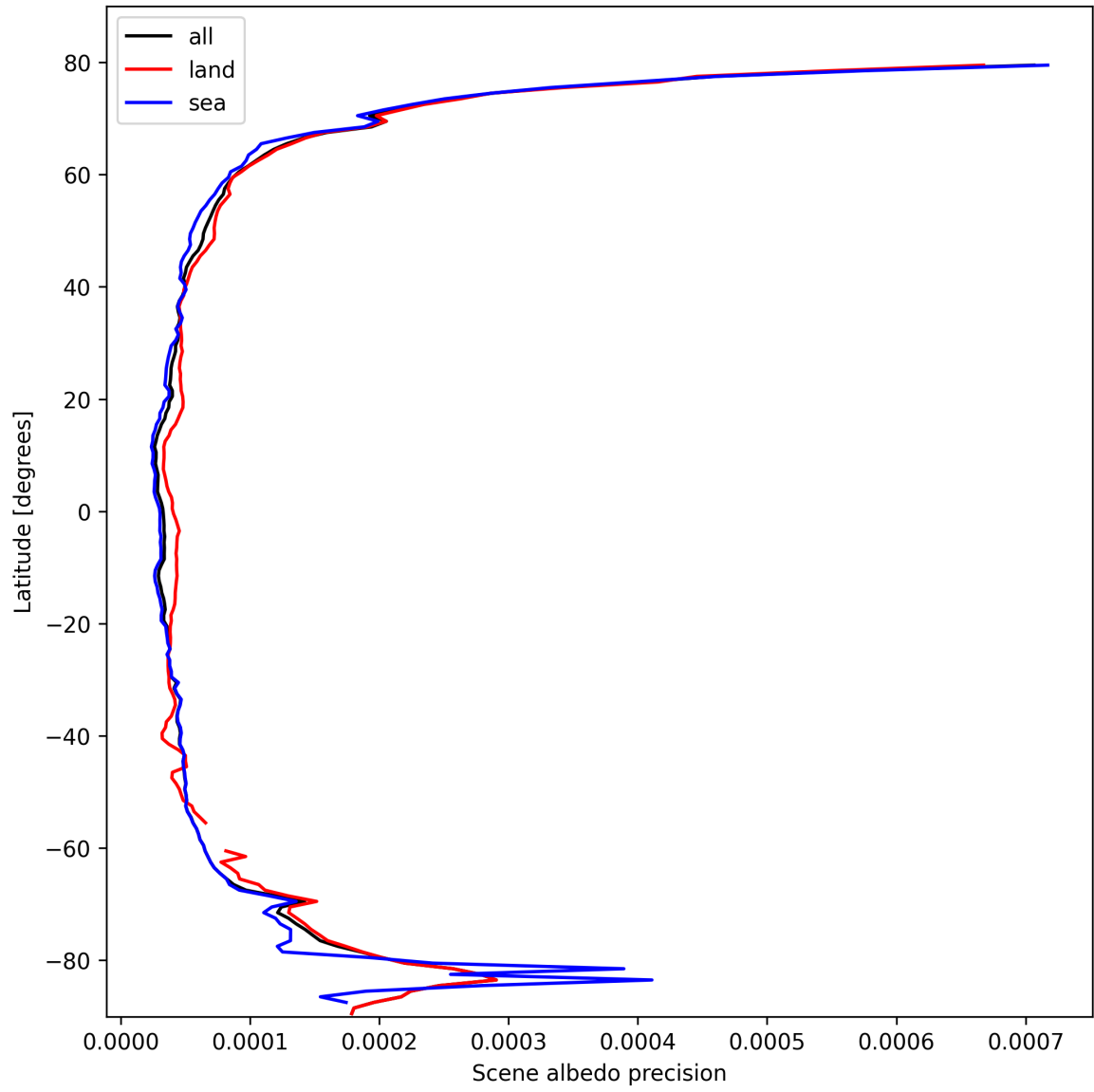
Figure 16: Zonal average of “Scene albedo precision” for 2025-02-25 to 2025-02-26.
