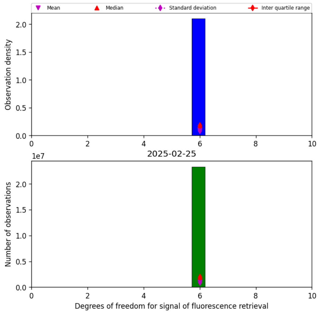
Figure 41: Histogram of “Degrees of freedom for signal of fluorescence retrieval” for 2025-02-25 to 2025-02-26
