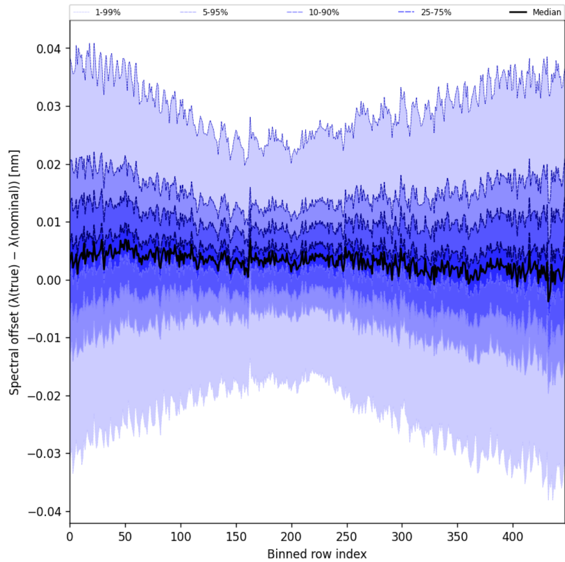
Figure 60: Along track statistics of “Spectral offset ( \lambda_{\text{true}} - \lambda_{\text{nominal}} )” for 2025-02-25 to 2025-02-26
