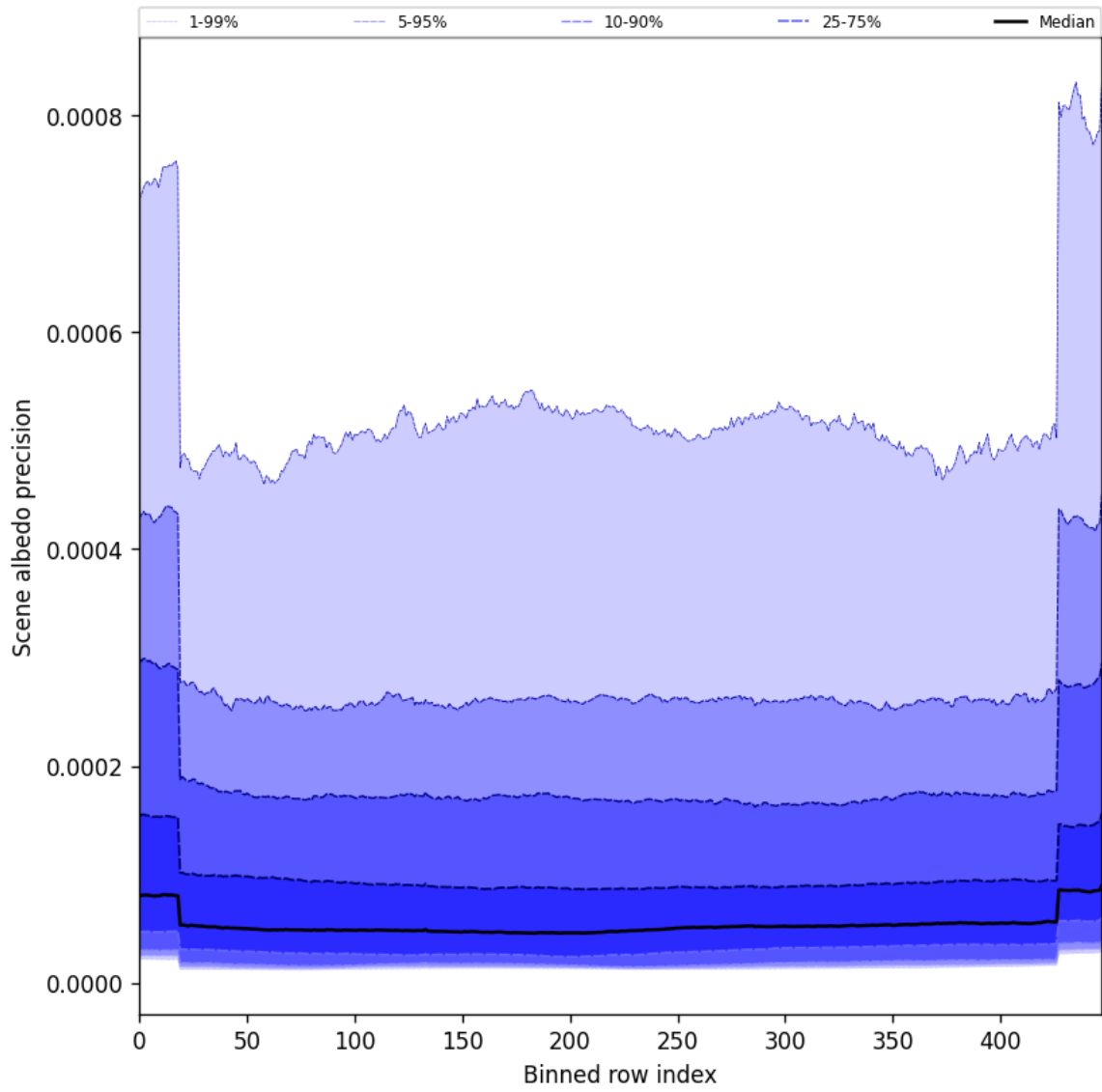
Figure 50: Along track statistics of “Scene albedo precision” for 2025-02-25 to 2025-02-26
