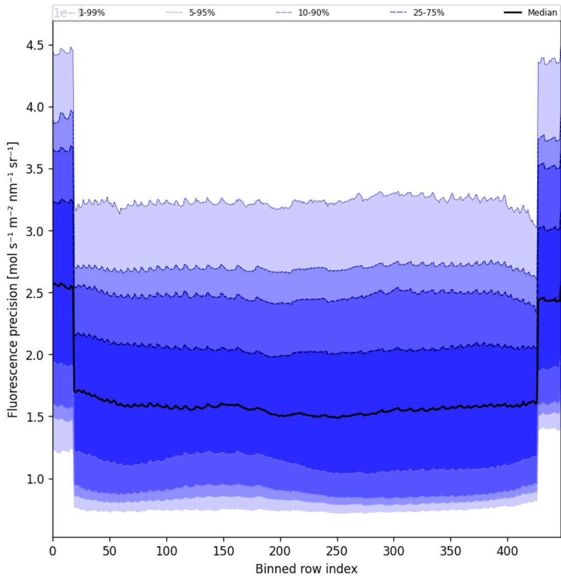
Figure 56: Along track statistics of “Fluorescence precision” for 2025-02-25 to 2025-02-26
