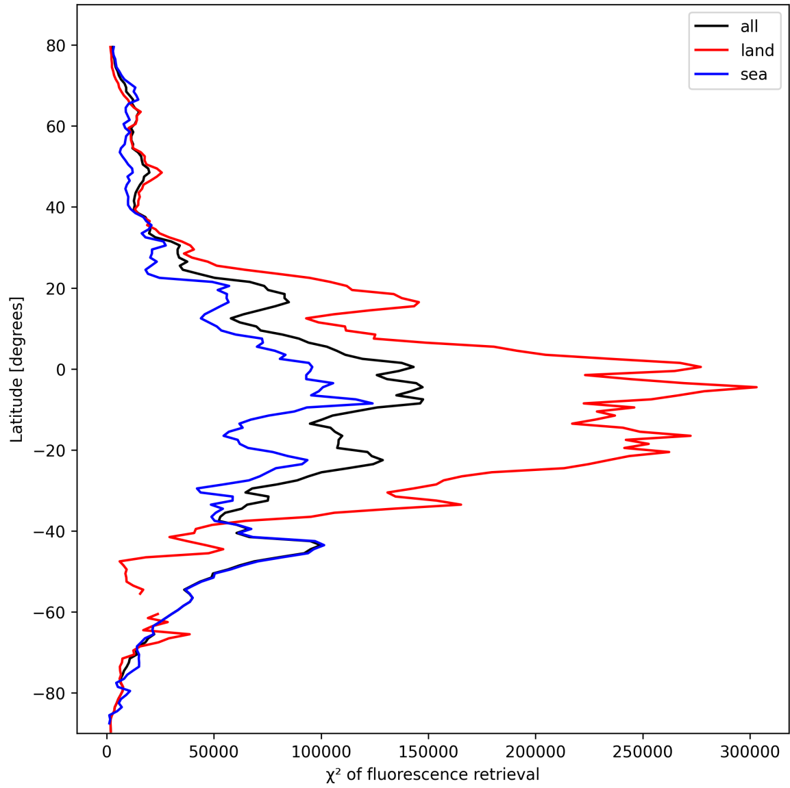
Figure 23: Zonal average of “ \chi^2 of fluorescence retrieval” for 2025-02-25 to 2025-02-26.
