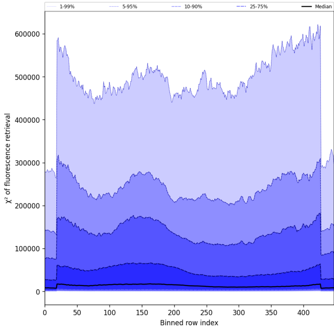
Figure 57: Along track statistics of “ \chi^2 of fluorescence retrieval” for 2025-02-25 to 2025-02-26
