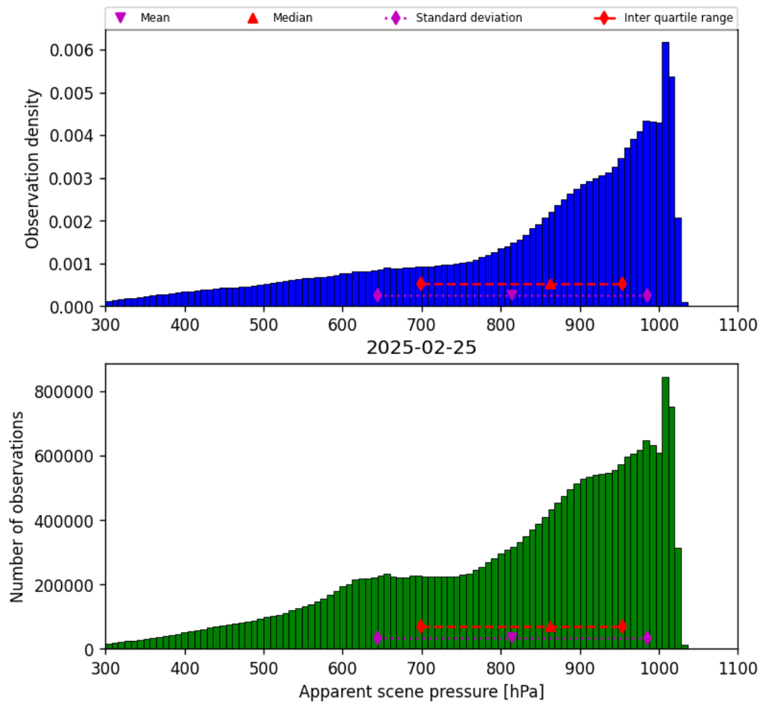
Figure 34: Histogram of “Apparent scene pressure” for 2025-02-25 to 2025-02-26
