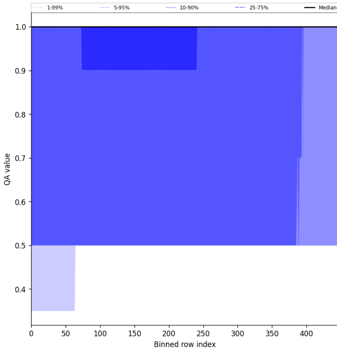
Figure 44: Along track statistics of “QA value” for 2025-02-25 to 2025-02-26
