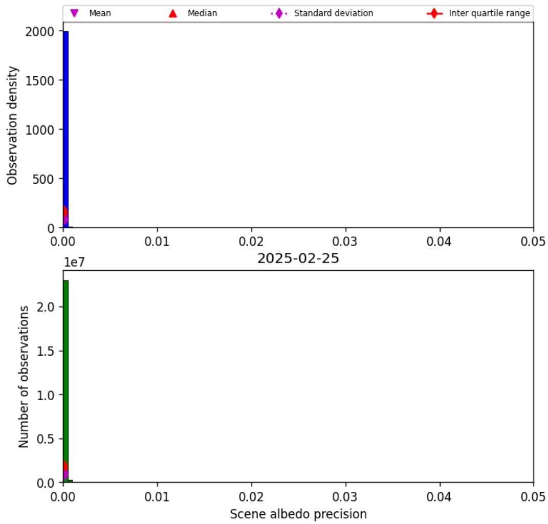
Figure 33: Histogram of “Scene albedo precision” for 2025-02-25 to 2025-02-26
