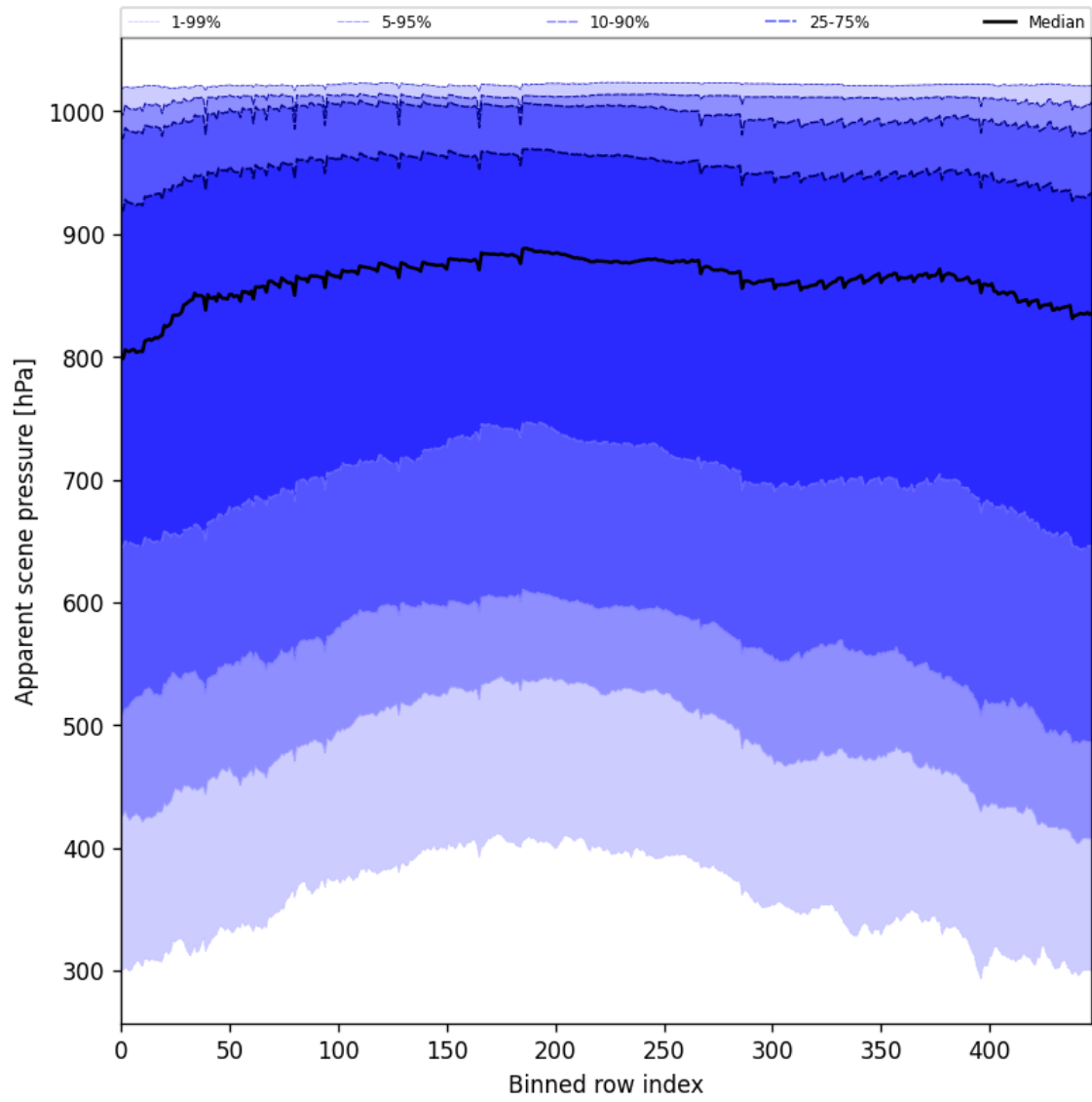
Figure 51: Along track statistics of “Apparent scene pressure” for 2025-02-25 to 2025-02-26
