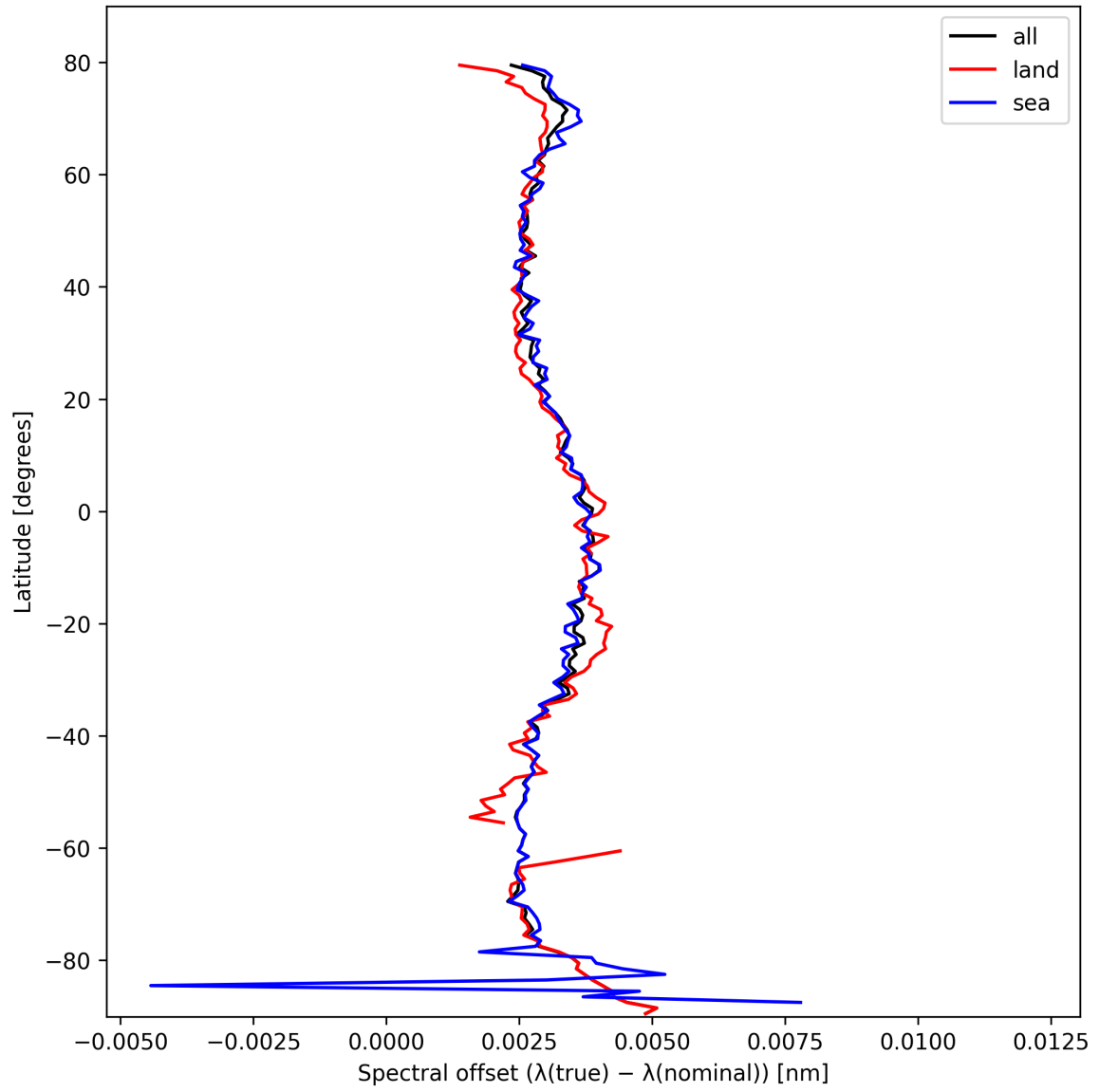
Figure 26: Zonal average of “Spectral offset ( \lambda_{\text{true}} - \lambda_{\text{nominal}} )” for 2025-02-25 to 2025-02-26.
