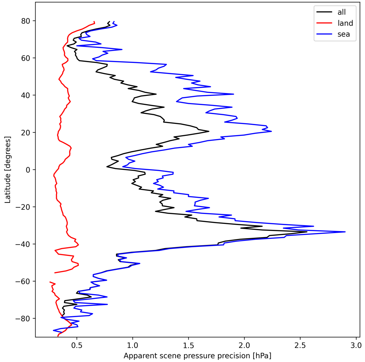
Figure 18: Zonal average of “Apparent scene pressure precision” for 2025-02-25 to 2025-02-26.
