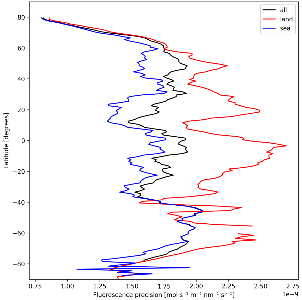
Figure 22: Zonal average of “Fluorescence precision” for 2025-02-25 to 2025-02-26.
