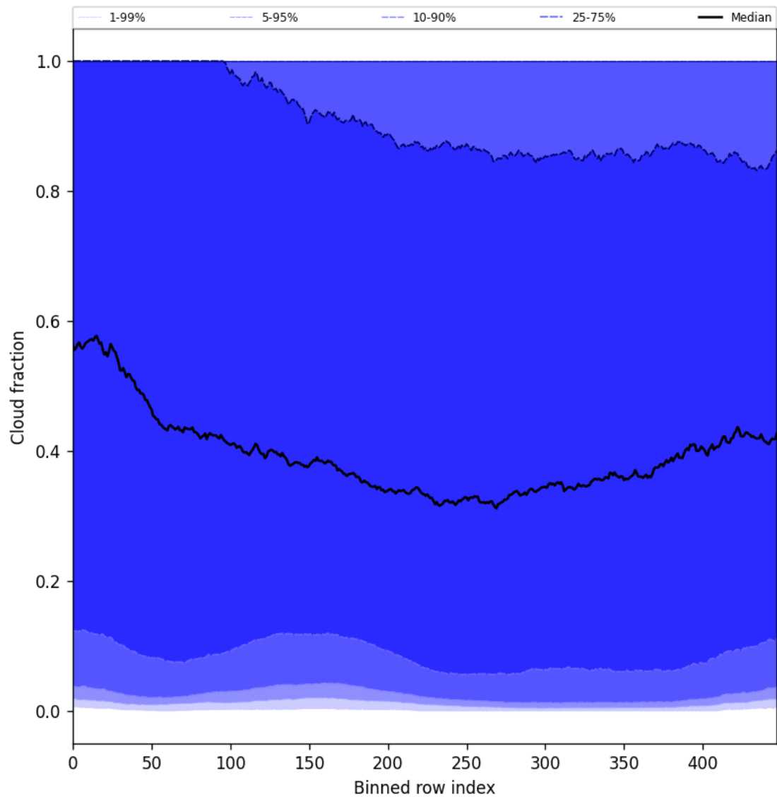
Figure 47: Along track statistics of “Cloud fraction” for 2025-02-25 to 2025-02-26
