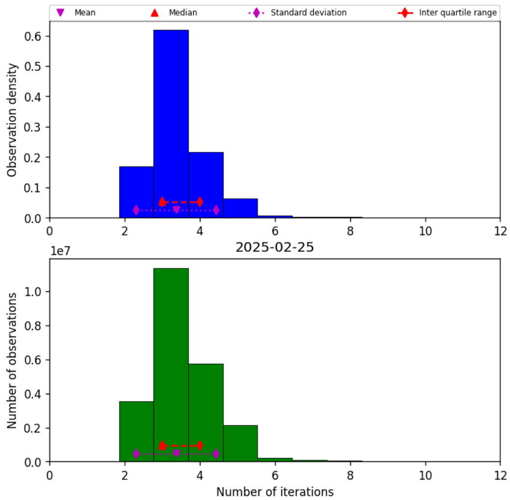
Figure 37: Histogram of “Number of iterations” for 2025-02-25 to 2025-02-26
