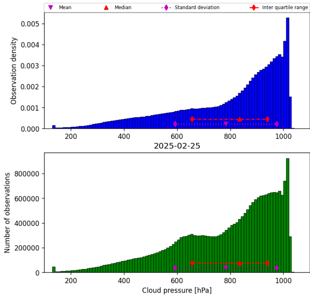
Figure 28: Histogram of “Cloud pressure” for 2025-02-25 to 2025-02-26
