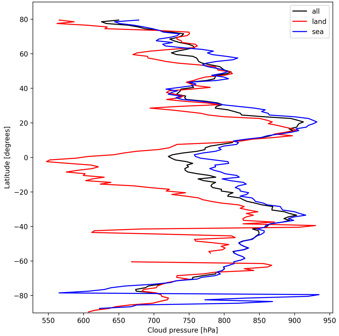
Figure 11: Zonal average of “Cloud pressure” for 2025-02-25 to 2025-02-26.
