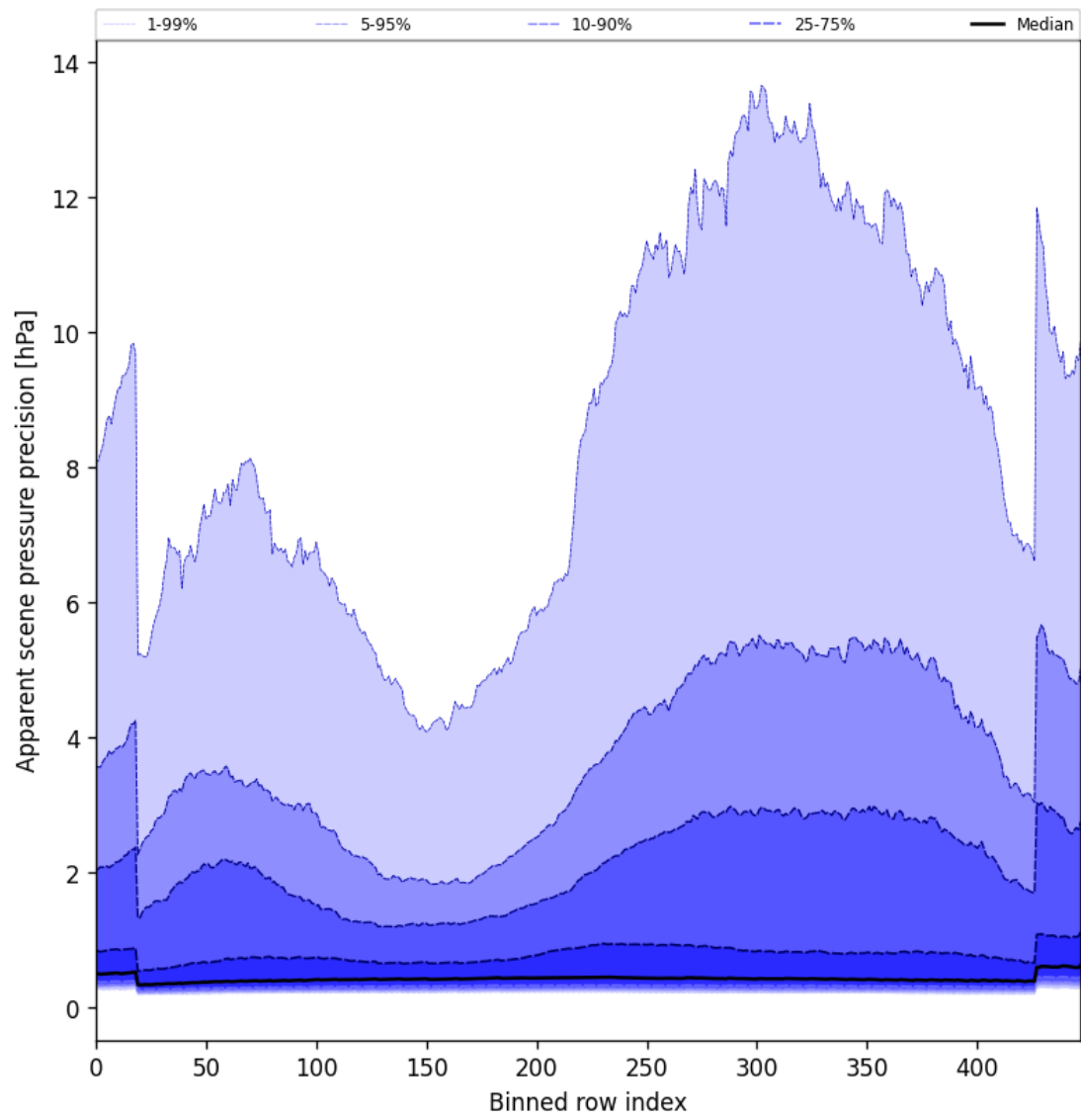
Figure 52: Along track statistics of “Apparent scene pressure precision” for 2025-02-25 to 2025-02-26
