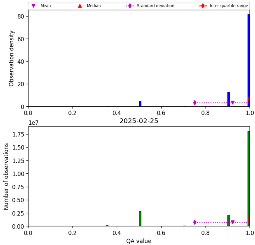
Figure 27: Histogram of “QA value” for 2025-02-25 to 2025-02-26
