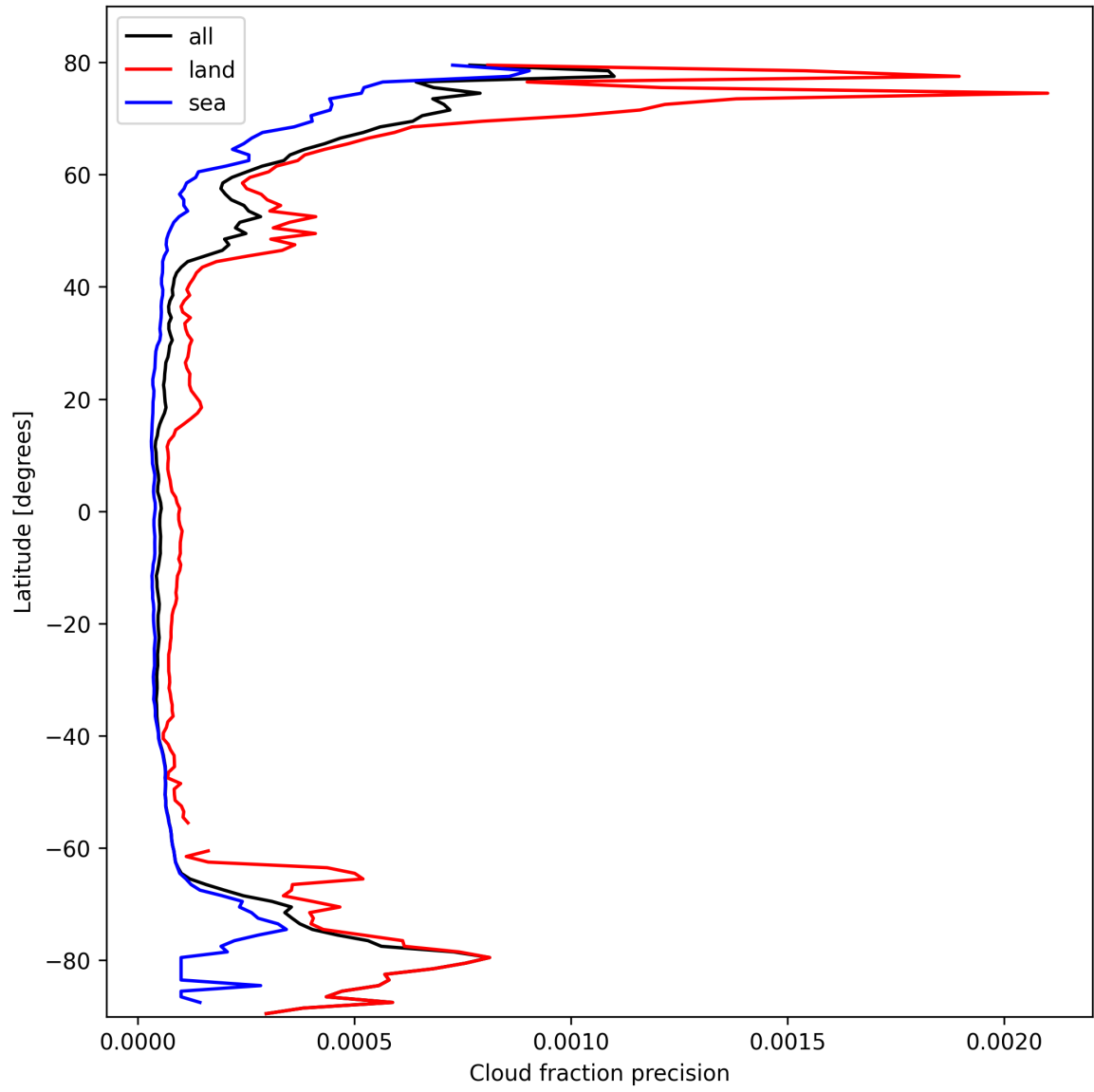
Figure 14: Zonal average of “Cloud fraction precision” for 2025-02-25 to 2025-02-26.
