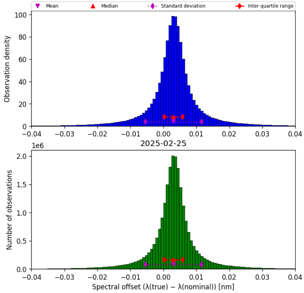
Figure 43: Histogram of “Spectral offset ( \lambda_{\text{true}} - \lambda_{\text{nominal}} )” for 2025-02-25 to 2025-02-26
