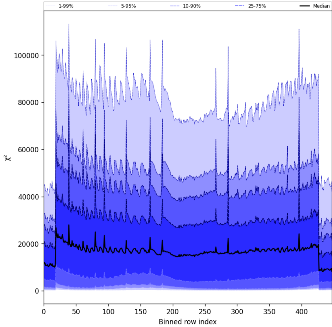
Figure 53: Along track statistics of “ \chi^2 ” for 2025-02-25 to 2025-02-26
