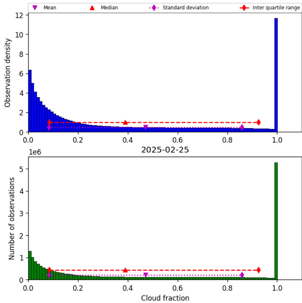
Figure 30: Histogram of “Cloud fraction” for 2025-02-25 to 2025-02-26
