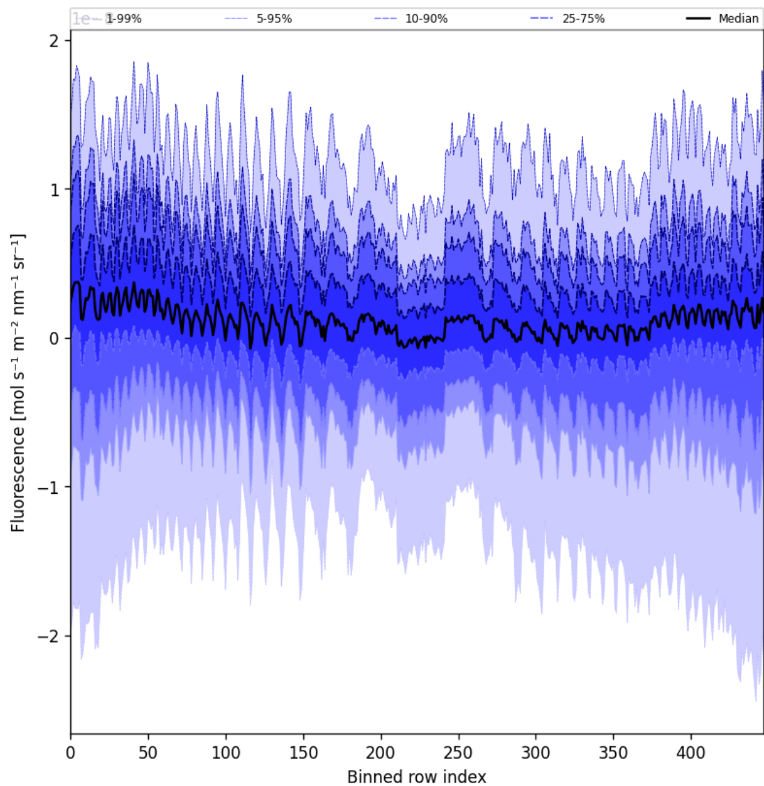
Figure 55: Along track statistics of “Fluorescence” for 2025-02-25 to 2025-02-26
