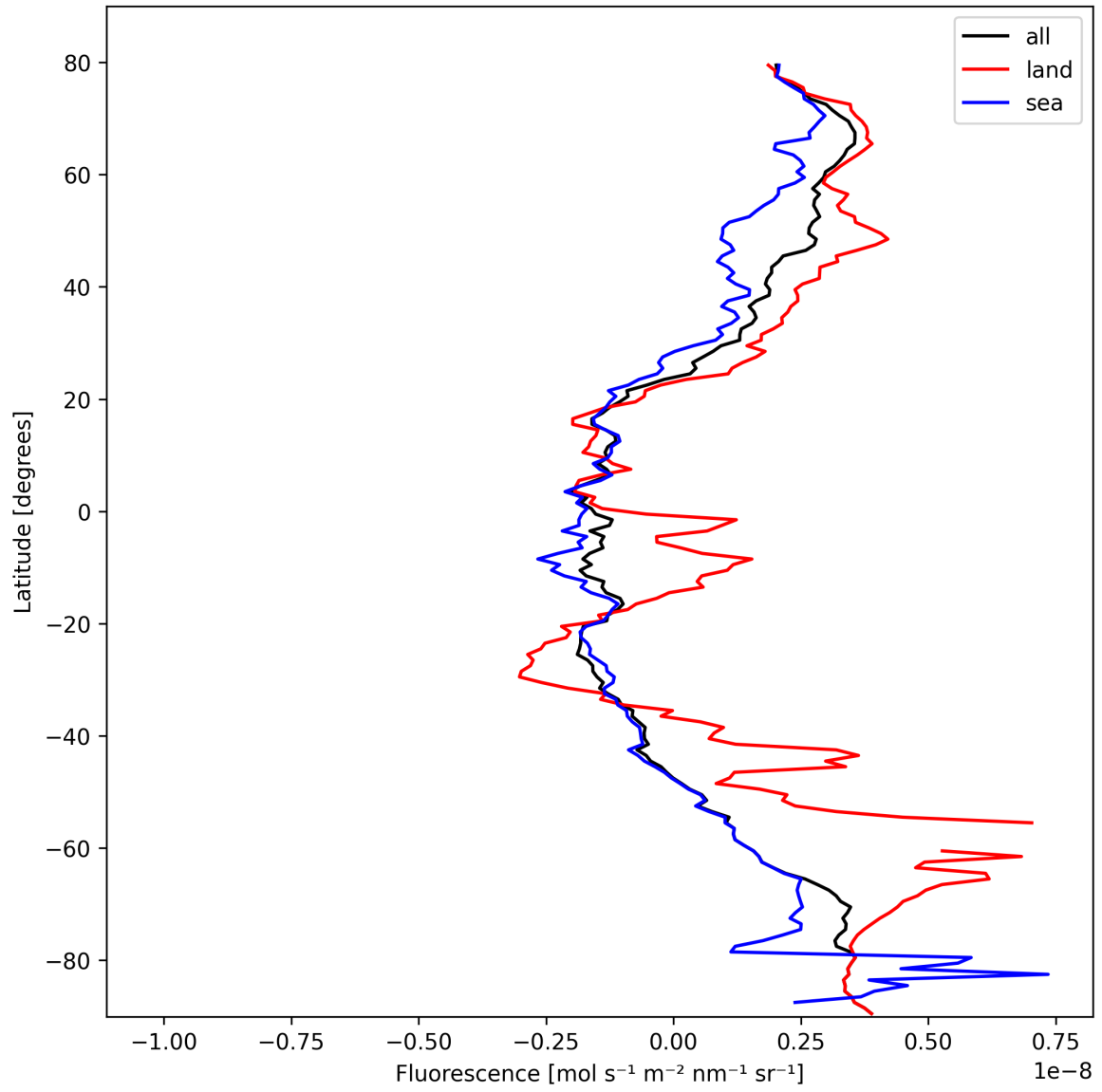
Figure 21: Zonal average of “Fluorescence” for 2025-02-25 to 2025-02-26.
