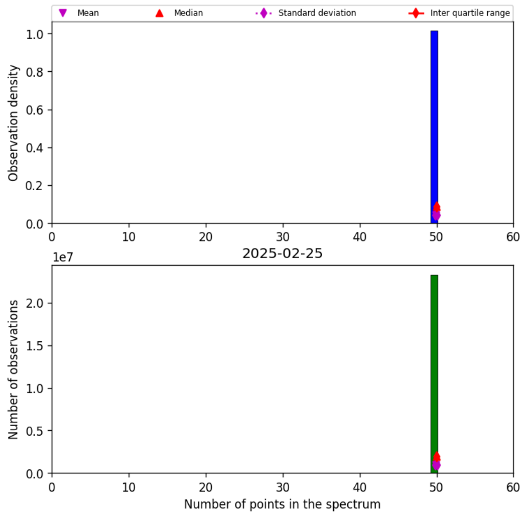
Figure 42: Histogram of “Number of points in the spectrum” for 2025-02-25 to 2025-02-26
