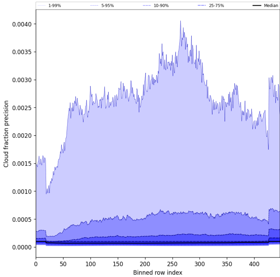
Figure 48: Along track statistics of “Cloud fraction precision” for 2025-02-25 to 2025-02-26
