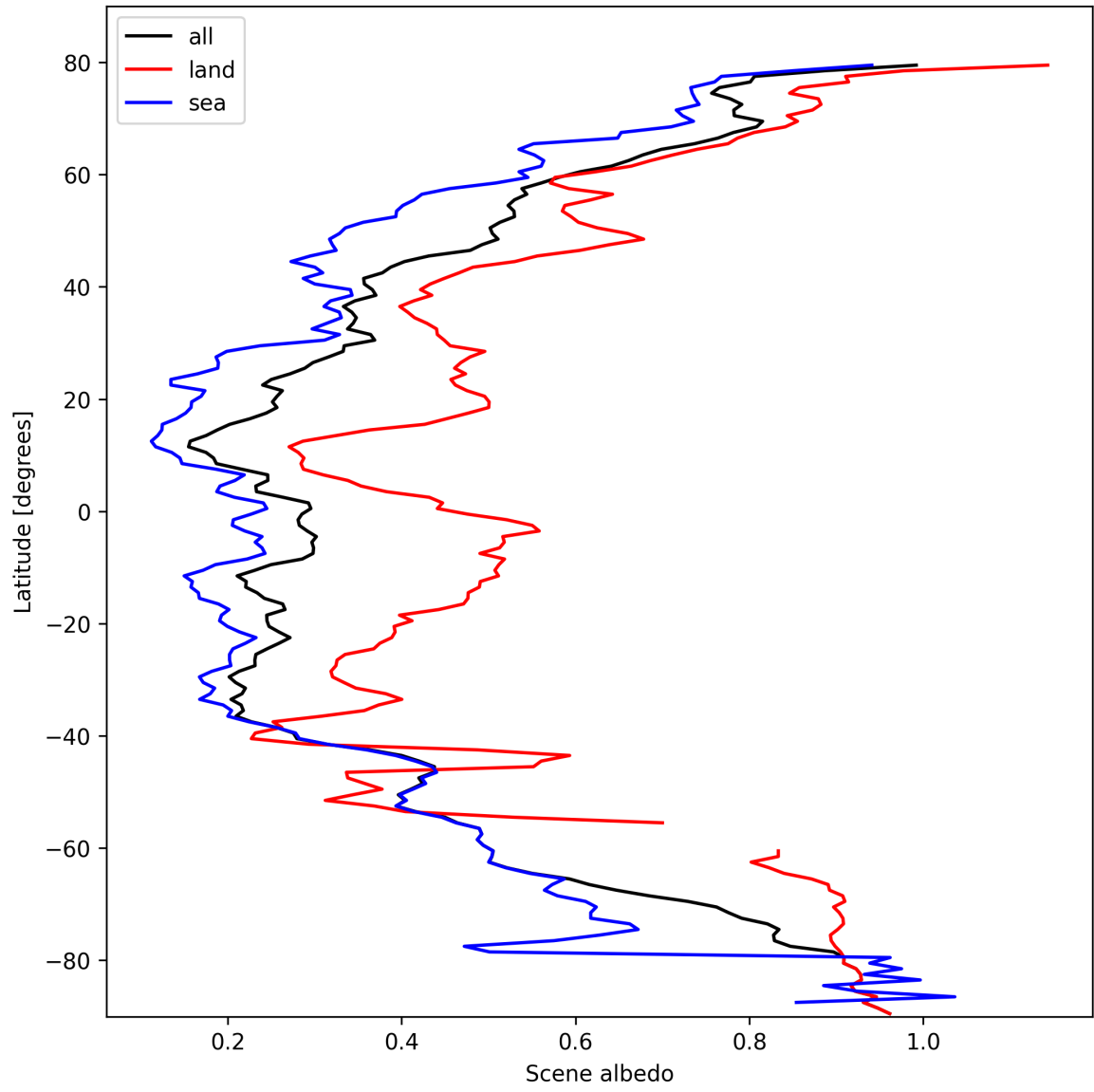
Figure 15: Zonal average of “Scene albedo” for 2025-02-25 to 2025-02-26.
