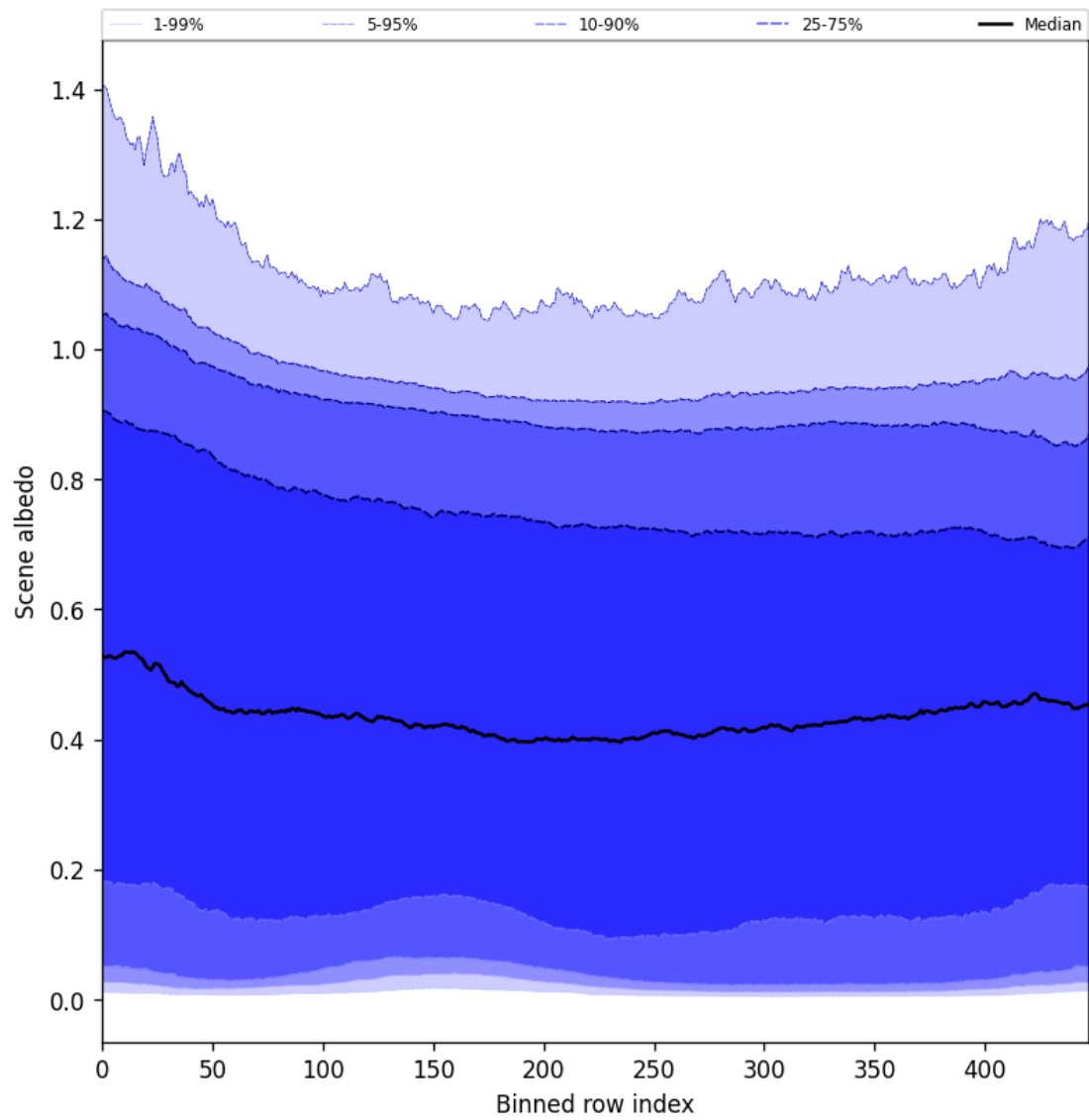
Figure 49: Along track statistics of “Scene albedo” for 2025-02-25 to 2025-02-26
