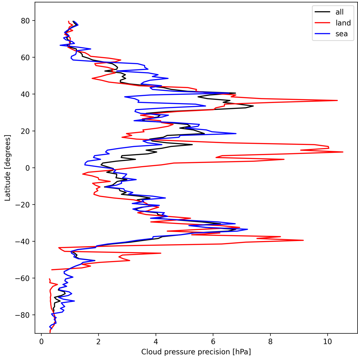
Figure 12: Zonal average of “Cloud pressure precision” for 2025-02-25 to 2025-02-26.
