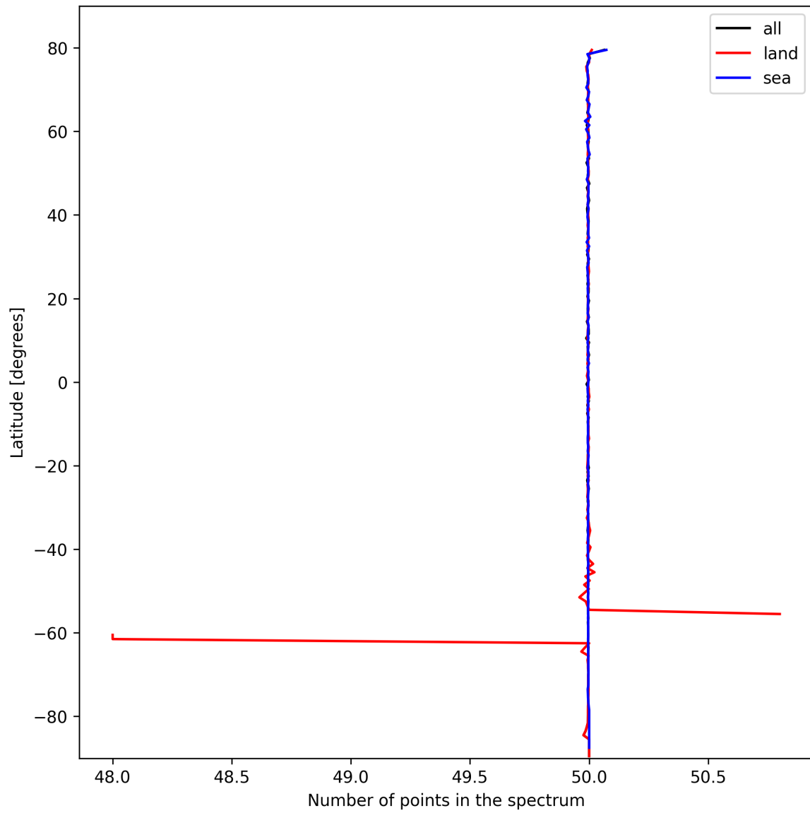
Figure 25: Zonal average of “Number of points in the spectrum” for 2025-02-25 to 2025-02-26.
