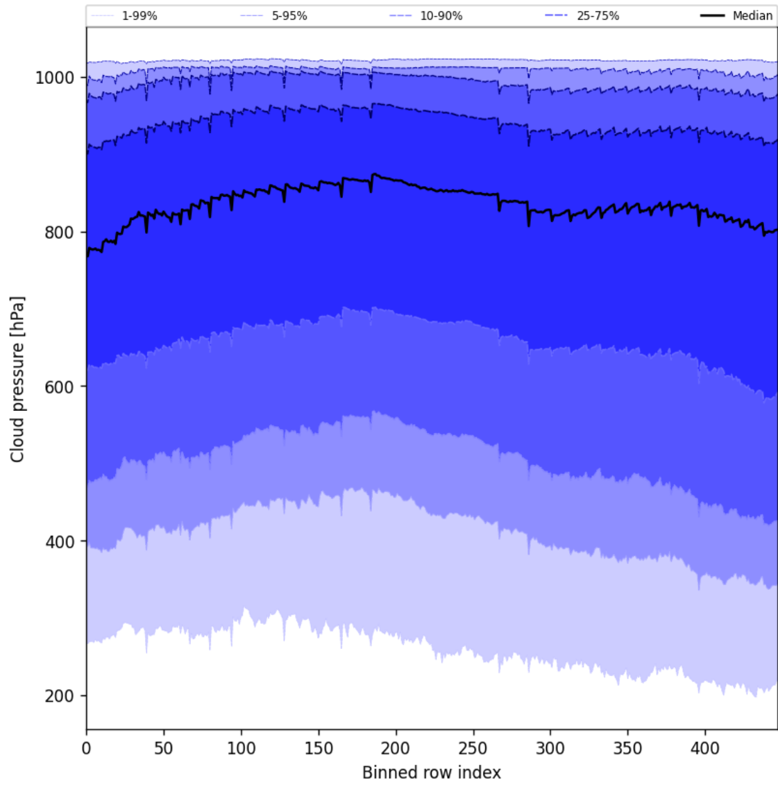
Figure 45: Along track statistics of “Cloud pressure” for 2025-02-25 to 2025-02-26
