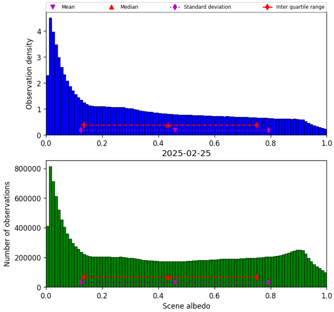
Figure 32: Histogram of “Scene albedo” for 2025-02-25 to 2025-02-26
