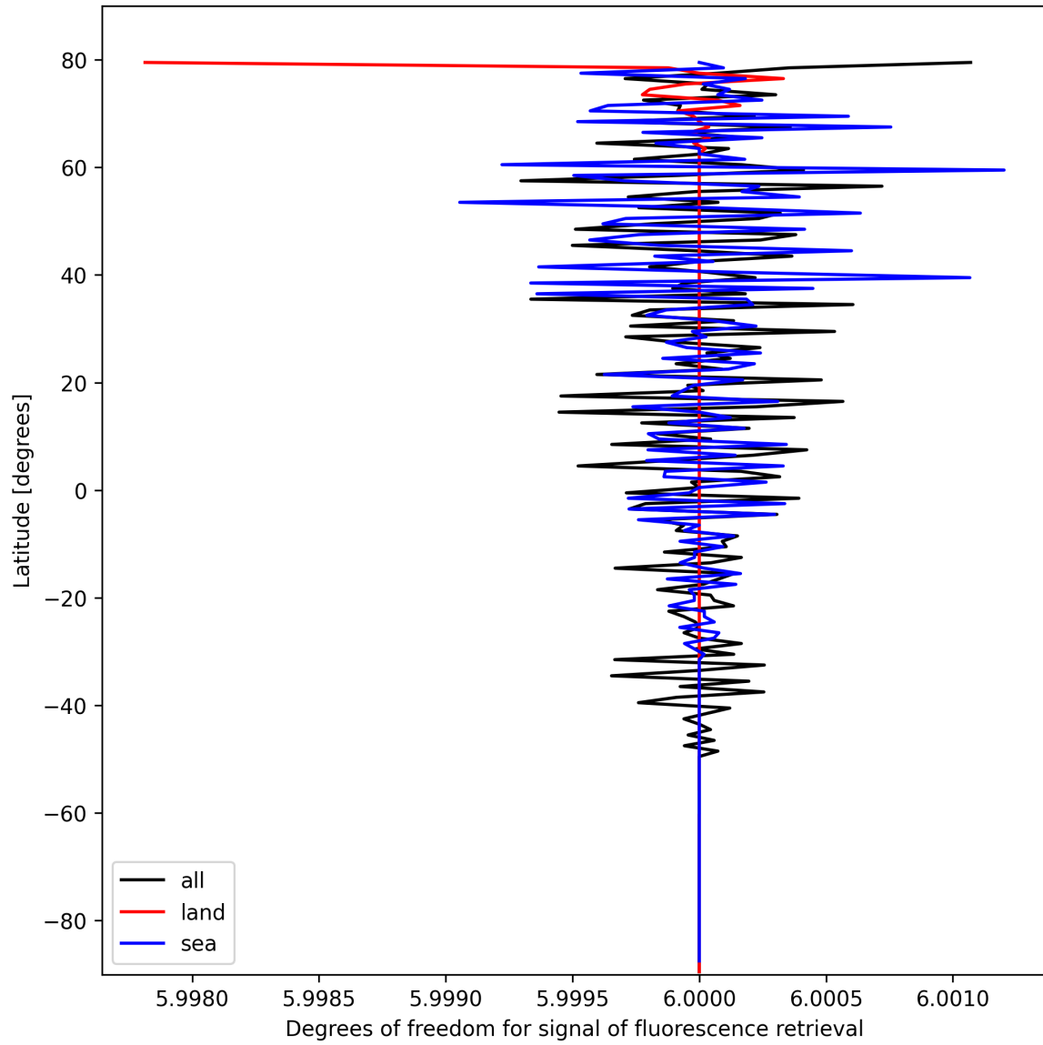
Figure 24: Zonal average of “Degrees of freedom for signal of fluorescence retrieval” for 2025-02-25 to 2025-02-26.
