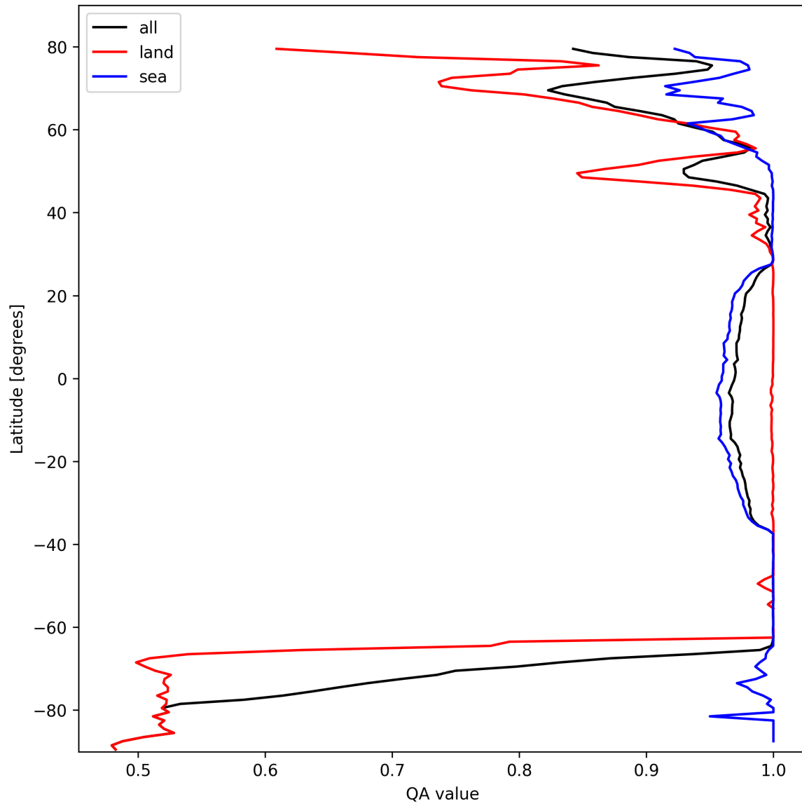
Figure 10: Zonal average of "QA value" for 2025-02-25 to 2025-02-26.
