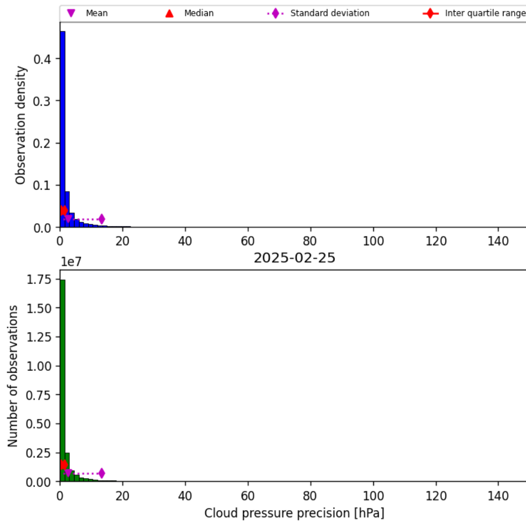
Figure 29: Histogram of “Cloud pressure precision” for 2025-02-25 to 2025-02-26
