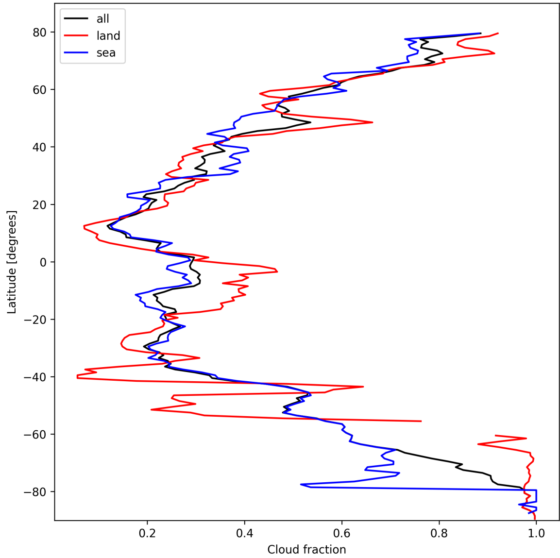
Figure 13: Zonal average of “Cloud fraction” for 2025-02-25 to 2025-02-26.
