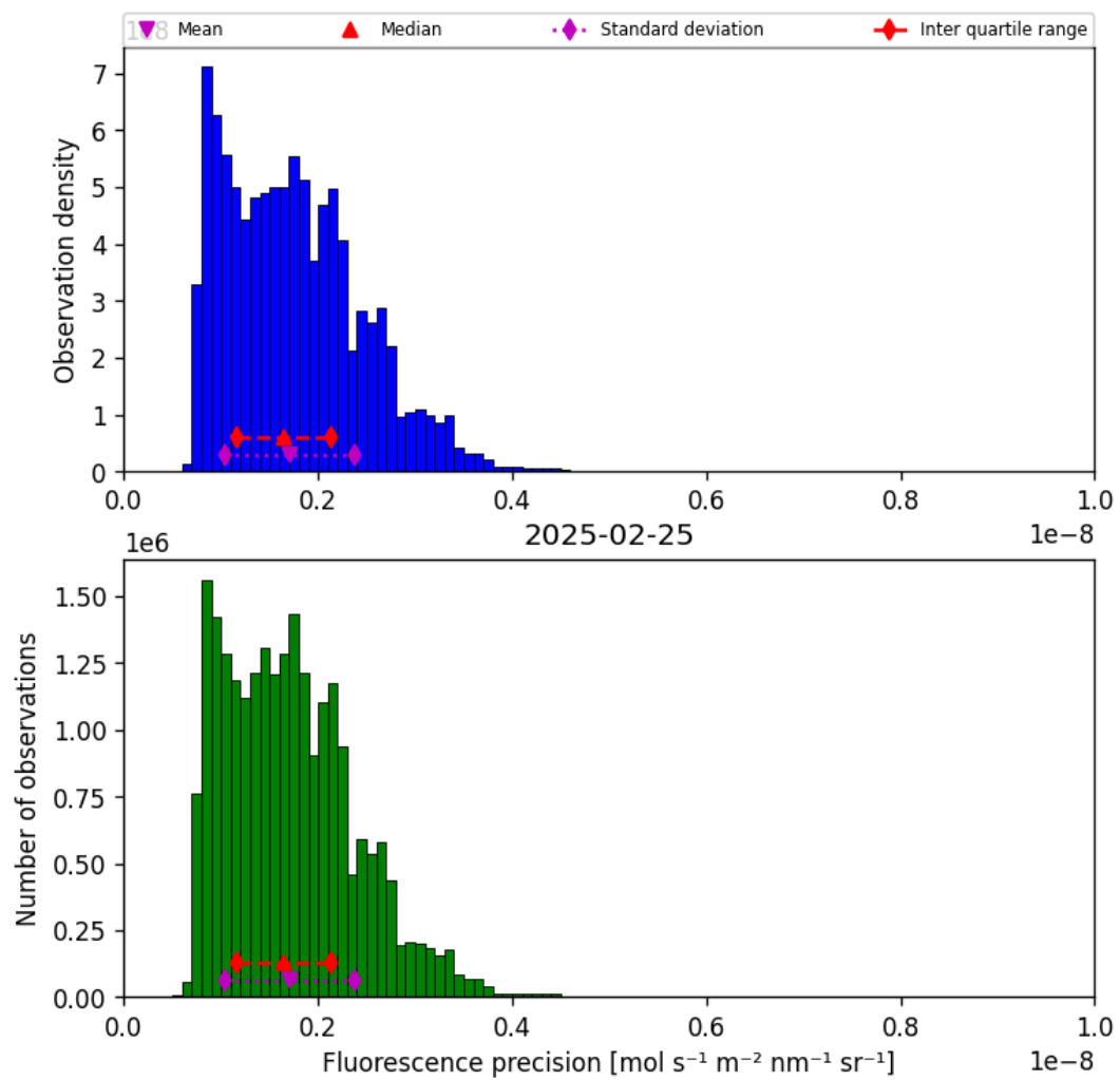
Figure 39: Histogram of “Fluorescence precision” for 2025-02-25 to 2025-02-26
