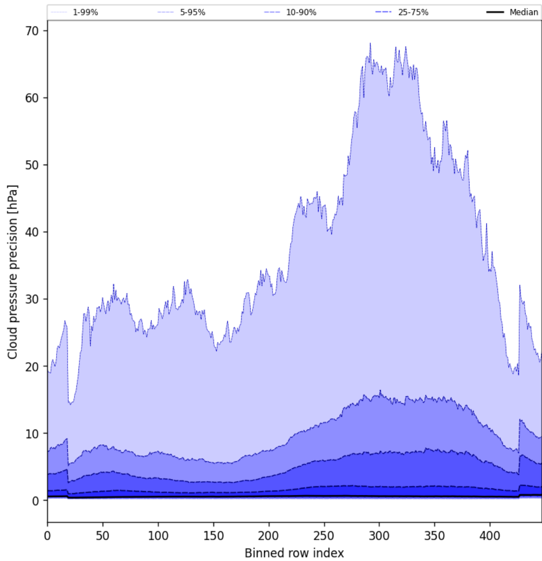
Figure 46: Along track statistics of “Cloud pressure precision” for 2025-02-25 to 2025-02-26
