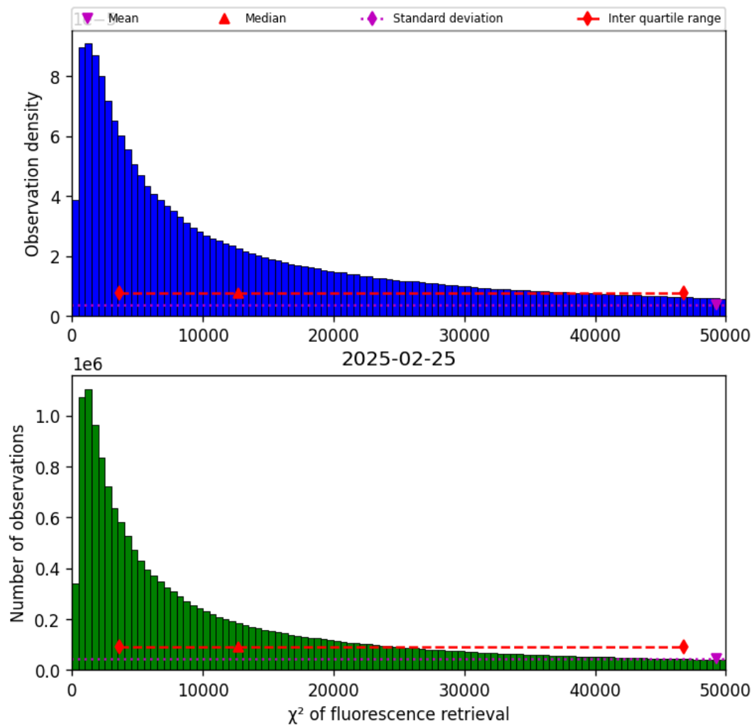
Figure 40: Histogram of “ \chi^2 of fluorescence retrieval” for 2025-02-25 to 2025-02-26
