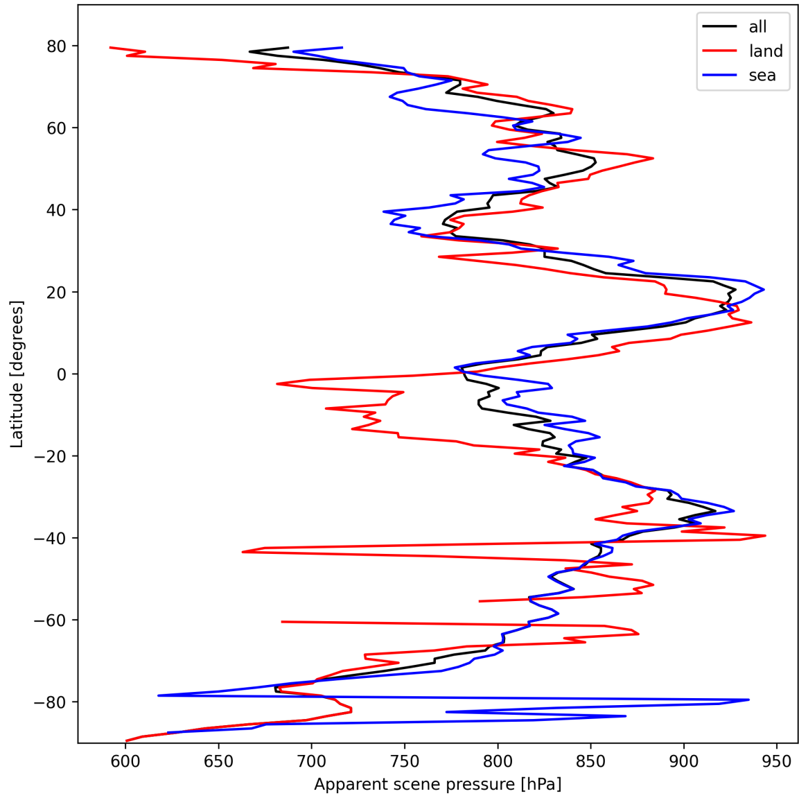
Figure 17: Zonal average of “Apparent scene pressure” for 2025-02-25 to 2025-02-26.
