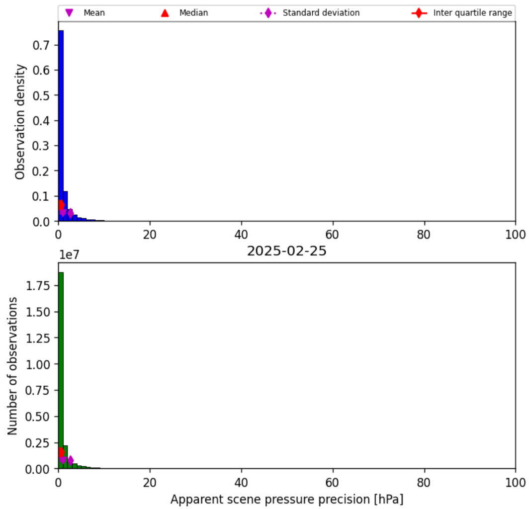
Figure 35: Histogram of “Apparent scene pressure precision” for 2025-02-25 to 2025-02-26
