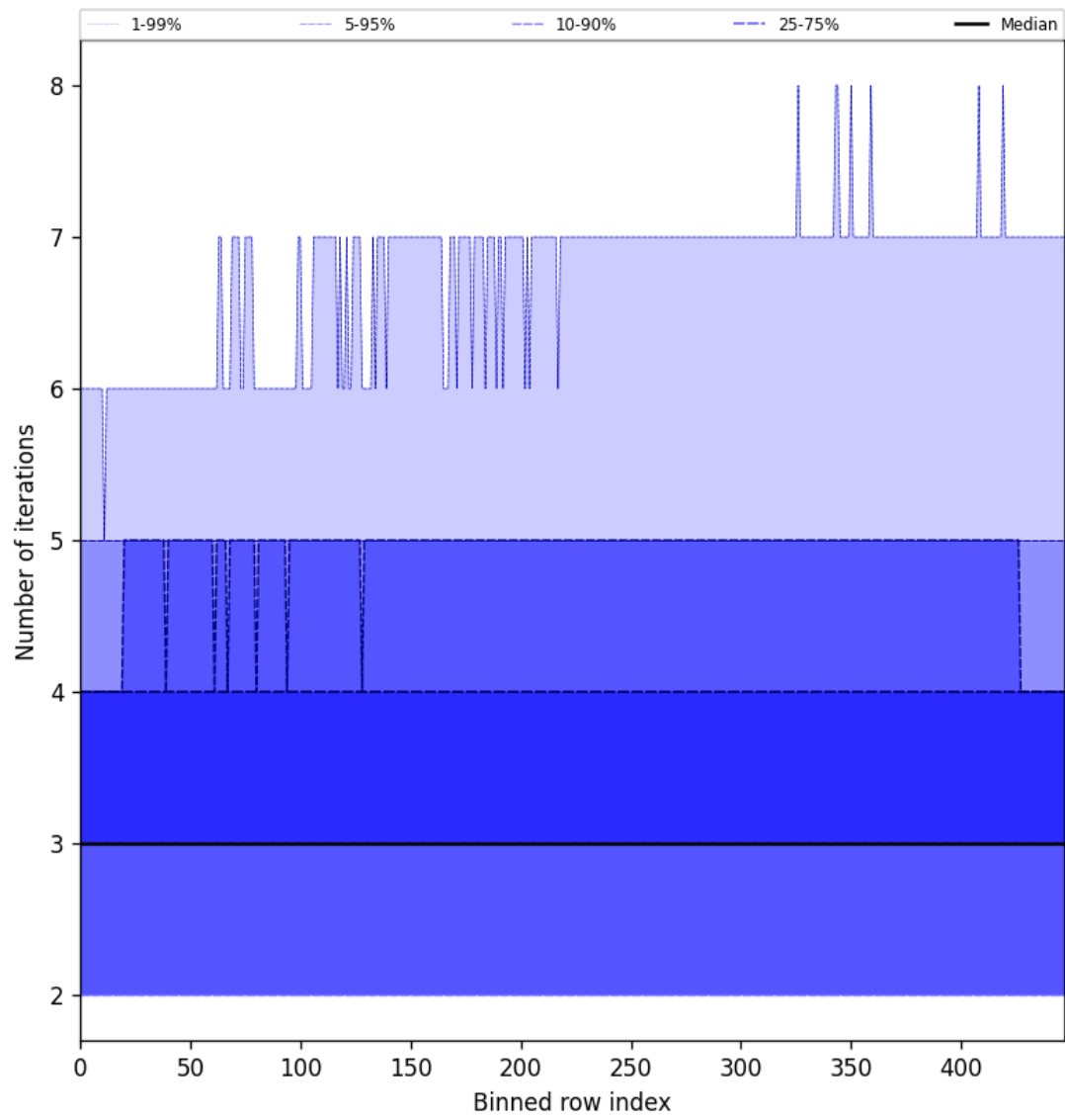
Figure 54: Along track statistics of “Number of iterations” for 2025-02-25 to 2025-02-26
