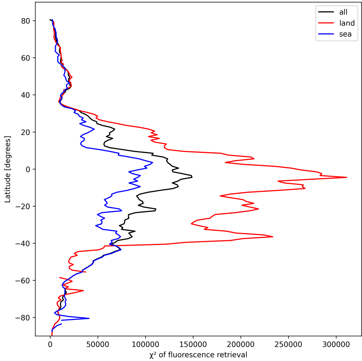
Figure 23: Zonal average of “ \chi^2 of fluorescence retrieval” for 2025-02-27 to 2025-02-27.
