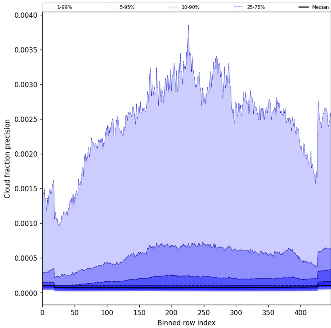
Figure 48: Along track statistics of “Cloud fraction precision” for 2025-02-27 to 2025-02-27
