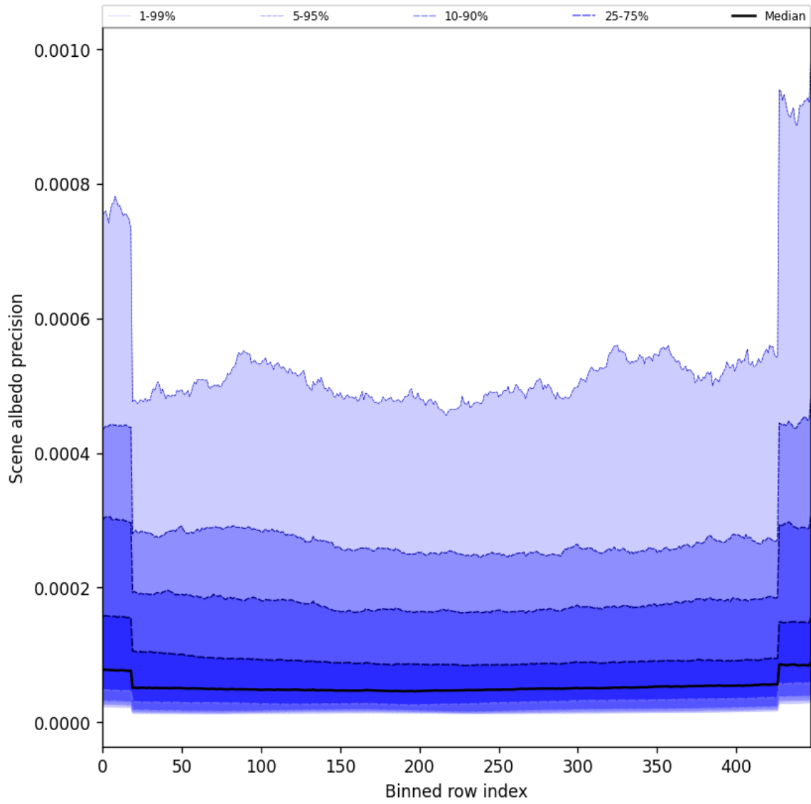
Figure 50: Along track statistics of “Scene albedo precision” for 2025-02-27 to 2025-02-27
