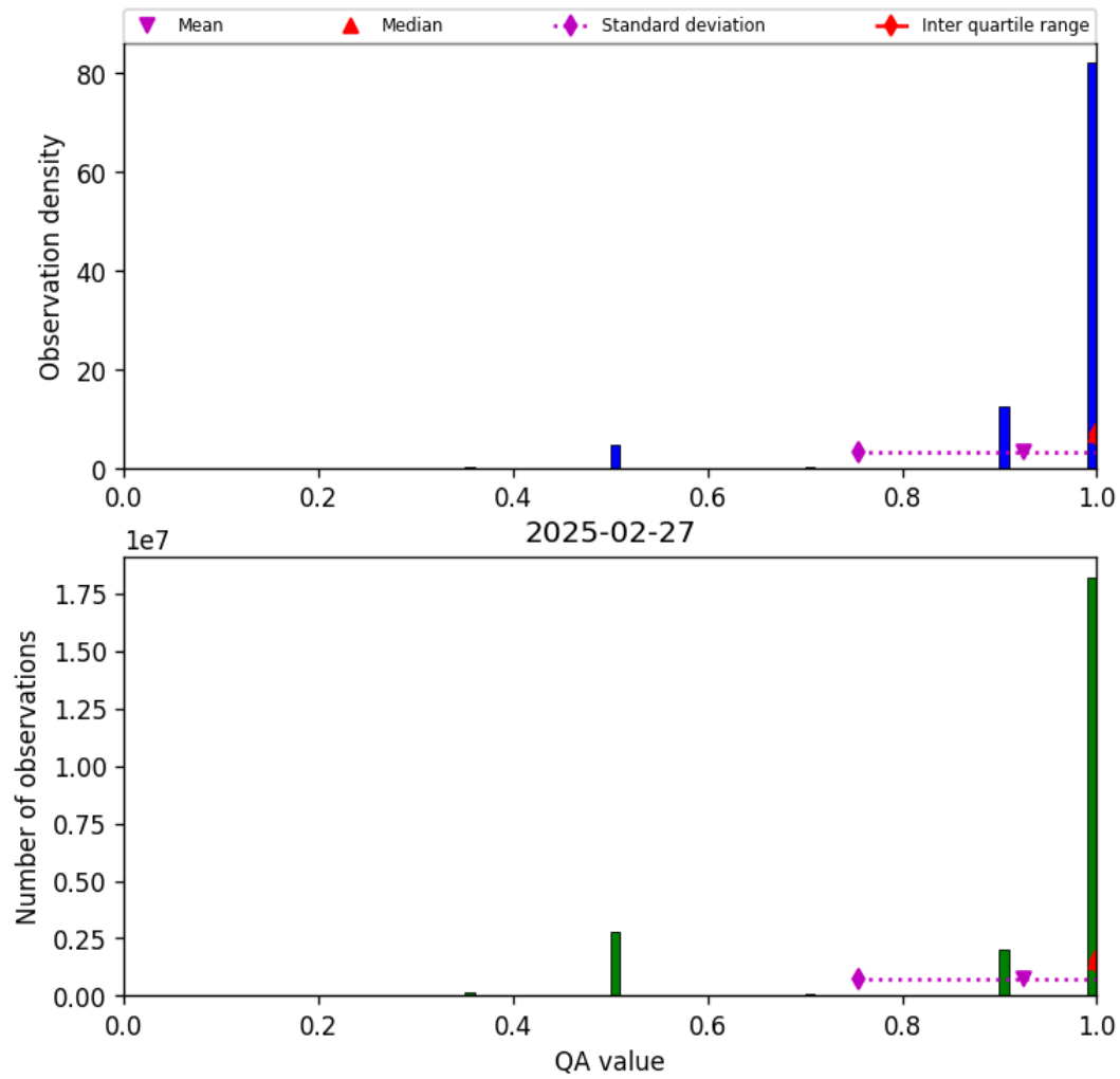
Figure 27: Histogram of “QA value” for 2025-02-27 to 2025-02-27
