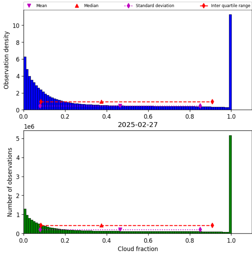
Figure 30: Histogram of “Cloud fraction” for 2025-02-27 to 2025-02-27
