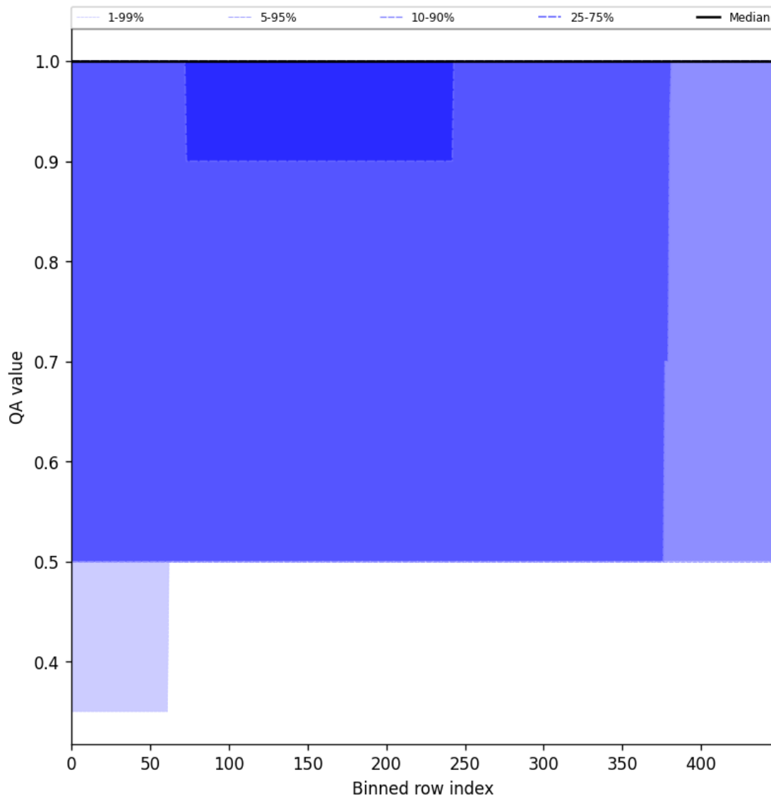
Figure 44: Along track statistics of “QA value” for 2025-02-27 to 2025-02-27
