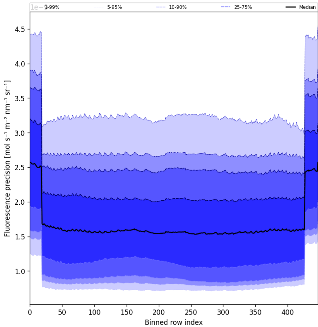
Figure 56: Along track statistics of “Fluorescence precision” for 2025-02-27 to 2025-02-27
