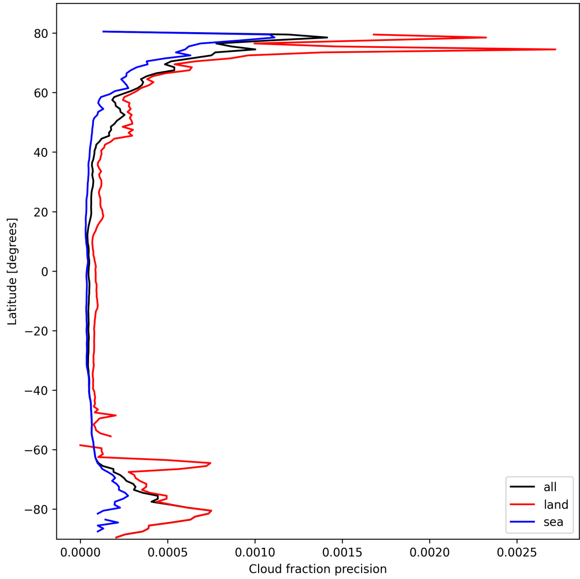
Figure 14: Zonal average of “Cloud fraction precision” for 2025-02-27 to 2025-02-27.
