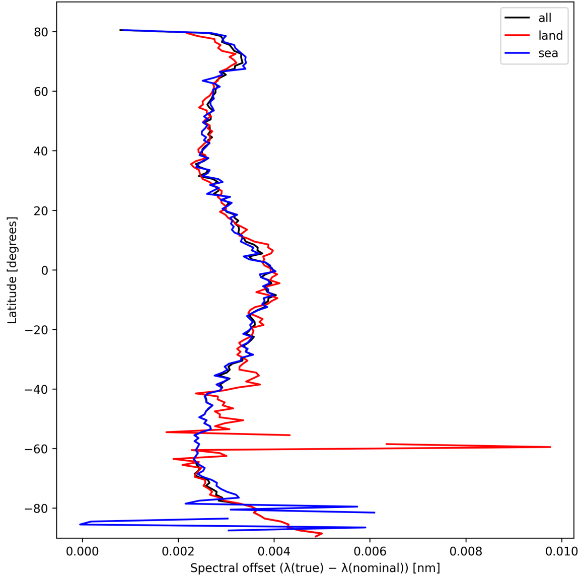
Figure 26: Zonal average of “Spectral offset ( \lambda_{\text{true}} - \lambda_{\text{nominal}} )” for 2025-02-27 to 2025-02-27.
