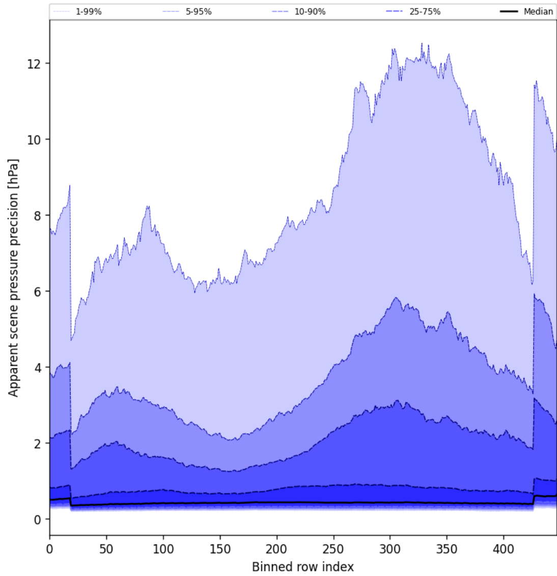
Figure 52: Along track statistics of “Apparent scene pressure precision” for 2025-02-27 to 2025-02-27
