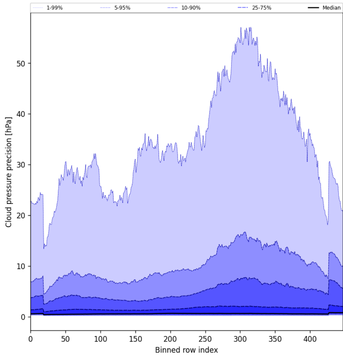
Figure 46: Along track statistics of “Cloud pressure precision” for 2025-02-27 to 2025-02-27
