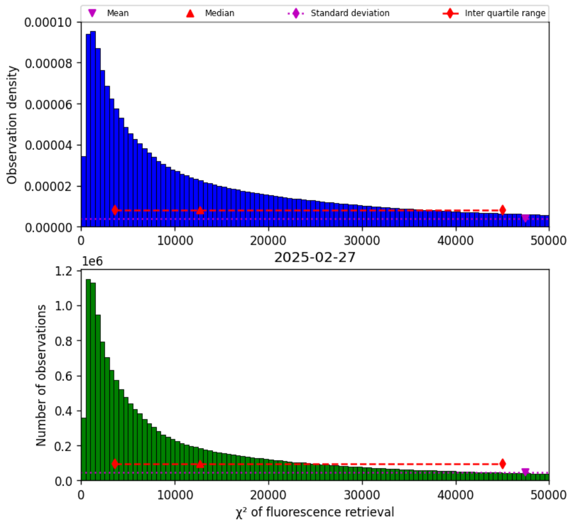
Figure 40: Histogram of “ \chi^2 of fluorescence retrieval” for 2025-02-27 to 2025-02-27
