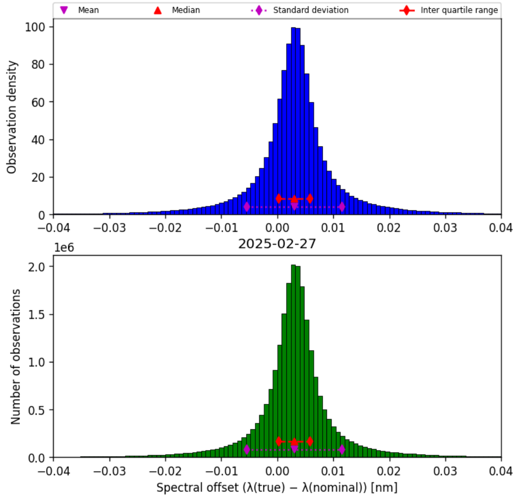
Figure 43: Histogram of “Spectral offset ( \lambda_{\text{true}} - \lambda_{\text{nominal}} )” for 2025-02-27 to 2025-02-27
