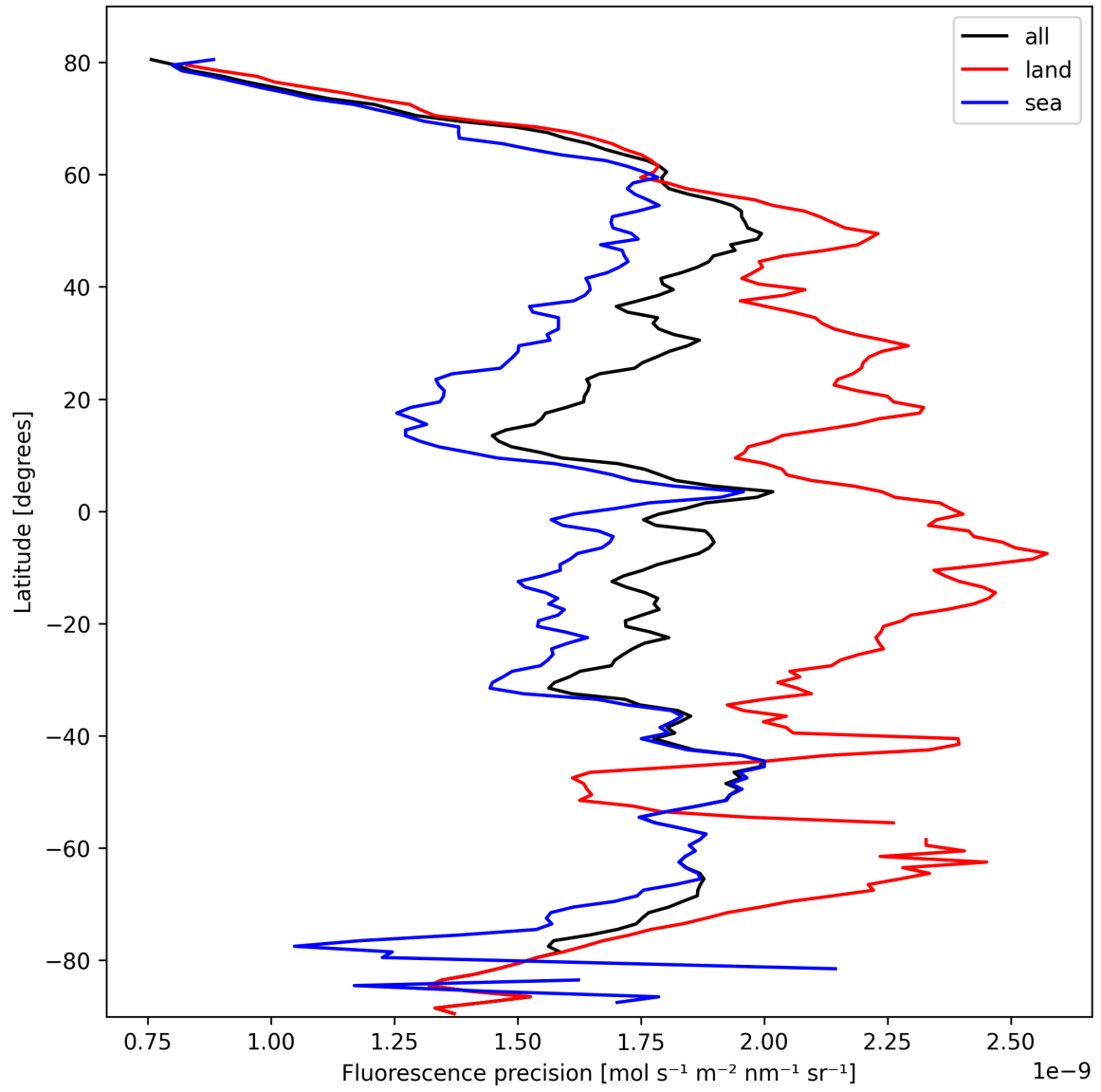
Figure 22: Zonal average of “Fluorescence precision” for 2025-02-27 to 2025-02-27.
