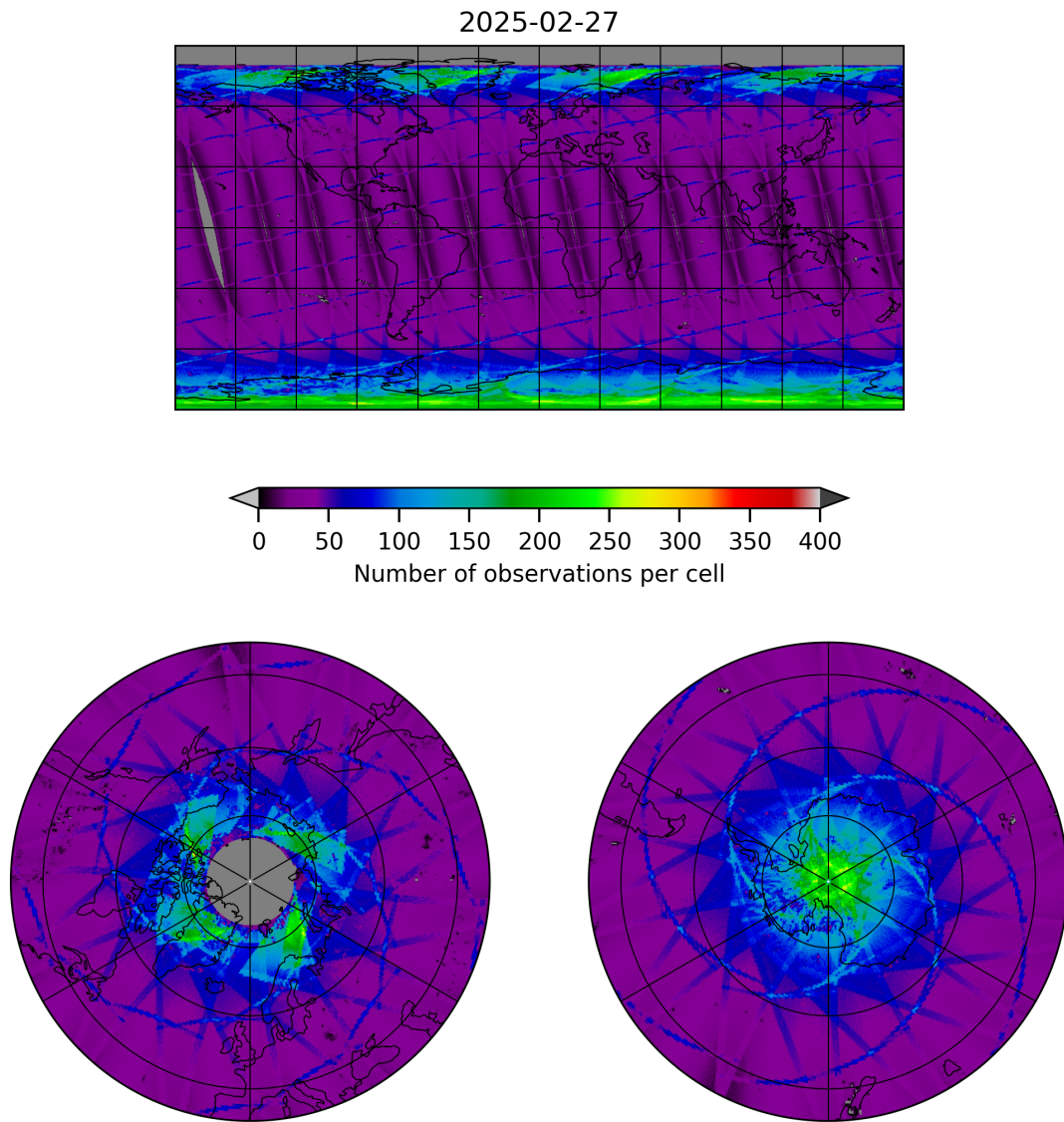
Figure 9: Map of the number of observations for 2025-02-27 to 2025-02-27
