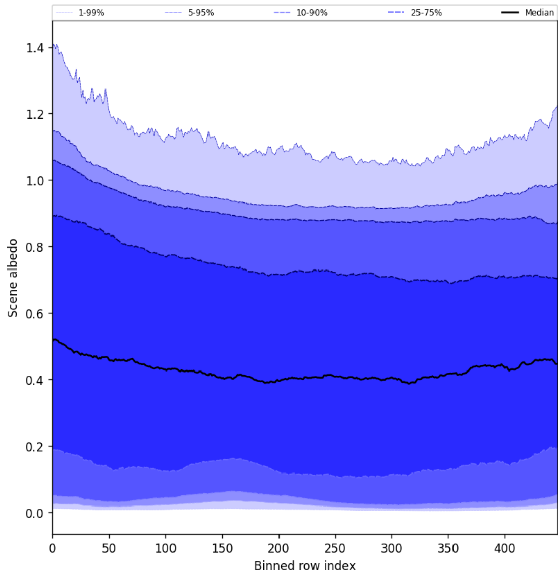
Figure 49: Along track statistics of “Scene albedo” for 2025-02-27 to 2025-02-27
