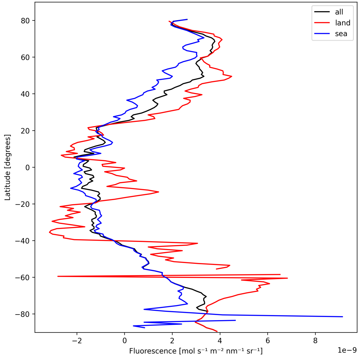
Figure 21: Zonal average of “Fluorescence” for 2025-02-27 to 2025-02-27.
