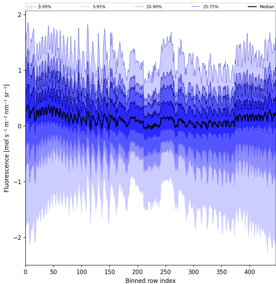
Figure 55: Along track statistics of “Fluorescence” for 2025-02-27 to 2025-02-27
