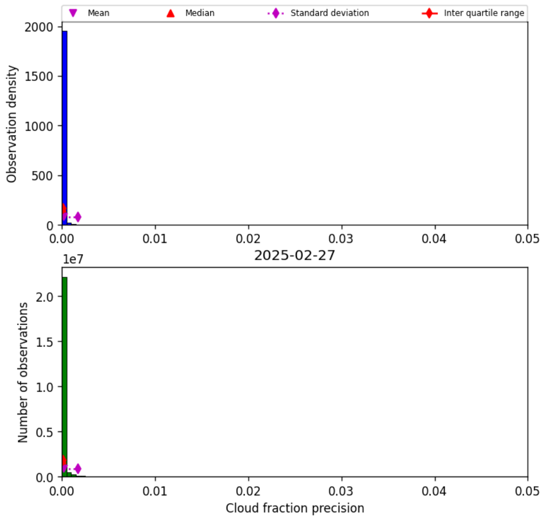
Figure 31: Histogram of “Cloud fraction precision” for 2025-02-27 to 2025-02-27
