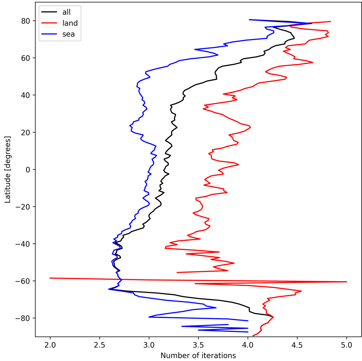
Figure 20: Zonal average of “Number of iterations” for 2025-02-27 to 2025-02-27.
