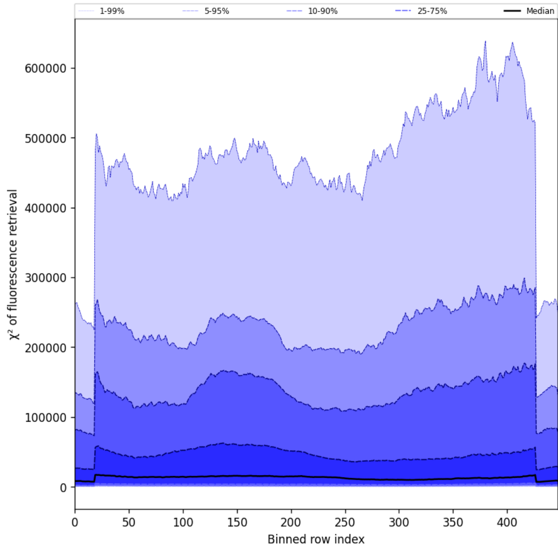
Figure 57: Along track statistics of “ \chi^2 of fluorescence retrieval” for 2025-02-27 to 2025-02-27
