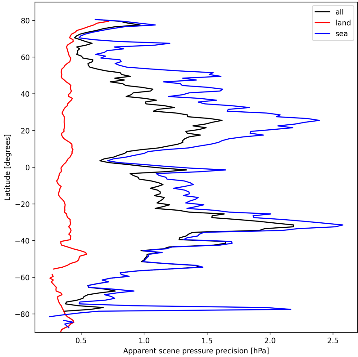
Figure 18: Zonal average of “Apparent scene pressure precision” for 2025-02-27 to 2025-02-27.
