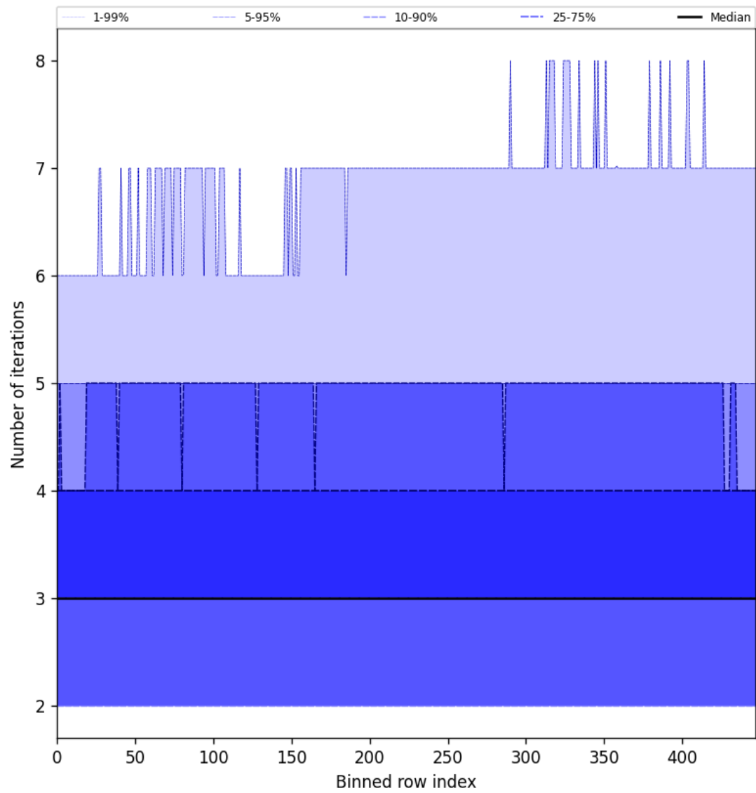
Figure 54: Along track statistics of “Number of iterations” for 2025-02-27 to 2025-02-27
