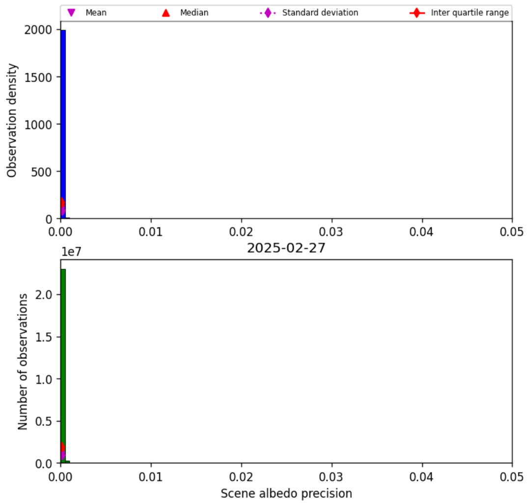
Figure 33: Histogram of “Scene albedo precision” for 2025-02-27 to 2025-02-27
