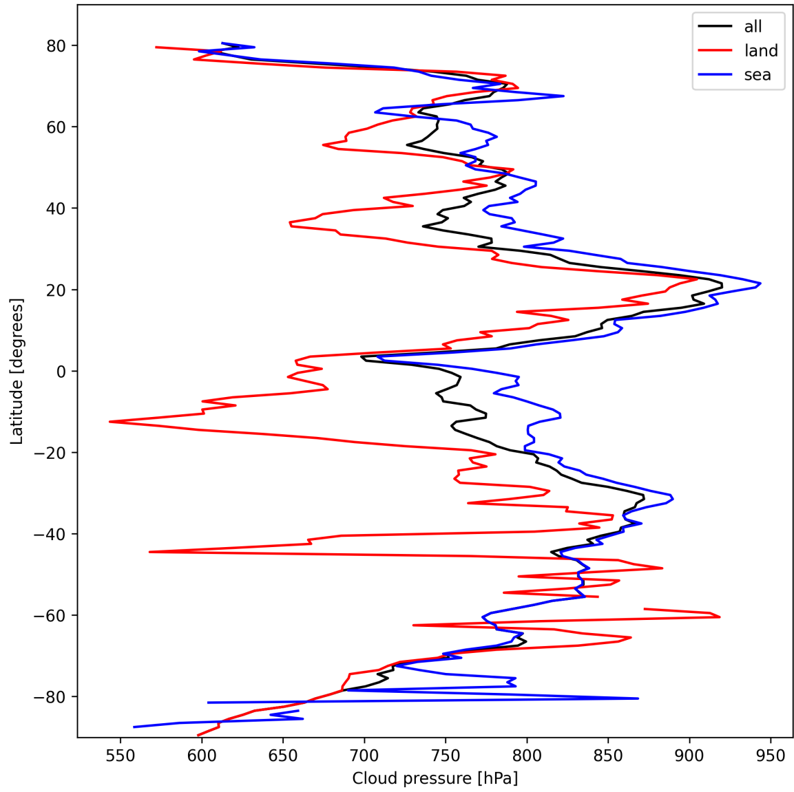
Figure 11: Zonal average of “Cloud pressure” for 2025-02-27 to 2025-02-27.
