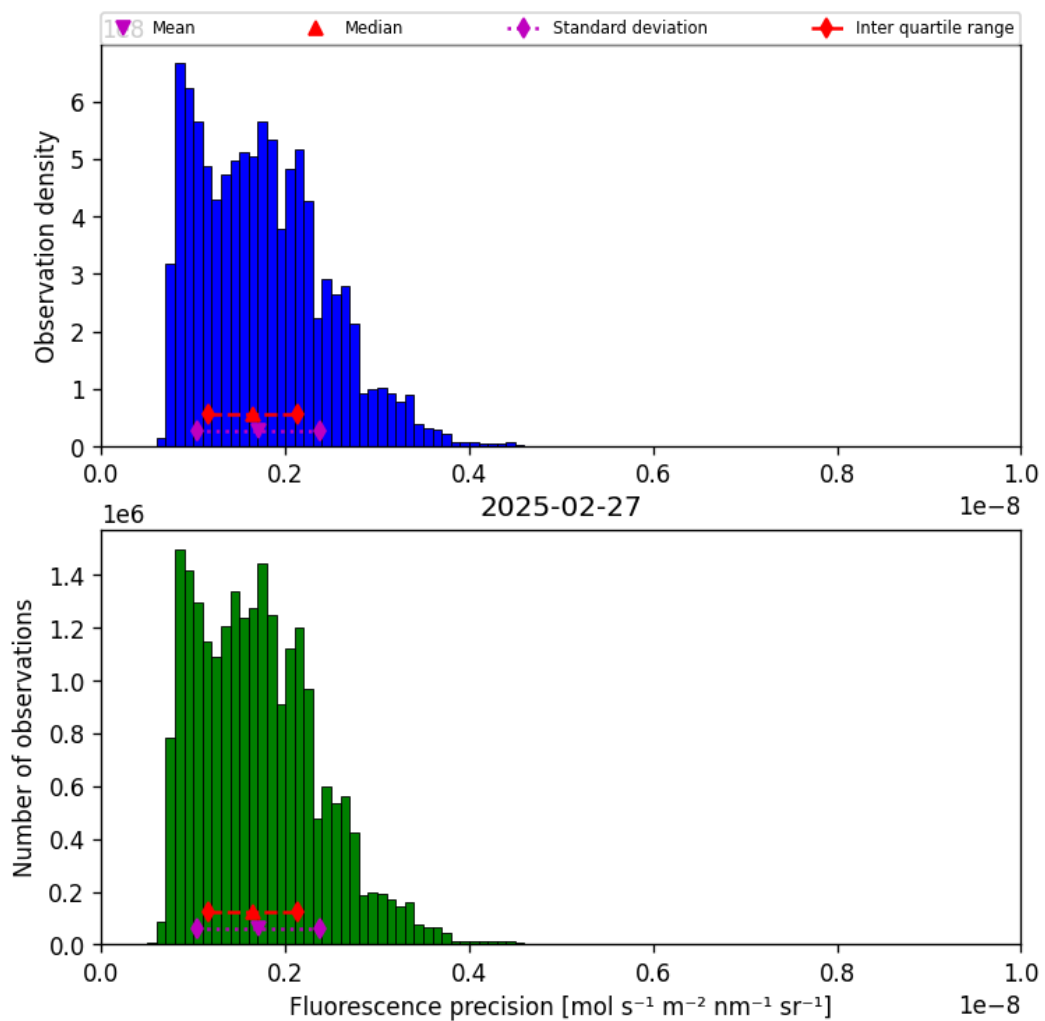
Figure 39: Histogram of “Fluorescence precision” for 2025-02-27 to 2025-02-27
