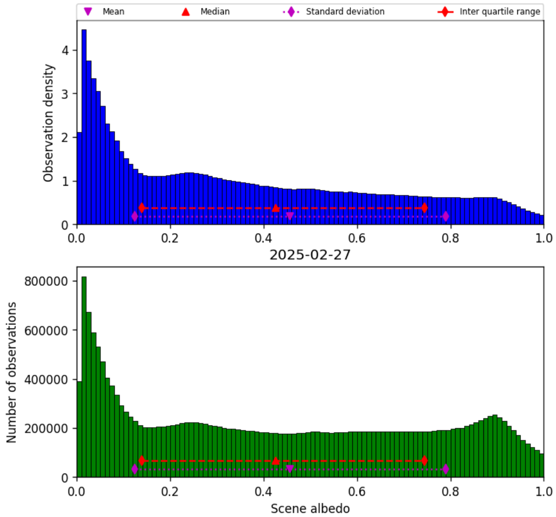
Figure 32: Histogram of “Scene albedo” for 2025-02-27 to 2025-02-27
