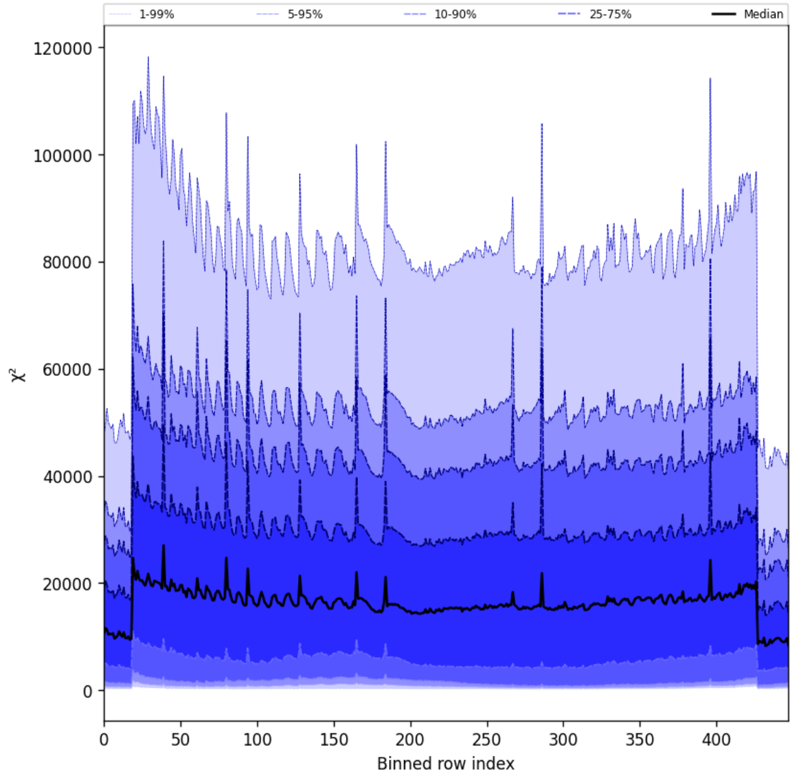
Figure 53: Along track statistics of “ \chi^2 ” for 2025-02-27 to 2025-02-27
