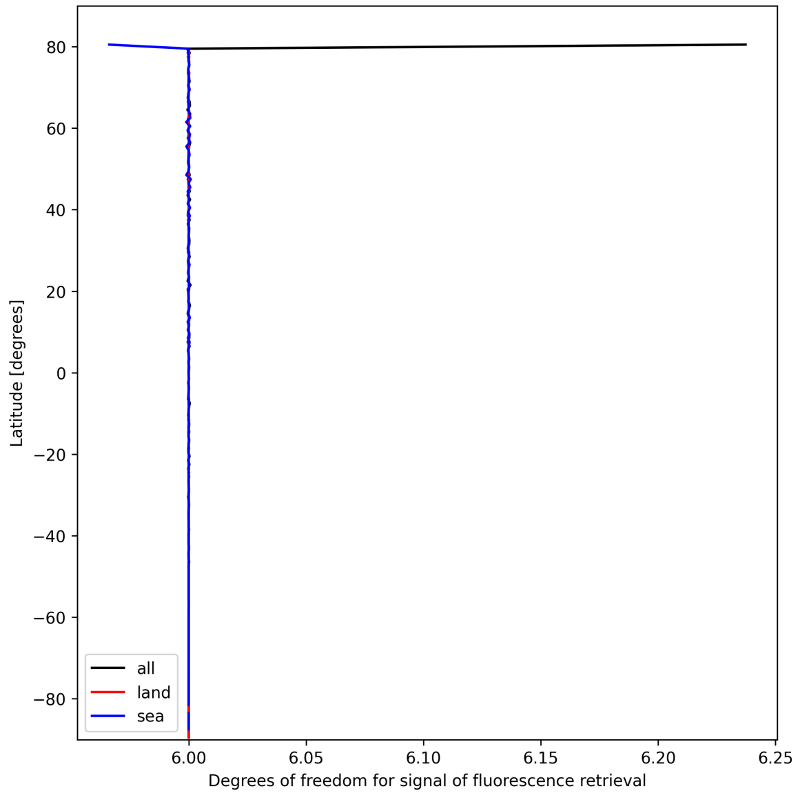
Figure 24: Zonal average of “Degrees of freedom for signal of fluorescence retrieval” for 2025-02-27 to 2025-02-27.
