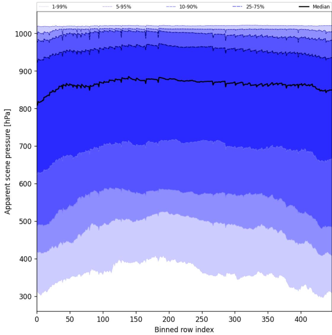
Figure 51: Along track statistics of “Apparent scene pressure” for 2025-02-27 to 2025-02-27
