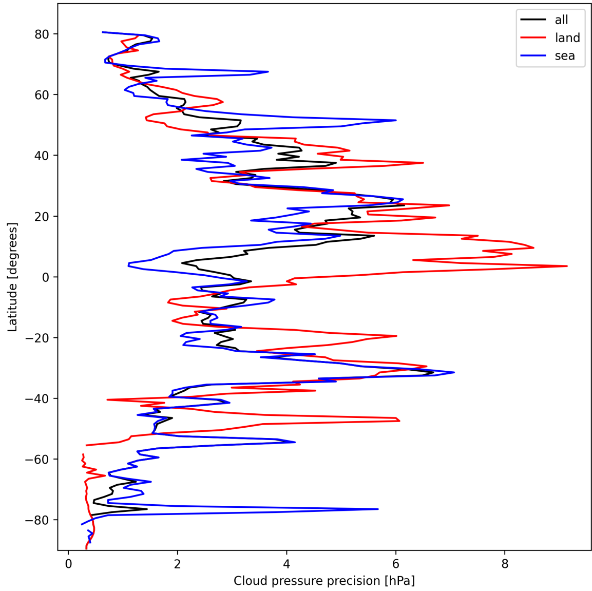
Figure 12: Zonal average of “Cloud pressure precision” for 2025-02-27 to 2025-02-27.
