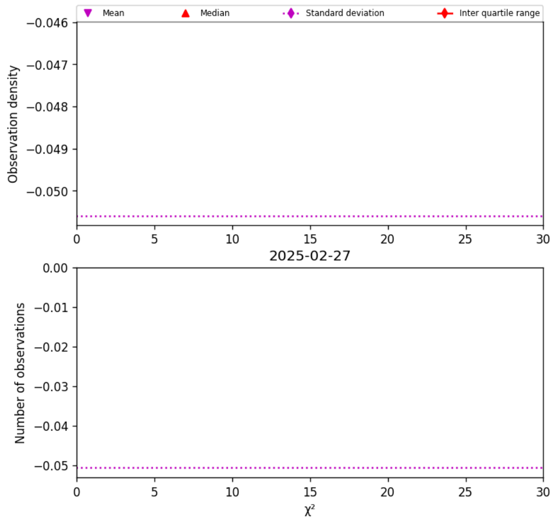
Figure 36: Histogram of " \chi^2 " for 2025-02-27 to 2025-02-27
