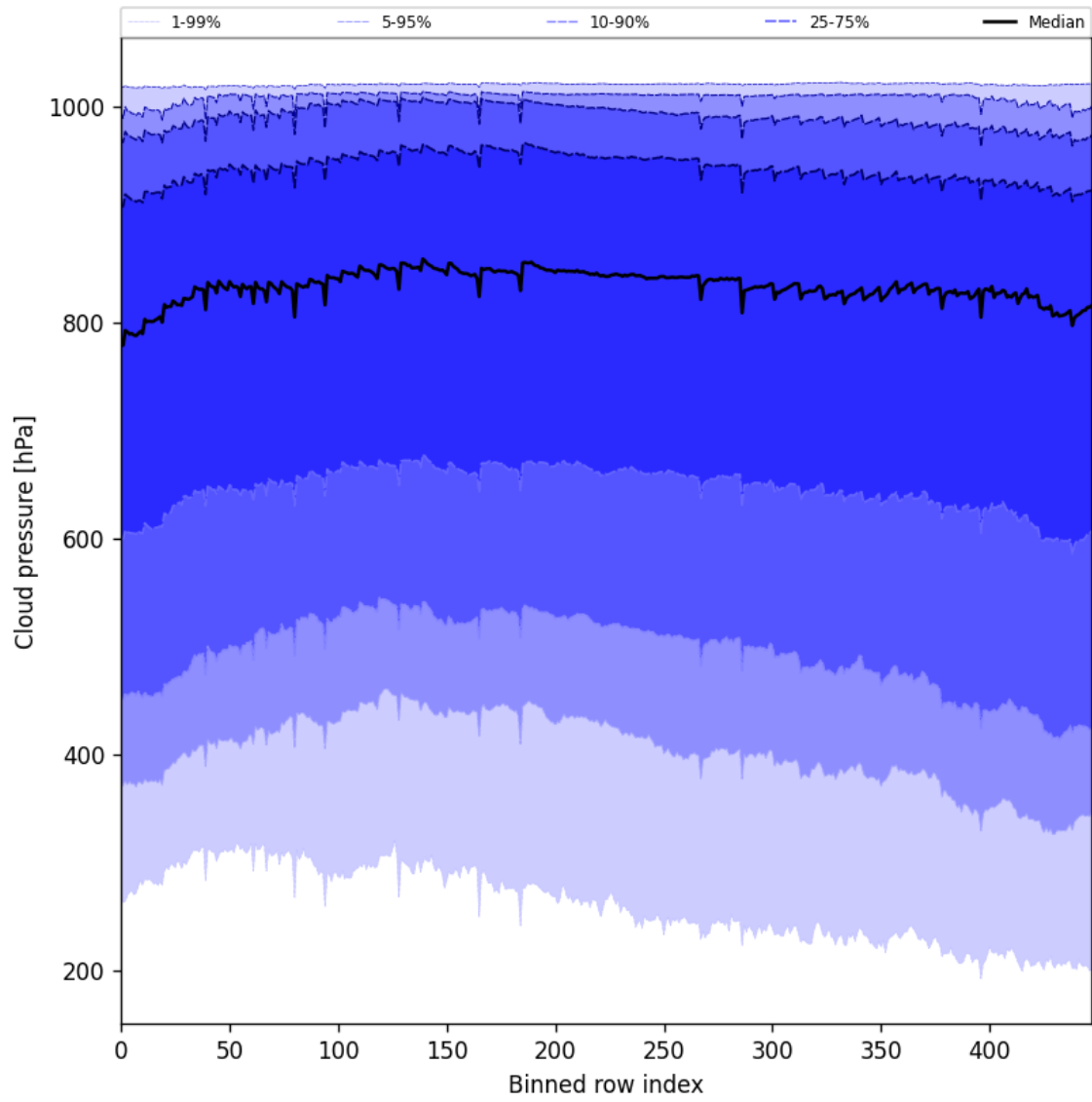
Figure 45: Along track statistics of “Cloud pressure” for 2025-02-27 to 2025-02-27
