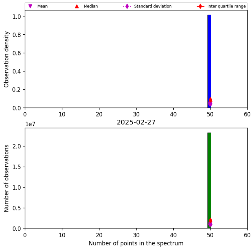
Figure 42: Histogram of “Number of points in the spectrum” for 2025-02-27 to 2025-02-27
