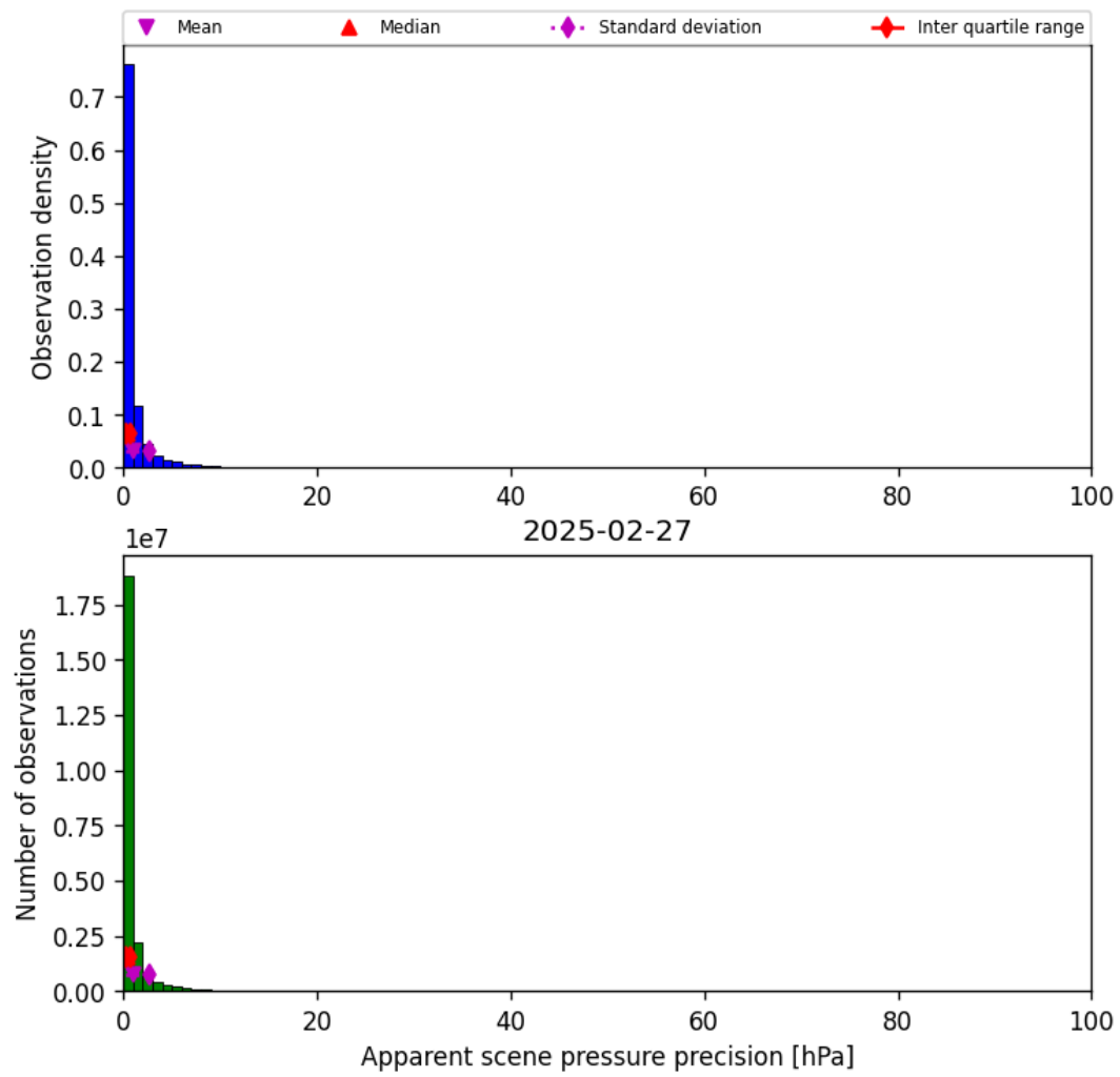
Figure 35: Histogram of “Apparent scene pressure precision” for 2025-02-27 to 2025-02-27
