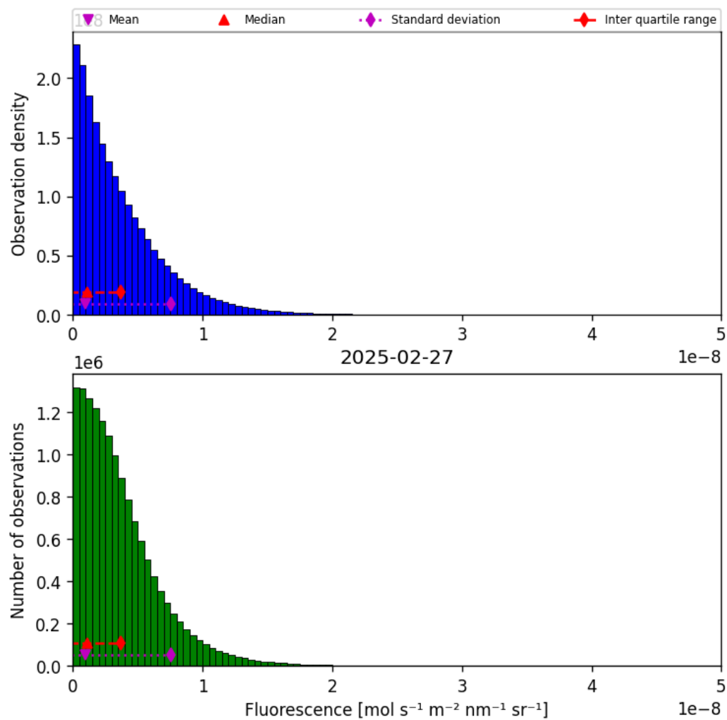
Figure 38: Histogram of “Fluorescence” for 2025-02-27 to 2025-02-27
