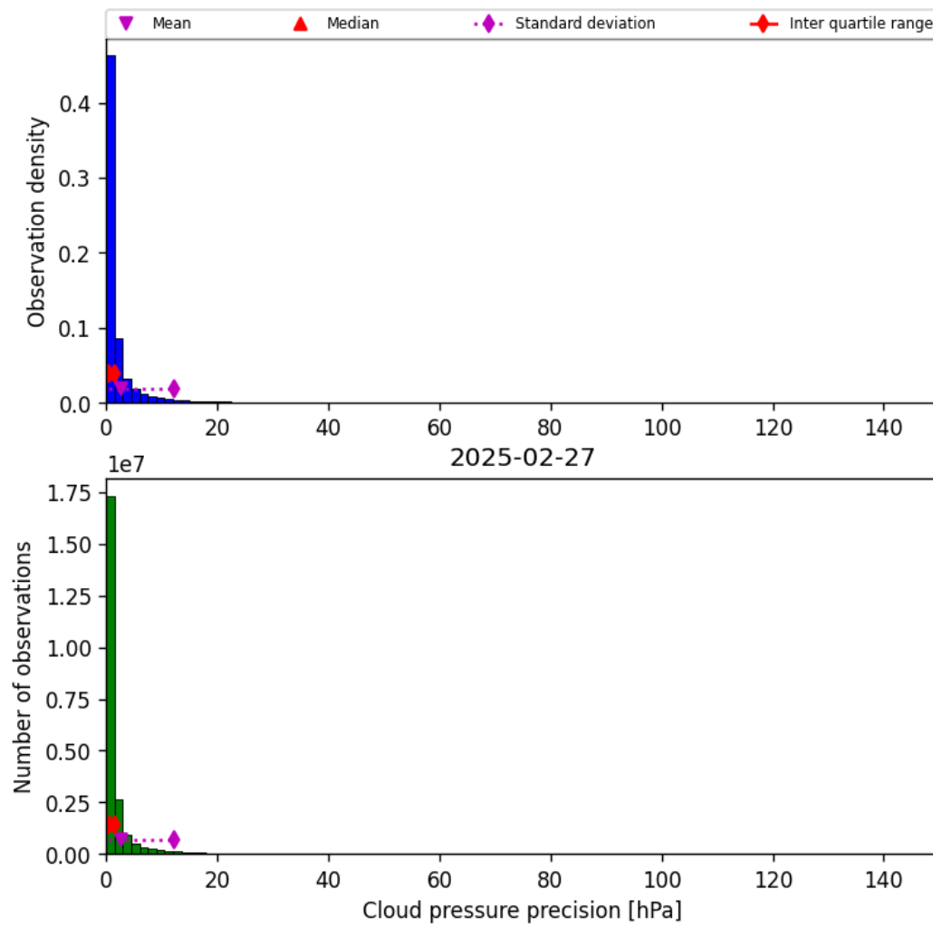
Figure 29: Histogram of “Cloud pressure precision” for 2025-02-27 to 2025-02-27
