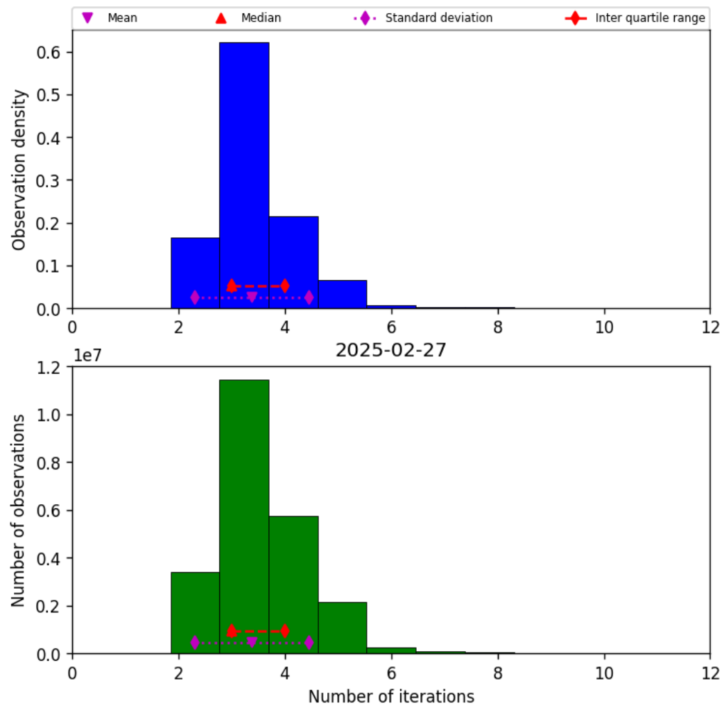
Figure 37: Histogram of “Number of iterations” for 2025-02-27 to 2025-02-27
