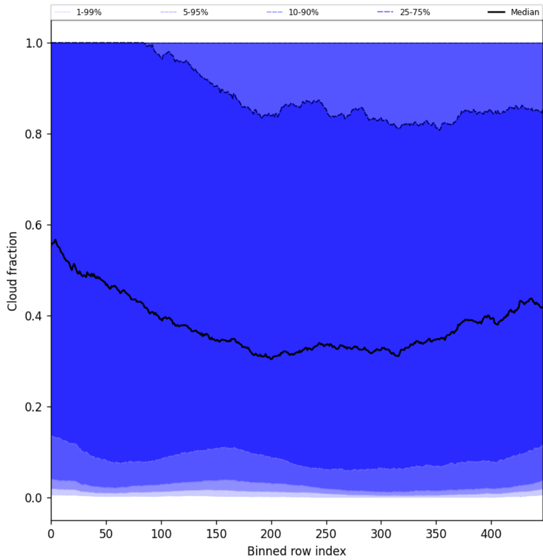
Figure 47: Along track statistics of “Cloud fraction” for 2025-02-27 to 2025-02-27
