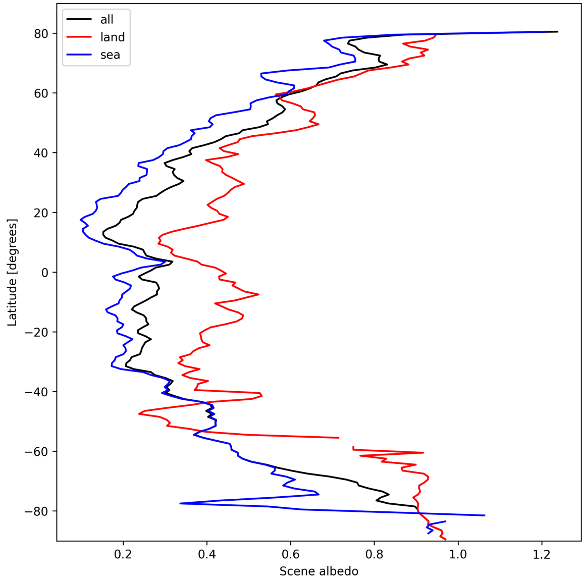
Figure 15: Zonal average of “Scene albedo” for 2025-02-27 to 2025-02-27.
