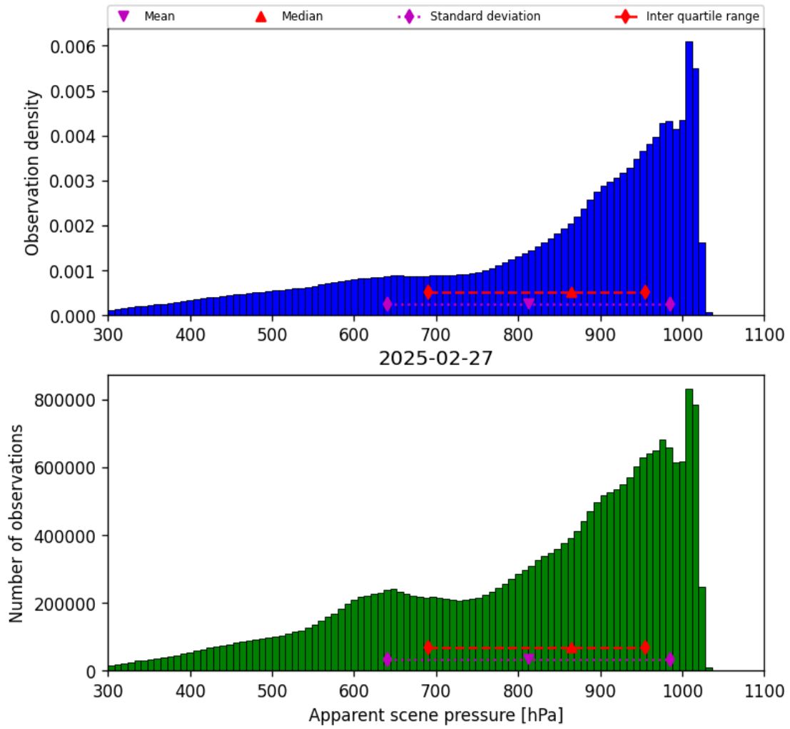
Figure 34: Histogram of “Apparent scene pressure” for 2025-02-27 to 2025-02-27
