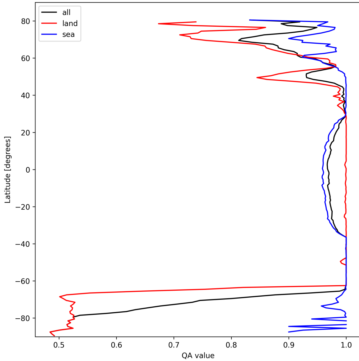
Figure 10: Zonal average of “QA value” for 2025-02-27 to 2025-02-27.
