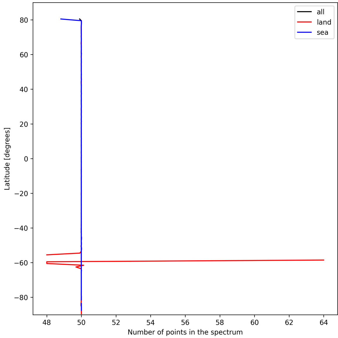
Figure 25: Zonal average of “Number of points in the spectrum” for 2025-02-27 to 2025-02-27.
