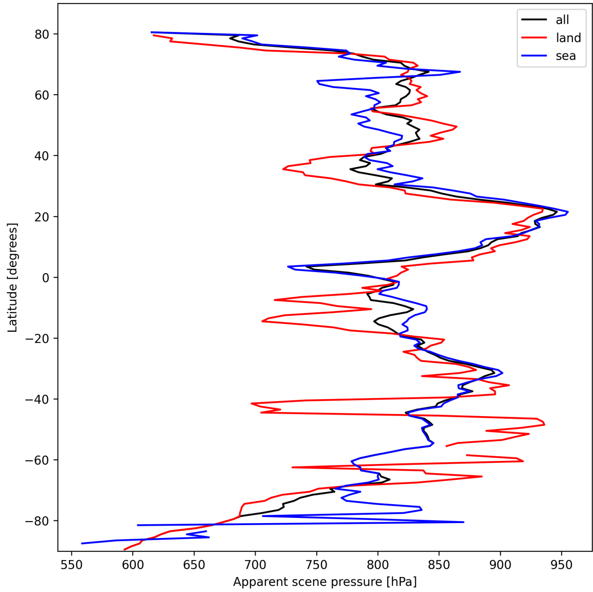
Figure 17: Zonal average of “Apparent scene pressure” for 2025-02-27 to 2025-02-27.
