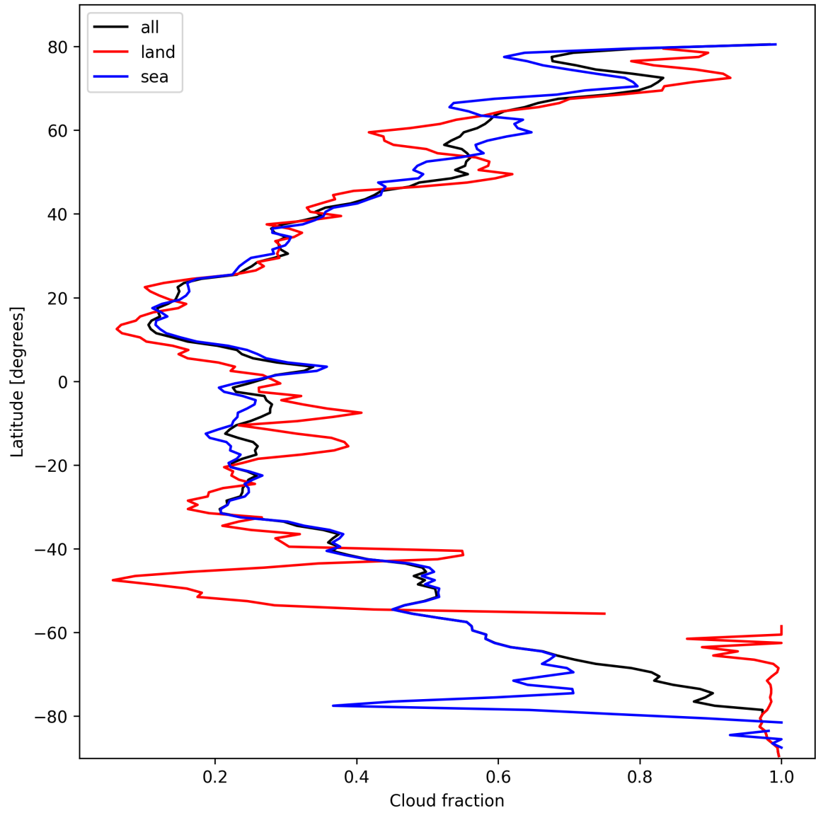
Figure 13: Zonal average of “Cloud fraction” for 2025-02-27 to 2025-02-27.
