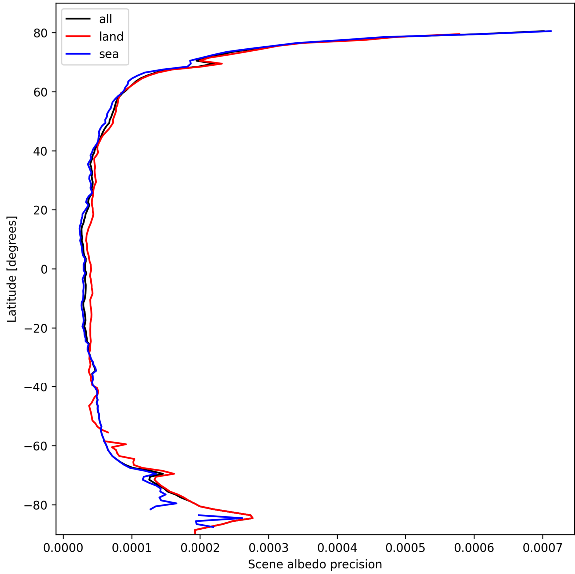
Figure 16: Zonal average of “Scene albedo precision” for 2025-02-27 to 2025-02-27.
