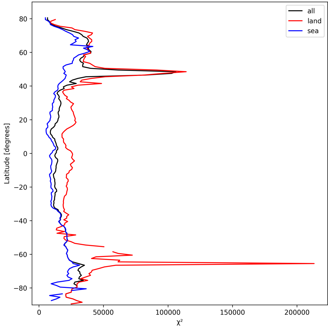
Figure 19: Zonal average of “ \chi^2 ” for 2025-02-27 to 2025-02-27.
