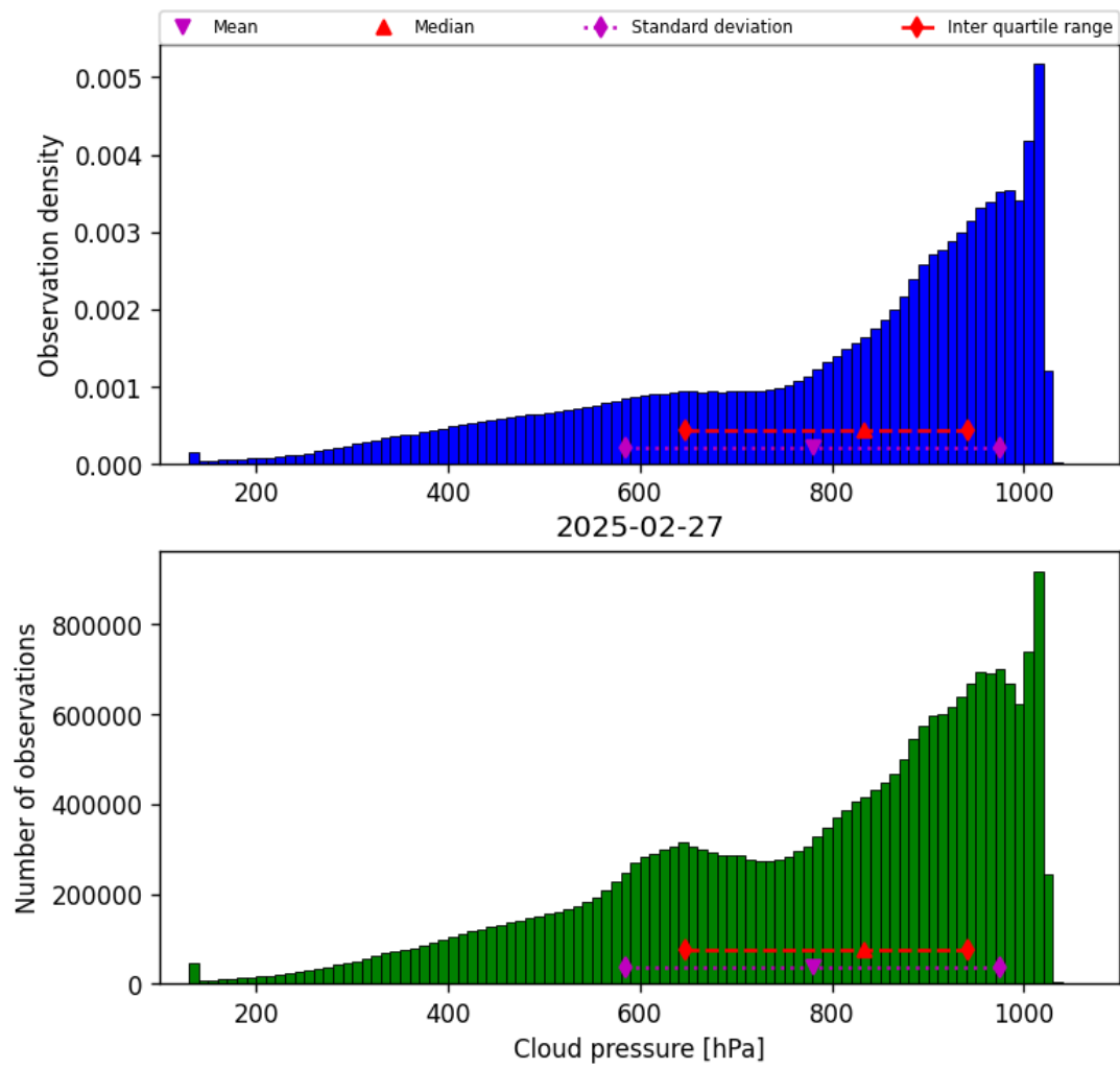
Figure 28: Histogram of “Cloud pressure” for 2025-02-27 to 2025-02-27
