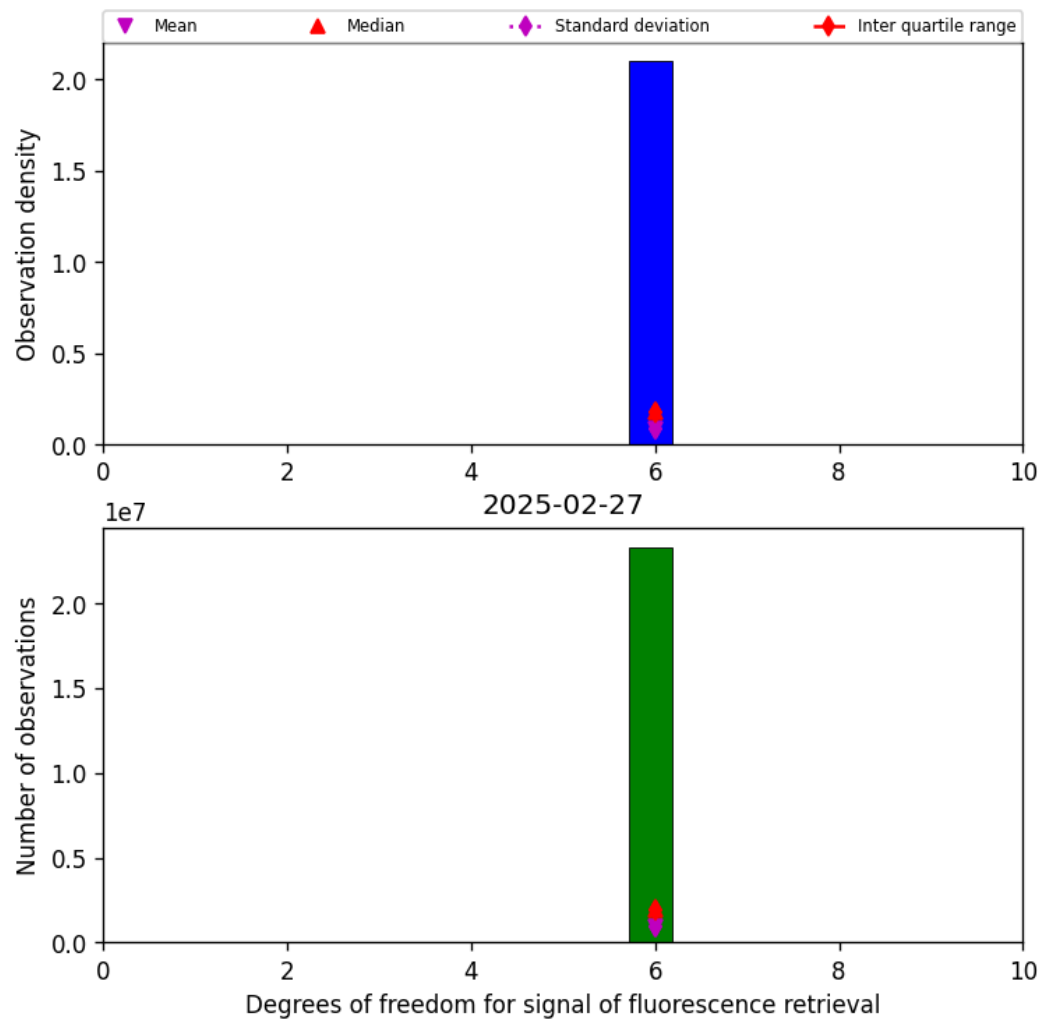
Figure 41: Histogram of “Degrees of freedom for signal of fluorescence retrieval” for 2025-02-27 to 2025-02-27
