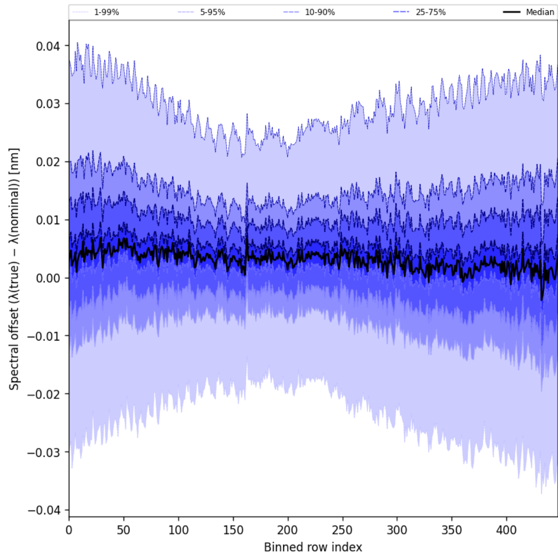
Figure 60: Along track statistics of “Spectral offset ( \lambda_{\text{true}} - \lambda_{\text{nominal}} )” for 2025-02-27 to 2025-02-27
