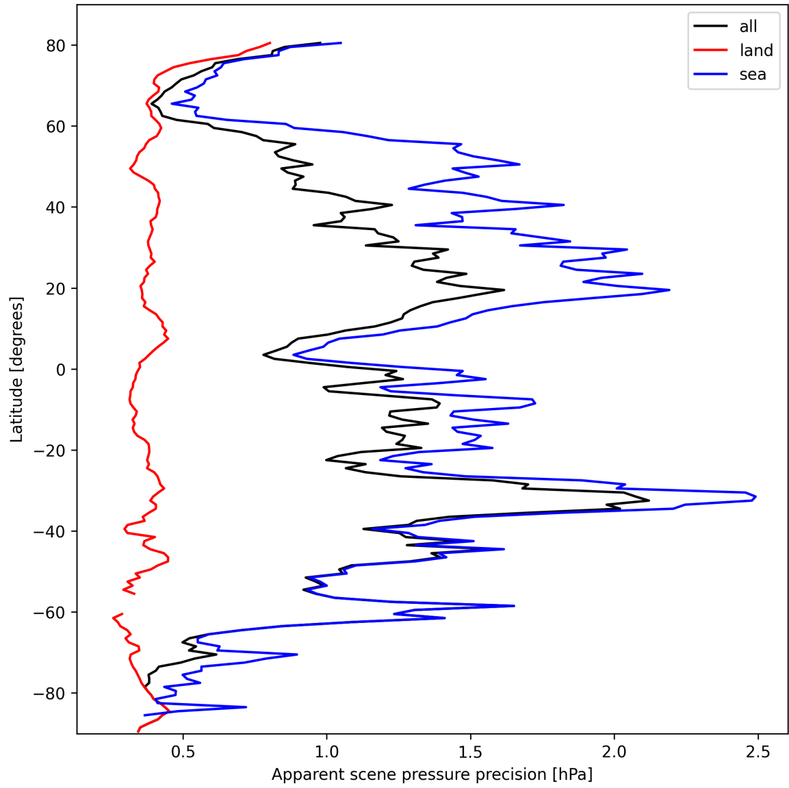
Figure 18: Zonal average of “Apparent scene pressure precision” for 2025-02-28 to 2025-03-01.
