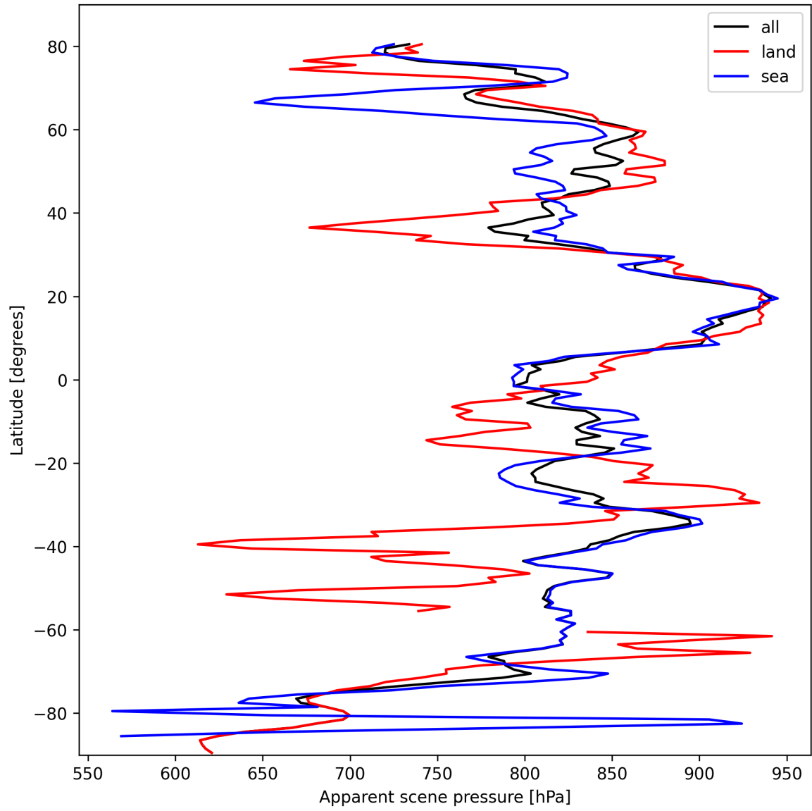
Figure 17: Zonal average of “Apparent scene pressure” for 2025-02-28 to 2025-03-01.
