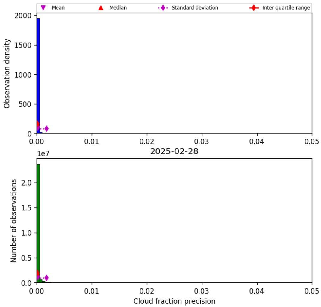
Figure 31: Histogram of “Cloud fraction precision” for 2025-02-28 to 2025-03-01
