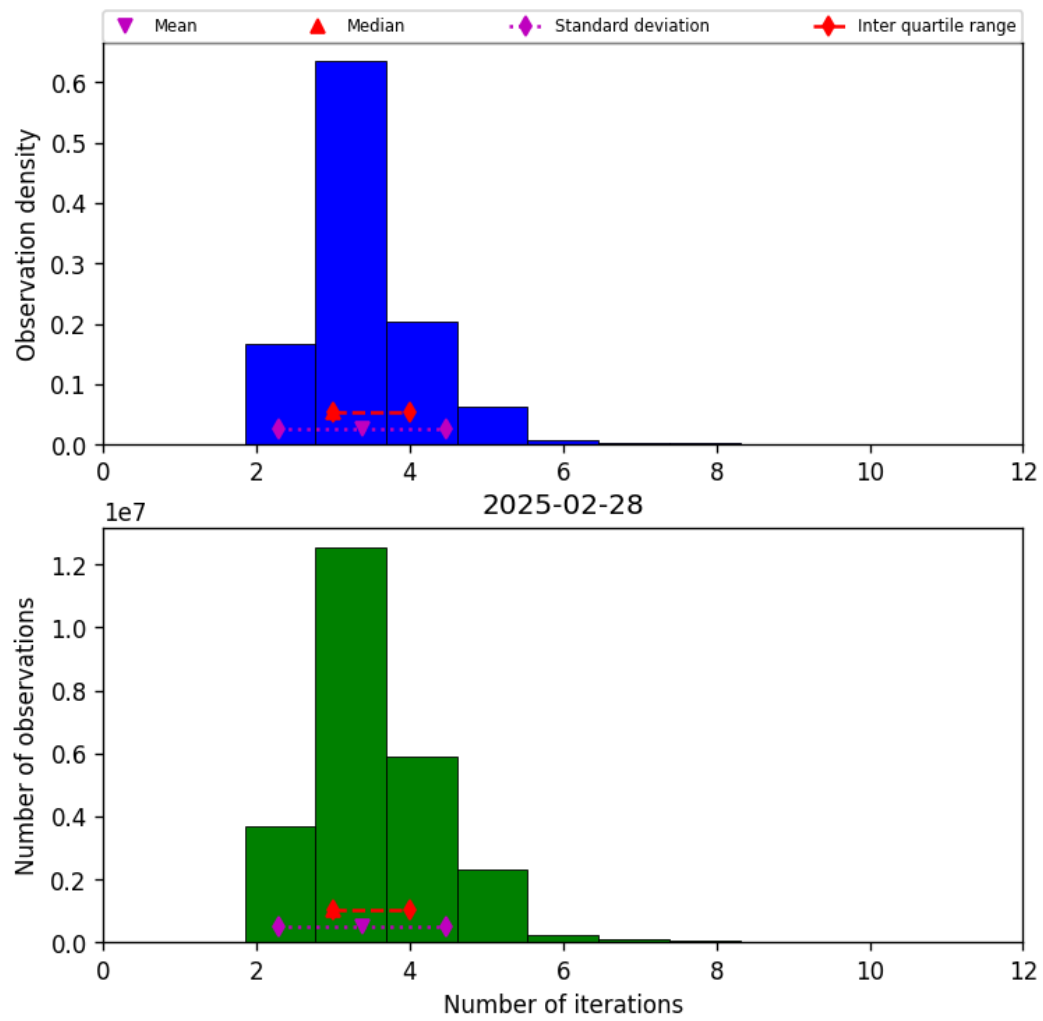
Figure 37: Histogram of “Number of iterations” for 2025-02-28 to 2025-03-01
