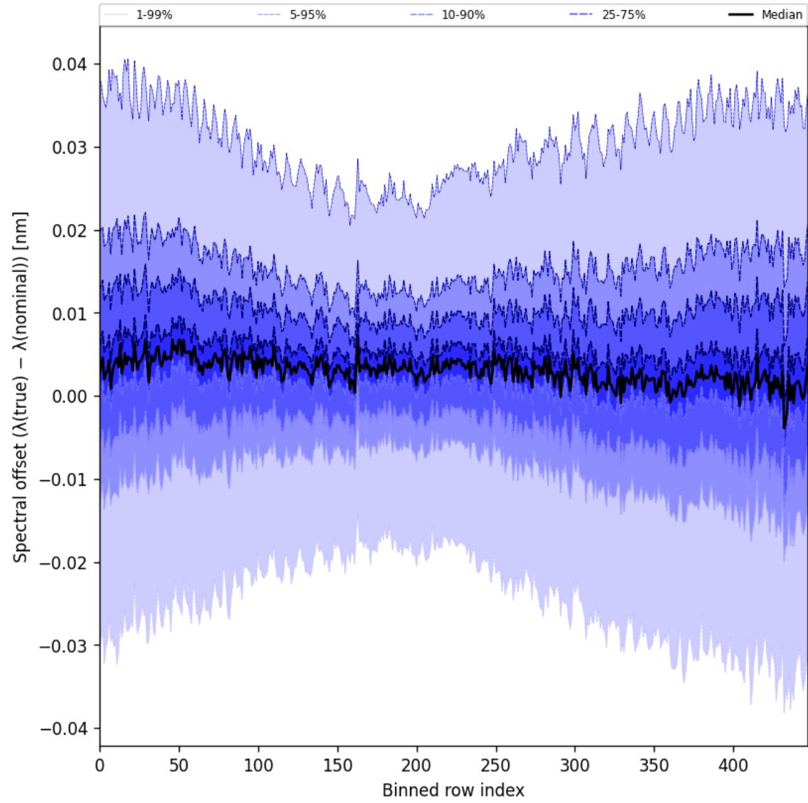
Figure 60: Along track statistics of “Spectral offset ( \lambda_{\text{true}} - \lambda_{\text{nominal}} )” for 2025-02-28 to 2025-03-01
