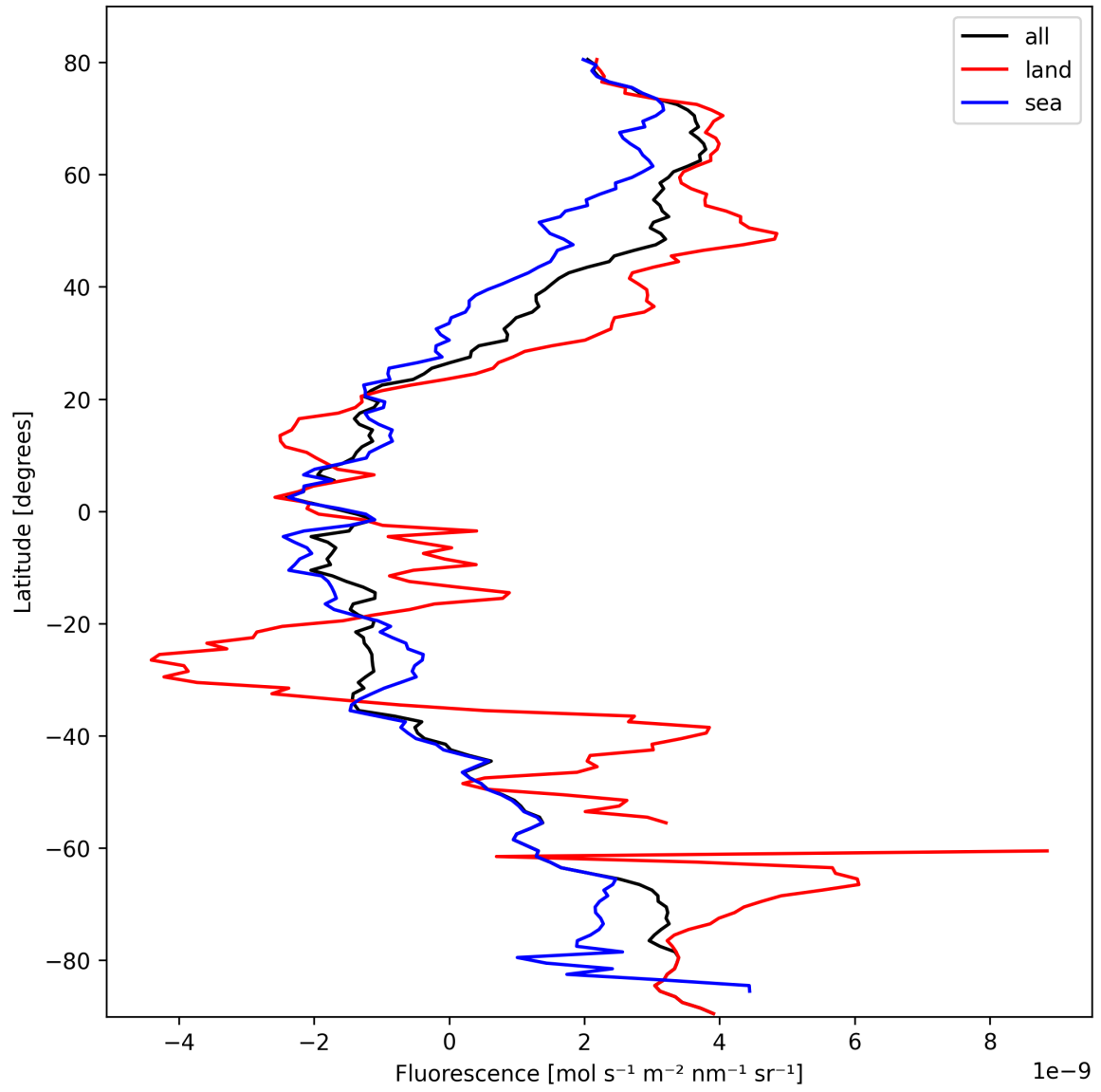
Figure 21: Zonal average of “Fluorescence” for 2025-02-28 to 2025-03-01.
