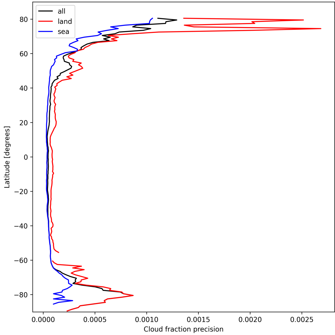
Figure 14: Zonal average of “Cloud fraction precision” for 2025-02-28 to 2025-03-01.
