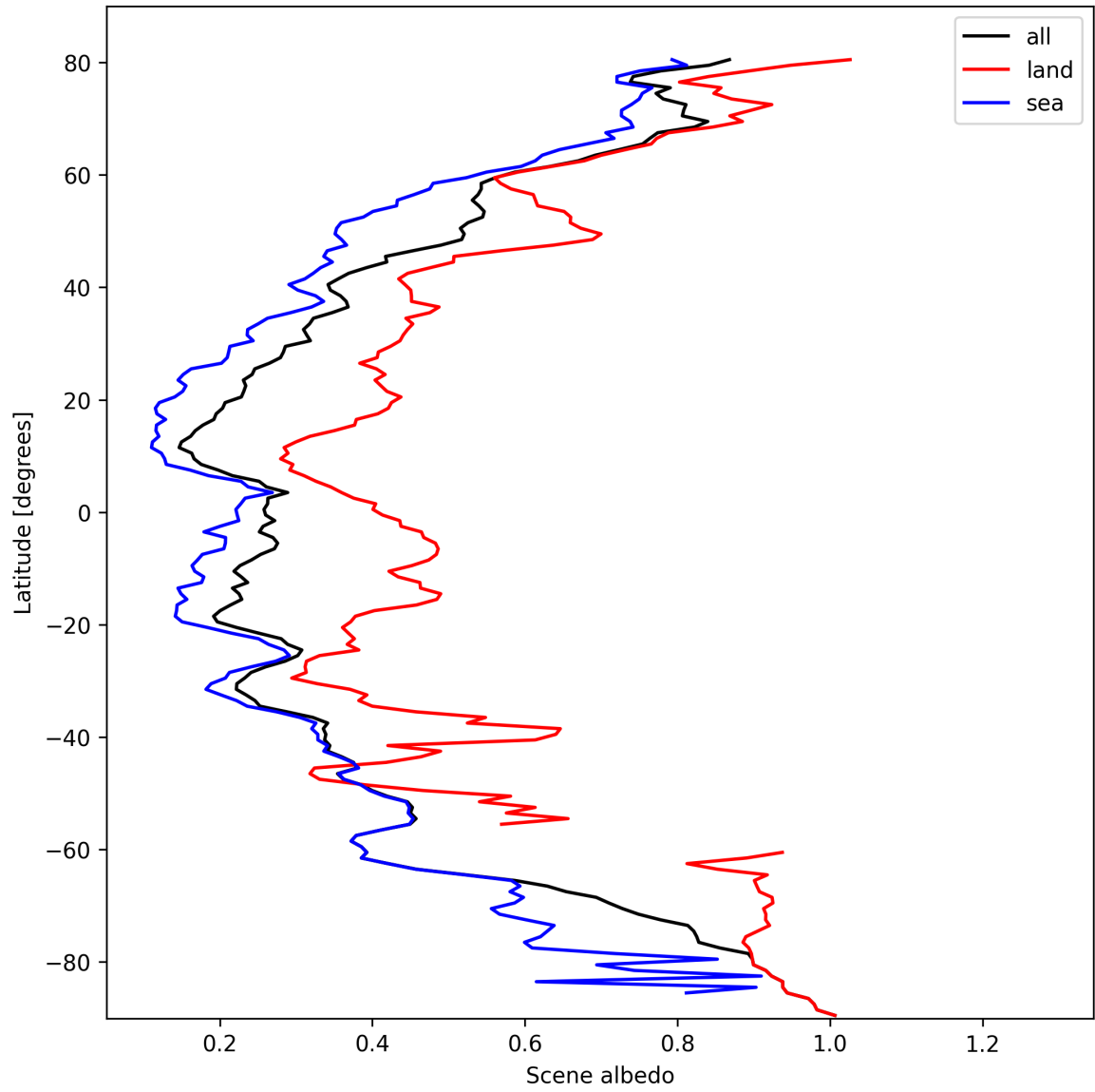
Figure 15: Zonal average of “Scene albedo” for 2025-02-28 to 2025-03-01.
