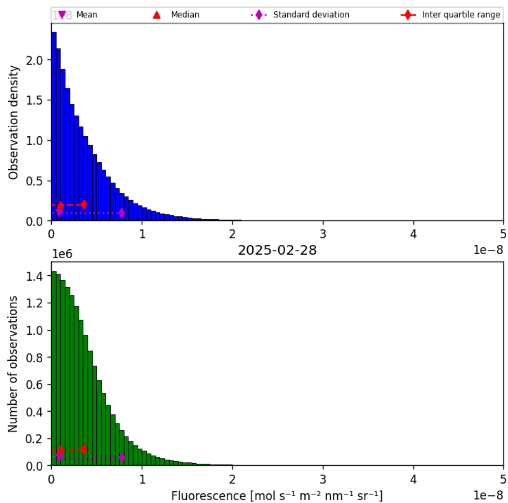
Figure 38: Histogram of “Fluorescence” for 2025-02-28 to 2025-03-01
