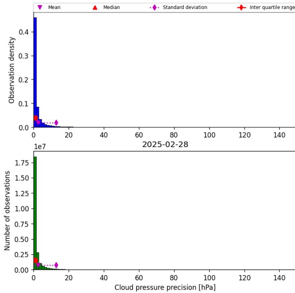
Figure 29: Histogram of “Cloud pressure precision” for 2025-02-28 to 2025-03-01
