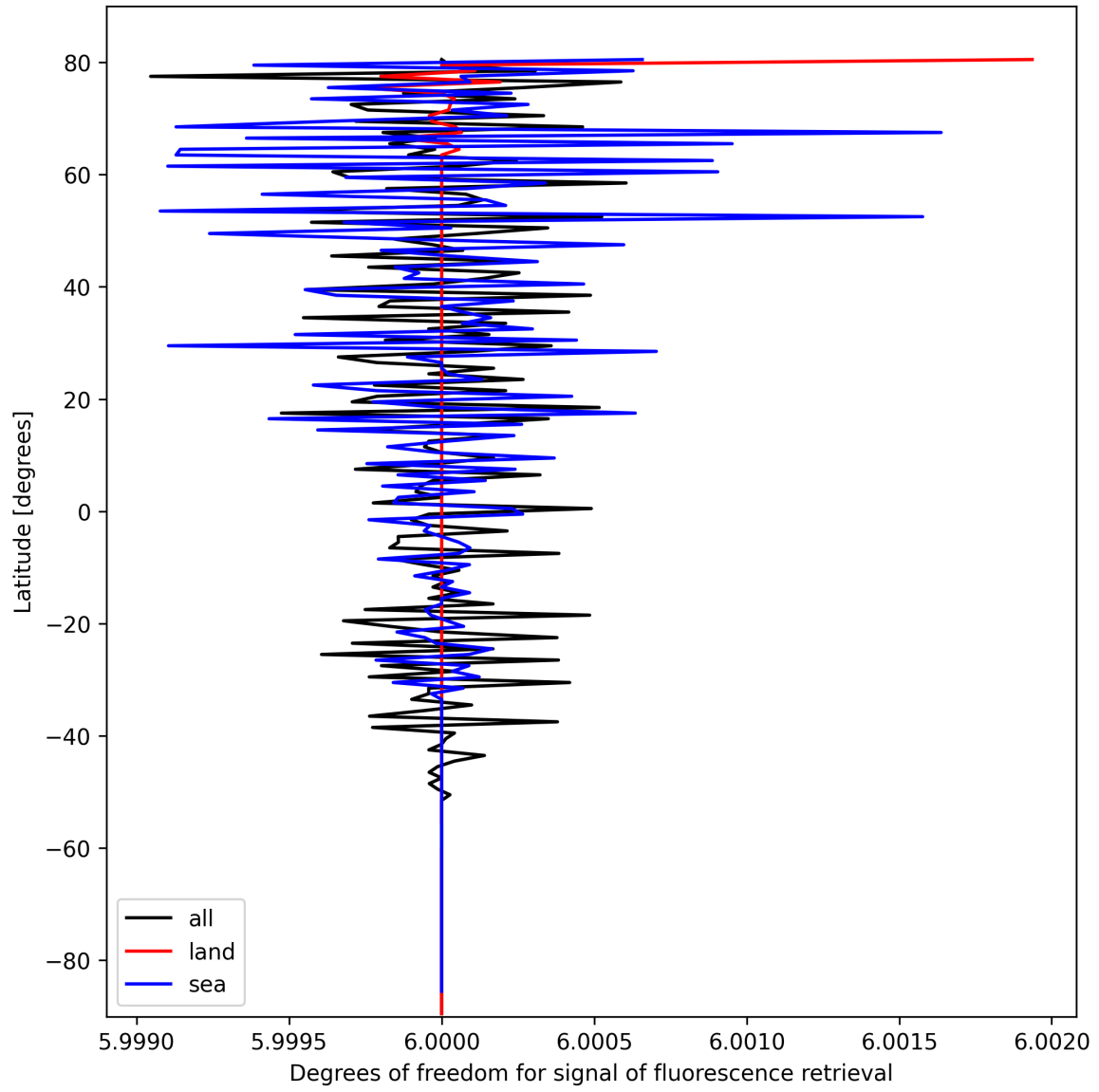
Figure 24: Zonal average of “Degrees of freedom for signal of fluorescence retrieval” for 2025-02-28 to 2025-03-01.
