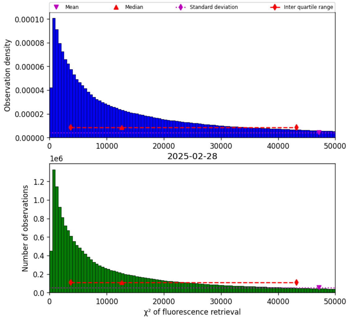
Figure 40: Histogram of “ \chi^2 of fluorescence retrieval” for 2025-02-28 to 2025-03-01
