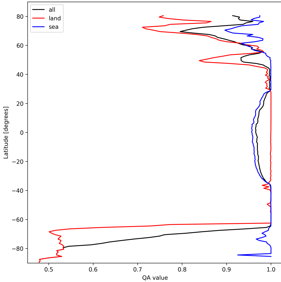
Figure 10: Zonal average of “QA value” for 2025-02-28 to 2025-03-01.
