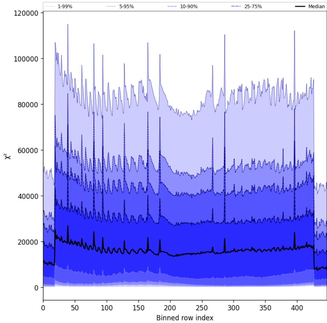
Figure 53: Along track statistics of “ \chi^2 ” for 2025-02-28 to 2025-03-01
