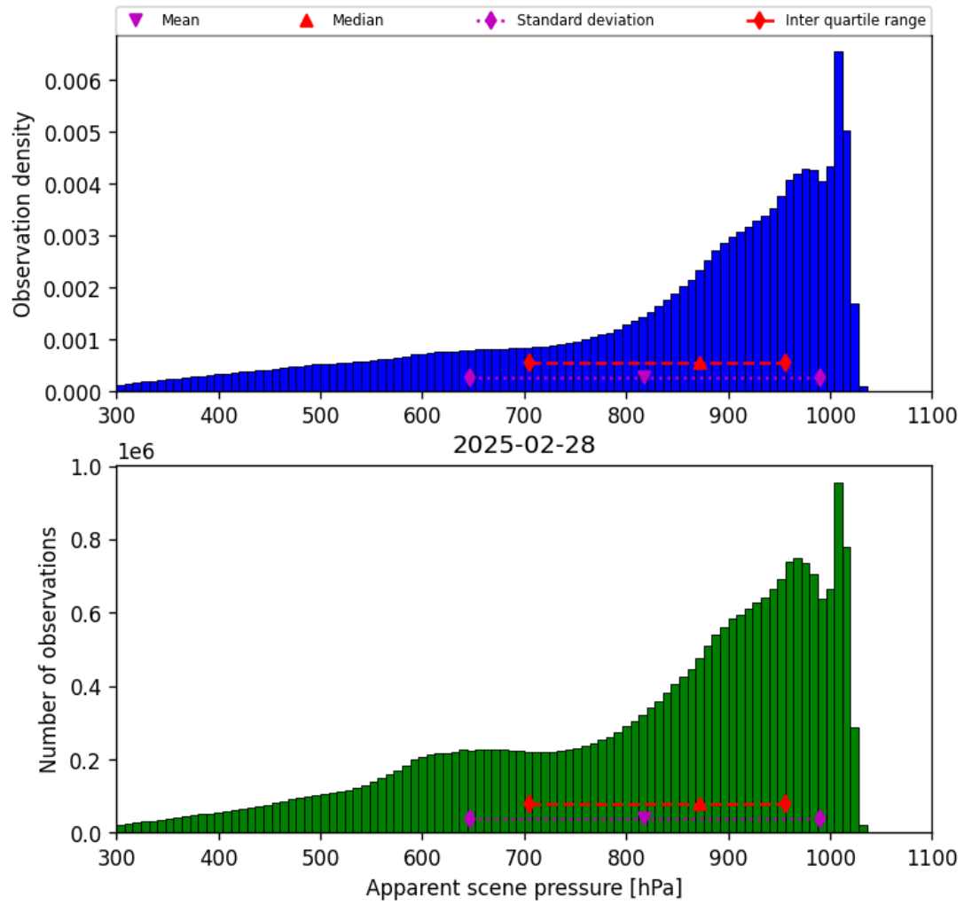
Figure 34: Histogram of “Apparent scene pressure” for 2025-02-28 to 2025-03-01
