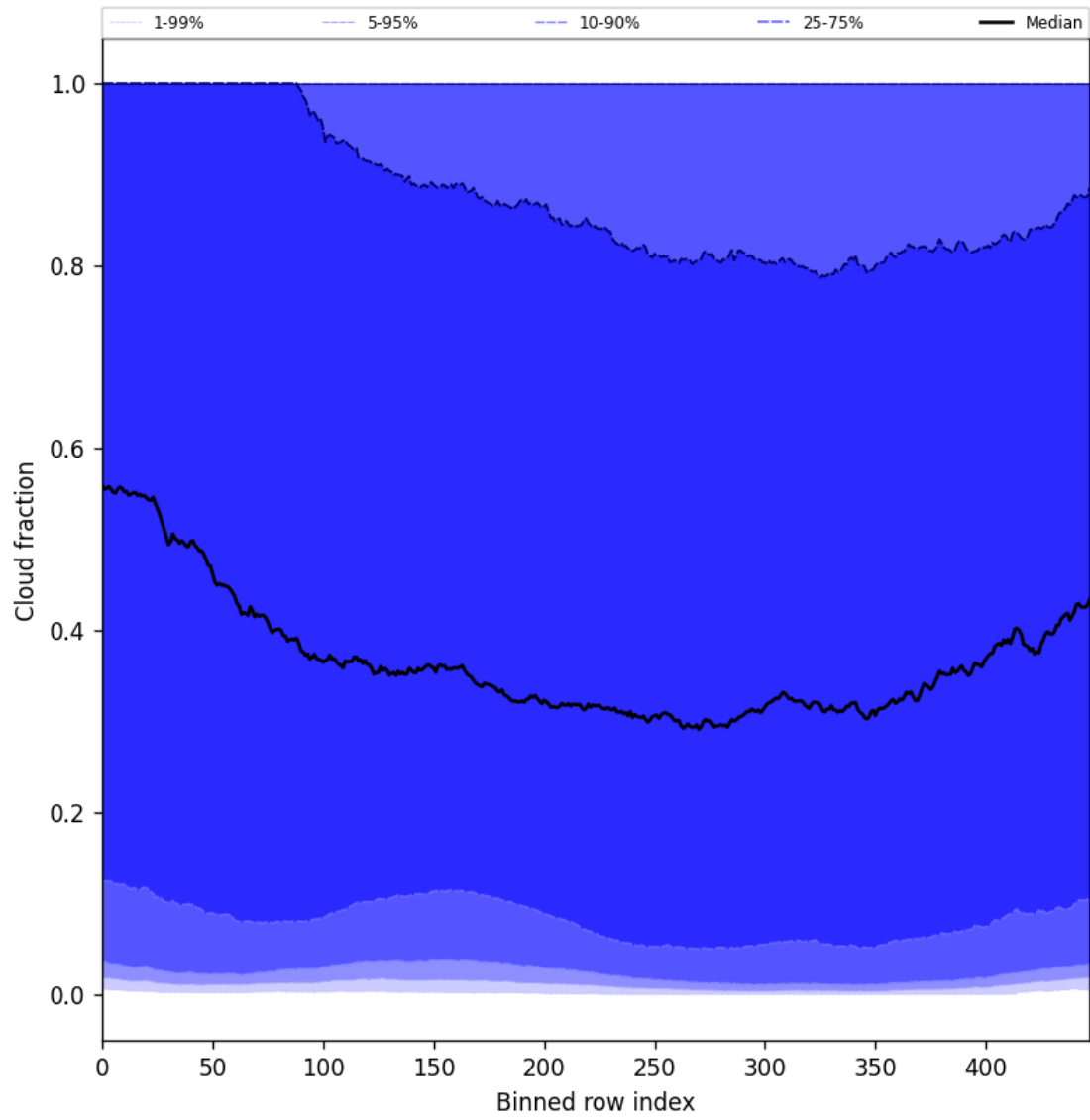
Figure 47: Along track statistics of “Cloud fraction” for 2025-02-28 to 2025-03-01
