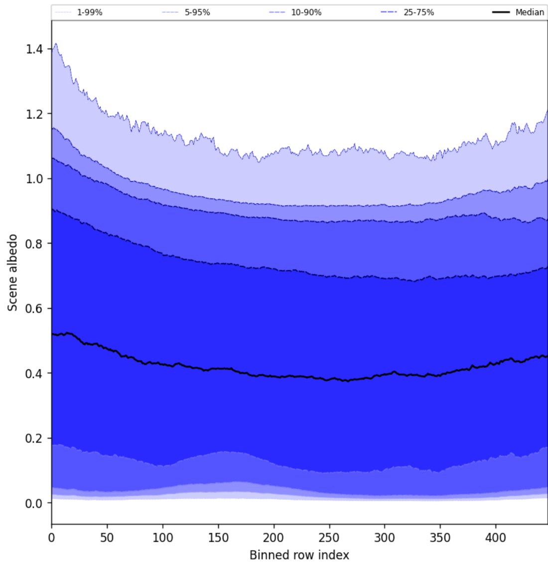
Figure 49: Along track statistics of “Scene albedo” for 2025-02-28 to 2025-03-01
