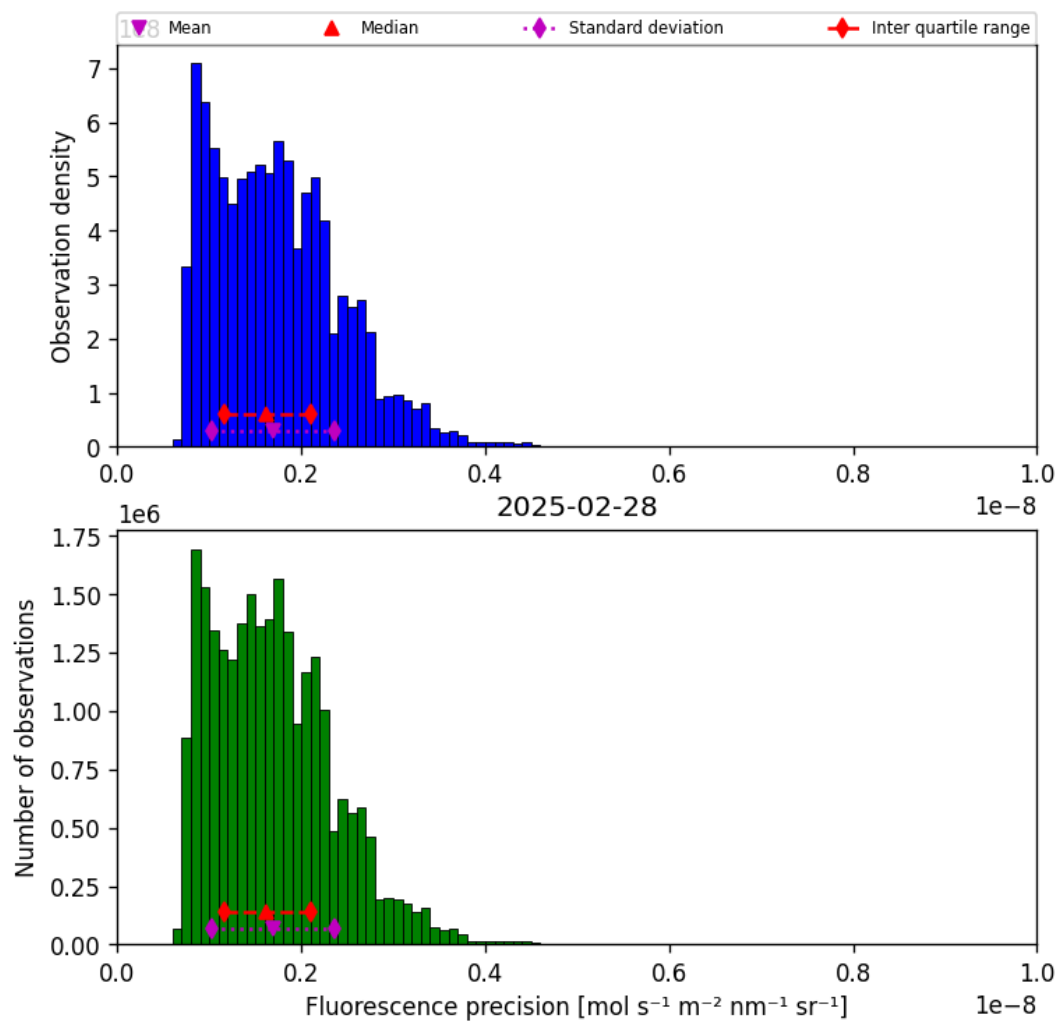
Figure 39: Histogram of “Fluorescence precision” for 2025-02-28 to 2025-03-01
