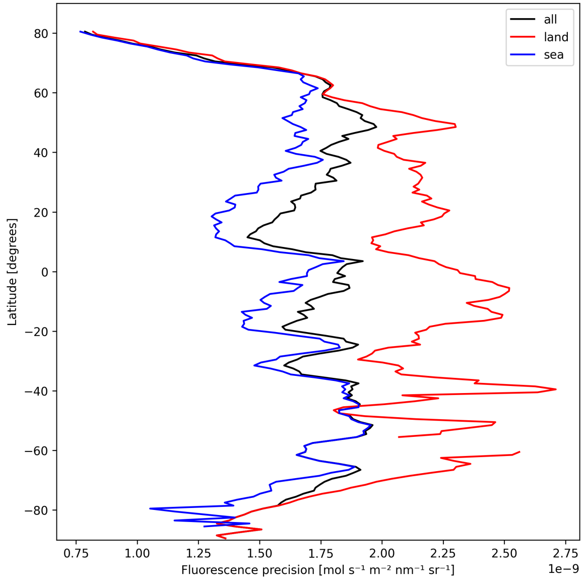
Figure 22: Zonal average of “Fluorescence precision” for 2025-02-28 to 2025-03-01.
