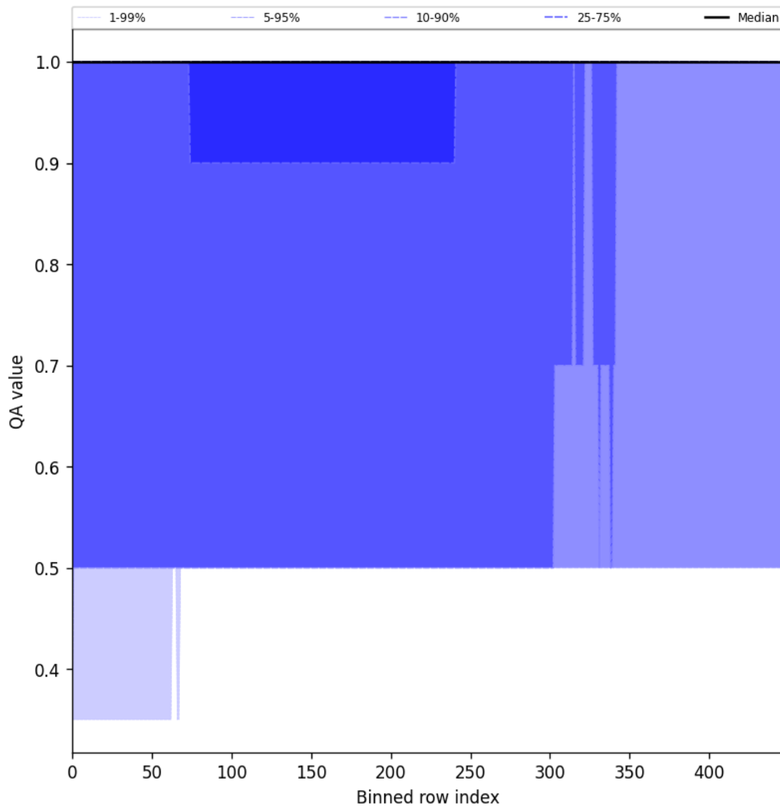
Figure 44: Along track statistics of “QA value” for 2025-02-28 to 2025-03-01
