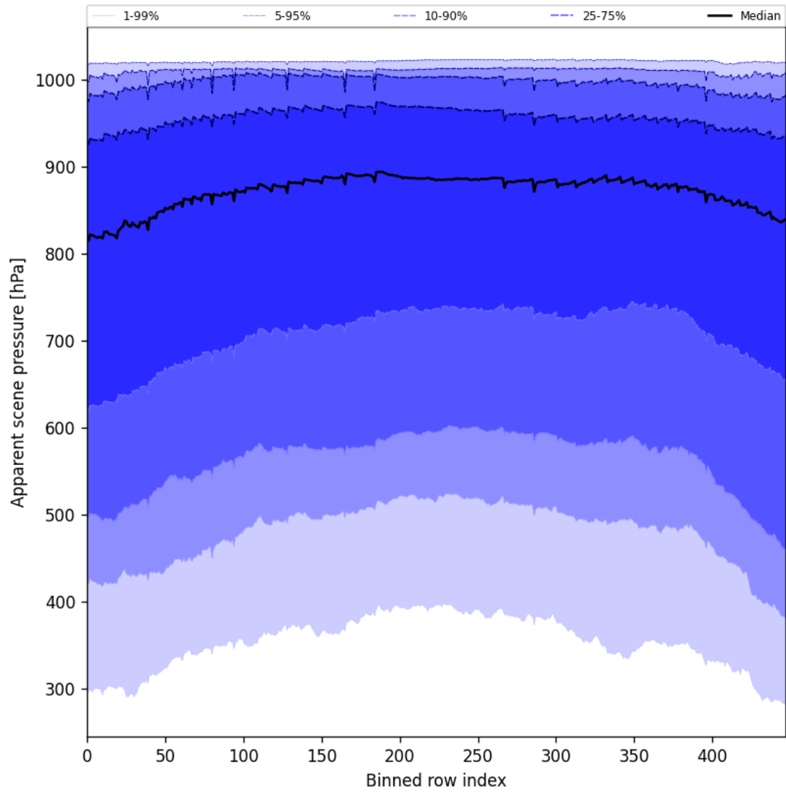
Figure 51: Along track statistics of “Apparent scene pressure” for 2025-02-28 to 2025-03-01
