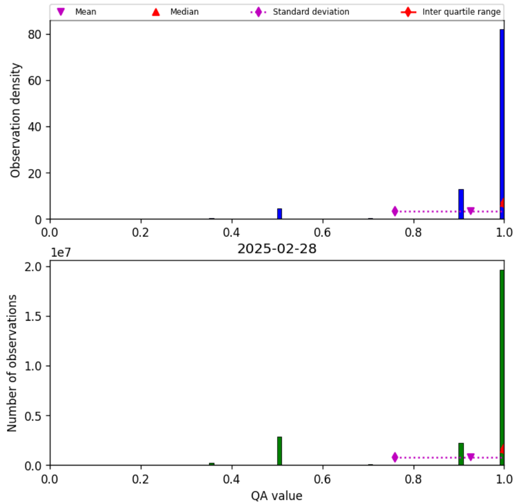
Figure 27: Histogram of “QA value” for 2025-02-28 to 2025-03-01
