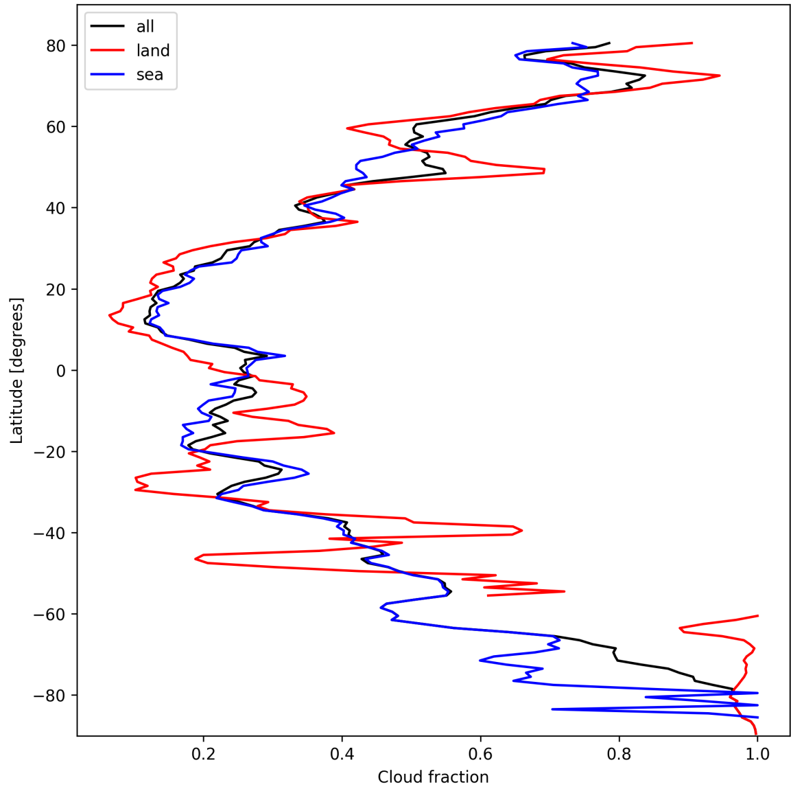
Figure 13: Zonal average of “Cloud fraction” for 2025-02-28 to 2025-03-01.
