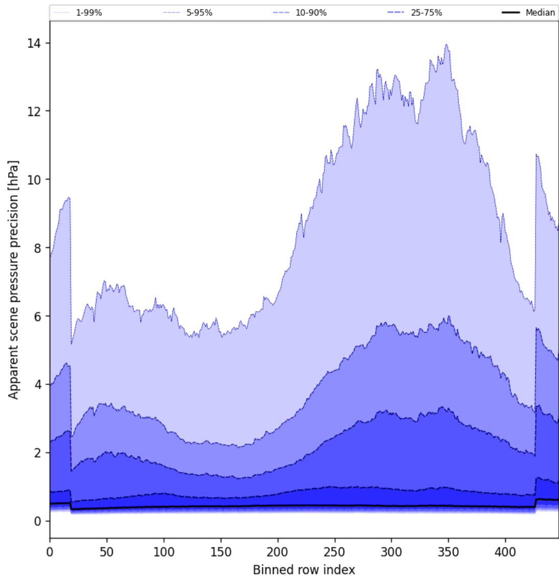
Figure 52: Along track statistics of “Apparent scene pressure precision” for 2025-02-28 to 2025-03-01
