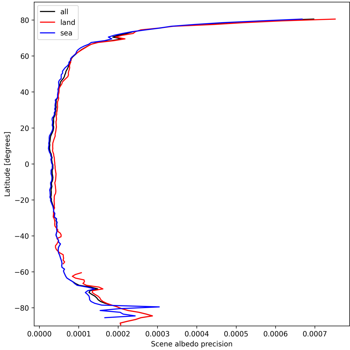
Figure 16: Zonal average of “Scene albedo precision” for 2025-02-28 to 2025-03-01.
