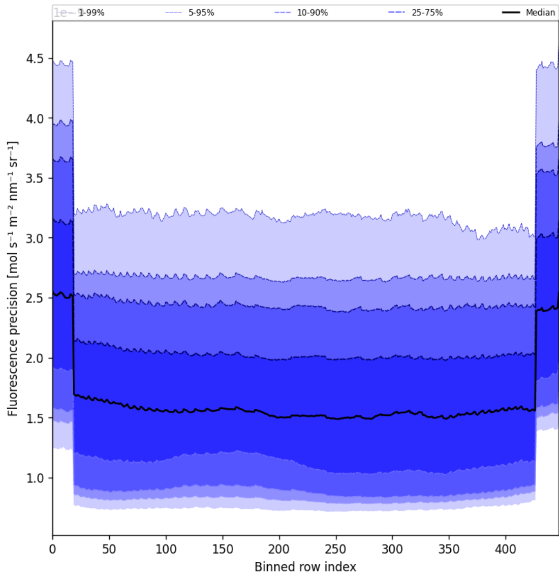
Figure 56: Along track statistics of “Fluorescence precision” for 2025-02-28 to 2025-03-01
