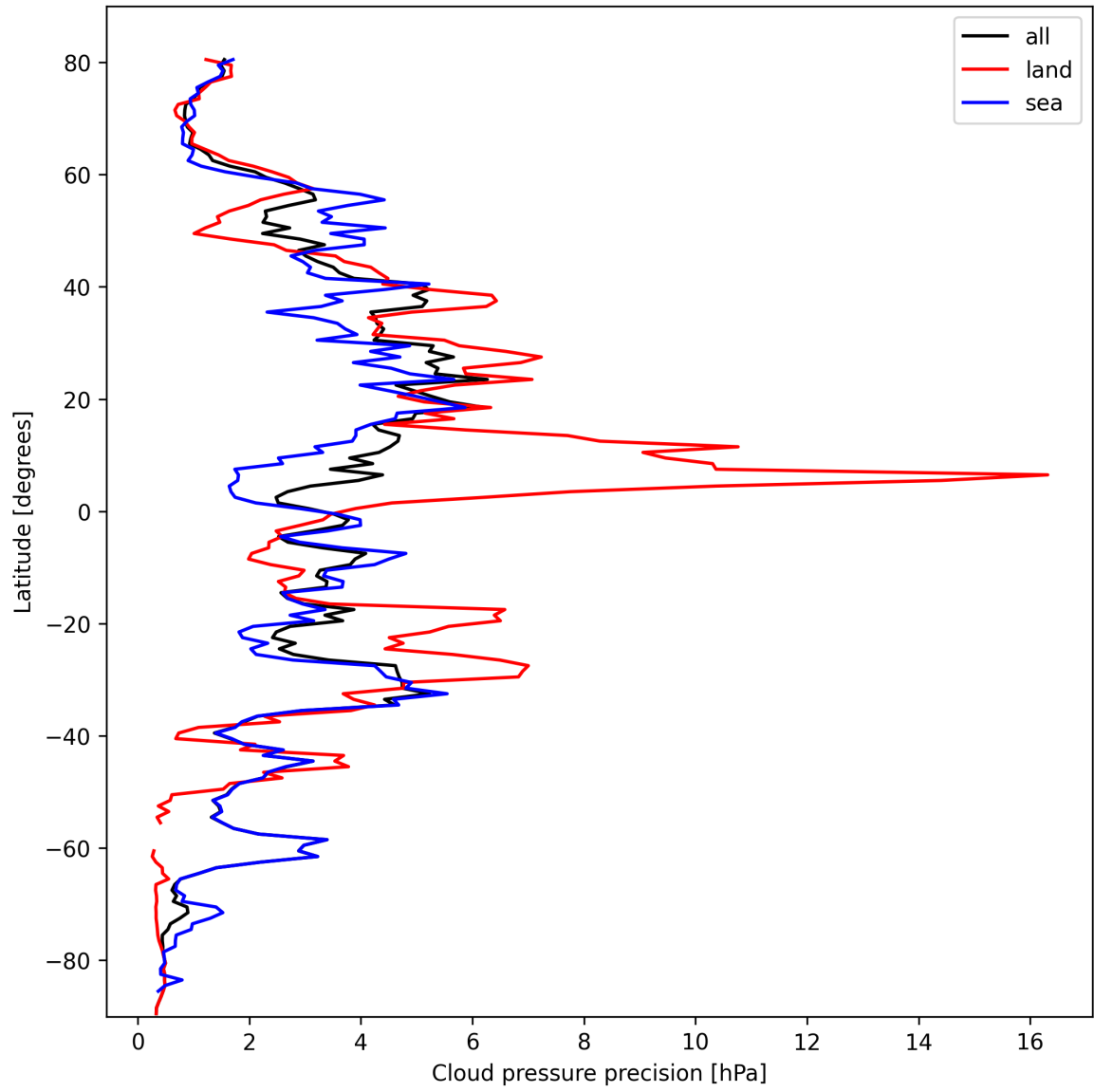
Figure 12: Zonal average of “Cloud pressure precision” for 2025-02-28 to 2025-03-01.
