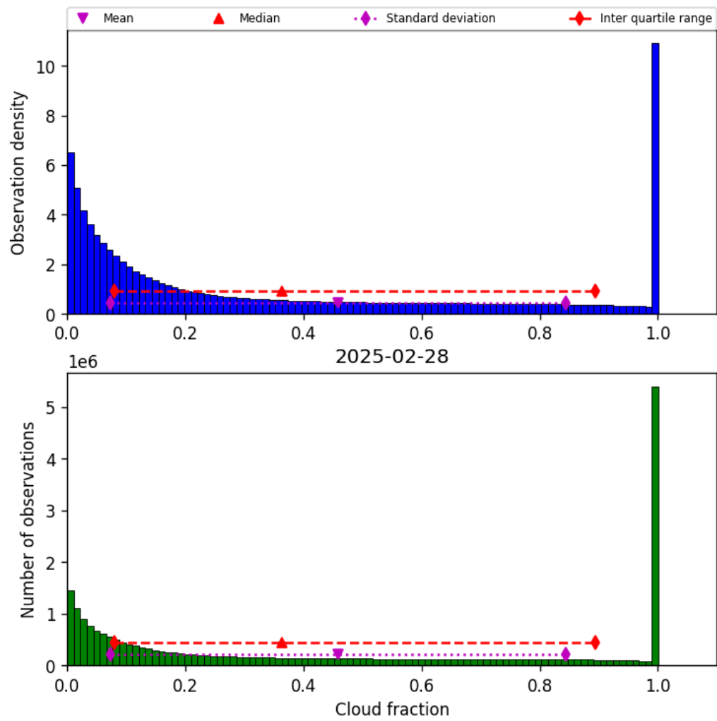
Figure 30: Histogram of “Cloud fraction” for 2025-02-28 to 2025-03-01
