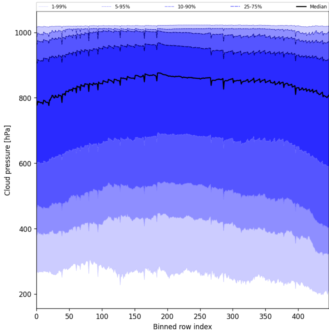
Figure 45: Along track statistics of “Cloud pressure” for 2025-02-28 to 2025-03-01
