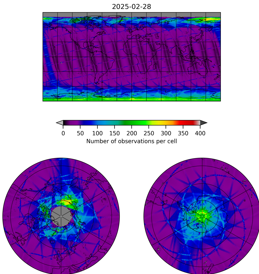
Figure 9: Map of the number of observations for 2025-02-28 to 2025-03-01
