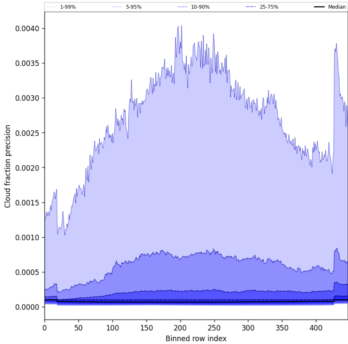
Figure 48: Along track statistics of “Cloud fraction precision” for 2025-02-28 to 2025-03-01
