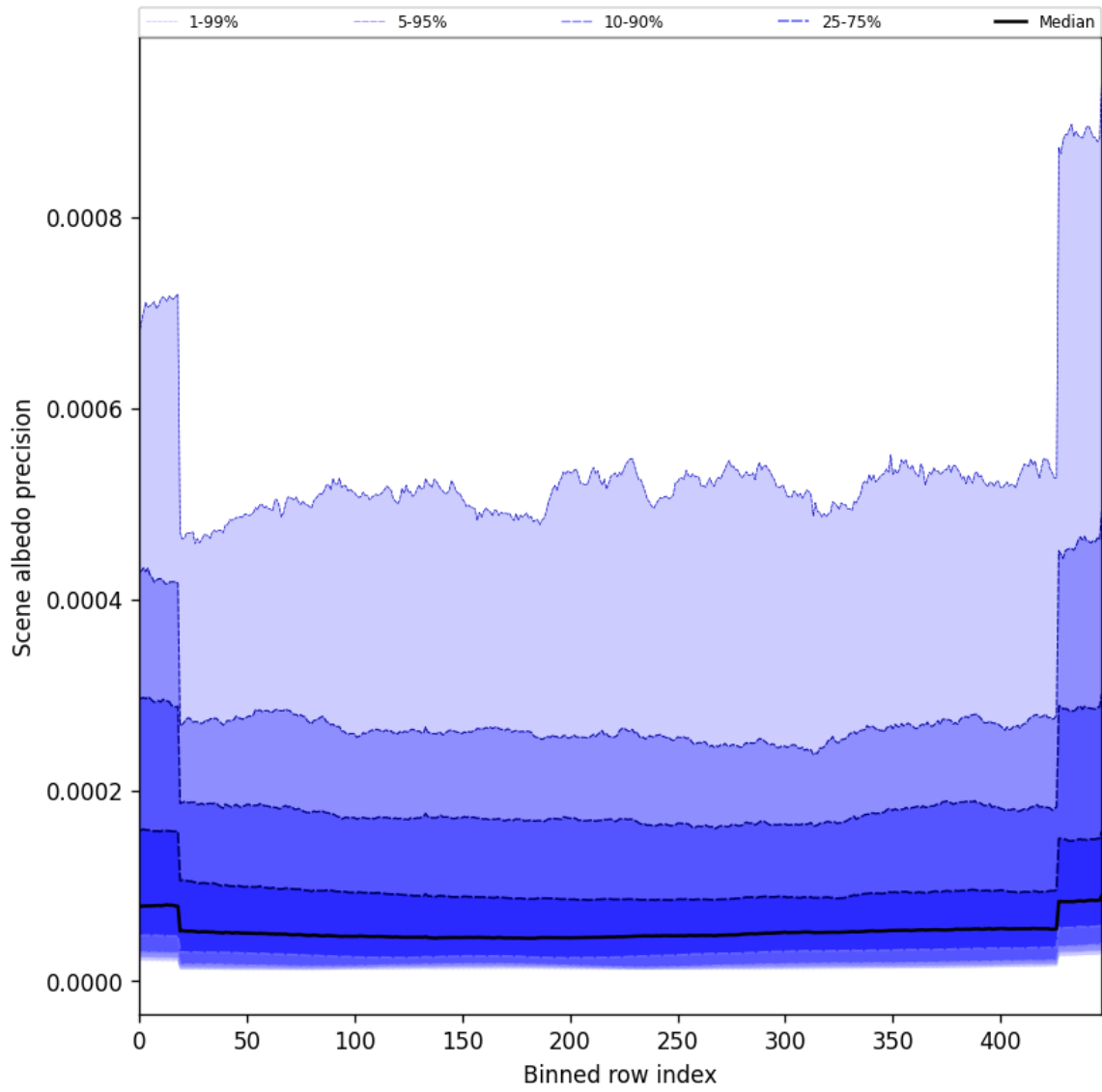
Figure 50: Along track statistics of “Scene albedo precision” for 2025-02-28 to 2025-03-01
