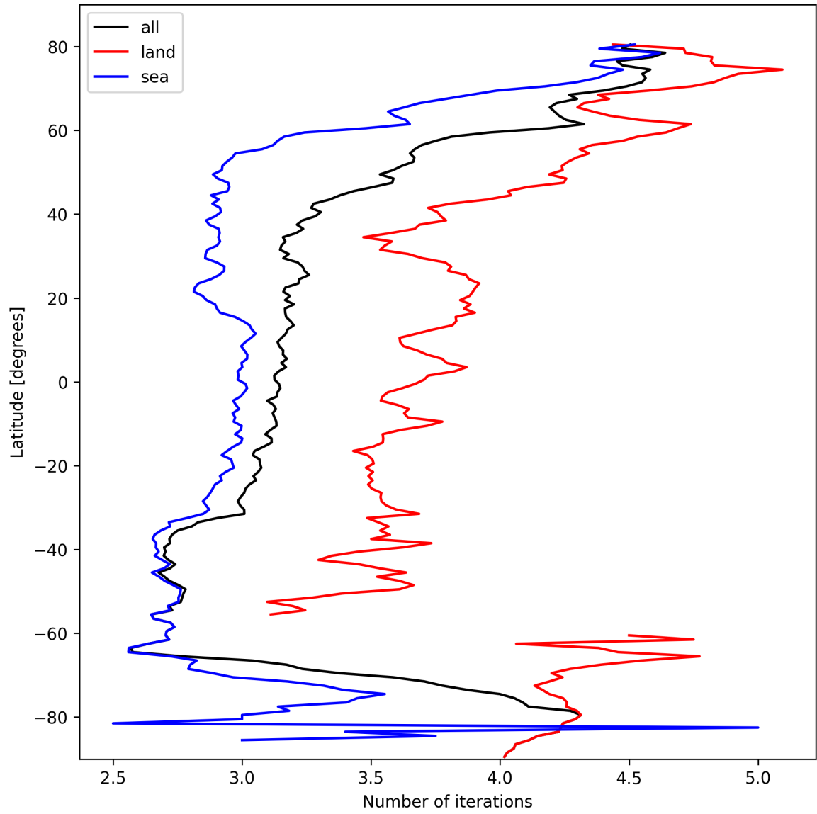
Figure 20: Zonal average of “Number of iterations” for 2025-02-28 to 2025-03-01.
