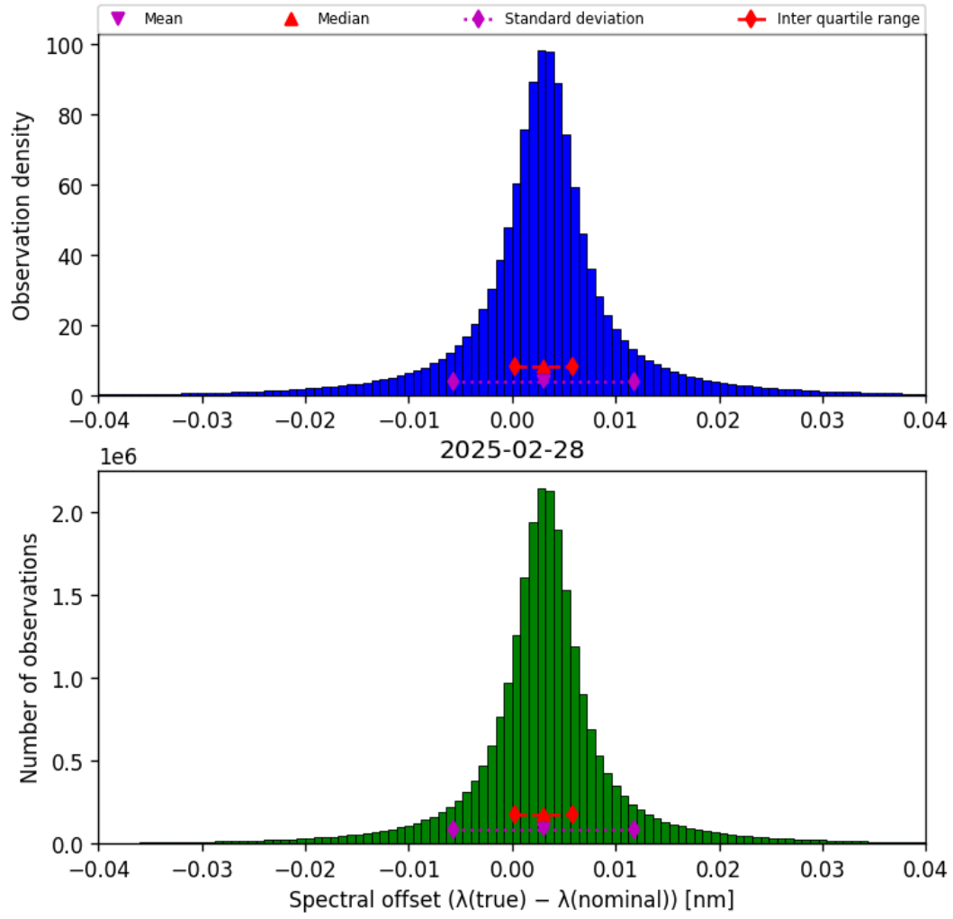
Figure 43: Histogram of “Spectral offset ( \lambda_{\text{true}} - \lambda_{\text{nominal}} )” for 2025-02-28 to 2025-03-01
