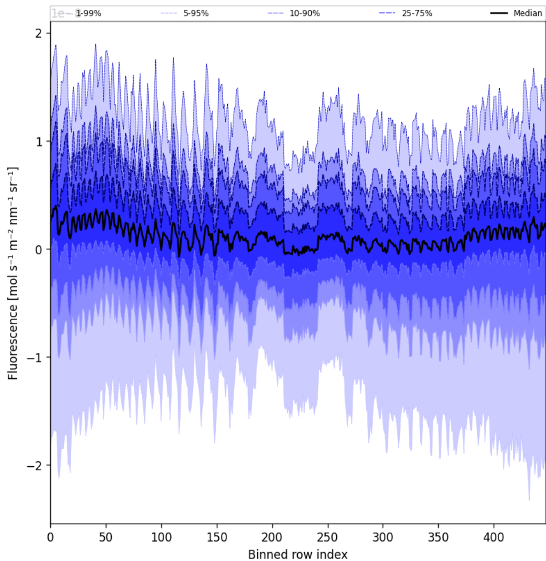
Figure 55: Along track statistics of “Fluorescence” for 2025-02-28 to 2025-03-01
