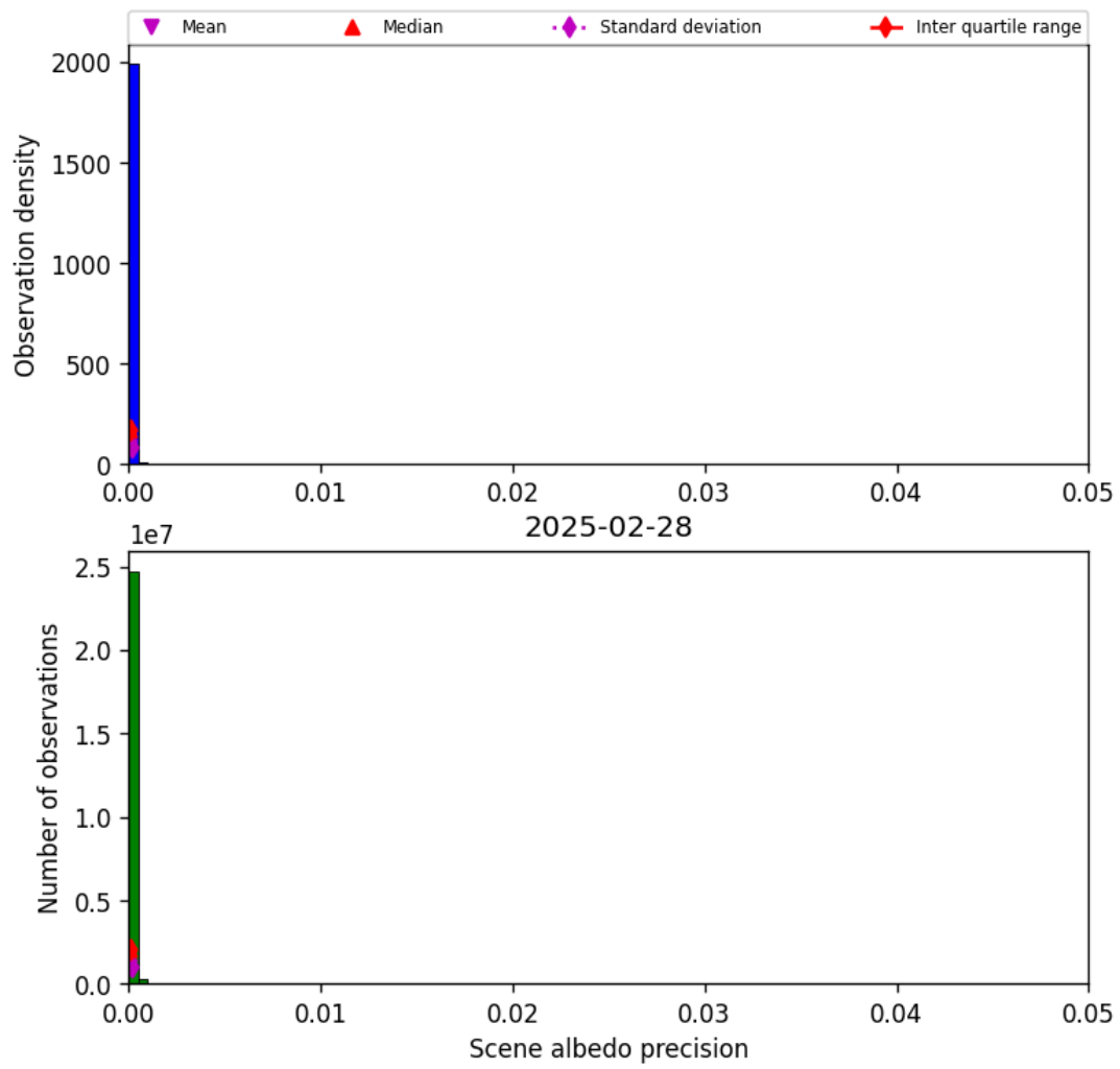
Figure 33: Histogram of “Scene albedo precision” for 2025-02-28 to 2025-03-01
