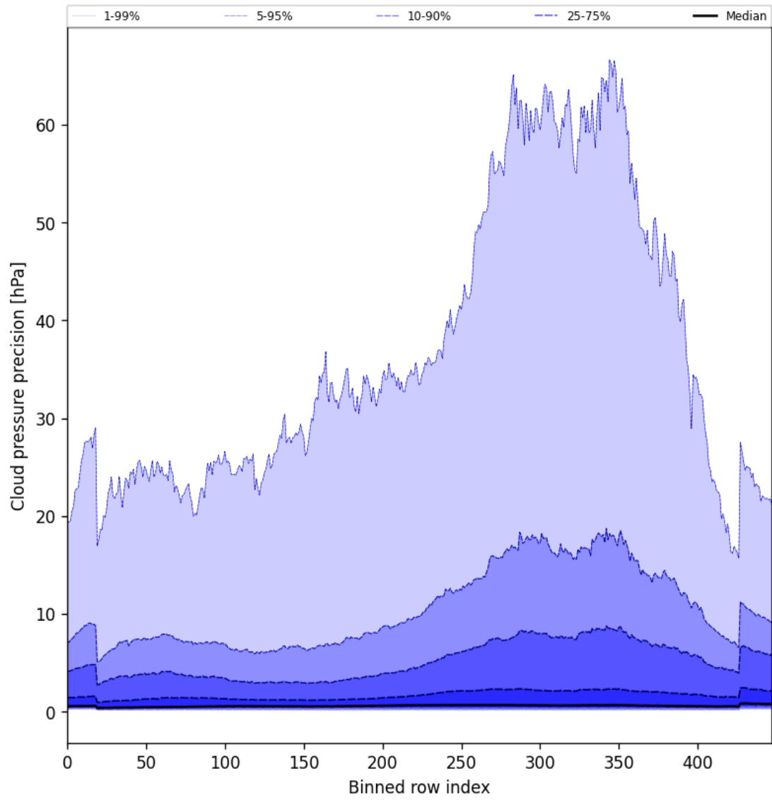
Figure 46: Along track statistics of “Cloud pressure precision” for 2025-02-28 to 2025-03-01
