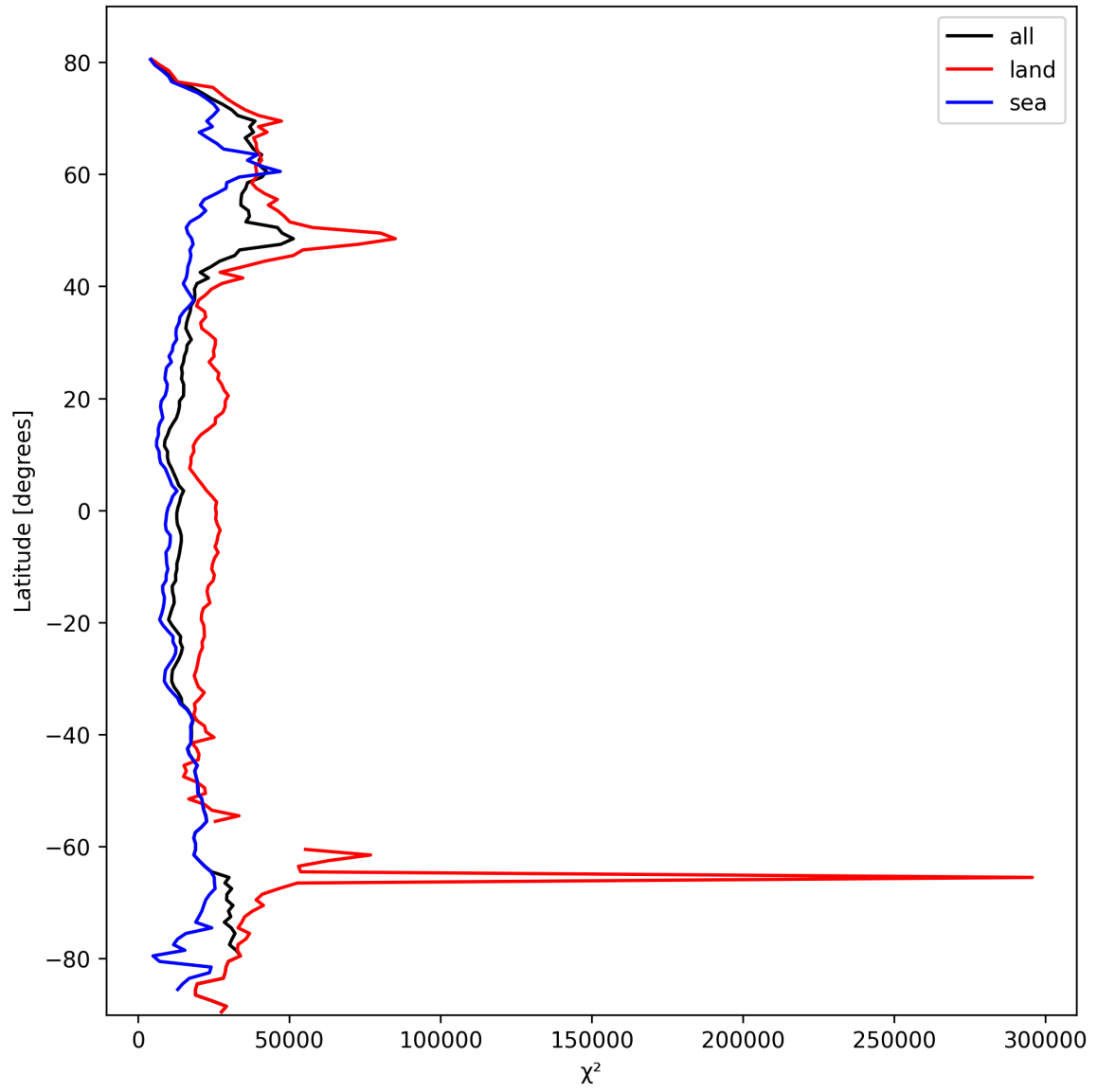
Figure 19: Zonal average of “ \chi^2 ” for 2025-02-28 to 2025-03-01.
