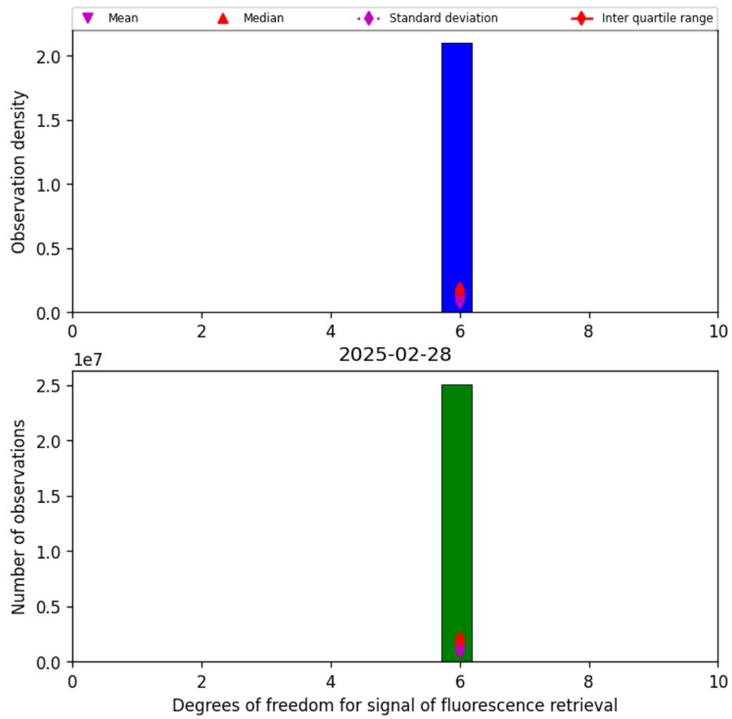
Figure 41: Histogram of “Degrees of freedom for signal of fluorescence retrieval” for 2025-02-28 to 2025-03-01
