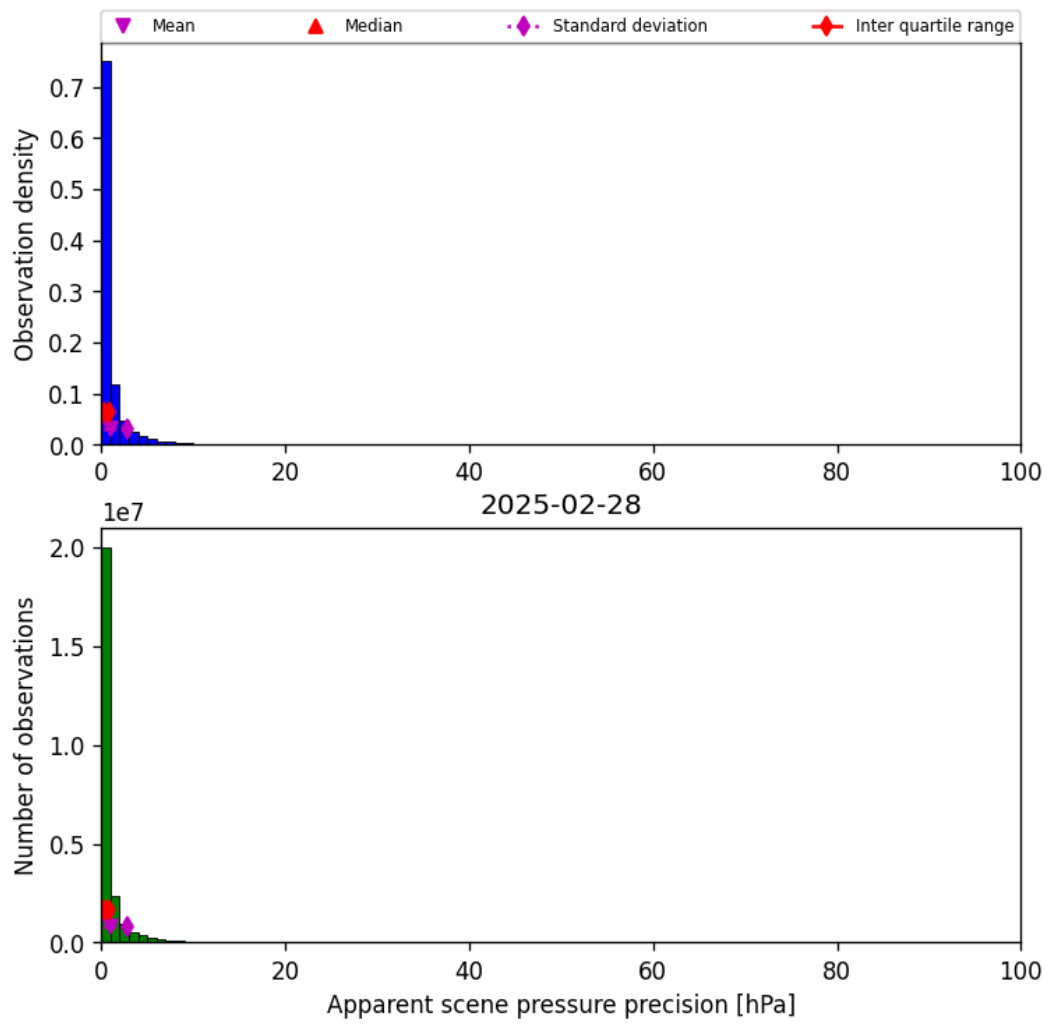
Figure 35: Histogram of “Apparent scene pressure precision” for 2025-02-28 to 2025-03-01
