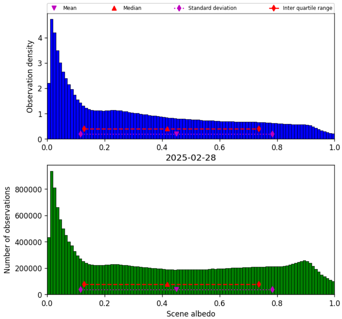
Figure 32: Histogram of “Scene albedo” for 2025-02-28 to 2025-03-01
