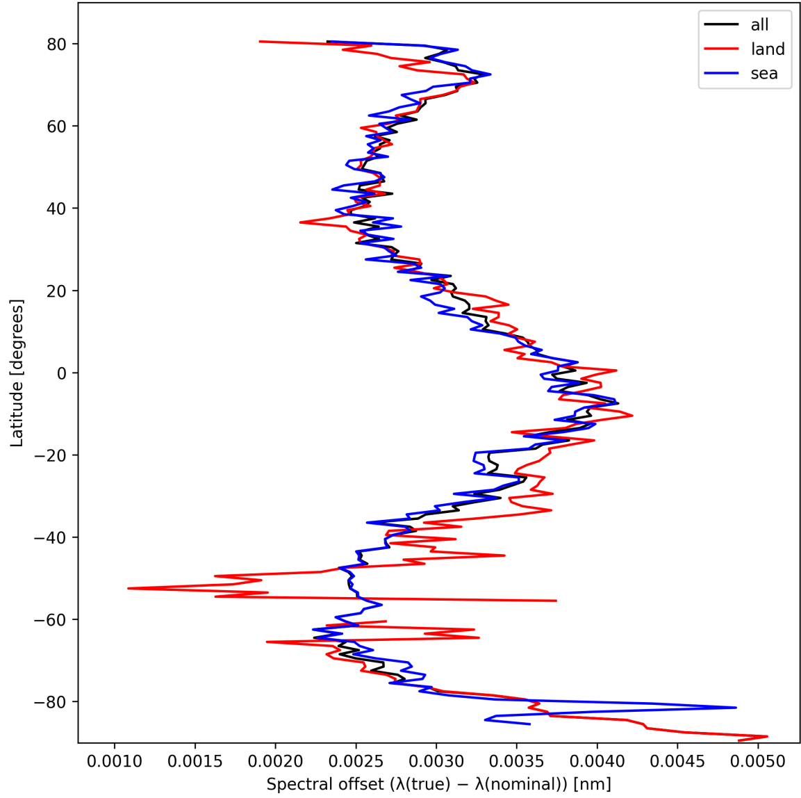
Figure 26: Zonal average of “Spectral offset ( \lambda_{\text{true}} - \lambda_{\text{nominal}} )” for 2025-02-28 to 2025-03-01.
