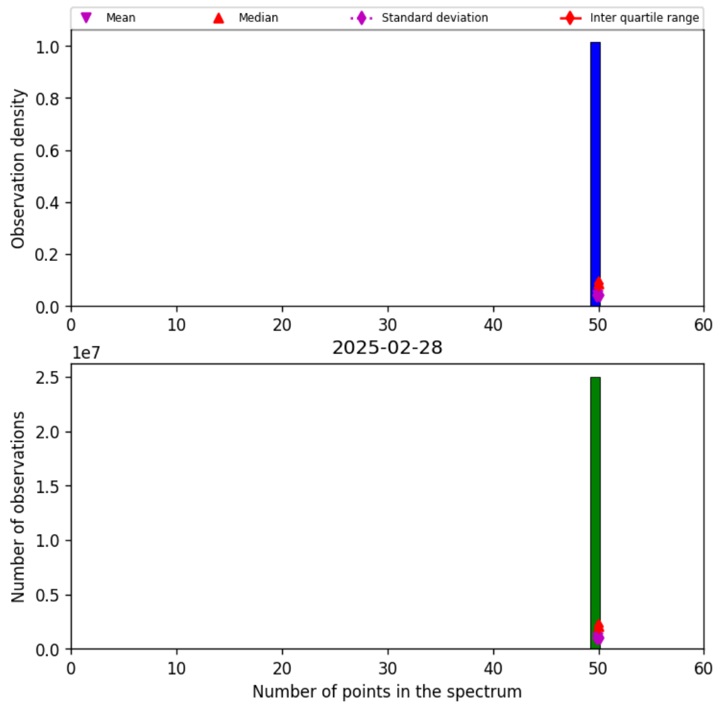
Figure 42: Histogram of “Number of points in the spectrum” for 2025-02-28 to 2025-03-01
