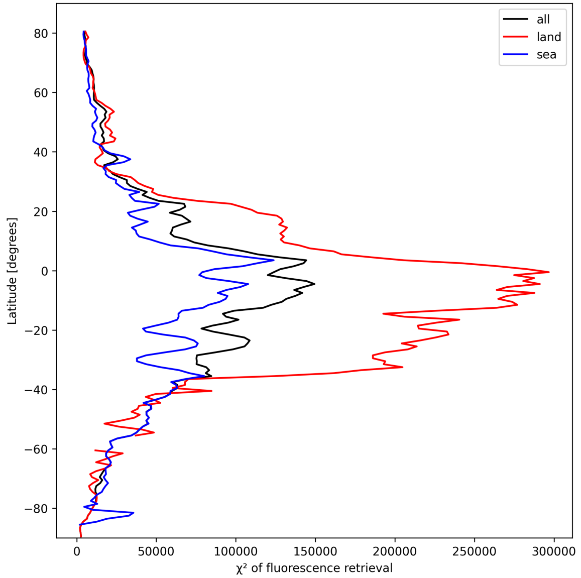
Figure 23: Zonal average of “ \chi^2 of fluorescence retrieval” for 2025-02-28 to 2025-03-01.
