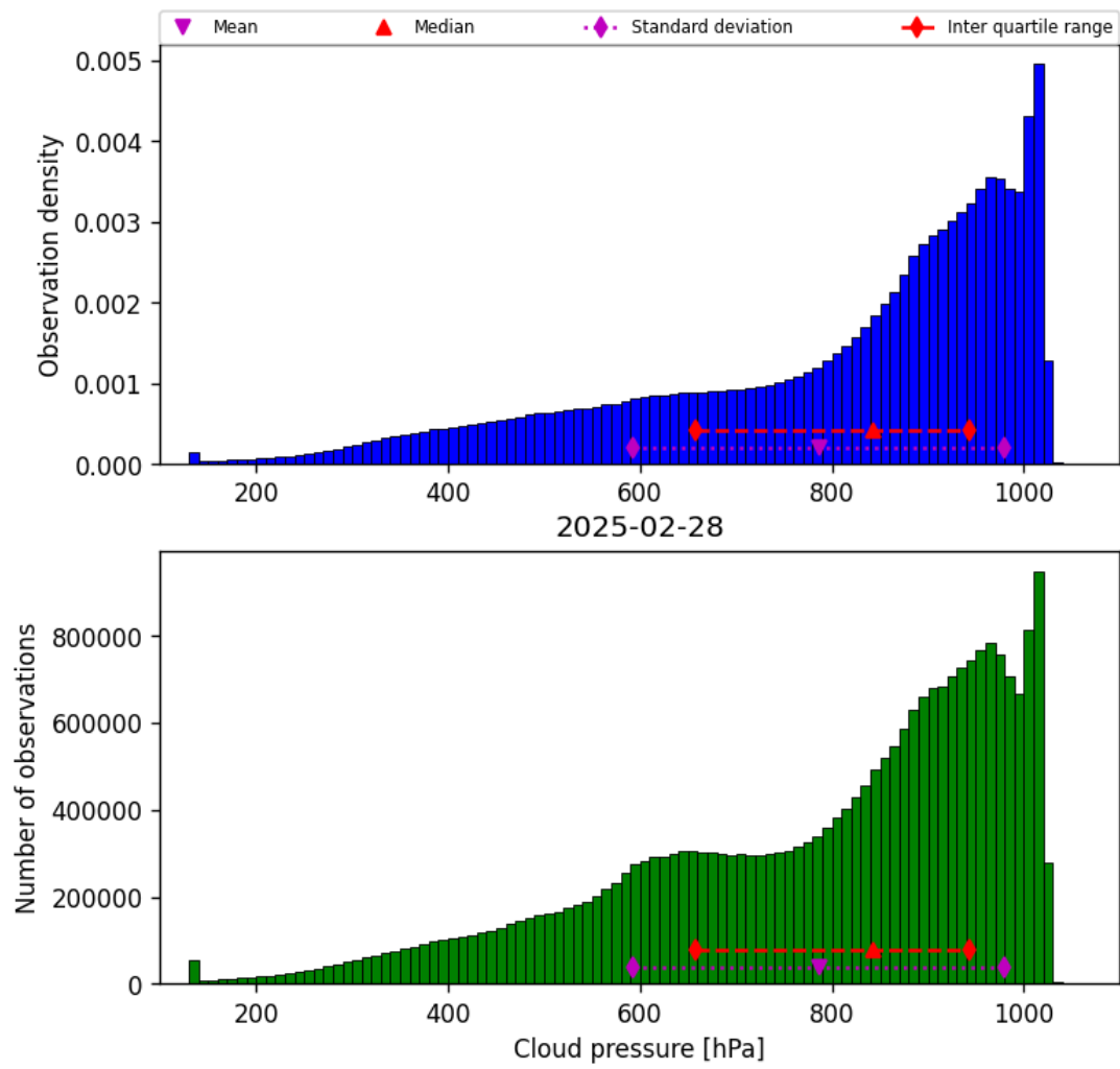
Figure 28: Histogram of “Cloud pressure” for 2025-02-28 to 2025-03-01
