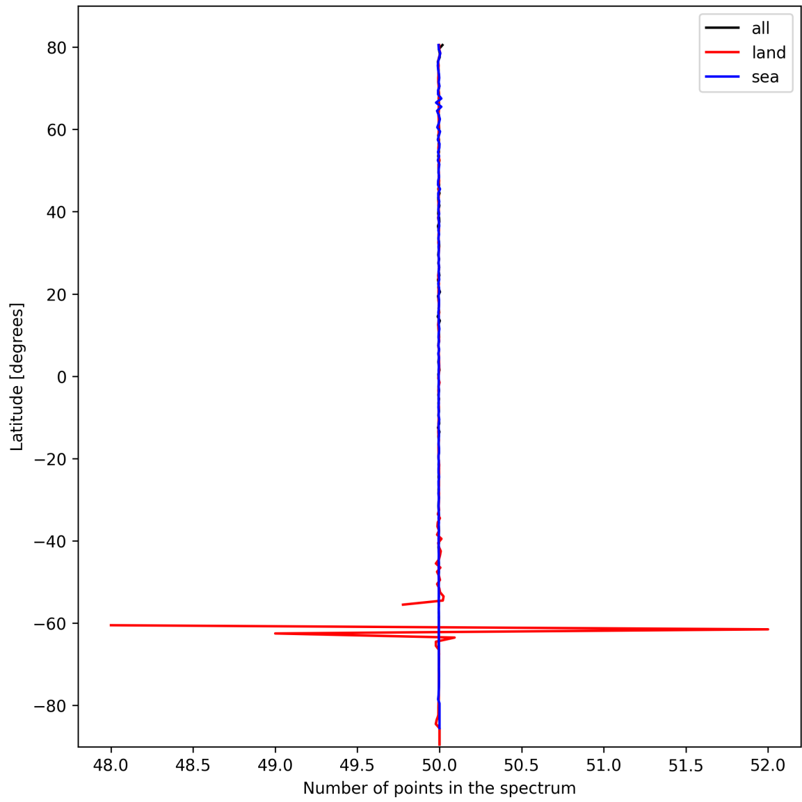
Figure 25: Zonal average of “Number of points in the spectrum” for 2025-02-28 to 2025-03-01.
