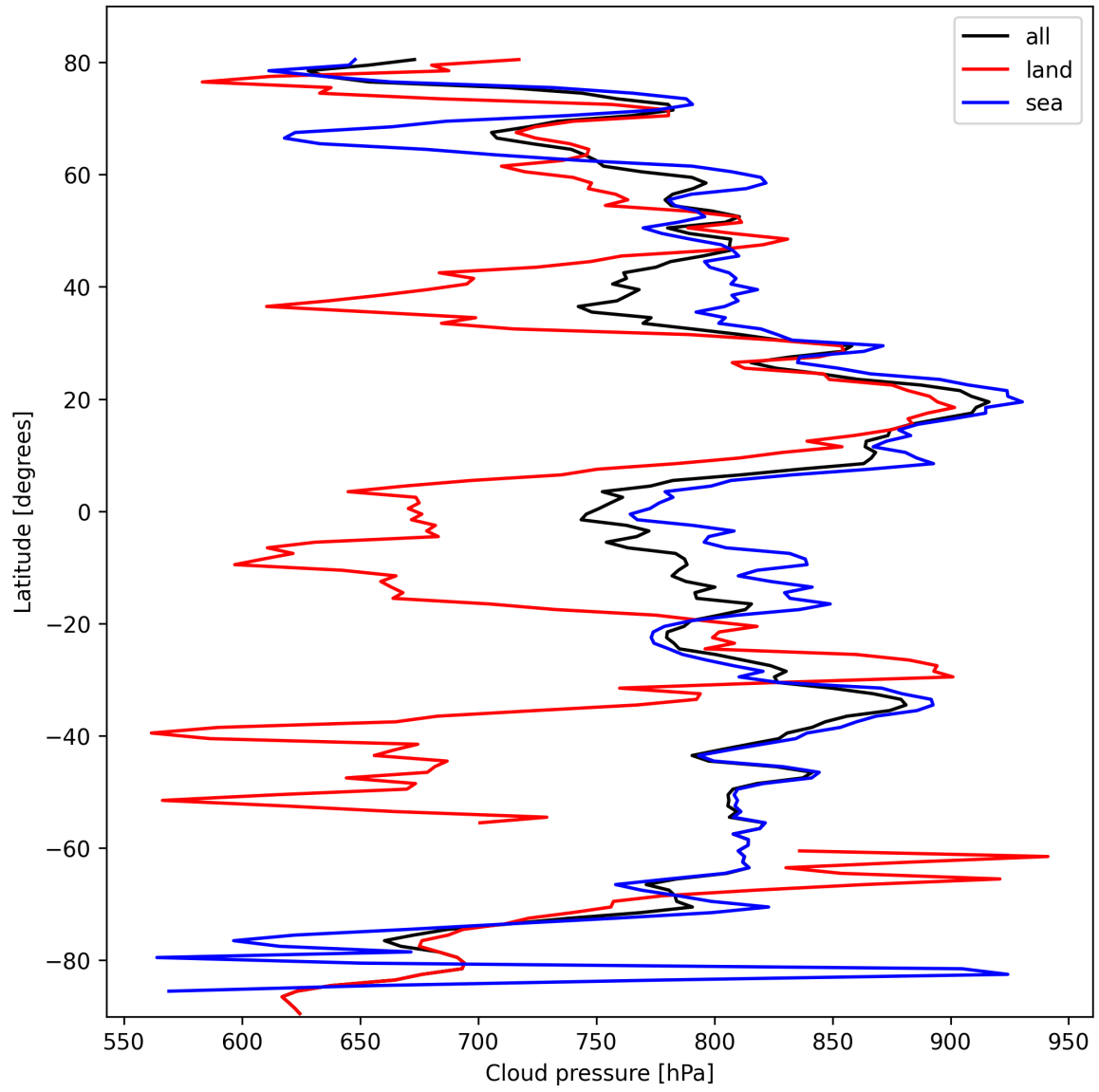
Figure 11: Zonal average of “Cloud pressure” for 2025-02-28 to 2025-03-01.
