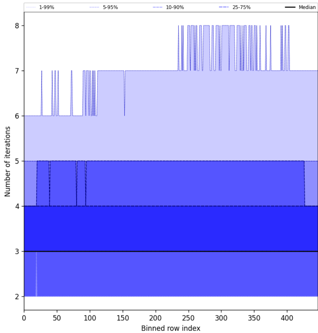
Figure 54: Along track statistics of “Number of iterations” for 2025-02-28 to 2025-03-01
