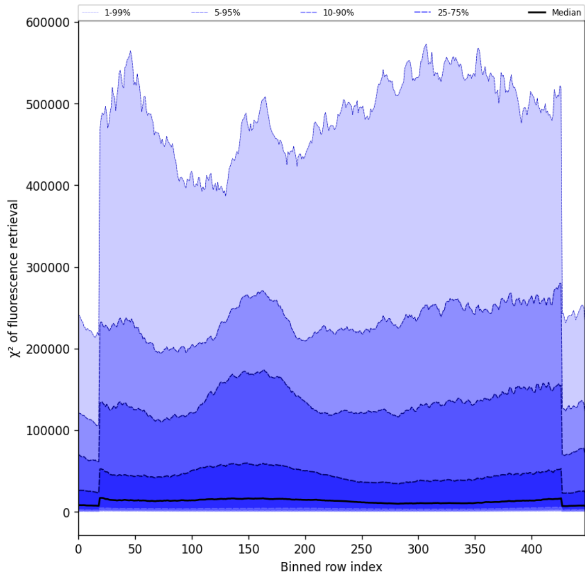
Figure 57: Along track statistics of “ \chi^2 of fluorescence retrieval” for 2025-02-28 to 2025-03-01
