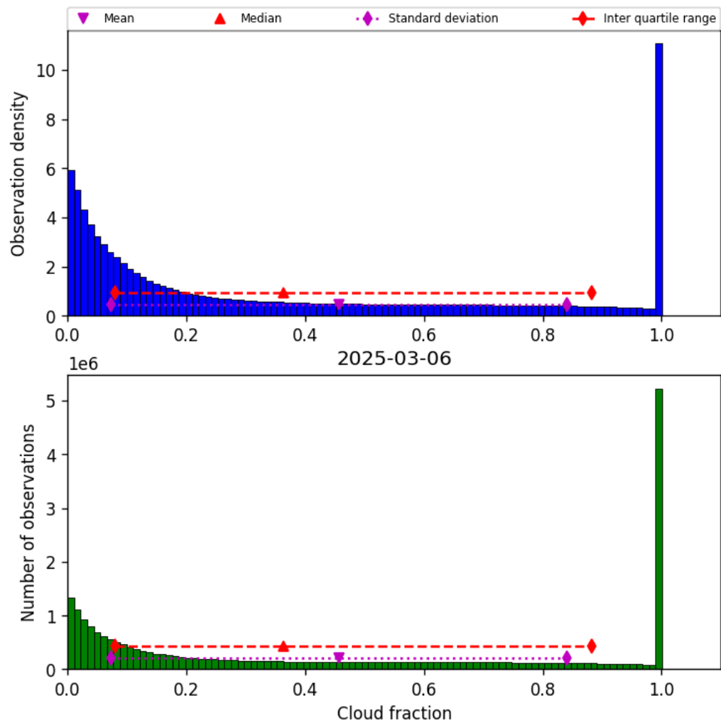
Figure 30: Histogram of “Cloud fraction” for 2025-03-06 to 2025-03-07
