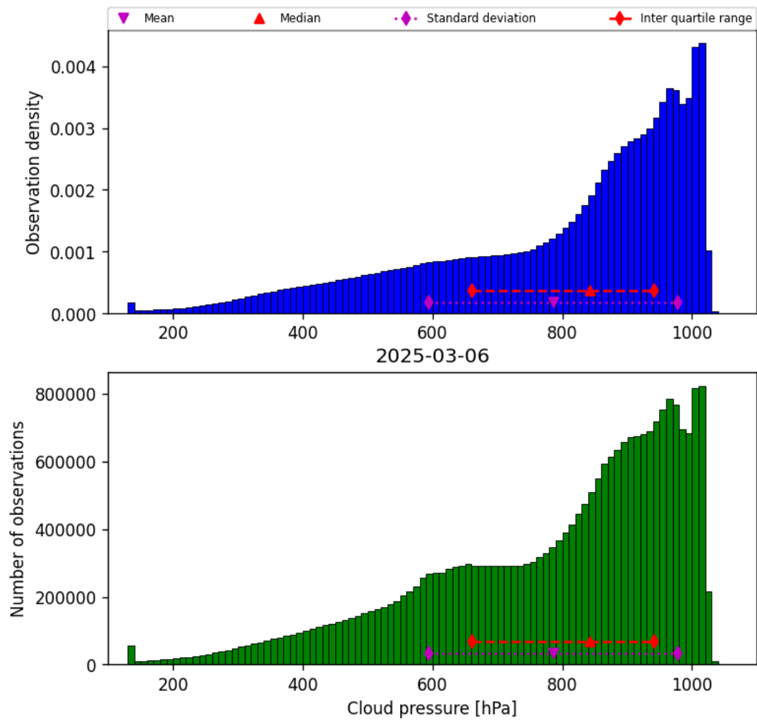
Figure 28: Histogram of “Cloud pressure” for 2025-03-06 to 2025-03-07
