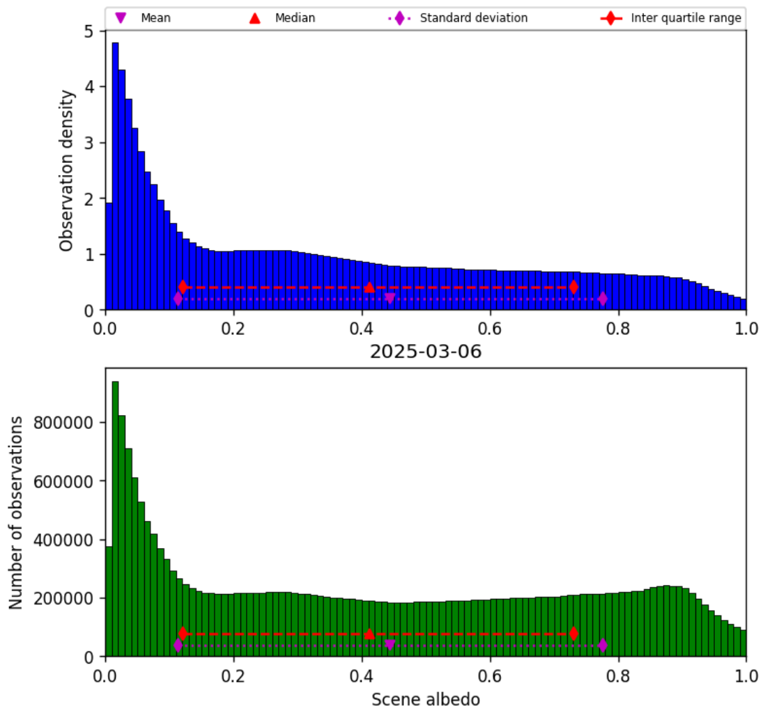
Figure 32: Histogram of “Scene albedo” for 2025-03-06 to 2025-03-07
