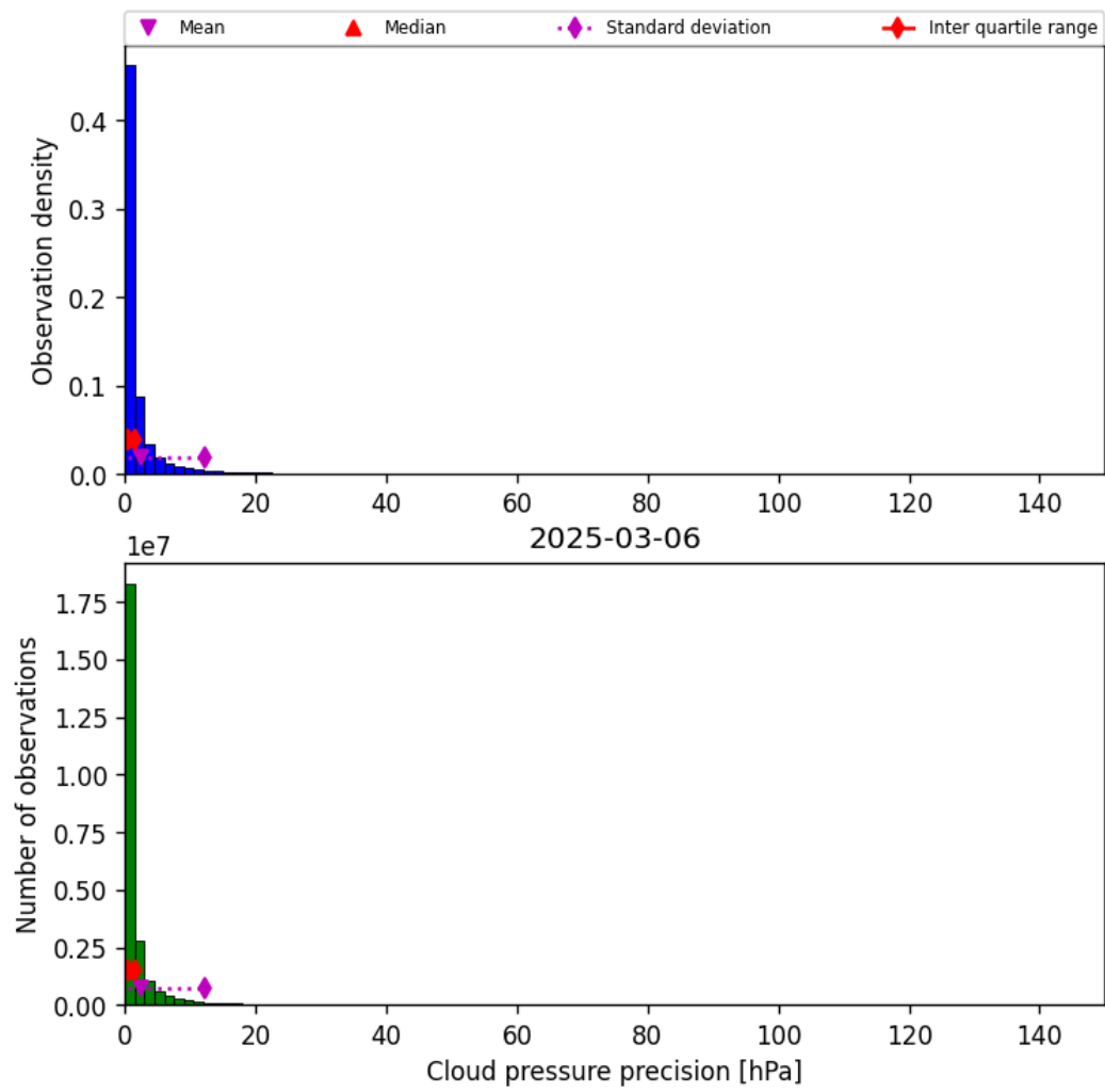
Figure 29: Histogram of “Cloud pressure precision” for 2025-03-06 to 2025-03-07
