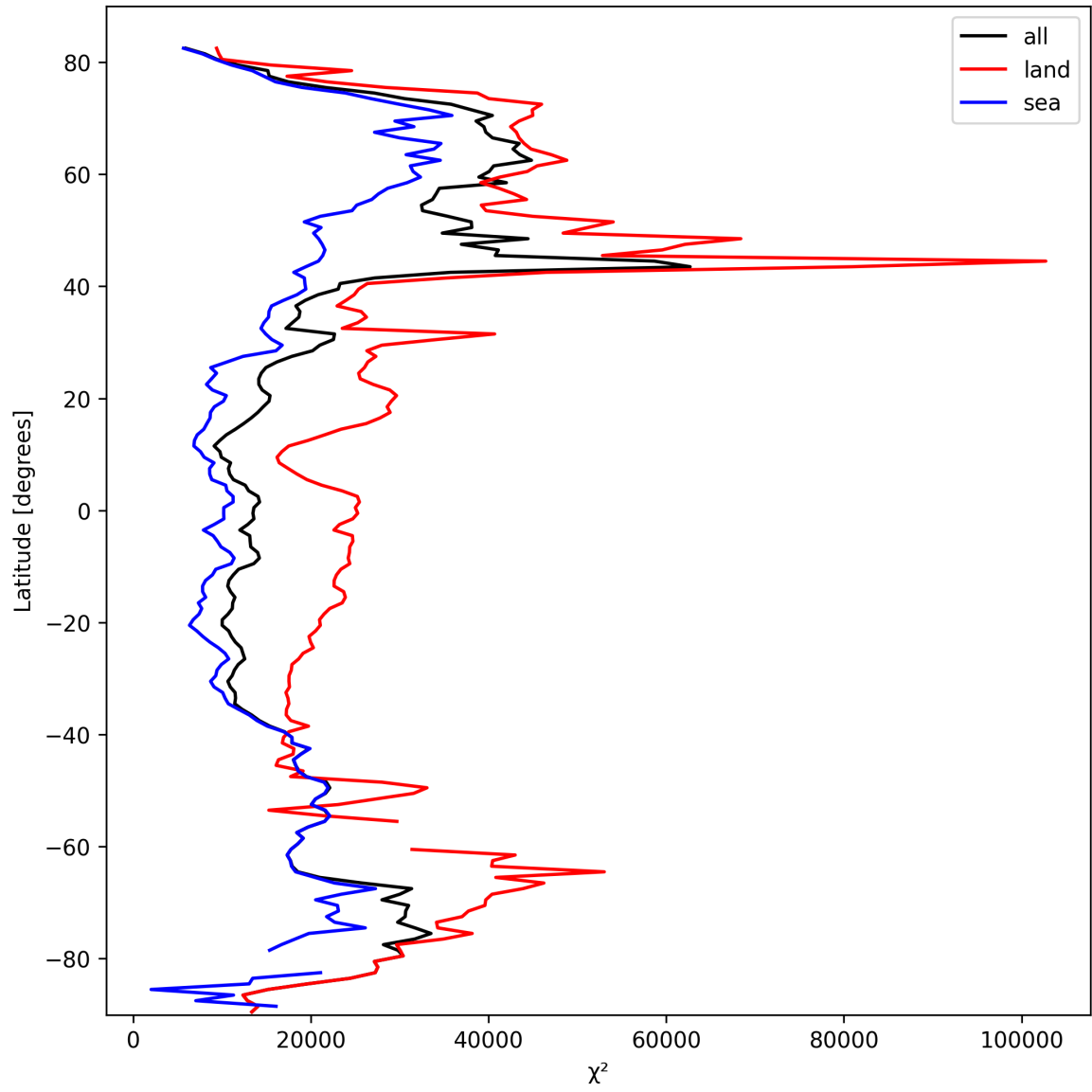
Figure 19: Zonal average of “ \chi^2 ” for 2025-03-06 to 2025-03-07.
