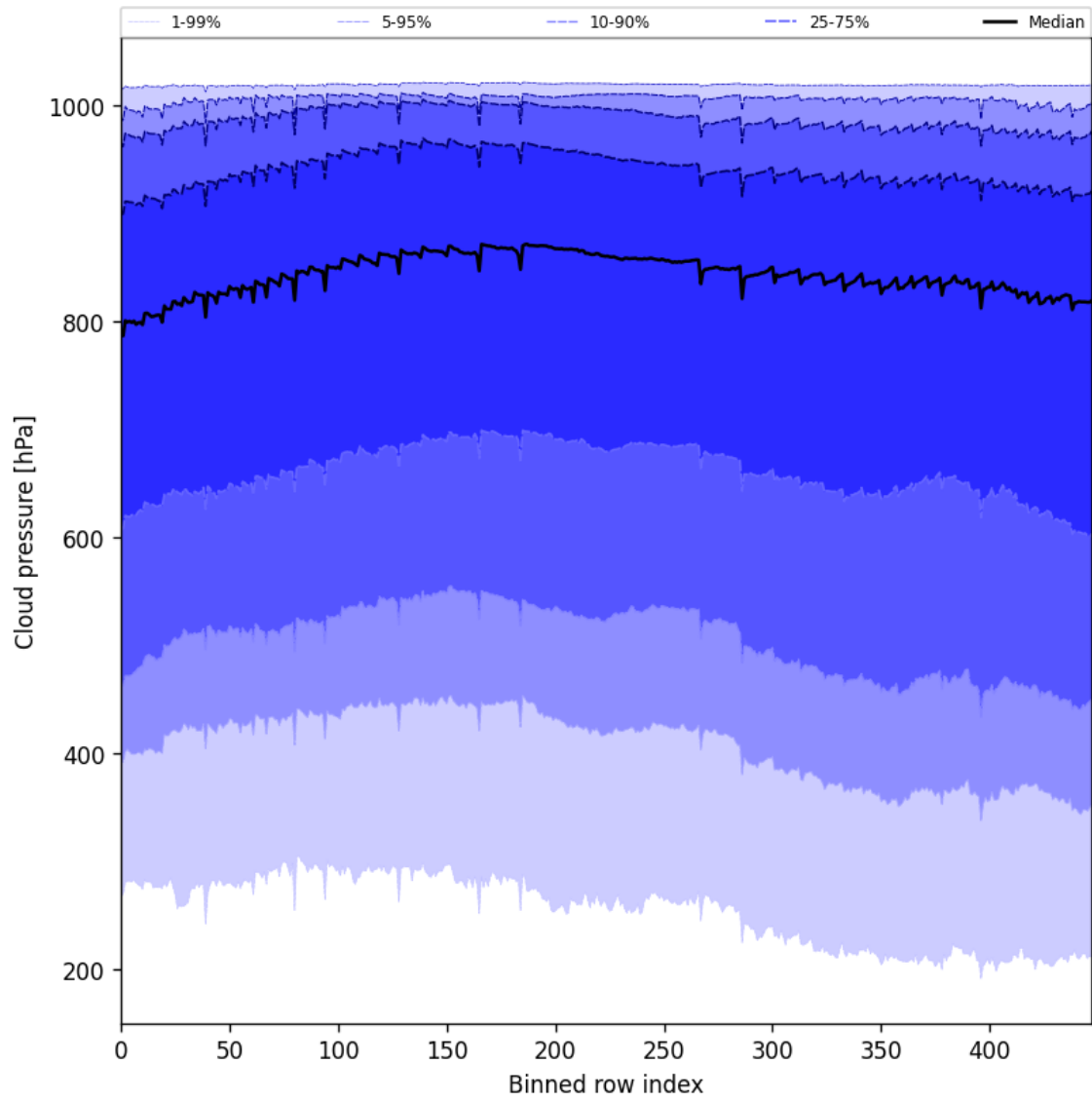
Figure 45: Along track statistics of “Cloud pressure” for 2025-03-06 to 2025-03-07
