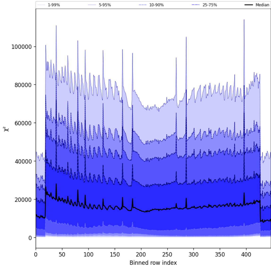
Figure 53: Along track statistics of “ \chi^2 ” for 2025-03-06 to 2025-03-07
