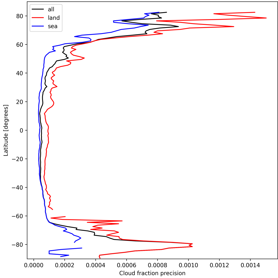
Figure 14: Zonal average of “Cloud fraction precision” for 2025-03-06 to 2025-03-07.
