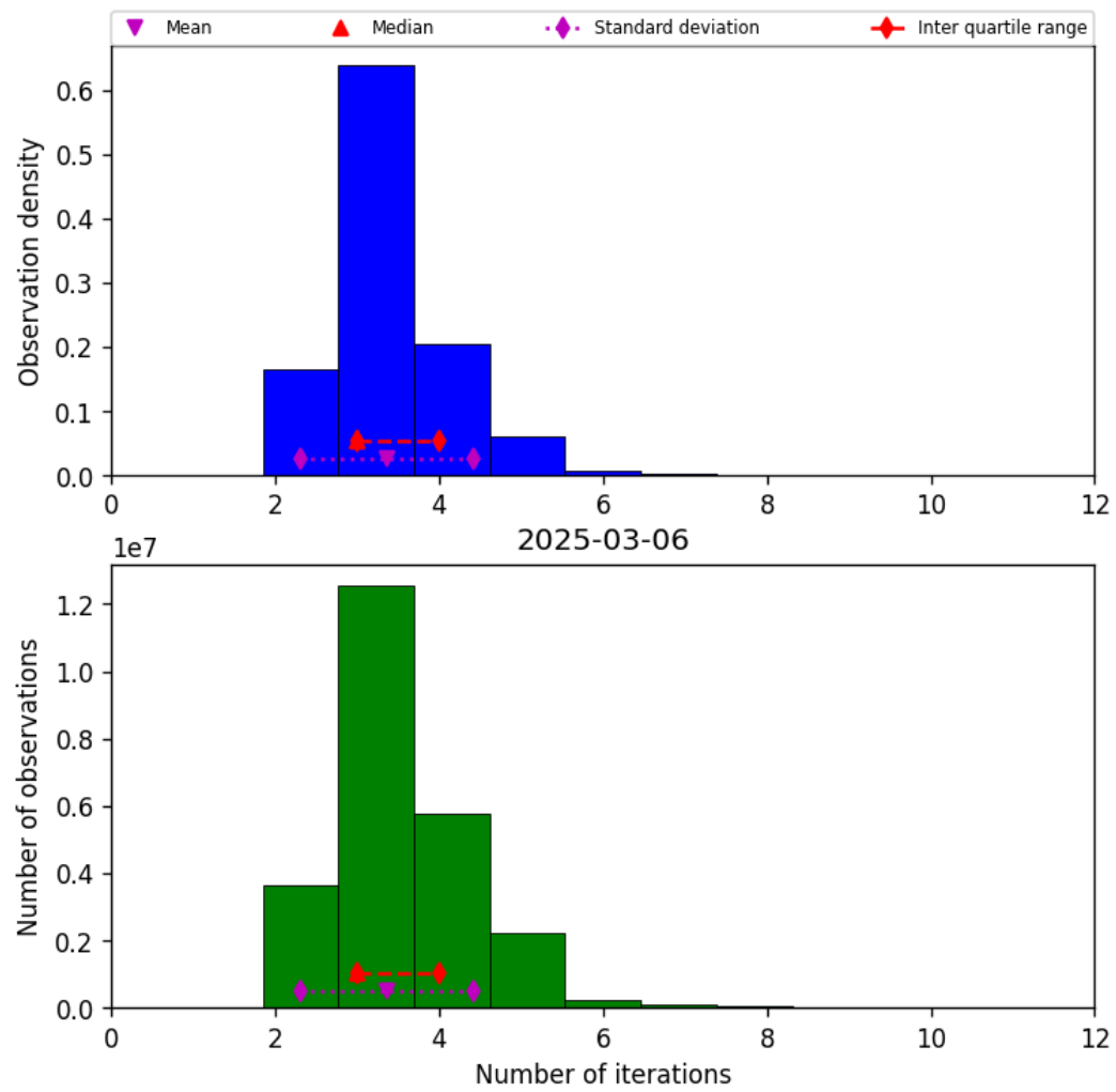
Figure 37: Histogram of “Number of iterations” for 2025-03-06 to 2025-03-07
