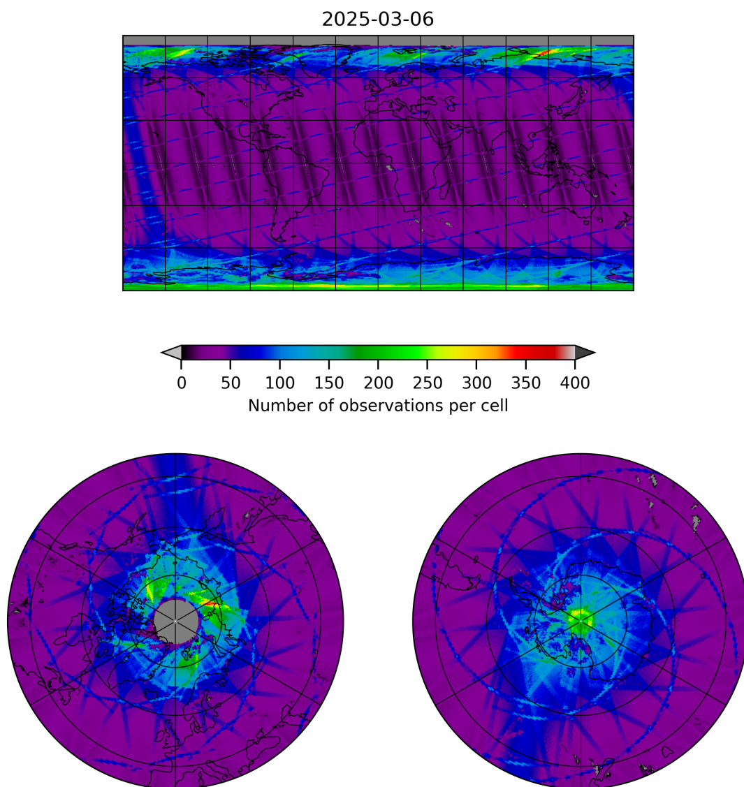
Figure 9: Map of the number of observations for 2025-03-06 to 2025-03-07
