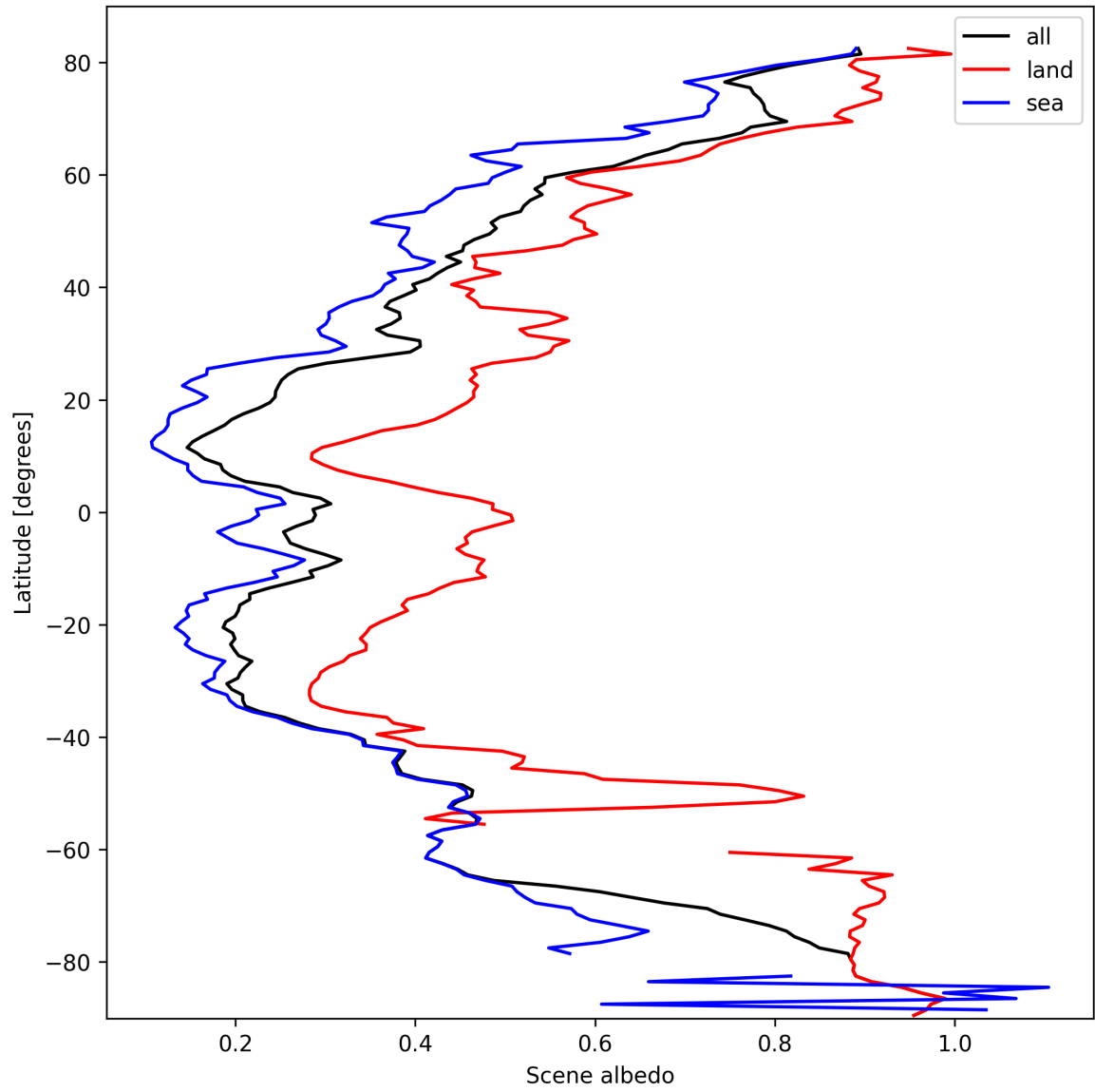
Figure 15: Zonal average of “Scene albedo” for 2025-03-06 to 2025-03-07.
