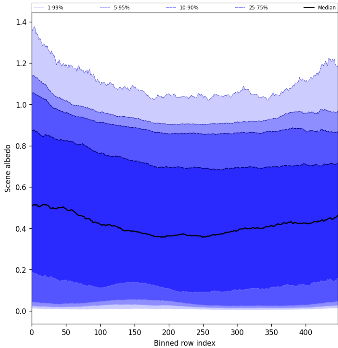
Figure 49: Along track statistics of “Scene albedo” for 2025-03-06 to 2025-03-07
