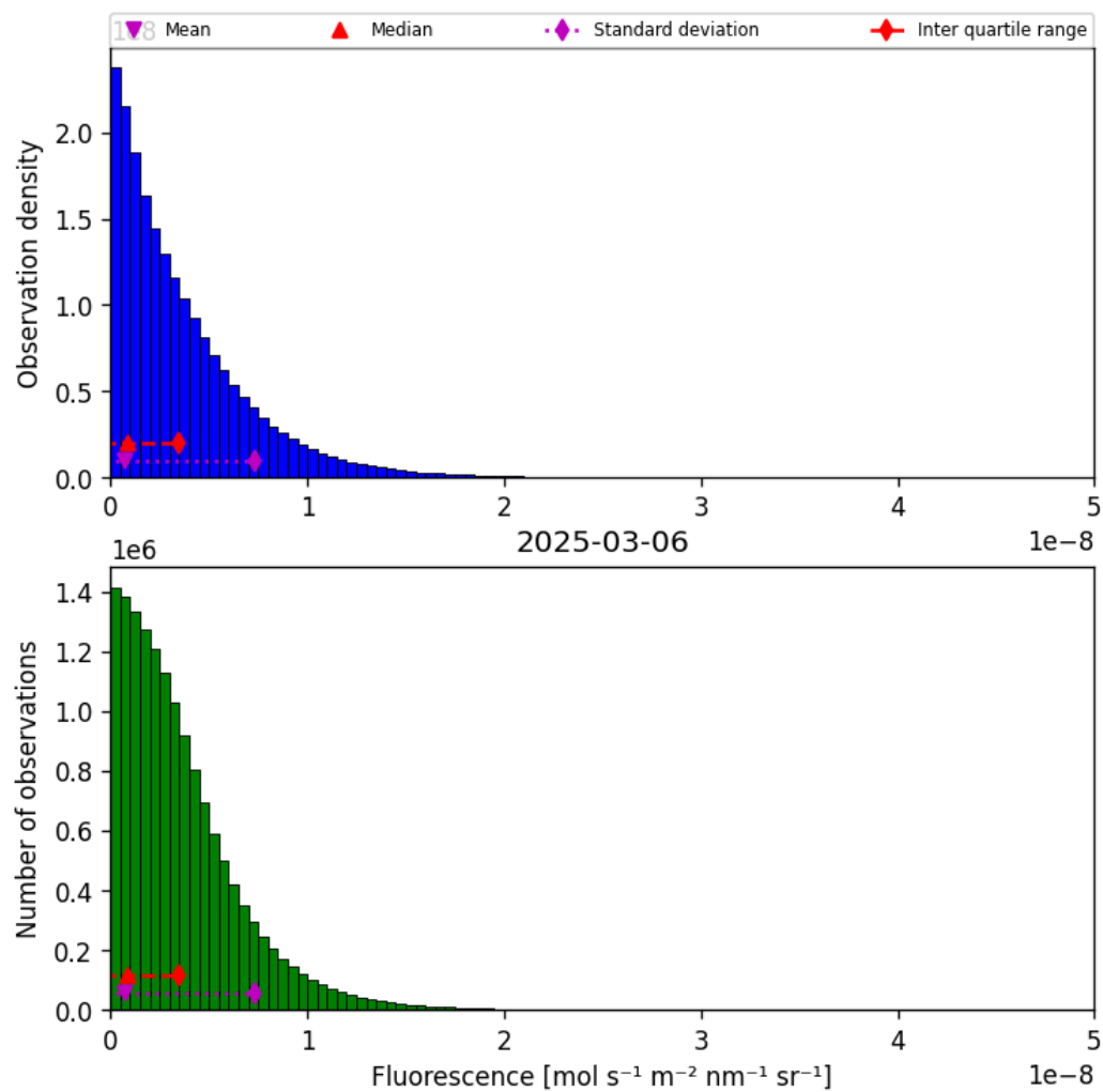
Figure 38: Histogram of “Fluorescence” for 2025-03-06 to 2025-03-07
