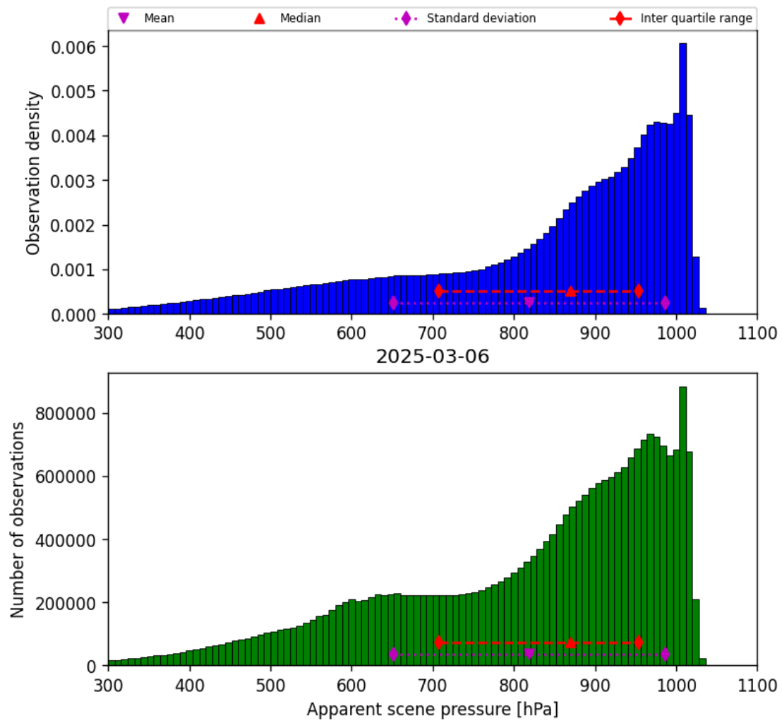
Figure 34: Histogram of “Apparent scene pressure” for 2025-03-06 to 2025-03-07
