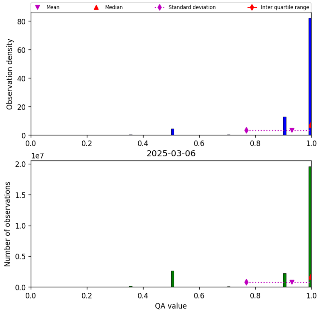
Figure 27: Histogram of “QA value” for 2025-03-06 to 2025-03-07
