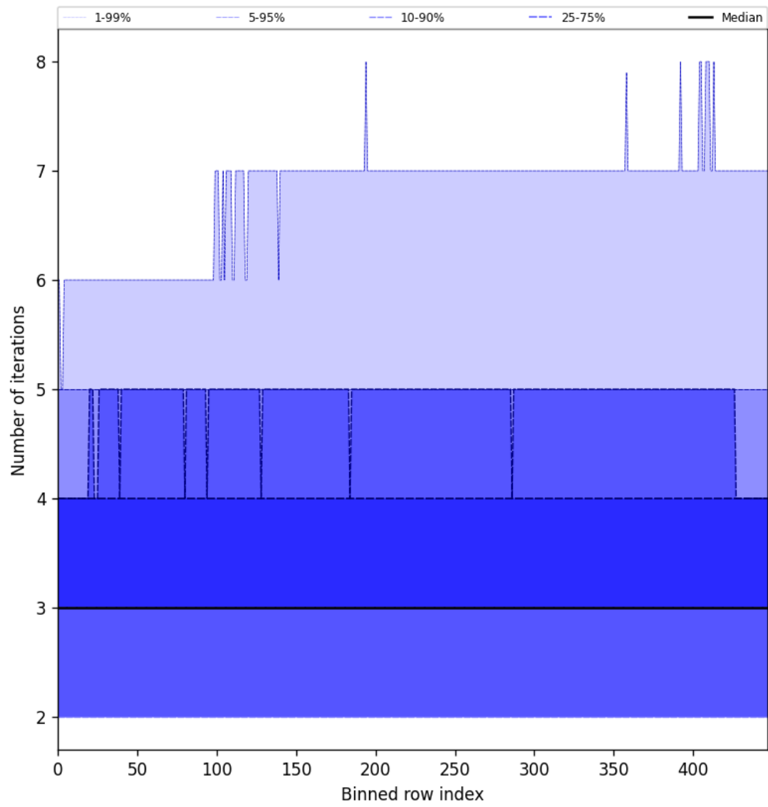
Figure 54: Along track statistics of “Number of iterations” for 2025-03-06 to 2025-03-07
