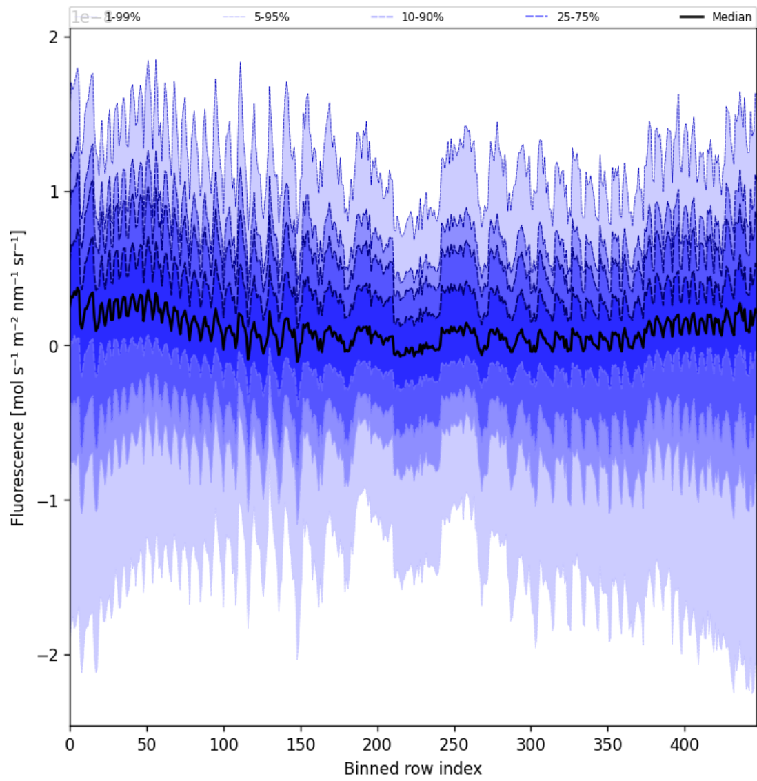
Figure 55: Along track statistics of “Fluorescence” for 2025-03-06 to 2025-03-07
