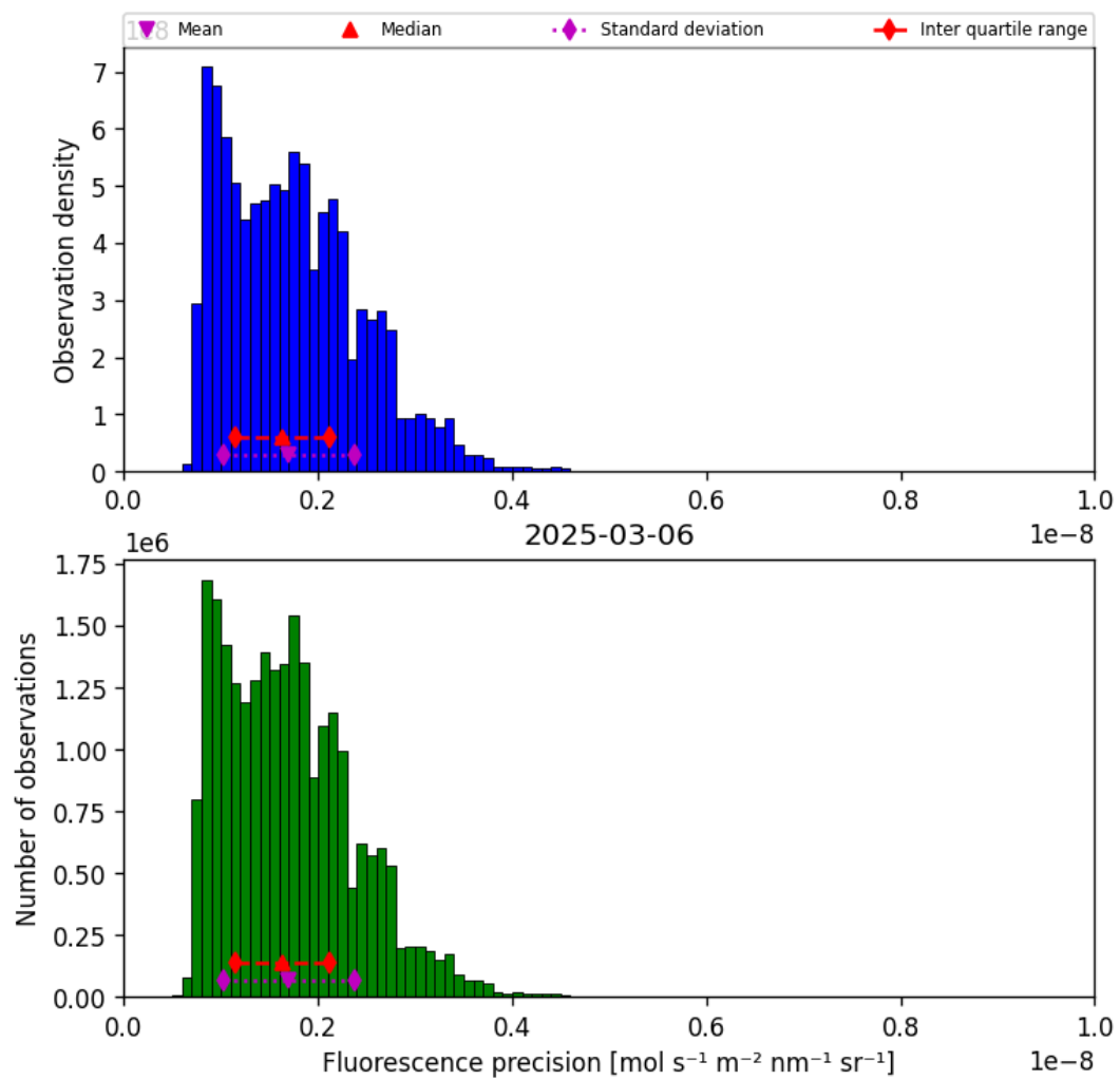
Figure 39: Histogram of “Fluorescence precision” for 2025-03-06 to 2025-03-07
