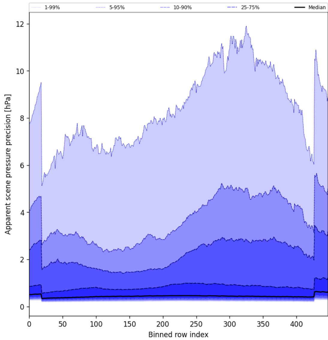
Figure 52: Along track statistics of “Apparent scene pressure precision” for 2025-03-06 to 2025-03-07
