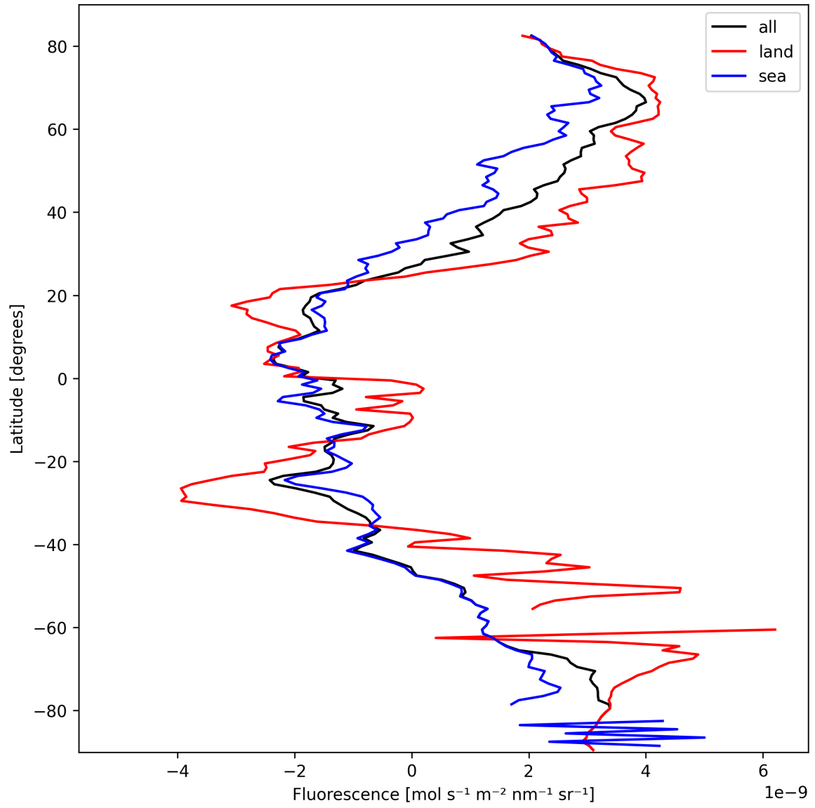
Figure 21: Zonal average of “Fluorescence” for 2025-03-06 to 2025-03-07.
