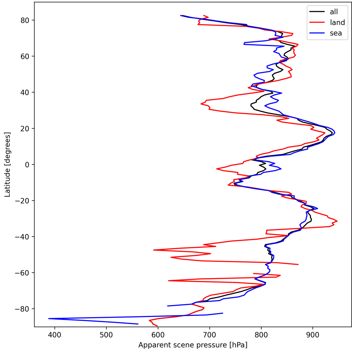
Figure 17: Zonal average of “Apparent scene pressure” for 2025-03-06 to 2025-03-07.
