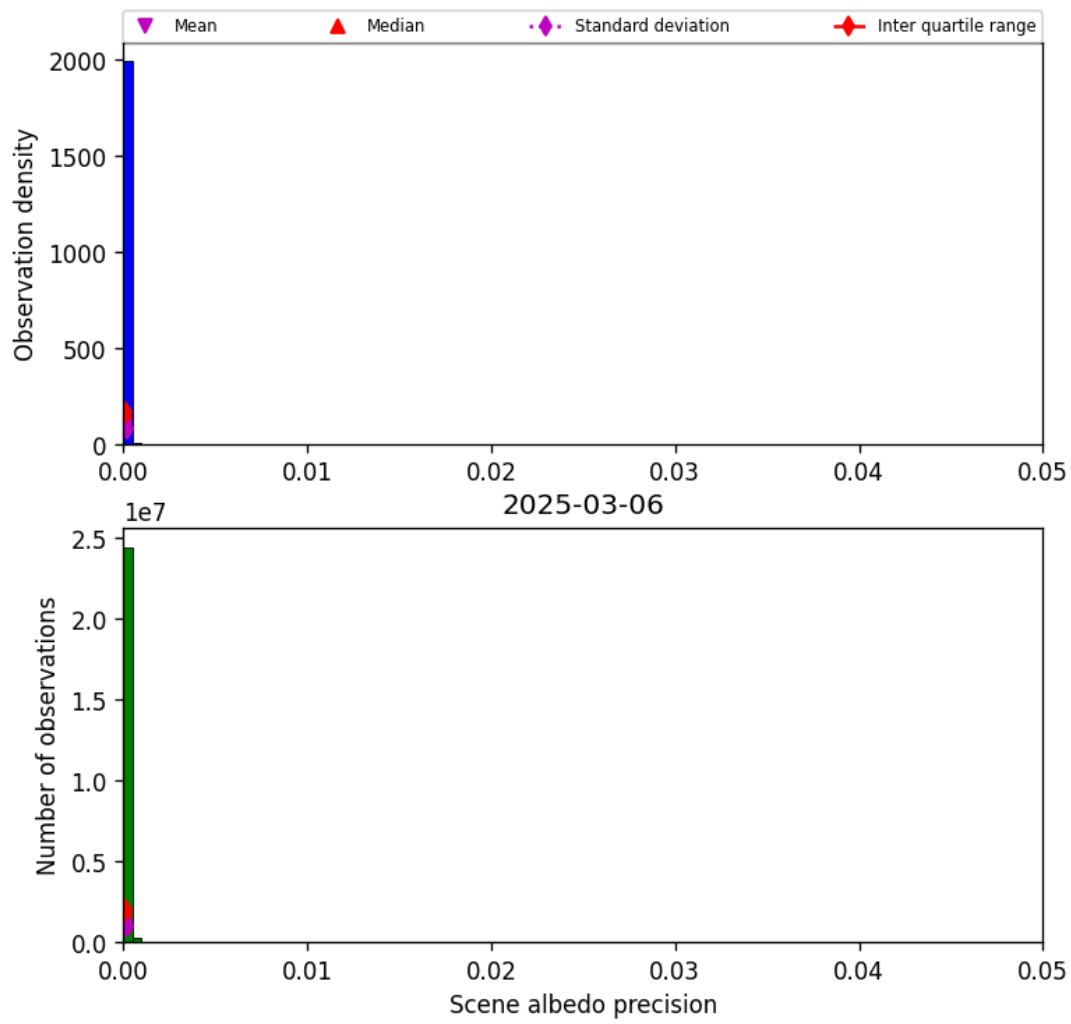
Figure 33: Histogram of “Scene albedo precision” for 2025-03-06 to 2025-03-07
