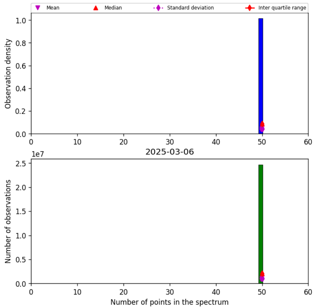
Figure 42: Histogram of “Number of points in the spectrum” for 2025-03-06 to 2025-03-07
