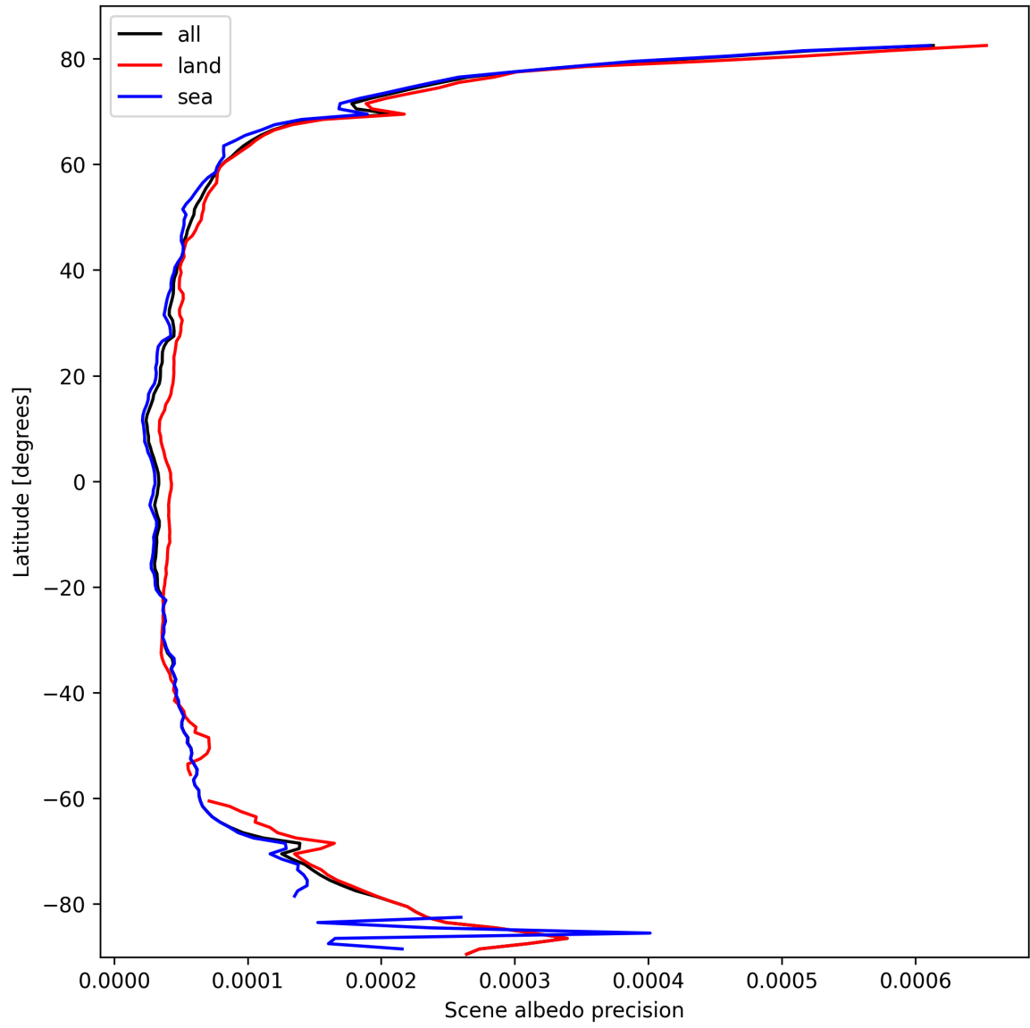
Figure 16: Zonal average of “Scene albedo precision” for 2025-03-06 to 2025-03-07.
