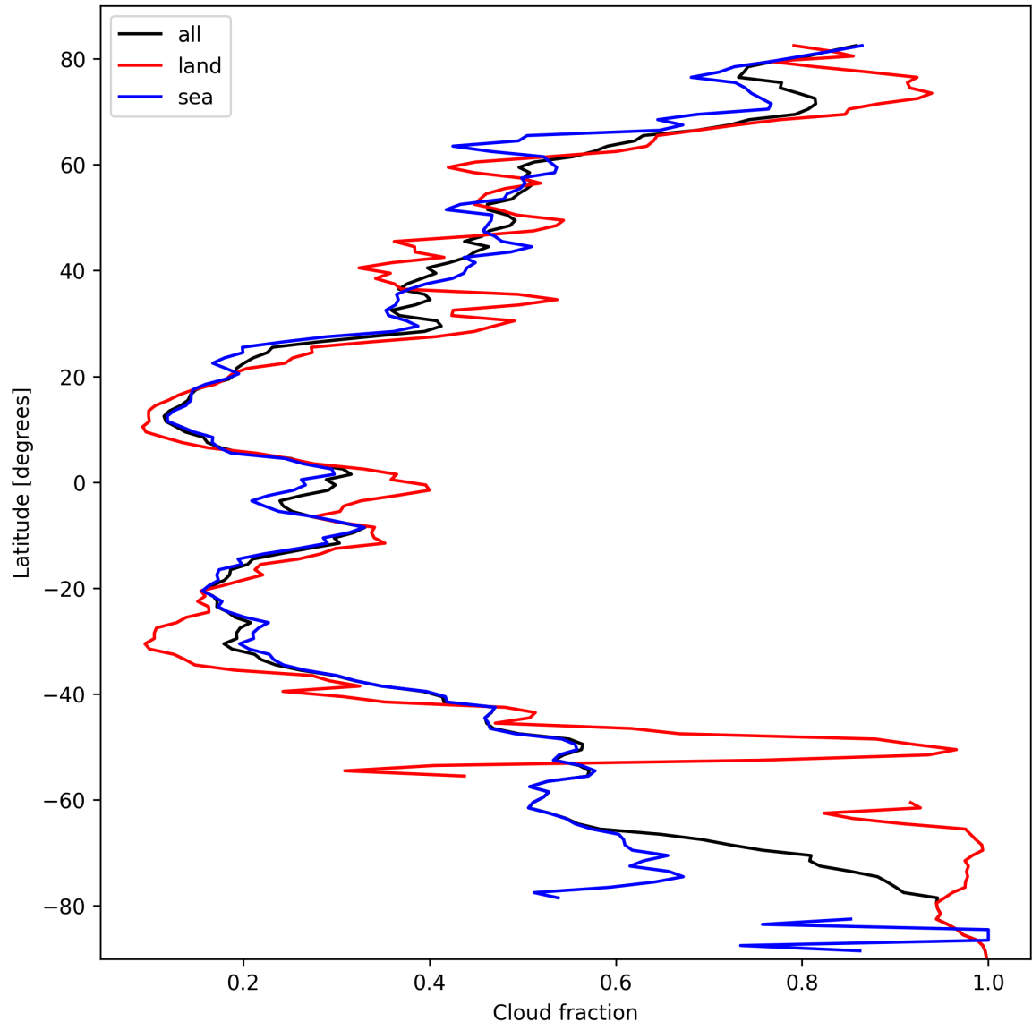
Figure 13: Zonal average of “Cloud fraction” for 2025-03-06 to 2025-03-07.
