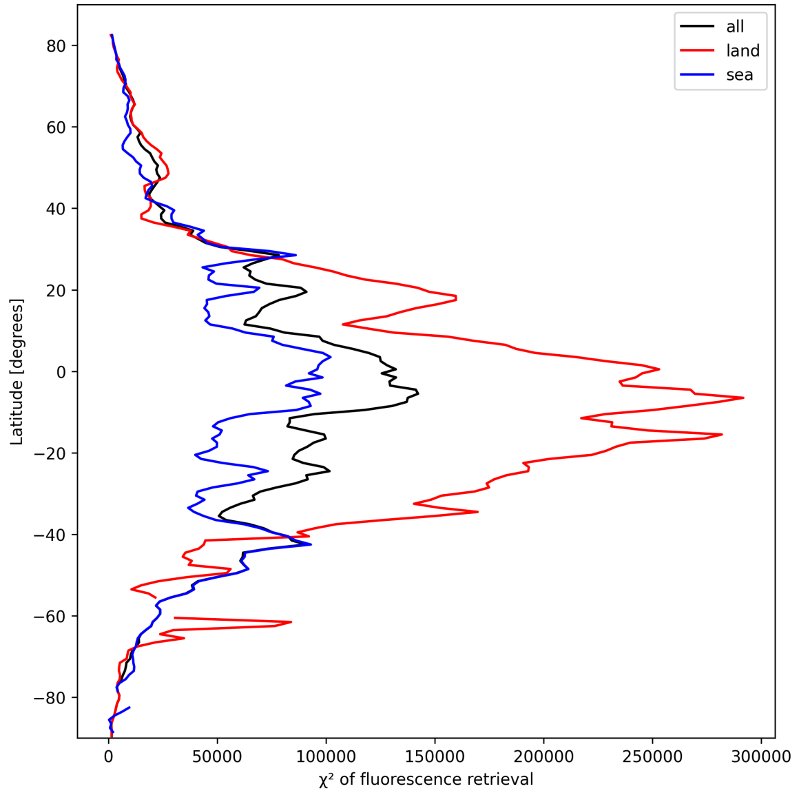
Figure 23: Zonal average of “ \chi^2 of fluorescence retrieval” for 2025-03-06 to 2025-03-07.
