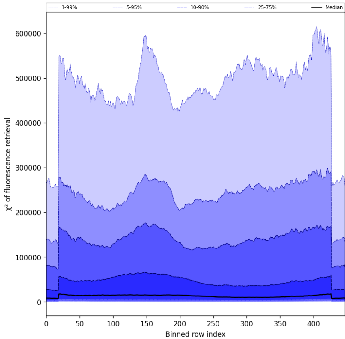
Figure 57: Along track statistics of “ \chi^2 of fluorescence retrieval” for 2025-03-06 to 2025-03-07
