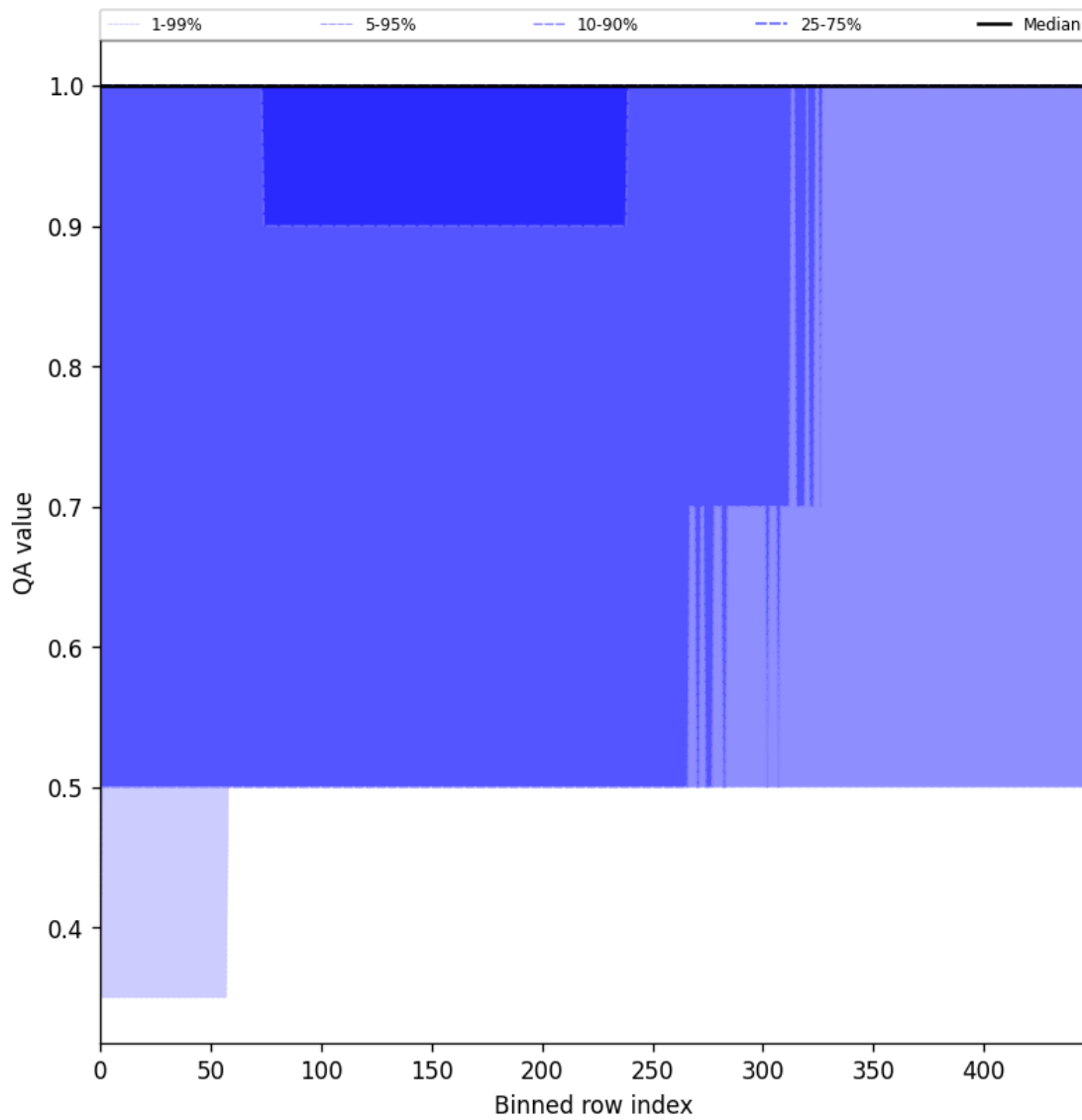
Figure 44: Along track statistics of “QA value” for 2025-03-06 to 2025-03-07
