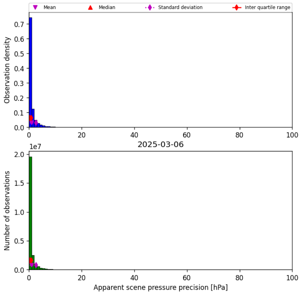
Figure 35: Histogram of “Apparent scene pressure precision” for 2025-03-06 to 2025-03-07
