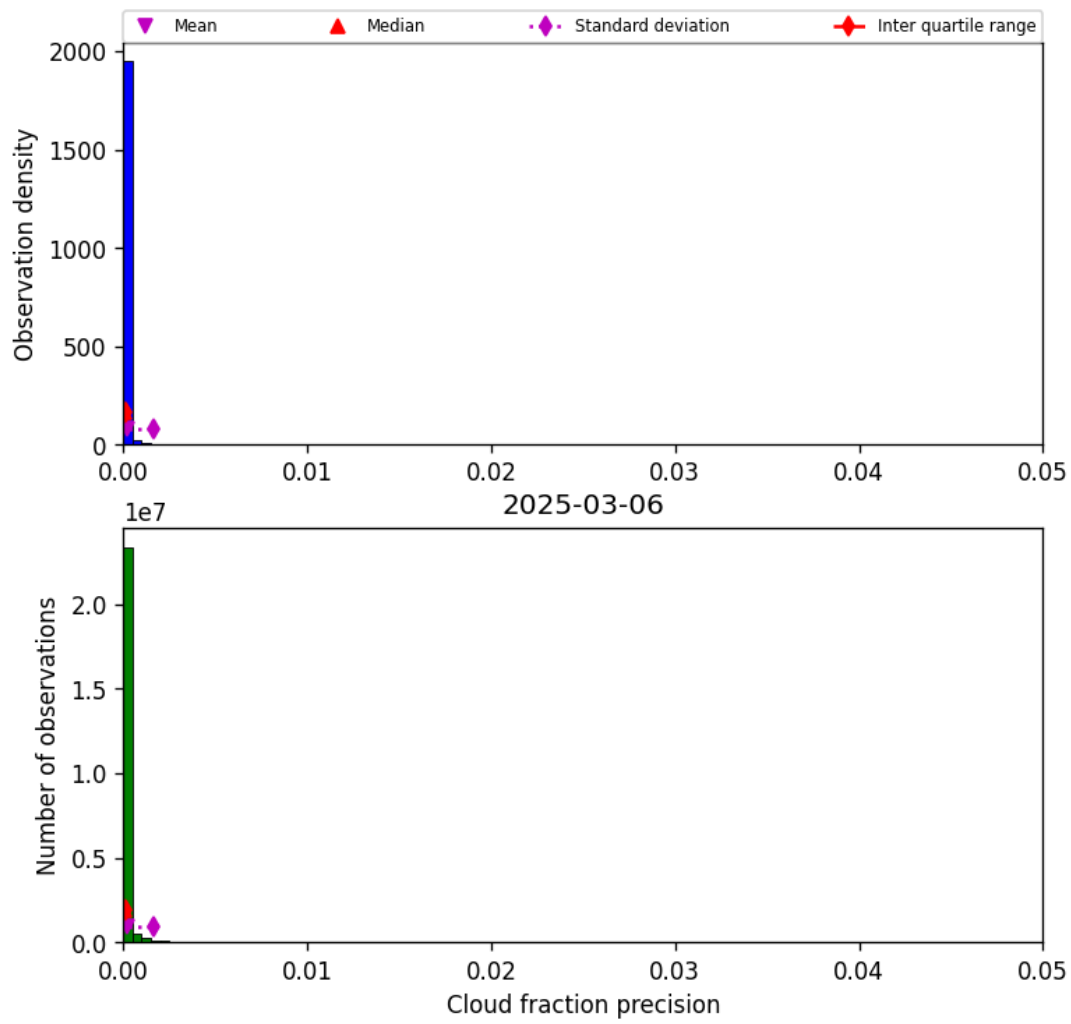
Figure 31: Histogram of “Cloud fraction precision” for 2025-03-06 to 2025-03-07
