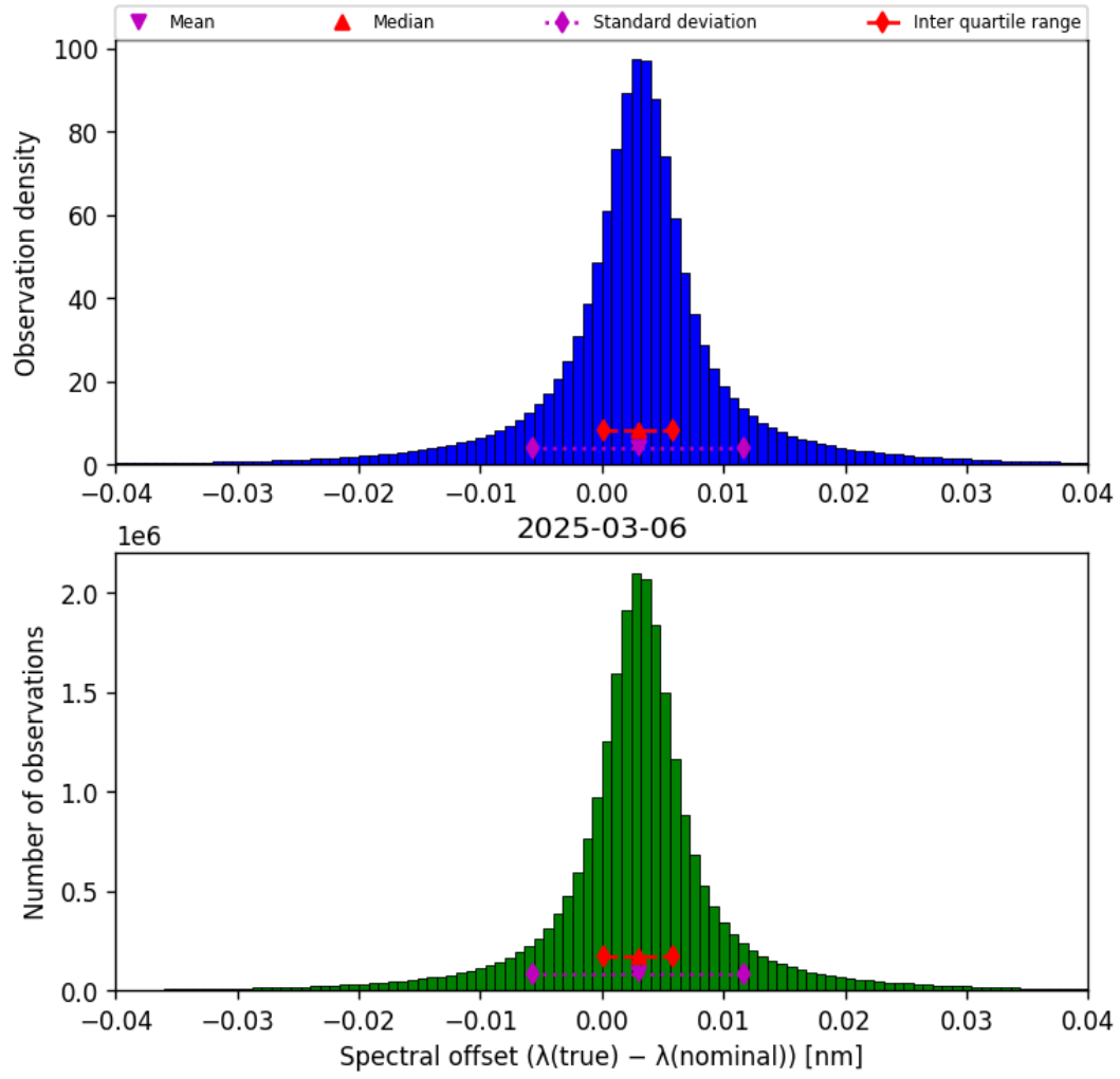
Figure 43: Histogram of “Spectral offset ( \lambda_{\text{true}} - \lambda_{\text{nominal}} )” for 2025-03-06 to 2025-03-07
