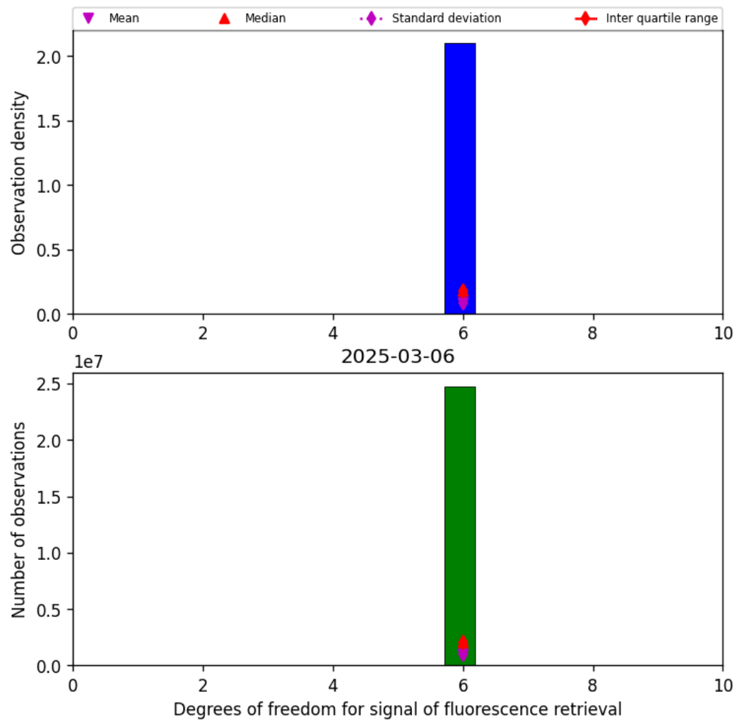
Figure 41: Histogram of “Degrees of freedom for signal of fluorescence retrieval” for 2025-03-06 to 2025-03-07
