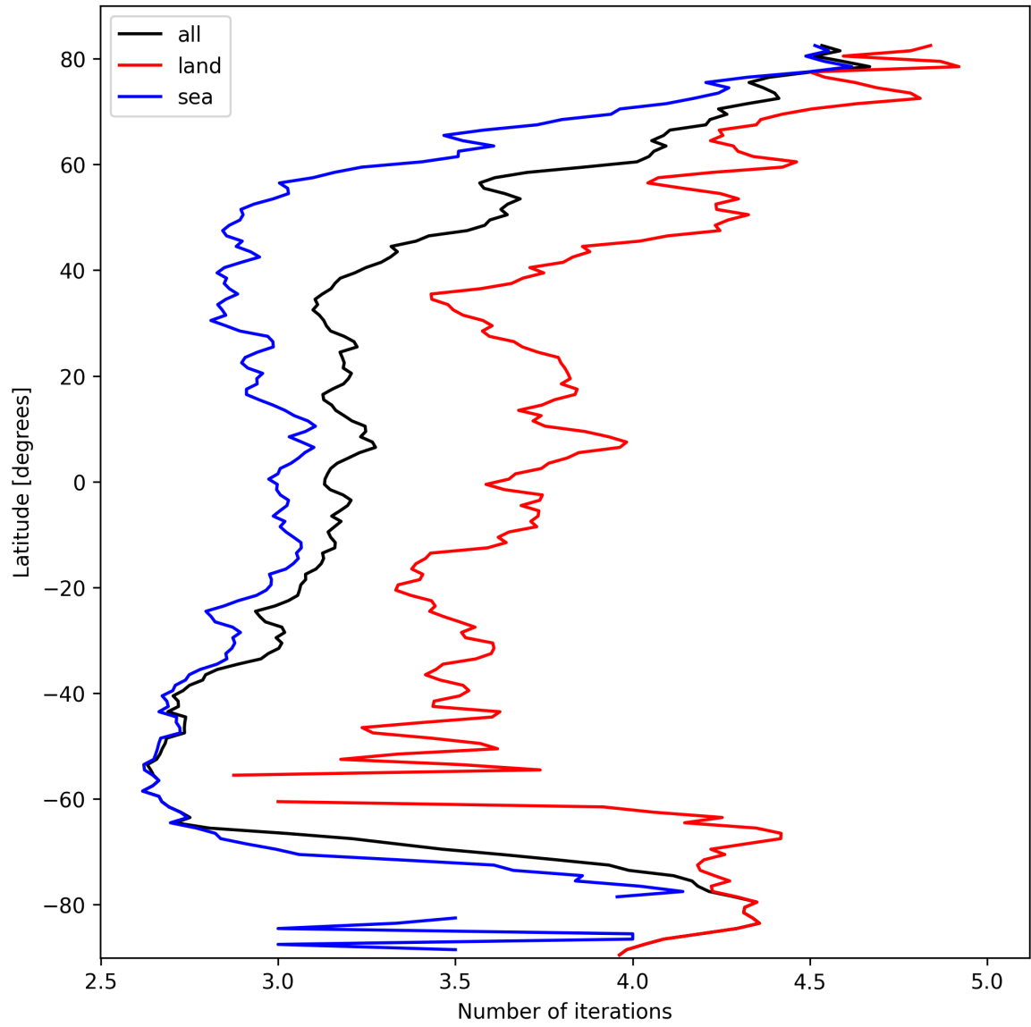
Figure 20: Zonal average of “Number of iterations” for 2025-03-06 to 2025-03-07.
