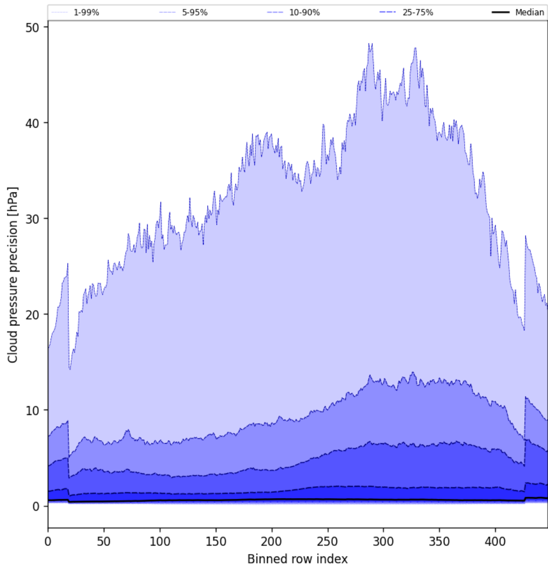
Figure 46: Along track statistics of “Cloud pressure precision” for 2025-03-06 to 2025-03-07
