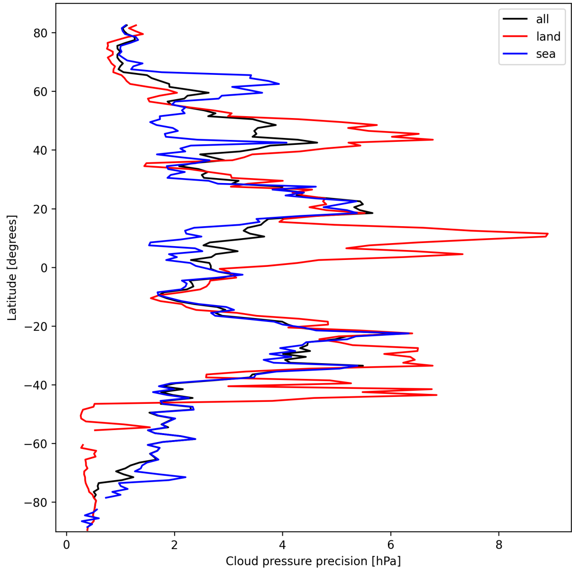
Figure 12: Zonal average of "Cloud pressure precision" for 2025-03-06 to 2025-03-07.
