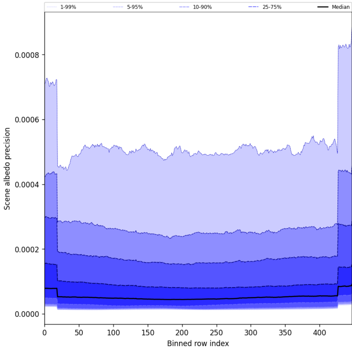
Figure 50: Along track statistics of “Scene albedo precision” for 2025-03-06 to 2025-03-07
