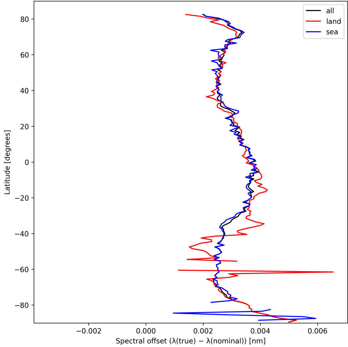
Figure 26: Zonal average of “Spectral offset ( \lambda_{\text{true}} - \lambda_{\text{nominal}} )” for 2025-03-06 to 2025-03-07.
