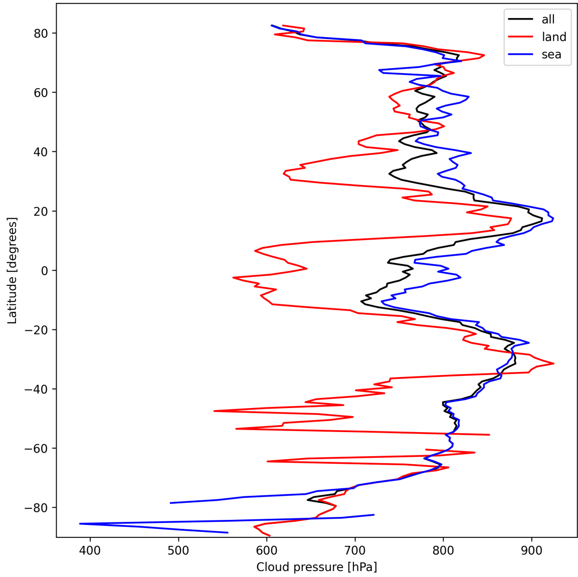
Figure 11: Zonal average of “Cloud pressure” for 2025-03-06 to 2025-03-07.
