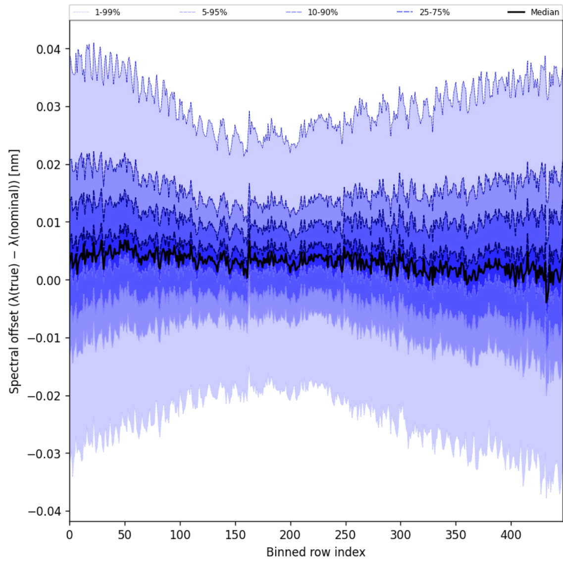
Figure 60: Along track statistics of “Spectral offset ( \lambda_{\text{true}} - \lambda_{\text{nominal}} )” for 2025-03-06 to 2025-03-07
