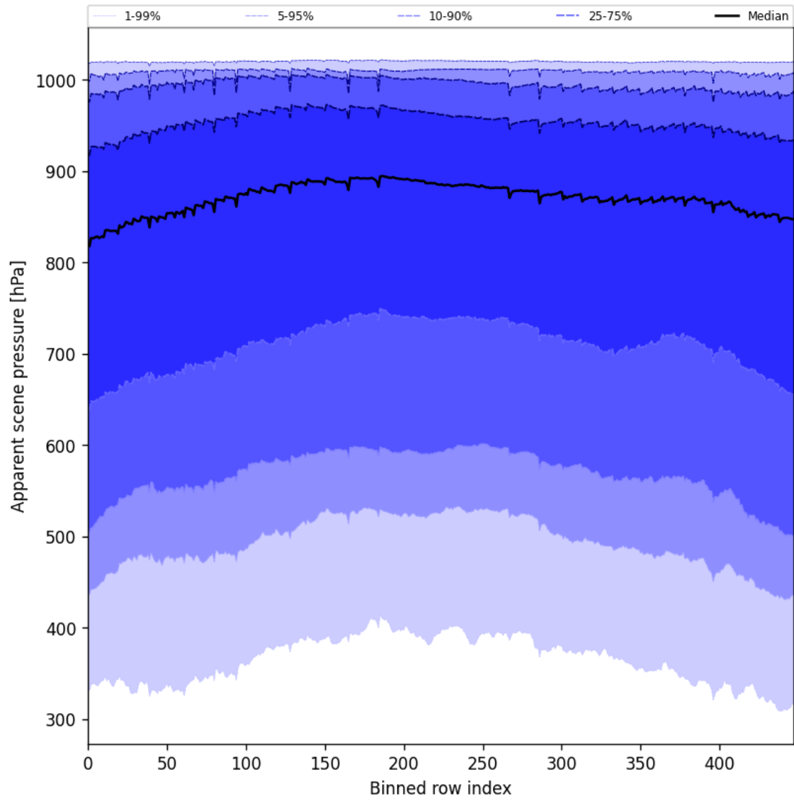
Figure 51: Along track statistics of “Apparent scene pressure” for 2025-03-06 to 2025-03-07
