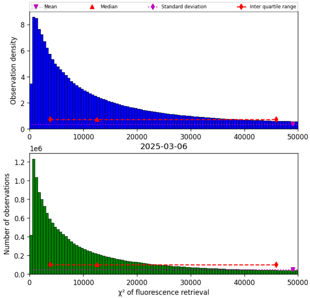
Figure 40: Histogram of “ \chi^2 of fluorescence retrieval” for 2025-03-06 to 2025-03-07
