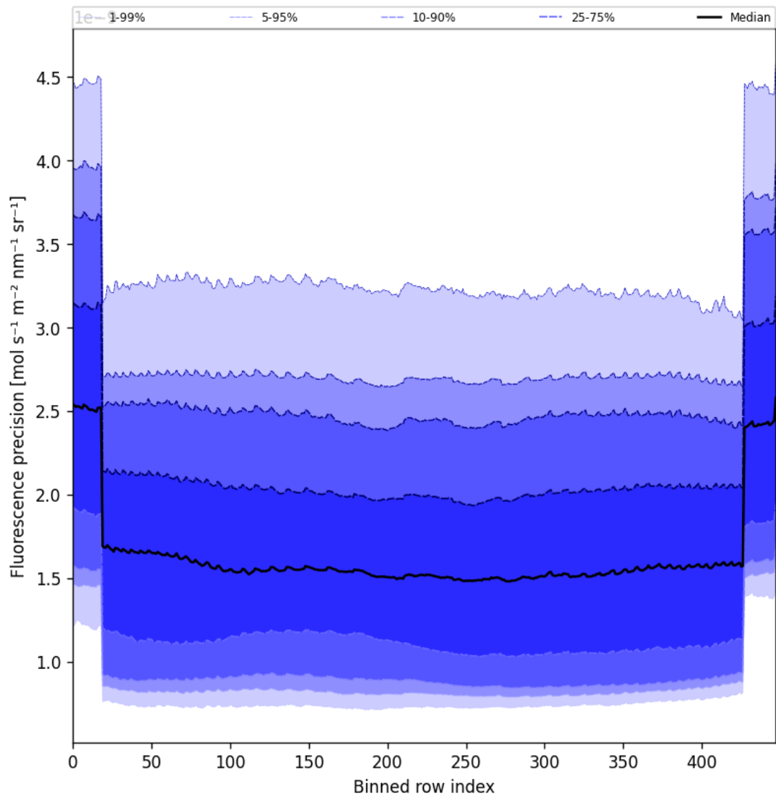
Figure 56: Along track statistics of “Fluorescence precision” for 2025-03-06 to 2025-03-07
