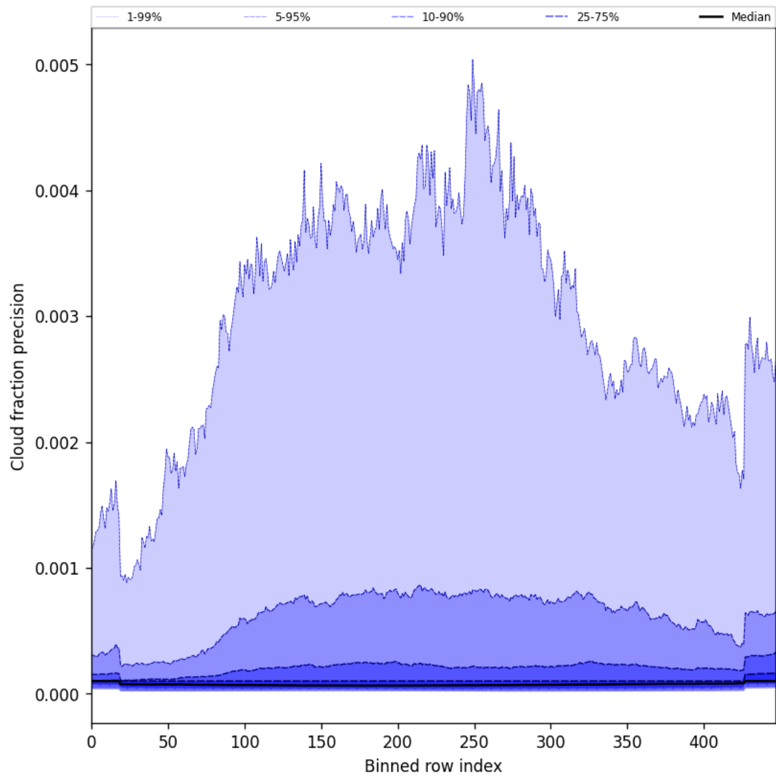
Figure 48: Along track statistics of “Cloud fraction precision” for 2025-03-06 to 2025-03-07
