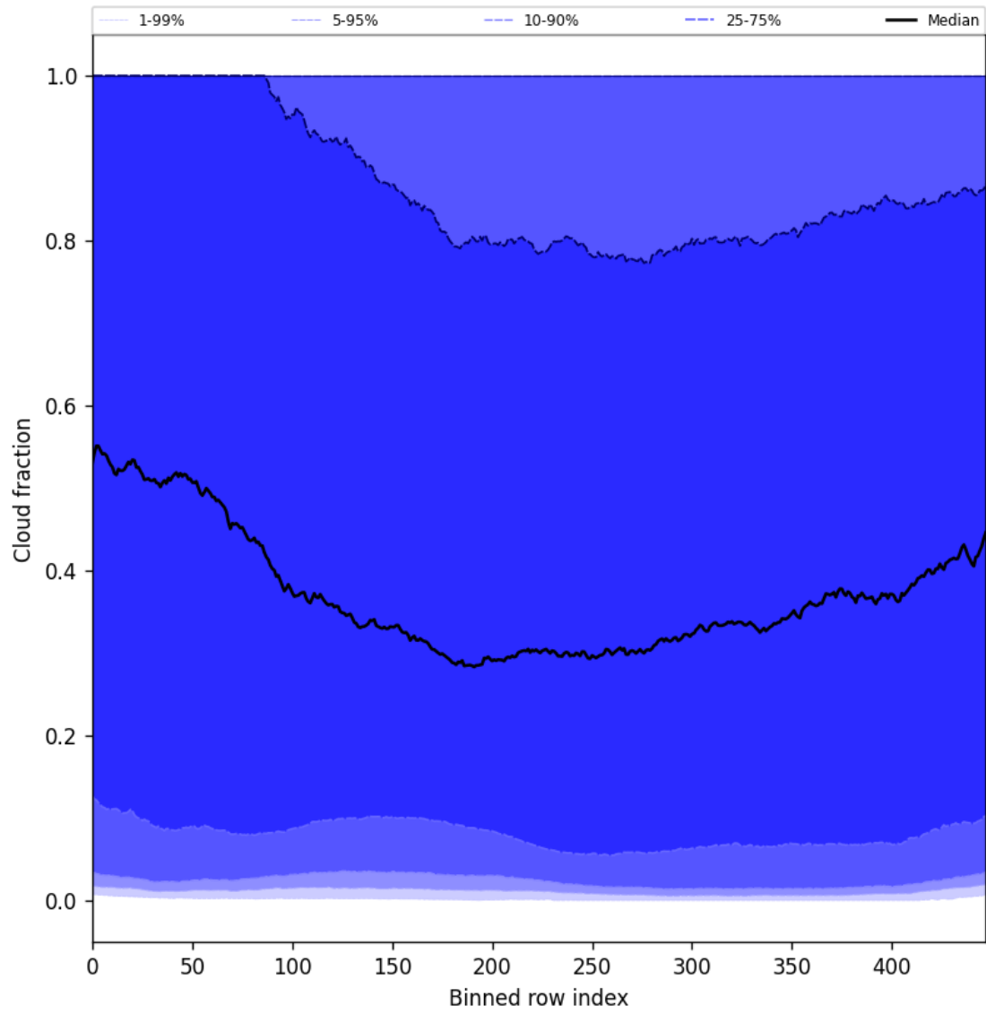
Figure 47: Along track statistics of “Cloud fraction” for 2025-03-06 to 2025-03-07
