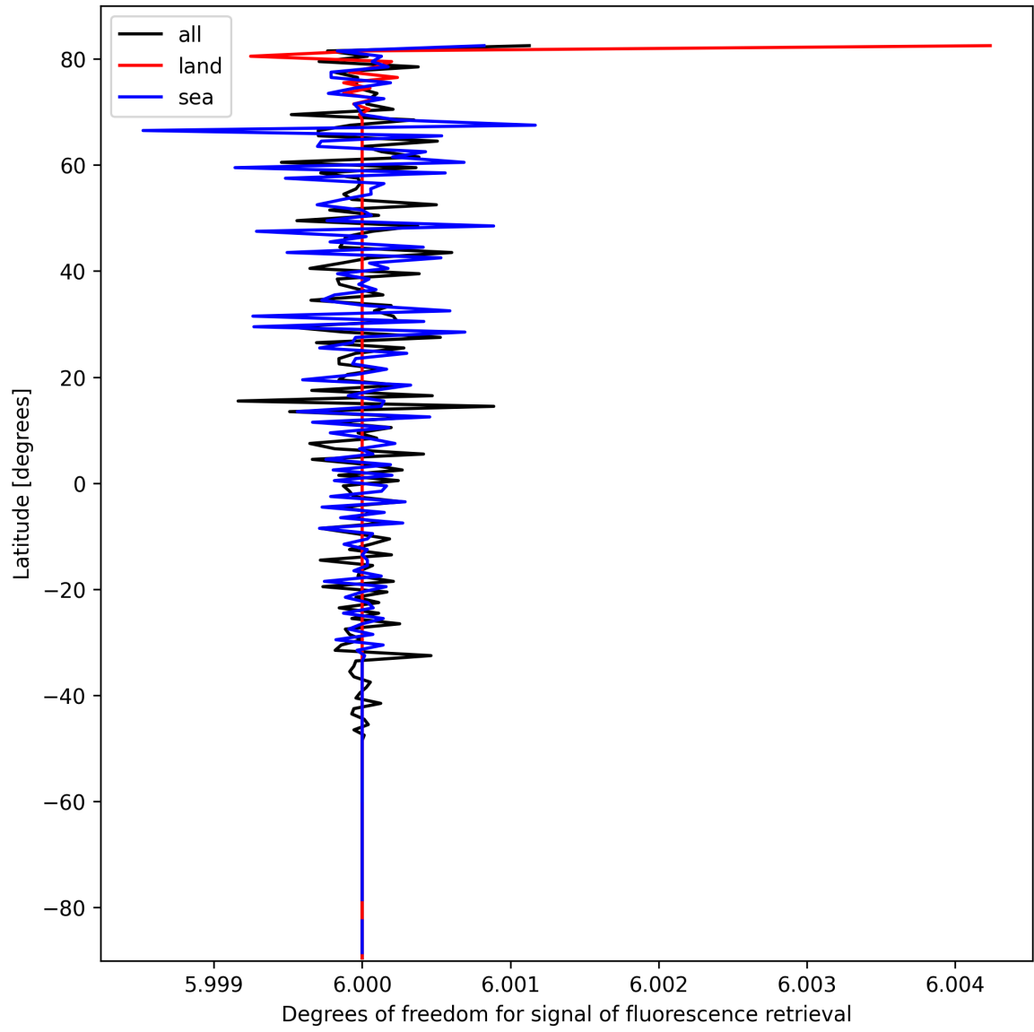
Figure 24: Zonal average of “Degrees of freedom for signal of fluorescence retrieval” for 2025-03-06 to 2025-03-07.
