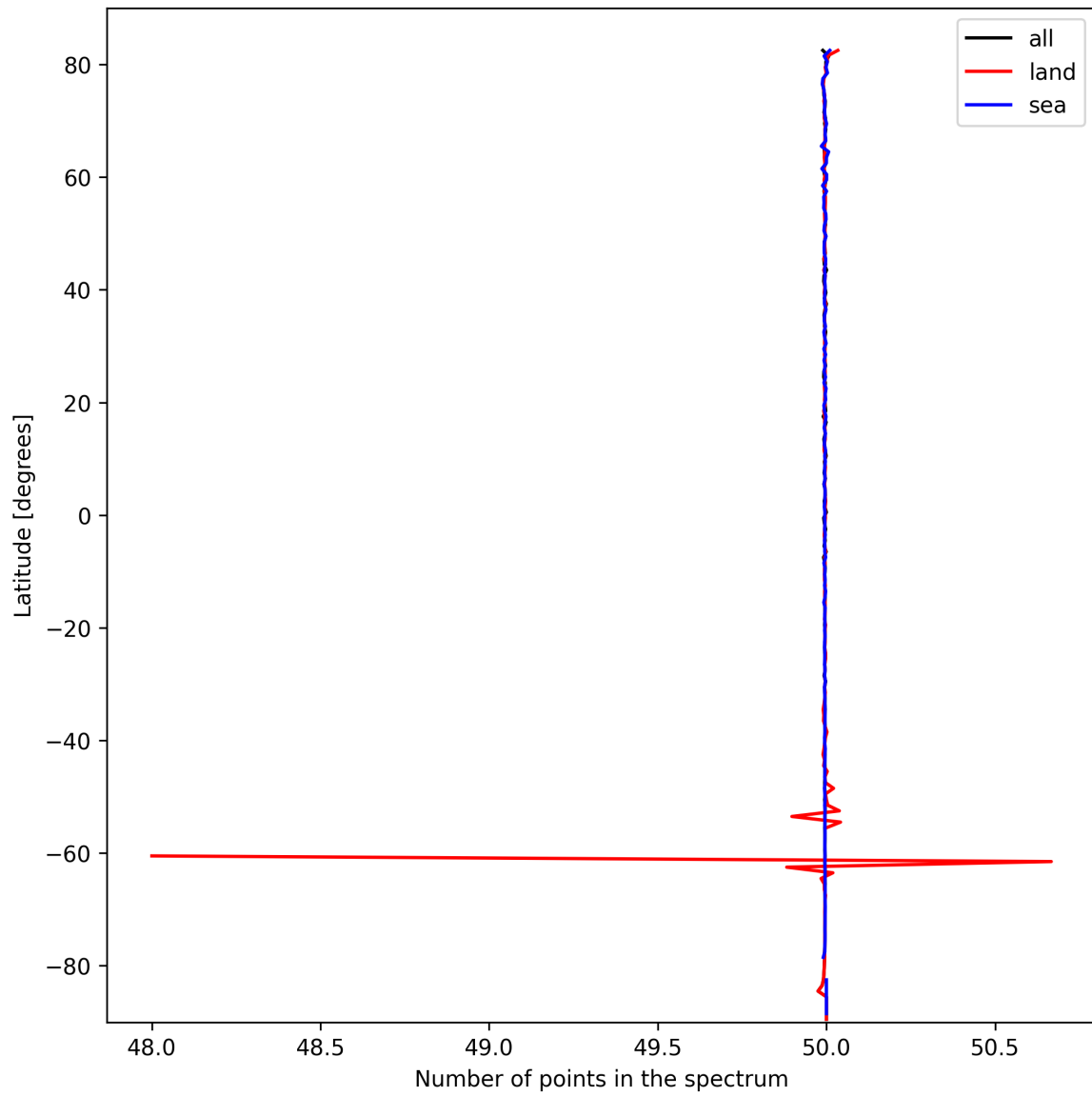
Figure 25: Zonal average of “Number of points in the spectrum” for 2025-03-06 to 2025-03-07.
