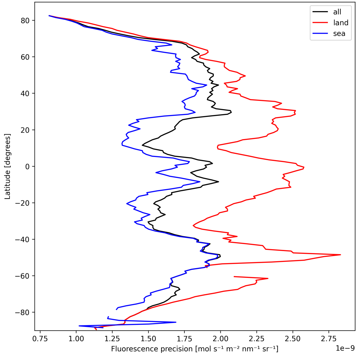
Figure 22: Zonal average of “Fluorescence precision” for 2025-03-06 to 2025-03-07.
