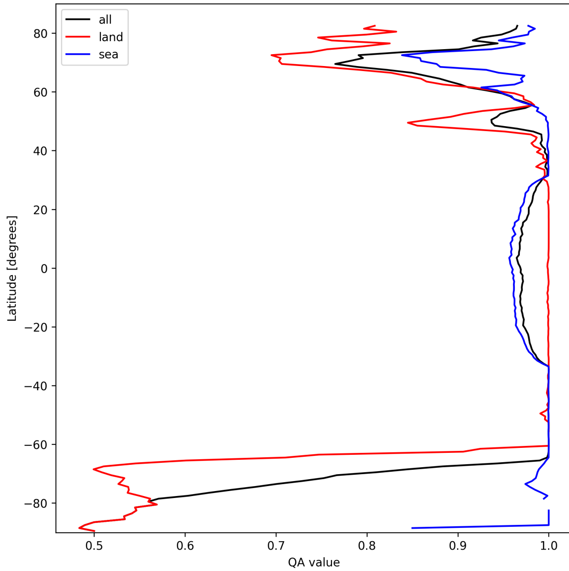
Figure 10: Zonal average of “QA value” for 2025-03-06 to 2025-03-07.
