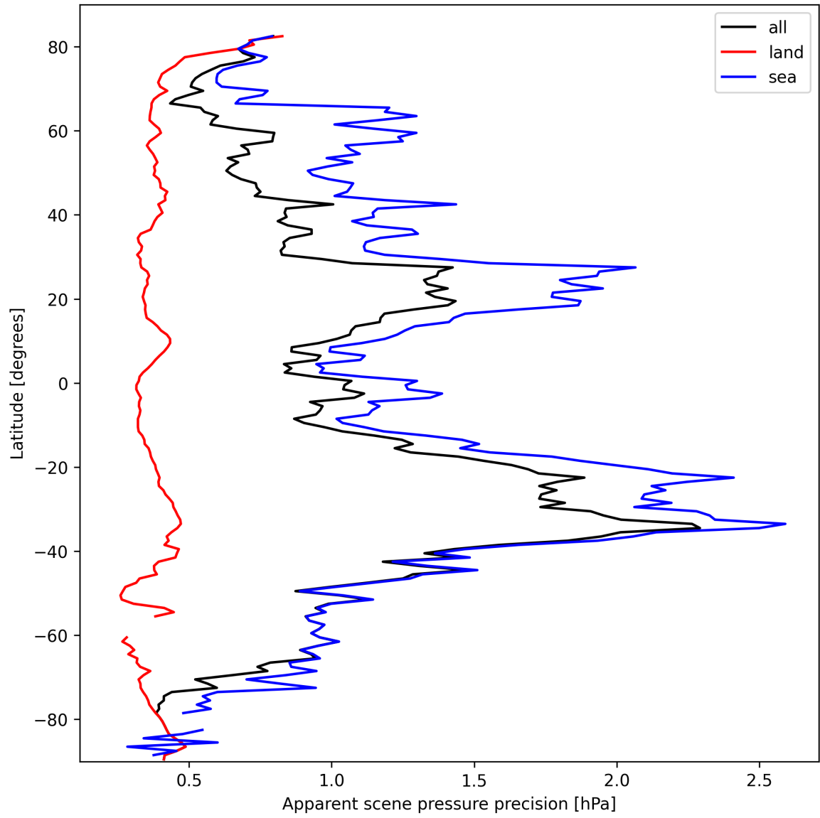
Figure 18: Zonal average of “Apparent scene pressure precision” for 2025-03-06 to 2025-03-07.
