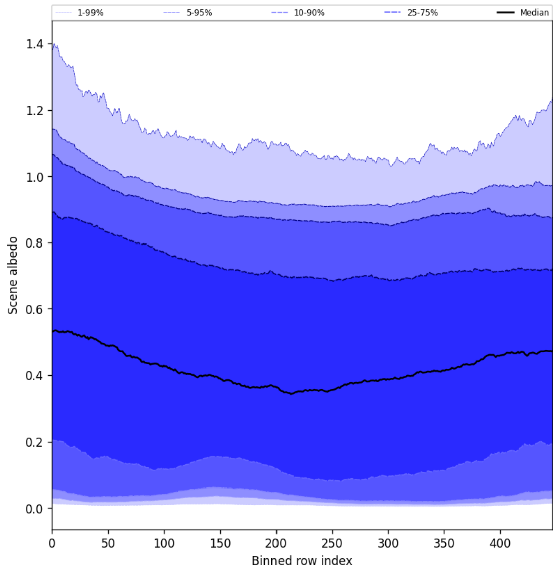
Figure 49: Along track statistics of “Scene albedo” for 2025-03-07 to 2025-03-08
