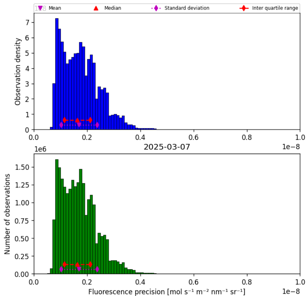
Figure 39: Histogram of “Fluorescence precision” for 2025-03-07 to 2025-03-08
