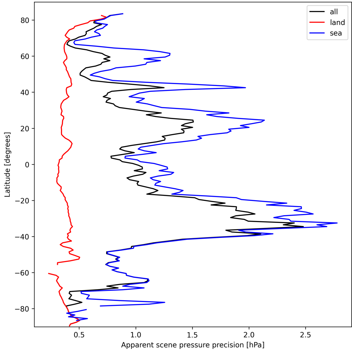
Figure 18: Zonal average of “Apparent scene pressure precision” for 2025-03-07 to 2025-03-08.
