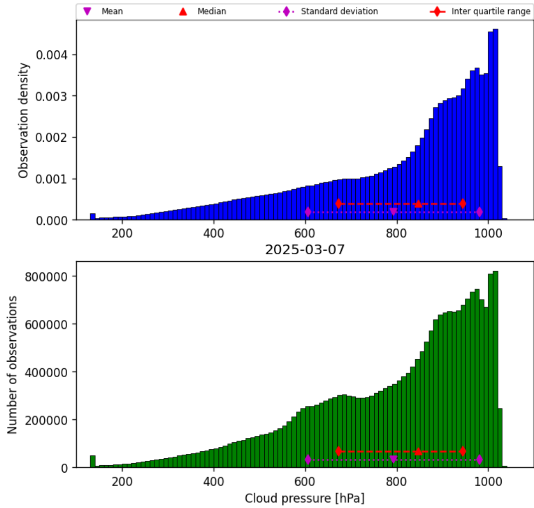
Figure 28: Histogram of “Cloud pressure” for 2025-03-07 to 2025-03-08
