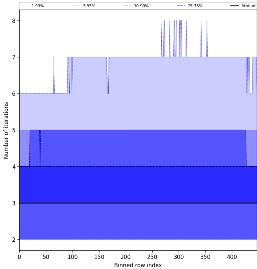
Figure 54: Along track statistics of “Number of iterations” for 2025-03-07 to 2025-03-08
