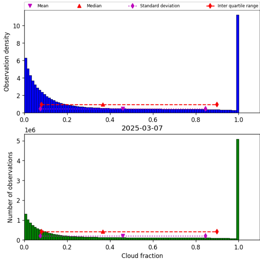
Figure 30: Histogram of “Cloud fraction” for 2025-03-07 to 2025-03-08
