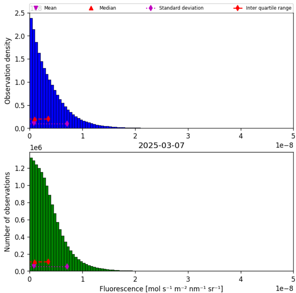
Figure 38: Histogram of “Fluorescence” for 2025-03-07 to 2025-03-08
