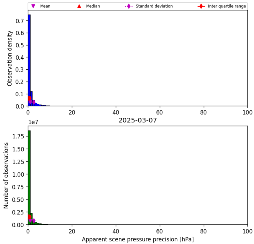
Figure 35: Histogram of “Apparent scene pressure precision” for 2025-03-07 to 2025-03-08
