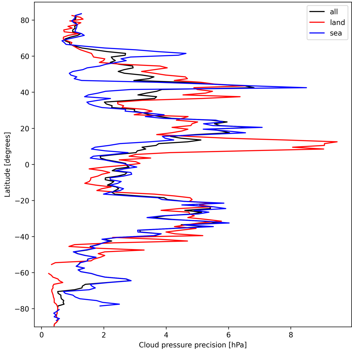
Figure 12: Zonal average of "Cloud pressure precision" for 2025-03-07 to 2025-03-08.
