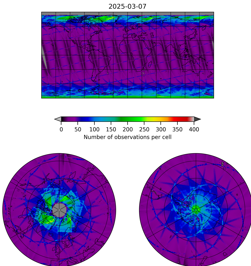
Figure 9: Map of the number of observations for 2025-03-07 to 2025-03-08
