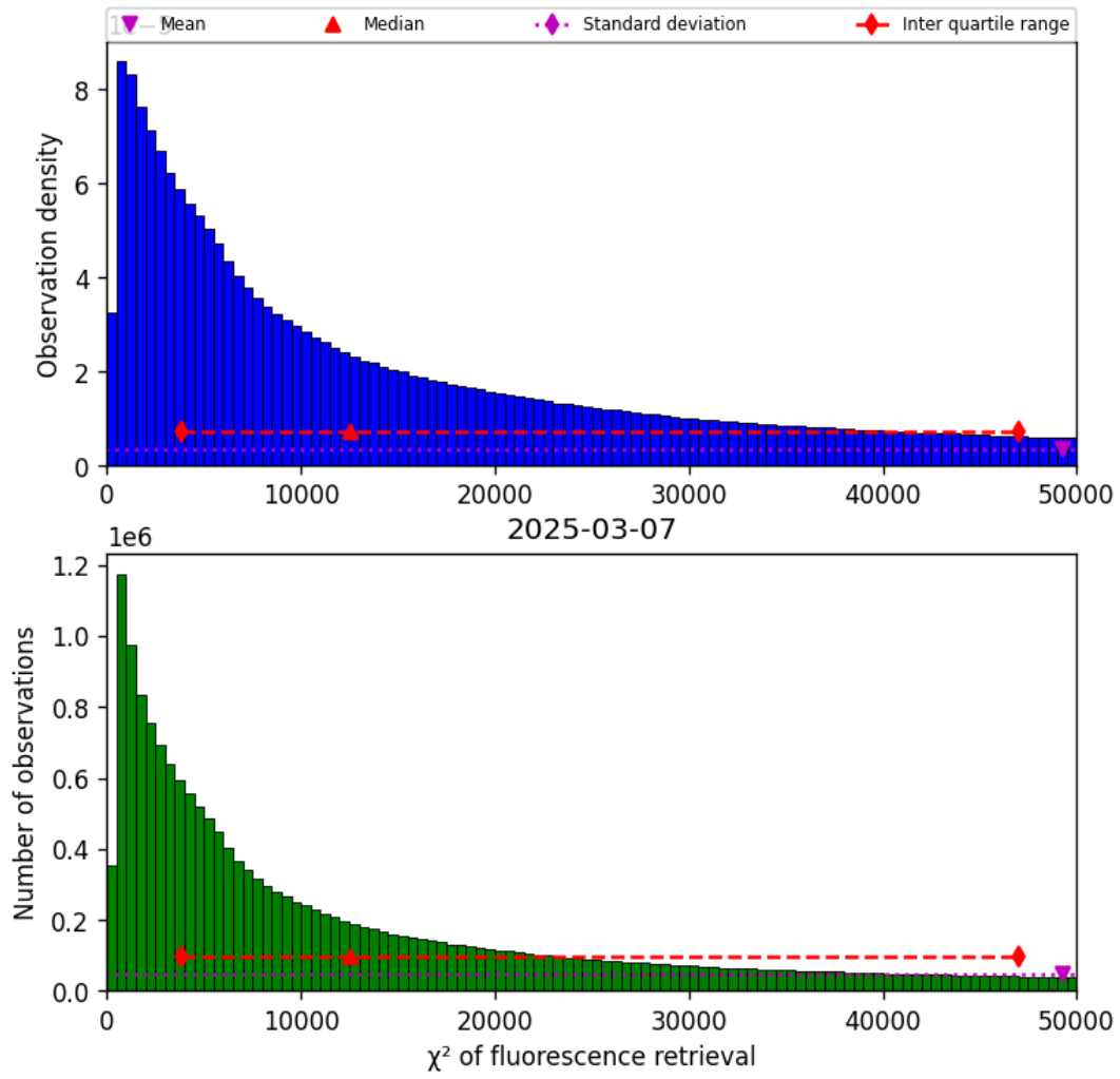
Figure 40: Histogram of “ \chi^2 of fluorescence retrieval” for 2025-03-07 to 2025-03-08
