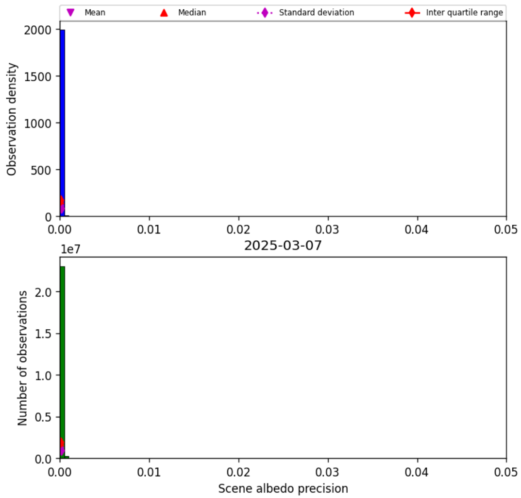
Figure 33: Histogram of “Scene albedo precision” for 2025-03-07 to 2025-03-08
