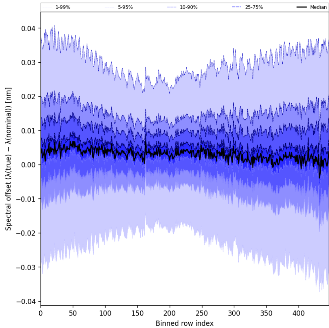
Figure 60: Along track statistics of “Spectral offset ( \lambda_{\text{true}} - \lambda_{\text{nominal}} )” for 2025-03-07 to 2025-03-08
