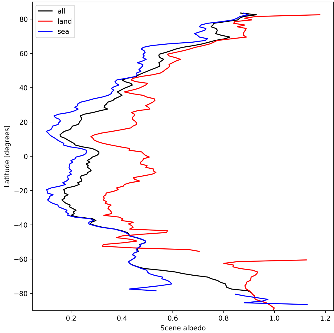
Figure 15: Zonal average of “Scene albedo” for 2025-03-07 to 2025-03-08.
