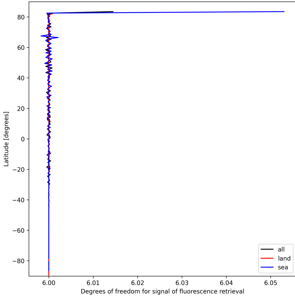
Figure 24: Zonal average of “Degrees of freedom for signal of fluorescence retrieval” for 2025-03-07 to 2025-03-08.
