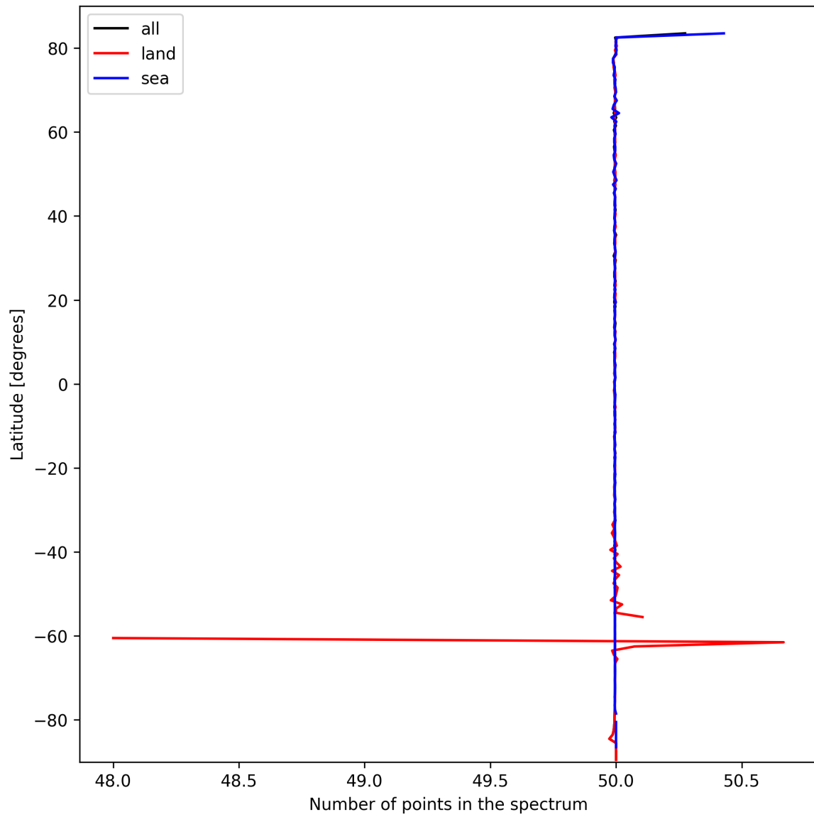
Figure 25: Zonal average of “Number of points in the spectrum” for 2025-03-07 to 2025-03-08.
