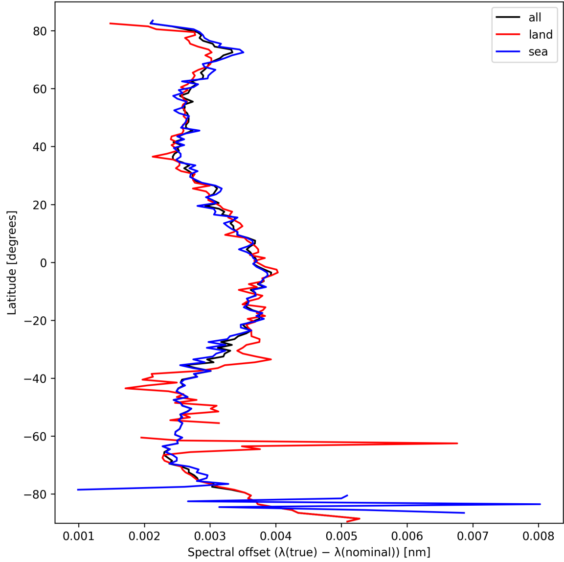
Figure 26: Zonal average of “Spectral offset ( \lambda_{\text{true}} - \lambda_{\text{nominal}} )” for 2025-03-07 to 2025-03-08.
