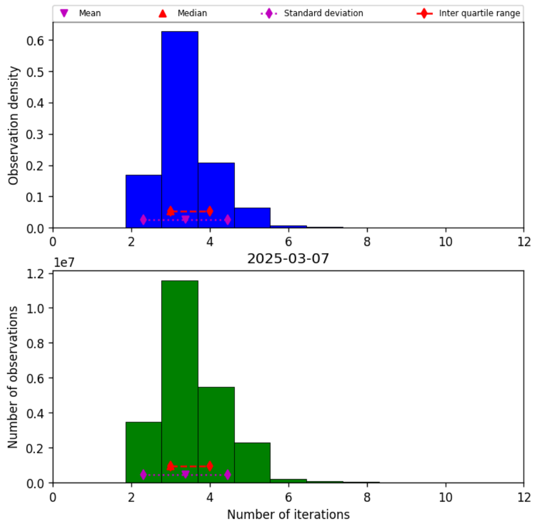
Figure 37: Histogram of “Number of iterations” for 2025-03-07 to 2025-03-08
