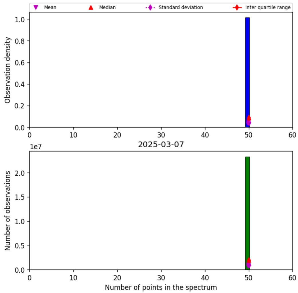
Figure 42: Histogram of “Number of points in the spectrum” for 2025-03-07 to 2025-03-08
