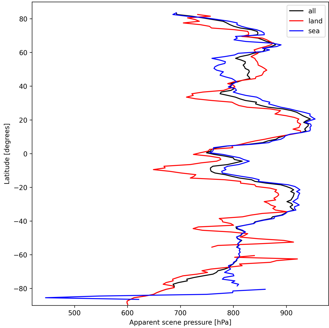
Figure 17: Zonal average of “Apparent scene pressure” for 2025-03-07 to 2025-03-08.
