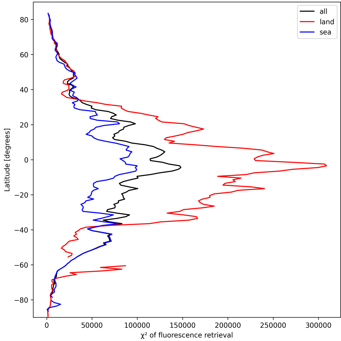
Figure 23: Zonal average of “ \chi^2 of fluorescence retrieval” for 2025-03-07 to 2025-03-08.
