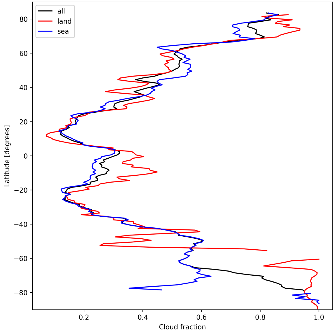
Figure 13: Zonal average of “Cloud fraction” for 2025-03-07 to 2025-03-08.
