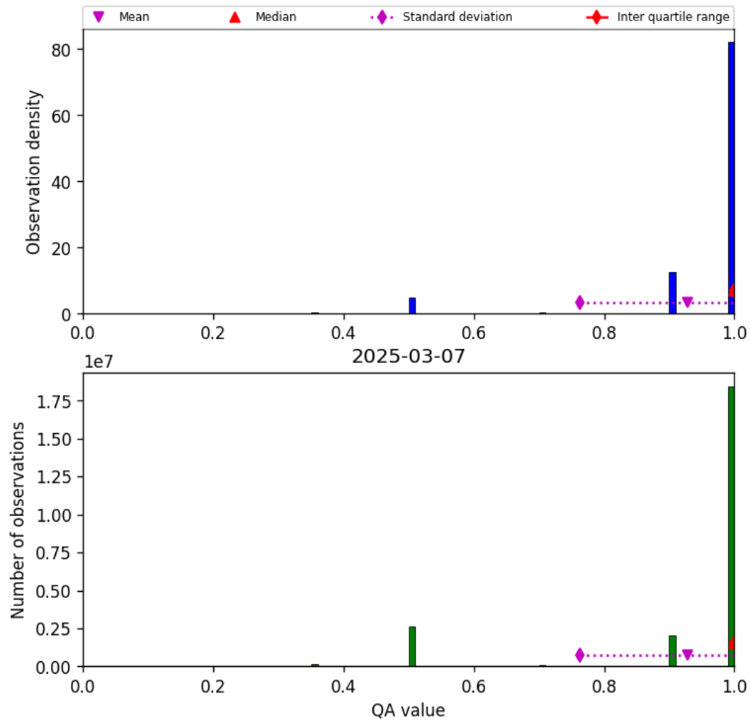
Figure 27: Histogram of “QA value” for 2025-03-07 to 2025-03-08
