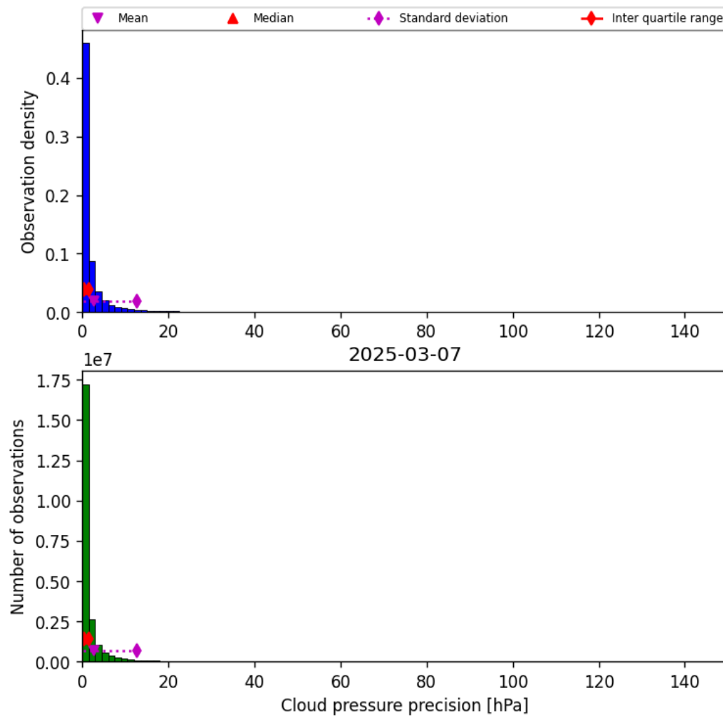
Figure 29: Histogram of “Cloud pressure precision” for 2025-03-07 to 2025-03-08
