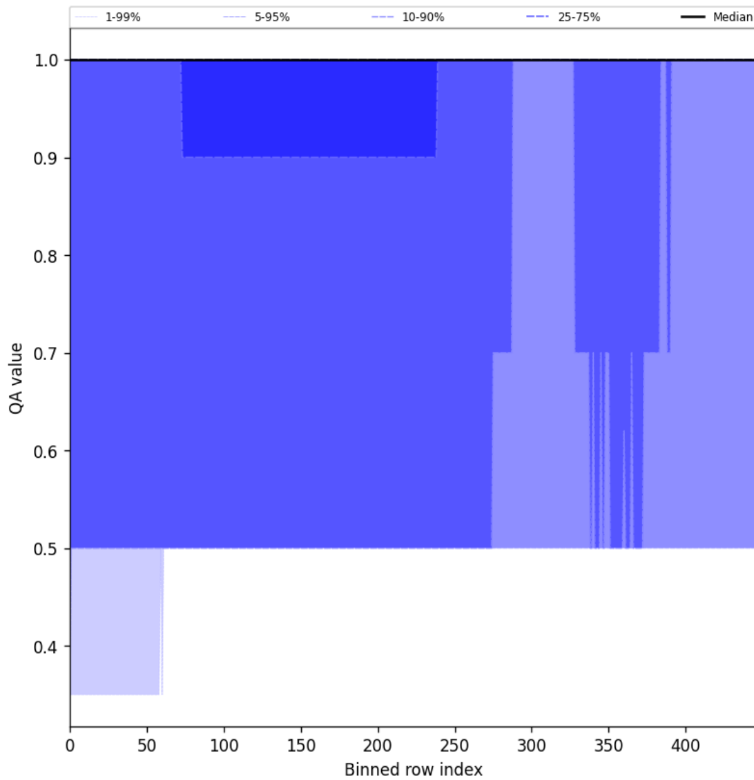
Figure 44: Along track statistics of “QA value” for 2025-03-07 to 2025-03-08
