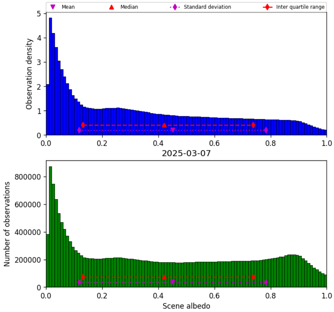
Figure 32: Histogram of “Scene albedo” for 2025-03-07 to 2025-03-08
