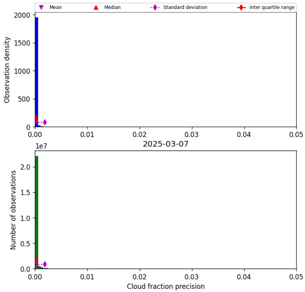
Figure 31: Histogram of “Cloud fraction precision” for 2025-03-07 to 2025-03-08
