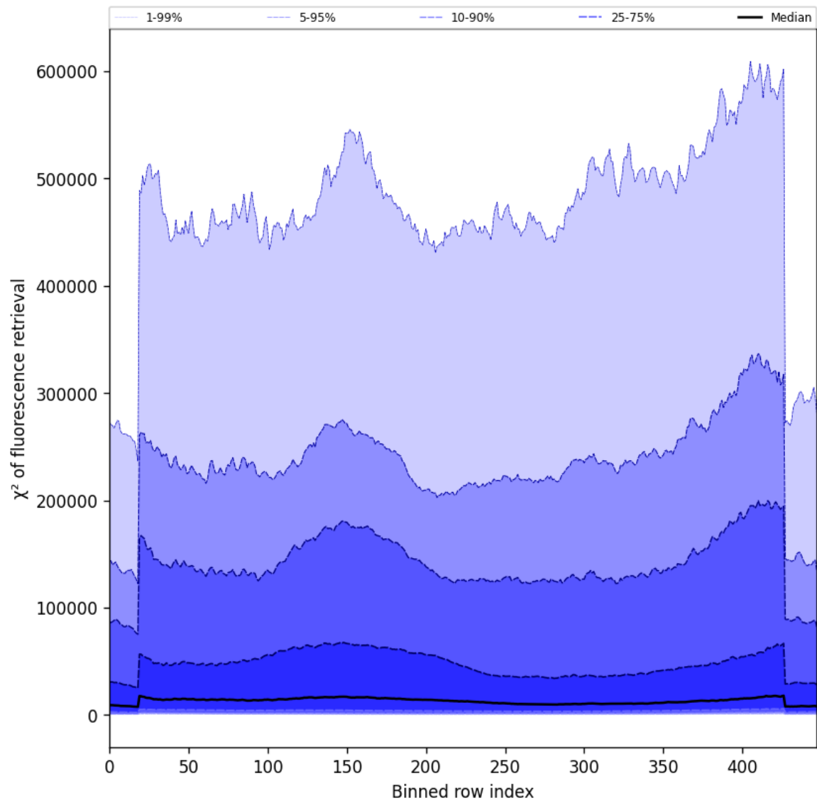
Figure 57: Along track statistics of “ \chi^2 of fluorescence retrieval” for 2025-03-07 to 2025-03-08
