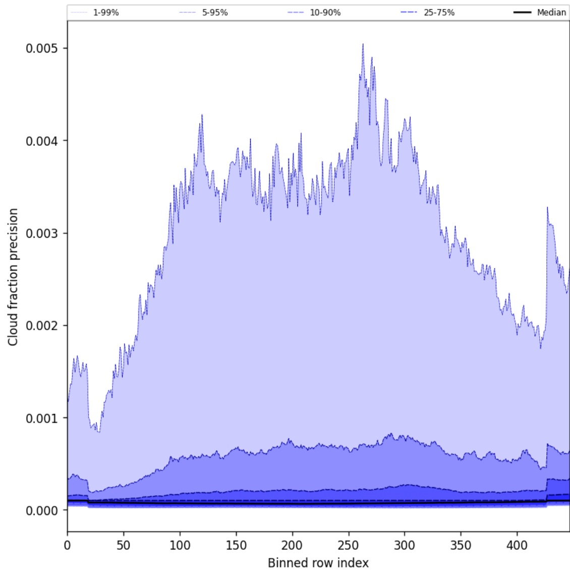
Figure 48: Along track statistics of “Cloud fraction precision” for 2025-03-07 to 2025-03-08
