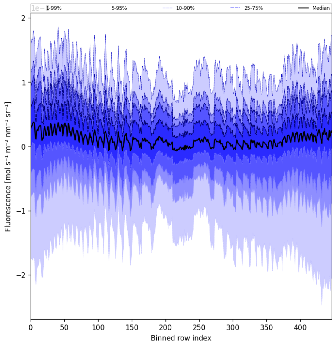
Figure 55: Along track statistics of “Fluorescence” for 2025-03-07 to 2025-03-08
