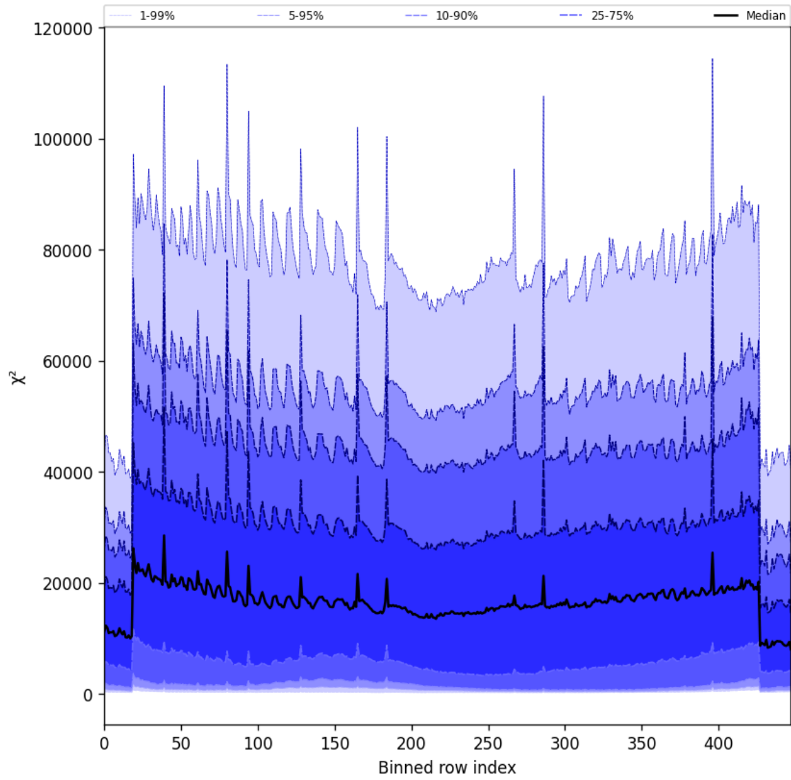
Figure 53: Along track statistics of “ \chi^2 ” for 2025-03-07 to 2025-03-08
