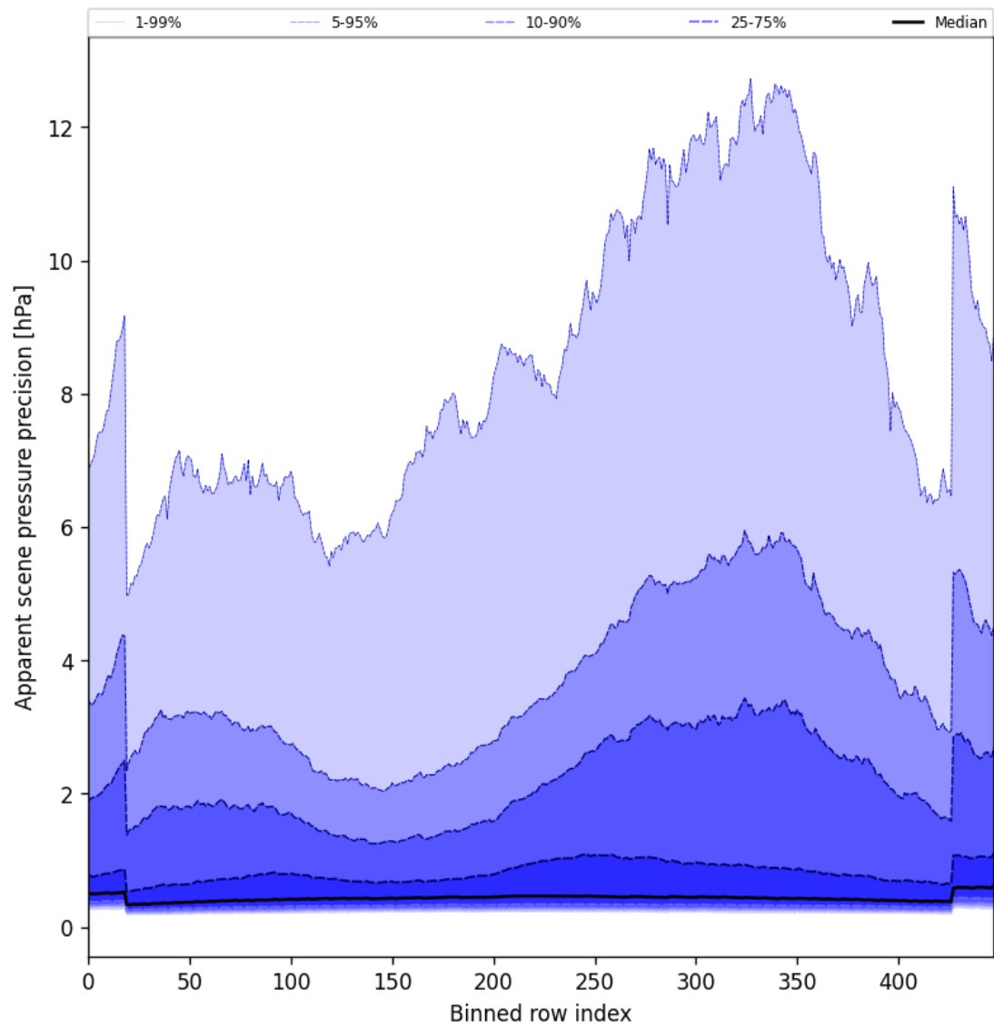
Figure 52: Along track statistics of “Apparent scene pressure precision” for 2025-03-07 to 2025-03-08
