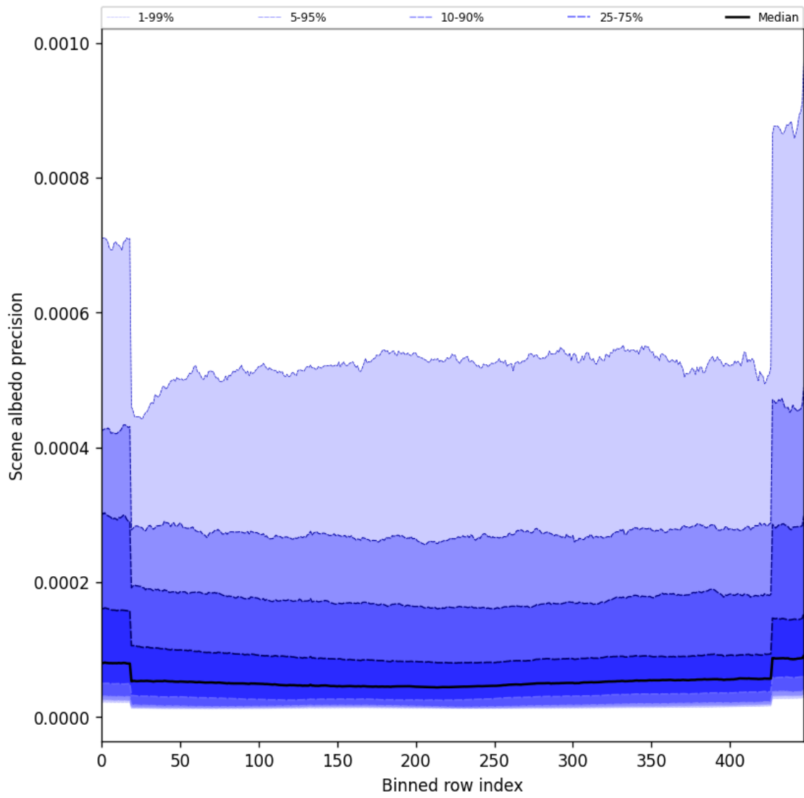
Figure 50: Along track statistics of “Scene albedo precision” for 2025-03-07 to 2025-03-08
