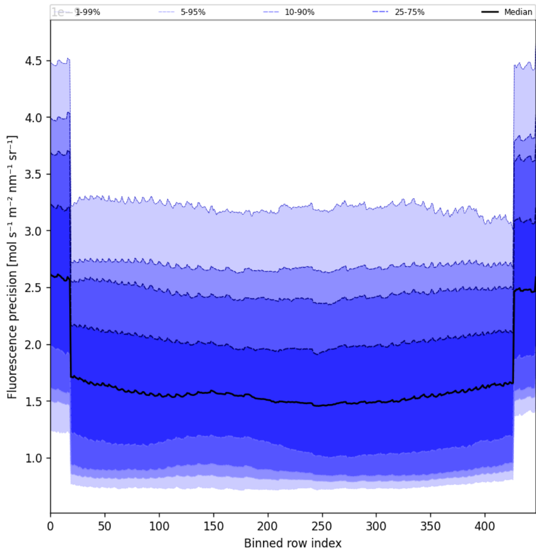
Figure 56: Along track statistics of “Fluorescence precision” for 2025-03-07 to 2025-03-08
