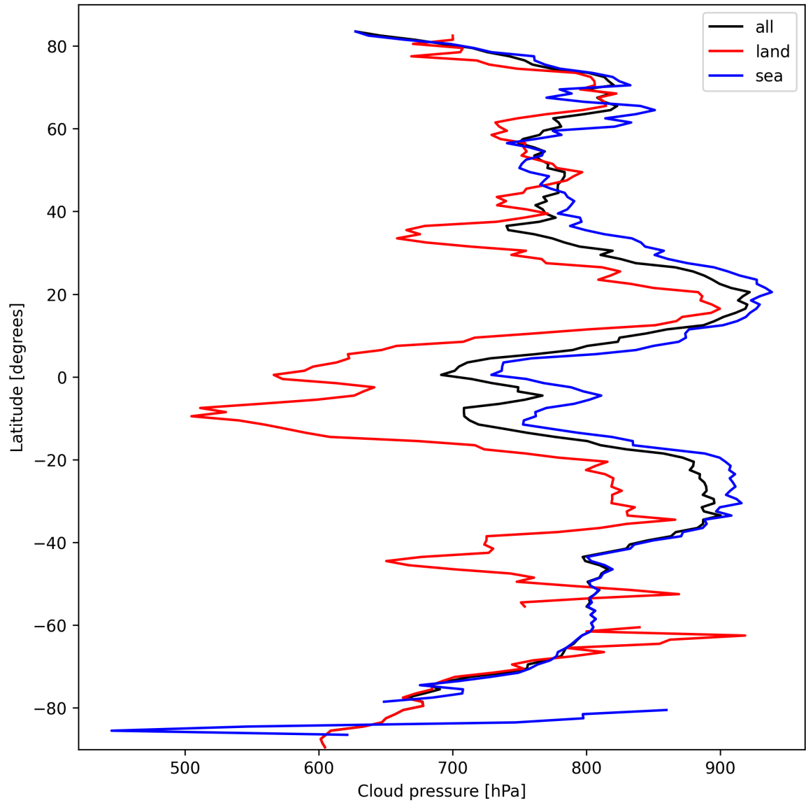
Figure 11: Zonal average of “Cloud pressure” for 2025-03-07 to 2025-03-08.
