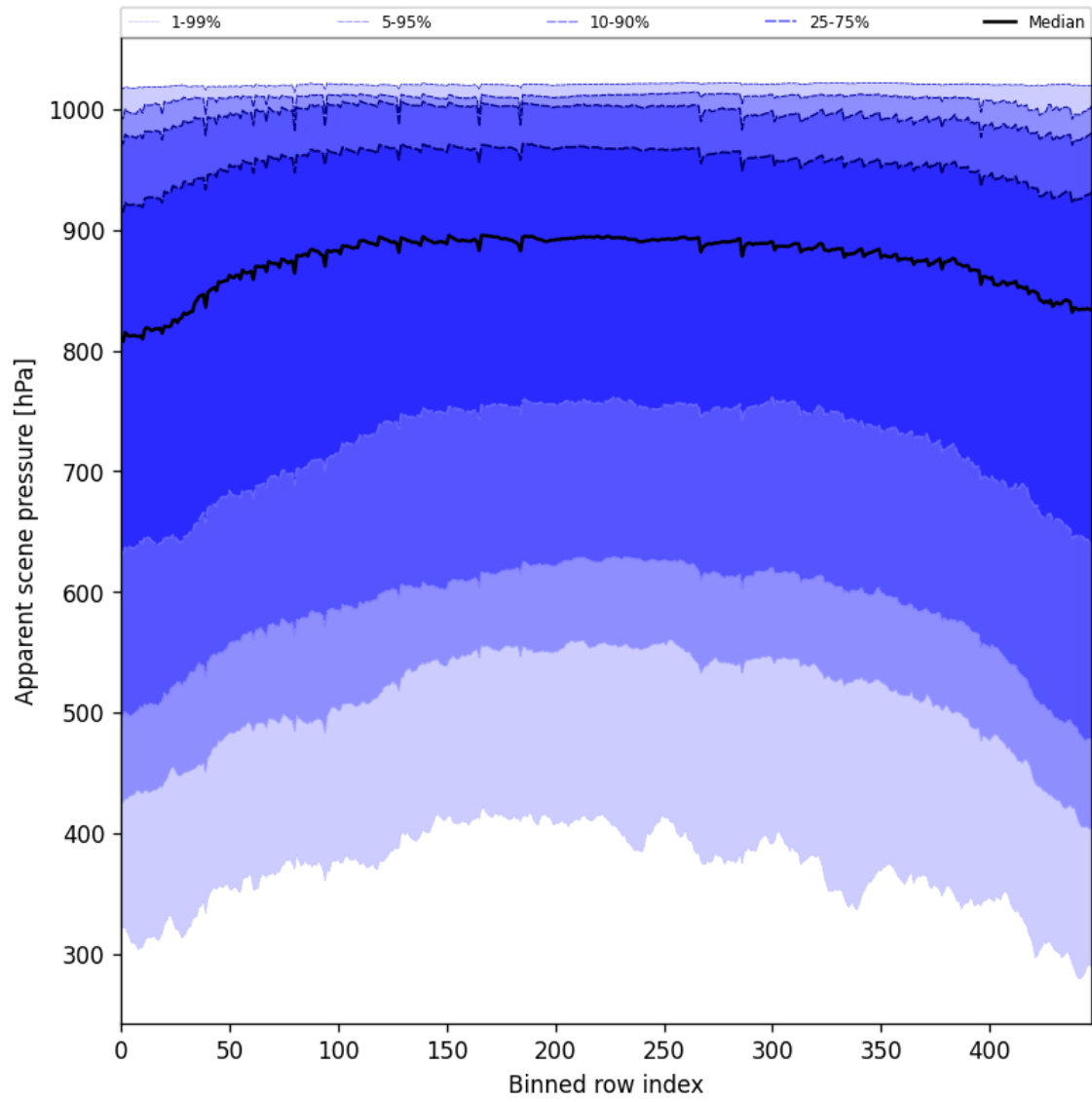
Figure 51: Along track statistics of “Apparent scene pressure” for 2025-03-07 to 2025-03-08
