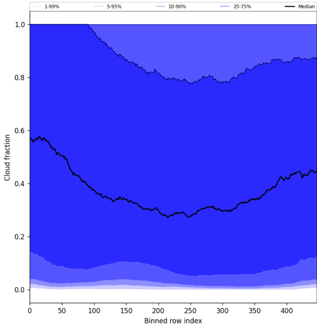
Figure 47: Along track statistics of “Cloud fraction” for 2025-03-07 to 2025-03-08
