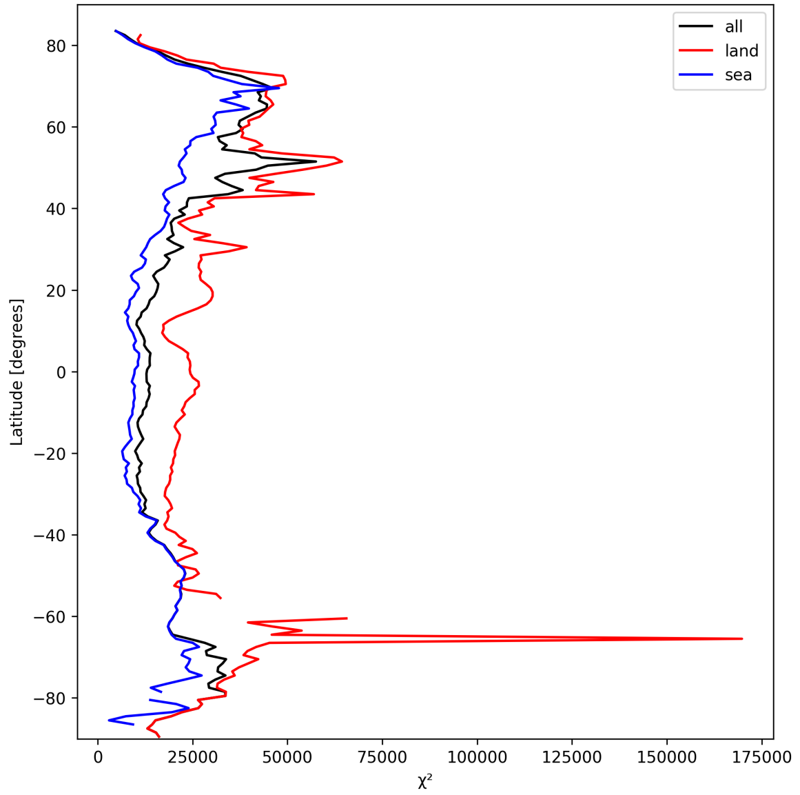
Figure 19: Zonal average of “ \chi^2 ” for 2025-03-07 to 2025-03-08.
