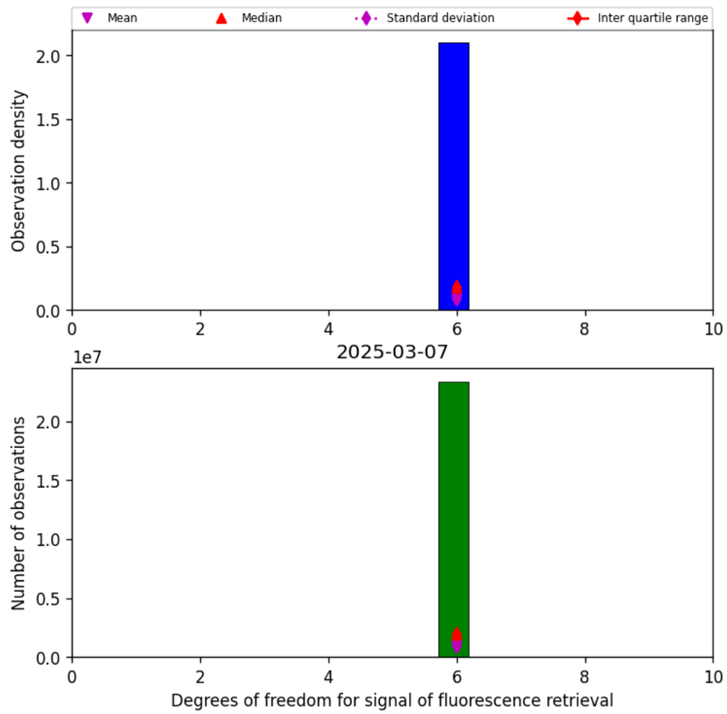
Figure 41: Histogram of “Degrees of freedom for signal of fluorescence retrieval” for 2025-03-07 to 2025-03-08
