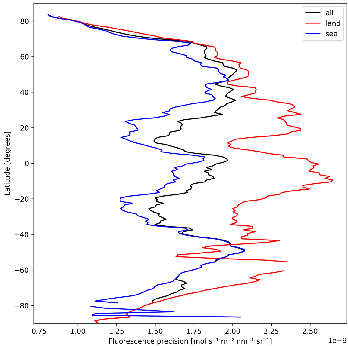
Figure 22: Zonal average of “Fluorescence precision” for 2025-03-07 to 2025-03-08.
