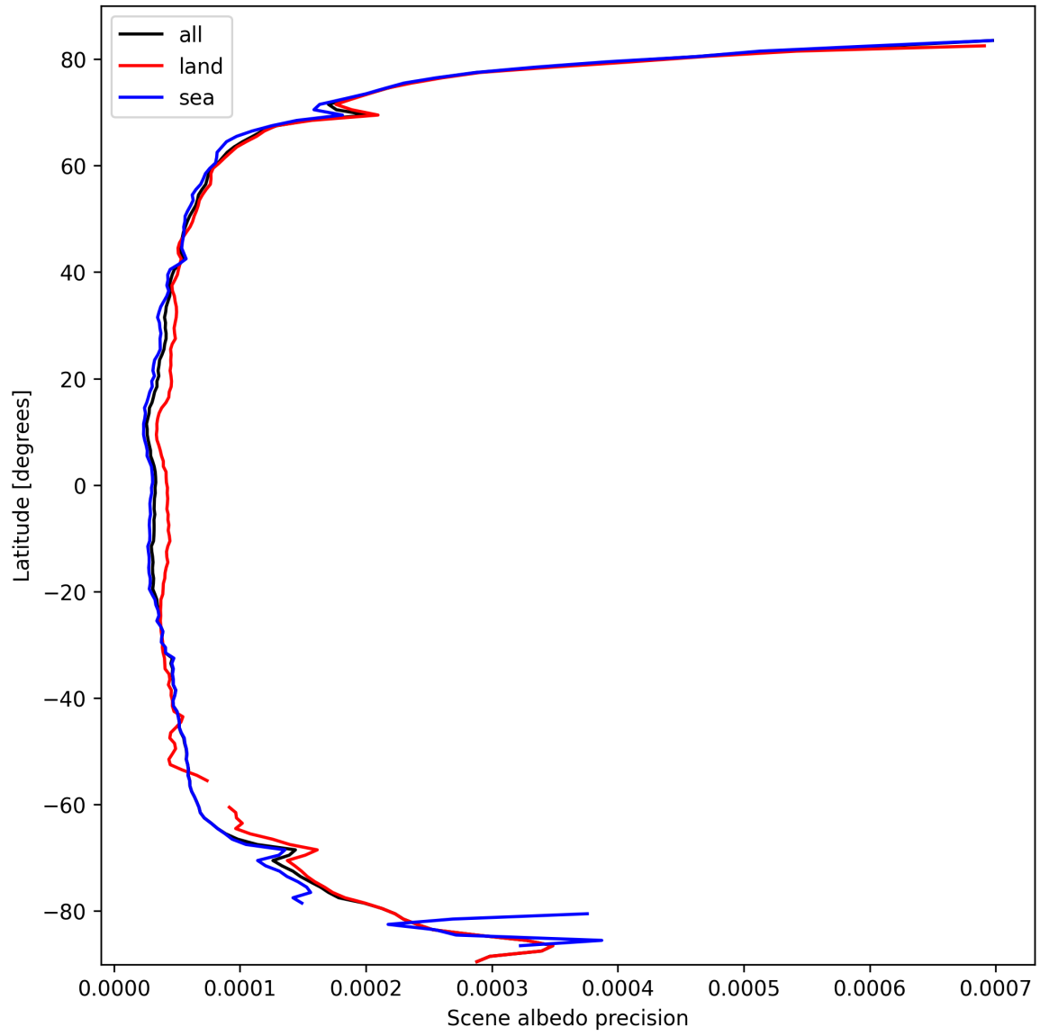
Figure 16: Zonal average of “Scene albedo precision” for 2025-03-07 to 2025-03-08.
