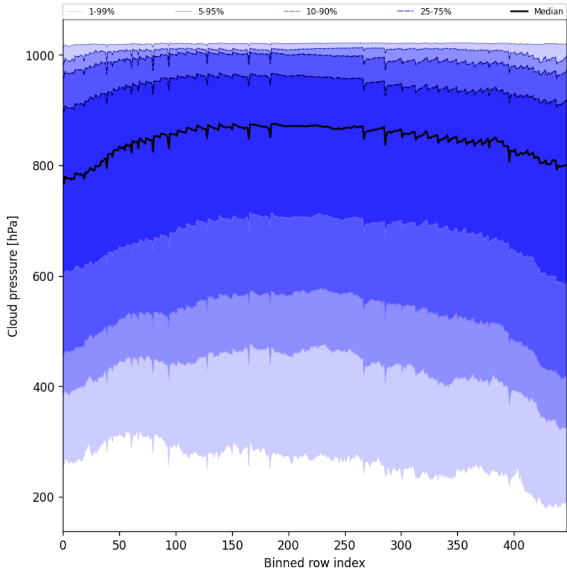
Figure 45: Along track statistics of “Cloud pressure” for 2025-03-07 to 2025-03-08
