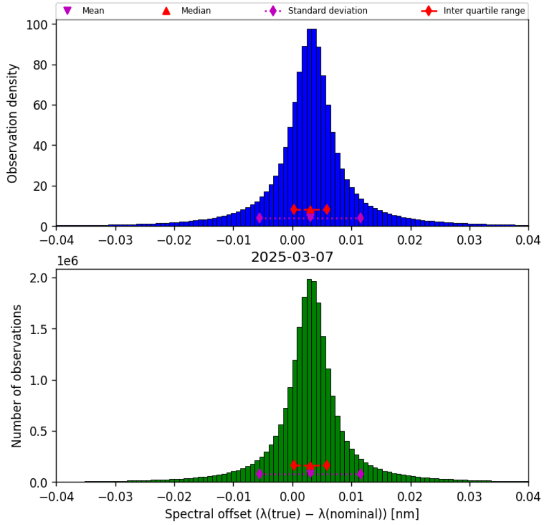
Figure 43: Histogram of “Spectral offset ( \lambda_{\text{true}} - \lambda_{\text{nominal}} )” for 2025-03-07 to 2025-03-08
