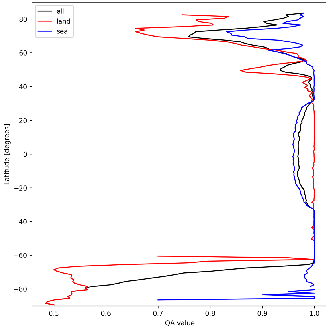
Figure 10: Zonal average of “QA value” for 2025-03-07 to 2025-03-08.
