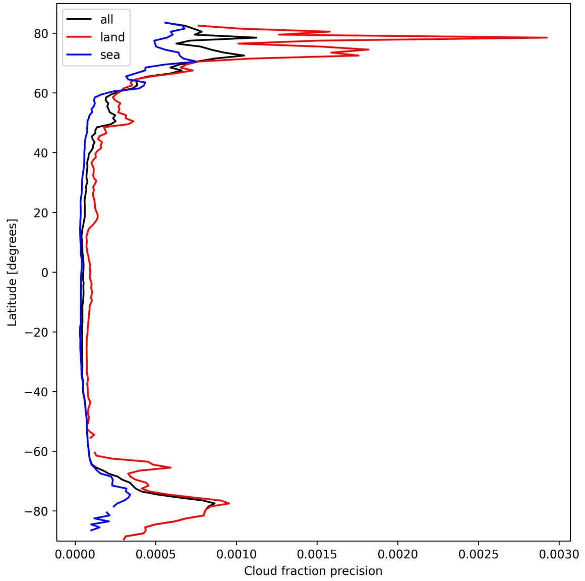
Figure 14: Zonal average of “Cloud fraction precision” for 2025-03-07 to 2025-03-08.
