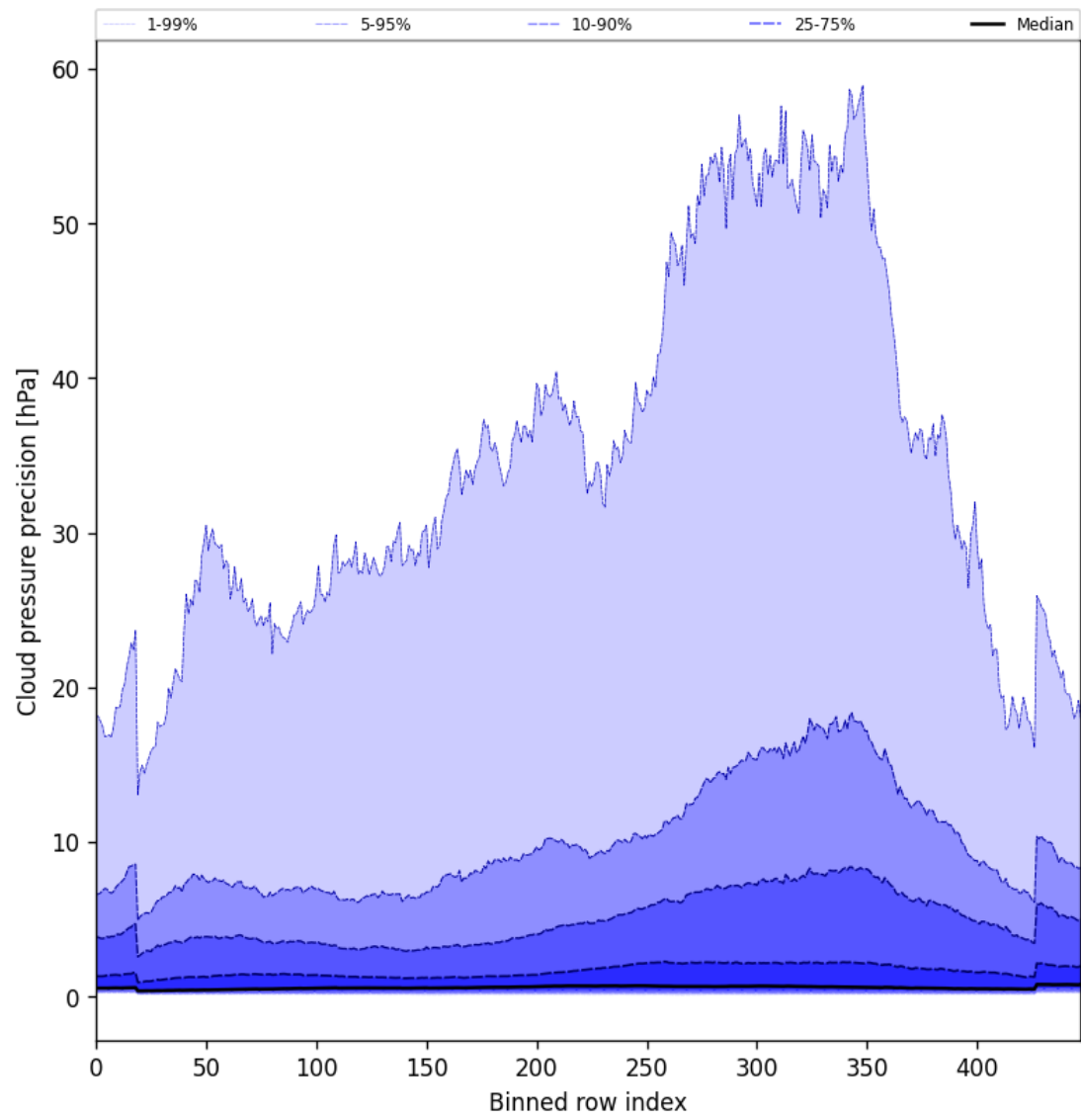
Figure 46: Along track statistics of “Cloud pressure precision” for 2025-03-07 to 2025-03-08
