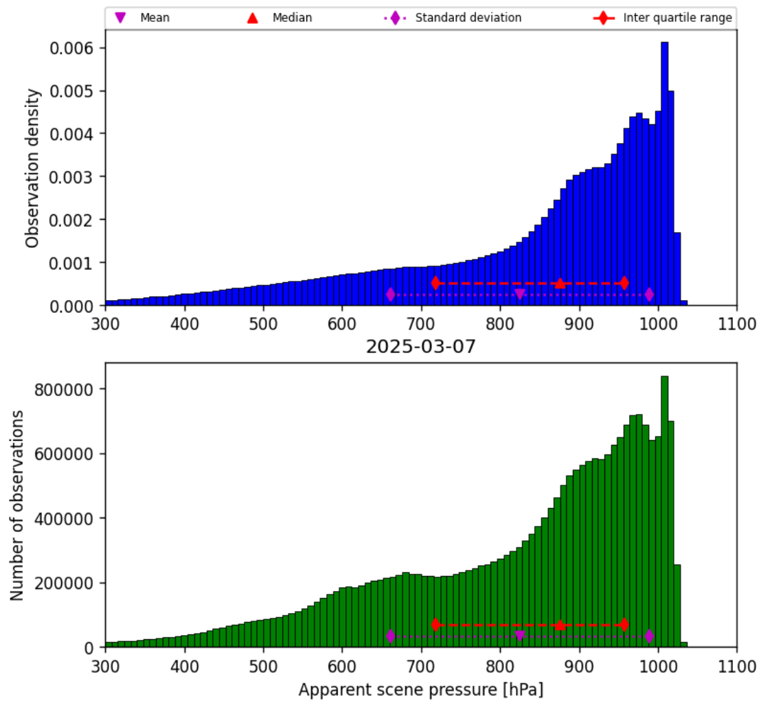
Figure 34: Histogram of “Apparent scene pressure” for 2025-03-07 to 2025-03-08
