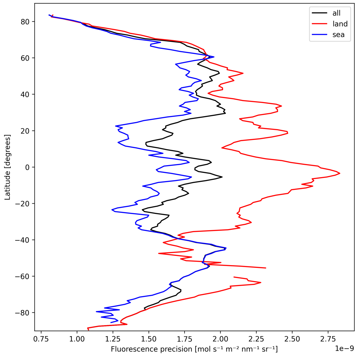
Figure 22: Zonal average of “Fluorescence precision” for 2025-03-08 to 2025-03-09.
