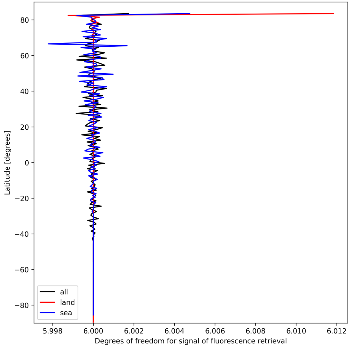
Figure 24: Zonal average of “Degrees of freedom for signal of fluorescence retrieval” for 2025-03-08 to 2025-03-09.
