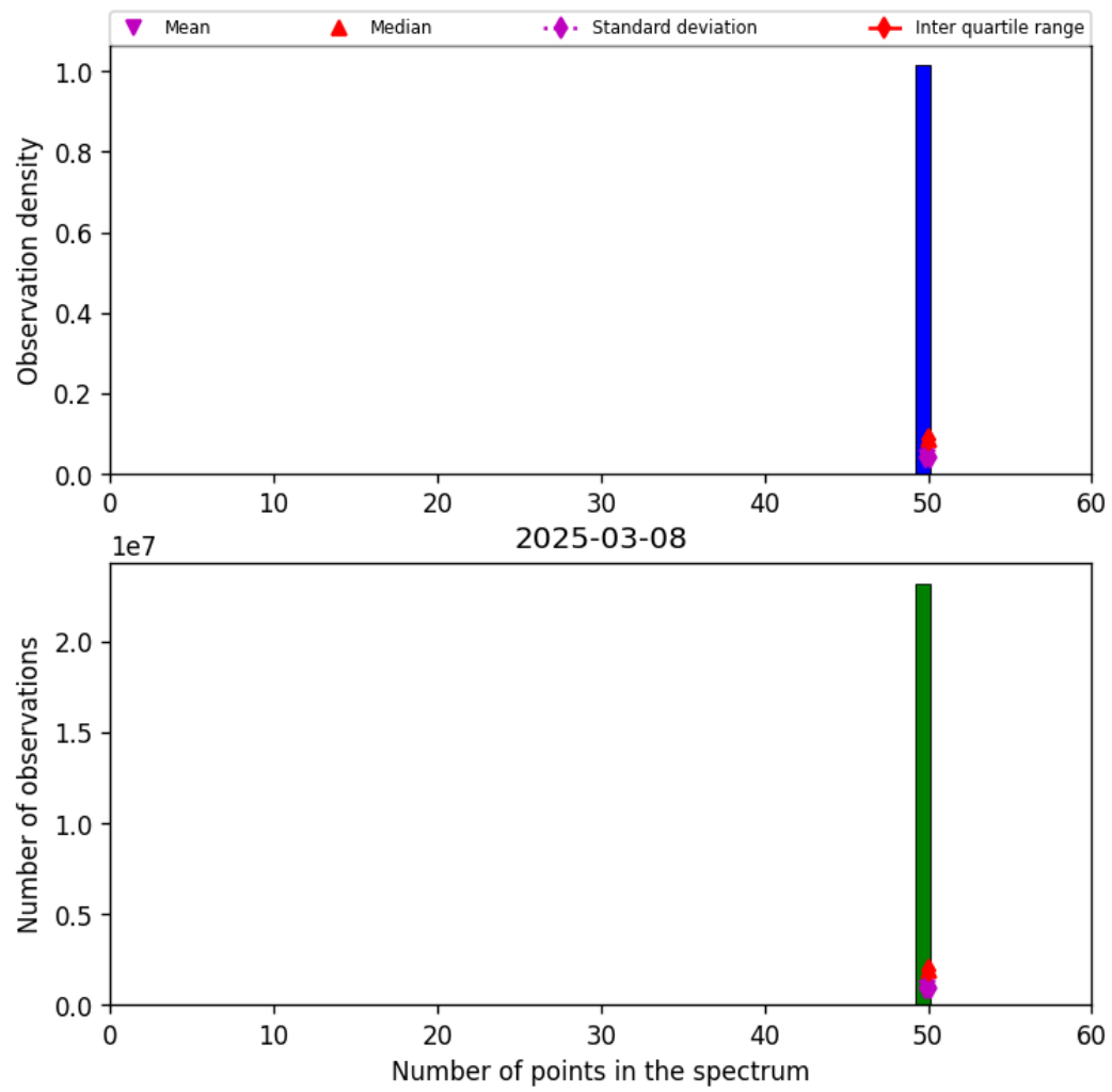
Figure 42: Histogram of “Number of points in the spectrum” for 2025-03-08 to 2025-03-09
