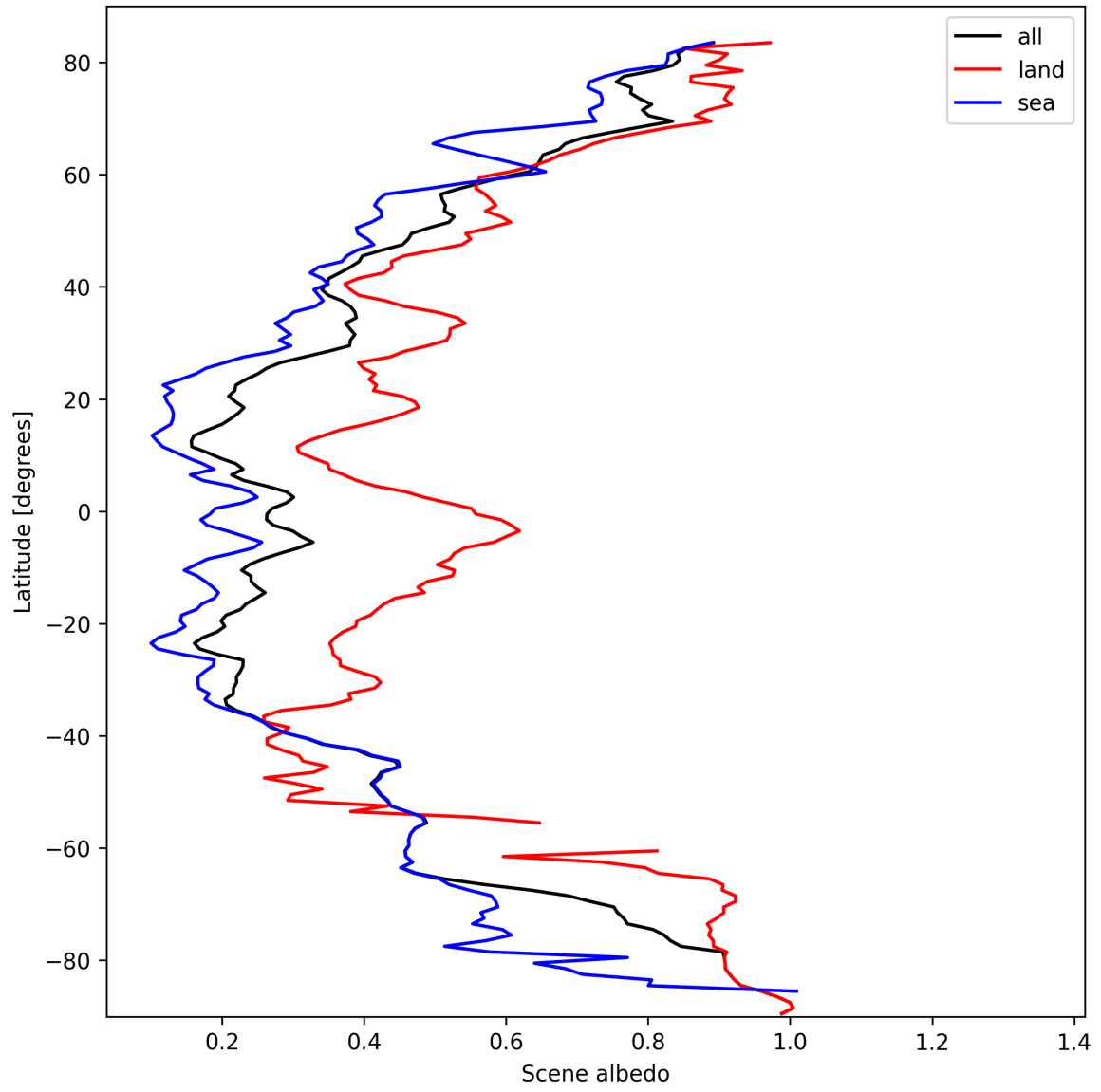
Figure 15: Zonal average of “Scene albedo” for 2025-03-08 to 2025-03-09.
