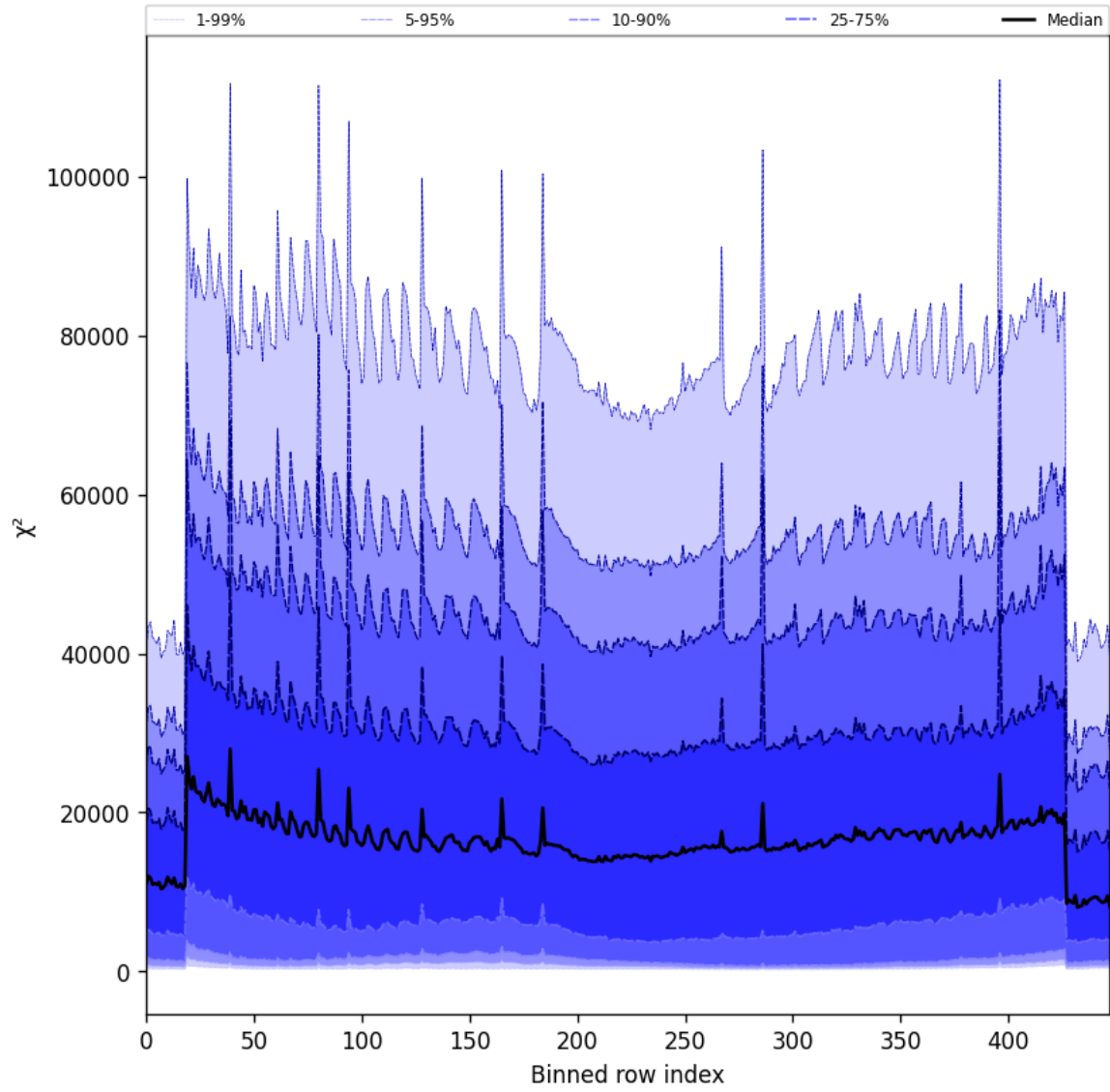
Figure 53: Along track statistics of “ \chi^2 ” for 2025-03-08 to 2025-03-09
