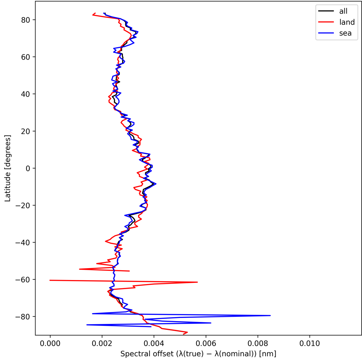
Figure 26: Zonal average of “Spectral offset ( \lambda_{\text{true}} - \lambda_{\text{nominal}} )” for 2025-03-08 to 2025-03-09.
