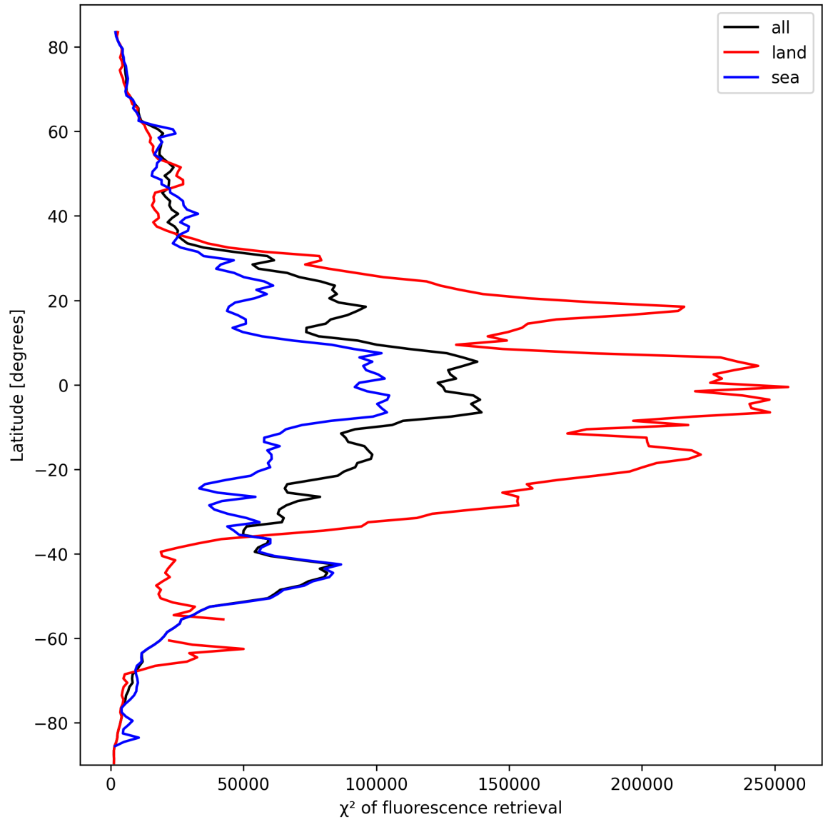
Figure 23: Zonal average of “ \chi^2 of fluorescence retrieval” for 2025-03-08 to 2025-03-09.
