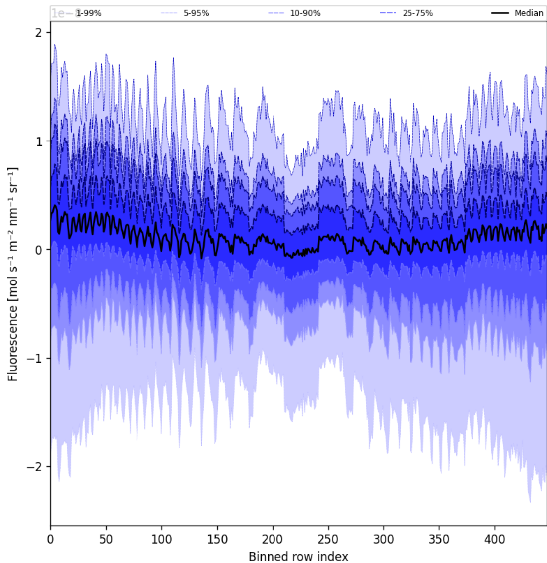
Figure 55: Along track statistics of "Fluorescence" for 2025-03-08 to 2025-03-09
