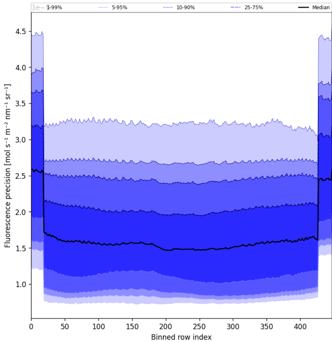
Figure 56: Along track statistics of “Fluorescence precision” for 2025-03-08 to 2025-03-09
