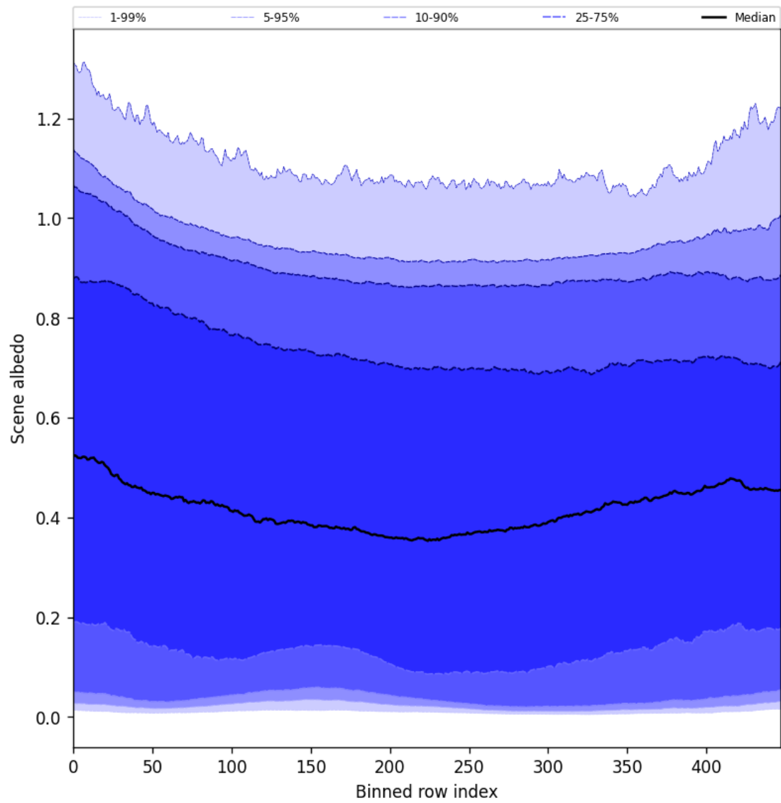
Figure 49: Along track statistics of “Scene albedo” for 2025-03-08 to 2025-03-09
