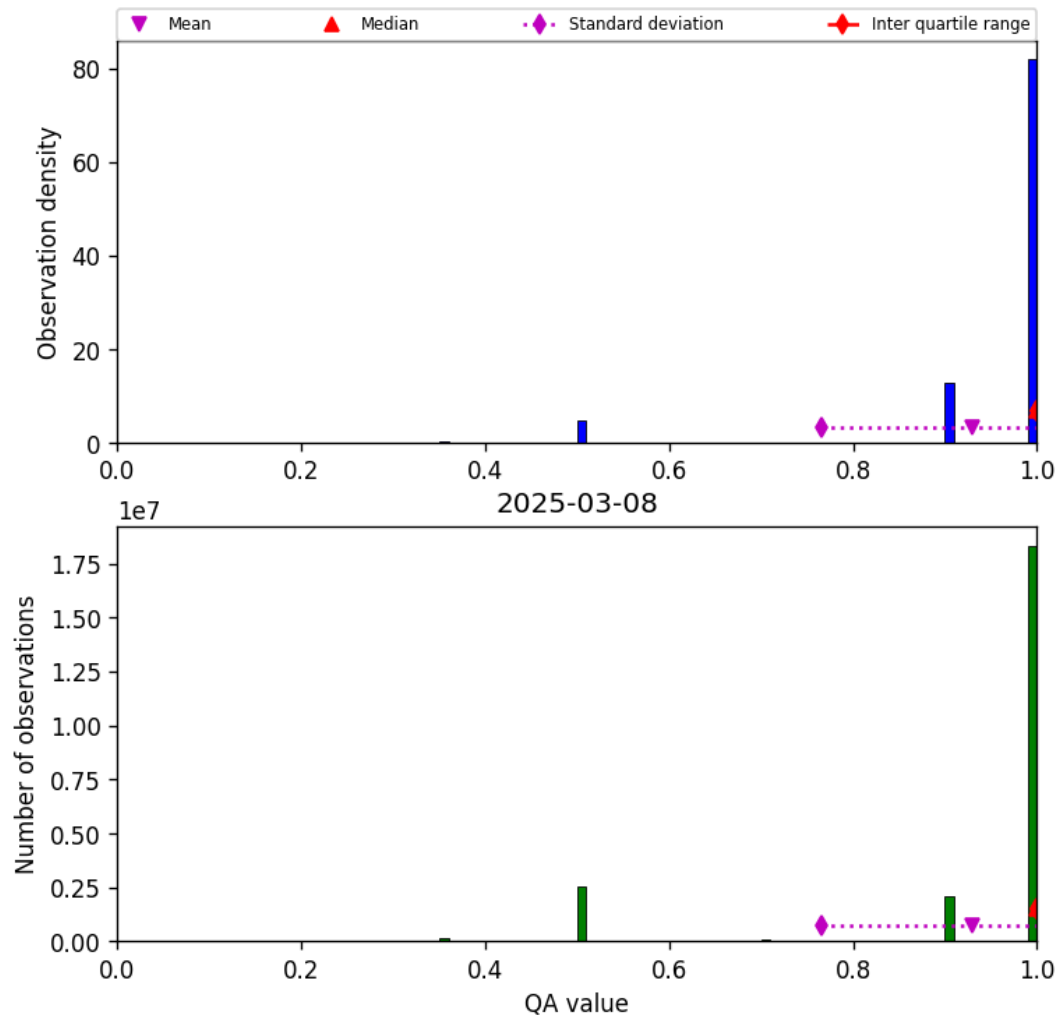
Figure 27: Histogram of “QA value” for 2025-03-08 to 2025-03-09
