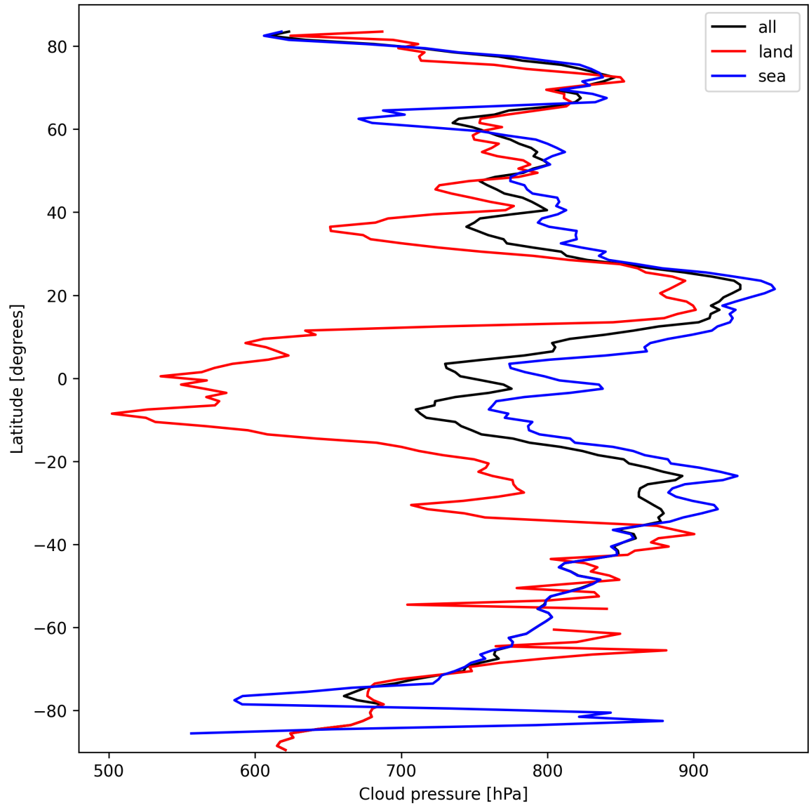
Figure 11: Zonal average of “Cloud pressure” for 2025-03-08 to 2025-03-09.
