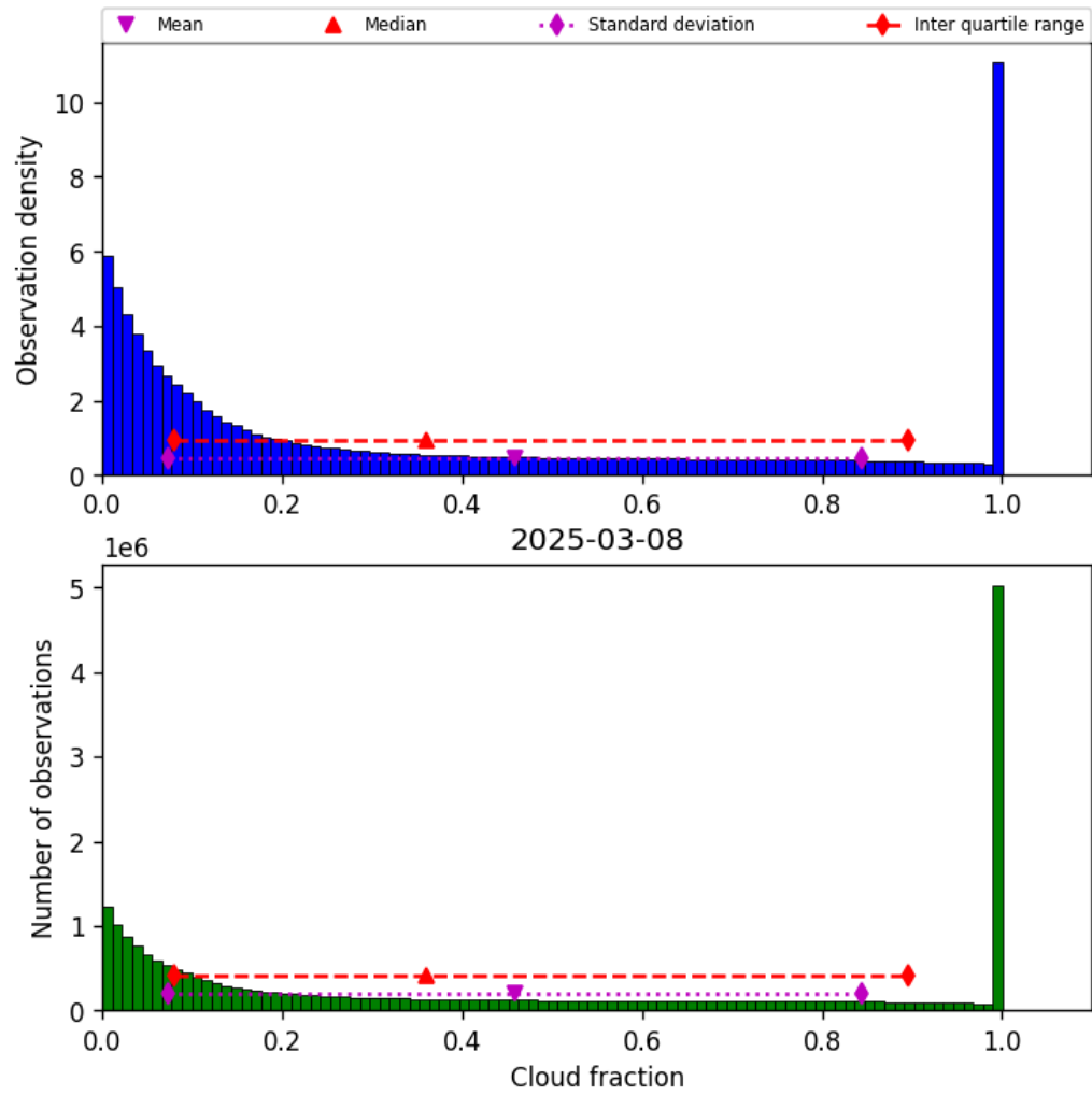
Figure 30: Histogram of “Cloud fraction” for 2025-03-08 to 2025-03-09
