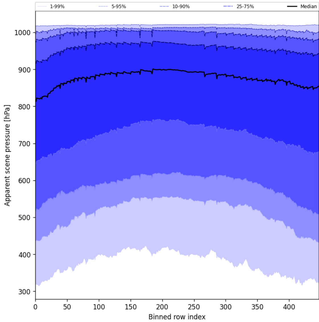
Figure 51: Along track statistics of “Apparent scene pressure” for 2025-03-08 to 2025-03-09
