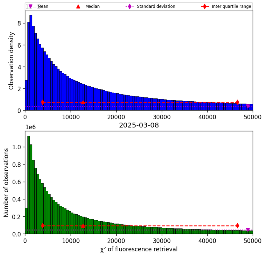
Figure 40: Histogram of “ \chi^2 of fluorescence retrieval” for 2025-03-08 to 2025-03-09
