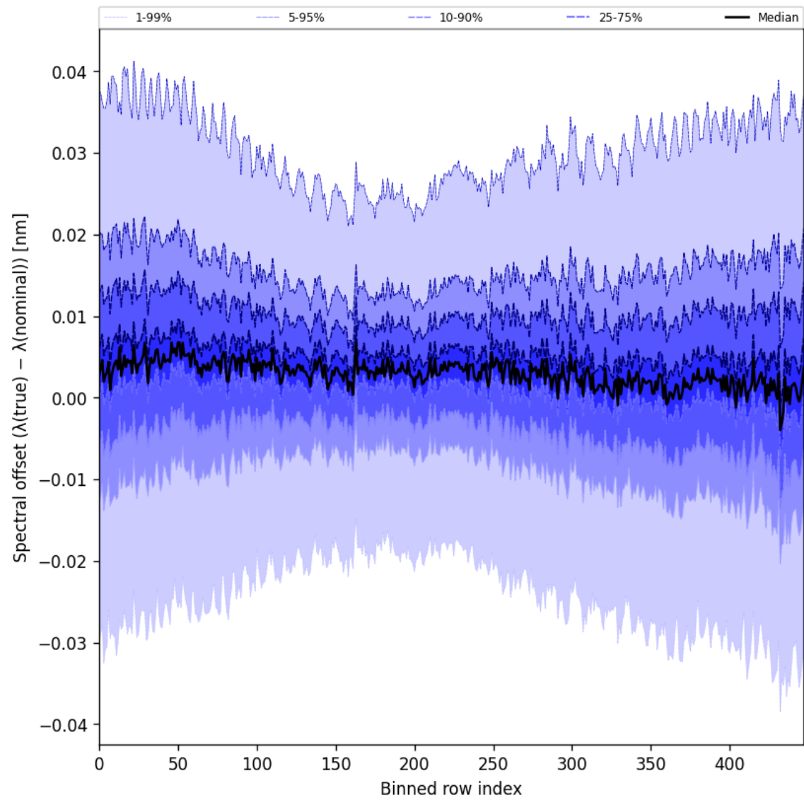
Figure 60: Along track statistics of “Spectral offset ( \lambda_{\text{true}} - \lambda_{\text{nominal}} )” for 2025-03-08 to 2025-03-09
