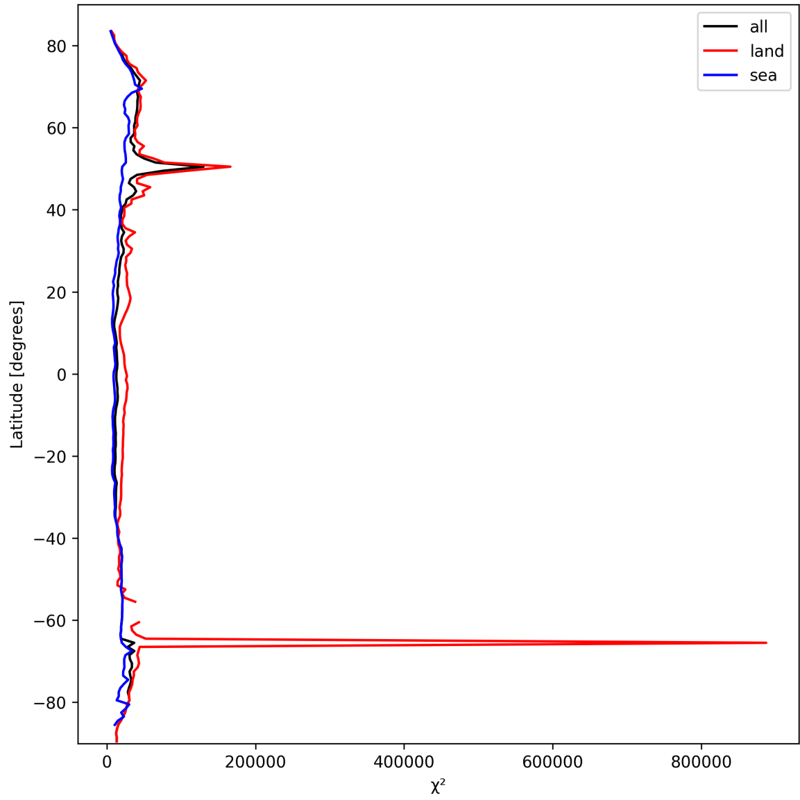
Figure 19: Zonal average of “ \chi^2 ” for 2025-03-08 to 2025-03-09.
