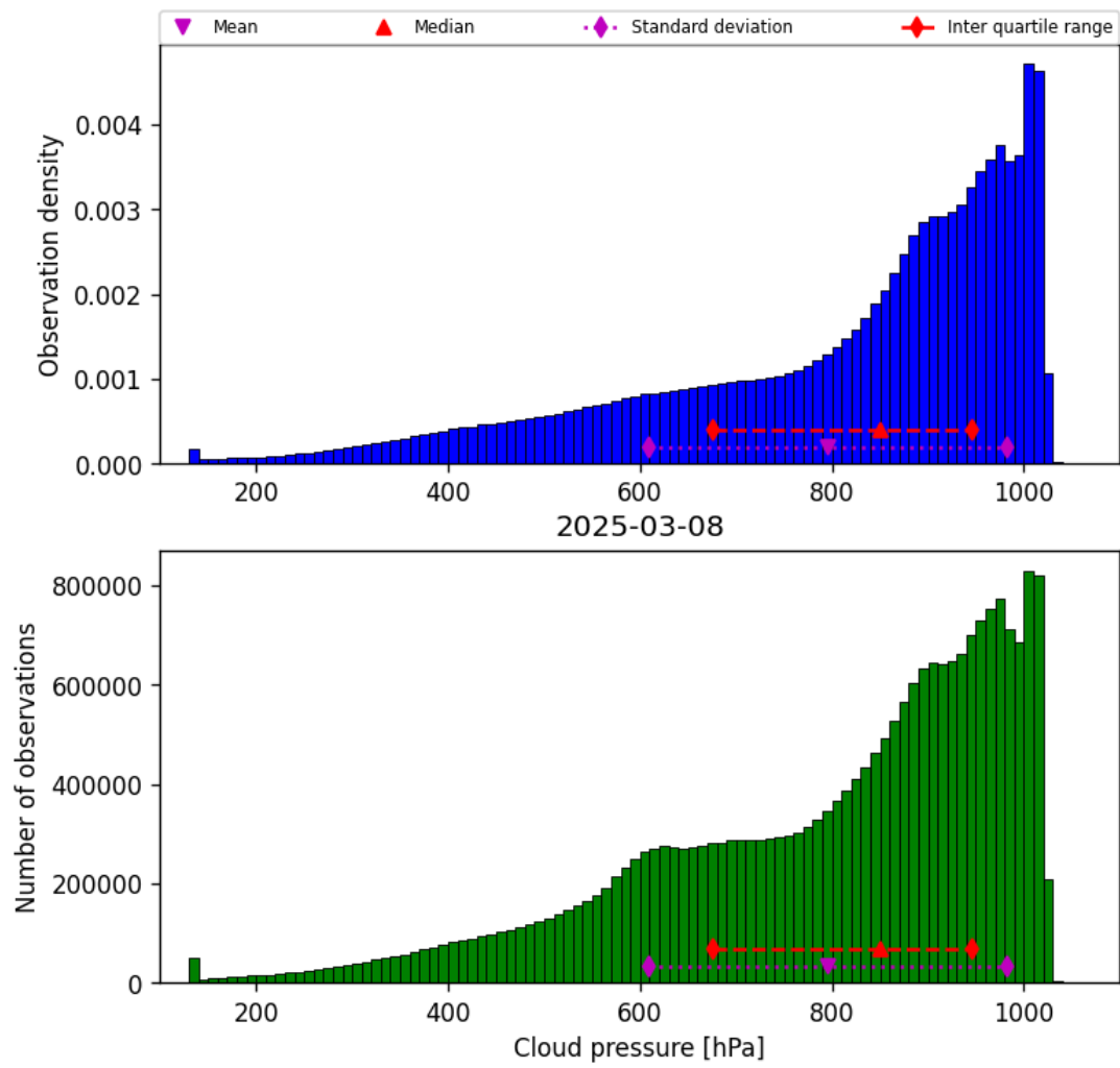
Figure 28: Histogram of “Cloud pressure” for 2025-03-08 to 2025-03-09
