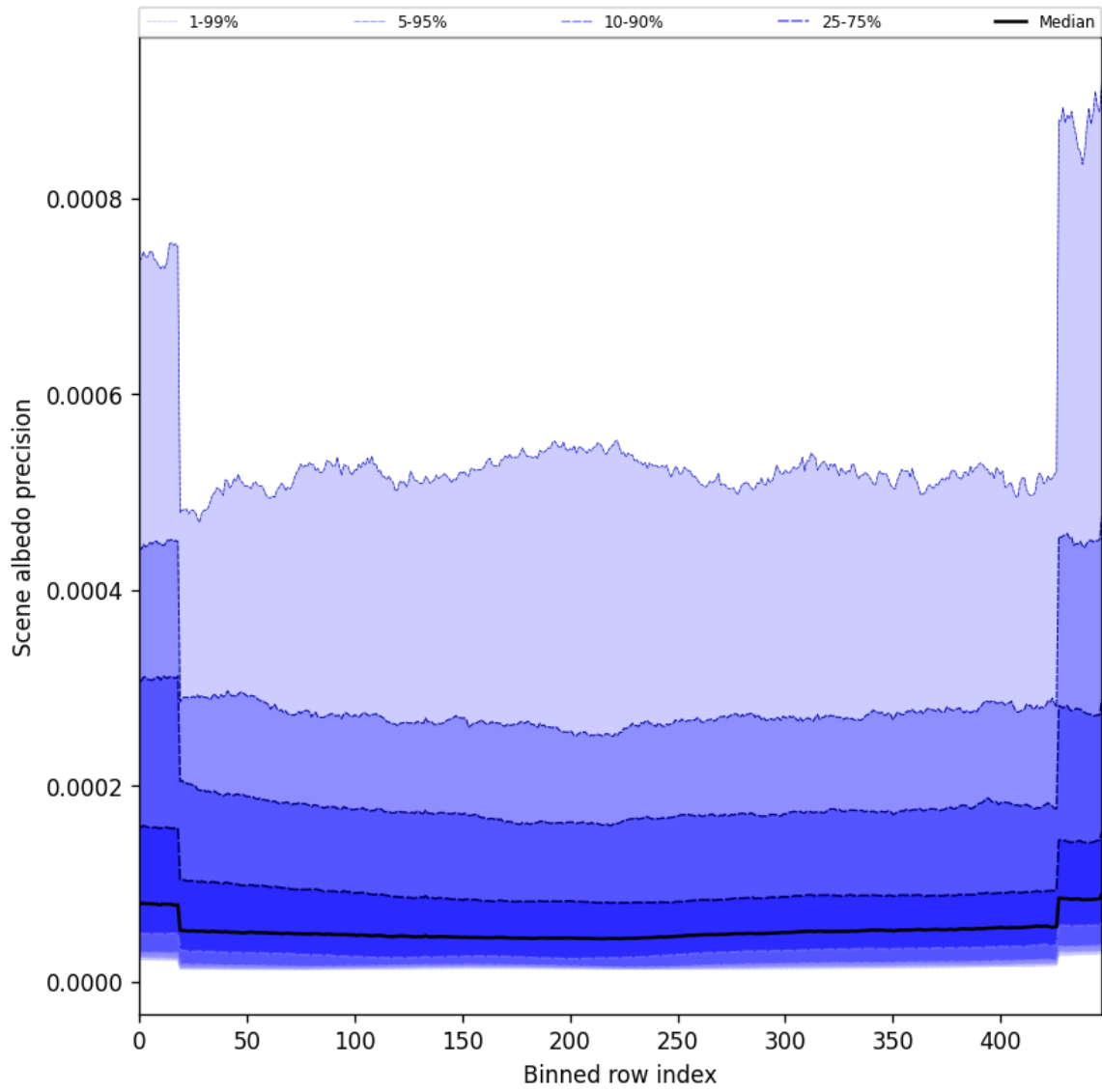
Figure 50: Along track statistics of “Scene albedo precision” for 2025-03-08 to 2025-03-09
