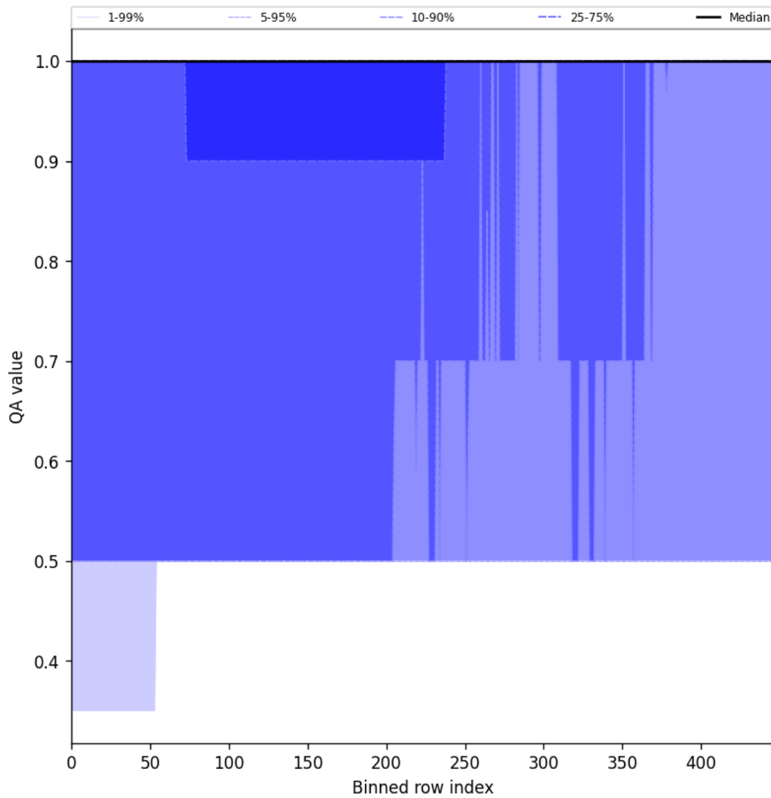
Figure 44: Along track statistics of “QA value” for 2025-03-08 to 2025-03-09
