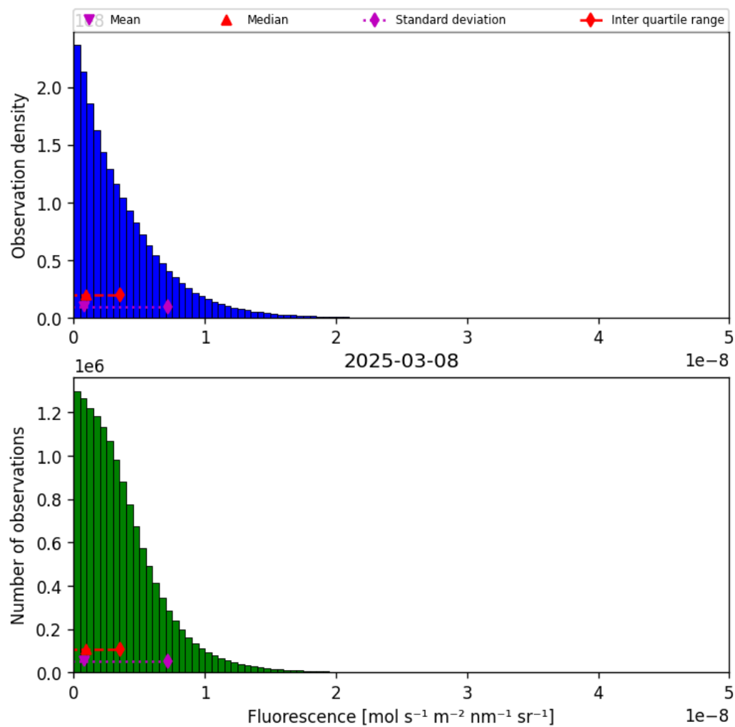
Figure 38: Histogram of “Fluorescence” for 2025-03-08 to 2025-03-09
