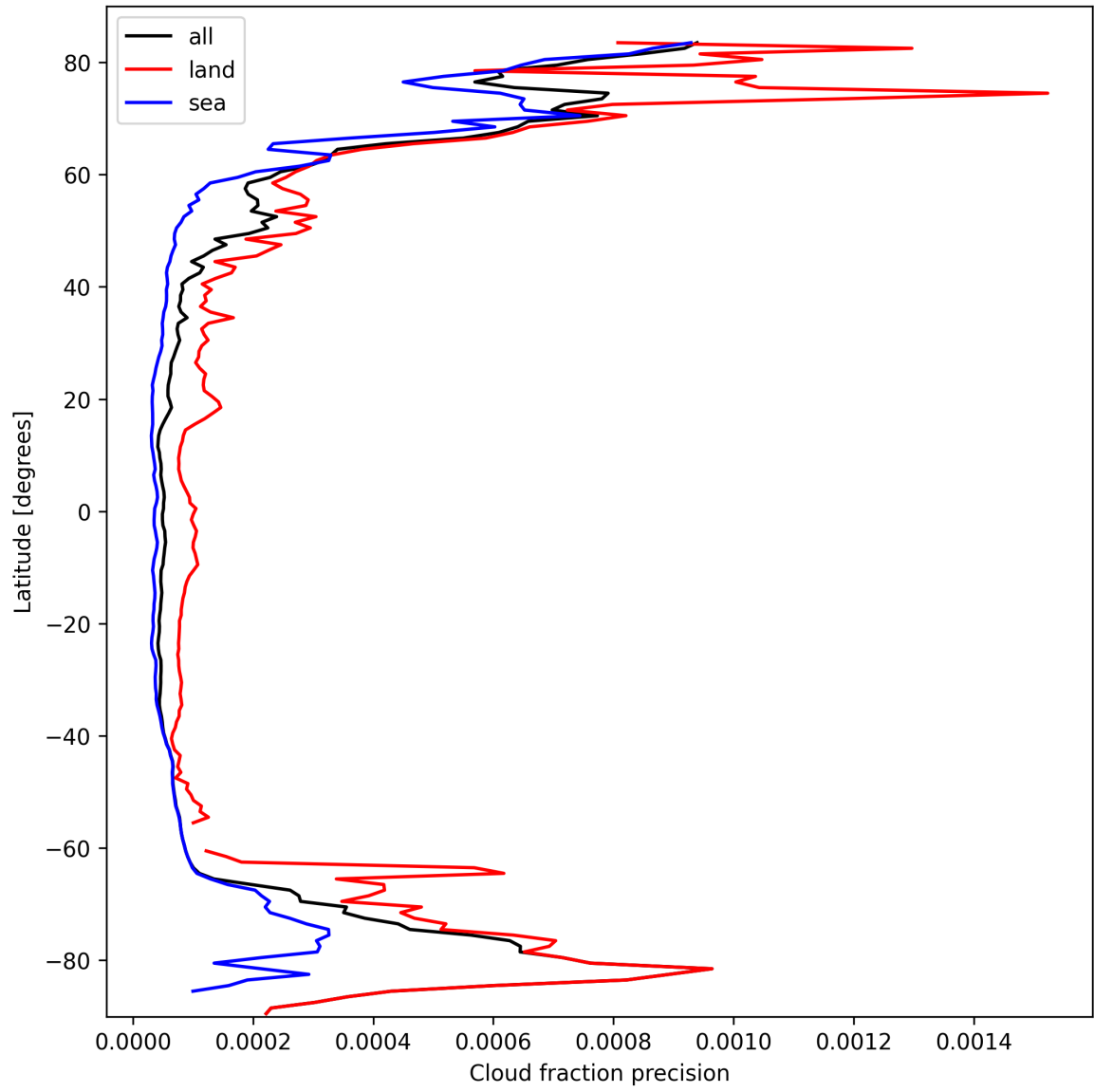
Figure 14: Zonal average of “Cloud fraction precision” for 2025-03-08 to 2025-03-09.
