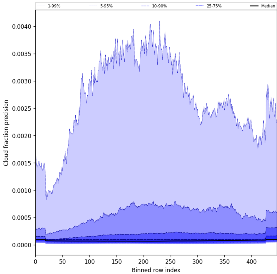
Figure 48: Along track statistics of “Cloud fraction precision” for 2025-03-08 to 2025-03-09
