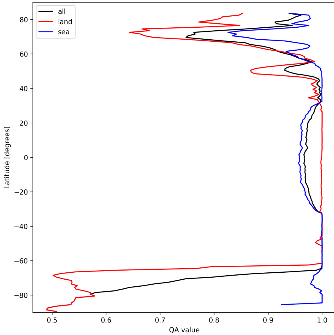
Figure 10: Zonal average of “QA value” for 2025-03-08 to 2025-03-09.
