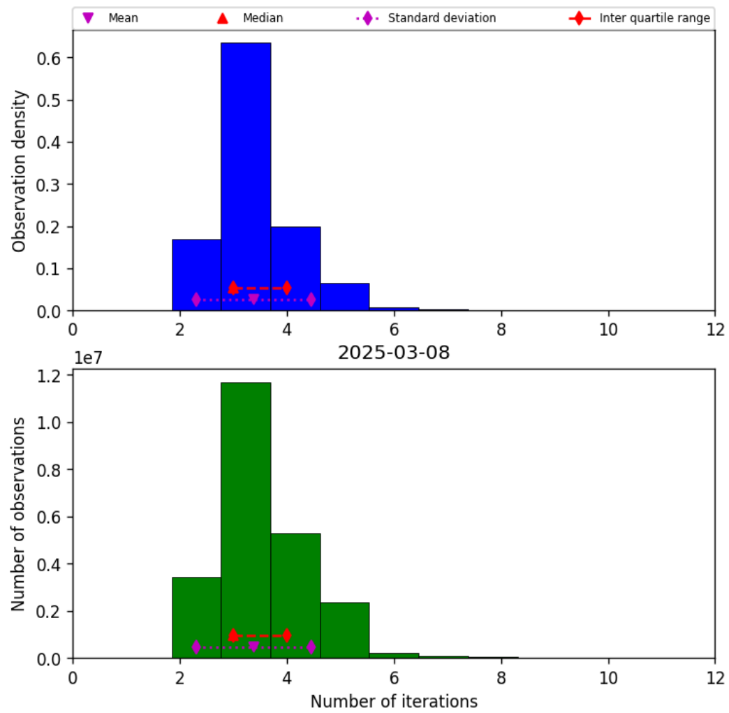
Figure 37: Histogram of “Number of iterations” for 2025-03-08 to 2025-03-09
