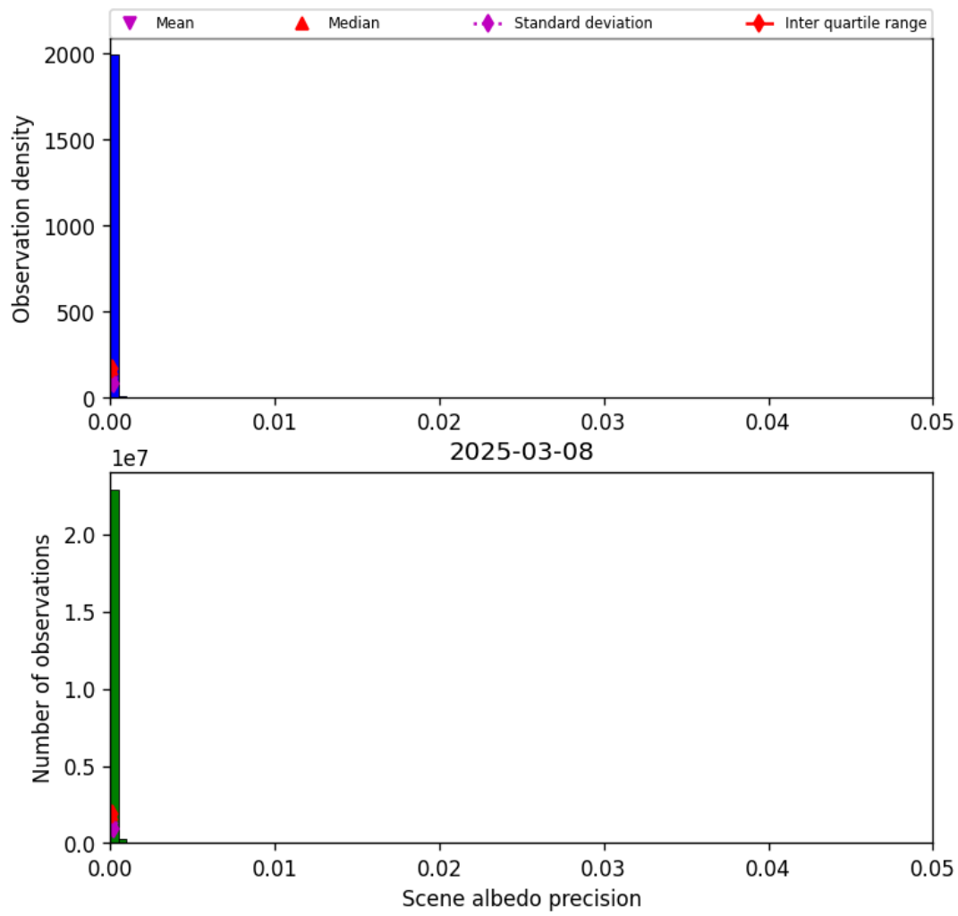
Figure 33: Histogram of “Scene albedo precision” for 2025-03-08 to 2025-03-09
