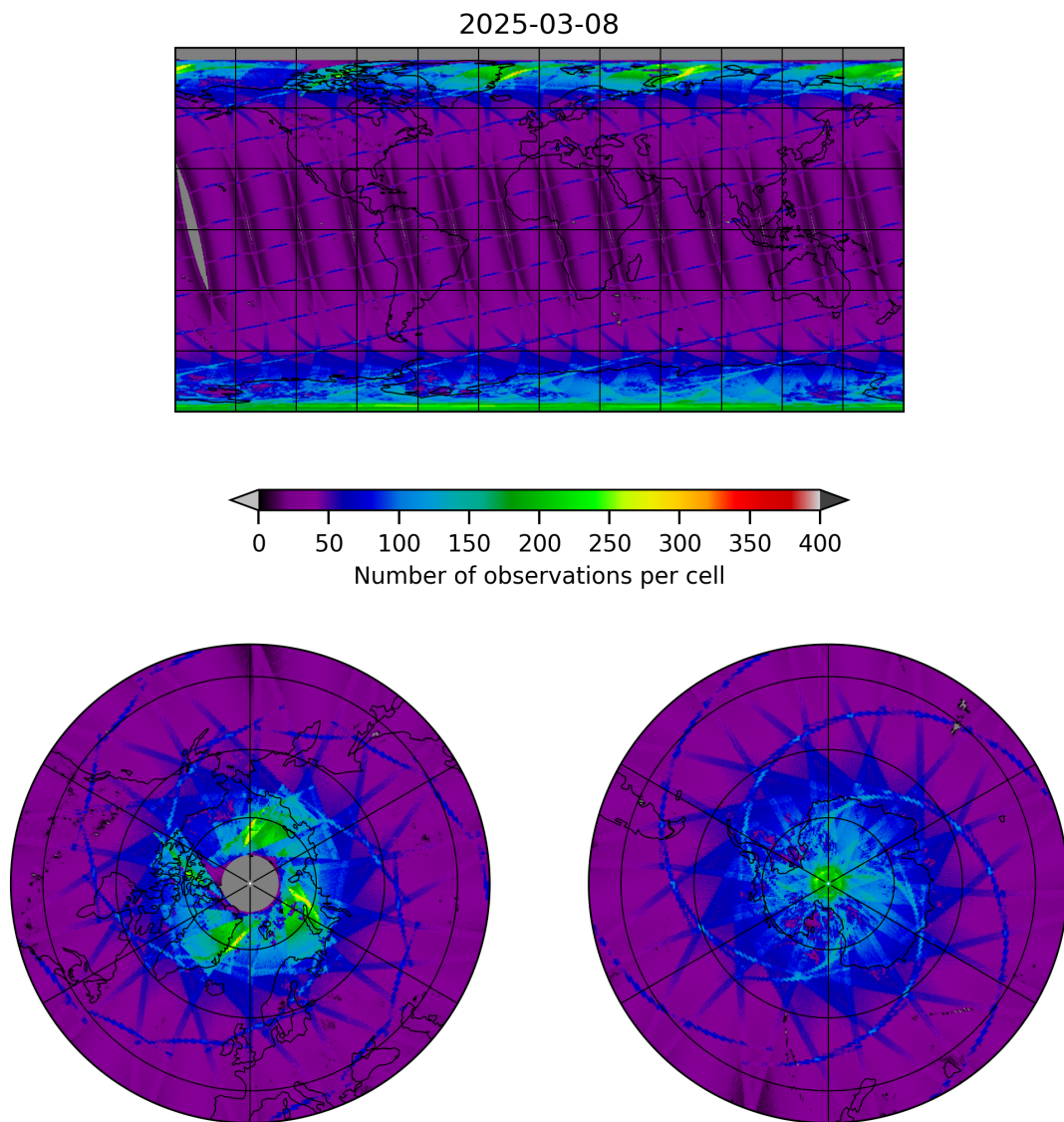
Figure 9: Map of the number of observations for 2025-03-08 to 2025-03-09
