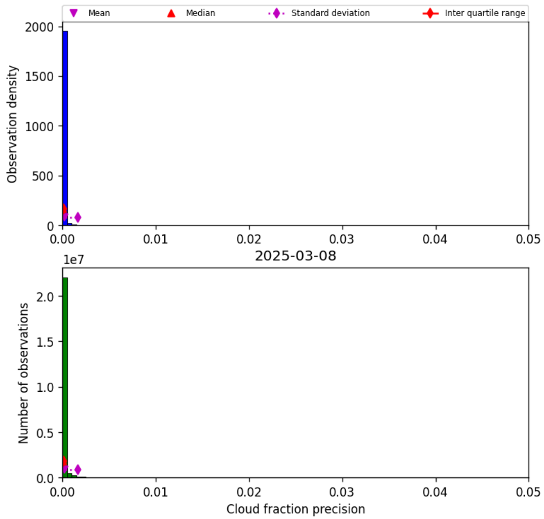
Figure 31: Histogram of “Cloud fraction precision” for 2025-03-08 to 2025-03-09
