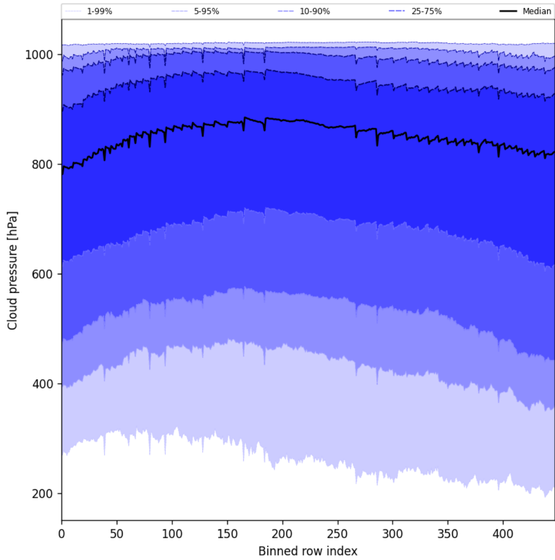
Figure 45: Along track statistics of “Cloud pressure” for 2025-03-08 to 2025-03-09
