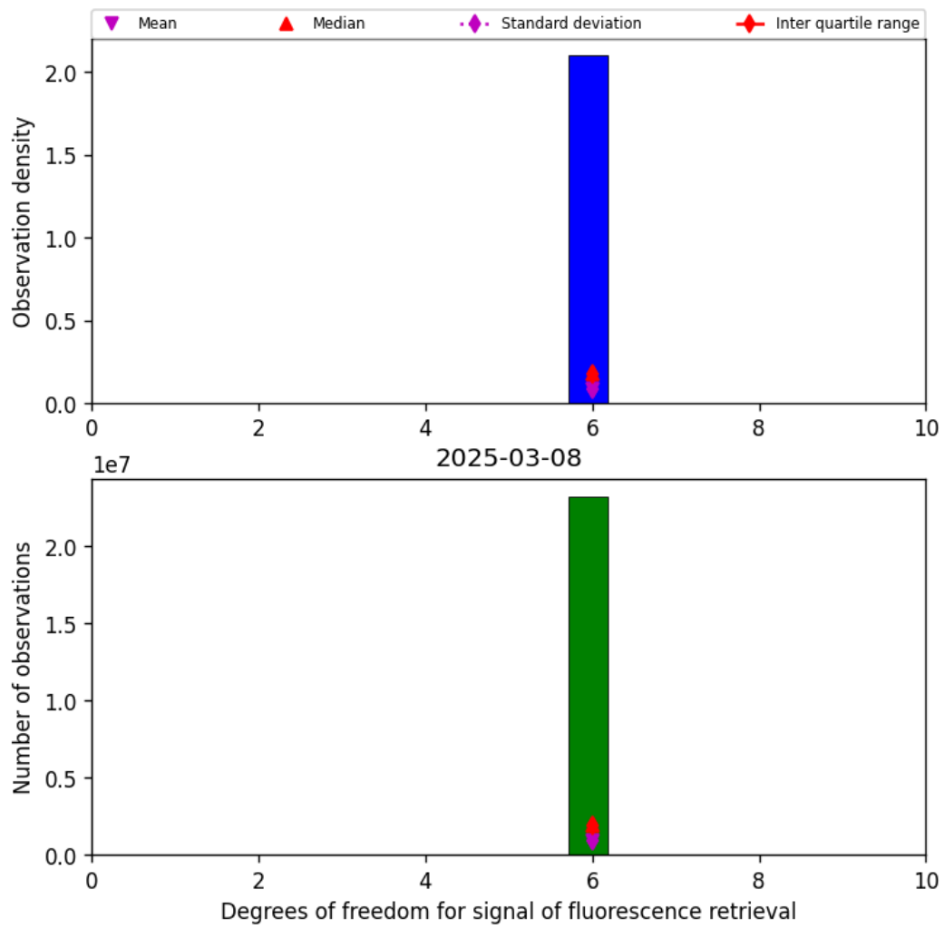
Figure 41: Histogram of “Degrees of freedom for signal of fluorescence retrieval” for 2025-03-08 to 2025-03-09
