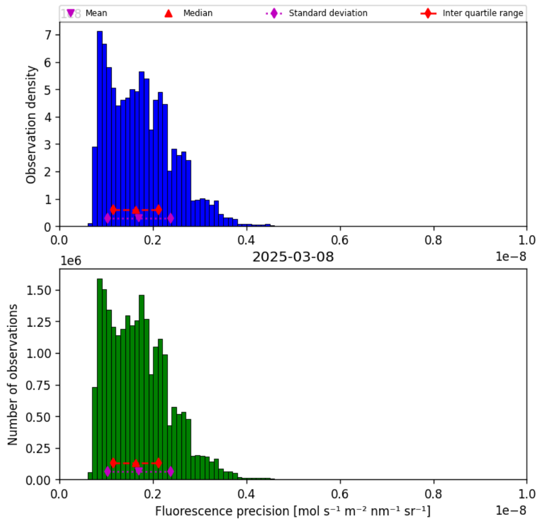
Figure 39: Histogram of “Fluorescence precision” for 2025-03-08 to 2025-03-09
