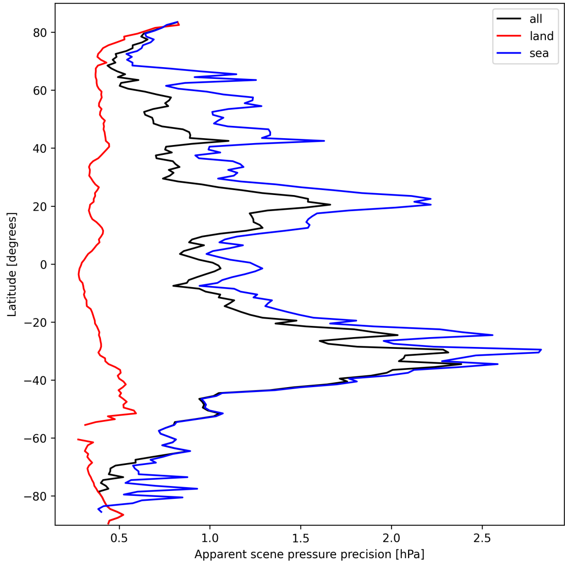
Figure 18: Zonal average of “Apparent scene pressure precision” for 2025-03-08 to 2025-03-09.
