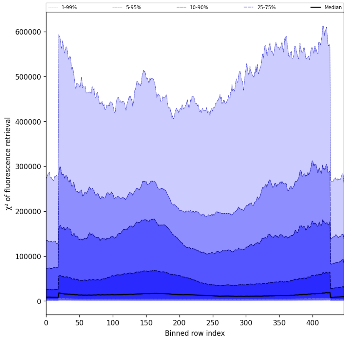
Figure 57: Along track statistics of “ \chi^2 of fluorescence retrieval” for 2025-03-08 to 2025-03-09
