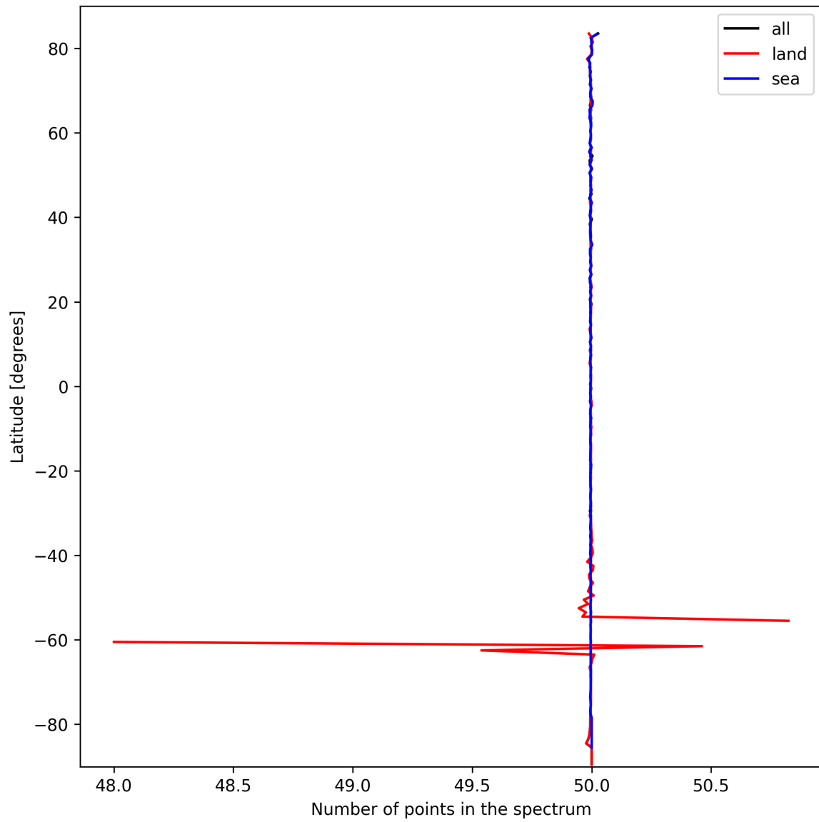
Figure 25: Zonal average of “Number of points in the spectrum” for 2025-03-08 to 2025-03-09.
