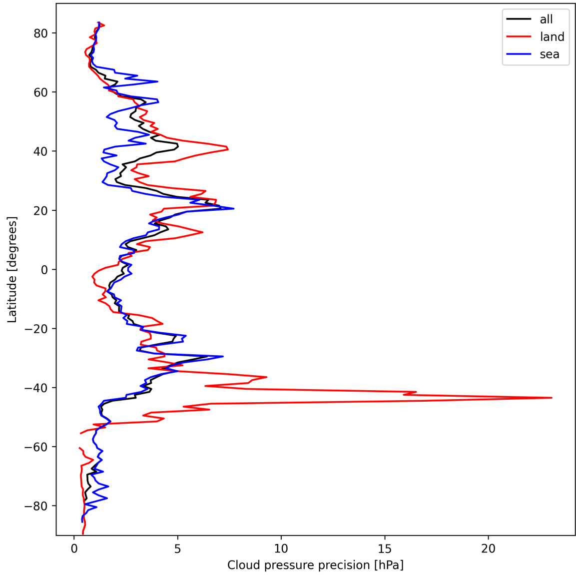
Figure 12: Zonal average of “Cloud pressure precision” for 2025-03-08 to 2025-03-09.
