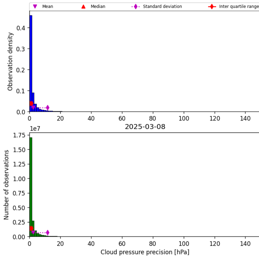
Figure 29: Histogram of “Cloud pressure precision” for 2025-03-08 to 2025-03-09
