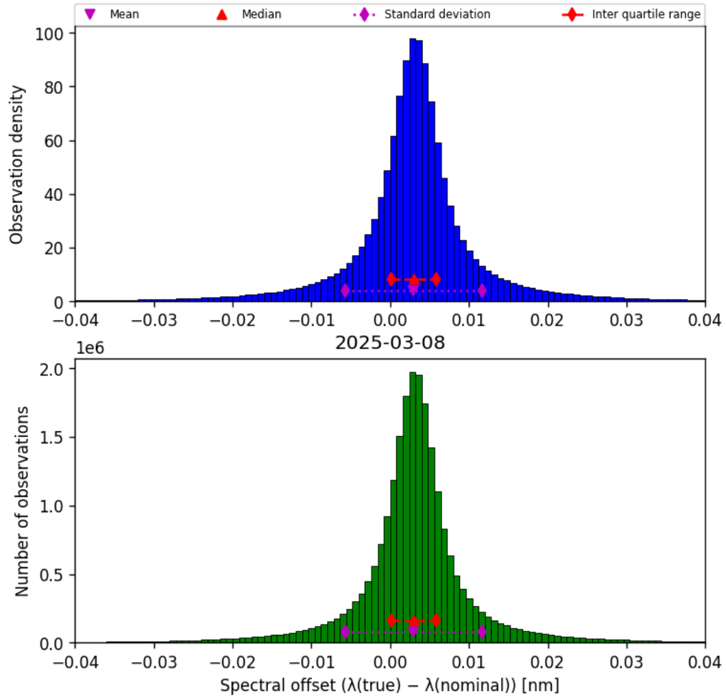
Figure 43: Histogram of “Spectral offset ( \lambda_{\text{true}} - \lambda_{\text{nominal}} )” for 2025-03-08 to 2025-03-09
