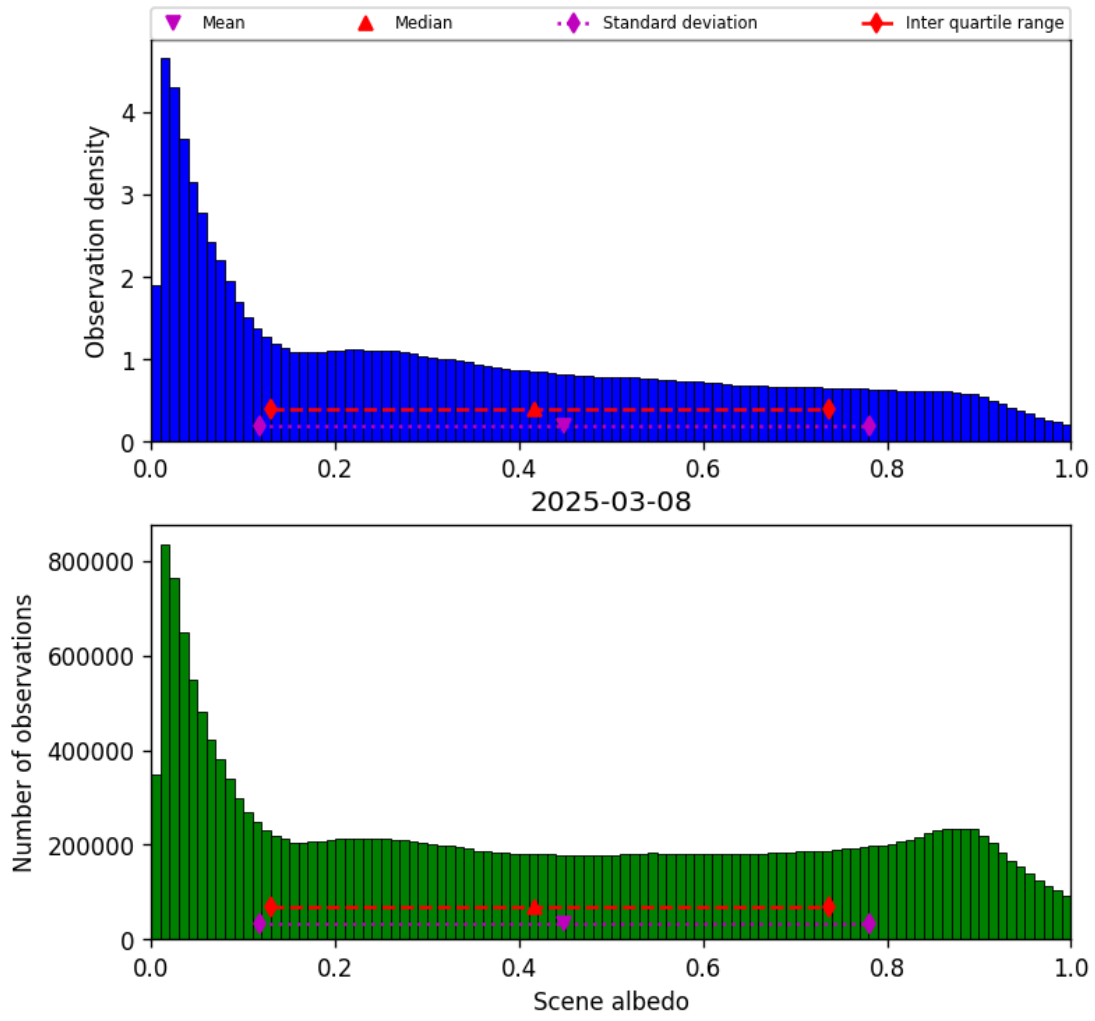
Figure 32: Histogram of “Scene albedo” for 2025-03-08 to 2025-03-09
