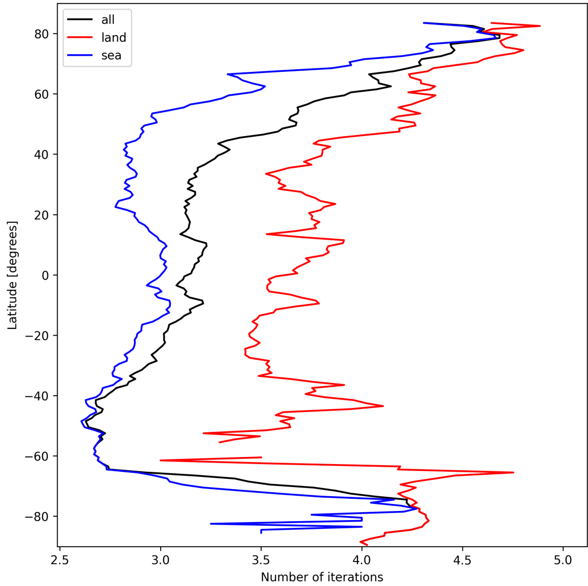
Figure 20: Zonal average of “Number of iterations” for 2025-03-08 to 2025-03-09.
