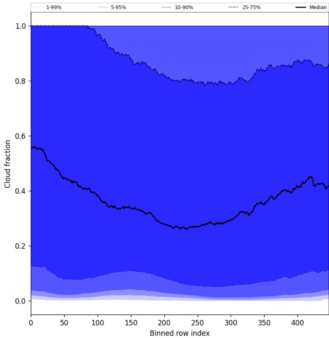
Figure 47: Along track statistics of “Cloud fraction” for 2025-03-08 to 2025-03-09
