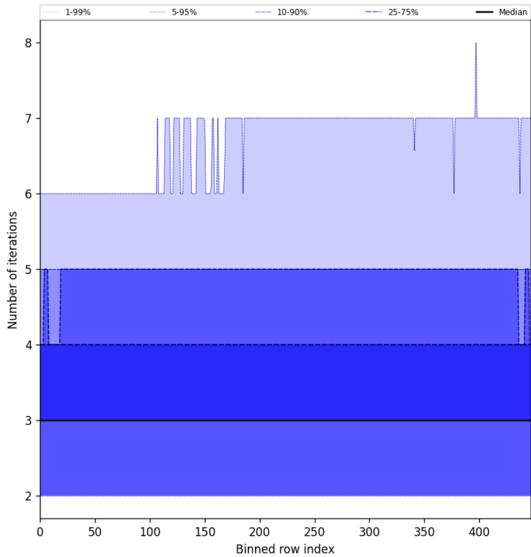
Figure 54: Along track statistics of “Number of iterations” for 2025-03-08 to 2025-03-09
