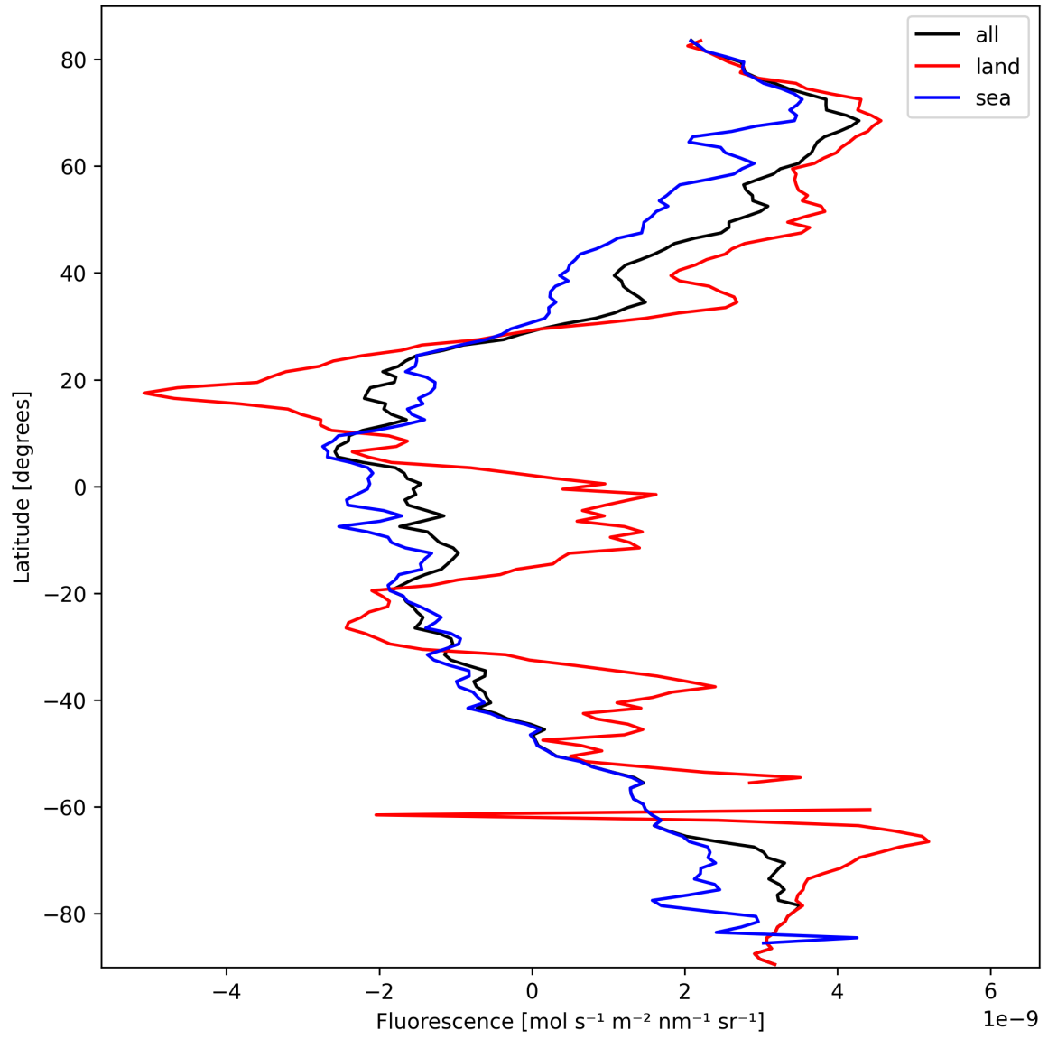
Figure 21: Zonal average of “Fluorescence” for 2025-03-08 to 2025-03-09.
