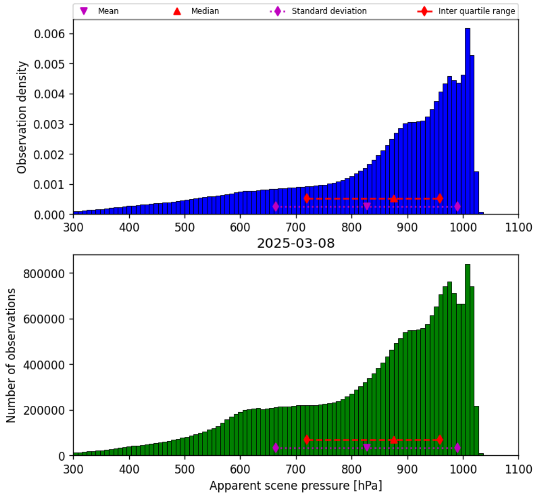
Figure 34: Histogram of “Apparent scene pressure” for 2025-03-08 to 2025-03-09
