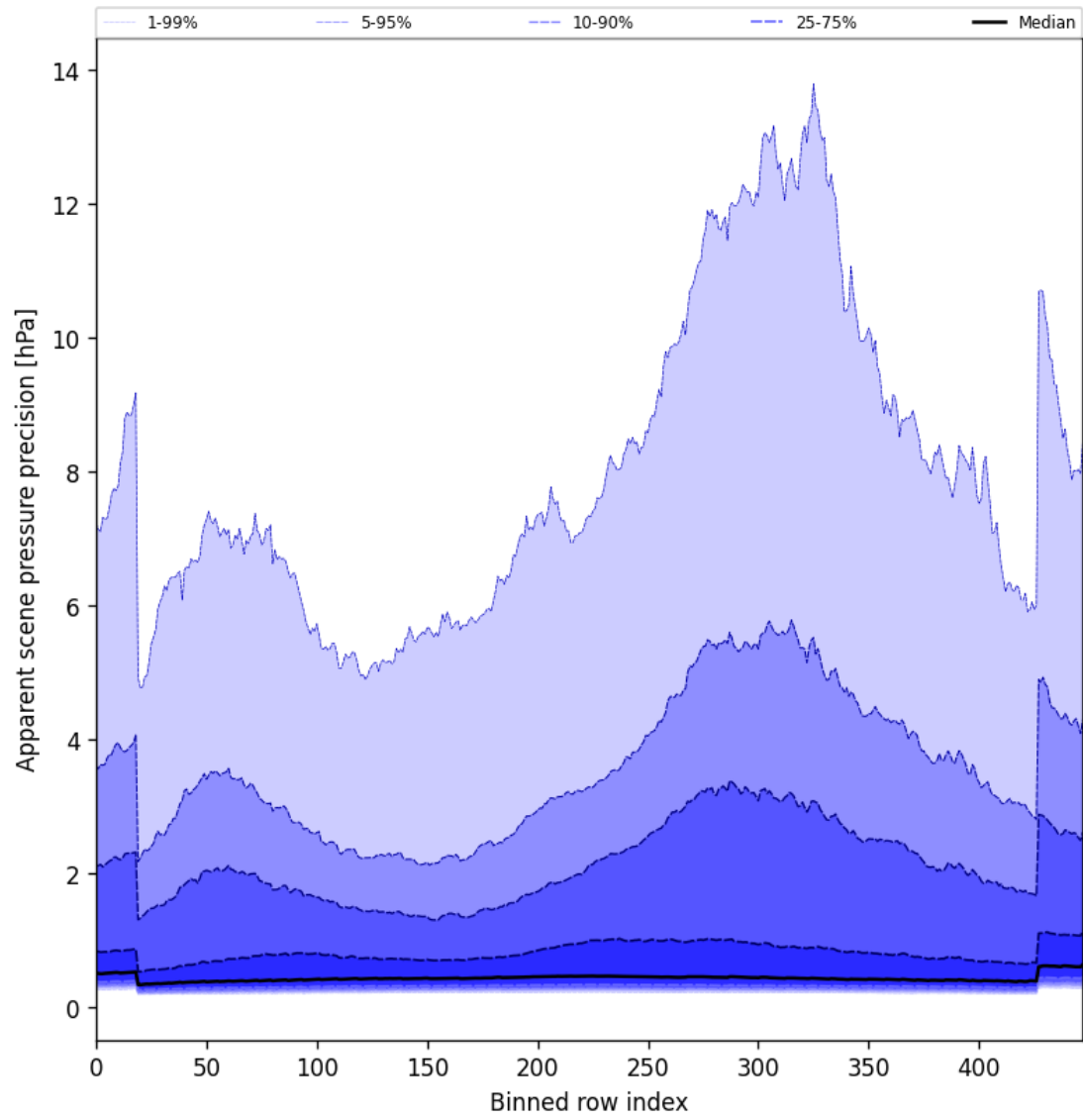
Figure 52: Along track statistics of “Apparent scene pressure precision” for 2025-03-08 to 2025-03-09
