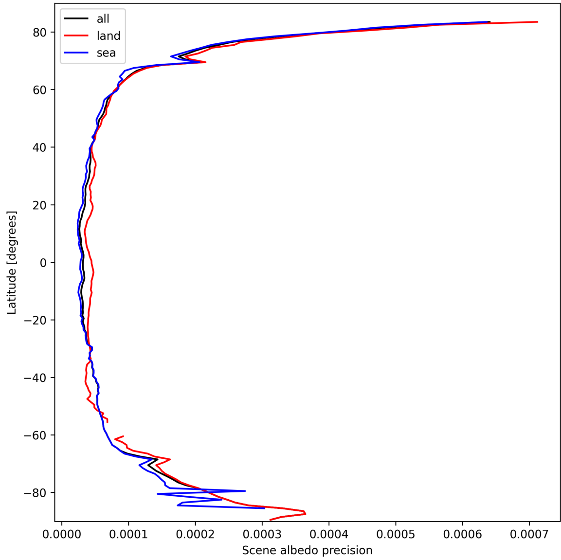
Figure 16: Zonal average of “Scene albedo precision” for 2025-03-08 to 2025-03-09.
