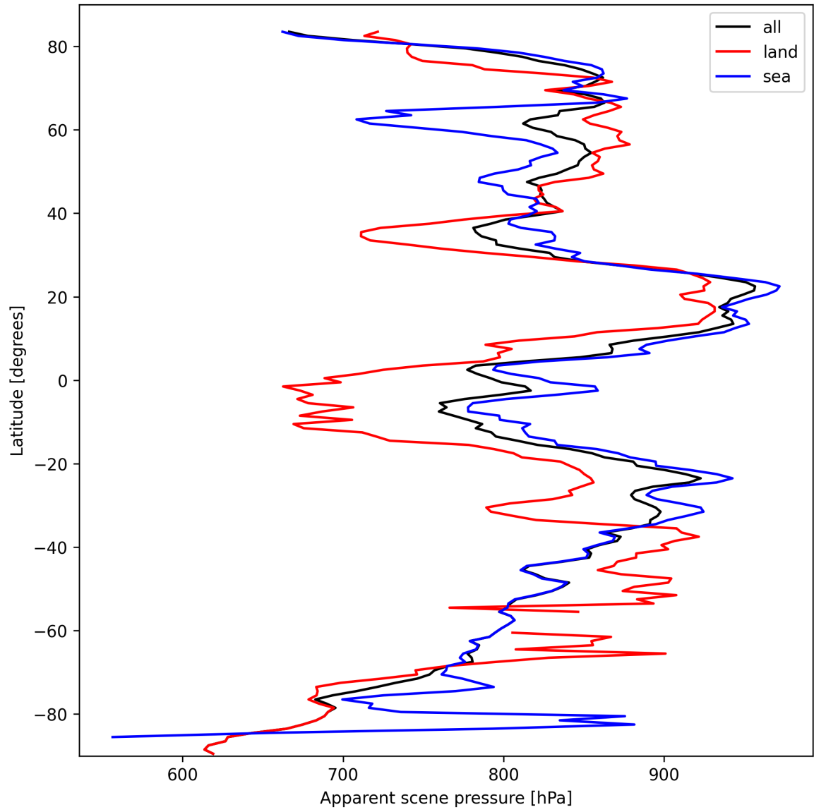
Figure 17: Zonal average of “Apparent scene pressure” for 2025-03-08 to 2025-03-09.
