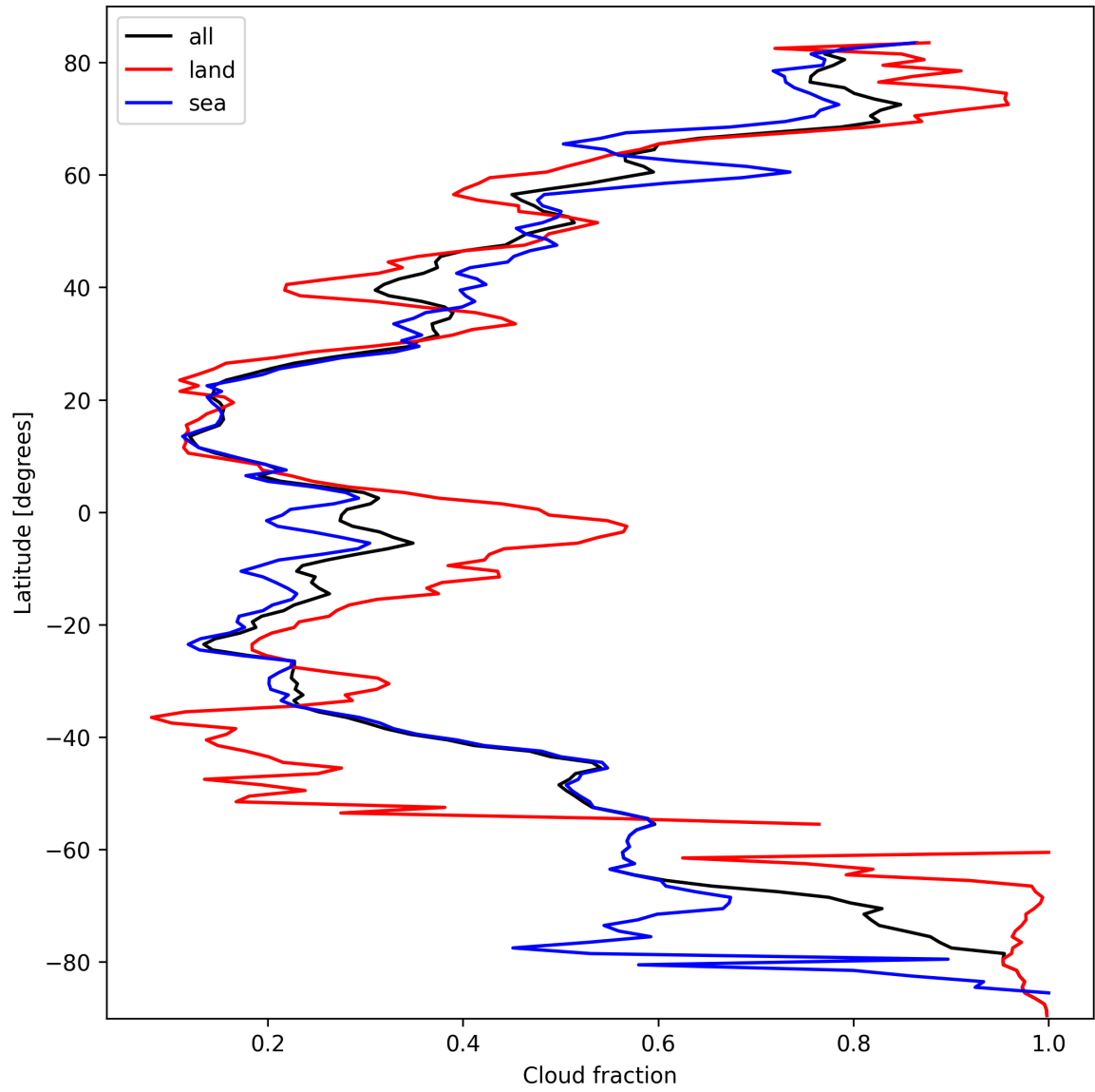
Figure 13: Zonal average of “Cloud fraction” for 2025-03-08 to 2025-03-09.
