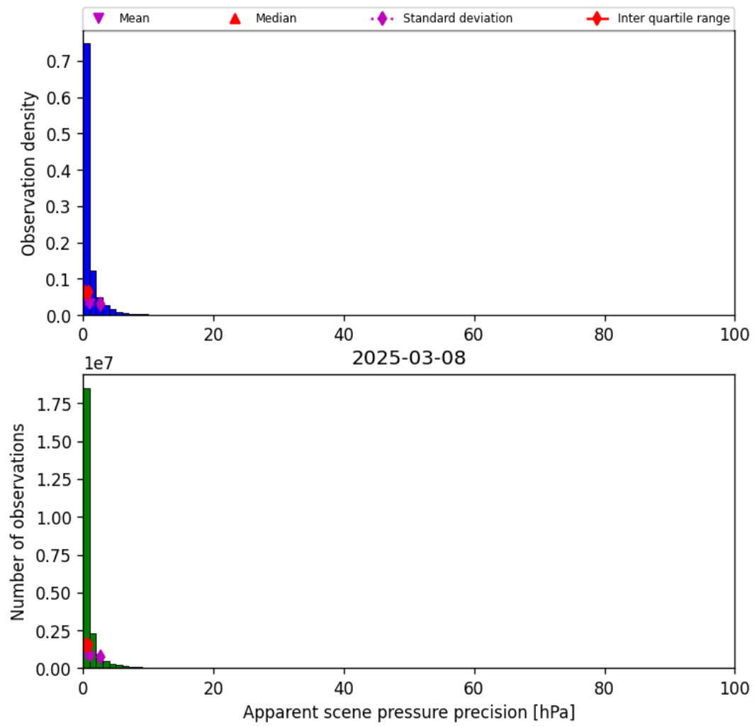
Figure 35: Histogram of “Apparent scene pressure precision” for 2025-03-08 to 2025-03-09
