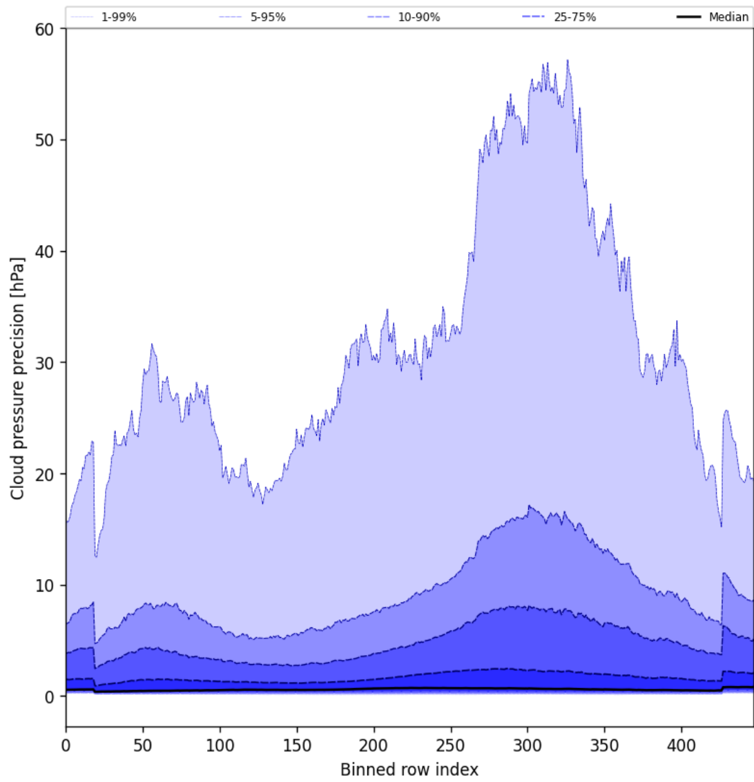
Figure 46: Along track statistics of “Cloud pressure precision” for 2025-03-08 to 2025-03-09
