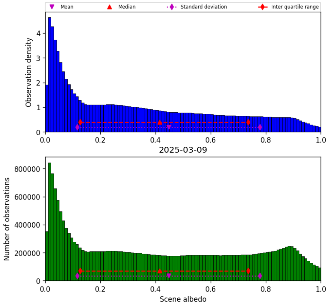
Figure 32: Histogram of “Scene albedo” for 2025-03-09 to 2025-03-10
