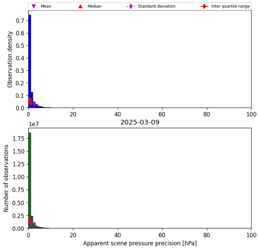
Figure 35: Histogram of “Apparent scene pressure precision” for 2025-03-09 to 2025-03-10
