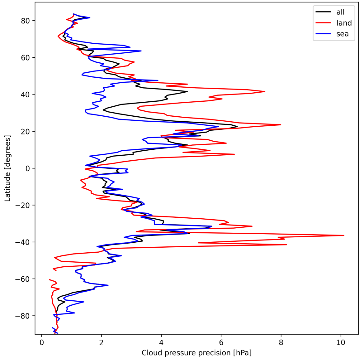
Figure 12: Zonal average of “Cloud pressure precision” for 2025-03-09 to 2025-03-10.
