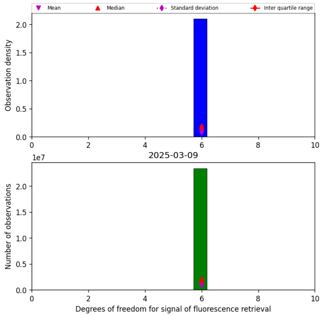
Figure 41: Histogram of “Degrees of freedom for signal of fluorescence retrieval” for 2025-03-09 to 2025-03-10
