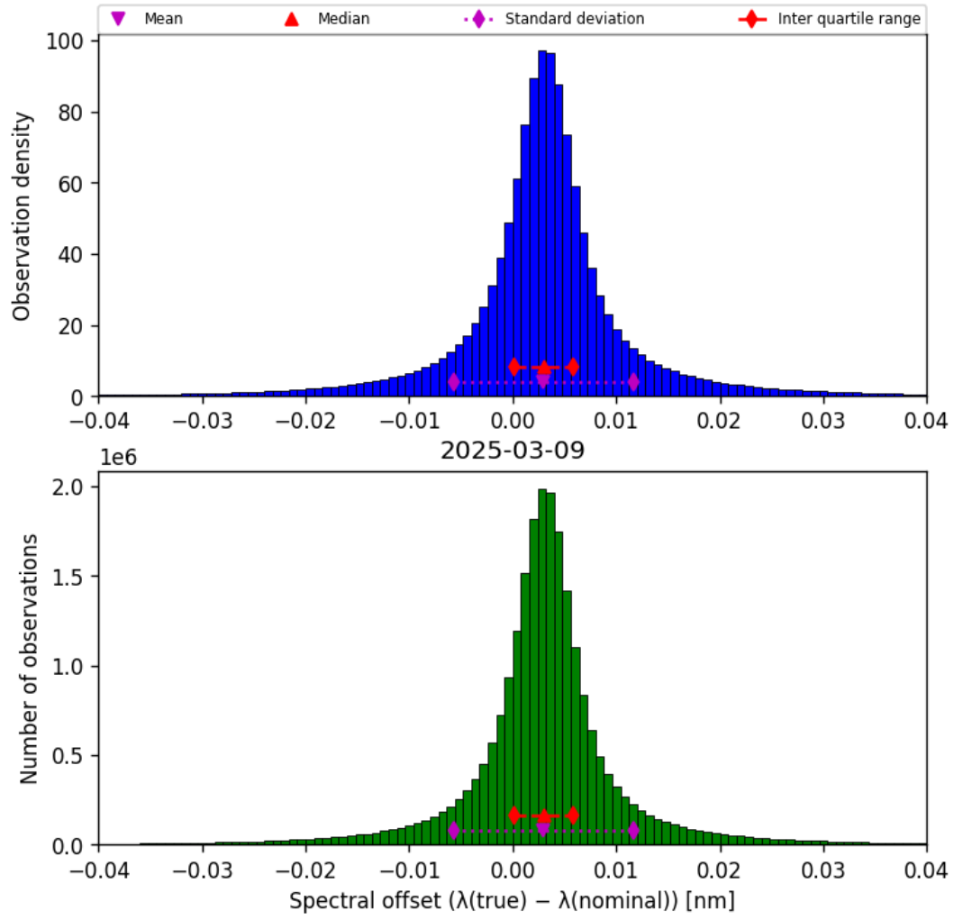
Figure 43: Histogram of “Spectral offset ( \lambda_{\text{true}} - \lambda_{\text{nominal}} )” for 2025-03-09 to 2025-03-10
