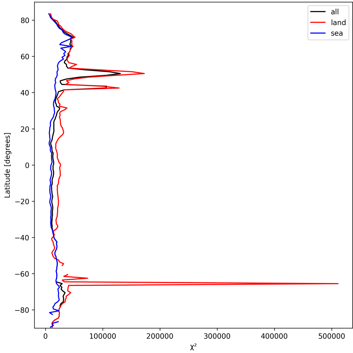
Figure 19: Zonal average of “ \chi^2 ” for 2025-03-09 to 2025-03-10.
