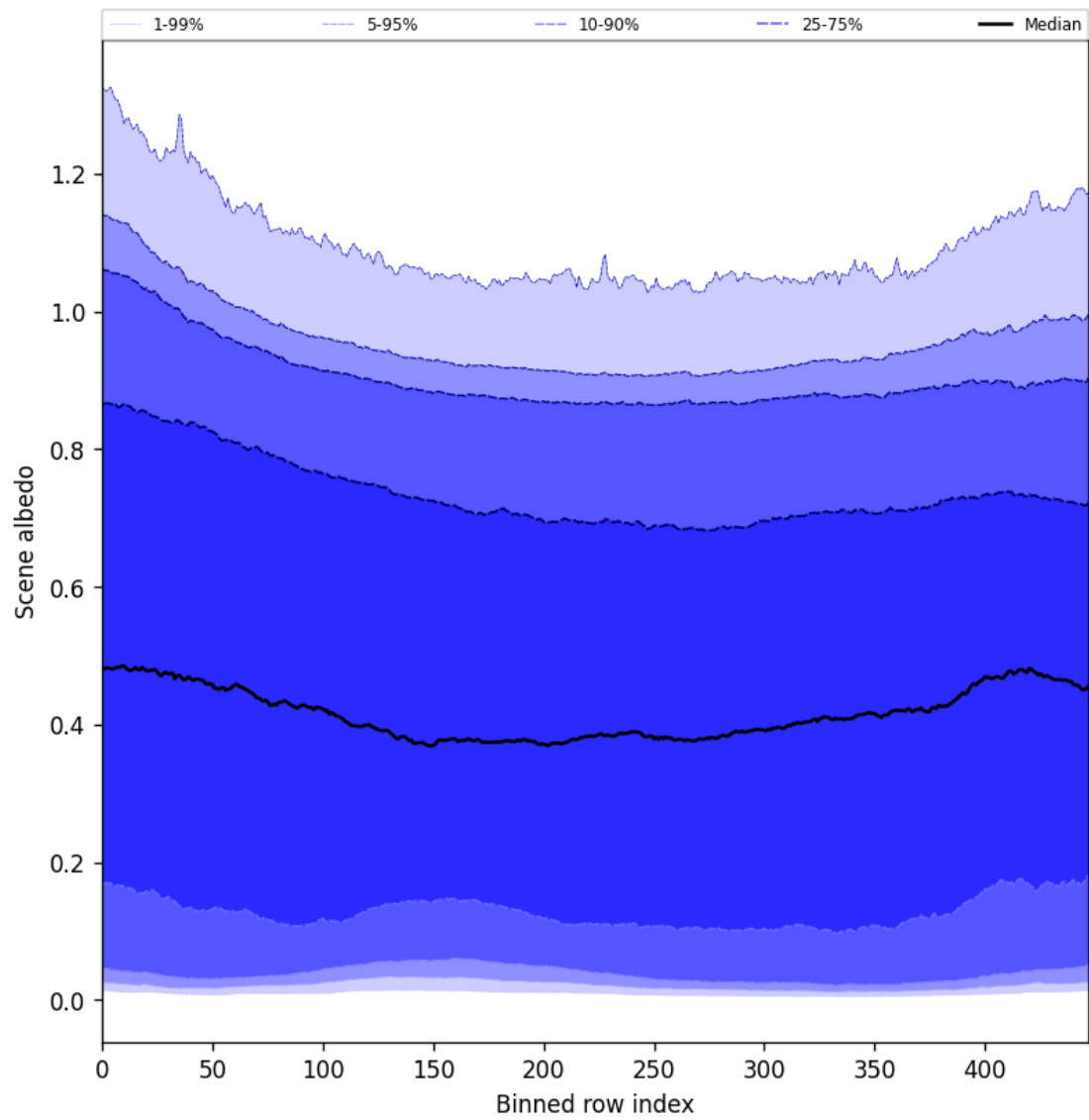
Figure 49: Along track statistics of “Scene albedo” for 2025-03-09 to 2025-03-10
