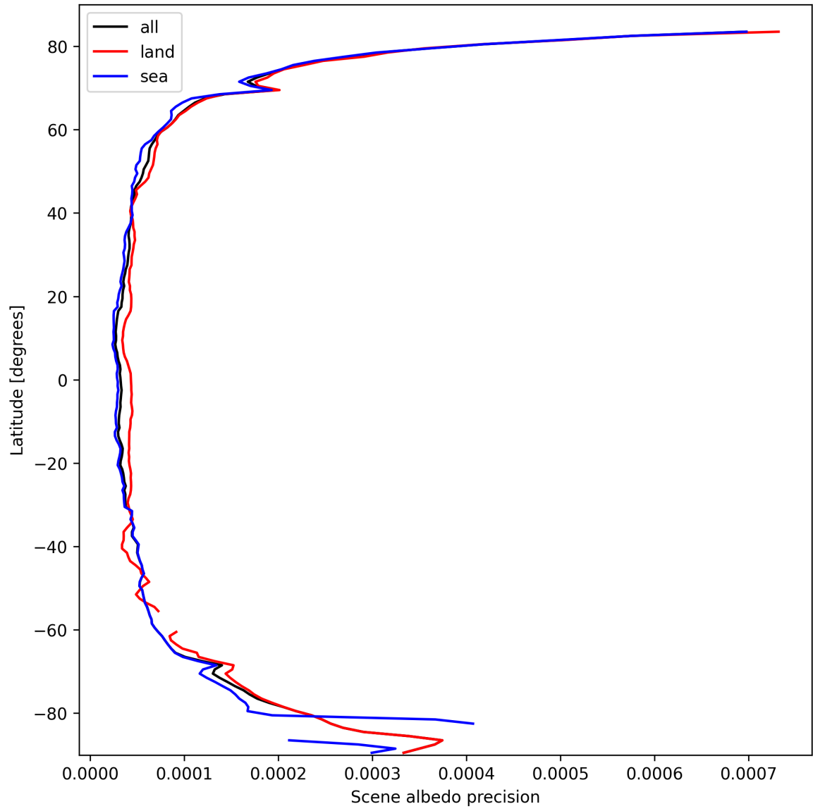
Figure 16: Zonal average of “Scene albedo precision” for 2025-03-09 to 2025-03-10.
