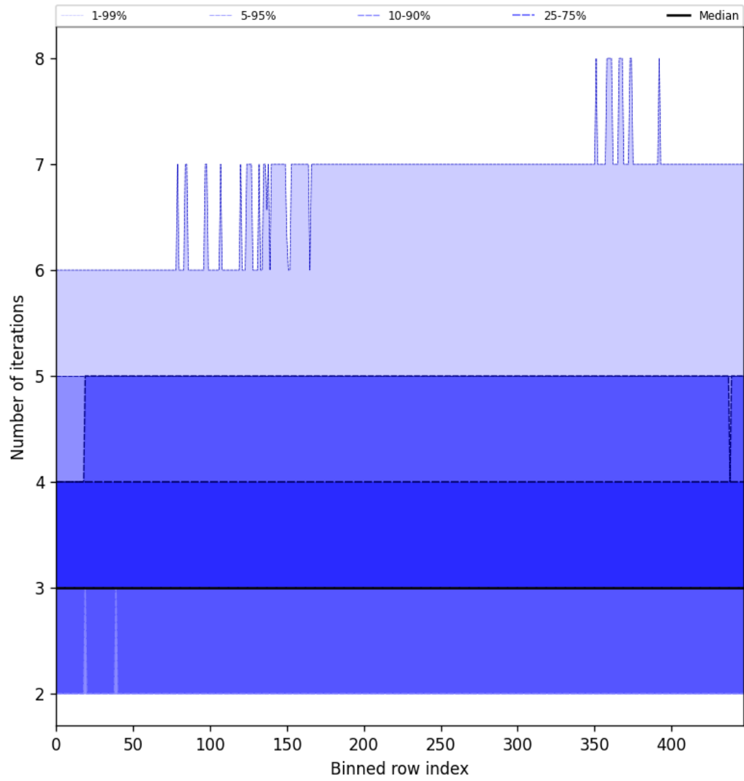
Figure 54: Along track statistics of “Number of iterations” for 2025-03-09 to 2025-03-10
