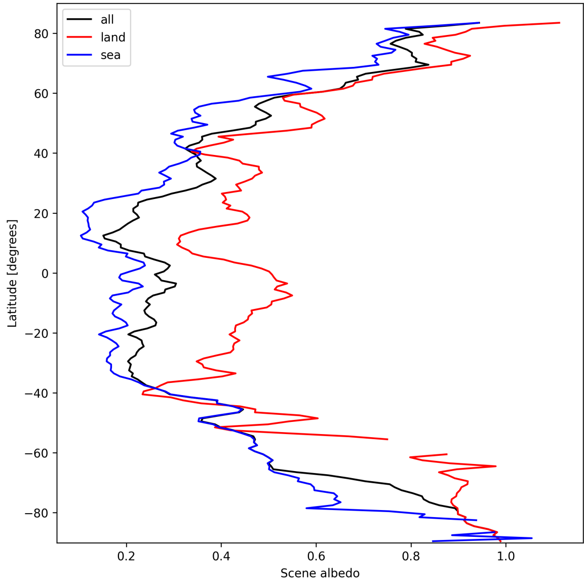
Figure 15: Zonal average of “Scene albedo” for 2025-03-09 to 2025-03-10.
