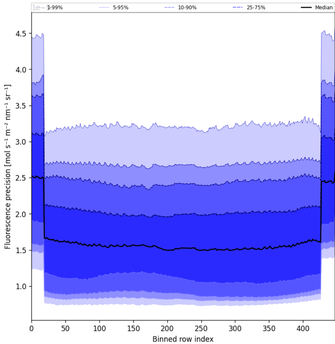
Figure 56: Along track statistics of “Fluorescence precision” for 2025-03-09 to 2025-03-10
