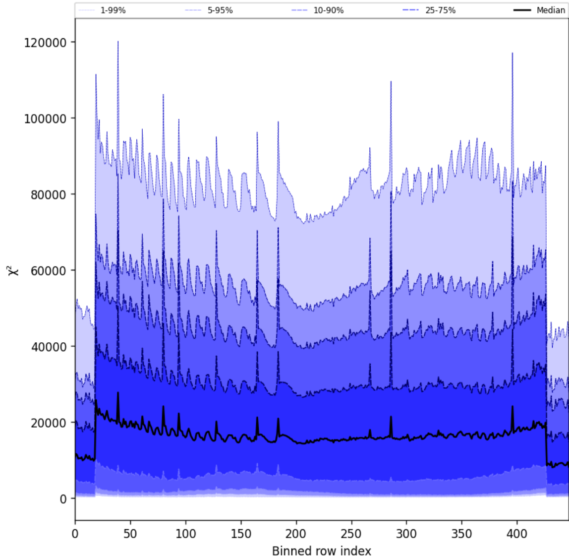
Figure 53: Along track statistics of “ \chi^2 ” for 2025-03-09 to 2025-03-10
