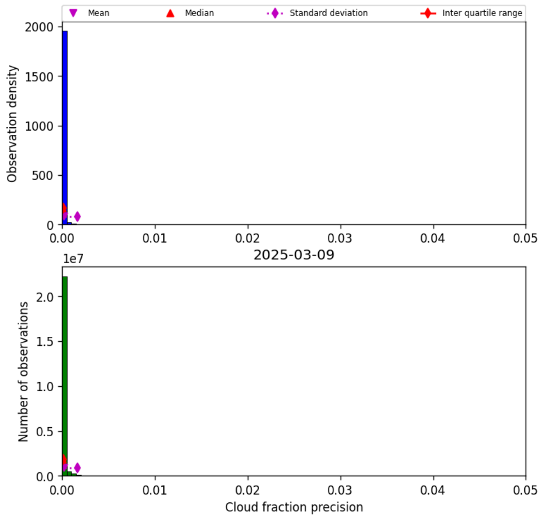
Figure 31: Histogram of “Cloud fraction precision” for 2025-03-09 to 2025-03-10
