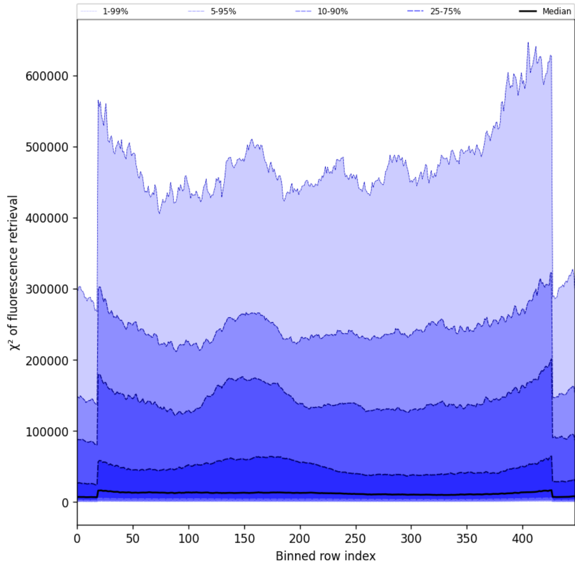
Figure 57: Along track statistics of “ \chi^2 of fluorescence retrieval” for 2025-03-09 to 2025-03-10
