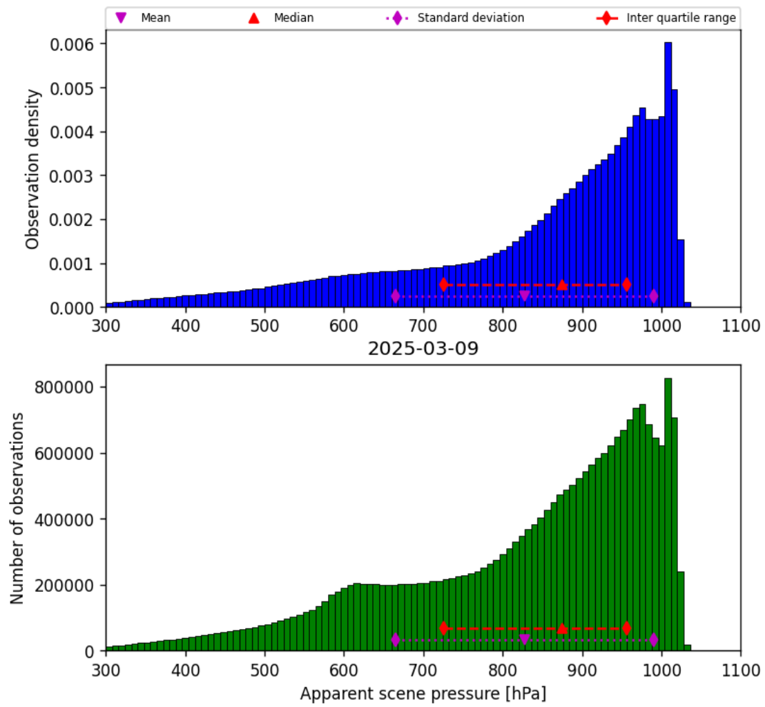
Figure 34: Histogram of “Apparent scene pressure” for 2025-03-09 to 2025-03-10
