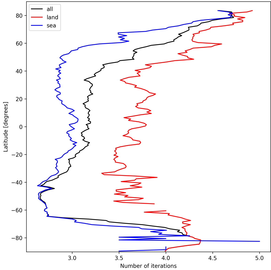
Figure 20: Zonal average of “Number of iterations” for 2025-03-09 to 2025-03-10.
