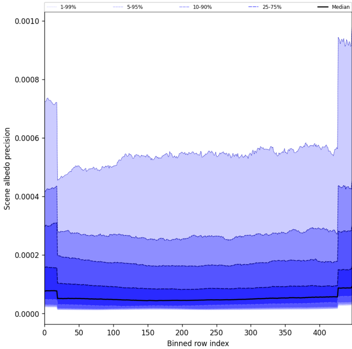
Figure 50: Along track statistics of “Scene albedo precision” for 2025-03-09 to 2025-03-10
