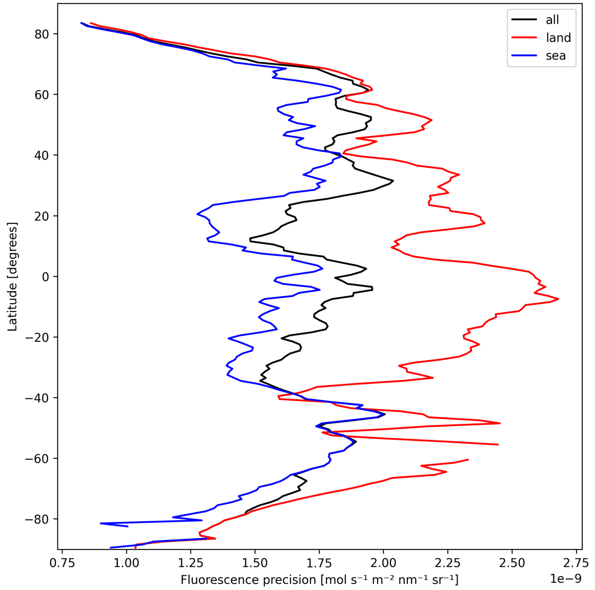
Figure 22: Zonal average of “Fluorescence precision” for 2025-03-09 to 2025-03-10.
