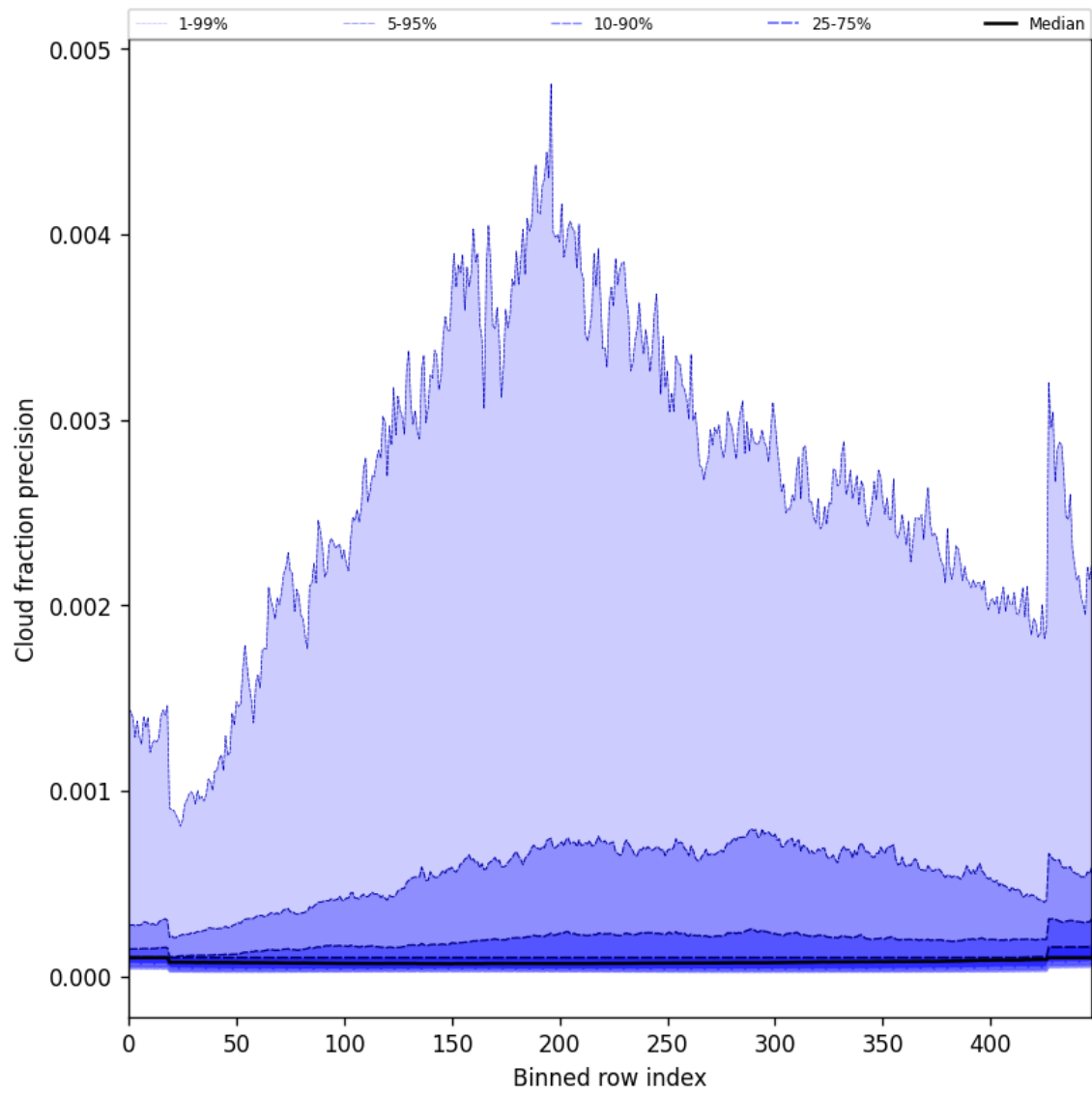
Figure 48: Along track statistics of “Cloud fraction precision” for 2025-03-09 to 2025-03-10
