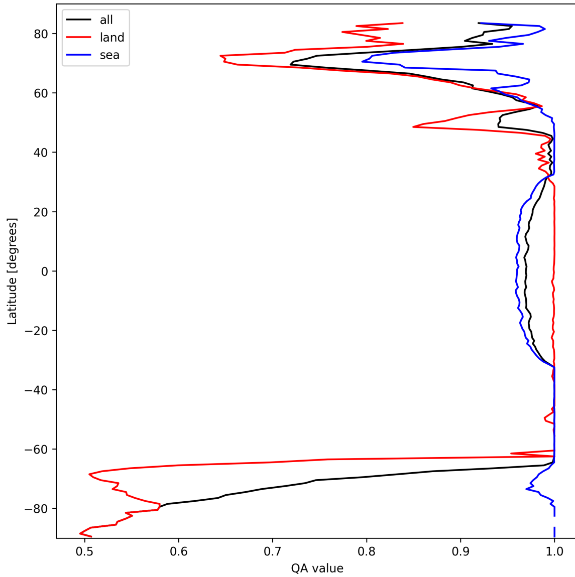
Figure 10: Zonal average of “QA value” for 2025-03-09 to 2025-03-10.
