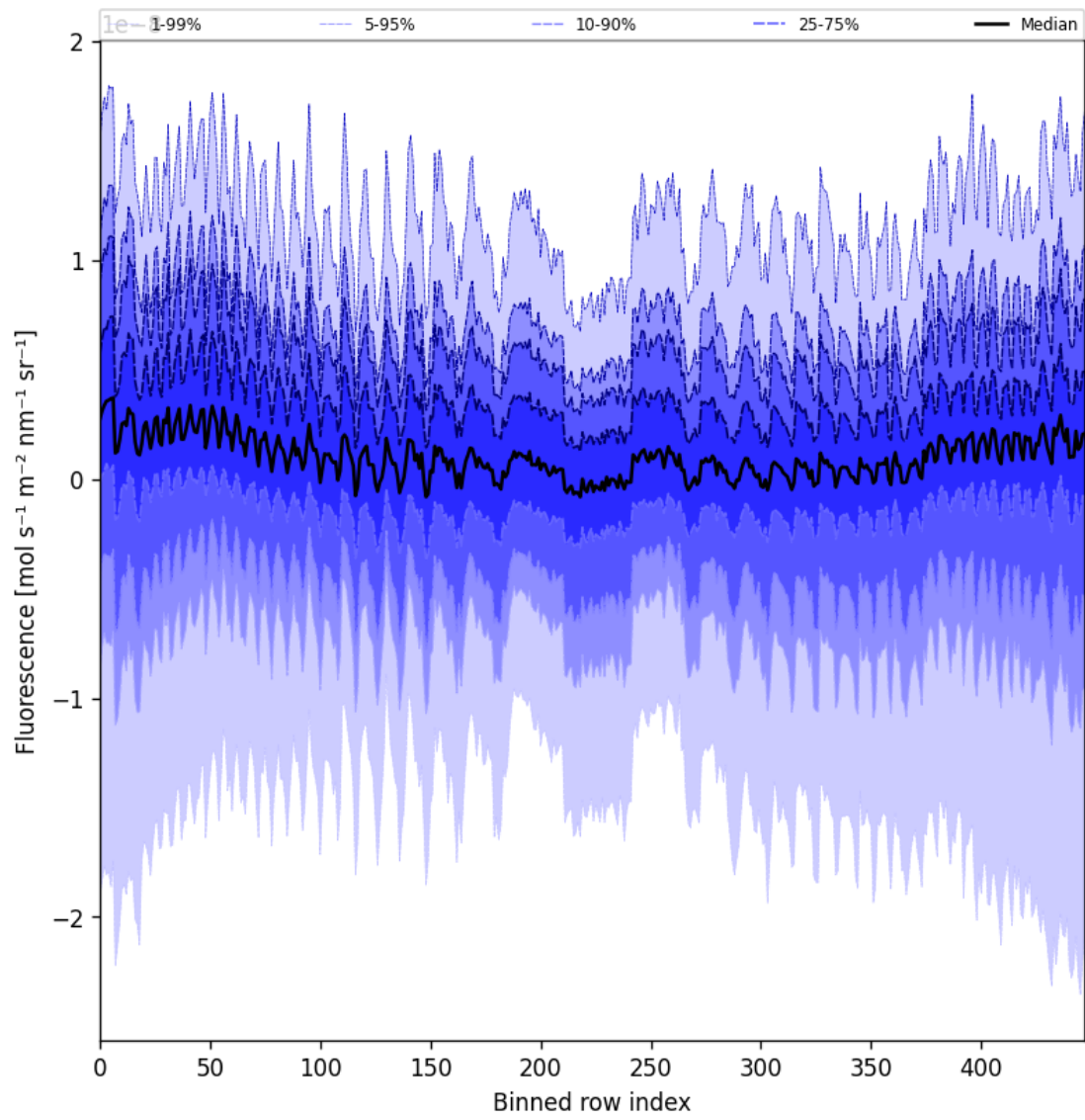
Figure 55: Along track statistics of “Fluorescence” for 2025-03-09 to 2025-03-10
