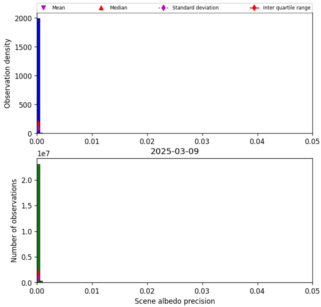
Figure 33: Histogram of “Scene albedo precision” for 2025-03-09 to 2025-03-10
