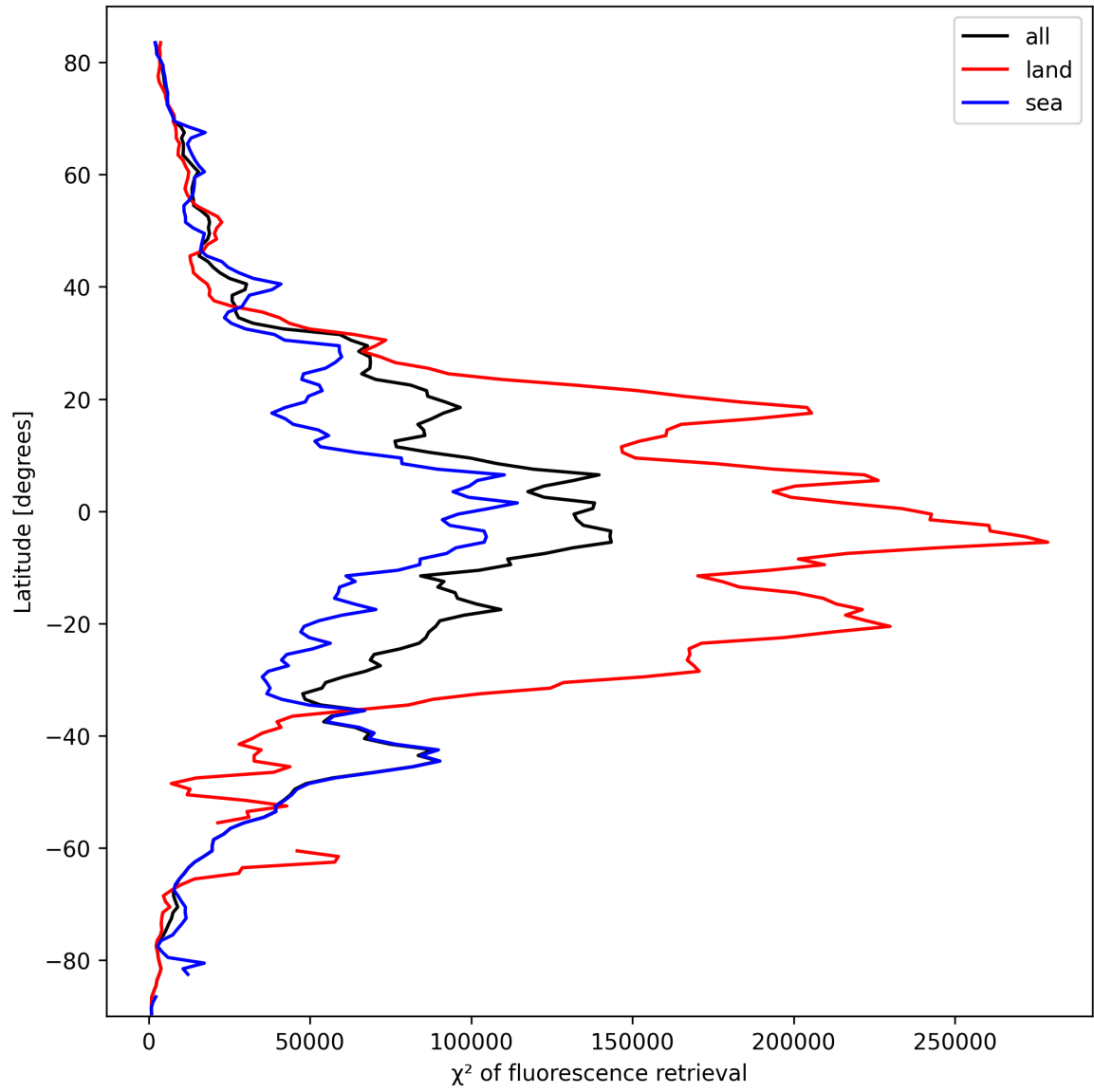
Figure 23: Zonal average of “ \chi^2 of fluorescence retrieval” for 2025-03-09 to 2025-03-10.
