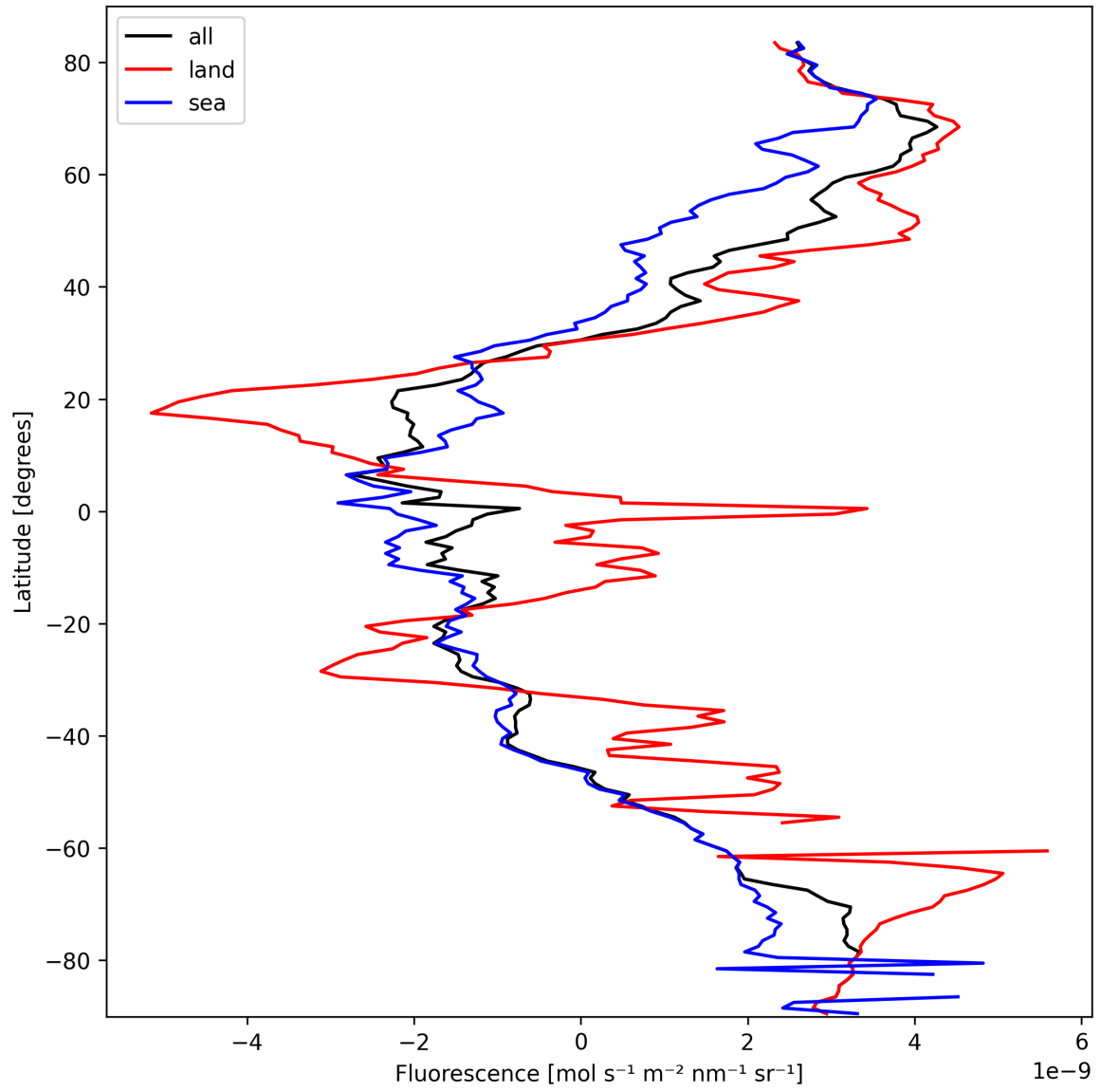
Figure 21: Zonal average of “Fluorescence” for 2025-03-09 to 2025-03-10.
