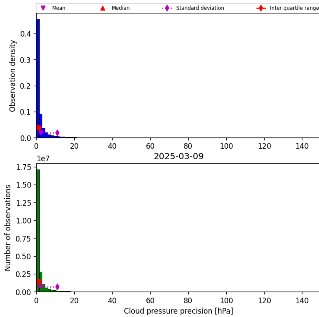
Figure 29: Histogram of “Cloud pressure precision” for 2025-03-09 to 2025-03-10
