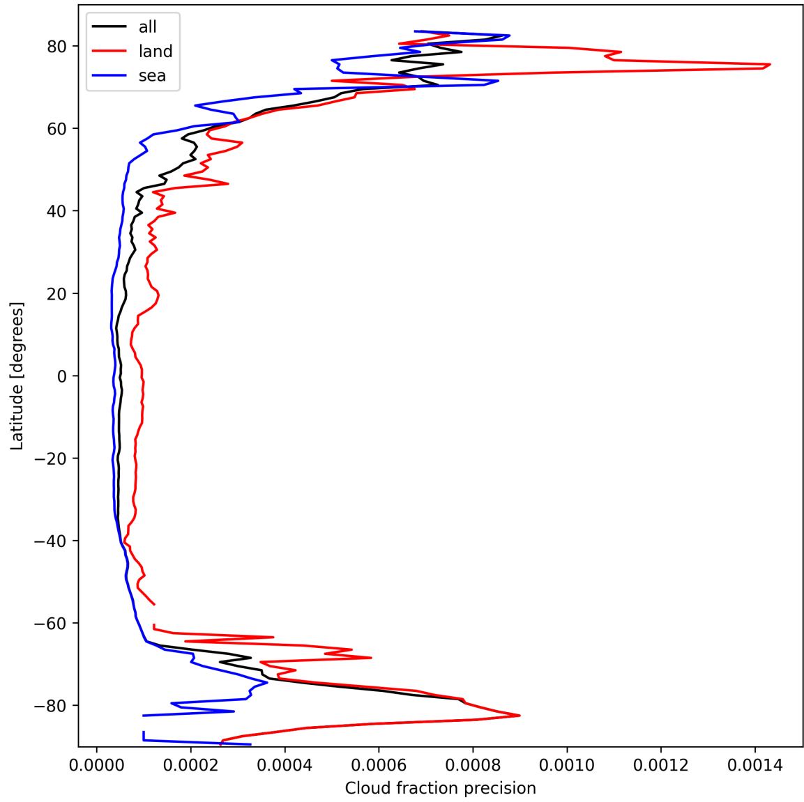
Figure 14: Zonal average of “Cloud fraction precision” for 2025-03-09 to 2025-03-10.
