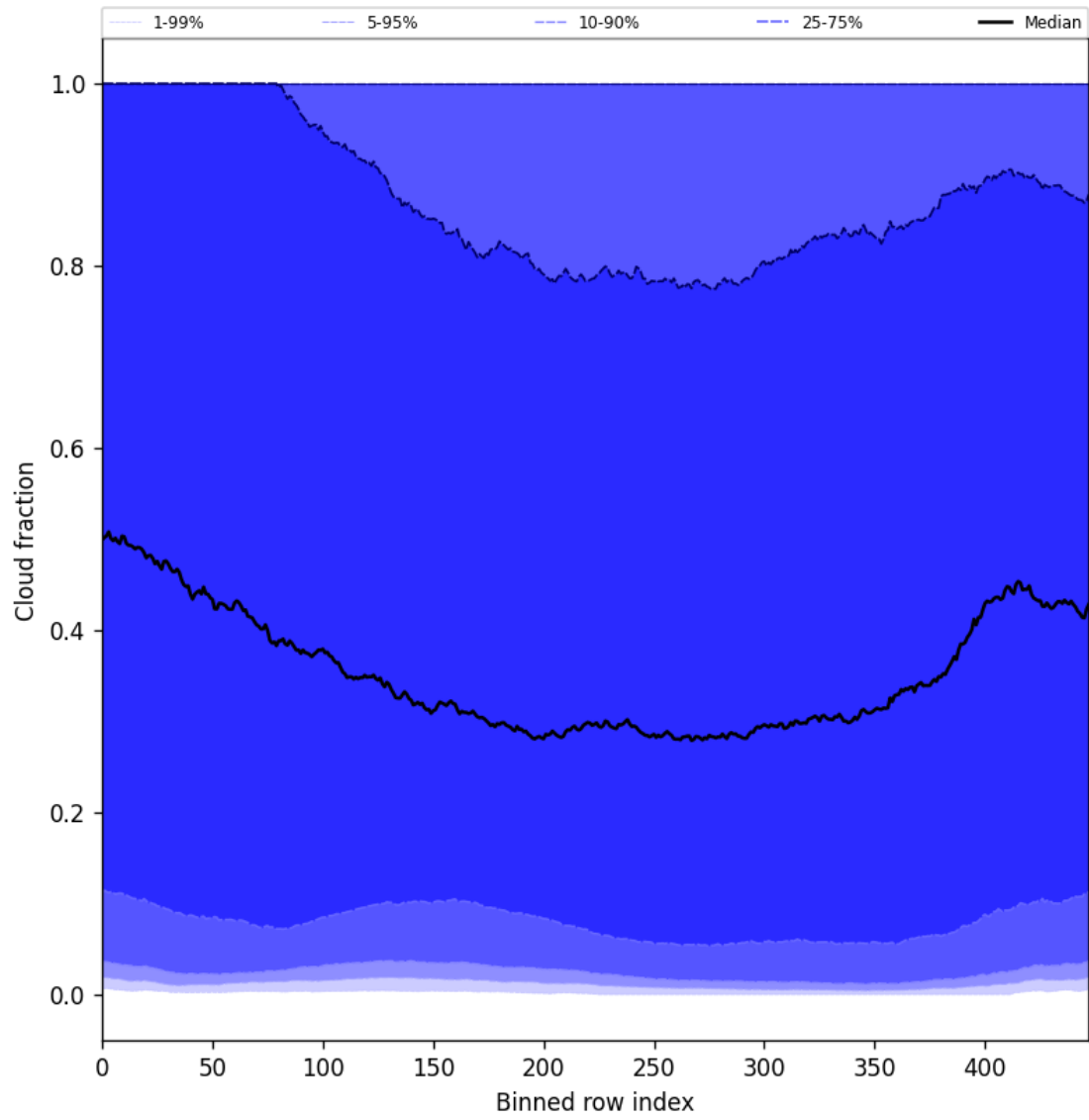
Figure 47: Along track statistics of “Cloud fraction” for 2025-03-09 to 2025-03-10
