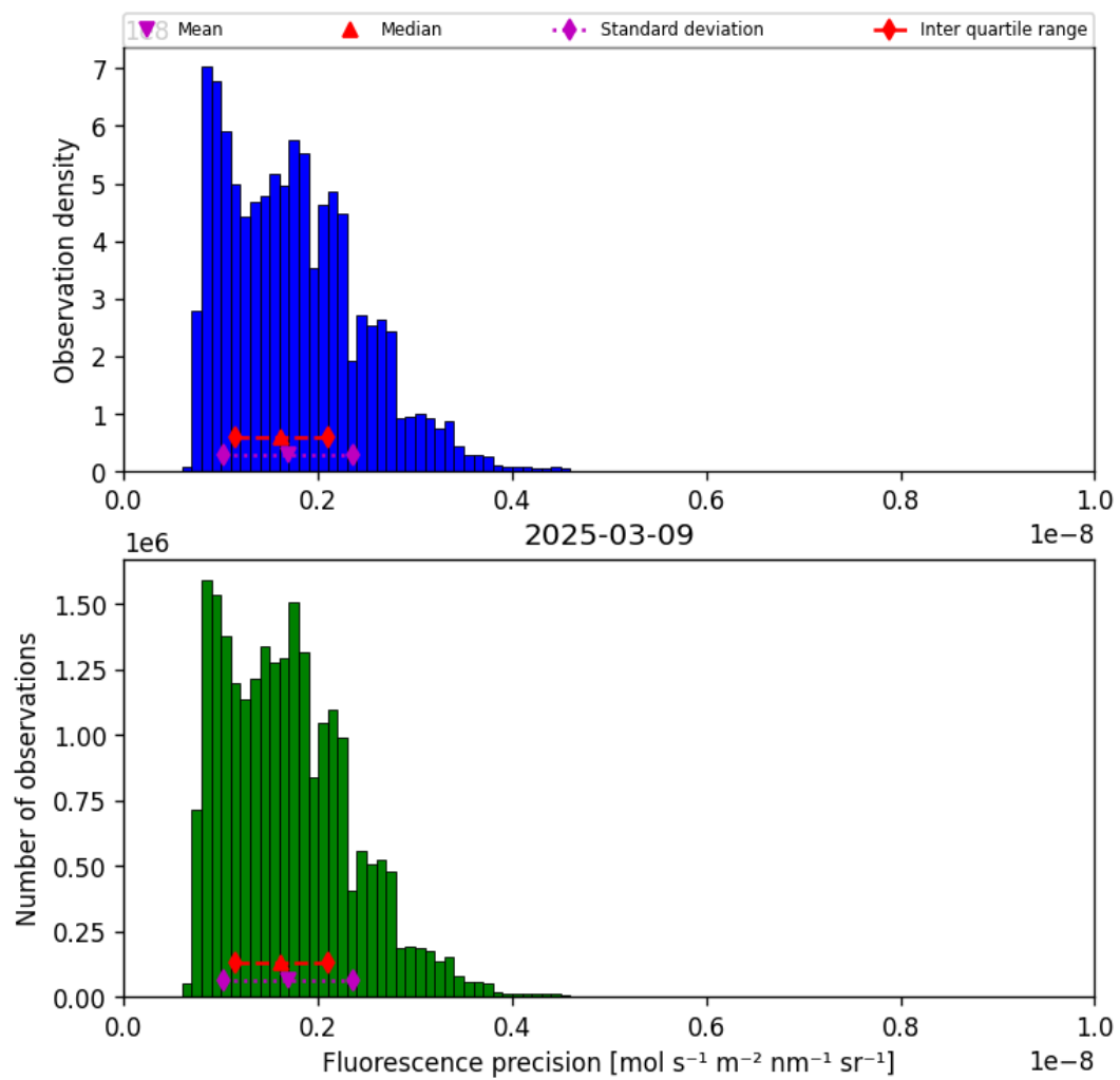
Figure 39: Histogram of “Fluorescence precision” for 2025-03-09 to 2025-03-10
