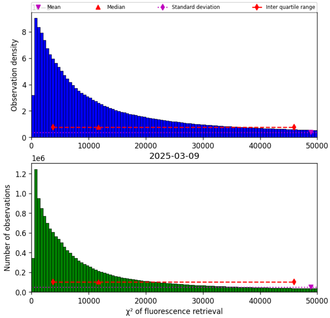
Figure 40: Histogram of “ \chi^2 of fluorescence retrieval” for 2025-03-09 to 2025-03-10
