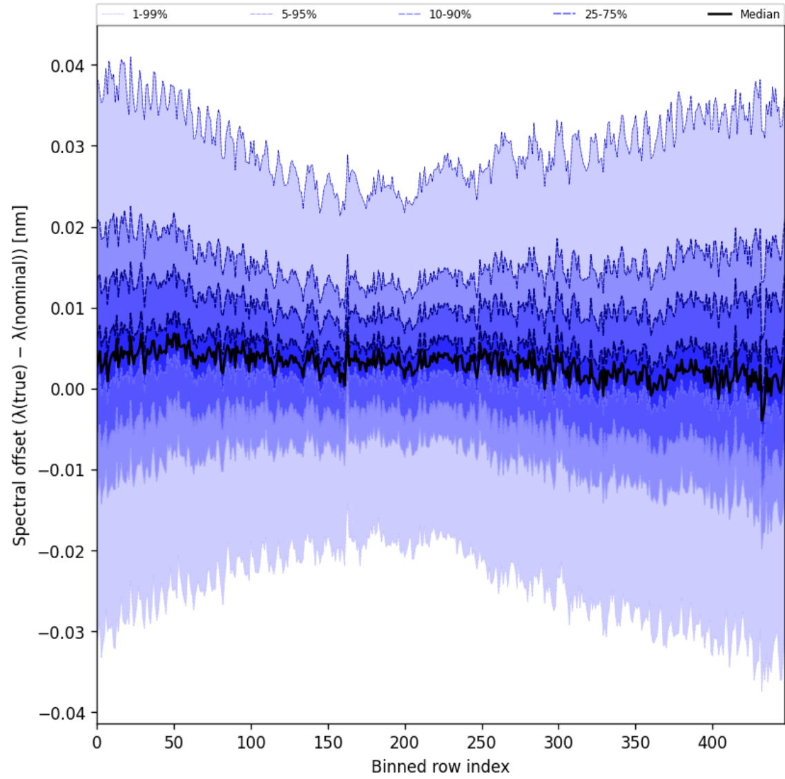
Figure 60: Along track statistics of “Spectral offset ( \lambda_{\text{true}} - \lambda_{\text{nominal}} )” for 2025-03-09 to 2025-03-10
