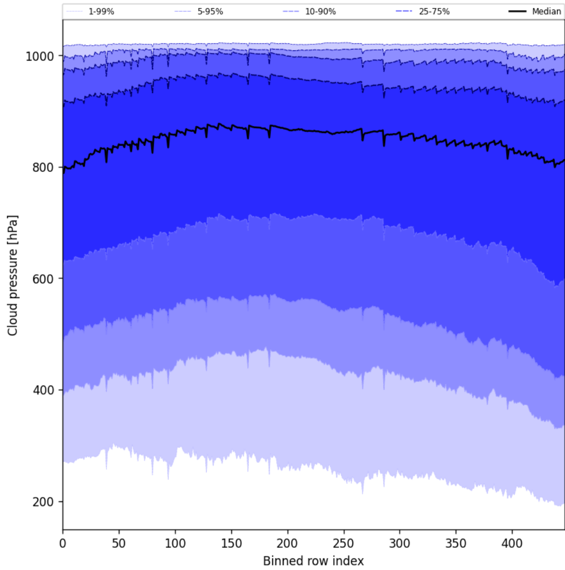
Figure 45: Along track statistics of “Cloud pressure” for 2025-03-09 to 2025-03-10
