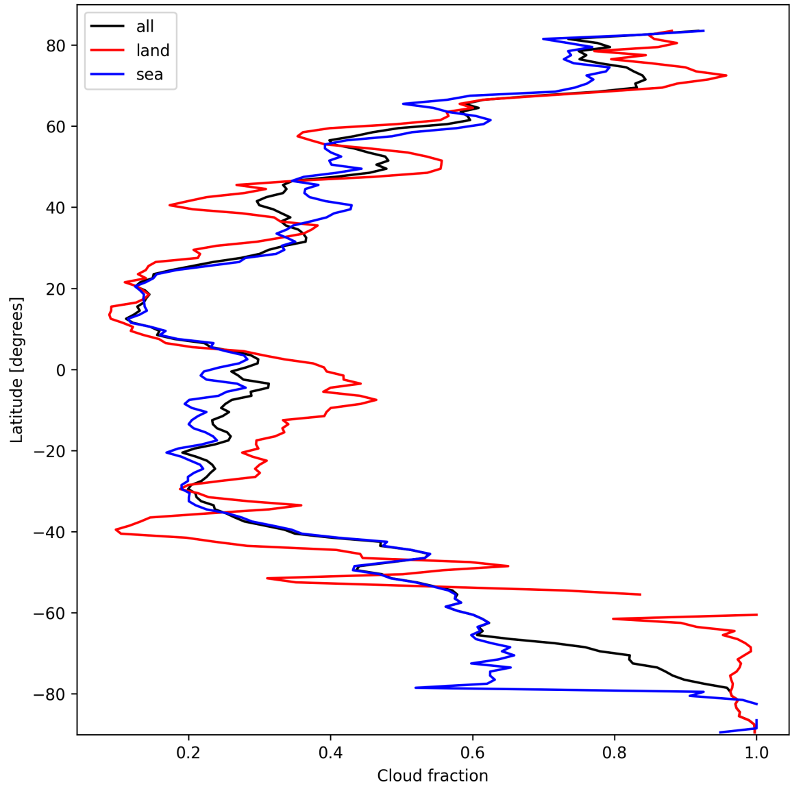
Figure 13: Zonal average of “Cloud fraction” for 2025-03-09 to 2025-03-10.
