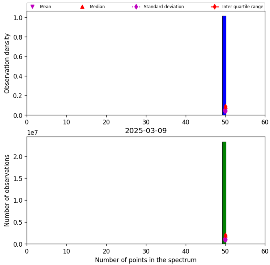
Figure 42: Histogram of “Number of points in the spectrum” for 2025-03-09 to 2025-03-10
