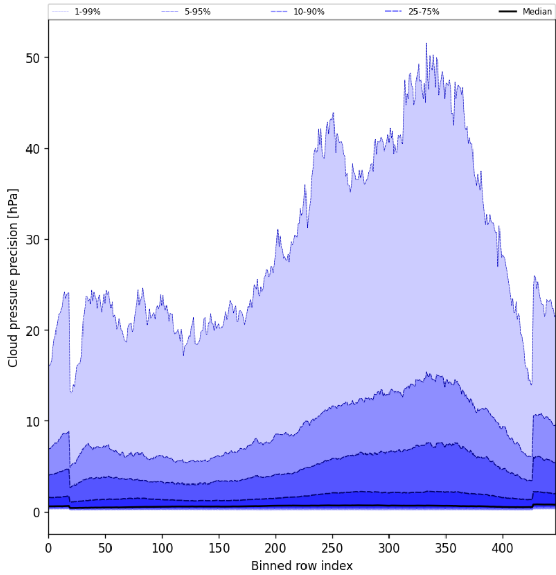
Figure 46: Along track statistics of “Cloud pressure precision” for 2025-03-09 to 2025-03-10
