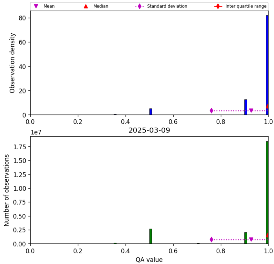
Figure 27: Histogram of “QA value” for 2025-03-09 to 2025-03-10
