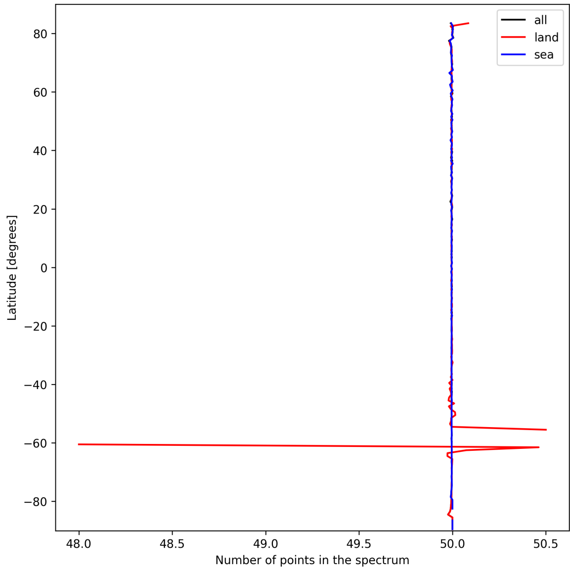
Figure 25: Zonal average of “Number of points in the spectrum” for 2025-03-09 to 2025-03-10.
