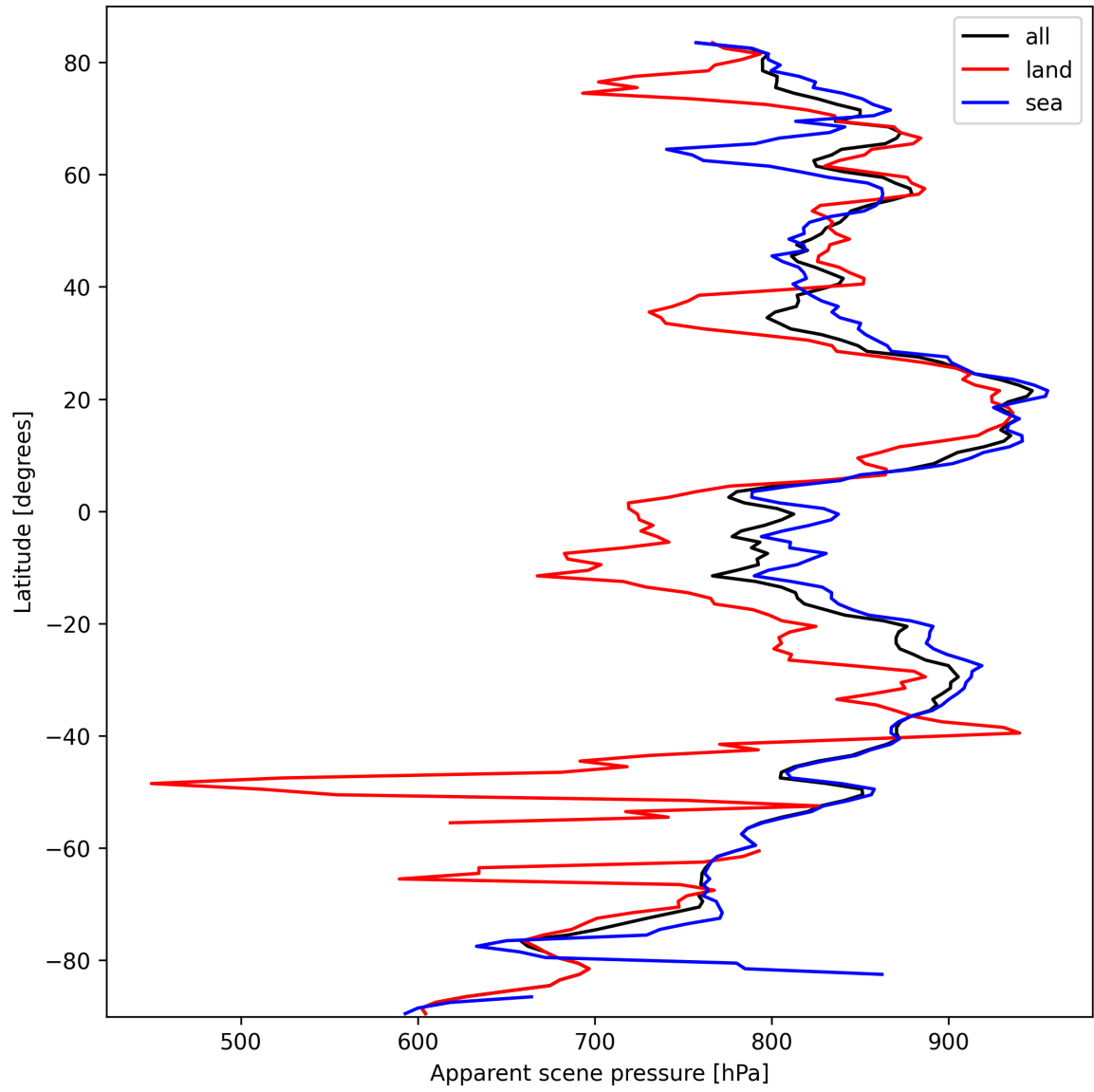
Figure 17: Zonal average of “Apparent scene pressure” for 2025-03-09 to 2025-03-10.
