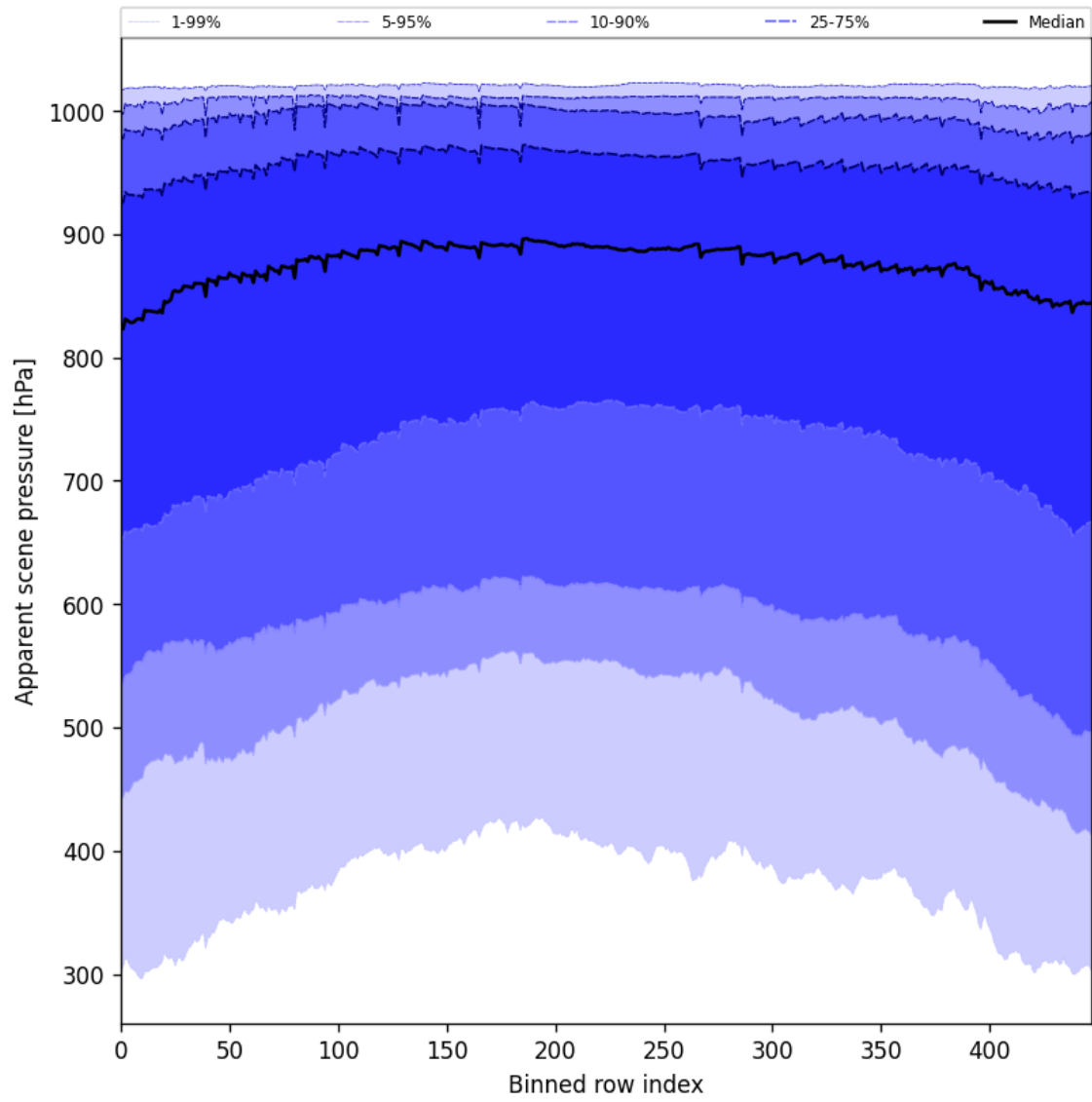
Figure 51: Along track statistics of “Apparent scene pressure” for 2025-03-09 to 2025-03-10
