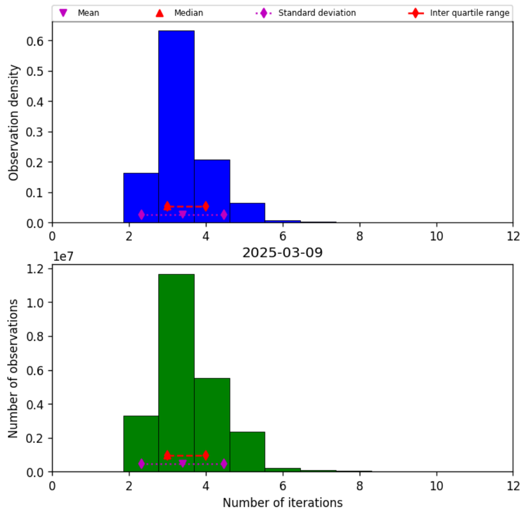
Figure 37: Histogram of “Number of iterations” for 2025-03-09 to 2025-03-10
