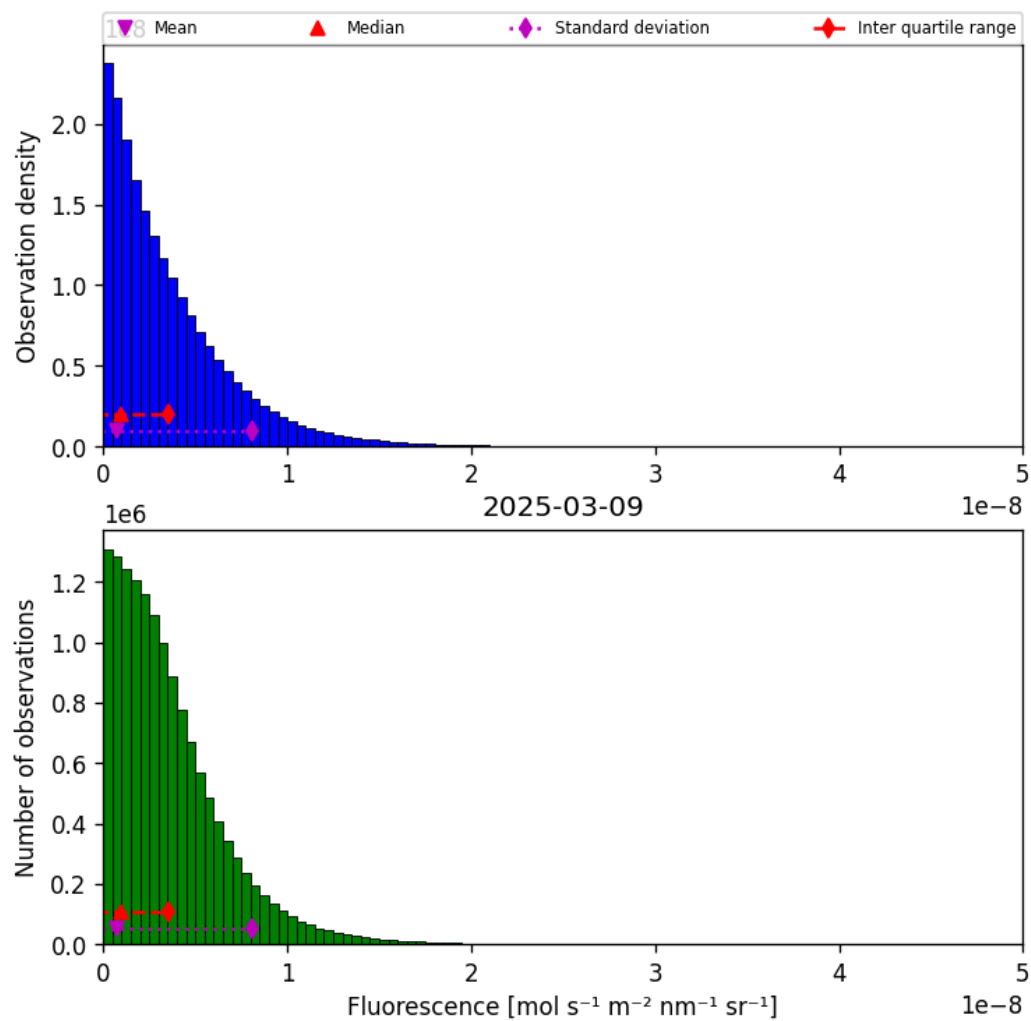
Figure 38: Histogram of “Fluorescence” for 2025-03-09 to 2025-03-10
