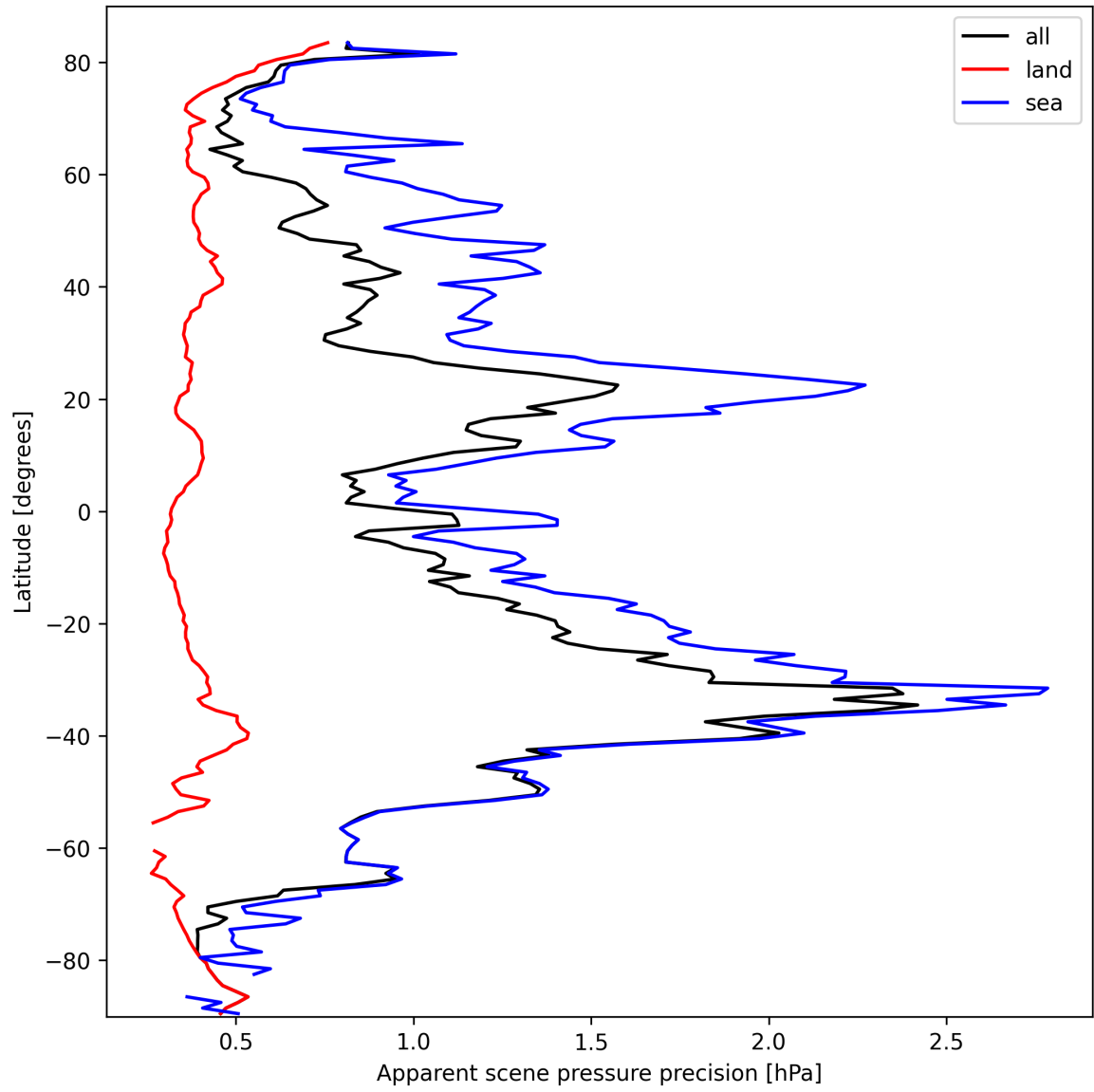
Figure 18: Zonal average of “Apparent scene pressure precision” for 2025-03-09 to 2025-03-10.
