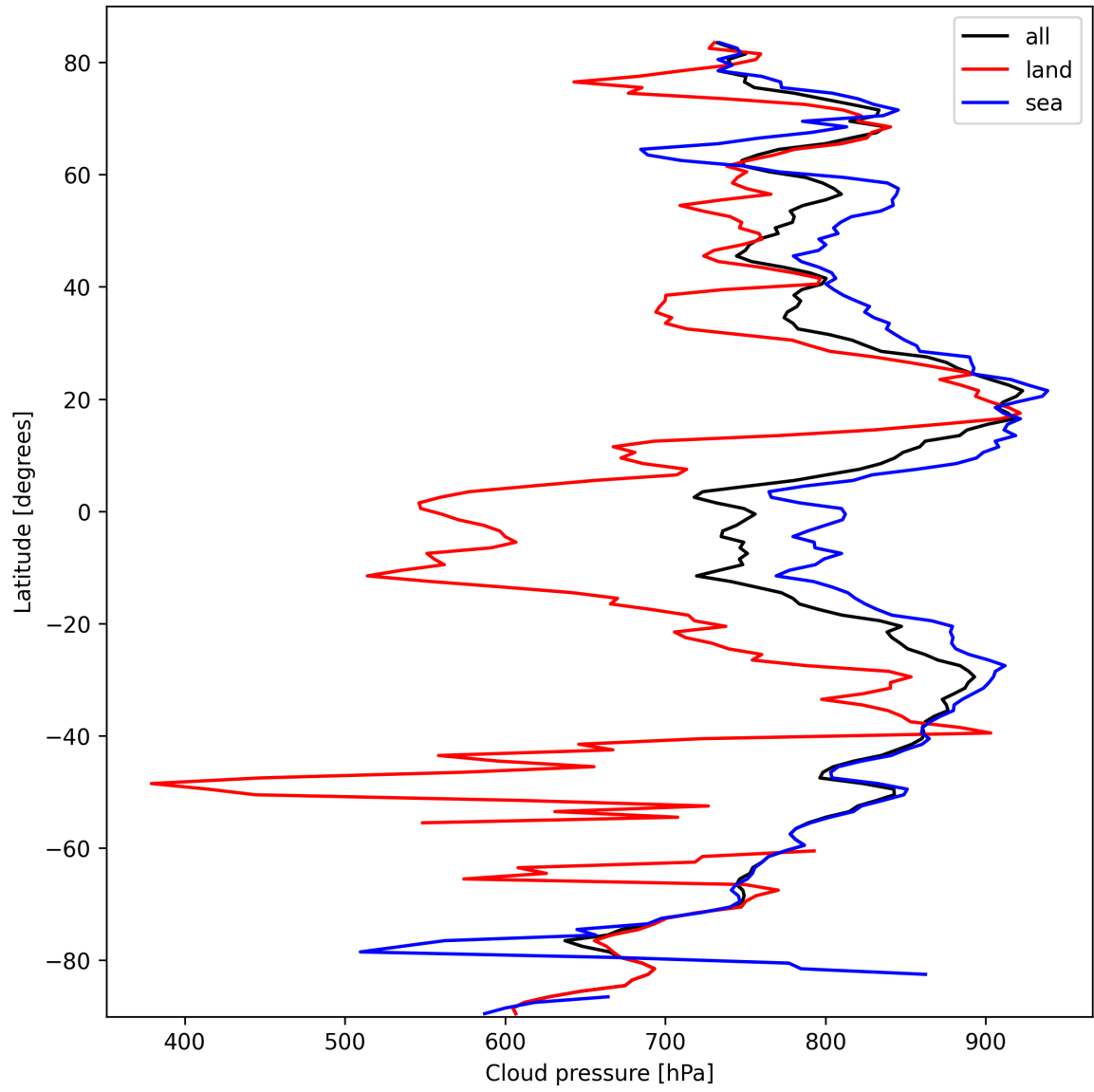
Figure 11: Zonal average of “Cloud pressure” for 2025-03-09 to 2025-03-10.
