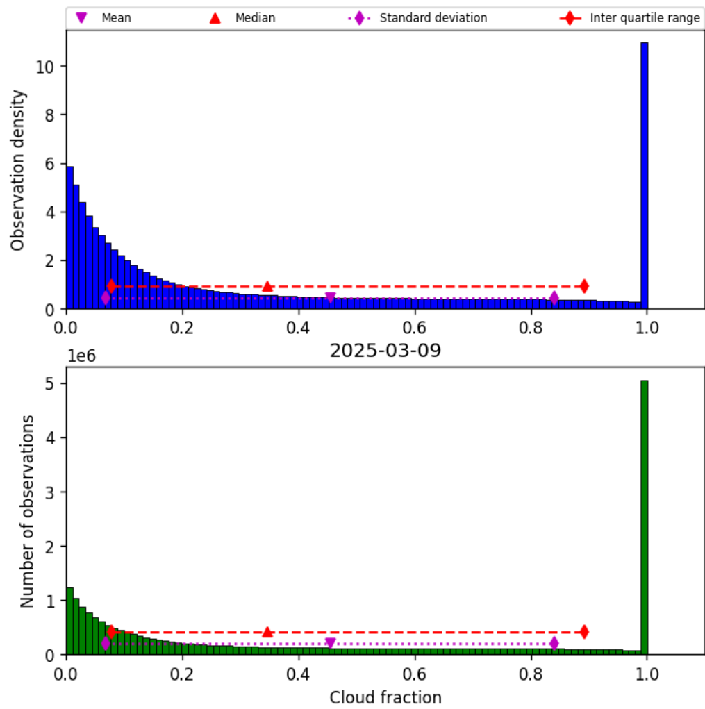
Figure 30: Histogram of “Cloud fraction” for 2025-03-09 to 2025-03-10
