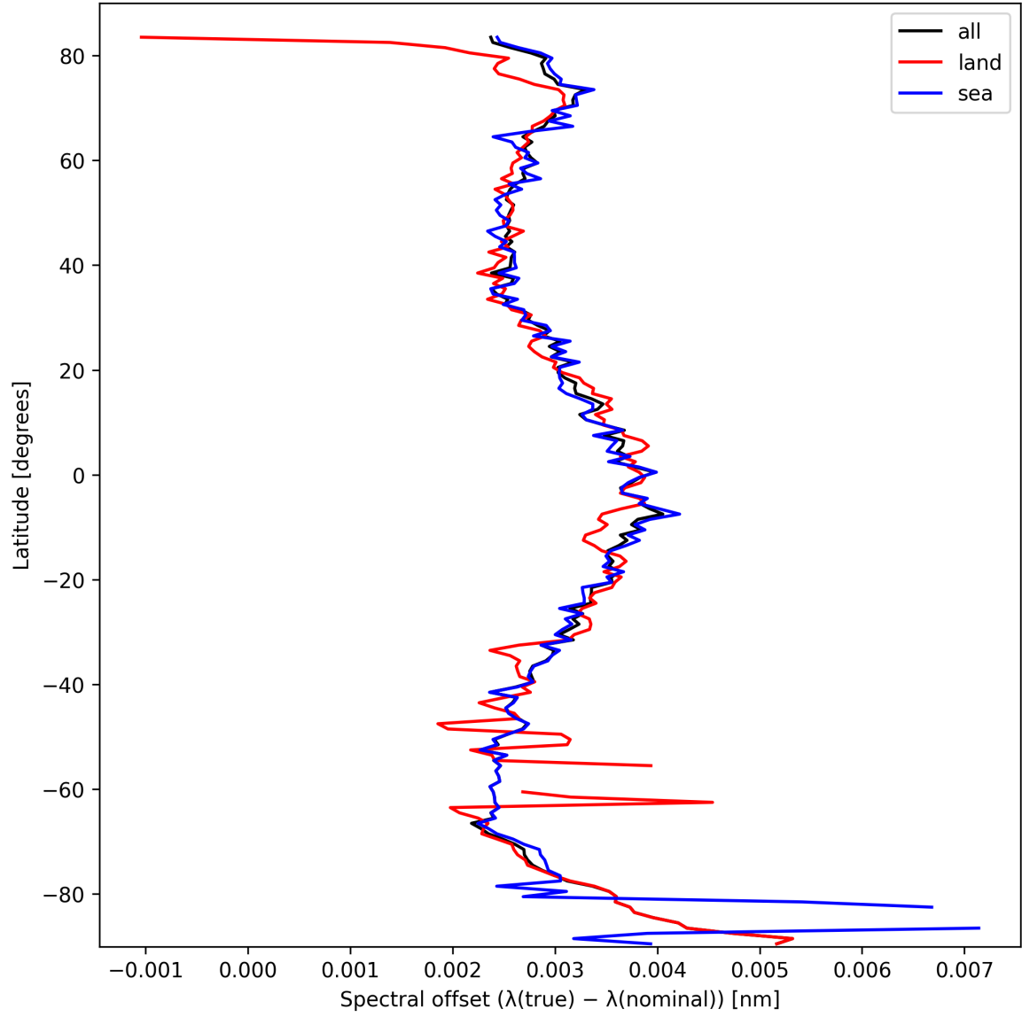
Figure 26: Zonal average of “Spectral offset ( \lambda_{\text{true}} - \lambda_{\text{nominal}} )” for 2025-03-09 to 2025-03-10.
