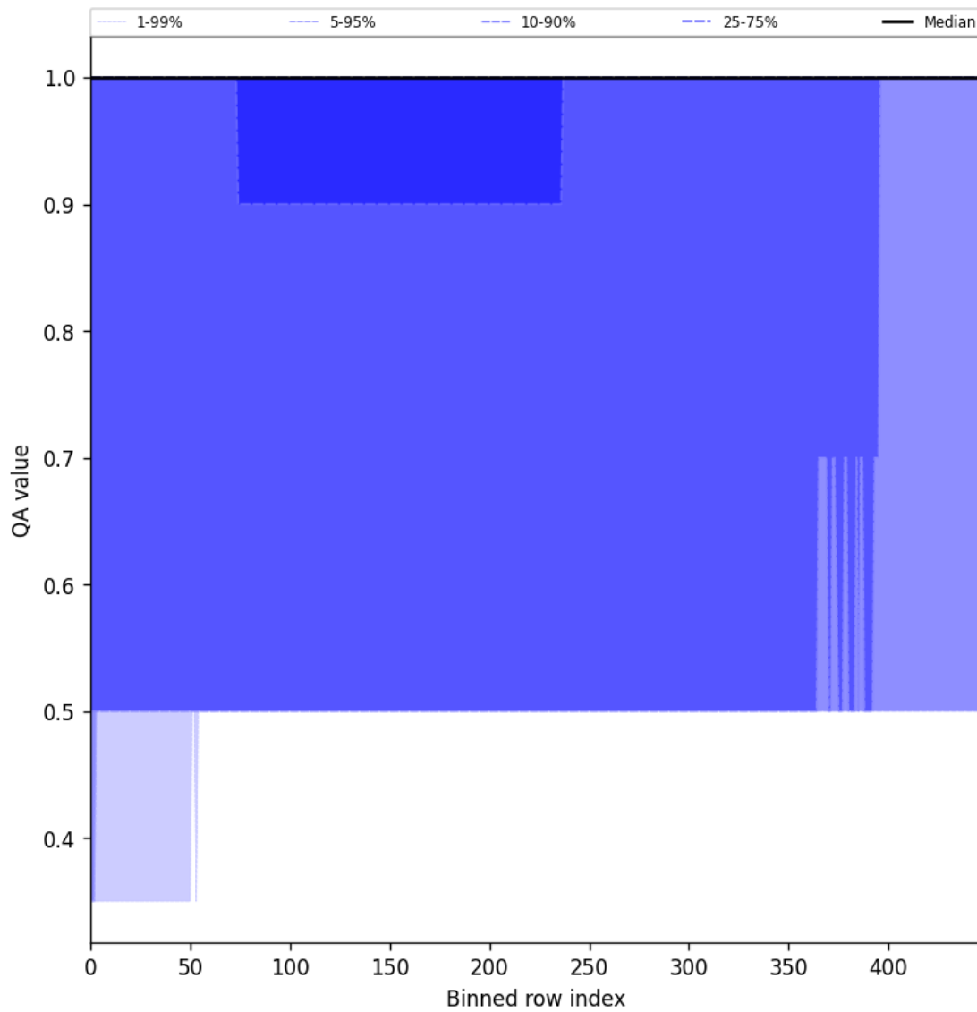
Figure 44: Along track statistics of “QA value” for 2025-03-09 to 2025-03-10
