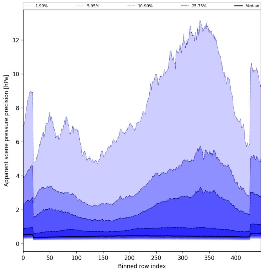
Figure 52: Along track statistics of “Apparent scene pressure precision” for 2025-03-09 to 2025-03-10
