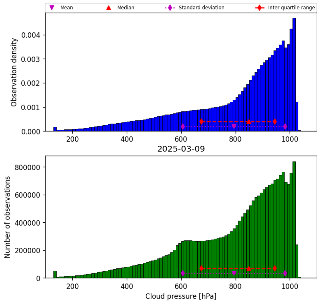
Figure 28: Histogram of “Cloud pressure” for 2025-03-09 to 2025-03-10
