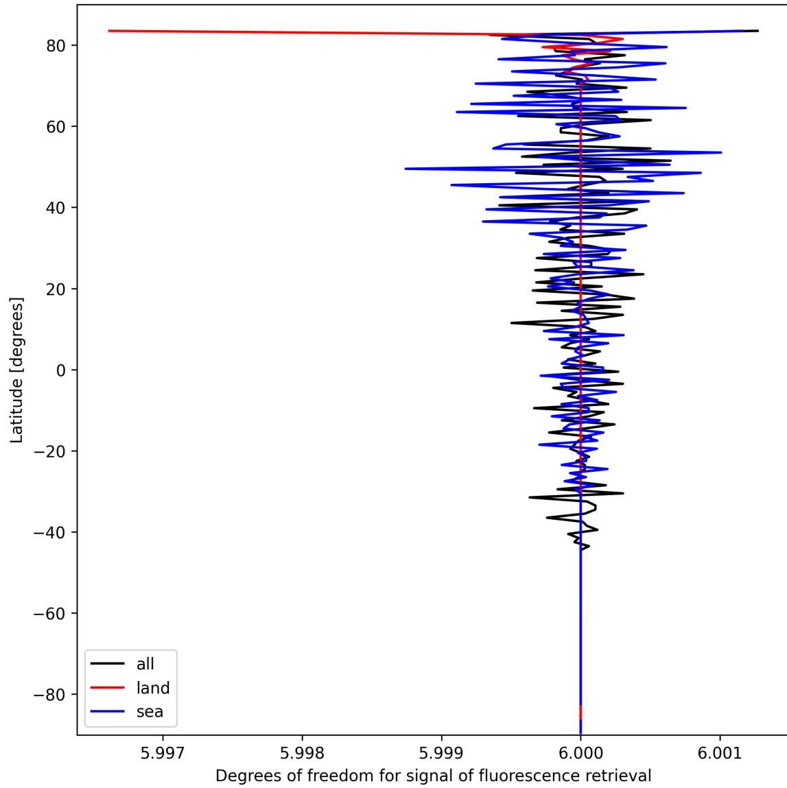
Figure 24: Zonal average of “Degrees of freedom for signal of fluorescence retrieval” for 2025-03-09 to 2025-03-10.
