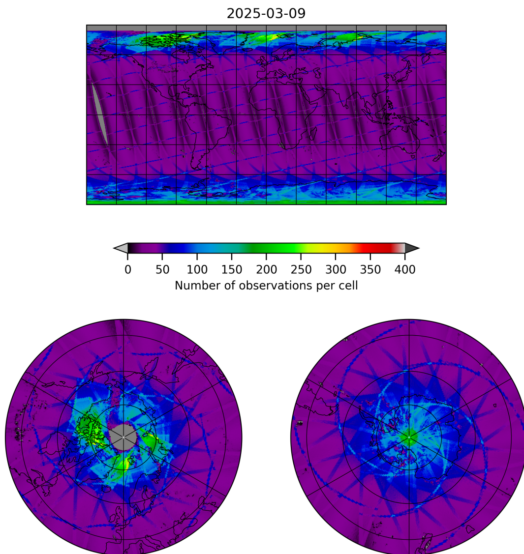
Figure 9: Map of the number of observations for 2025-03-09 to 2025-03-10
