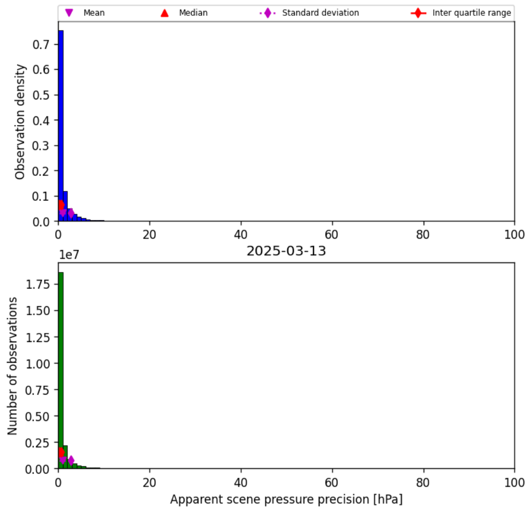
Figure 35: Histogram of “Apparent scene pressure precision” for 2025-03-13 to 2025-03-14
