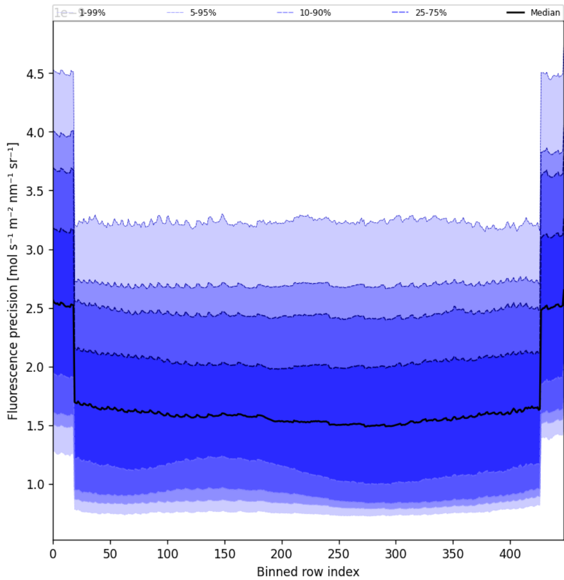
Figure 56: Along track statistics of “Fluorescence precision” for 2025-03-13 to 2025-03-14
