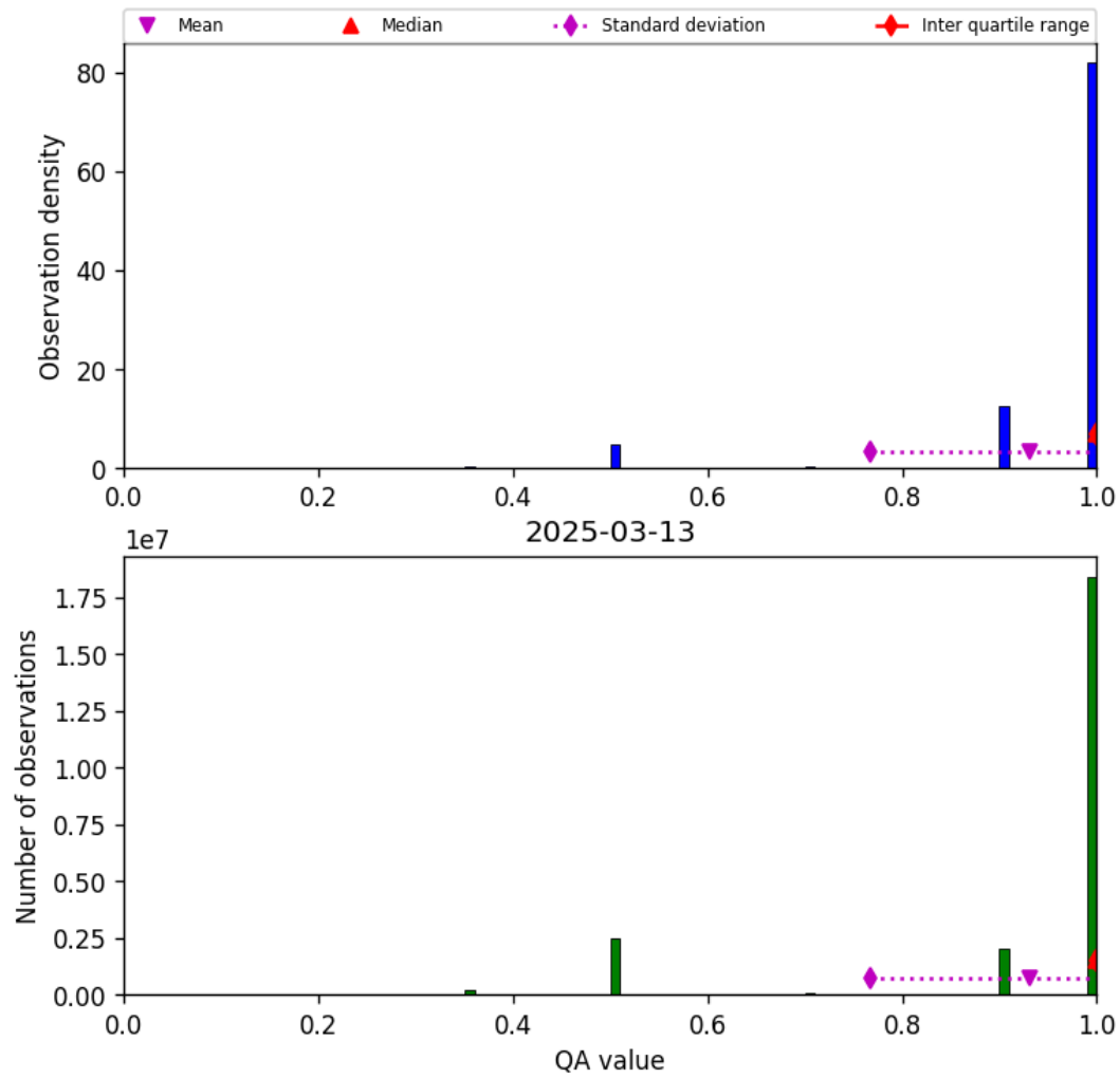
Figure 27: Histogram of “QA value” for 2025-03-13 to 2025-03-14
