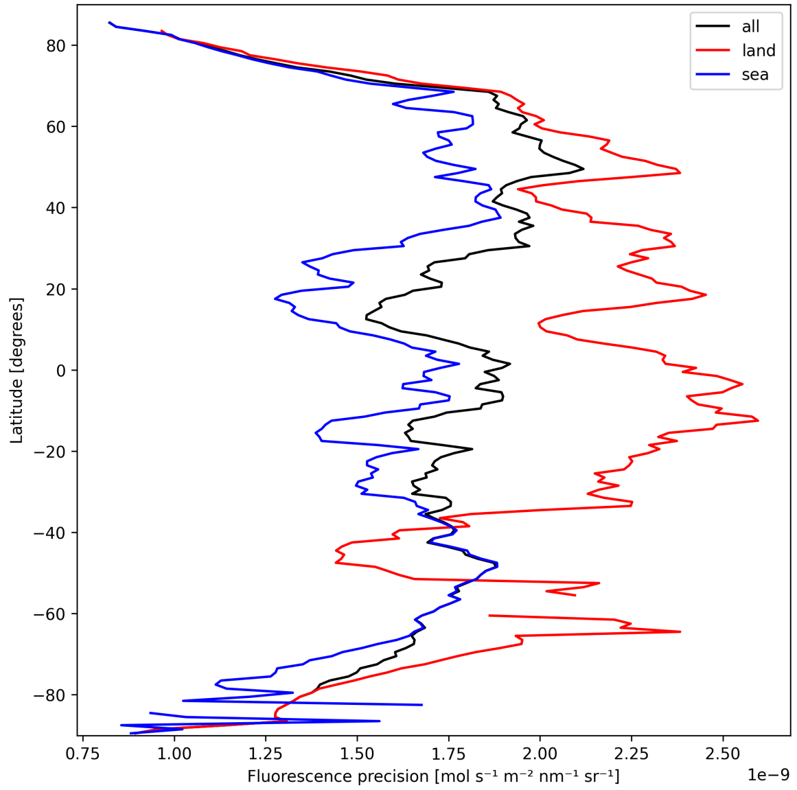
Figure 22: Zonal average of “Fluorescence precision” for 2025-03-13 to 2025-03-14.
