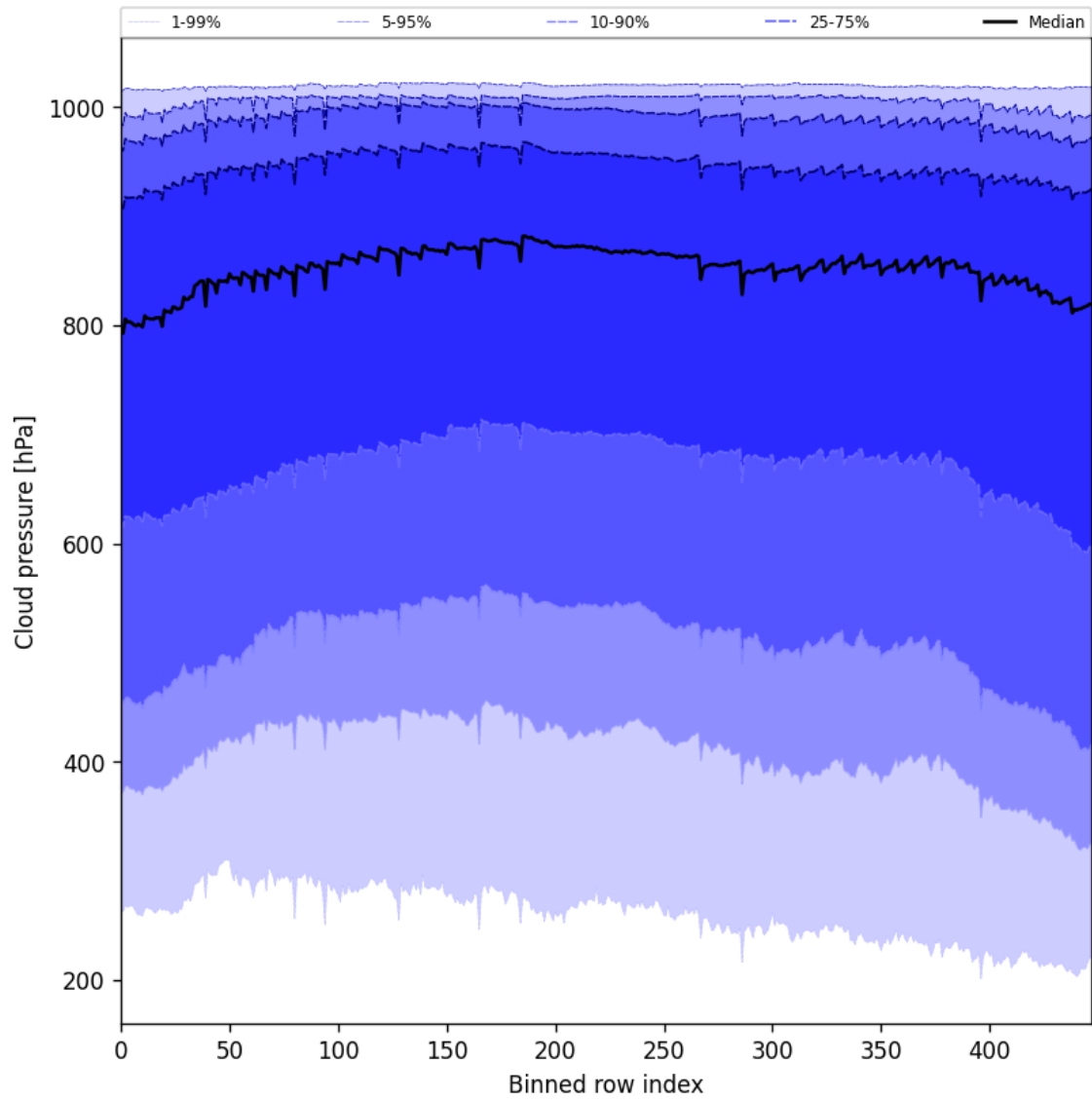
Figure 45: Along track statistics of “Cloud pressure” for 2025-03-13 to 2025-03-14
