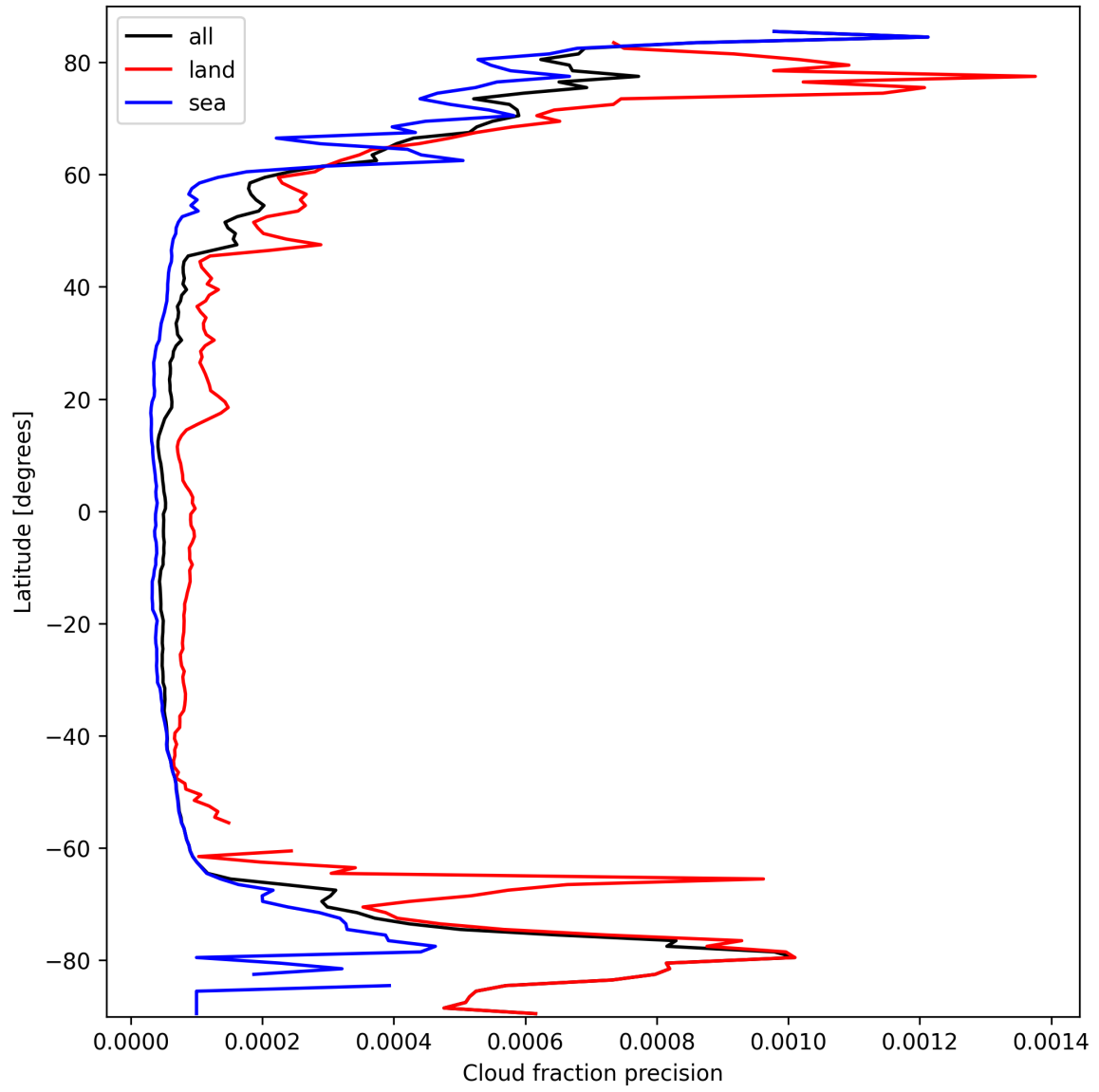
Figure 14: Zonal average of “Cloud fraction precision” for 2025-03-13 to 2025-03-14.
