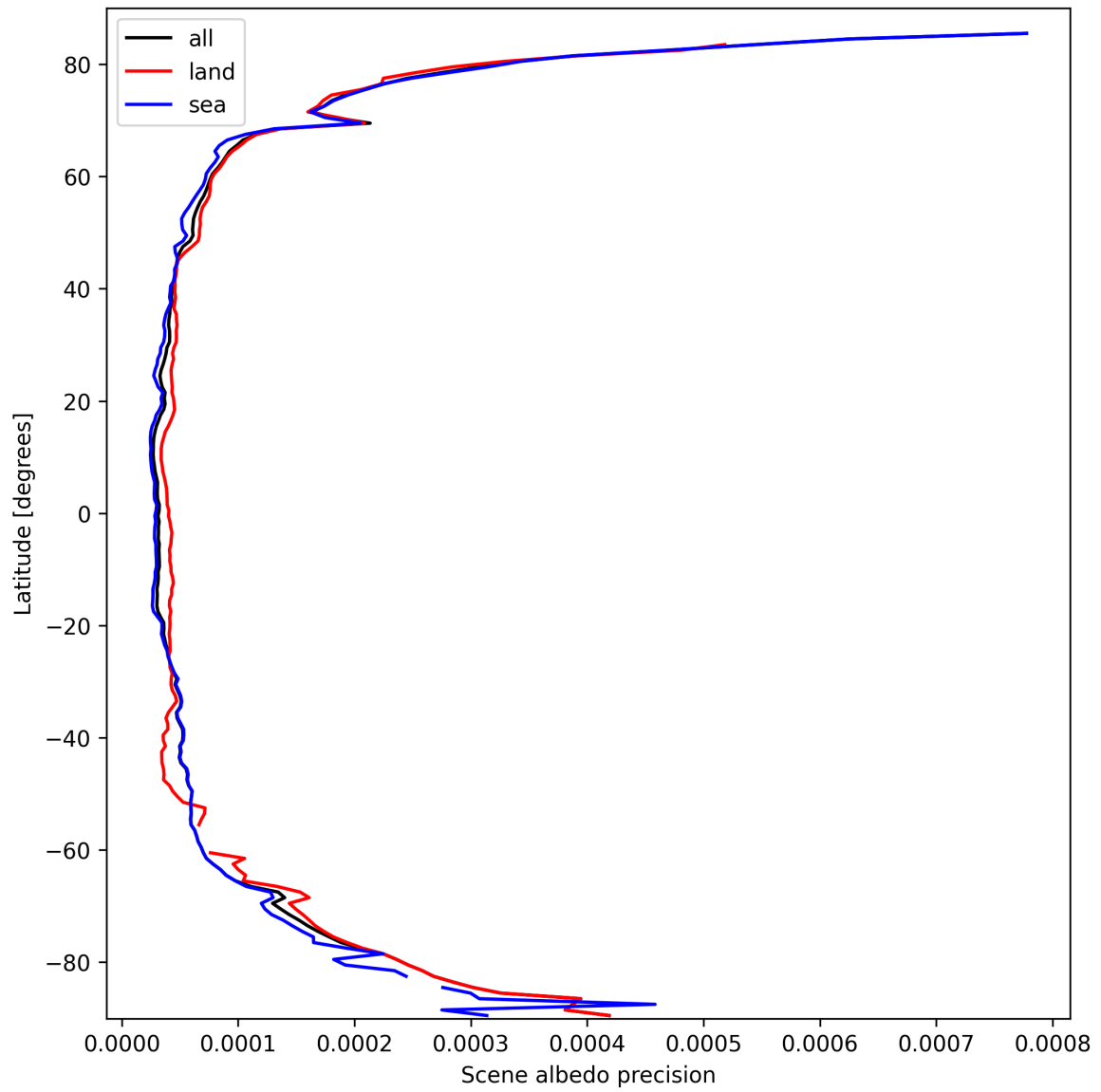
Figure 16: Zonal average of “Scene albedo precision” for 2025-03-13 to 2025-03-14.
