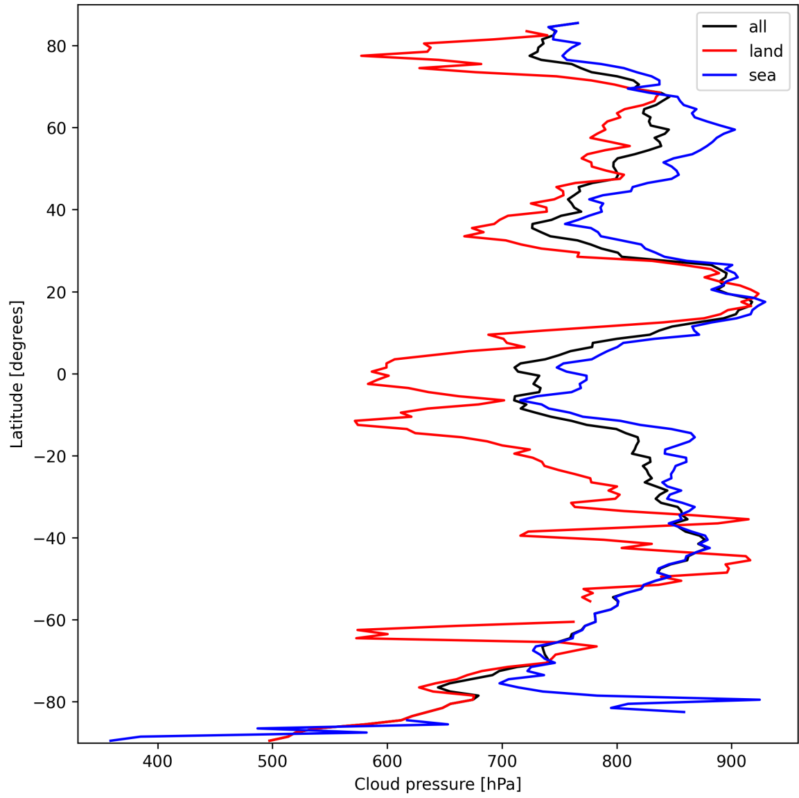
Figure 11: Zonal average of “Cloud pressure” for 2025-03-13 to 2025-03-14.
