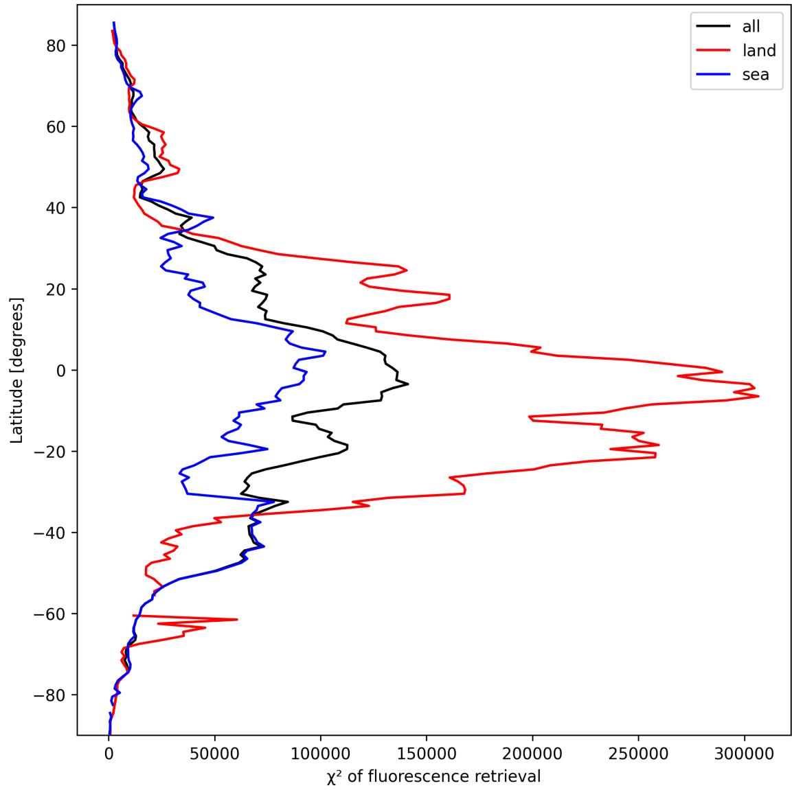
Figure 23: Zonal average of “ \chi^2 of fluorescence retrieval” for 2025-03-13 to 2025-03-14.
