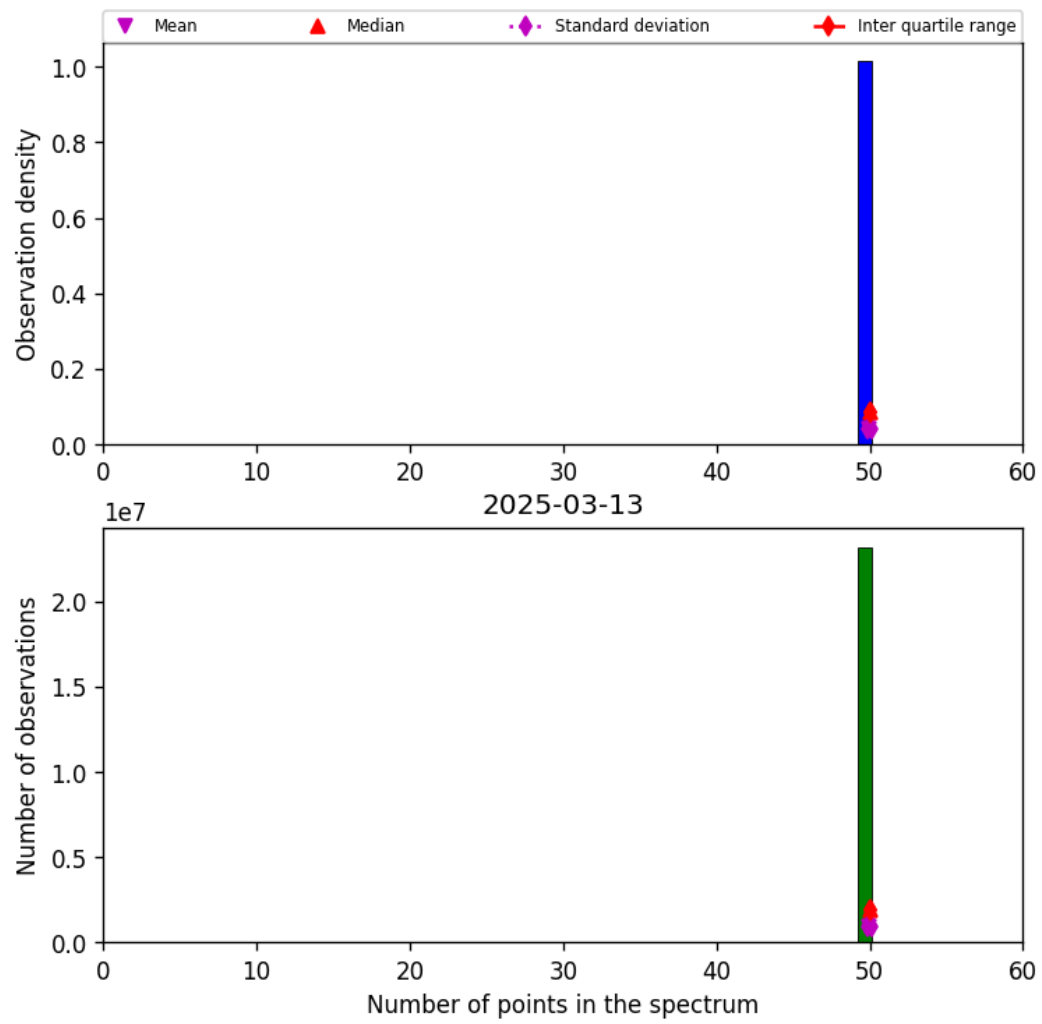
Figure 42: Histogram of “Number of points in the spectrum” for 2025-03-13 to 2025-03-14
