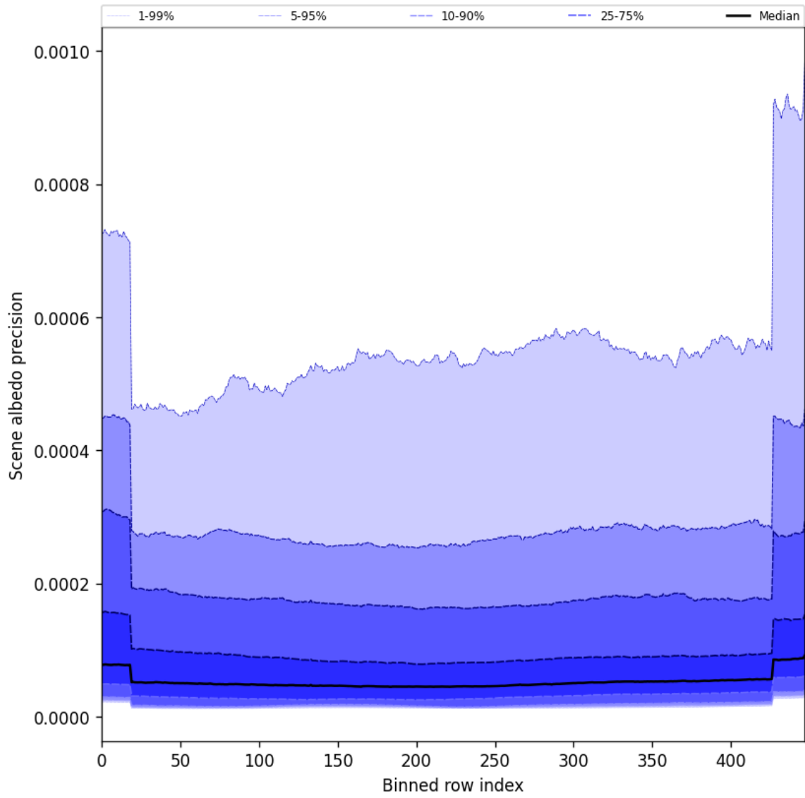
Figure 50: Along track statistics of “Scene albedo precision” for 2025-03-13 to 2025-03-14
