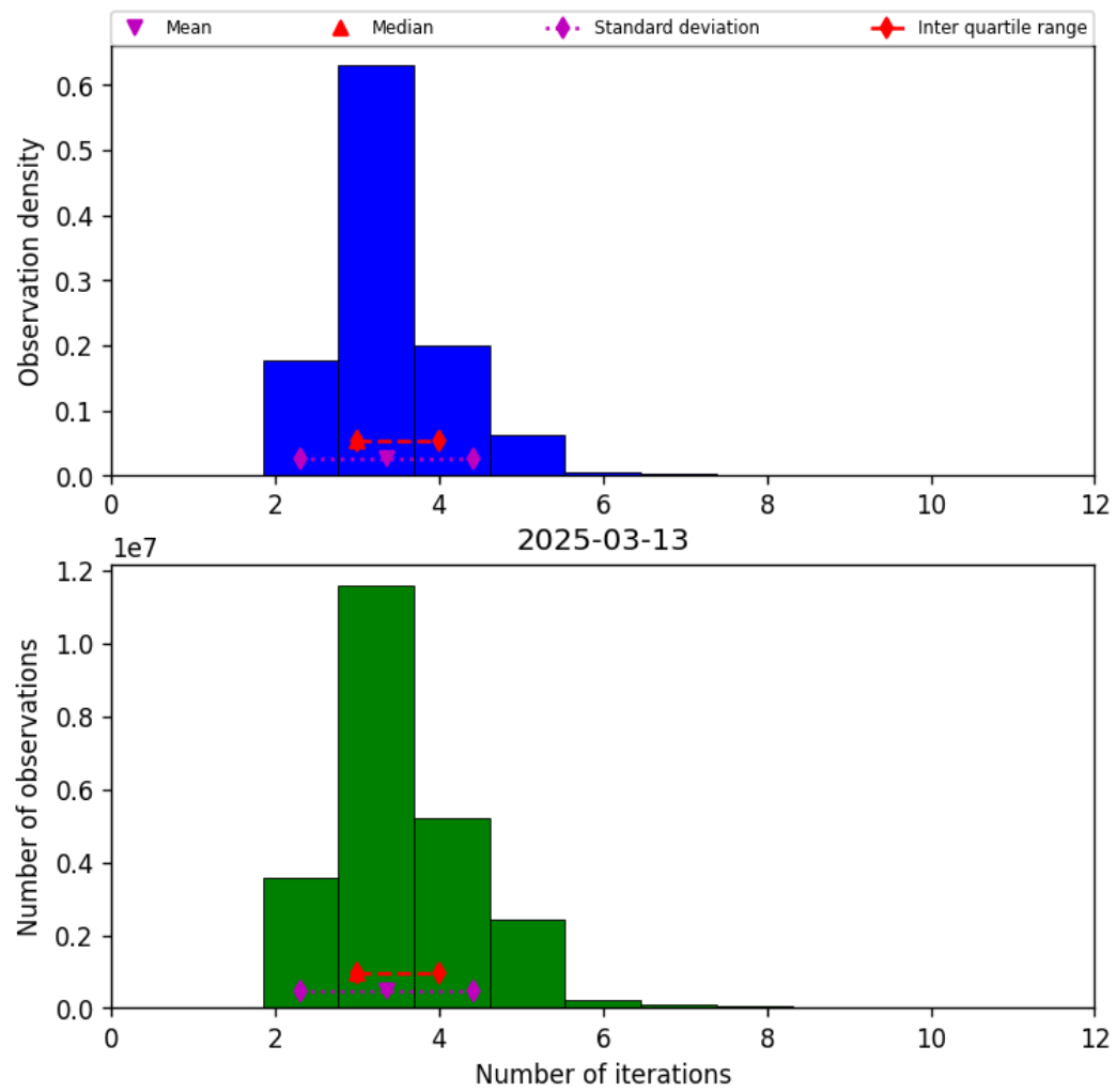
Figure 37: Histogram of “Number of iterations” for 2025-03-13 to 2025-03-14
