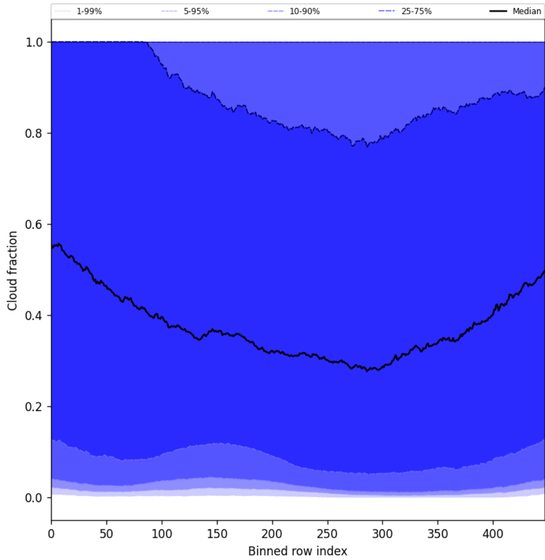
Figure 47: Along track statistics of “Cloud fraction” for 2025-03-13 to 2025-03-14
