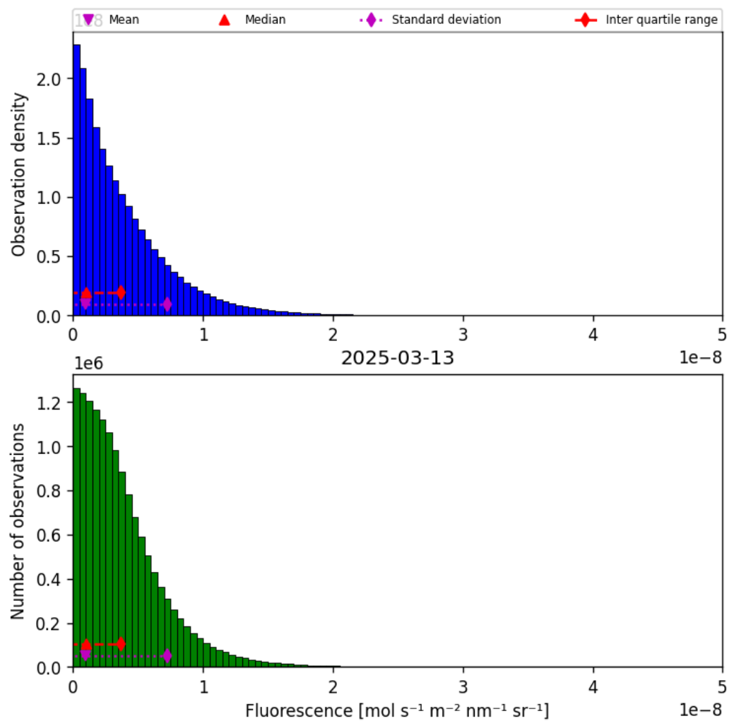
Figure 38: Histogram of “Fluorescence” for 2025-03-13 to 2025-03-14
