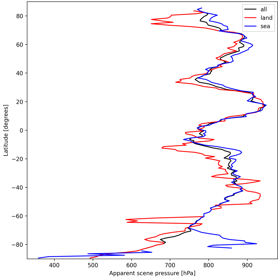
Figure 17: Zonal average of “Apparent scene pressure” for 2025-03-13 to 2025-03-14.
