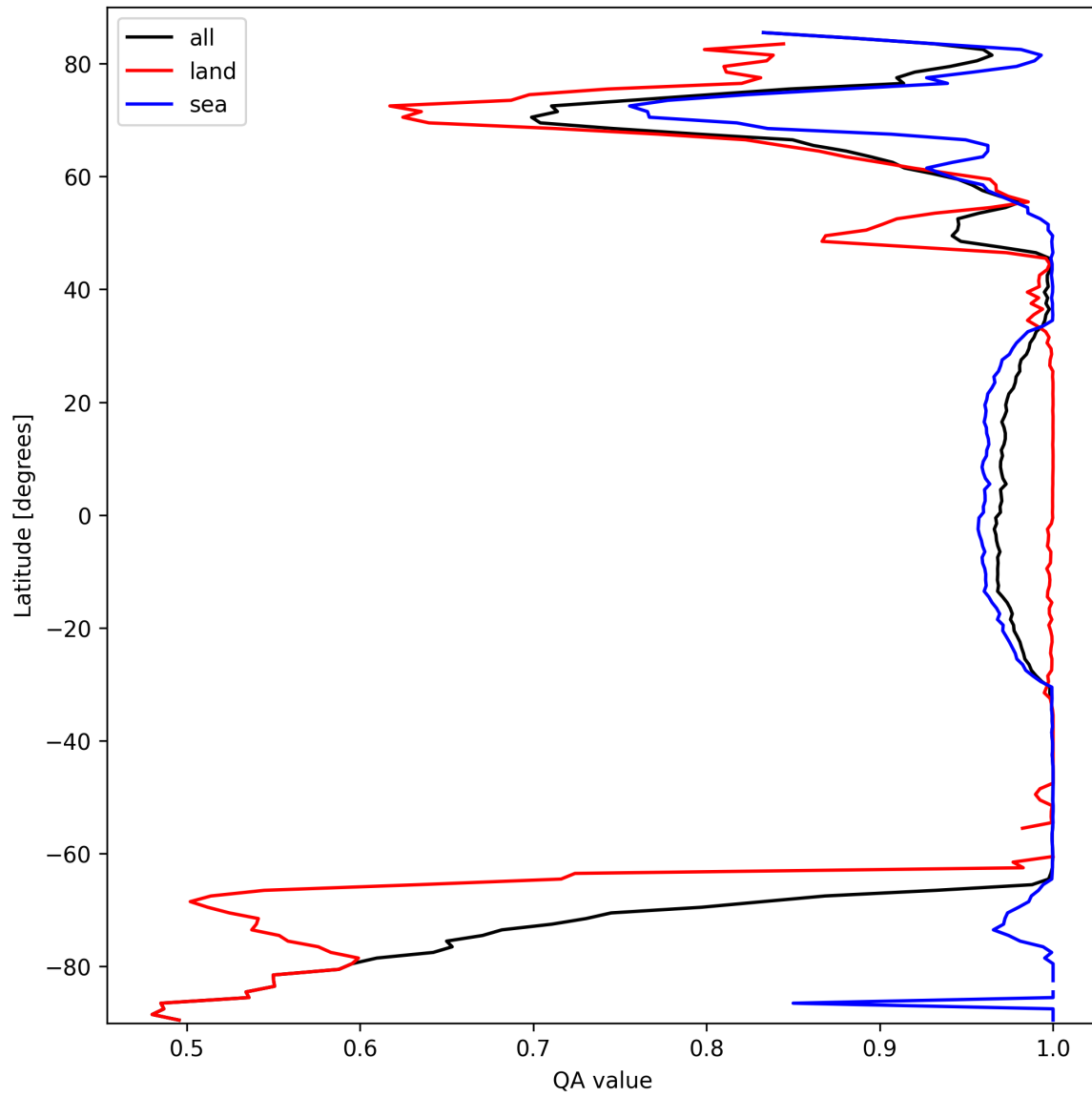
Figure 10: Zonal average of “QA value” for 2025-03-13 to 2025-03-14.
