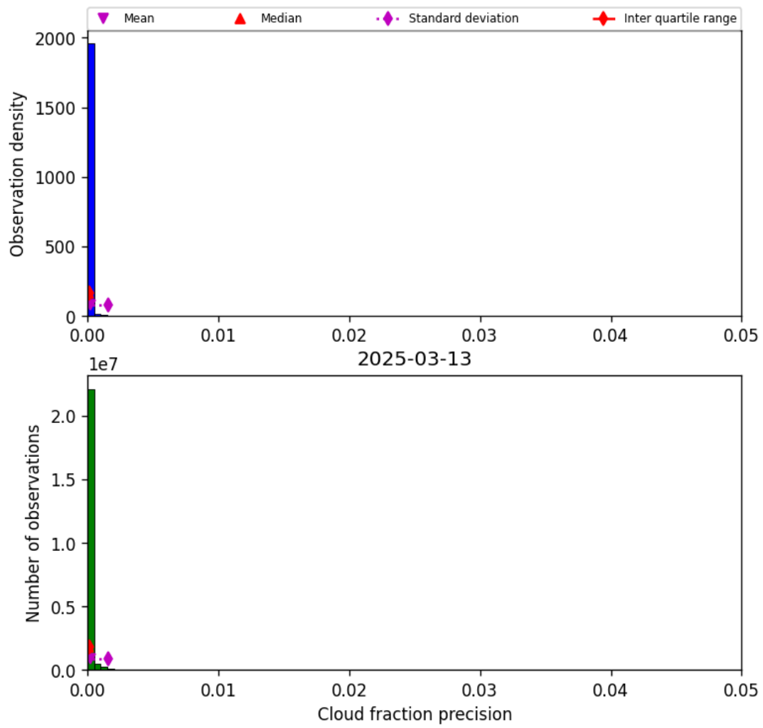
Figure 31: Histogram of “Cloud fraction precision” for 2025-03-13 to 2025-03-14
