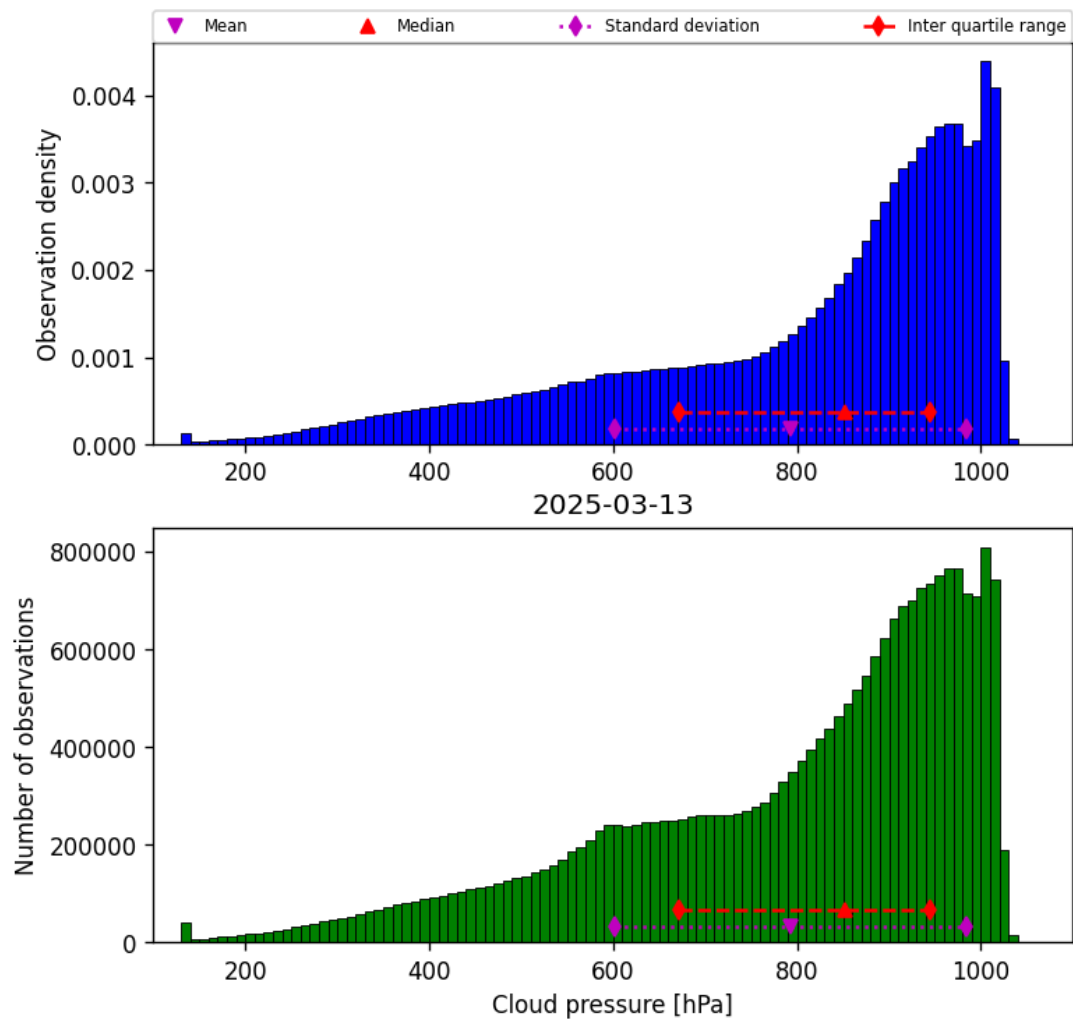
Figure 28: Histogram of “Cloud pressure” for 2025-03-13 to 2025-03-14
