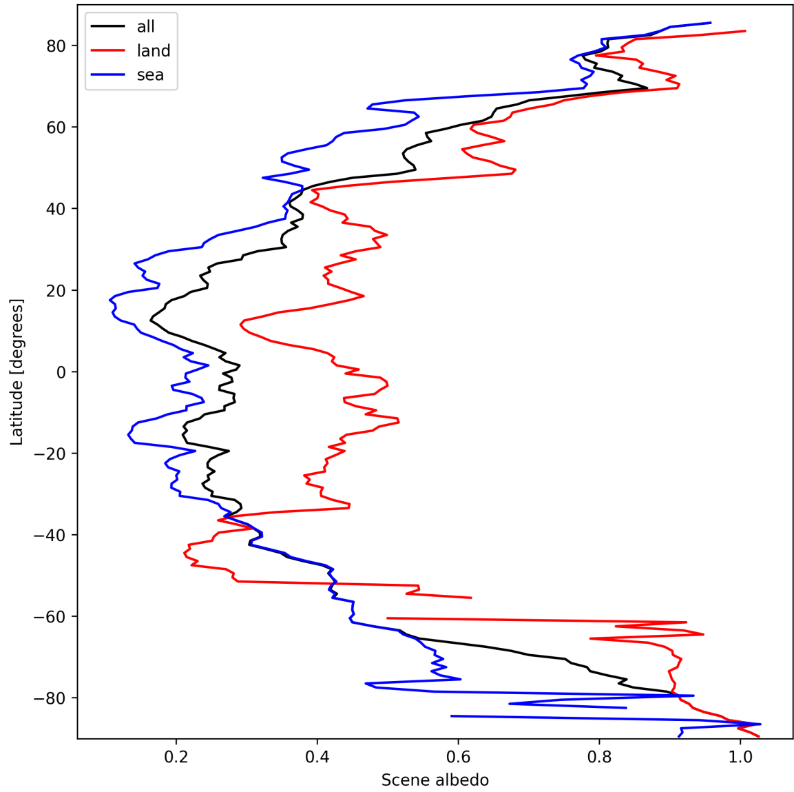
Figure 15: Zonal average of “Scene albedo” for 2025-03-13 to 2025-03-14.
