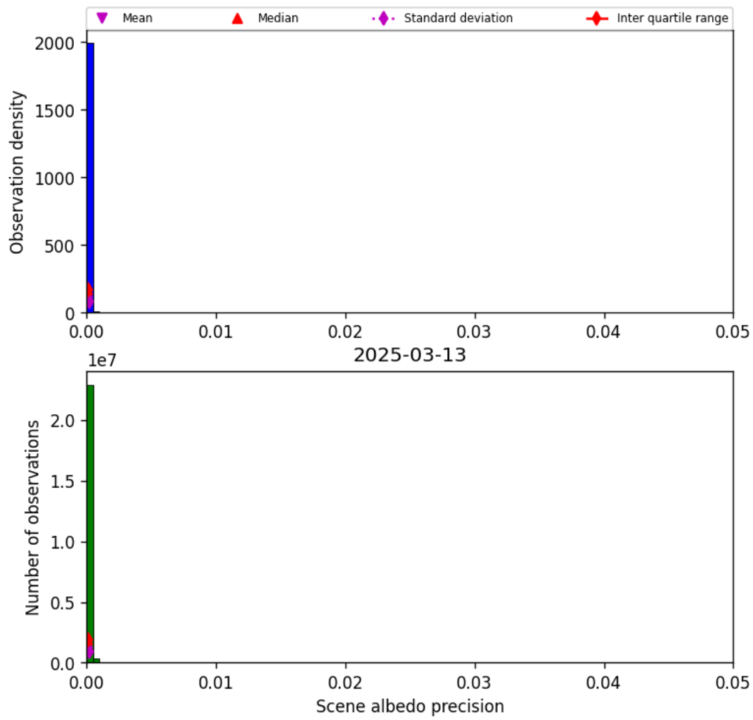
Figure 33: Histogram of “Scene albedo precision” for 2025-03-13 to 2025-03-14
