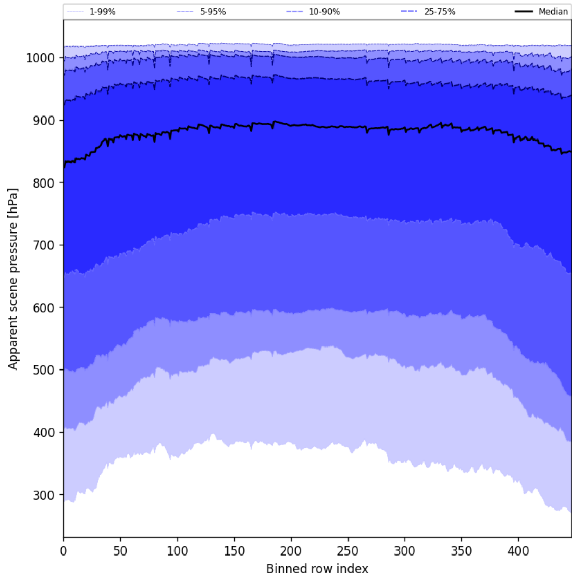
Figure 51: Along track statistics of “Apparent scene pressure” for 2025-03-13 to 2025-03-14
