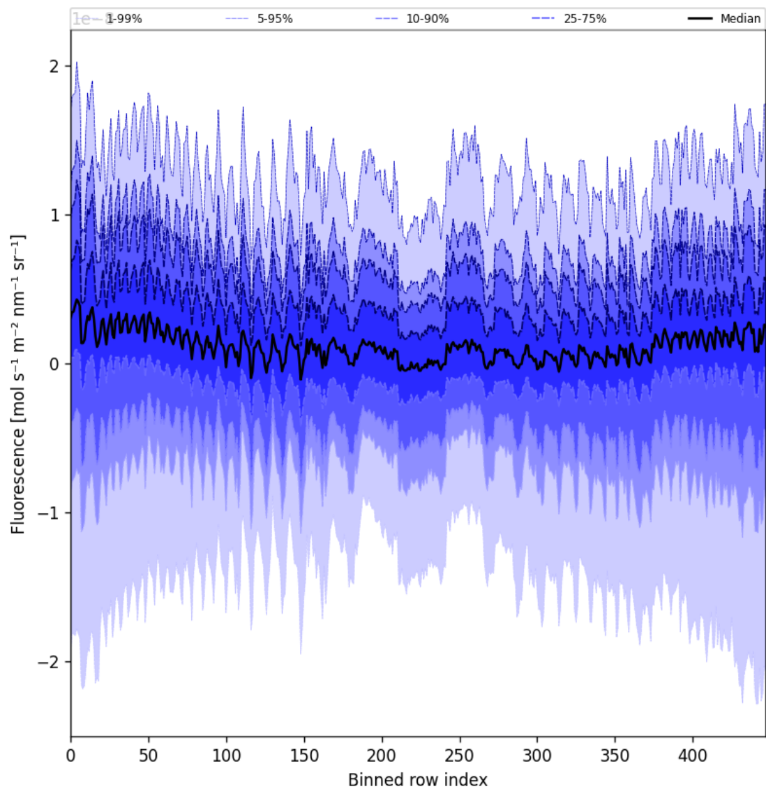
Figure 55: Along track statistics of “Fluorescence” for 2025-03-13 to 2025-03-14
