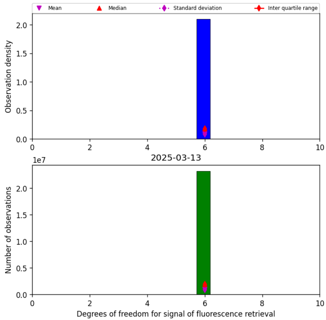
Figure 41: Histogram of “Degrees of freedom for signal of fluorescence retrieval” for 2025-03-13 to 2025-03-14
