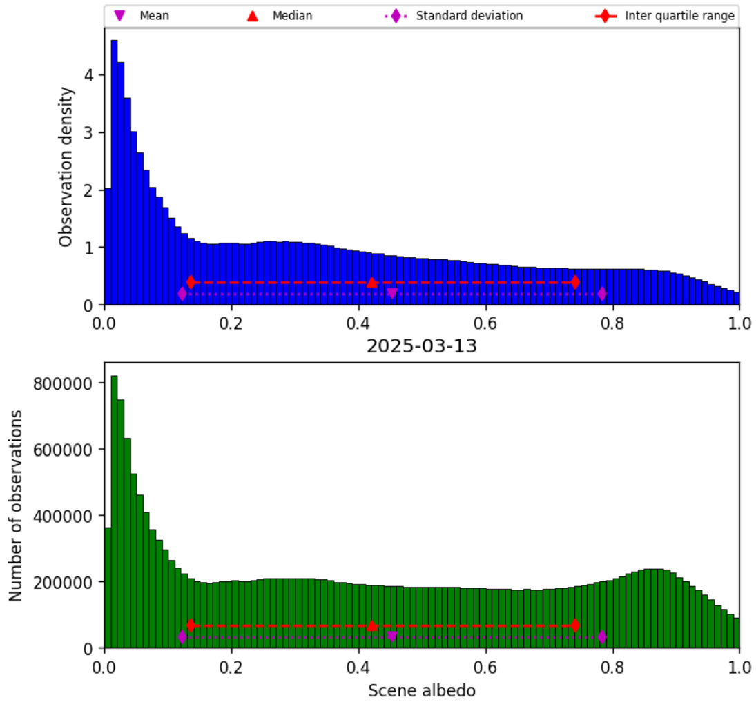
Figure 32: Histogram of “Scene albedo” for 2025-03-13 to 2025-03-14
