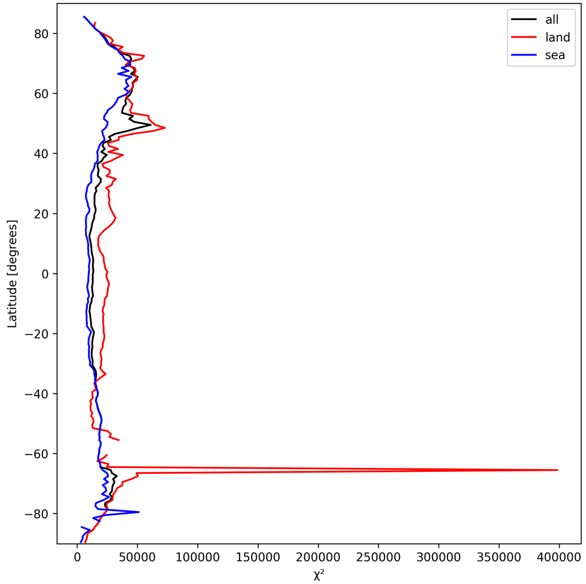
Figure 19: Zonal average of “ \chi^2 ” for 2025-03-13 to 2025-03-14.
