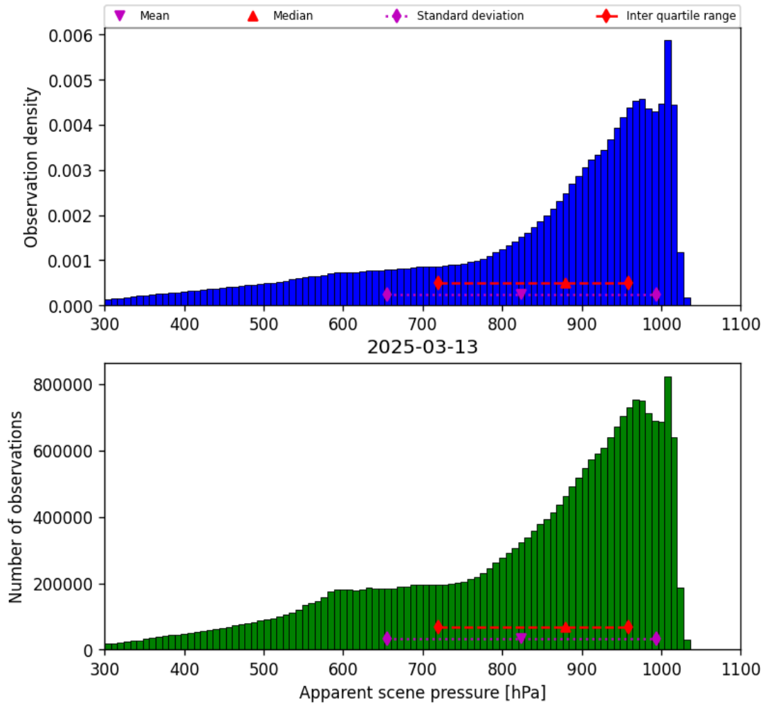
Figure 34: Histogram of “Apparent scene pressure” for 2025-03-13 to 2025-03-14
