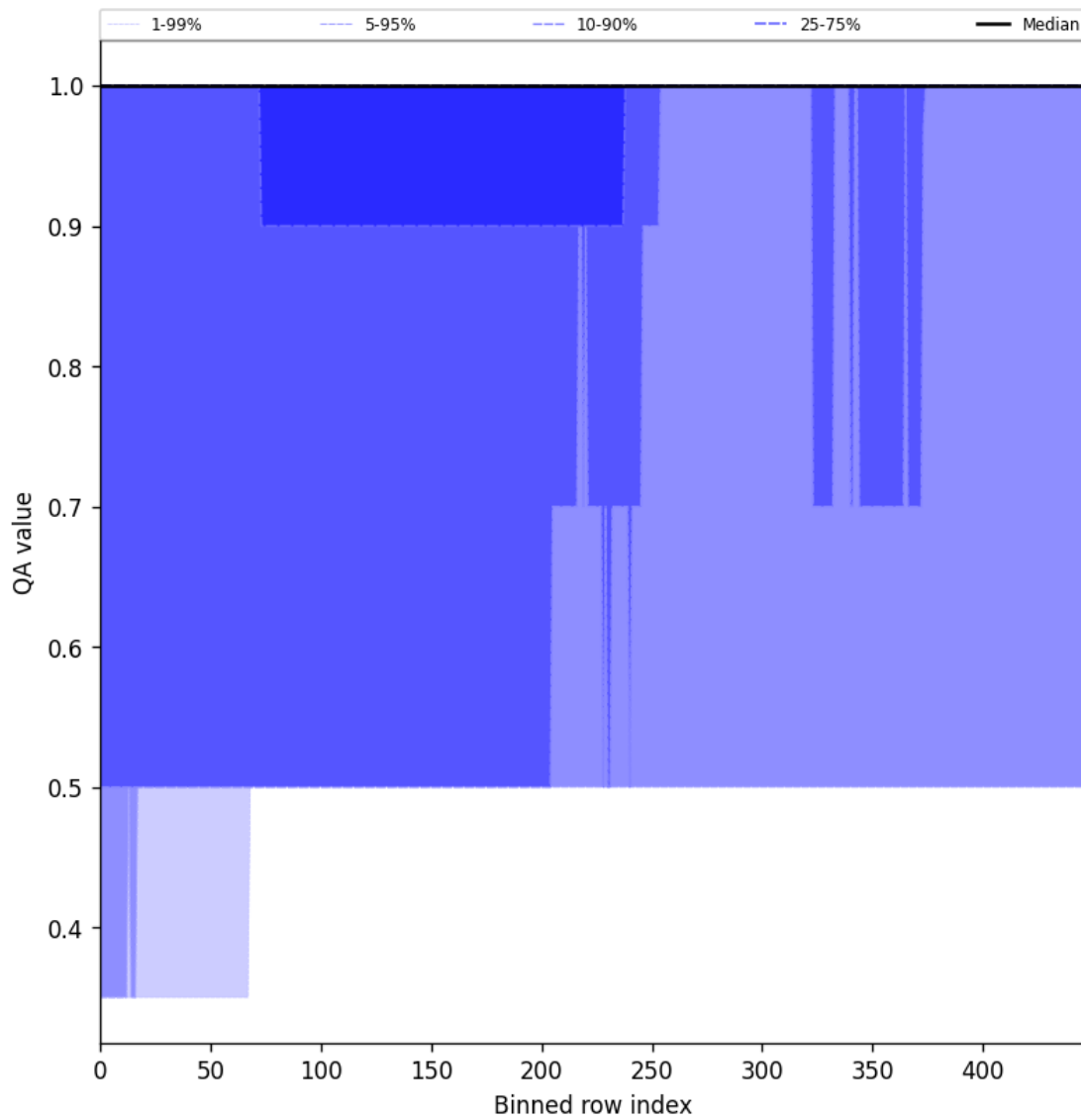
Figure 44: Along track statistics of “QA value” for 2025-03-13 to 2025-03-14
