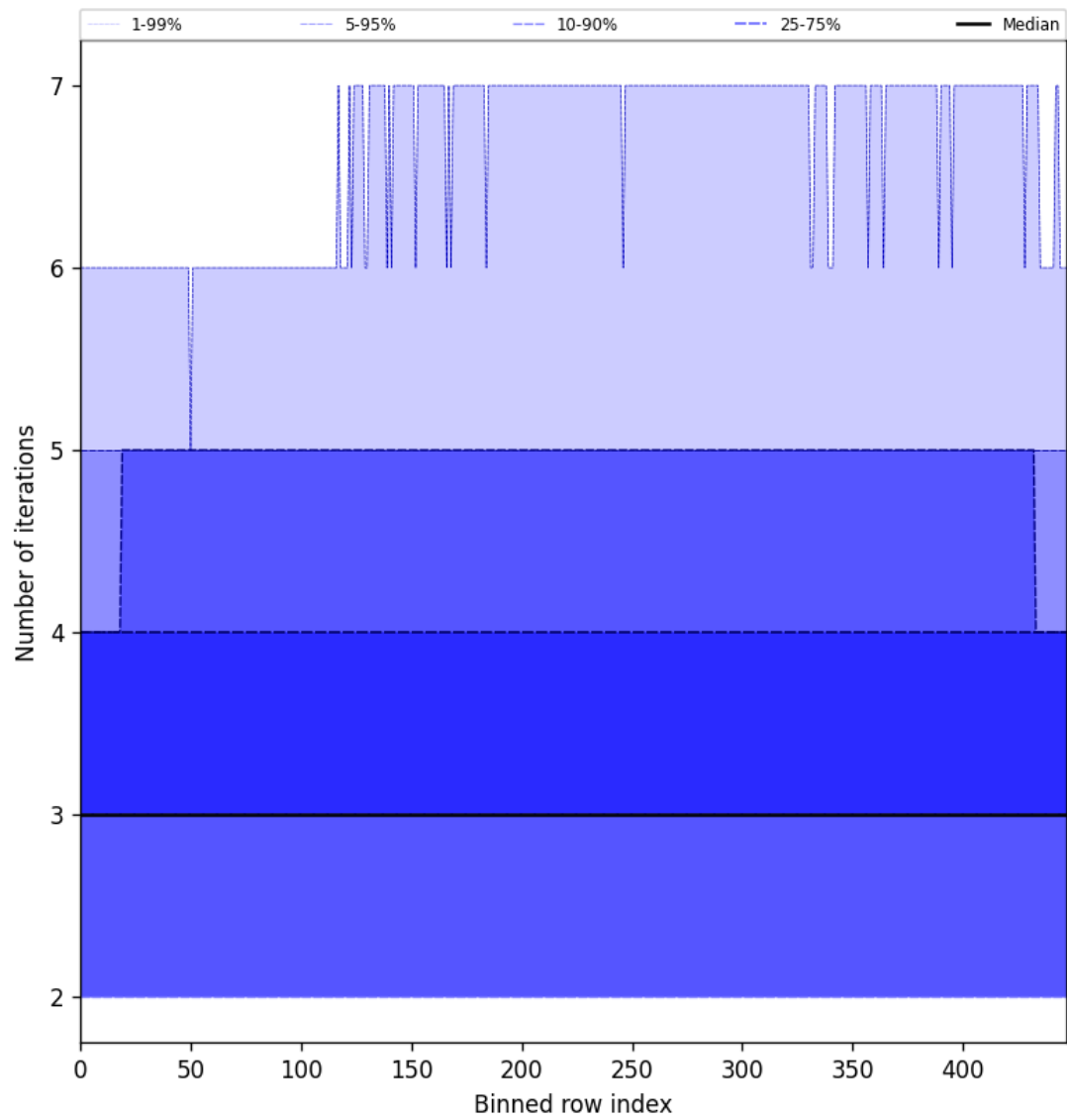
Figure 54: Along track statistics of “Number of iterations” for 2025-03-13 to 2025-03-14
