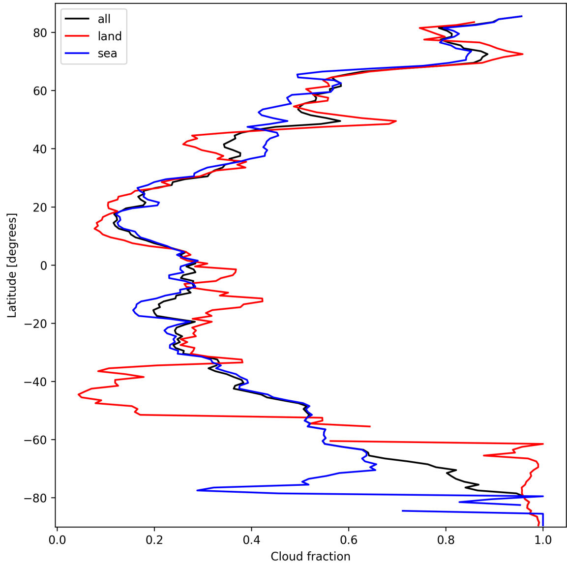
Figure 13: Zonal average of “Cloud fraction” for 2025-03-13 to 2025-03-14.
