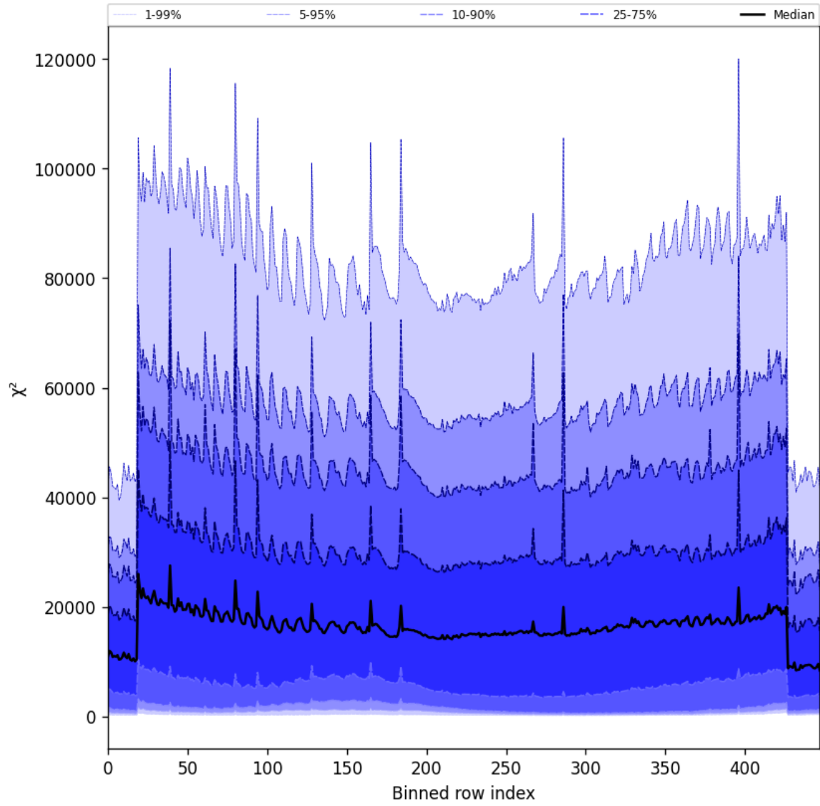
Figure 53: Along track statistics of “ \chi^2 ” for 2025-03-13 to 2025-03-14
