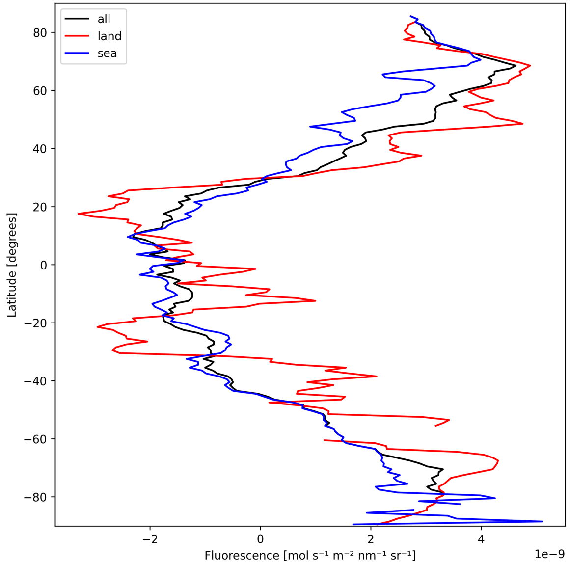
Figure 21: Zonal average of “Fluorescence” for 2025-03-13 to 2025-03-14.
