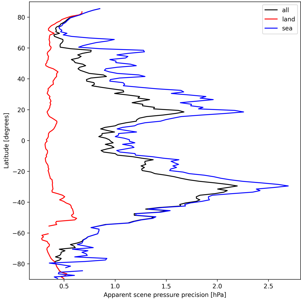
Figure 18: Zonal average of “Apparent scene pressure precision” for 2025-03-13 to 2025-03-14.
