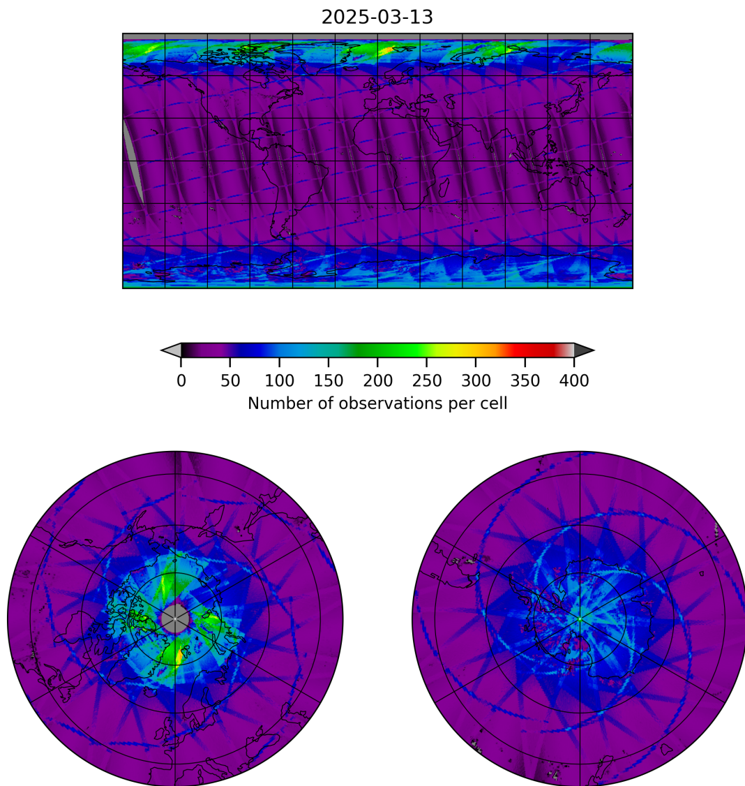
Figure 9: Map of the number of observations for 2025-03-13 to 2025-03-14
