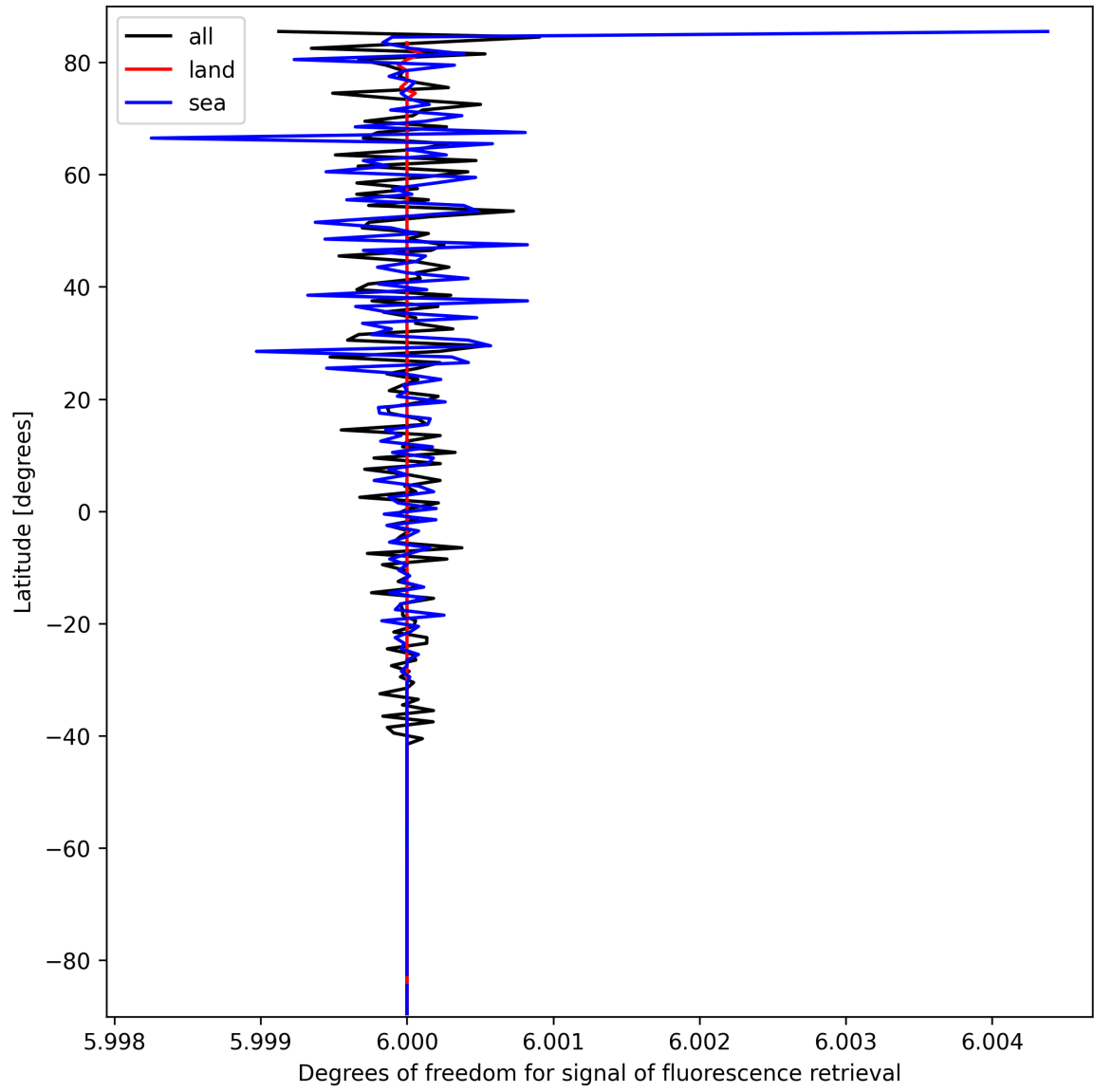
Figure 24: Zonal average of “Degrees of freedom for signal of fluorescence retrieval” for 2025-03-13 to 2025-03-14.
