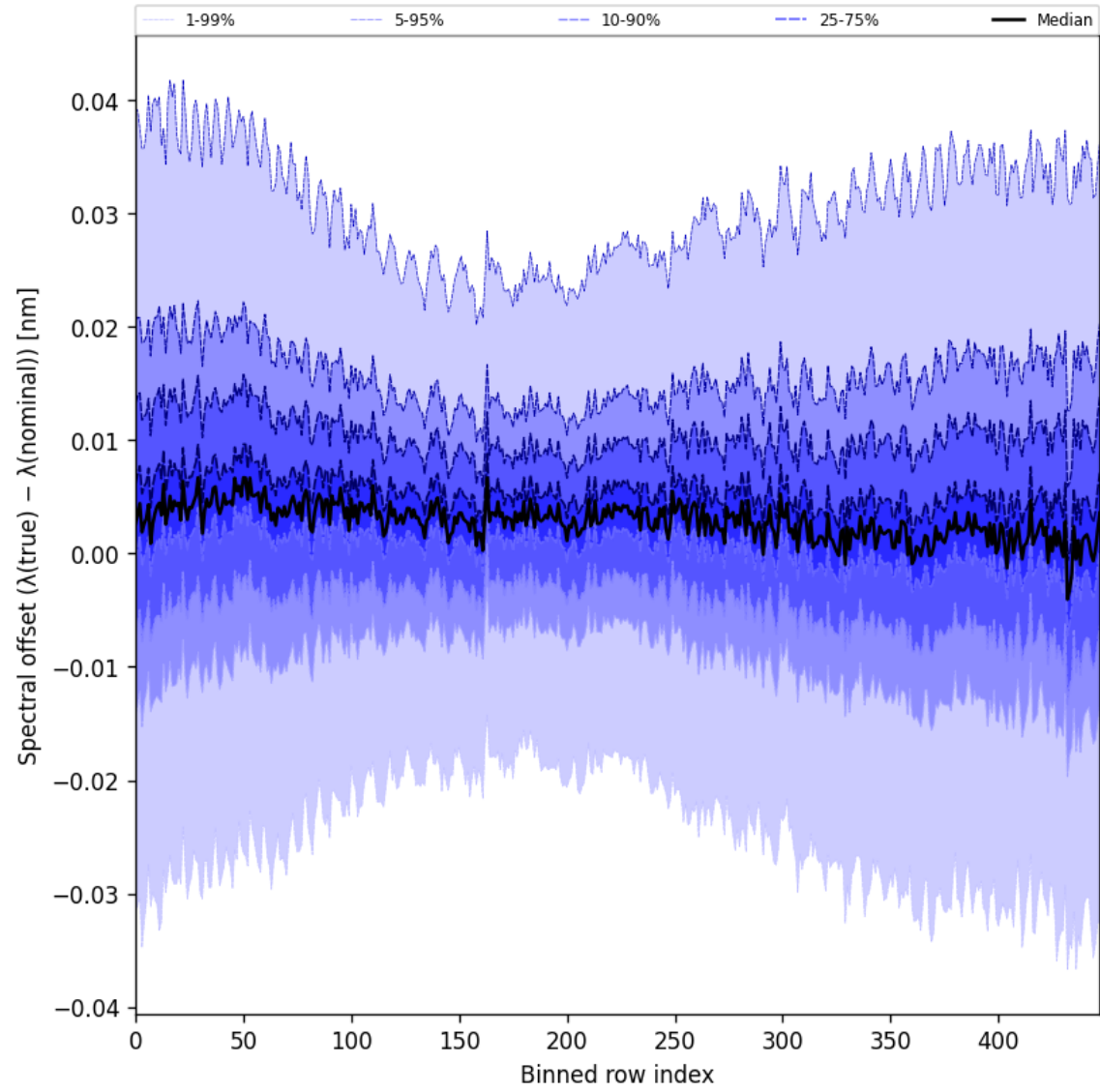
Figure 60: Along track statistics of “Spectral offset ( \lambda_{\text{true}} - \lambda_{\text{nominal}} )” for 2025-03-13 to 2025-03-14
