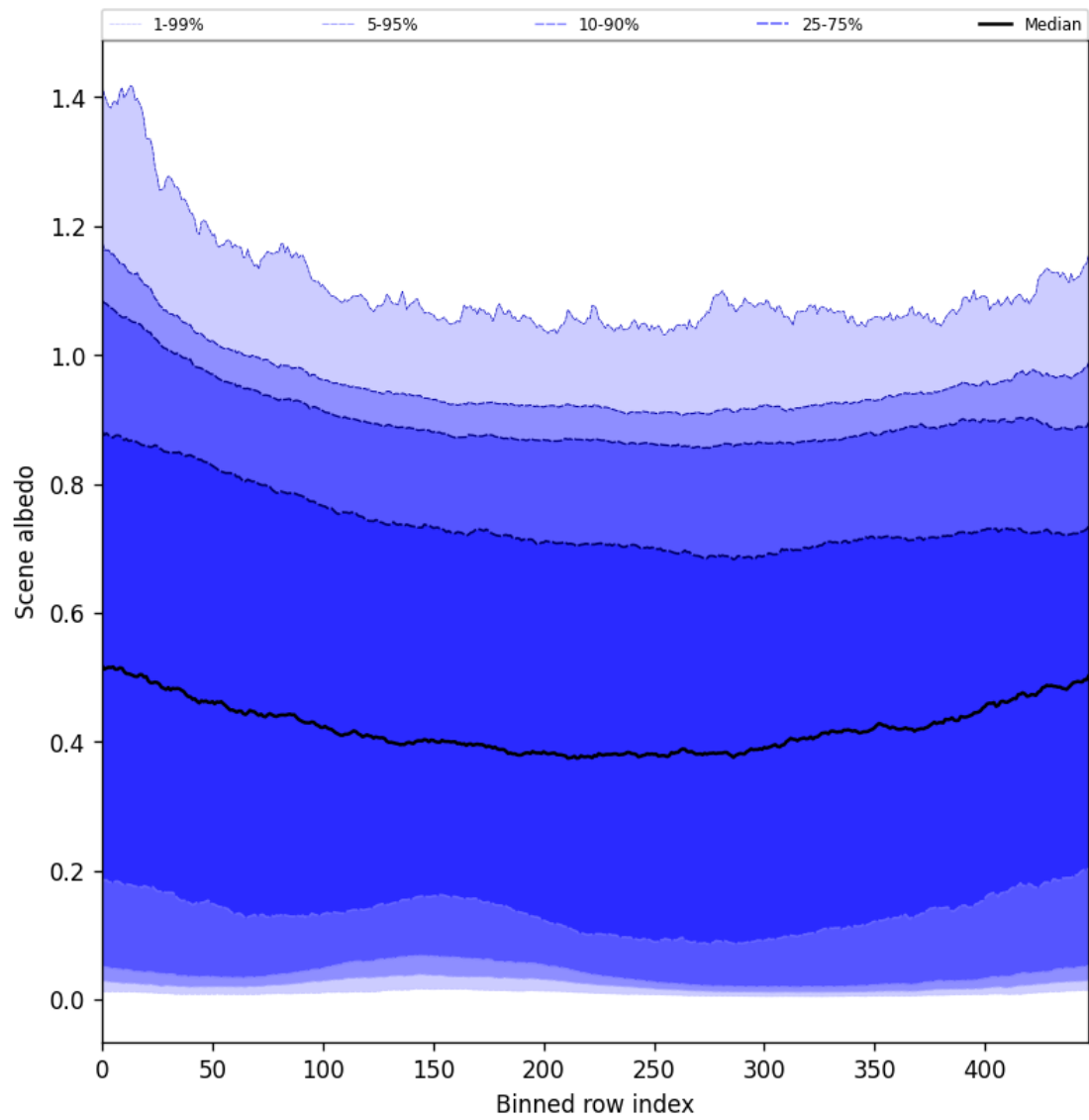
Figure 49: Along track statistics of “Scene albedo” for 2025-03-13 to 2025-03-14
