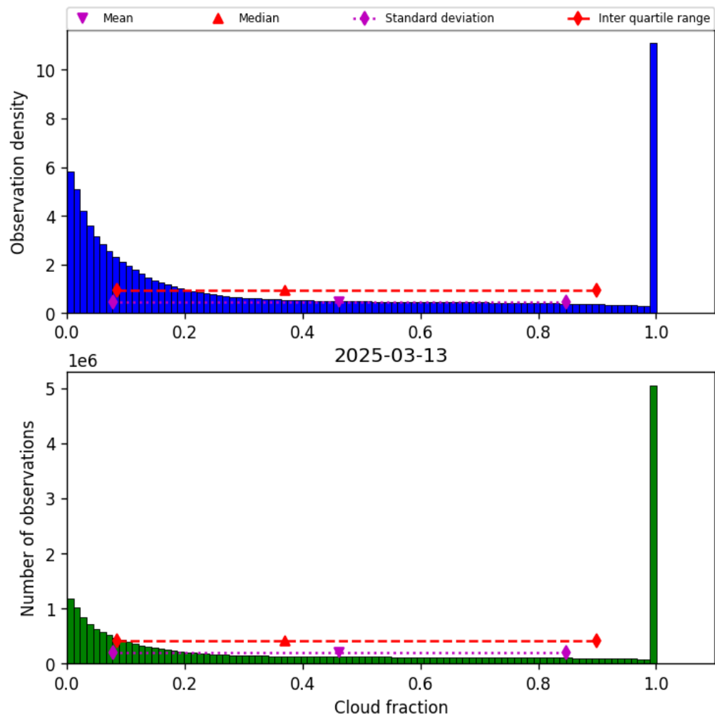
Figure 30: Histogram of “Cloud fraction” for 2025-03-13 to 2025-03-14
