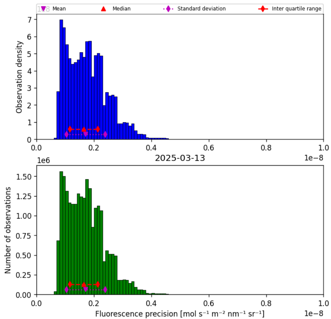
Figure 39: Histogram of “Fluorescence precision” for 2025-03-13 to 2025-03-14
