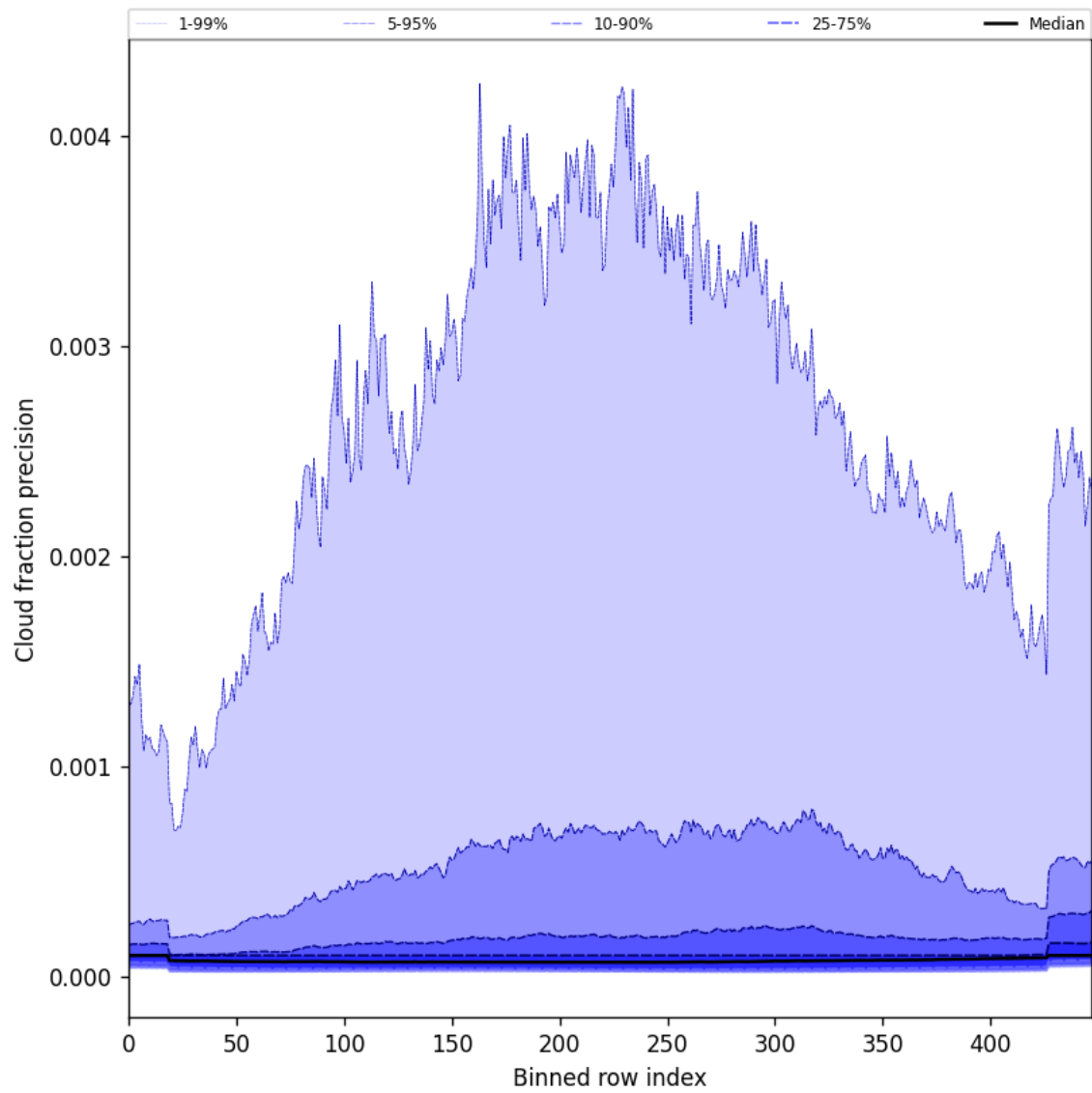
Figure 48: Along track statistics of “Cloud fraction precision” for 2025-03-13 to 2025-03-14
