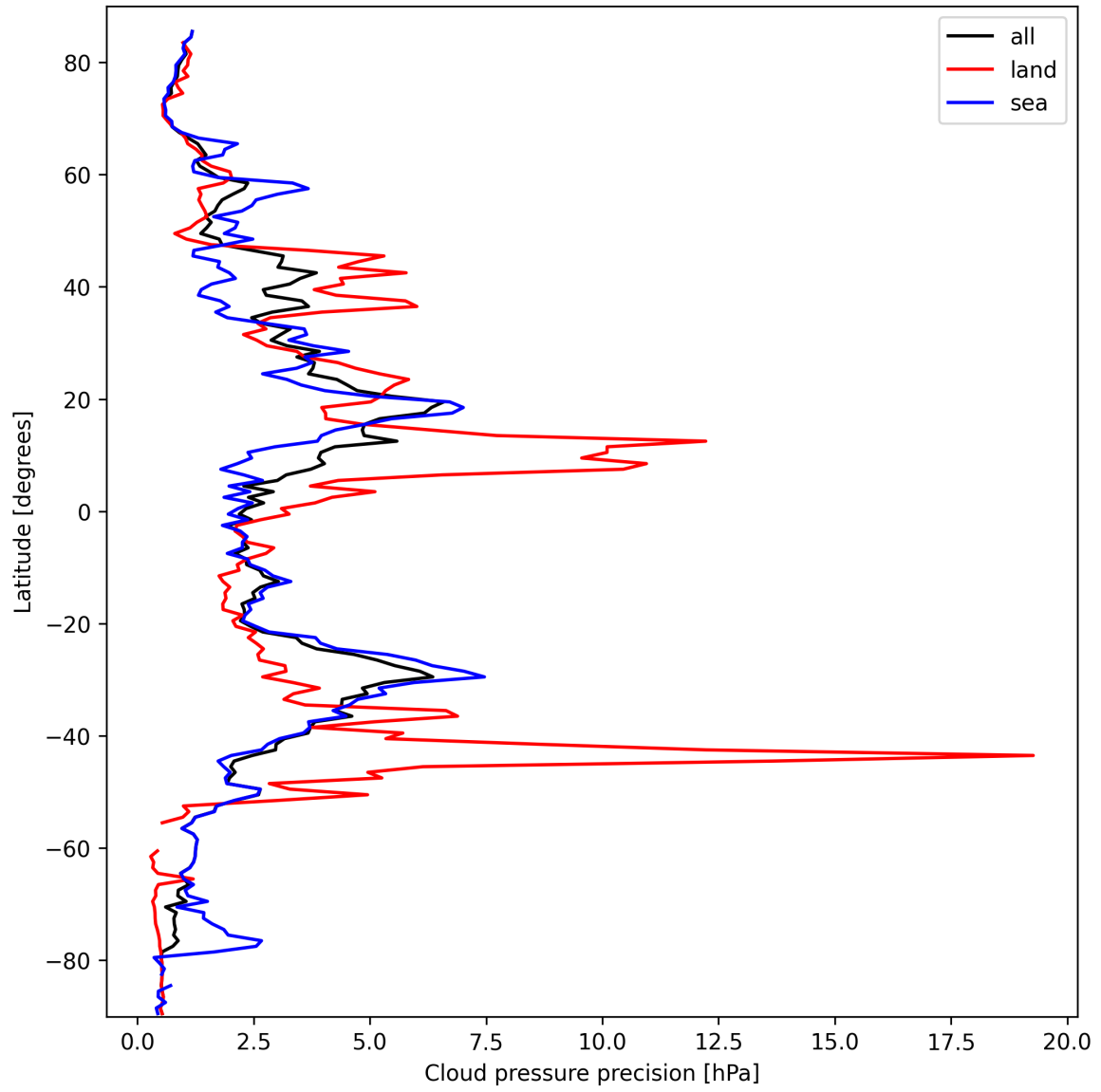
Figure 12: Zonal average of “Cloud pressure precision” for 2025-03-13 to 2025-03-14.
