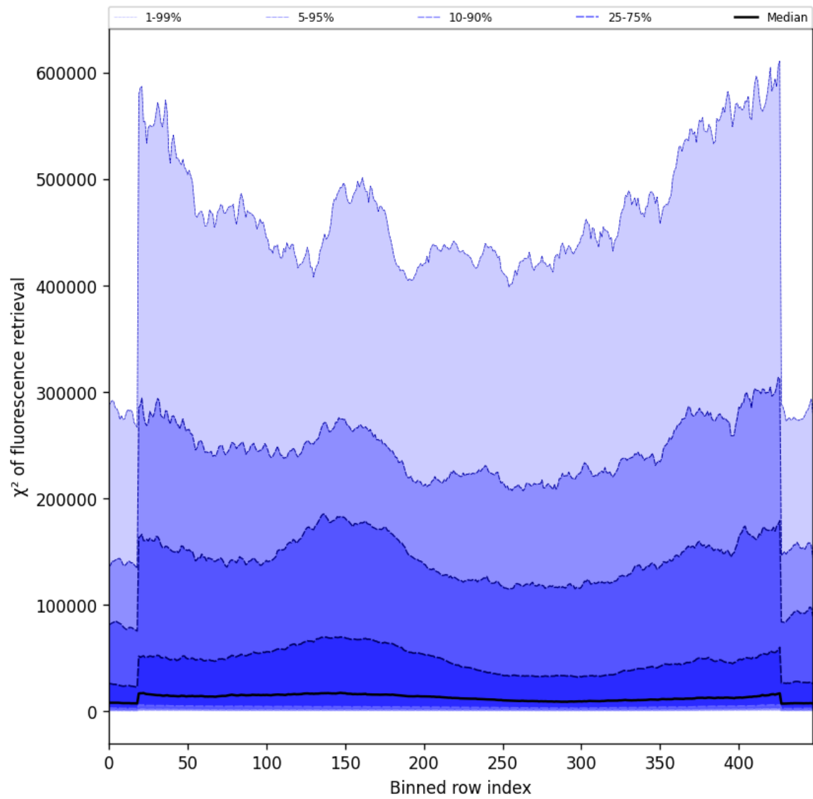
Figure 57: Along track statistics of “ \chi^2 of fluorescence retrieval” for 2025-03-13 to 2025-03-14
