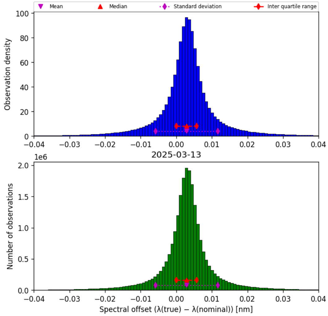
Figure 43: Histogram of “Spectral offset ( \lambda_{\text{true}} - \lambda_{\text{nominal}} )” for 2025-03-13 to 2025-03-14
