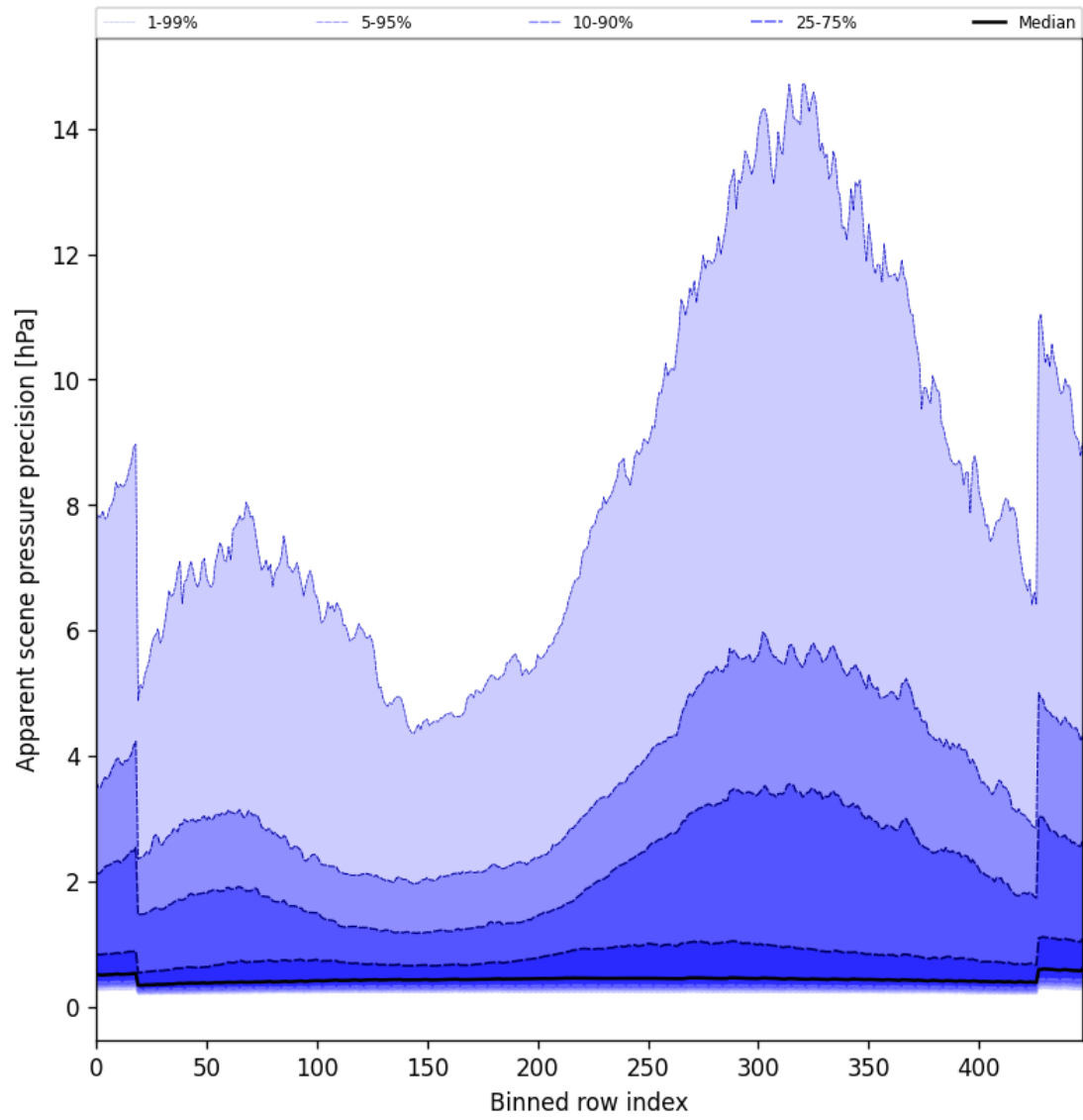
Figure 52: Along track statistics of “Apparent scene pressure precision” for 2025-03-13 to 2025-03-14
