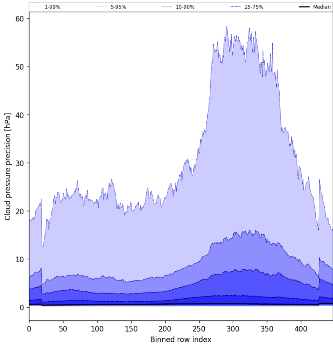
Figure 46: Along track statistics of “Cloud pressure precision” for 2025-03-13 to 2025-03-14
