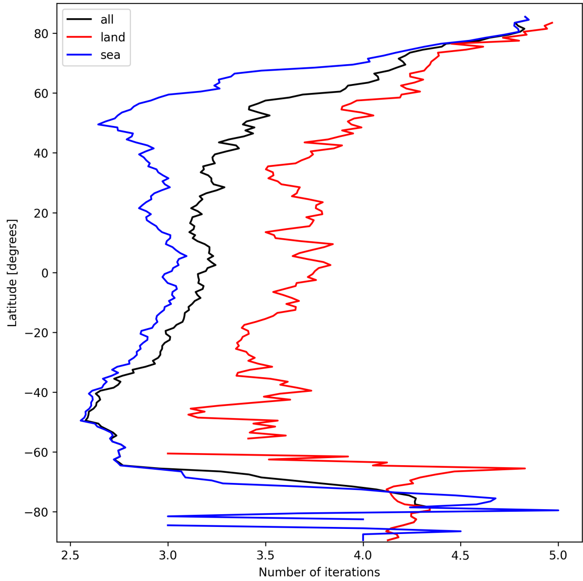
Figure 20: Zonal average of “Number of iterations” for 2025-03-13 to 2025-03-14.
