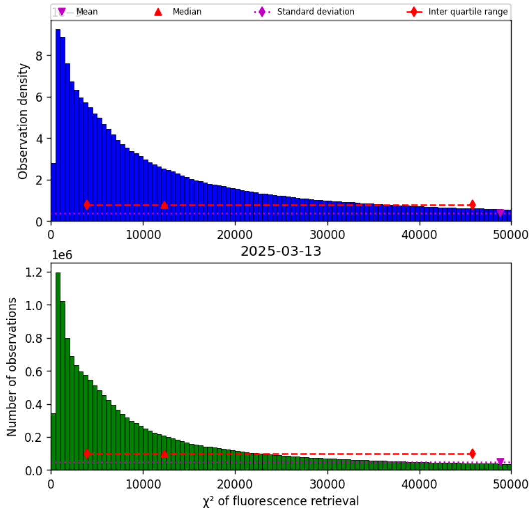
Figure 40: Histogram of “ \chi^2 of fluorescence retrieval” for 2025-03-13 to 2025-03-14
