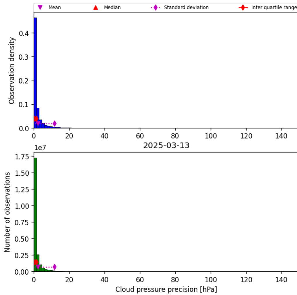
Figure 29: Histogram of “Cloud pressure precision” for 2025-03-13 to 2025-03-14
