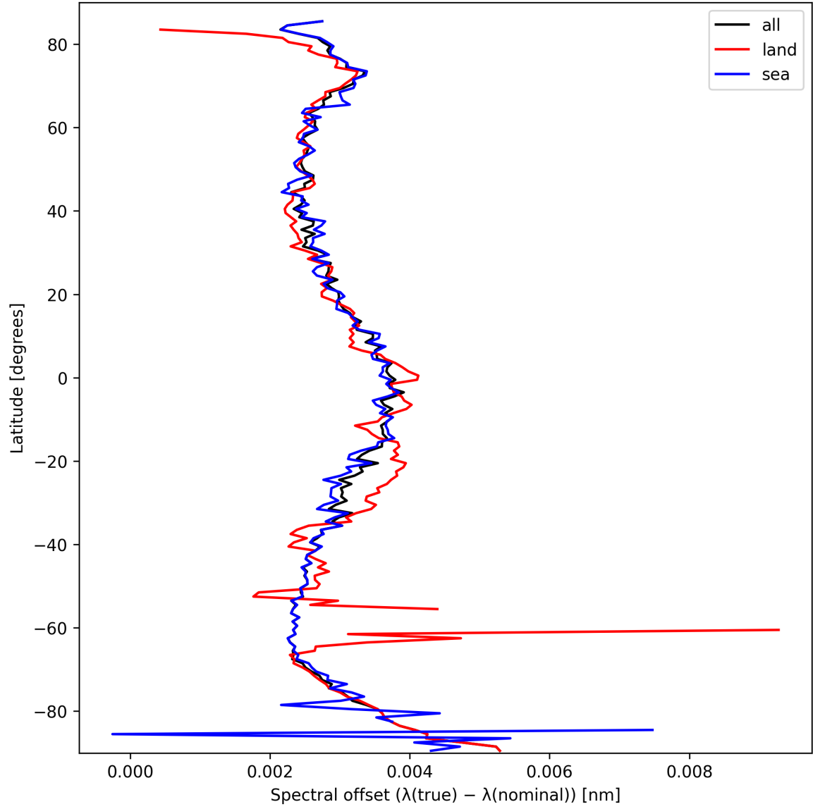
Figure 26: Zonal average of “Spectral offset ( \lambda_{\text{true}} - \lambda_{\text{nominal}} )” for 2025-03-13 to 2025-03-14.
