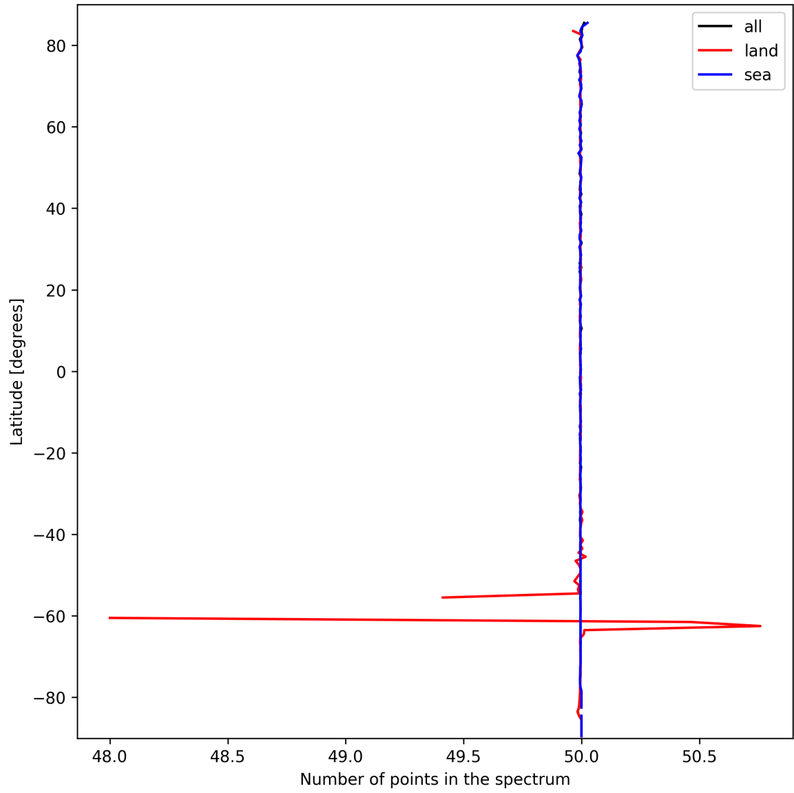
Figure 25: Zonal average of “Number of points in the spectrum” for 2025-03-13 to 2025-03-14.
