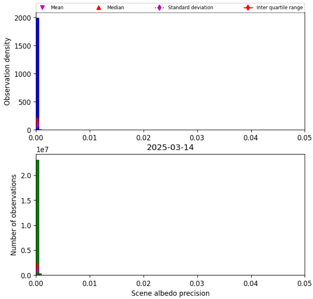
Figure 33: Histogram of “Scene albedo precision” for 2025-03-14 to 2025-03-15
