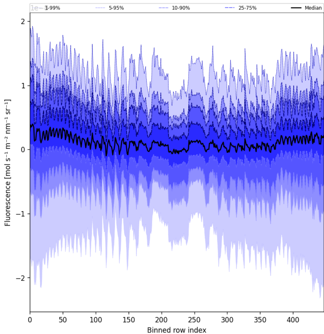
Figure 55: Along track statistics of “Fluorescence” for 2025-03-14 to 2025-03-15
