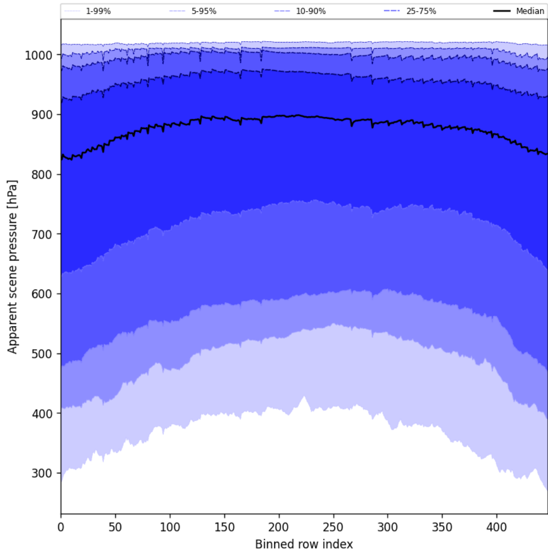
Figure 51: Along track statistics of “Apparent scene pressure” for 2025-03-14 to 2025-03-15
