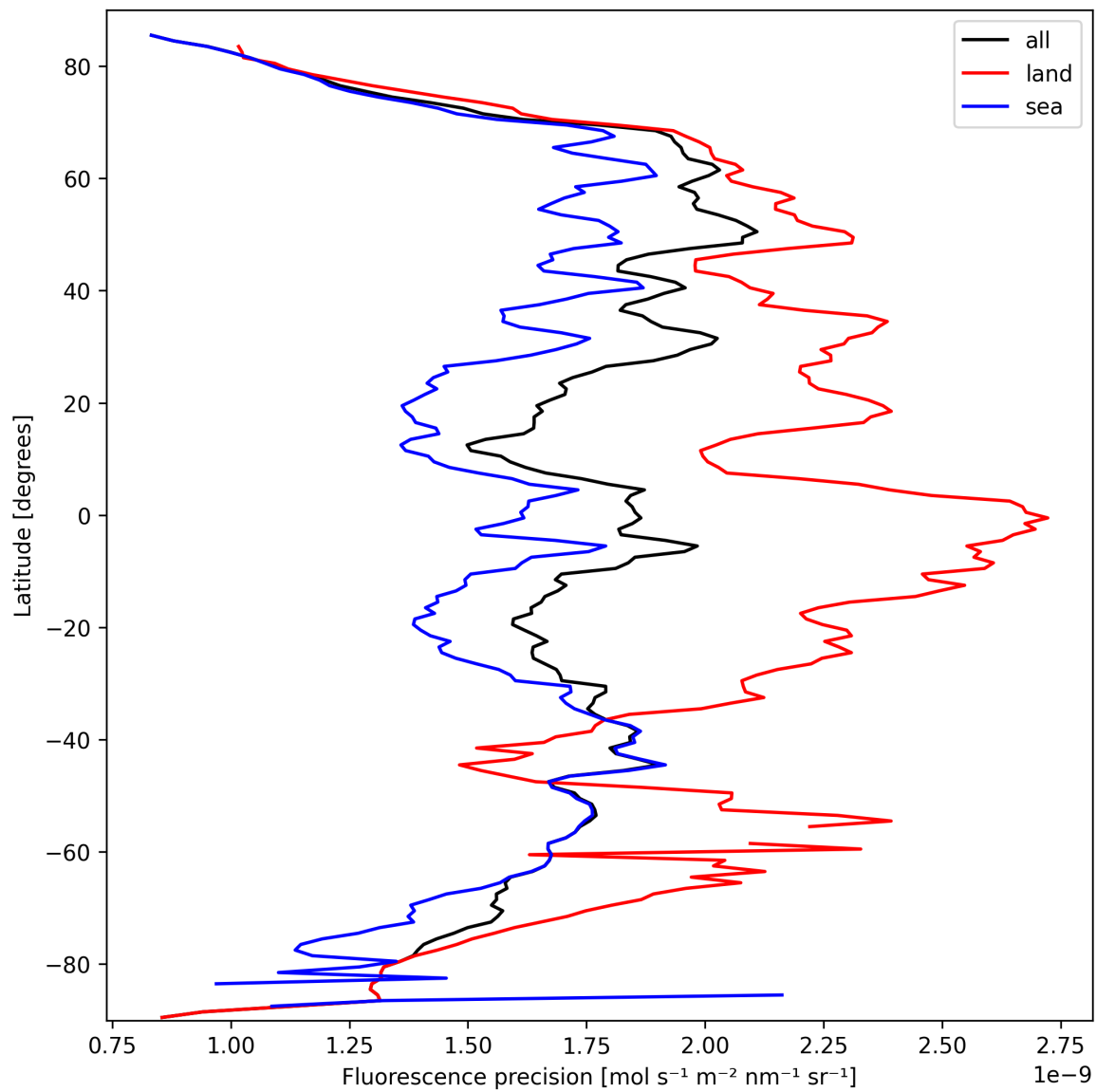
Figure 22: Zonal average of “Fluorescence precision” for 2025-03-14 to 2025-03-15.
