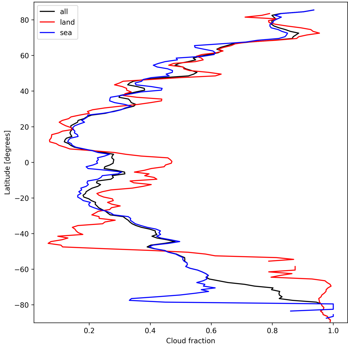
Figure 13: Zonal average of “Cloud fraction” for 2025-03-14 to 2025-03-15.
