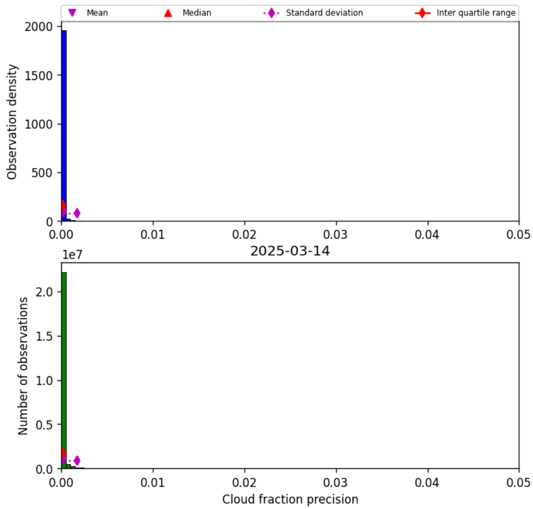
Figure 31: Histogram of “Cloud fraction precision” for 2025-03-14 to 2025-03-15
