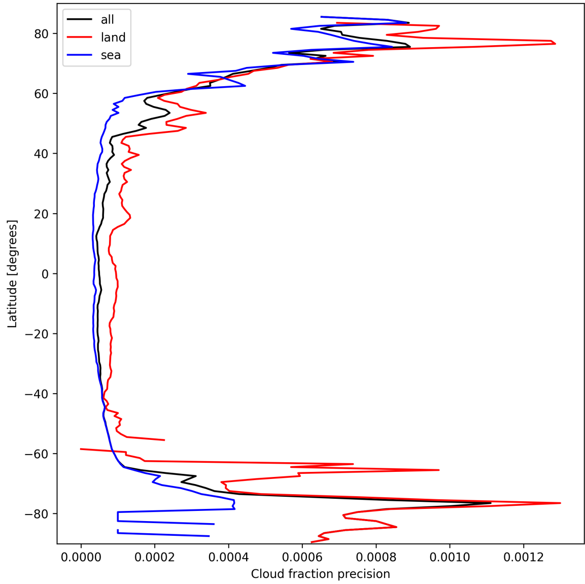
Figure 14: Zonal average of “Cloud fraction precision” for 2025-03-14 to 2025-03-15.
