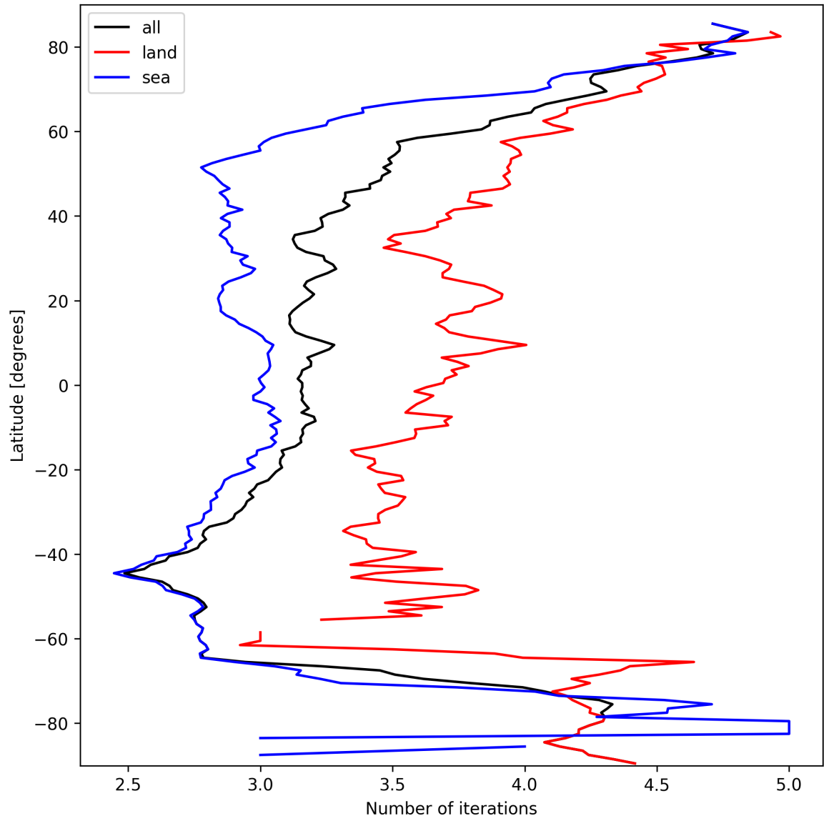
Figure 20: Zonal average of “Number of iterations” for 2025-03-14 to 2025-03-15.
