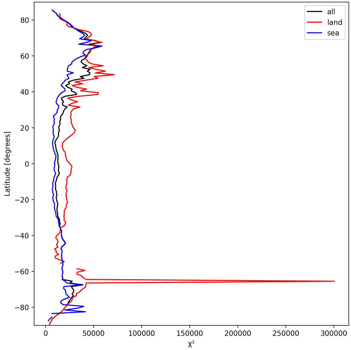
Figure 19: Zonal average of “ \chi^2 ” for 2025-03-14 to 2025-03-15.
