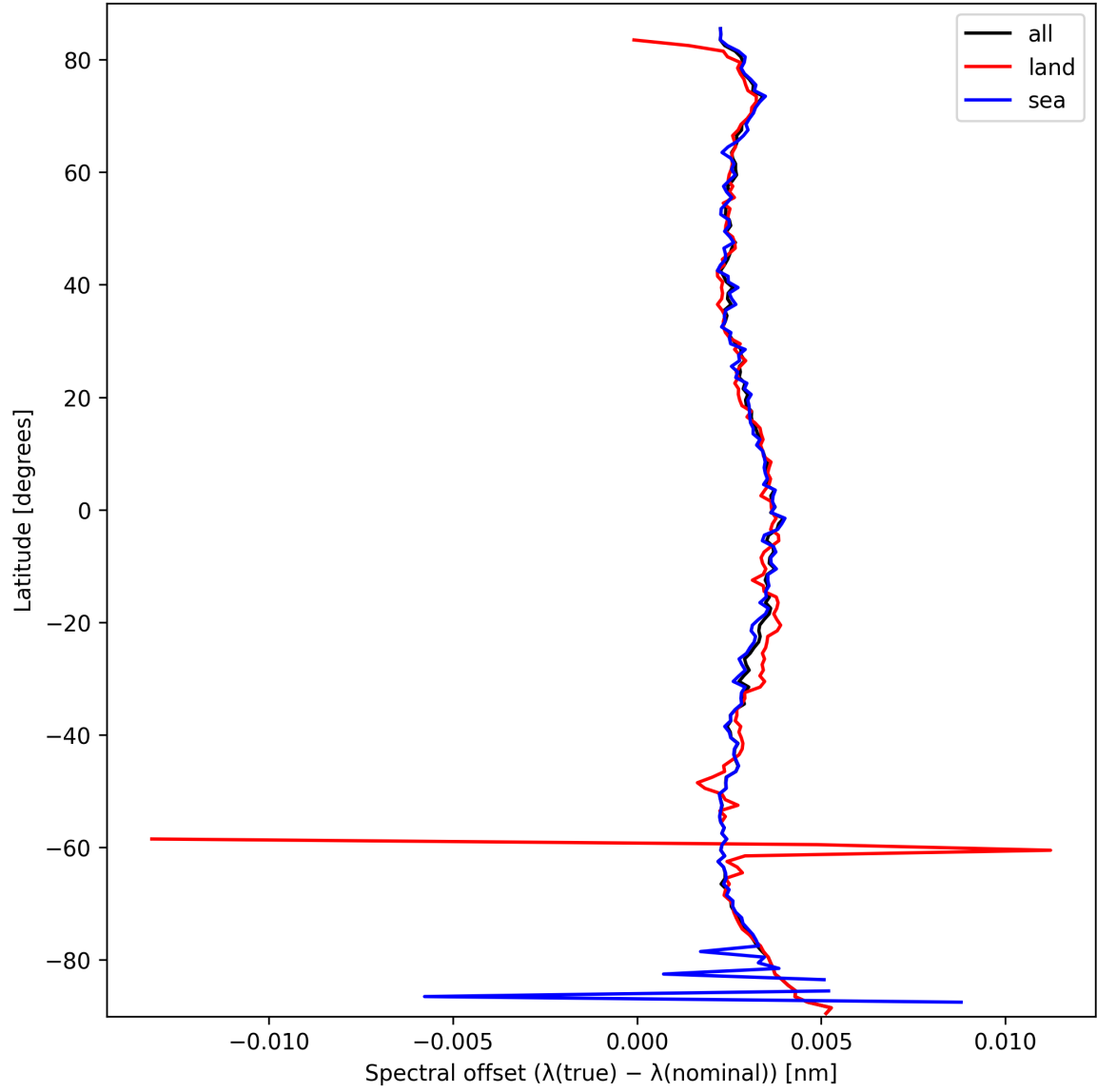
Figure 26: Zonal average of “Spectral offset ( \lambda_{\text{true}} - \lambda_{\text{nominal}} )” for 2025-03-14 to 2025-03-15.
