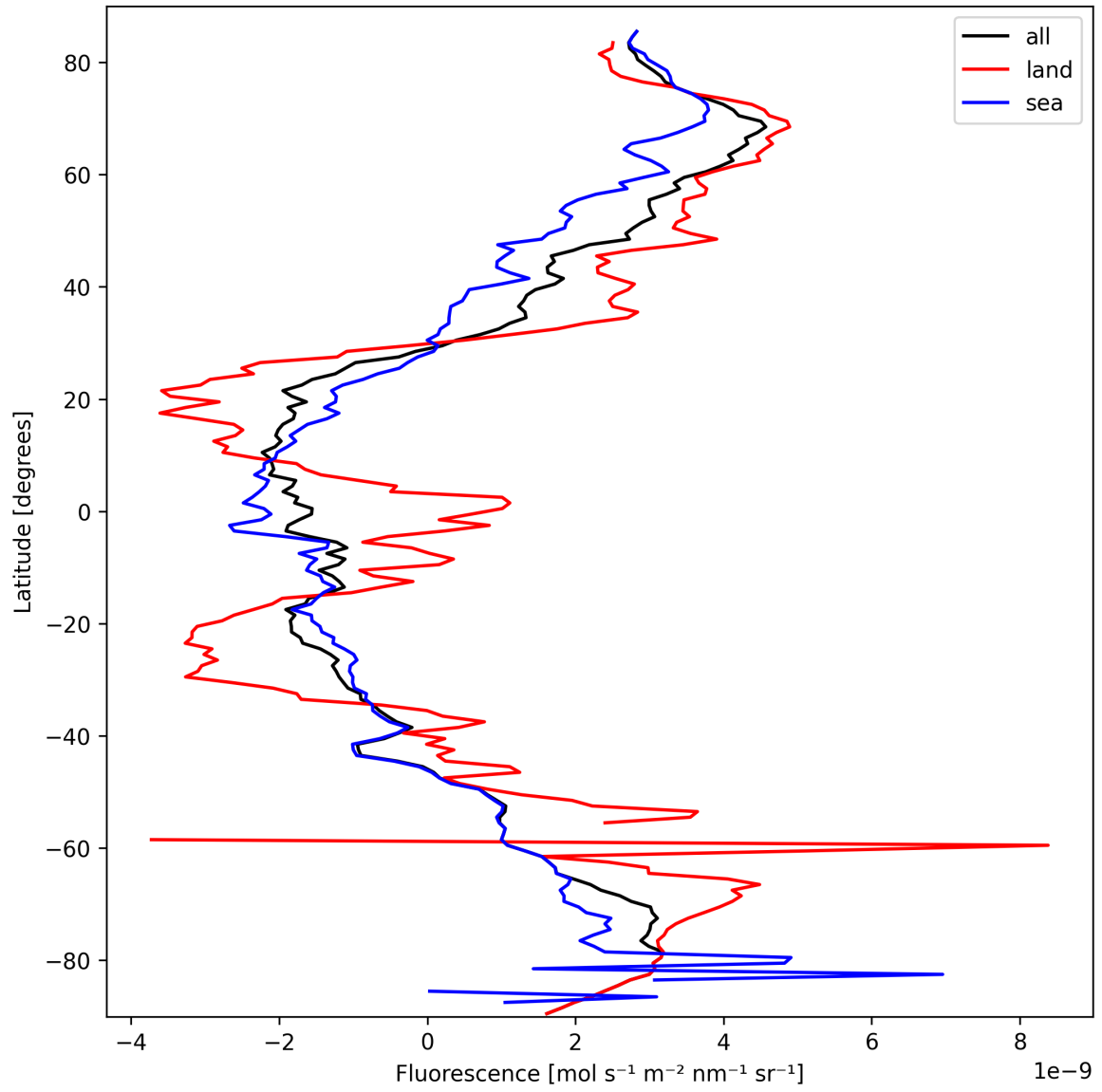
Figure 21: Zonal average of “Fluorescence” for 2025-03-14 to 2025-03-15.
