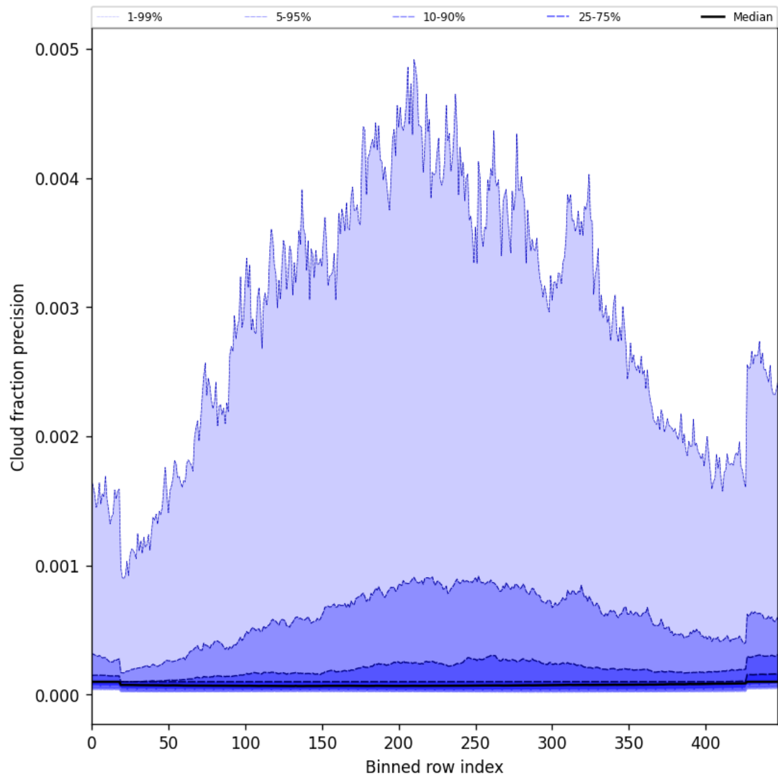
Figure 48: Along track statistics of “Cloud fraction precision” for 2025-03-14 to 2025-03-15
