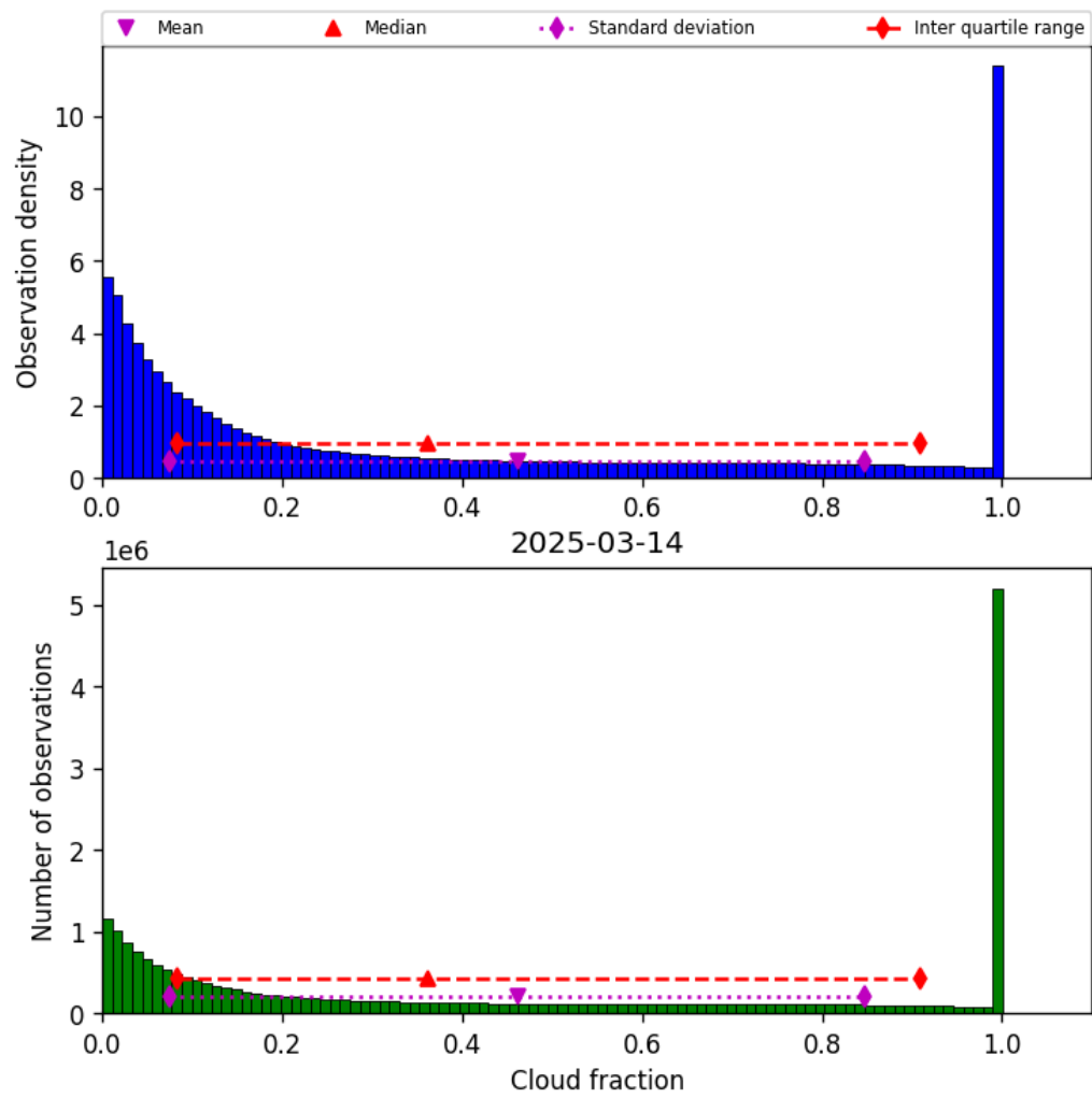
Figure 30: Histogram of “Cloud fraction” for 2025-03-14 to 2025-03-15
