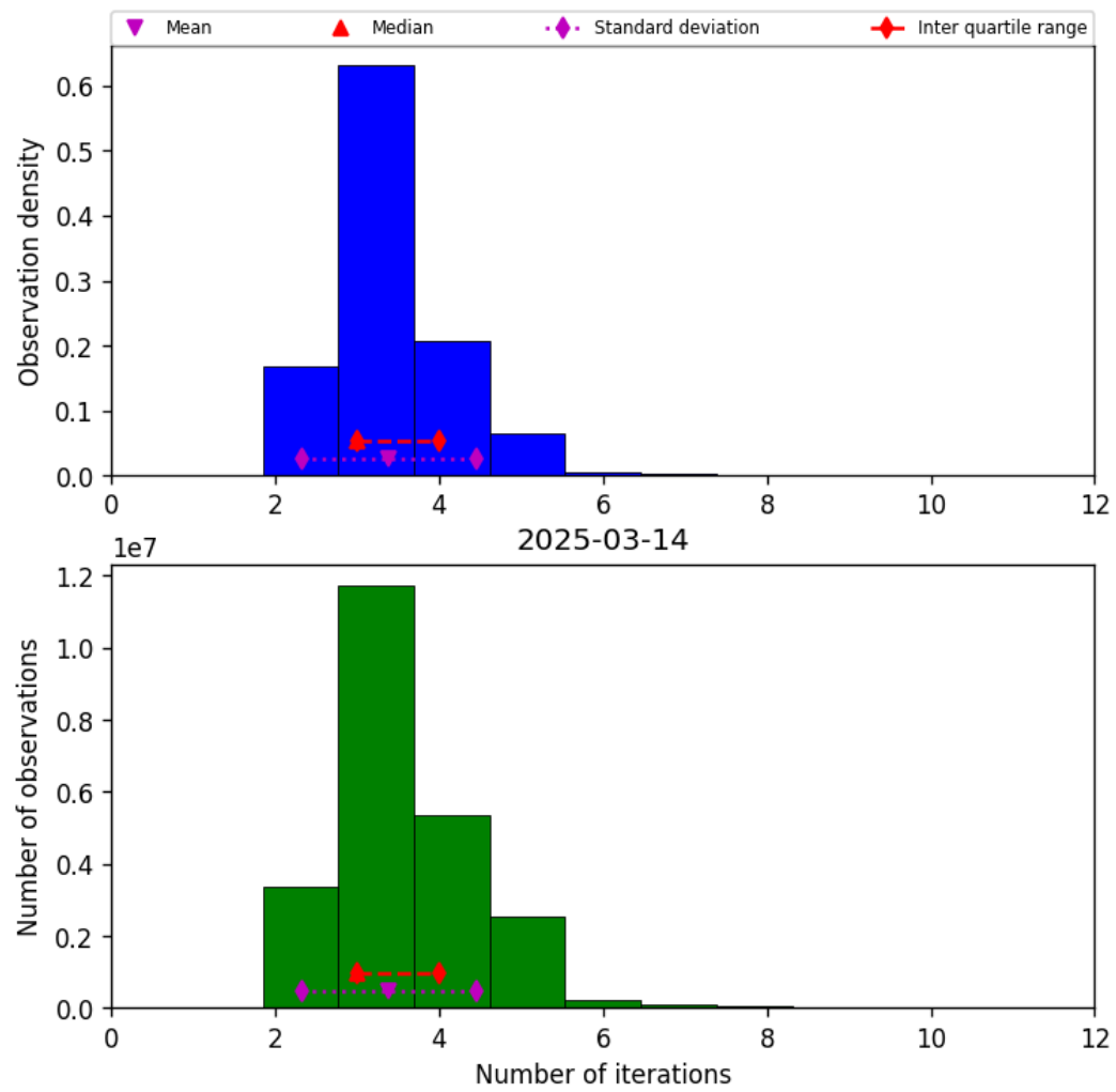
Figure 37: Histogram of “Number of iterations” for 2025-03-14 to 2025-03-15
