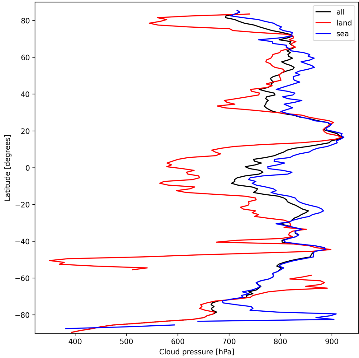
Figure 11: Zonal average of “Cloud pressure” for 2025-03-14 to 2025-03-15.
