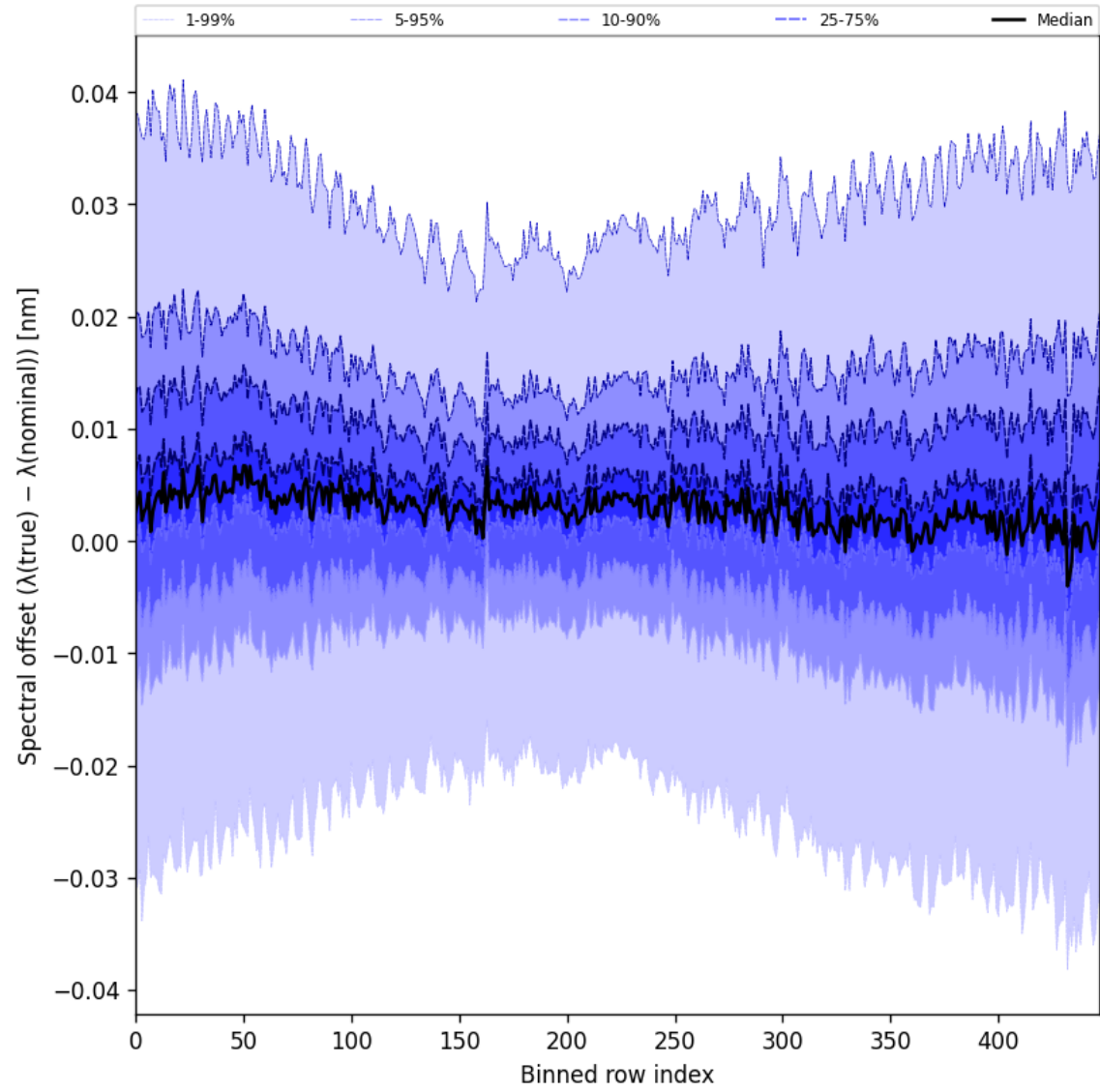
Figure 60: Along track statistics of “Spectral offset ( \lambda_{\text{true}} - \lambda_{\text{nominal}} )” for 2025-03-14 to 2025-03-15
