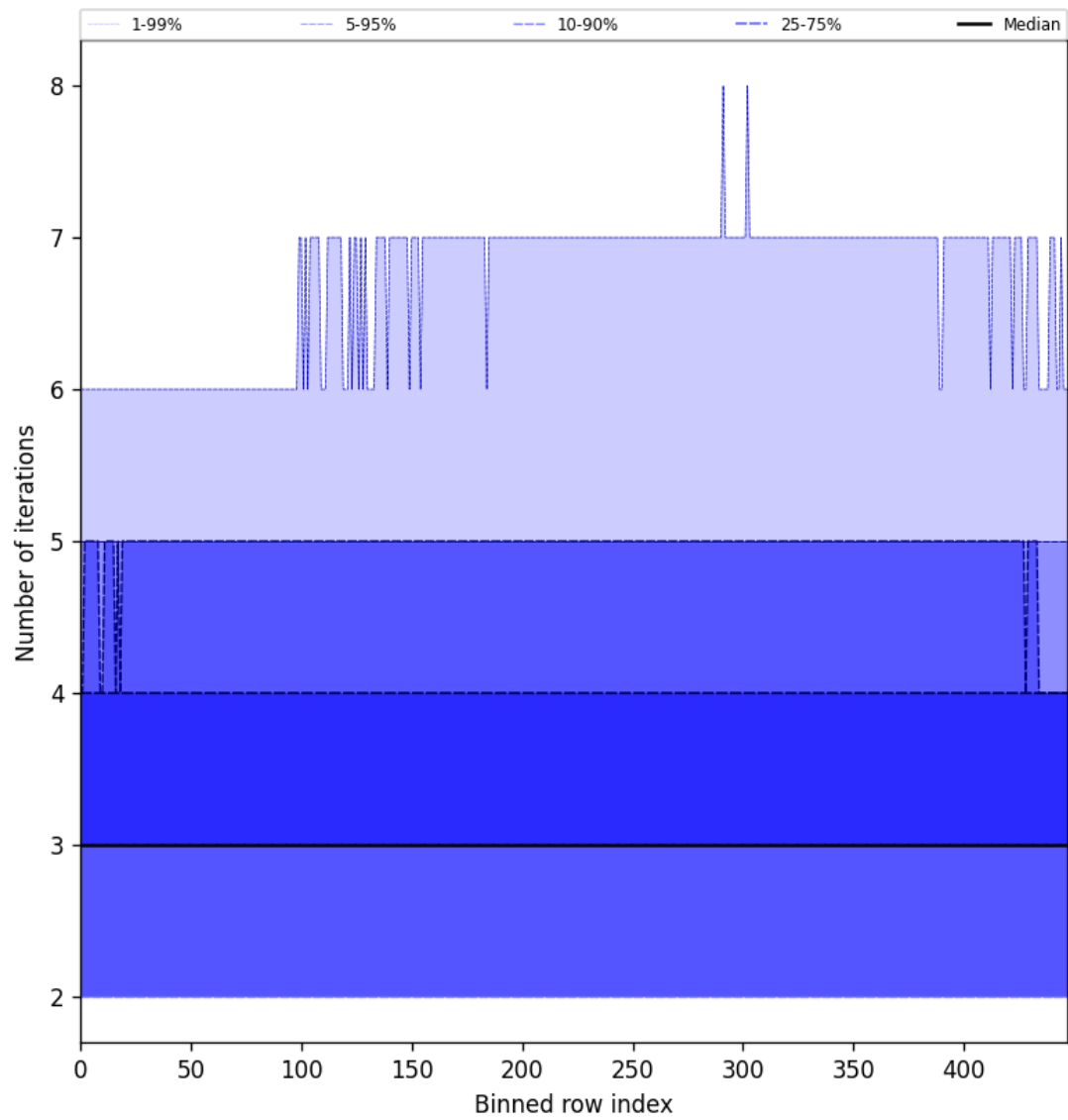
Figure 54: Along track statistics of “Number of iterations” for 2025-03-14 to 2025-03-15
