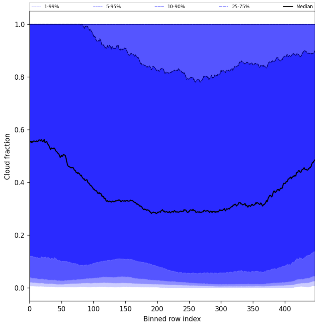
Figure 47: Along track statistics of “Cloud fraction” for 2025-03-14 to 2025-03-15
