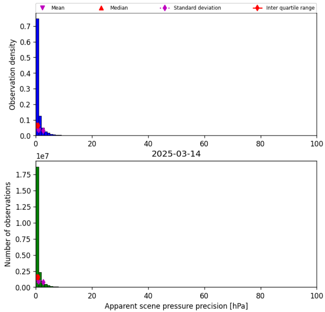
Figure 35: Histogram of “Apparent scene pressure precision” for 2025-03-14 to 2025-03-15
