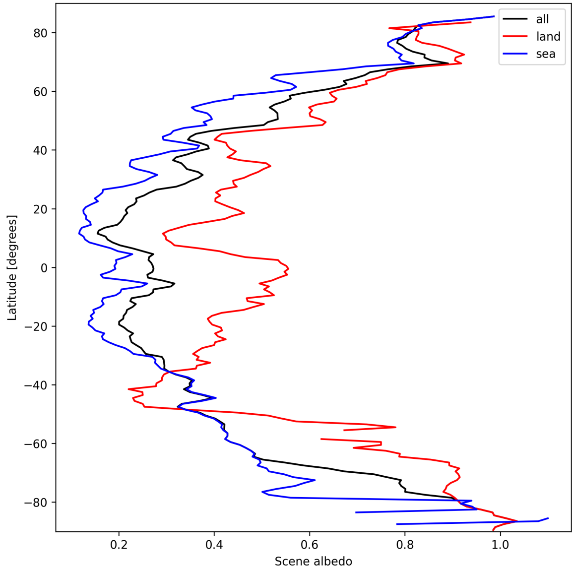
Figure 15: Zonal average of “Scene albedo” for 2025-03-14 to 2025-03-15.
