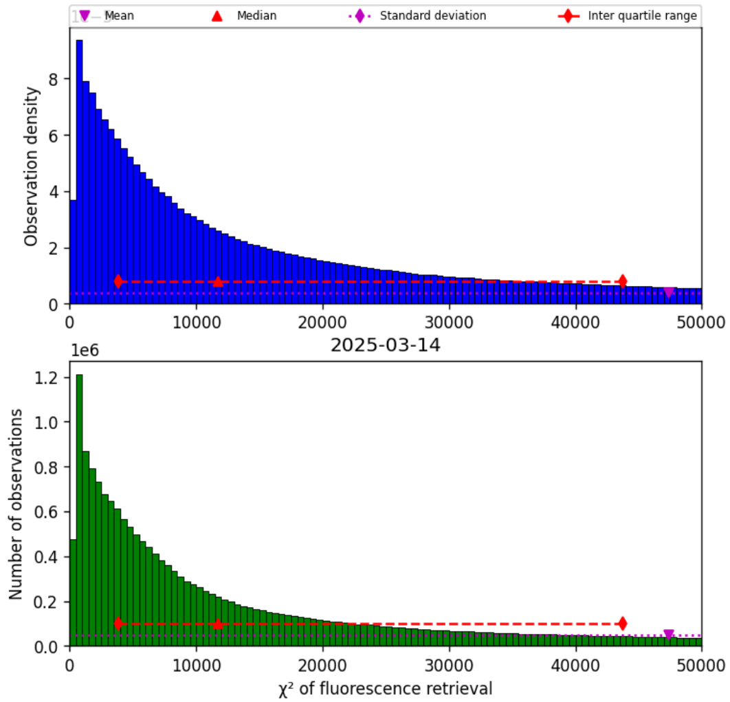
Figure 40: Histogram of “ \chi^2 of fluorescence retrieval” for 2025-03-14 to 2025-03-15
