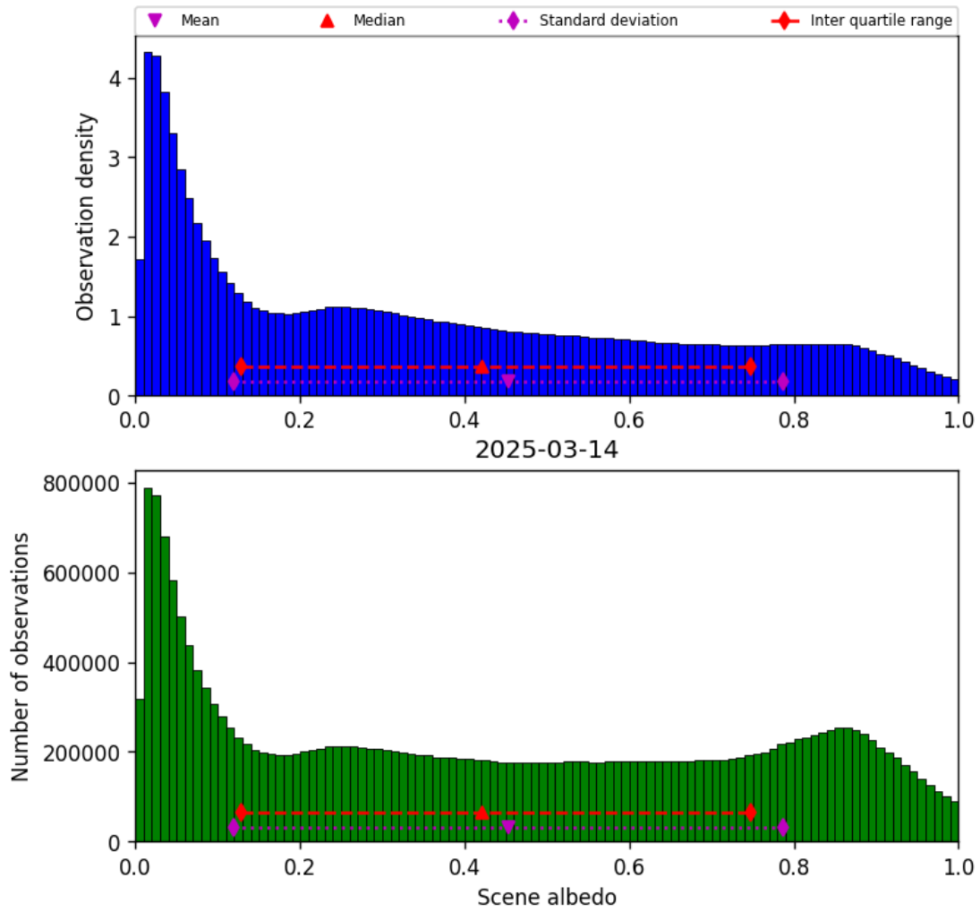
Figure 32: Histogram of “Scene albedo” for 2025-03-14 to 2025-03-15
