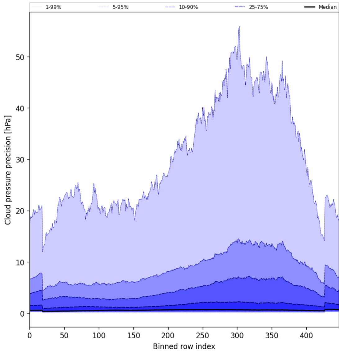
Figure 46: Along track statistics of “Cloud pressure precision” for 2025-03-14 to 2025-03-15
