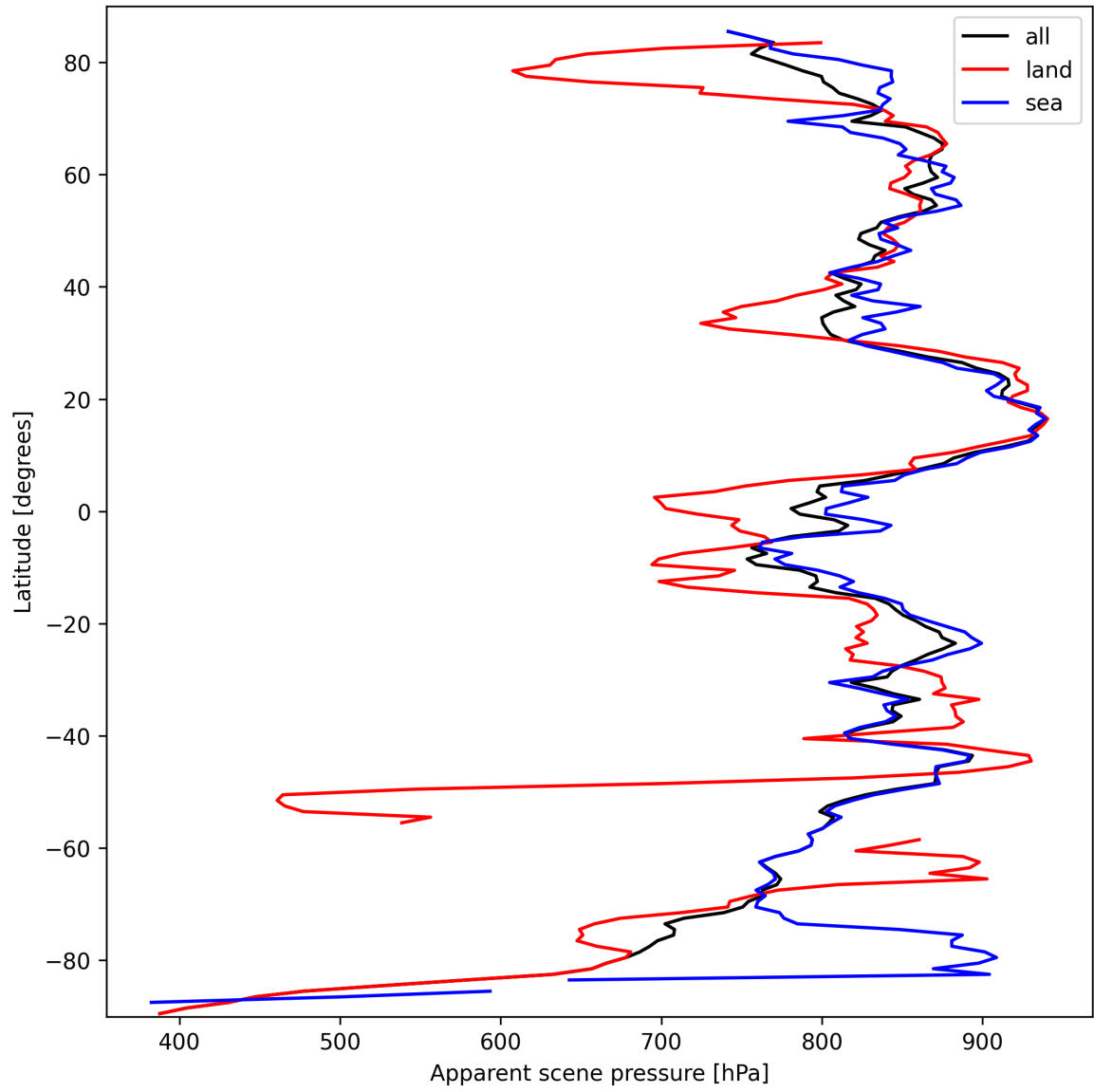
Figure 17: Zonal average of “Apparent scene pressure” for 2025-03-14 to 2025-03-15.
