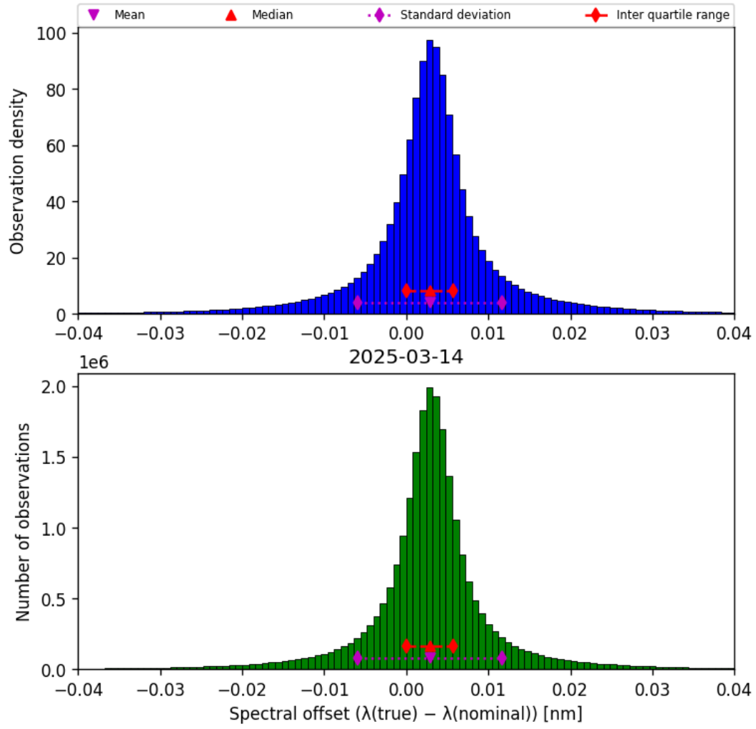
Figure 43: Histogram of “Spectral offset ( \lambda_{\text{true}} - \lambda_{\text{nominal}} )” for 2025-03-14 to 2025-03-15
