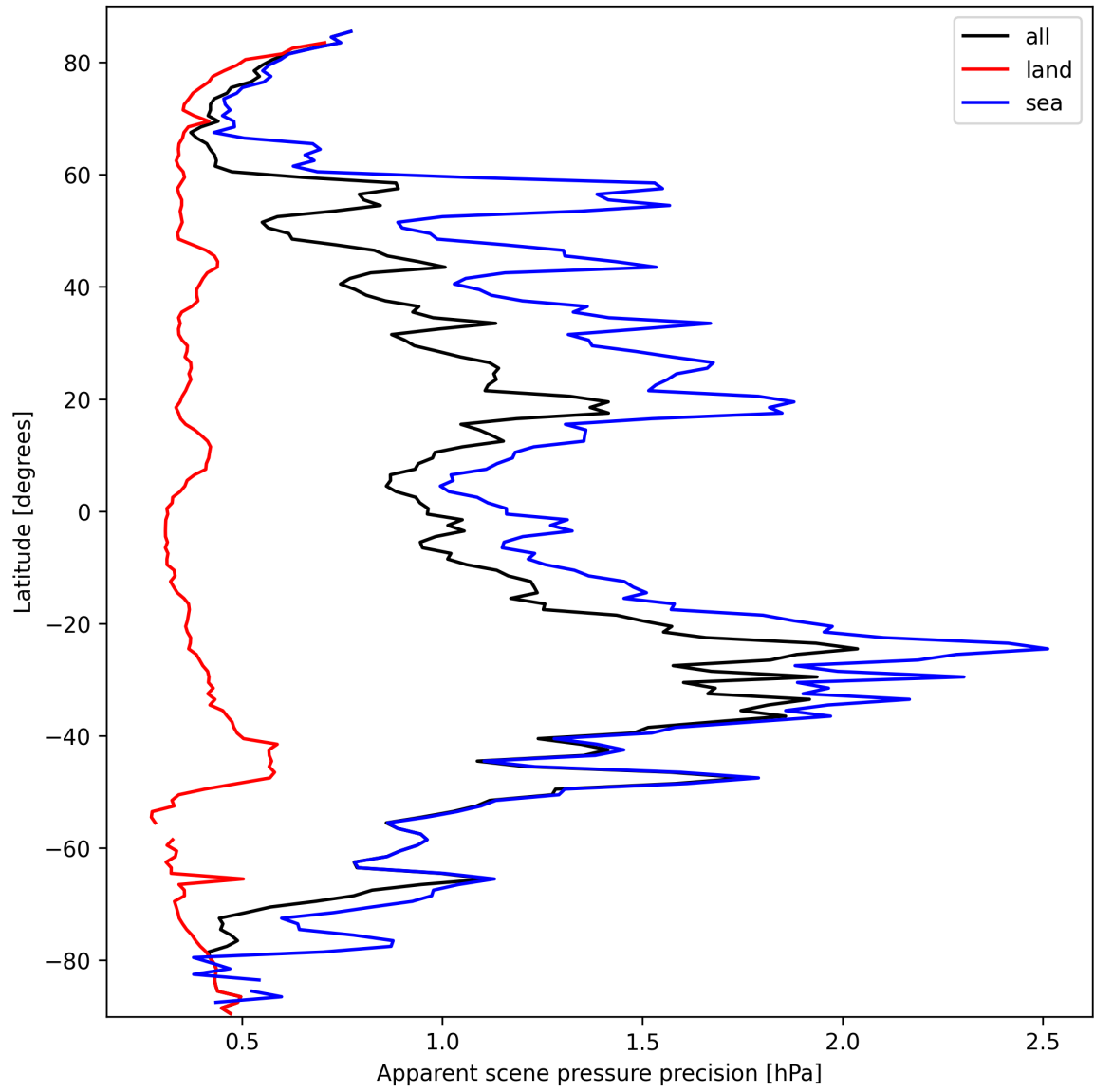
Figure 18: Zonal average of “Apparent scene pressure precision” for 2025-03-14 to 2025-03-15.
