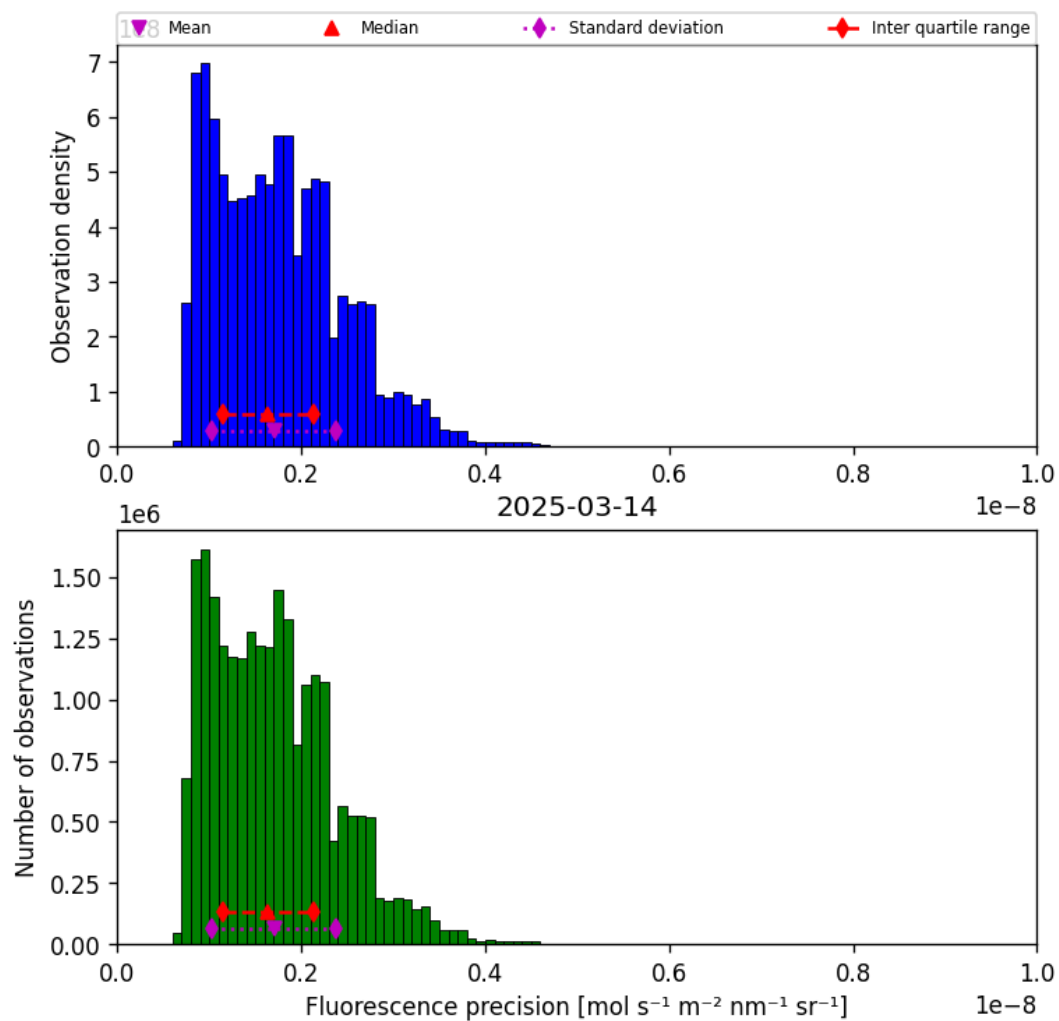
Figure 39: Histogram of “Fluorescence precision” for 2025-03-14 to 2025-03-15
