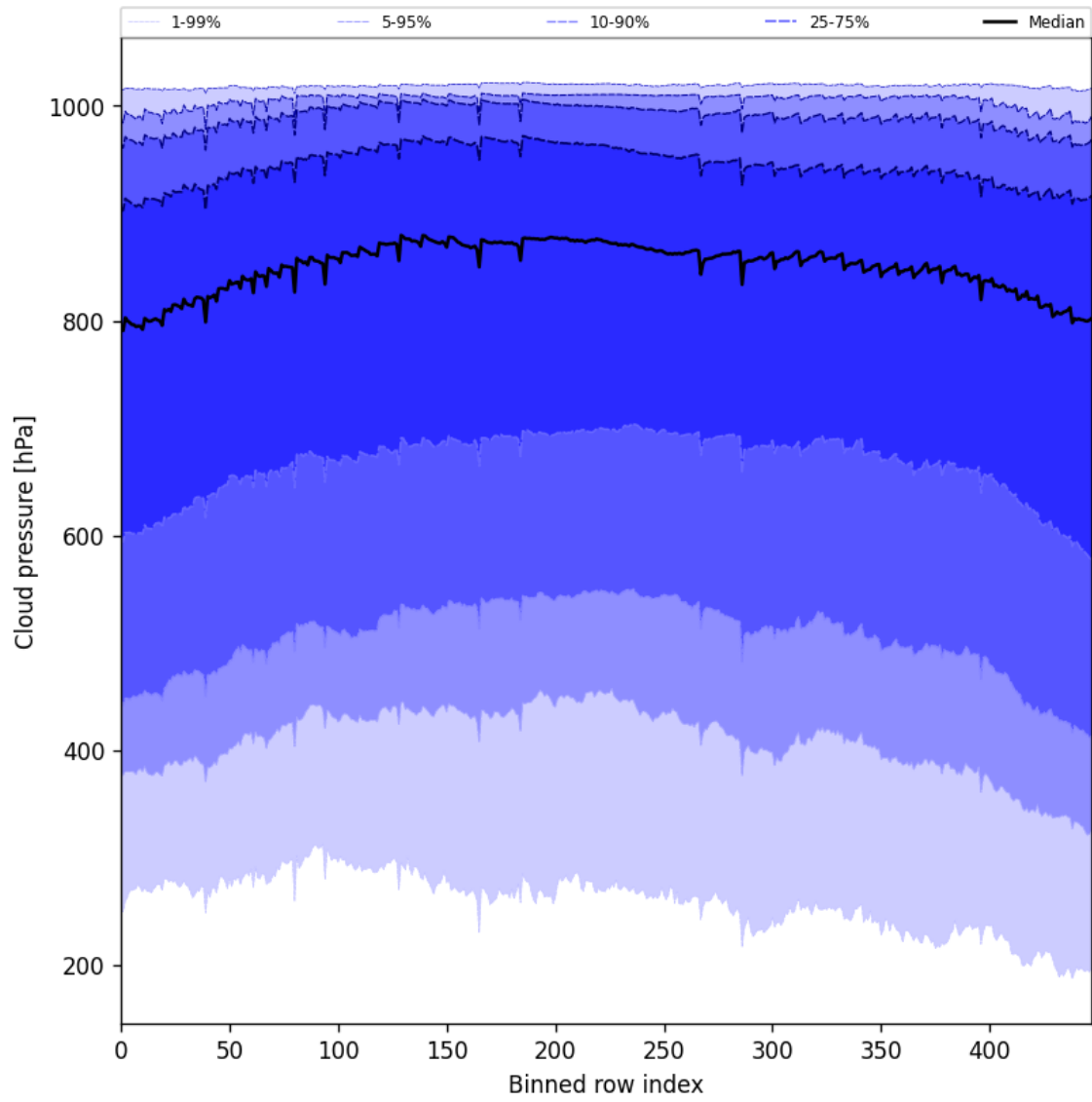
Figure 45: Along track statistics of “Cloud pressure” for 2025-03-14 to 2025-03-15
