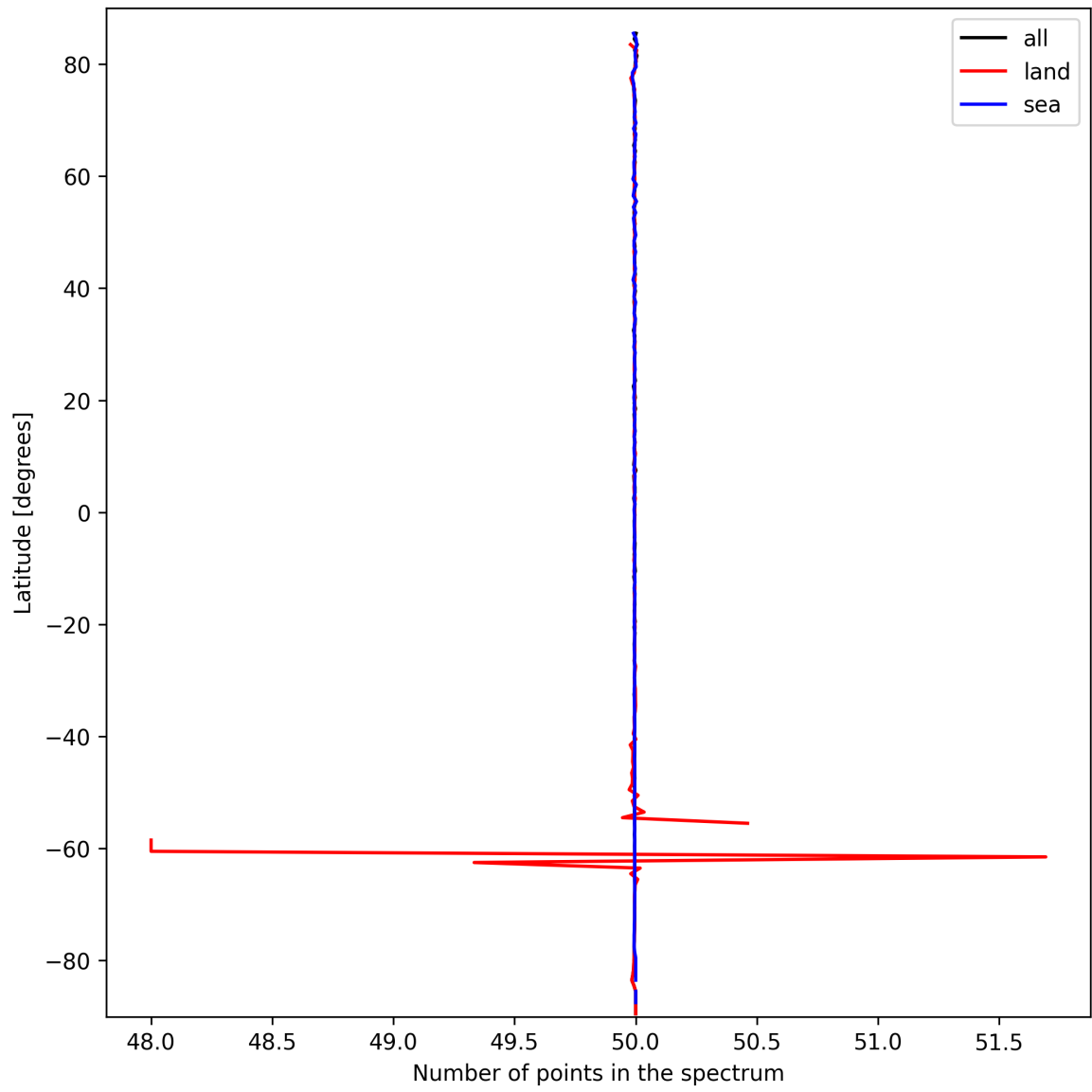
Figure 25: Zonal average of “Number of points in the spectrum” for 2025-03-14 to 2025-03-15.
