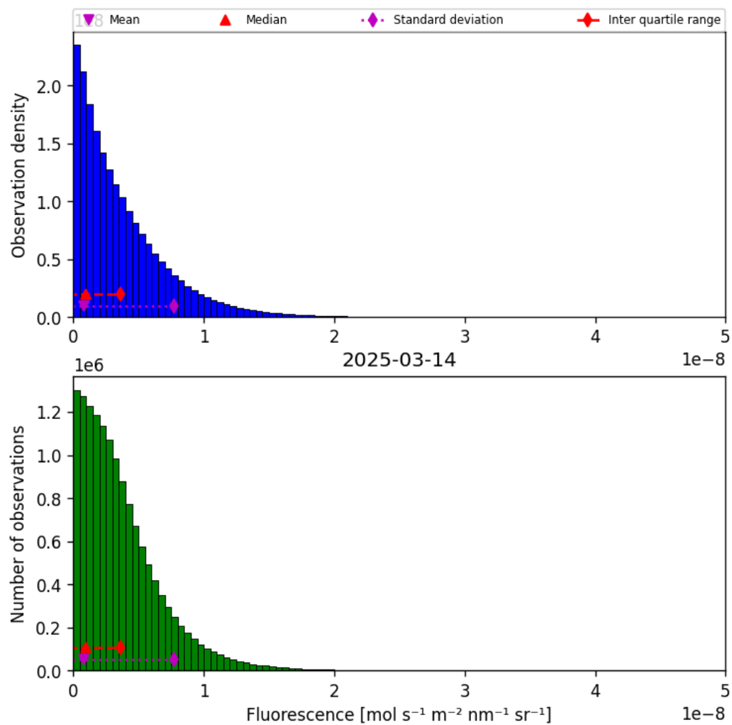
Figure 38: Histogram of “Fluorescence” for 2025-03-14 to 2025-03-15
