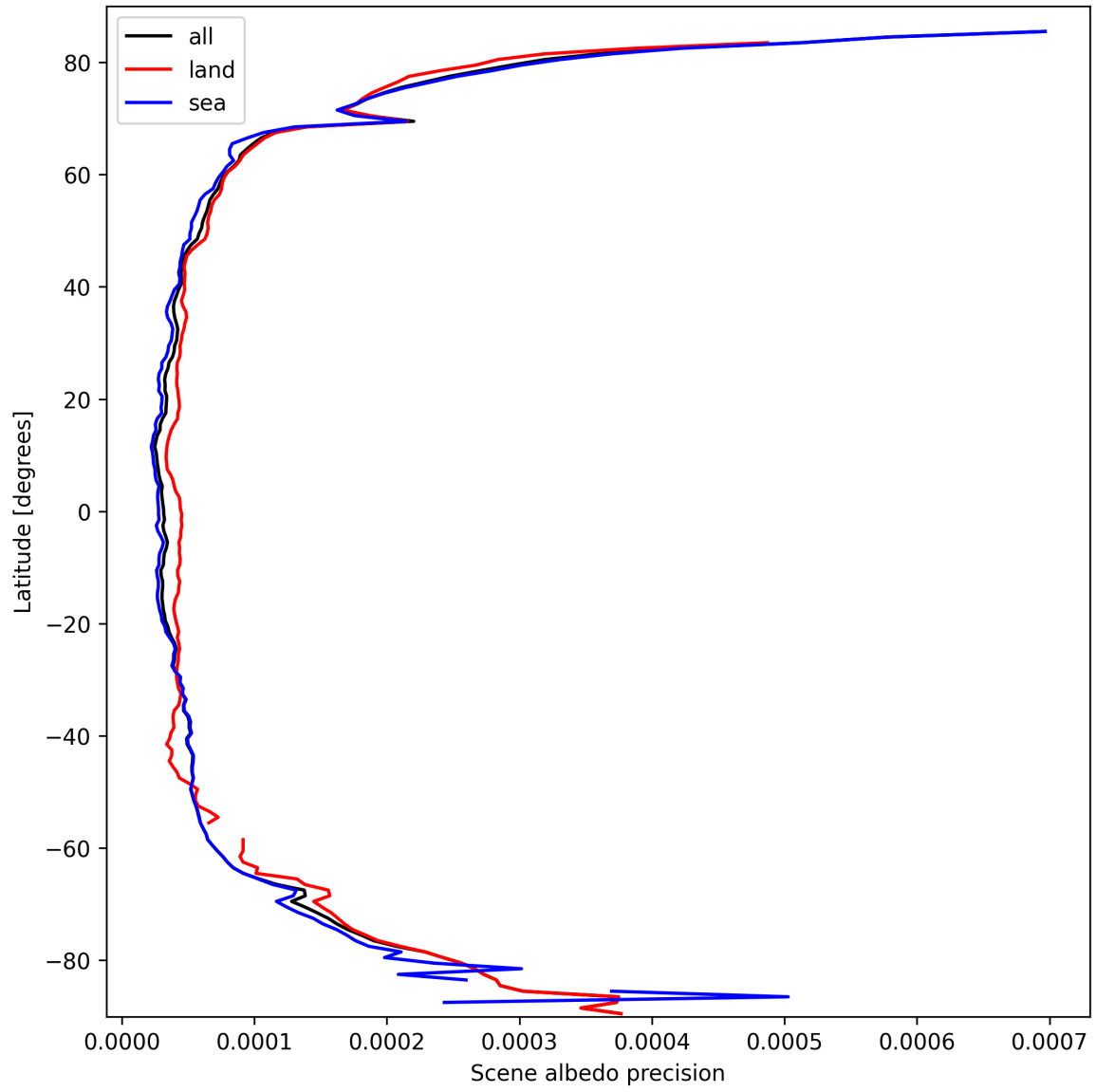
Figure 16: Zonal average of “Scene albedo precision” for 2025-03-14 to 2025-03-15.
