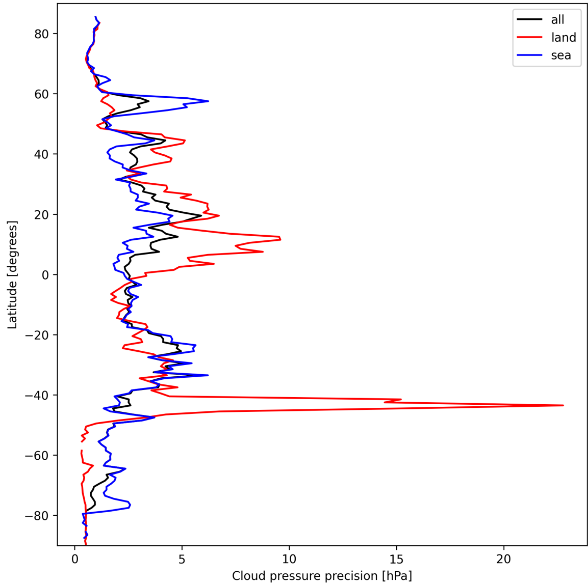
Figure 12: Zonal average of “Cloud pressure precision” for 2025-03-14 to 2025-03-15.
