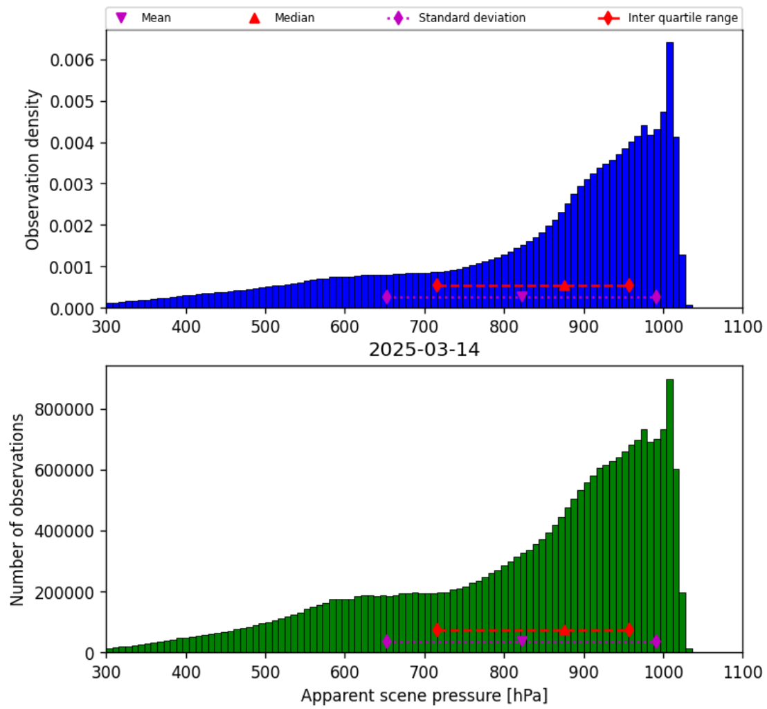
Figure 34: Histogram of “Apparent scene pressure” for 2025-03-14 to 2025-03-15
