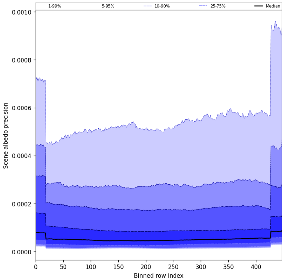
Figure 50: Along track statistics of “Scene albedo precision” for 2025-03-14 to 2025-03-15
