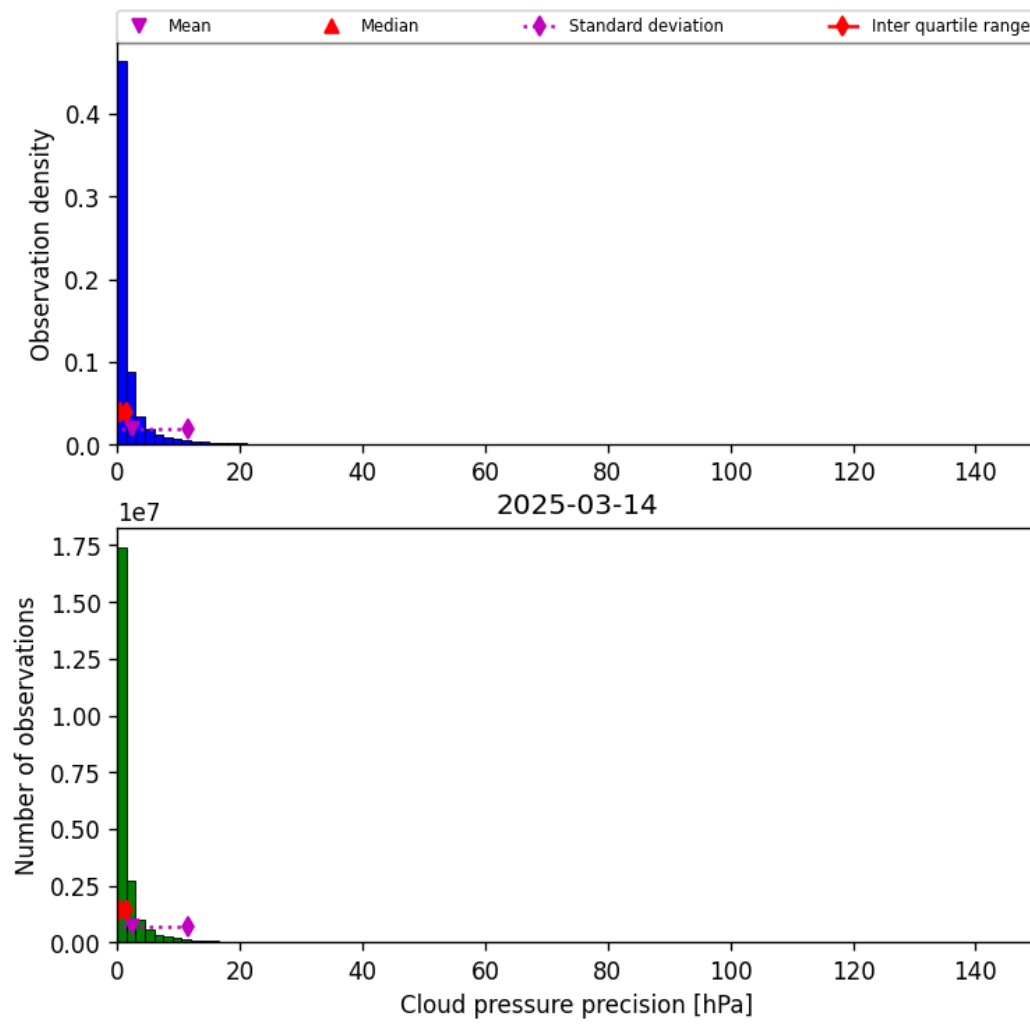
Figure 29: Histogram of “Cloud pressure precision” for 2025-03-14 to 2025-03-15
