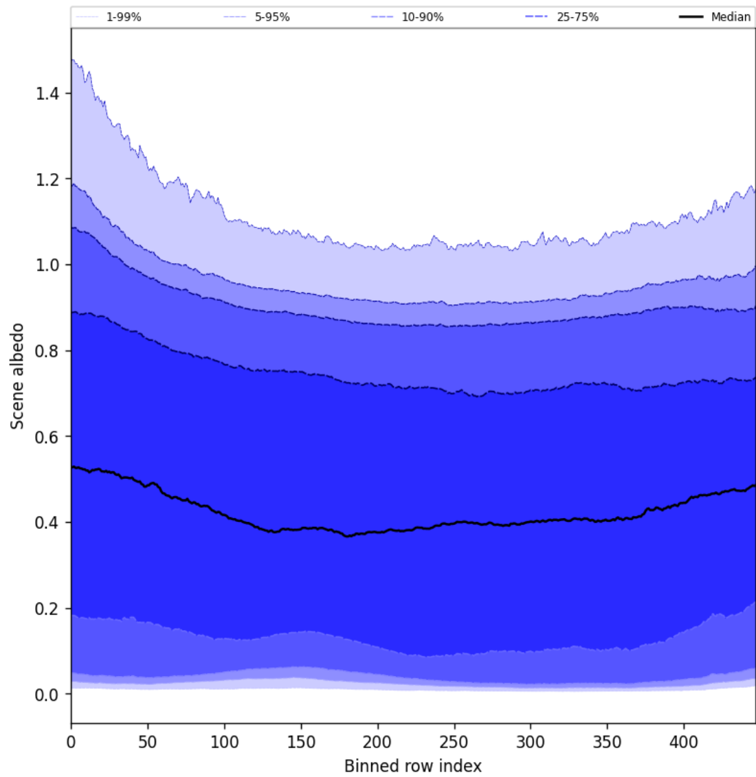
Figure 49: Along track statistics of “Scene albedo” for 2025-03-14 to 2025-03-15
