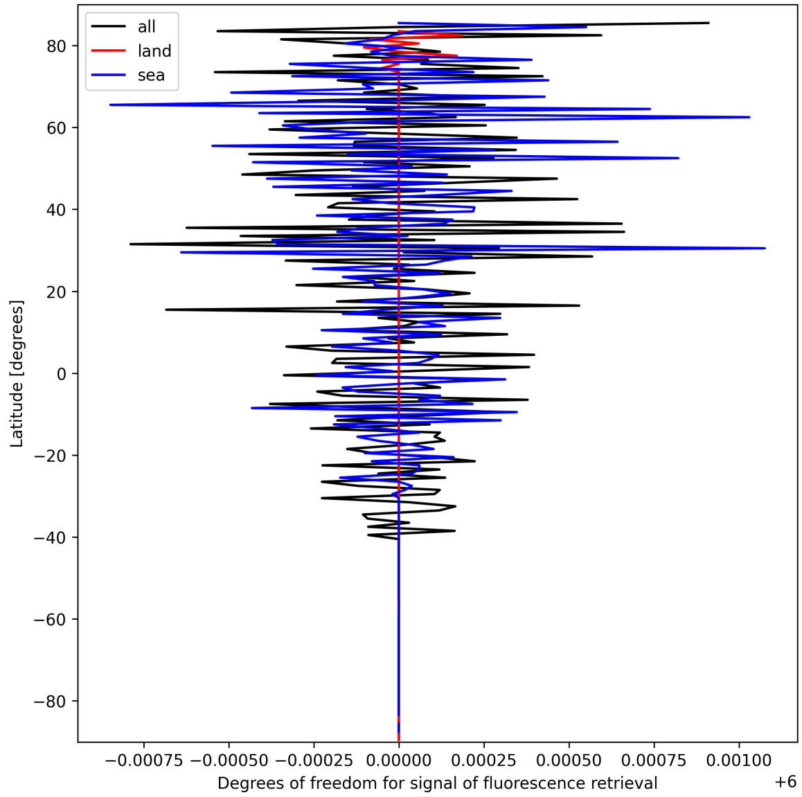
Figure 24: Zonal average of “Degrees of freedom for signal of fluorescence retrieval” for 2025-03-14 to 2025-03-15.
