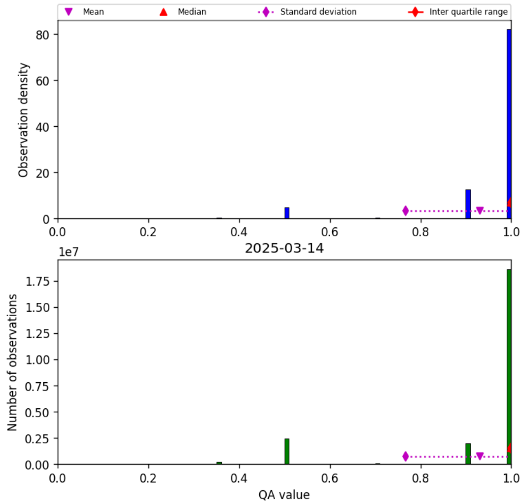
Figure 27: Histogram of “QA value” for 2025-03-14 to 2025-03-15
