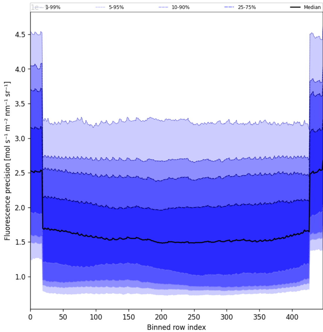
Figure 56: Along track statistics of “Fluorescence precision” for 2025-03-14 to 2025-03-15
