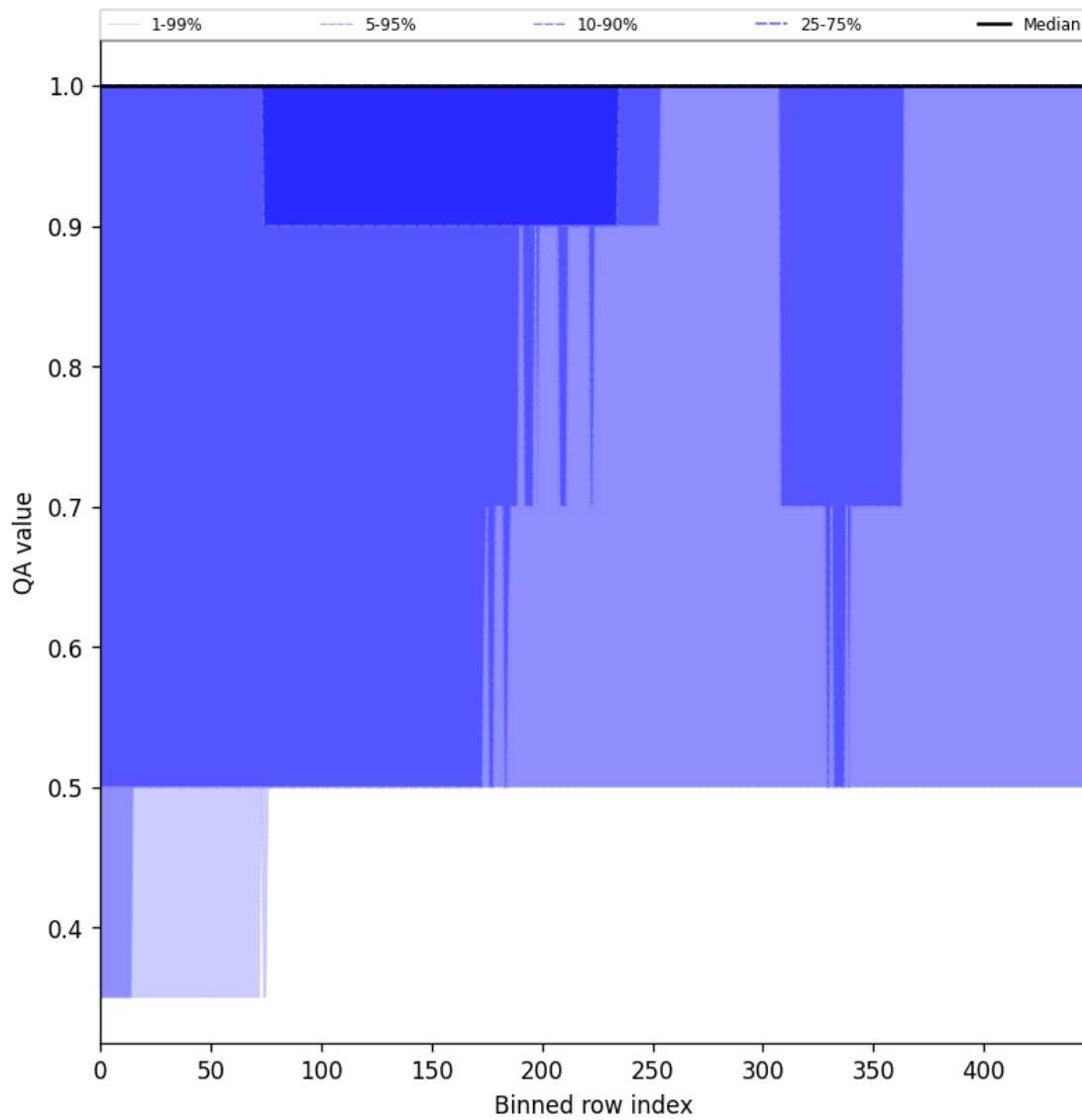
Figure 44: Along track statistics of “QA value” for 2025-03-14 to 2025-03-15
