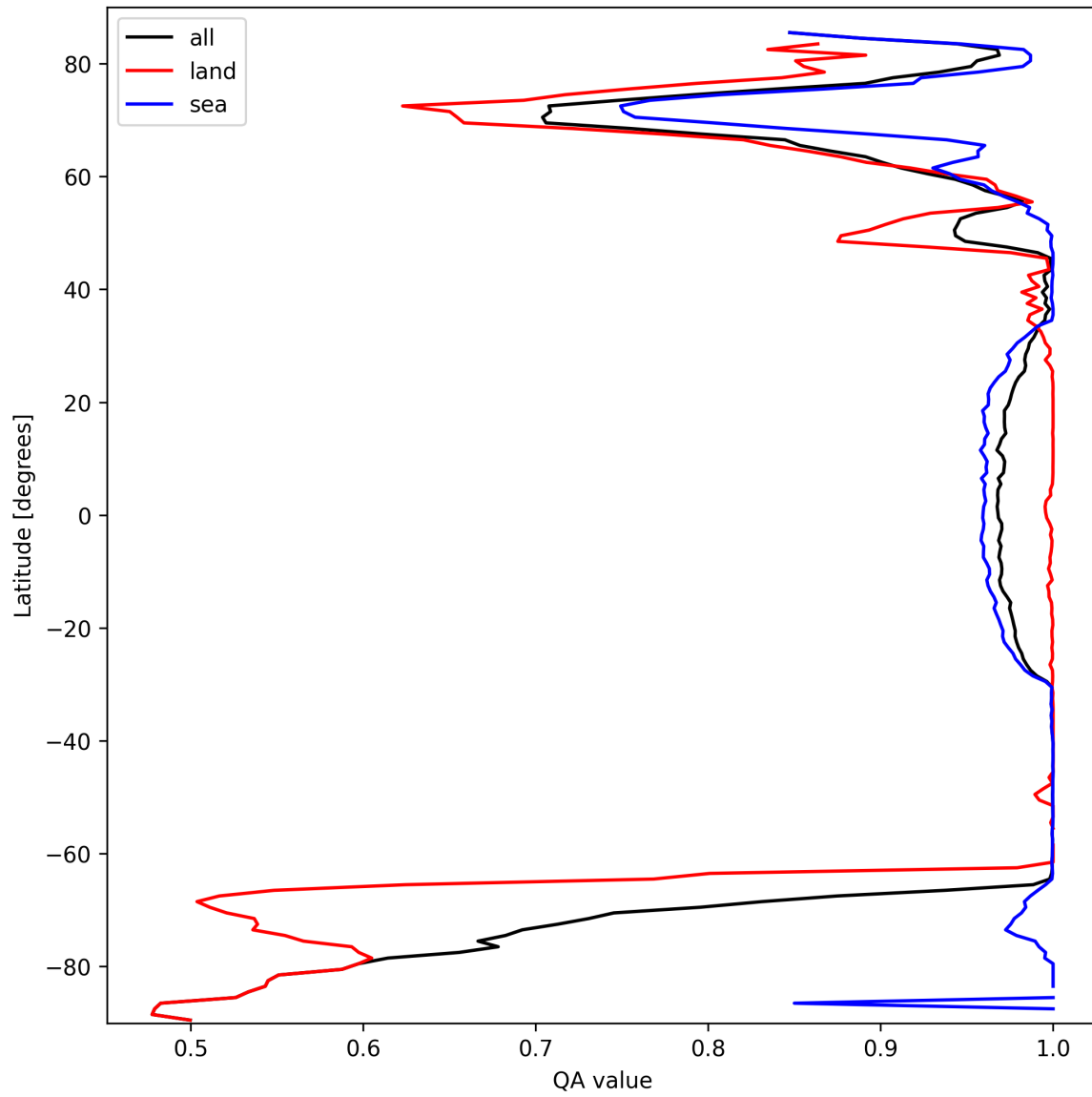
Figure 10: Zonal average of "QA value" for 2025-03-14 to 2025-03-15.
