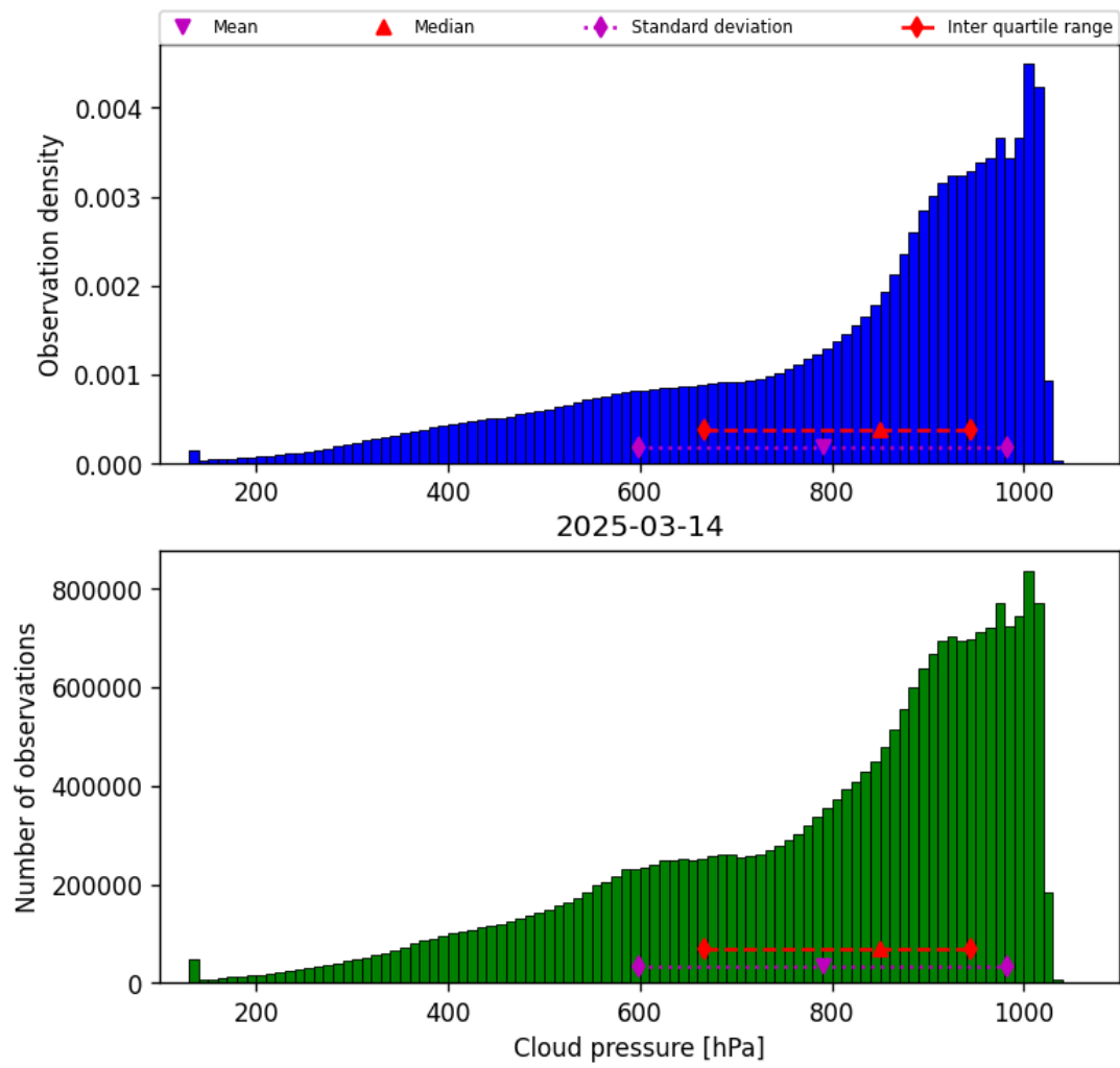
Figure 28: Histogram of “Cloud pressure” for 2025-03-14 to 2025-03-15
