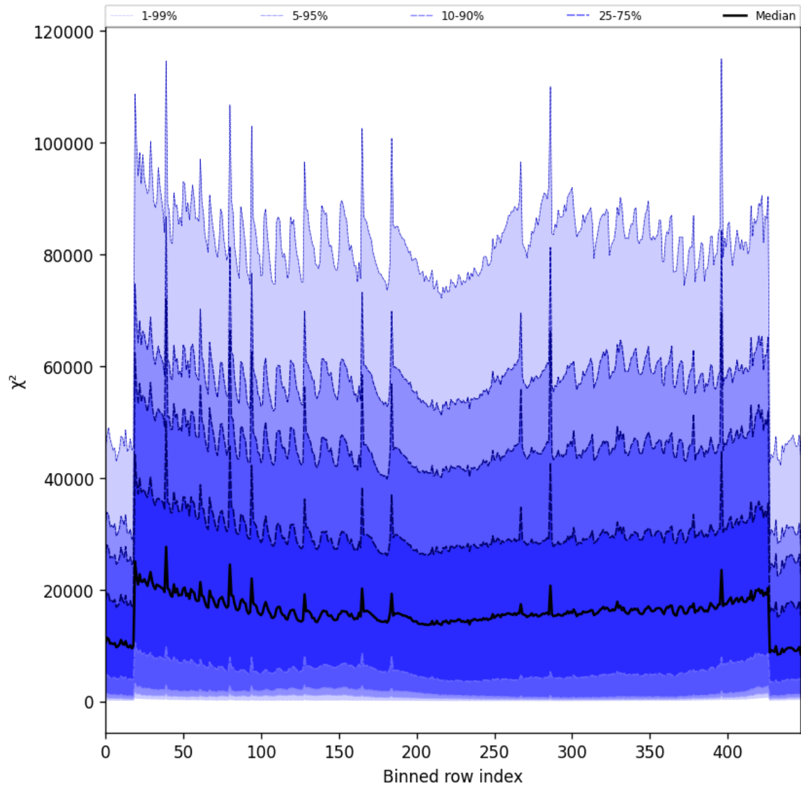
Figure 53: Along track statistics of “ \chi^2 ” for 2025-03-14 to 2025-03-15
