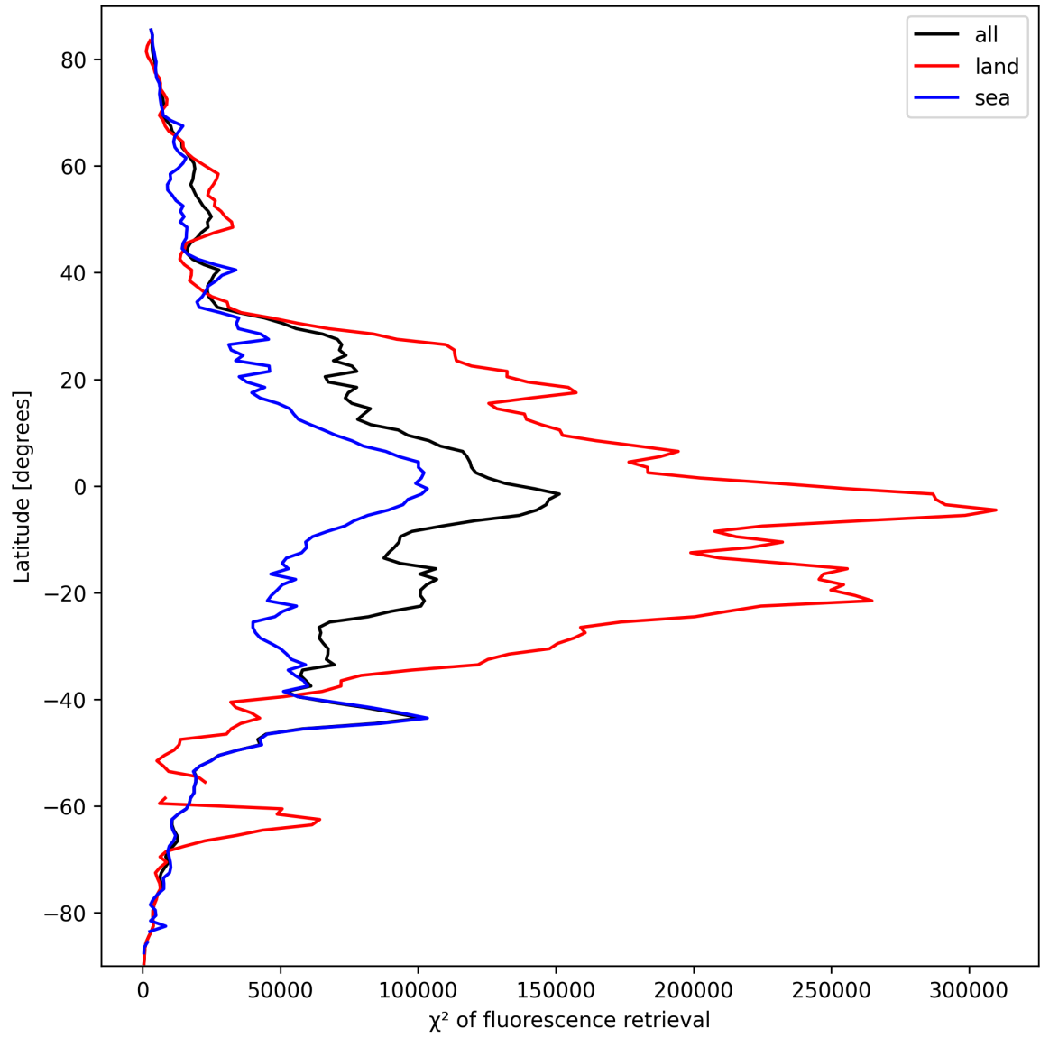
Figure 23: Zonal average of “ \chi^2 of fluorescence retrieval” for 2025-03-14 to 2025-03-15.
