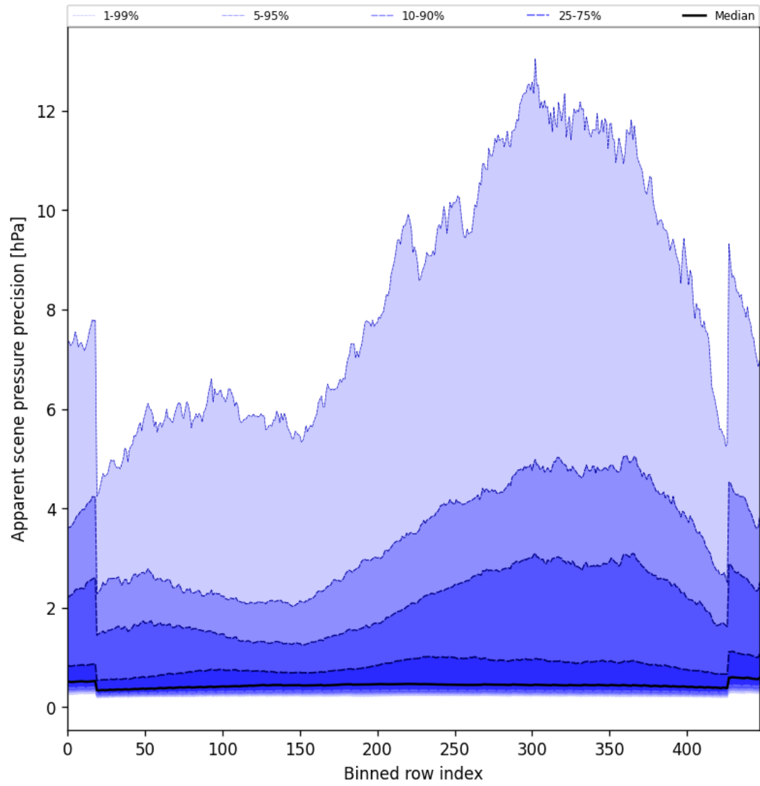
Figure 52: Along track statistics of “Apparent scene pressure precision” for 2025-03-14 to 2025-03-15
