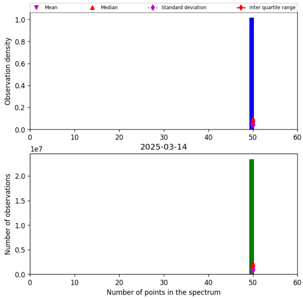
Figure 42: Histogram of “Number of points in the spectrum” for 2025-03-14 to 2025-03-15
