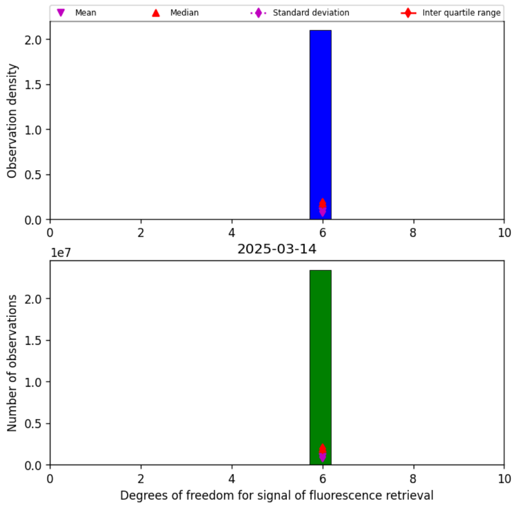
Figure 41: Histogram of “Degrees of freedom for signal of fluorescence retrieval” for 2025-03-14 to 2025-03-15
