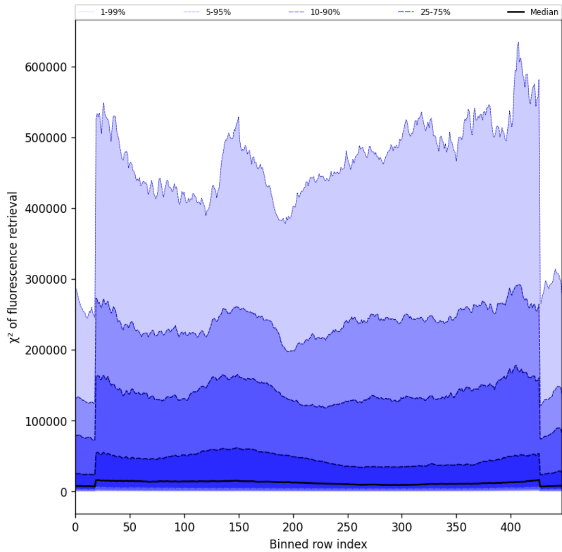
Figure 57: Along track statistics of “ \chi^2 of fluorescence retrieval” for 2025-03-14 to 2025-03-15
