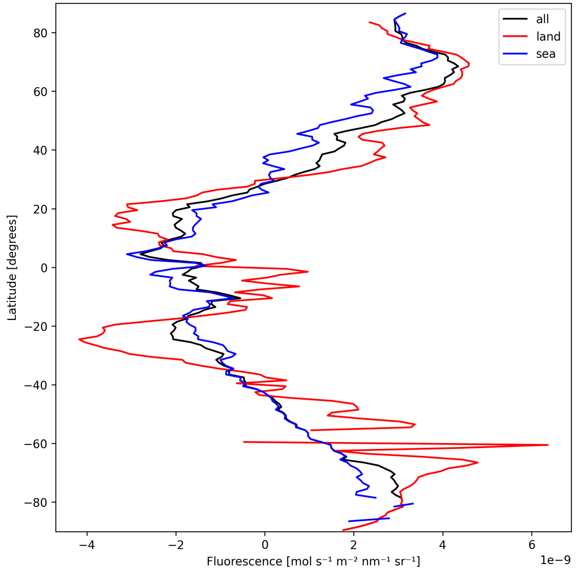
Figure 21: Zonal average of “Fluorescence” for 2025-03-15 to 2025-03-15.
