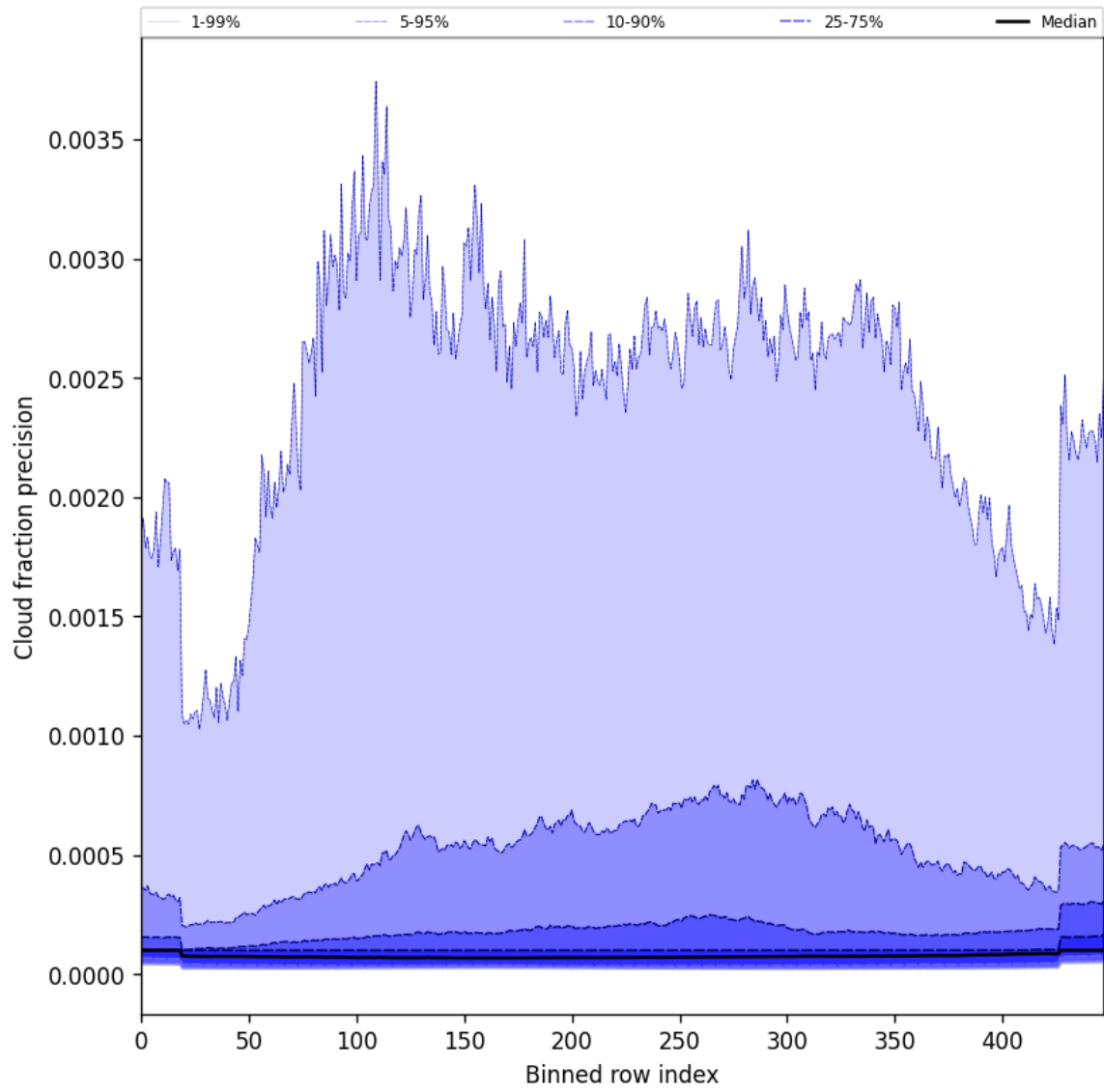
Figure 48: Along track statistics of “Cloud fraction precision” for 2025-03-15 to 2025-03-15
