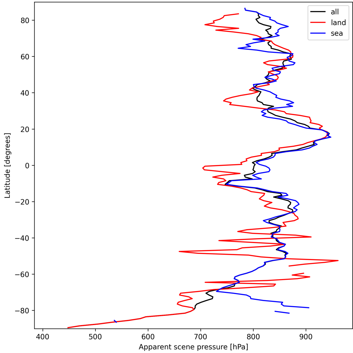
Figure 17: Zonal average of “Apparent scene pressure” for 2025-03-15 to 2025-03-15.
