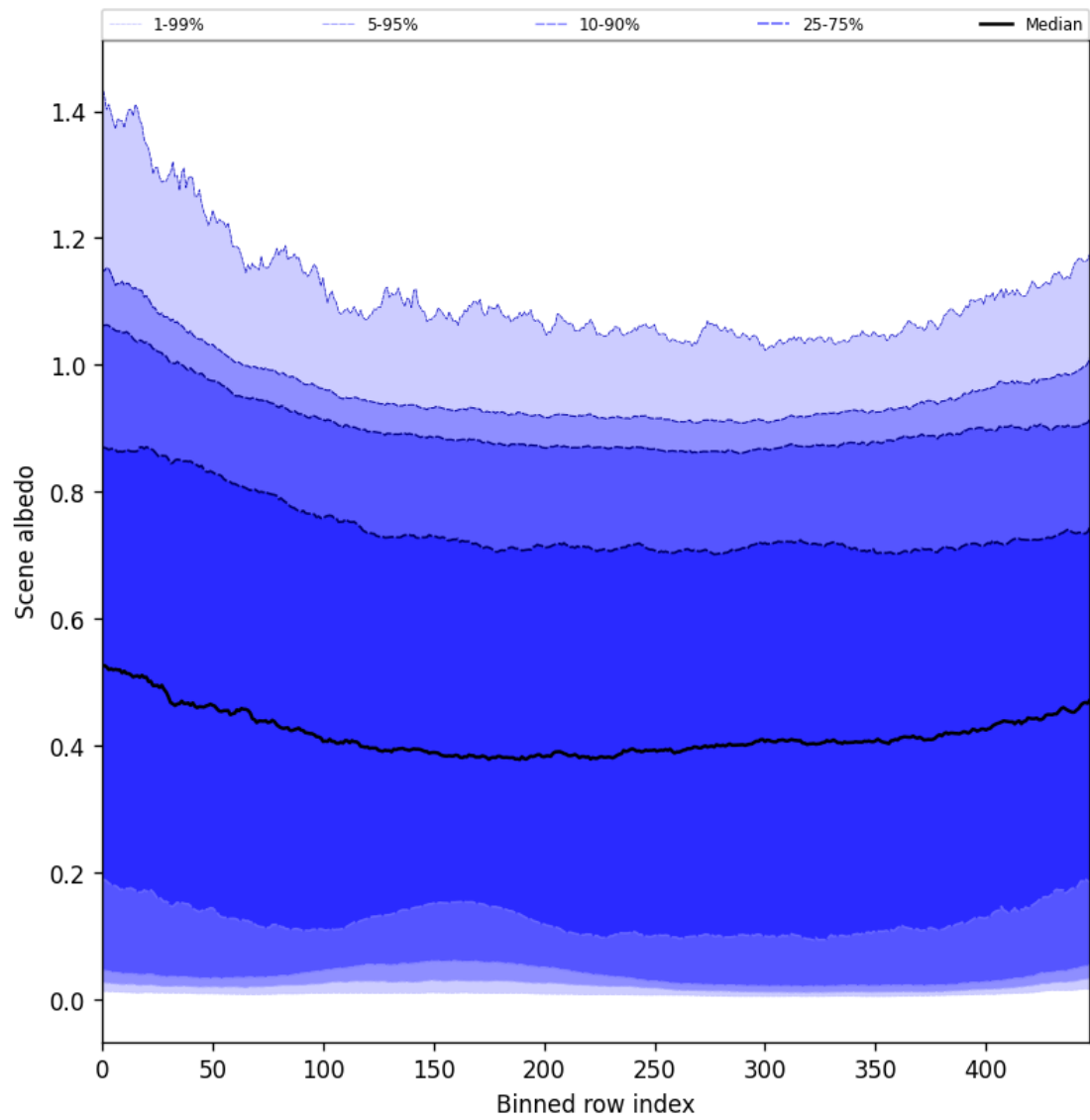
Figure 49: Along track statistics of “Scene albedo” for 2025-03-15 to 2025-03-15
