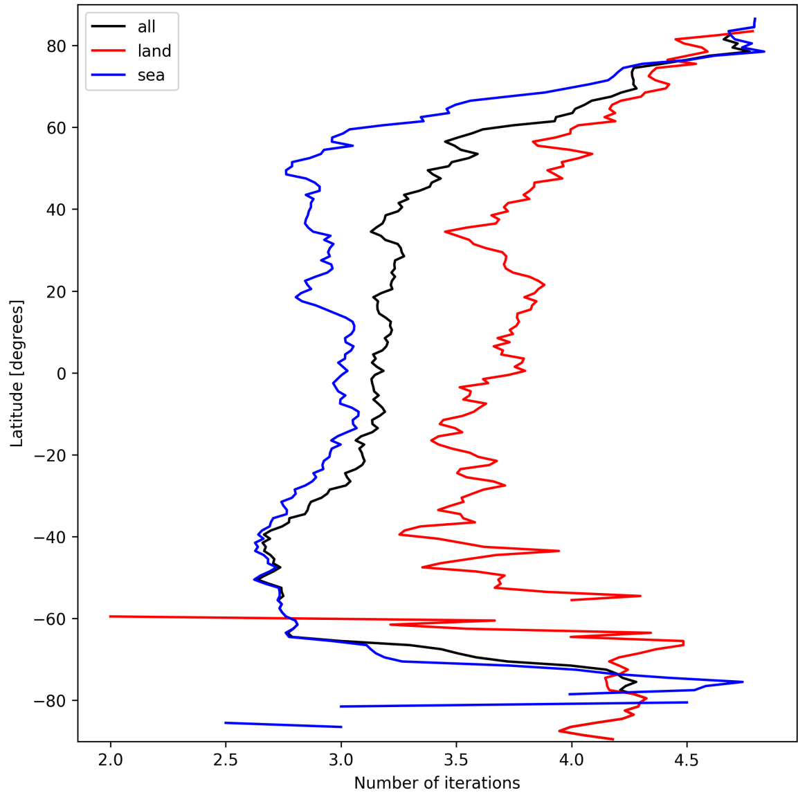
Figure 20: Zonal average of “Number of iterations” for 2025-03-15 to 2025-03-15.
