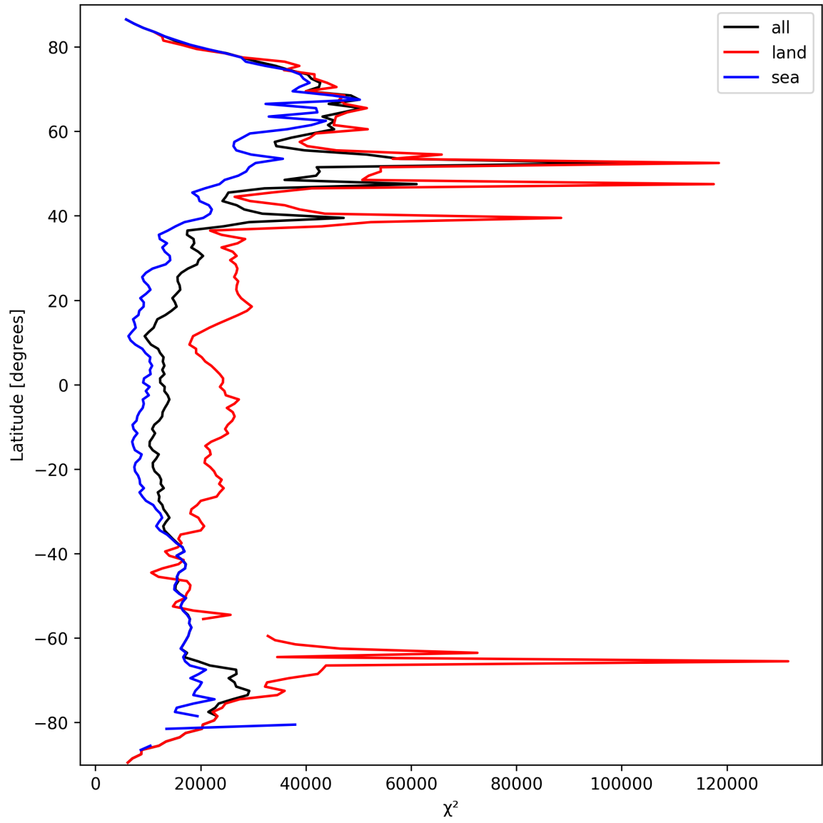
Figure 19: Zonal average of “ \chi^2 ” for 2025-03-15 to 2025-03-15.
