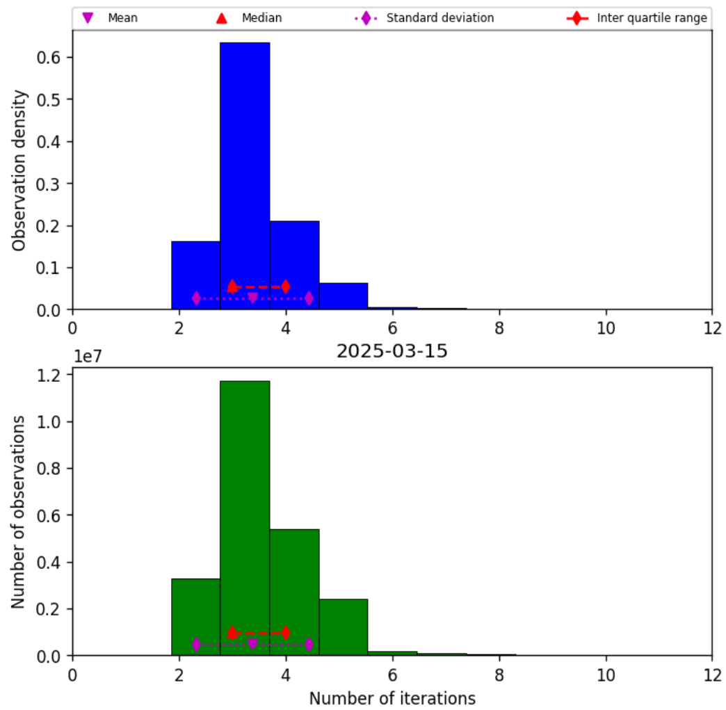
Figure 37: Histogram of “Number of iterations” for 2025-03-15 to 2025-03-15
