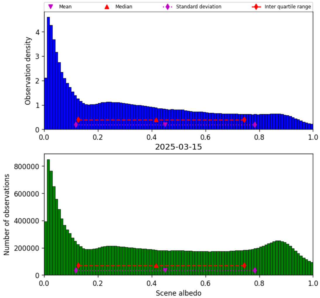
Figure 32: Histogram of “Scene albedo” for 2025-03-15 to 2025-03-15
