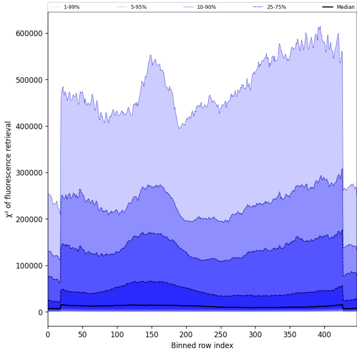
Figure 57: Along track statistics of “ \chi^2 of fluorescence retrieval” for 2025-03-15 to 2025-03-15
