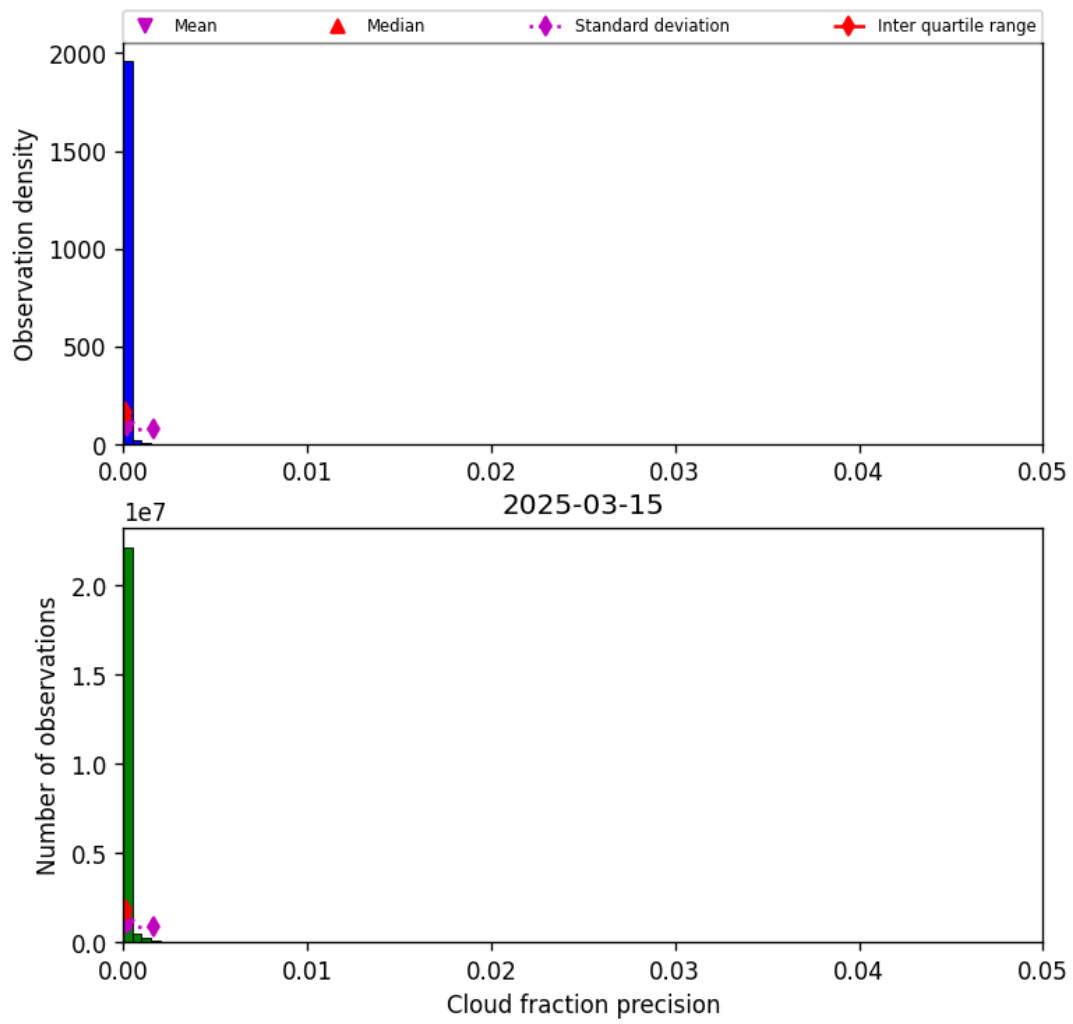
Figure 31: Histogram of “Cloud fraction precision” for 2025-03-15 to 2025-03-15
