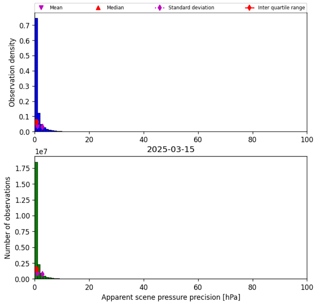
Figure 35: Histogram of “Apparent scene pressure precision” for 2025-03-15 to 2025-03-15
