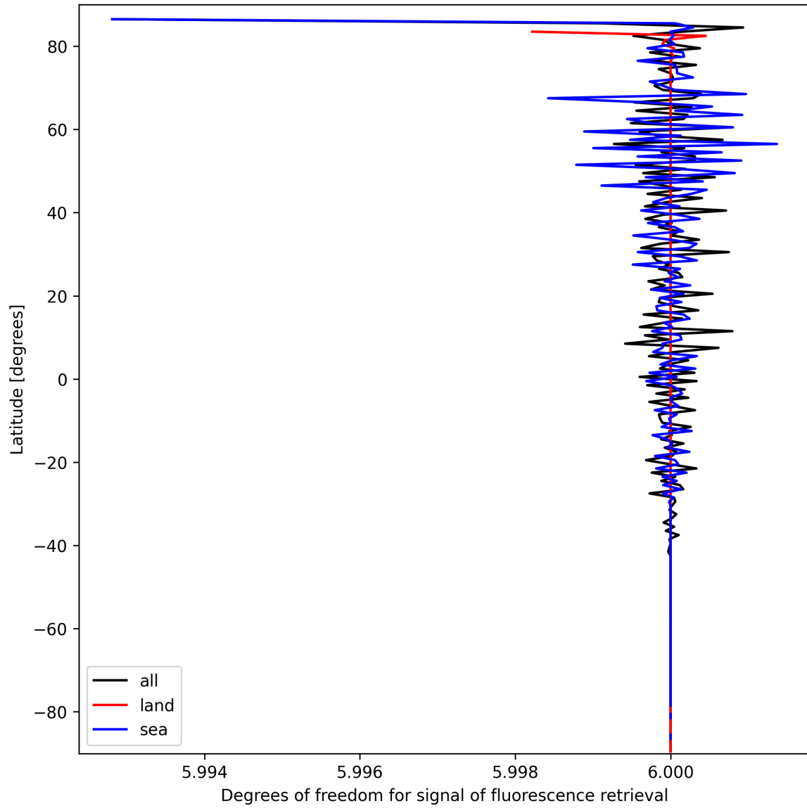
Figure 24: Zonal average of “Degrees of freedom for signal of fluorescence retrieval” for 2025-03-15 to 2025-03-15.
