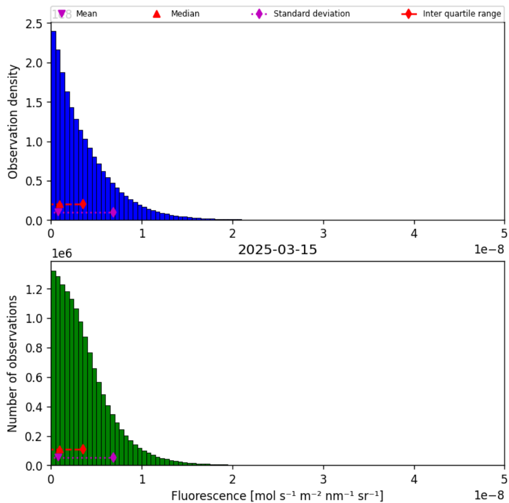
Figure 38: Histogram of “Fluorescence” for 2025-03-15 to 2025-03-15
