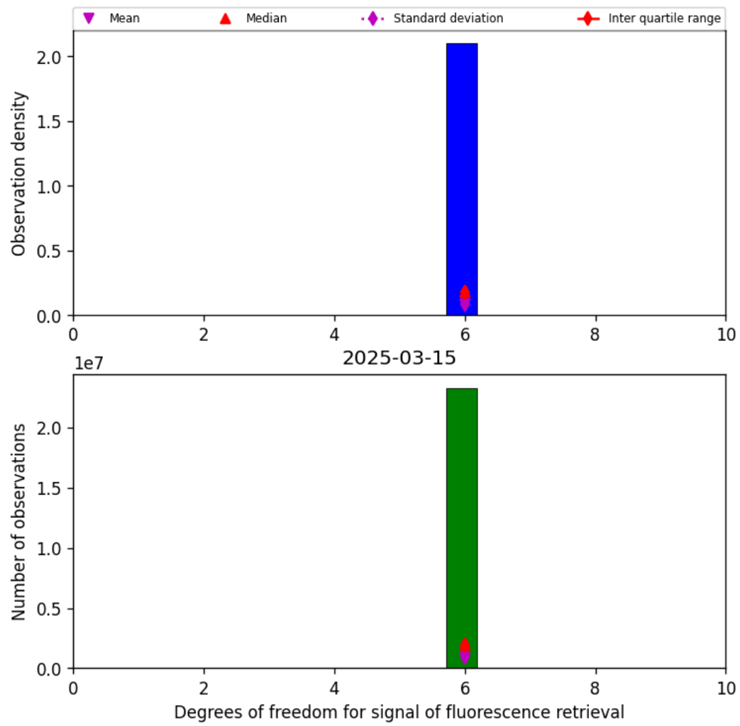
Figure 41: Histogram of “Degrees of freedom for signal of fluorescence retrieval” for 2025-03-15 to 2025-03-15
