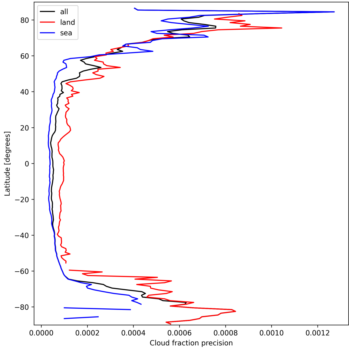
Figure 14: Zonal average of “Cloud fraction precision” for 2025-03-15 to 2025-03-15.
