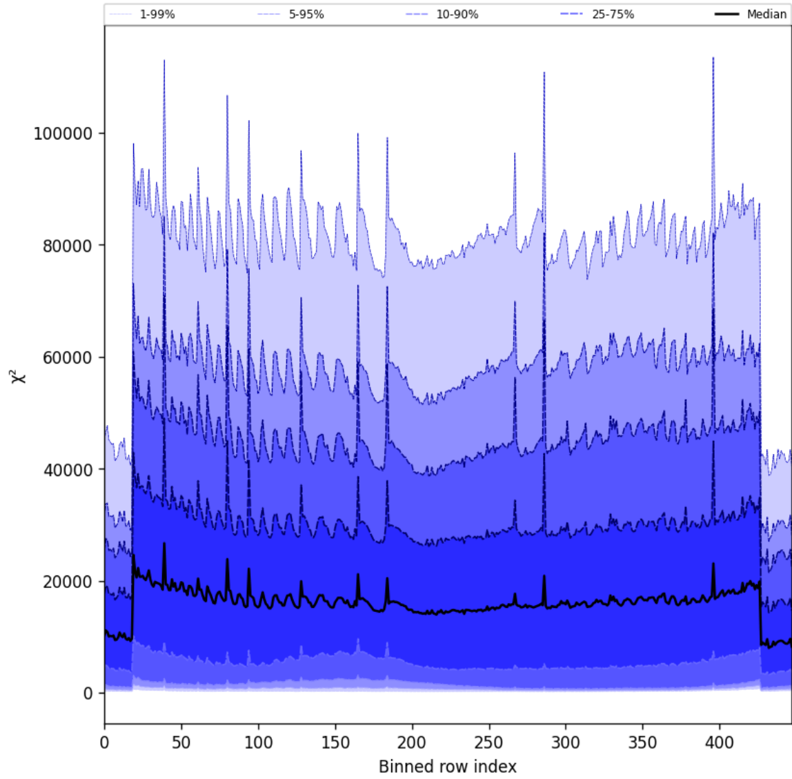
Figure 53: Along track statistics of “ \chi^2 ” for 2025-03-15 to 2025-03-15
