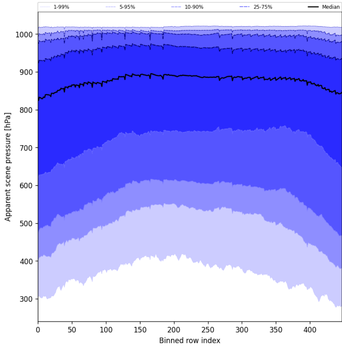
Figure 51: Along track statistics of “Apparent scene pressure” for 2025-03-15 to 2025-03-15
