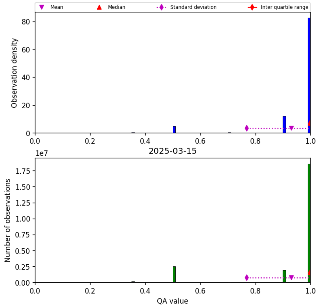
Figure 27: Histogram of “QA value” for 2025-03-15 to 2025-03-15
