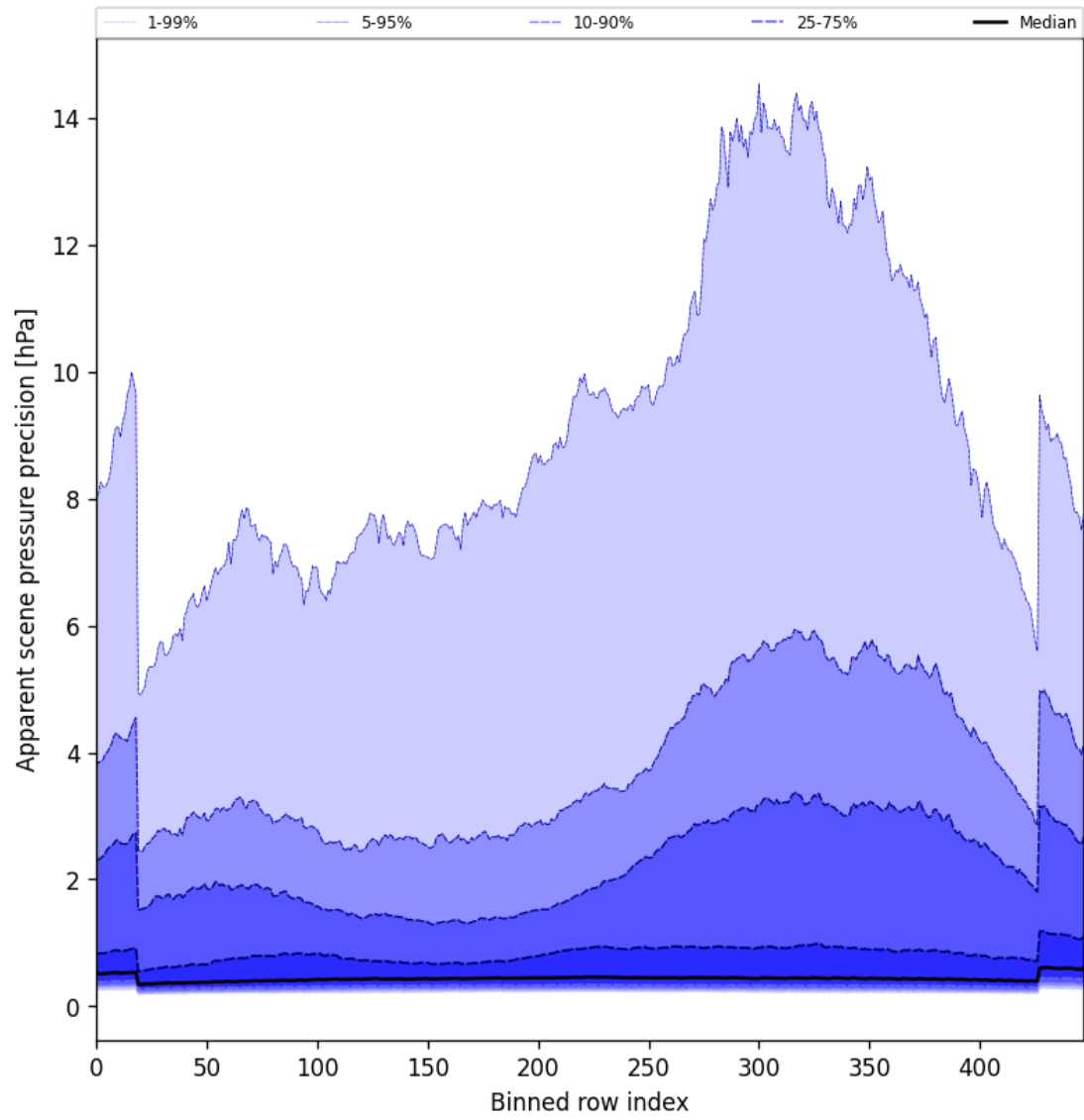
Figure 52: Along track statistics of “Apparent scene pressure precision” for 2025-03-15 to 2025-03-15
