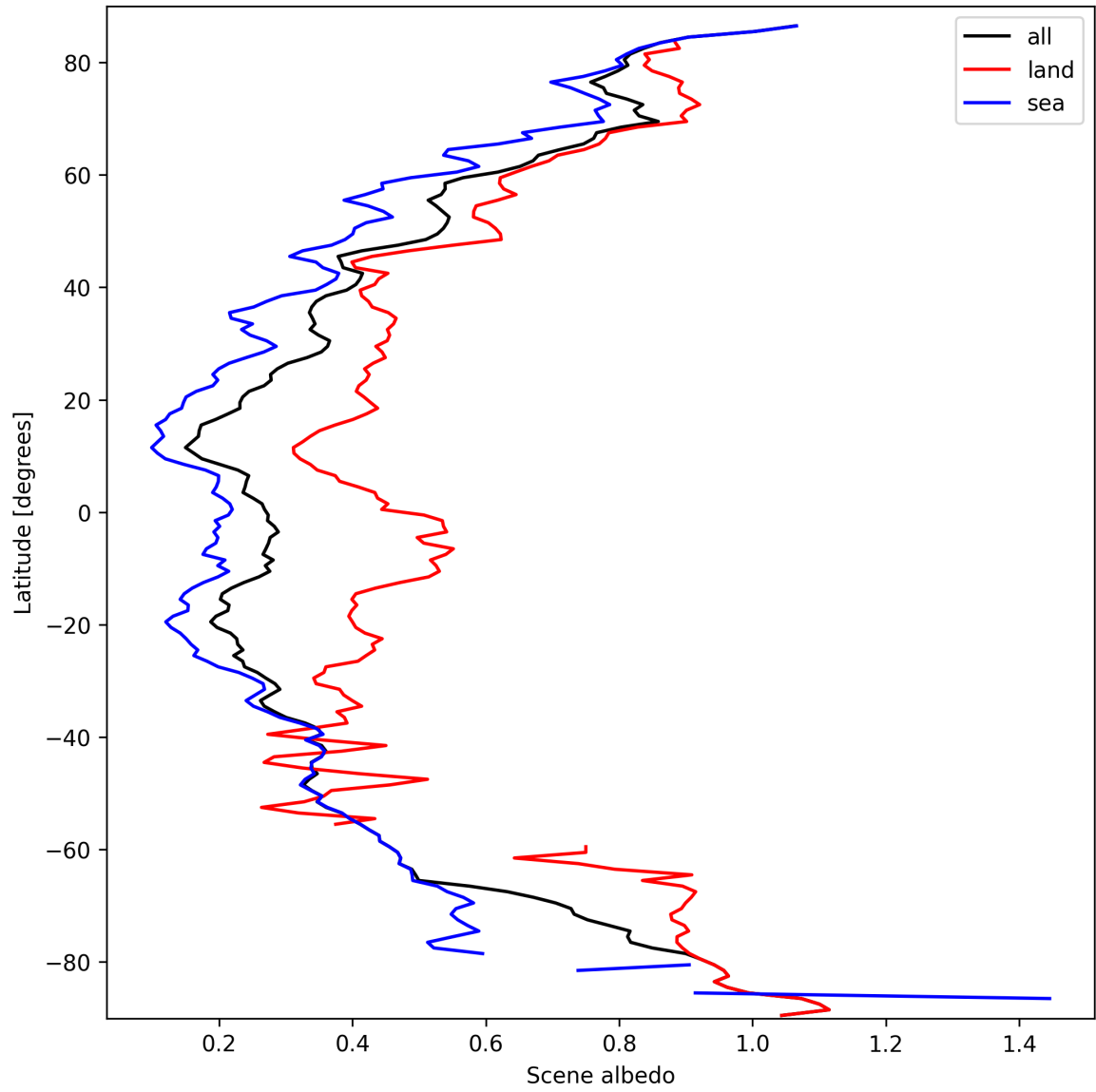
Figure 15: Zonal average of “Scene albedo” for 2025-03-15 to 2025-03-15.
