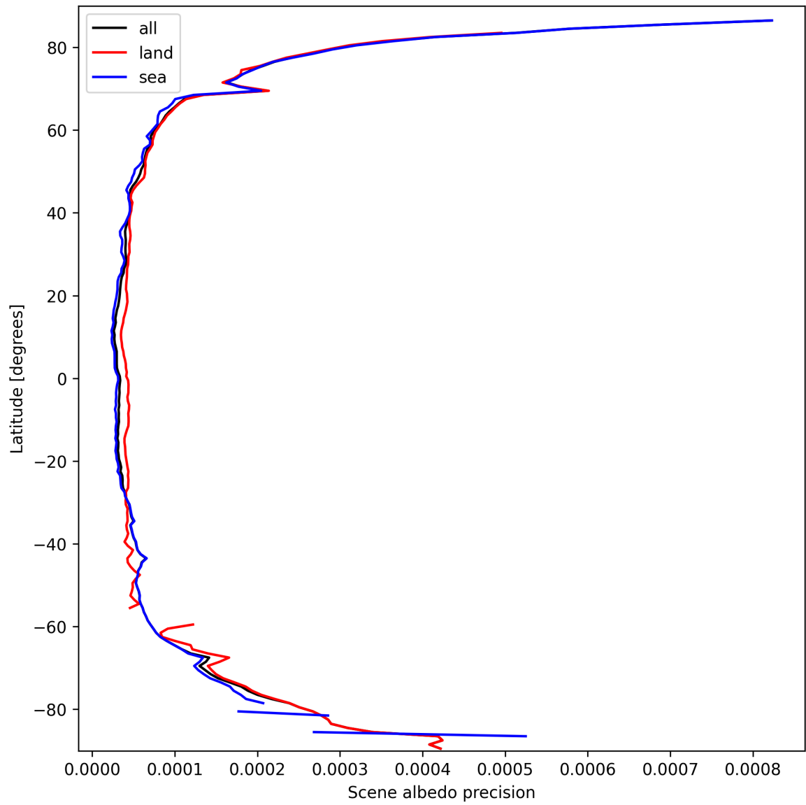
Figure 16: Zonal average of “Scene albedo precision” for 2025-03-15 to 2025-03-15.
