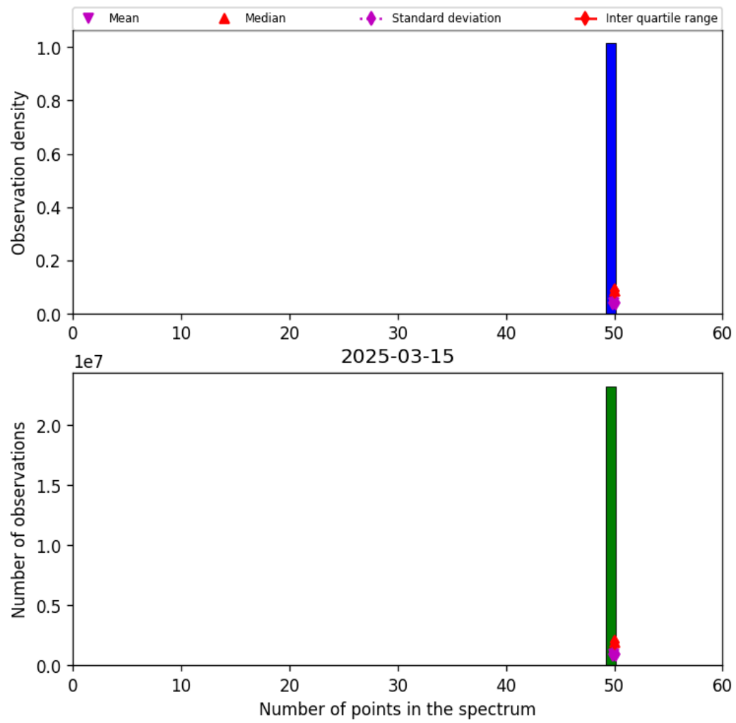
Figure 42: Histogram of "Number of points in the spectrum" for 2025-03-15 to 2025-03-15
