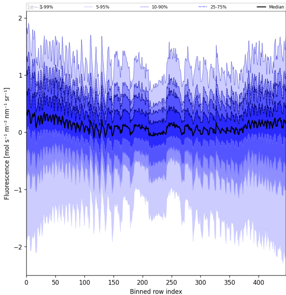
Figure 55: Along track statistics of “Fluorescence” for 2025-03-15 to 2025-03-15
