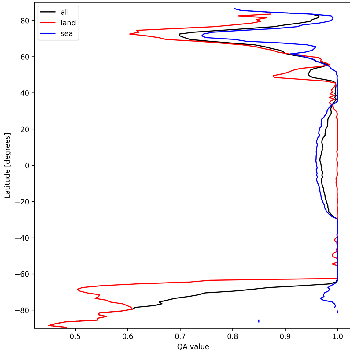
Figure 10: Zonal average of “QA value” for 2025-03-15 to 2025-03-15.
