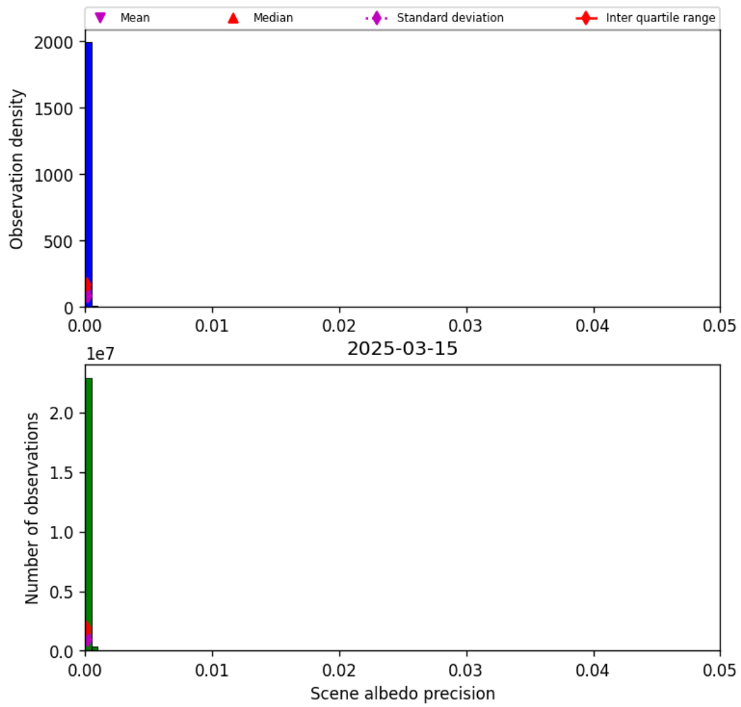
Figure 33: Histogram of “Scene albedo precision” for 2025-03-15 to 2025-03-15
