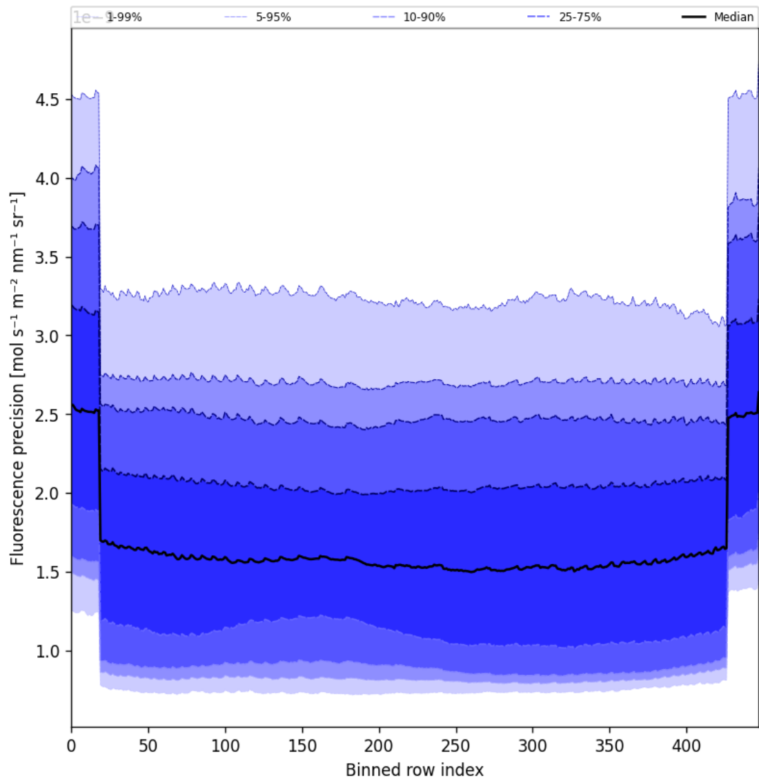
Figure 56: Along track statistics of “Fluorescence precision” for 2025-03-15 to 2025-03-15
