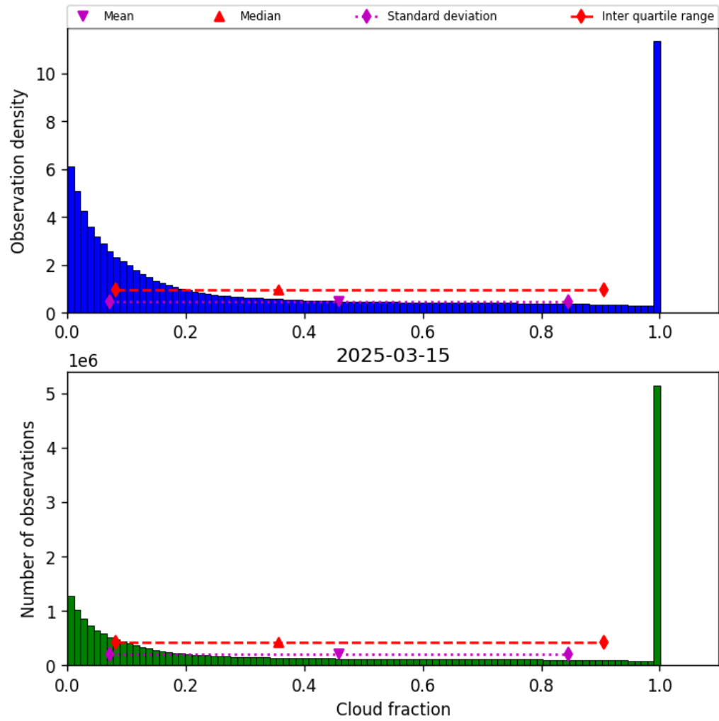
Figure 30: Histogram of “Cloud fraction” for 2025-03-15 to 2025-03-15
