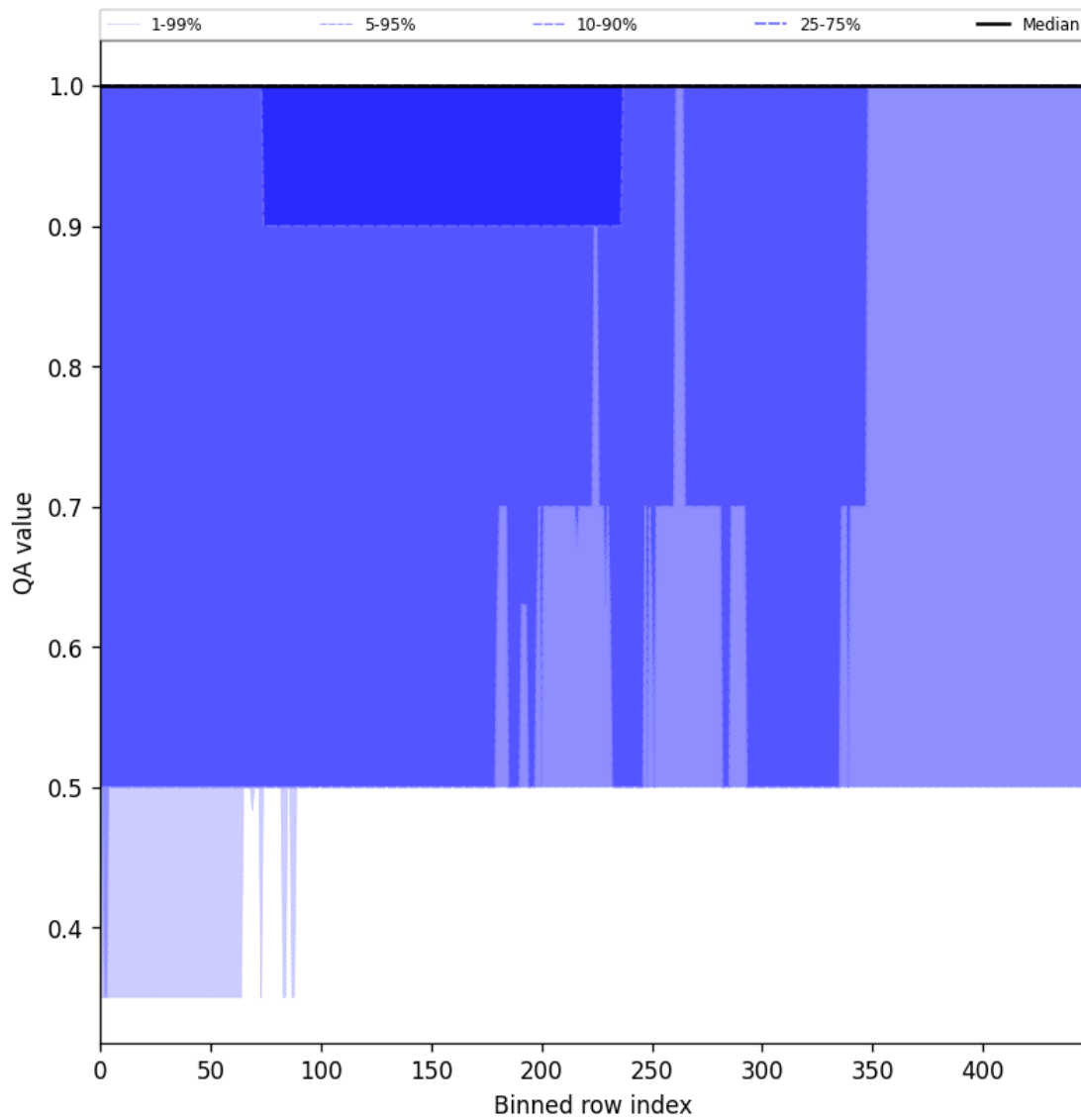
Figure 44: Along track statistics of "QA value" for 2025-03-15 to 2025-03-15
