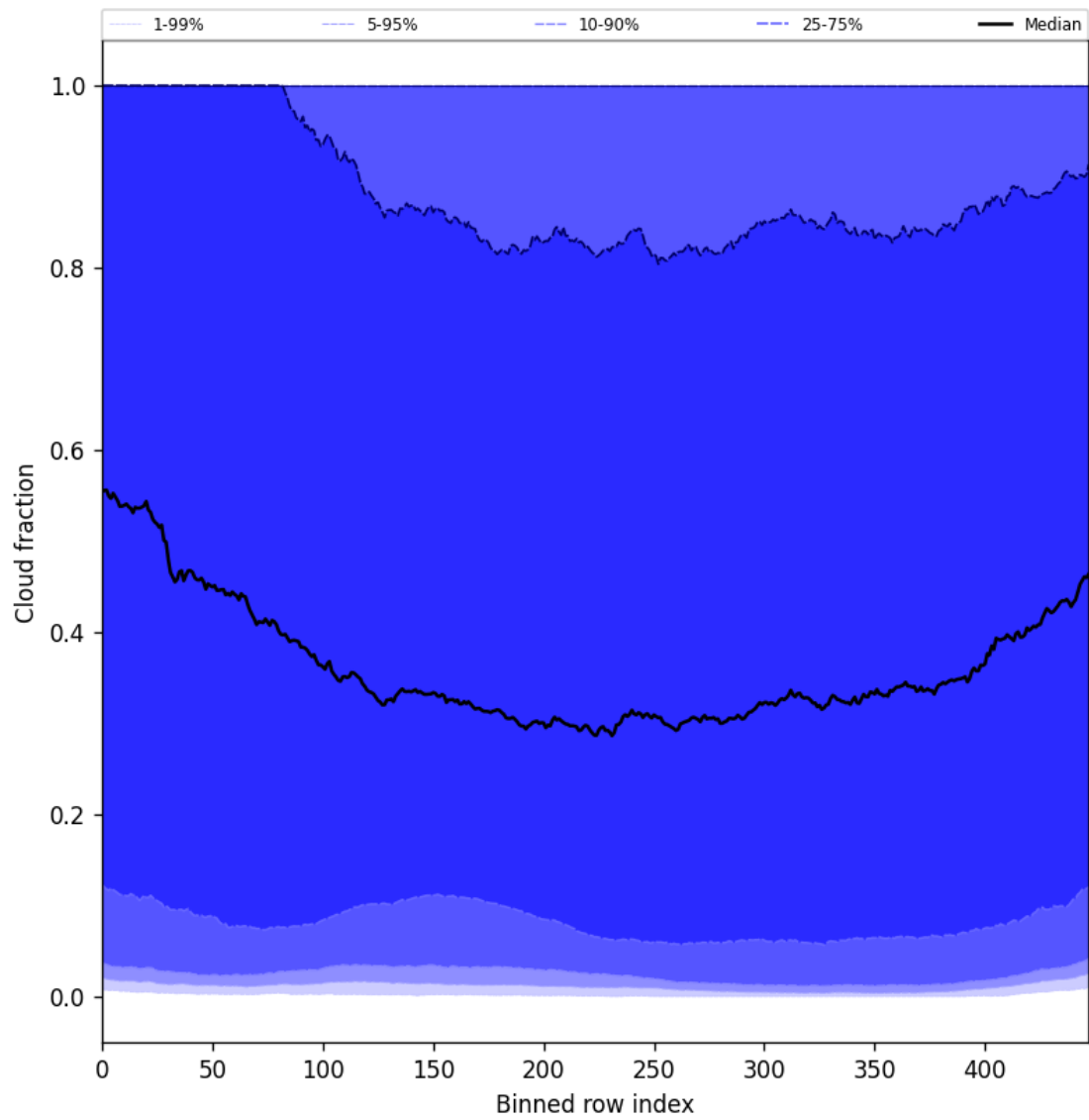
Figure 47: Along track statistics of “Cloud fraction” for 2025-03-15 to 2025-03-15
