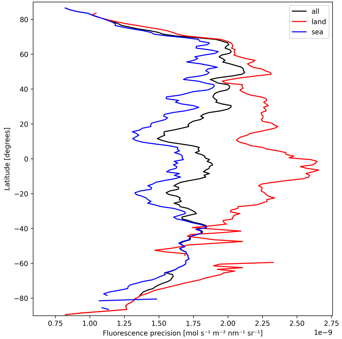
Figure 22: Zonal average of “Fluorescence precision” for 2025-03-15 to 2025-03-15.
