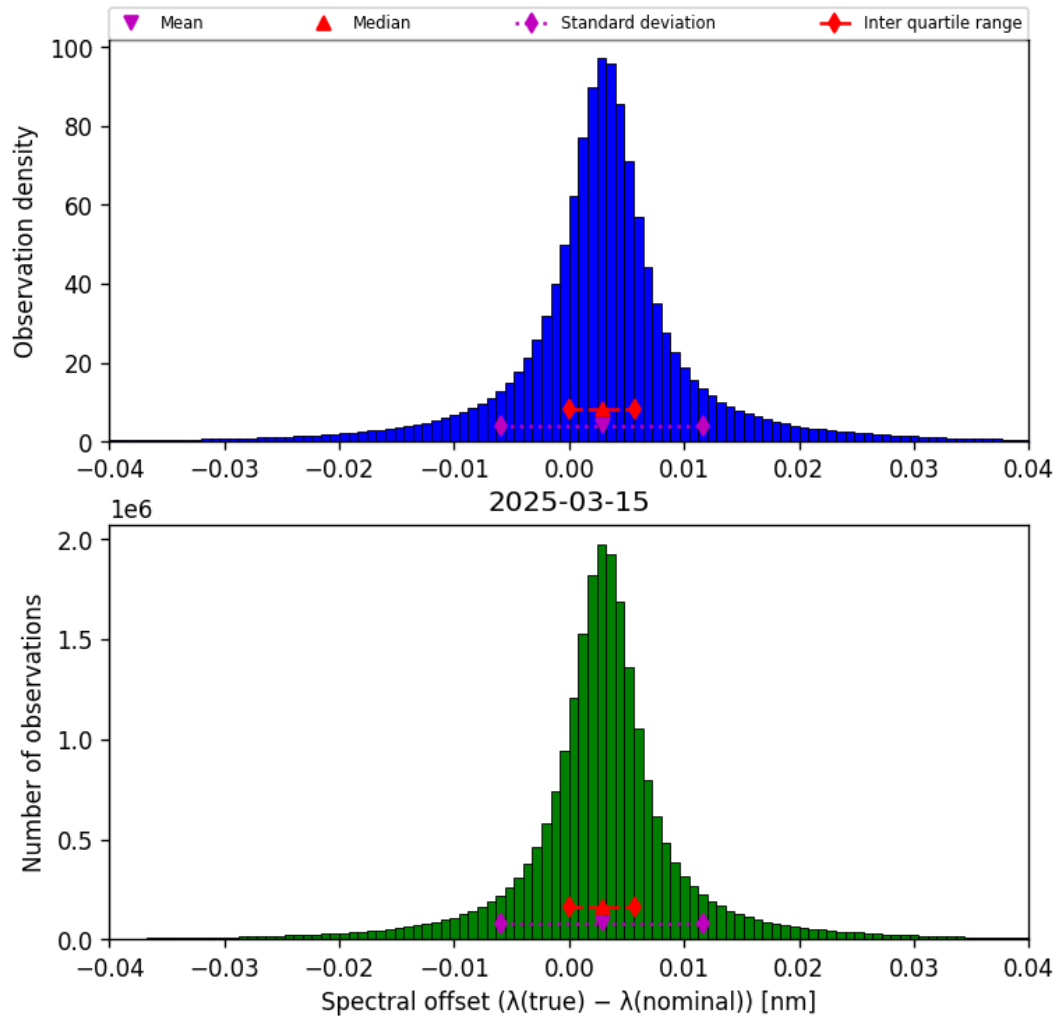
Figure 43: Histogram of “Spectral offset ( \lambda_{\text{true}} - \lambda_{\text{nominal}} )” for 2025-03-15 to 2025-03-15
