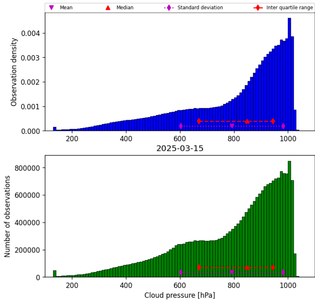
Figure 28: Histogram of “Cloud pressure” for 2025-03-15 to 2025-03-15
