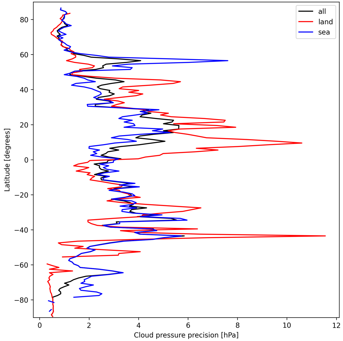
Figure 12: Zonal average of “Cloud pressure precision” for 2025-03-15 to 2025-03-15.
