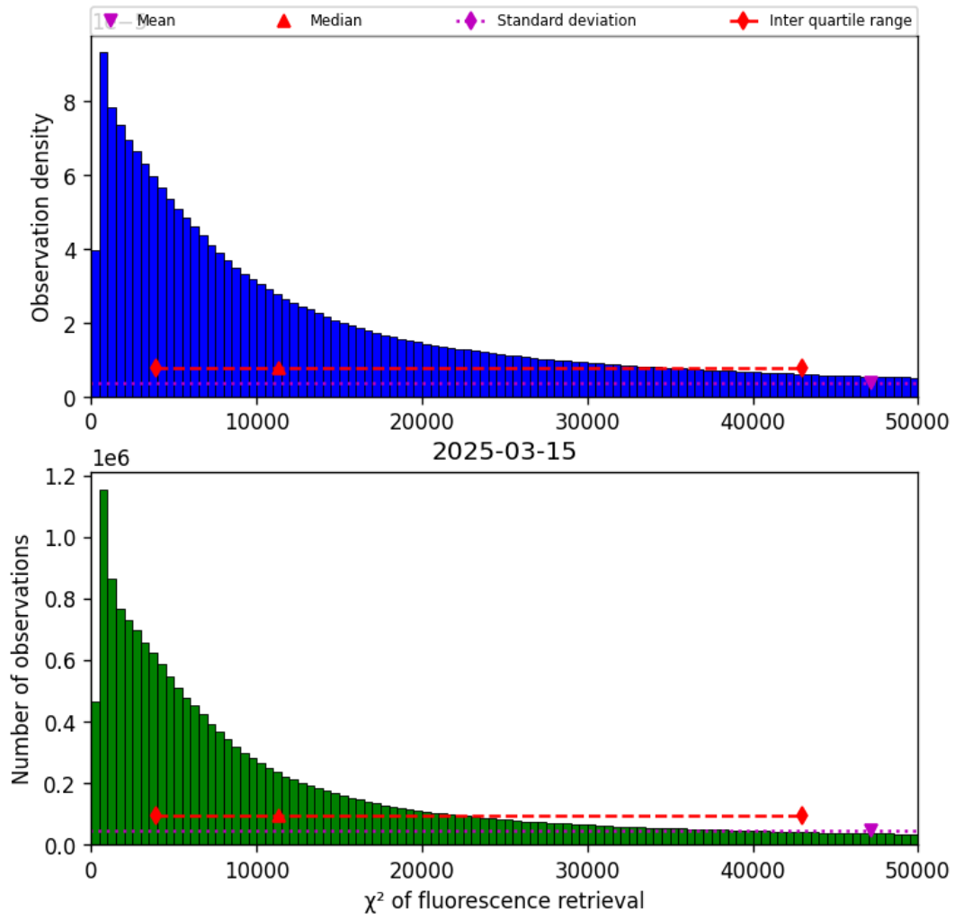
Figure 40: Histogram of “ \chi^2 of fluorescence retrieval” for 2025-03-15 to 2025-03-15
