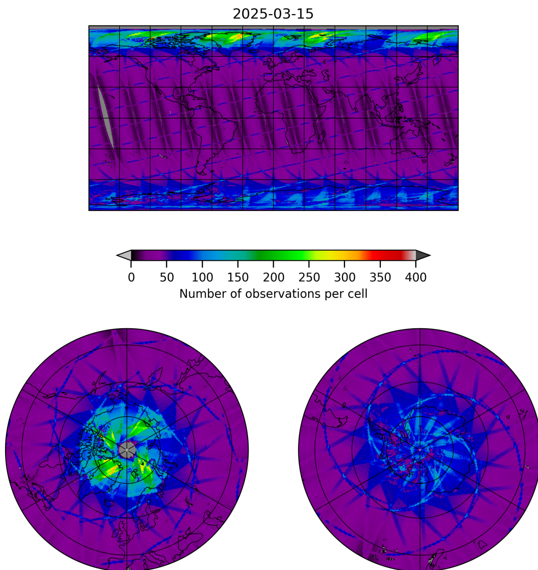
Figure 9: Map of the number of observations for 2025-03-15 to 2025-03-15
