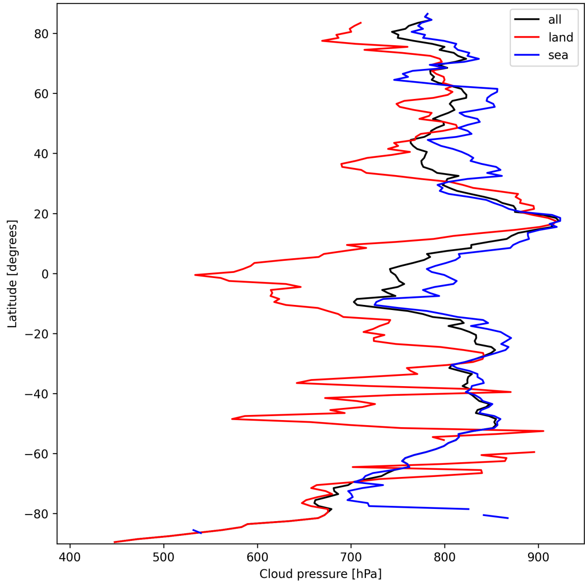
Figure 11: Zonal average of “Cloud pressure” for 2025-03-15 to 2025-03-15.
