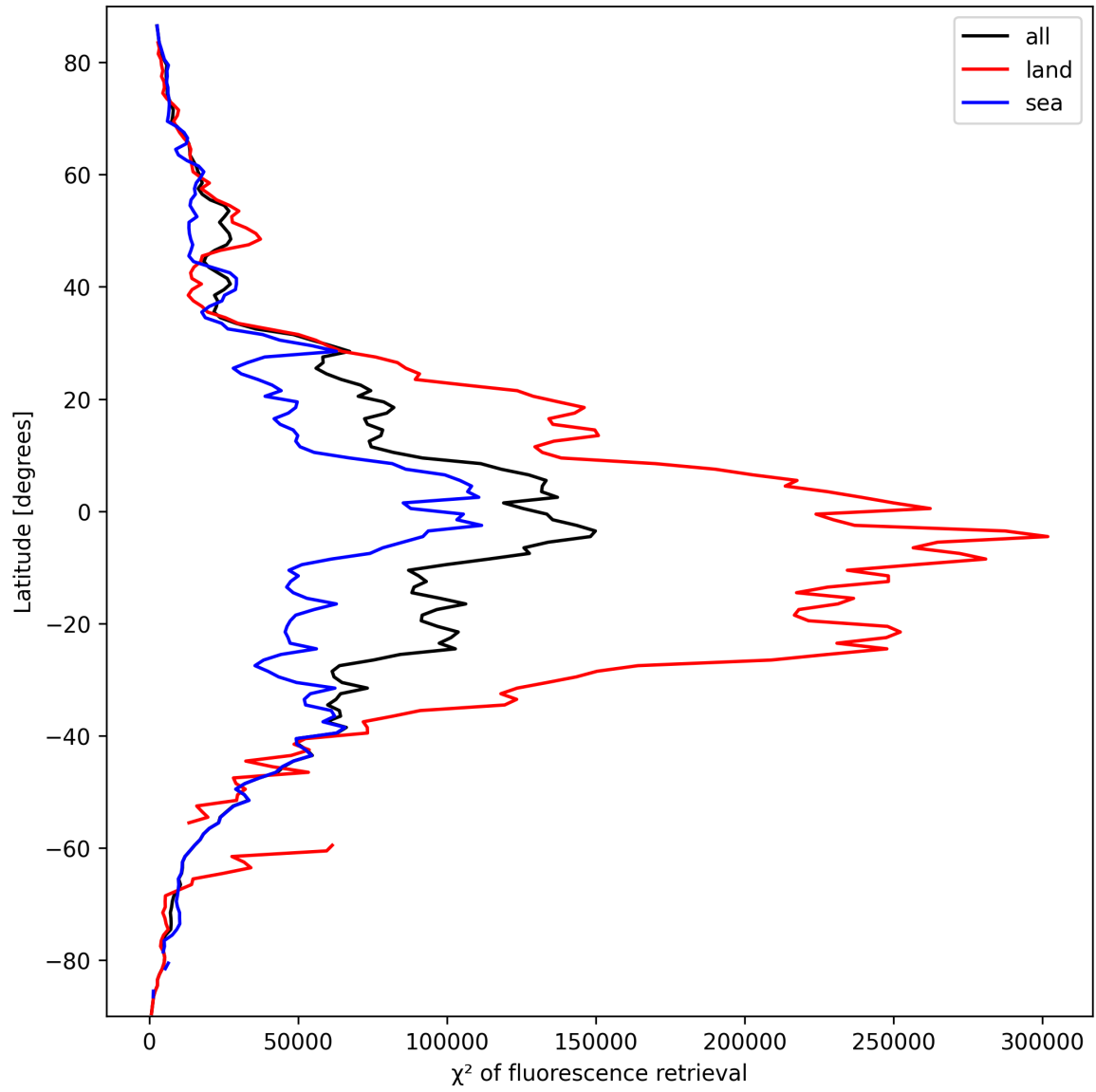
Figure 23: Zonal average of “ \chi^2 of fluorescence retrieval” for 2025-03-15 to 2025-03-15.
