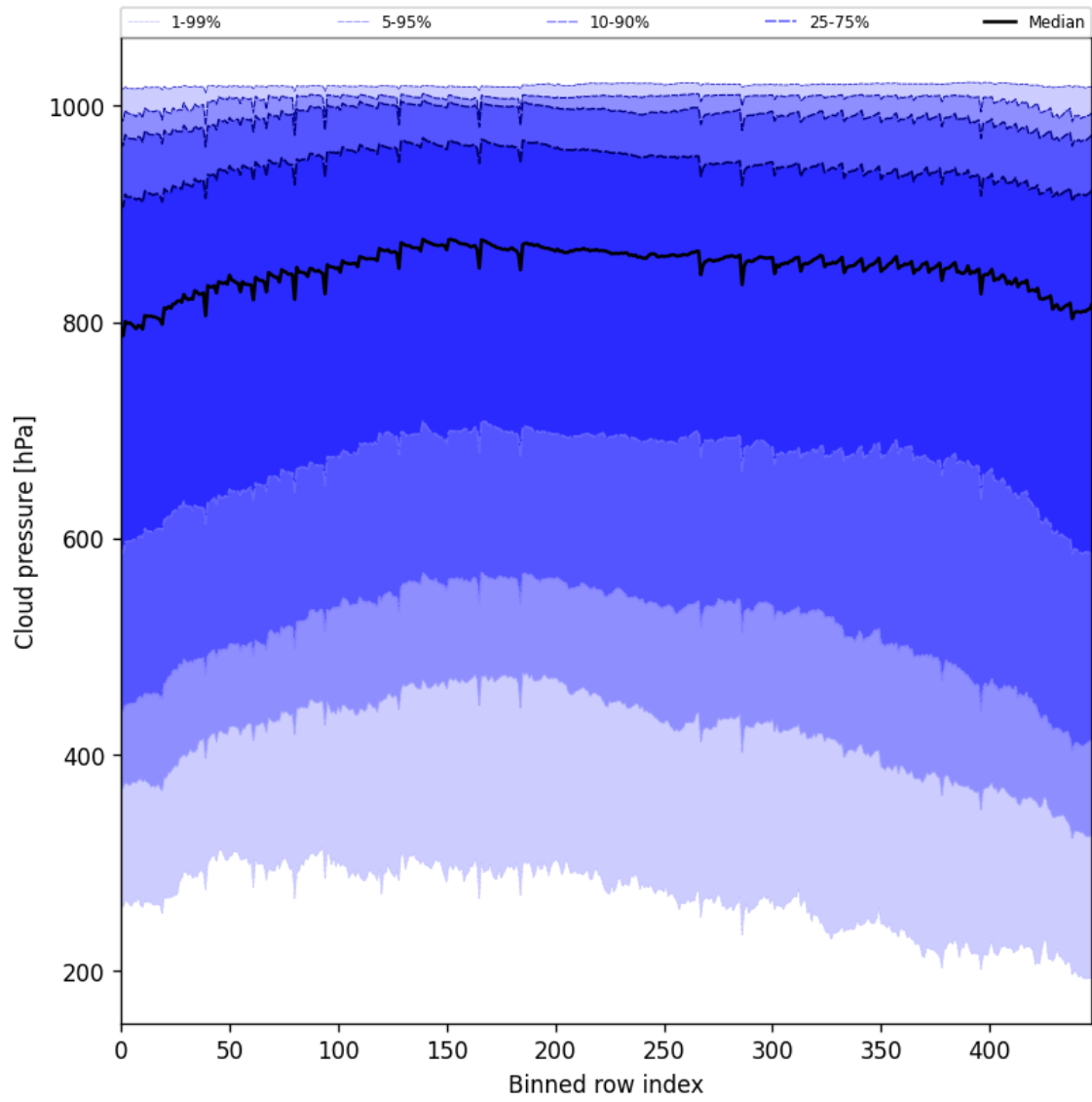
Figure 45: Along track statistics of “Cloud pressure” for 2025-03-15 to 2025-03-15
