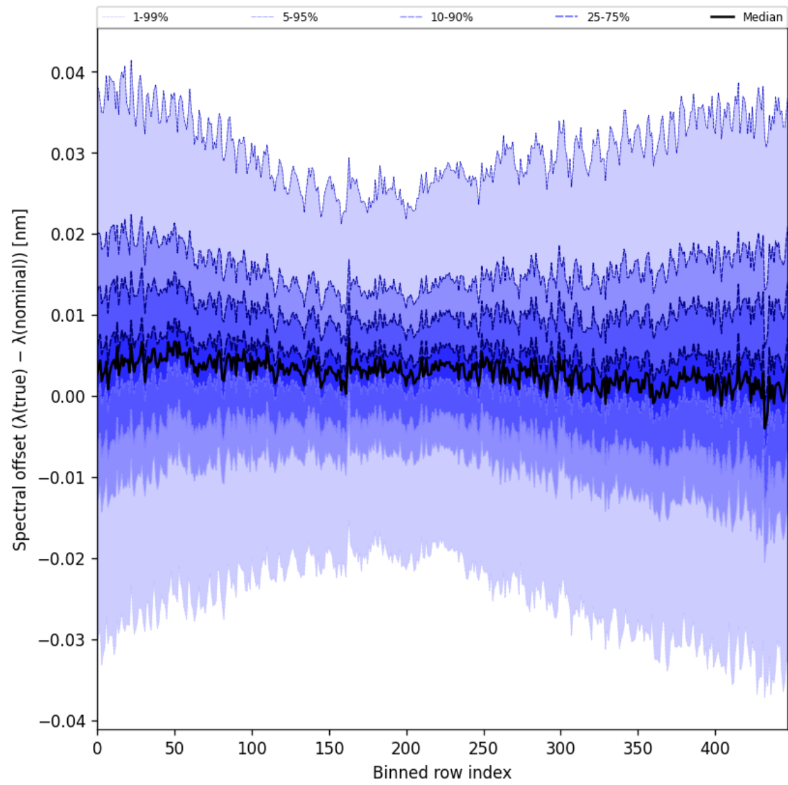
Figure 60: Along track statistics of “Spectral offset ( \lambda_{\text{true}} - \lambda_{\text{nominal}} )” for 2025-03-15 to 2025-03-15
