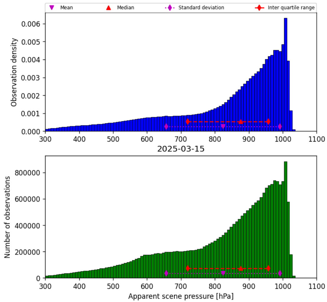
Figure 34: Histogram of “Apparent scene pressure” for 2025-03-15 to 2025-03-15
