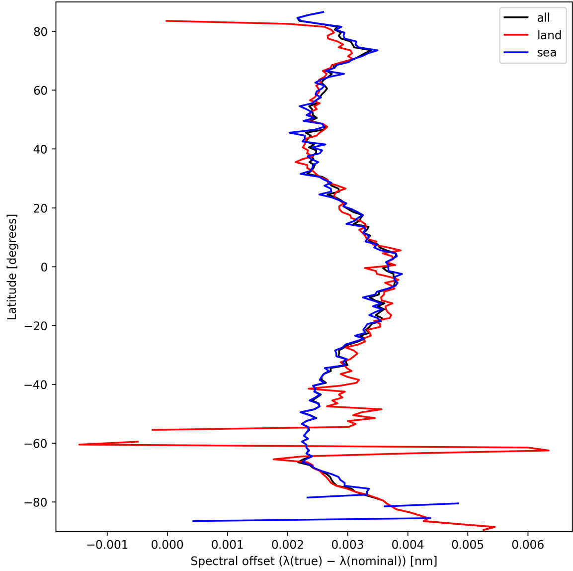
Figure 26: Zonal average of “Spectral offset ( \lambda_{\text{true}} - \lambda_{\text{nominal}} )” for 2025-03-15 to 2025-03-15.
