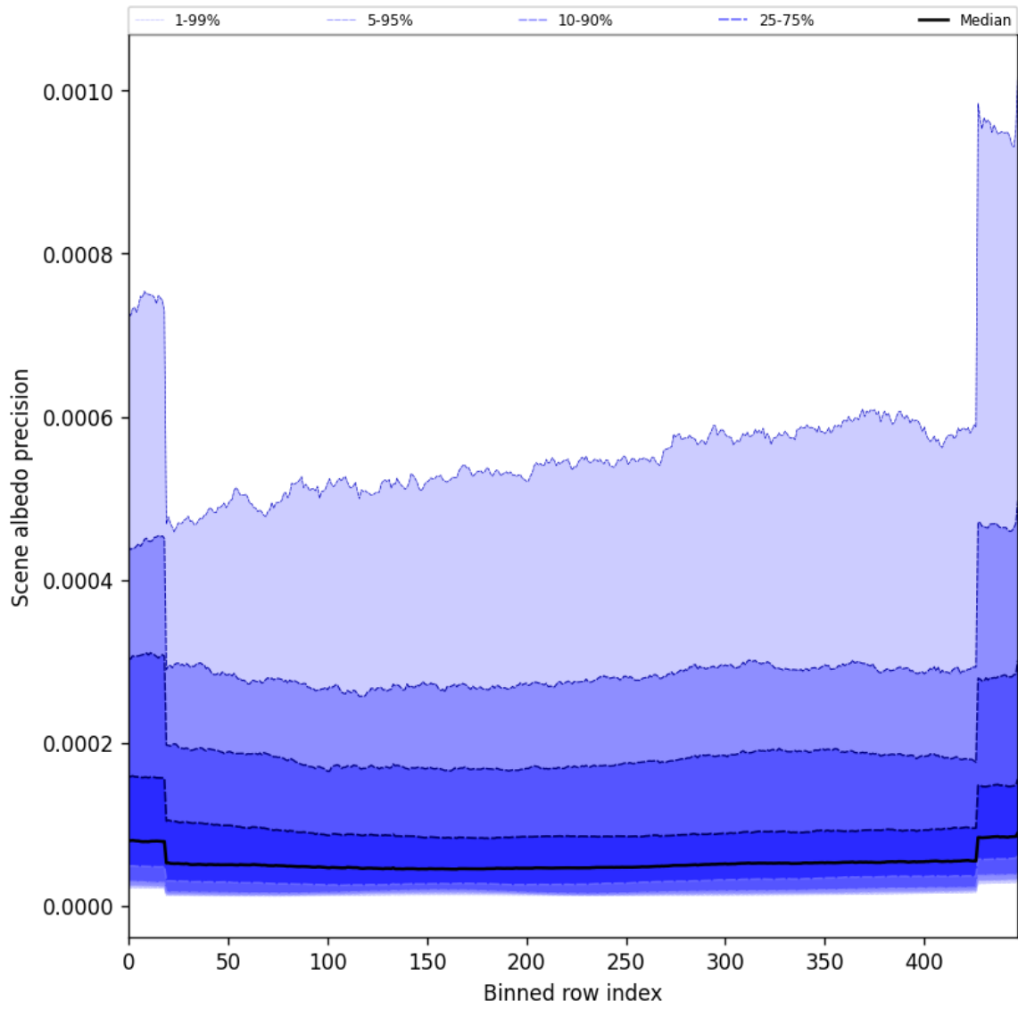
Figure 50: Along track statistics of “Scene albedo precision” for 2025-03-15 to 2025-03-15
