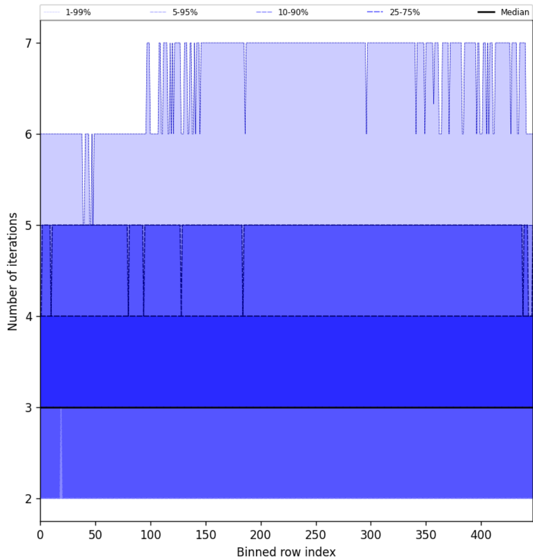
Figure 54: Along track statistics of “Number of iterations” for 2025-03-15 to 2025-03-15
