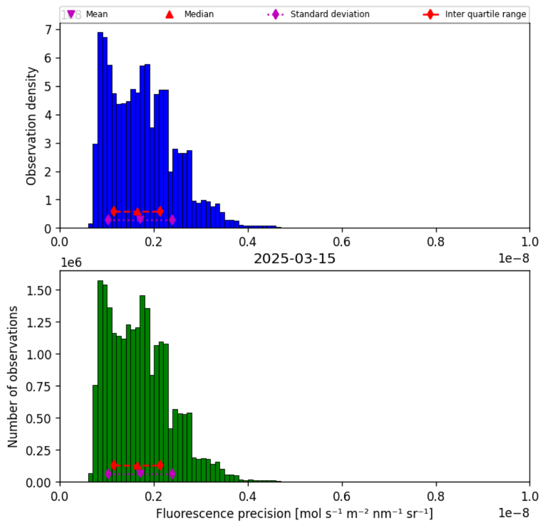
Figure 39: Histogram of “Fluorescence precision” for 2025-03-15 to 2025-03-15
