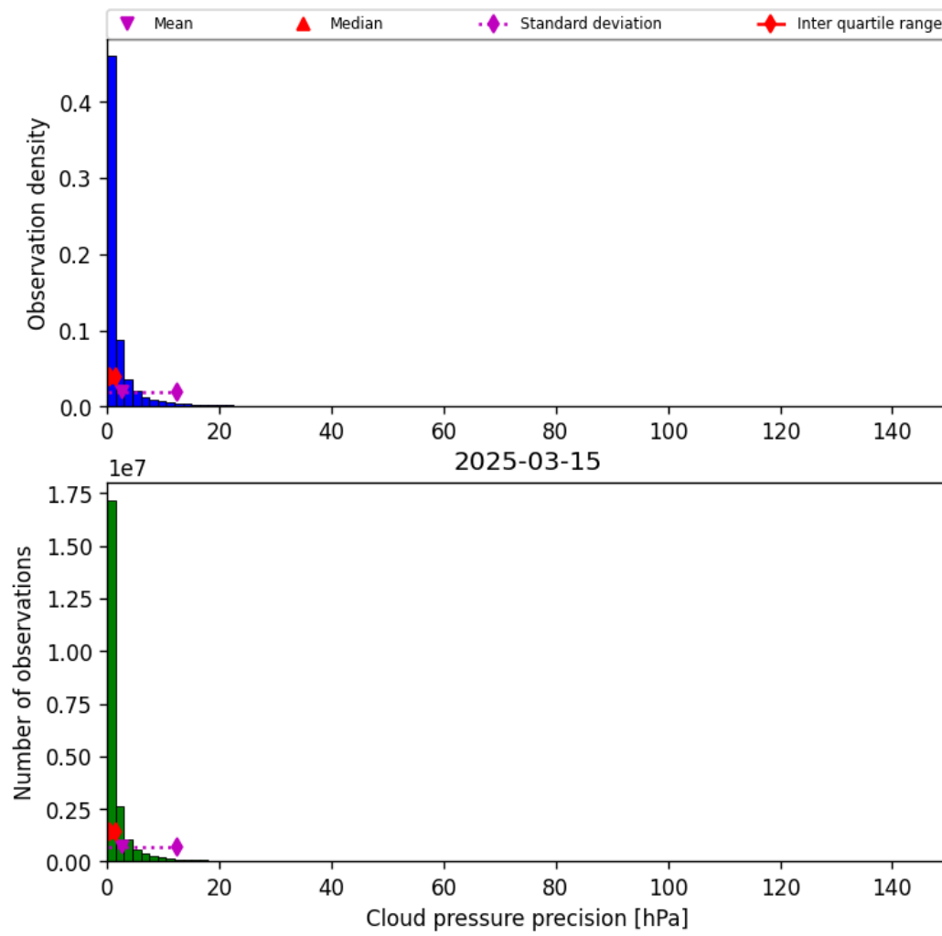
Figure 29: Histogram of “Cloud pressure precision” for 2025-03-15 to 2025-03-15
