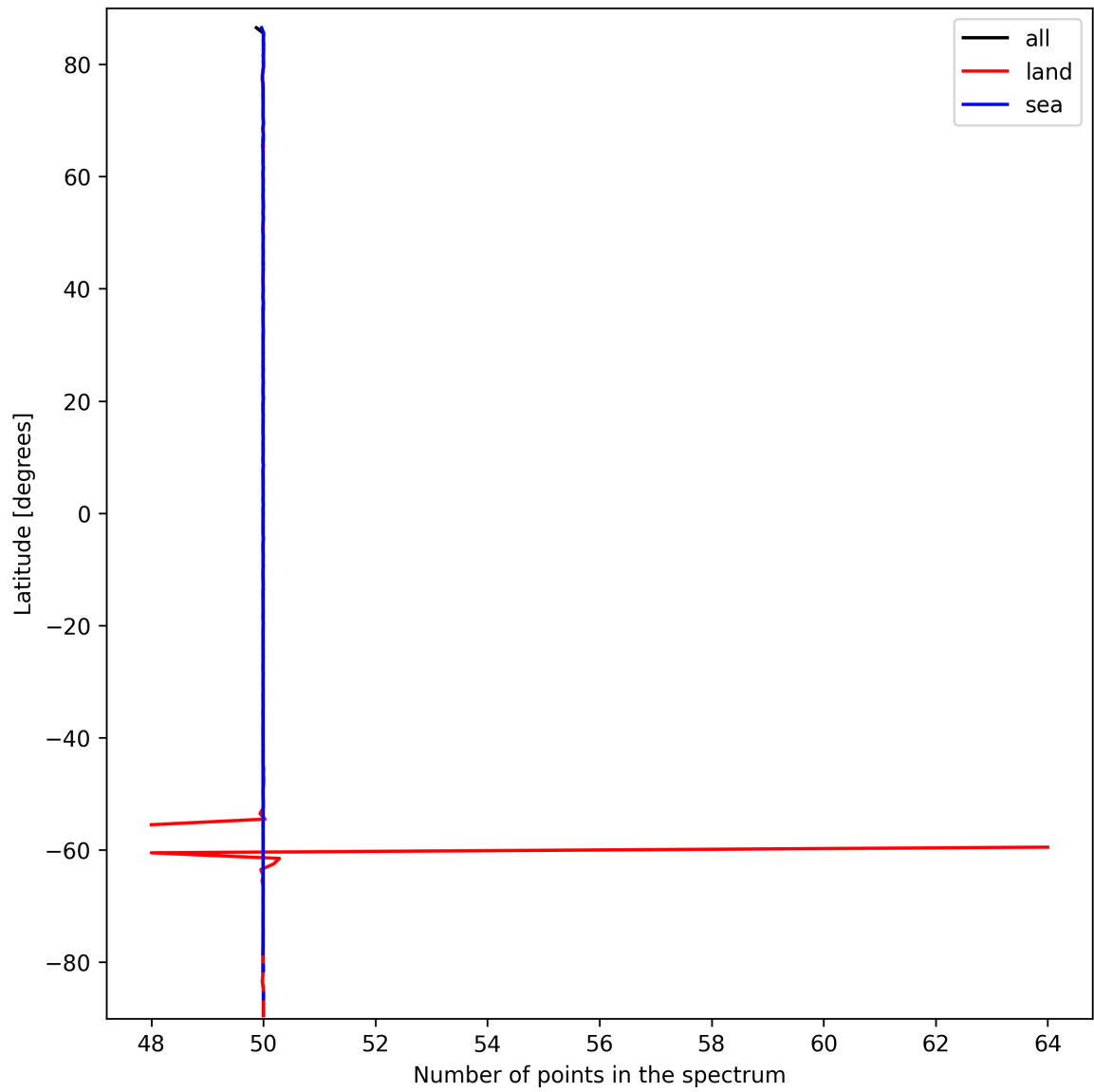
Figure 25: Zonal average of “Number of points in the spectrum” for 2025-03-15 to 2025-03-15.
