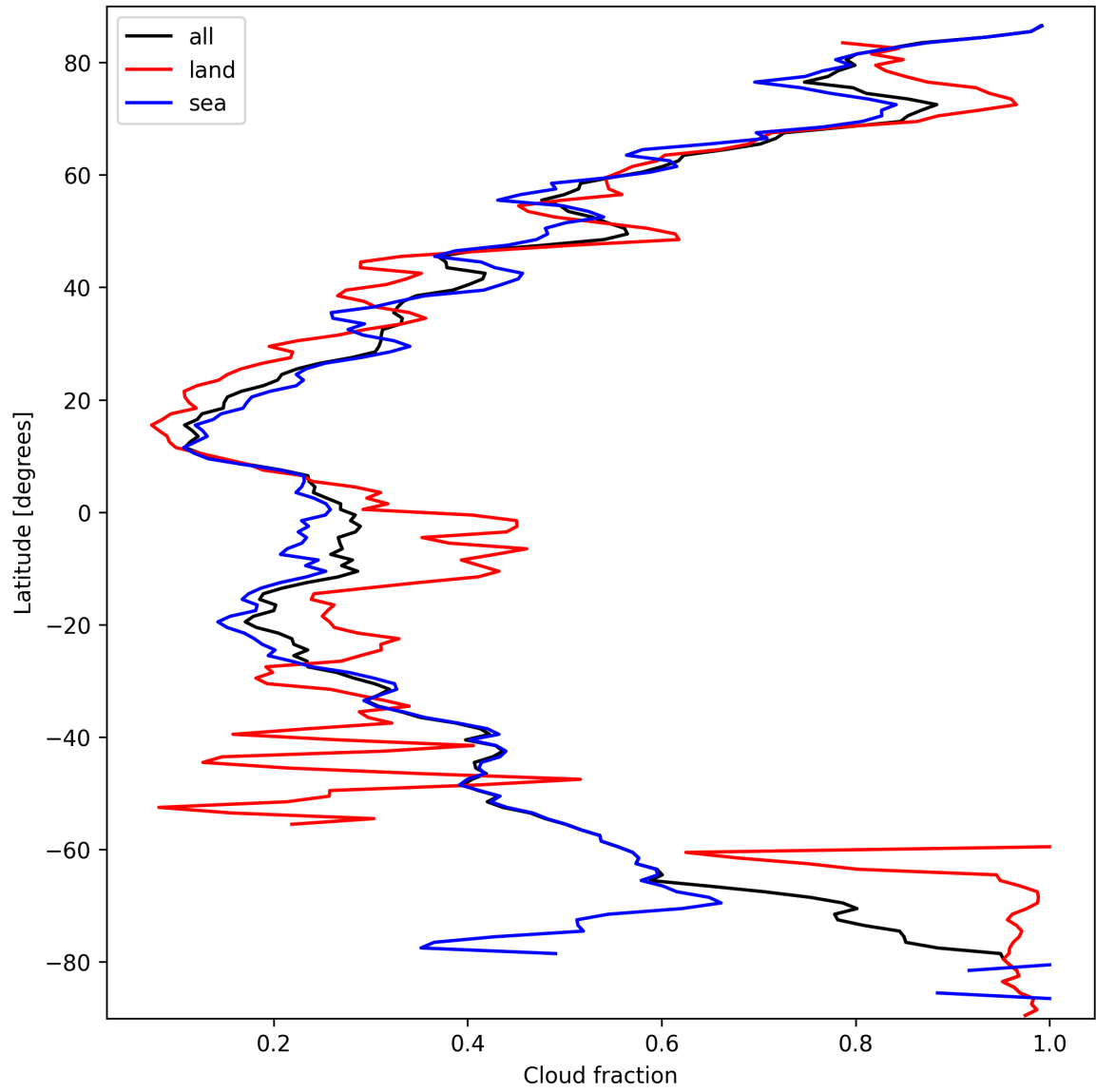
Figure 13: Zonal average of “Cloud fraction” for 2025-03-15 to 2025-03-15.
