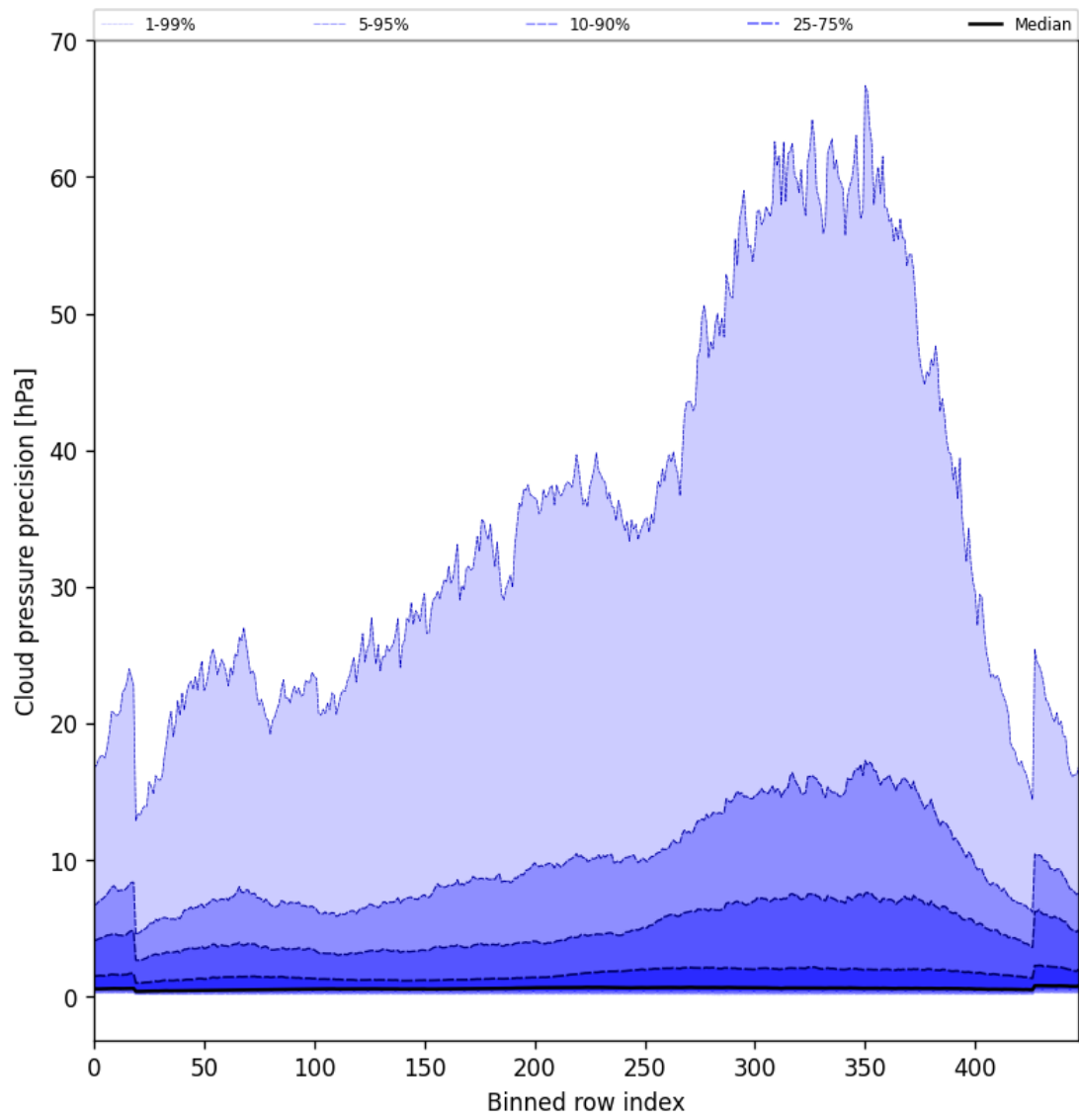
Figure 46: Along track statistics of “Cloud pressure precision” for 2025-03-15 to 2025-03-15
