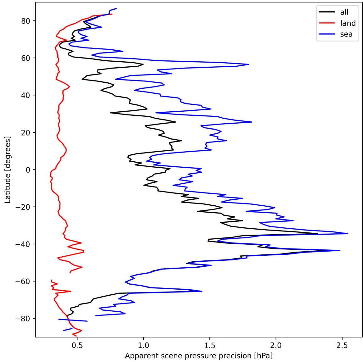
Figure 18: Zonal average of “Apparent scene pressure precision” for 2025-03-15 to 2025-03-15.
