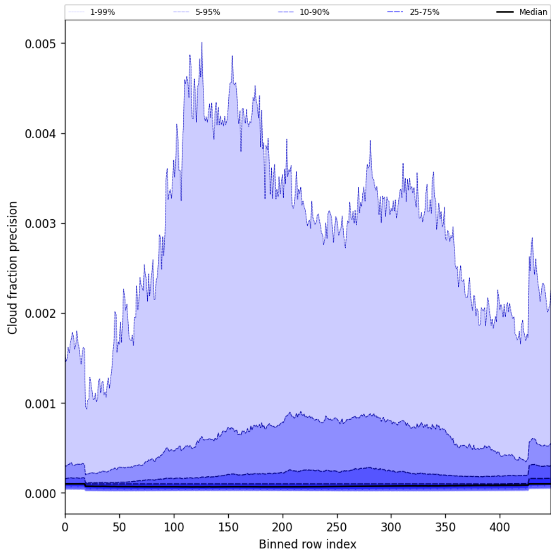
Figure 48: Along track statistics of “Cloud fraction precision” for 2025-03-20 to 2025-03-21
