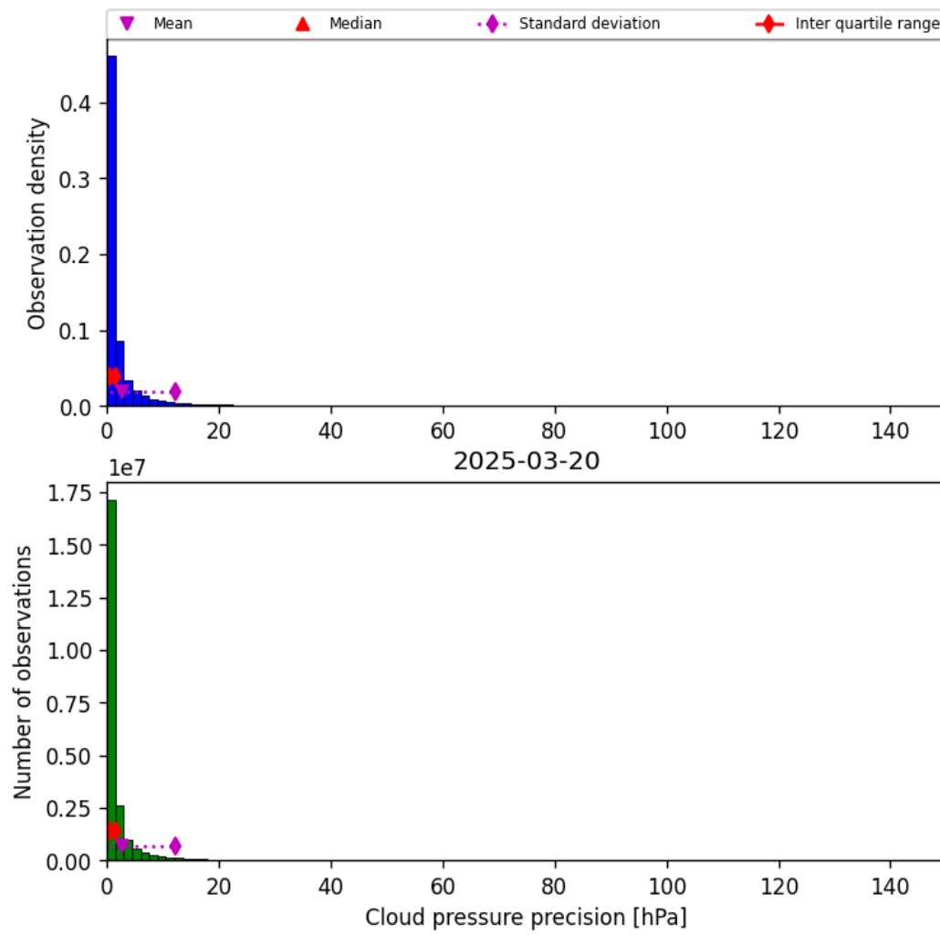
Figure 29: Histogram of “Cloud pressure precision” for 2025-03-20 to 2025-03-21
