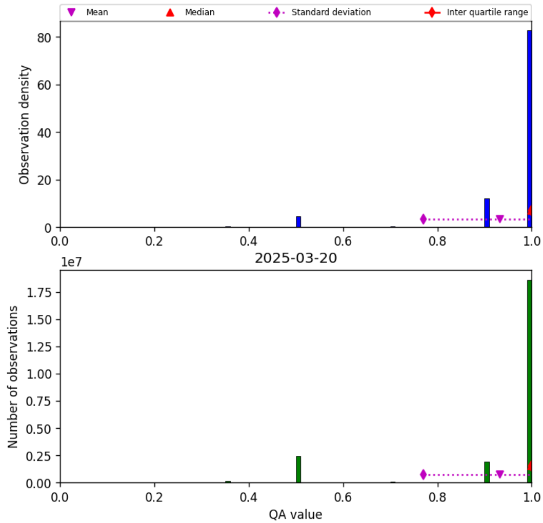
Figure 27: Histogram of “QA value” for 2025-03-20 to 2025-03-21
