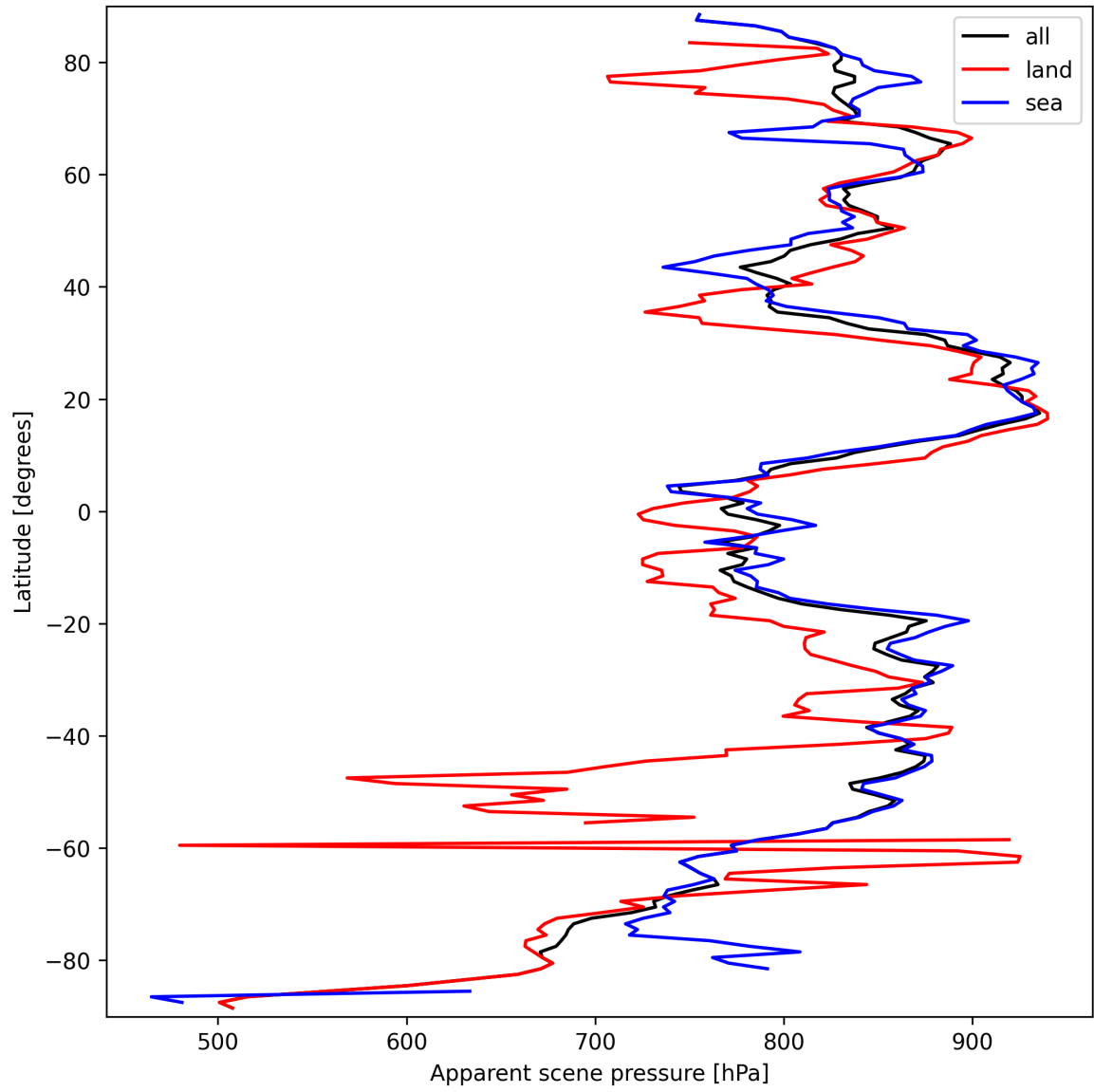
Figure 17: Zonal average of “Apparent scene pressure” for 2025-03-20 to 2025-03-21.
