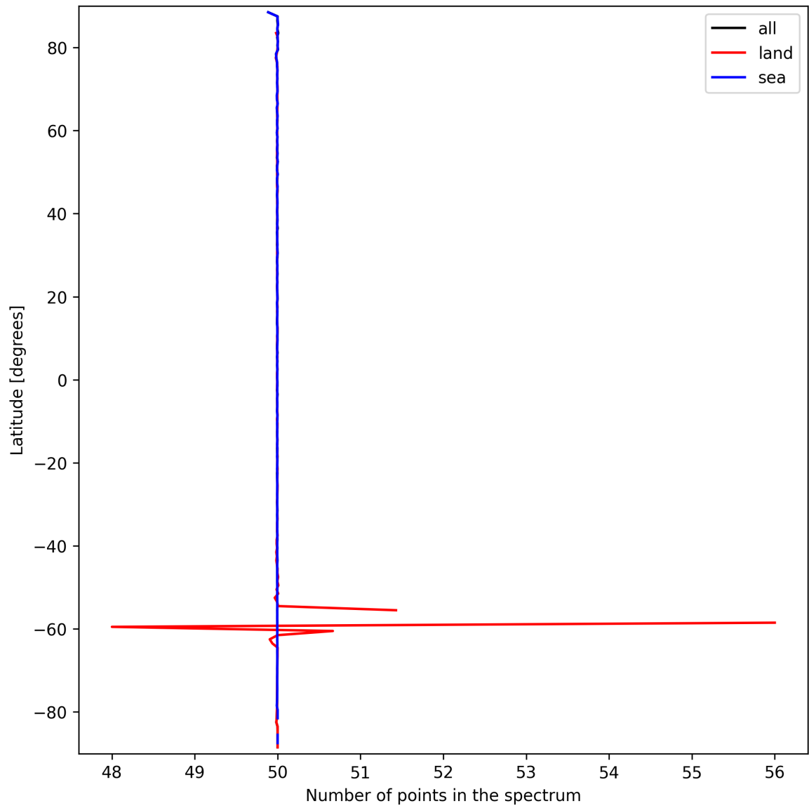
Figure 25: Zonal average of “Number of points in the spectrum” for 2025-03-20 to 2025-03-21.
