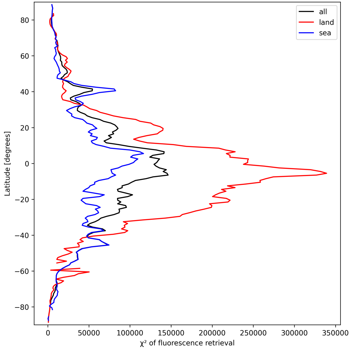
Figure 23: Zonal average of “ \chi^2 of fluorescence retrieval” for 2025-03-20 to 2025-03-21.
