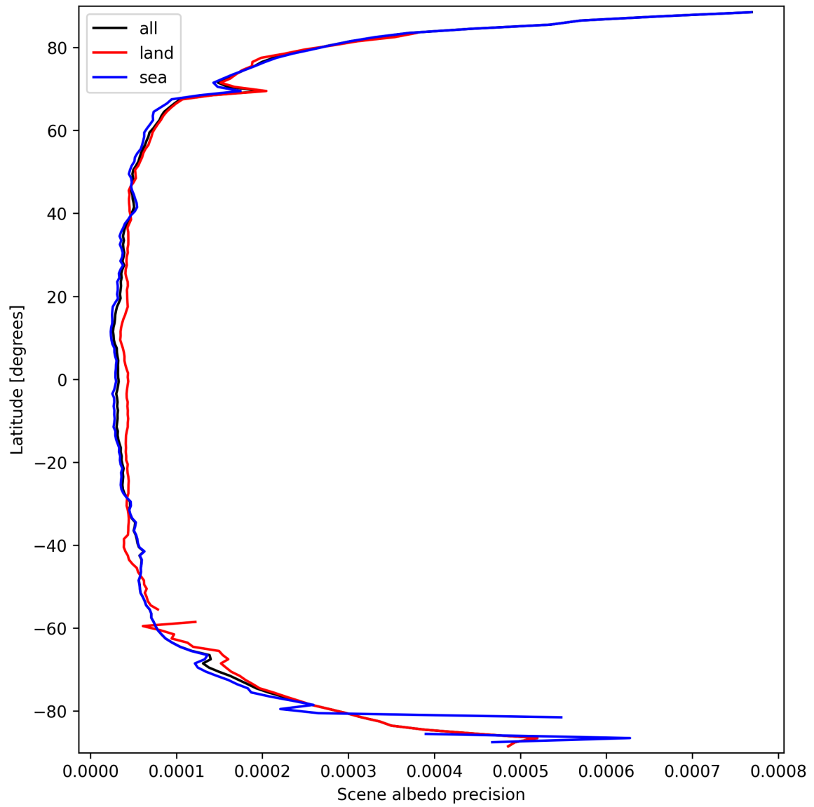
Figure 16: Zonal average of “Scene albedo precision” for 2025-03-20 to 2025-03-21.
