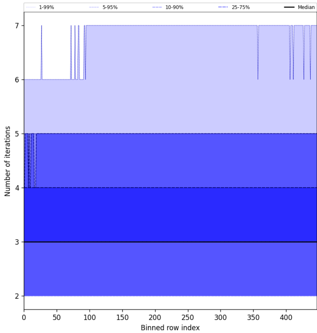
Figure 54: Along track statistics of “Number of iterations” for 2025-03-20 to 2025-03-21
