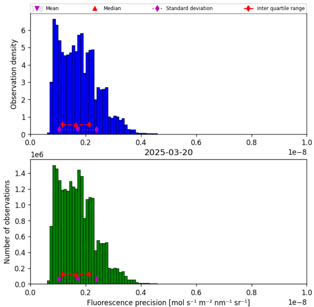
Figure 39: Histogram of “Fluorescence precision” for 2025-03-20 to 2025-03-21
