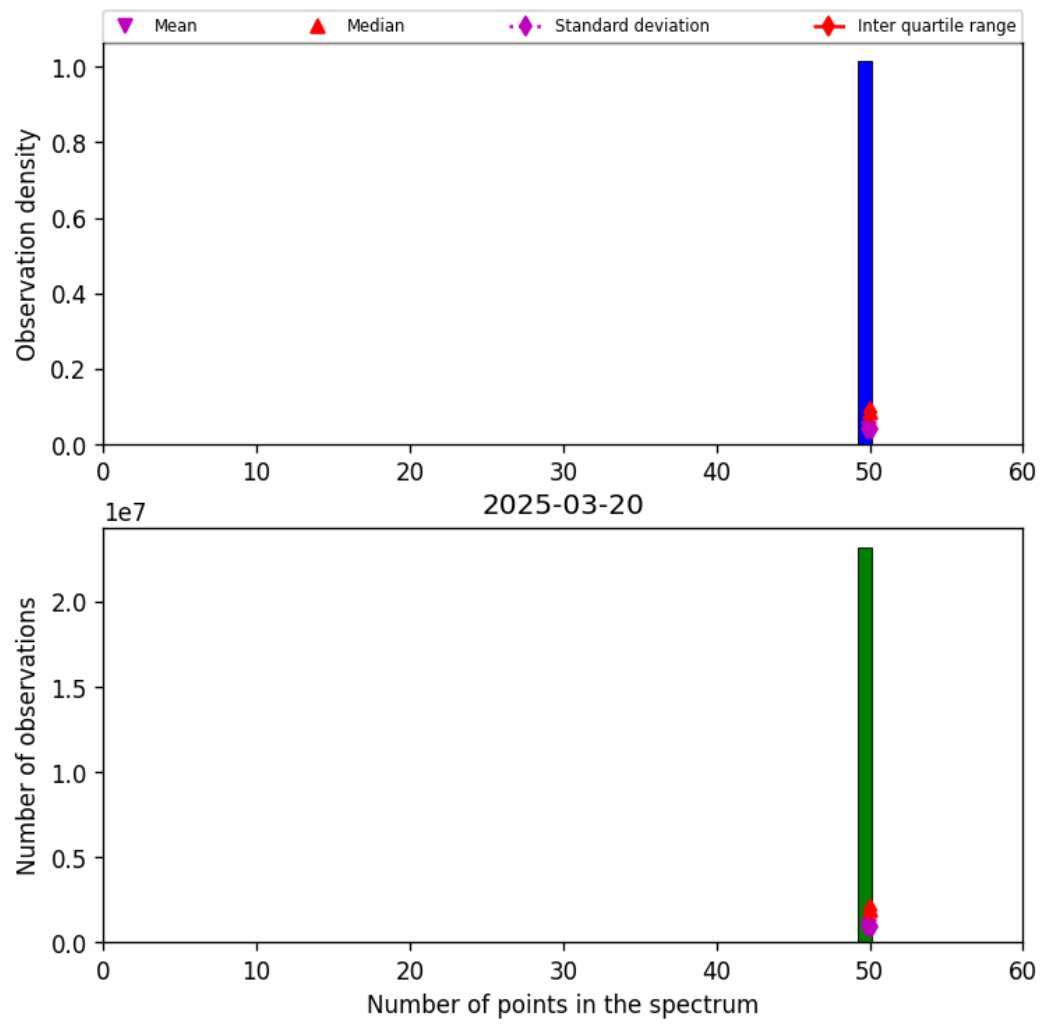
Figure 42: Histogram of “Number of points in the spectrum” for 2025-03-20 to 2025-03-21
