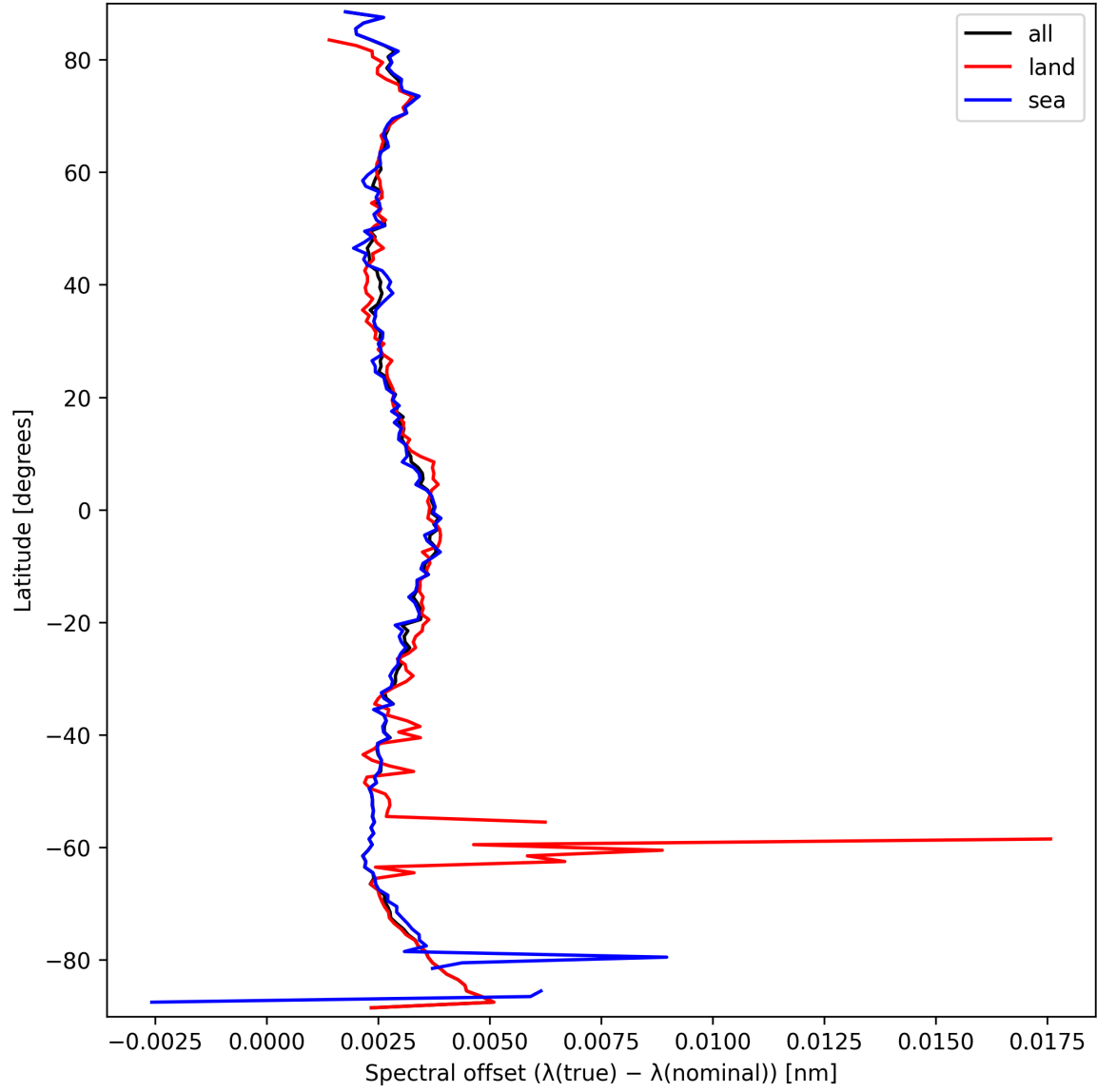
Figure 26: Zonal average of “Spectral offset ( \lambda_{\text{true}} - \lambda_{\text{nominal}} )” for 2025-03-20 to 2025-03-21.
