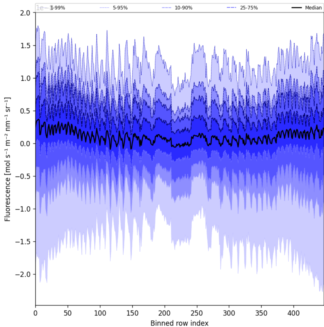
Figure 55: Along track statistics of “Fluorescence” for 2025-03-20 to 2025-03-21
