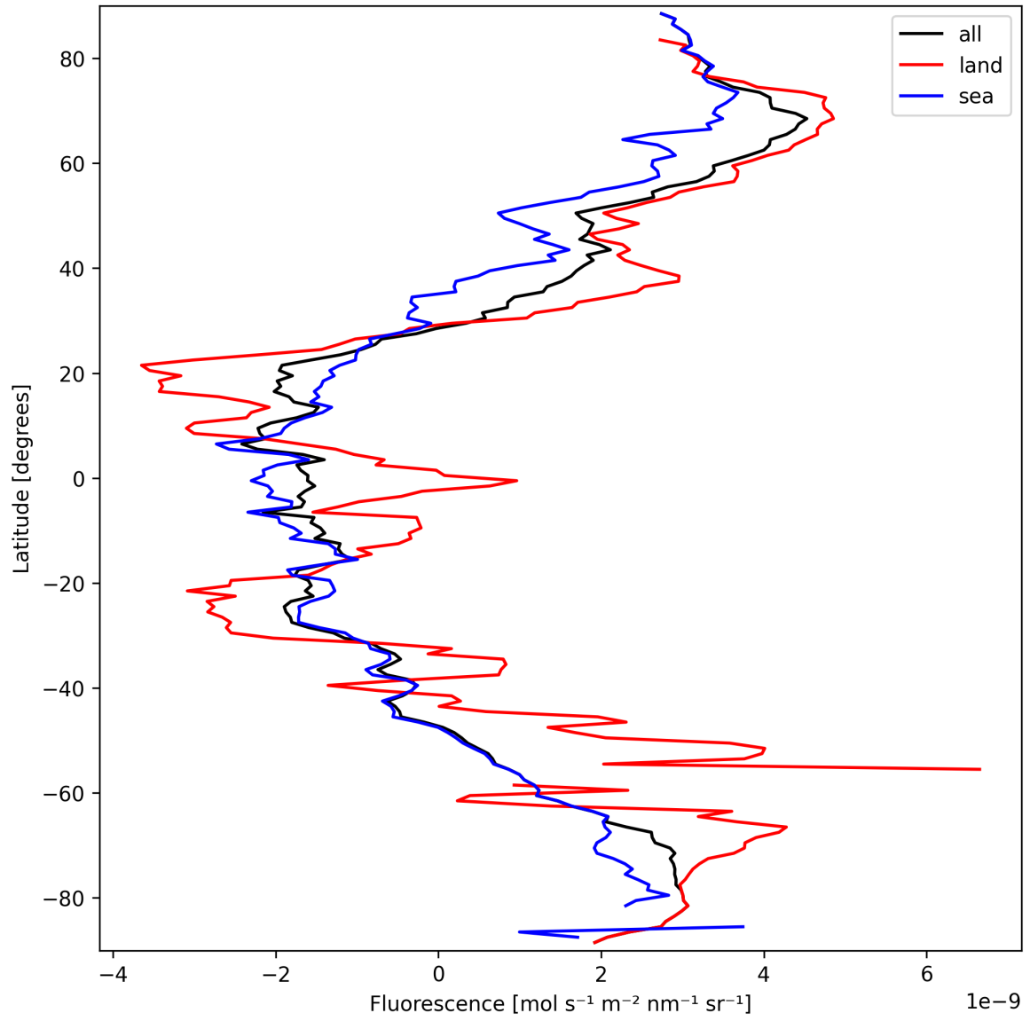
Figure 21: Zonal average of “Fluorescence” for 2025-03-20 to 2025-03-21.
