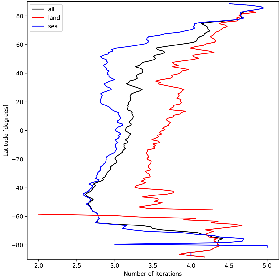
Figure 20: Zonal average of “Number of iterations” for 2025-03-20 to 2025-03-21.
