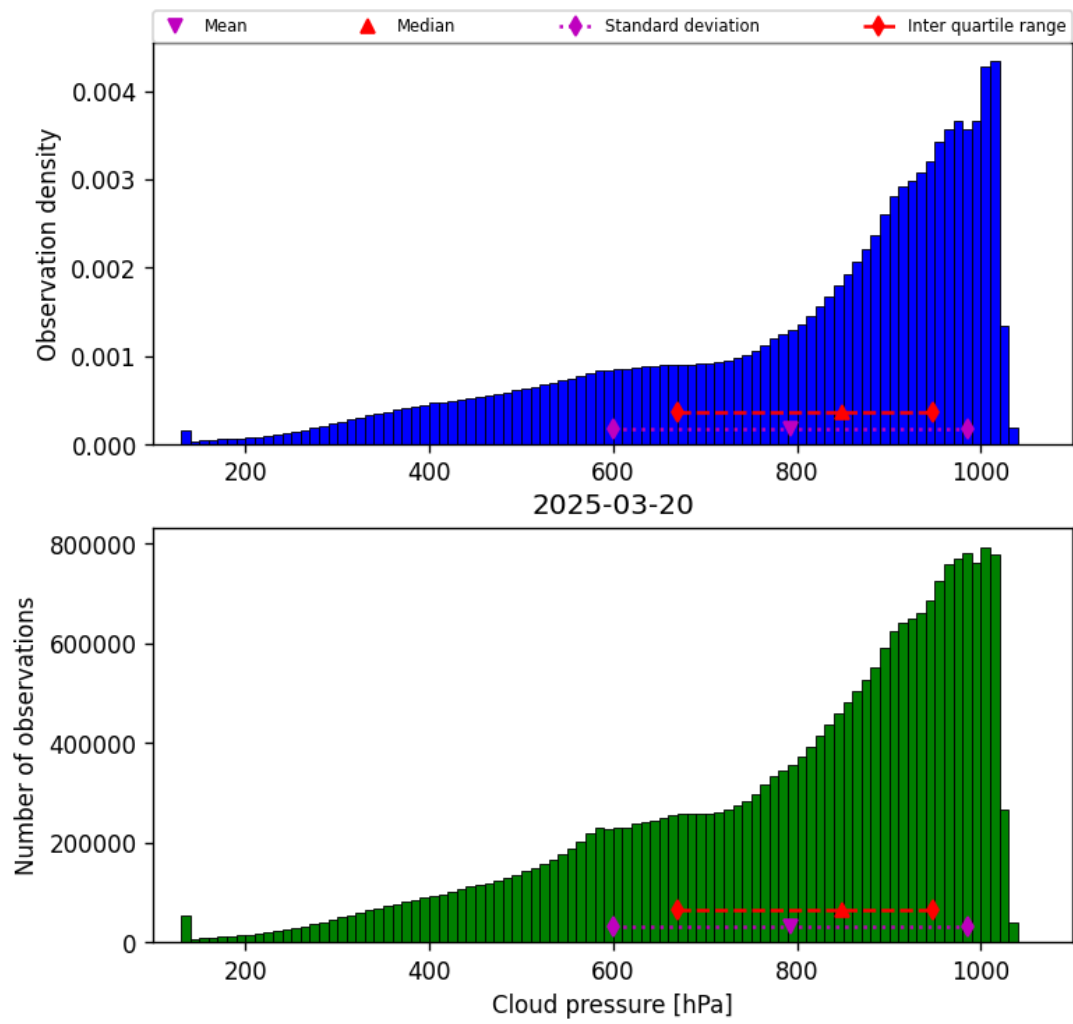
Figure 28: Histogram of “Cloud pressure” for 2025-03-20 to 2025-03-21
