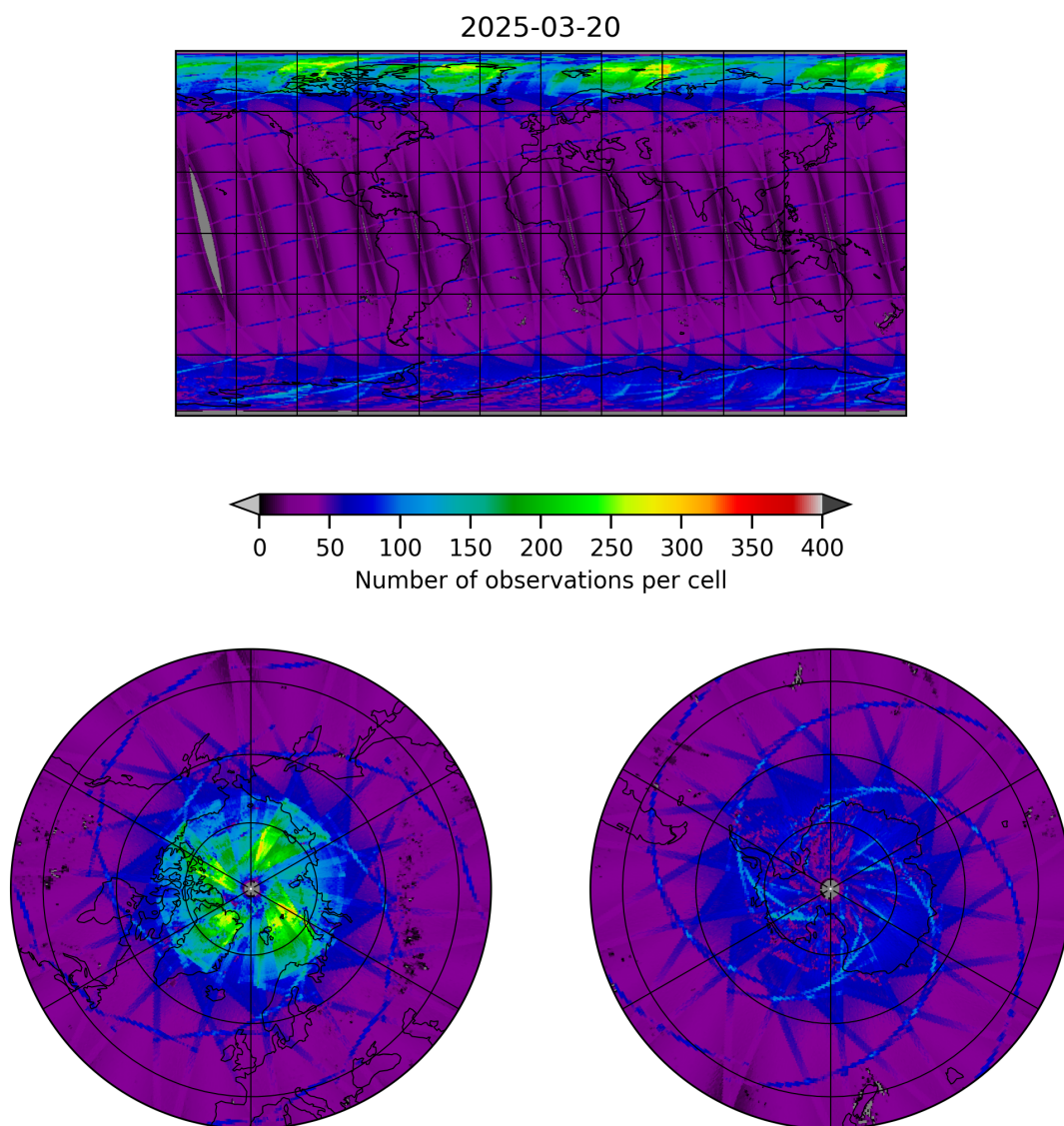
Figure 9: Map of the number of observations for 2025-03-20 to 2025-03-21
