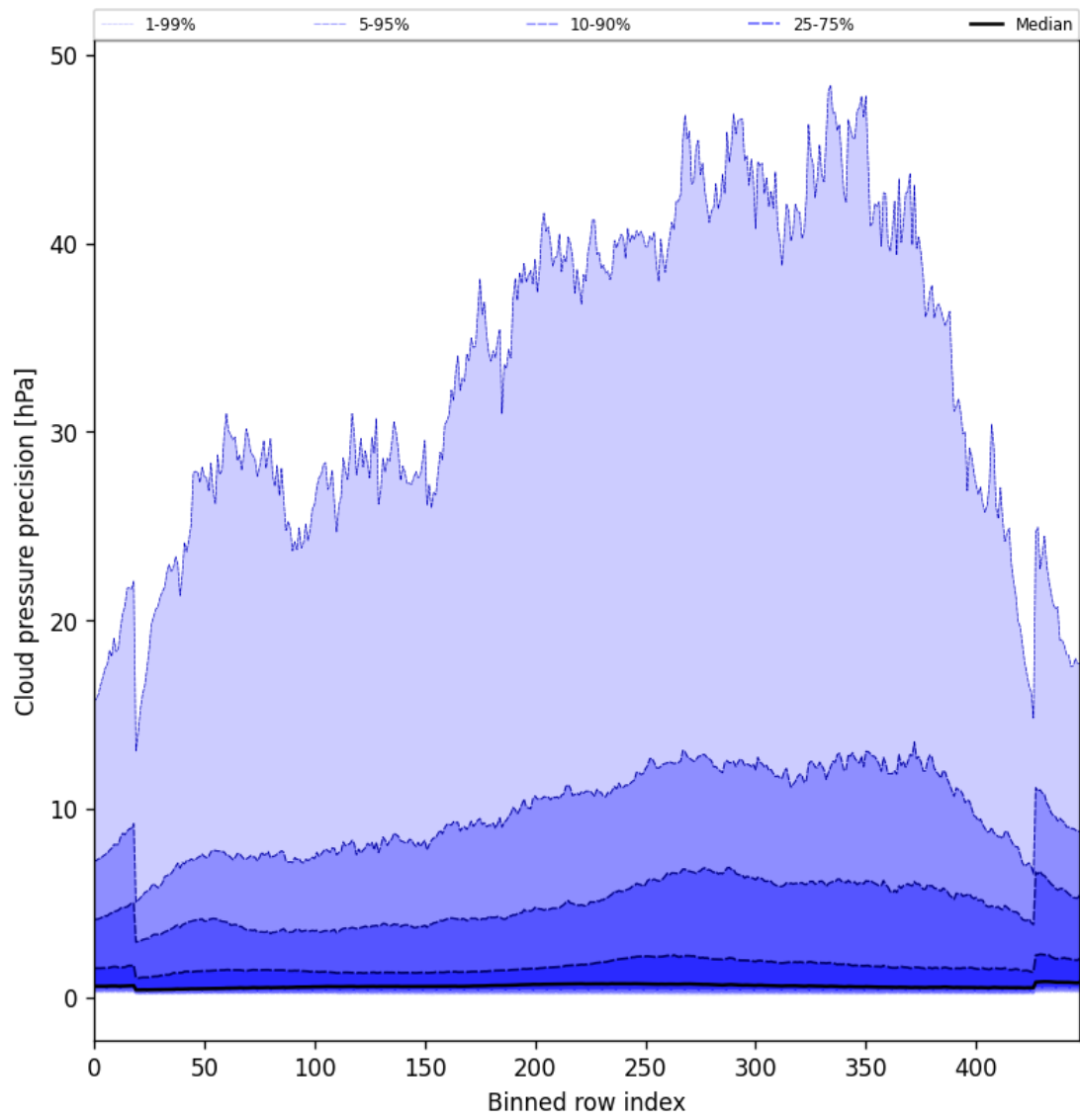
Figure 46: Along track statistics of “Cloud pressure precision” for 2025-03-20 to 2025-03-21
