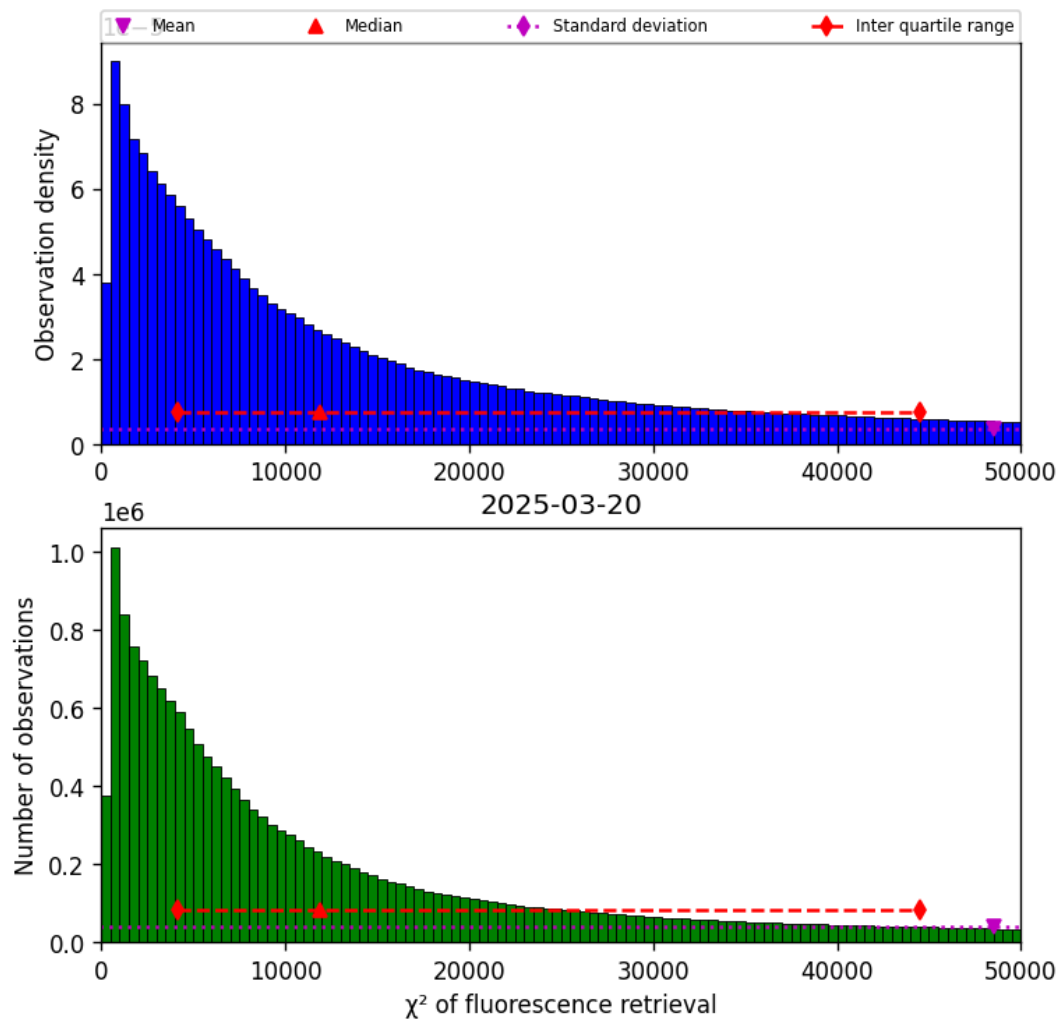
Figure 40: Histogram of “ \chi^2 of fluorescence retrieval” for 2025-03-20 to 2025-03-21
