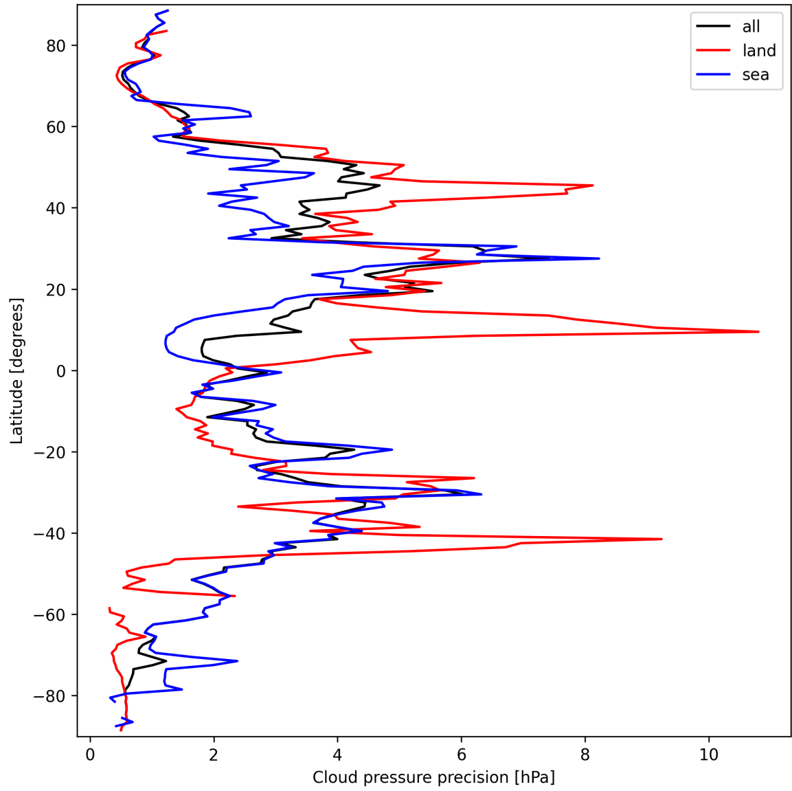
Figure 12: Zonal average of “Cloud pressure precision” for 2025-03-20 to 2025-03-21.
