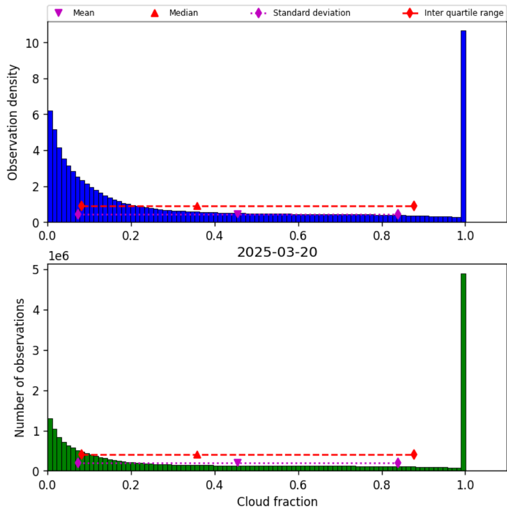
Figure 30: Histogram of “Cloud fraction” for 2025-03-20 to 2025-03-21
