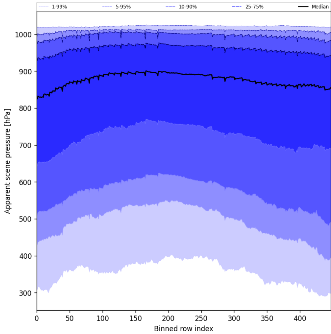
Figure 51: Along track statistics of “Apparent scene pressure” for 2025-03-20 to 2025-03-21
