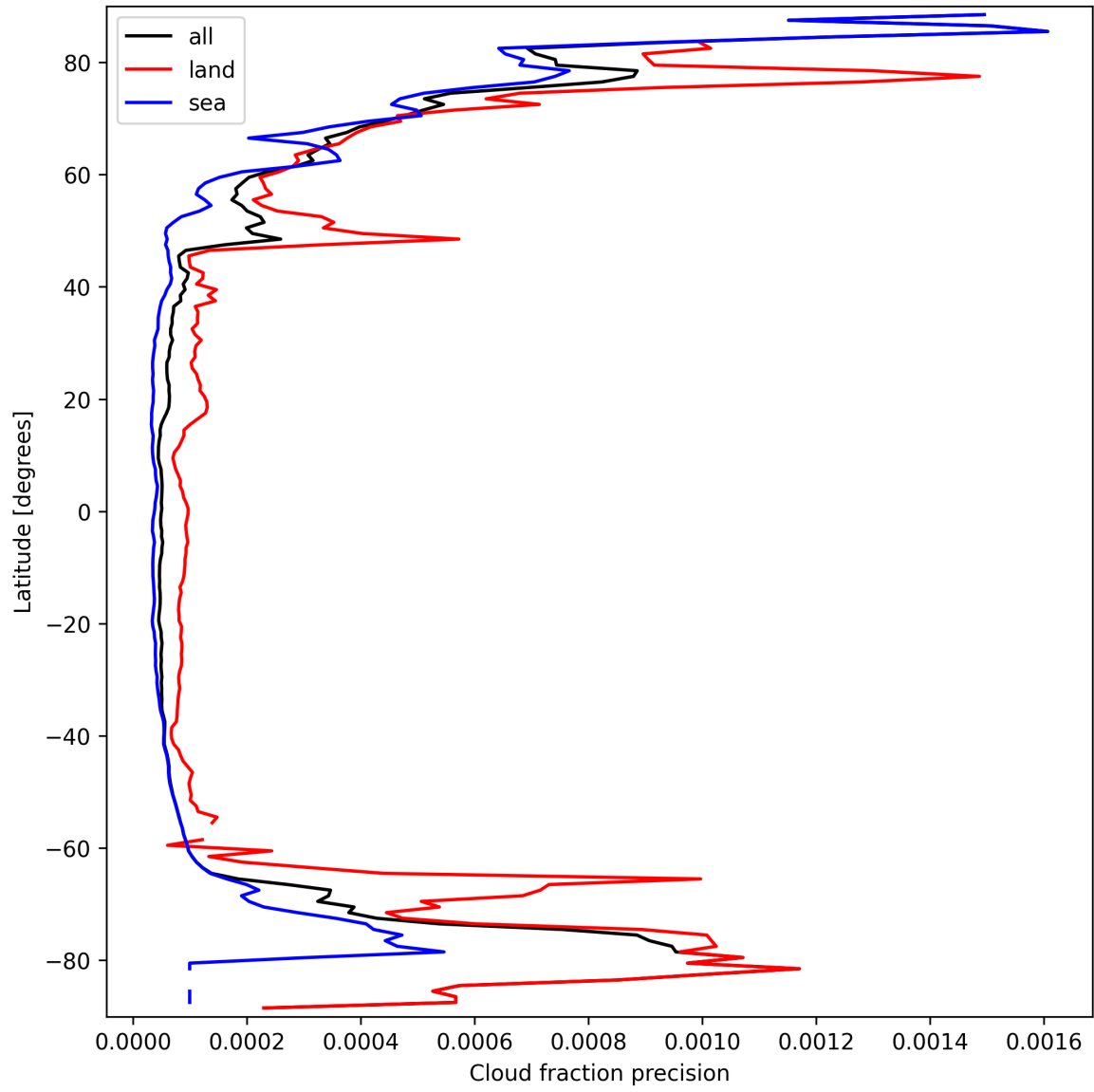
Figure 14: Zonal average of “Cloud fraction precision” for 2025-03-20 to 2025-03-21.
