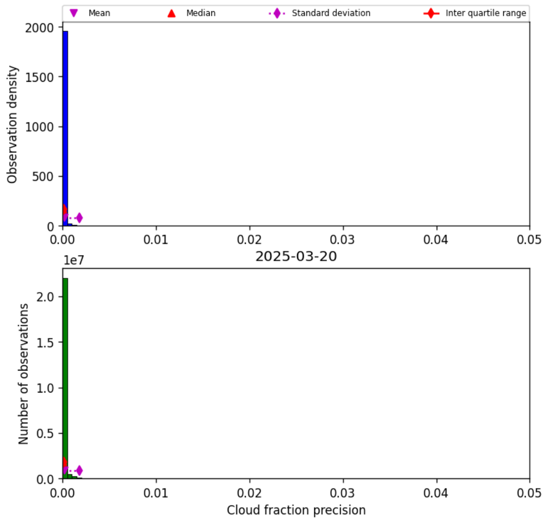
Figure 31: Histogram of “Cloud fraction precision” for 2025-03-20 to 2025-03-21
