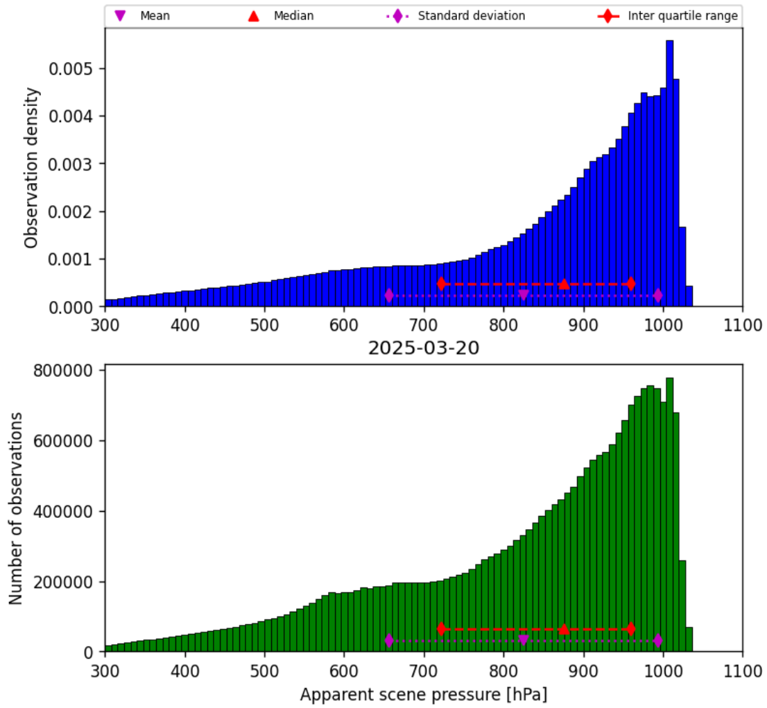
Figure 34: Histogram of “Apparent scene pressure” for 2025-03-20 to 2025-03-21
