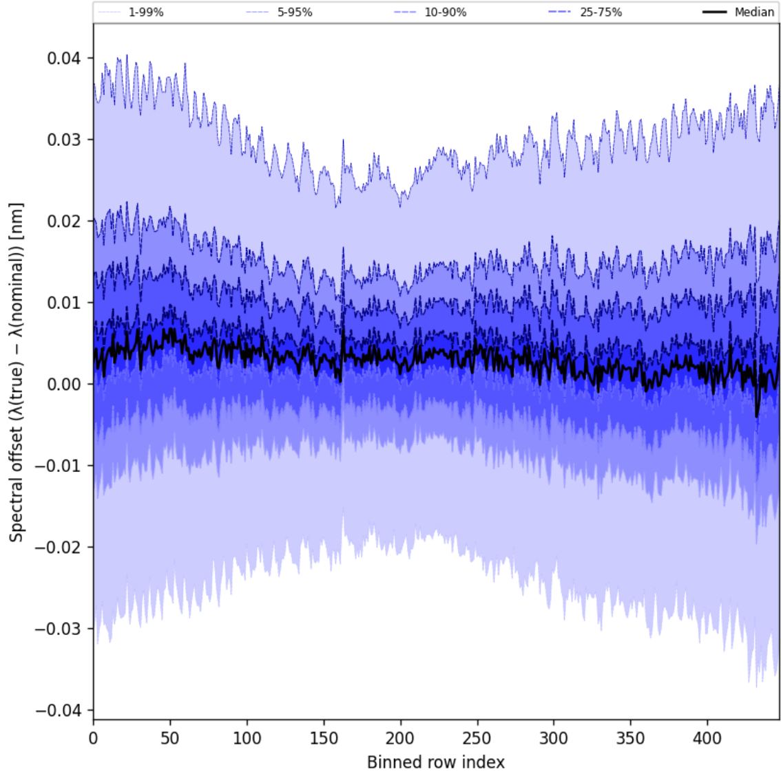
Figure 60: Along track statistics of “Spectral offset ( \lambda_{\text{true}} - \lambda_{\text{nominal}} )” for 2025-03-20 to 2025-03-21
