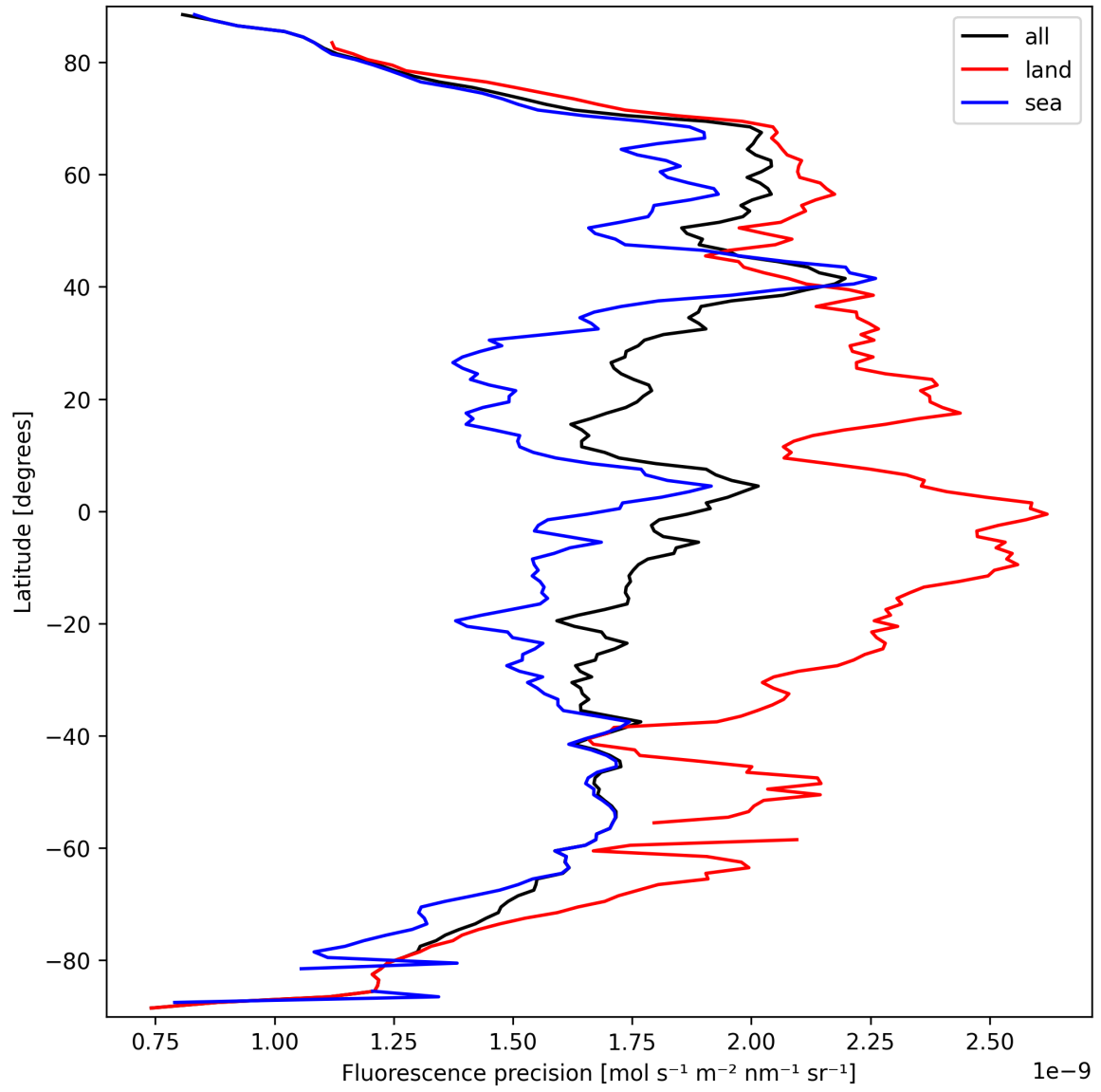
Figure 22: Zonal average of “Fluorescence precision” for 2025-03-20 to 2025-03-21.
