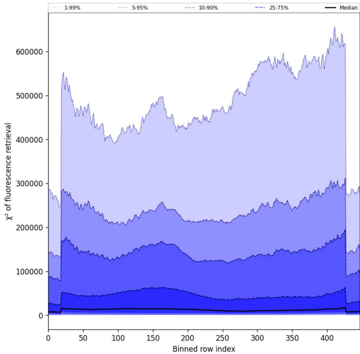
Figure 57: Along track statistics of “ \chi^2 of fluorescence retrieval” for 2025-03-20 to 2025-03-21
