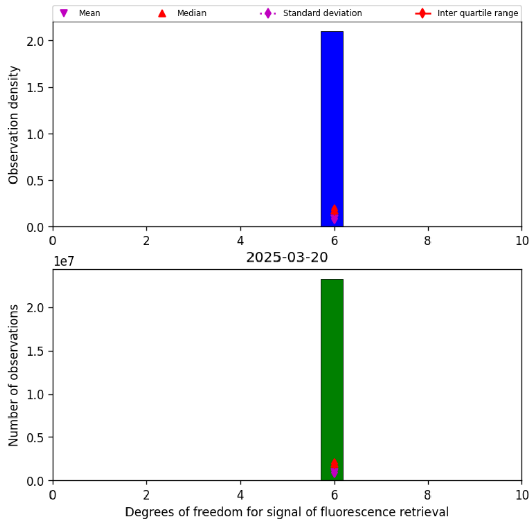
Figure 41: Histogram of “Degrees of freedom for signal of fluorescence retrieval” for 2025-03-20 to 2025-03-21
