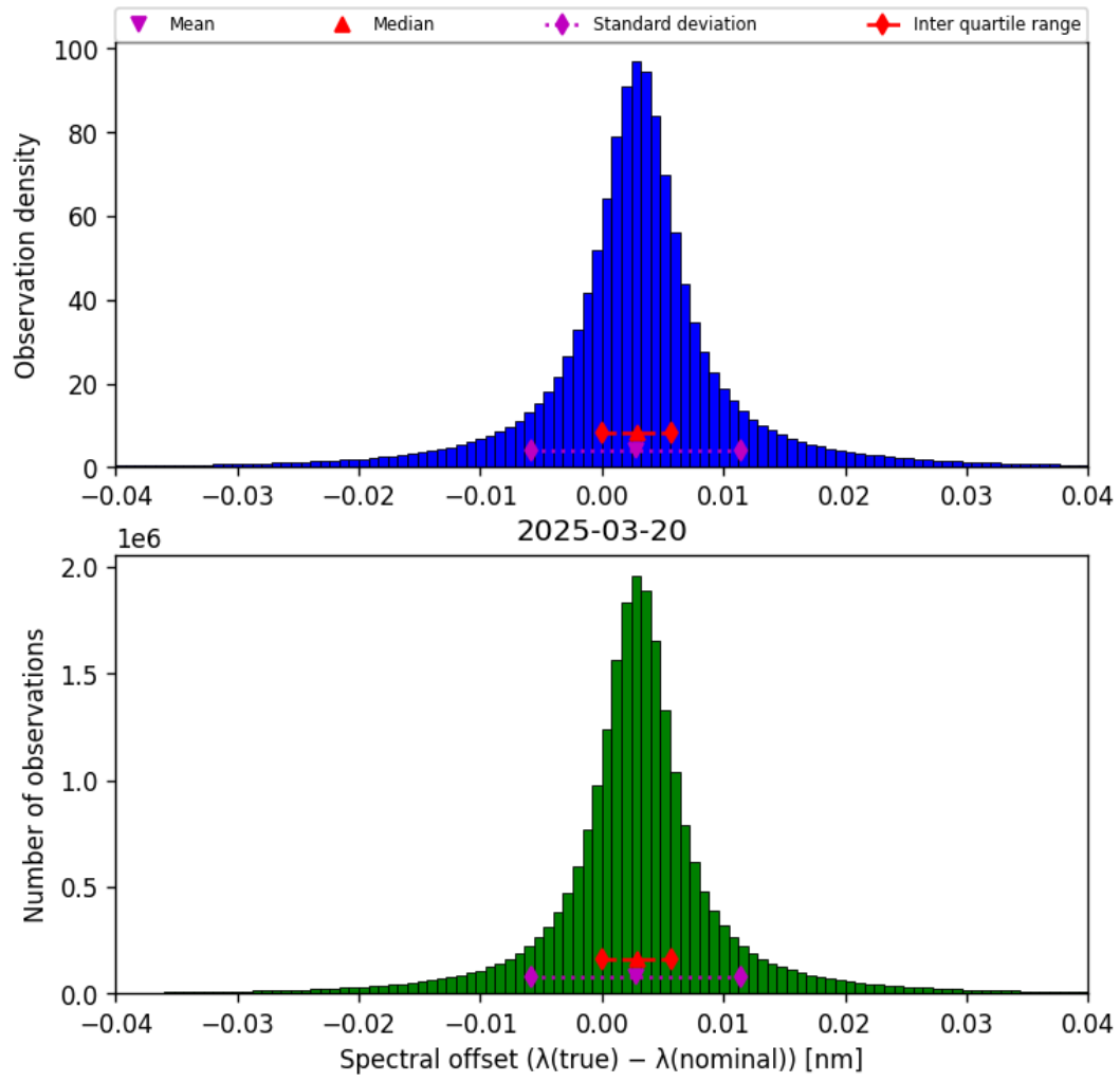
Figure 43: Histogram of “Spectral offset ( \lambda_{\text{true}} - \lambda_{\text{nominal}} )” for 2025-03-20 to 2025-03-21
