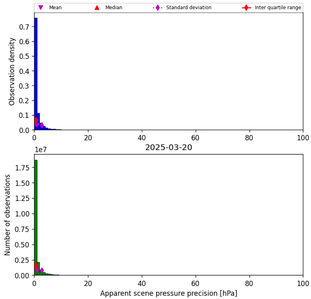
Figure 35: Histogram of “Apparent scene pressure precision” for 2025-03-20 to 2025-03-21
