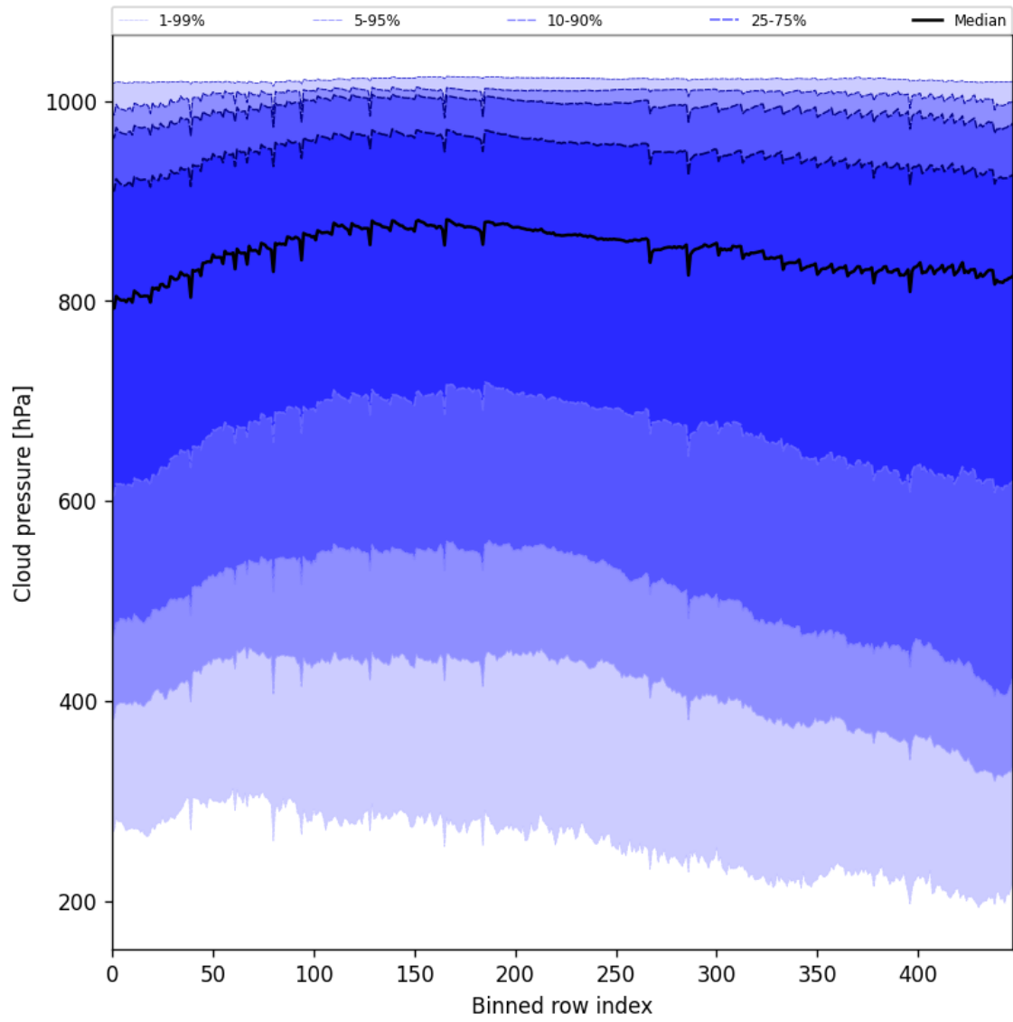
Figure 45: Along track statistics of “Cloud pressure” for 2025-03-20 to 2025-03-21
