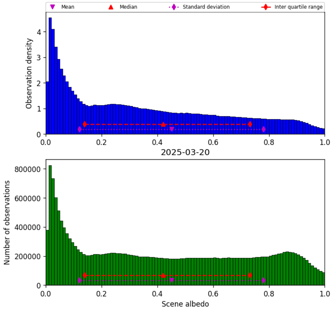
Figure 32: Histogram of “Scene albedo” for 2025-03-20 to 2025-03-21
