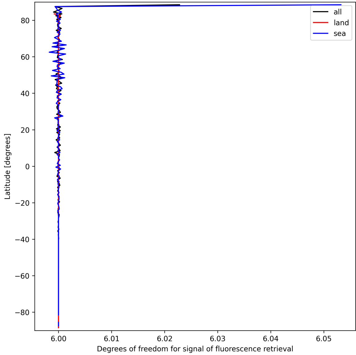
Figure 24: Zonal average of “Degrees of freedom for signal of fluorescence retrieval” for 2025-03-20 to 2025-03-21.
