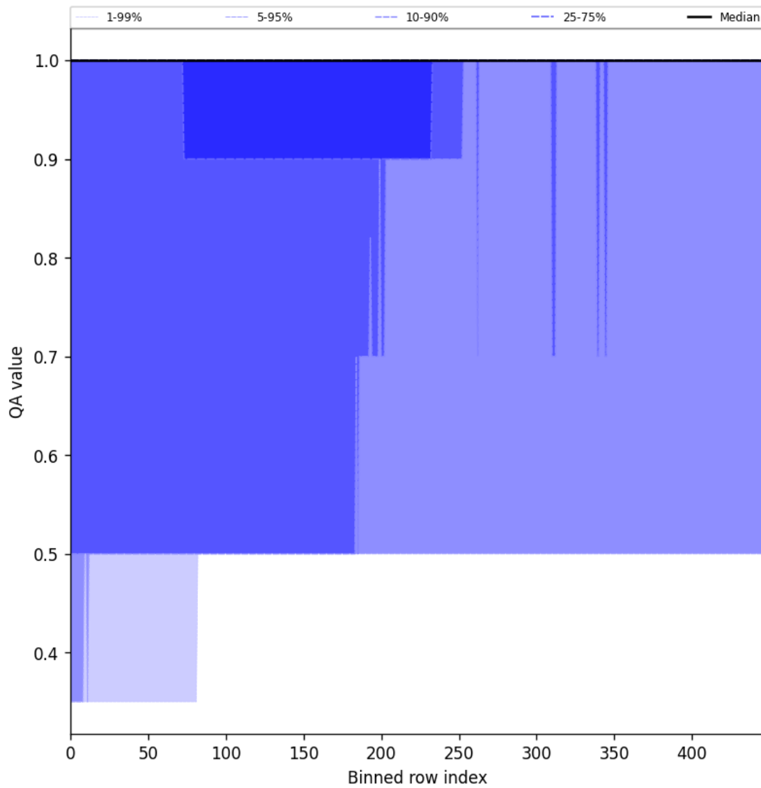
Figure 44: Along track statistics of “QA value” for 2025-03-20 to 2025-03-21
