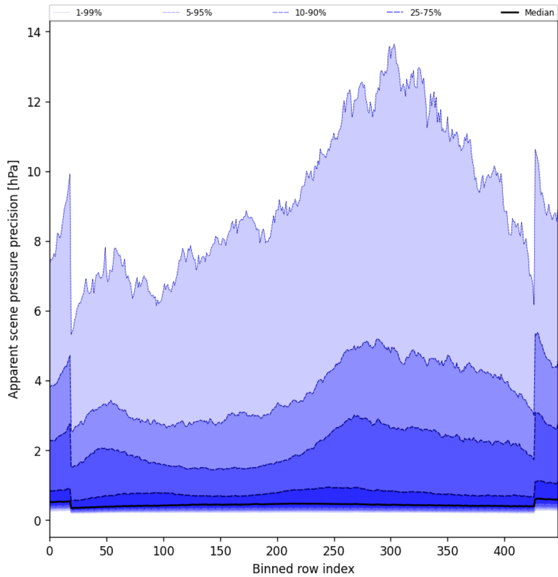
Figure 52: Along track statistics of “Apparent scene pressure precision” for 2025-03-20 to 2025-03-21
