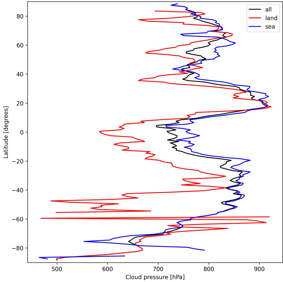
Figure 11: Zonal average of “Cloud pressure” for 2025-03-20 to 2025-03-21.
