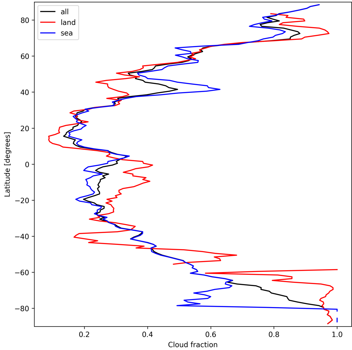
Figure 13: Zonal average of “Cloud fraction” for 2025-03-20 to 2025-03-21.
