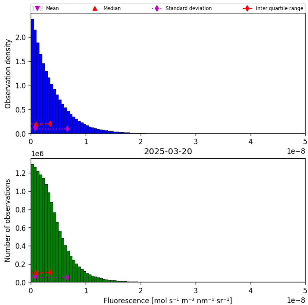
Figure 38: Histogram of “Fluorescence” for 2025-03-20 to 2025-03-21
