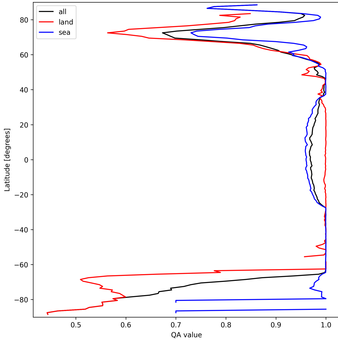
Figure 10: Zonal average of “QA value” for 2025-03-20 to 2025-03-21.
