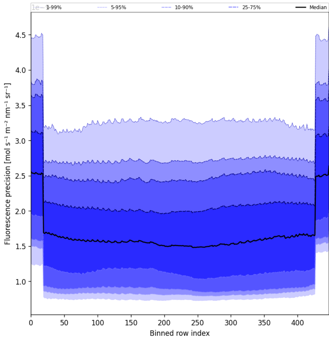
Figure 56: Along track statistics of “Fluorescence precision” for 2025-03-20 to 2025-03-21
