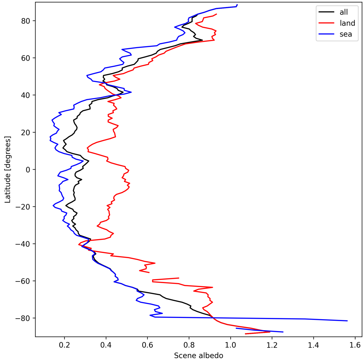
Figure 15: Zonal average of “Scene albedo” for 2025-03-20 to 2025-03-21.
