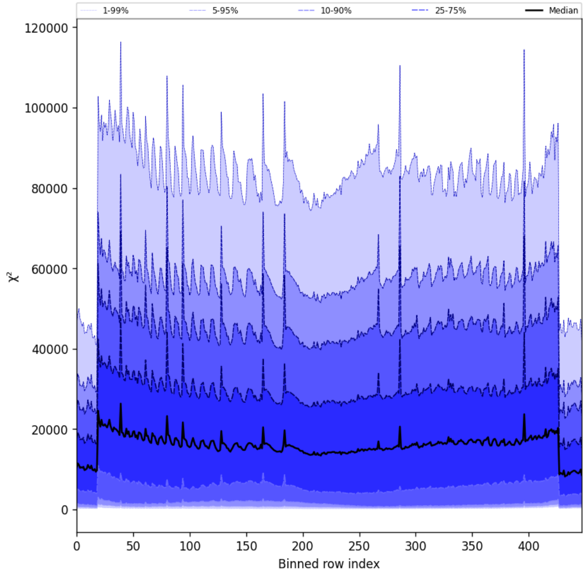
Figure 53: Along track statistics of “ \chi^2 ” for 2025-03-20 to 2025-03-21
