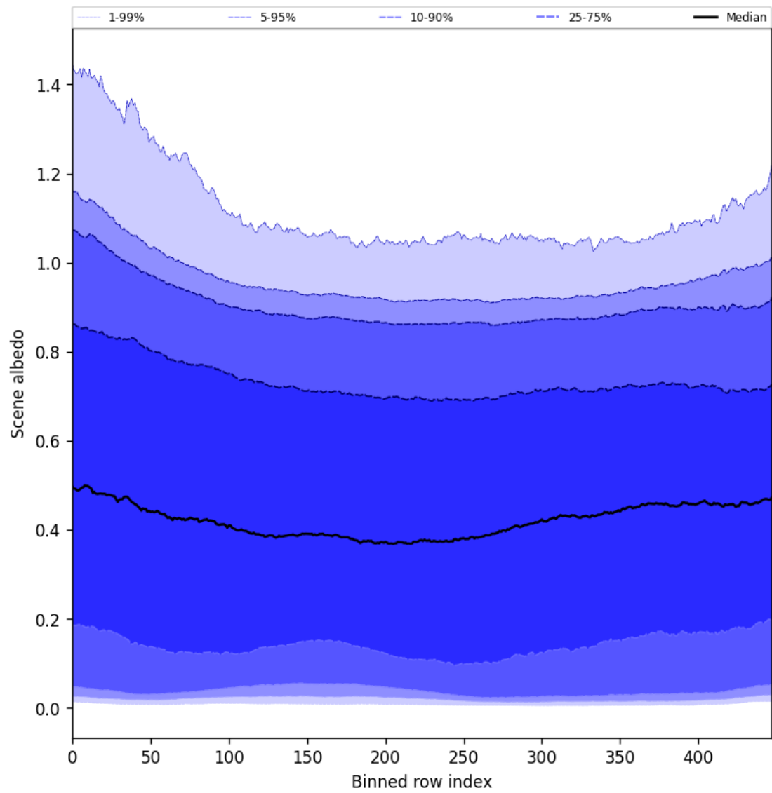
Figure 49: Along track statistics of “Scene albedo” for 2025-03-20 to 2025-03-21
