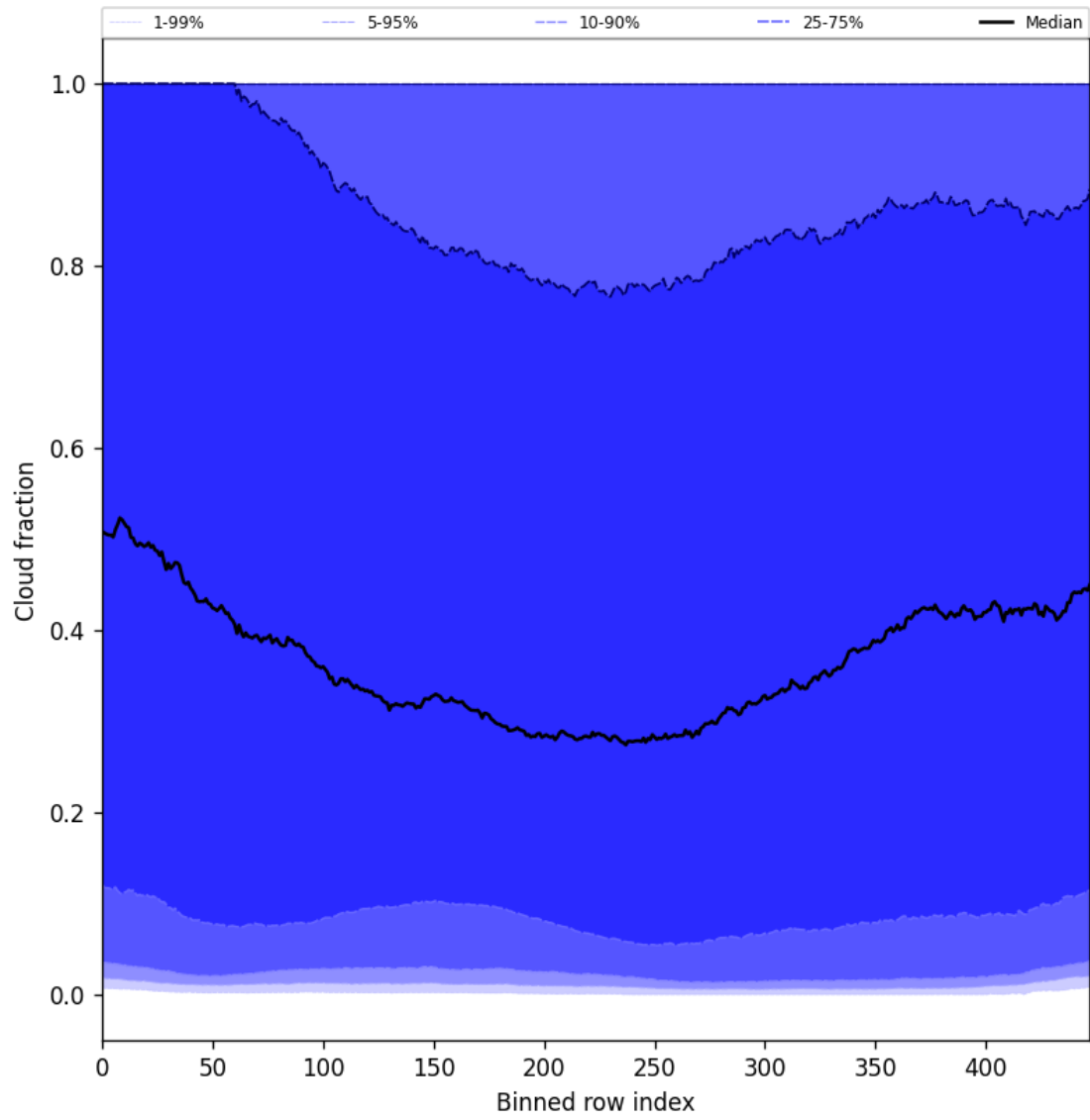
Figure 47: Along track statistics of “Cloud fraction” for 2025-03-20 to 2025-03-21
