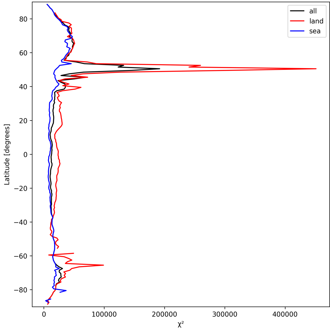
Figure 19: Zonal average of “ \chi^2 ” for 2025-03-20 to 2025-03-21.
