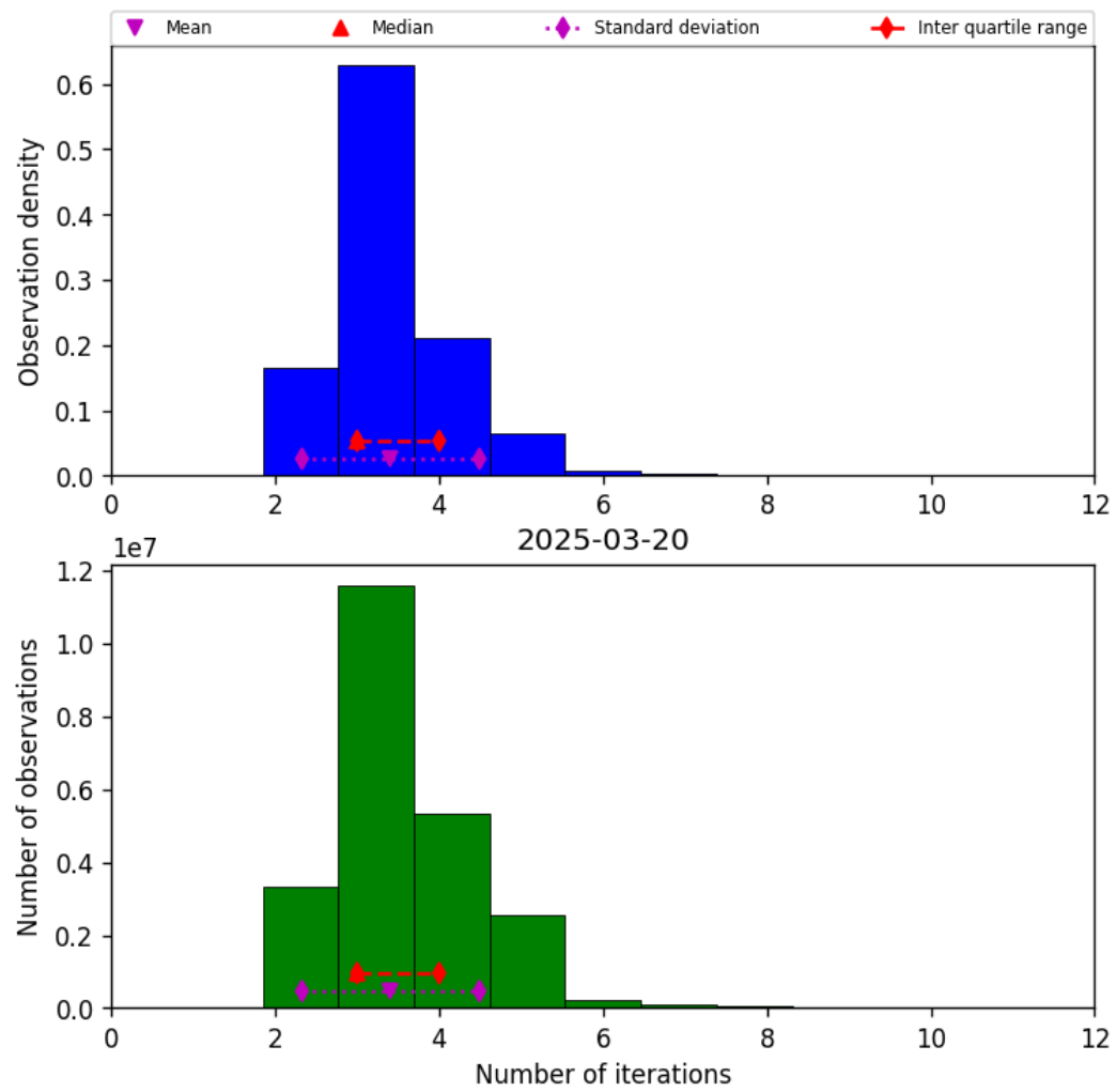
Figure 37: Histogram of “Number of iterations” for 2025-03-20 to 2025-03-21
