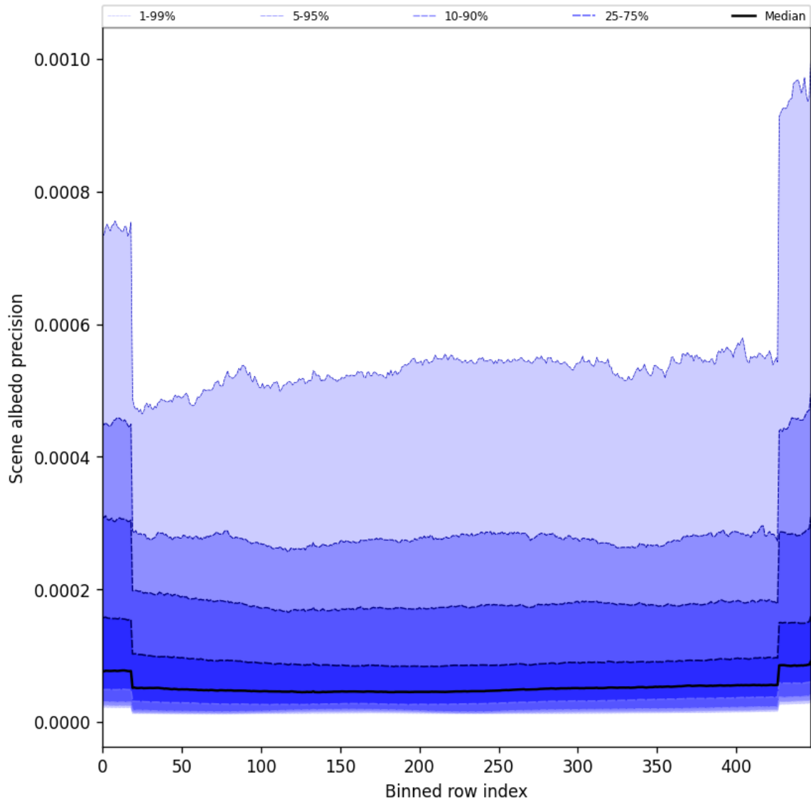
Figure 50: Along track statistics of “Scene albedo precision” for 2025-03-20 to 2025-03-21
