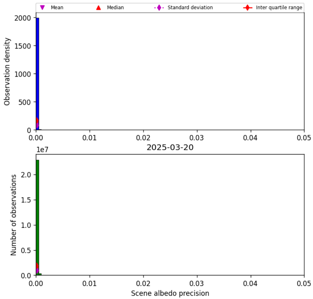
Figure 33: Histogram of “Scene albedo precision” for 2025-03-20 to 2025-03-21
