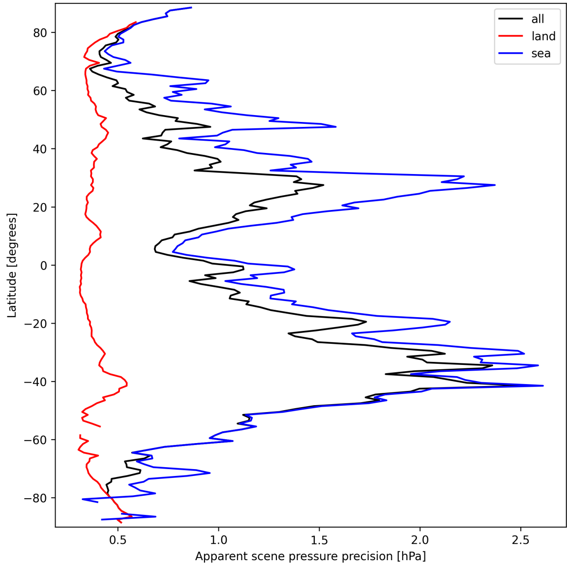
Figure 18: Zonal average of “Apparent scene pressure precision” for 2025-03-20 to 2025-03-21.
