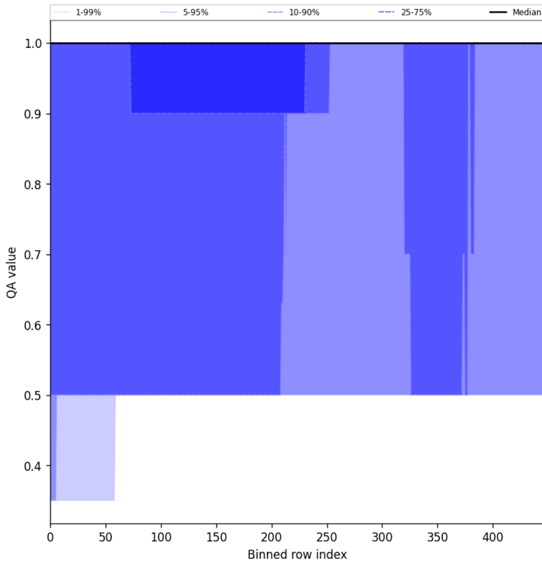
Figure 44: Along track statistics of “QA value” for 2025-03-25 to 2025-03-26
