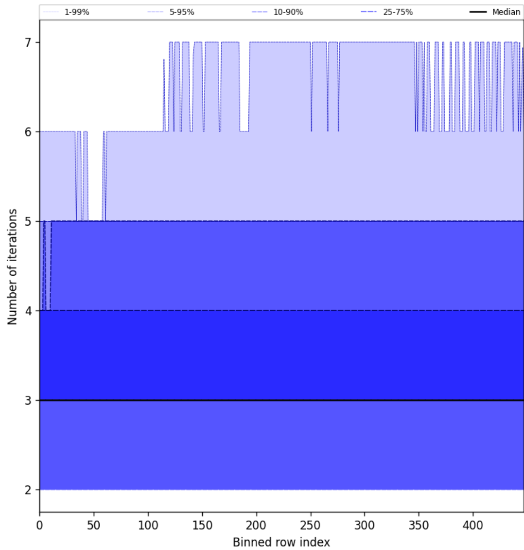
Figure 54: Along track statistics of “Number of iterations” for 2025-03-25 to 2025-03-26
