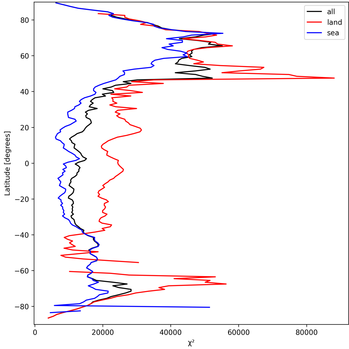
Figure 19: Zonal average of “ \chi^2 ” for 2025-03-25 to 2025-03-26.
