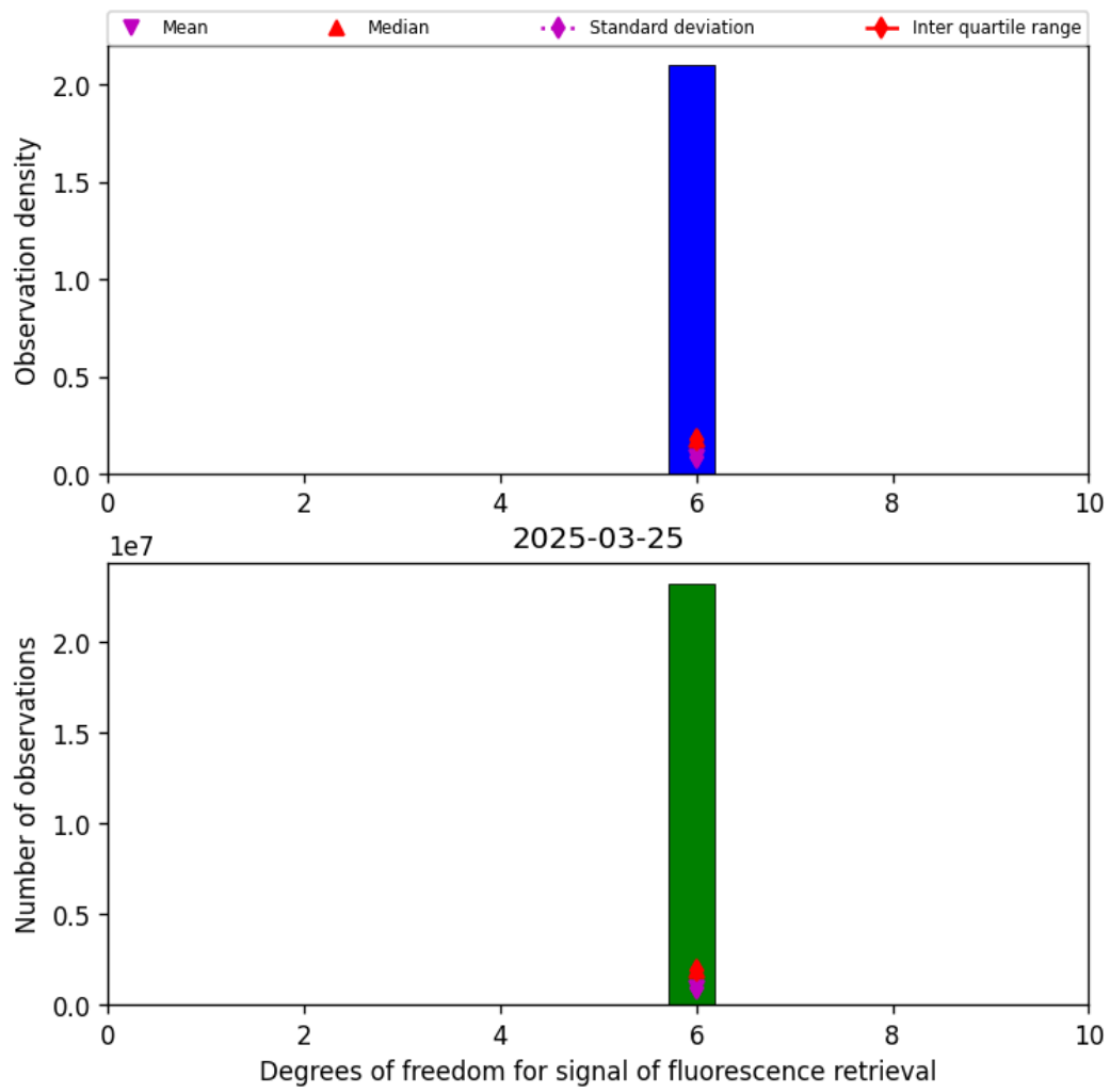
Figure 41: Histogram of “Degrees of freedom for signal of fluorescence retrieval” for 2025-03-25 to 2025-03-26
