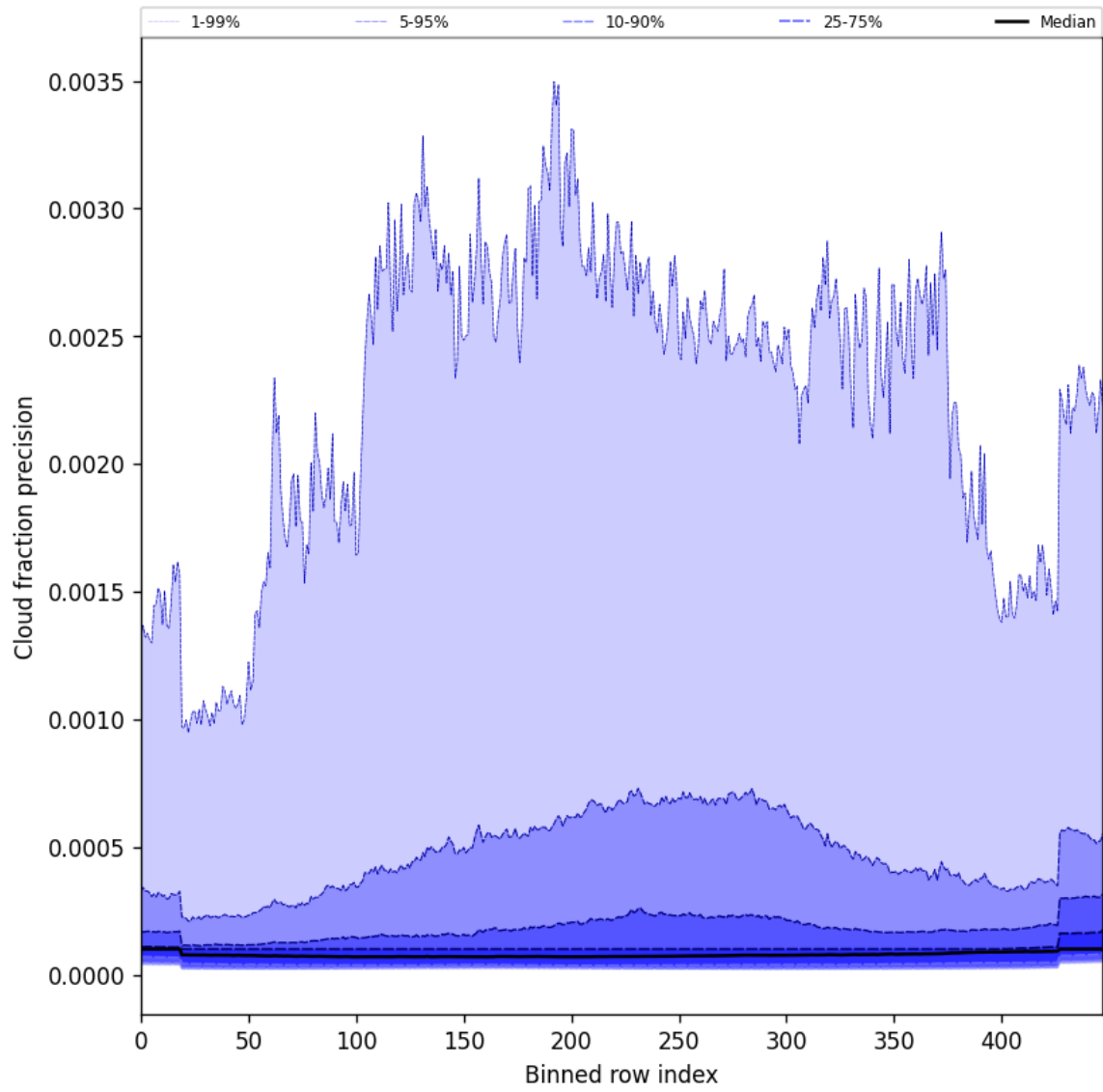
Figure 48: Along track statistics of “Cloud fraction precision” for 2025-03-25 to 2025-03-26
