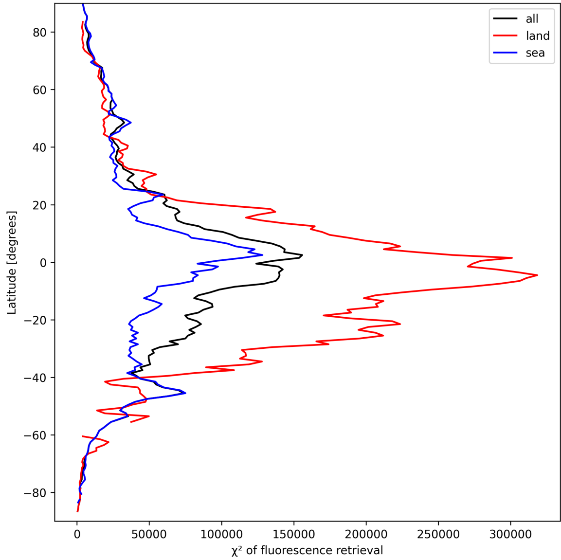
Figure 23: Zonal average of “ \chi^2 of fluorescence retrieval” for 2025-03-25 to 2025-03-26.
