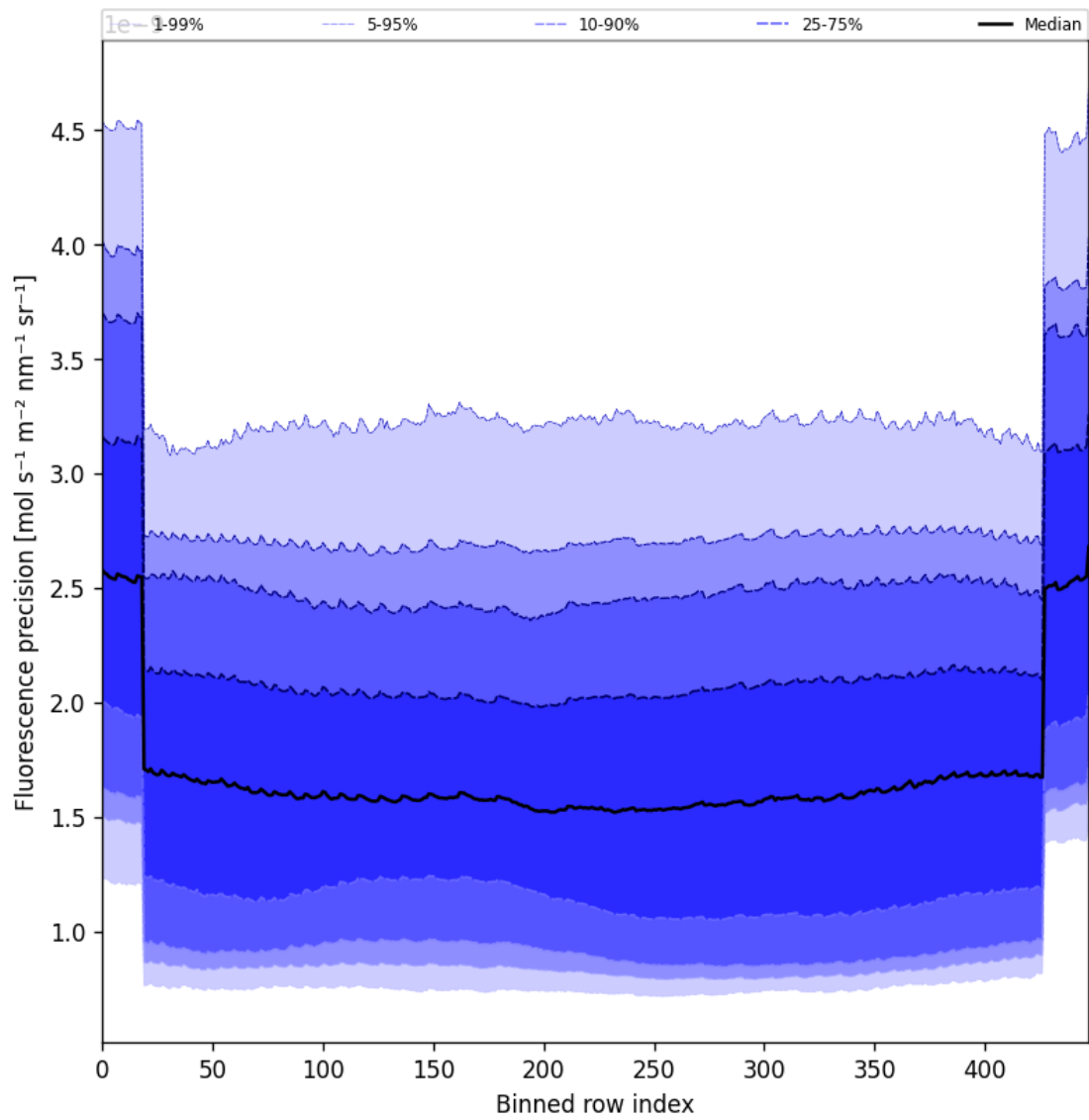
Figure 56: Along track statistics of “Fluorescence precision” for 2025-03-25 to 2025-03-26
