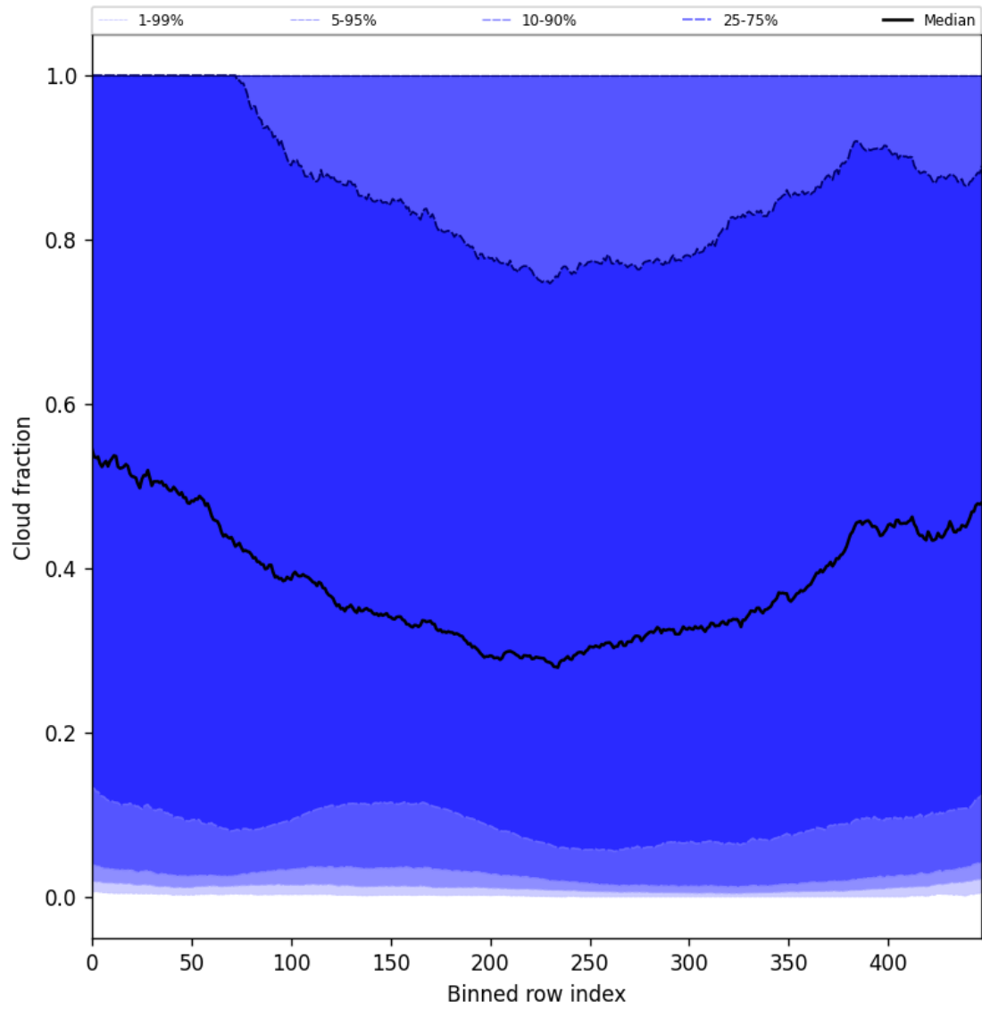
Figure 47: Along track statistics of “Cloud fraction” for 2025-03-25 to 2025-03-26
