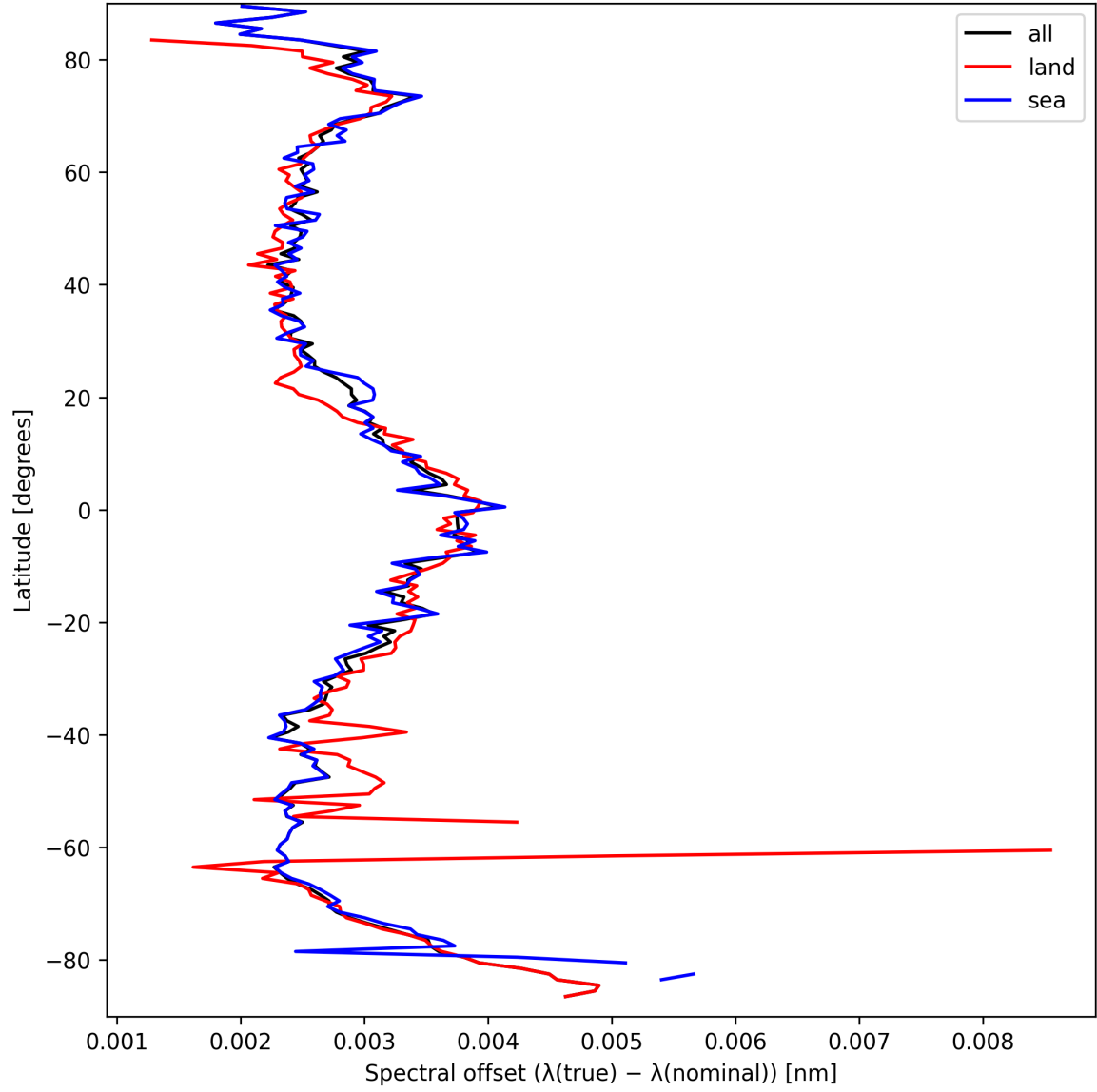
Figure 26: Zonal average of “Spectral offset ( \lambda_{\text{true}} - \lambda_{\text{nominal}} )” for 2025-03-25 to 2025-03-26.
