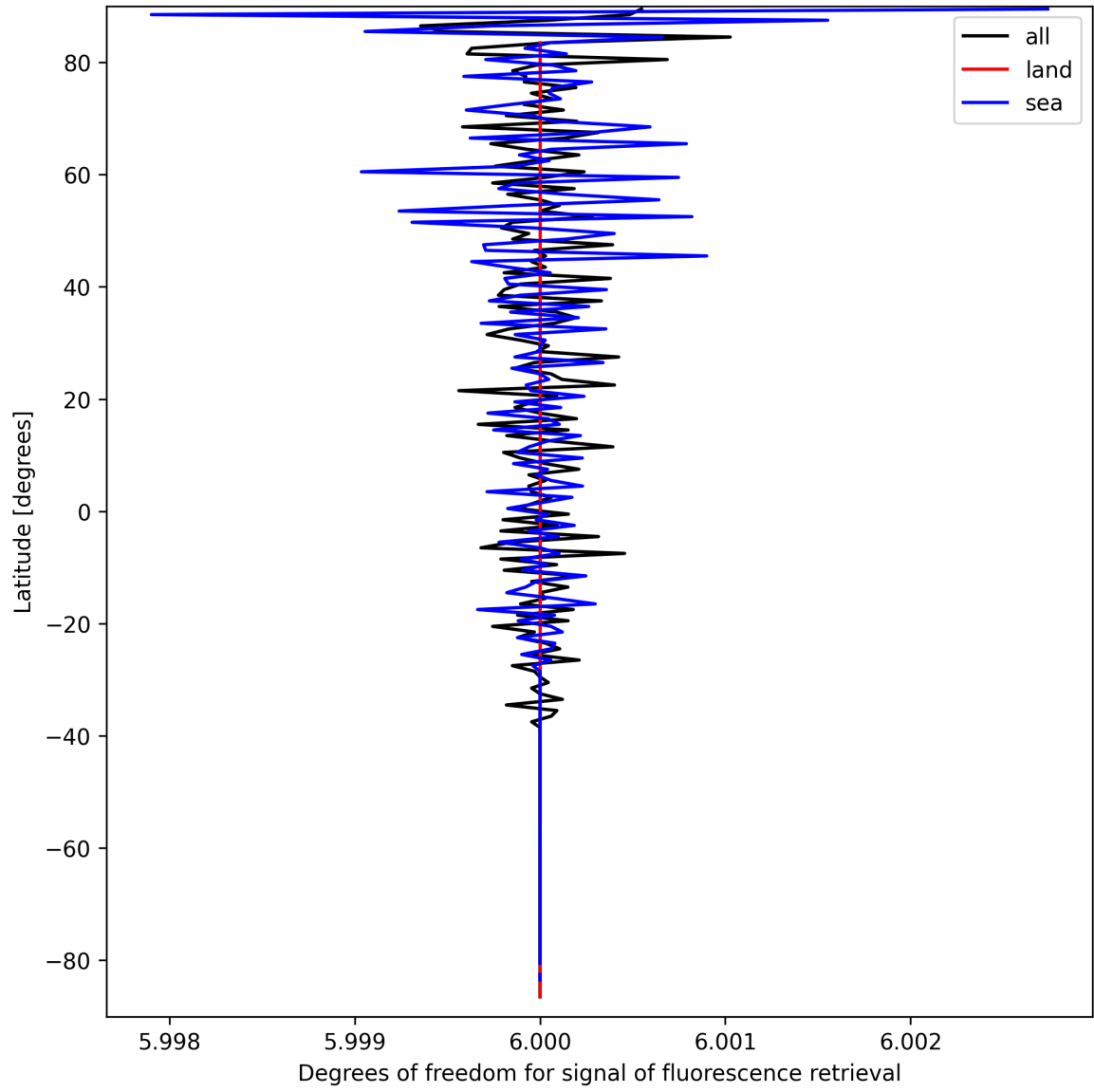
Figure 24: Zonal average of “Degrees of freedom for signal of fluorescence retrieval” for 2025-03-25 to 2025-03-26.
