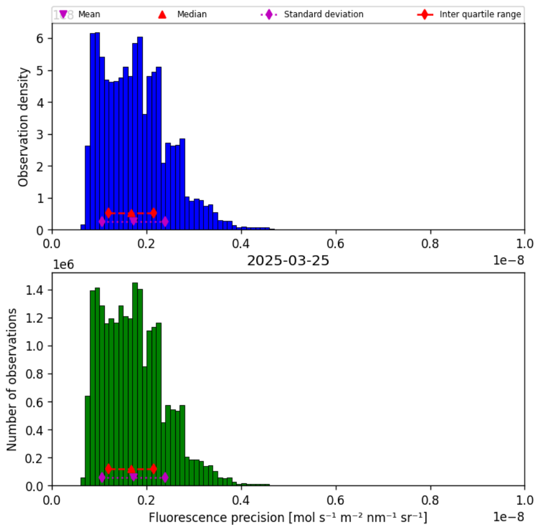
Figure 39: Histogram of “Fluorescence precision” for 2025-03-25 to 2025-03-26
