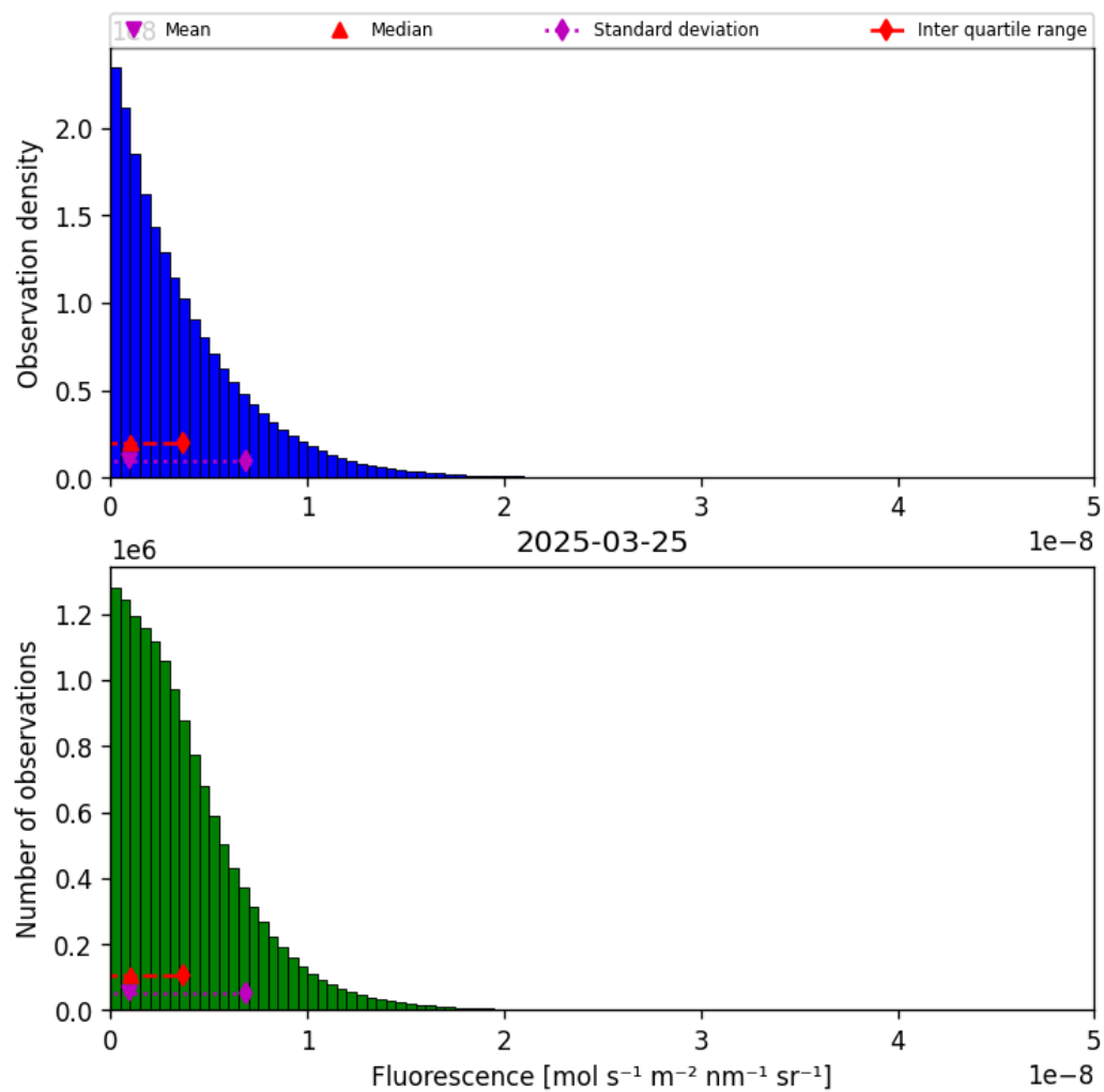
Figure 38: Histogram of “Fluorescence” for 2025-03-25 to 2025-03-26
