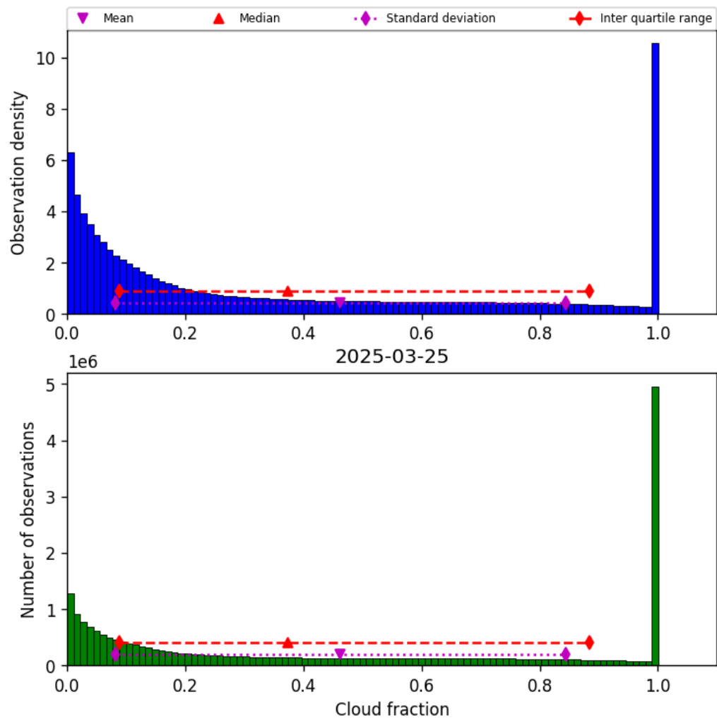
Figure 30: Histogram of “Cloud fraction” for 2025-03-25 to 2025-03-26
