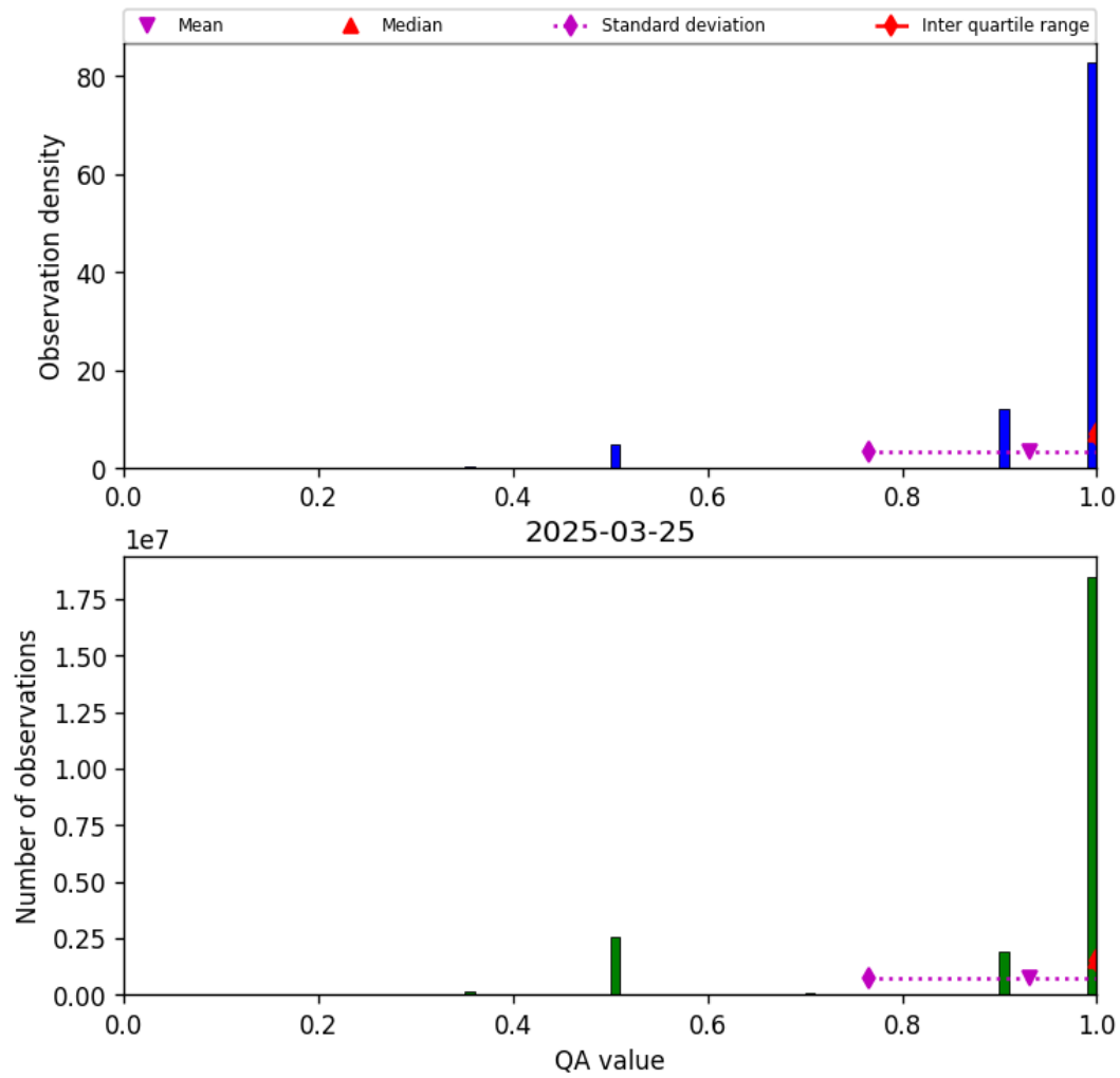
Figure 27: Histogram of “QA value” for 2025-03-25 to 2025-03-26
