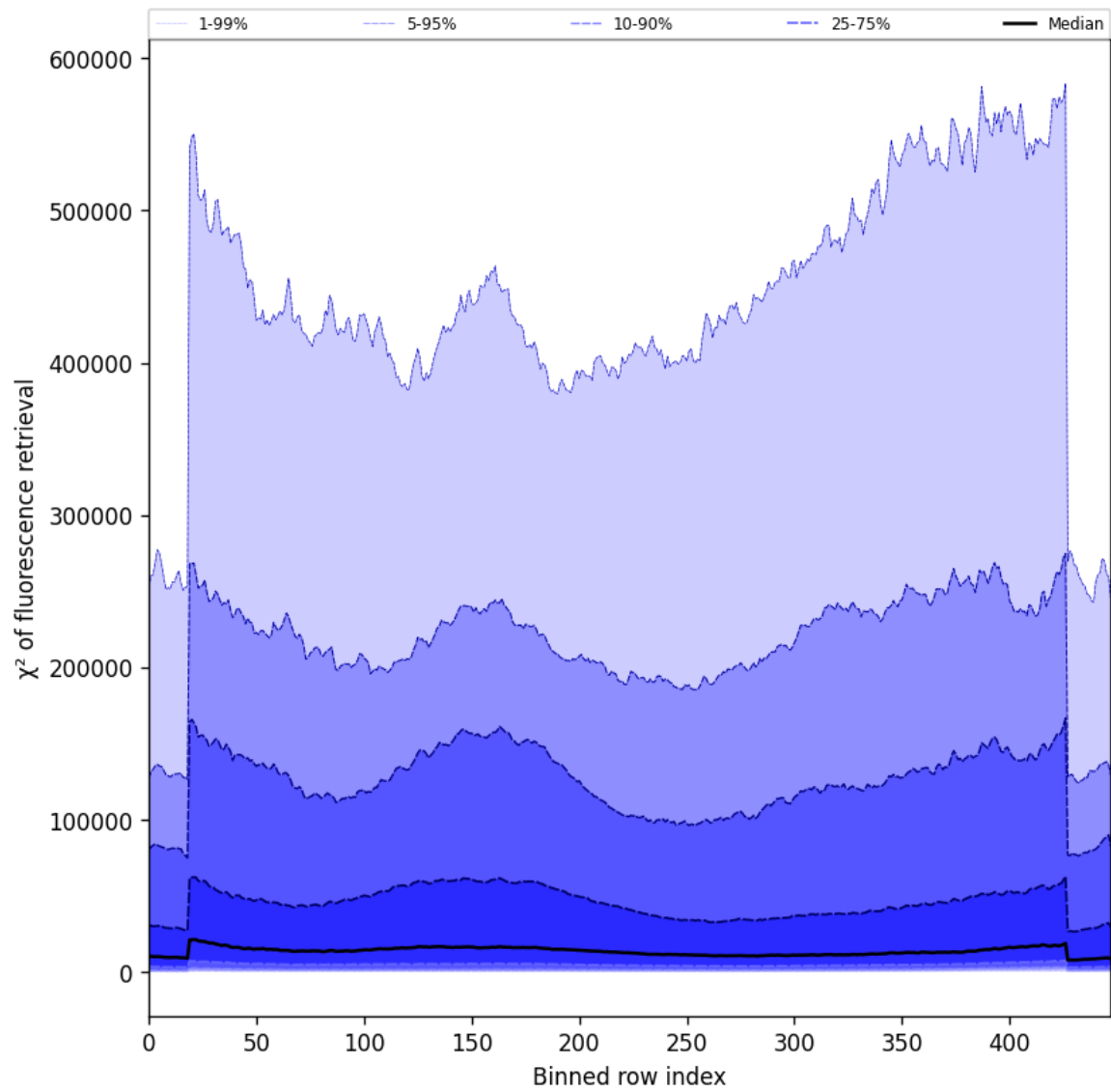
Figure 57: Along track statistics of “ \chi^2 of fluorescence retrieval” for 2025-03-25 to 2025-03-26
