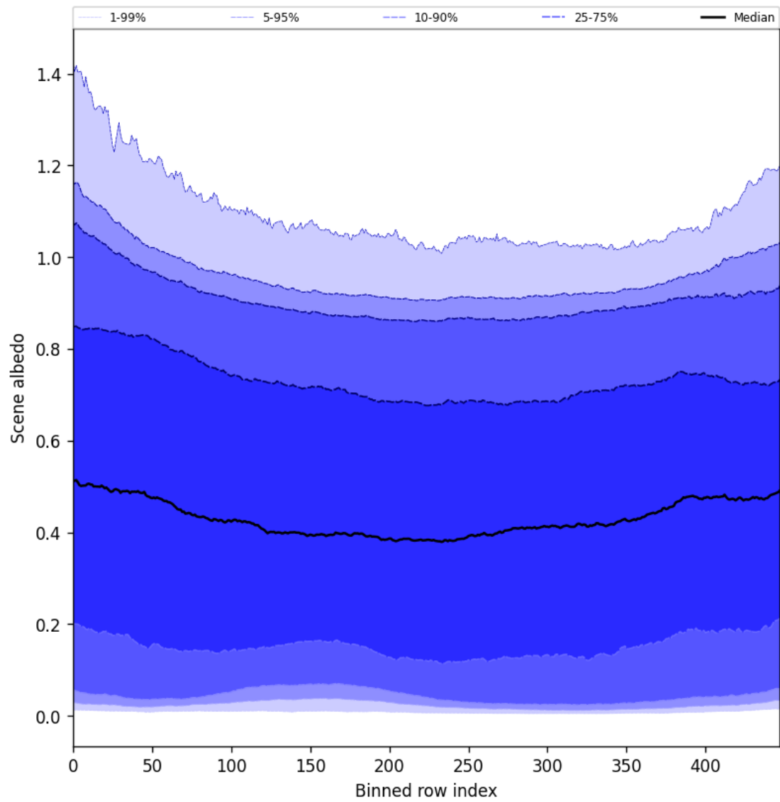
Figure 49: Along track statistics of “Scene albedo” for 2025-03-25 to 2025-03-26
