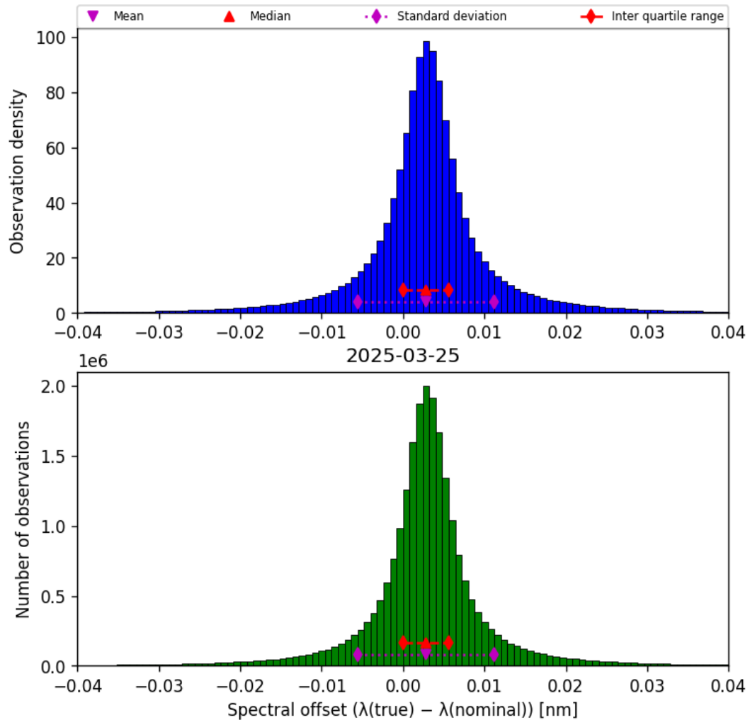
Figure 43: Histogram of “Spectral offset ( \lambda_{\text{true}} - \lambda_{\text{nominal}} )” for 2025-03-25 to 2025-03-26
