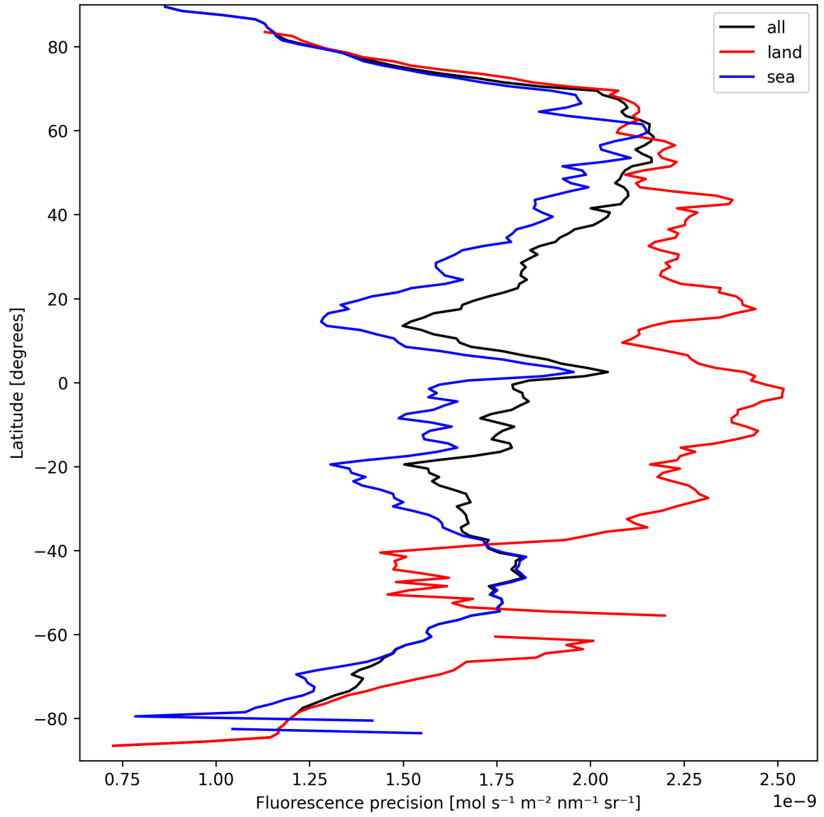
Figure 22: Zonal average of “Fluorescence precision” for 2025-03-25 to 2025-03-26.
