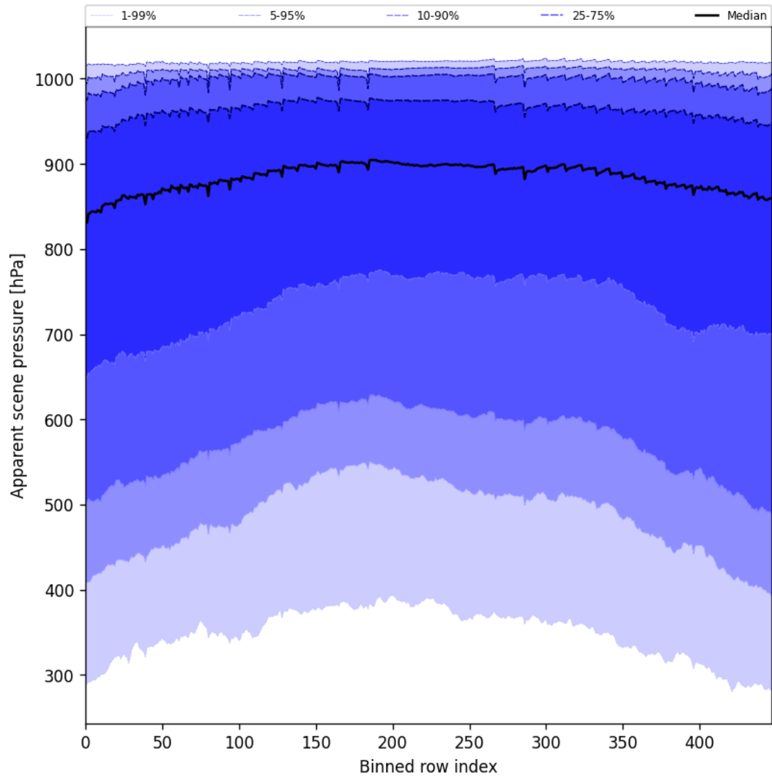
Figure 51: Along track statistics of “Apparent scene pressure” for 2025-03-25 to 2025-03-26
