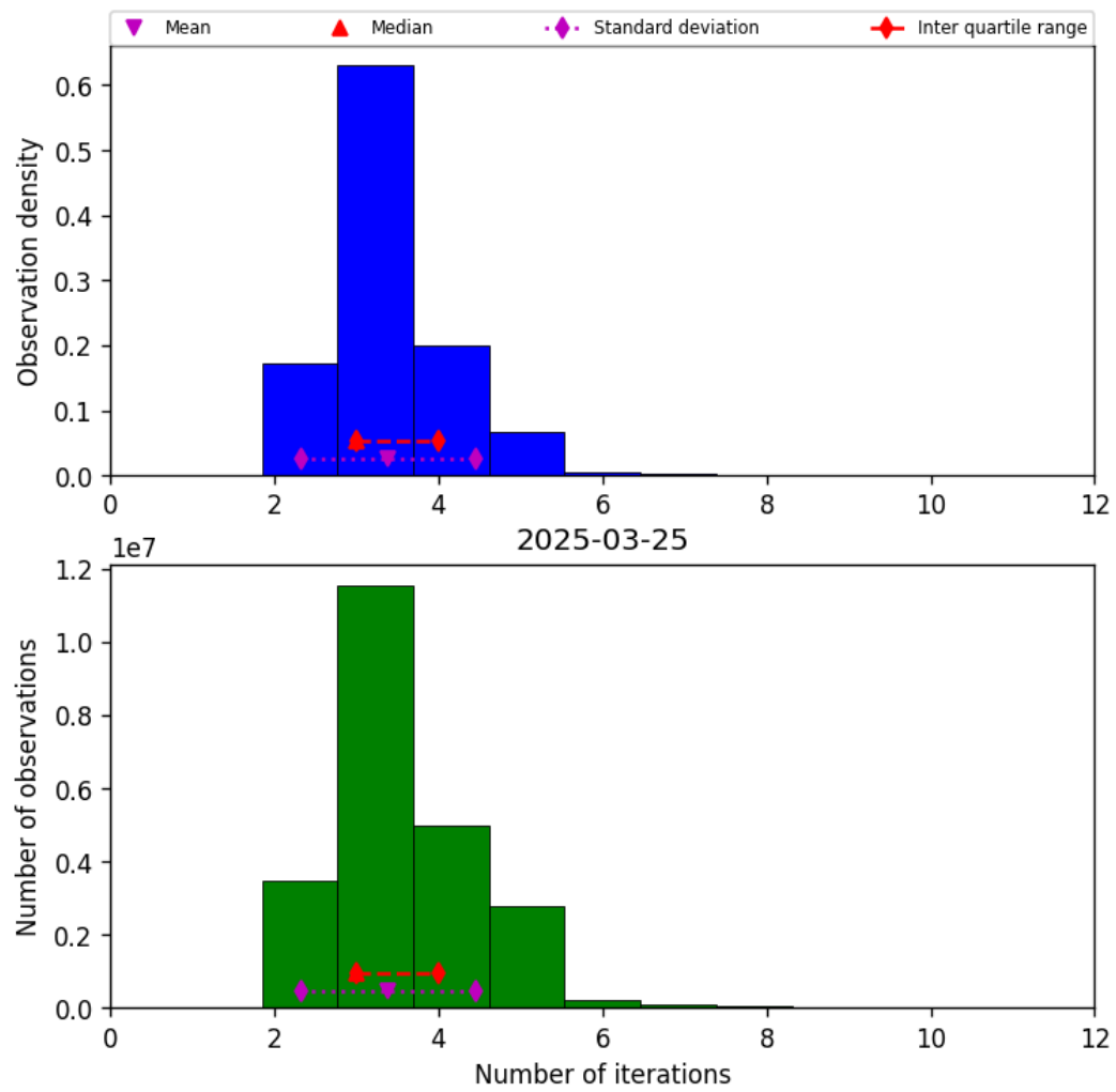
Figure 37: Histogram of “Number of iterations” for 2025-03-25 to 2025-03-26
