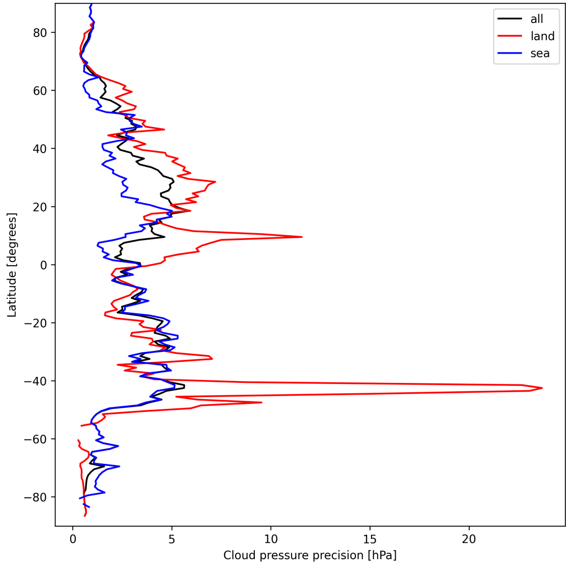
Figure 12: Zonal average of “Cloud pressure precision” for 2025-03-25 to 2025-03-26.
