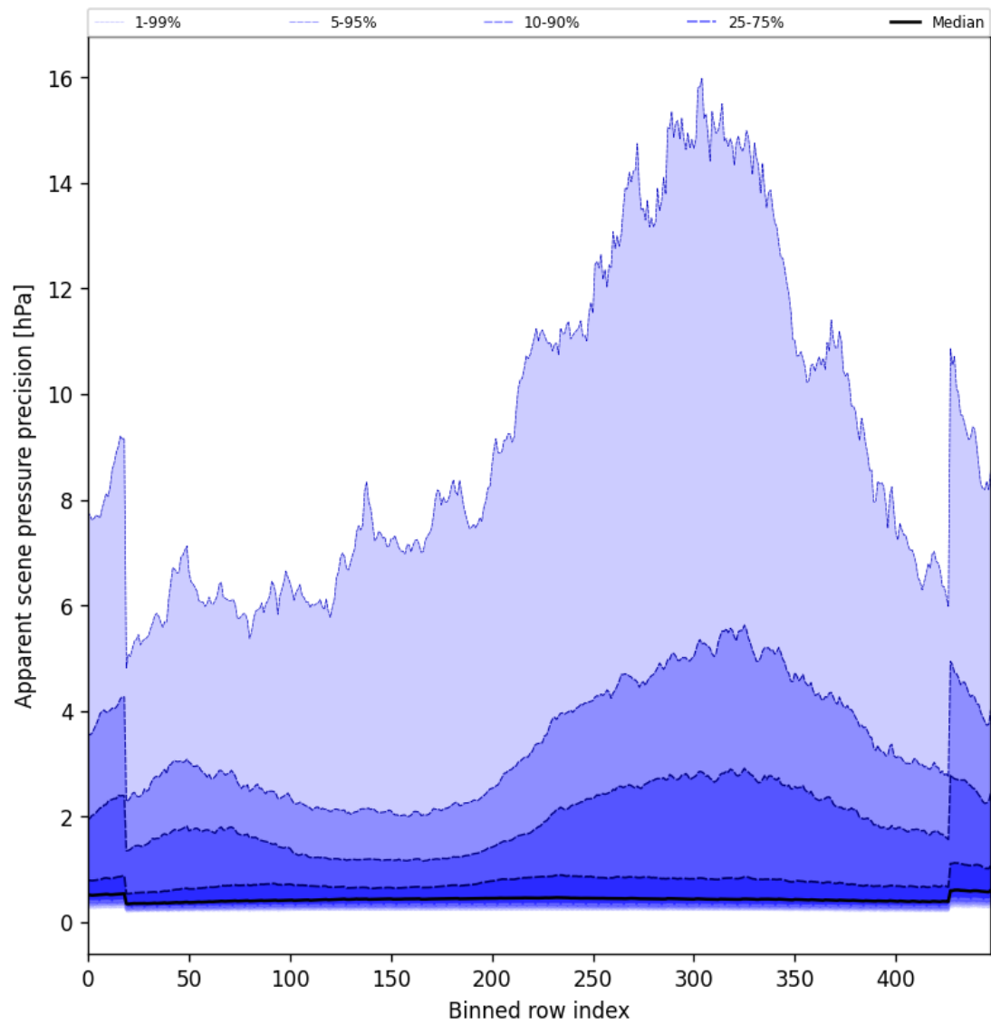
Figure 52: Along track statistics of “Apparent scene pressure precision” for 2025-03-25 to 2025-03-26
