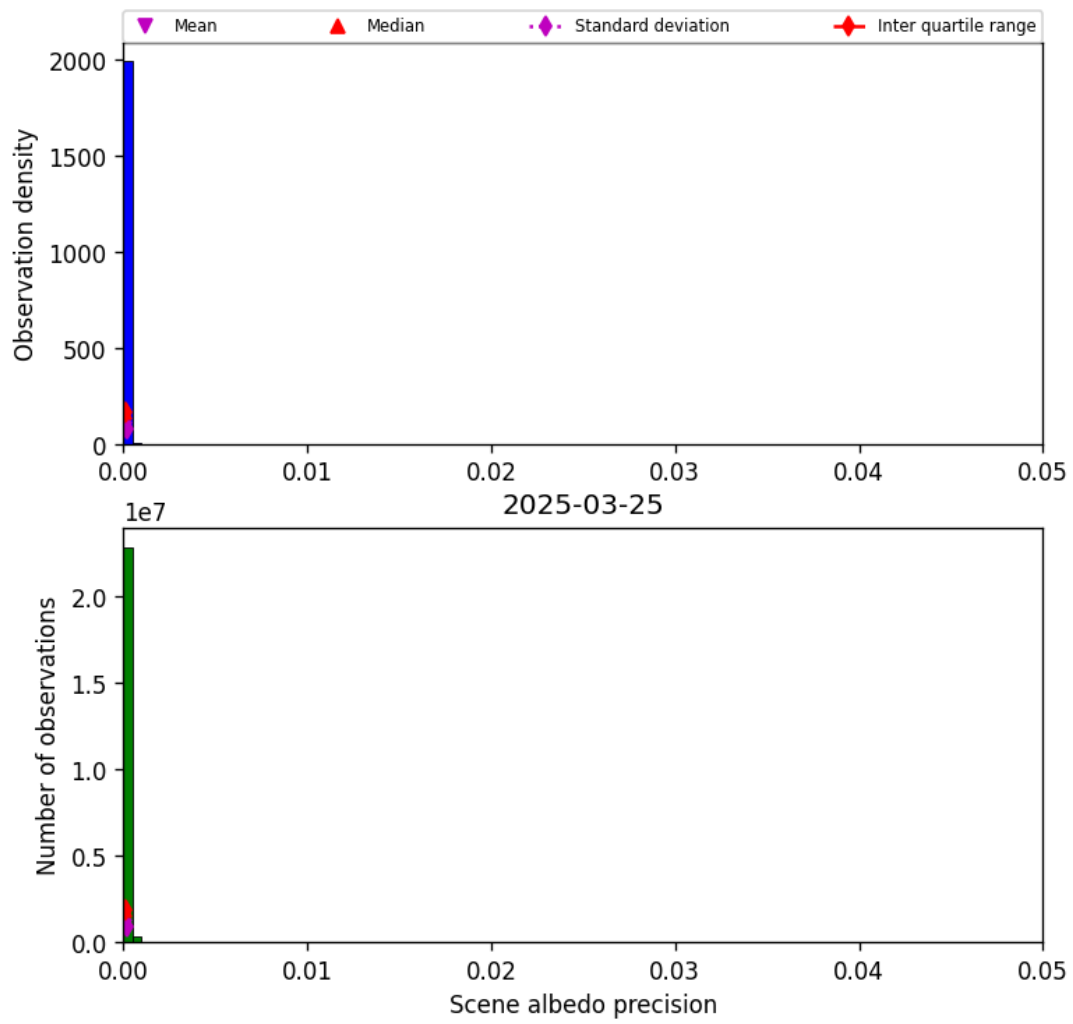
Figure 33: Histogram of “Scene albedo precision” for 2025-03-25 to 2025-03-26
