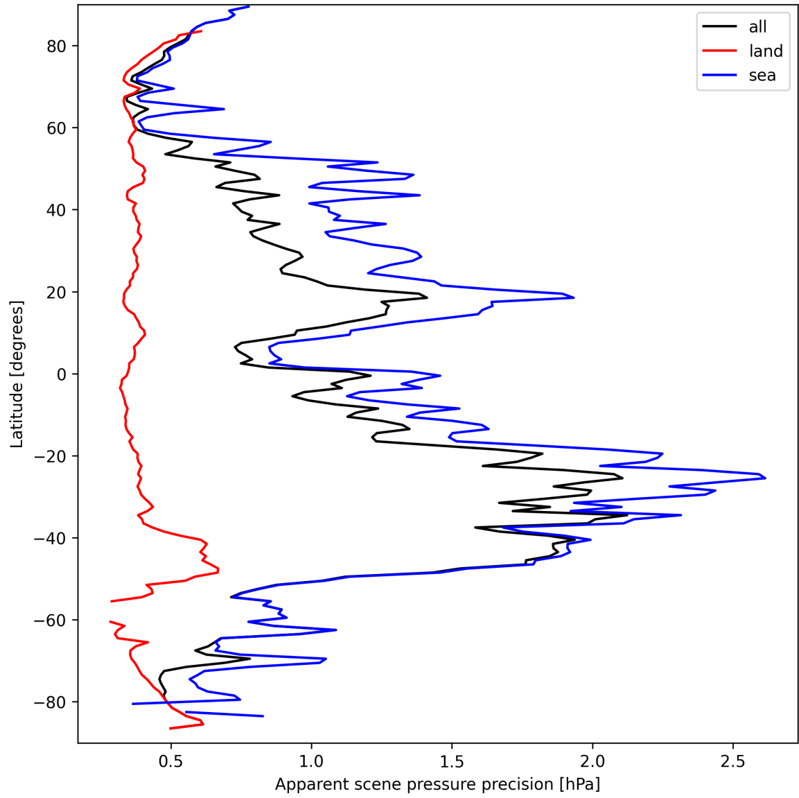
Figure 18: Zonal average of “Apparent scene pressure precision” for 2025-03-25 to 2025-03-26.
