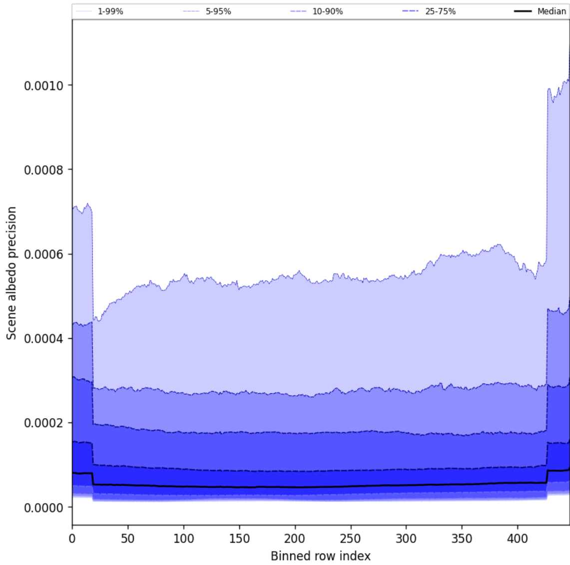
Figure 50: Along track statistics of “Scene albedo precision” for 2025-03-25 to 2025-03-26
