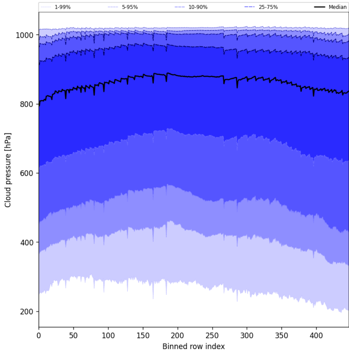
Figure 45: Along track statistics of “Cloud pressure” for 2025-03-25 to 2025-03-26
