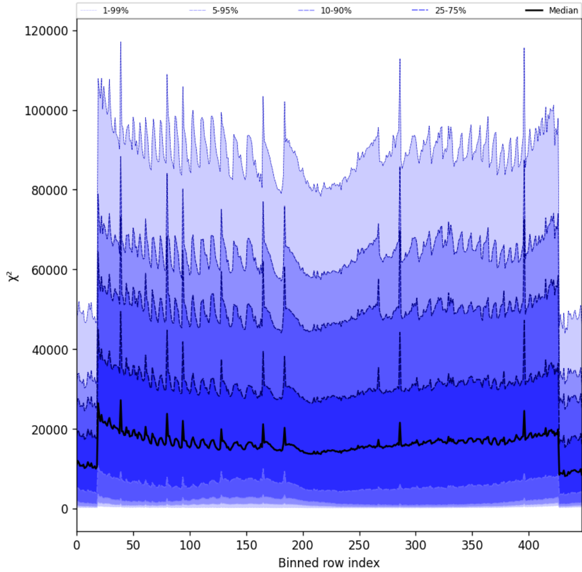
Figure 53: Along track statistics of “ \chi^2 ” for 2025-03-25 to 2025-03-26
