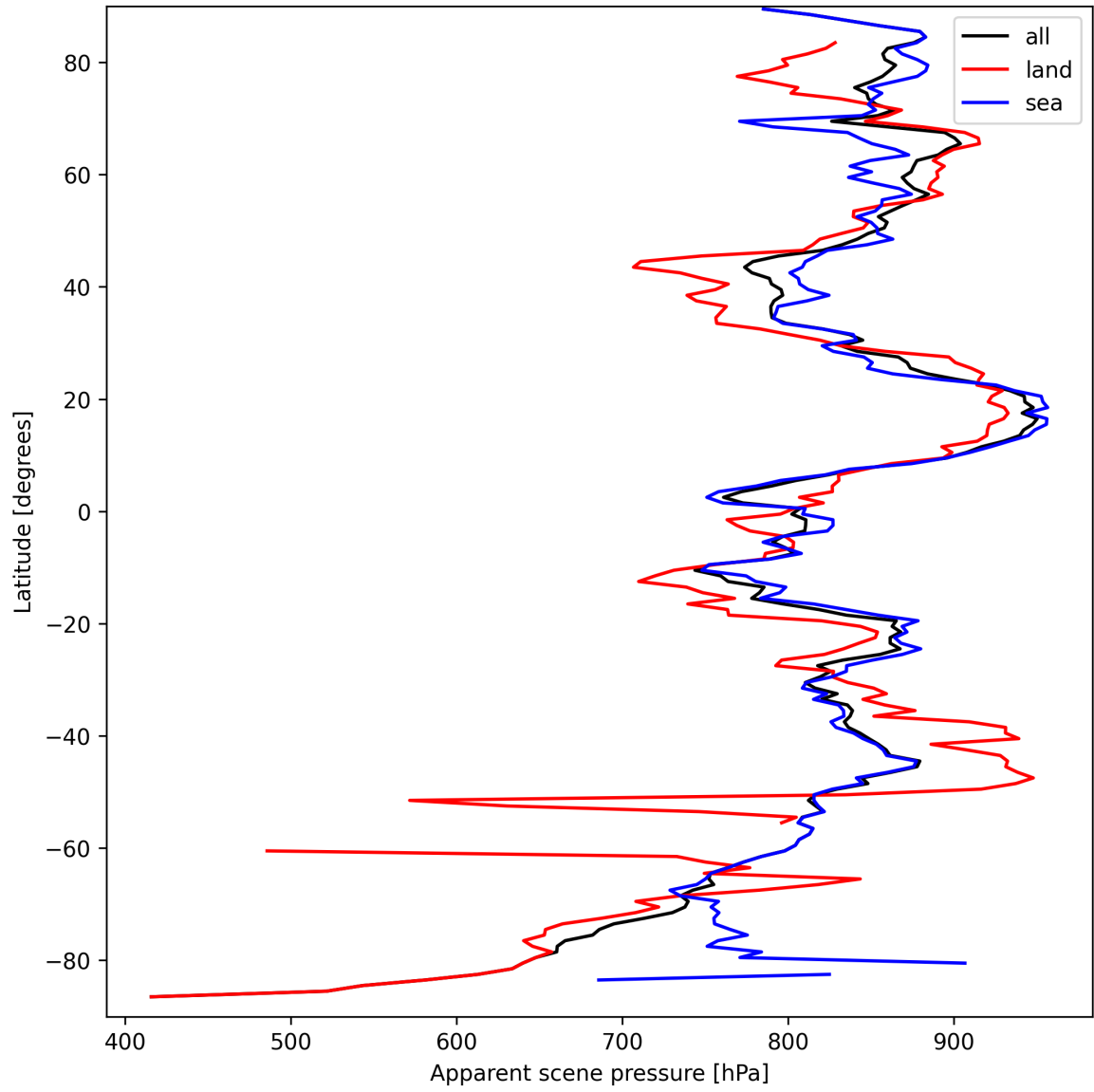
Figure 17: Zonal average of “Apparent scene pressure” for 2025-03-25 to 2025-03-26.
