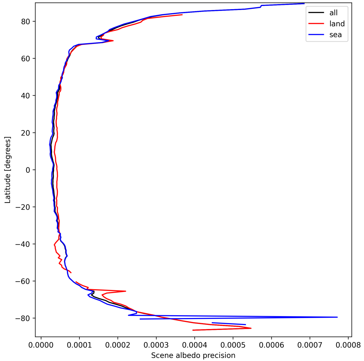
Figure 16: Zonal average of “Scene albedo precision” for 2025-03-25 to 2025-03-26.
