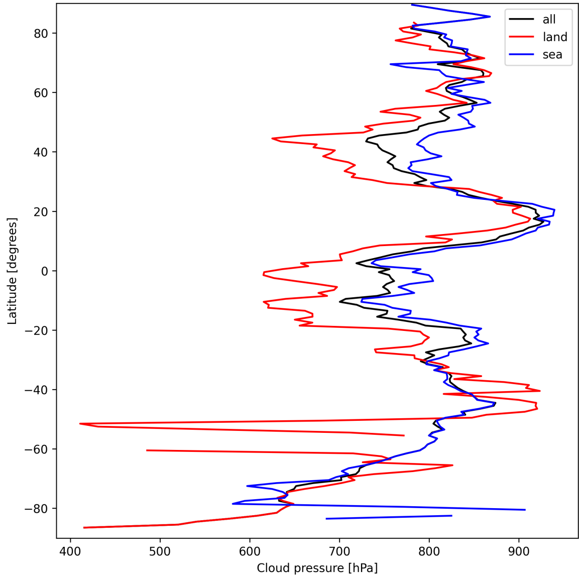
Figure 11: Zonal average of “Cloud pressure” for 2025-03-25 to 2025-03-26.
