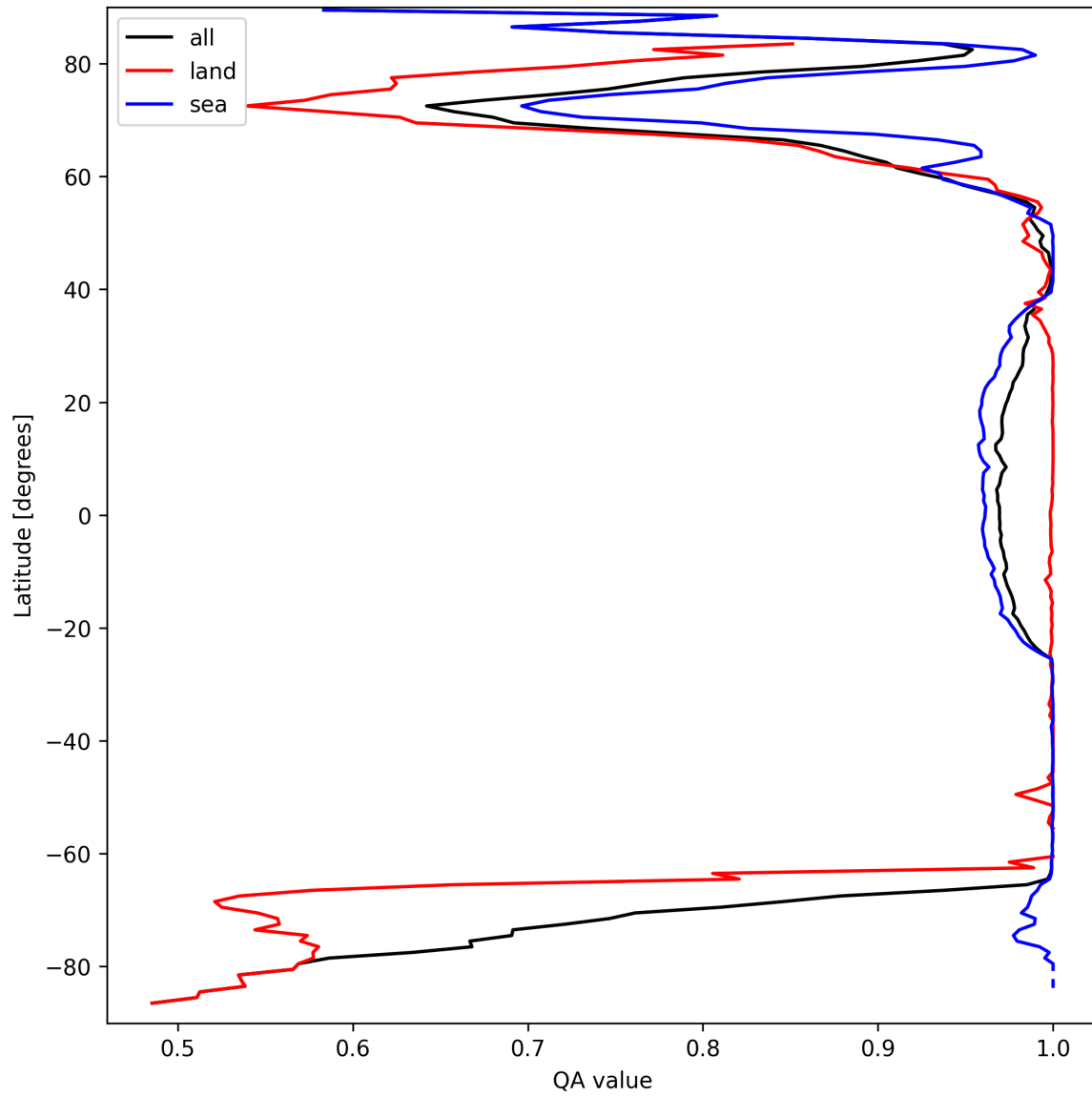
Figure 10: Zonal average of “QA value” for 2025-03-25 to 2025-03-26.
