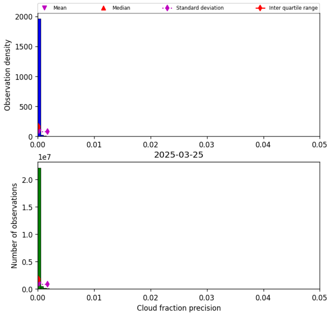
Figure 31: Histogram of “Cloud fraction precision” for 2025-03-25 to 2025-03-26
