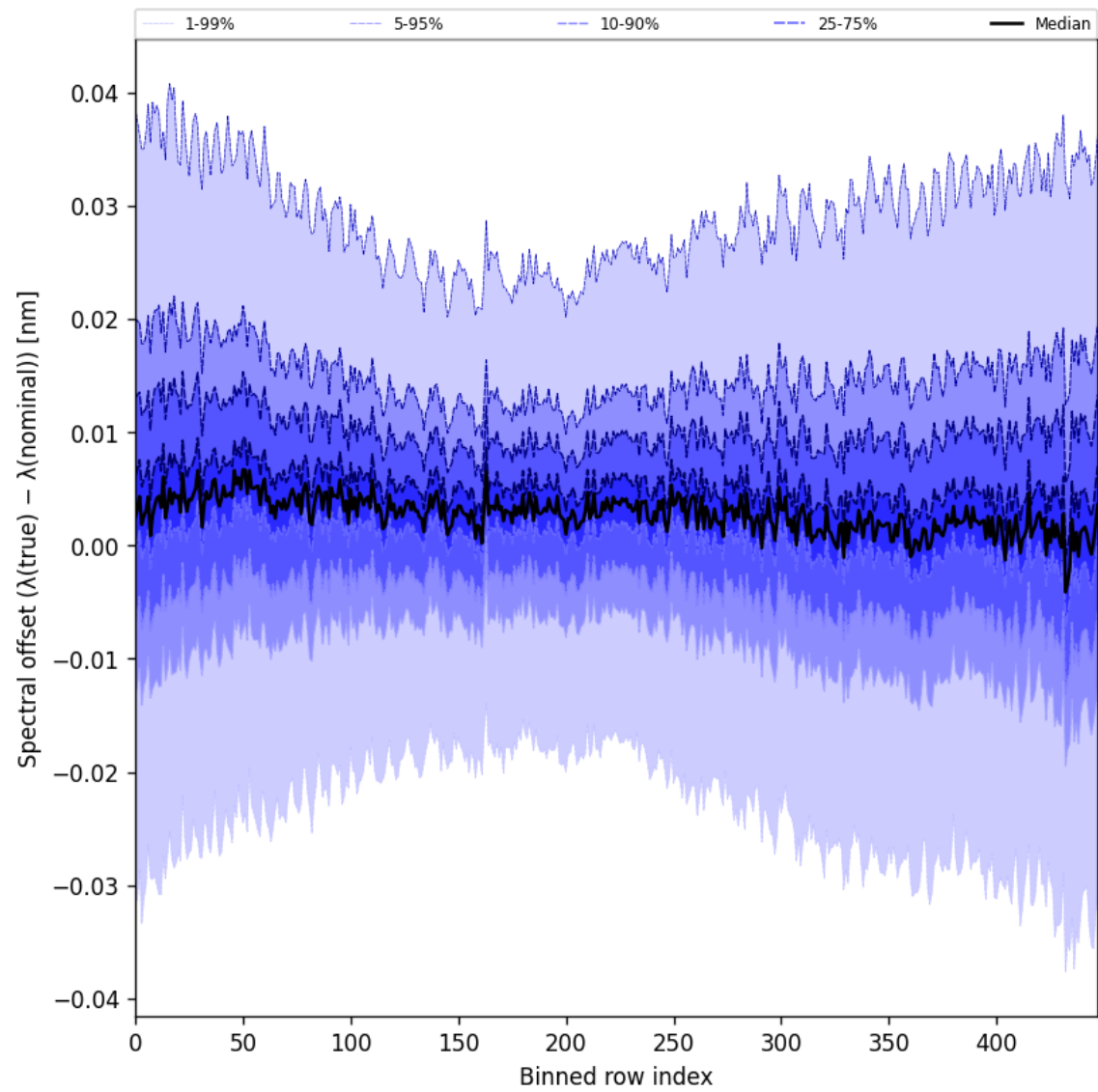
Figure 60: Along track statistics of “Spectral offset ( \lambda_{\text{true}} - \lambda_{\text{nominal}} )” for 2025-03-25 to 2025-03-26
