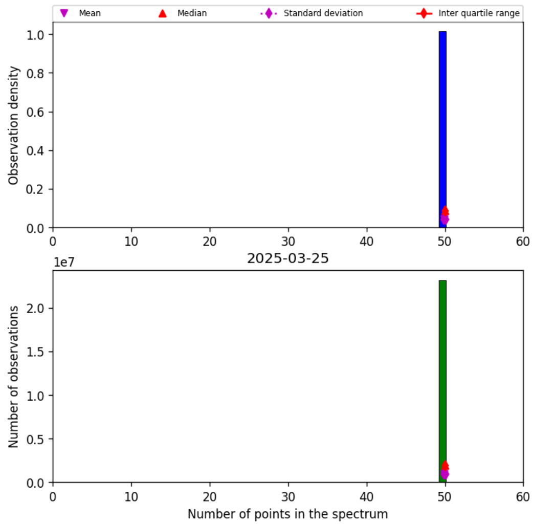
Figure 42: Histogram of "Number of points in the spectrum" for 2025-03-25 to 2025-03-26
