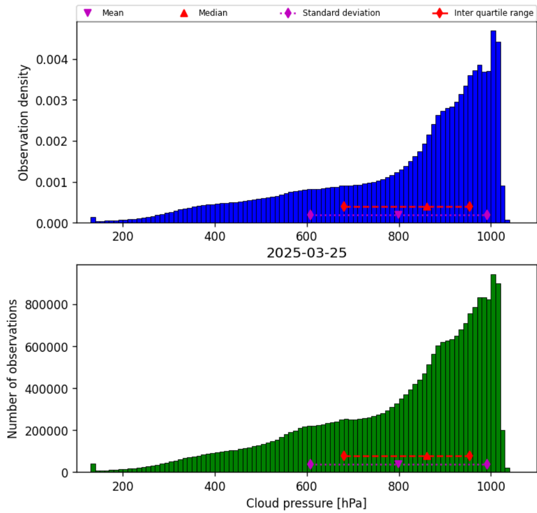
Figure 28: Histogram of “Cloud pressure” for 2025-03-25 to 2025-03-26
