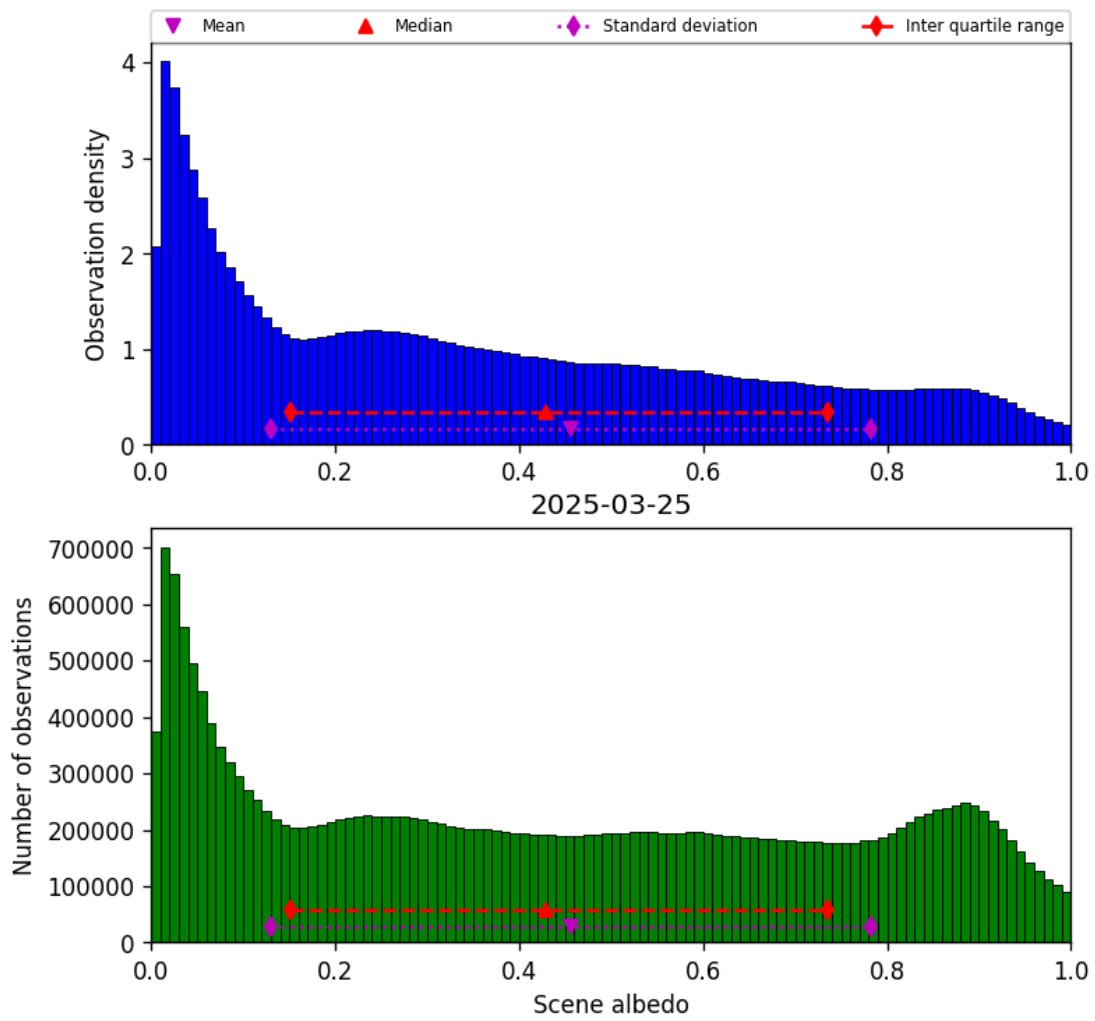
Figure 32: Histogram of “Scene albedo” for 2025-03-25 to 2025-03-26
