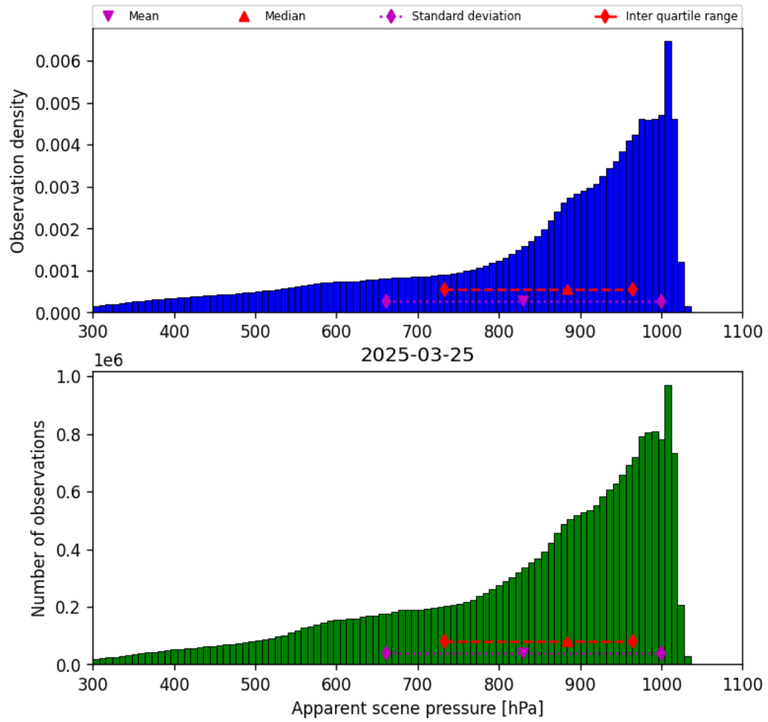
Figure 34: Histogram of “Apparent scene pressure” for 2025-03-25 to 2025-03-26
