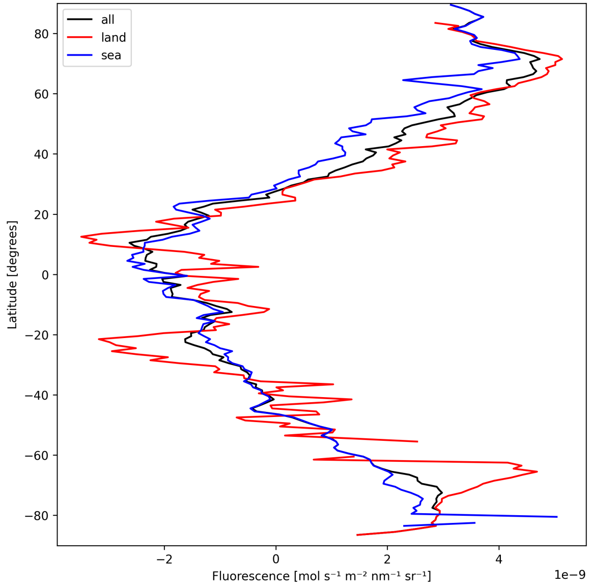
Figure 21: Zonal average of “Fluorescence” for 2025-03-25 to 2025-03-26.
