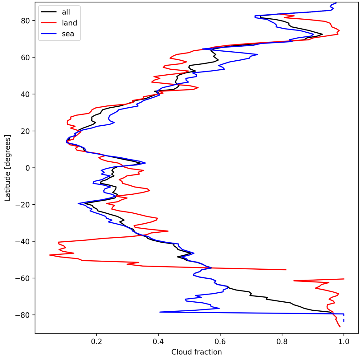
Figure 13: Zonal average of “Cloud fraction” for 2025-03-25 to 2025-03-26.
