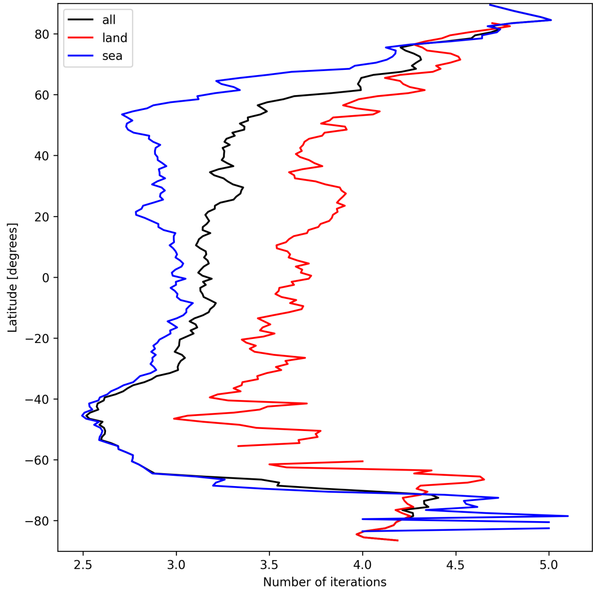
Figure 20: Zonal average of “Number of iterations” for 2025-03-25 to 2025-03-26.
