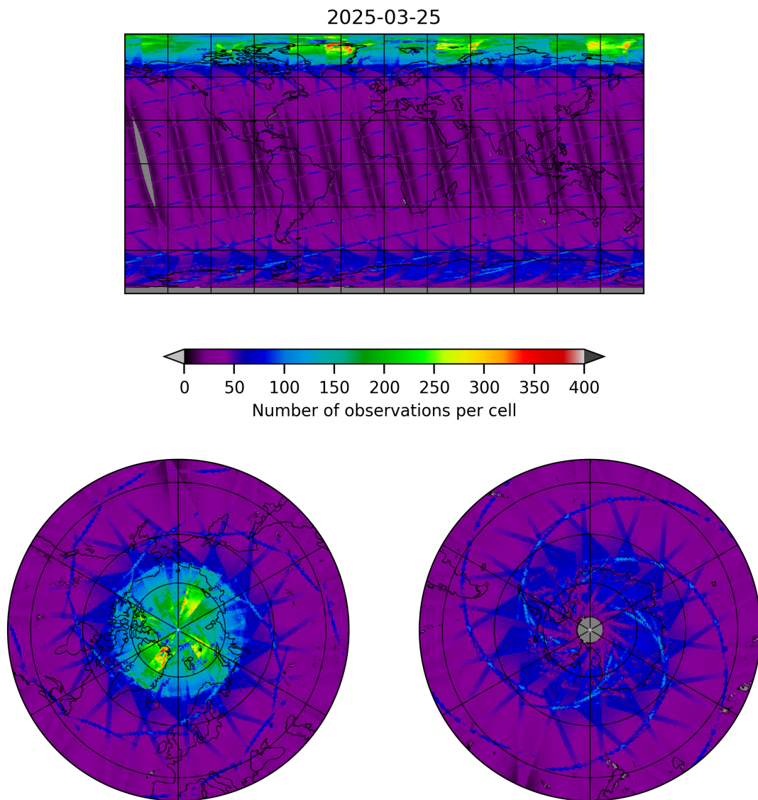
Figure 9: Map of the number of observations for 2025-03-25 to 2025-03-26
