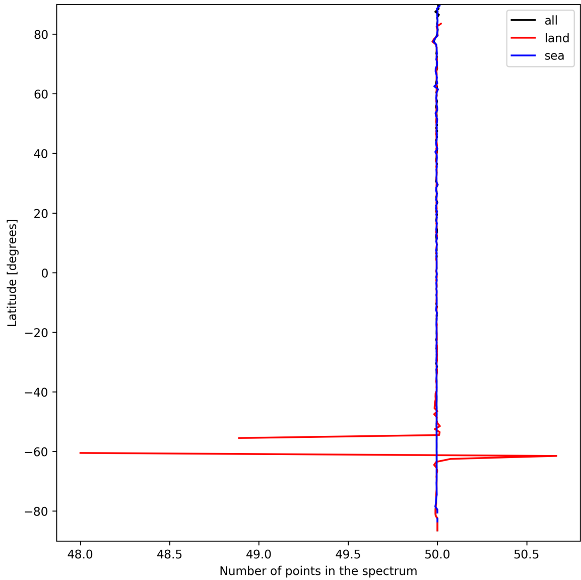
Figure 25: Zonal average of “Number of points in the spectrum” for 2025-03-25 to 2025-03-26.
