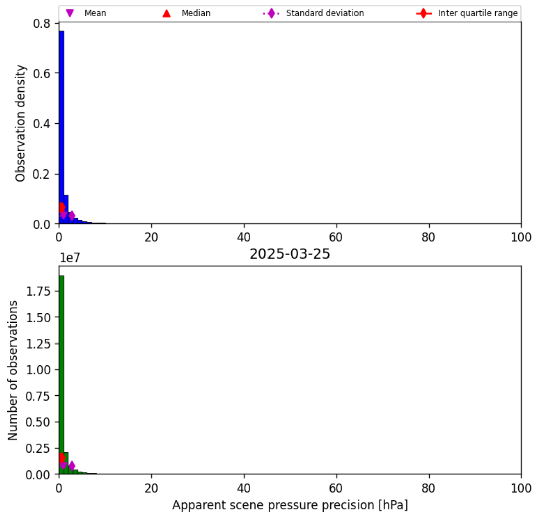
Figure 35: Histogram of “Apparent scene pressure precision” for 2025-03-25 to 2025-03-26
