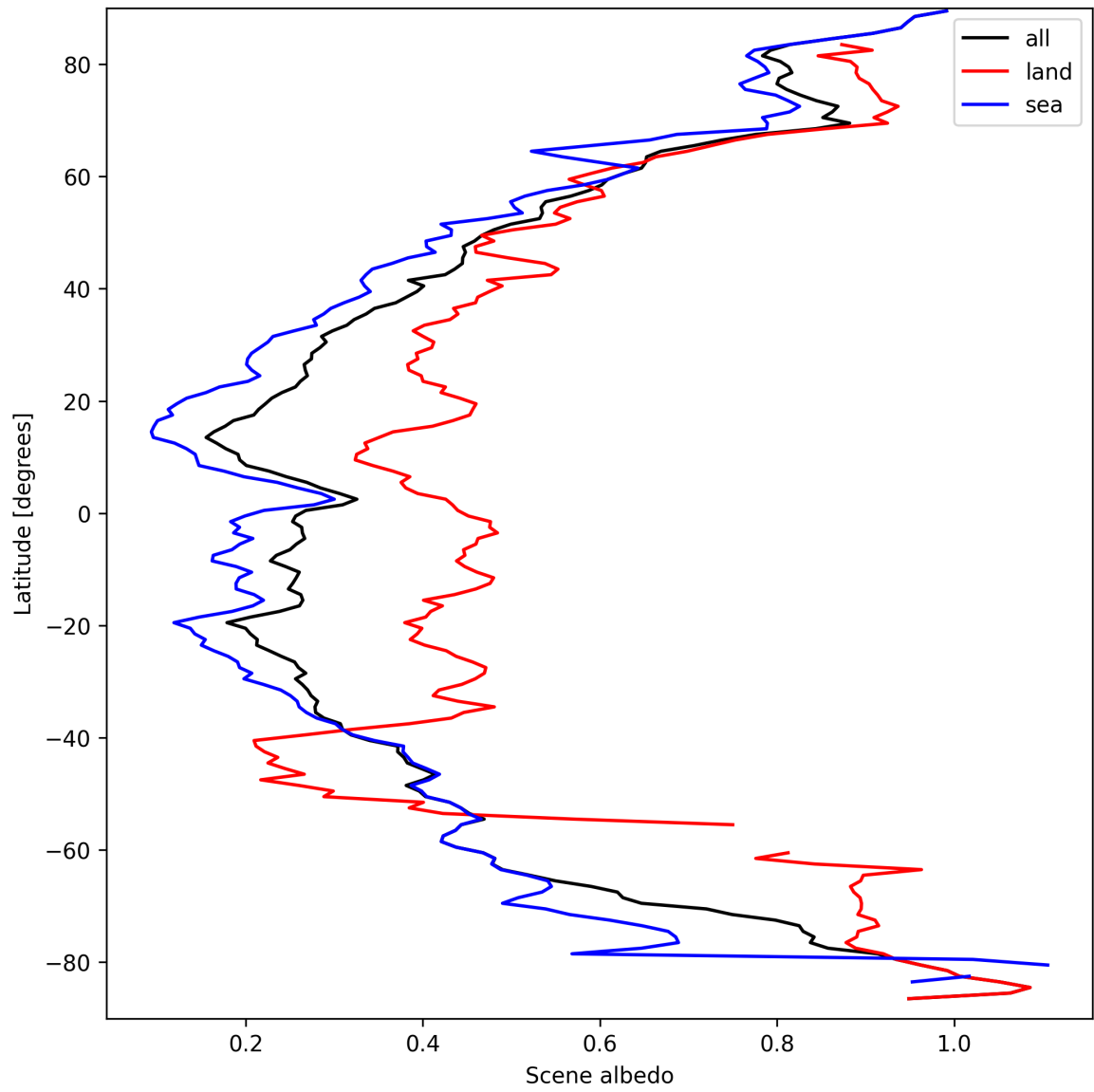
Figure 15: Zonal average of “Scene albedo” for 2025-03-25 to 2025-03-26.
