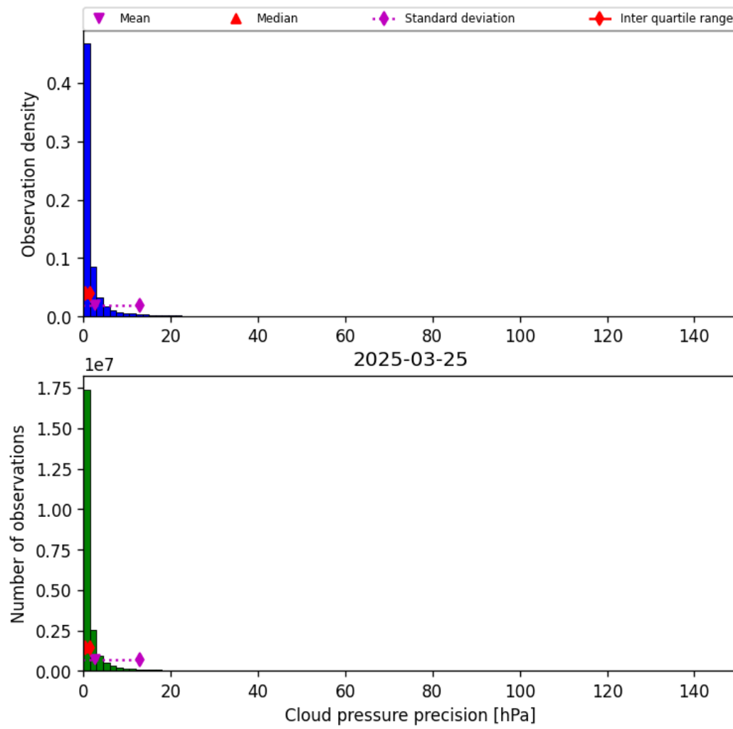
Figure 29: Histogram of “Cloud pressure precision” for 2025-03-25 to 2025-03-26
