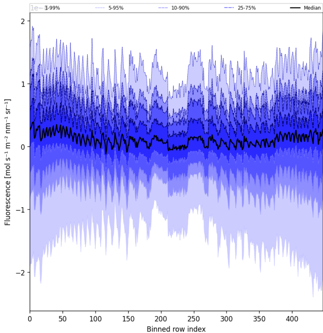
Figure 55: Along track statistics of “Fluorescence” for 2025-03-25 to 2025-03-26
