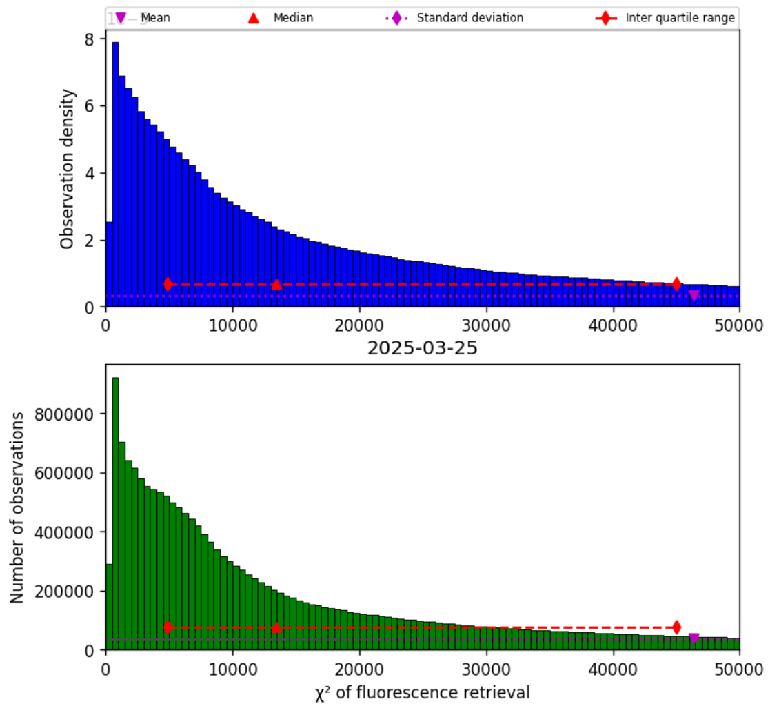
Figure 40: Histogram of “ \chi^2 of fluorescence retrieval” for 2025-03-25 to 2025-03-26
