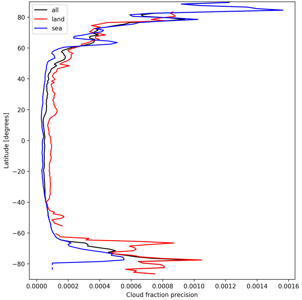
Figure 14: Zonal average of “Cloud fraction precision” for 2025-03-25 to 2025-03-26.
