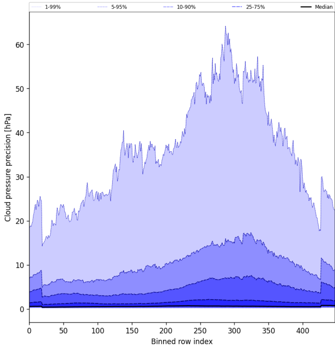
Figure 46: Along track statistics of “Cloud pressure precision” for 2025-03-25 to 2025-03-26
