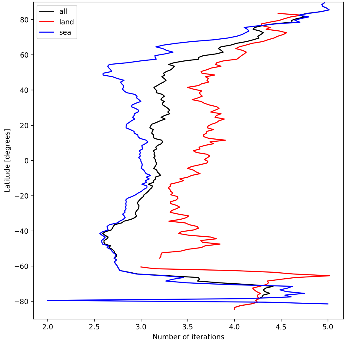
Figure 20: Zonal average of “Number of iterations” for 2025-03-28 to 2025-03-29.
