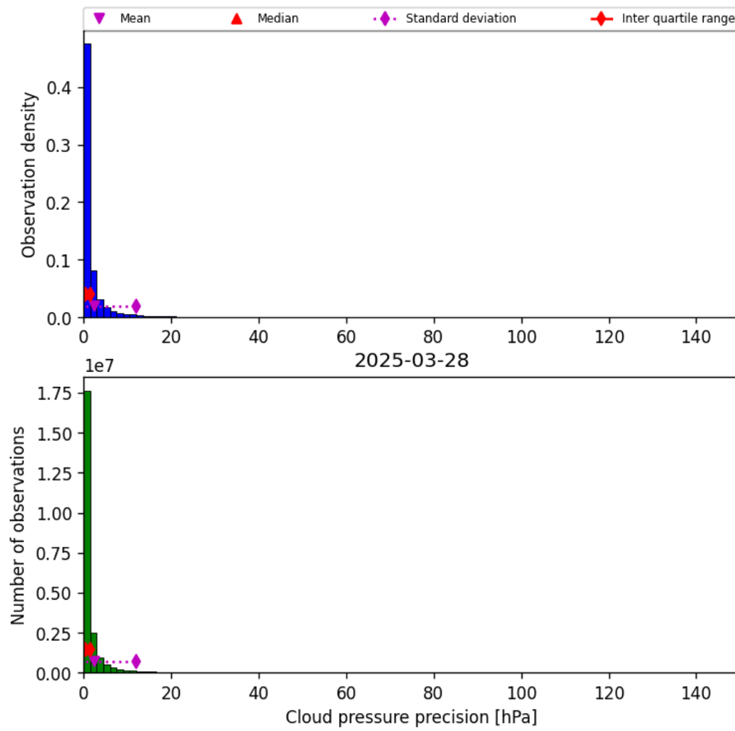
Figure 29: Histogram of “Cloud pressure precision” for 2025-03-28 to 2025-03-29
