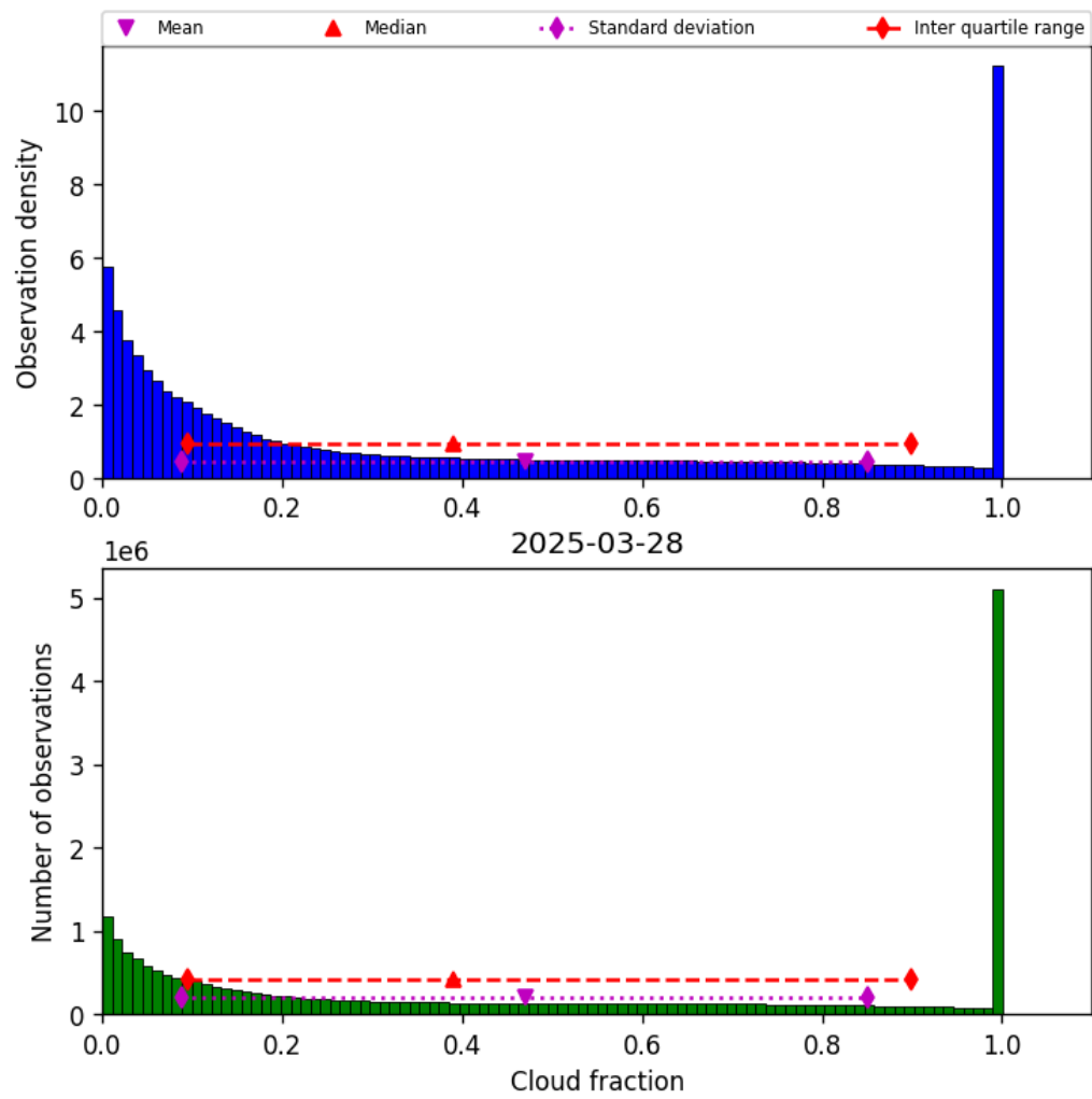
Figure 30: Histogram of “Cloud fraction” for 2025-03-28 to 2025-03-29
