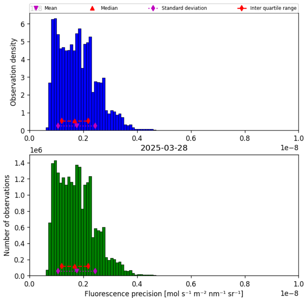
Figure 39: Histogram of “Fluorescence precision” for 2025-03-28 to 2025-03-29
