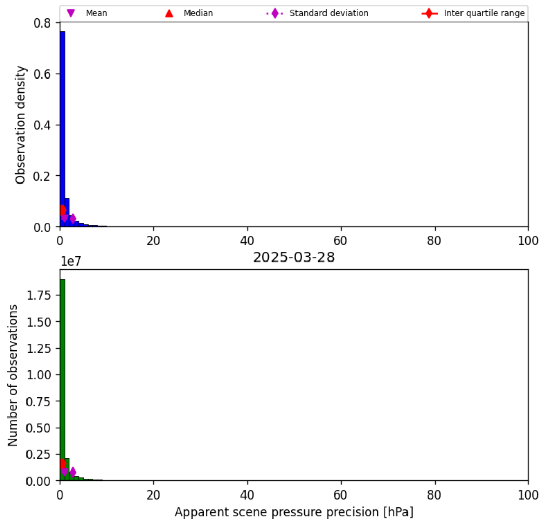
Figure 35: Histogram of “Apparent scene pressure precision” for 2025-03-28 to 2025-03-29
