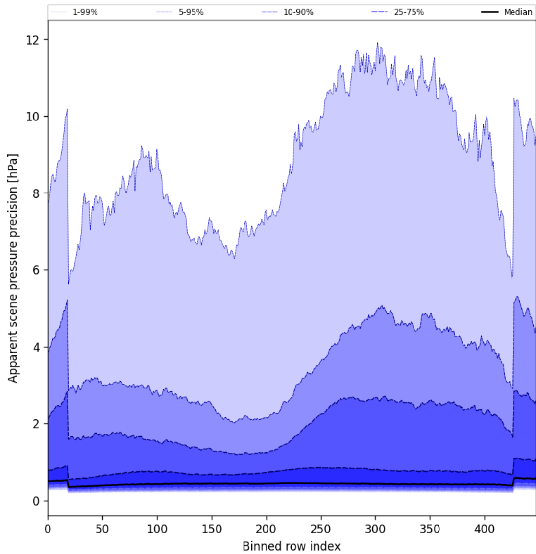
Figure 52: Along track statistics of “Apparent scene pressure precision” for 2025-03-28 to 2025-03-29
