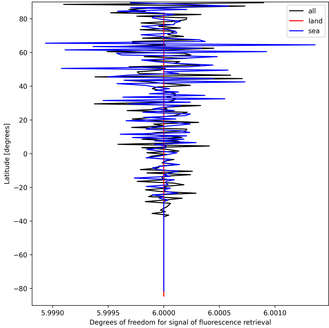
Figure 24: Zonal average of “Degrees of freedom for signal of fluorescence retrieval” for 2025-03-28 to 2025-03-29.
