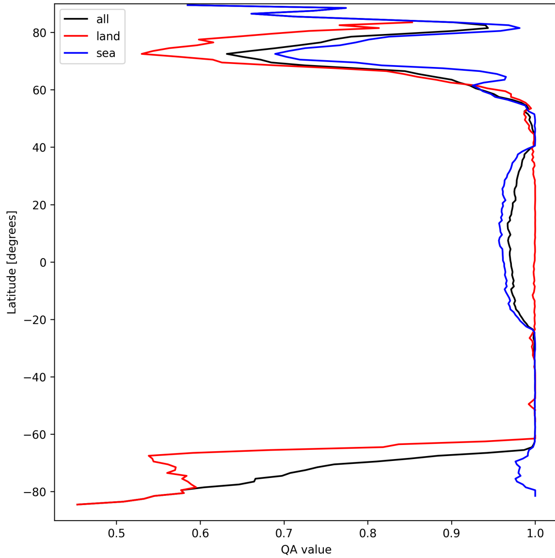
Figure 10: Zonal average of “QA value” for 2025-03-28 to 2025-03-29.
