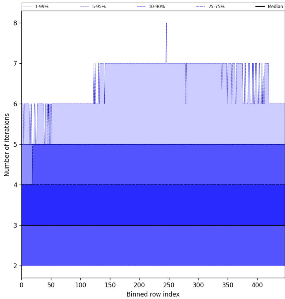
Figure 54: Along track statistics of “Number of iterations” for 2025-03-28 to 2025-03-29
