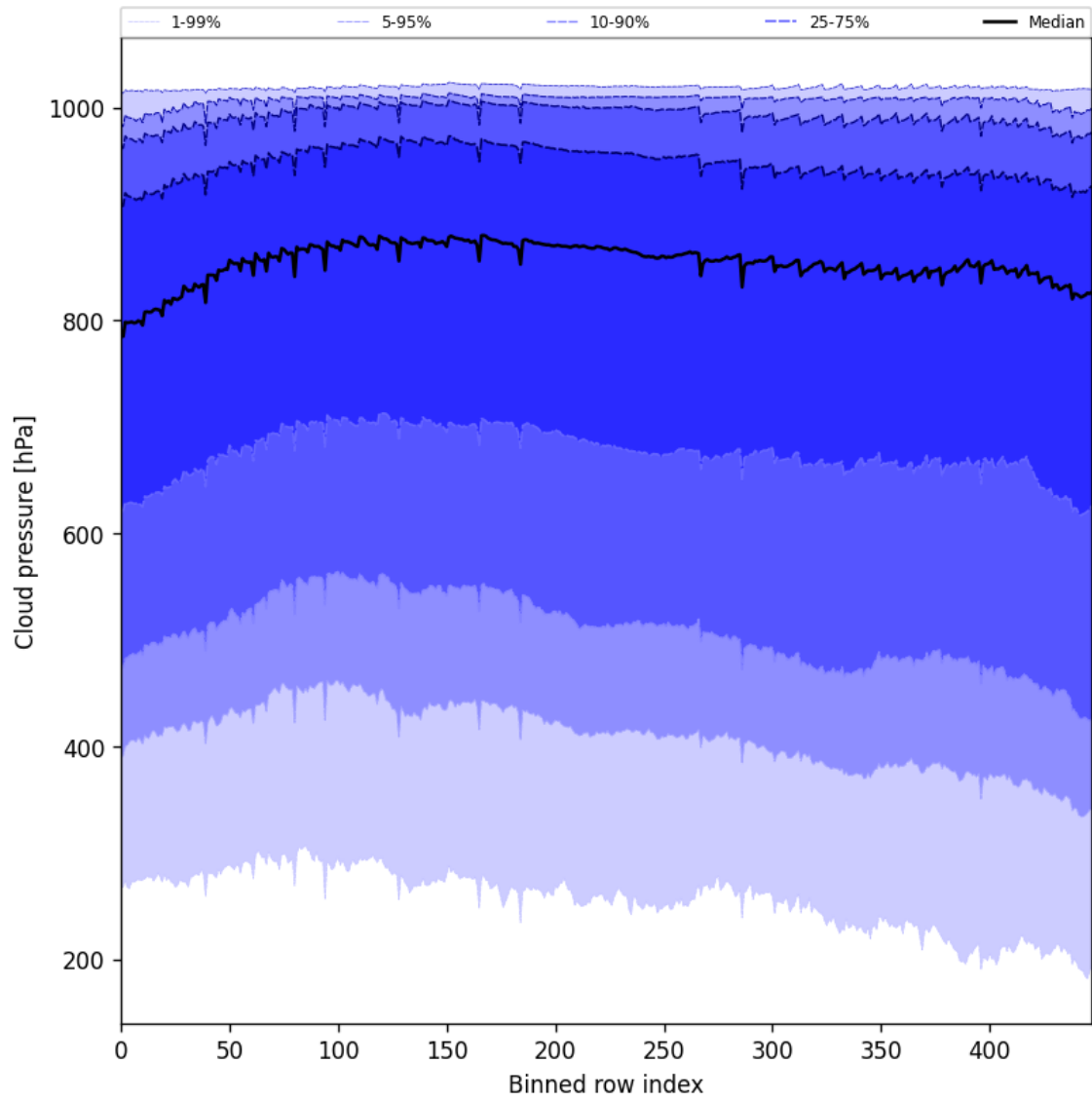
Figure 45: Along track statistics of “Cloud pressure” for 2025-03-28 to 2025-03-29
