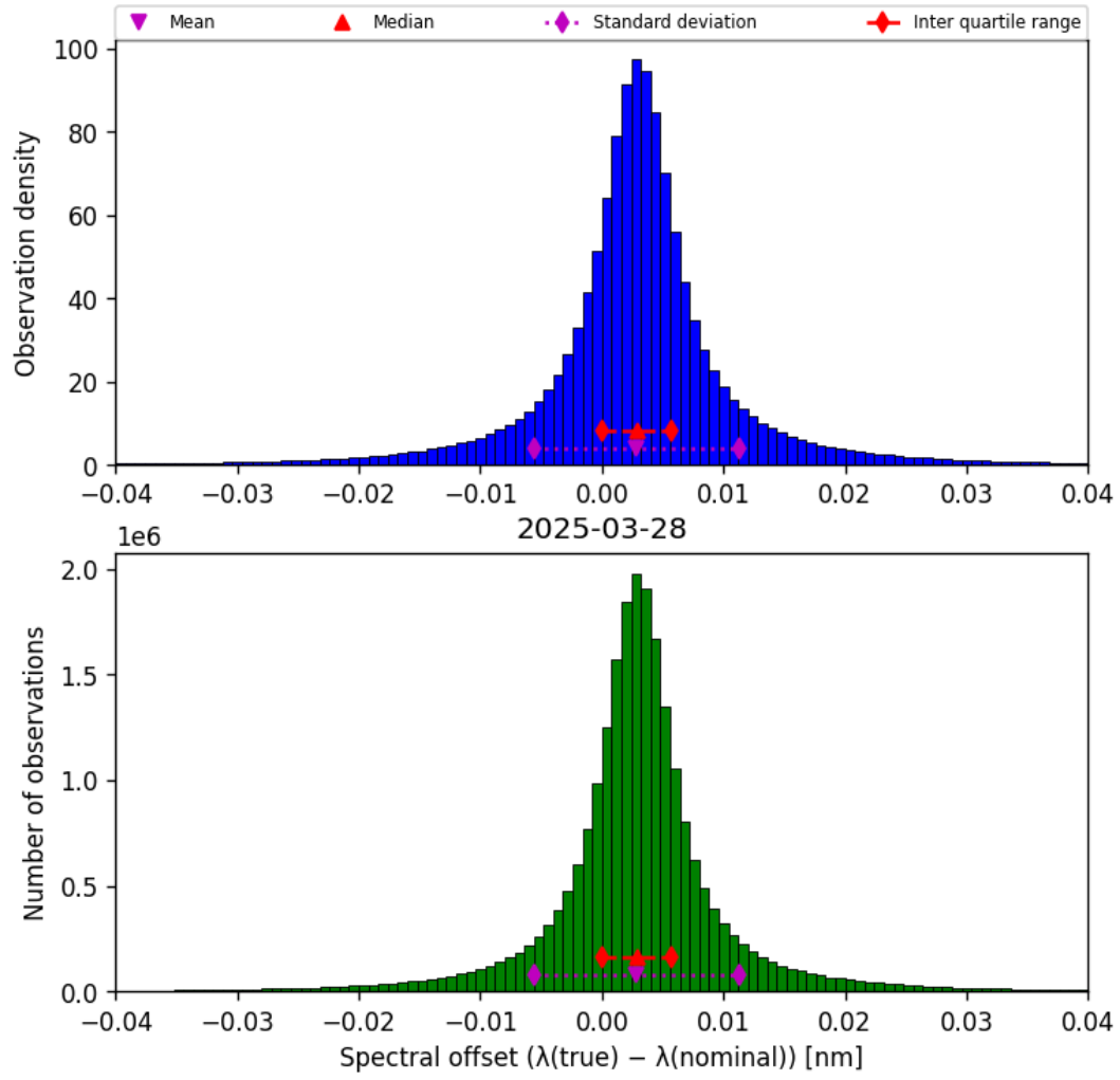
Figure 43: Histogram of “Spectral offset ( \lambda_{\text{true}} - \lambda_{\text{nominal}} )” for 2025-03-28 to 2025-03-29
