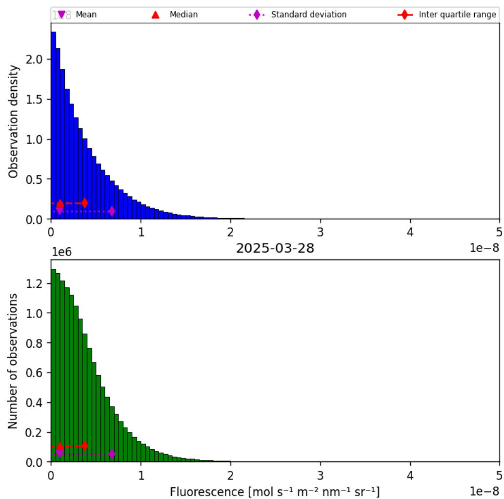
Figure 38: Histogram of “Fluorescence” for 2025-03-28 to 2025-03-29
