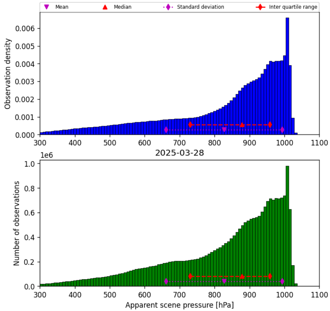
Figure 34: Histogram of “Apparent scene pressure” for 2025-03-28 to 2025-03-29
