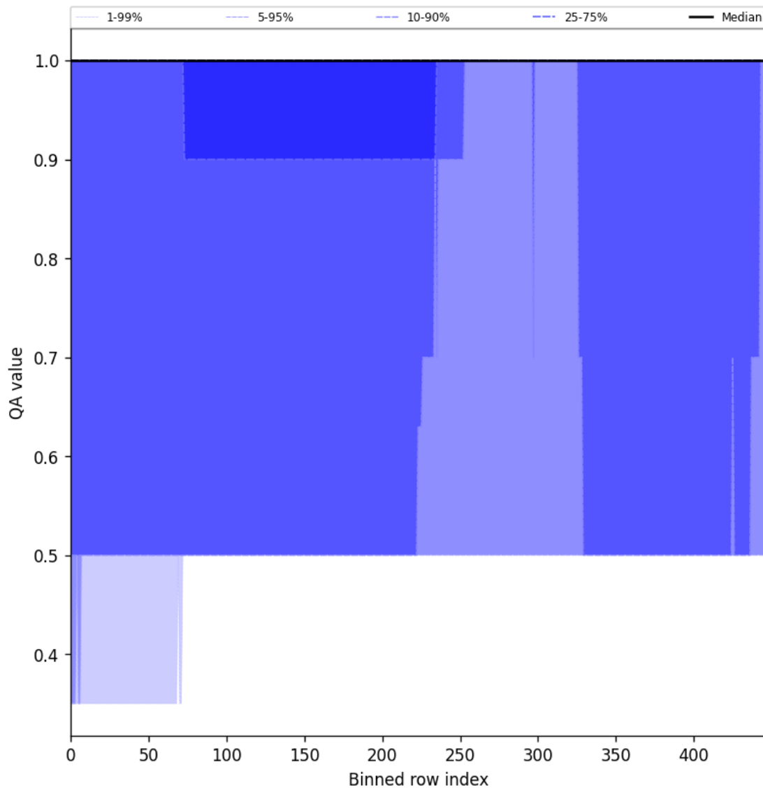
Figure 44: Along track statistics of “QA value” for 2025-03-28 to 2025-03-29
