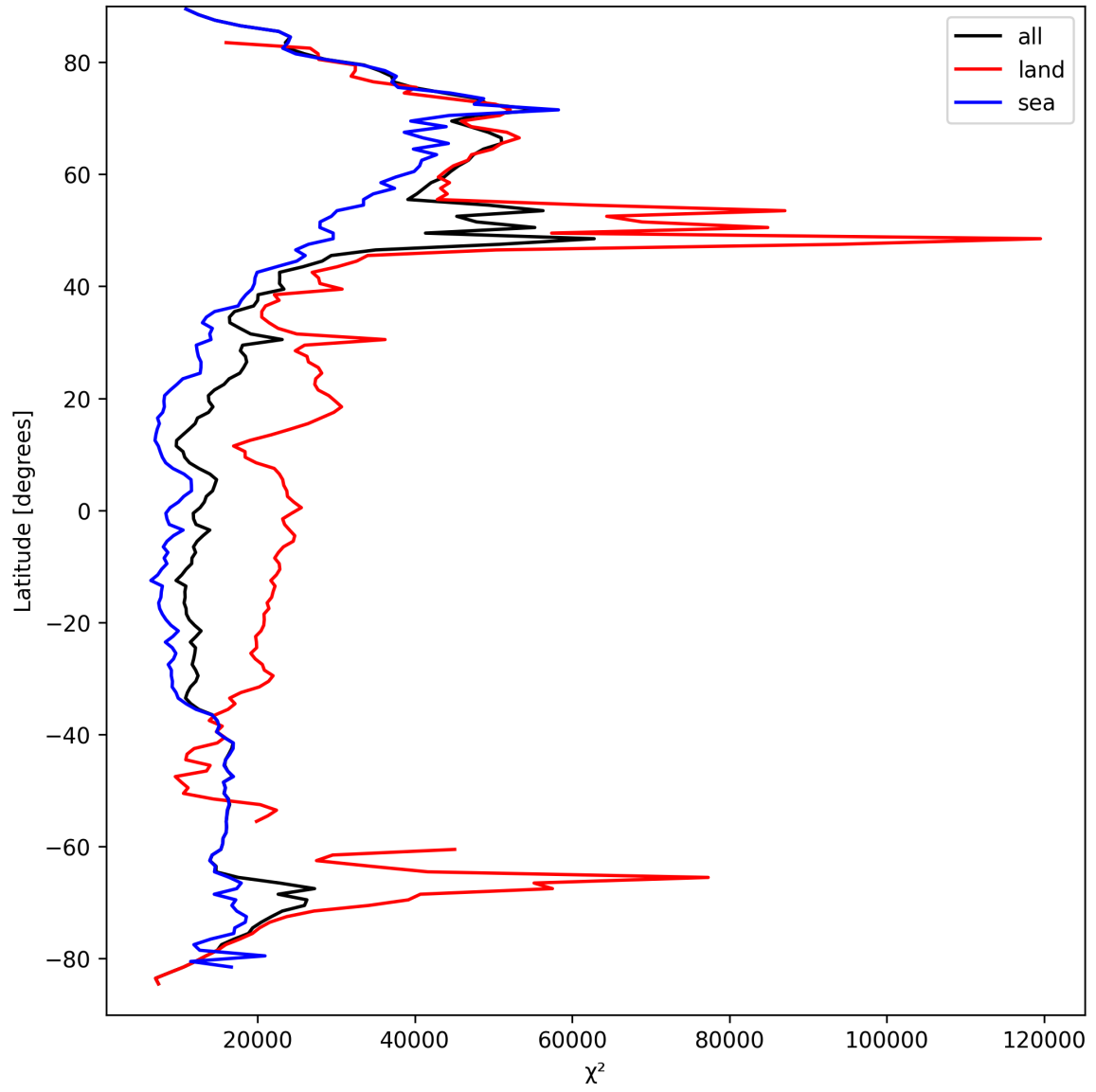
Figure 19: Zonal average of “ \chi^2 ” for 2025-03-28 to 2025-03-29.
