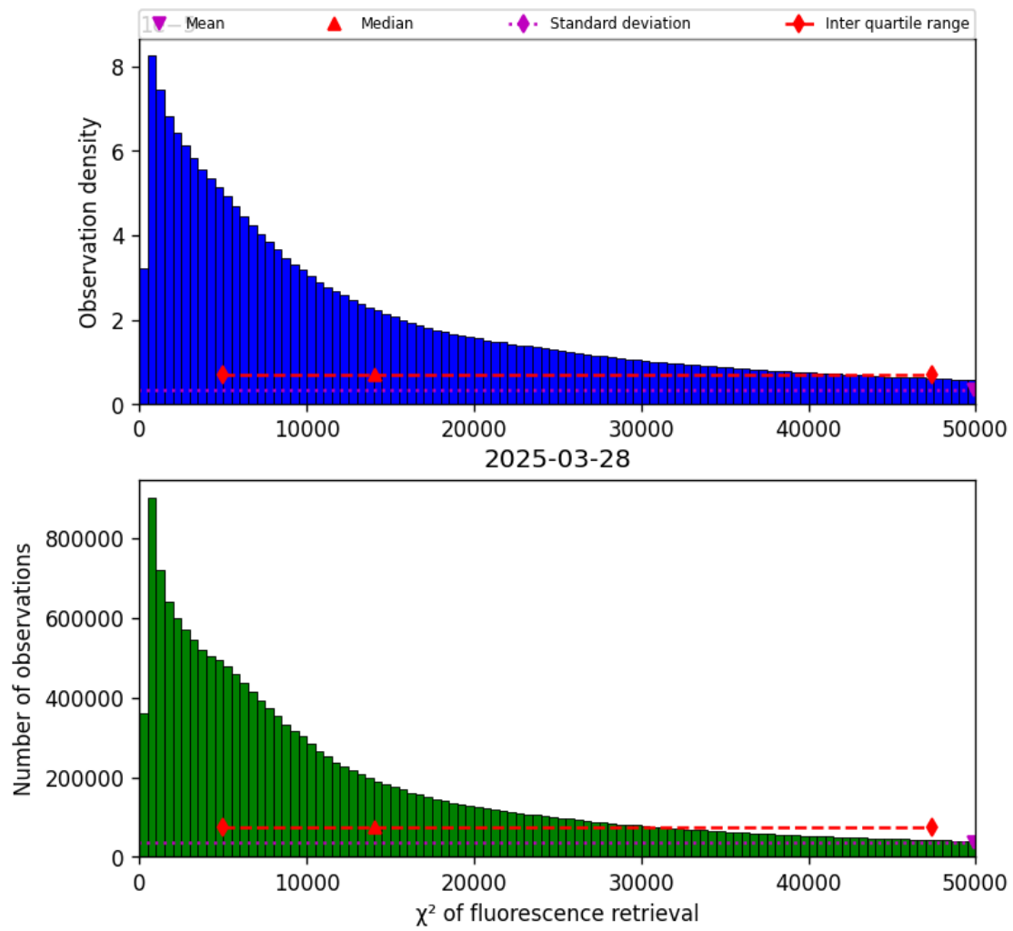
Figure 40: Histogram of “ \chi^2 of fluorescence retrieval” for 2025-03-28 to 2025-03-29
