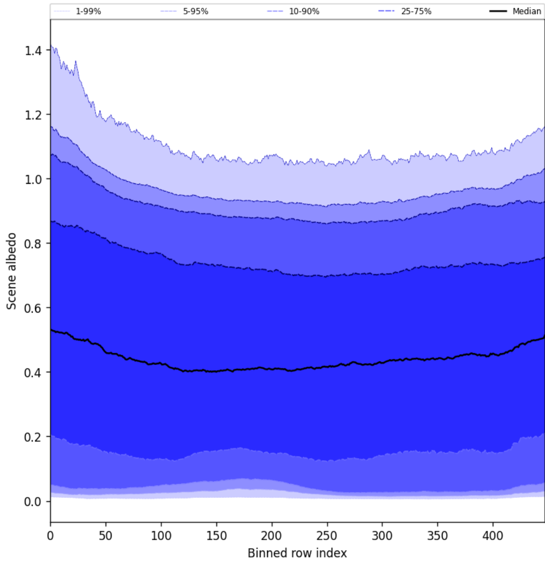
Figure 49: Along track statistics of “Scene albedo” for 2025-03-28 to 2025-03-29
