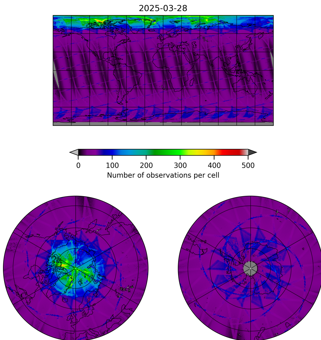
Figure 9: Map of the number of observations for 2025-03-28 to 2025-03-29
