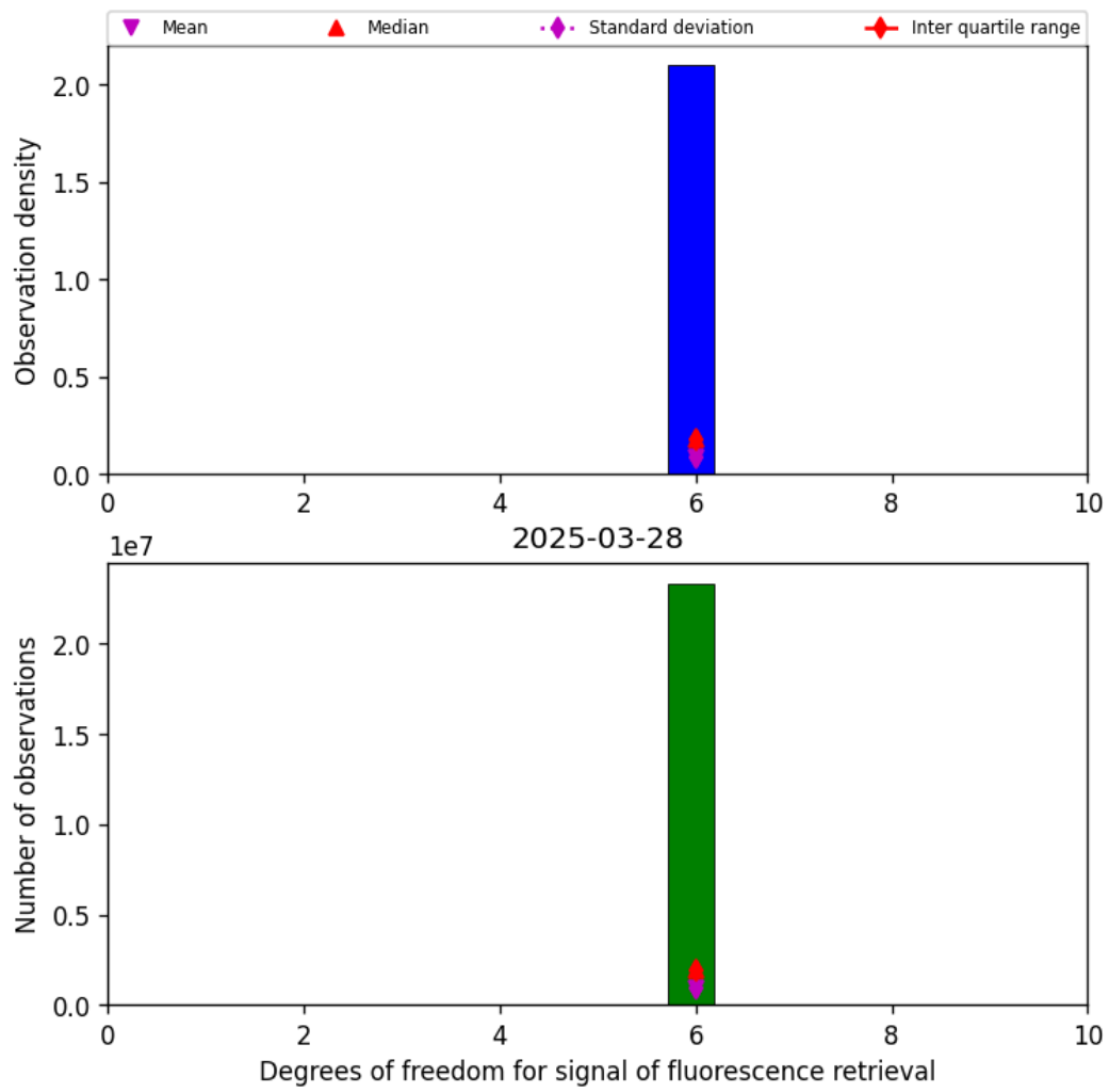
Figure 41: Histogram of “Degrees of freedom for signal of fluorescence retrieval” for 2025-03-28 to 2025-03-29
