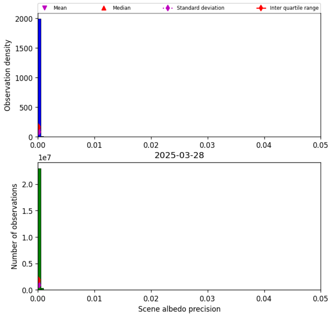
Figure 33: Histogram of “Scene albedo precision” for 2025-03-28 to 2025-03-29
