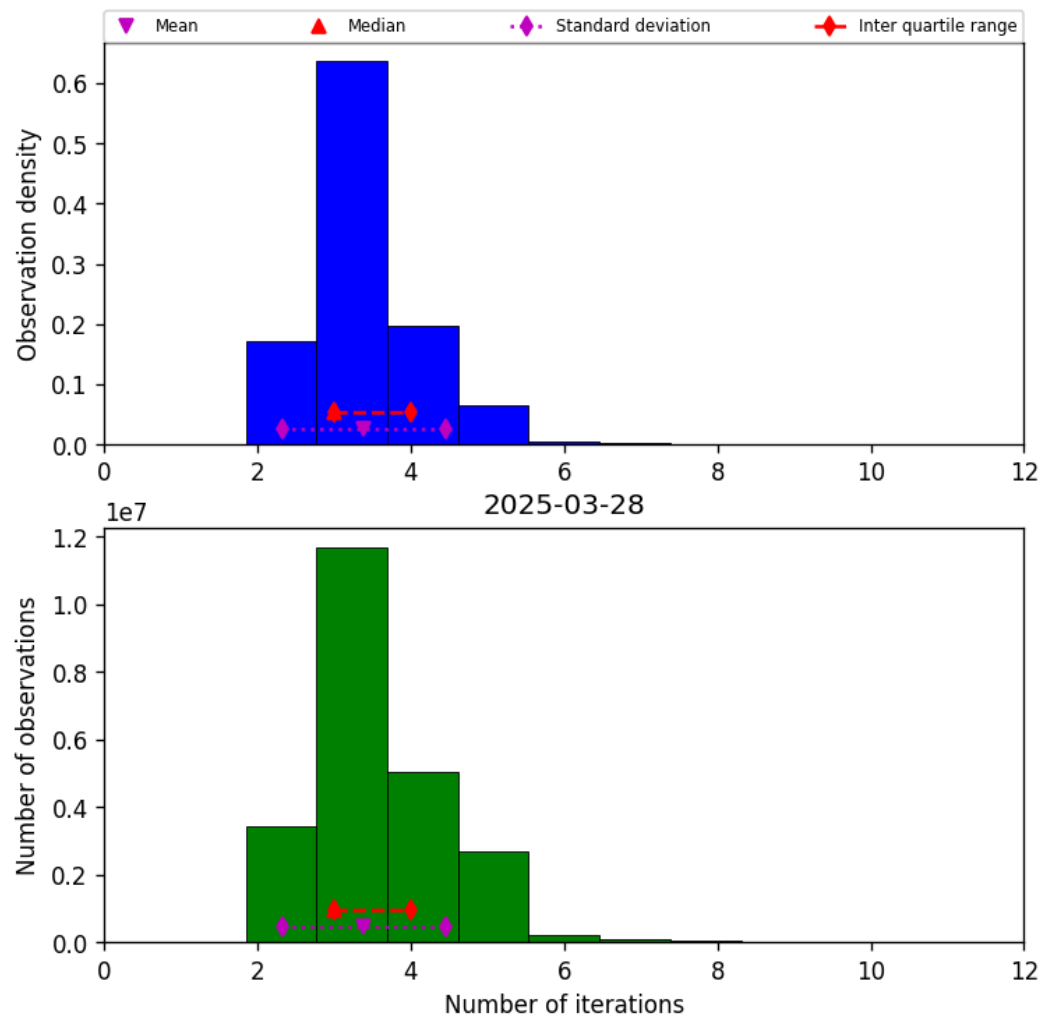
Figure 37: Histogram of “Number of iterations” for 2025-03-28 to 2025-03-29
