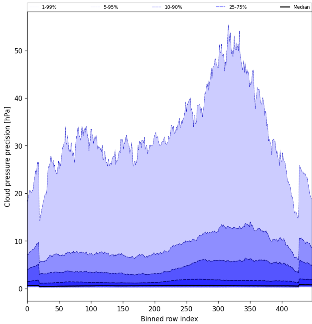
Figure 46: Along track statistics of “Cloud pressure precision” for 2025-03-28 to 2025-03-29
