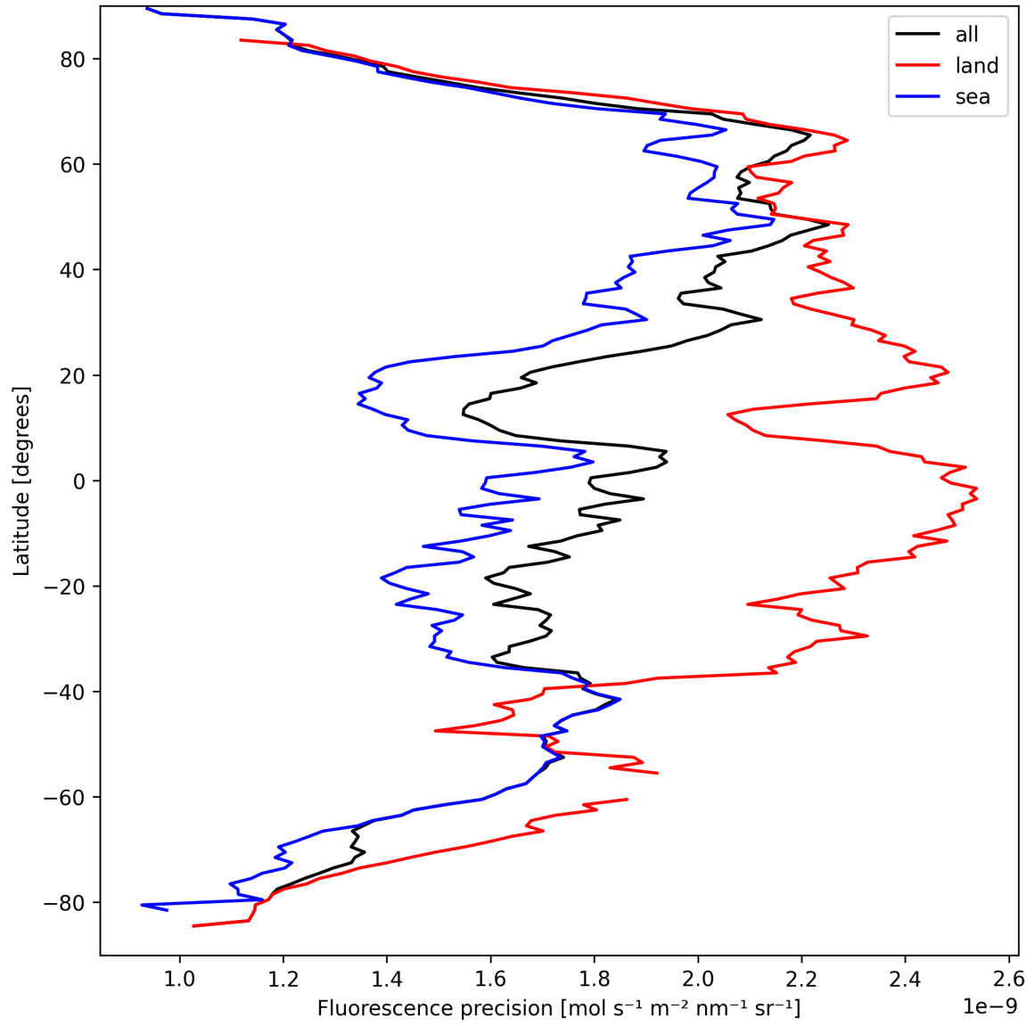
Figure 22: Zonal average of “Fluorescence precision” for 2025-03-28 to 2025-03-29.
