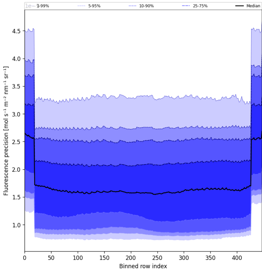
Figure 56: Along track statistics of “Fluorescence precision” for 2025-03-28 to 2025-03-29
