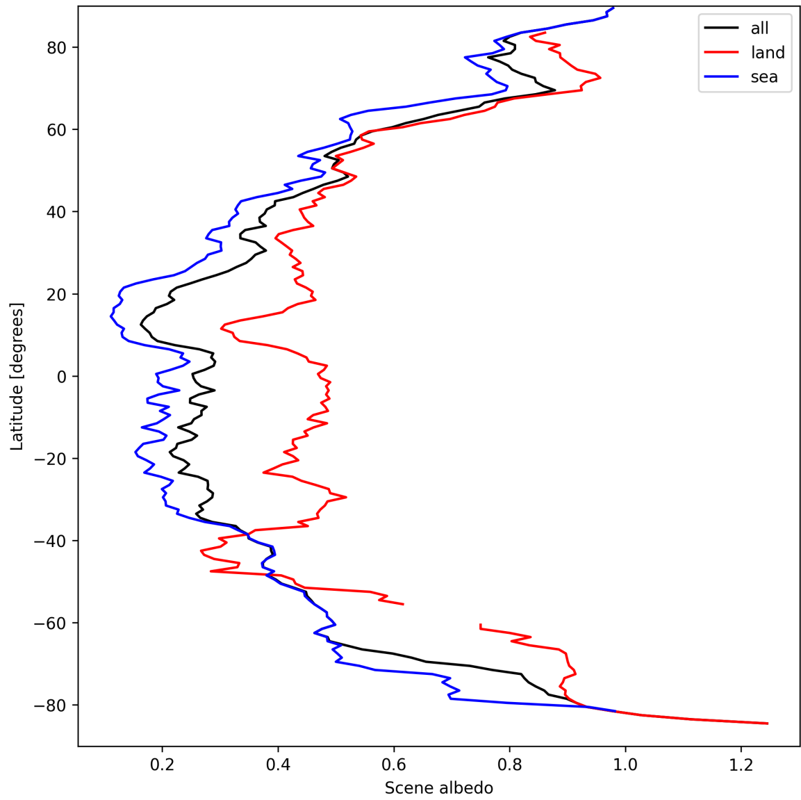
Figure 15: Zonal average of “Scene albedo” for 2025-03-28 to 2025-03-29.
