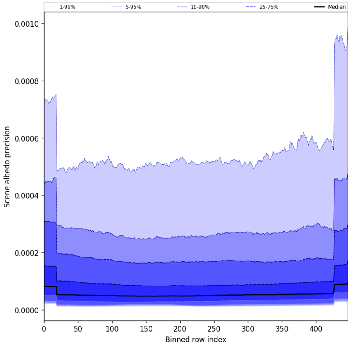
Figure 50: Along track statistics of “Scene albedo precision” for 2025-03-28 to 2025-03-29
