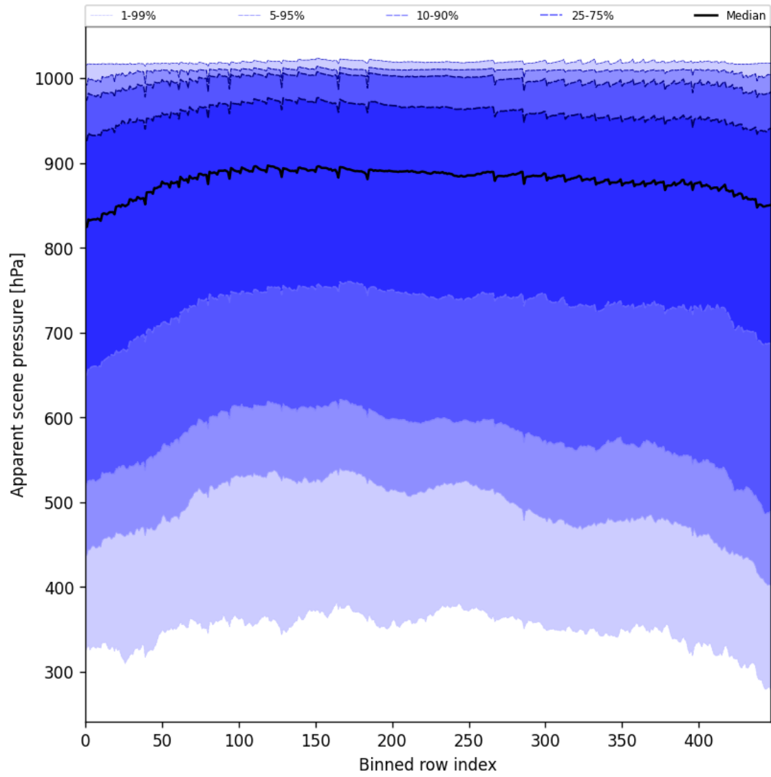
Figure 51: Along track statistics of “Apparent scene pressure” for 2025-03-28 to 2025-03-29
