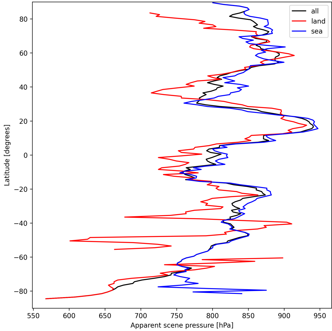
Figure 17: Zonal average of “Apparent scene pressure” for 2025-03-28 to 2025-03-29.
