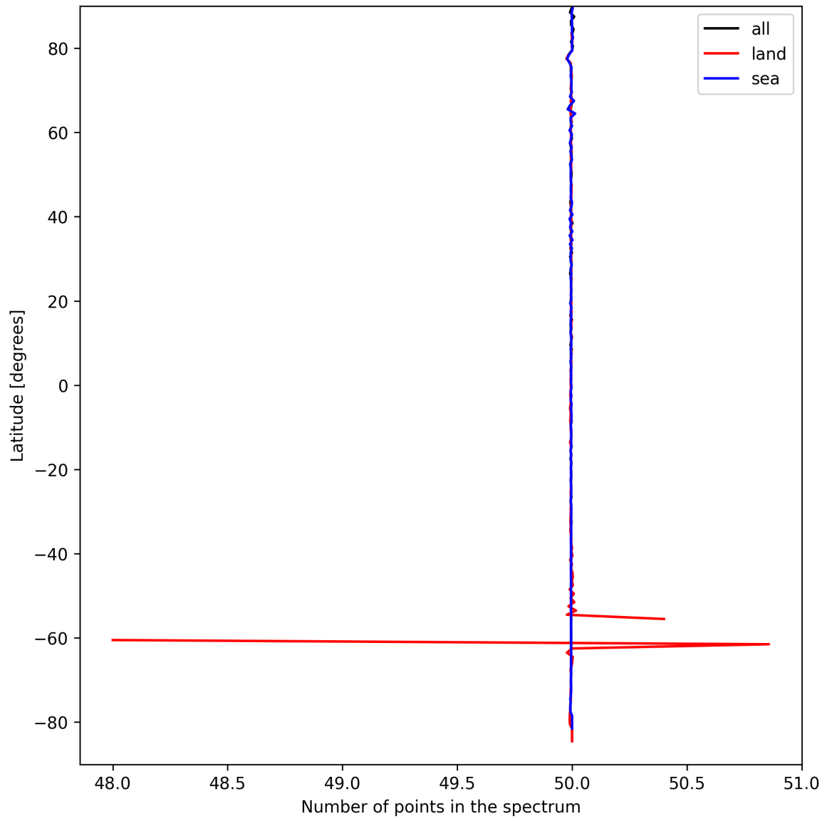
Figure 25: Zonal average of “Number of points in the spectrum” for 2025-03-28 to 2025-03-29.
