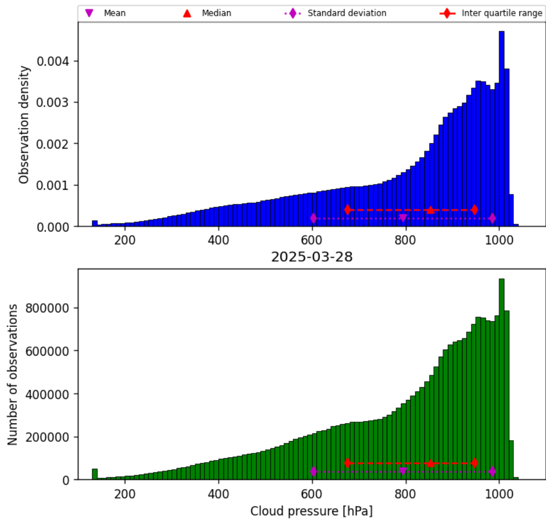
Figure 28: Histogram of “Cloud pressure” for 2025-03-28 to 2025-03-29
