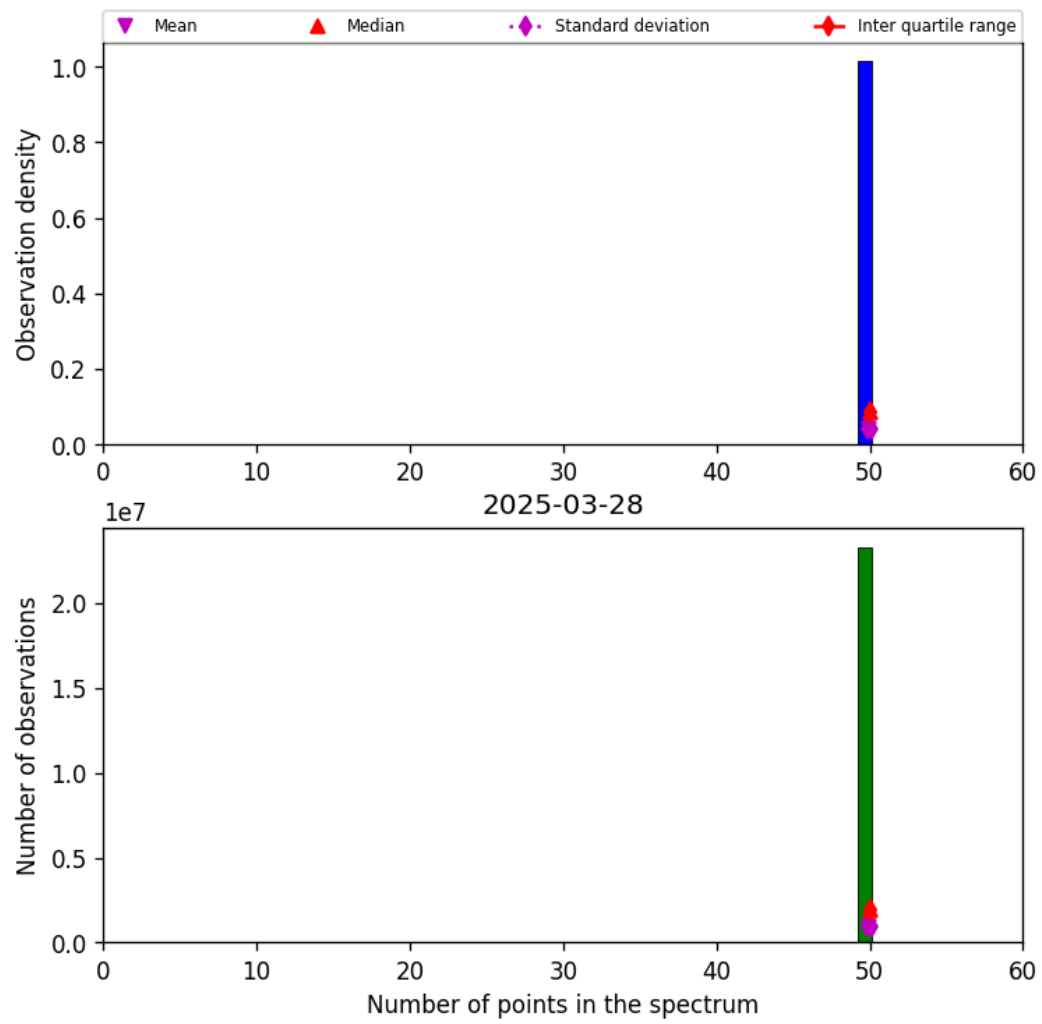
Figure 42: Histogram of “Number of points in the spectrum” for 2025-03-28 to 2025-03-29
