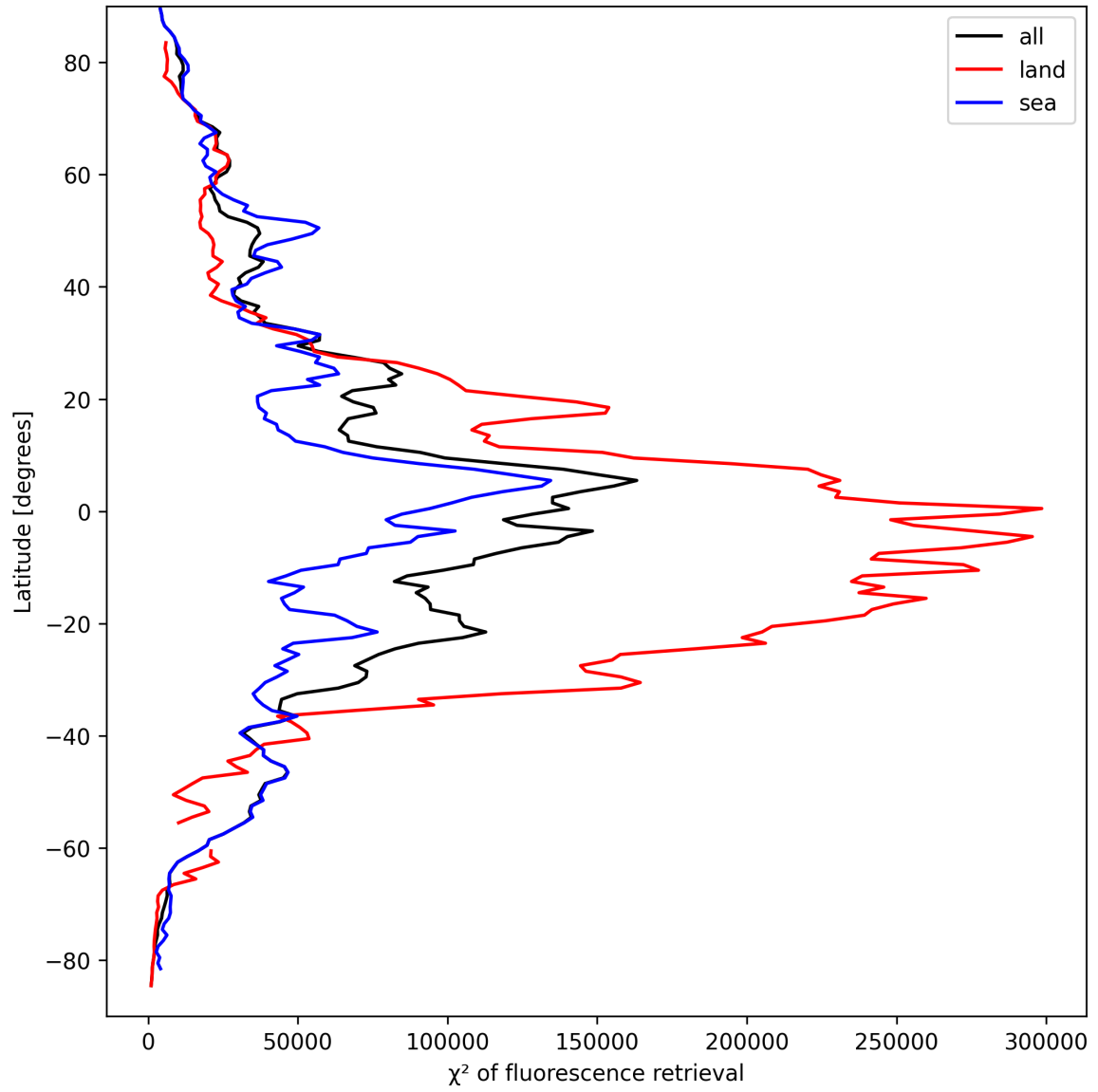
Figure 23: Zonal average of “ \chi^2 of fluorescence retrieval” for 2025-03-28 to 2025-03-29.
