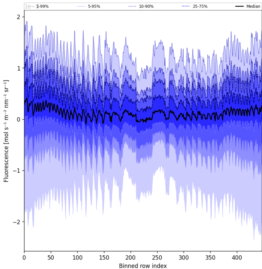
Figure 55: Along track statistics of “Fluorescence” for 2025-03-28 to 2025-03-29
