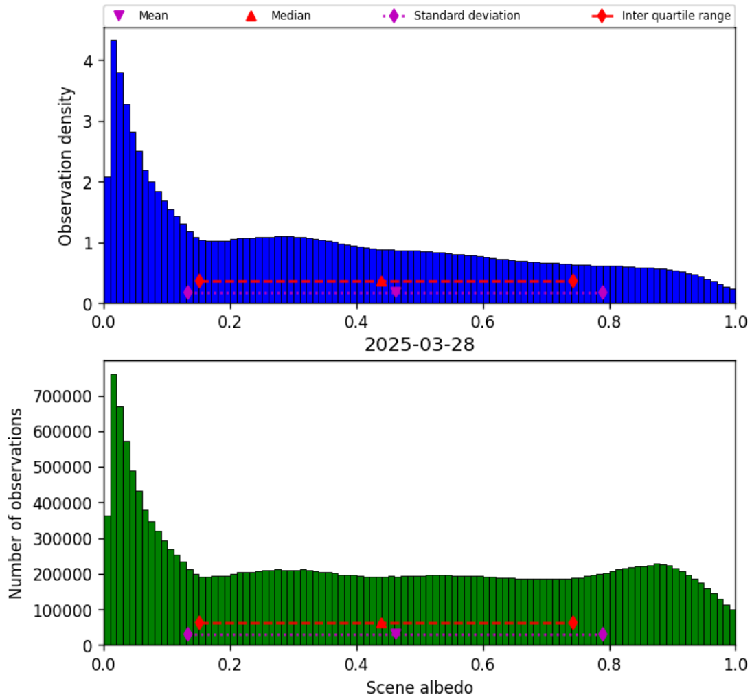
Figure 32: Histogram of “Scene albedo” for 2025-03-28 to 2025-03-29
