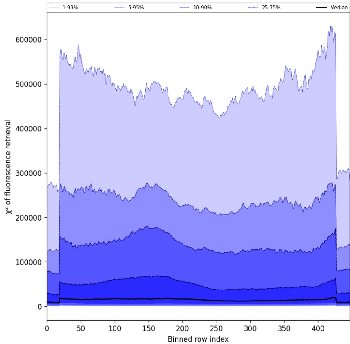
Figure 57: Along track statistics of “ \chi^2 of fluorescence retrieval” for 2025-03-28 to 2025-03-29
