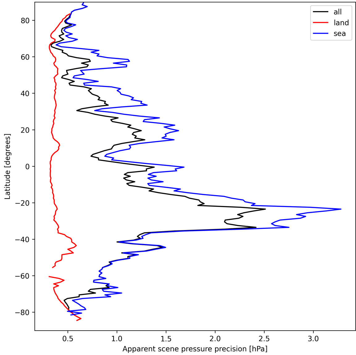
Figure 18: Zonal average of “Apparent scene pressure precision” for 2025-03-28 to 2025-03-29.
