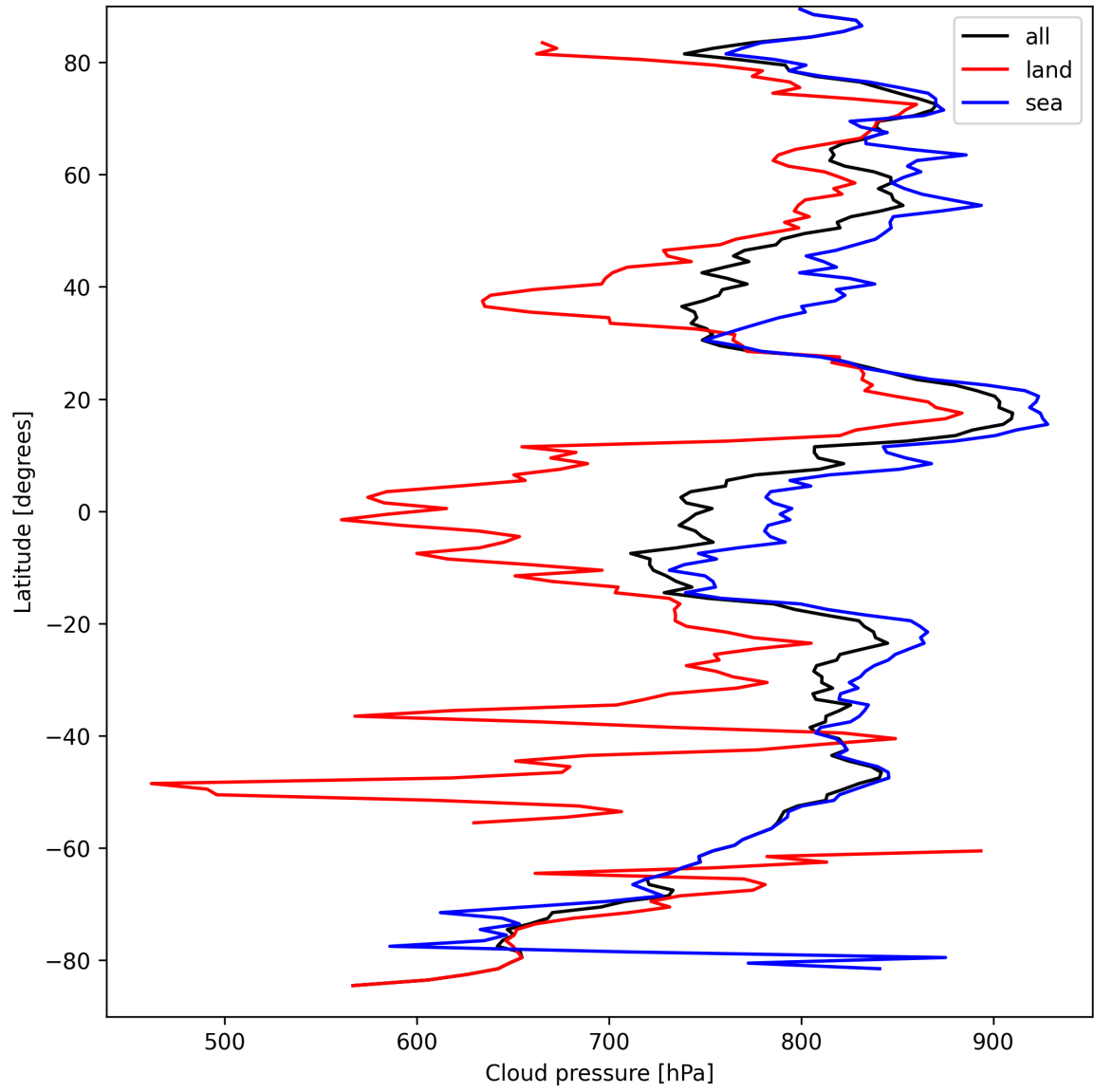
Figure 11: Zonal average of “Cloud pressure” for 2025-03-28 to 2025-03-29.
