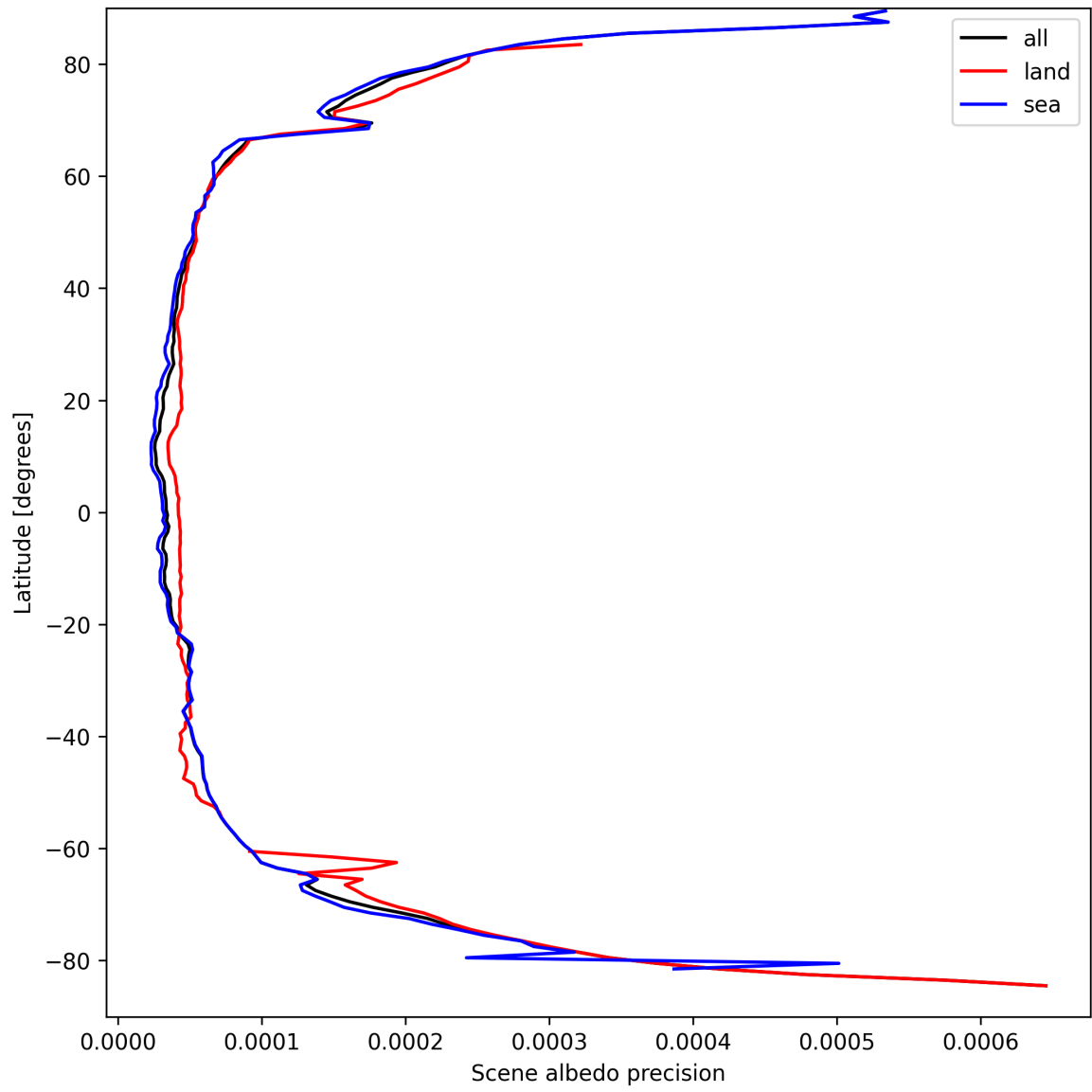
Figure 16: Zonal average of “Scene albedo precision” for 2025-03-28 to 2025-03-29.
