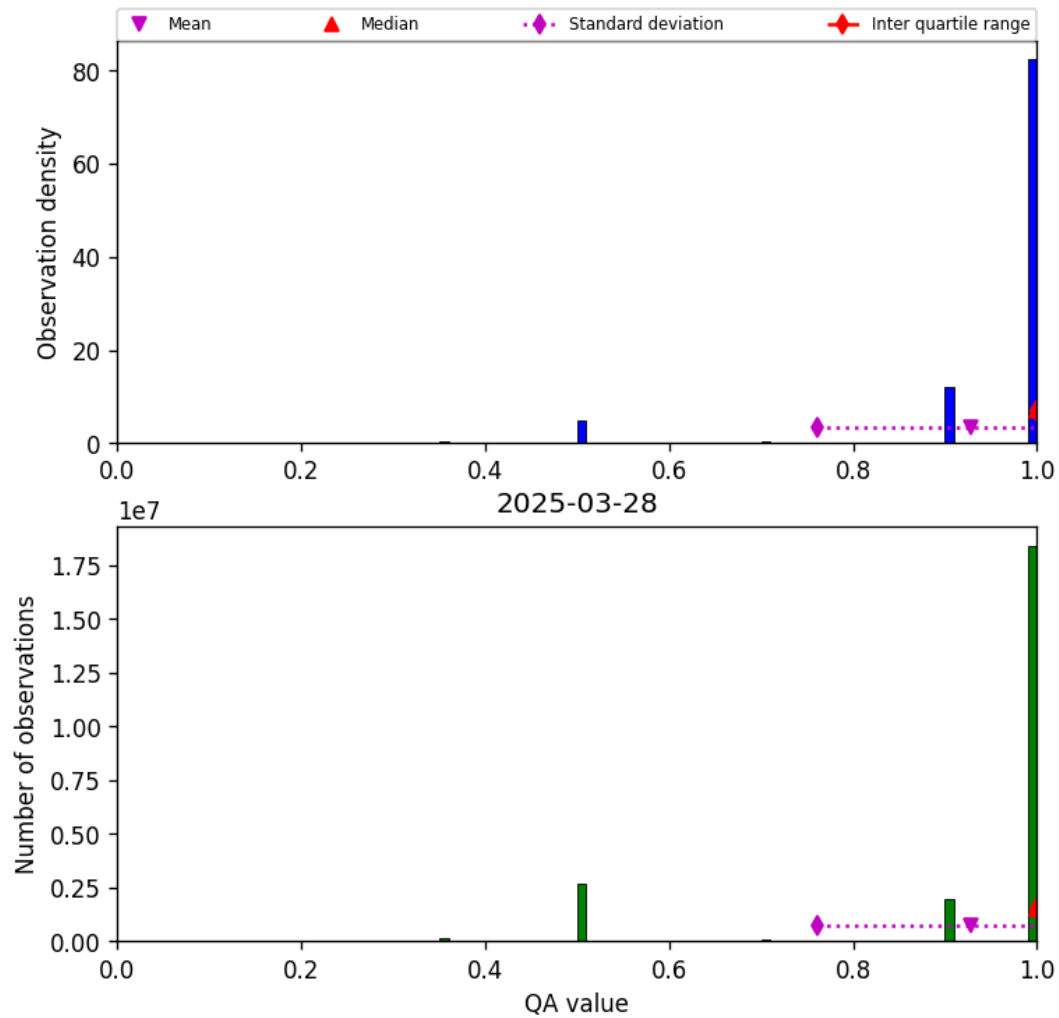
Figure 27: Histogram of “QA value” for 2025-03-28 to 2025-03-29
