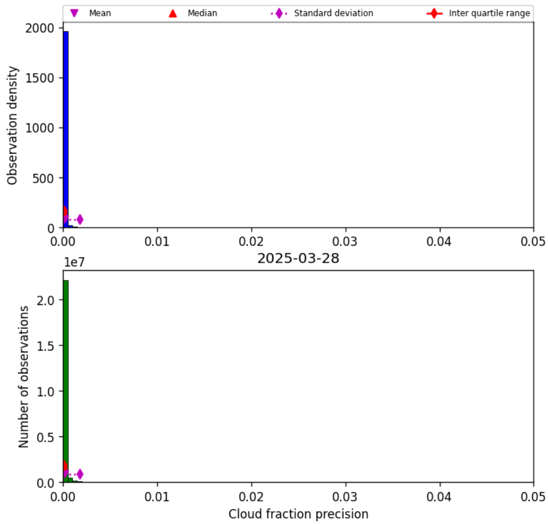
Figure 31: Histogram of “Cloud fraction precision” for 2025-03-28 to 2025-03-29
