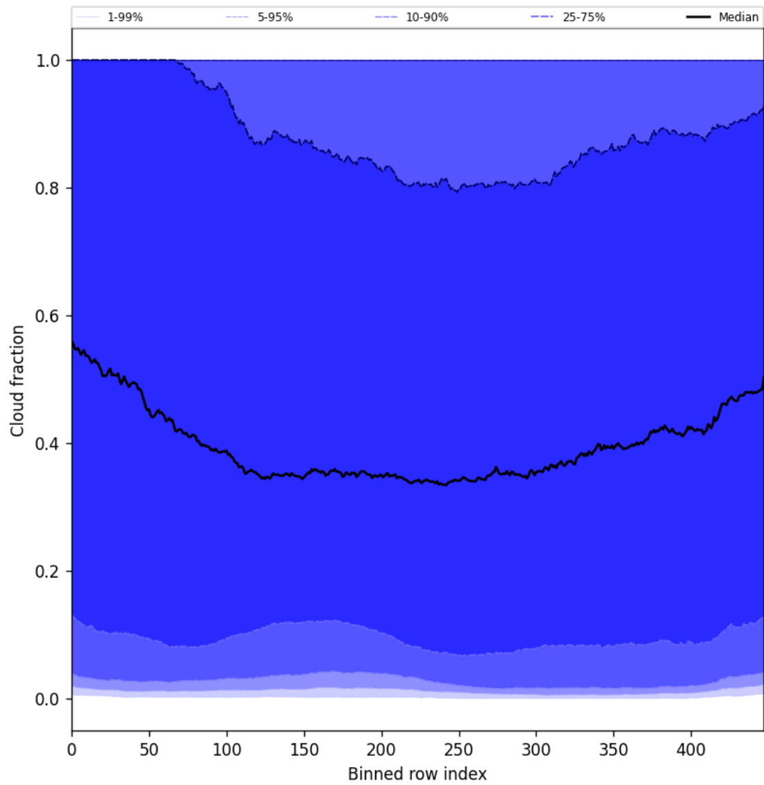
Figure 47: Along track statistics of “Cloud fraction” for 2025-03-28 to 2025-03-29
