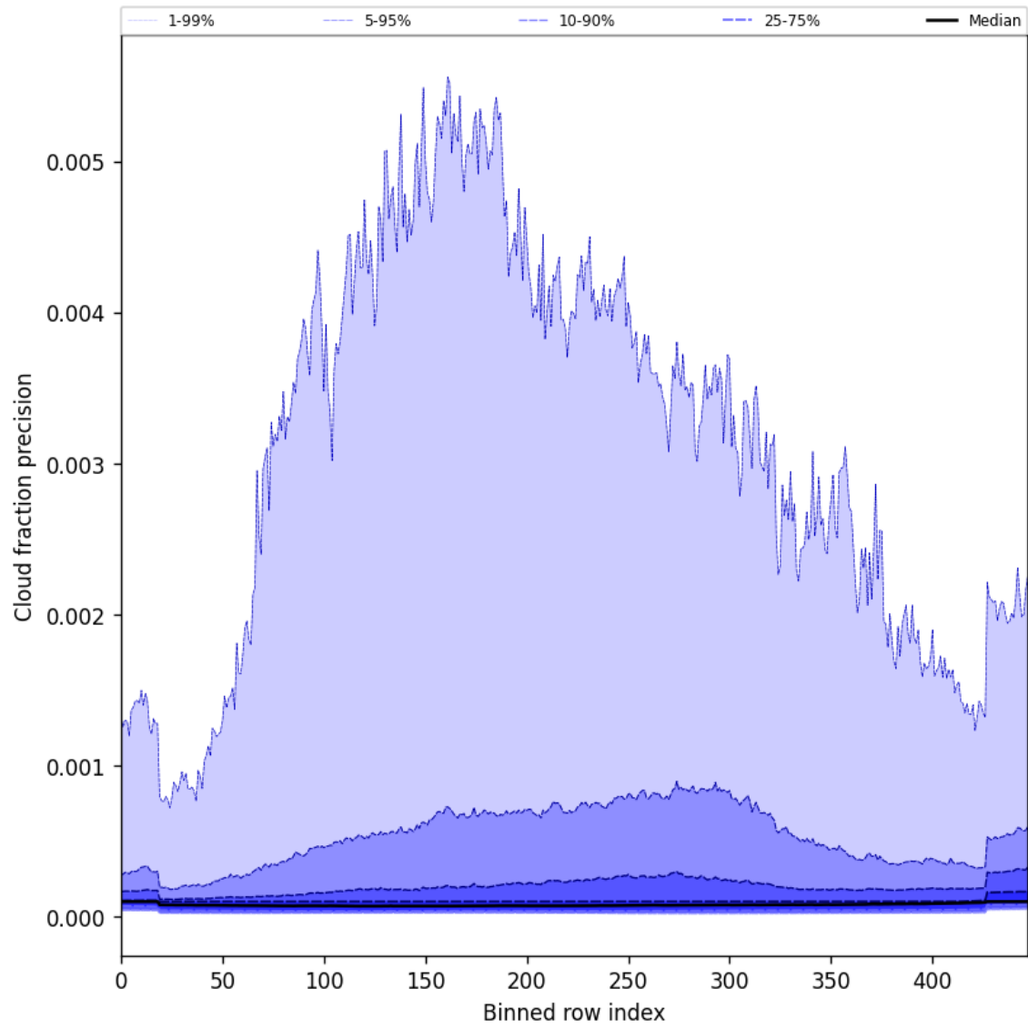
Figure 48: Along track statistics of “Cloud fraction precision” for 2025-03-28 to 2025-03-29
