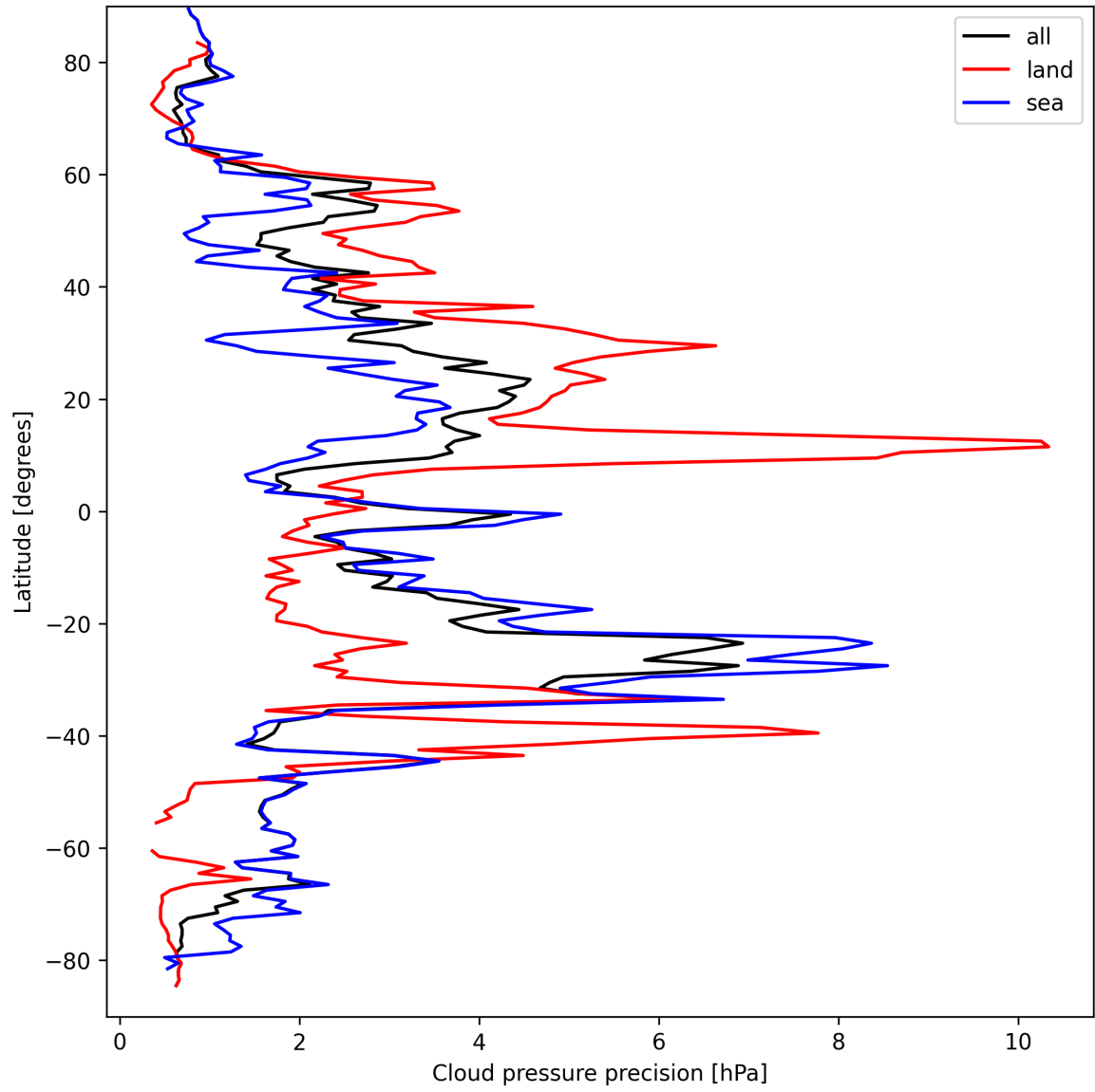
Figure 12: Zonal average of “Cloud pressure precision” for 2025-03-28 to 2025-03-29.
