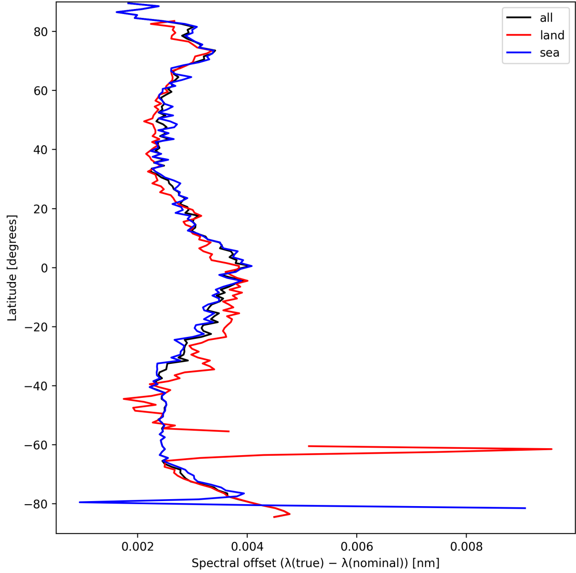
Figure 26: Zonal average of “Spectral offset ( \lambda_{\text{true}} - \lambda_{\text{nominal}} )” for 2025-03-28 to 2025-03-29.
