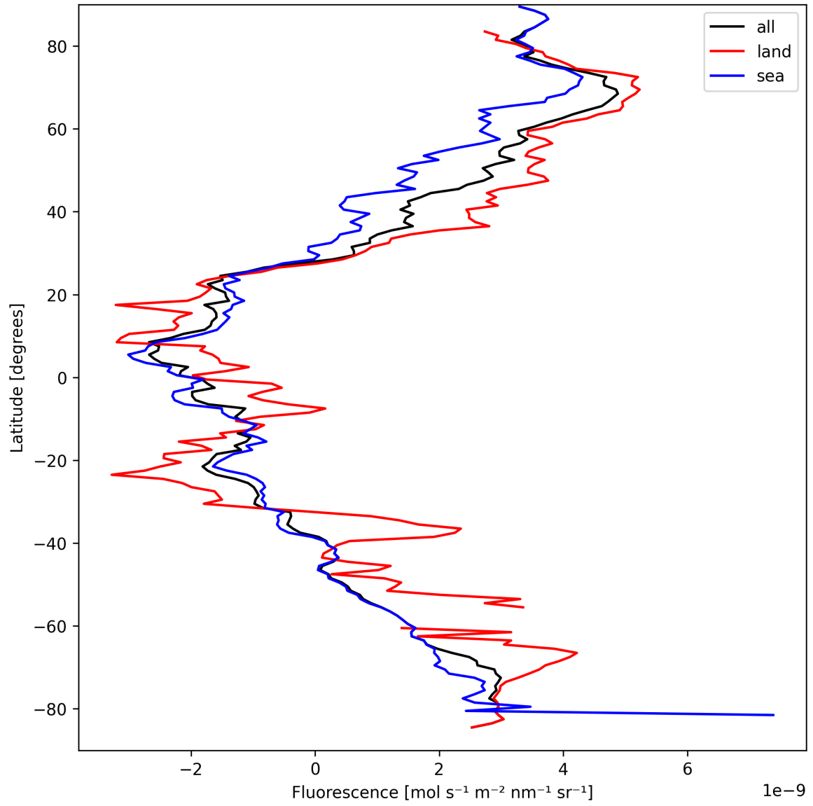
Figure 21: Zonal average of “Fluorescence” for 2025-03-28 to 2025-03-29.
