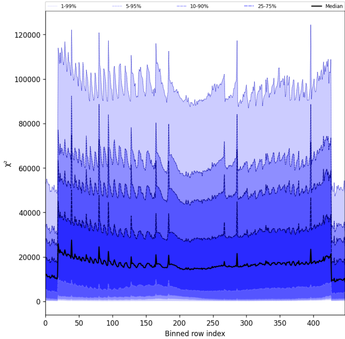
Figure 53: Along track statistics of “ \chi^2 ” for 2025-03-28 to 2025-03-29
