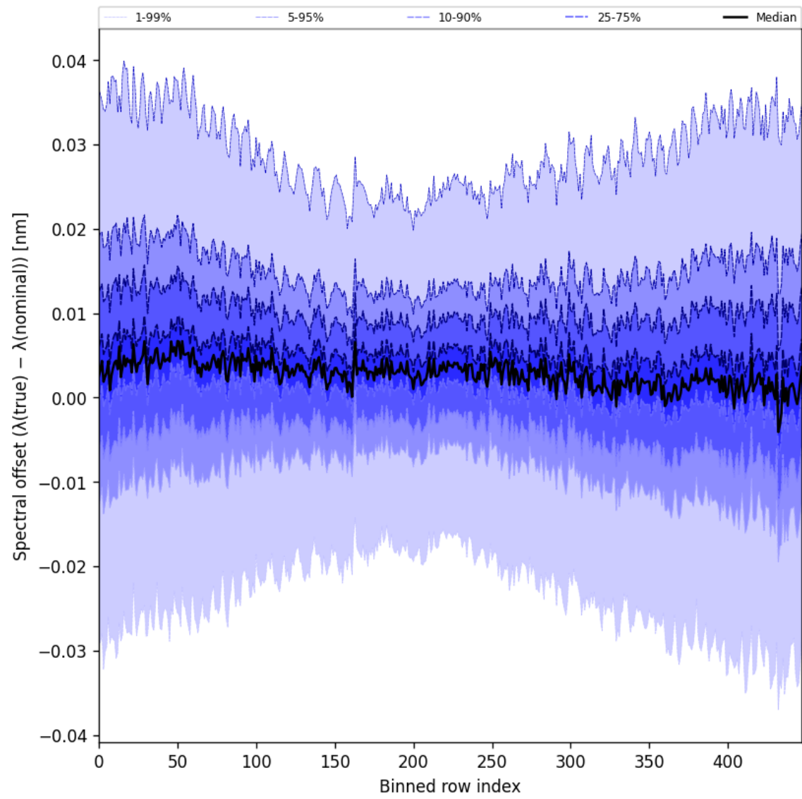
Figure 60: Along track statistics of “Spectral offset ( \lambda_{\text{true}} - \lambda_{\text{nominal}} )” for 2025-03-28 to 2025-03-29
