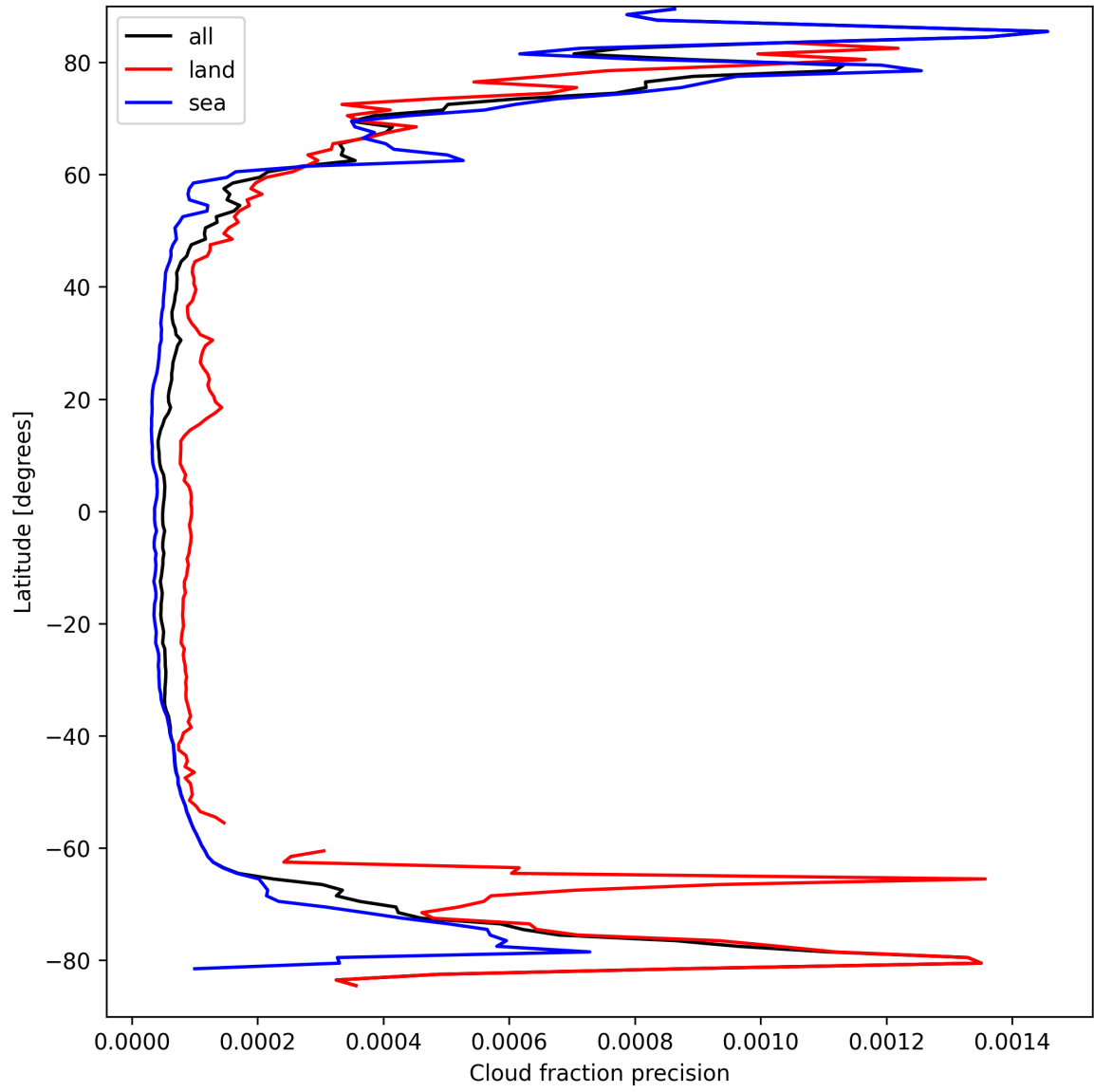
Figure 14: Zonal average of “Cloud fraction precision” for 2025-03-28 to 2025-03-29.
