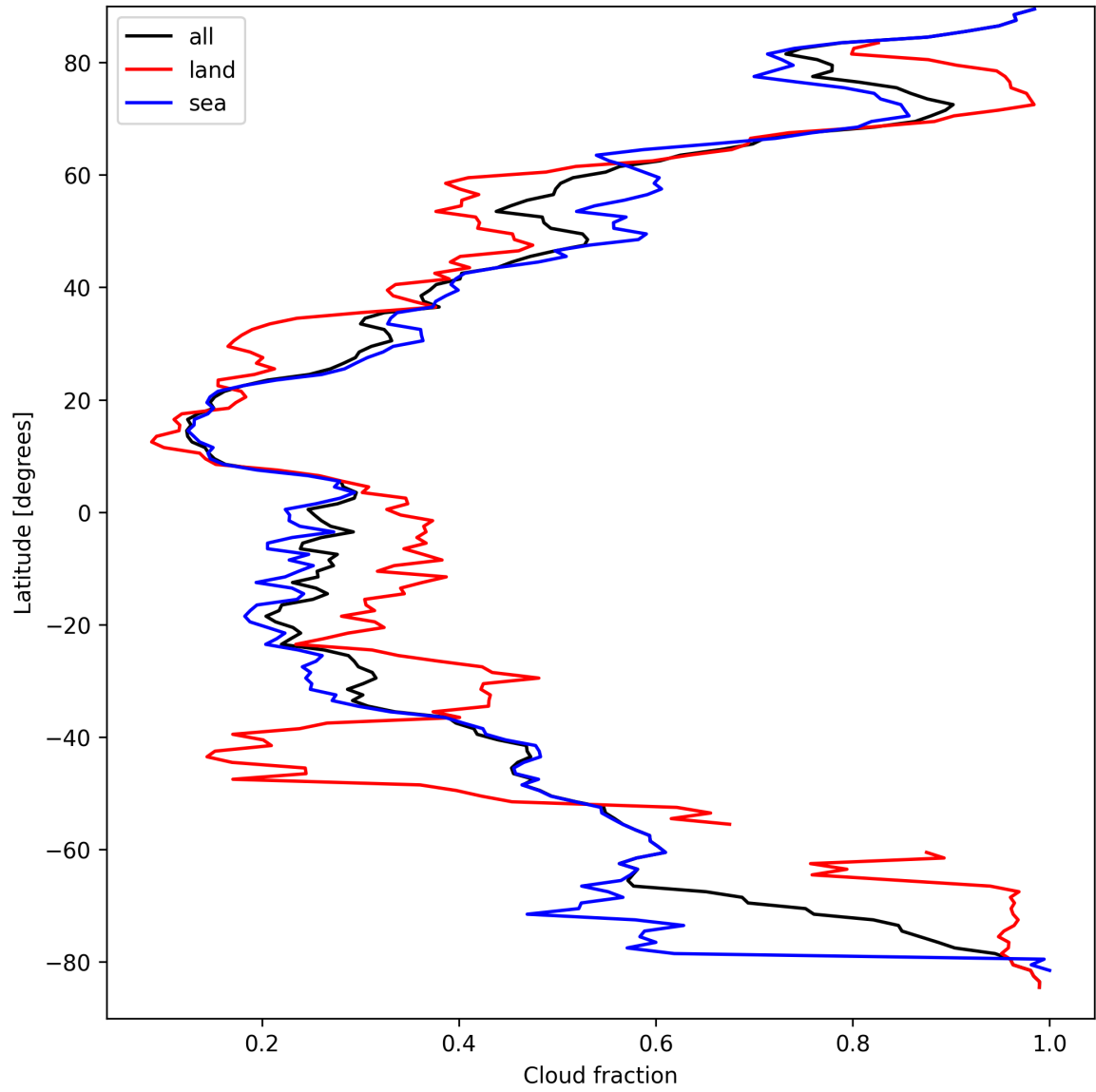
Figure 13: Zonal average of “Cloud fraction” for 2025-03-28 to 2025-03-29.
